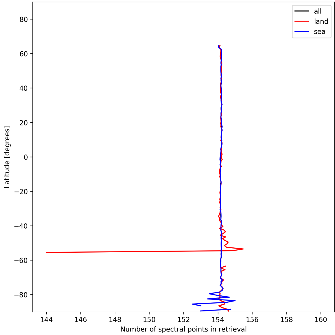
Figure 13: Zonal average of “Number of spectral points in retrieval” for 2024-11-23 to 2024-11-25.
