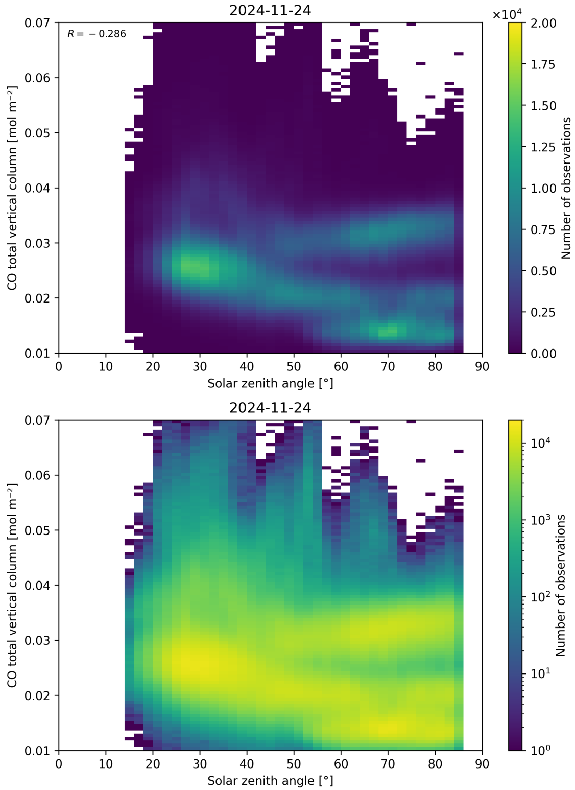
Figure 61: Scatter density plot of “Solar zenith angle” against “CO total vertical column” for 2024-11-23 to 2024-11-25.
