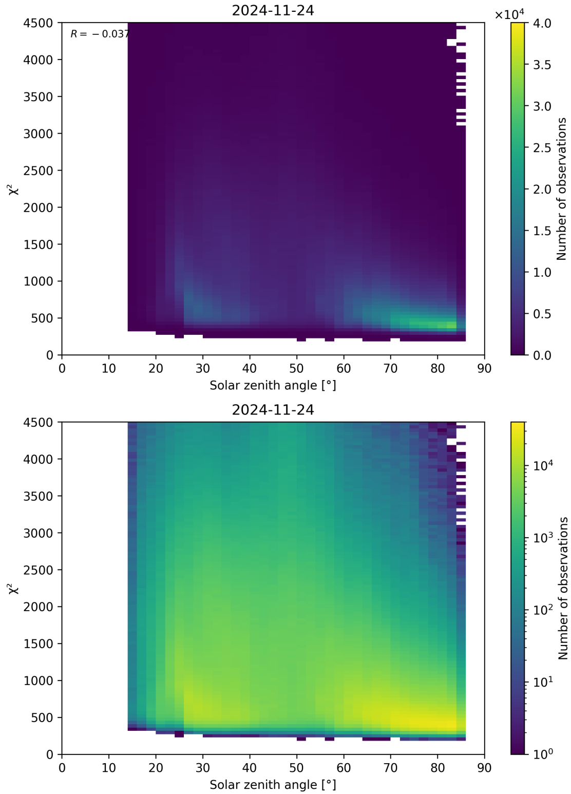
Figure 64: Scatter density plot of “Solar zenith angle” against “ \chi^2 ” for 2024-11-23 to 2024-11-25.
