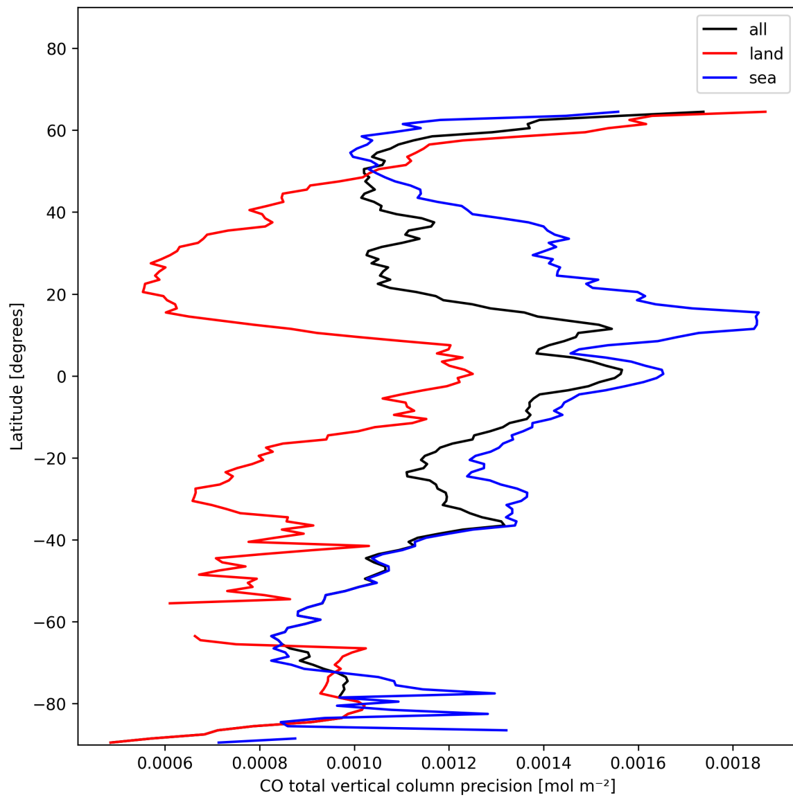
Figure 12: Zonal average of “CO total vertical column precision” for 2024-11-23 to 2024-11-25.
