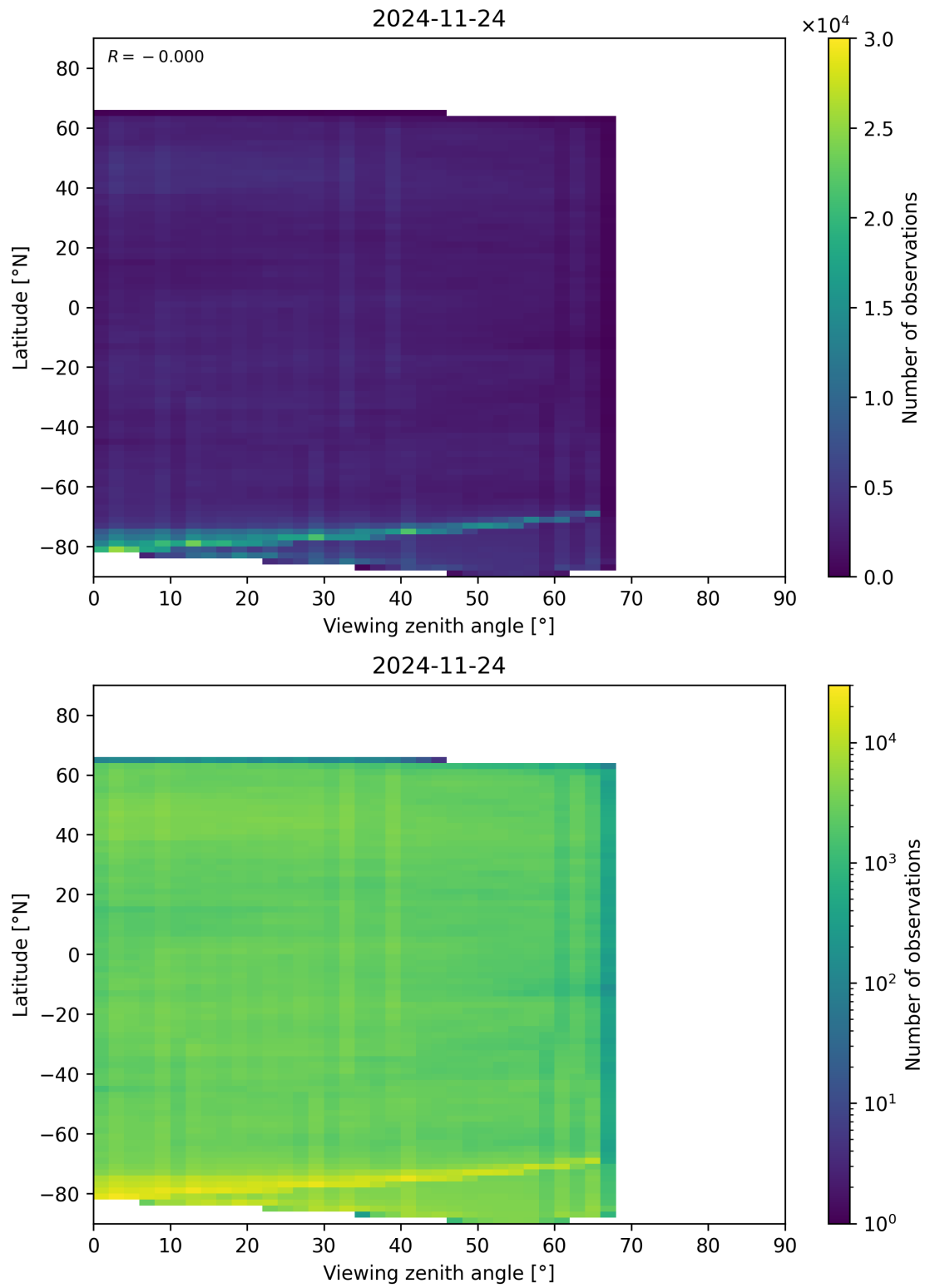
Figure 74: Scatter density plot of “Viewing zenith angle” against “Latitude” for 2024-11-23 to 2024-11-25.
