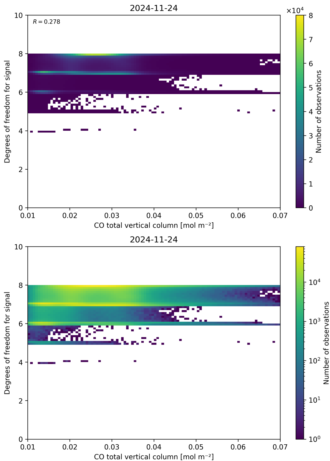
Figure 41: Scatter density plot of “CO total vertical column” against “Degrees of freedom for signal” for 2024-11-23 to 2024-11-25.
