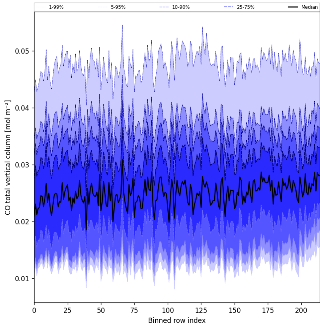
Figure 26: Along track statistics of “CO total vertical column” for 2024-11-23 to 2024-11-25
