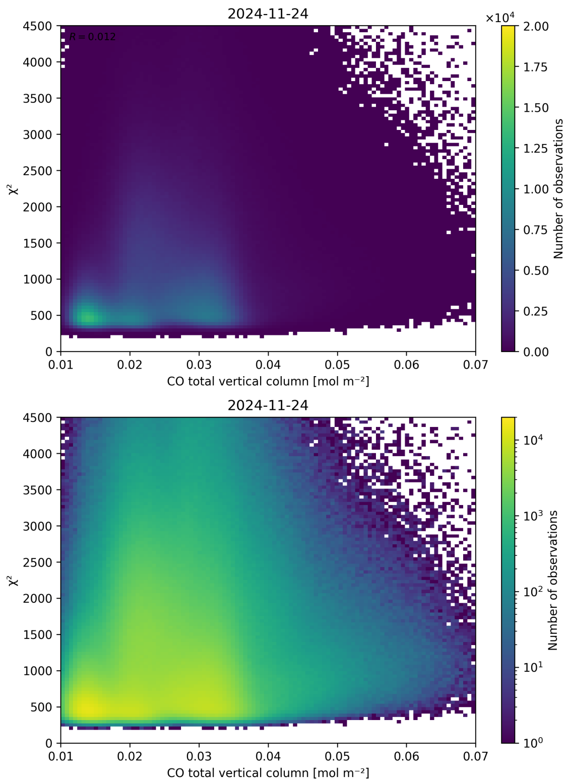
Figure 35: Scatter density plot of “CO total vertical column” against “ \chi^2 ” for 2024-11-23 to 2024-11-25.
