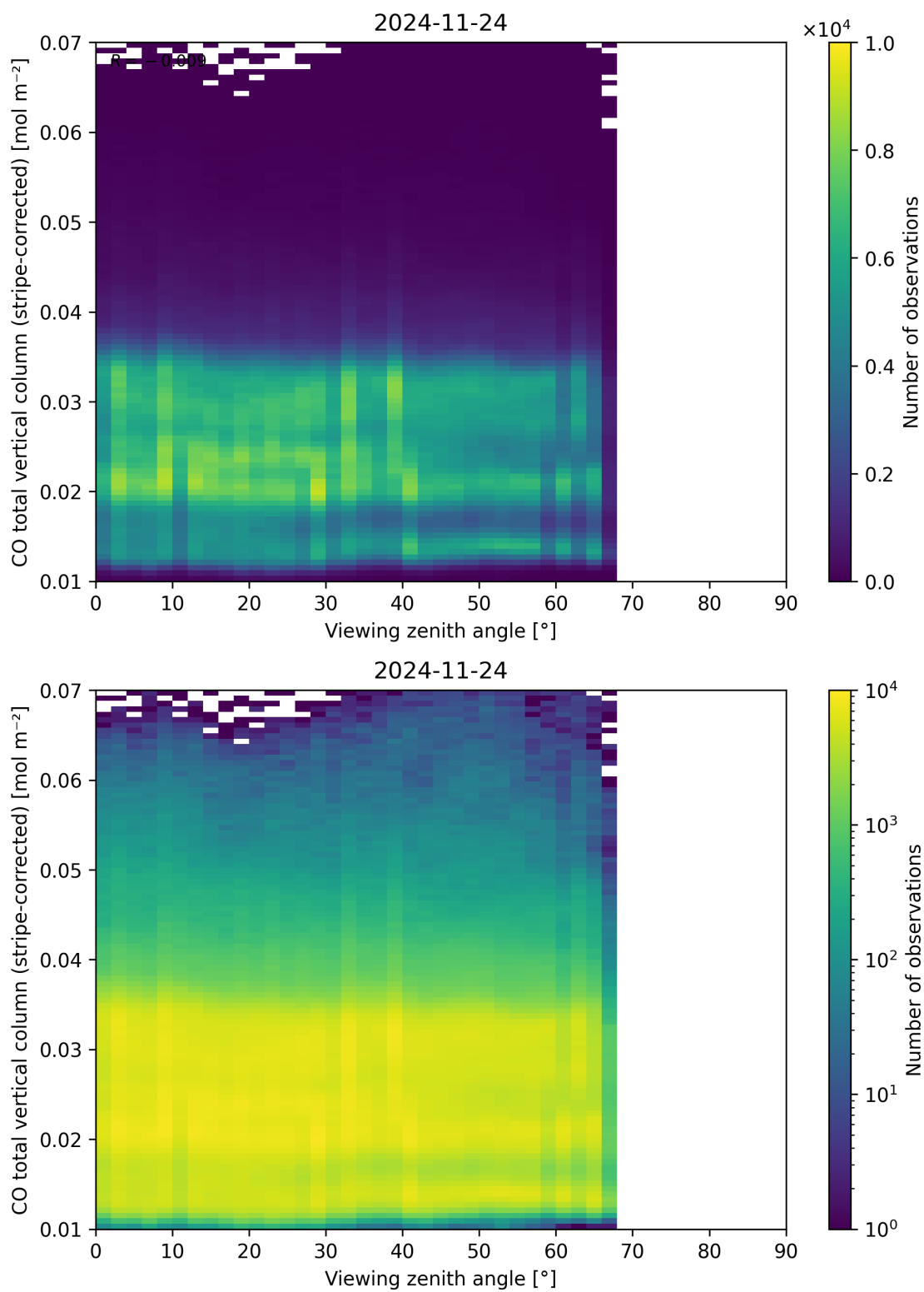
Figure 70: Scatter density plot of “Viewing zenith angle” against “CO total vertical column (stripe-corrected)” for 2024-11-23 to 2024-11-25.
