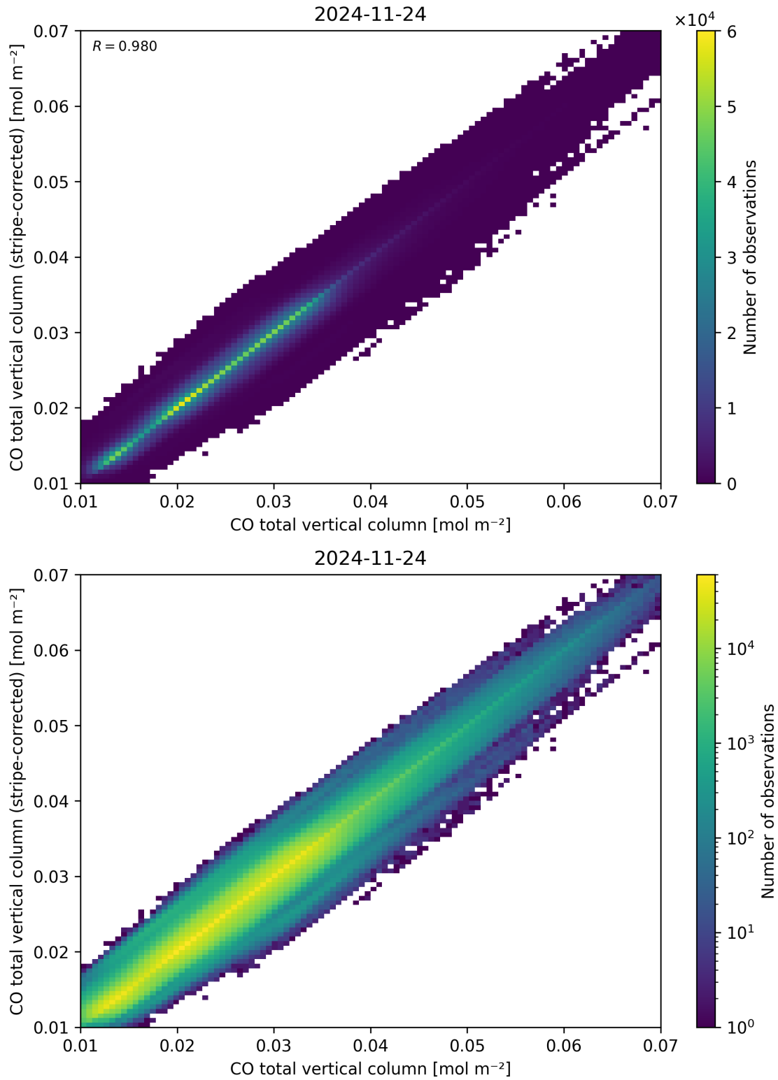
Figure 33: Scatter density plot of “CO total vertical column” against “CO total vertical column (stripe-corrected)” for 2024-11-23 to 2024-11-25.
