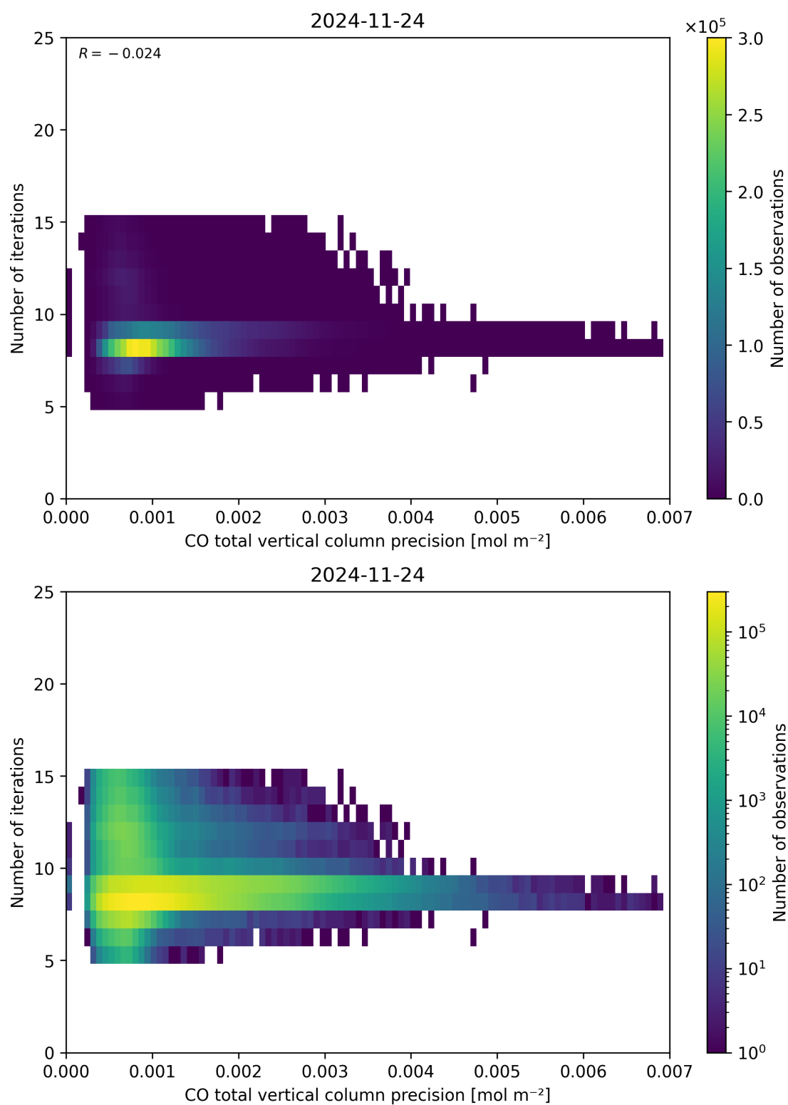
Figure 46: Scatter density plot of “CO total vertical column precision” against “Number of iterations” for 2024-11-23 to 2024-11-25.
