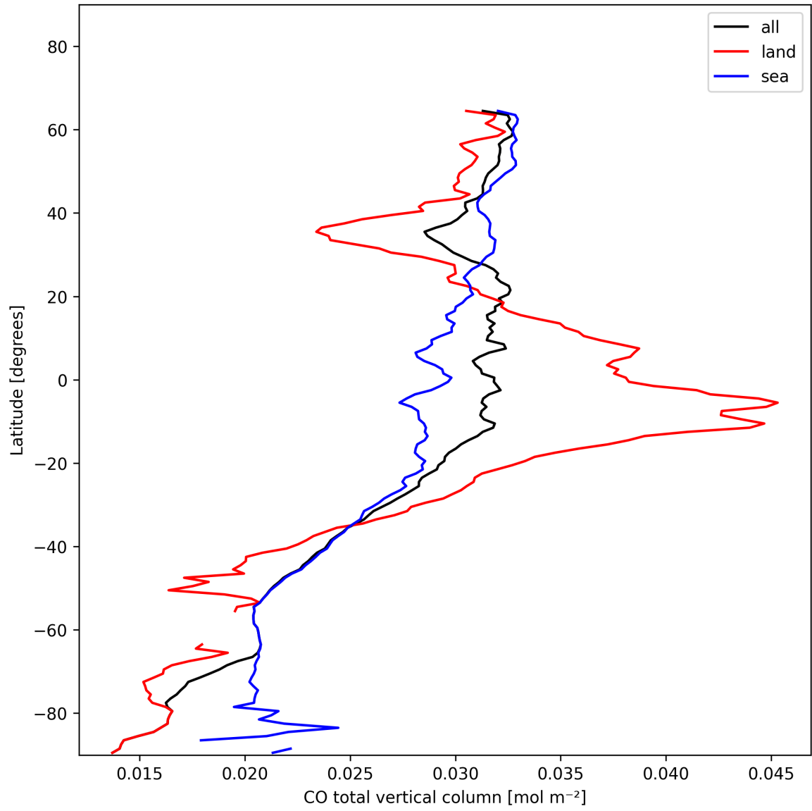
Figure 10: Zonal average of “CO total vertical column” for 2024-11-23 to 2024-11-25.
