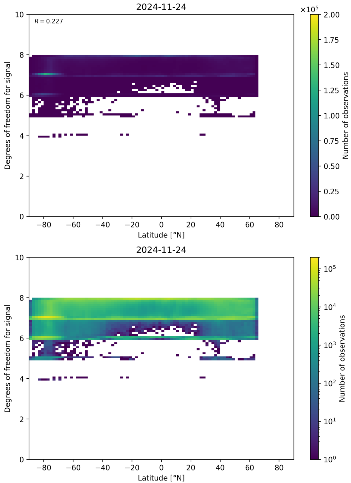
Figure 55: Scatter density plot of “Latitude” against “Degrees of freedom for signal” for 2024-11-23 to 2024-11-25.
