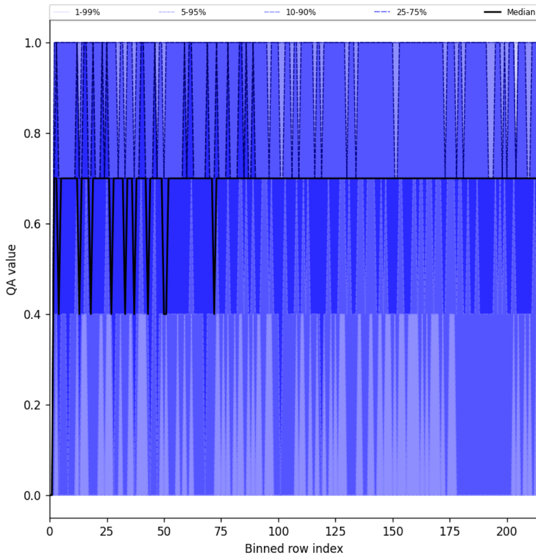
Figure 25: Along track statistics of “QA value” for 2024-11-23 to 2024-11-25
