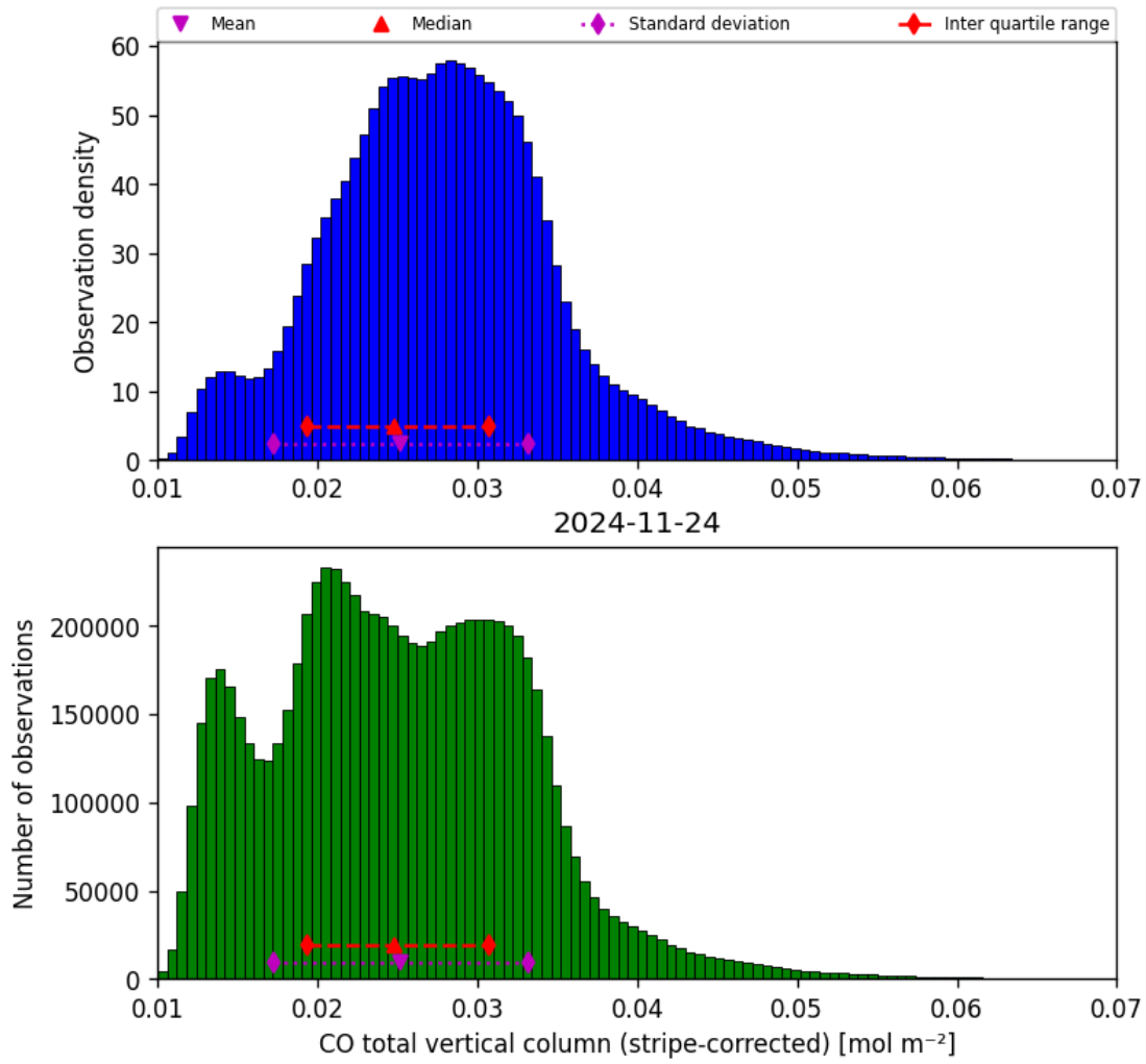
Figure 19: Histogram of “CO total vertical column (stripe-corrected)” for 2024-11-23 to 2024-11-25
