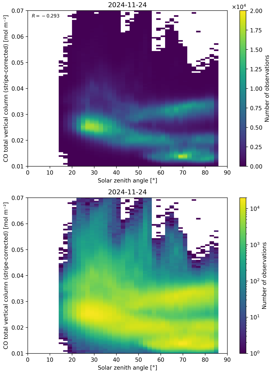
Figure 62: Scatter density plot of “Solar zenith angle” against “CO total vertical column (stripe-corrected)” for 2024-11-23 to 2024-11-25.
