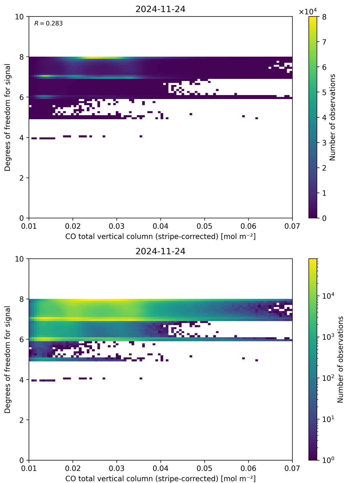
Figure 38: Scatter density plot of “CO total vertical column (stripe-corrected)” against “Degrees of freedom for signal” for 2024-11-23 to 2024-11-25.
