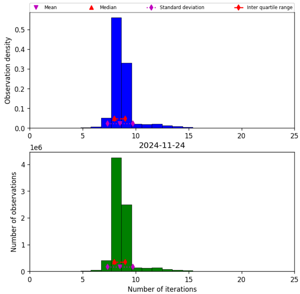
Figure 24: Histogram of “Number of iterations” for 2024-11-23 to 2024-11-25
