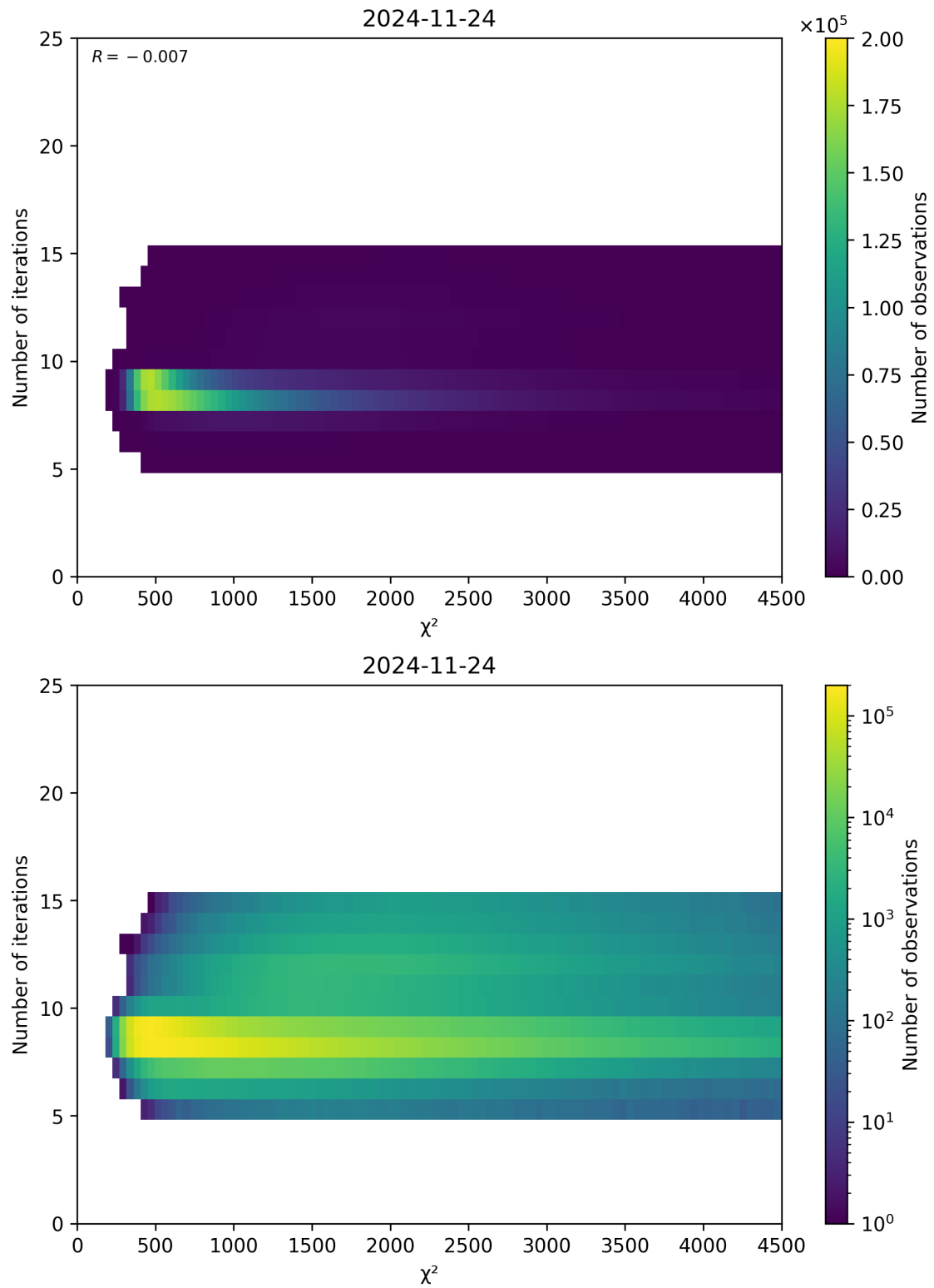
Figure 49: Scatter density plot of “ \chi^2 ” against “Number of iterations” for 2024-11-23 to 2024-11-25.
