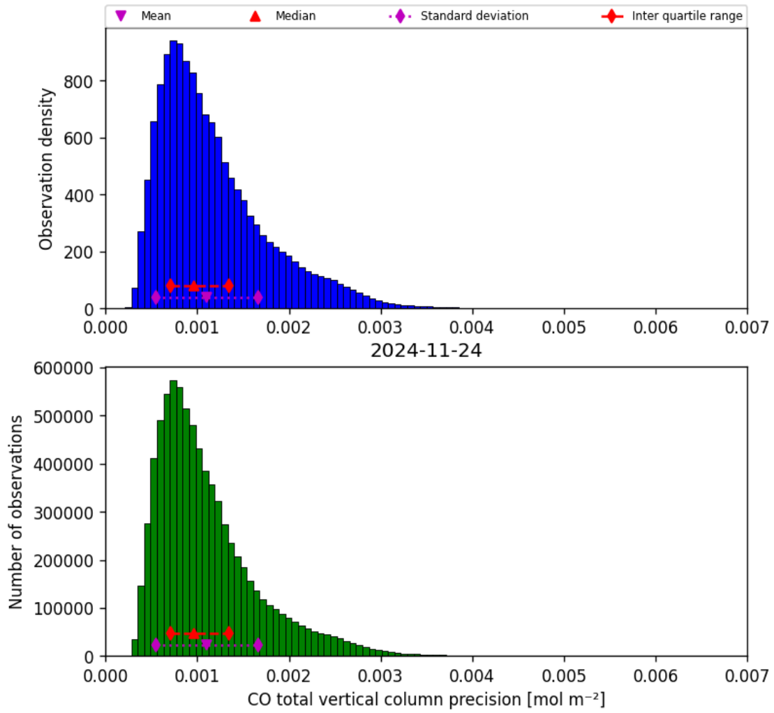
Figure 20: Histogram of “CO total vertical column precision” for 2024-11-23 to 2024-11-25
