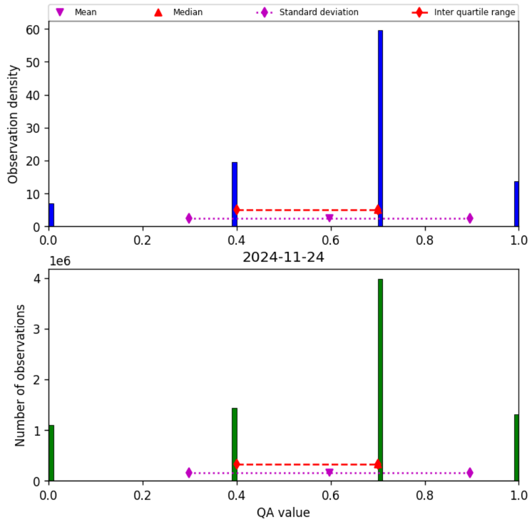
Figure 17: Histogram of “QA value” for 2024-11-23 to 2024-11-25
