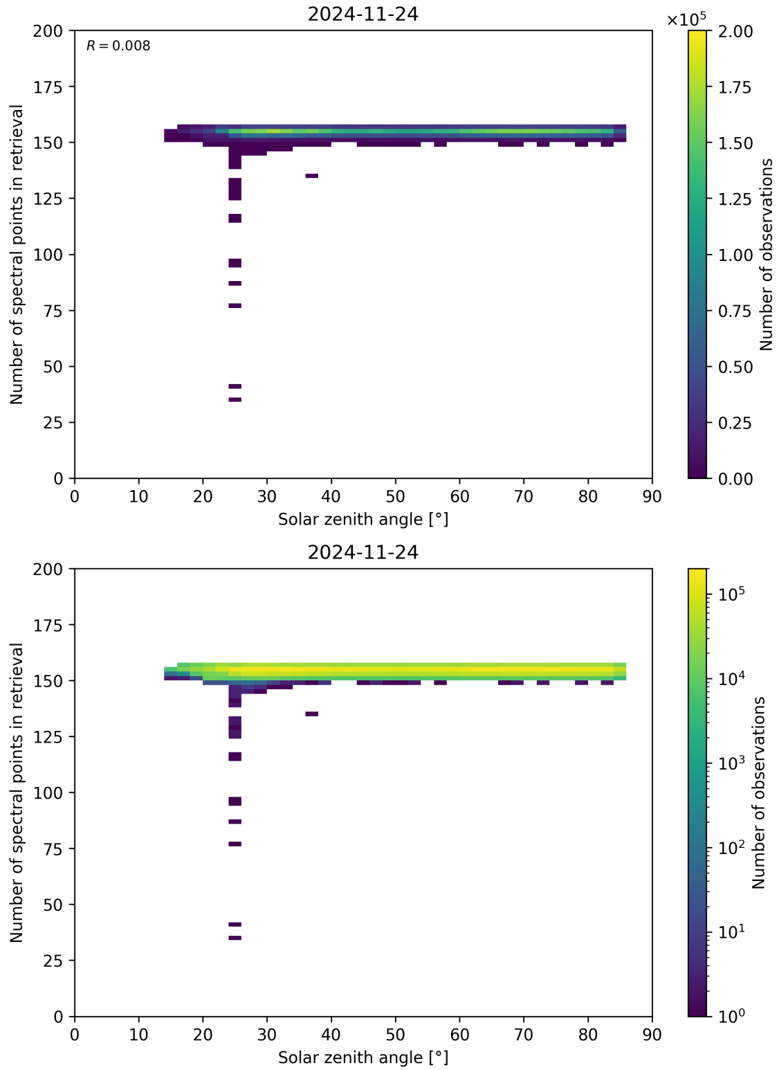
Figure 68: Scatter density plot of “Solar zenith angle” against “Number of spectral points in retrieval” for 2024-11-23 to 2024-11-25.
