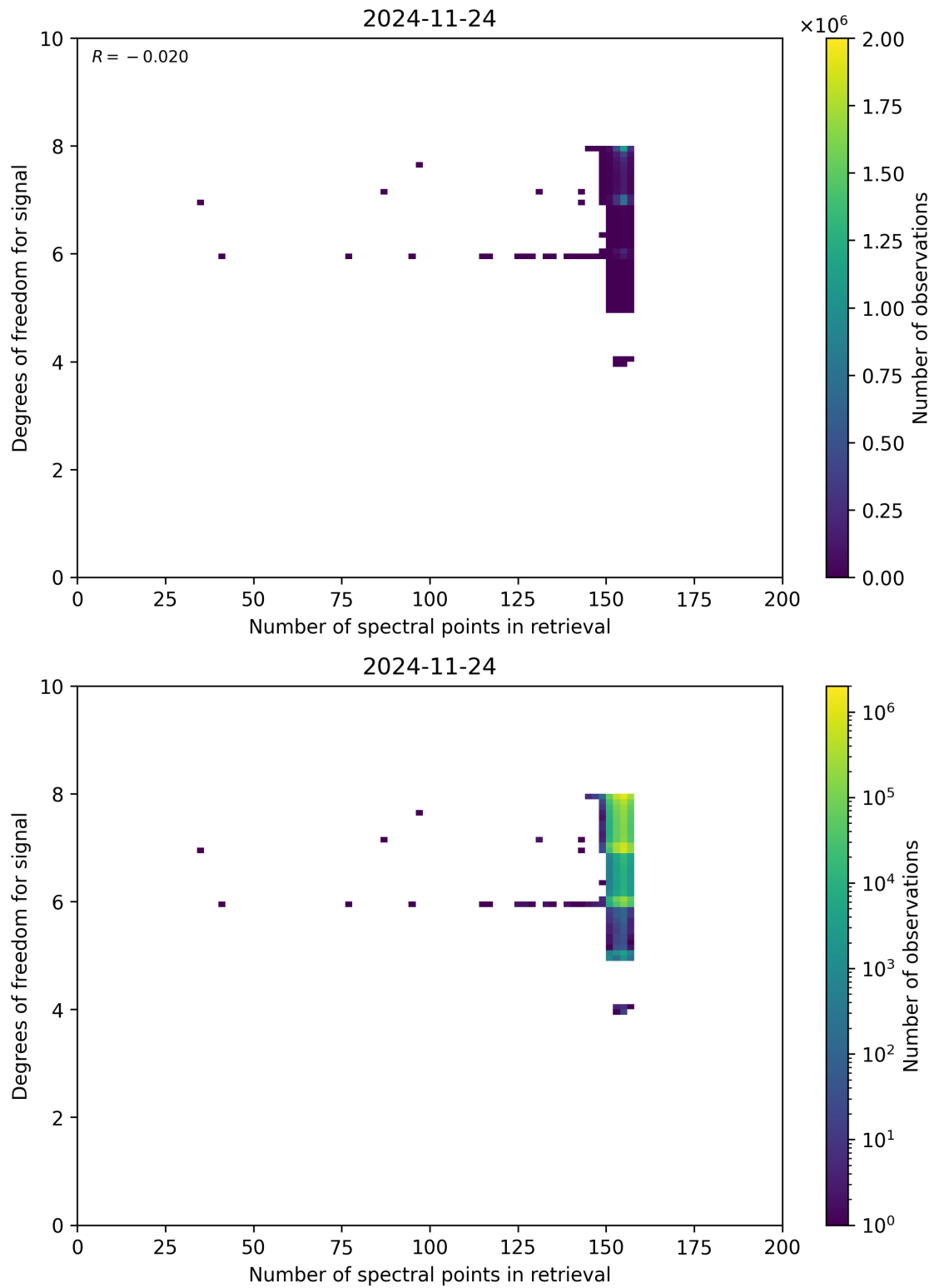
Figure 59: Scatter density plot of “Number of spectral points in retrieval” against “Degrees of freedom for signal” for 2024-11-23 to 2024-11-25.
