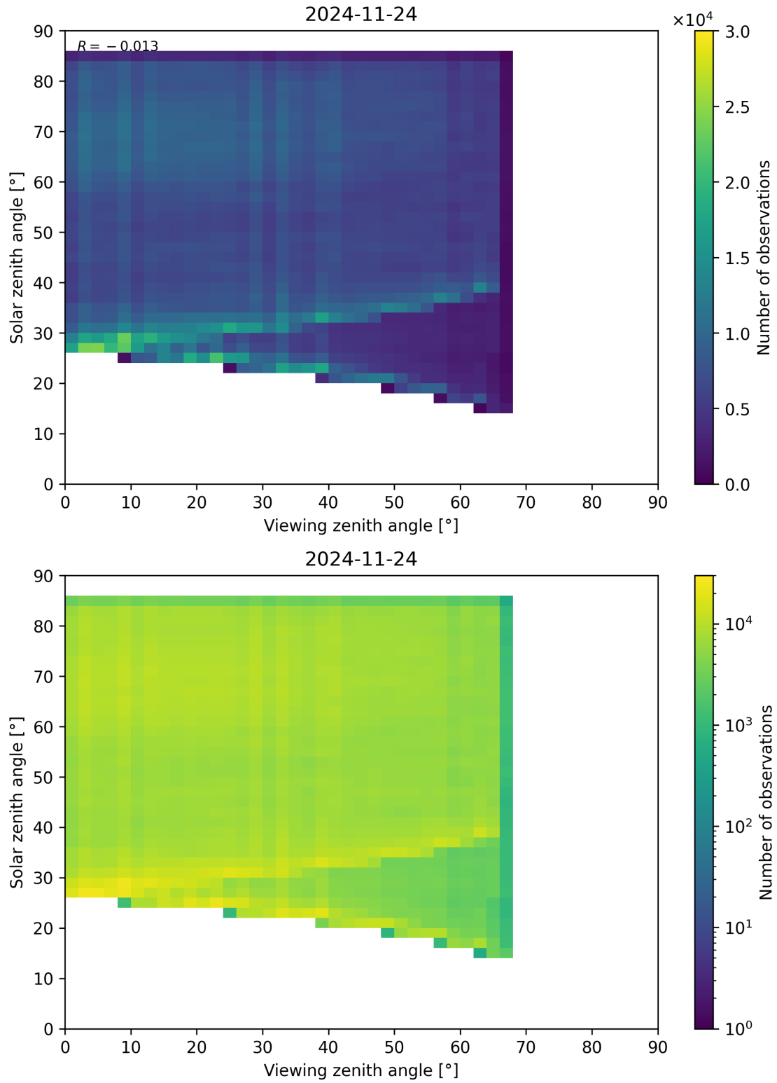
Figure 77: Scatter density plot of “Viewing zenith angle” against “Solar zenith angle” for 2024-11-23 to 2024-11-25.
