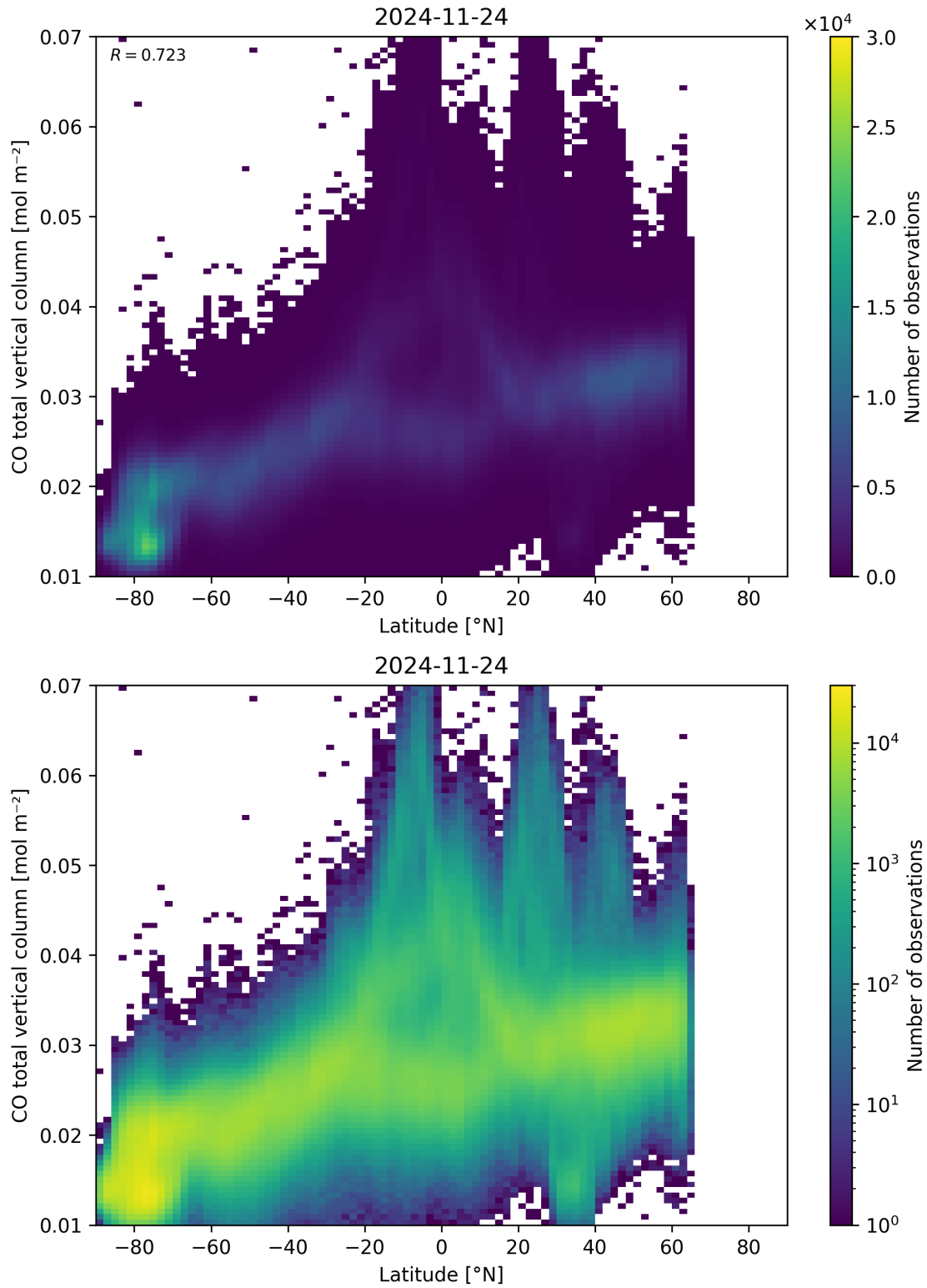
Figure 51: Scatter density plot of “Latitude” against “CO total vertical column” for 2024-11-23 to 2024-11-25.
