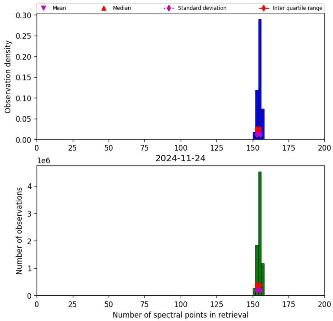
Figure 21: Histogram of “Number of spectral points in retrieval” for 2024-11-23 to 2024-11-25
