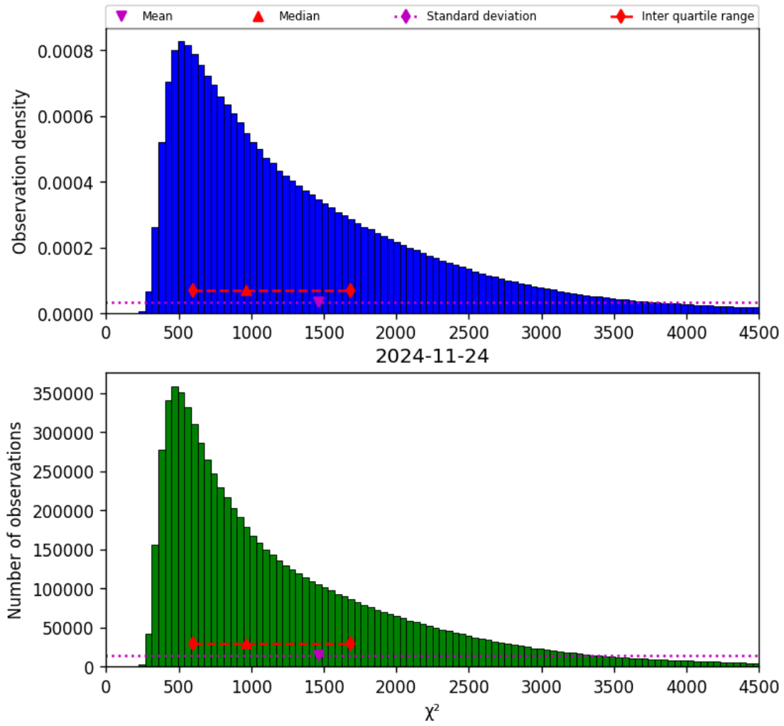
Figure 22: Histogram of “ \chi^2 ” for 2024-11-23 to 2024-11-25
