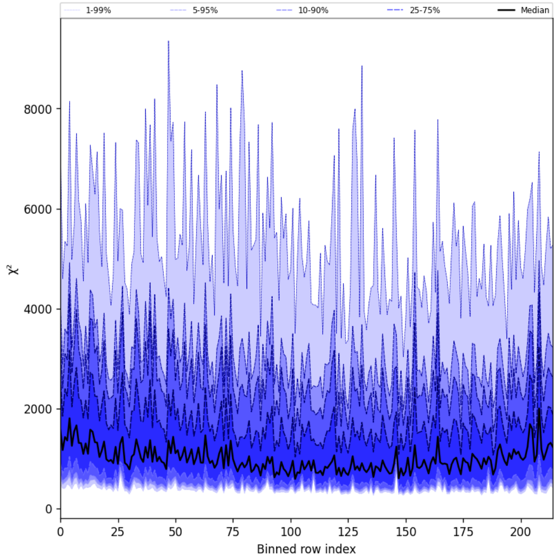
Figure 30: Along track statistics of “ \chi^2 ” for 2024-11-23 to 2024-11-25
