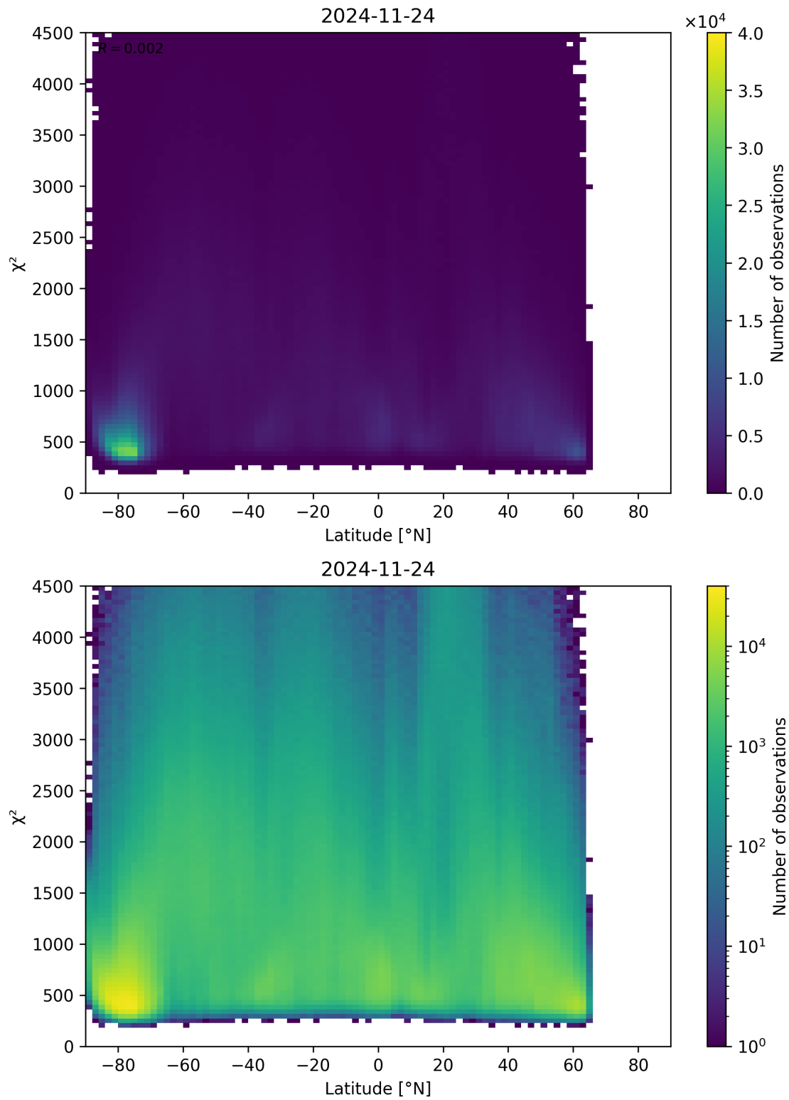
Figure 54: Scatter density plot of “Latitude” against “ \chi^2 ” for 2024-11-23 to 2024-11-25.
