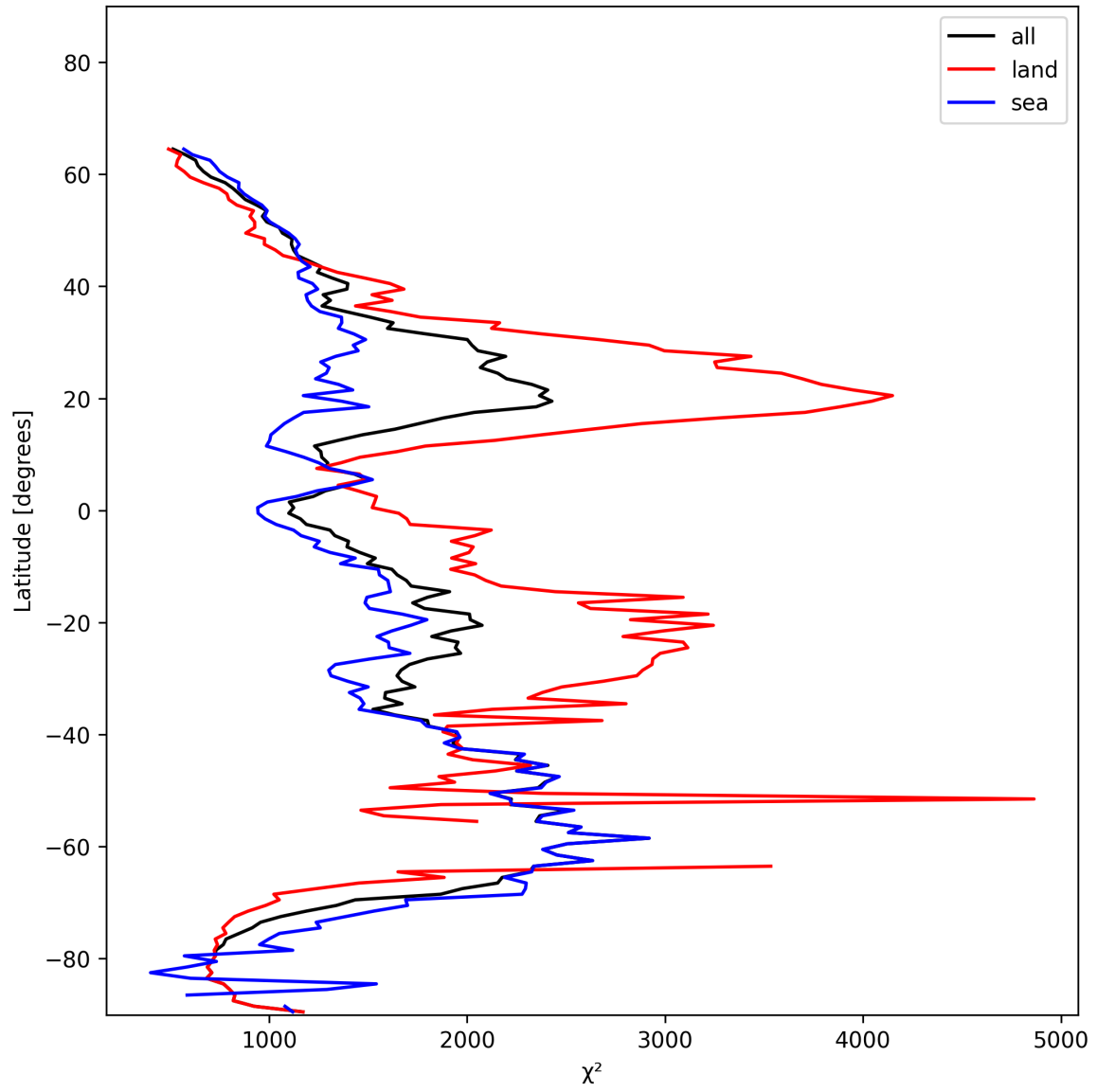
Figure 14: Zonal average of “ \chi^2 ” for 2024-11-23 to 2024-11-25.
