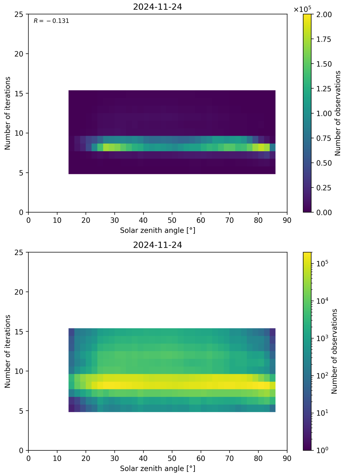
Figure 67: Scatter density plot of “Solar zenith angle” against “Number of iterations” for 2024-11-23 to 2024-11-25.
