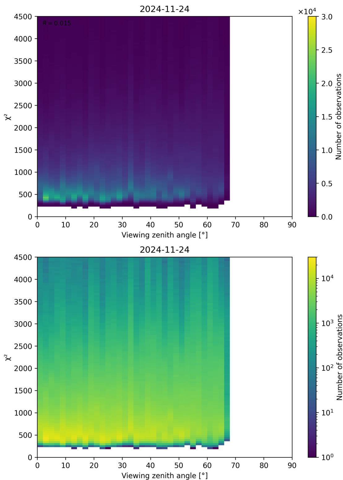
Figure 72: Scatter density plot of “Viewing zenith angle” against “ \chi^2 ” for 2024-11-23 to 2024-11-25.
