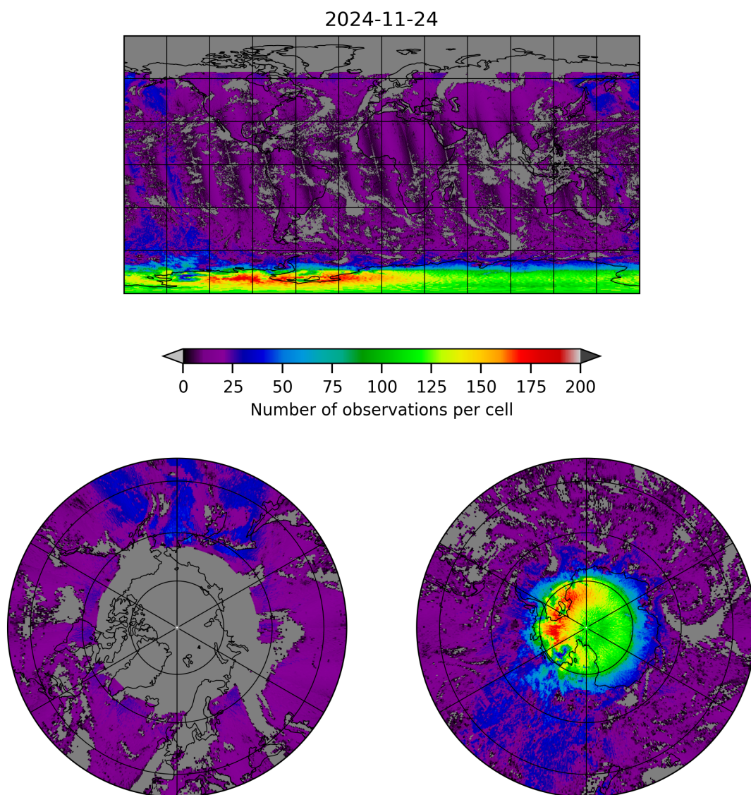
Figure 8: Map of the number of observations for 2024-11-23 to 2024-11-25
