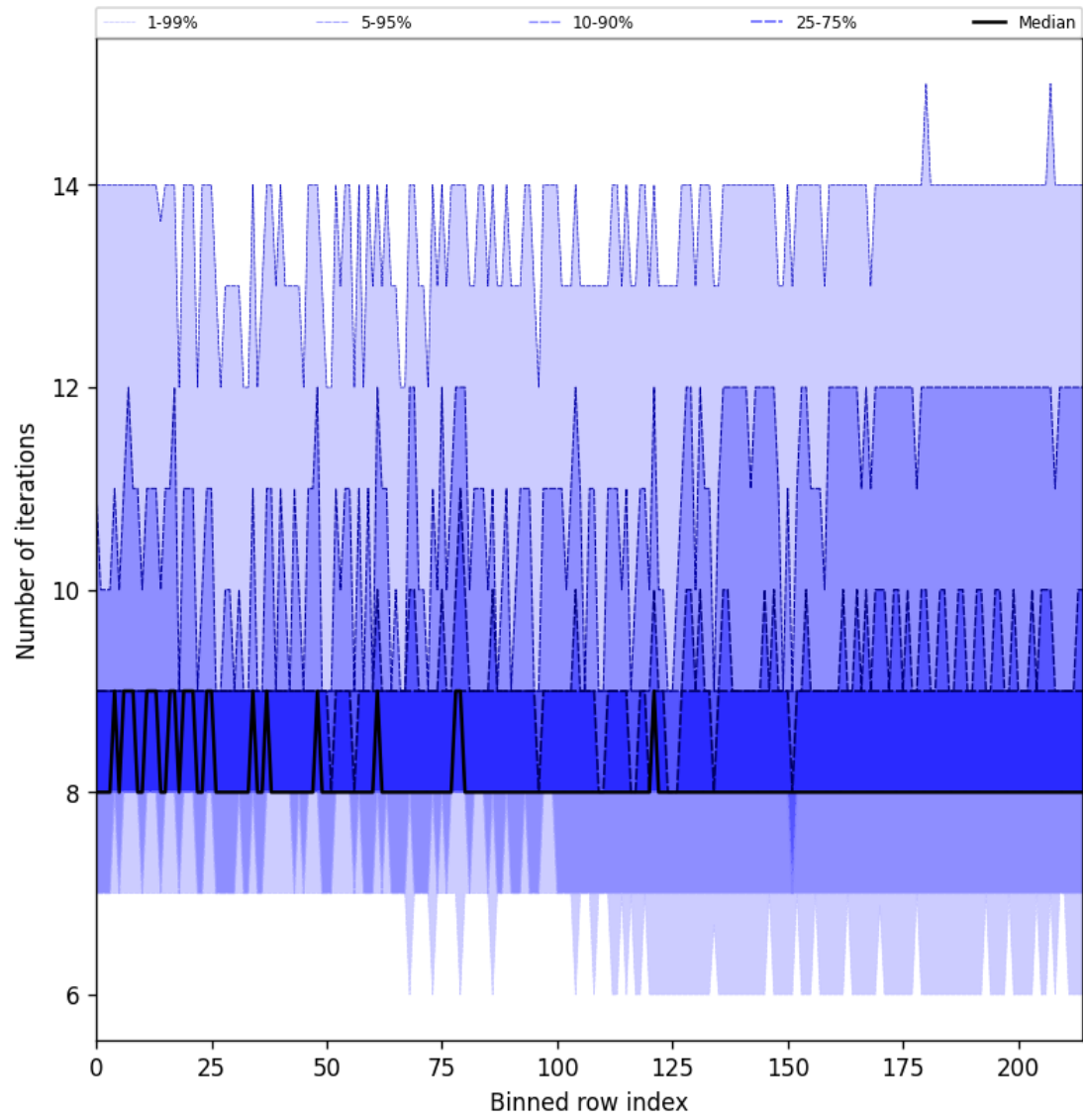
Figure 32: Along track statistics of “Number of iterations” for 2024-11-23 to 2024-11-25
