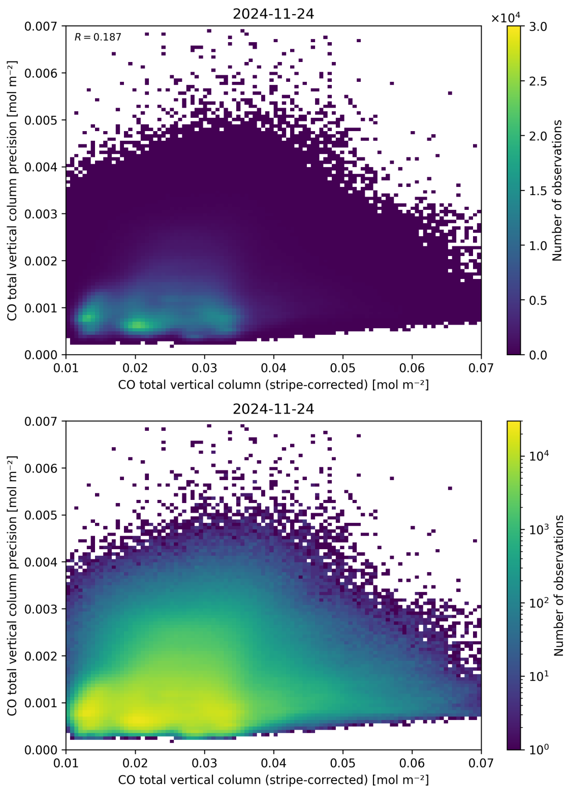
Figure 36: Scatter density plot of “CO total vertical column (stripe-corrected)” against “CO total vertical column precision” for 2024-11-23 to 2024-11-25.
