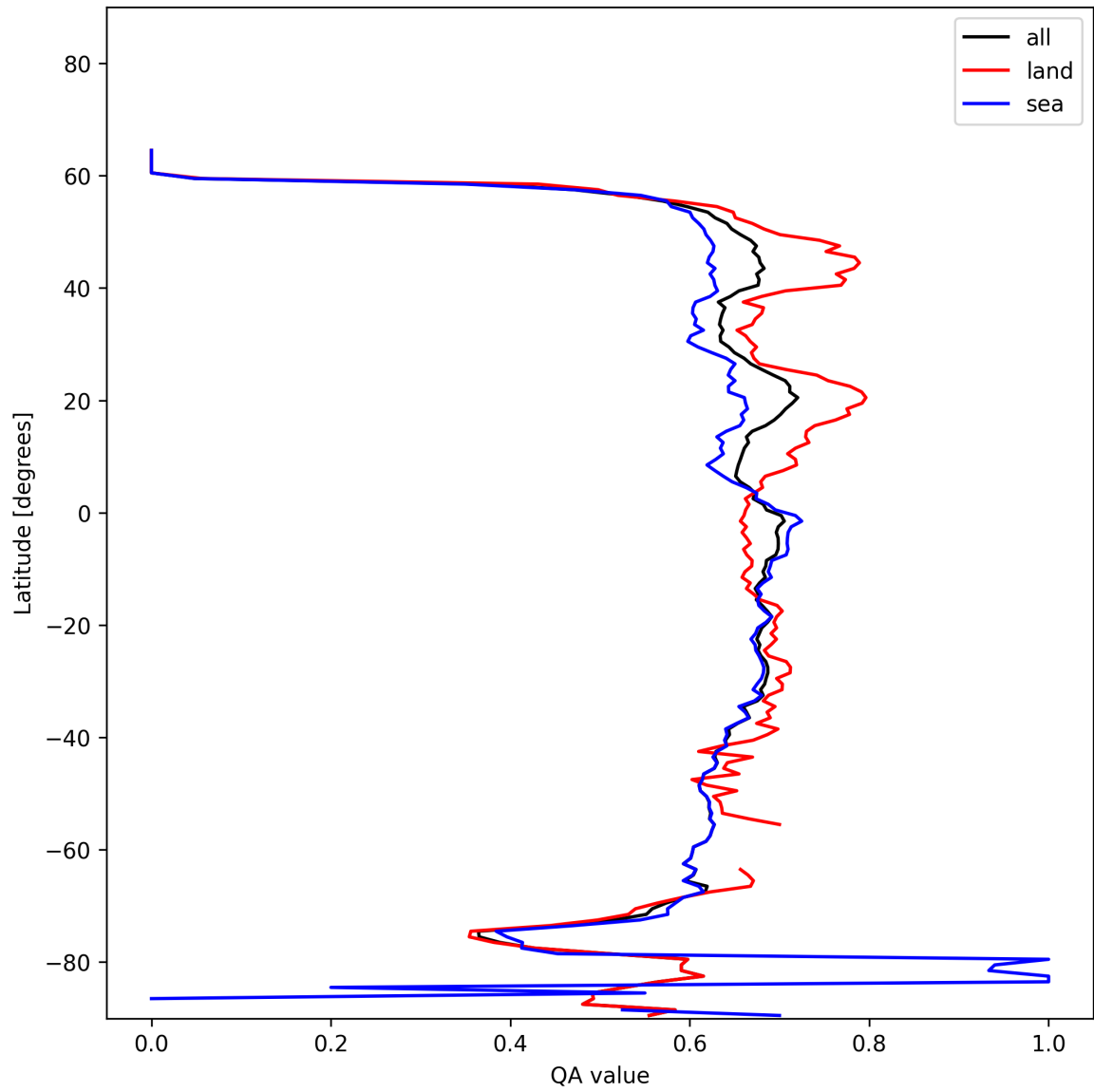
Figure 9: Zonal average of “QA value” for 2024-11-23 to 2024-11-25.
