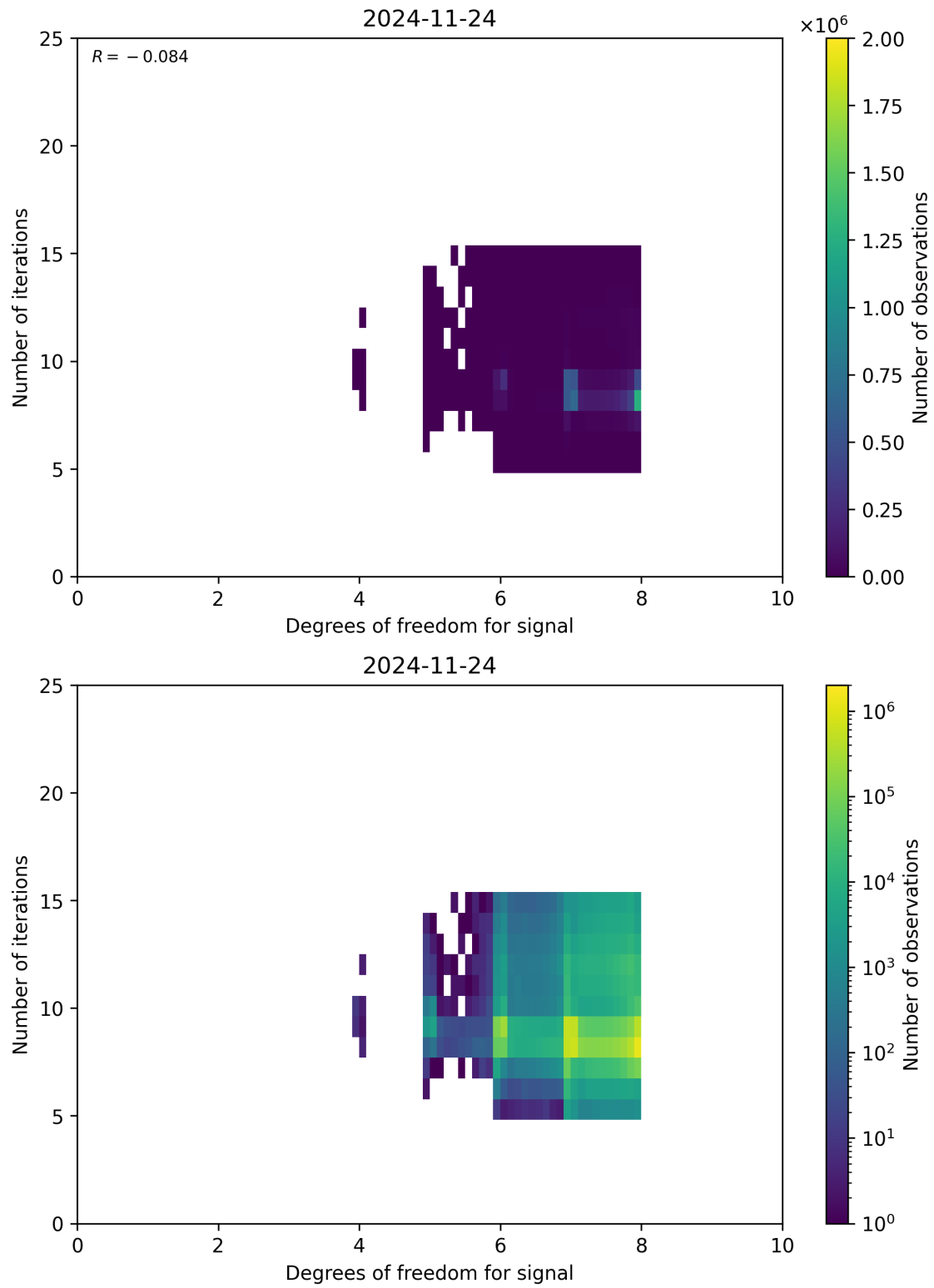
Figure 50: Scatter density plot of “Degrees of freedom for signal” against “Number of iterations” for 2024-11-23 to 2024-11-25.
