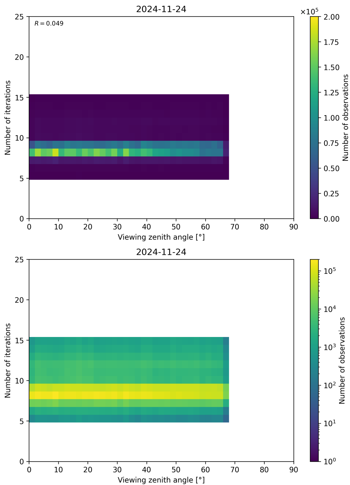
Figure 75: Scatter density plot of “Viewing zenith angle” against “Number of iterations” for 2024-11-23 to 2024-11-25.
