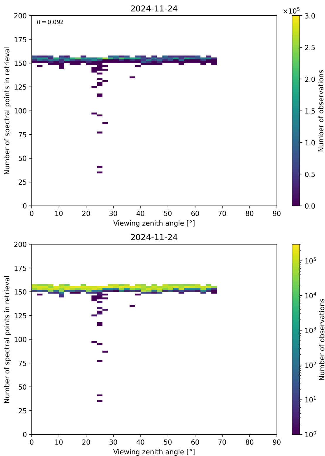
Figure 76: Scatter density plot of “Viewing zenith angle” against “Number of spectral points in retrieval” for 2024-11-23 to 2024-11-25.
