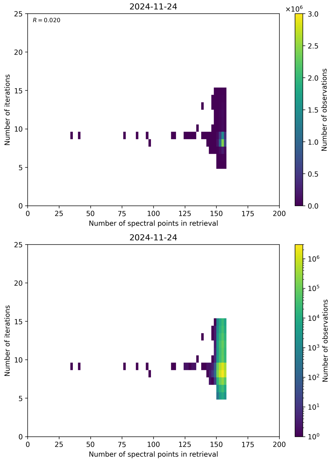
Figure 60: Scatter density plot of “Number of spectral points in retrieval” against “Number of iterations” for 2024-11-23 to 2024-11-25.
