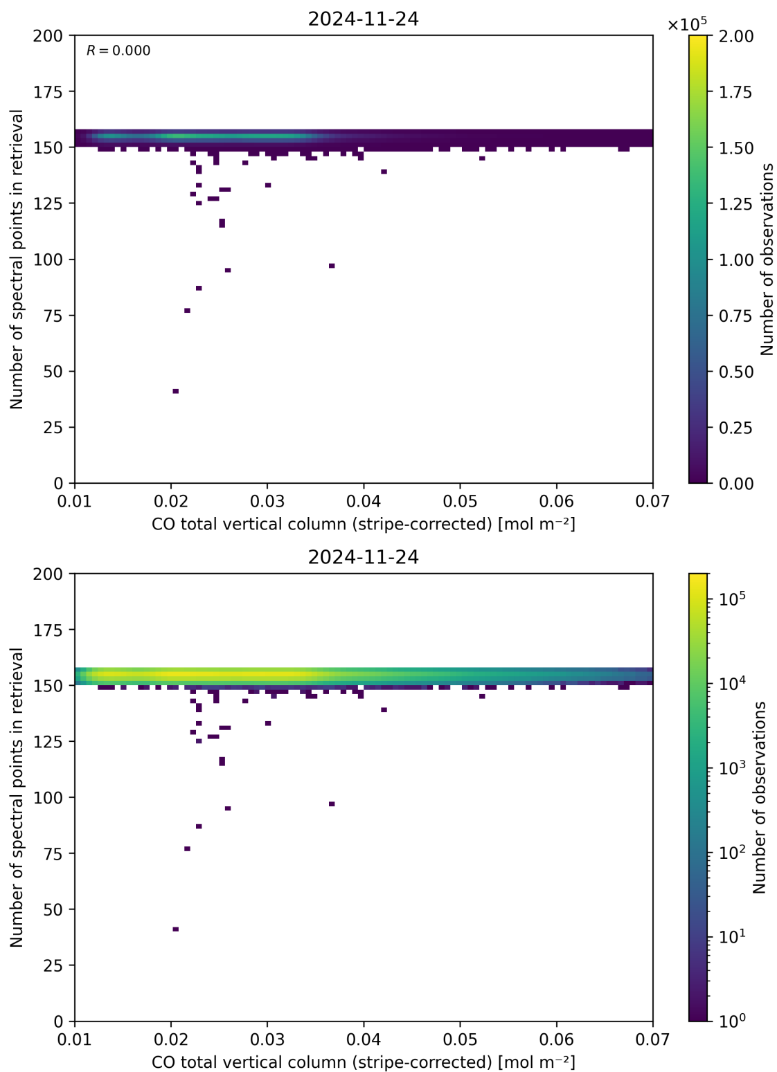
Figure 40: Scatter density plot of “CO total vertical column (stripe-corrected)” against “Number of spectral points in retrieval” for 2024-11-23 to 2024-11-25.
