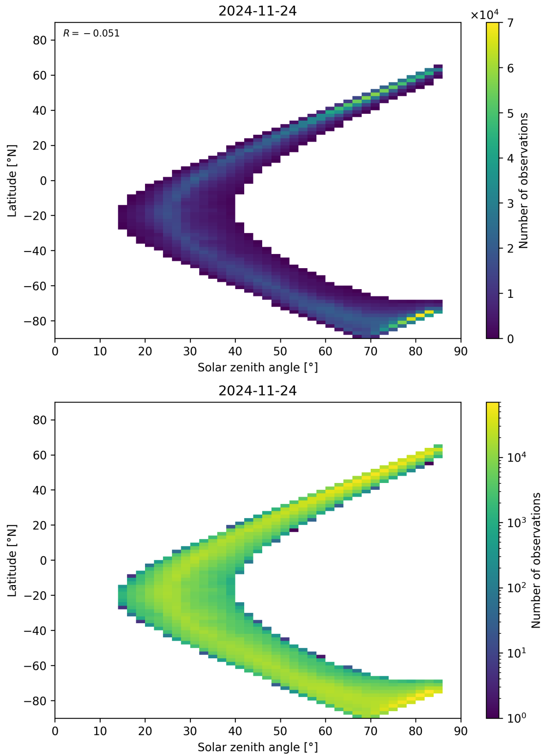
Figure 66: Scatter density plot of “Solar zenith angle” against “Latitude” for 2024-11-23 to 2024-11-25.
