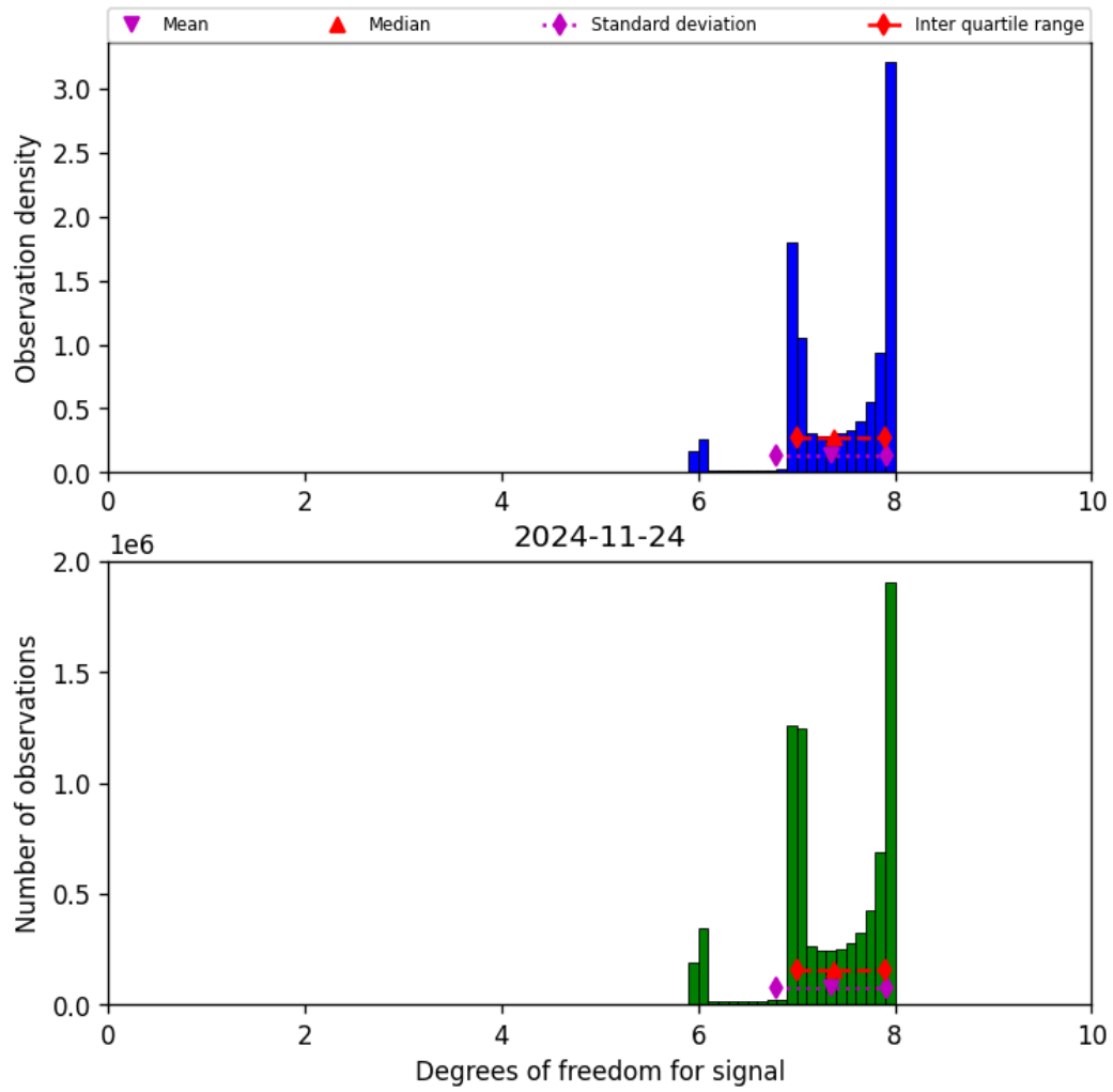
Figure 23: Histogram of “Degrees of freedom for signal” for 2024-11-23 to 2024-11-25
