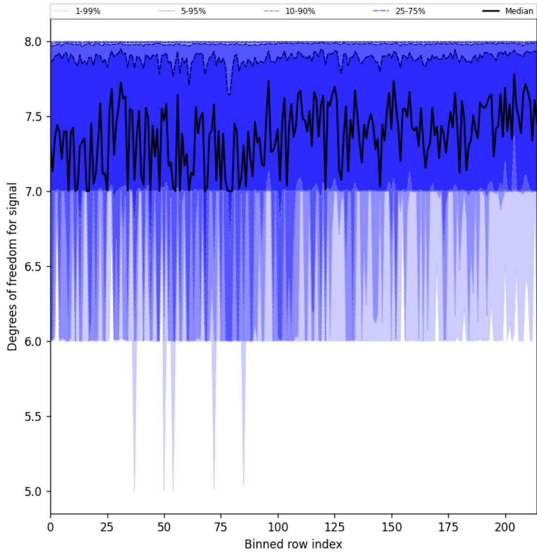
Figure 31: Along track statistics of “Degrees of freedom for signal” for 2024-11-23 to 2024-11-25
