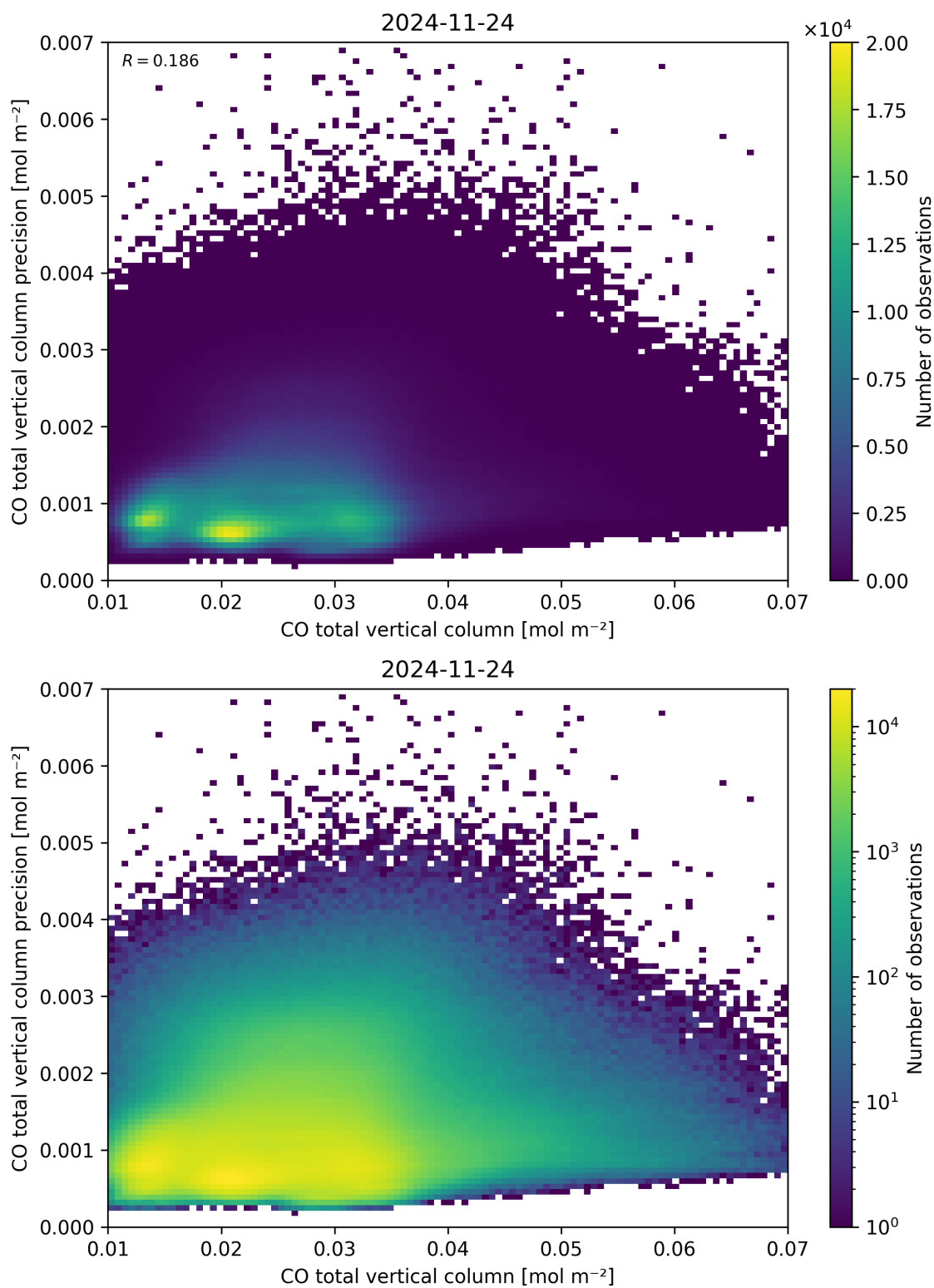
Figure 34: Scatter density plot of “CO total vertical column” against “CO total vertical column precision” for 2024-11-23 to 2024-11-25.
