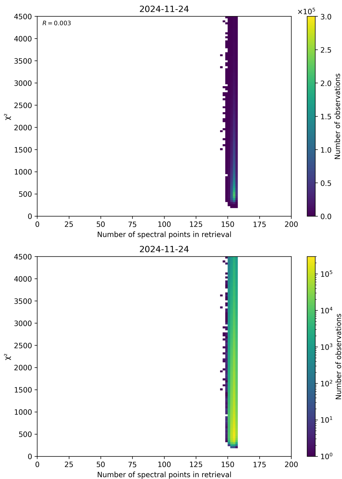
Figure 58: Scatter density plot of “Number of spectral points in retrieval” against “ \chi^2 ” for 2024-11-23 to 2024-11-25.
