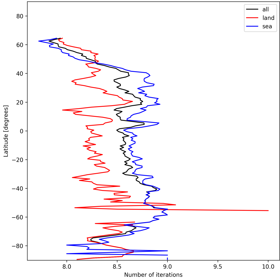
Figure 16: Zonal average of “Number of iterations” for 2024-11-23 to 2024-11-25.
