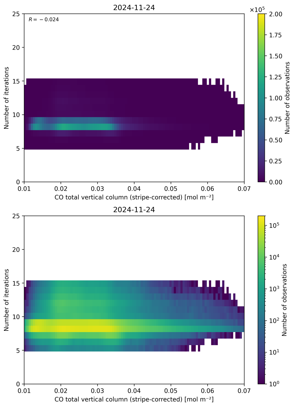
Figure 39: Scatter density plot of “CO total vertical column (stripe-corrected)” against “Number of iterations” for 2024-11-23 to 2024-11-25.
