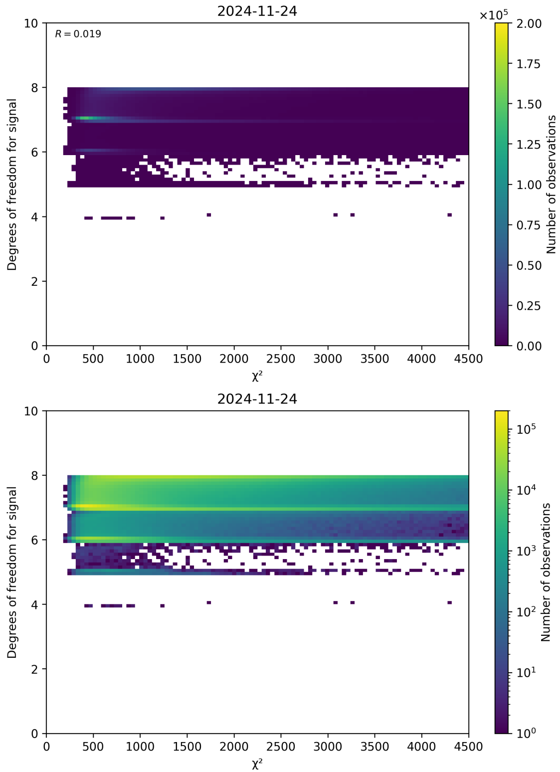
Figure 48: Scatter density plot of “ \chi^2 ” against “Degrees of freedom for signal” for 2024-11-23 to 2024-11-25.
