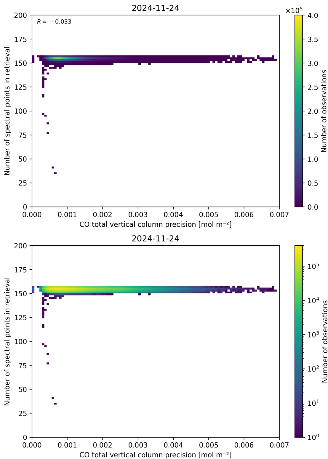
Figure 47: Scatter density plot of “CO total vertical column precision” against “Number of spectral points in retrieval” for 2024-11-23 to 2024-11-25.
