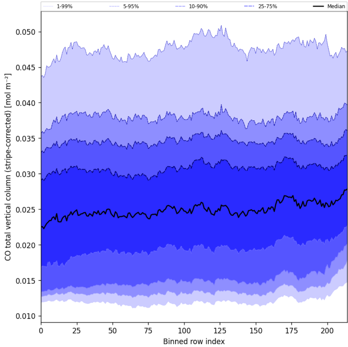
Figure 27: Along track statistics of “CO total vertical column (stripe-corrected)” for 2024-11-23 to 2024-11-25
