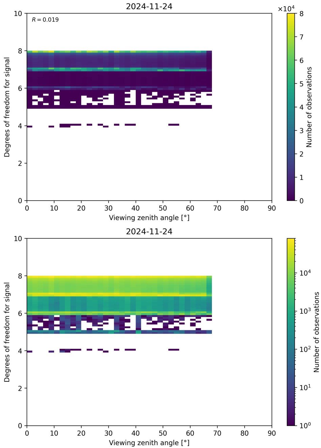
Figure 73: Scatter density plot of “Viewing zenith angle” against “Degrees of freedom for signal” for 2024-11-23 to 2024-11-25.
