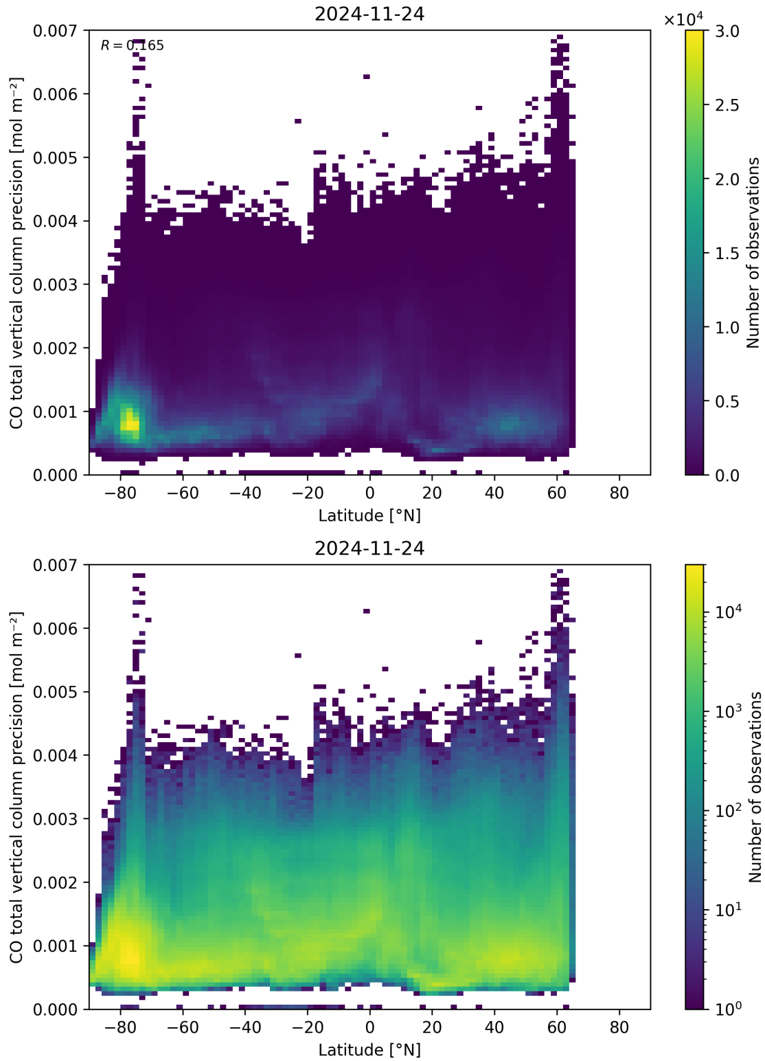
Figure 53: Scatter density plot of “Latitude” against “CO total vertical column precision” for 2024-11-23 to 2024-11-25.
