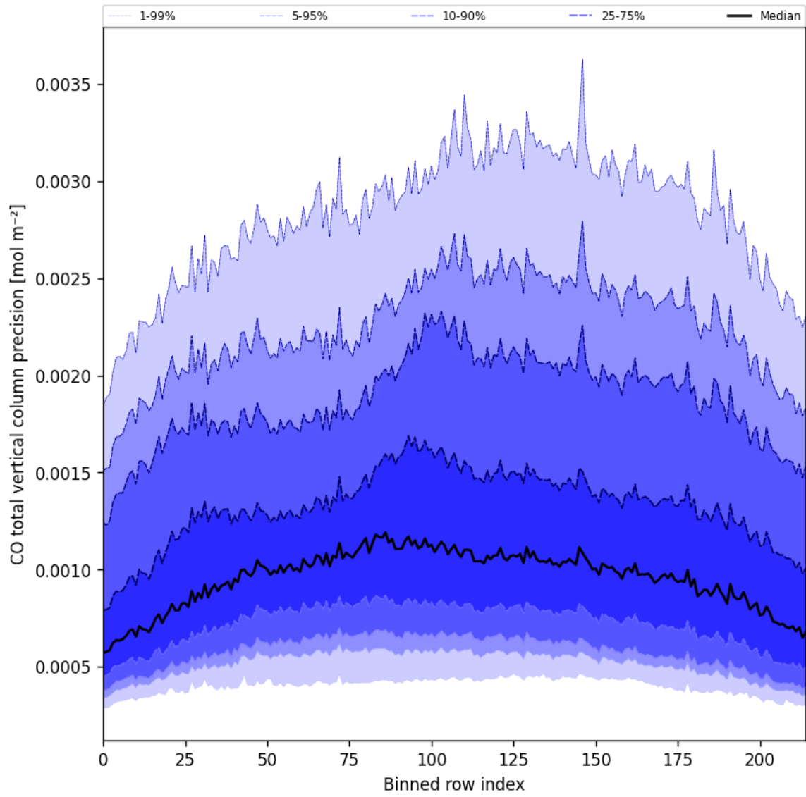
Figure 28: Along track statistics of “CO total vertical column precision” for 2024-11-23 to 2024-11-25
