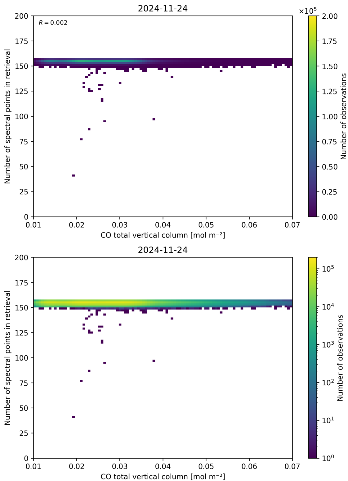
Figure 43: Scatter density plot of “CO total vertical column” against “Number of spectral points in retrieval” for 2024-11-23 to 2024-11-25.
