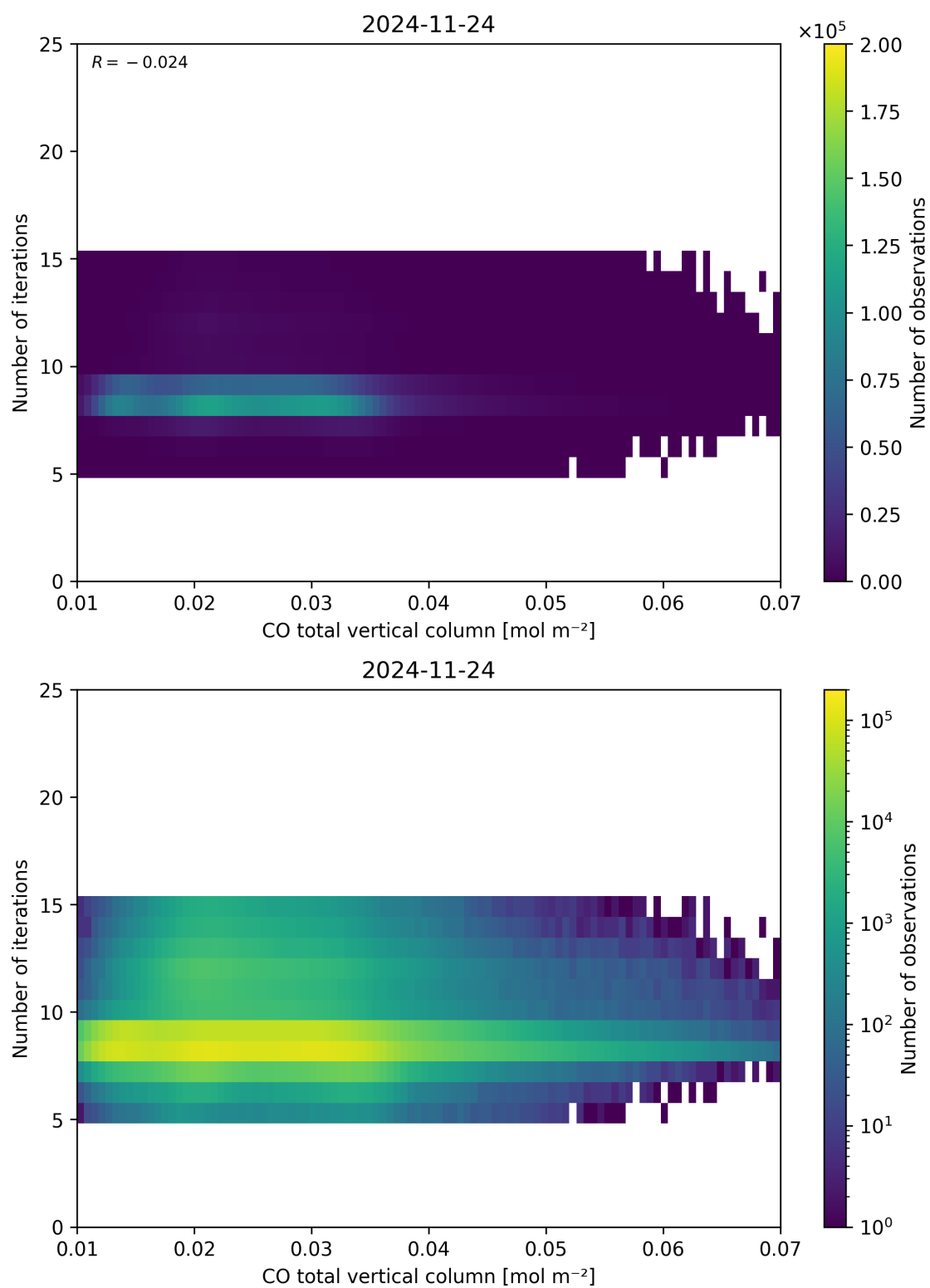
Figure 42: Scatter density plot of “CO total vertical column” against “Number of iterations” for 2024-11-23 to 2024-11-25.
