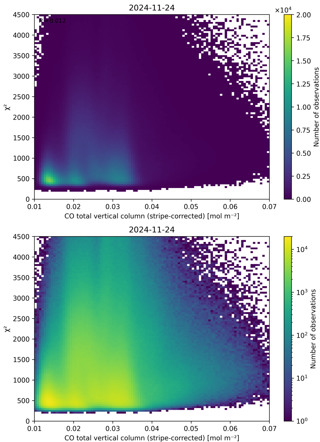
Figure 37: Scatter density plot of “CO total vertical column (stripe-corrected)” against “ \chi^2 ” for 2024-11-23 to 2024-11-25.
