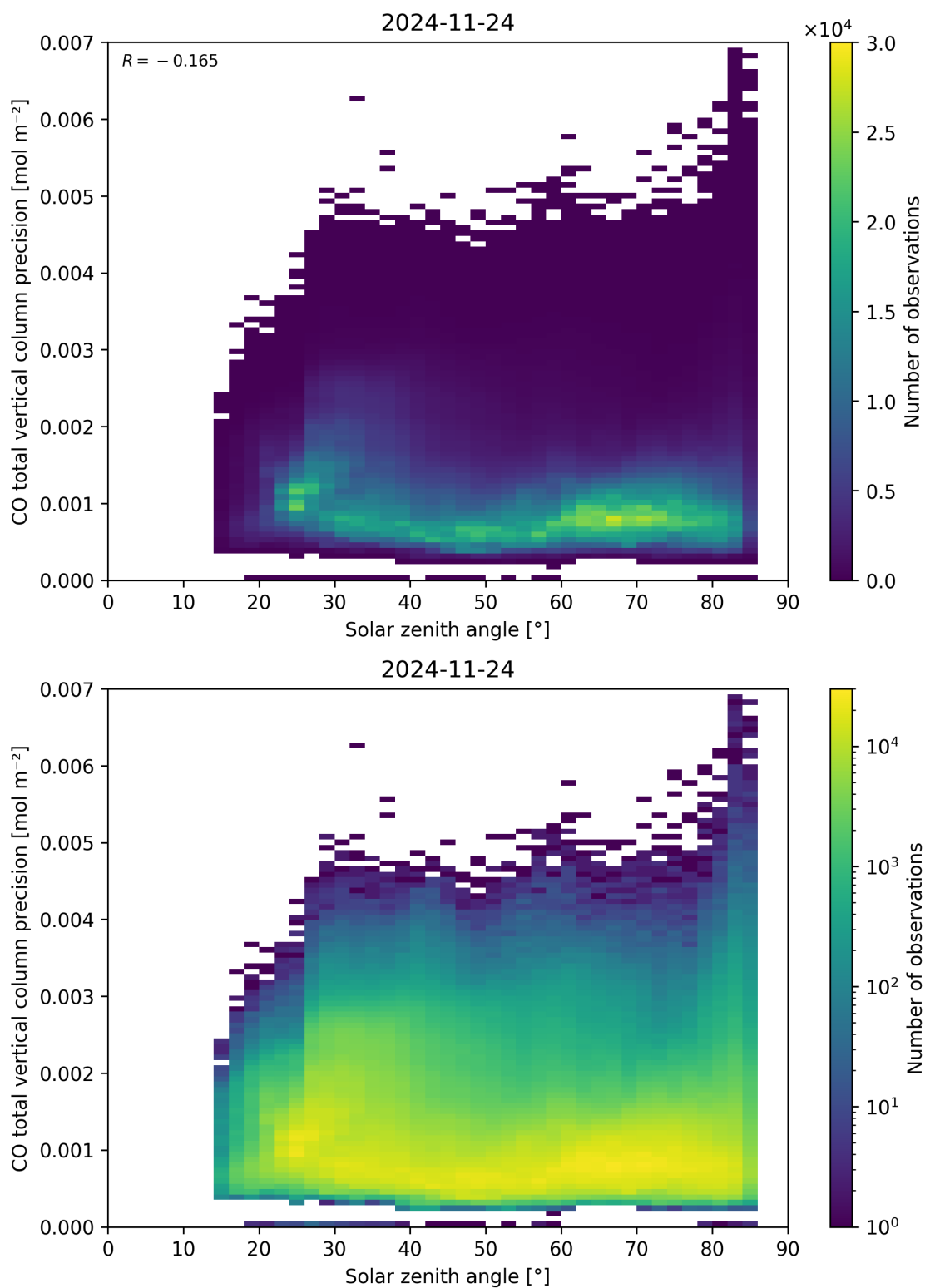
Figure 63: Scatter density plot of “Solar zenith angle” against “CO total vertical column precision” for 2024-11-23 to 2024-11-25.
