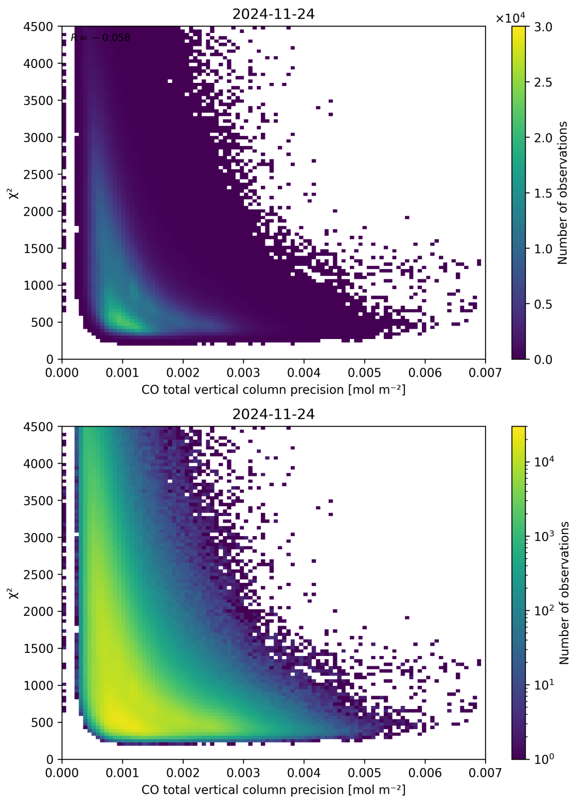
Figure 44: Scatter density plot of “CO total vertical column precision” against “ \chi^2 ” for 2024-11-23 to 2024-11-25.
