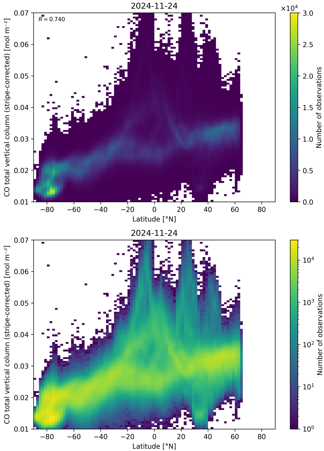
Figure 52: Scatter density plot of “Latitude” against “CO total vertical column (stripe-corrected)” for 2024-11-23 to 2024-11-25.
