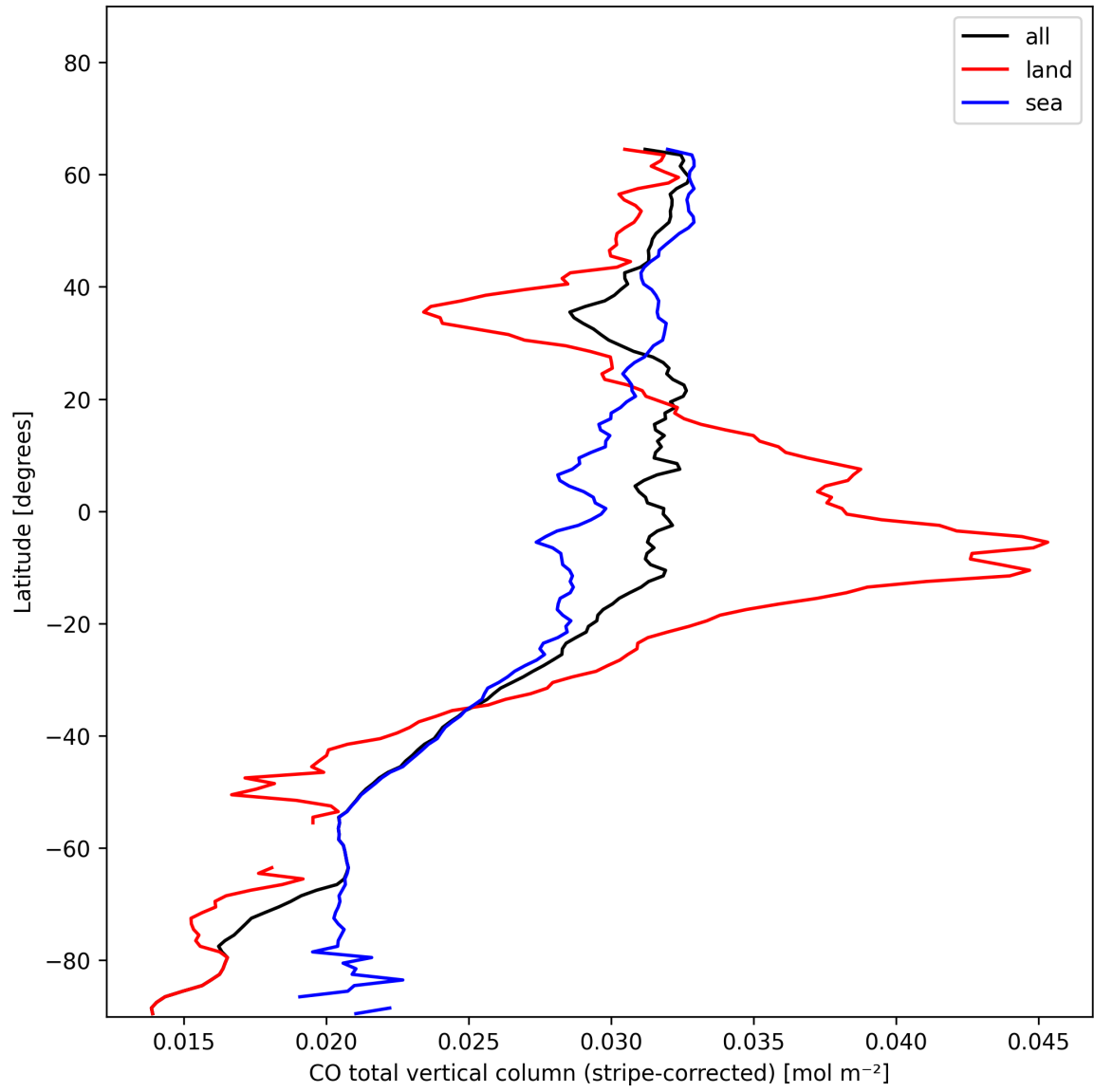
Figure 11: Zonal average of “CO total vertical column (stripe-corrected)” for 2024-11-23 to 2024-11-25.
