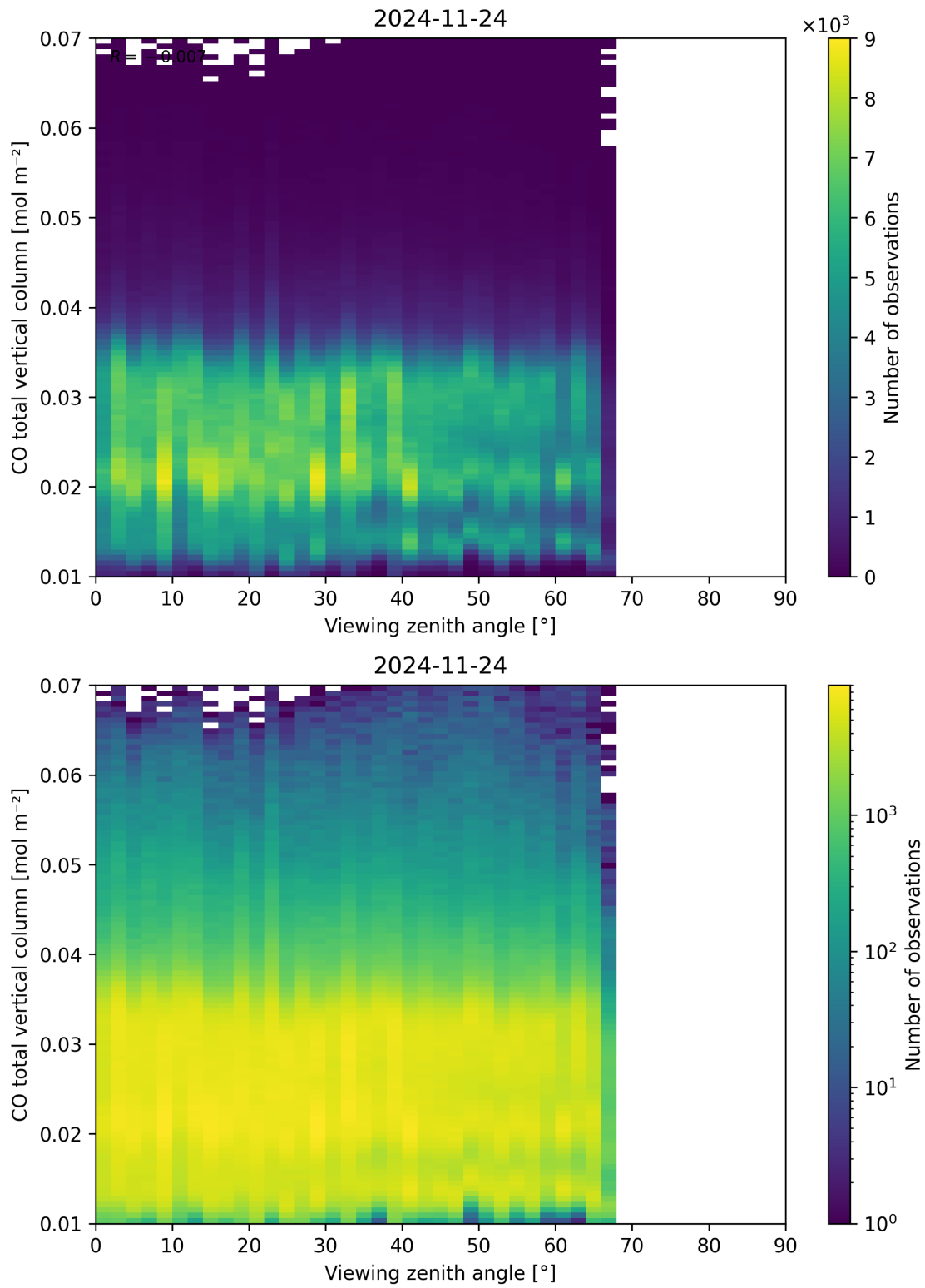
Figure 69: Scatter density plot of “Viewing zenith angle” against “CO total vertical column” for 2024-11-23 to 2024-11-25.
