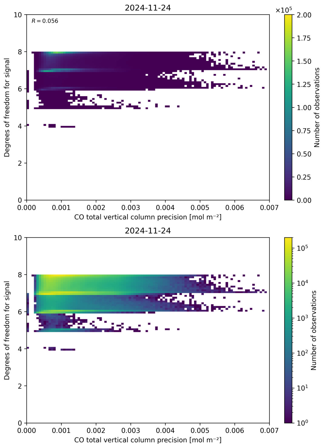
Figure 45: Scatter density plot of “CO total vertical column precision” against “Degrees of freedom for signal” for 2024-11-23 to 2024-11-25.
