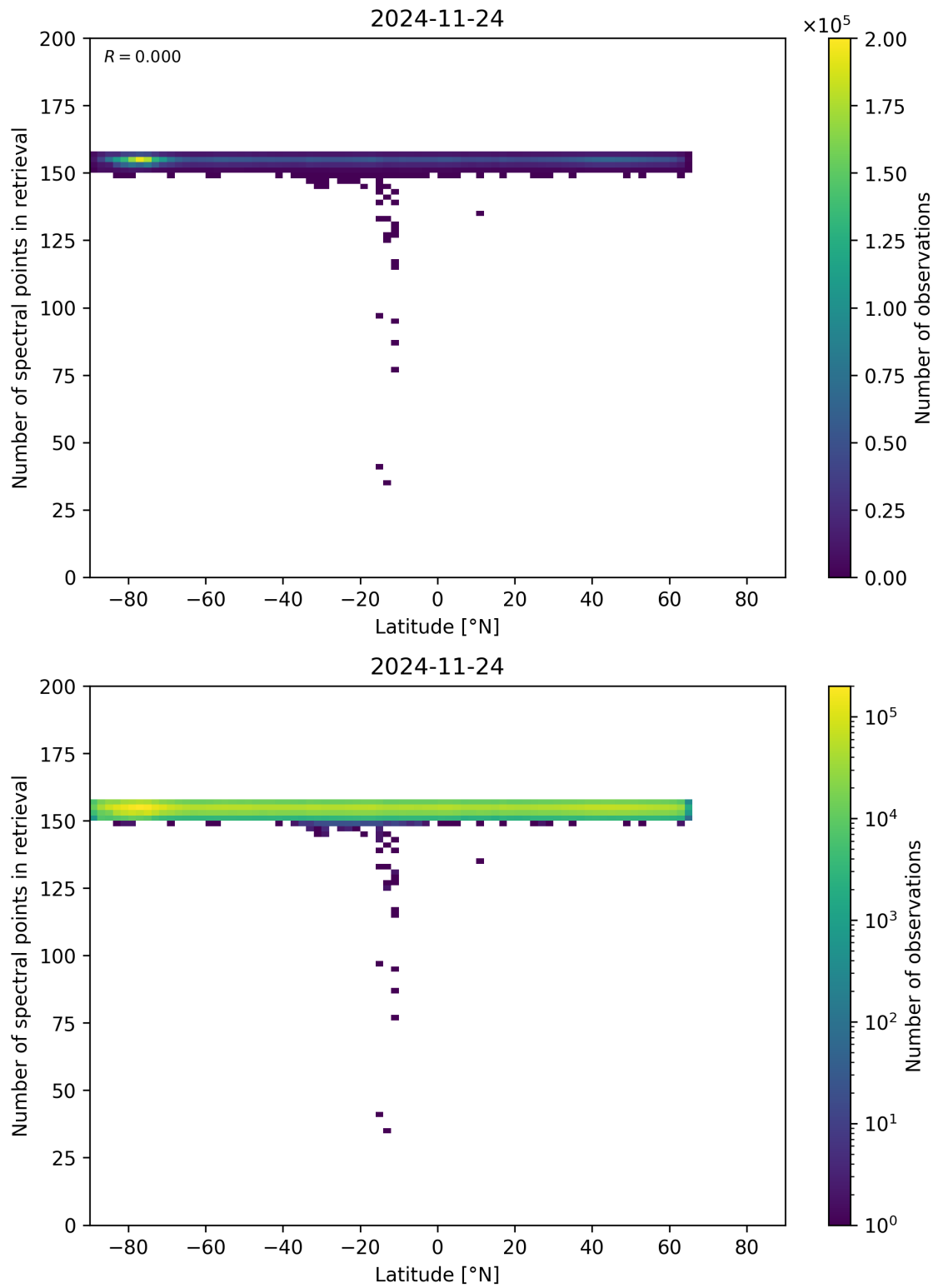
Figure 57: Scatter density plot of “Latitude” against “Number of spectral points in retrieval” for 2024-11-23 to 2024-11-25.
