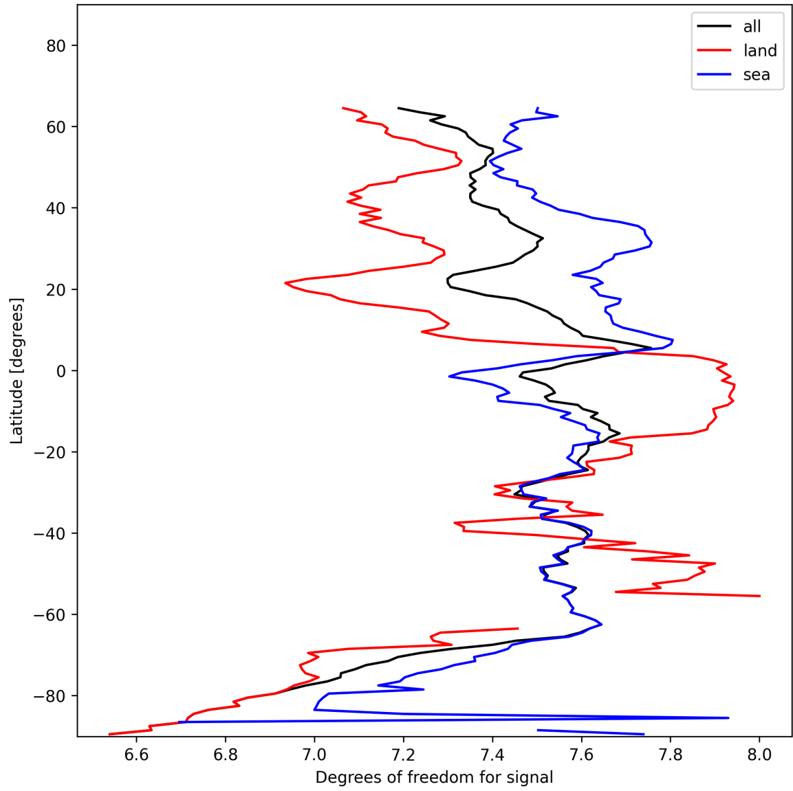
Figure 15: Zonal average of “Degrees of freedom for signal” for 2024-11-23 to 2024-11-25.
