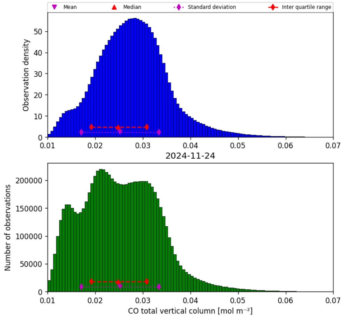
Figure 18: Histogram of “CO total vertical column” for 2024-11-23 to 2024-11-25
