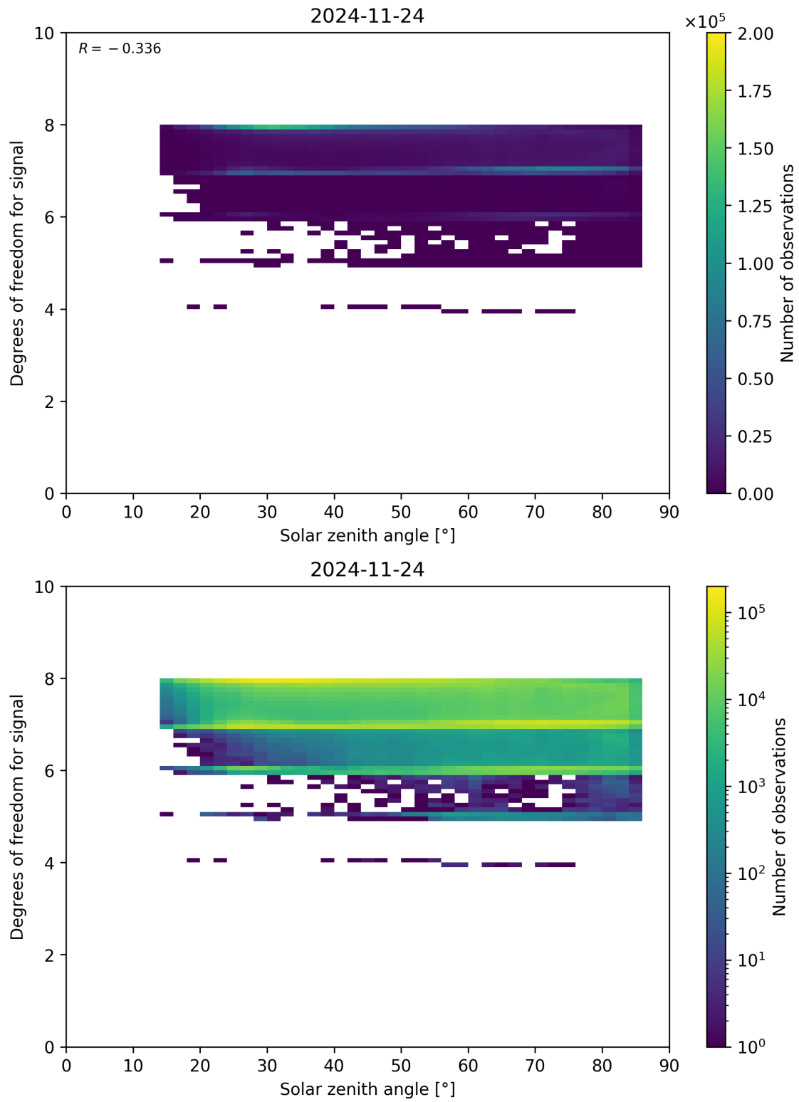
Figure 65: Scatter density plot of “Solar zenith angle” against “Degrees of freedom for signal” for 2024-11-23 to 2024-11-25.
