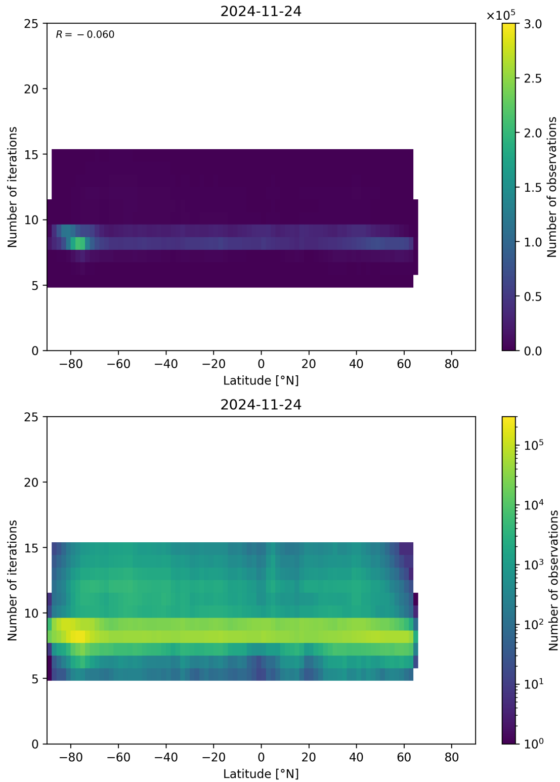
Figure 56: Scatter density plot of “Latitude” against “Number of iterations” for 2024-11-23 to 2024-11-25.
