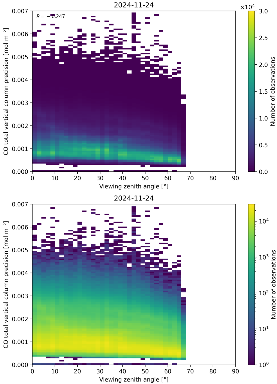
Figure 71: Scatter density plot of “Viewing zenith angle” against “CO total vertical column precision” for 2024-11-23 to 2024-11-25.
