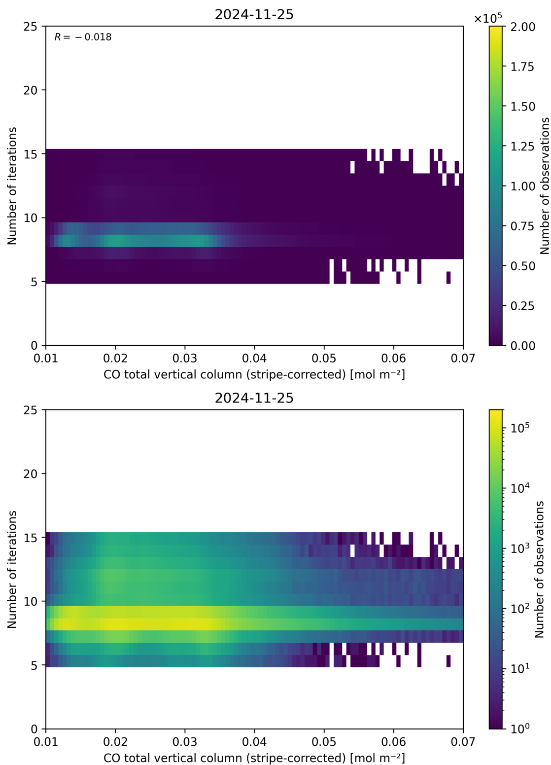
Figure 39: Scatter density plot of “CO total vertical column (stripe-corrected)” against “Number of iterations” for 2024-11-25 to 2024-11-26.
