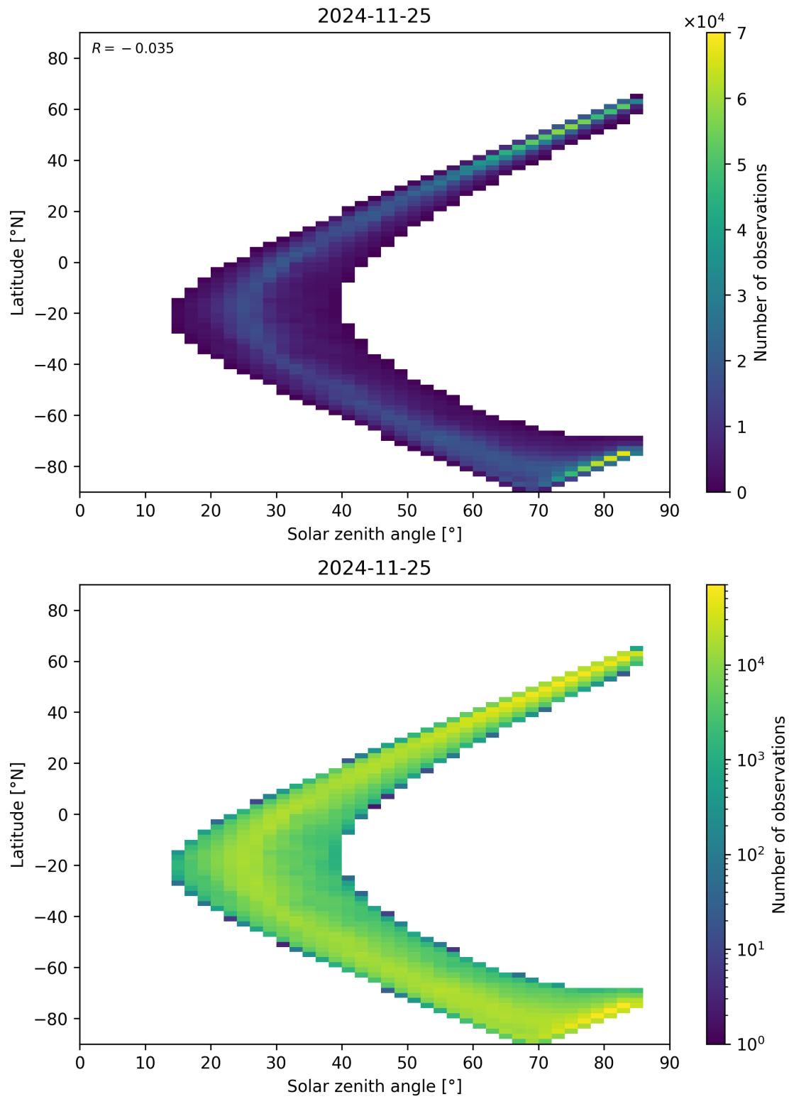
Figure 66: Scatter density plot of “Solar zenith angle” against “Latitude” for 2024-11-25 to 2024-11-26.
