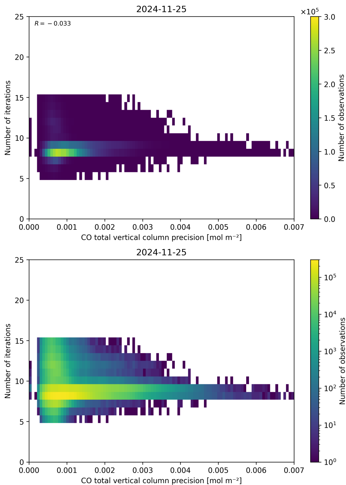
Figure 46: Scatter density plot of “CO total vertical column precision” against “Number of iterations” for 2024-11-25 to 2024-11-26.
