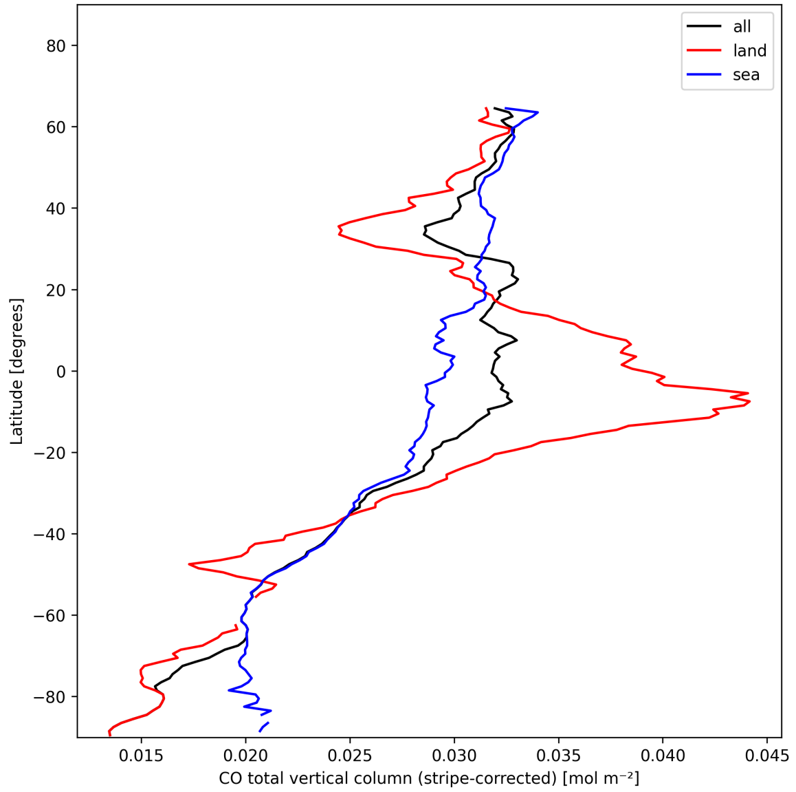
Figure 11: Zonal average of “CO total vertical column (stripe-corrected)” for 2024-11-25 to 2024-11-26.
