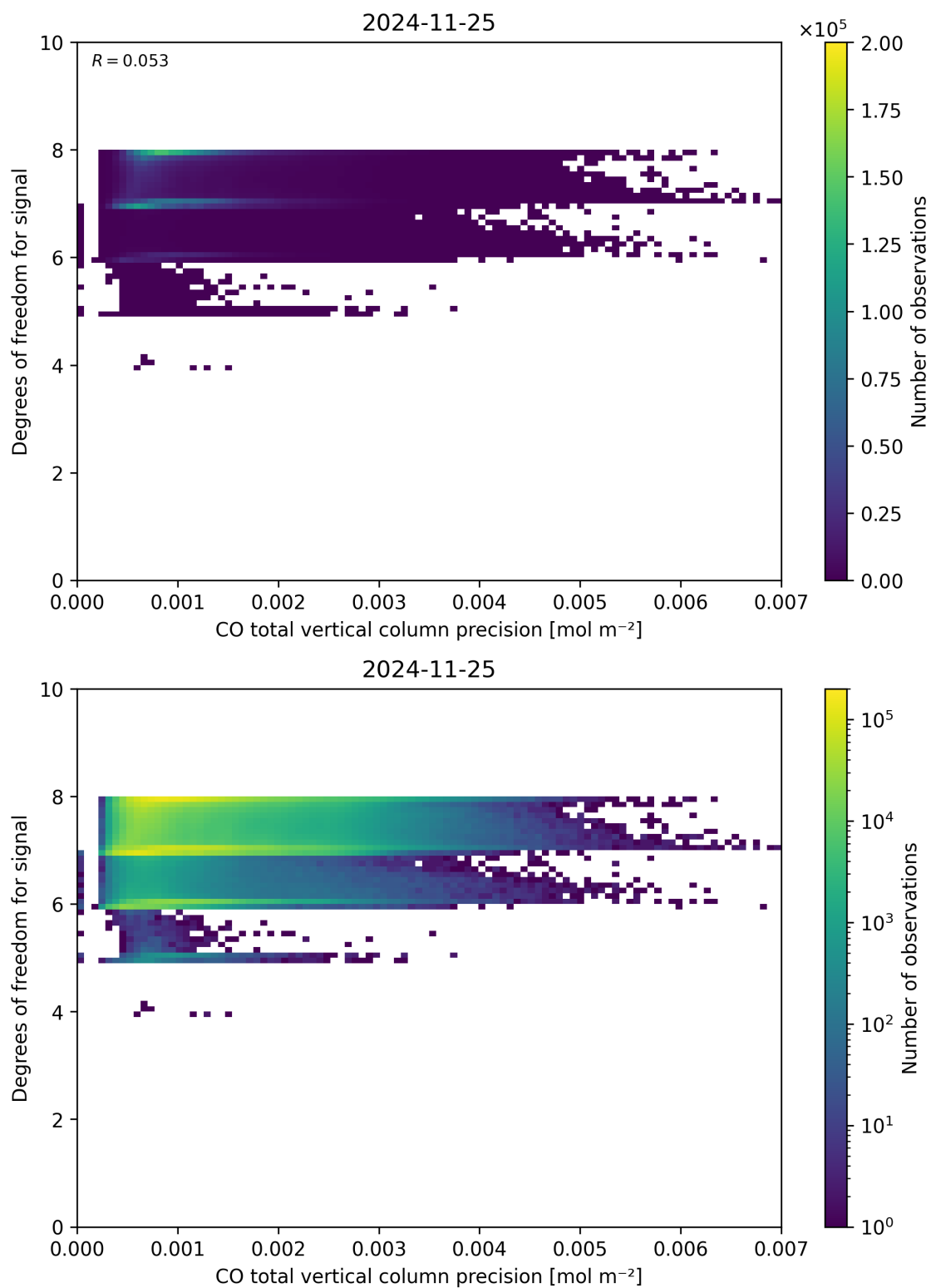
Figure 45: Scatter density plot of “CO total vertical column precision” against “Degrees of freedom for signal” for 2024-11-25 to 2024-11-26.
