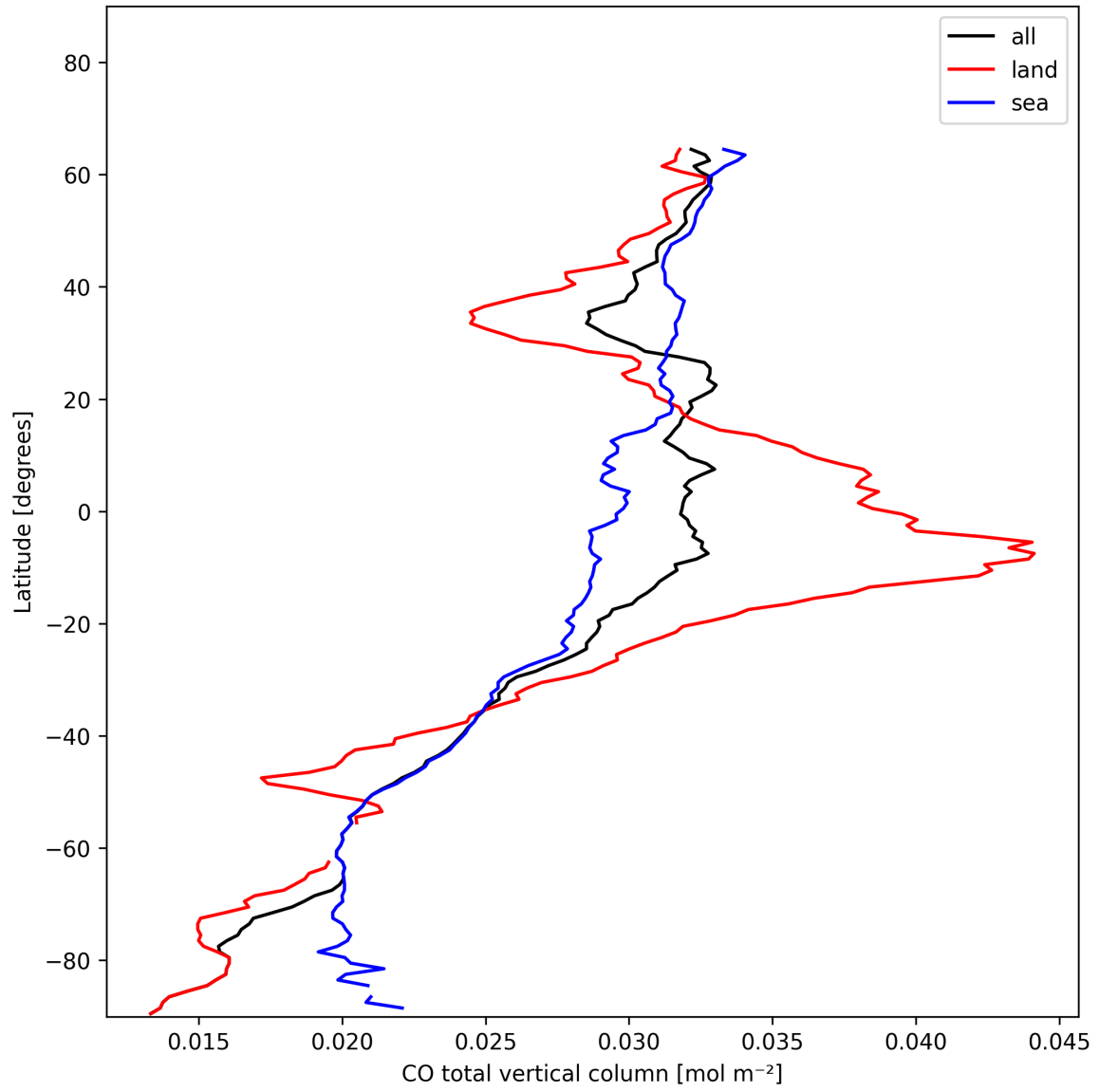
Figure 10: Zonal average of “CO total vertical column” for 2024-11-25 to 2024-11-26.
