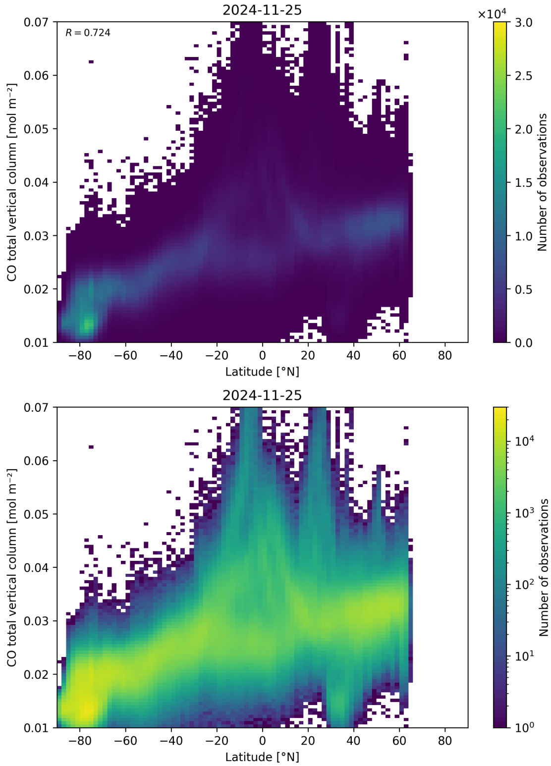
Figure 51: Scatter density plot of “Latitude” against “CO total vertical column” for 2024-11-25 to 2024-11-26.
