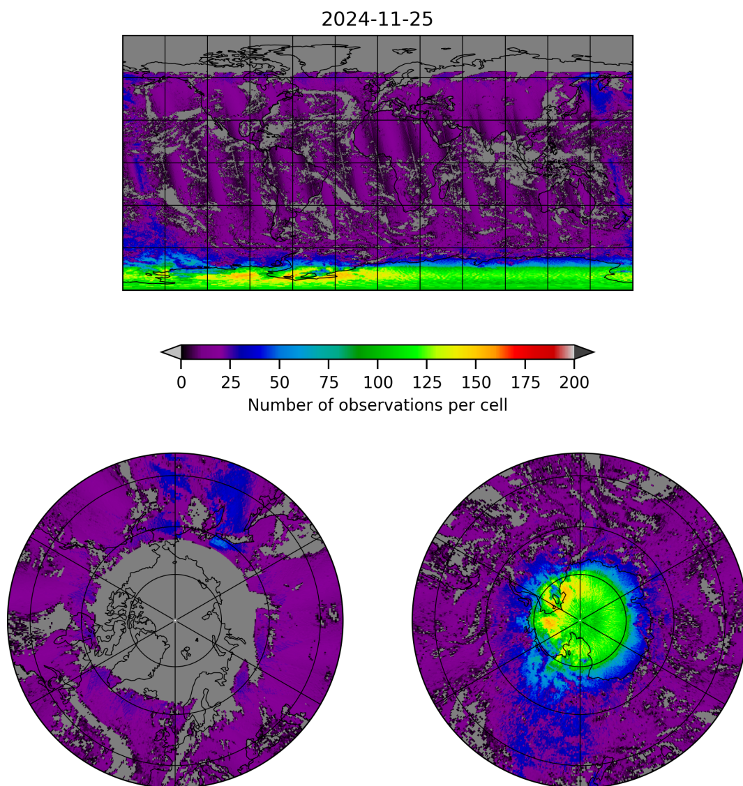
Figure 8: Map of the number of observations for 2024-11-25 to 2024-11-26
