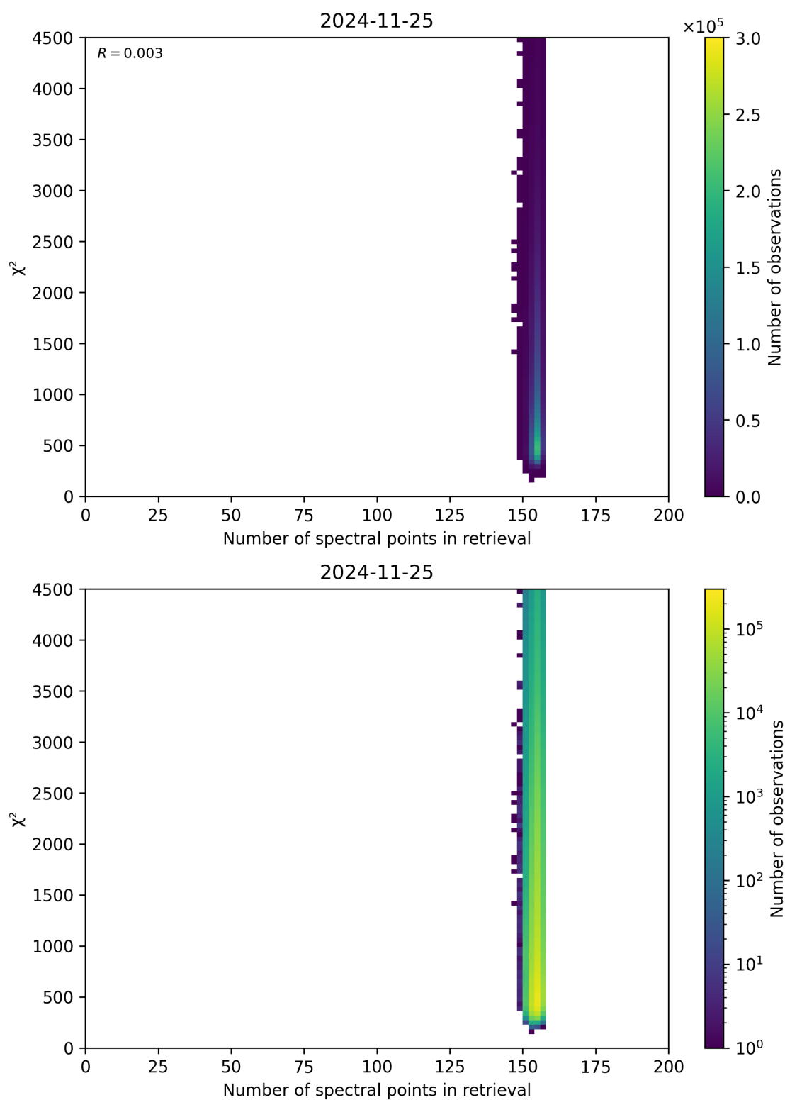
Figure 58: Scatter density plot of “Number of spectral points in retrieval” against “ \chi^2 ” for 2024-11-25 to 2024-11-26.
