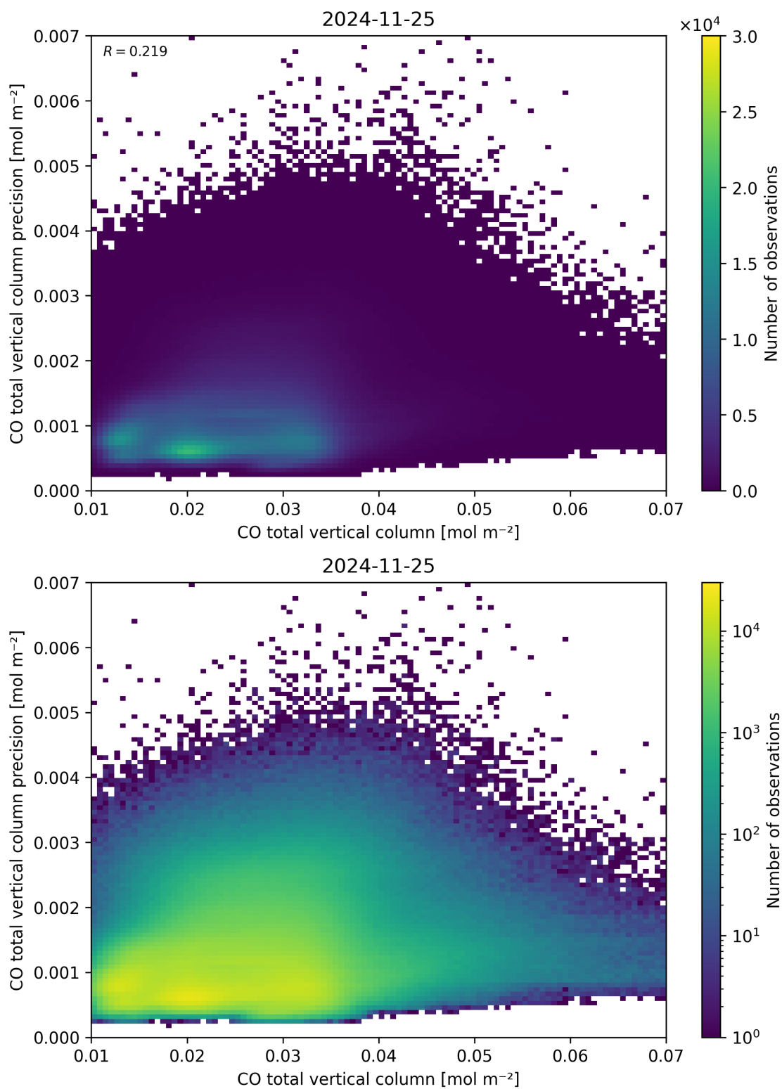
Figure 34: Scatter density plot of “CO total vertical column” against “CO total vertical column precision” for 2024-11-25 to 2024-11-26.
