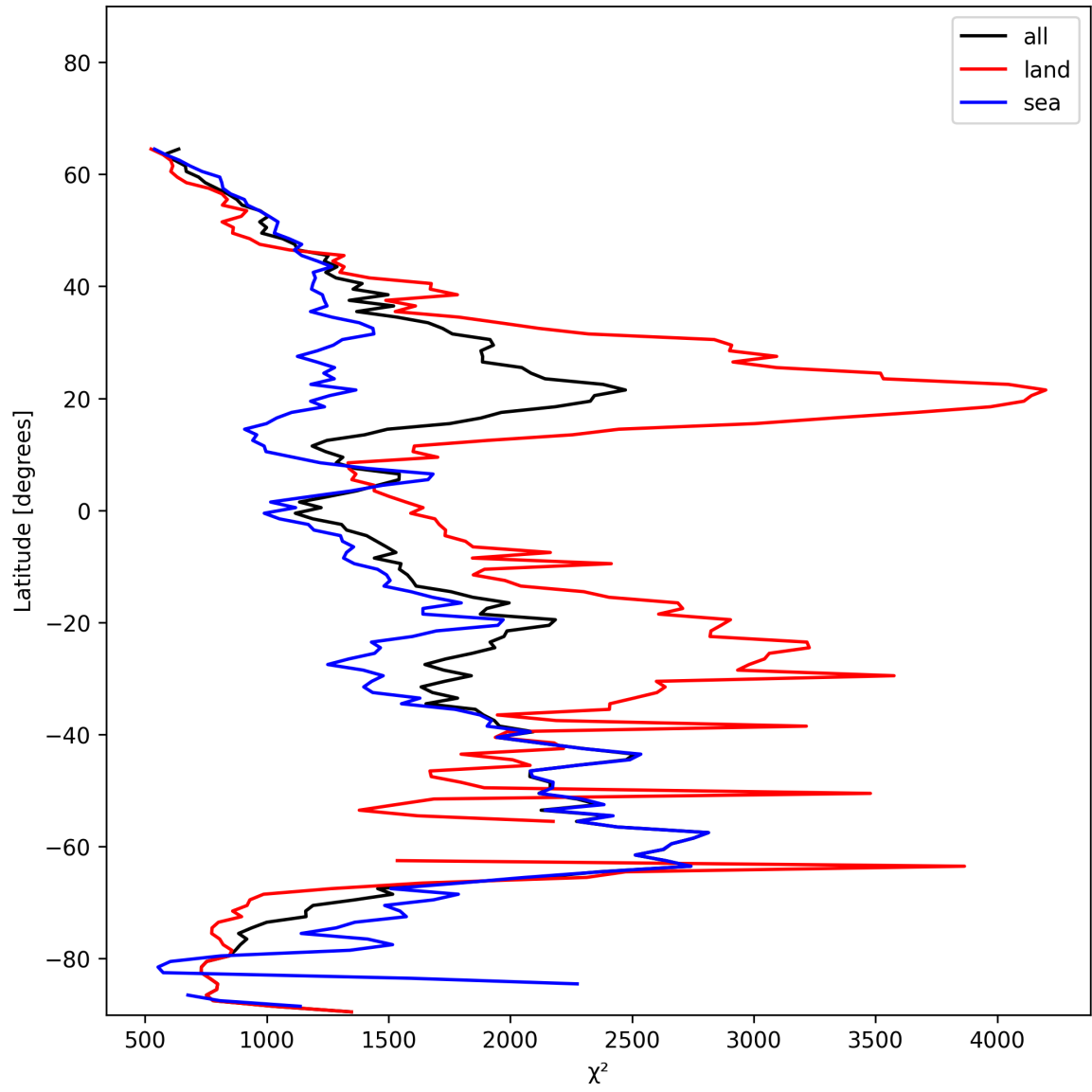
Figure 14: Zonal average of “ \chi^2 ” for 2024-11-25 to 2024-11-26.
