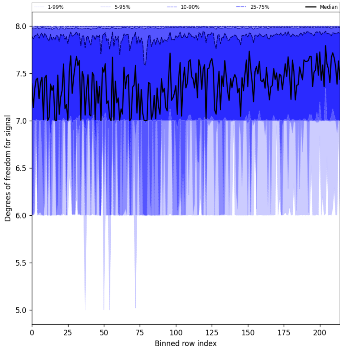
Figure 31: Along track statistics of “Degrees of freedom for signal” for 2024-11-25 to 2024-11-26
