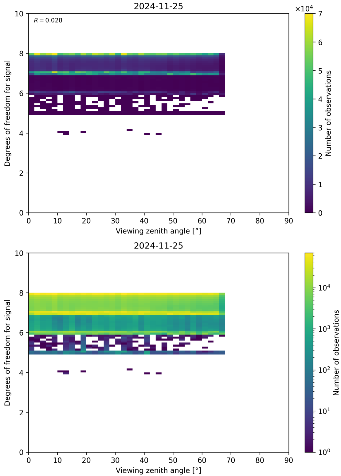
Figure 73: Scatter density plot of “Viewing zenith angle” against “Degrees of freedom for signal” for 2024-11-25 to 2024-11-26.
