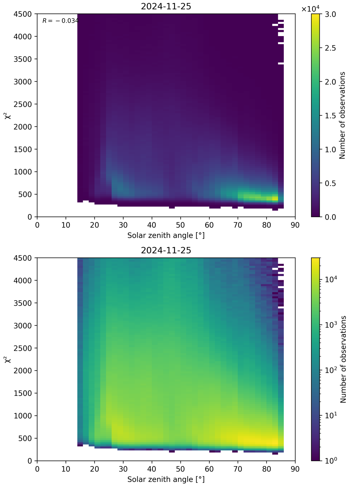
Figure 64: Scatter density plot of “Solar zenith angle” against “ \chi^2 ” for 2024-11-25 to 2024-11-26.
