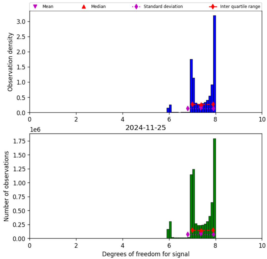
Figure 23: Histogram of “Degrees of freedom for signal” for 2024-11-25 to 2024-11-26
