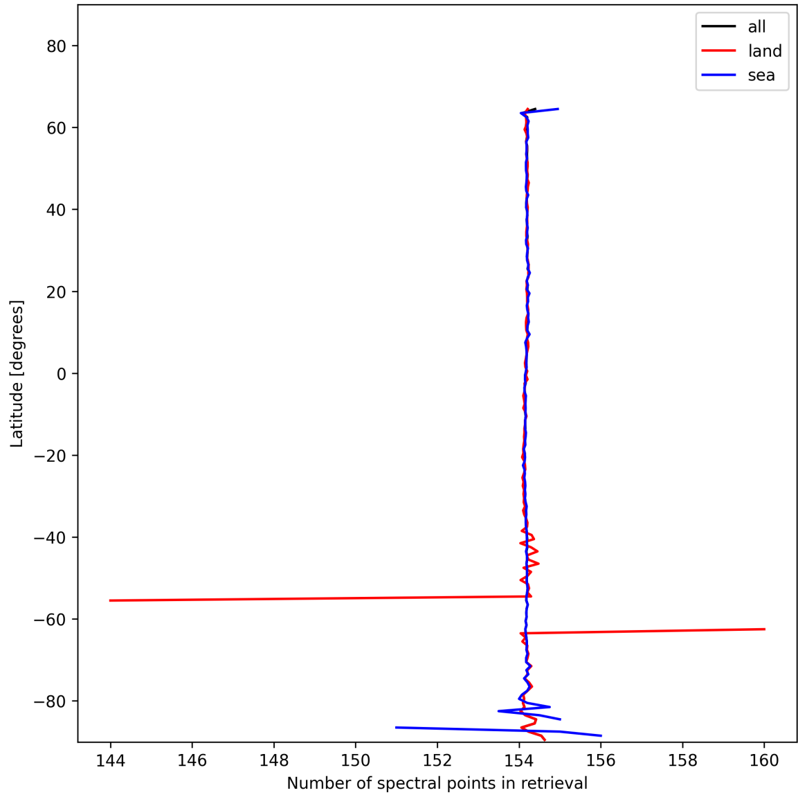
Figure 13: Zonal average of “Number of spectral points in retrieval” for 2024-11-25 to 2024-11-26.
