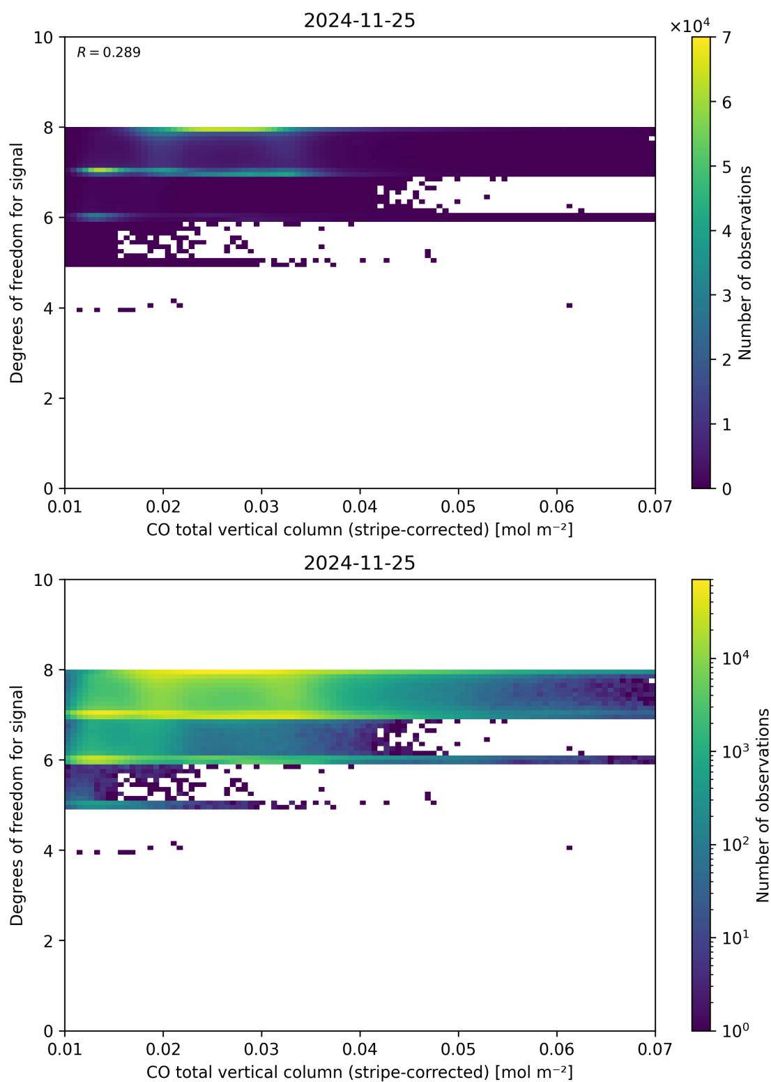
Figure 38: Scatter density plot of “CO total vertical column (stripe-corrected)” against “Degrees of freedom for signal” for 2024-11-25 to 2024-11-26.
