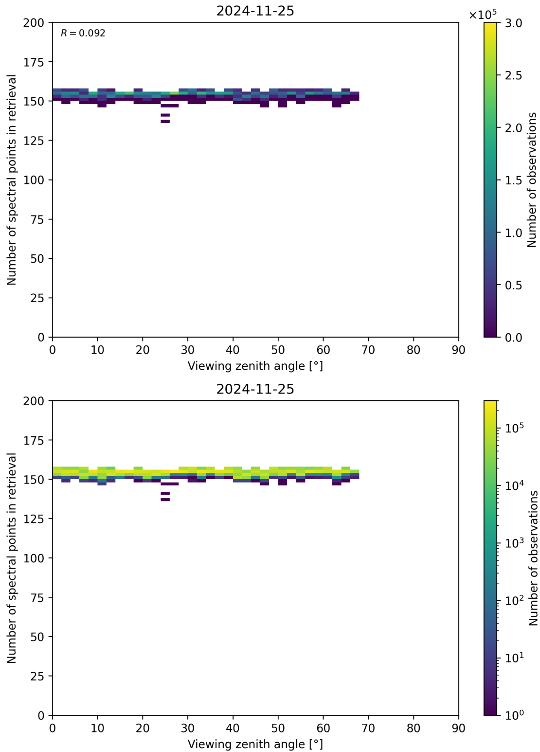
Figure 76: Scatter density plot of “Viewing zenith angle” against “Number of spectral points in retrieval” for 2024-11-25 to 2024-11-26.
