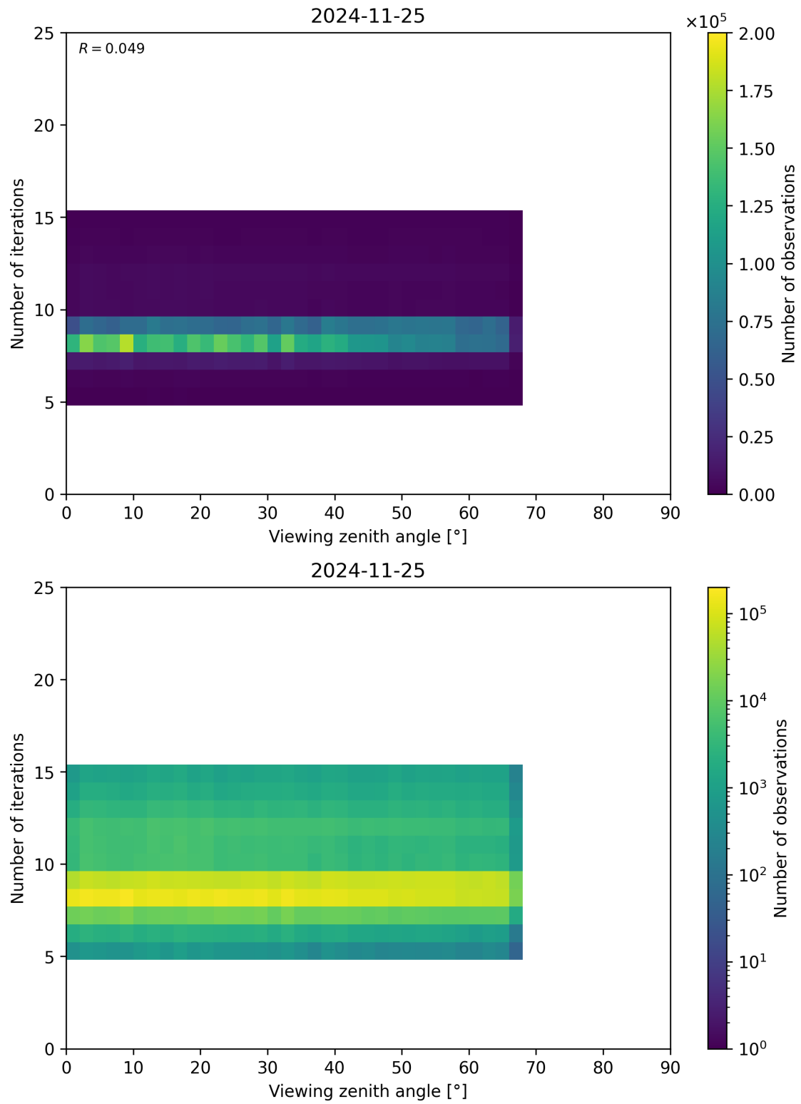
Figure 75: Scatter density plot of “Viewing zenith angle” against “Number of iterations” for 2024-11-25 to 2024-11-26.
