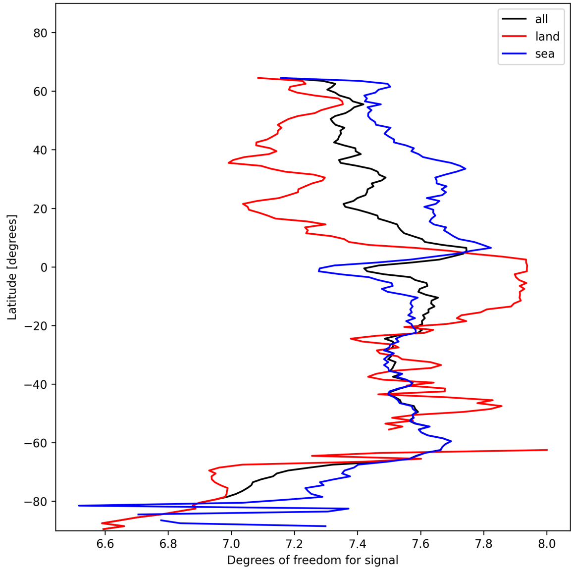
Figure 15: Zonal average of “Degrees of freedom for signal” for 2024-11-25 to 2024-11-26.
