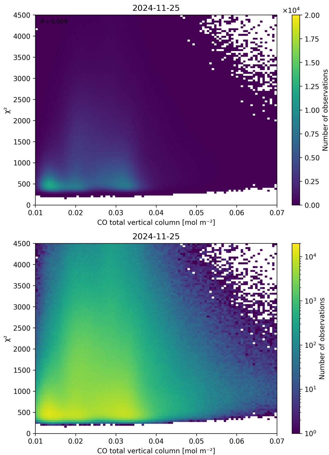
Figure 35: Scatter density plot of “CO total vertical column” against “ \chi^2 ” for 2024-11-25 to 2024-11-26.
