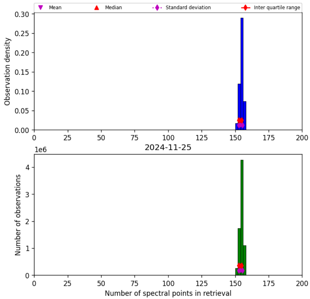
Figure 21: Histogram of “Number of spectral points in retrieval” for 2024-11-25 to 2024-11-26
