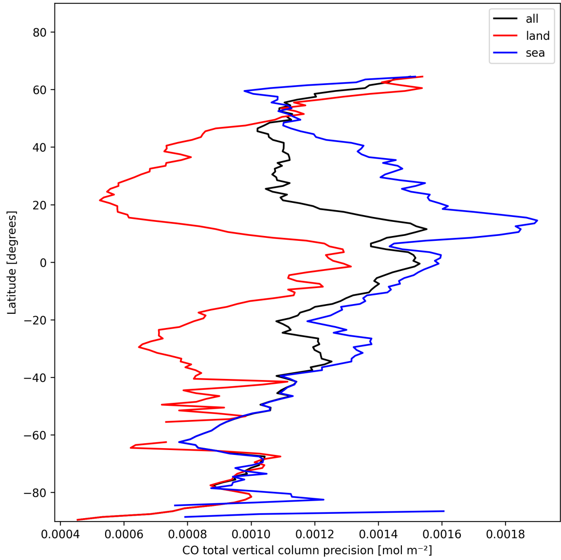
Figure 12: Zonal average of “CO total vertical column precision” for 2024-11-25 to 2024-11-26.
