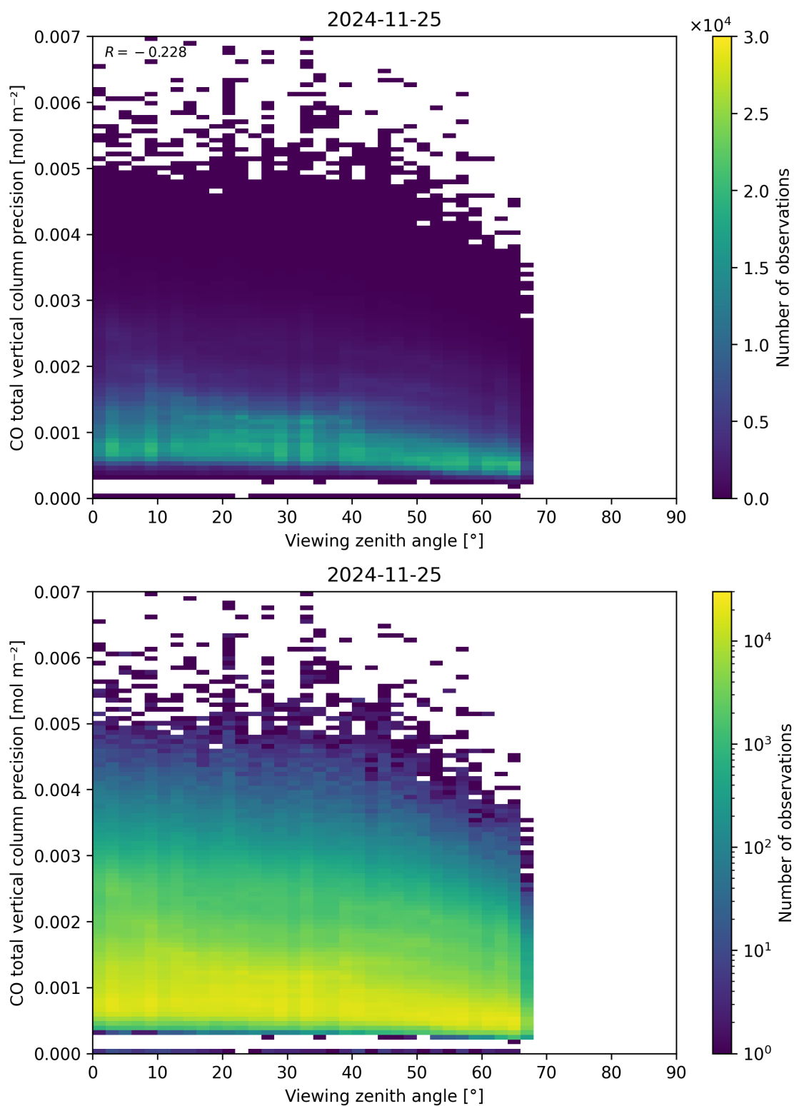
Figure 71: Scatter density plot of “Viewing zenith angle” against “CO total vertical column precision” for 2024-11-25 to 2024-11-26.
