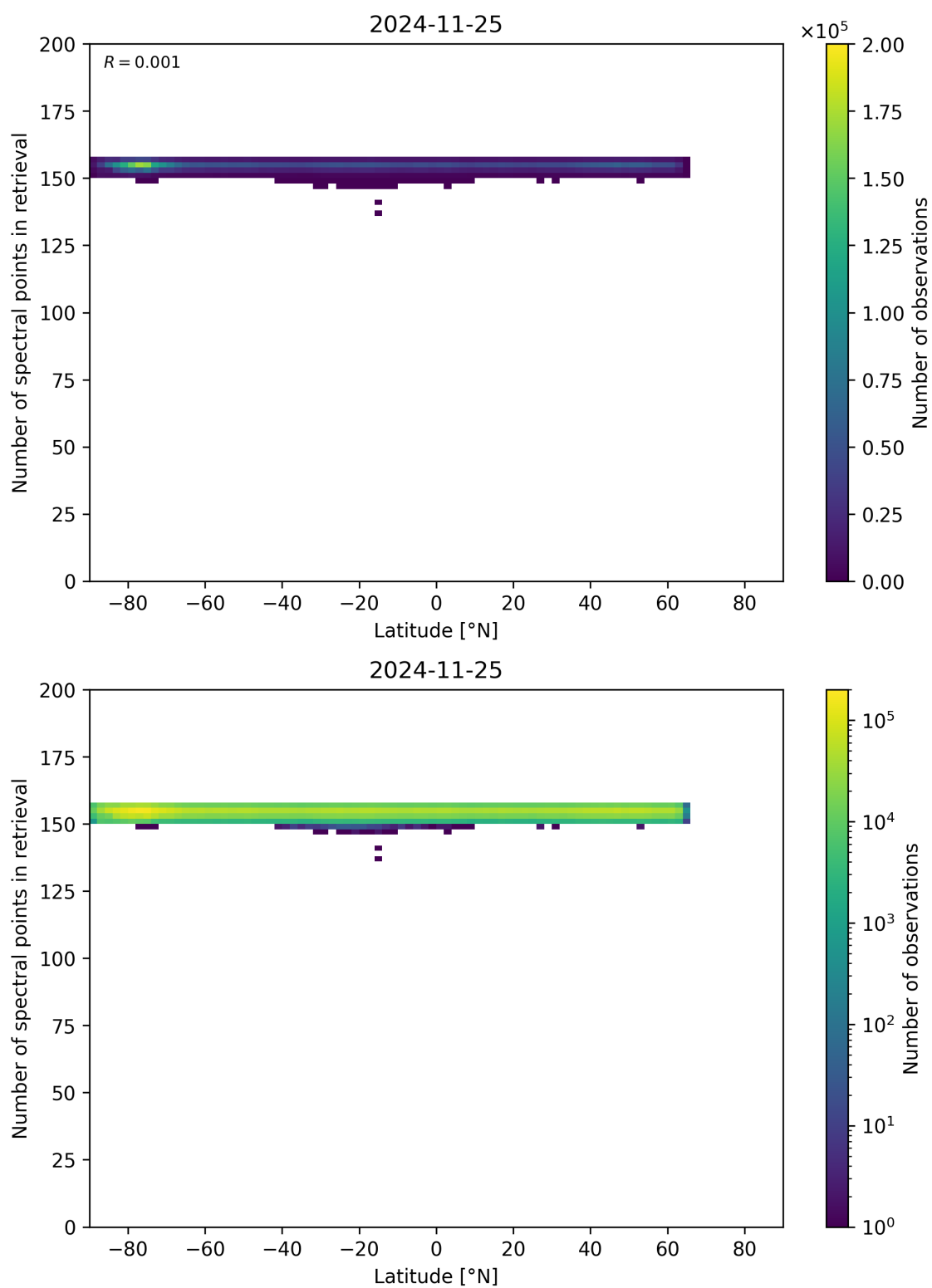
Figure 57: Scatter density plot of “Latitude” against “Number of spectral points in retrieval” for 2024-11-25 to 2024-11-26.
