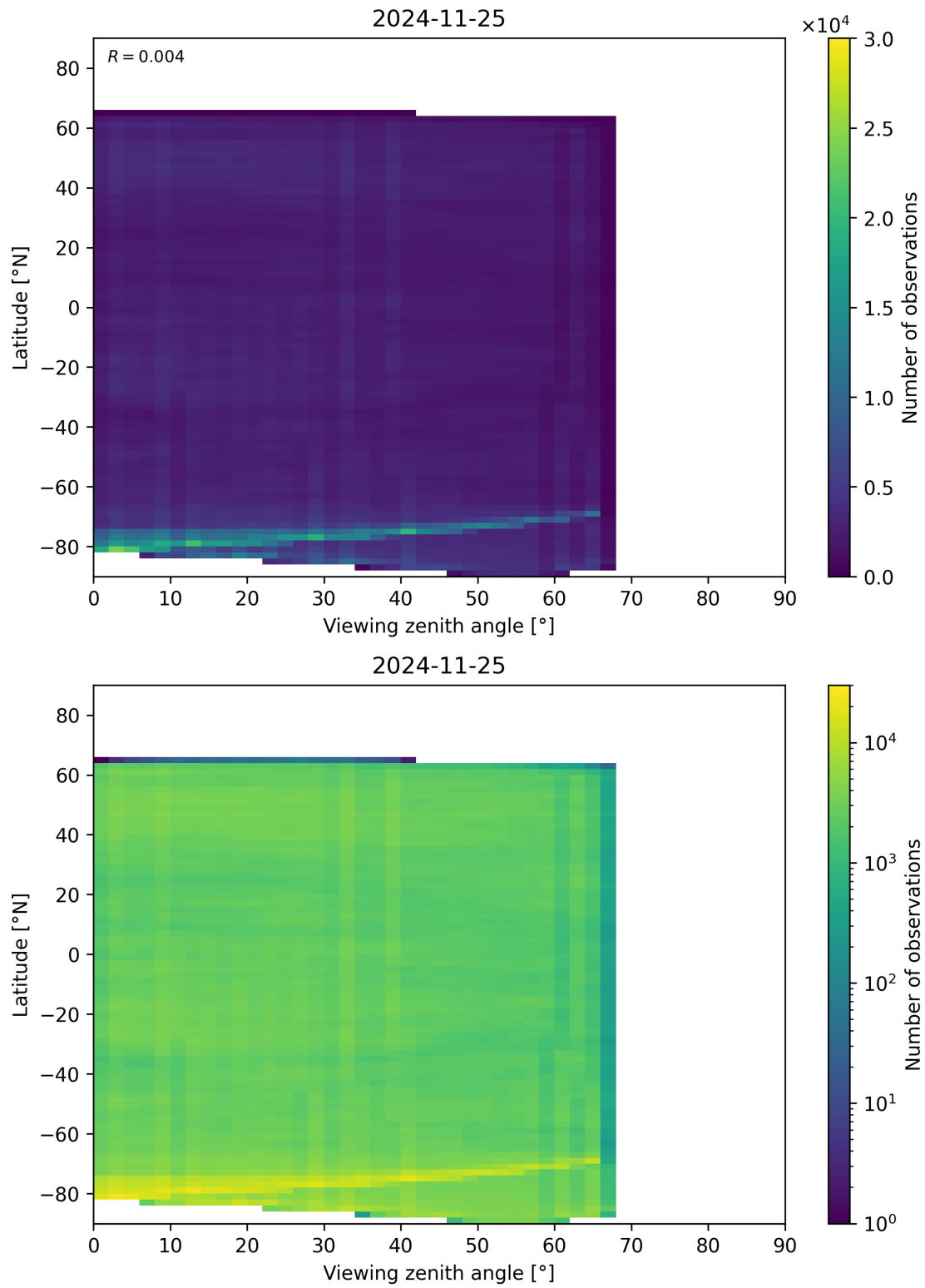
Figure 74: Scatter density plot of “Viewing zenith angle” against “Latitude” for 2024-11-25 to 2024-11-26.
