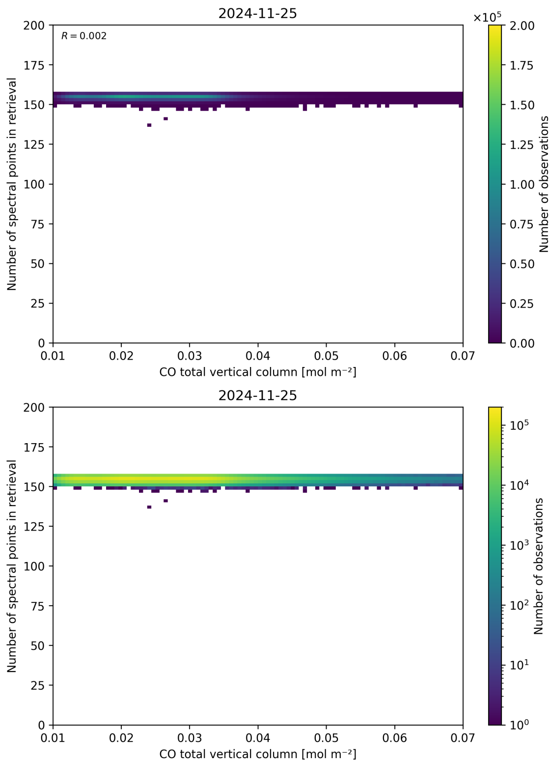
Figure 43: Scatter density plot of “CO total vertical column” against “Number of spectral points in retrieval” for 2024-11-25 to 2024-11-26.
