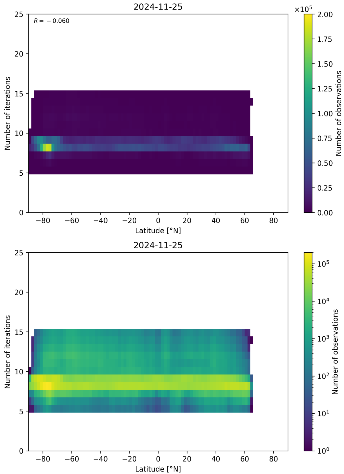
Figure 56: Scatter density plot of “Latitude” against “Number of iterations” for 2024-11-25 to 2024-11-26.
