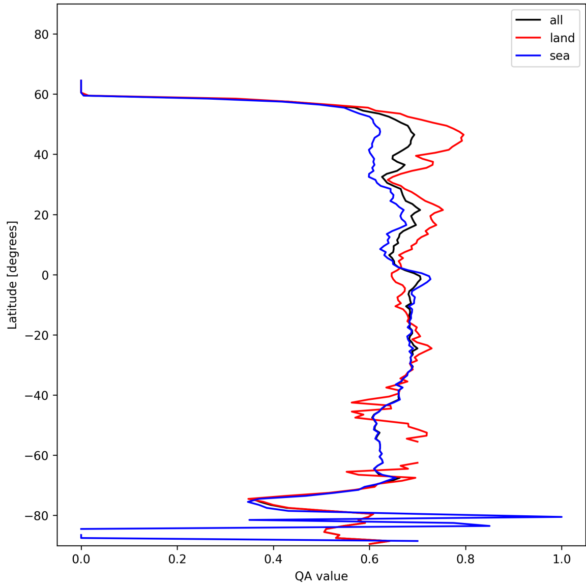
Figure 9: Zonal average of “QA value” for 2024-11-25 to 2024-11-26.
