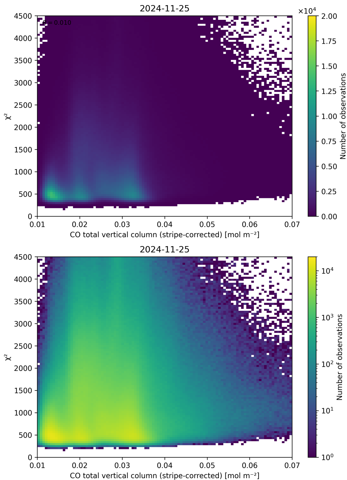
Figure 37: Scatter density plot of “CO total vertical column (stripe-corrected)” against “ \chi^2 ” for 2024-11-25 to 2024-11-26.
