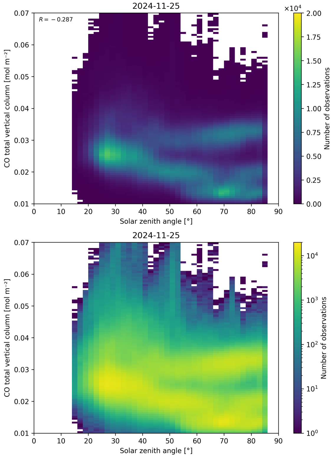
Figure 61: Scatter density plot of “Solar zenith angle” against “CO total vertical column” for 2024-11-25 to 2024-11-26.
