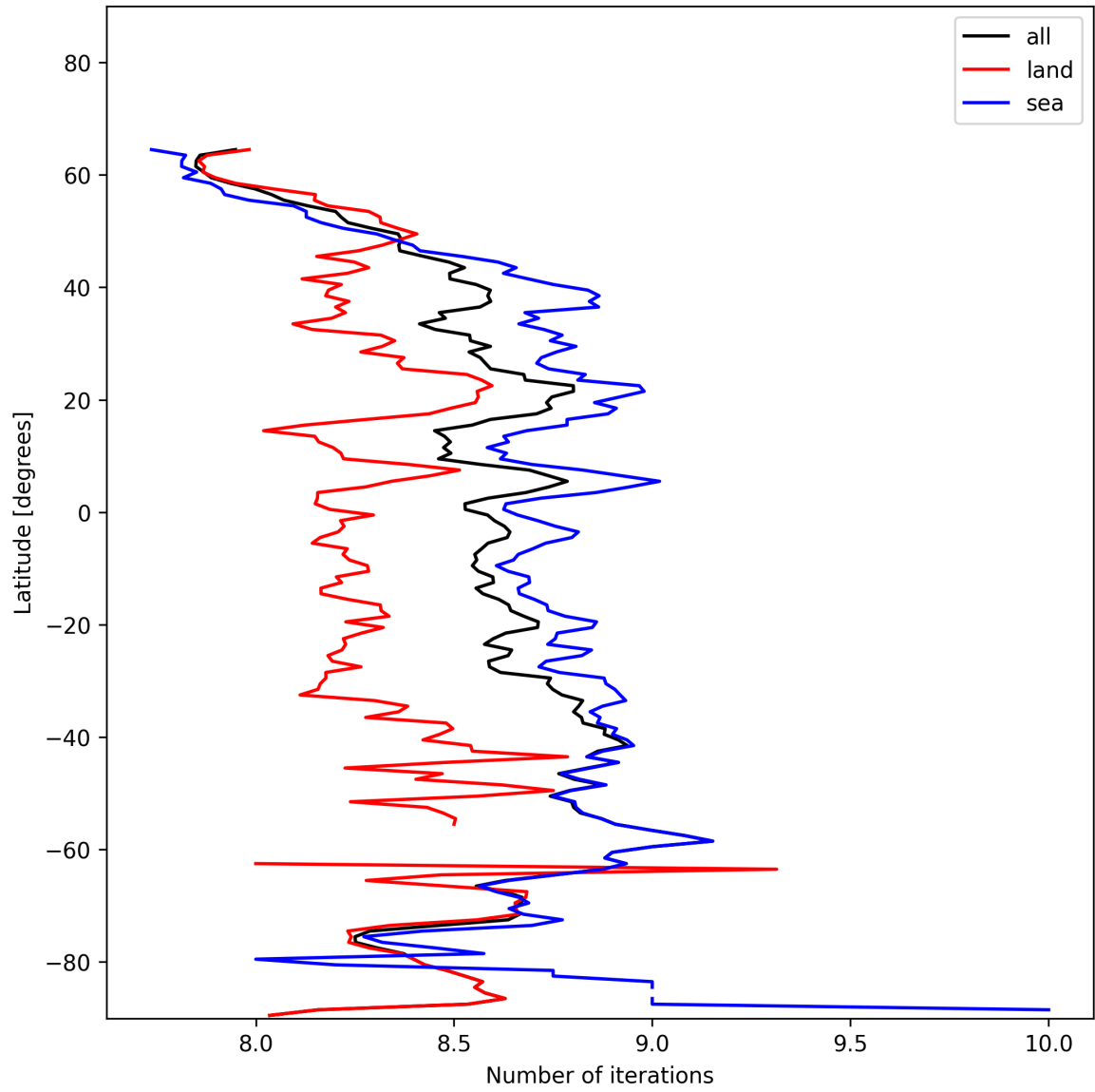
Figure 16: Zonal average of “Number of iterations” for 2024-11-25 to 2024-11-26.
