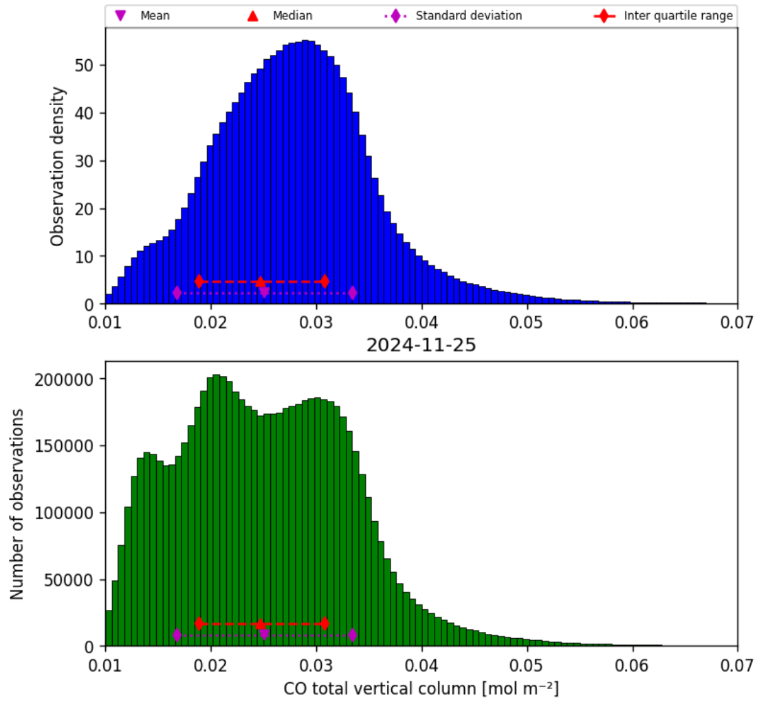
Figure 18: Histogram of “CO total vertical column” for 2024-11-25 to 2024-11-26
