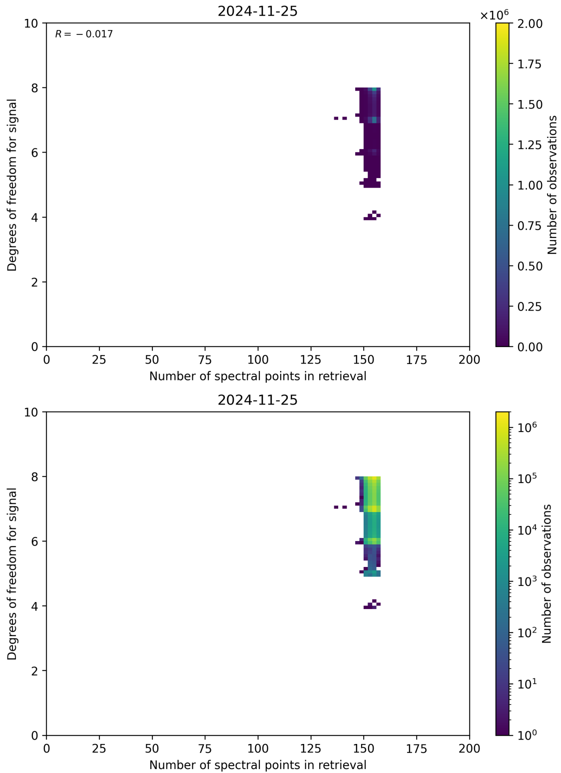
Figure 59: Scatter density plot of “Number of spectral points in retrieval” against “Degrees of freedom for signal” for 2024-11-25 to 2024-11-26.
