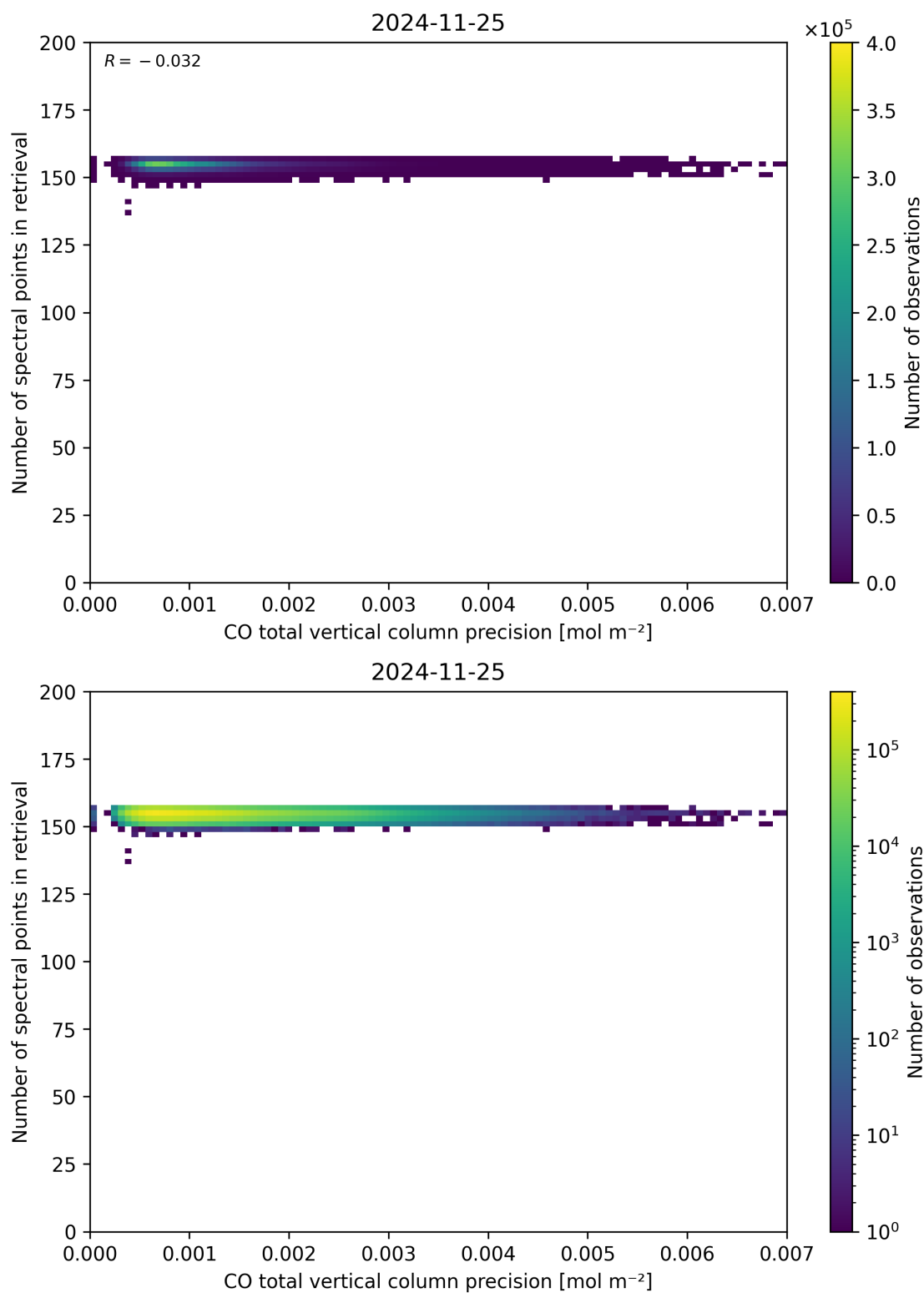
Figure 47: Scatter density plot of “CO total vertical column precision” against “Number of spectral points in retrieval” for 2024-11-25 to 2024-11-26.
