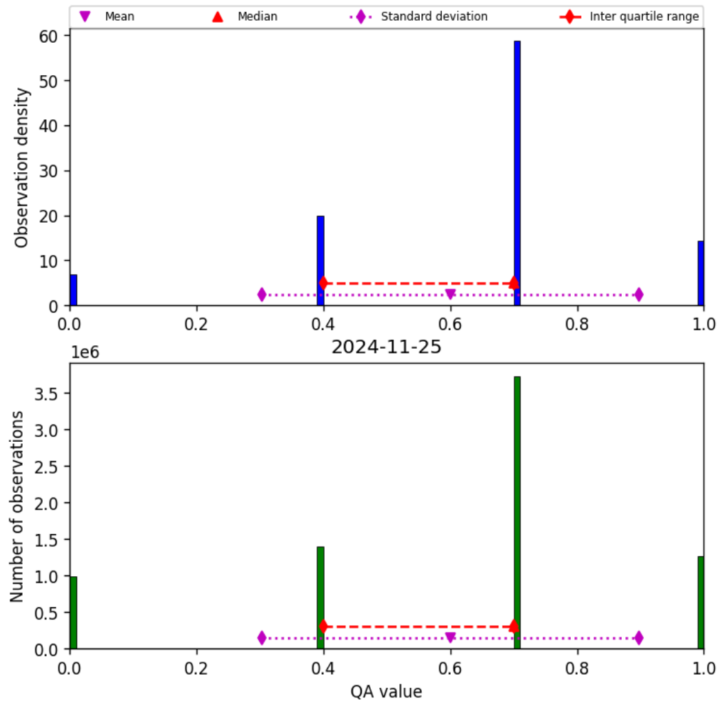
Figure 17: Histogram of “QA value” for 2024-11-25 to 2024-11-26
