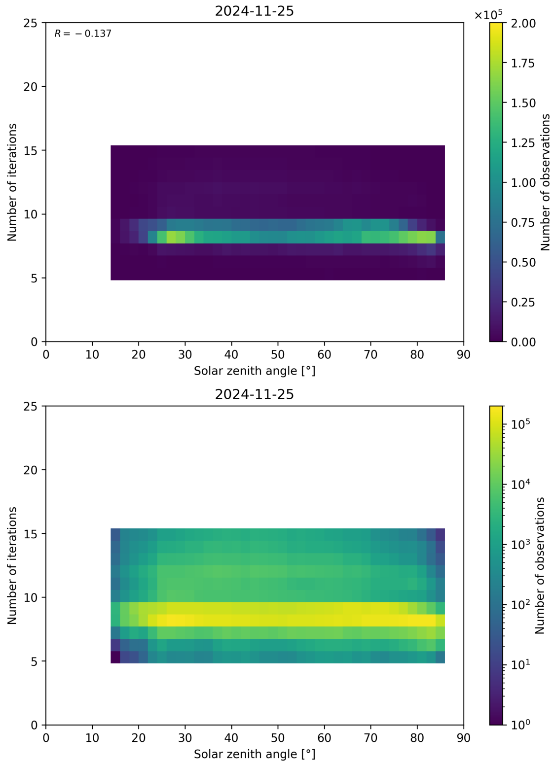
Figure 67: Scatter density plot of “Solar zenith angle” against “Number of iterations” for 2024-11-25 to 2024-11-26.
