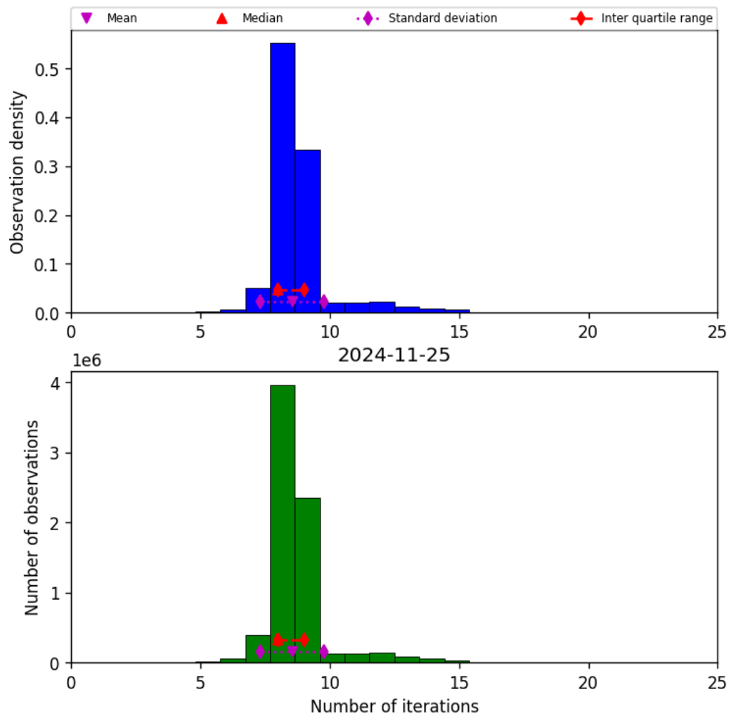
Figure 24: Histogram of “Number of iterations” for 2024-11-25 to 2024-11-26
