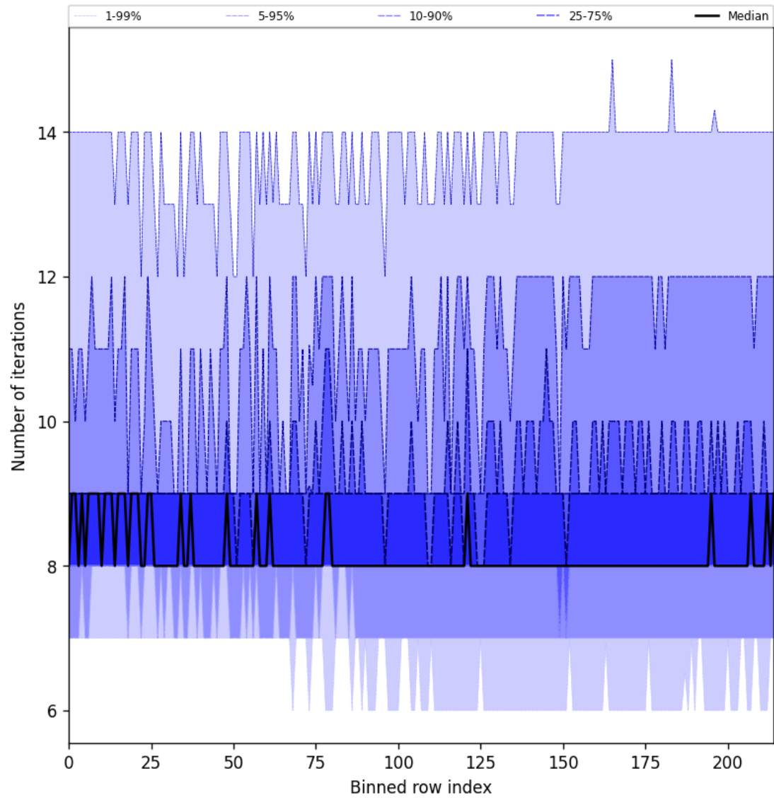
Figure 32: Along track statistics of “Number of iterations” for 2024-11-25 to 2024-11-26
