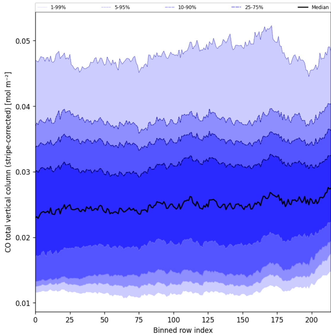
Figure 27: Along track statistics of “CO total vertical column (stripe-corrected)” for 2024-11-25 to 2024-11-26
