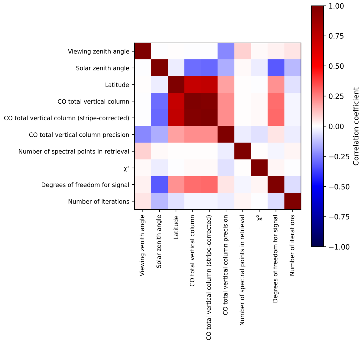
Figure 2: Map of correlation matrix for 2024-11-25 to 2024-11-26.
