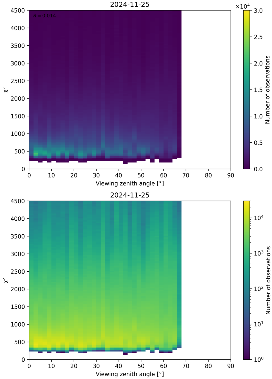
Figure 72: Scatter density plot of “Viewing zenith angle” against “ \chi^2 ” for 2024-11-25 to 2024-11-26.
