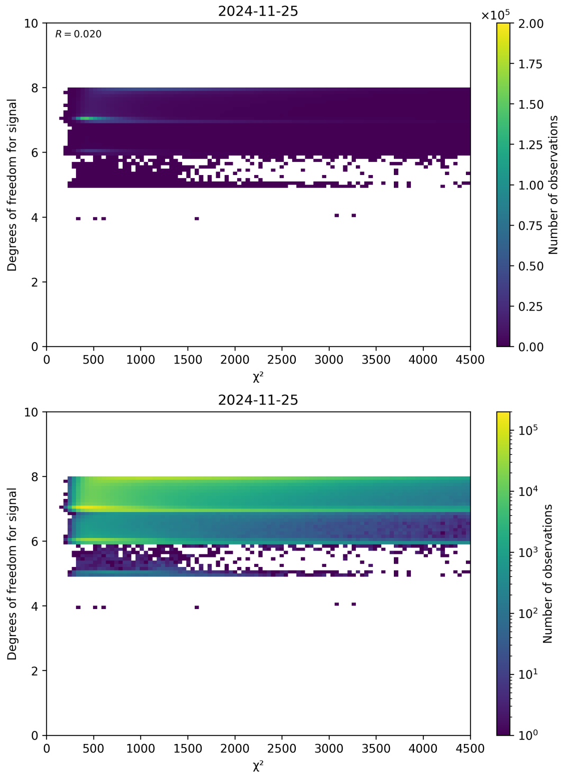
Figure 48: Scatter density plot of “ \chi^2 ” against “Degrees of freedom for signal” for 2024-11-25 to 2024-11-26.
