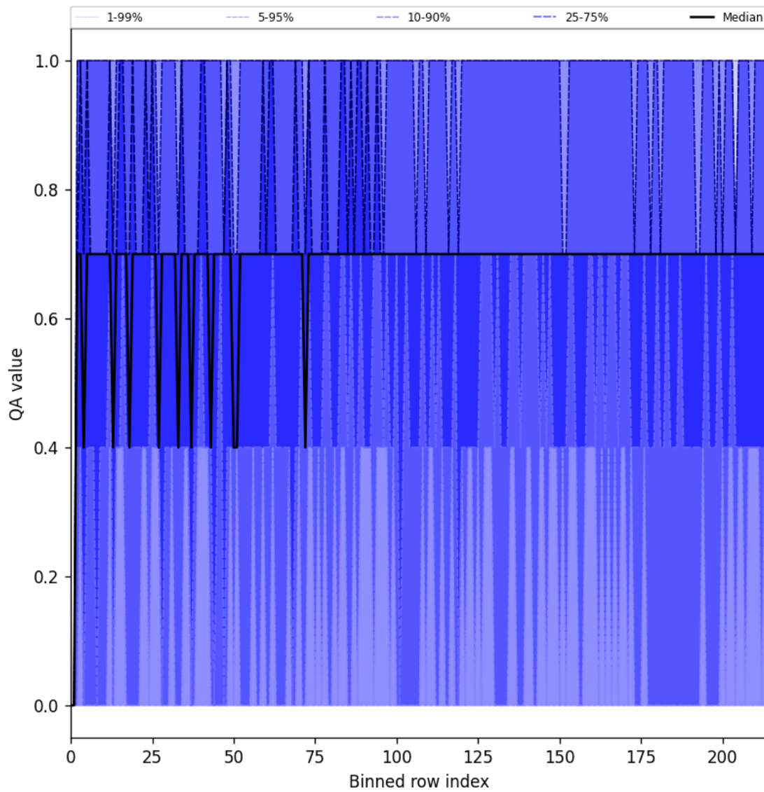
Figure 25: Along track statistics of “QA value” for 2024-11-25 to 2024-11-26
