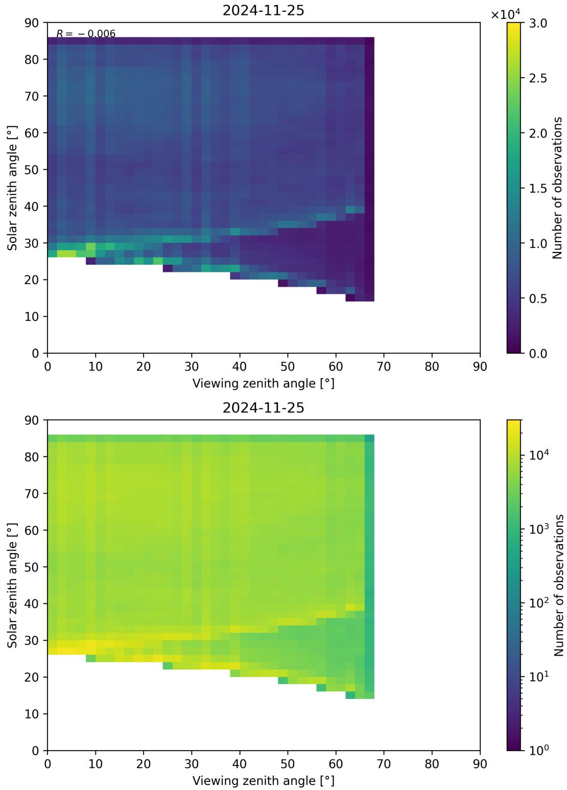
Figure 77: Scatter density plot of “Viewing zenith angle” against “Solar zenith angle” for 2024-11-25 to 2024-11-26.
