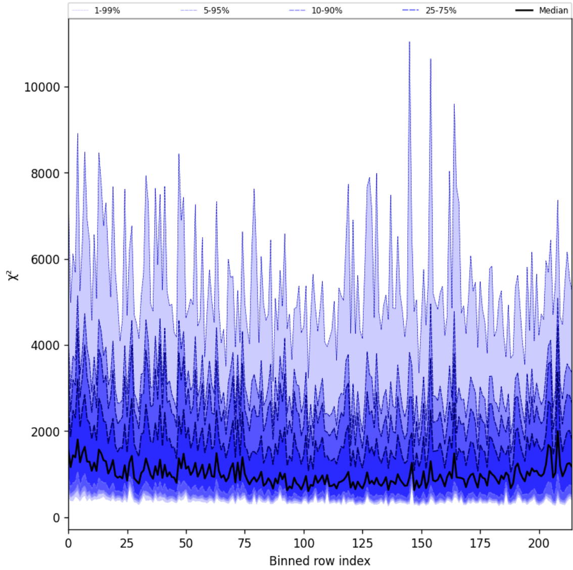
Figure 30: Along track statistics of “ \chi^2 ” for 2024-11-25 to 2024-11-26
