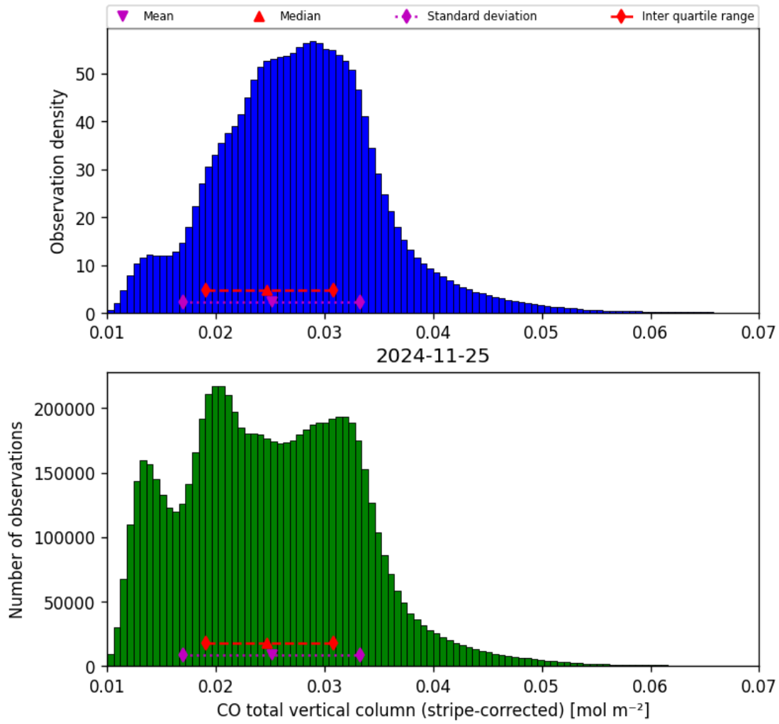
Figure 19: Histogram of “CO total vertical column (stripe-corrected)” for 2024-11-25 to 2024-11-26
