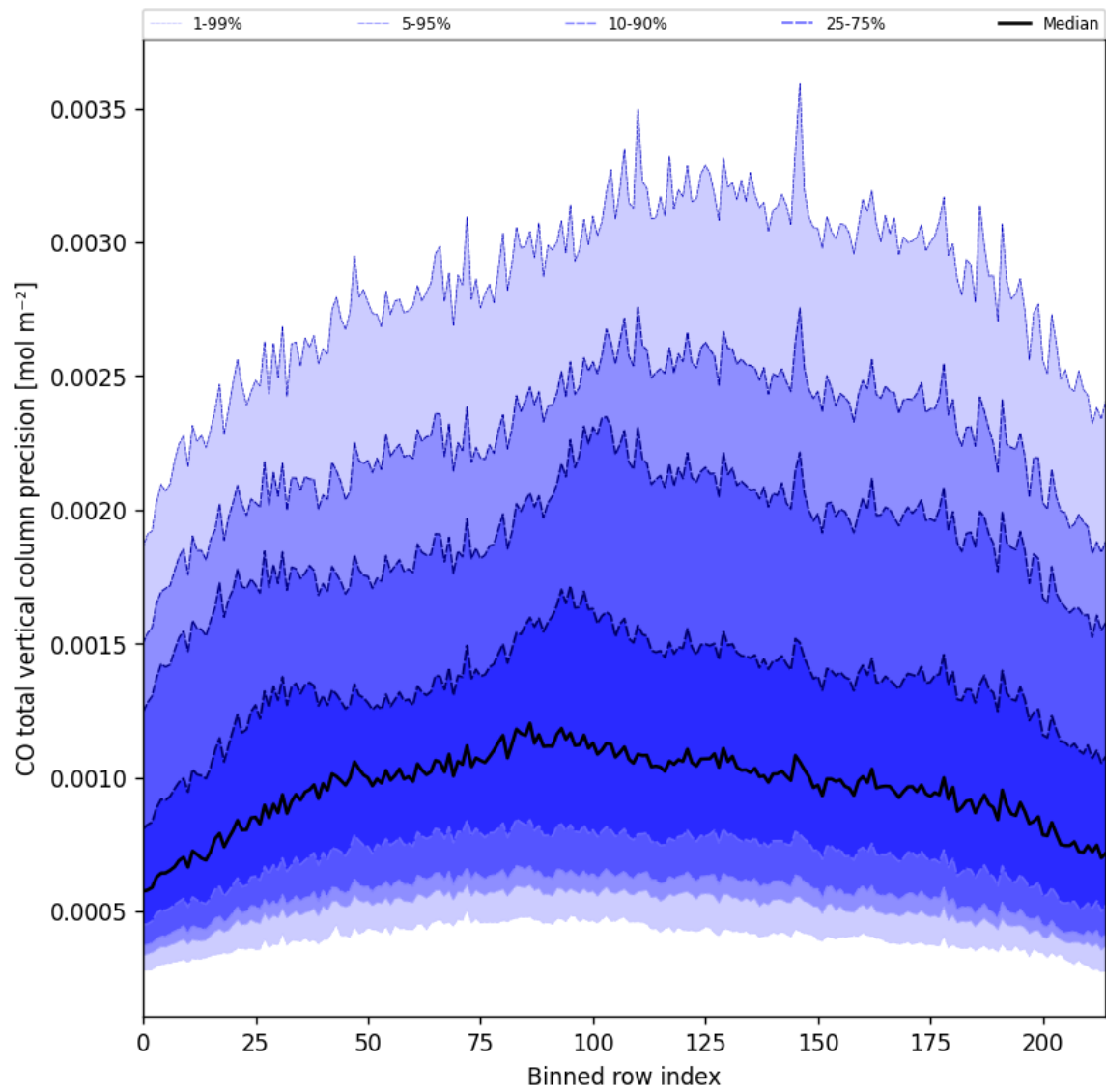
Figure 28: Along track statistics of “CO total vertical column precision” for 2024-11-25 to 2024-11-26
