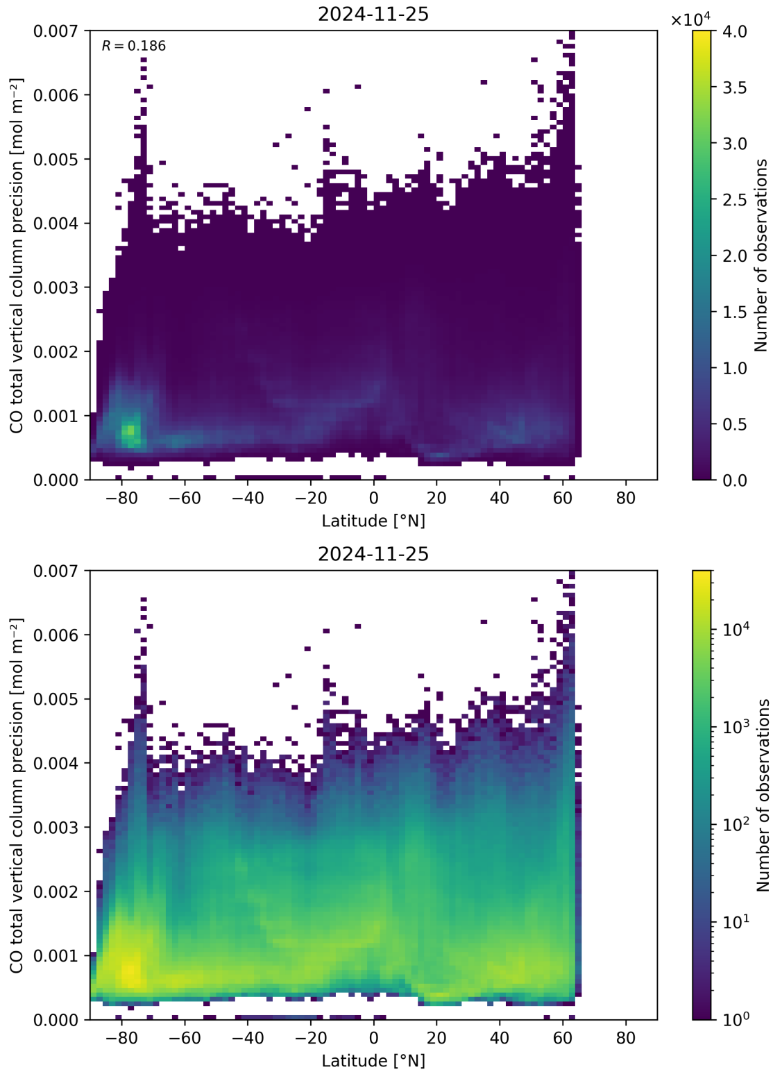
Figure 53: Scatter density plot of “Latitude” against “CO total vertical column precision” for 2024-11-25 to 2024-11-26.
