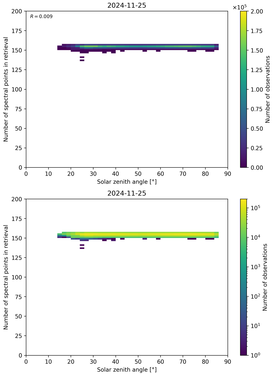
Figure 68: Scatter density plot of “Solar zenith angle” against “Number of spectral points in retrieval” for 2024-11-25 to 2024-11-26.
