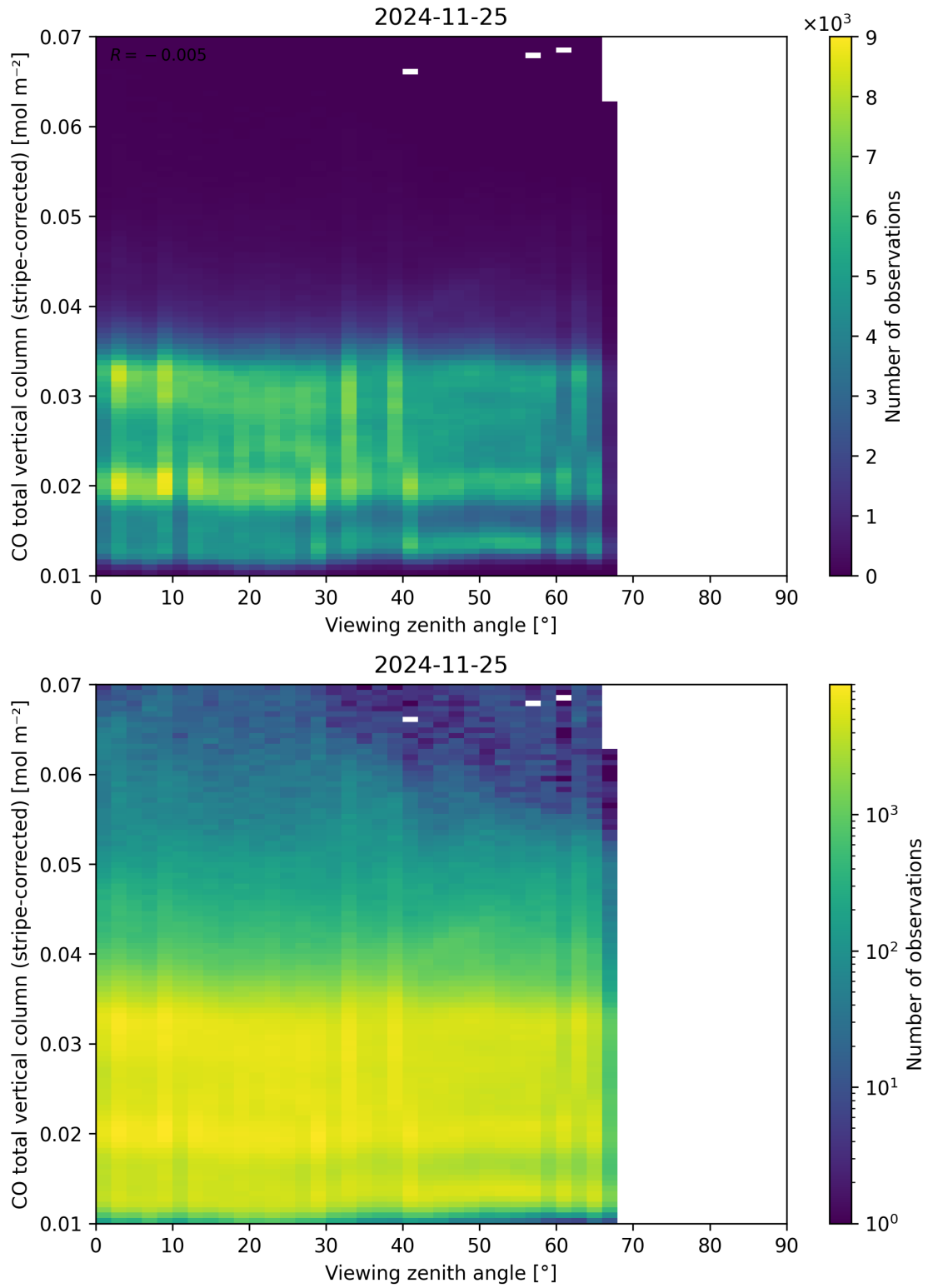
Figure 70: Scatter density plot of “Viewing zenith angle” against “CO total vertical column (stripe-corrected)” for 2024-11-25 to 2024-11-26.
