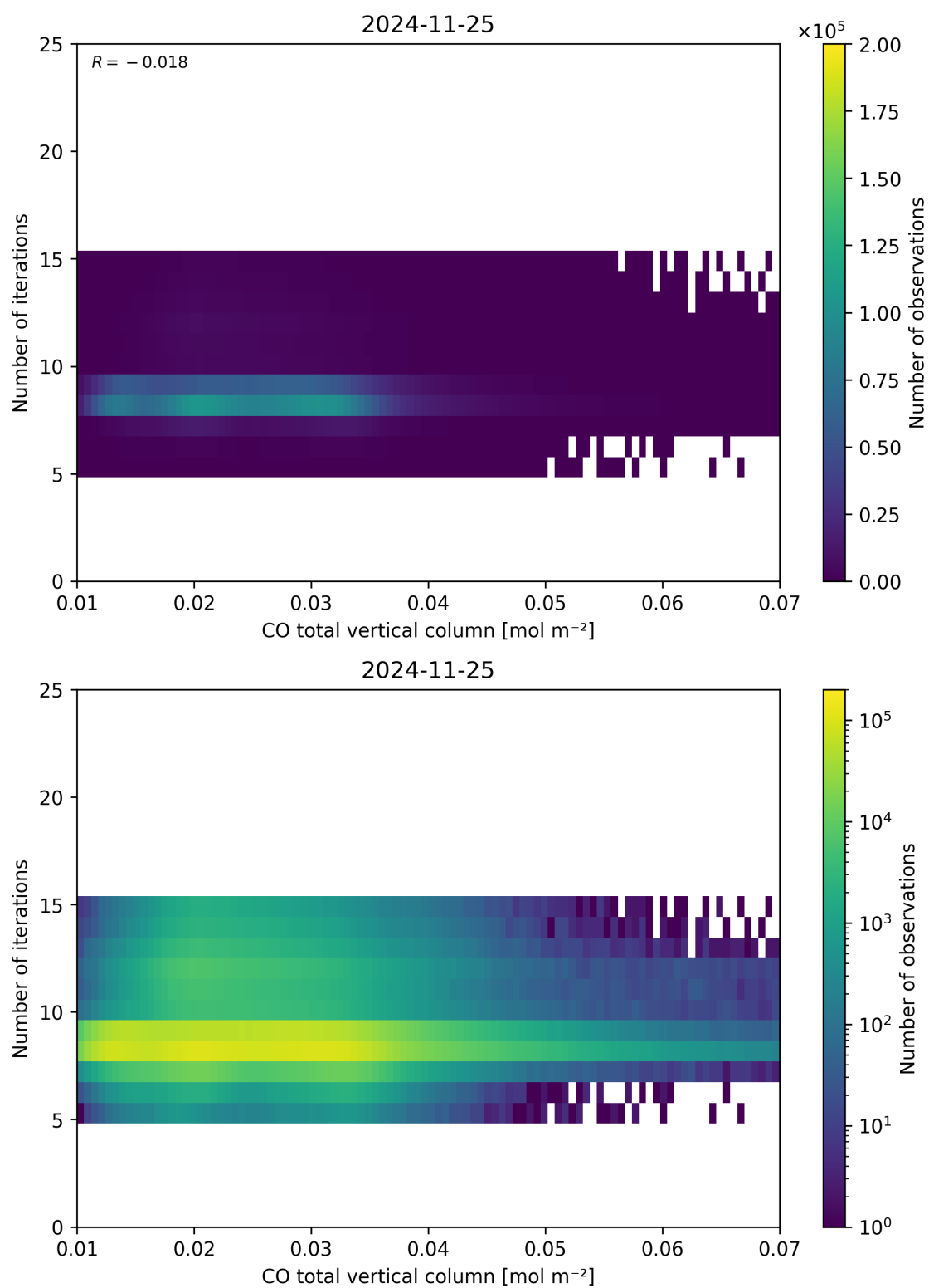
Figure 42: Scatter density plot of “CO total vertical column” against “Number of iterations” for 2024-11-25 to 2024-11-26.
