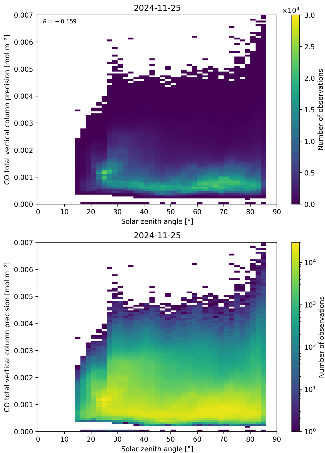
Figure 63: Scatter density plot of “Solar zenith angle” against “CO total vertical column precision” for 2024-11-25 to 2024-11-26.
