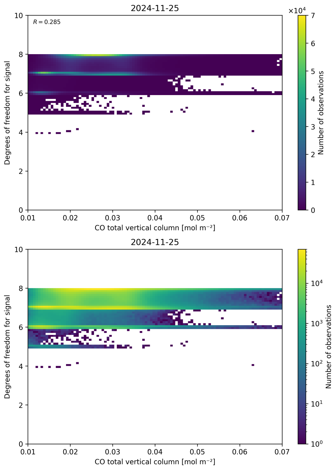
Figure 41: Scatter density plot of “CO total vertical column” against “Degrees of freedom for signal” for 2024-11-25 to 2024-11-26.
