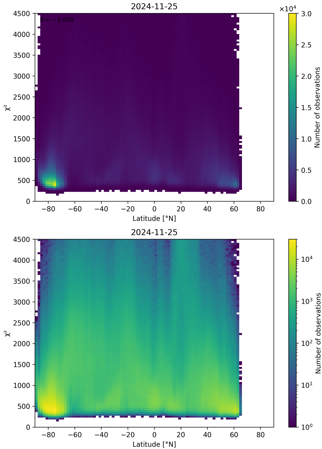
Figure 54: Scatter density plot of “Latitude” against “ \chi^2 ” for 2024-11-25 to 2024-11-26.
