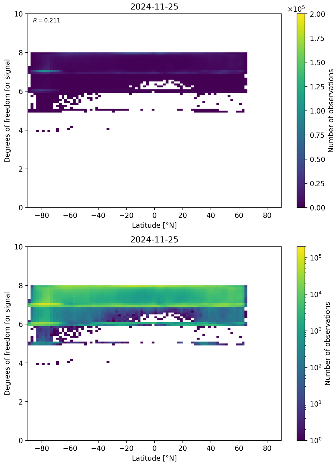
Figure 55: Scatter density plot of “Latitude” against “Degrees of freedom for signal” for 2024-11-25 to 2024-11-26.
