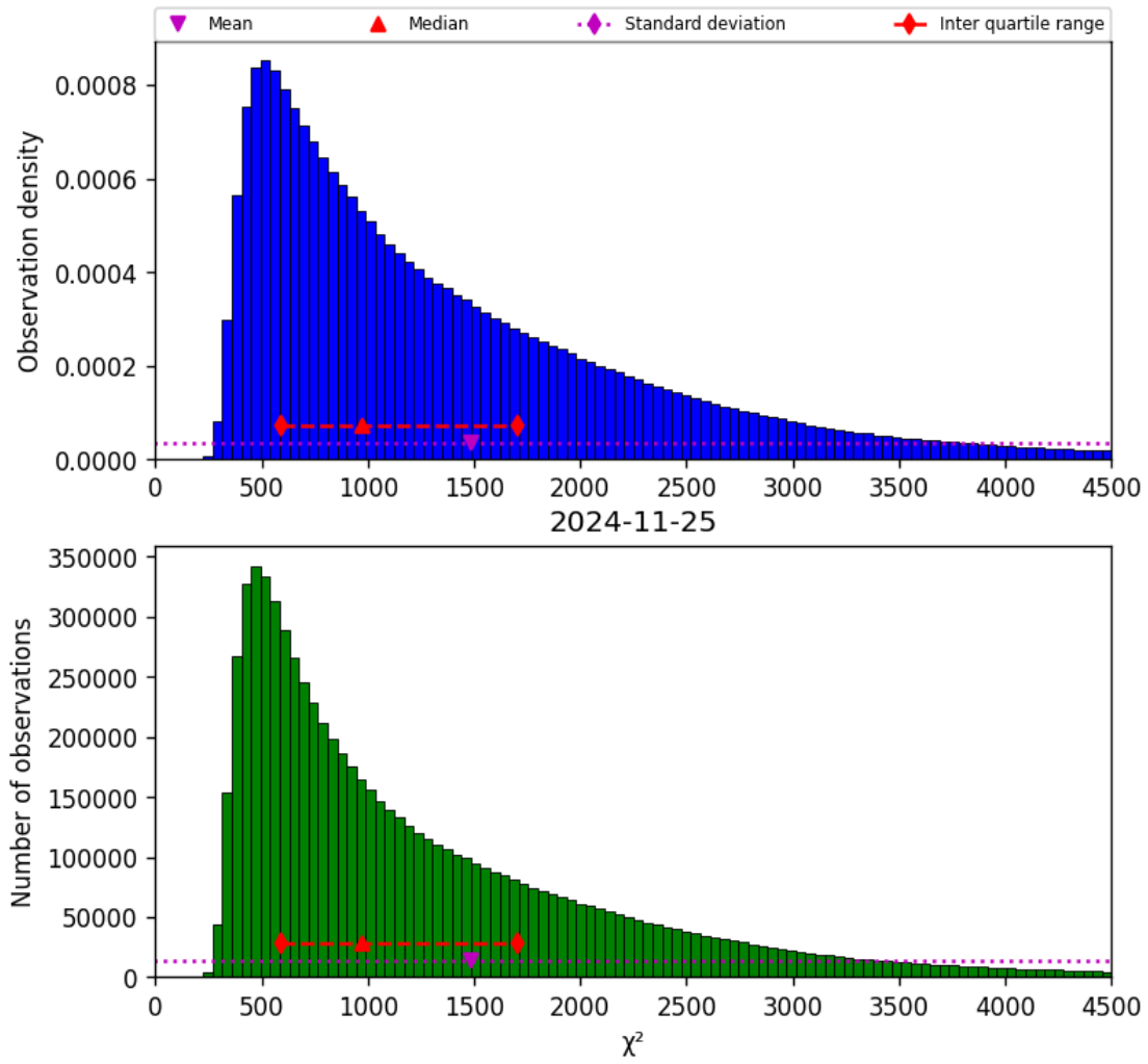
Figure 22: Histogram of “ \chi^2 ” for 2024-11-25 to 2024-11-26
