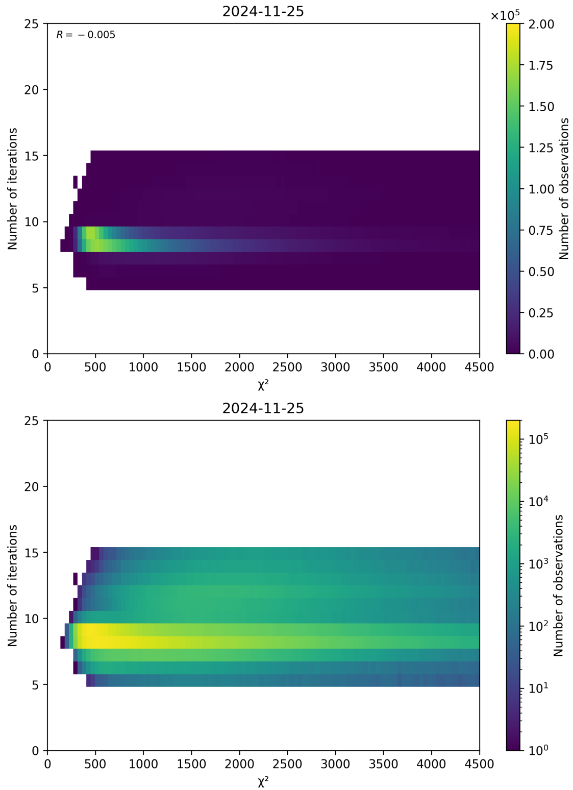
Figure 49: Scatter density plot of “ \chi^2 ” against “Number of iterations” for 2024-11-25 to 2024-11-26.
