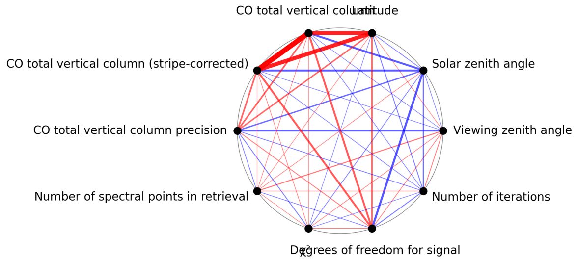
Figure 1: Map of correlation graph for 2024-11-25 to 2024-11-26.
