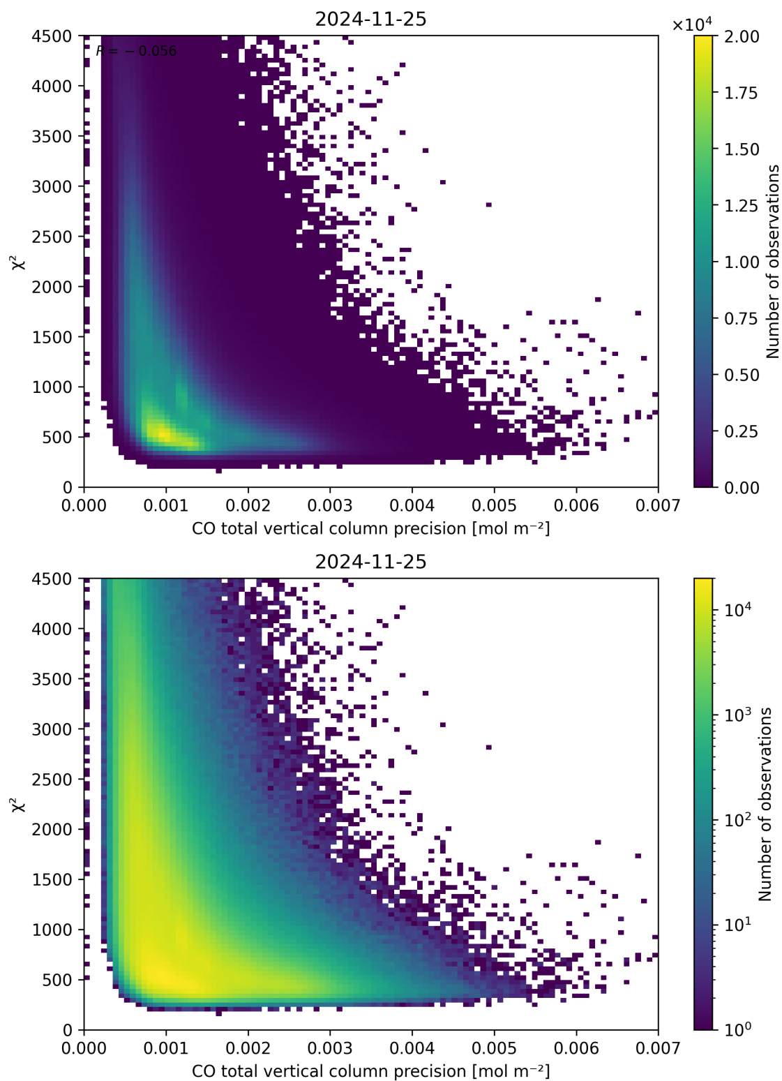
Figure 44: Scatter density plot of “CO total vertical column precision” against “ \chi^2 ” for 2024-11-25 to 2024-11-26.
