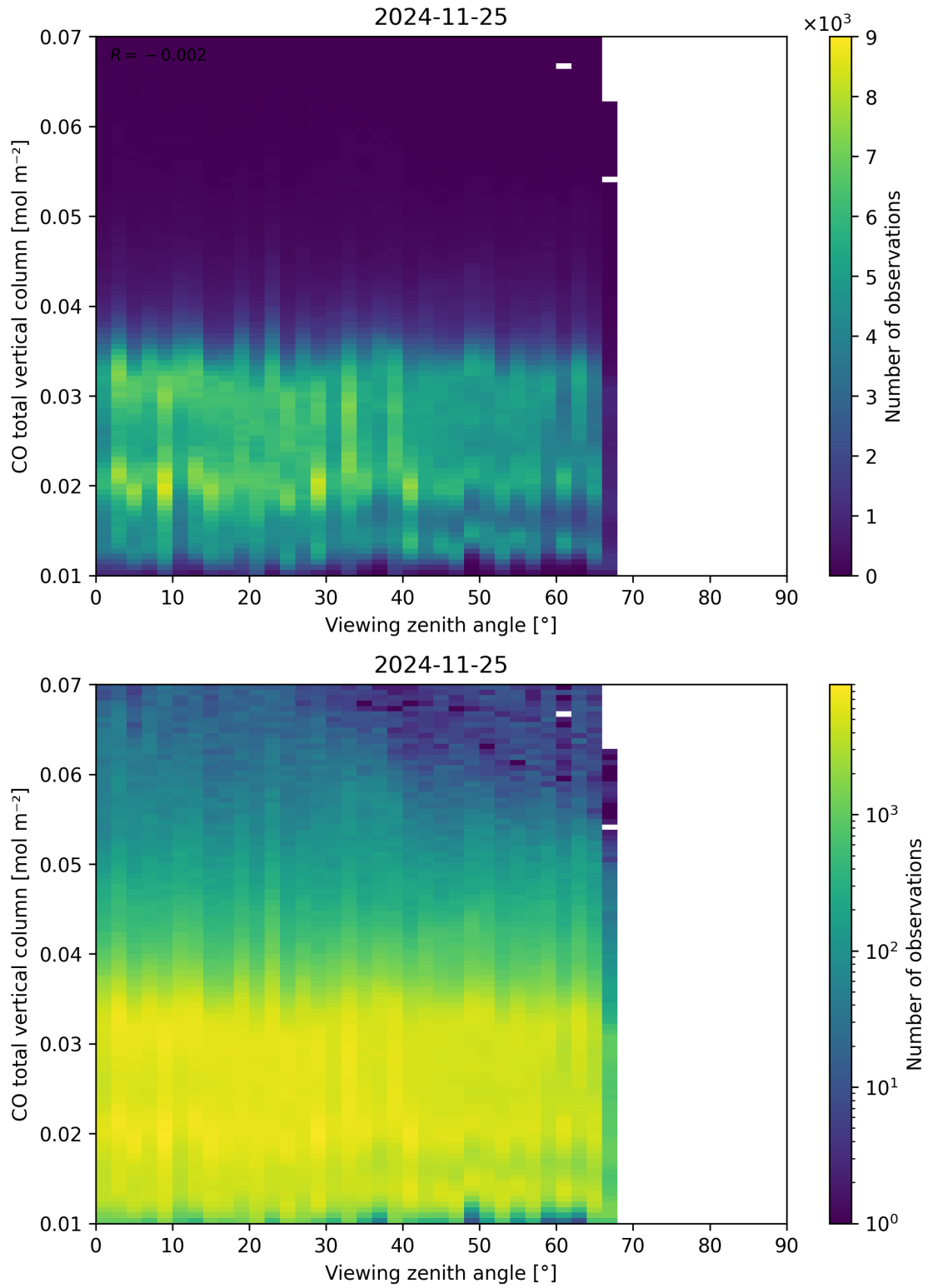
Figure 69: Scatter density plot of “Viewing zenith angle” against “CO total vertical column” for 2024-11-25 to 2024-11-26.
