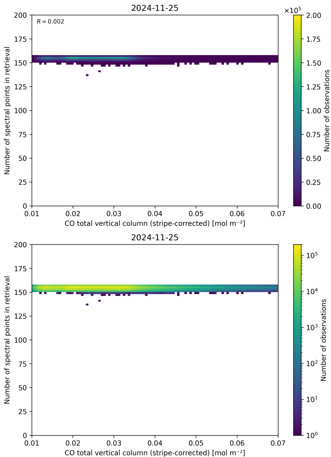
Figure 40: Scatter density plot of “CO total vertical column (stripe-corrected)” against “Number of spectral points in retrieval” for 2024-11-25 to 2024-11-26.
