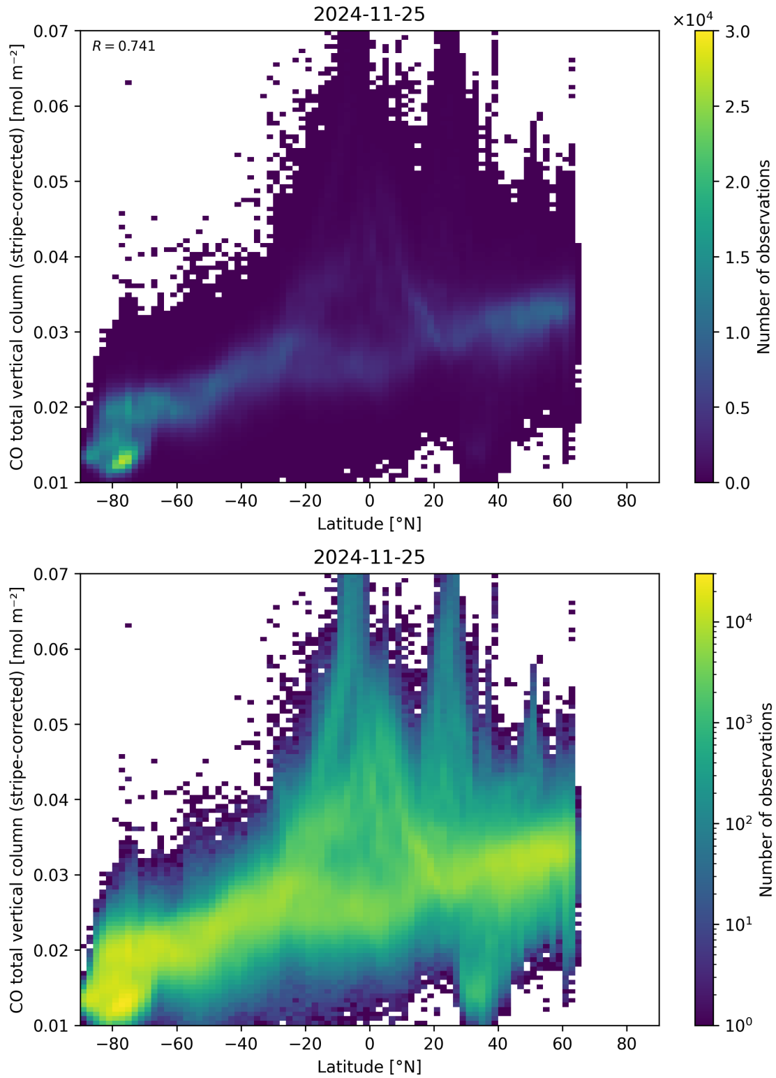
Figure 52: Scatter density plot of “Latitude” against “CO total vertical column (stripe-corrected)” for 2024-11-25 to 2024-11-26.
