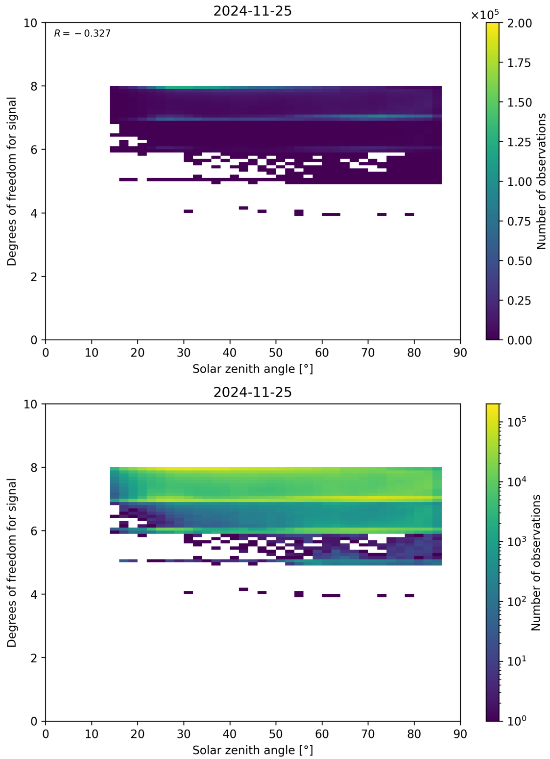
Figure 65: Scatter density plot of “Solar zenith angle” against “Degrees of freedom for signal” for 2024-11-25 to 2024-11-26.
