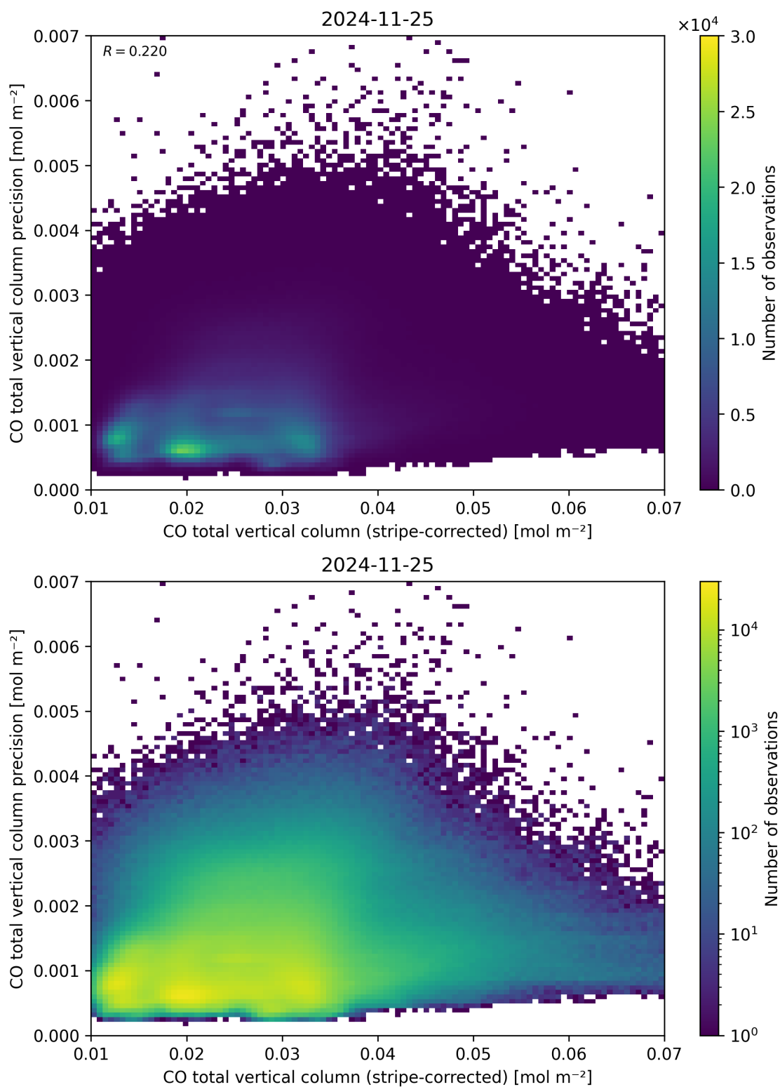
Figure 36: Scatter density plot of “CO total vertical column (stripe-corrected)” against “CO total vertical column precision” for 2024-11-25 to 2024-11-26.
