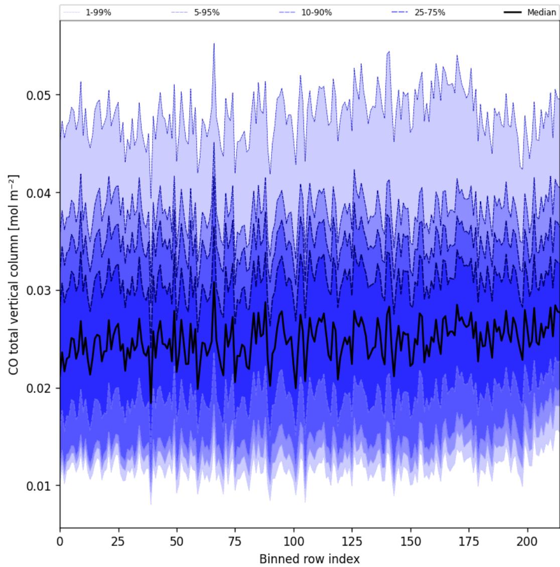
Figure 26: Along track statistics of “CO total vertical column” for 2024-11-25 to 2024-11-26
