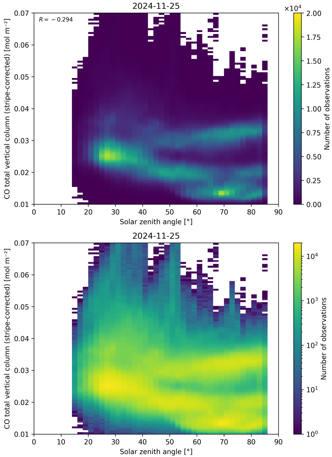
Figure 62: Scatter density plot of “Solar zenith angle” against “CO total vertical column (stripe-corrected)” for 2024-11-25 to 2024-11-26.
