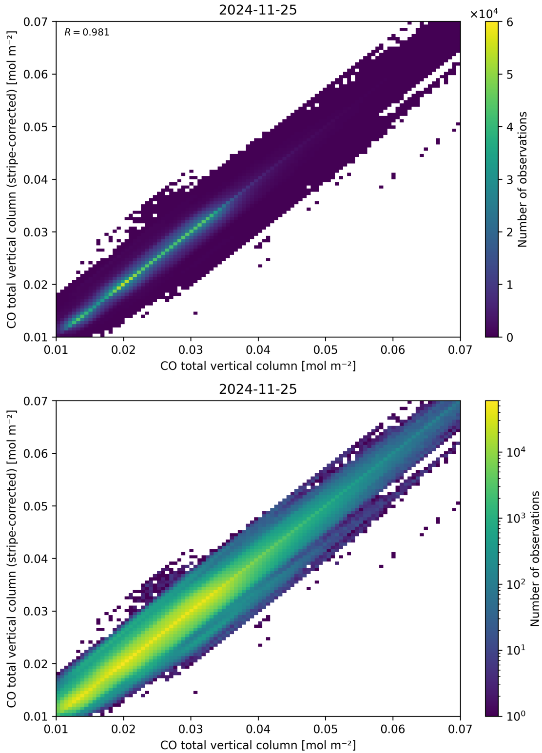
Figure 33: Scatter density plot of “CO total vertical column” against “CO total vertical column (stripe-corrected)” for 2024-11-25 to 2024-11-26.
