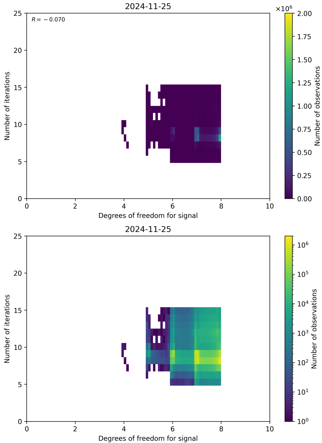
Figure 50: Scatter density plot of “Degrees of freedom for signal” against “Number of iterations” for 2024-11-25 to 2024-11-26.
