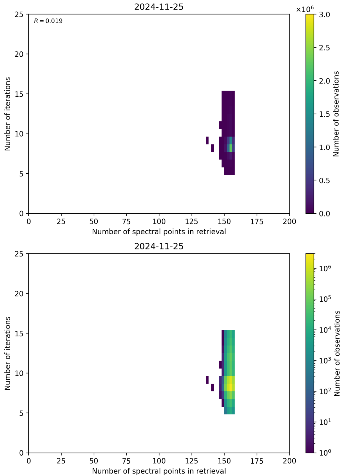
Figure 60: Scatter density plot of “Number of spectral points in retrieval” against “Number of iterations” for 2024-11-25 to 2024-11-26.
