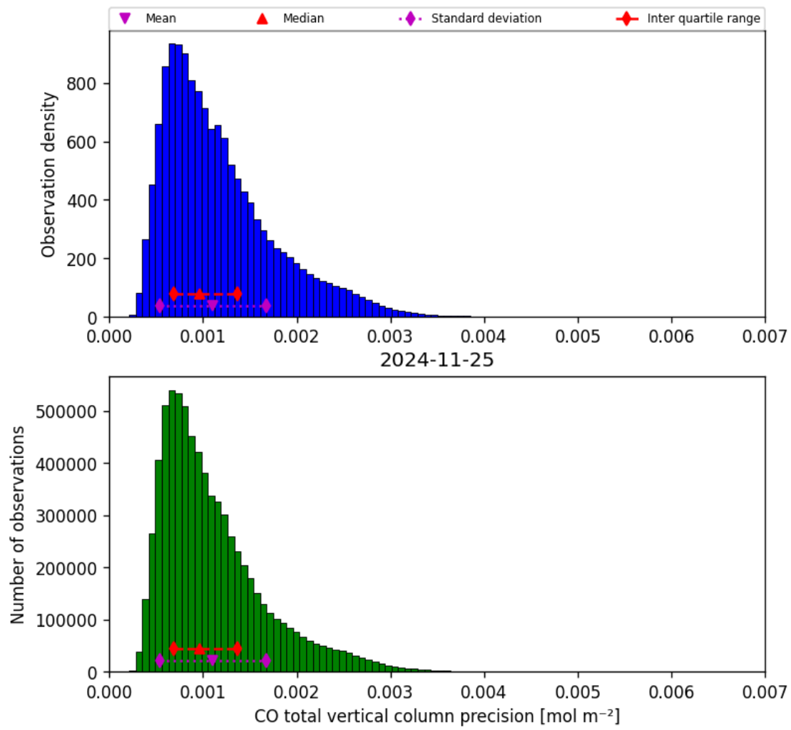
Figure 20: Histogram of “CO total vertical column precision” for 2024-11-25 to 2024-11-26
