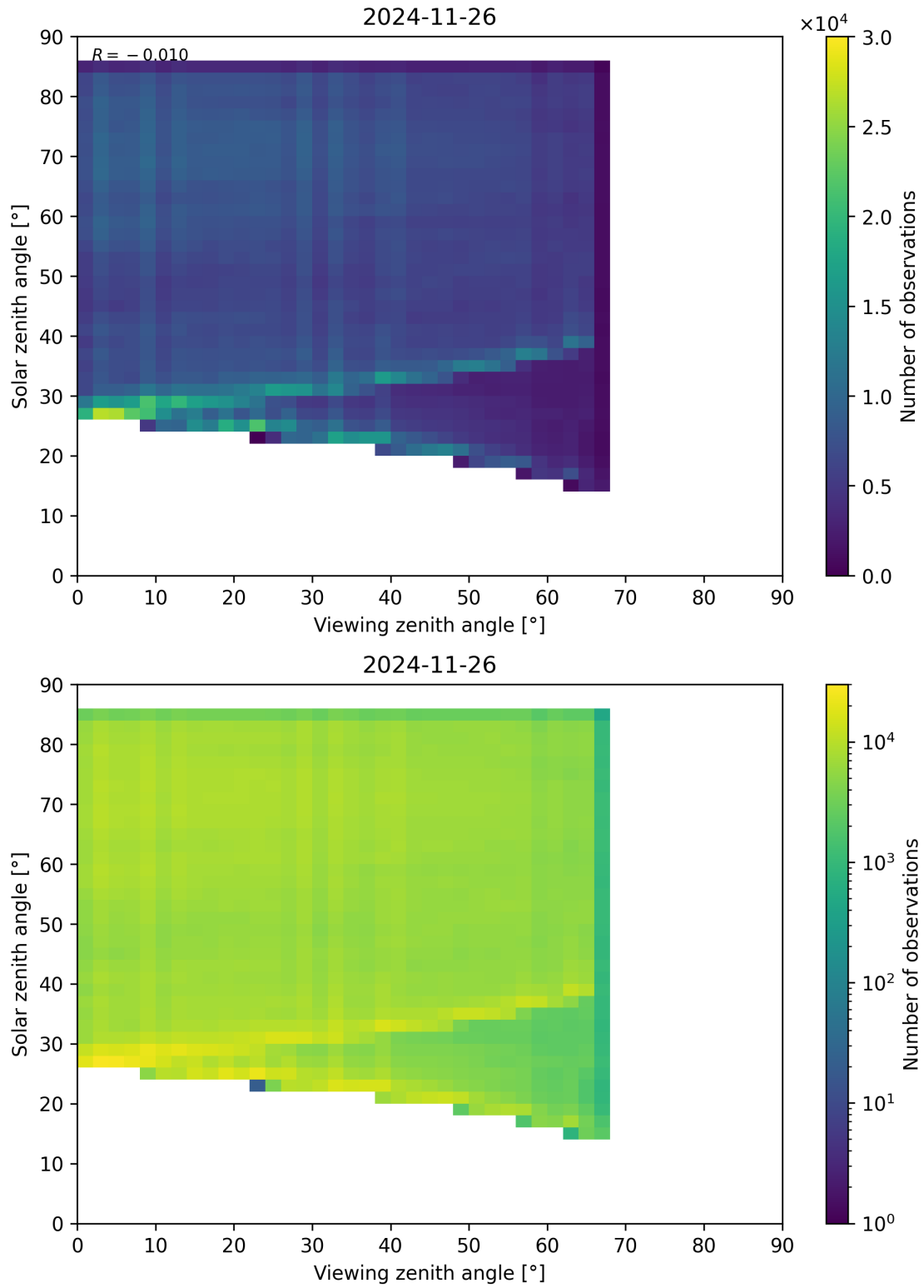
Figure 77: Scatter density plot of “Viewing zenith angle” against “Solar zenith angle” for 2024-11-25 to 2024-11-27.
