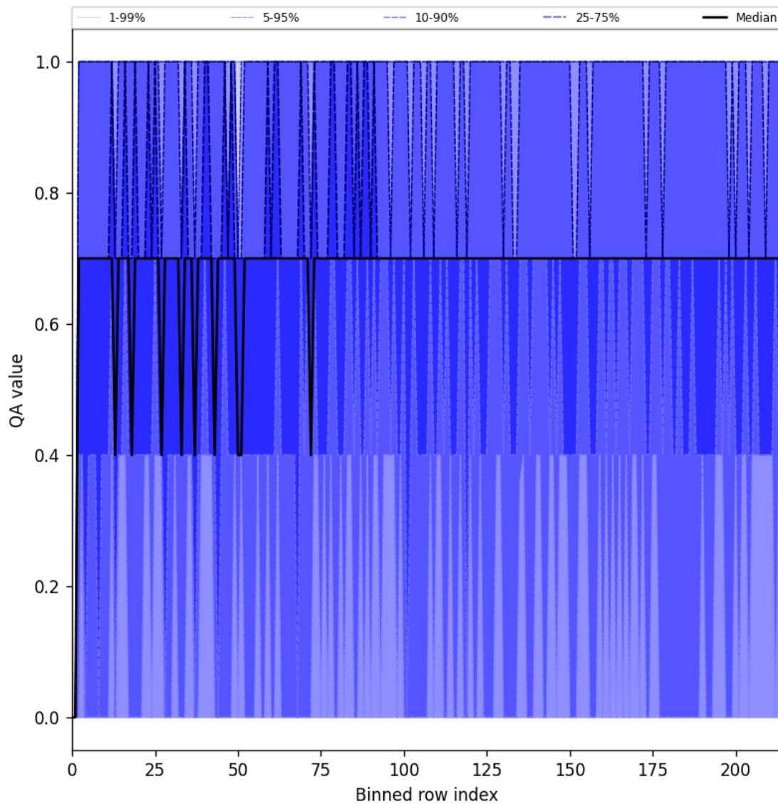
Figure 25: Along track statistics of “QA value” for 2024-11-25 to 2024-11-27
