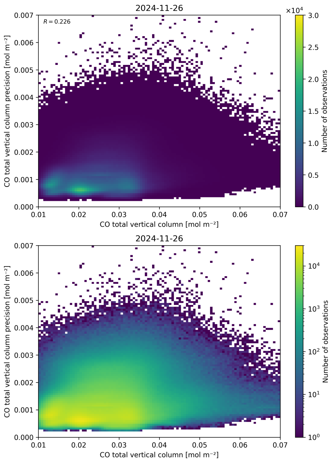
Figure 34: Scatter density plot of “CO total vertical column” against “CO total vertical column precision” for 2024-11-25 to 2024-11-27.
