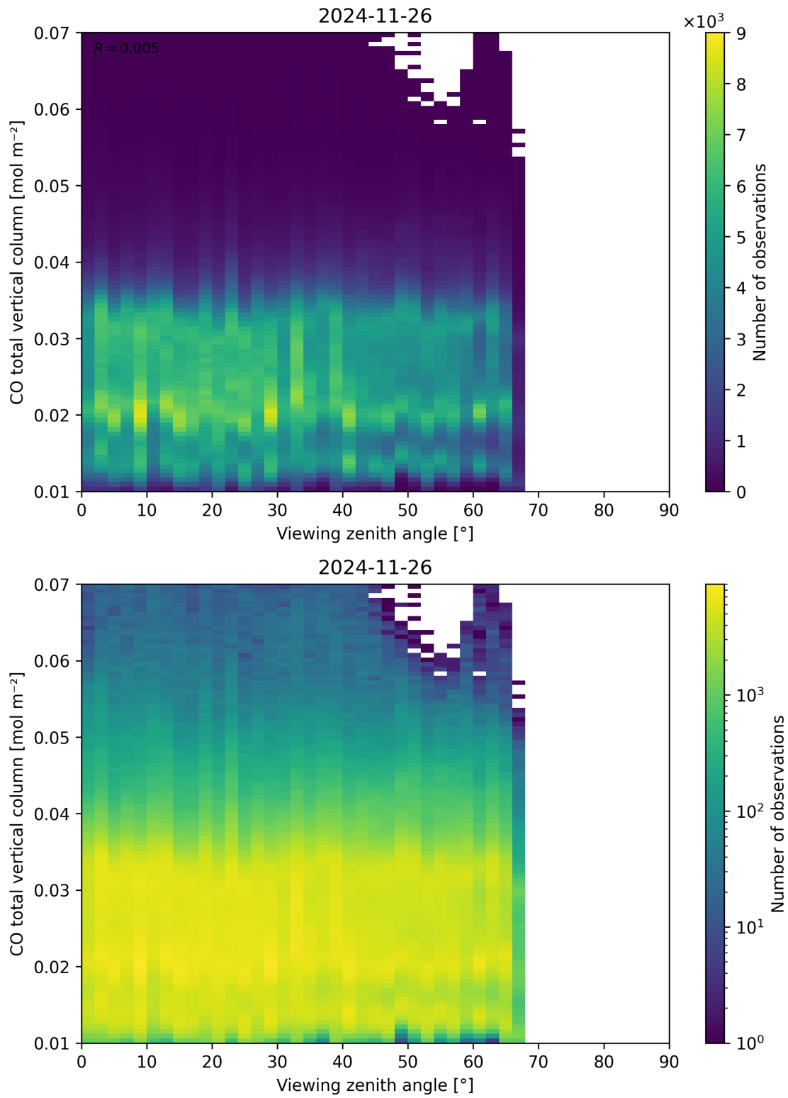
Figure 69: Scatter density plot of “Viewing zenith angle” against “CO total vertical column” for 2024-11-25 to 2024-11-27.
