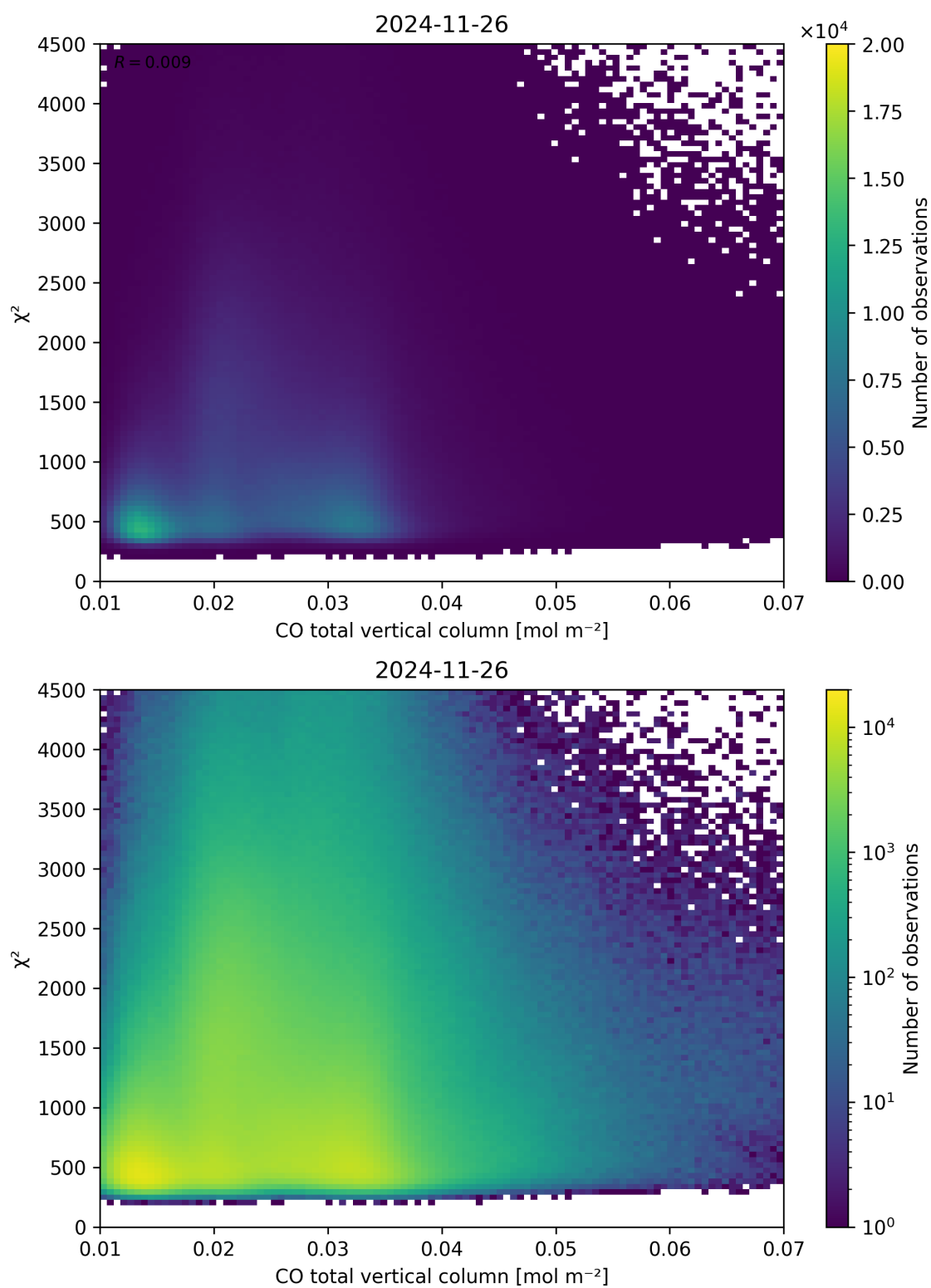
Figure 35: Scatter density plot of “CO total vertical column” against “ \chi^2 ” for 2024-11-25 to 2024-11-27.
