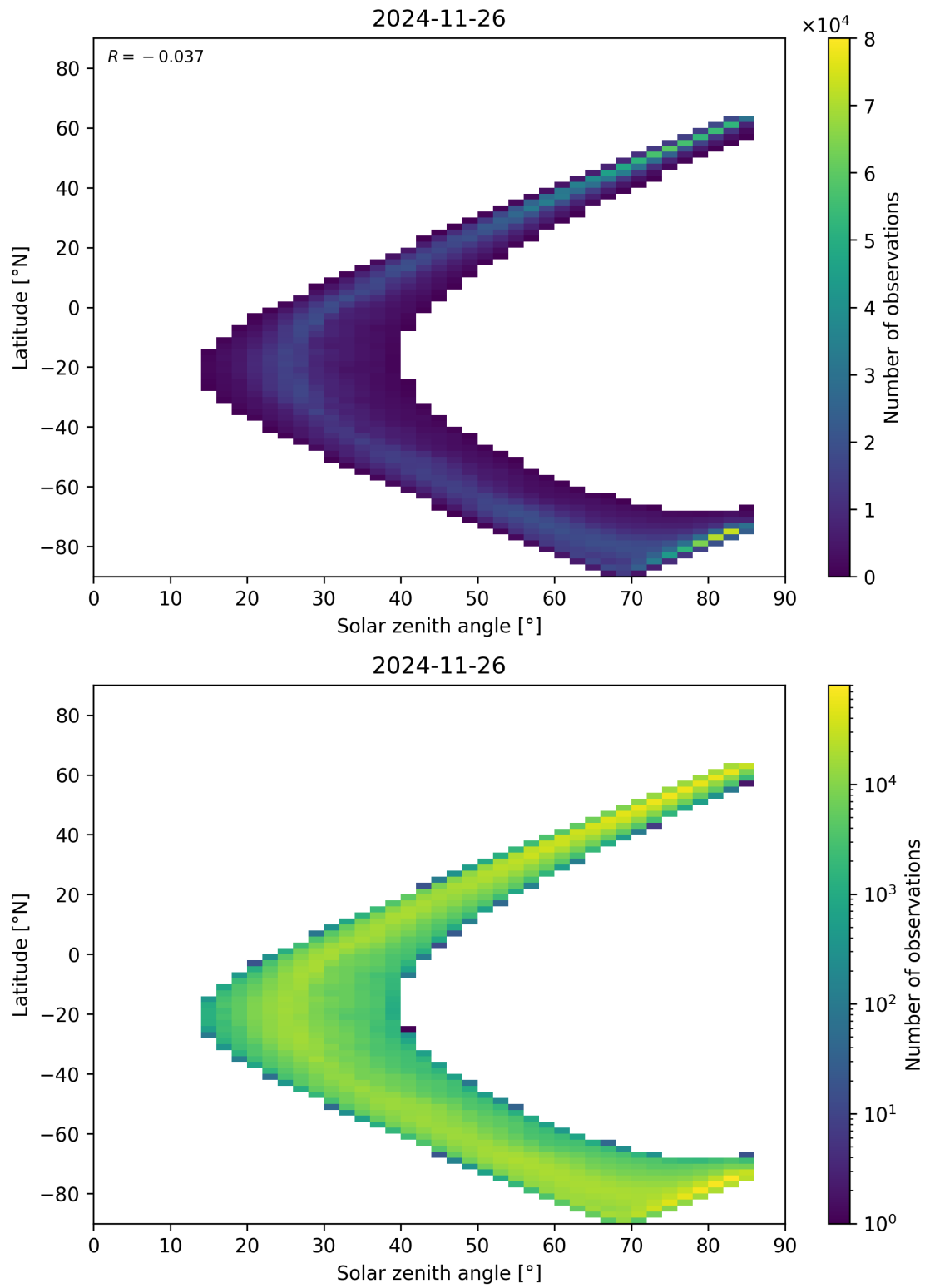
Figure 66: Scatter density plot of “Solar zenith angle” against “Latitude” for 2024-11-25 to 2024-11-27.
