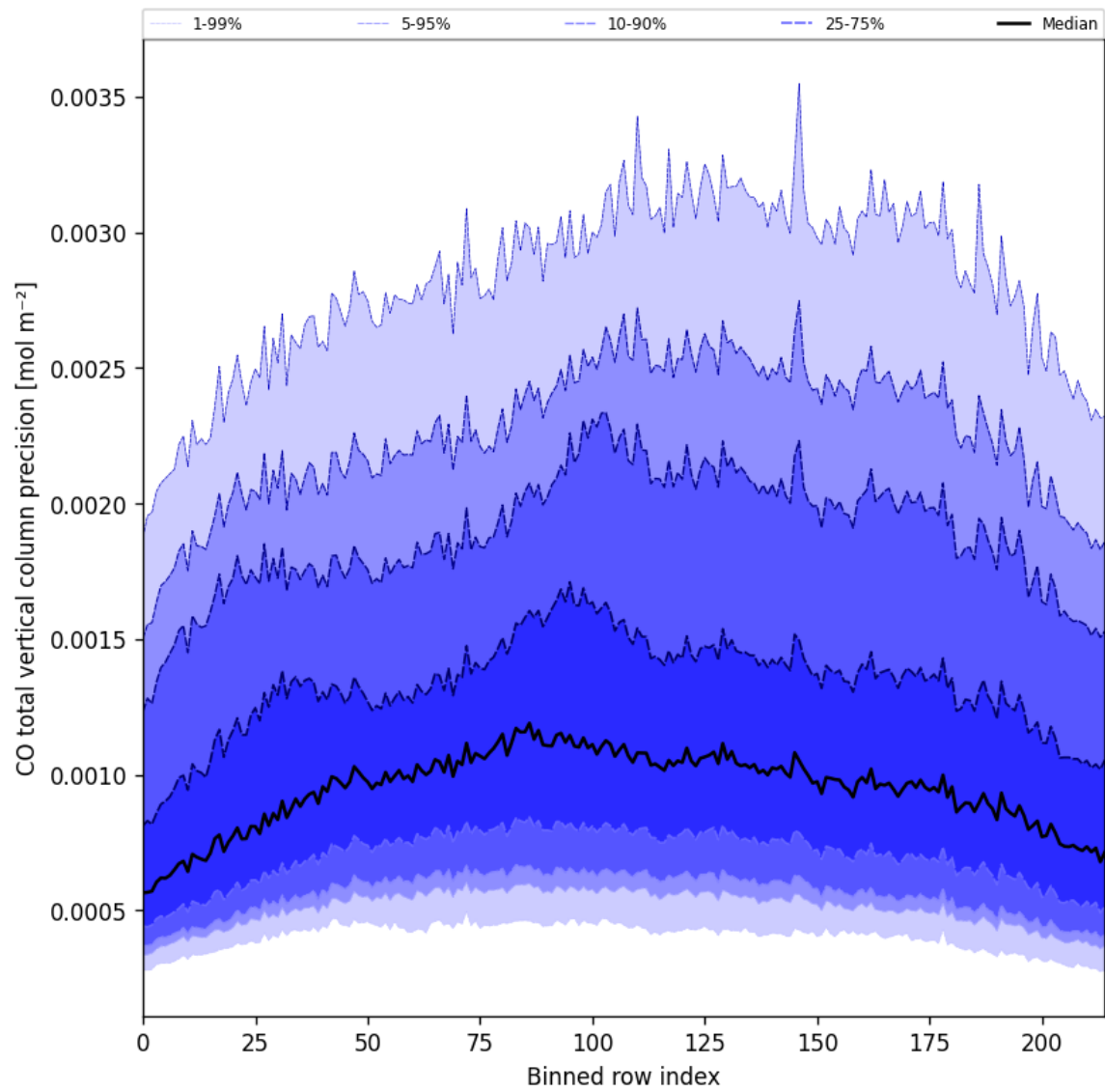
Figure 28: Along track statistics of “CO total vertical column precision” for 2024-11-25 to 2024-11-27
