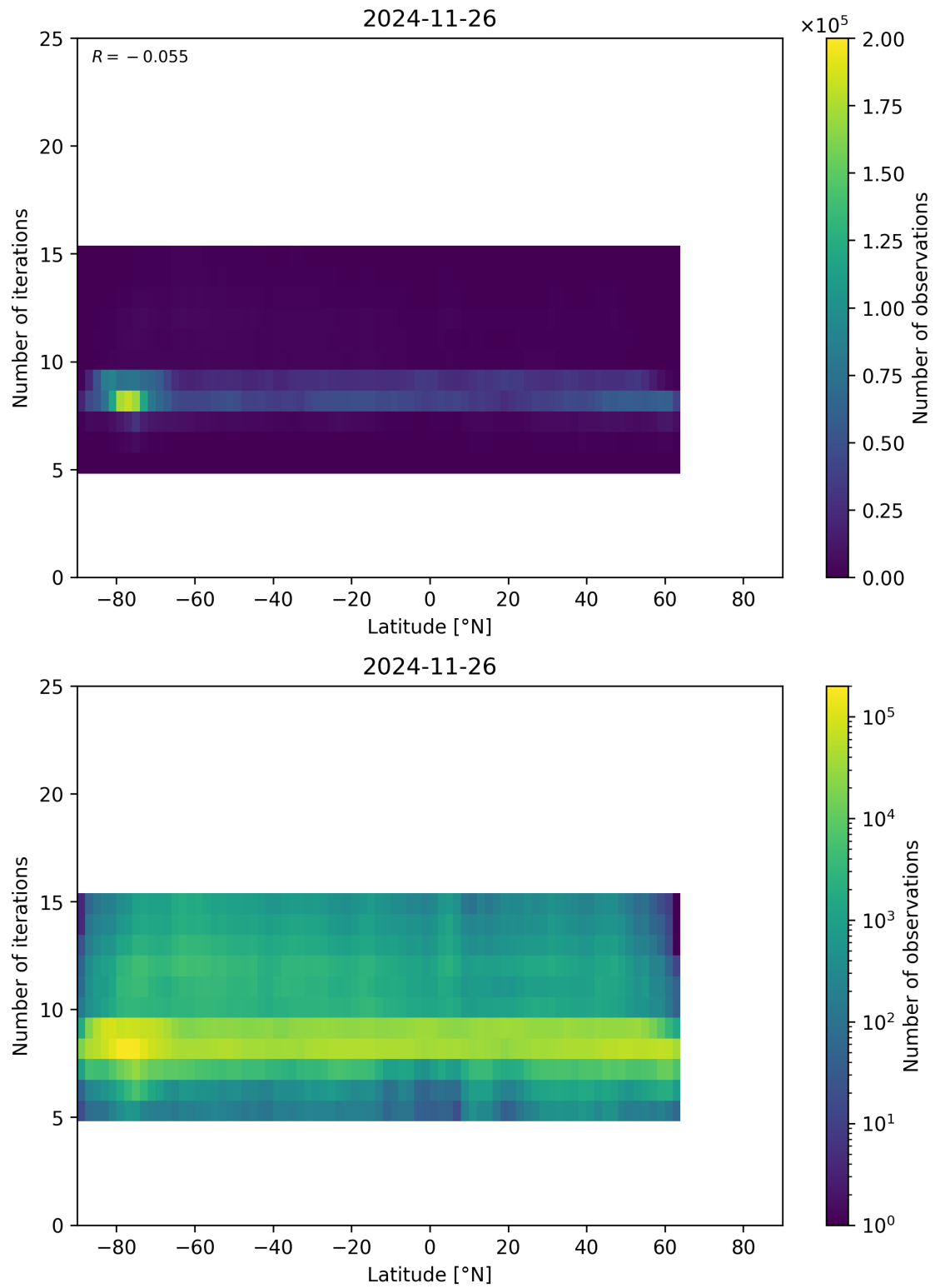
Figure 56: Scatter density plot of “Latitude” against “Number of iterations” for 2024-11-25 to 2024-11-27.
