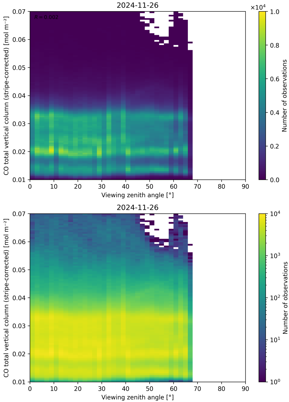
Figure 70: Scatter density plot of “Viewing zenith angle” against “CO total vertical column (stripe-corrected)” for 2024-11-25 to 2024-11-27.
