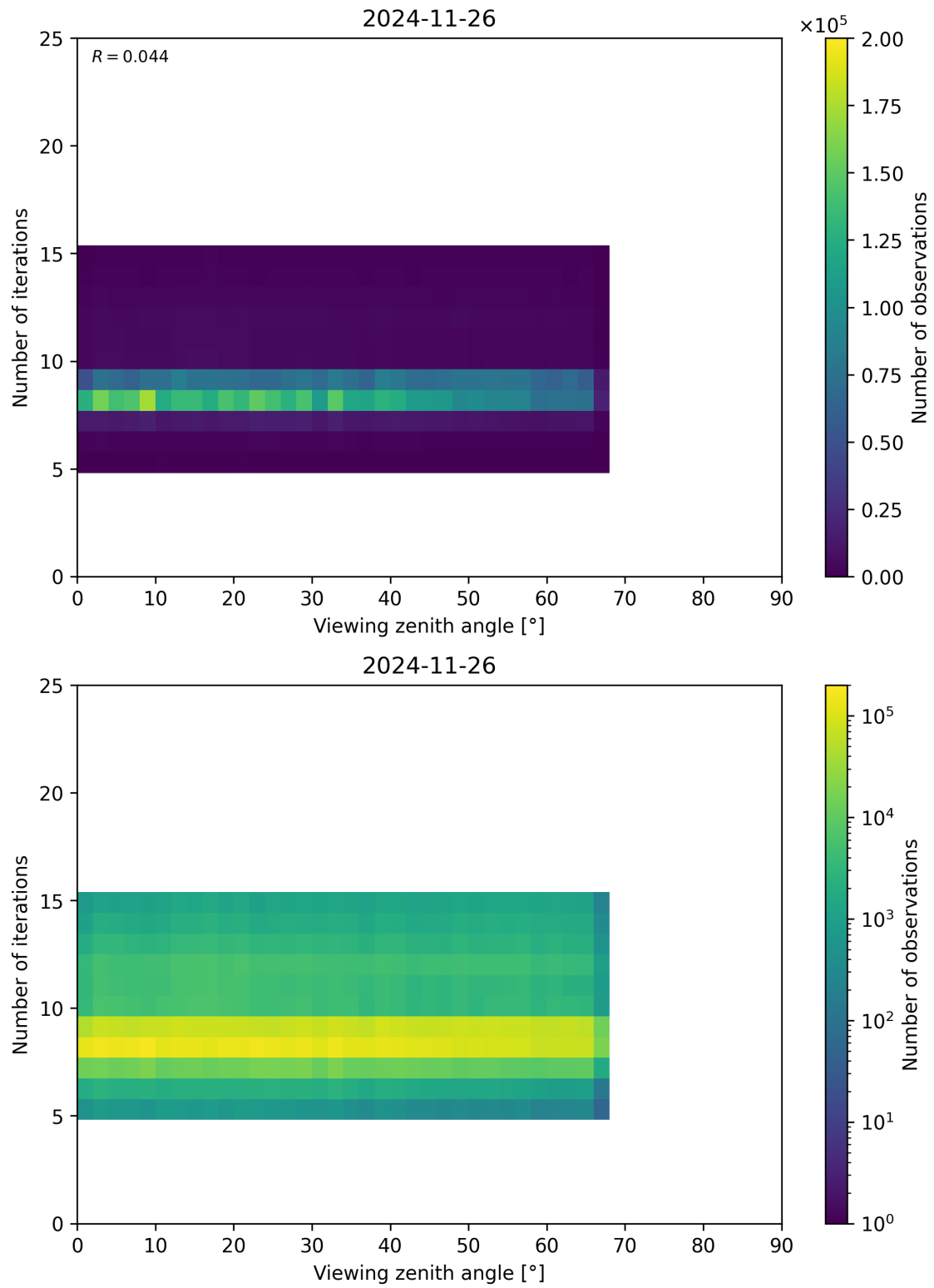
Figure 75: Scatter density plot of “Viewing zenith angle” against “Number of iterations” for 2024-11-25 to 2024-11-27.
