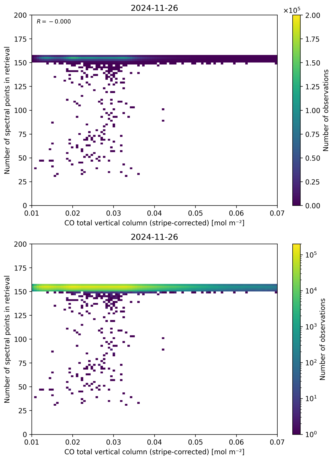
Figure 40: Scatter density plot of “CO total vertical column (stripe-corrected)” against “Number of spectral points in retrieval” for 2024-11-25 to 2024-11-27.
