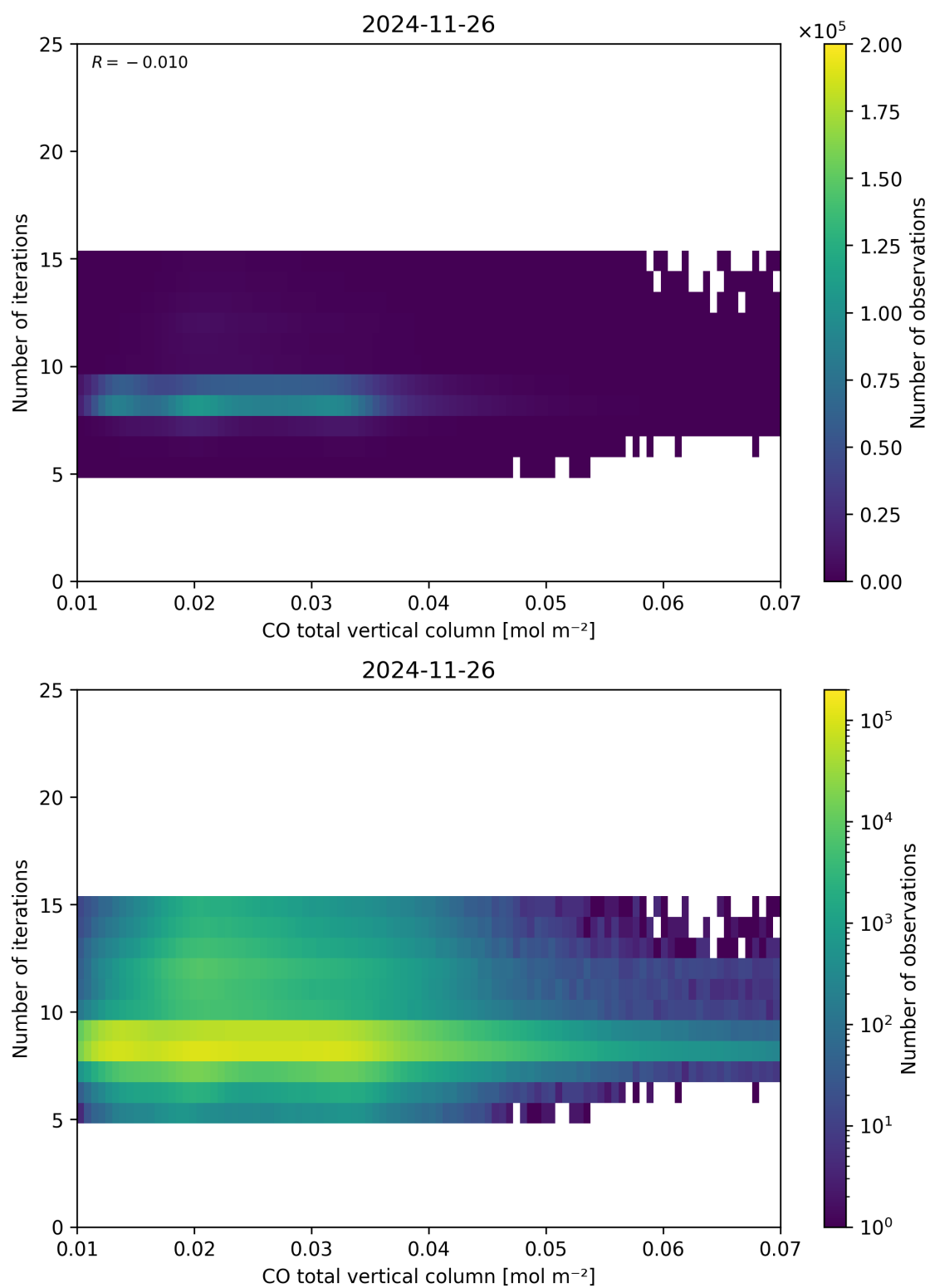
Figure 42: Scatter density plot of “CO total vertical column” against “Number of iterations” for 2024-11-25 to 2024-11-27.
