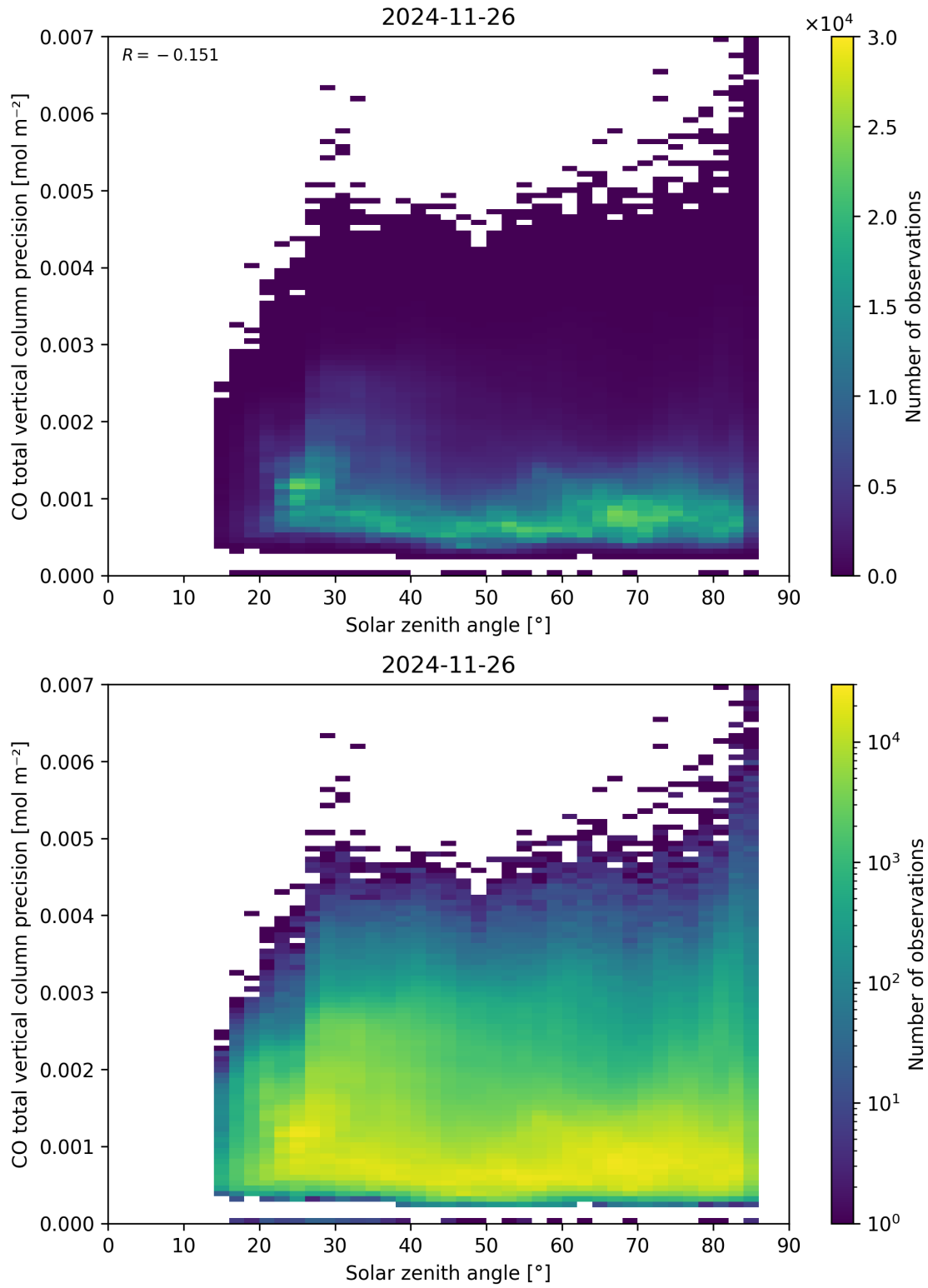
Figure 63: Scatter density plot of “Solar zenith angle” against “CO total vertical column precision” for 2024-11-25 to 2024-11-27.
