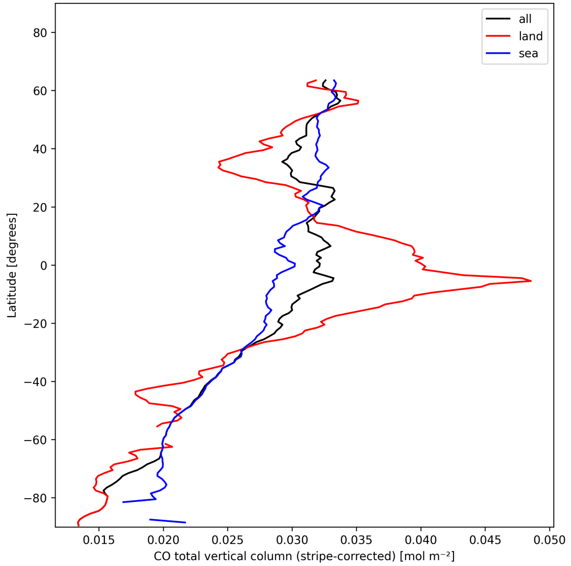
Figure 11: Zonal average of “CO total vertical column (stripe-corrected)” for 2024-11-25 to 2024-11-27.
