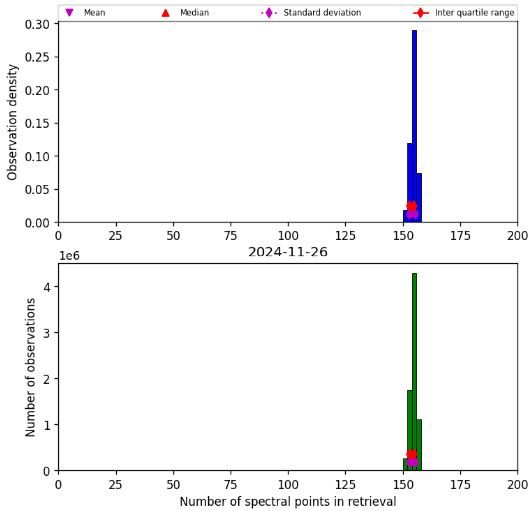
Figure 21: Histogram of “Number of spectral points in retrieval” for 2024-11-25 to 2024-11-27
