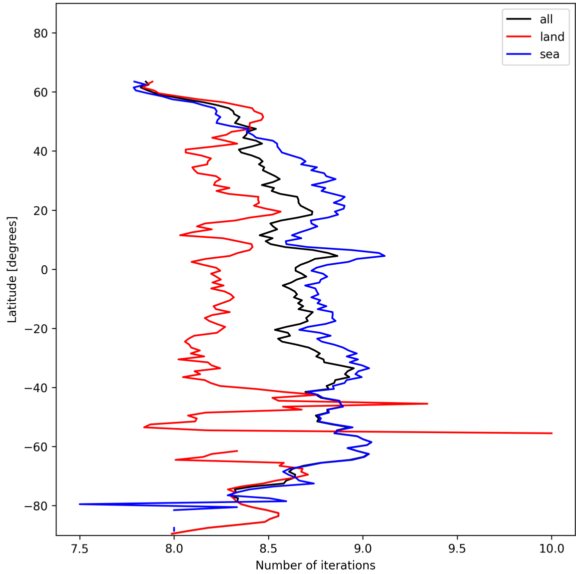
Figure 16: Zonal average of “Number of iterations” for 2024-11-25 to 2024-11-27.
