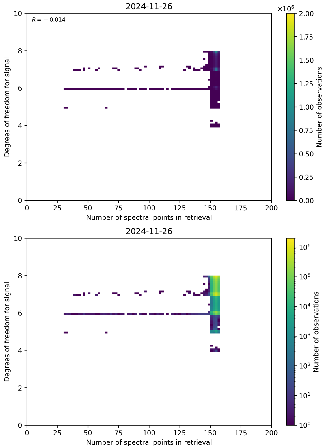
Figure 59: Scatter density plot of “Number of spectral points in retrieval” against “Degrees of freedom for signal” for 2024-11-25 to 2024-11-27.
