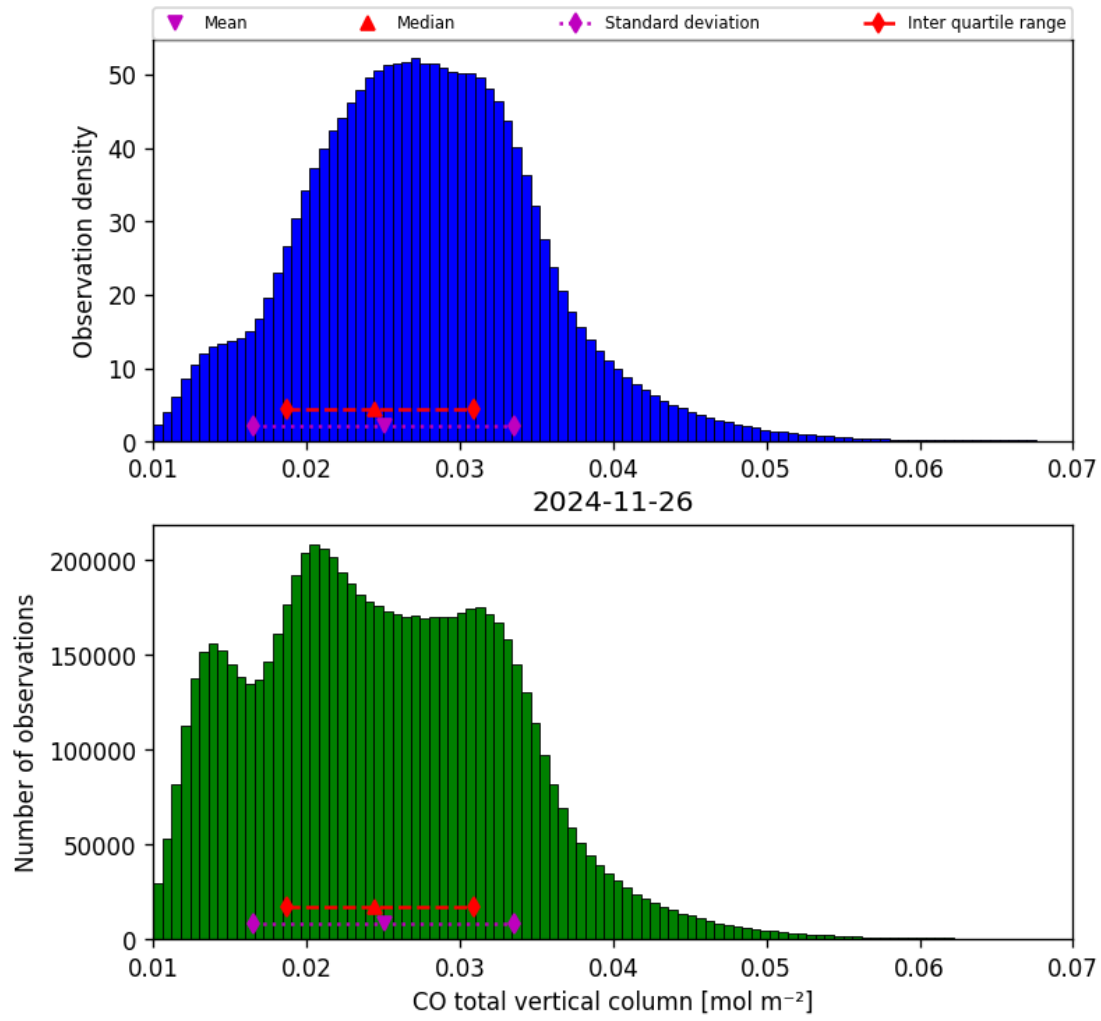
Figure 18: Histogram of “CO total vertical column” for 2024-11-25 to 2024-11-27
