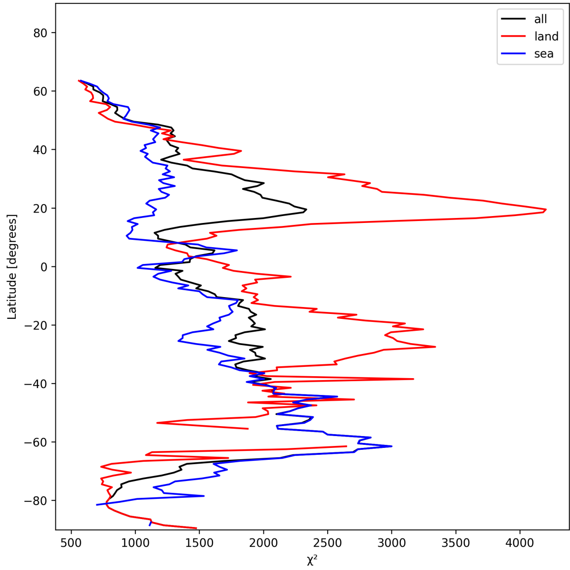
Figure 14: Zonal average of “ \chi^2 ” for 2024-11-25 to 2024-11-27.
