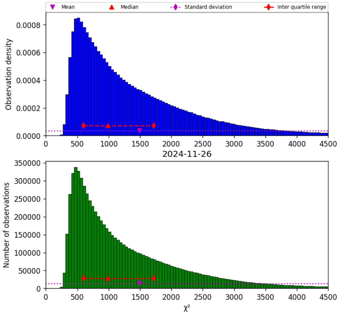
Figure 22: Histogram of “ \chi^2 ” for 2024-11-25 to 2024-11-27
