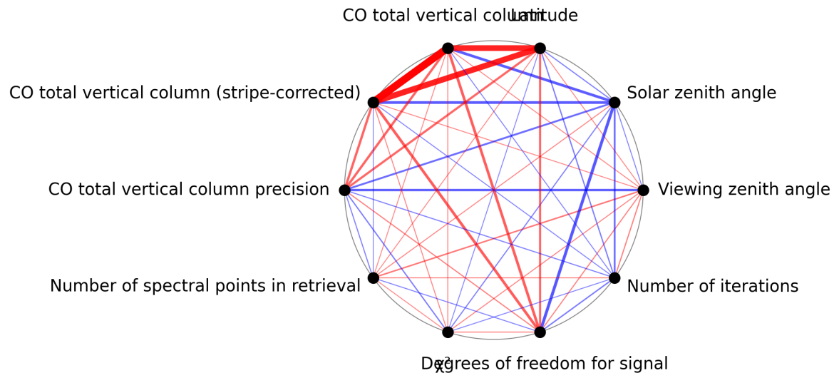
Figure 1: Map of correlation graph for 2024-11-25 to 2024-11-27.
