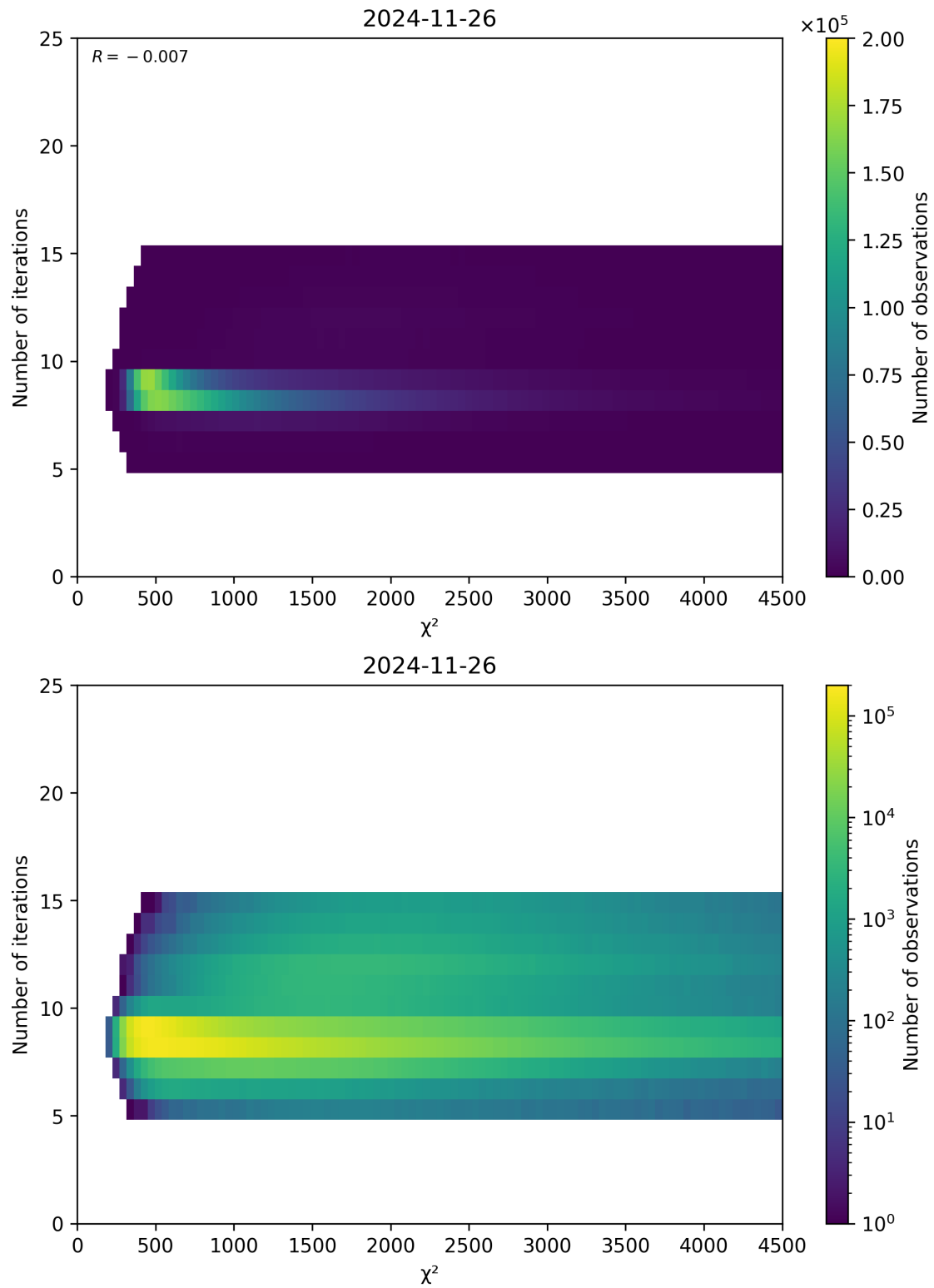
Figure 49: Scatter density plot of “ \chi^2 ” against “Number of iterations” for 2024-11-25 to 2024-11-27.
