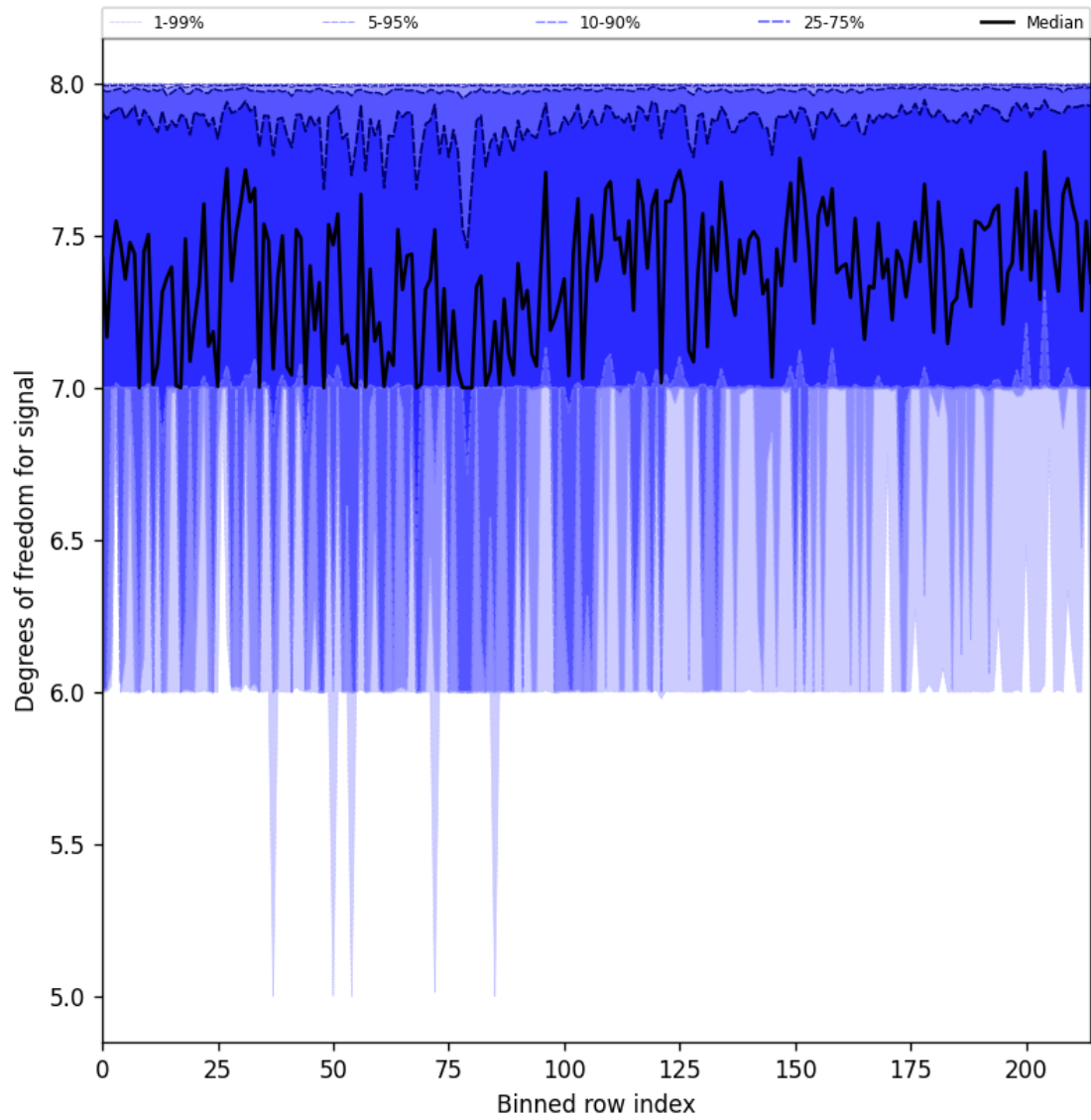
Figure 31: Along track statistics of “Degrees of freedom for signal” for 2024-11-25 to 2024-11-27
