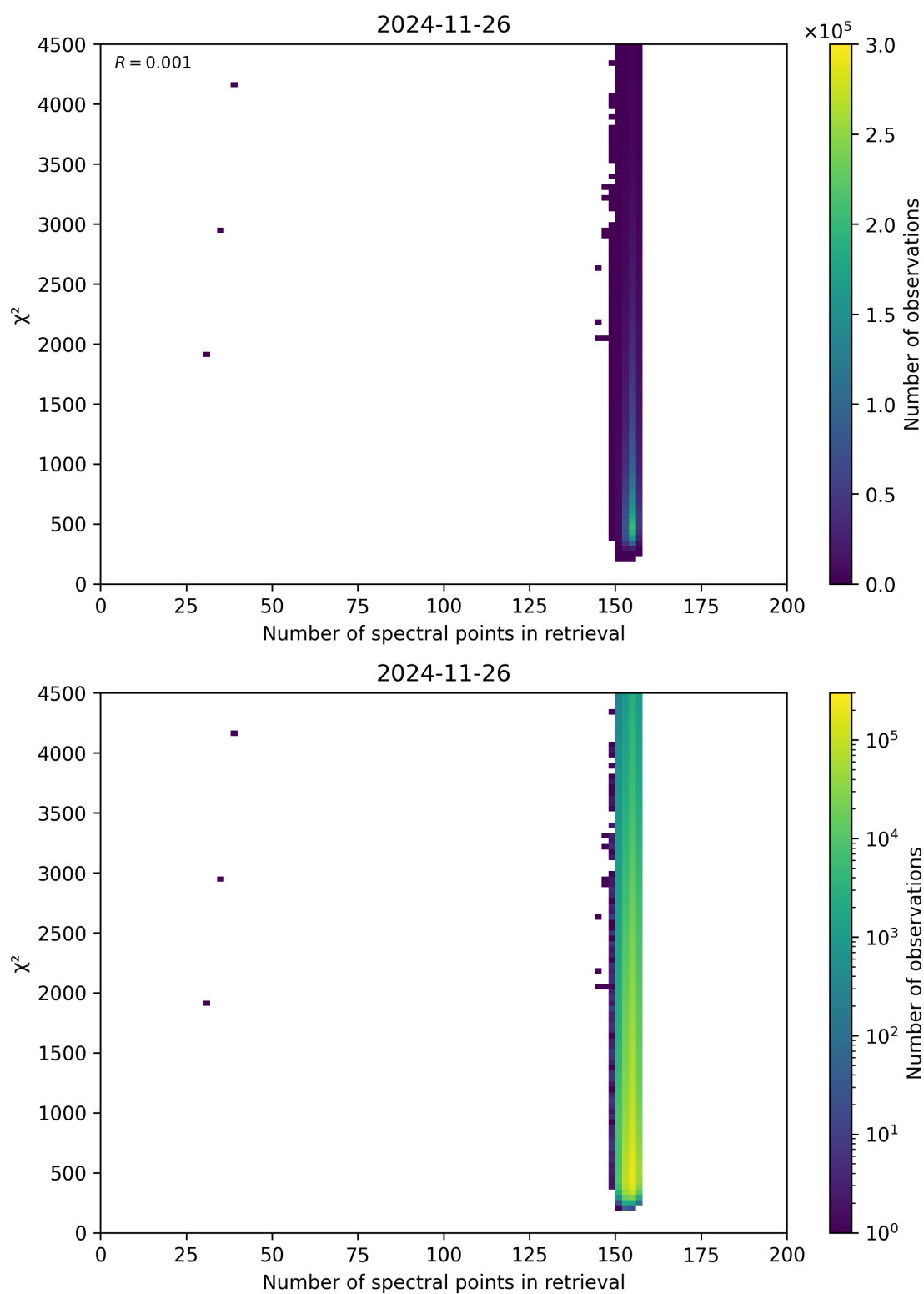
Figure 58: Scatter density plot of “Number of spectral points in retrieval” against “ \chi^2 ” for 2024-11-25 to 2024-11-27.
