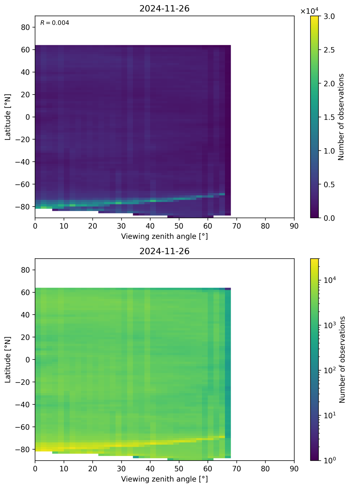
Figure 74: Scatter density plot of “Viewing zenith angle” against “Latitude” for 2024-11-25 to 2024-11-27.
