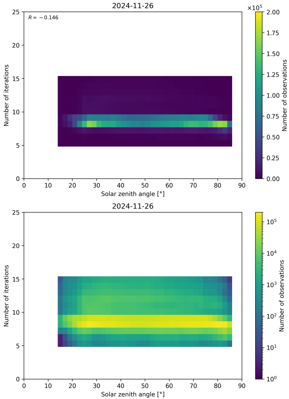
Figure 67: Scatter density plot of “Solar zenith angle” against “Number of iterations” for 2024-11-25 to 2024-11-27.
