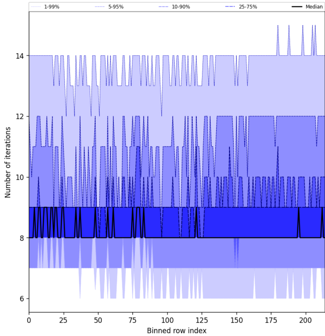
Figure 32: Along track statistics of “Number of iterations” for 2024-11-25 to 2024-11-27
