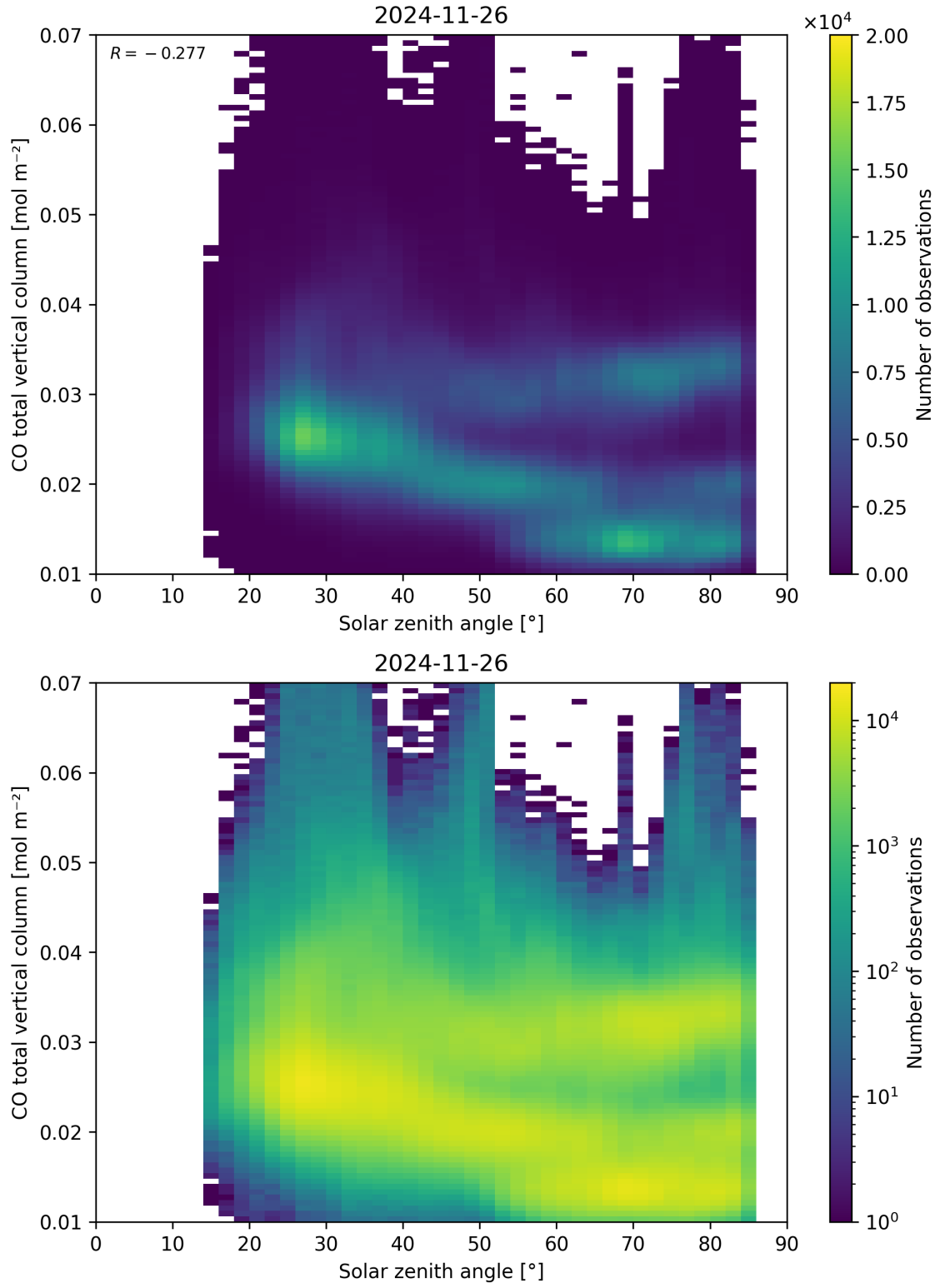
Figure 61: Scatter density plot of “Solar zenith angle” against “CO total vertical column” for 2024-11-25 to 2024-11-27.
