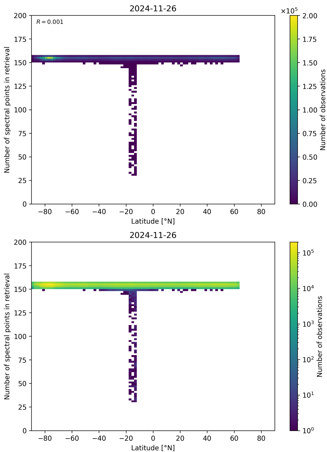
Figure 57: Scatter density plot of “Latitude” against “Number of spectral points in retrieval” for 2024-11-25 to 2024-11-27.
