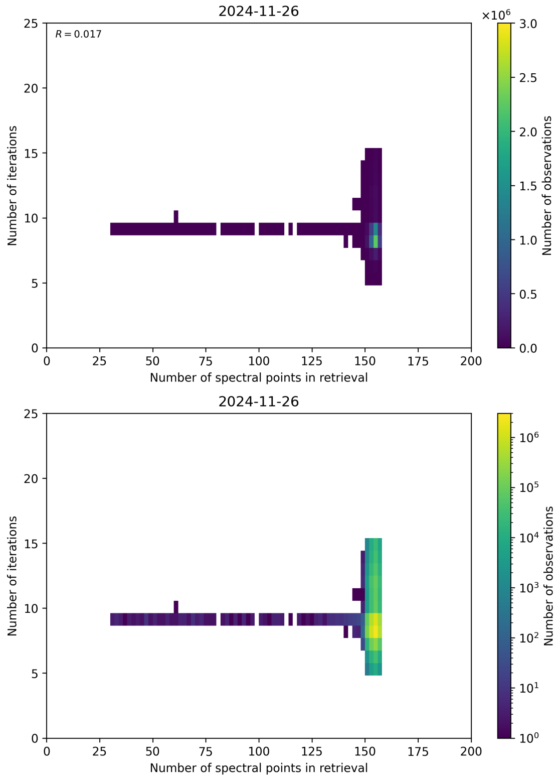
Figure 60: Scatter density plot of “Number of spectral points in retrieval” against “Number of iterations” for 2024-11-25 to 2024-11-27.
