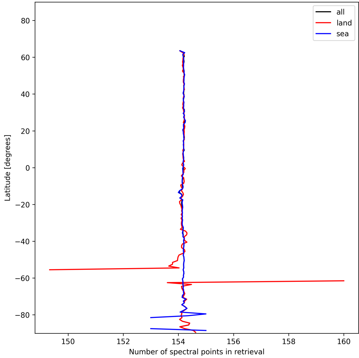
Figure 13: Zonal average of “Number of spectral points in retrieval” for 2024-11-25 to 2024-11-27.
