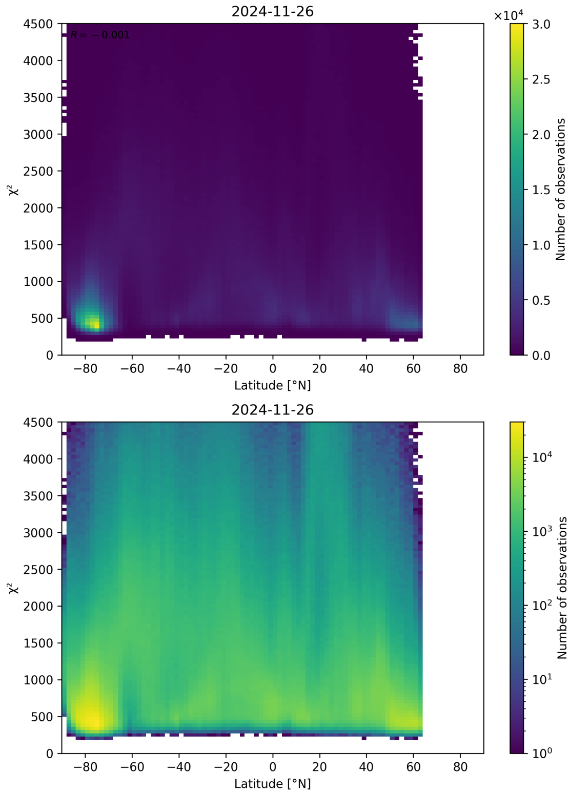
Figure 54: Scatter density plot of “Latitude” against “ \chi^2 ” for 2024-11-25 to 2024-11-27.
