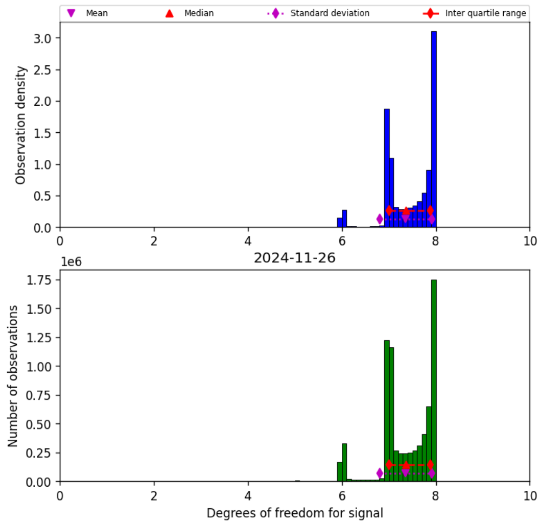
Figure 23: Histogram of “Degrees of freedom for signal” for 2024-11-25 to 2024-11-27
