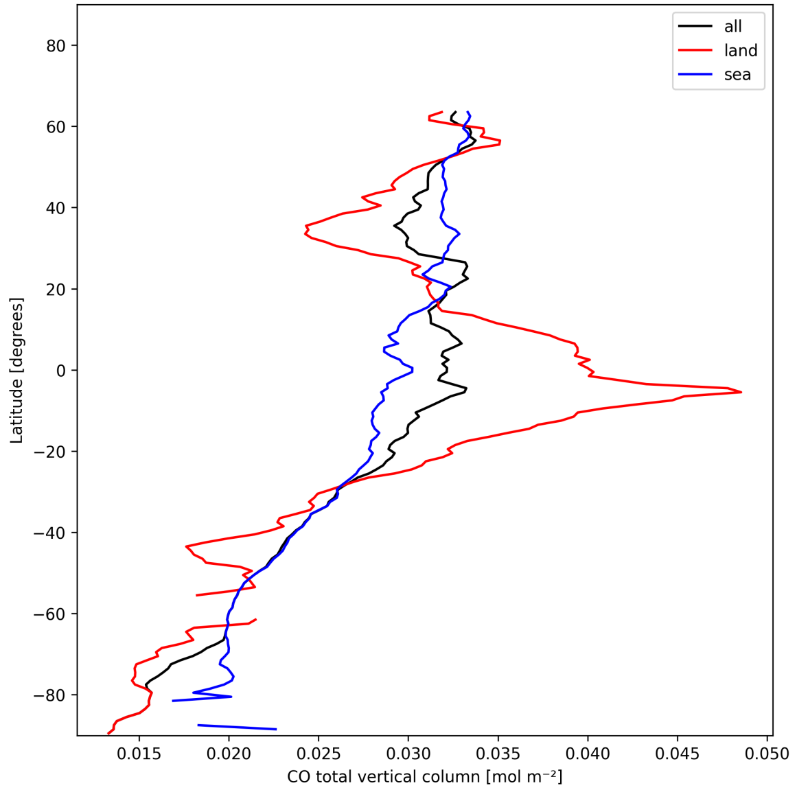
Figure 10: Zonal average of “CO total vertical column” for 2024-11-25 to 2024-11-27.
