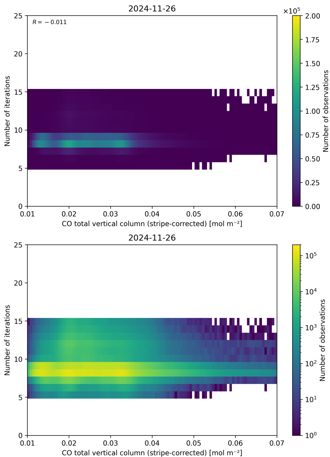
Figure 39: Scatter density plot of “CO total vertical column (stripe-corrected)” against “Number of iterations” for 2024-11-25 to 2024-11-27.
