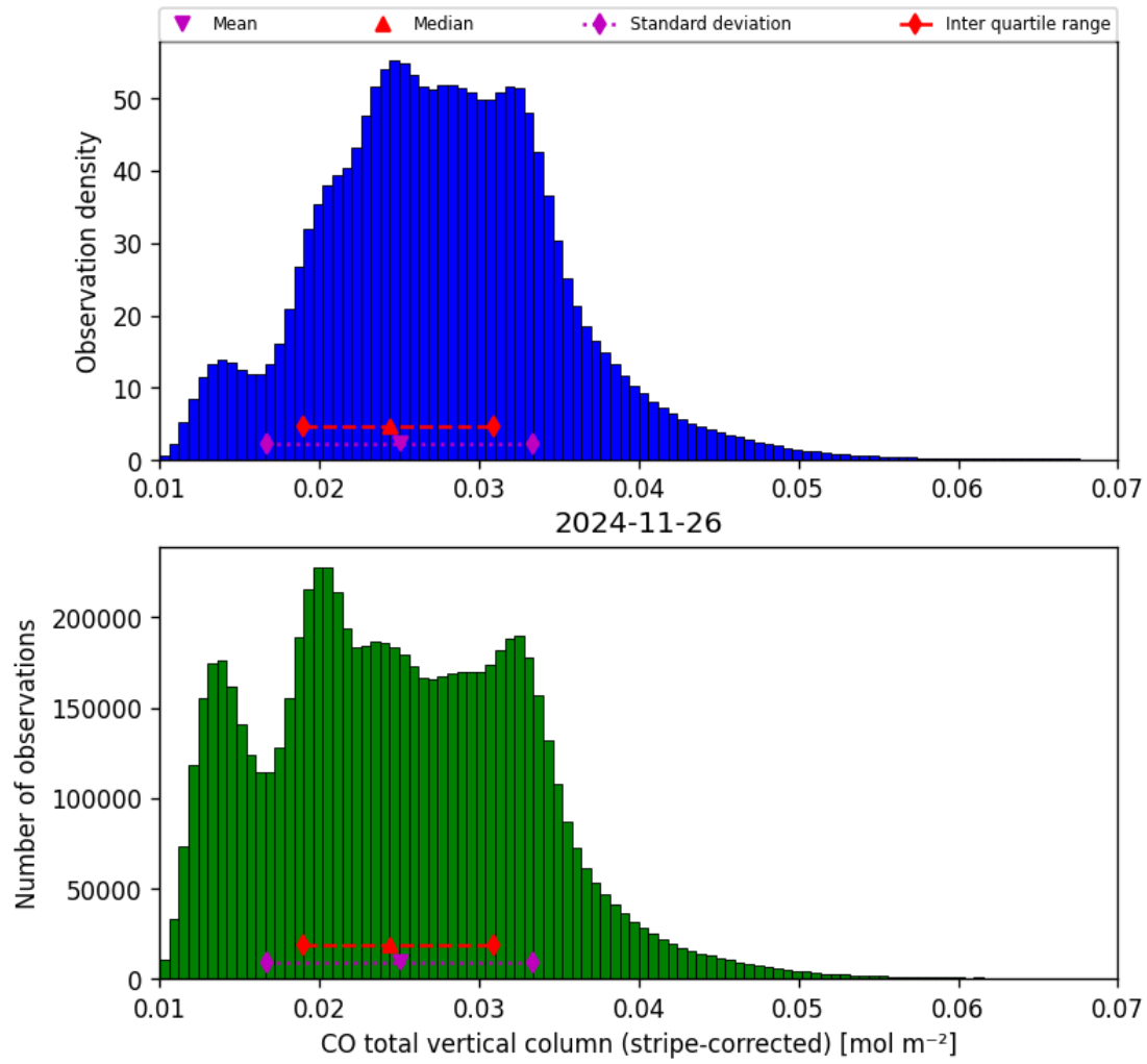
Figure 19: Histogram of “CO total vertical column (stripe-corrected)” for 2024-11-25 to 2024-11-27
