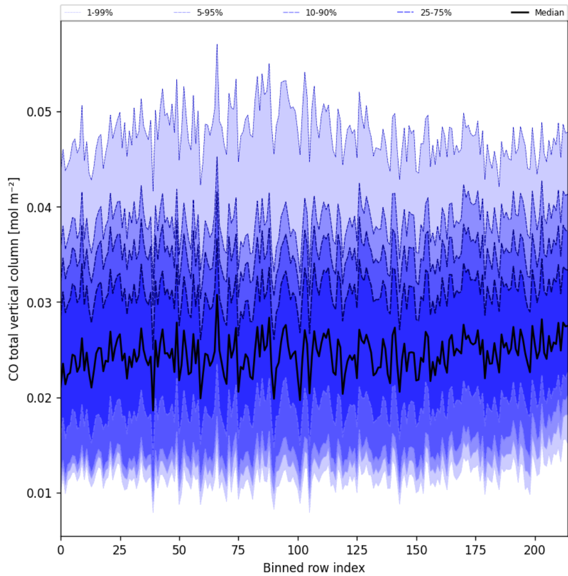
Figure 26: Along track statistics of “CO total vertical column” for 2024-11-25 to 2024-11-27
