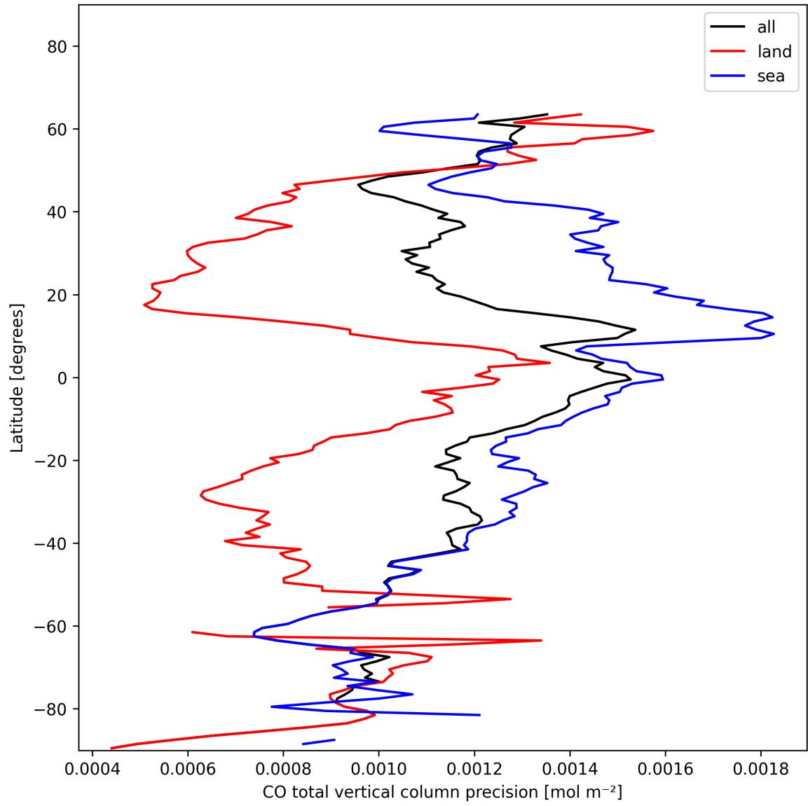
Figure 12: Zonal average of “CO total vertical column precision” for 2024-11-25 to 2024-11-27.
