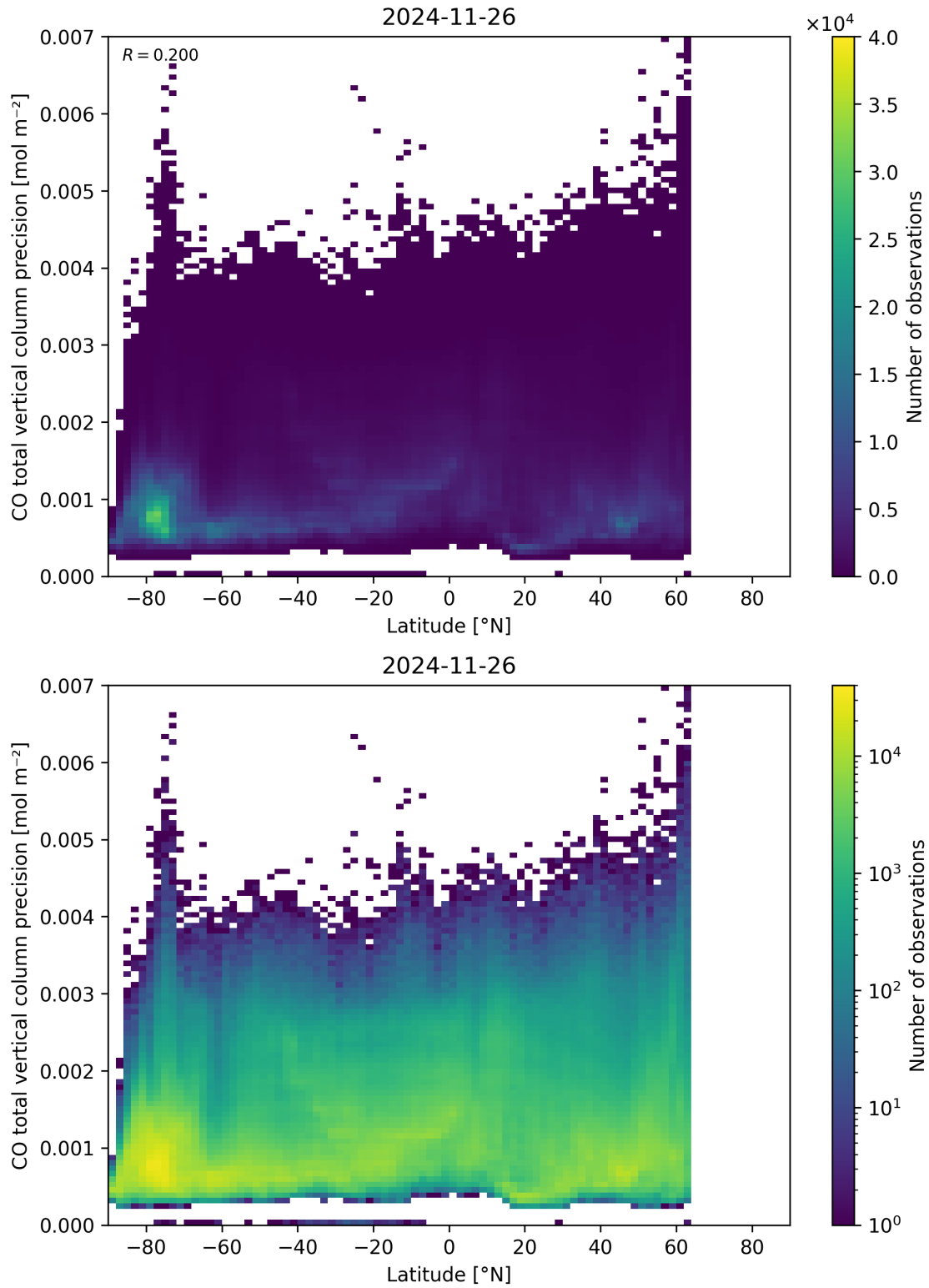
Figure 53: Scatter density plot of “Latitude” against “CO total vertical column precision” for 2024-11-25 to 2024-11-27.
