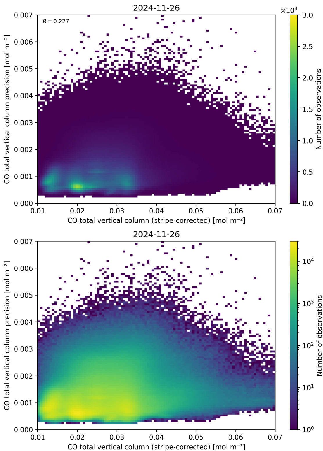
Figure 36: Scatter density plot of “CO total vertical column (stripe-corrected)” against “CO total vertical column precision” for 2024-11-25 to 2024-11-27.
