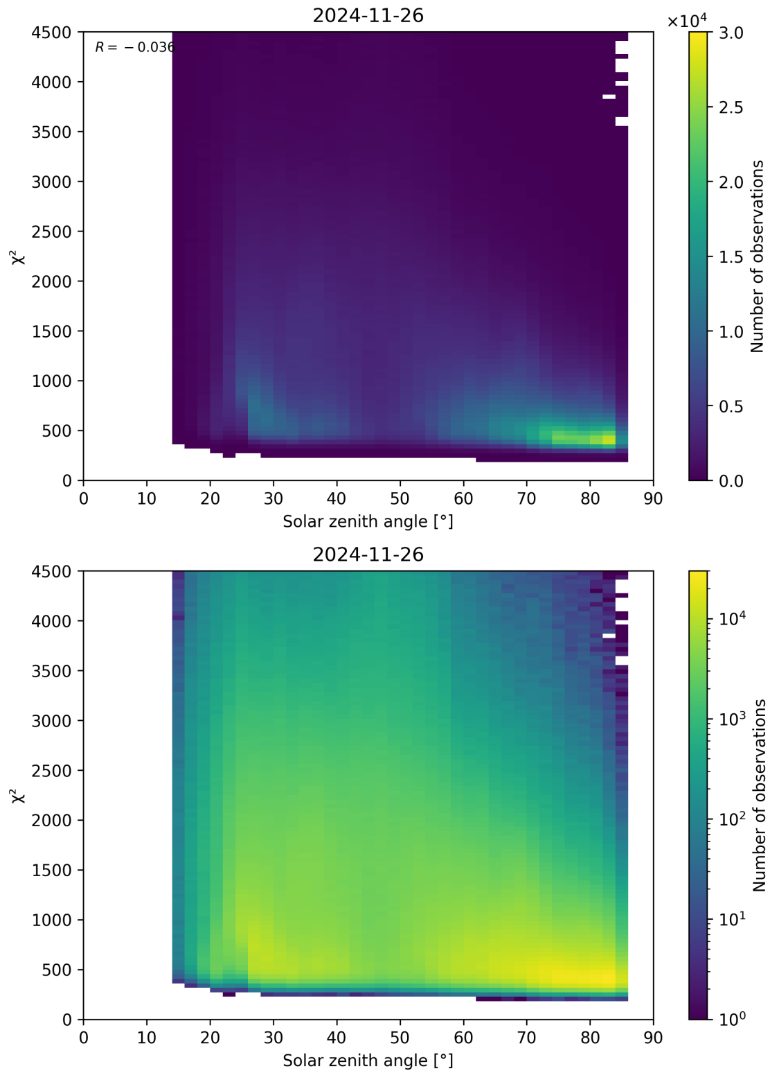
Figure 64: Scatter density plot of “Solar zenith angle” against “ \chi^2 ” for 2024-11-25 to 2024-11-27.
