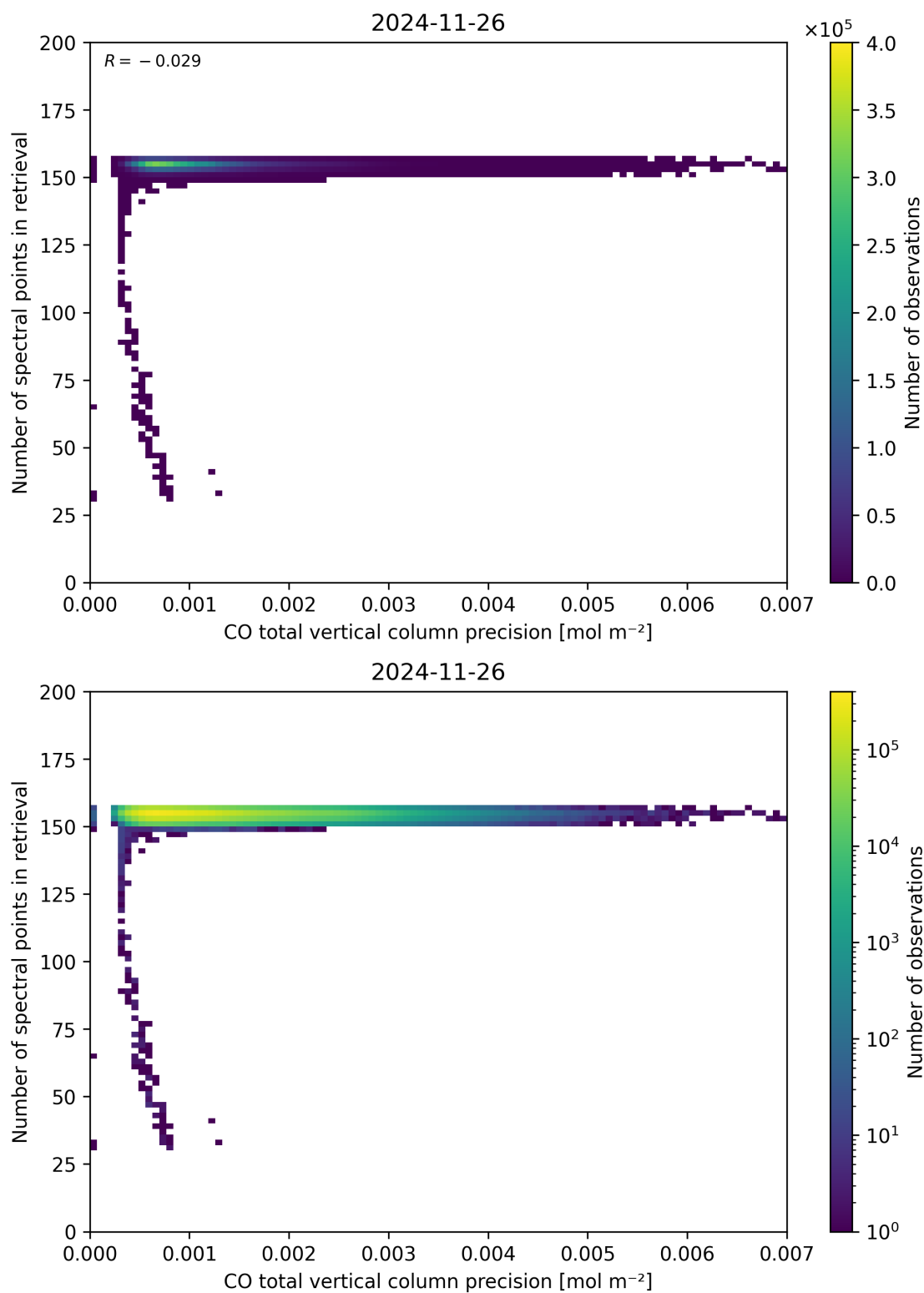
Figure 47: Scatter density plot of “CO total vertical column precision” against “Number of spectral points in retrieval” for 2024-11-25 to 2024-11-27.
