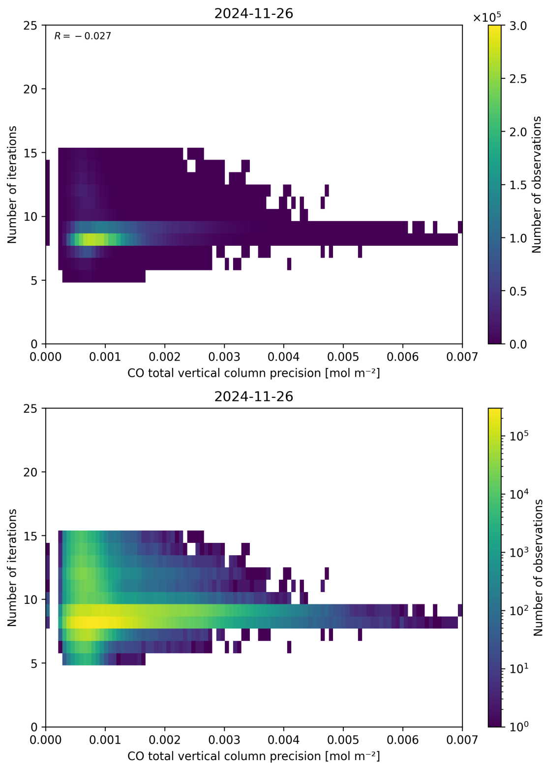
Figure 46: Scatter density plot of “CO total vertical column precision” against “Number of iterations” for 2024-11-25 to 2024-11-27.
