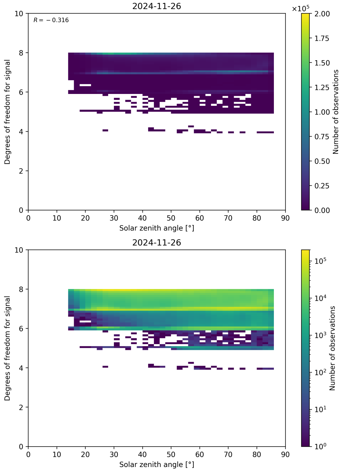
Figure 65: Scatter density plot of “Solar zenith angle” against “Degrees of freedom for signal” for 2024-11-25 to 2024-11-27.
