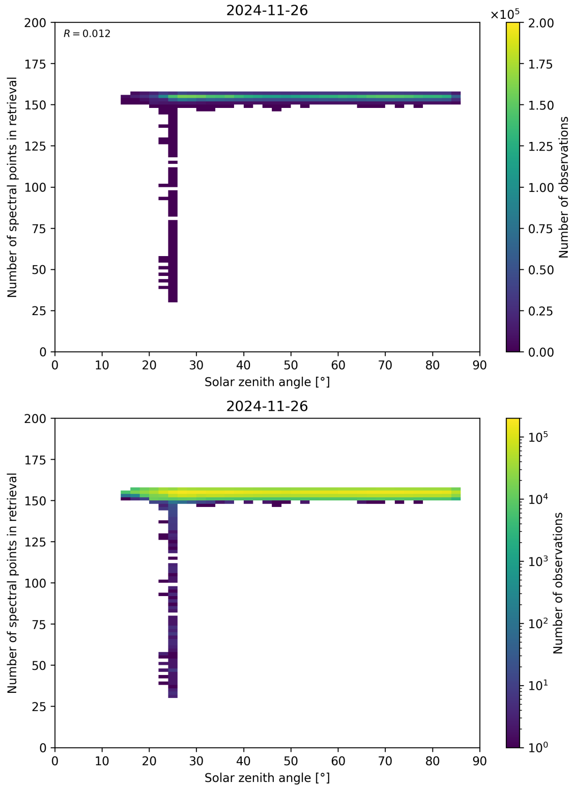
Figure 68: Scatter density plot of “Solar zenith angle” against “Number of spectral points in retrieval” for 2024-11-25 to 2024-11-27.
