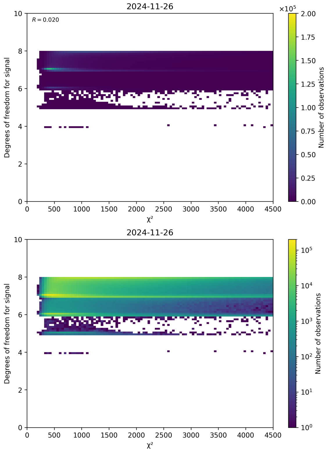
Figure 48: Scatter density plot of “ \chi^2 ” against “Degrees of freedom for signal” for 2024-11-25 to 2024-11-27.
