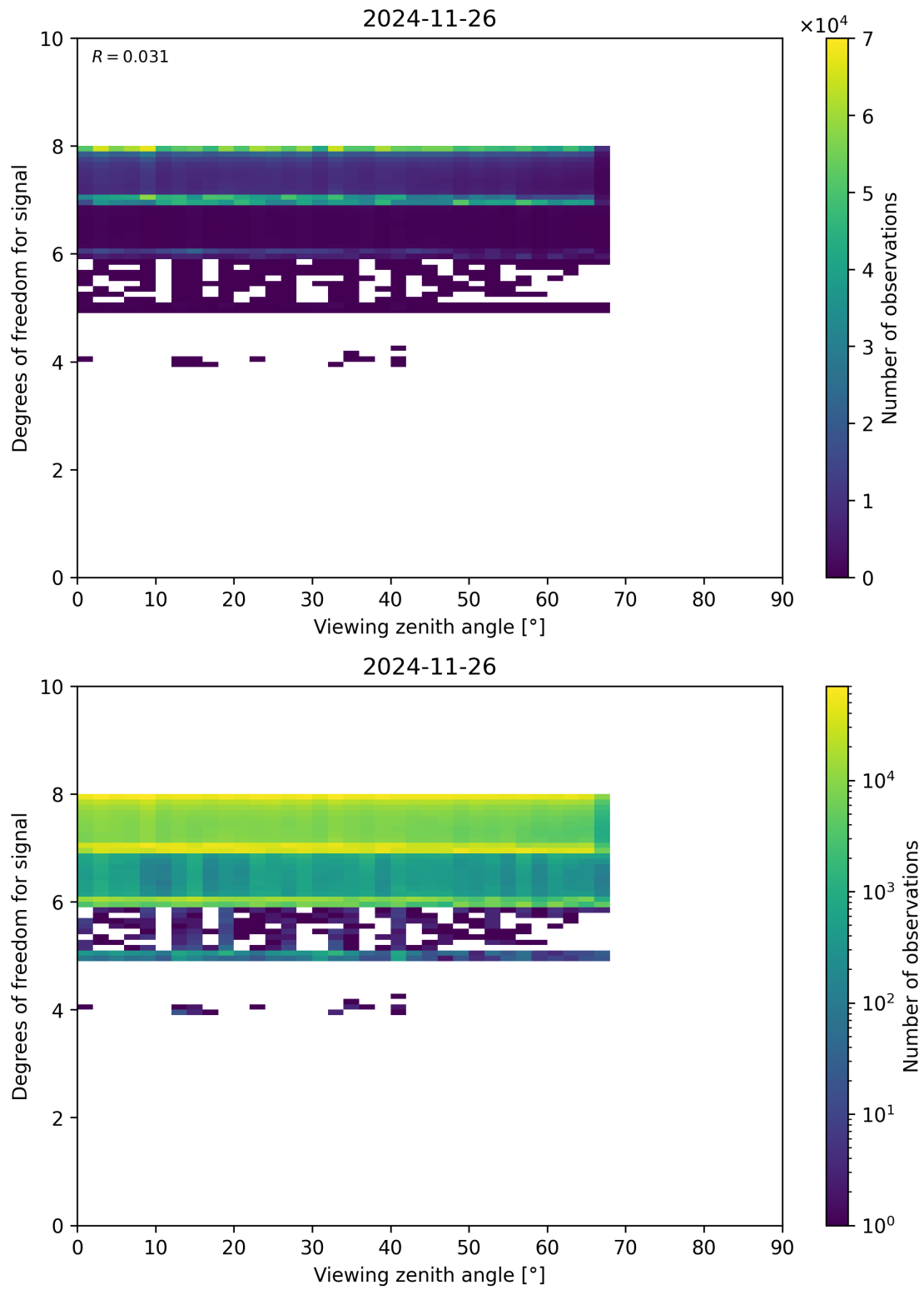
Figure 73: Scatter density plot of “Viewing zenith angle” against “Degrees of freedom for signal” for 2024-11-25 to 2024-11-27.
