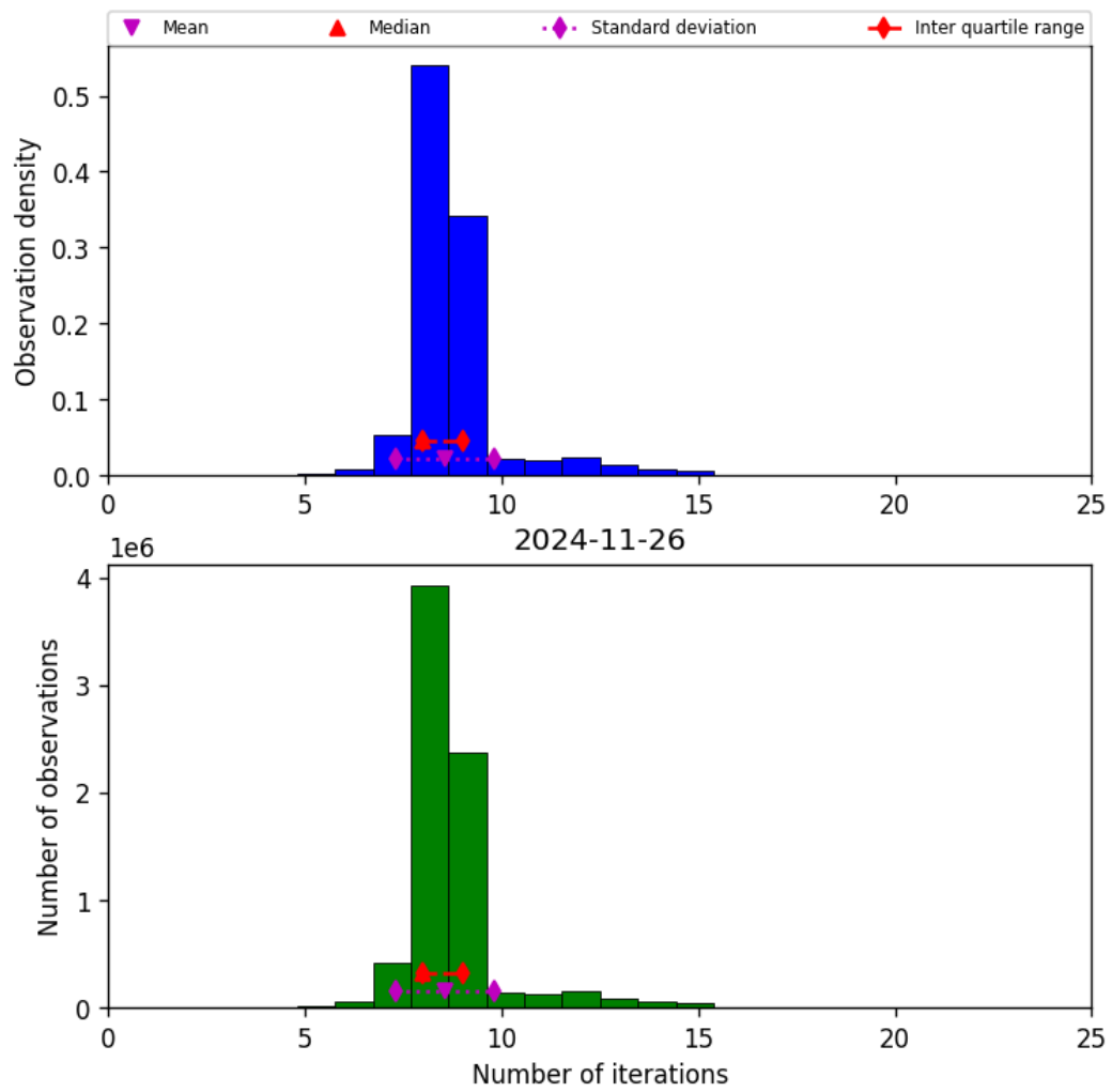
Figure 24: Histogram of “Number of iterations” for 2024-11-25 to 2024-11-27
