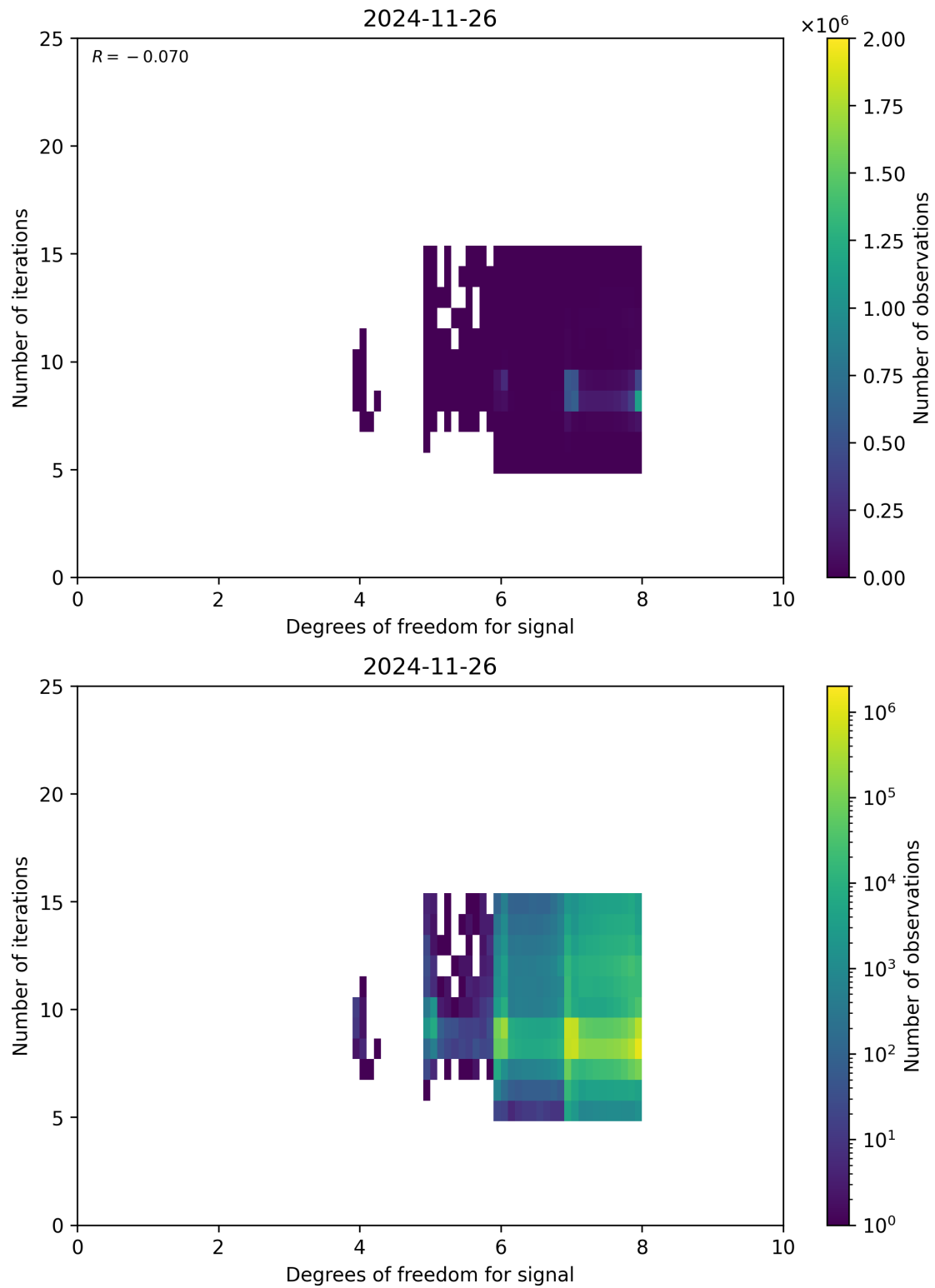
Figure 50: Scatter density plot of “Degrees of freedom for signal” against “Number of iterations” for 2024-11-25 to 2024-11-27.
