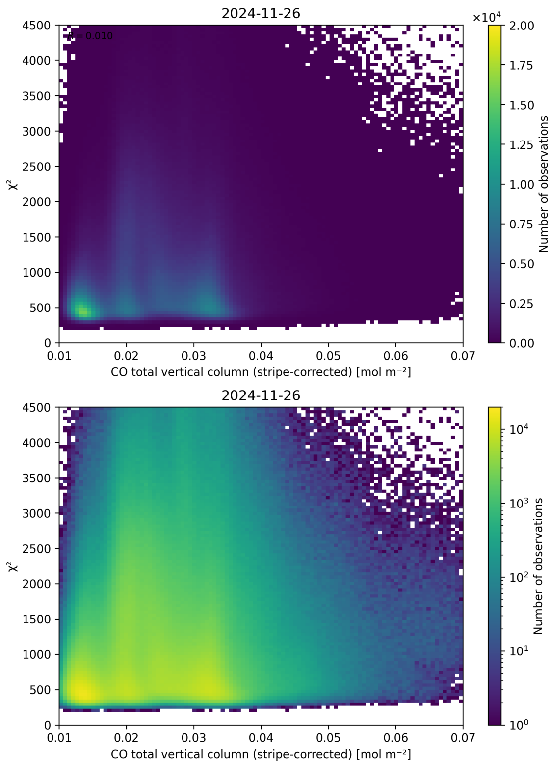
Figure 37: Scatter density plot of “CO total vertical column (stripe-corrected)” against “ \chi^2 ” for 2024-11-25 to 2024-11-27.
