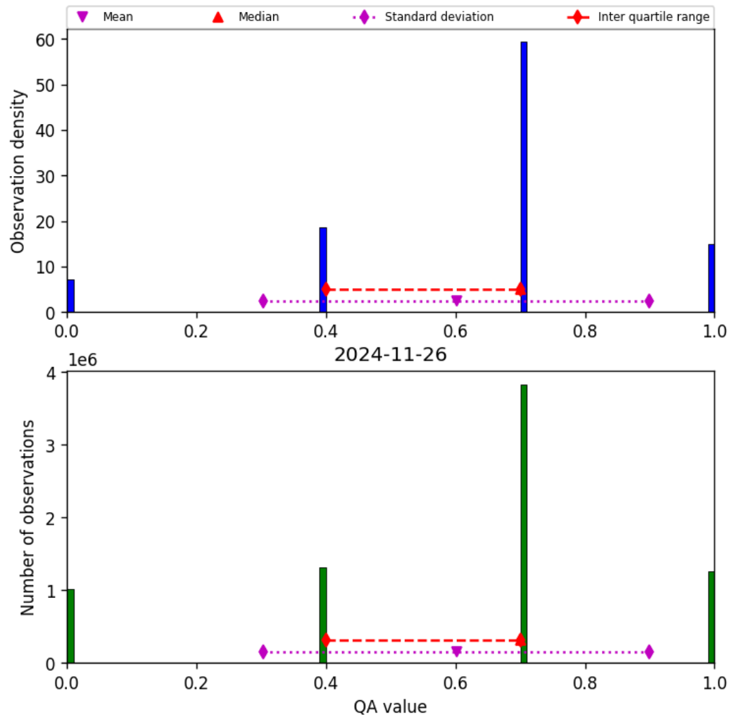
Figure 17: Histogram of “QA value” for 2024-11-25 to 2024-11-27
