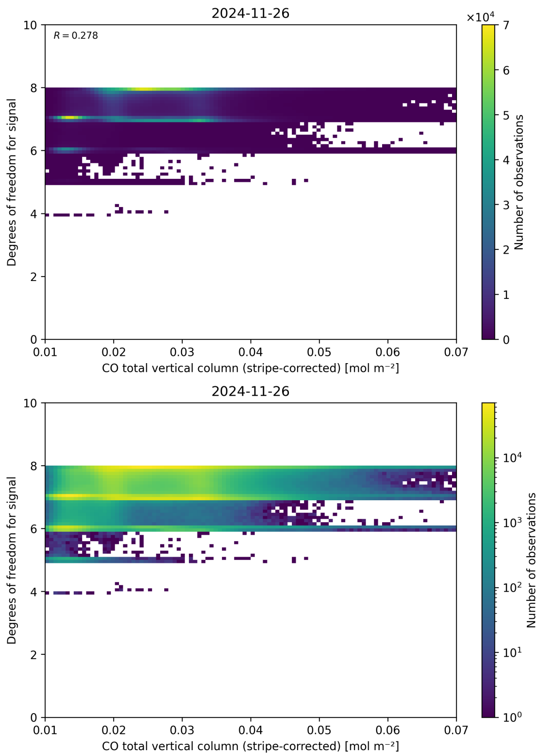
Figure 38: Scatter density plot of “CO total vertical column (stripe-corrected)” against “Degrees of freedom for signal” for 2024-11-25 to 2024-11-27.
