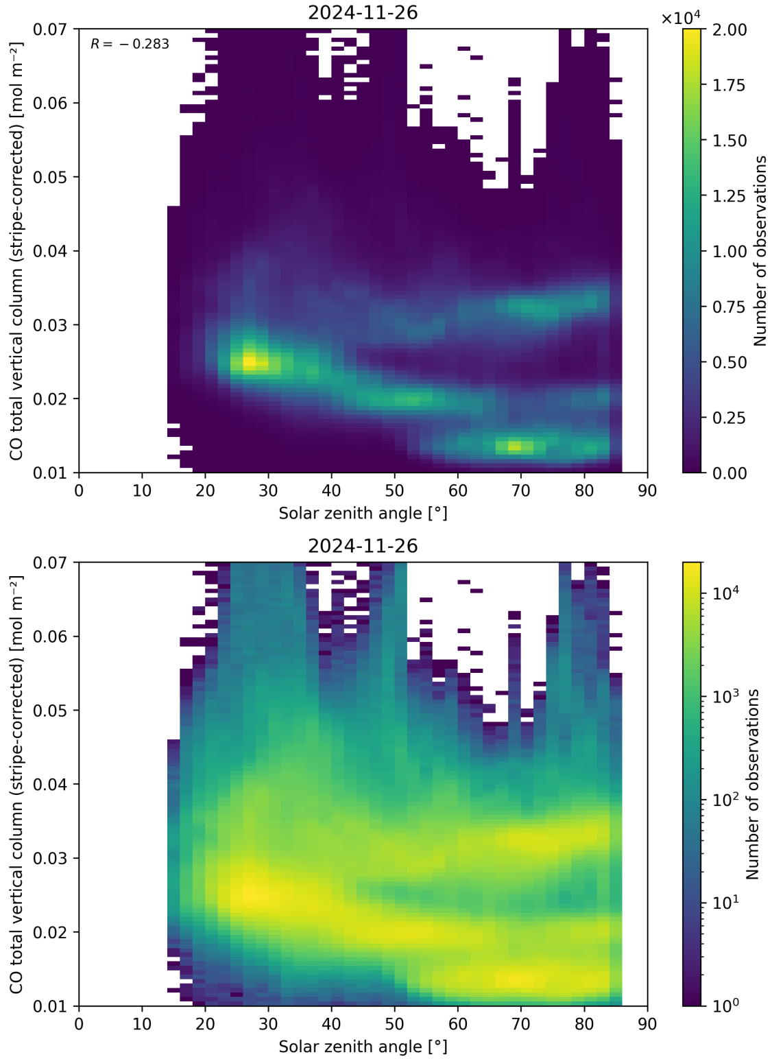
Figure 62: Scatter density plot of “Solar zenith angle” against “CO total vertical column (stripe-corrected)” for 2024-11-25 to 2024-11-27.
