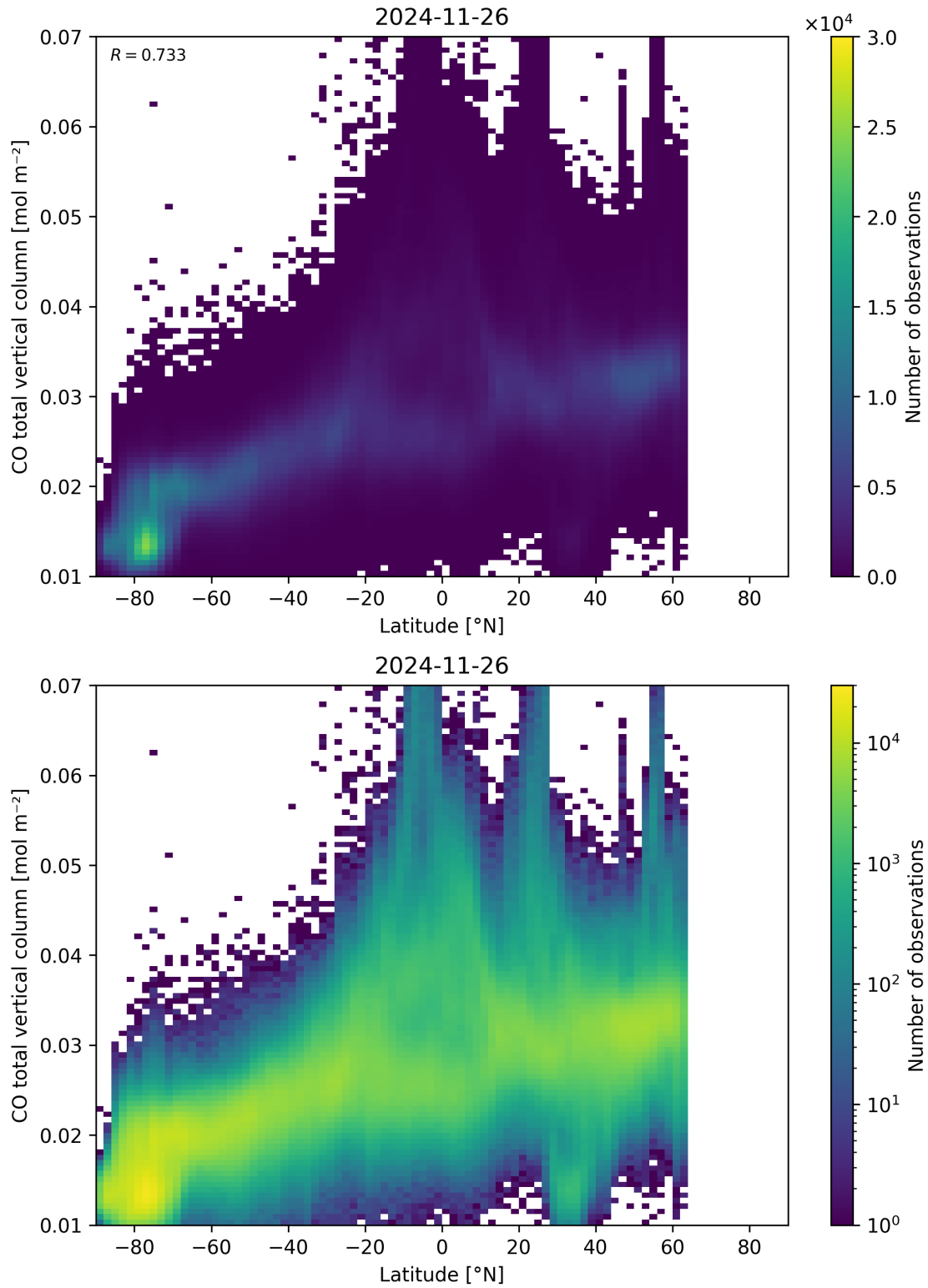
Figure 51: Scatter density plot of “Latitude” against “CO total vertical column” for 2024-11-25 to 2024-11-27.
