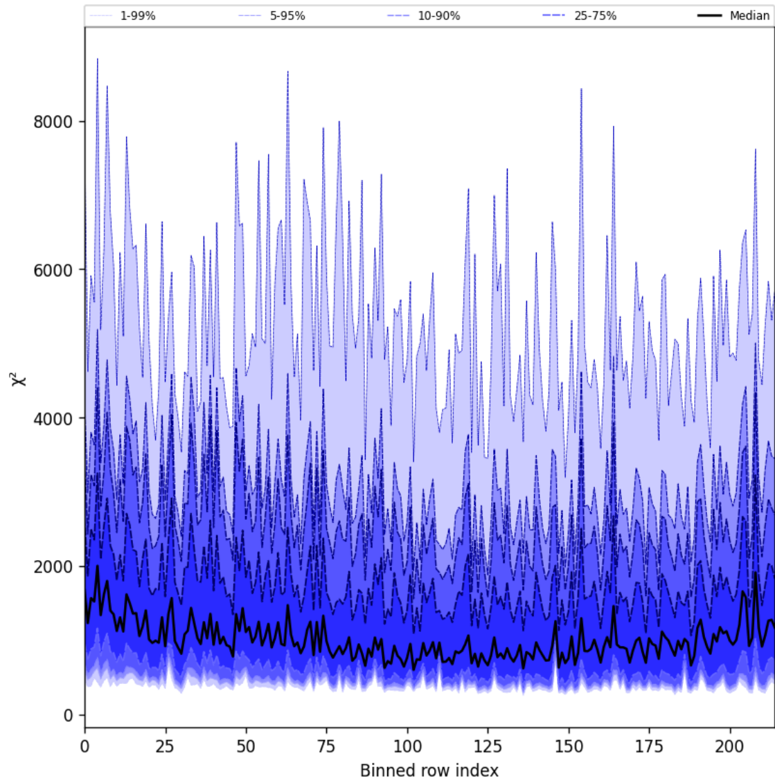
Figure 30: Along track statistics of “ \chi^2 ” for 2024-11-25 to 2024-11-27
