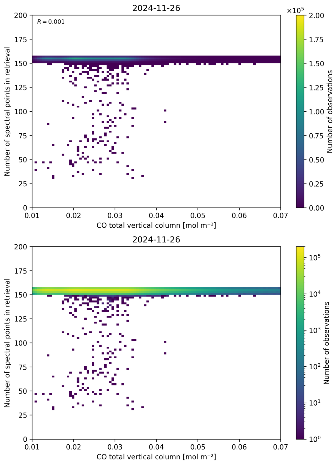
Figure 43: Scatter density plot of “CO total vertical column” against “Number of spectral points in retrieval” for 2024-11-25 to 2024-11-27.
