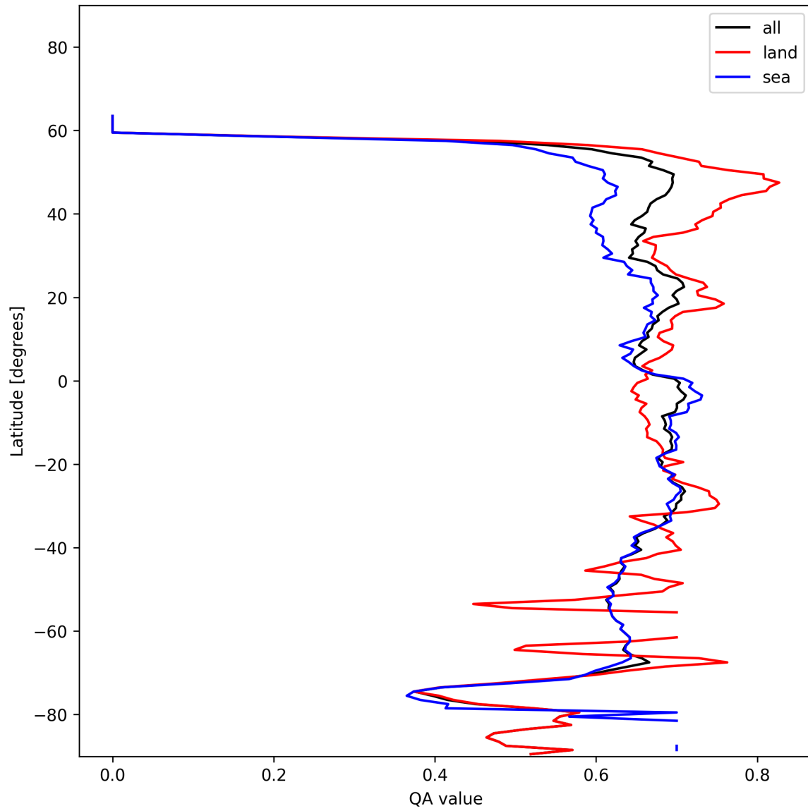
Figure 9: Zonal average of “QA value” for 2024-11-25 to 2024-11-27.
