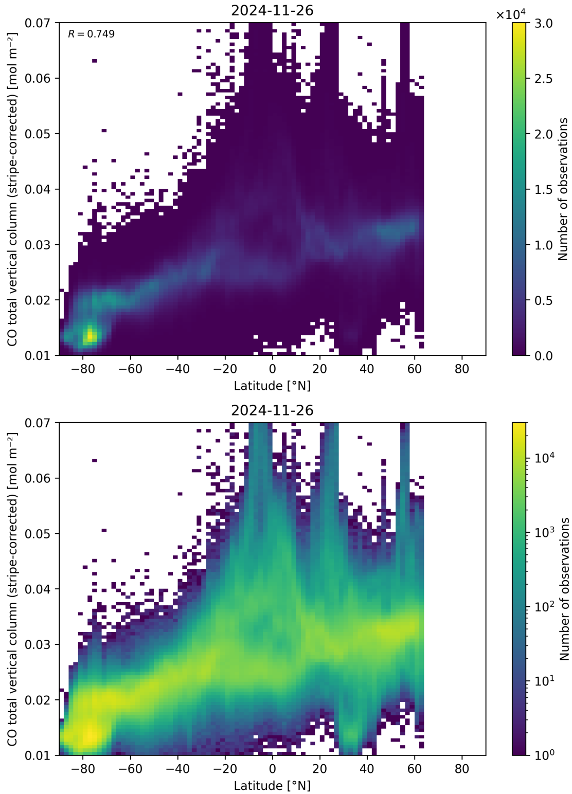
Figure 52: Scatter density plot of “Latitude” against “CO total vertical column (stripe-corrected)” for 2024-11-25 to 2024-11-27.
