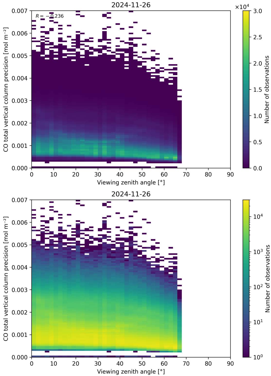
Figure 71: Scatter density plot of “Viewing zenith angle” against “CO total vertical column precision” for 2024-11-25 to 2024-11-27.
