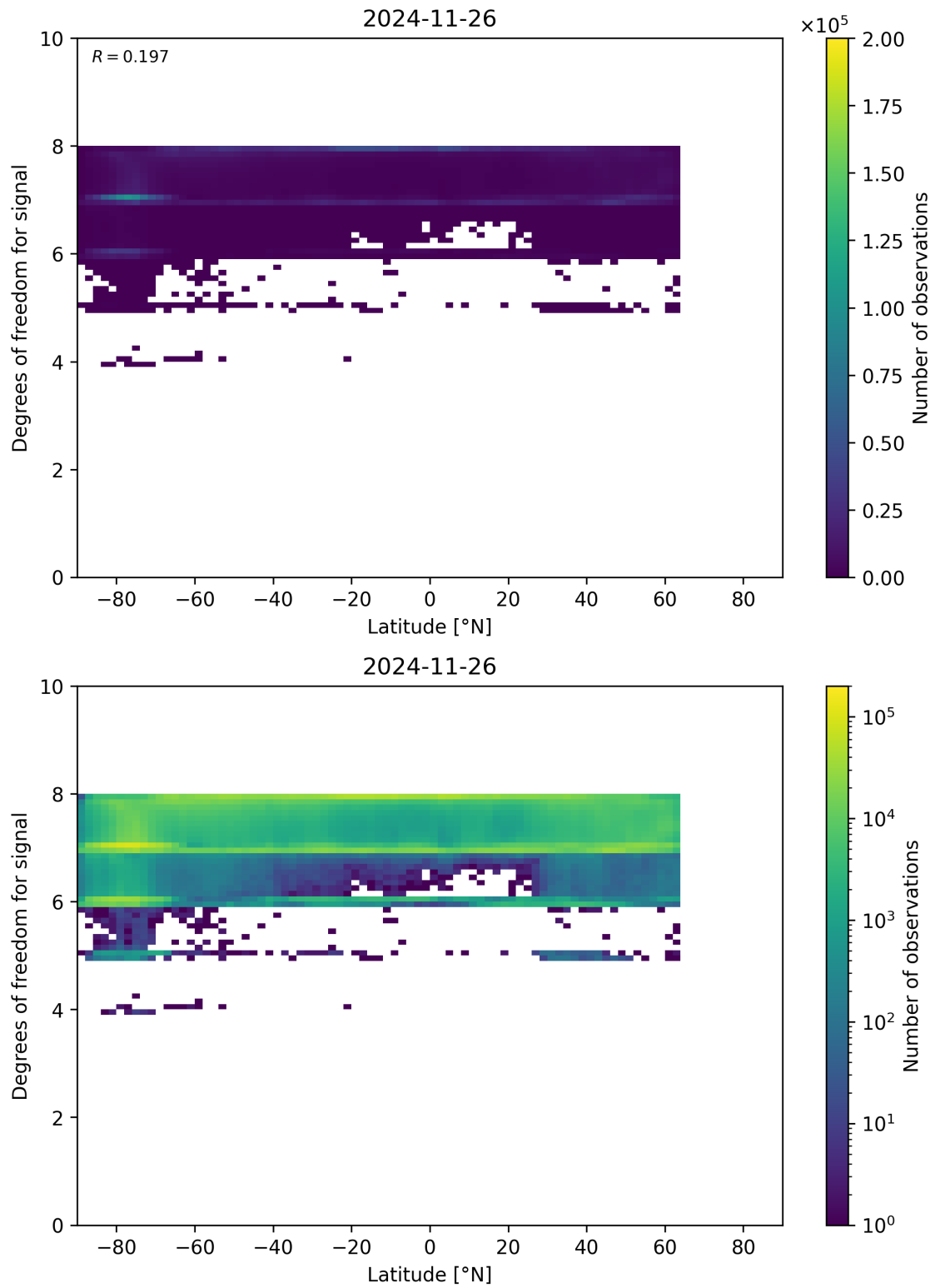
Figure 55: Scatter density plot of “Latitude” against “Degrees of freedom for signal” for 2024-11-25 to 2024-11-27.
