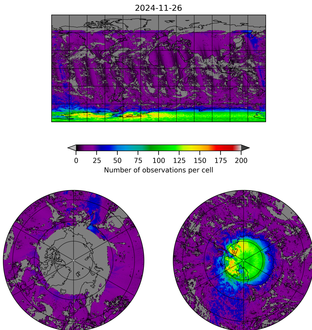
Figure 8: Map of the number of observations for 2024-11-25 to 2024-11-27
