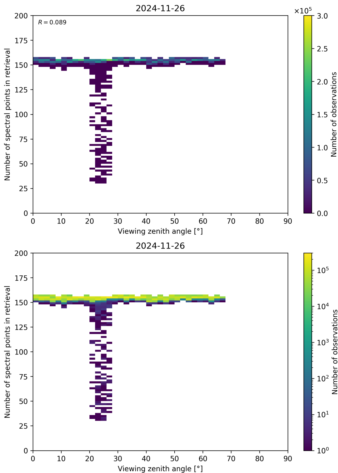
Figure 76: Scatter density plot of “Viewing zenith angle” against “Number of spectral points in retrieval” for 2024-11-25 to 2024-11-27.
