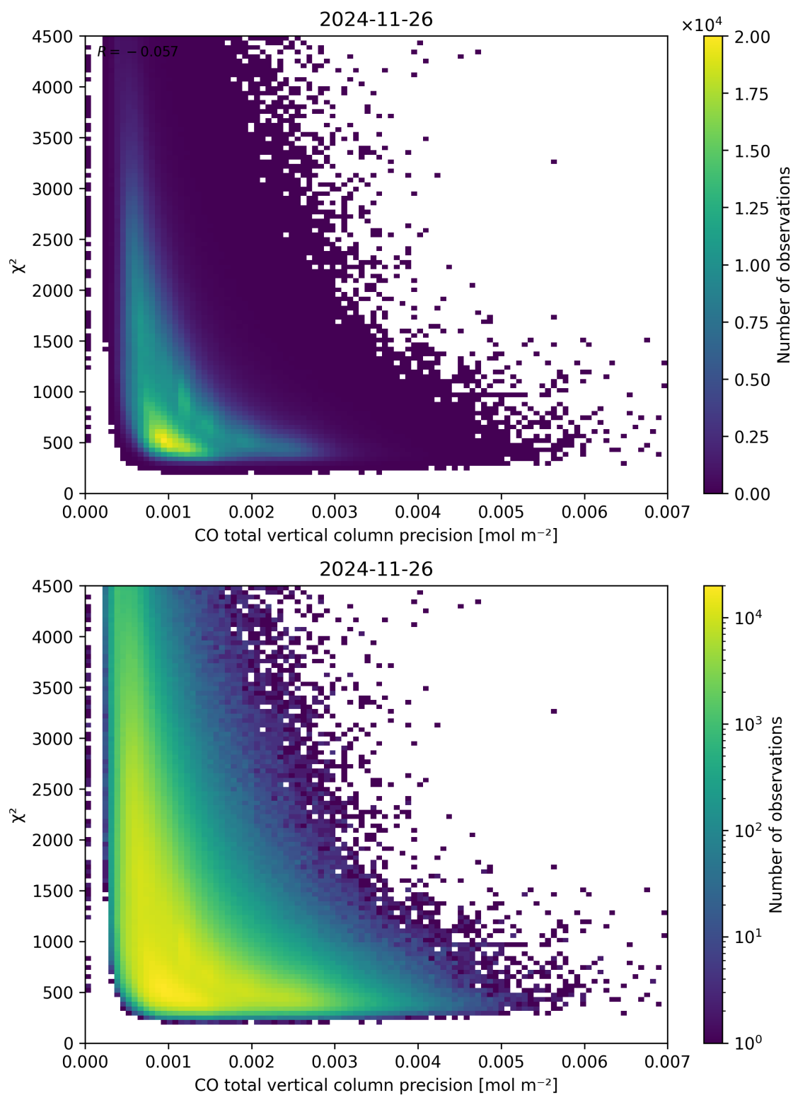
Figure 44: Scatter density plot of “CO total vertical column precision” against “ \chi^2 ” for 2024-11-25 to 2024-11-27.
