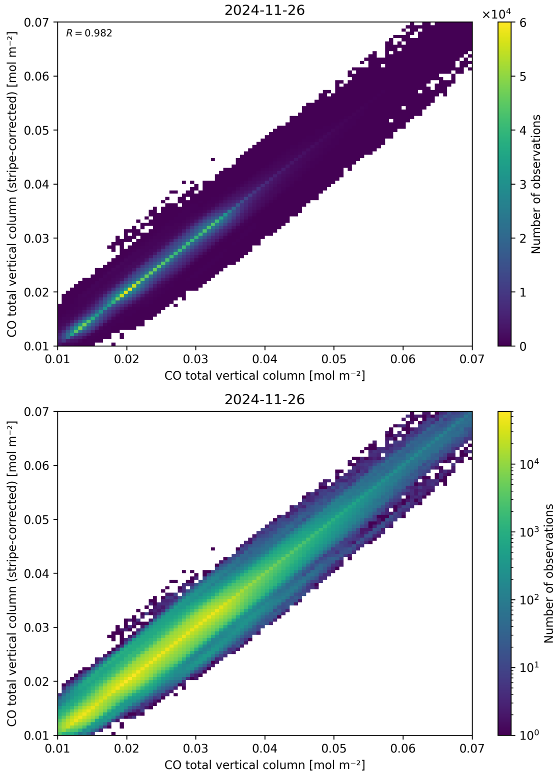
Figure 33: Scatter density plot of “CO total vertical column” against “CO total vertical column (stripe-corrected)” for 2024-11-25 to 2024-11-27.
