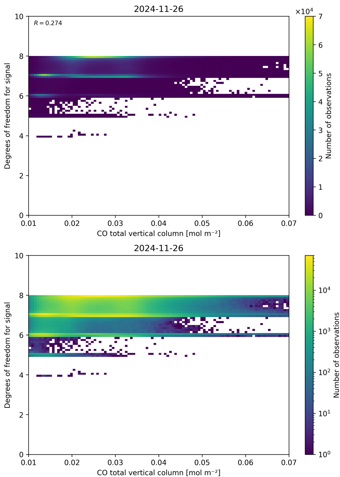
Figure 41: Scatter density plot of “CO total vertical column” against “Degrees of freedom for signal” for 2024-11-25 to 2024-11-27.
