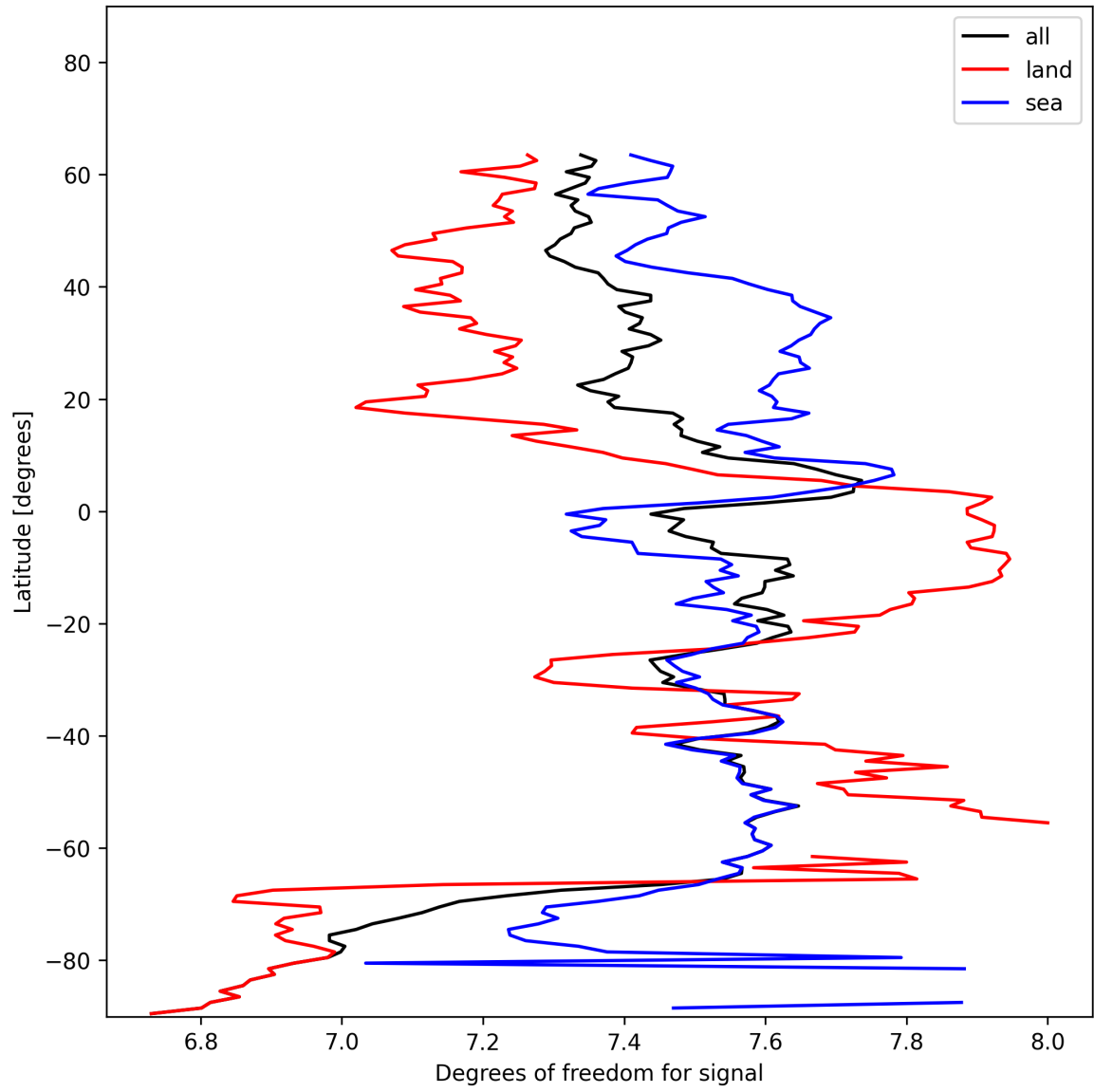
Figure 15: Zonal average of “Degrees of freedom for signal” for 2024-11-25 to 2024-11-27.
