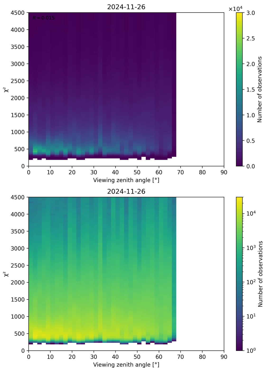
Figure 72: Scatter density plot of “Viewing zenith angle” against “ \chi^2 ” for 2024-11-25 to 2024-11-27.
