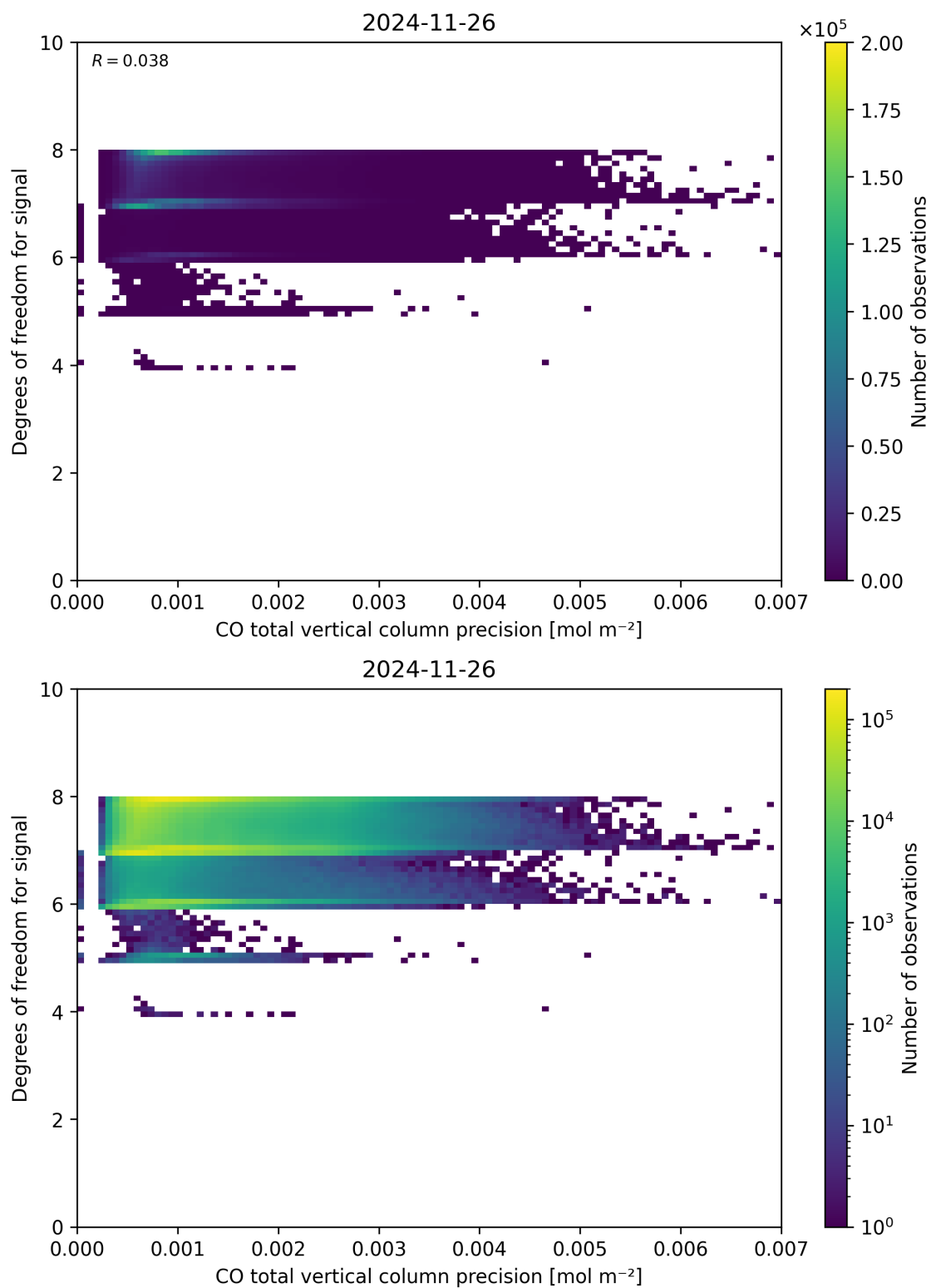
Figure 45: Scatter density plot of “CO total vertical column precision” against “Degrees of freedom for signal” for 2024-11-25 to 2024-11-27.
