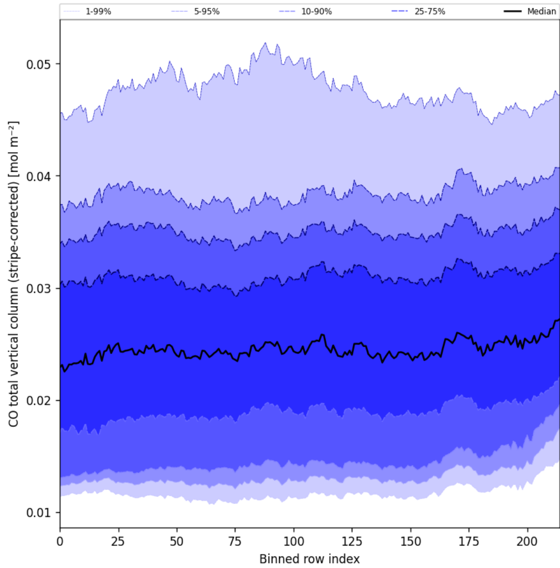
Figure 27: Along track statistics of “CO total vertical column (stripe-corrected)” for 2024-11-25 to 2024-11-27
