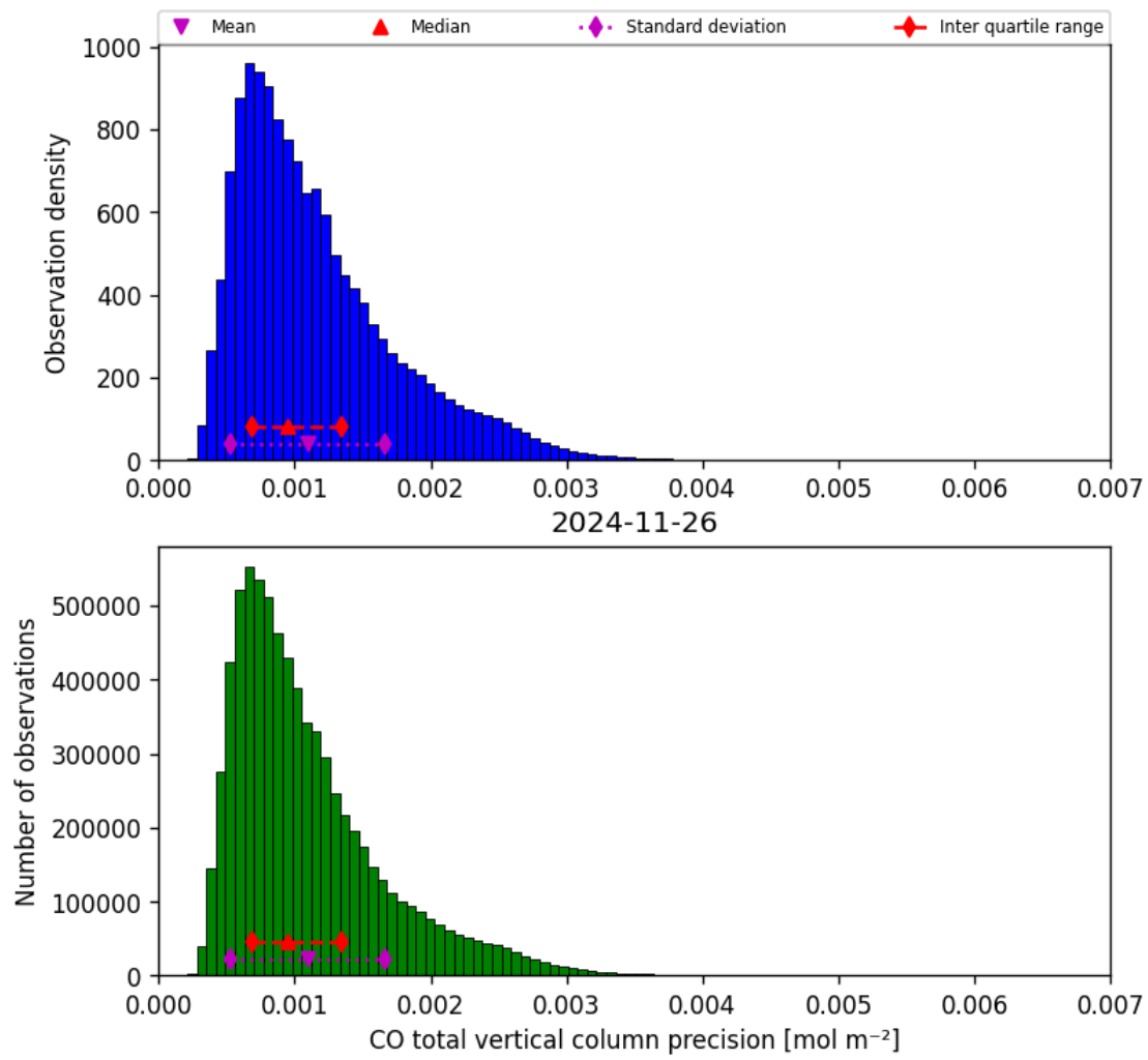
Figure 20: Histogram of “CO total vertical column precision” for 2024-11-25 to 2024-11-27
