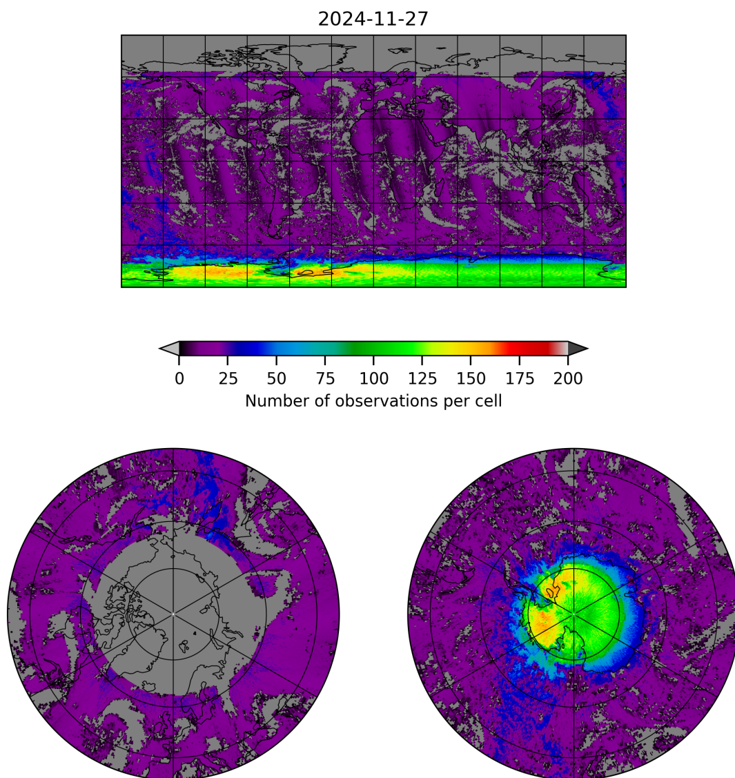
Figure 8: Map of the number of observations for 2024-11-26 to 2024-11-28
