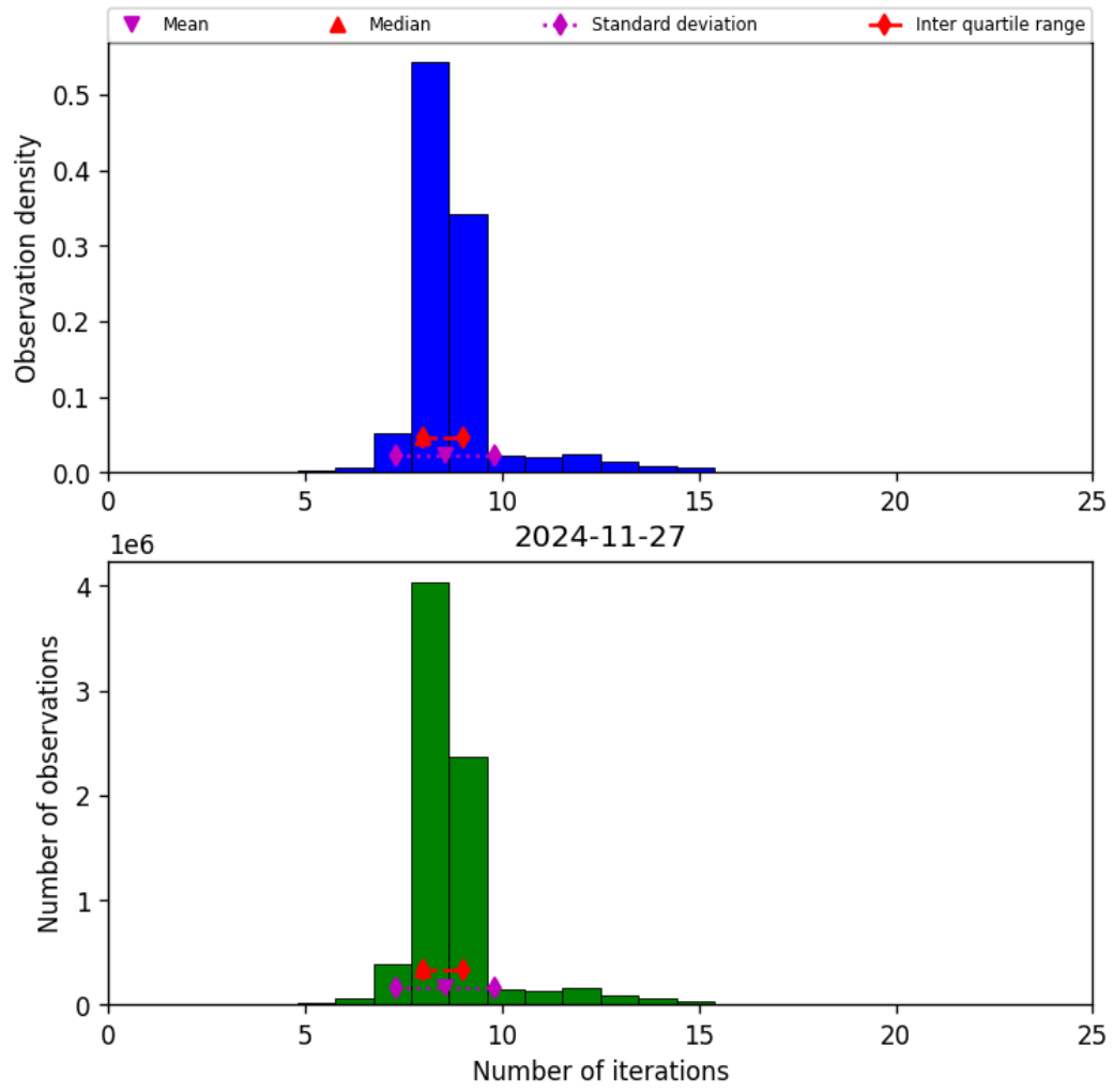
Figure 24: Histogram of “Number of iterations” for 2024-11-26 to 2024-11-28
