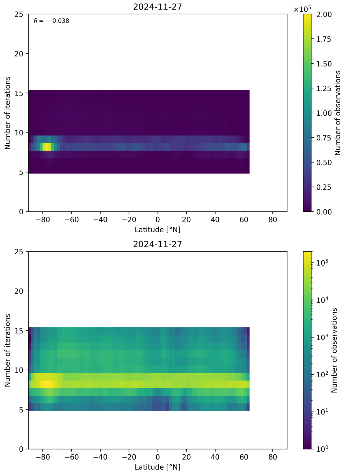
Figure 56: Scatter density plot of “Latitude” against “Number of iterations” for 2024-11-26 to 2024-11-28.
