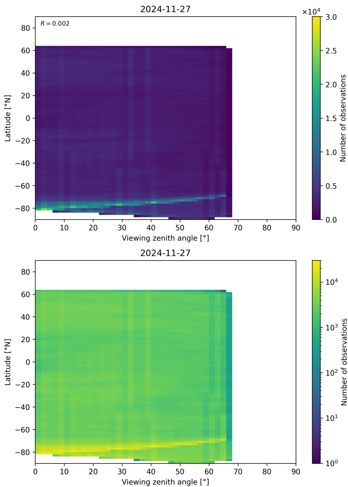
Figure 74: Scatter density plot of “Viewing zenith angle” against “Latitude” for 2024-11-26 to 2024-11-28.
