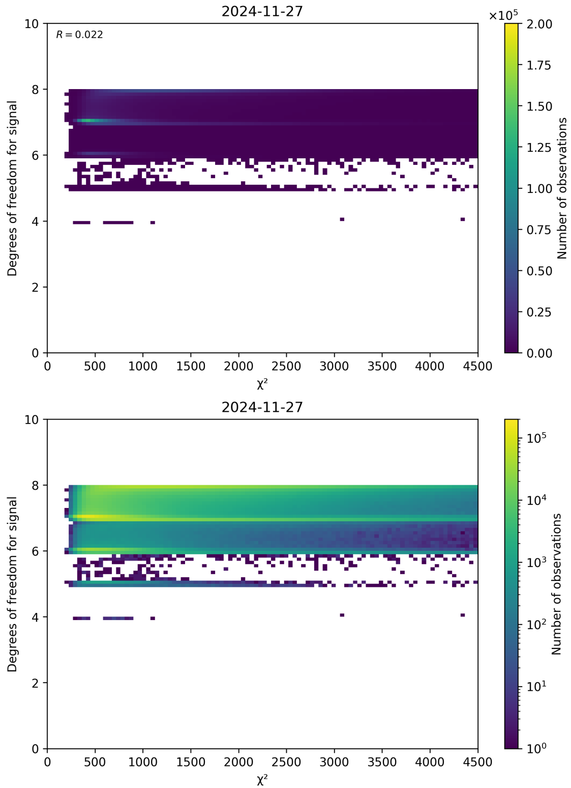
Figure 48: Scatter density plot of “ \chi^2 ” against “Degrees of freedom for signal” for 2024-11-26 to 2024-11-28.
