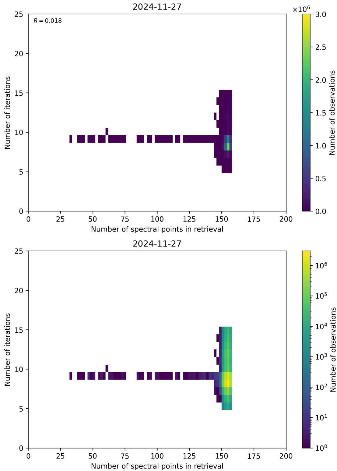
Figure 60: Scatter density plot of “Number of spectral points in retrieval” against “Number of iterations” for 2024-11-26 to 2024-11-28.
