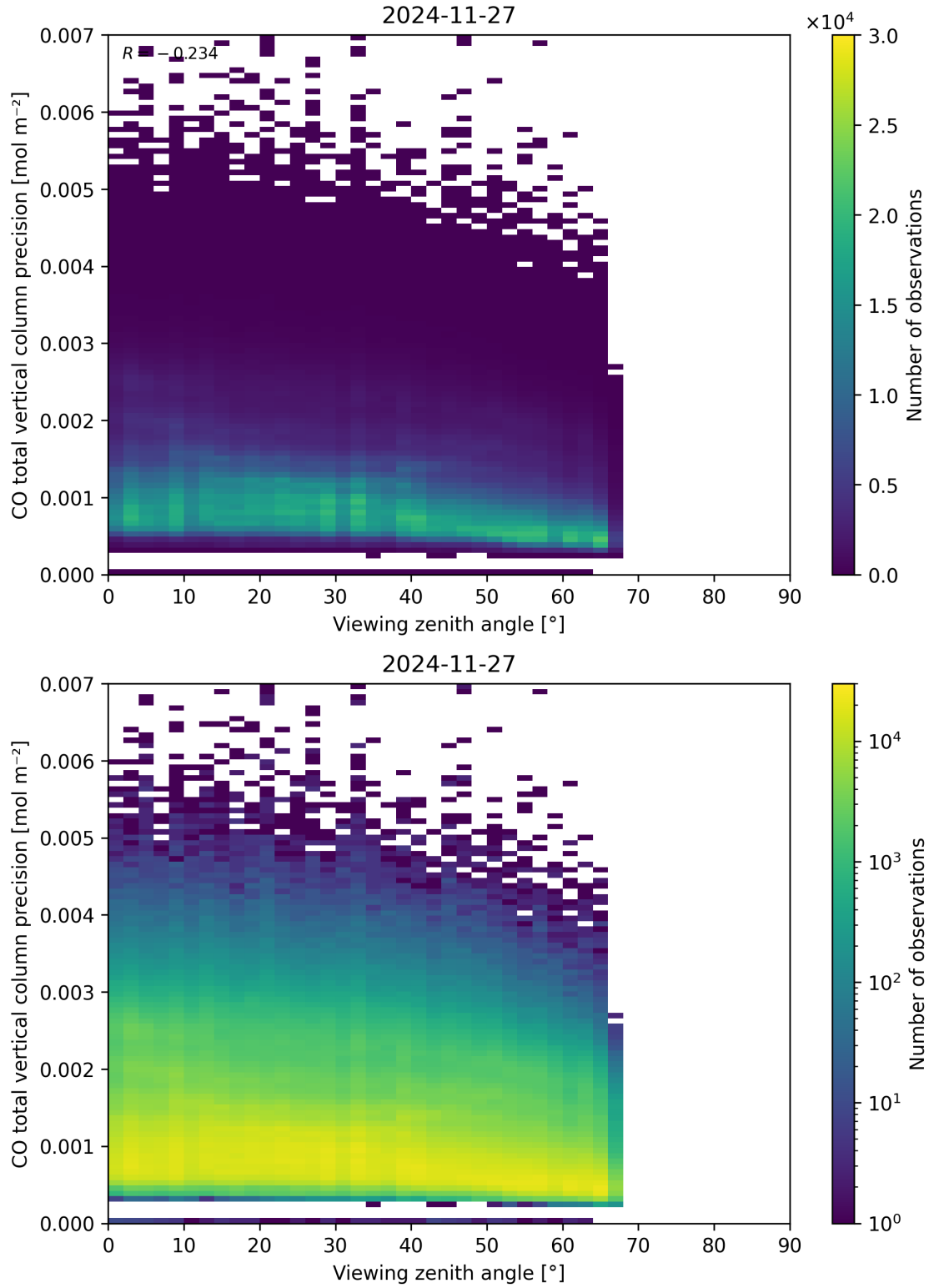
Figure 71: Scatter density plot of “Viewing zenith angle” against “CO total vertical column precision” for 2024-11-26 to 2024-11-28.
