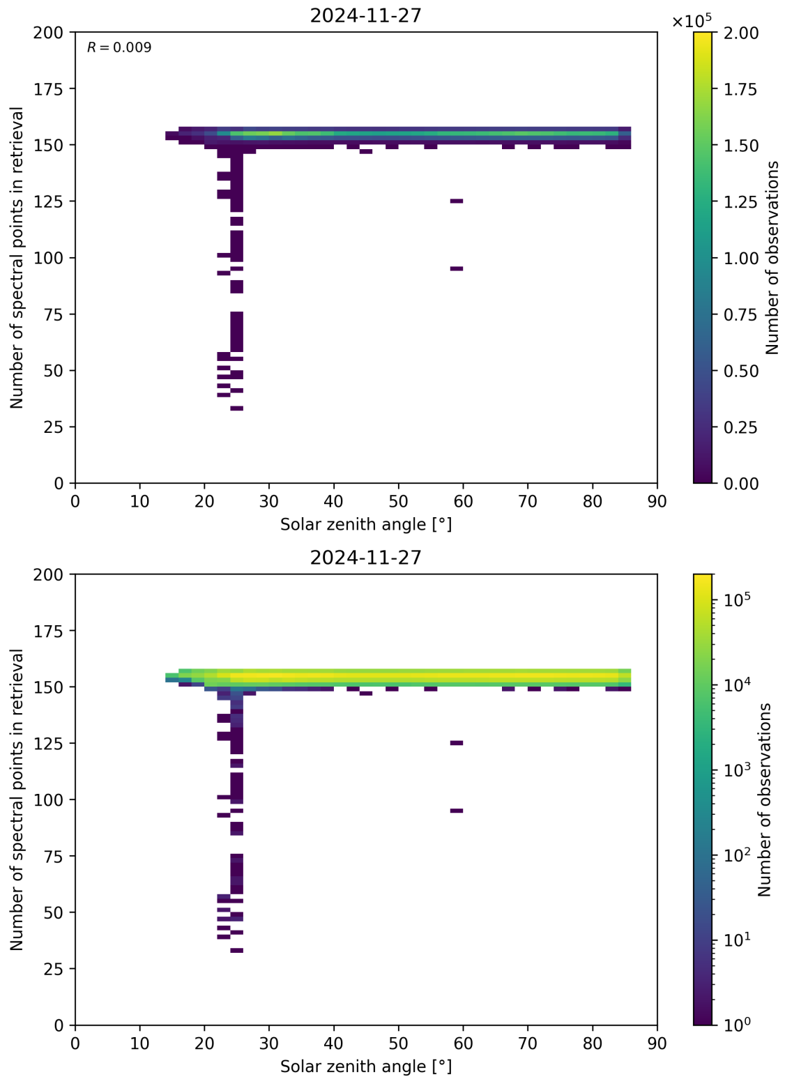
Figure 68: Scatter density plot of “Solar zenith angle” against “Number of spectral points in retrieval” for 2024-11-26 to 2024-11-28.
