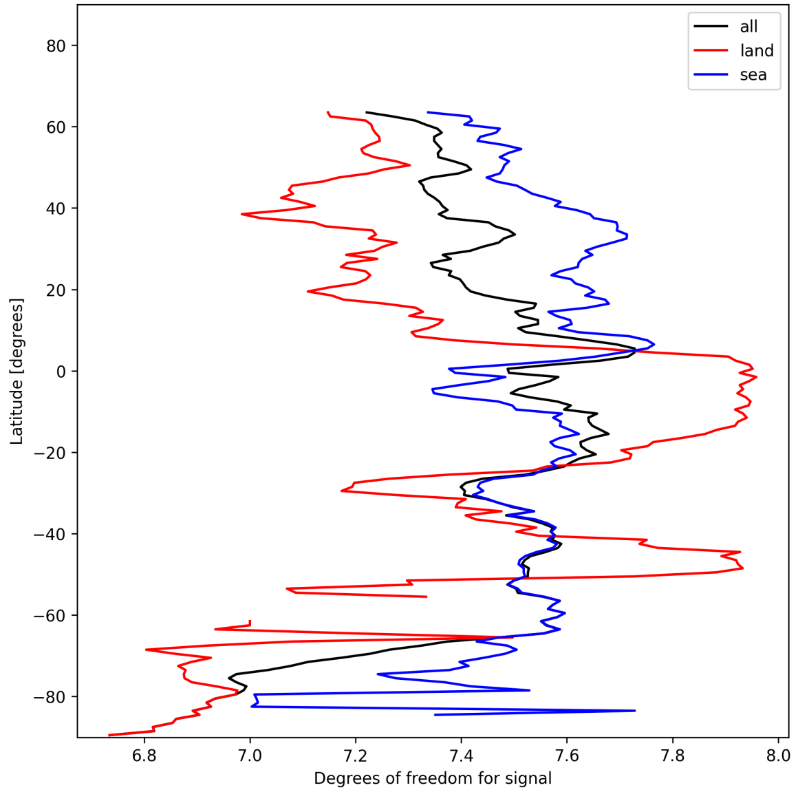
Figure 15: Zonal average of “Degrees of freedom for signal” for 2024-11-26 to 2024-11-28.
