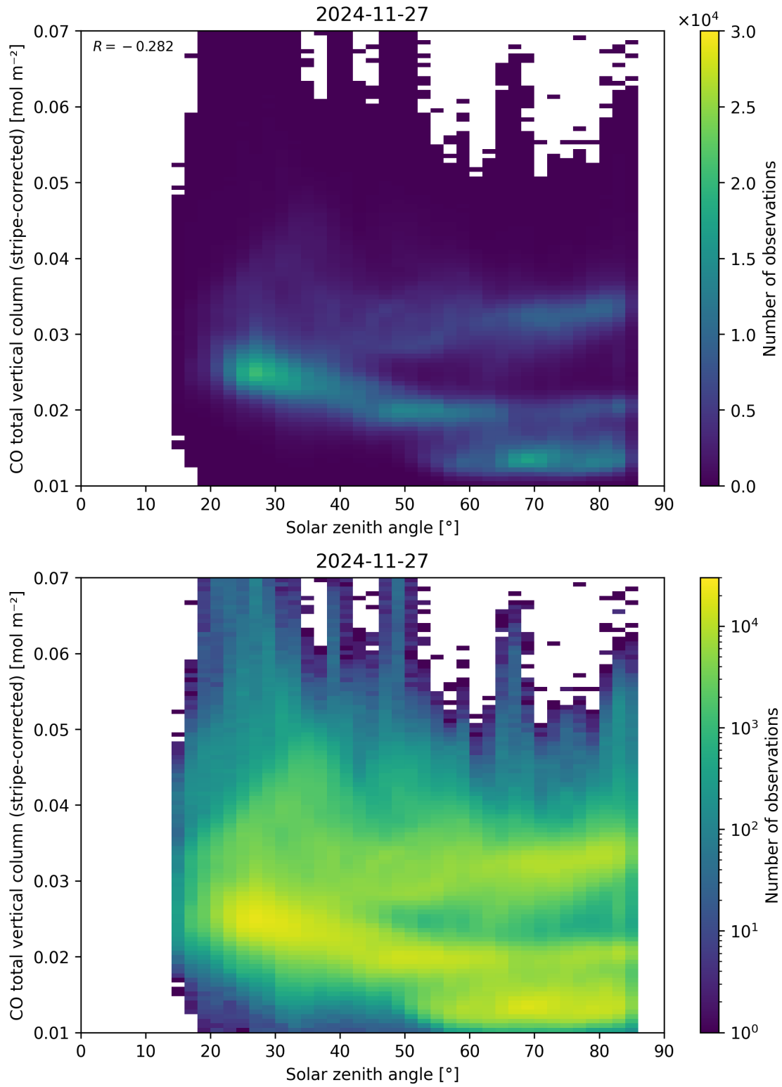
Figure 62: Scatter density plot of “Solar zenith angle” against “CO total vertical column (stripe-corrected)” for 2024-11-26 to 2024-11-28.
