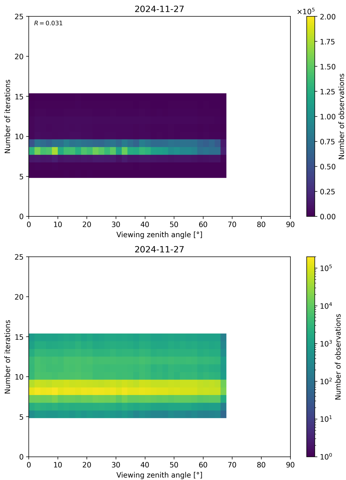
Figure 75: Scatter density plot of “Viewing zenith angle” against “Number of iterations” for 2024-11-26 to 2024-11-28.
