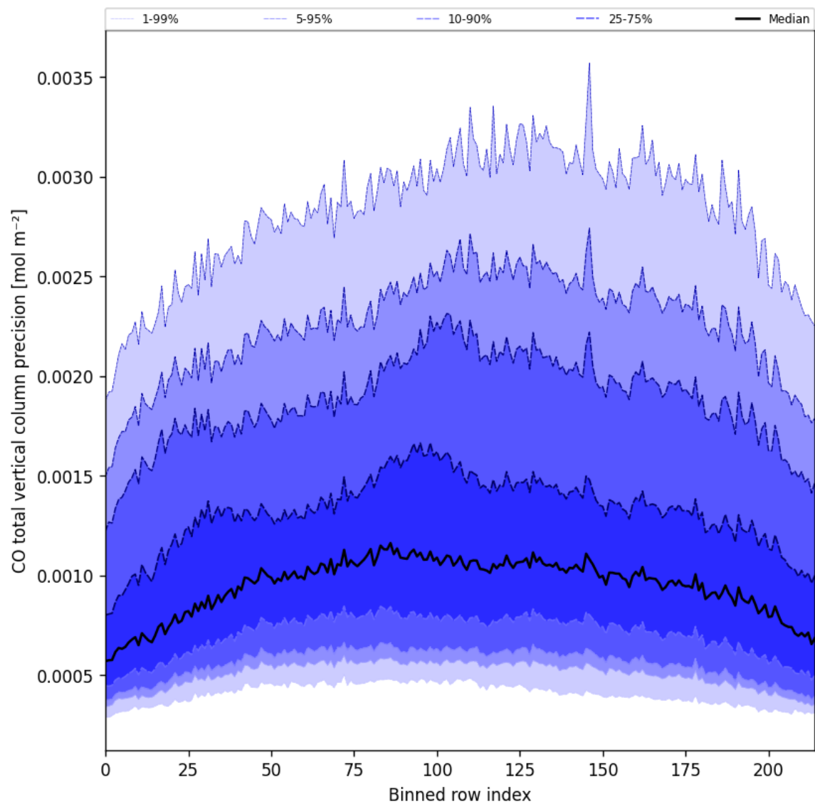
Figure 28: Along track statistics of “CO total vertical column precision” for 2024-11-26 to 2024-11-28
