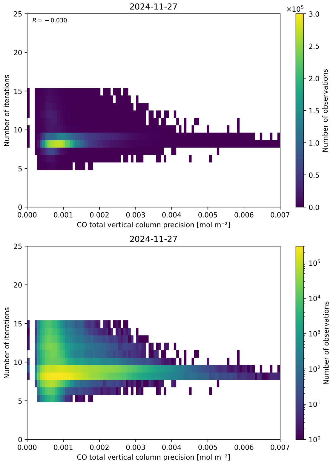
Figure 46: Scatter density plot of “CO total vertical column precision” against “Number of iterations” for 2024-11-26 to 2024-11-28.
