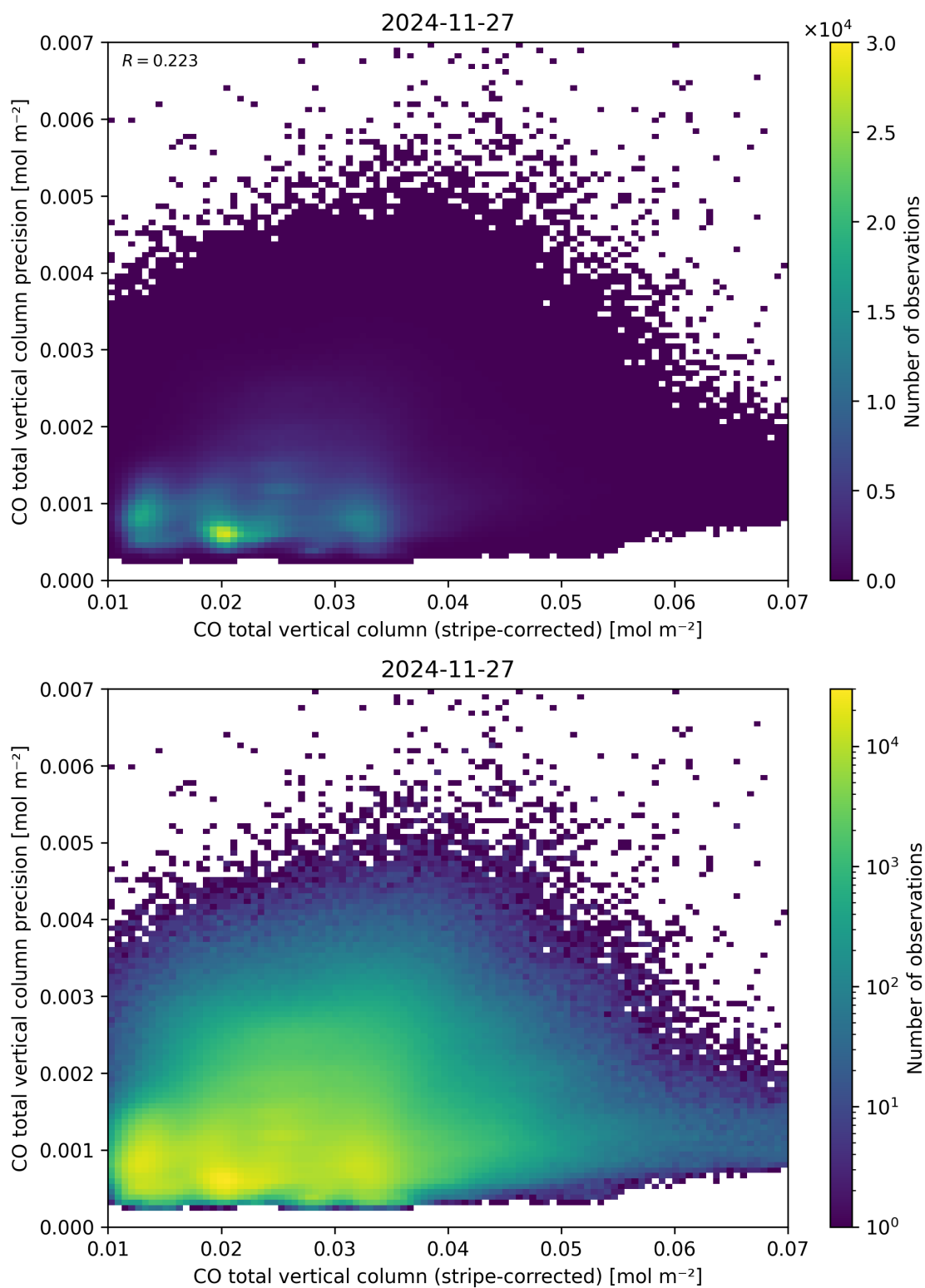
Figure 36: Scatter density plot of “CO total vertical column (stripe-corrected)” against “CO total vertical column precision” for 2024-11-26 to 2024-11-28.
