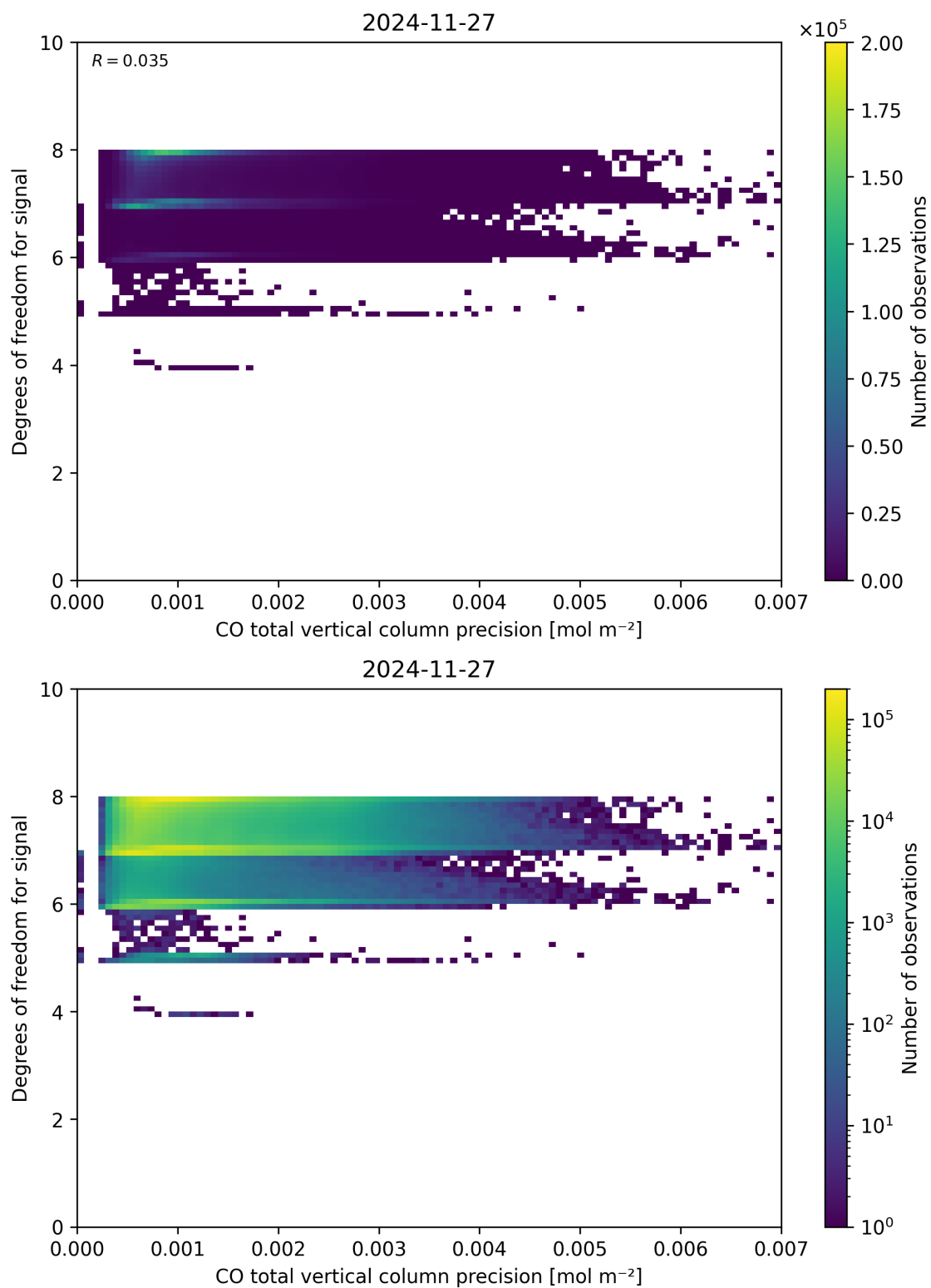
Figure 45: Scatter density plot of “CO total vertical column precision” against “Degrees of freedom for signal” for 2024-11-26 to 2024-11-28.
