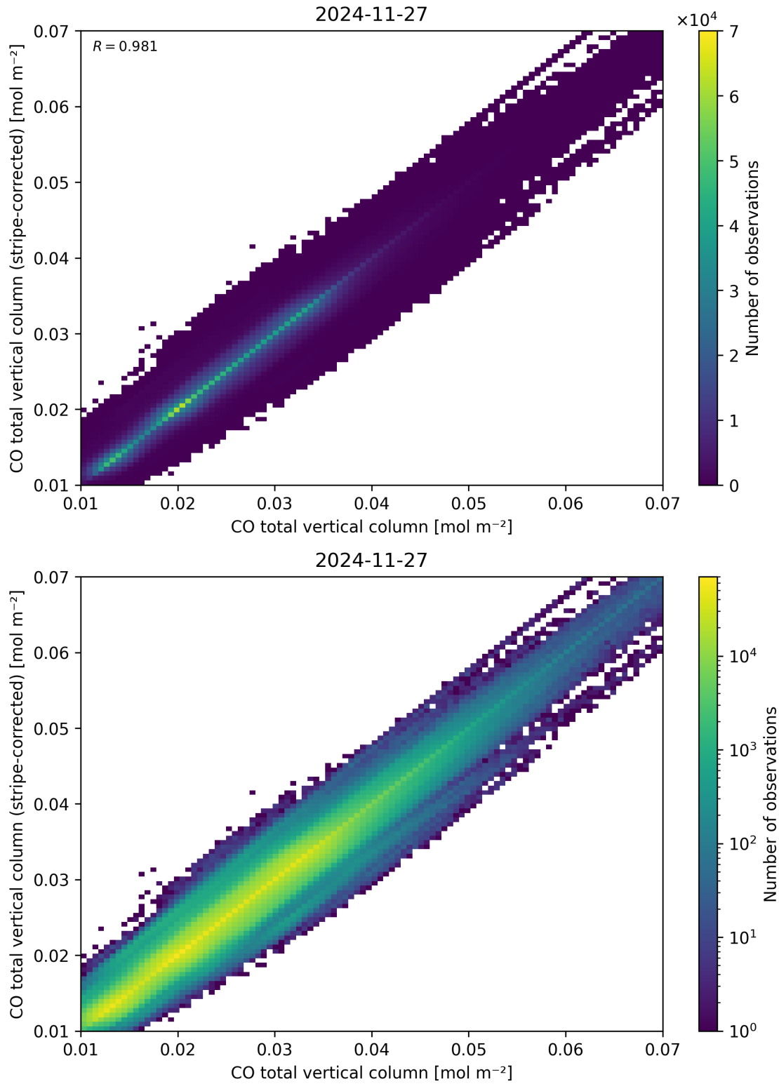
Figure 33: Scatter density plot of “CO total vertical column” against “CO total vertical column (stripe-corrected)” for 2024-11-26 to 2024-11-28.
