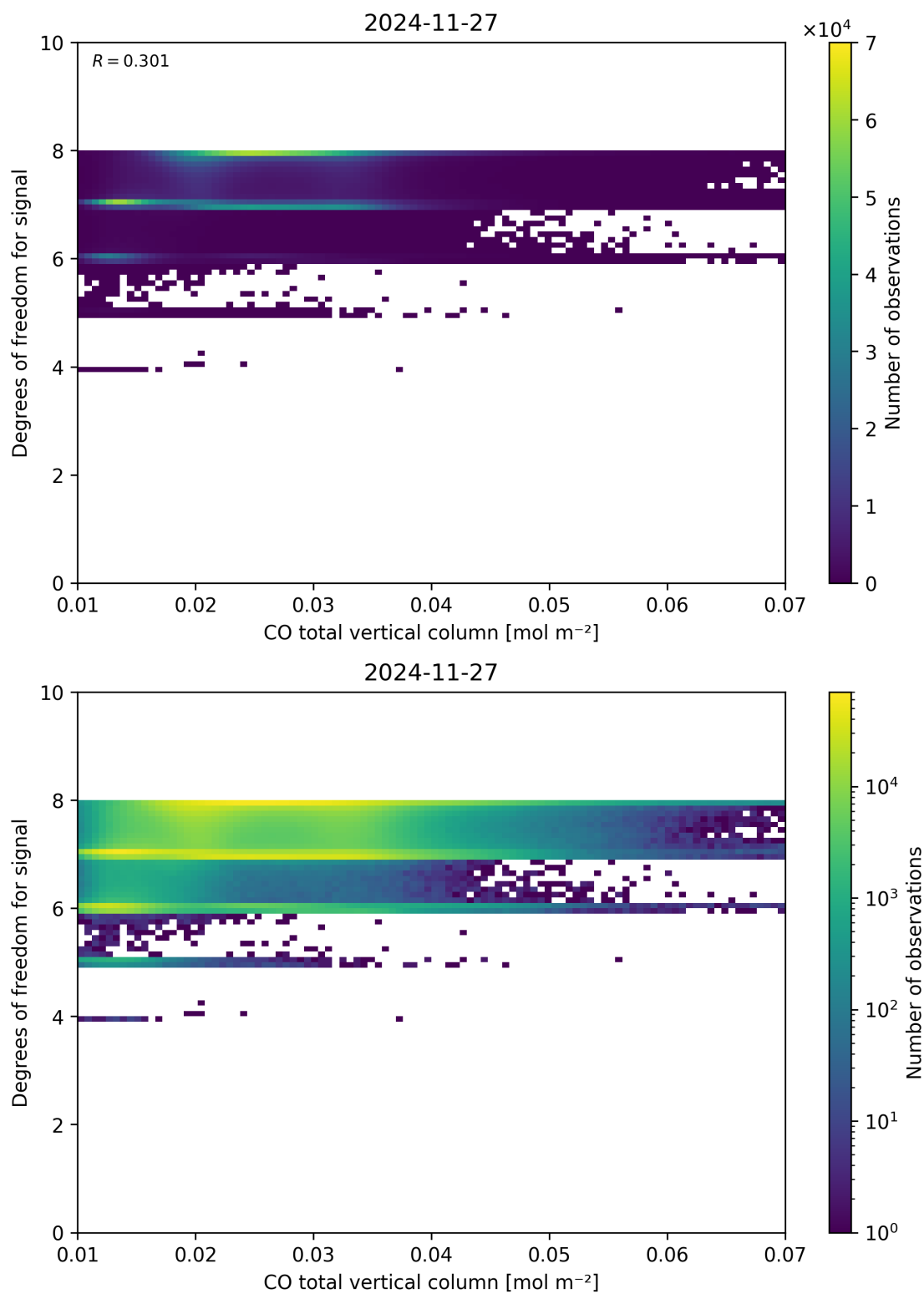
Figure 41: Scatter density plot of “CO total vertical column” against “Degrees of freedom for signal” for 2024-11-26 to 2024-11-28.
