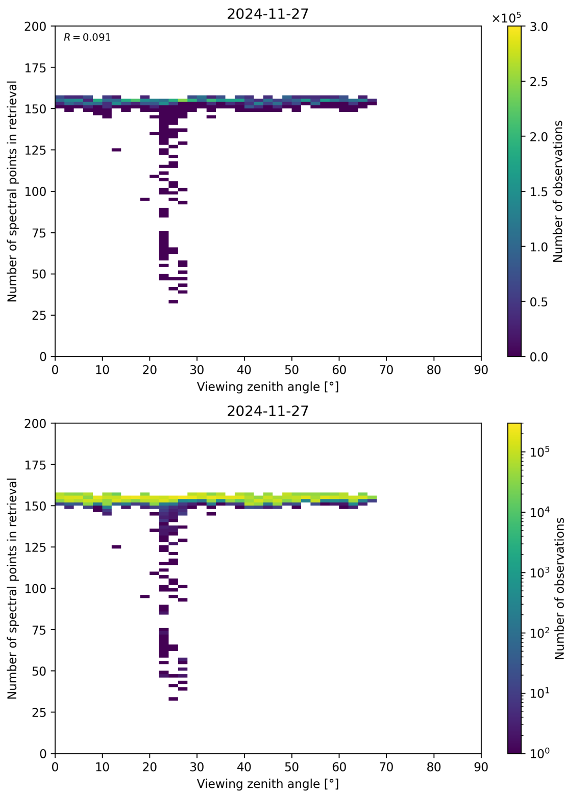
Figure 76: Scatter density plot of “Viewing zenith angle” against “Number of spectral points in retrieval” for 2024-11-26 to 2024-11-28.
