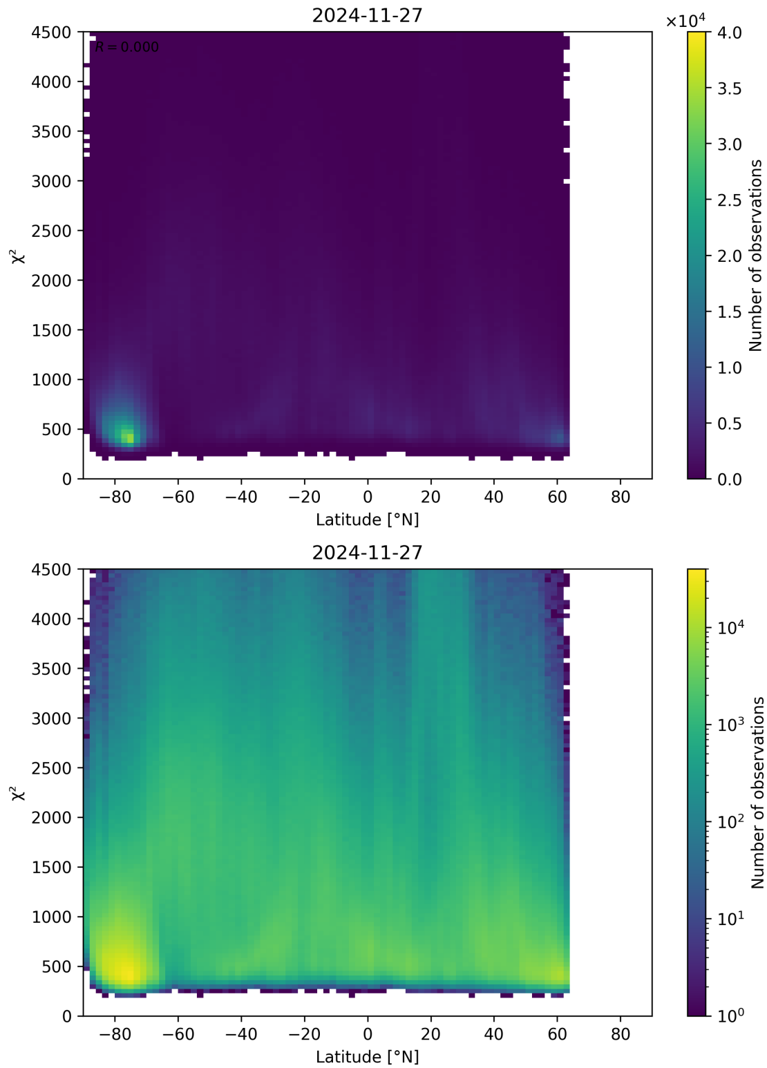
Figure 54: Scatter density plot of “Latitude” against “ \chi^2 ” for 2024-11-26 to 2024-11-28.
