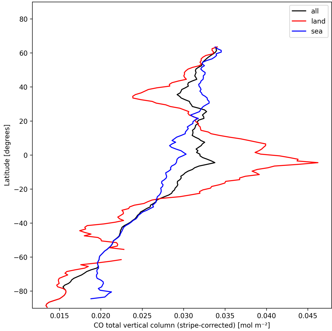
Figure 11: Zonal average of “CO total vertical column (stripe-corrected)” for 2024-11-26 to 2024-11-28.
