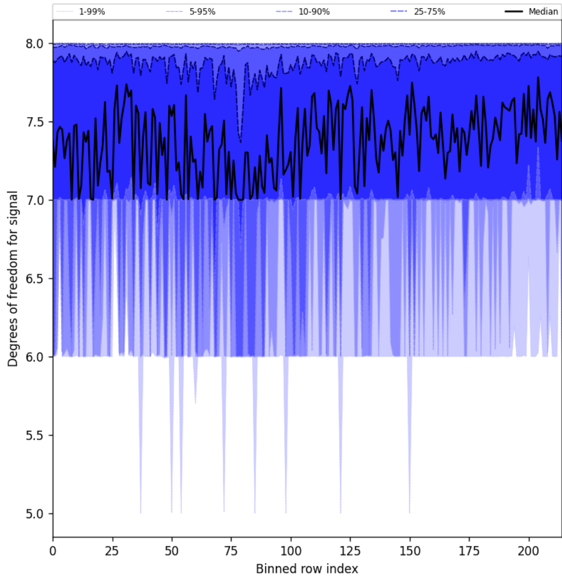
Figure 31: Along track statistics of “Degrees of freedom for signal” for 2024-11-26 to 2024-11-28
