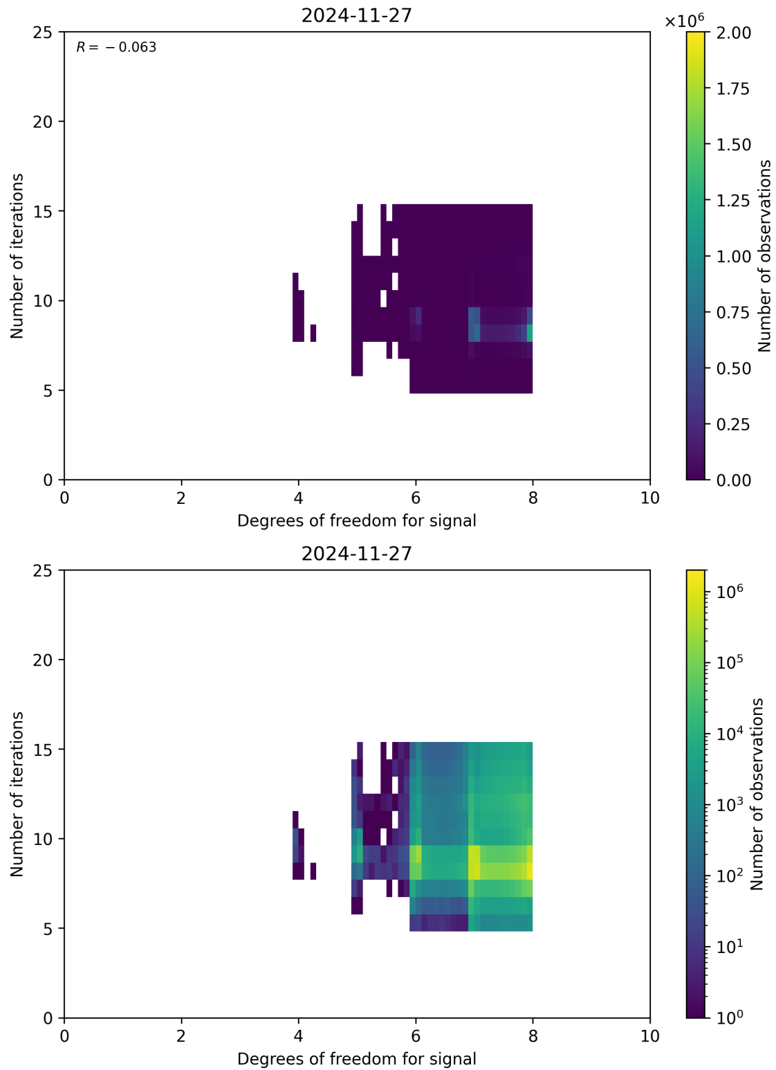
Figure 50: Scatter density plot of “Degrees of freedom for signal” against “Number of iterations” for 2024-11-26 to 2024-11-28.
