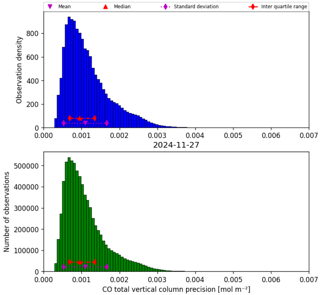
Figure 20: Histogram of “CO total vertical column precision” for 2024-11-26 to 2024-11-28
