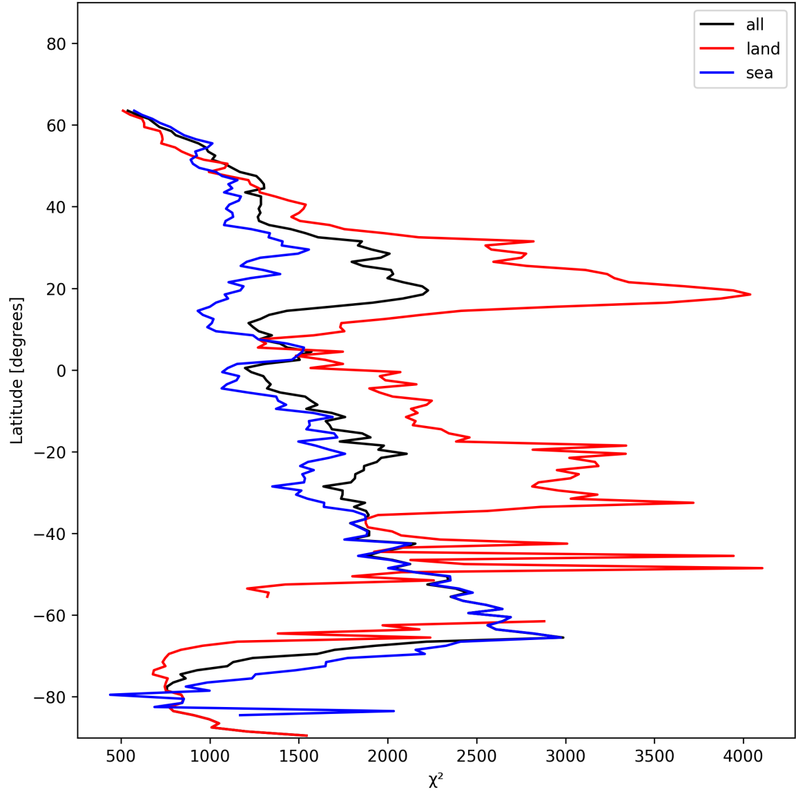
Figure 14: Zonal average of “ \chi^2 ” for 2024-11-26 to 2024-11-28.
