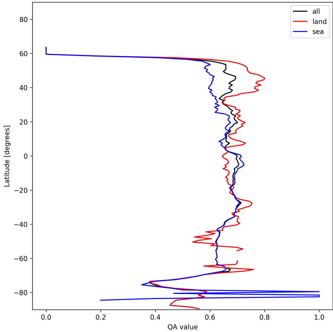
Figure 9: Zonal average of “QA value” for 2024-11-26 to 2024-11-28.
