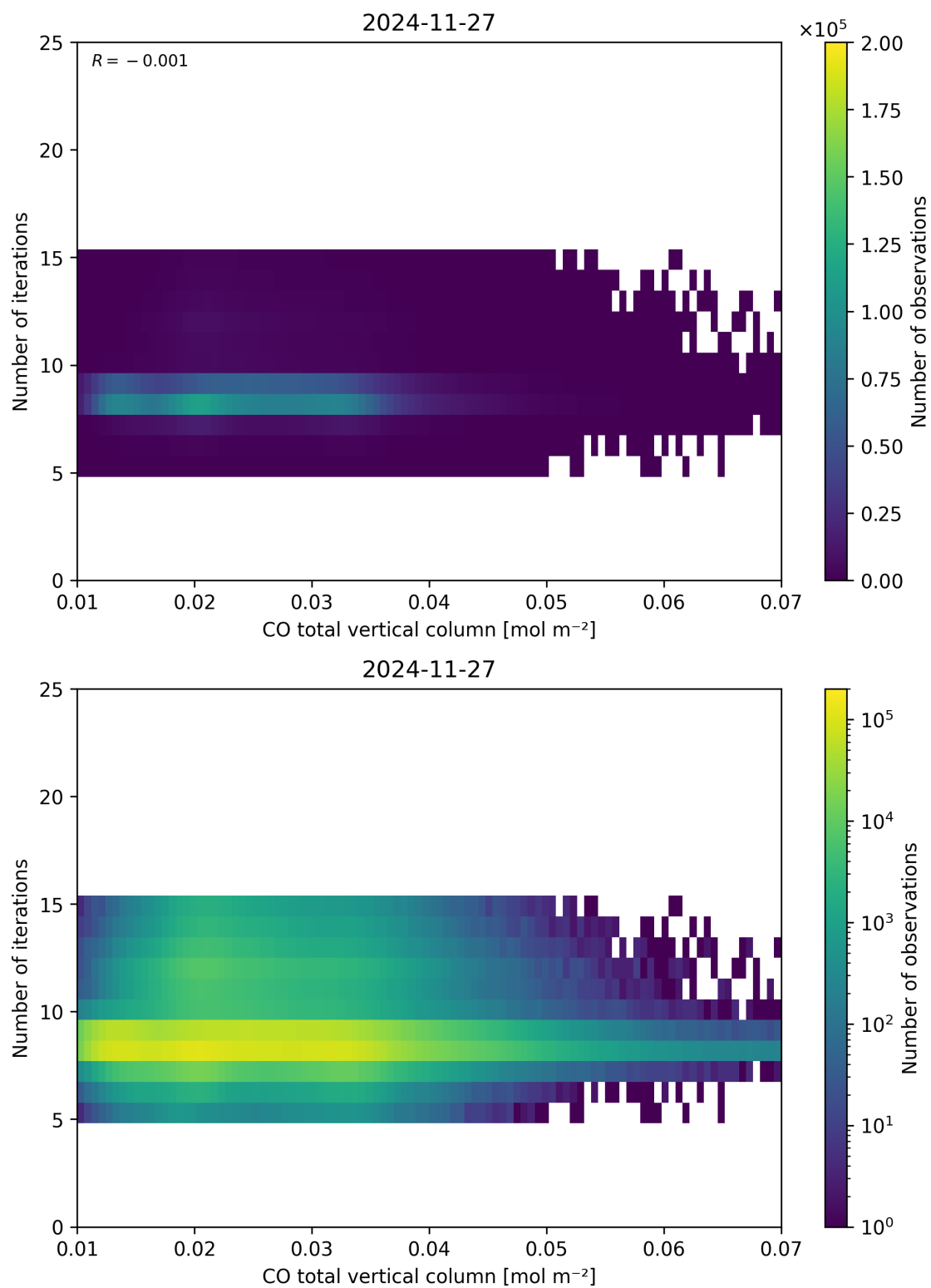
Figure 42: Scatter density plot of “CO total vertical column” against “Number of iterations” for 2024-11-26 to 2024-11-28.
