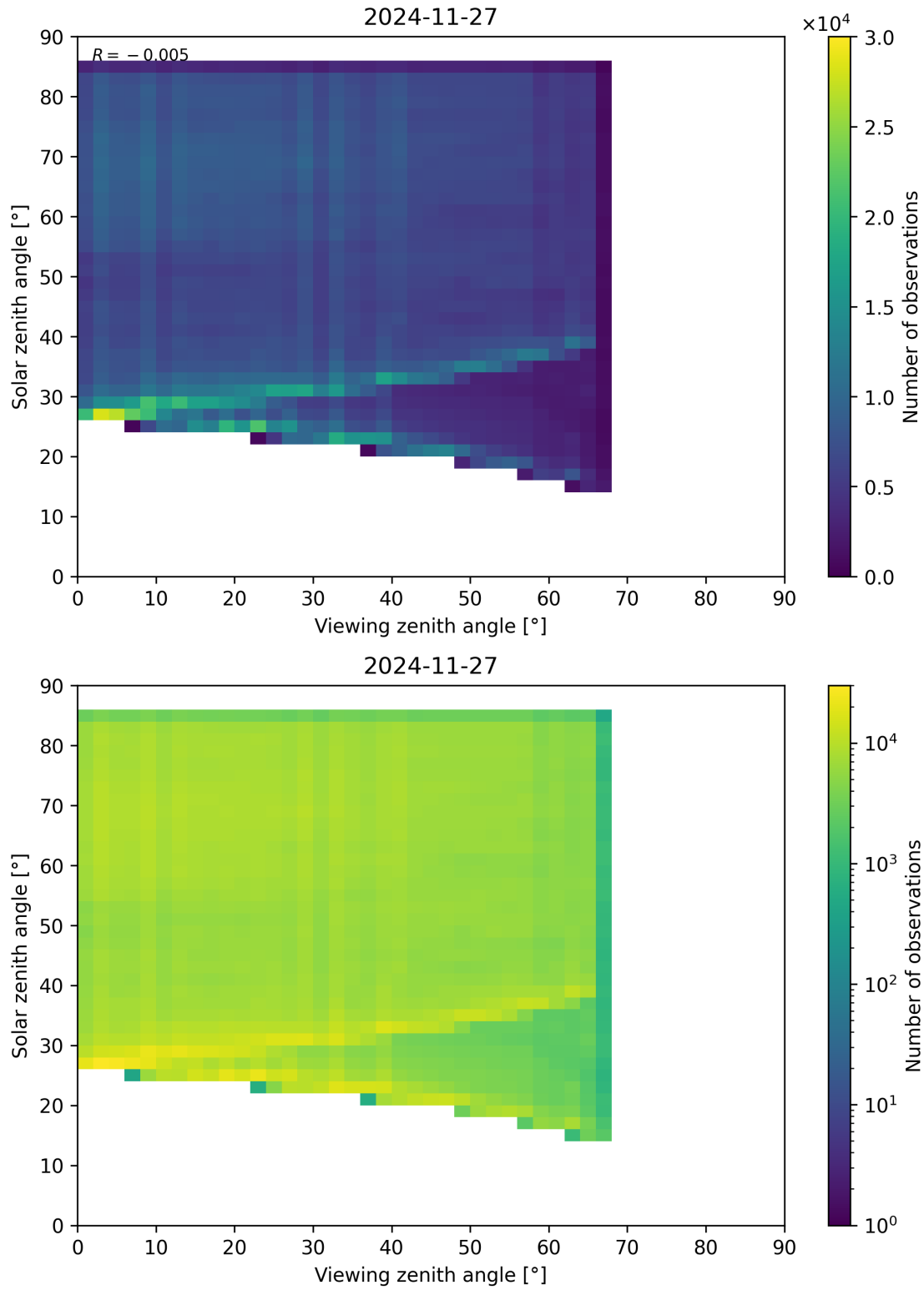
Figure 77: Scatter density plot of “Viewing zenith angle” against “Solar zenith angle” for 2024-11-26 to 2024-11-28.
