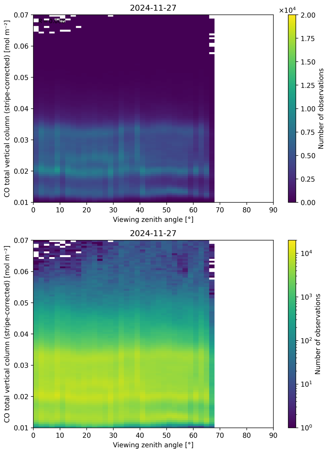
Figure 70: Scatter density plot of “Viewing zenith angle” against “CO total vertical column (stripe-corrected)” for 2024-11-26 to 2024-11-28.
