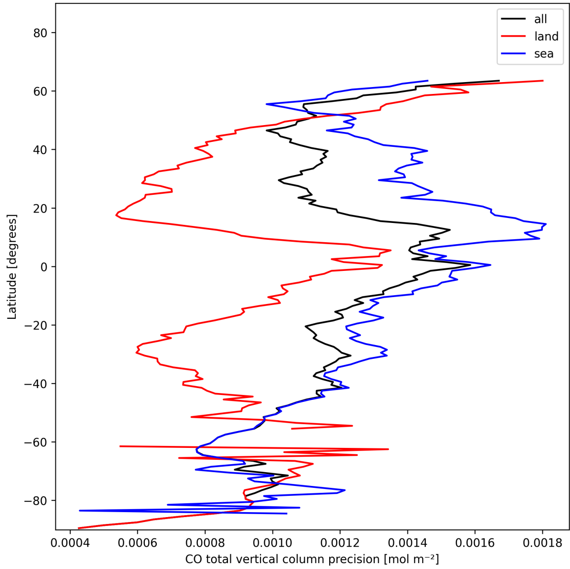
Figure 12: Zonal average of “CO total vertical column precision” for 2024-11-26 to 2024-11-28.
