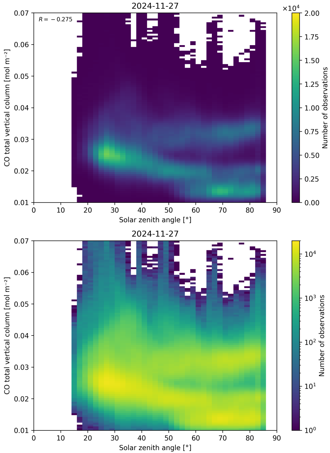
Figure 61: Scatter density plot of “Solar zenith angle” against “CO total vertical column” for 2024-11-26 to 2024-11-28.
