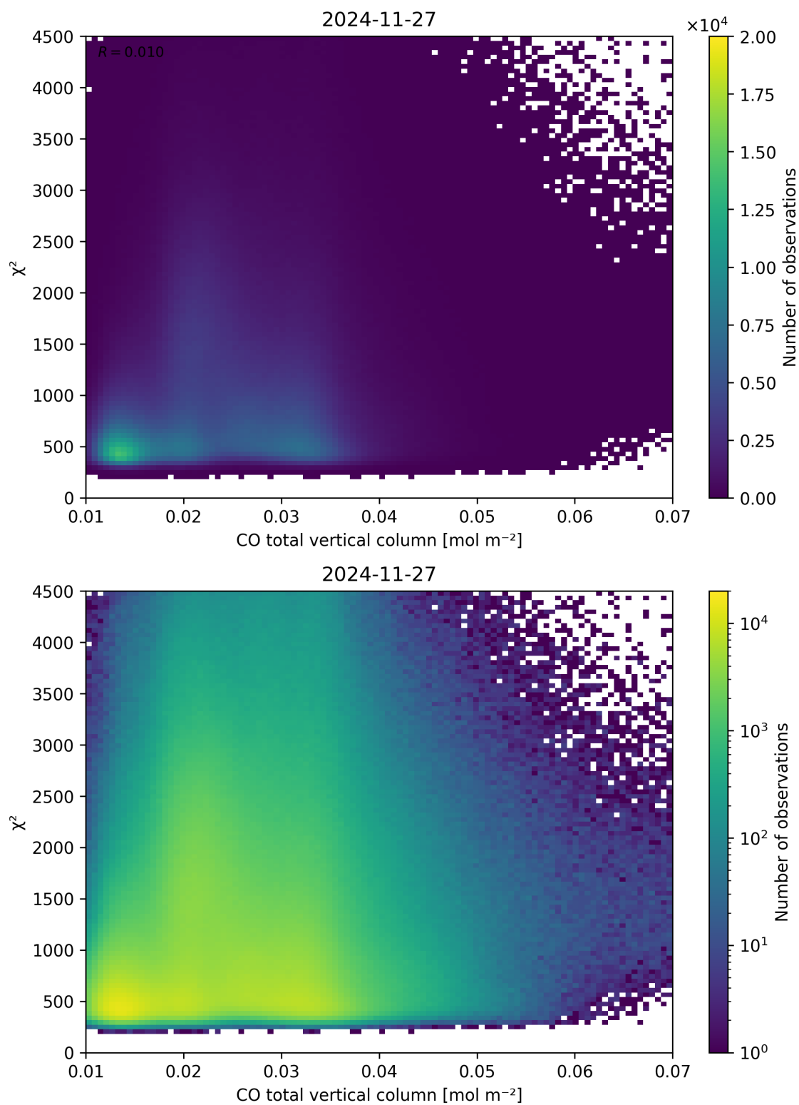
Figure 35: Scatter density plot of “CO total vertical column” against “ \chi^2 ” for 2024-11-26 to 2024-11-28.
