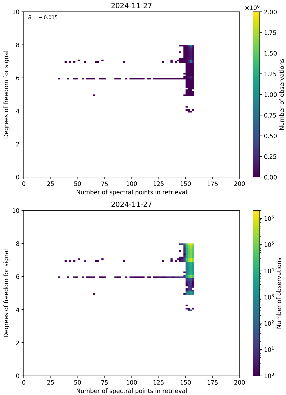
Figure 59: Scatter density plot of “Number of spectral points in retrieval” against “Degrees of freedom for signal” for 2024-11-26 to 2024-11-28.
