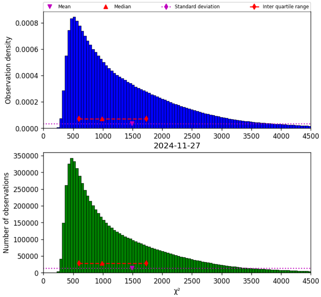
Figure 22: Histogram of “ \chi^2 ” for 2024-11-26 to 2024-11-28
