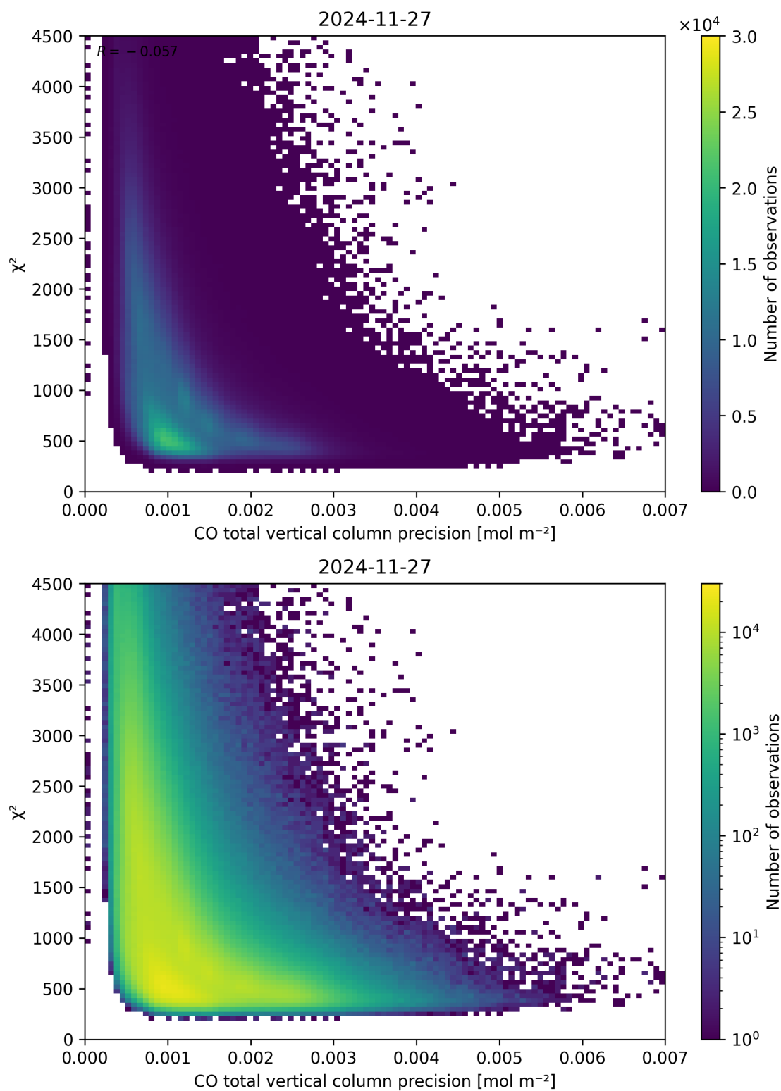
Figure 44: Scatter density plot of “CO total vertical column precision” against “ \chi^2 ” for 2024-11-26 to 2024-11-28.
