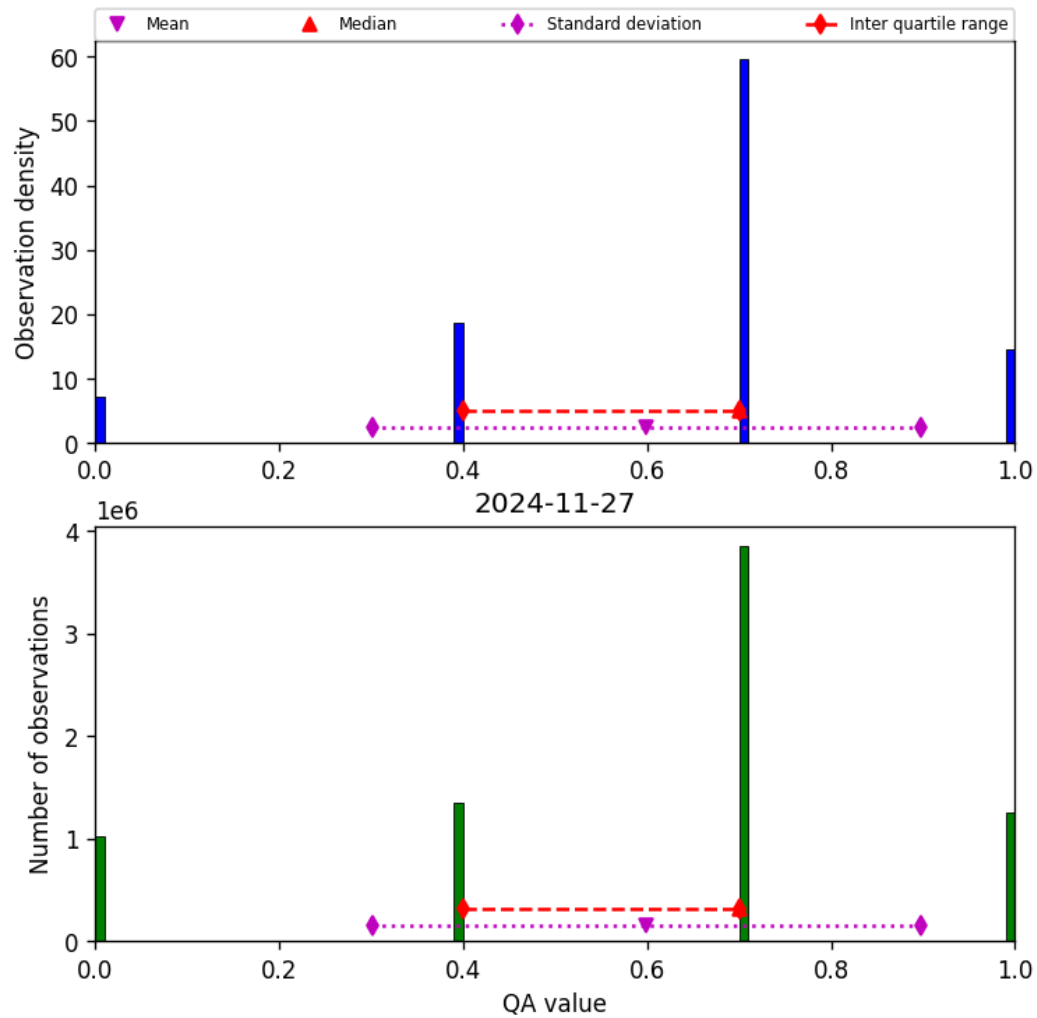
Figure 17: Histogram of “QA value” for 2024-11-26 to 2024-11-28
