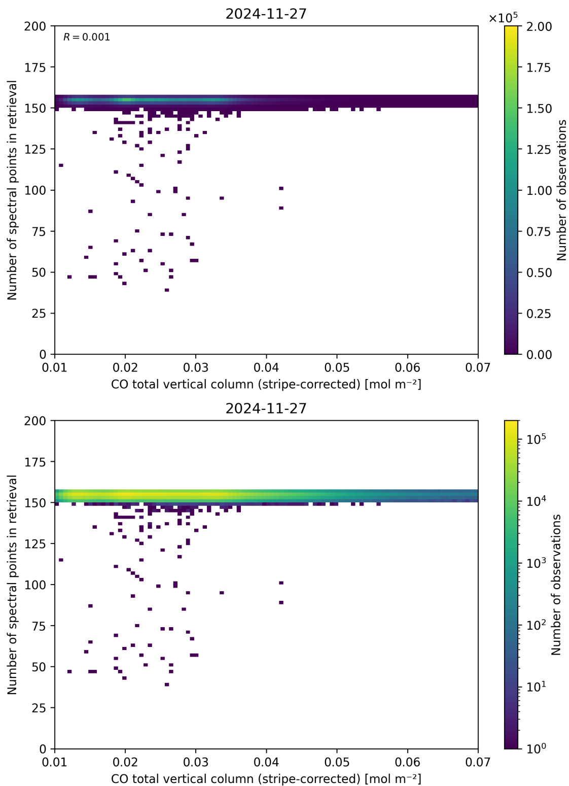
Figure 40: Scatter density plot of “CO total vertical column (stripe-corrected)” against “Number of spectral points in retrieval” for 2024-11-26 to 2024-11-28.
