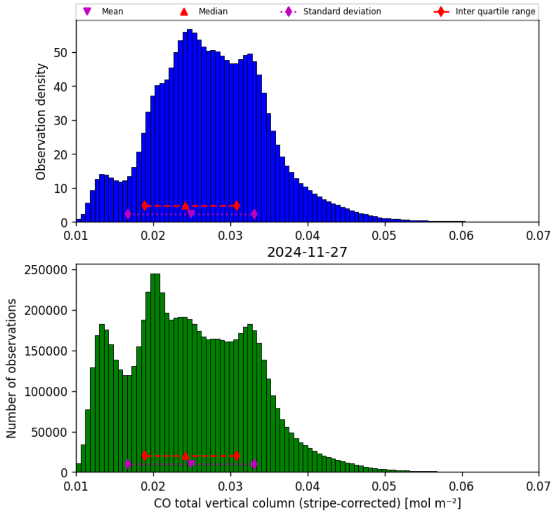
Figure 19: Histogram of “CO total vertical column (stripe-corrected)” for 2024-11-26 to 2024-11-28
