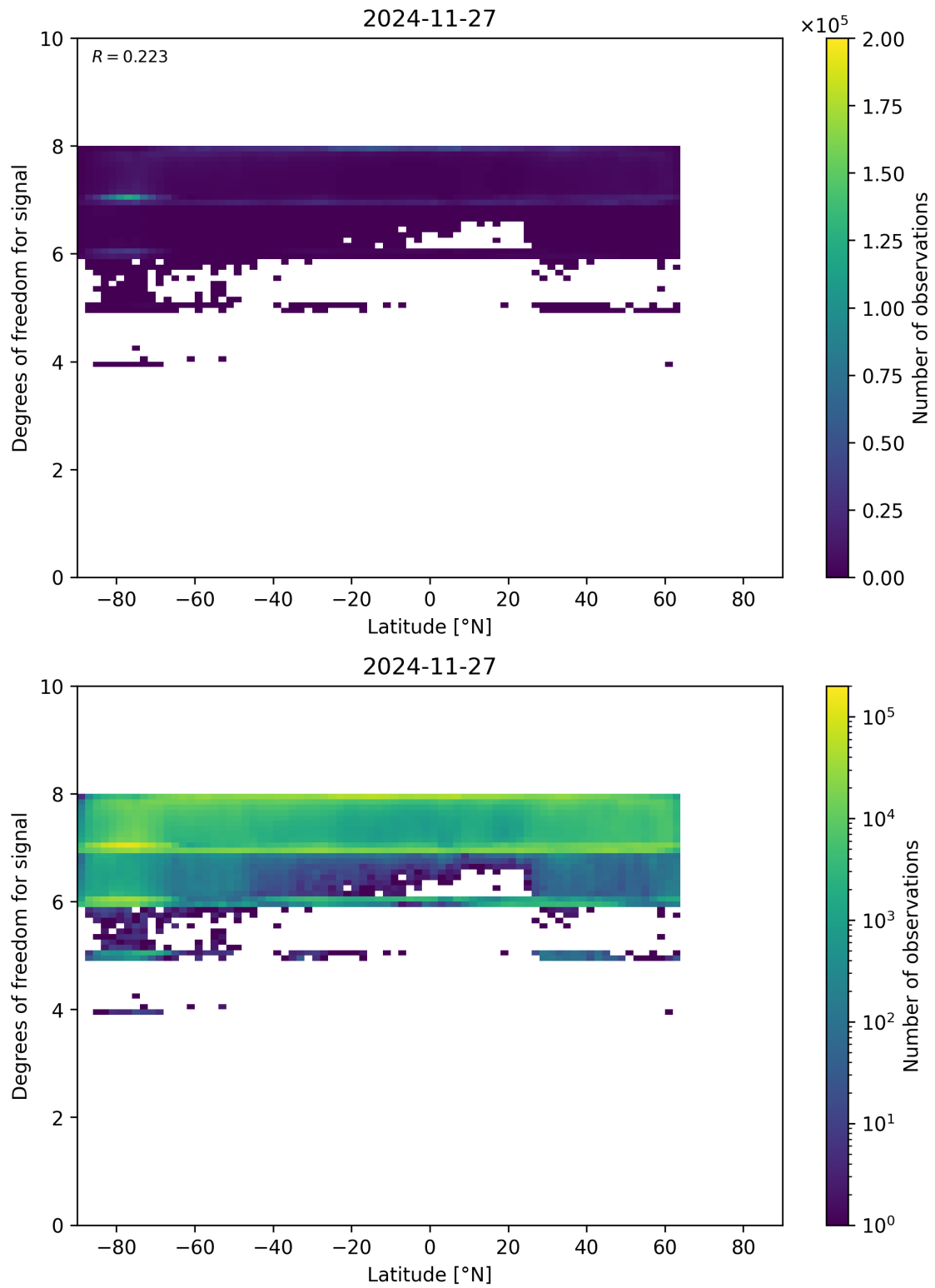
Figure 55: Scatter density plot of “Latitude” against “Degrees of freedom for signal” for 2024-11-26 to 2024-11-28.
