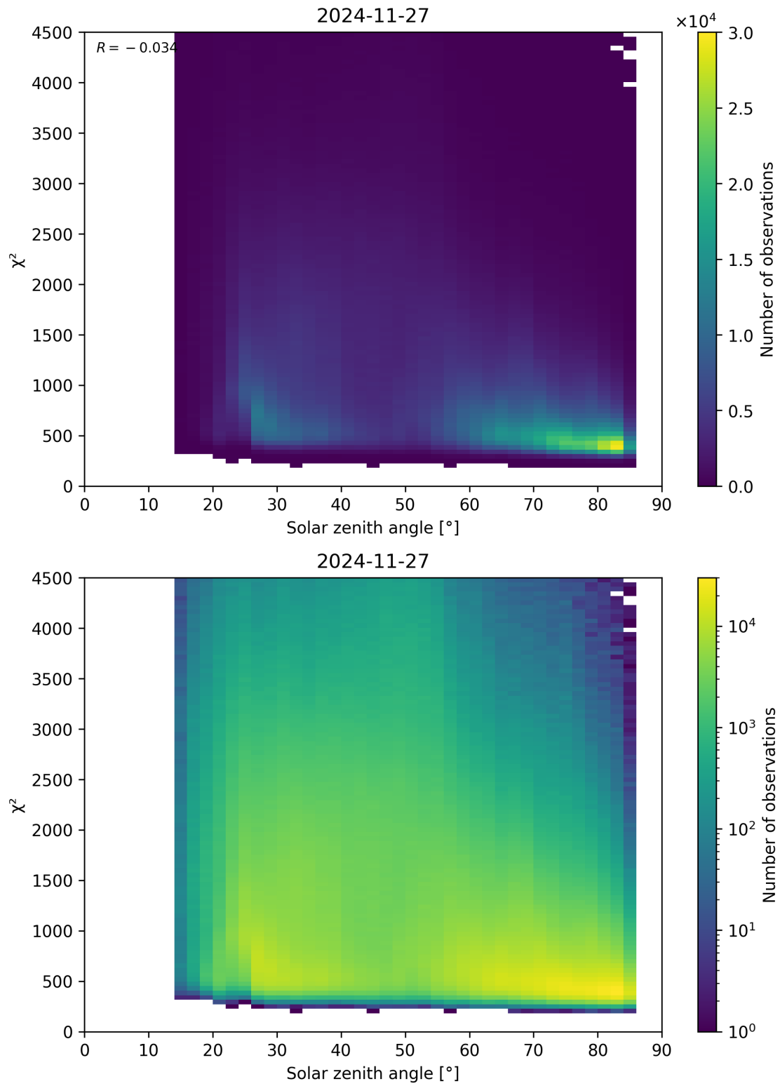
Figure 64: Scatter density plot of “Solar zenith angle” against “ \chi^2 ” for 2024-11-26 to 2024-11-28.
