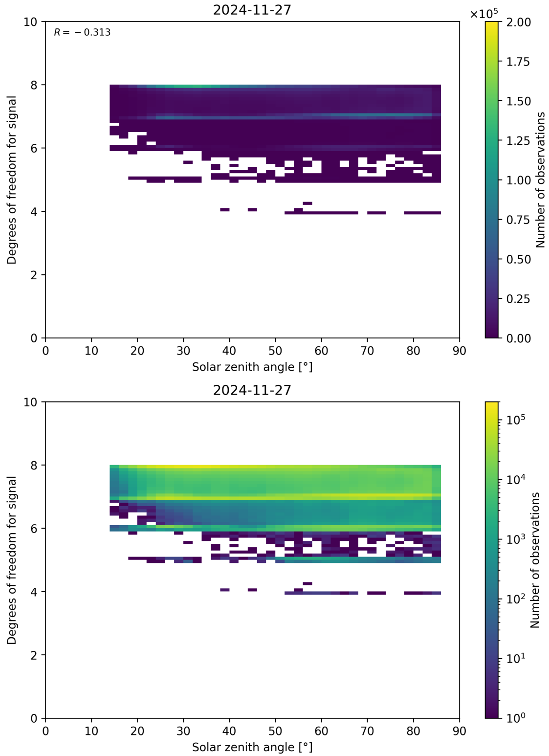
Figure 65: Scatter density plot of “Solar zenith angle” against “Degrees of freedom for signal” for 2024-11-26 to 2024-11-28.
