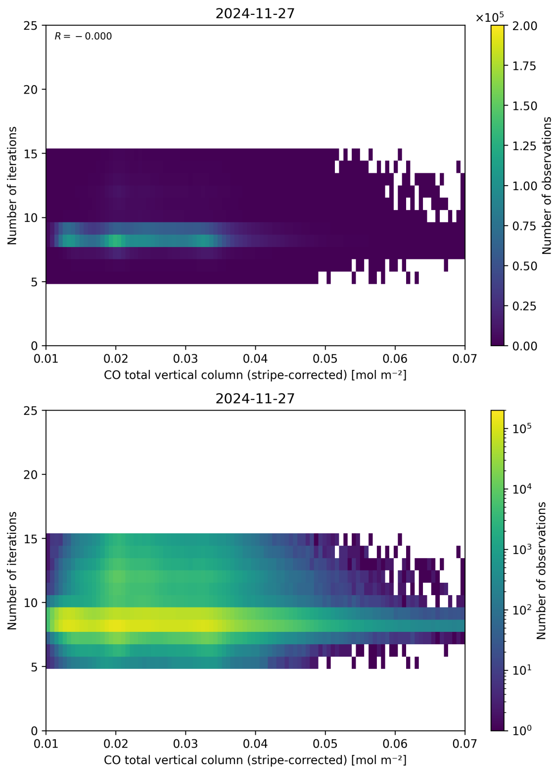
Figure 39: Scatter density plot of “CO total vertical column (stripe-corrected)” against “Number of iterations” for 2024-11-26 to 2024-11-28.
