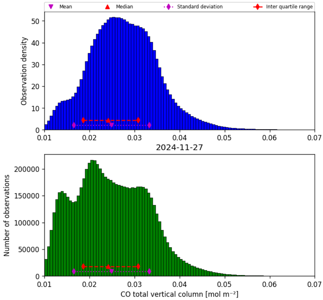
Figure 18: Histogram of “CO total vertical column” for 2024-11-26 to 2024-11-28
