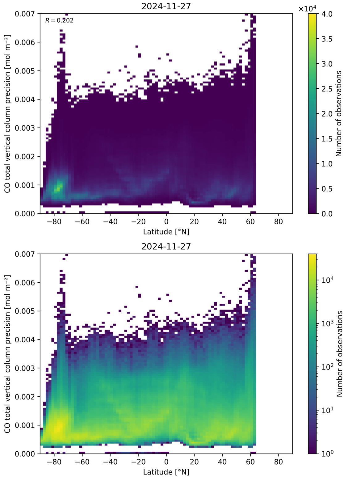
Figure 53: Scatter density plot of “Latitude” against “CO total vertical column precision” for 2024-11-26 to 2024-11-28.
