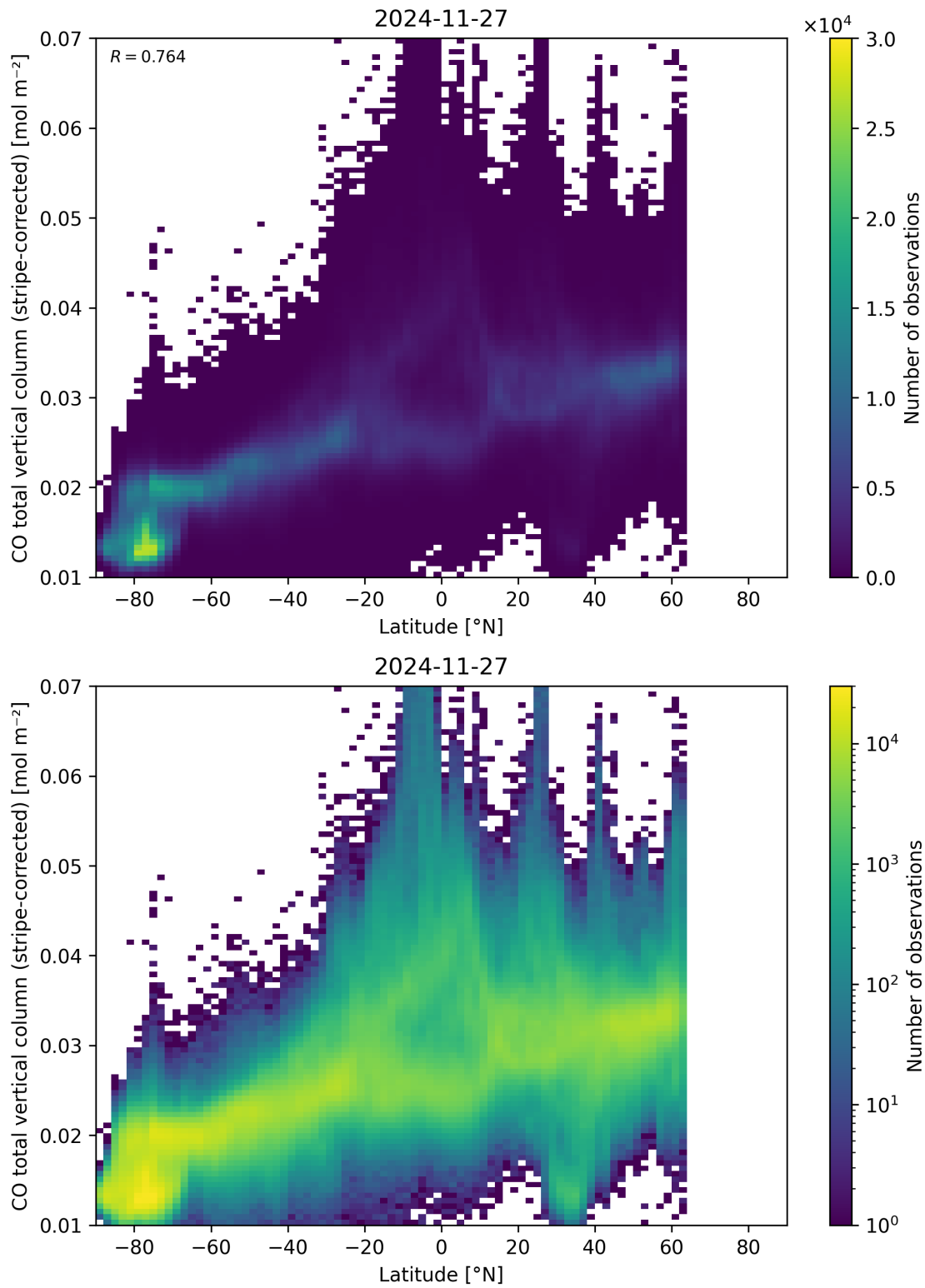
Figure 52: Scatter density plot of “Latitude” against “CO total vertical column (stripe-corrected)” for 2024-11-26 to 2024-11-28.
