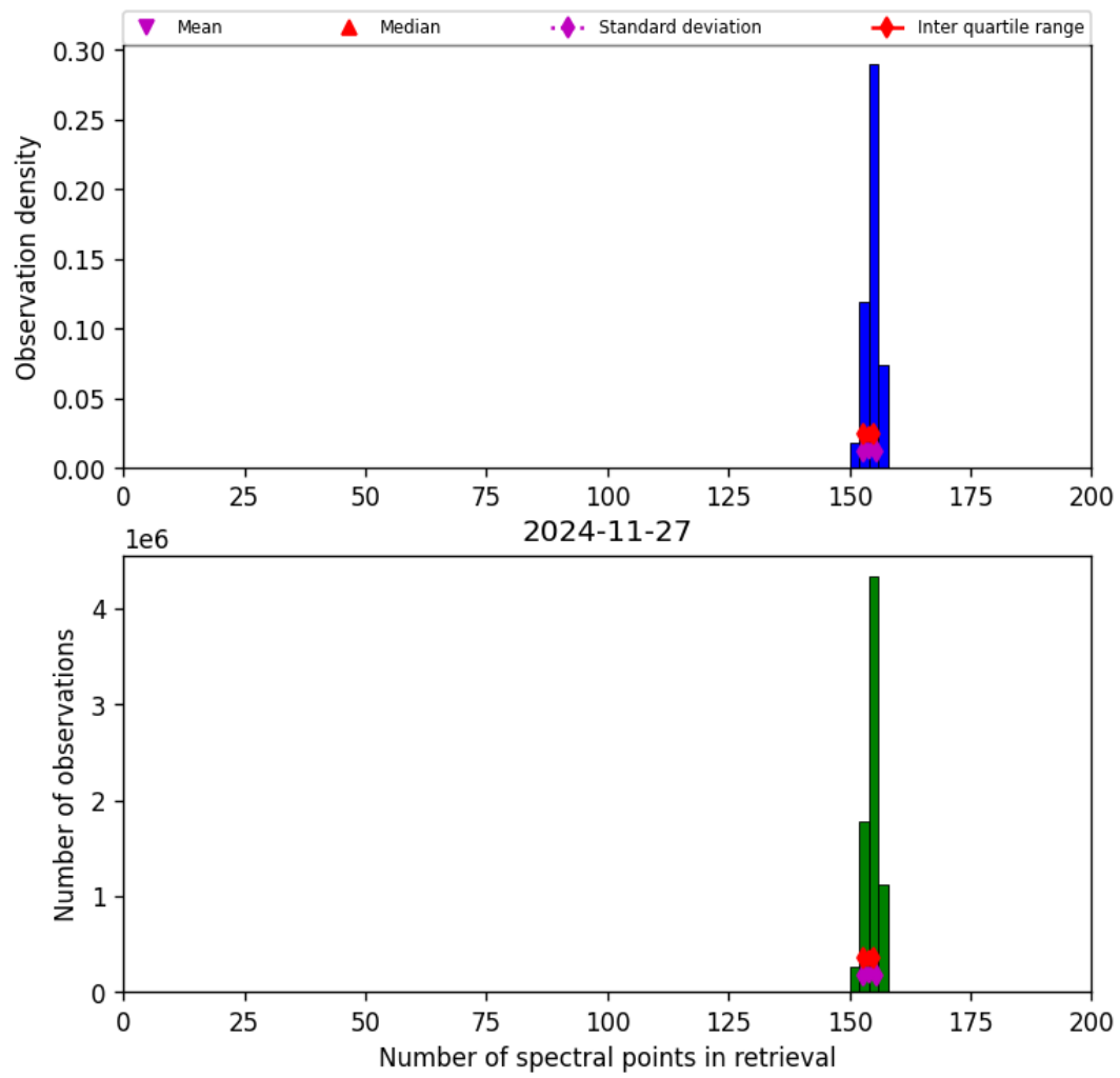
Figure 21: Histogram of “Number of spectral points in retrieval” for 2024-11-26 to 2024-11-28
