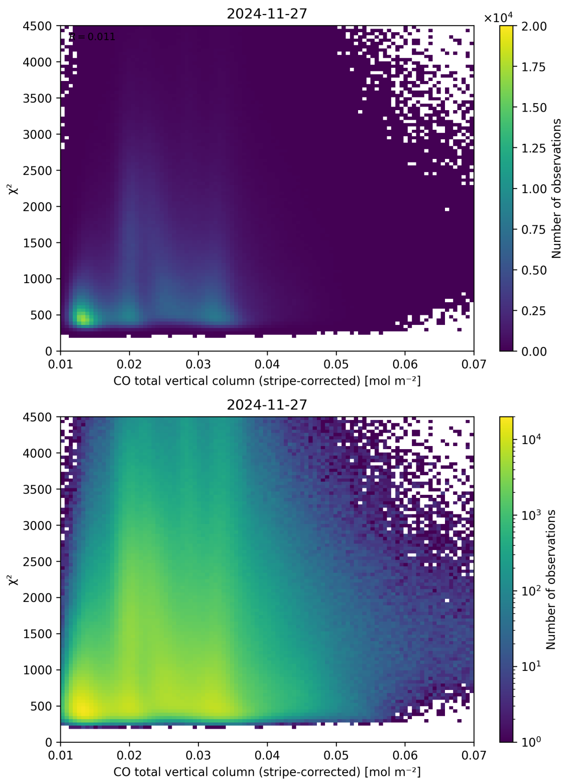
Figure 37: Scatter density plot of “CO total vertical column (stripe-corrected)” against “ \chi^2 ” for 2024-11-26 to 2024-11-28.
