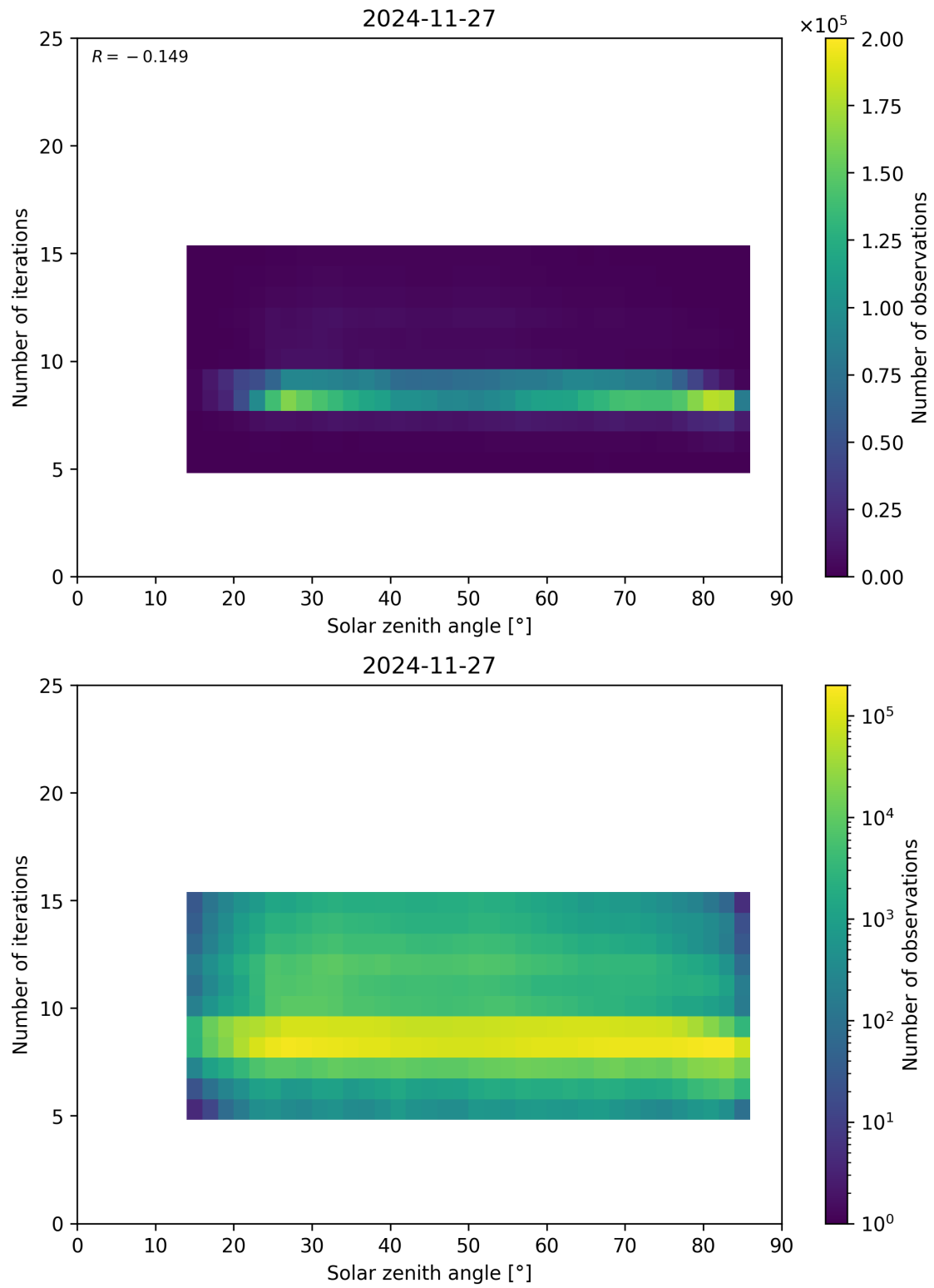
Figure 67: Scatter density plot of “Solar zenith angle” against “Number of iterations” for 2024-11-26 to 2024-11-28.
