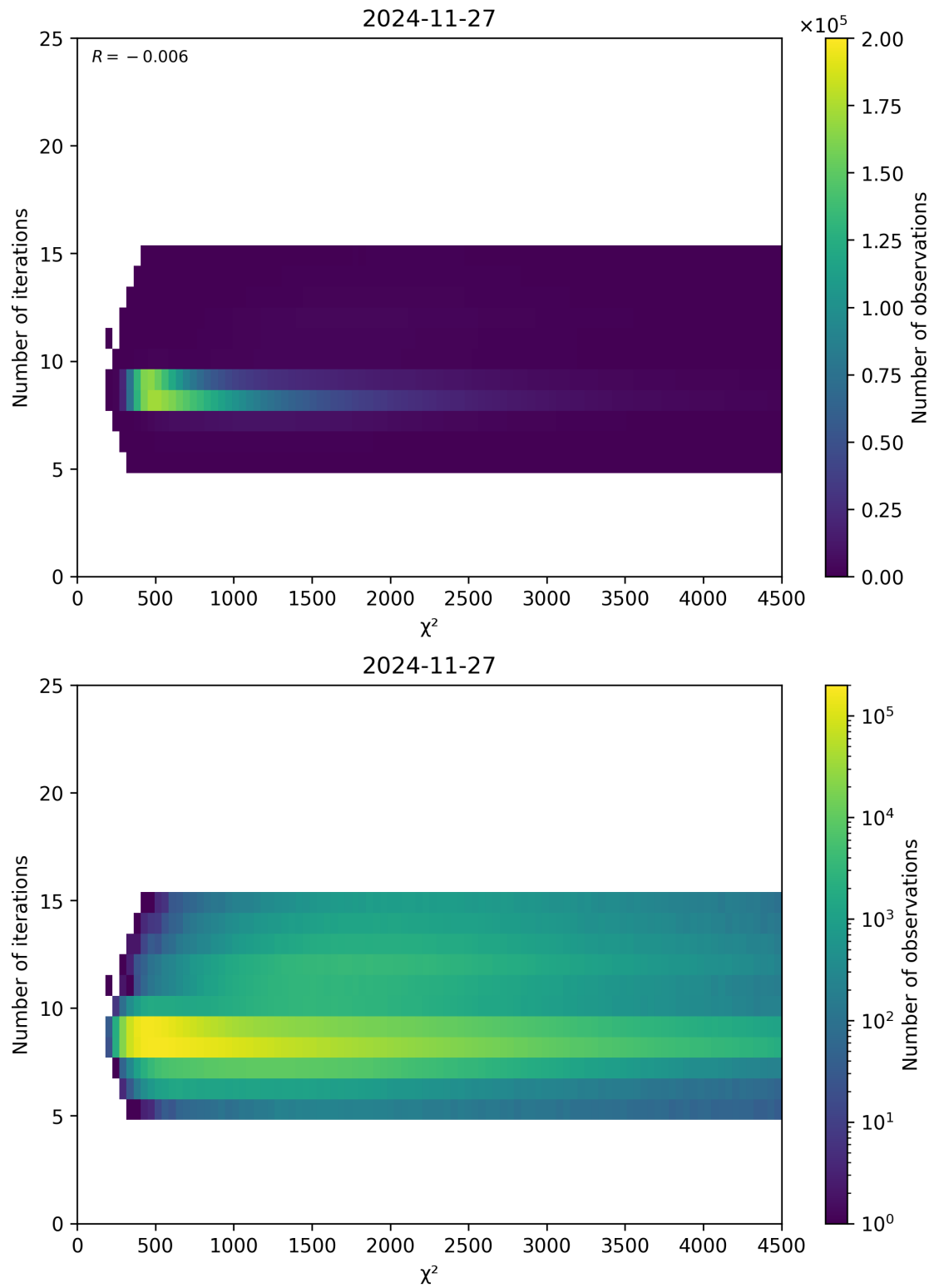
Figure 49: Scatter density plot of “ \chi^2 ” against “Number of iterations” for 2024-11-26 to 2024-11-28.
