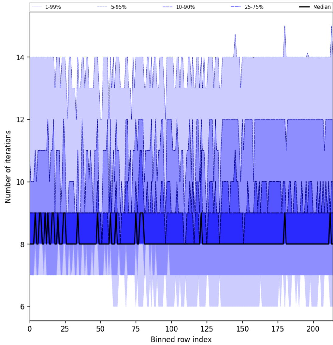
Figure 32: Along track statistics of “Number of iterations” for 2024-11-26 to 2024-11-28
