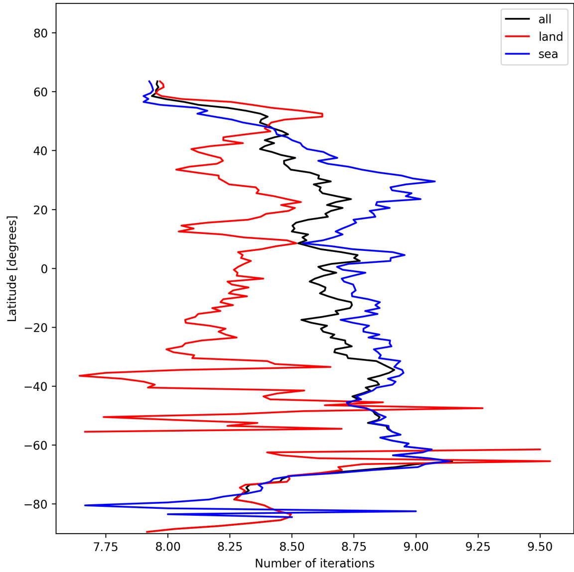
Figure 16: Zonal average of “Number of iterations” for 2024-11-26 to 2024-11-28.
