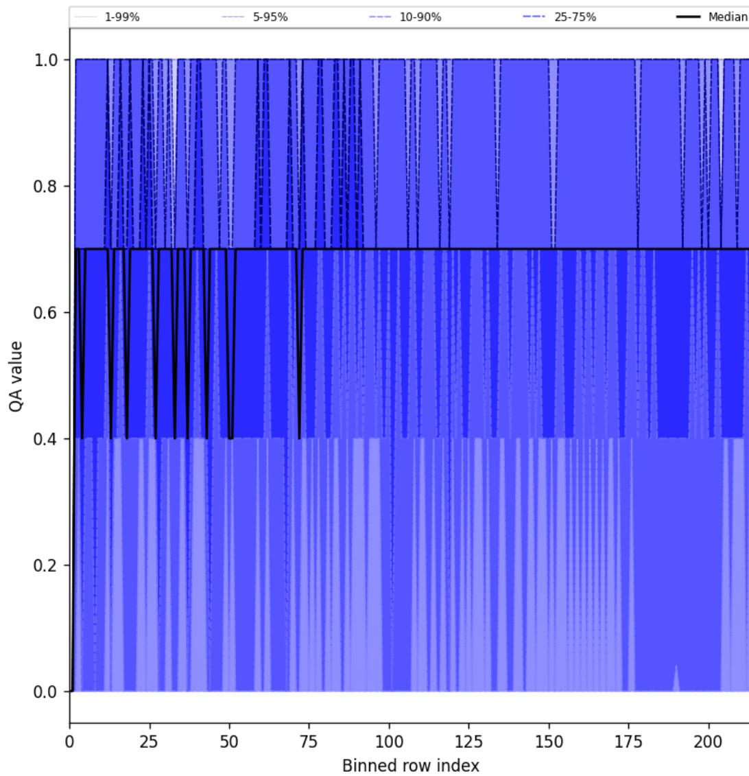
Figure 25: Along track statistics of “QA value” for 2024-11-26 to 2024-11-28
