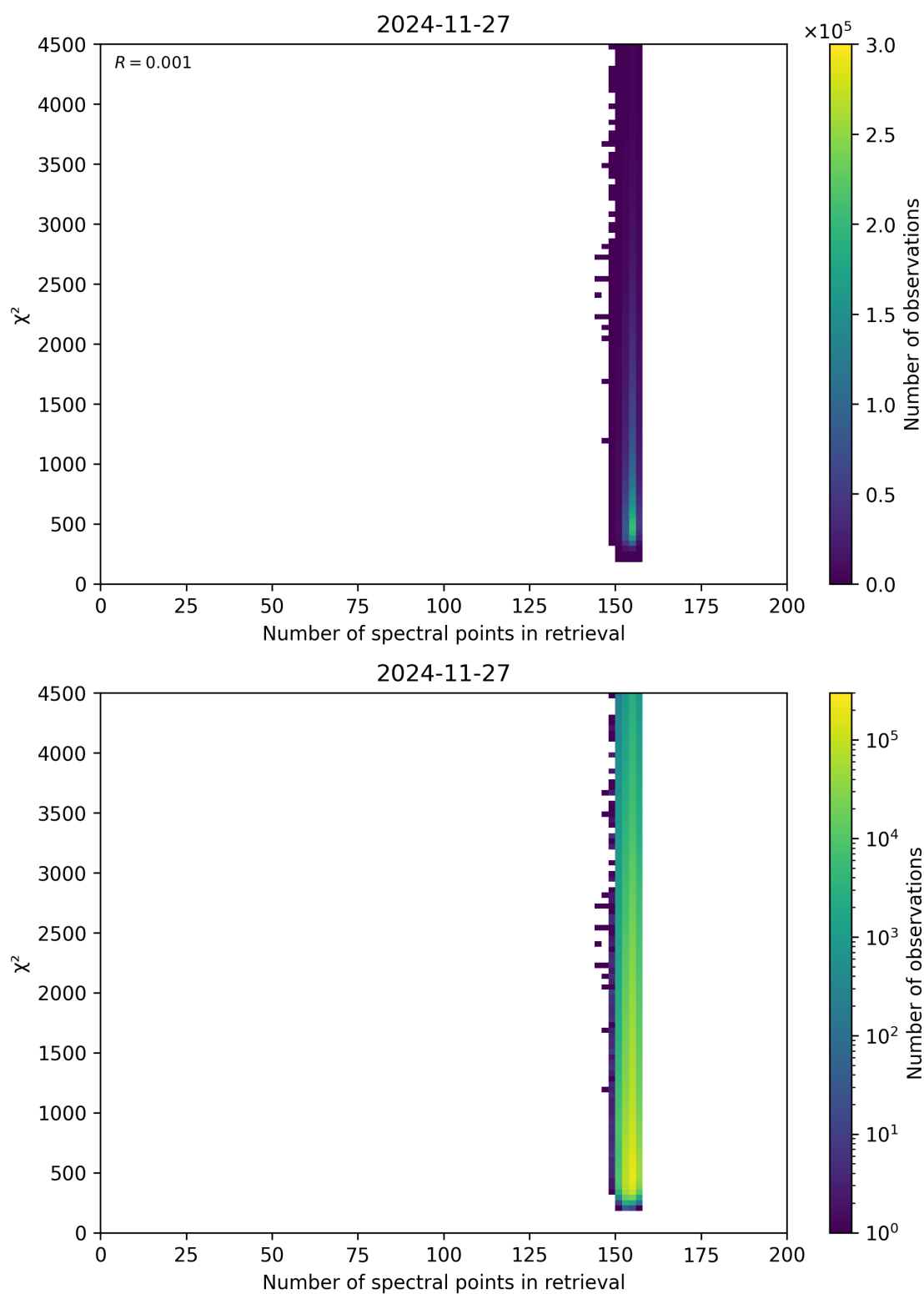
Figure 58: Scatter density plot of “Number of spectral points in retrieval” against “ \chi^2 ” for 2024-11-26 to 2024-11-28.
