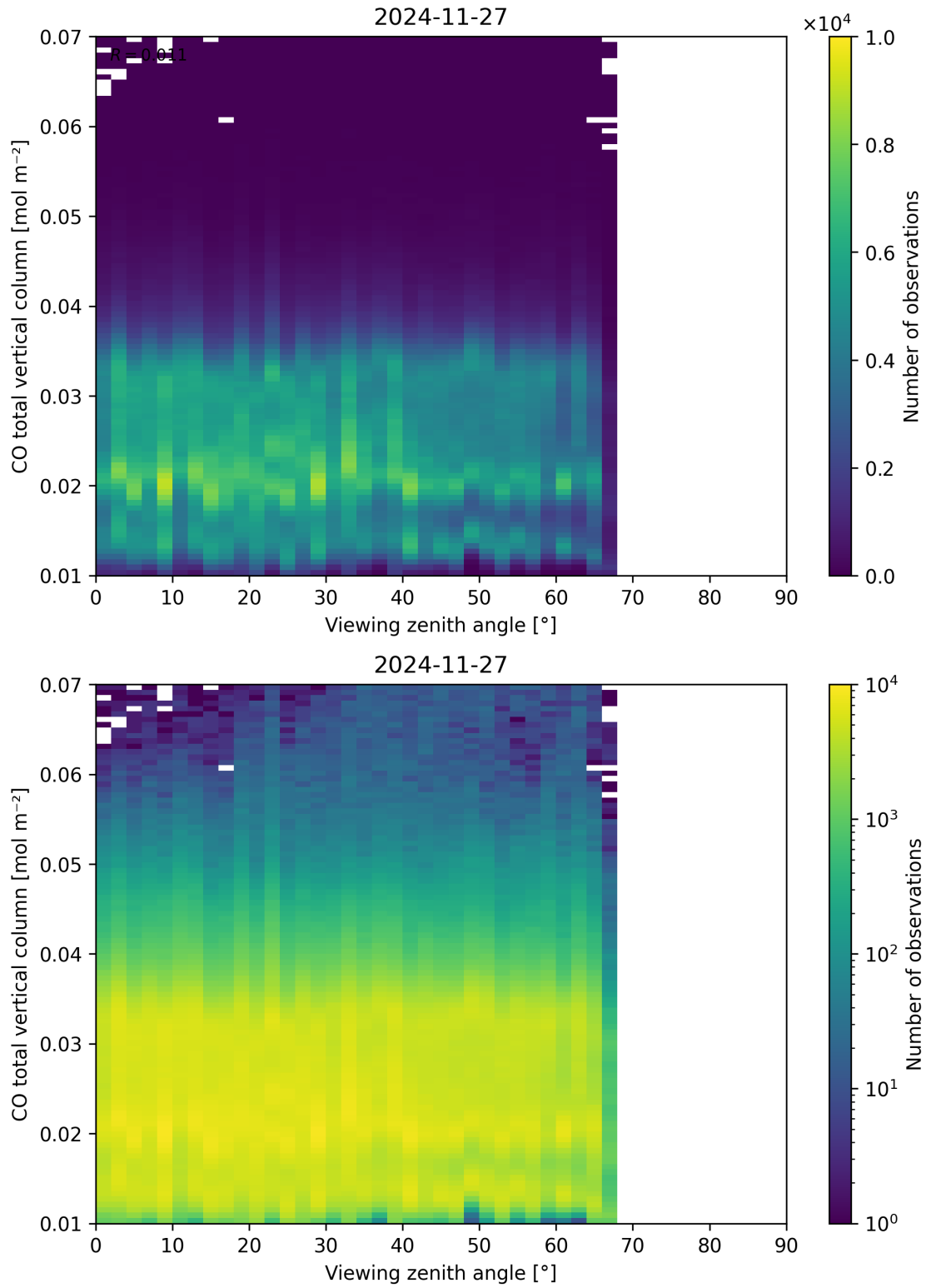
Figure 69: Scatter density plot of “Viewing zenith angle” against “CO total vertical column” for 2024-11-26 to 2024-11-28.
