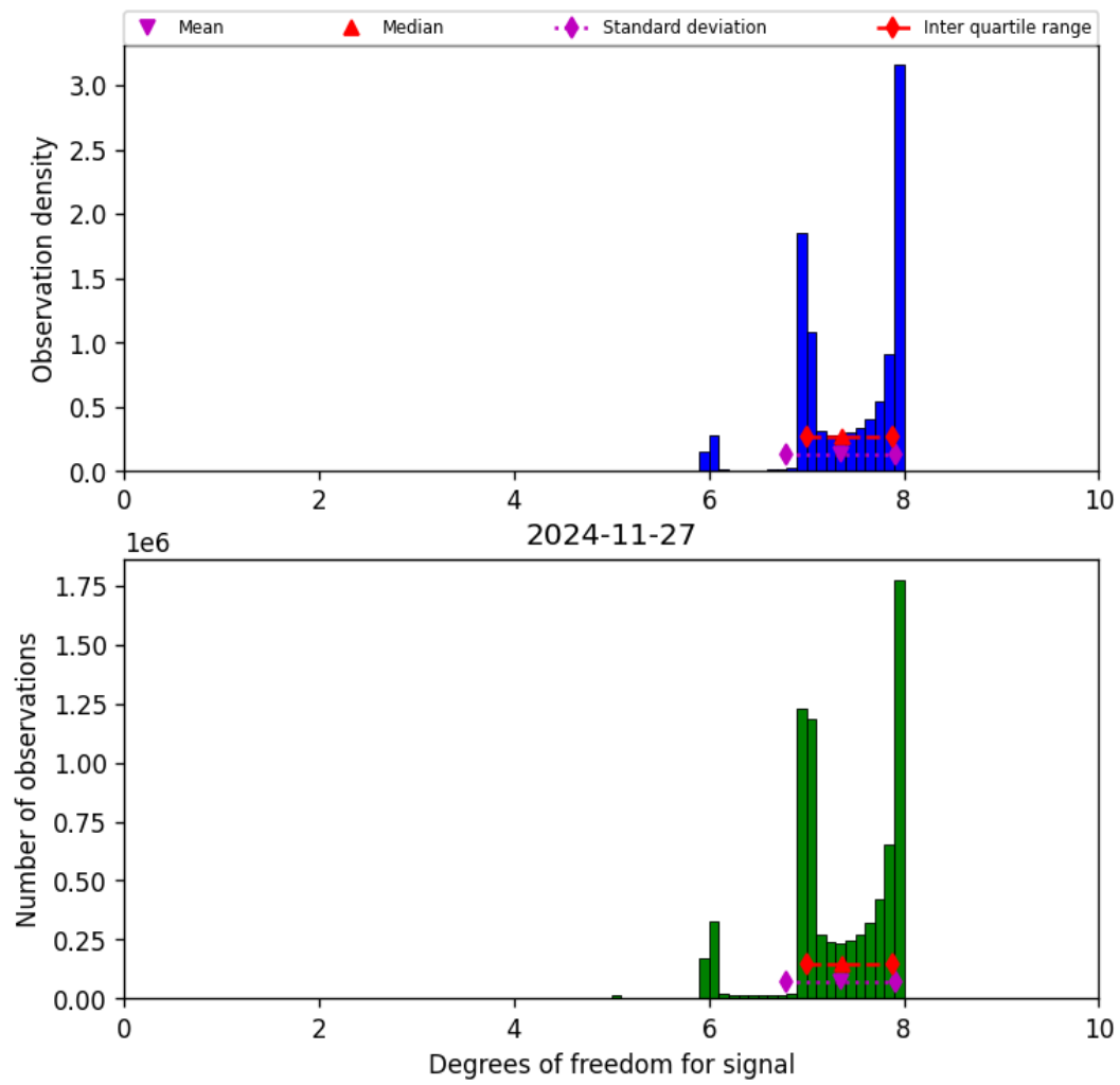
Figure 23: Histogram of “Degrees of freedom for signal” for 2024-11-26 to 2024-11-28
