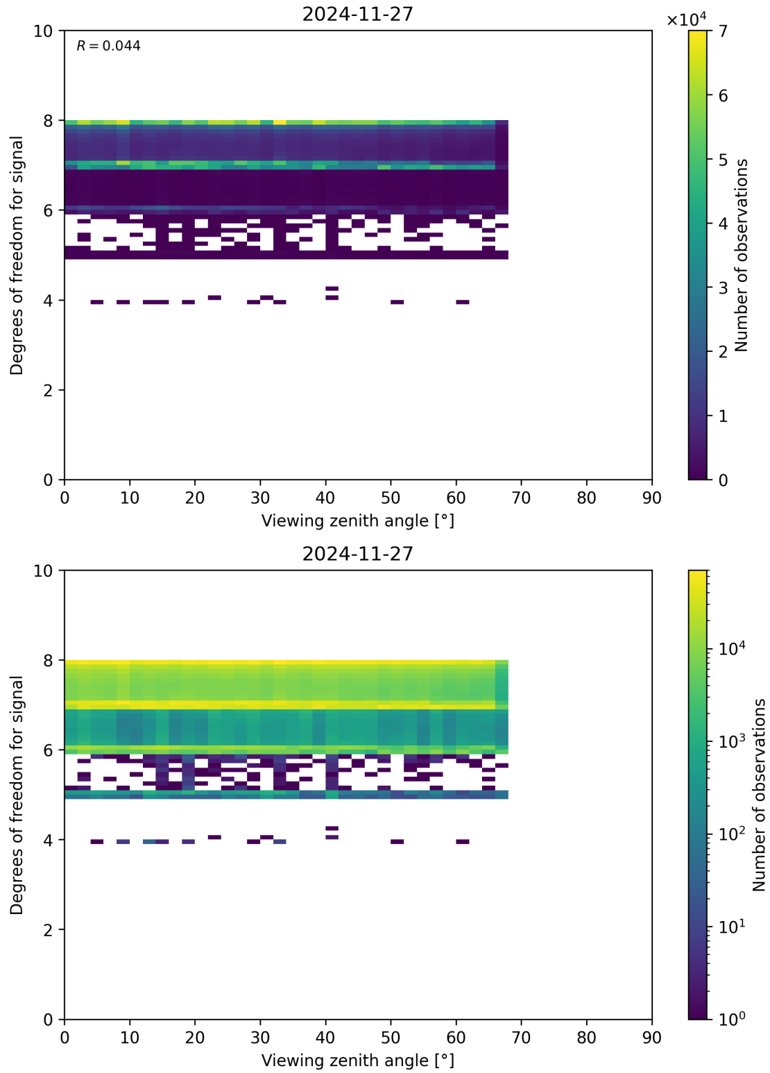
Figure 73: Scatter density plot of “Viewing zenith angle” against “Degrees of freedom for signal” for 2024-11-26 to 2024-11-28.
