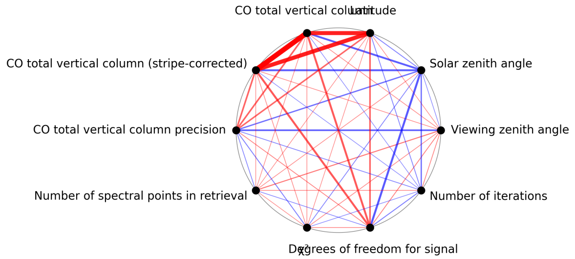
Figure 1: Map of correlation graph for 2024-11-26 to 2024-11-28.
