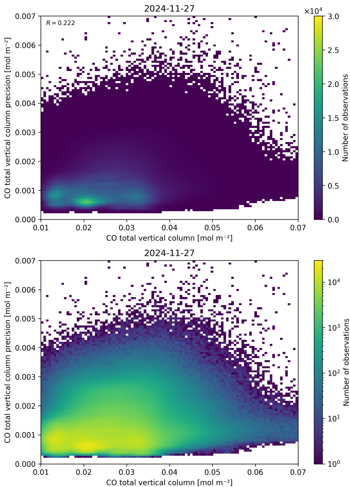
Figure 34: Scatter density plot of “CO total vertical column” against “CO total vertical column precision” for 2024-11-26 to 2024-11-28.
