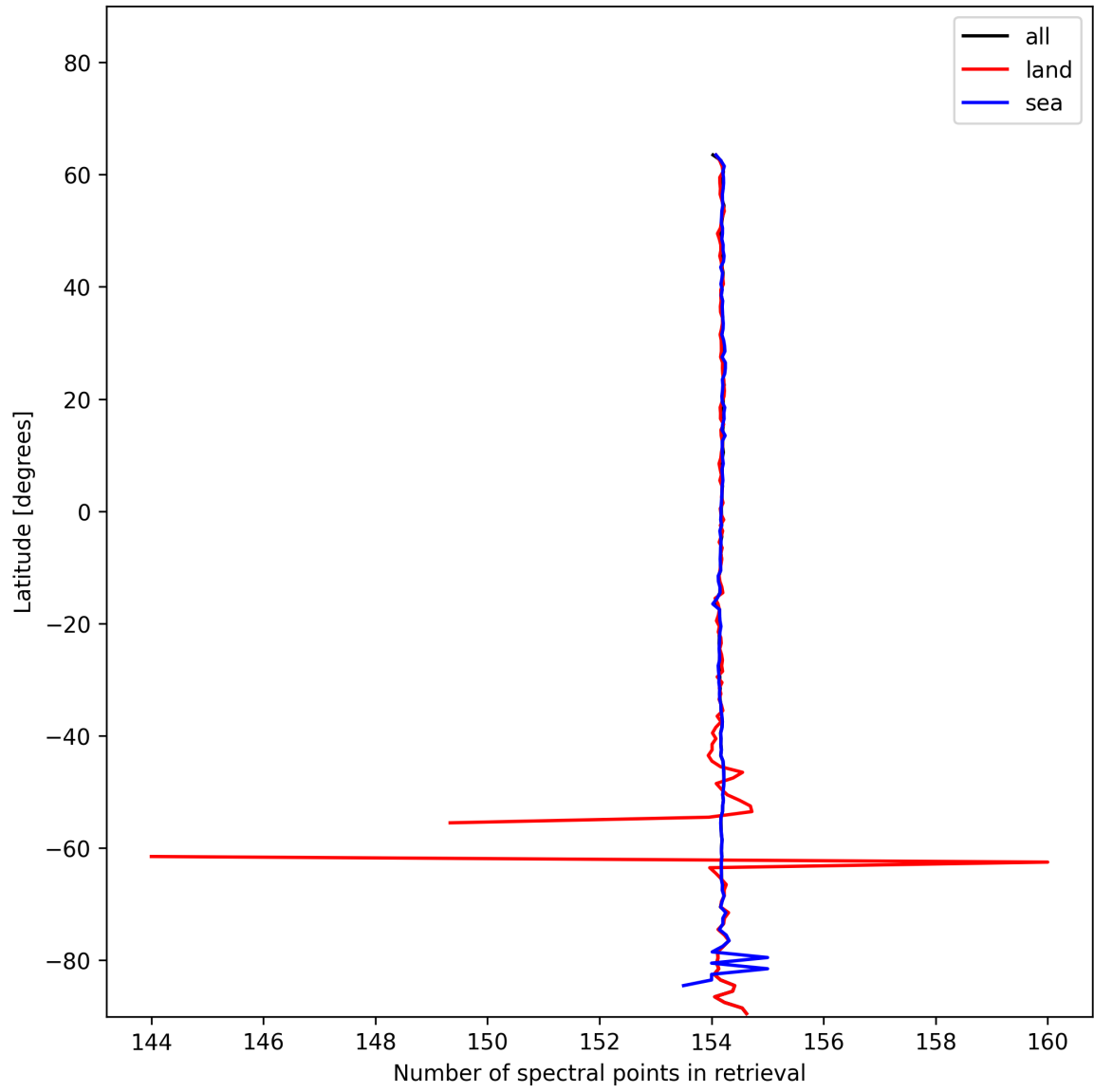
Figure 13: Zonal average of “Number of spectral points in retrieval” for 2024-11-26 to 2024-11-28.
