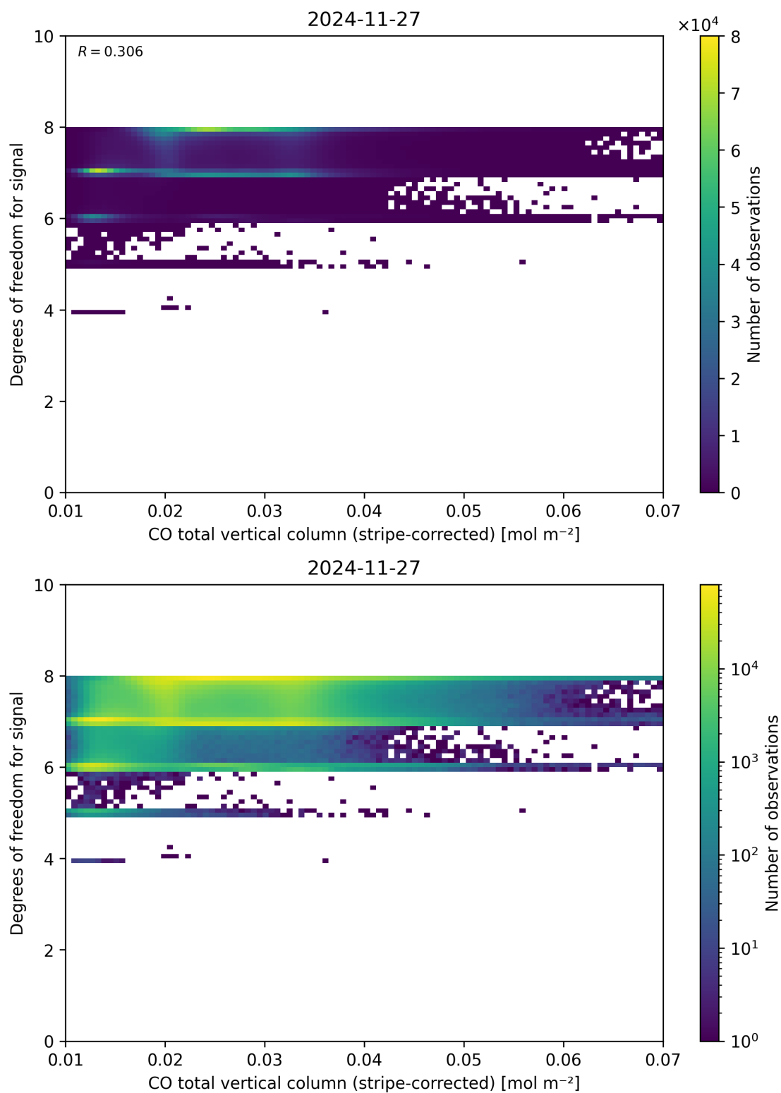
Figure 38: Scatter density plot of “CO total vertical column (stripe-corrected)” against “Degrees of freedom for signal” for 2024-11-26 to 2024-11-28.
