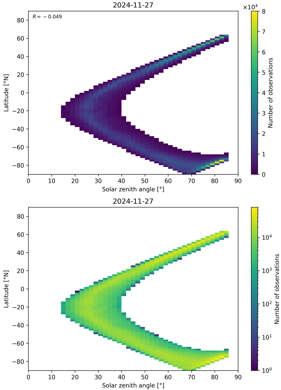
Figure 66: Scatter density plot of “Solar zenith angle” against “Latitude” for 2024-11-26 to 2024-11-28.
