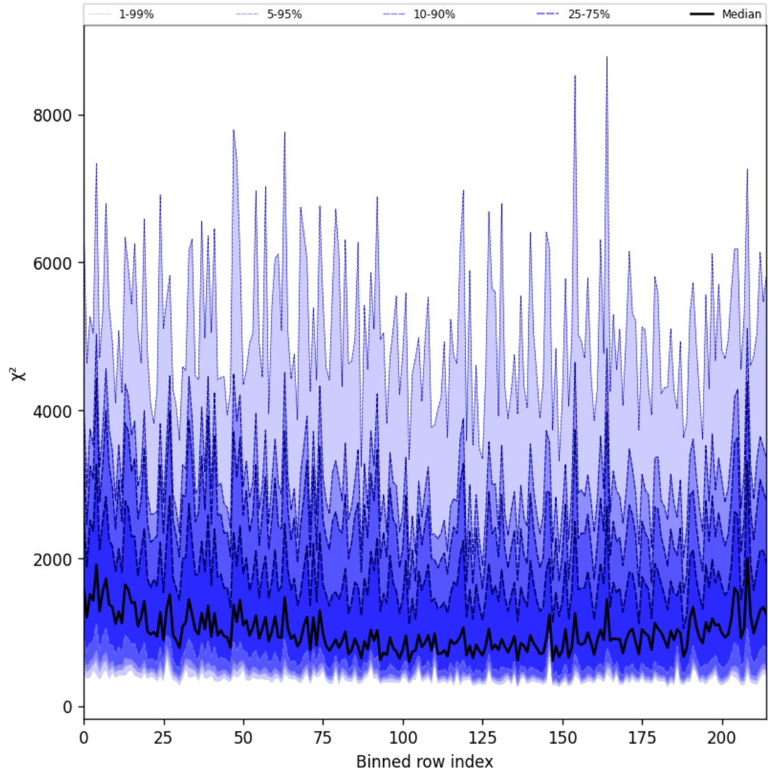
Figure 30: Along track statistics of “ \chi^2 ” for 2024-11-26 to 2024-11-28
