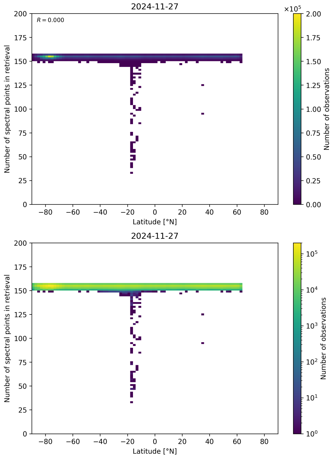
Figure 57: Scatter density plot of “Latitude” against “Number of spectral points in retrieval” for 2024-11-26 to 2024-11-28.
