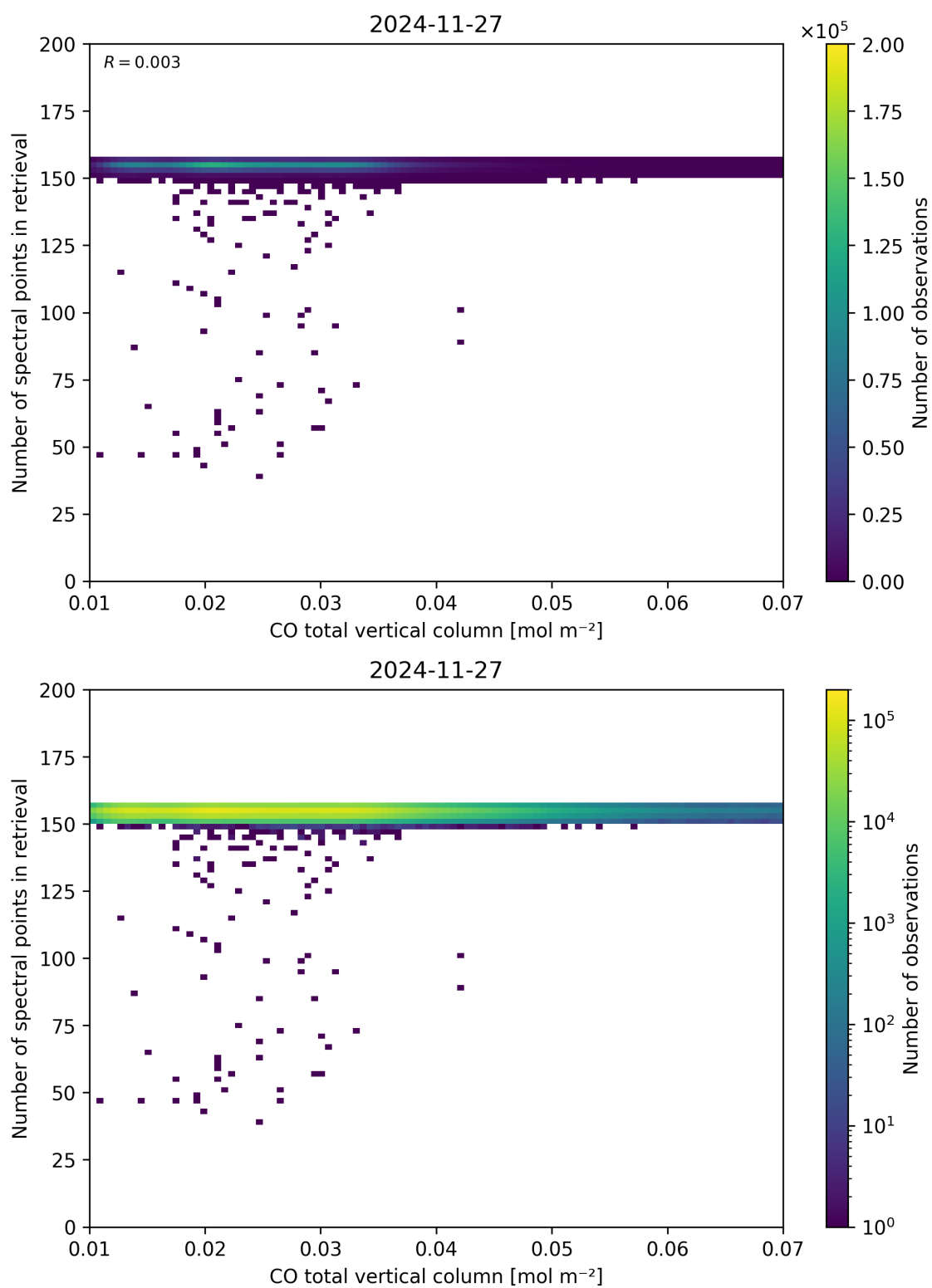
Figure 43: Scatter density plot of “CO total vertical column” against “Number of spectral points in retrieval” for 2024-11-26 to 2024-11-28.
