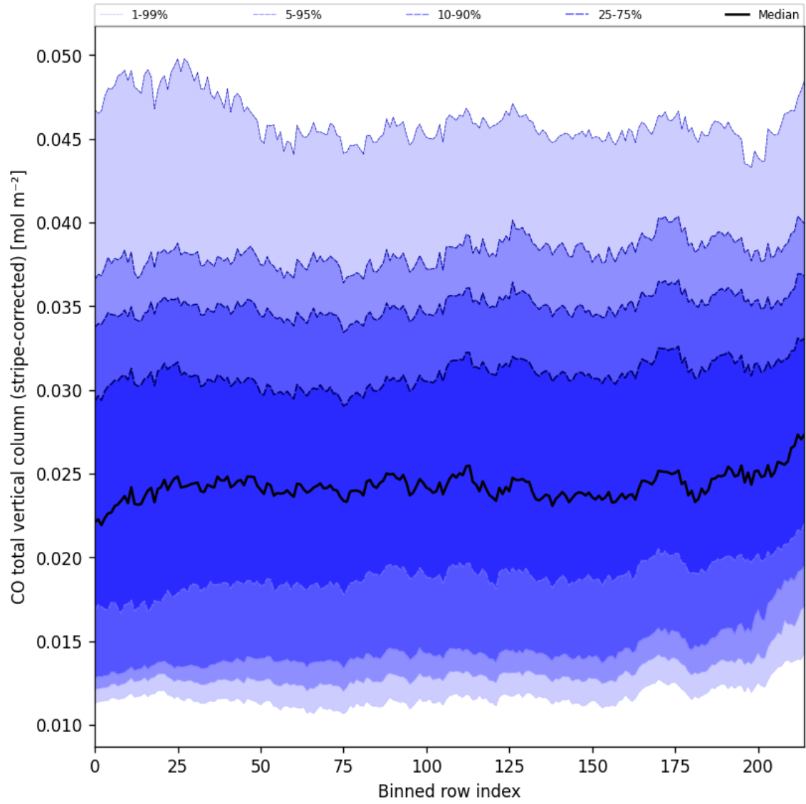
Figure 27: Along track statistics of “CO total vertical column (stripe-corrected)” for 2024-11-26 to 2024-11-28
