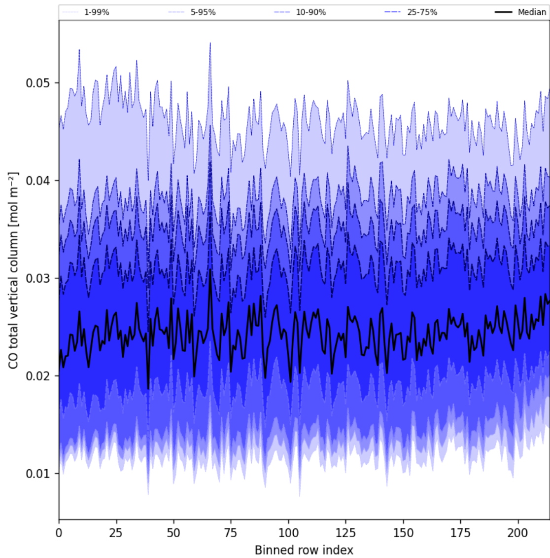
Figure 26: Along track statistics of "CO total vertical column" for 2024-11-26 to 2024-11-28
