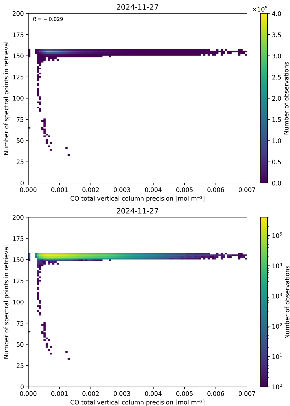
Figure 47: Scatter density plot of “CO total vertical column precision” against “Number of spectral points in retrieval” for 2024-11-26 to 2024-11-28.
