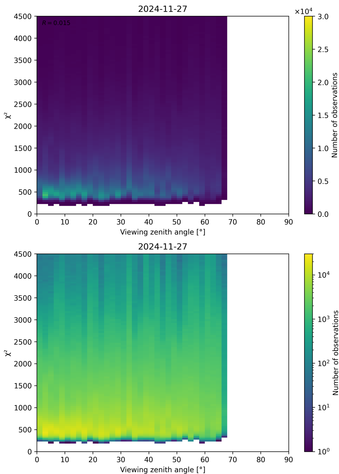
Figure 72: Scatter density plot of “Viewing zenith angle” against “ \chi^2 ” for 2024-11-26 to 2024-11-28.
