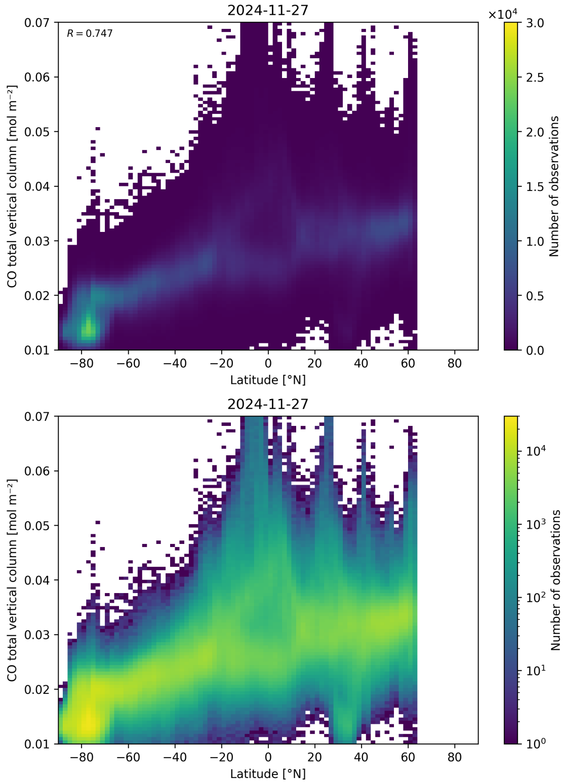
Figure 51: Scatter density plot of “Latitude” against “CO total vertical column” for 2024-11-26 to 2024-11-28.
