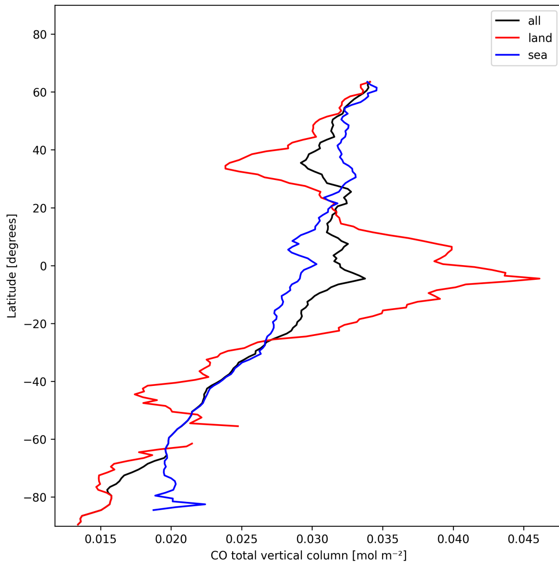
Figure 10: Zonal average of “CO total vertical column” for 2024-11-26 to 2024-11-28.
