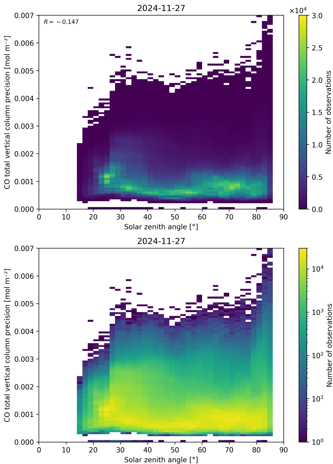
Figure 63: Scatter density plot of “Solar zenith angle” against “CO total vertical column precision” for 2024-11-26 to 2024-11-28.
