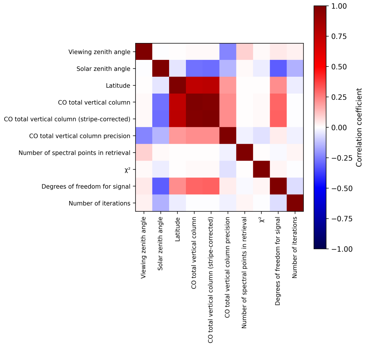
Figure 2: Map of correlation matrix for 2024-11-26 to 2024-11-28.
