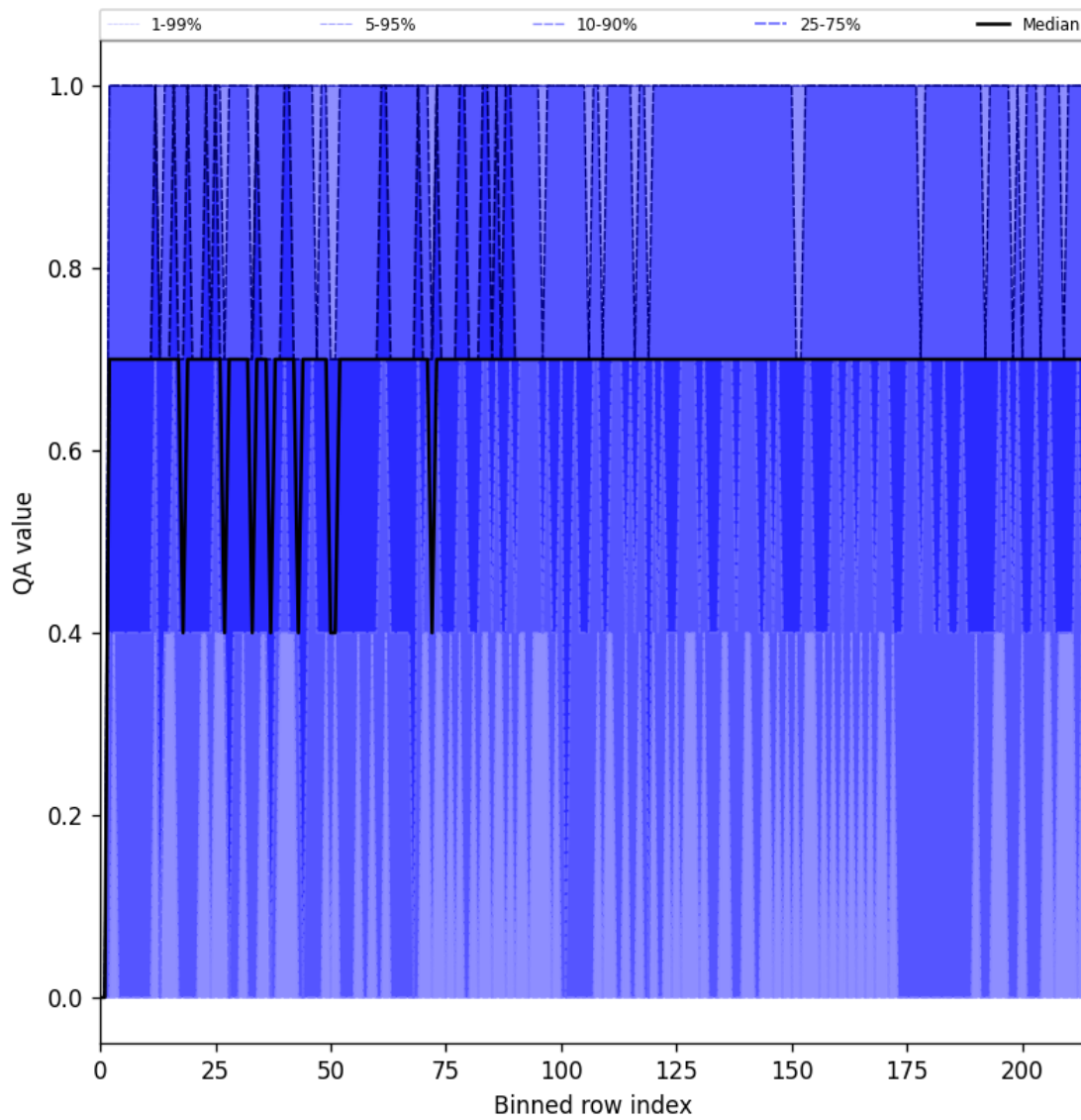
Figure 25: Along track statistics of “QA value” for 2024-11-27 to 2024-11-29
