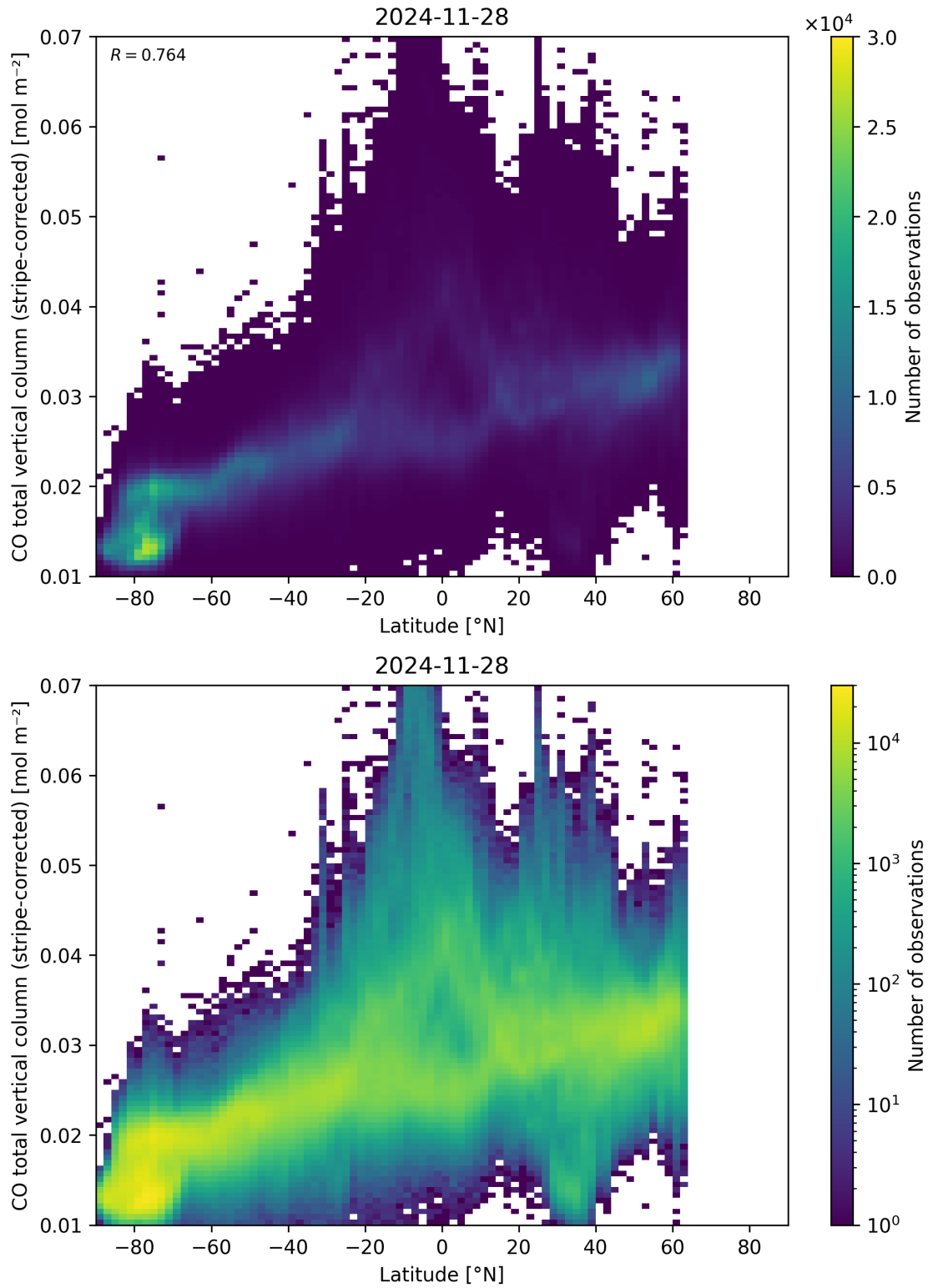
Figure 52: Scatter density plot of “Latitude” against “CO total vertical column (stripe-corrected)” for 2024-11-27 to 2024-11-29.
