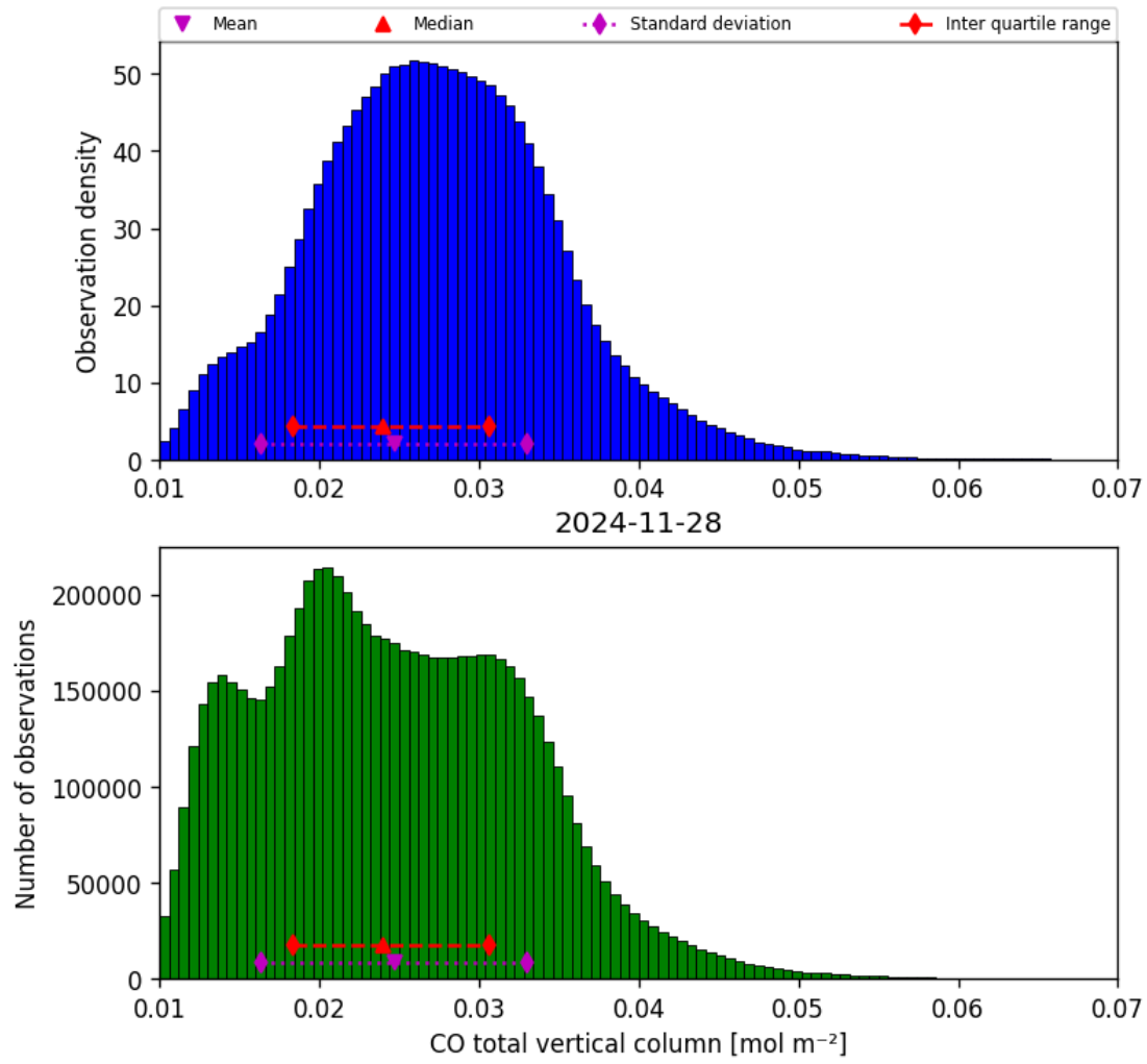
Figure 18: Histogram of “CO total vertical column” for 2024-11-27 to 2024-11-29
