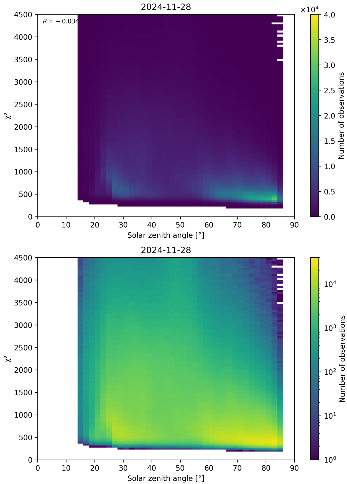
Figure 64: Scatter density plot of “Solar zenith angle” against “ \chi^2 ” for 2024-11-27 to 2024-11-29.
