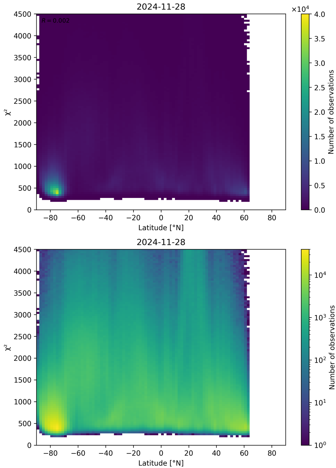
Figure 54: Scatter density plot of “Latitude” against “ \chi^2 ” for 2024-11-27 to 2024-11-29.
