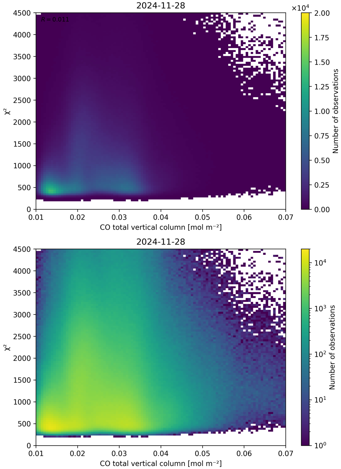
Figure 35: Scatter density plot of “CO total vertical column” against “ \chi^2 ” for 2024-11-27 to 2024-11-29.
