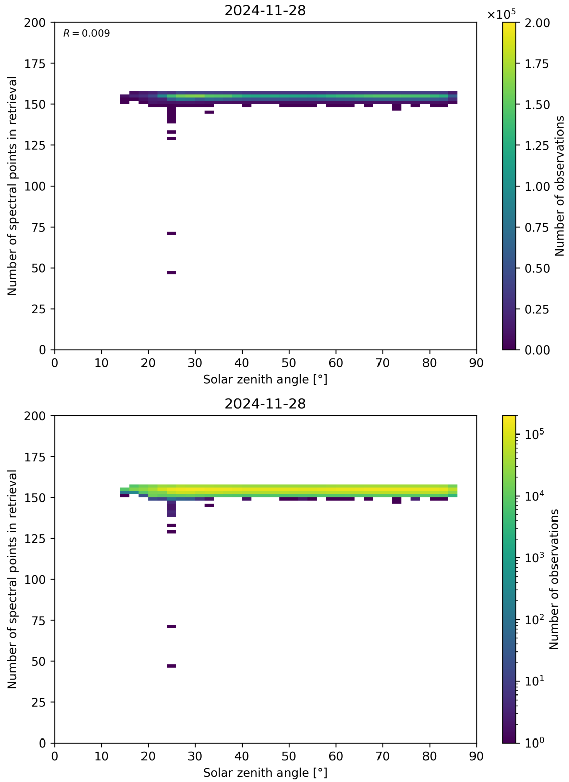
Figure 68: Scatter density plot of “Solar zenith angle” against “Number of spectral points in retrieval” for 2024-11-27 to 2024-11-29.
