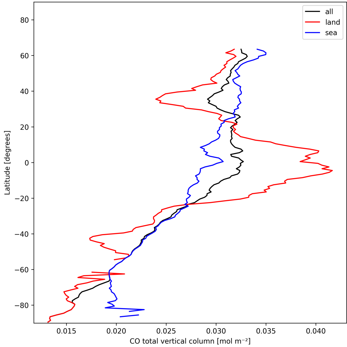
Figure 10: Zonal average of “CO total vertical column” for 2024-11-27 to 2024-11-29.
