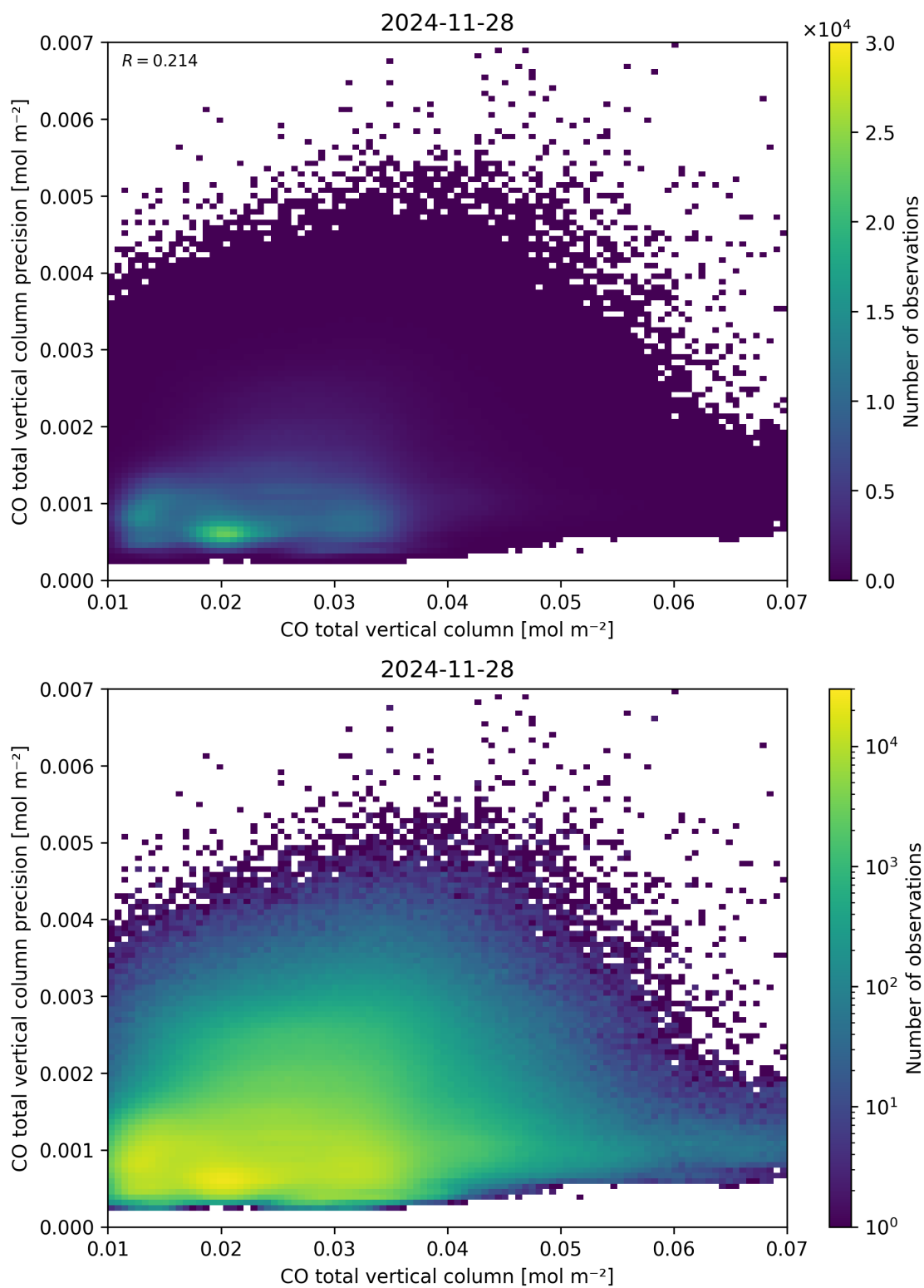
Figure 34: Scatter density plot of “CO total vertical column” against “CO total vertical column precision” for 2024-11-27 to 2024-11-29.
