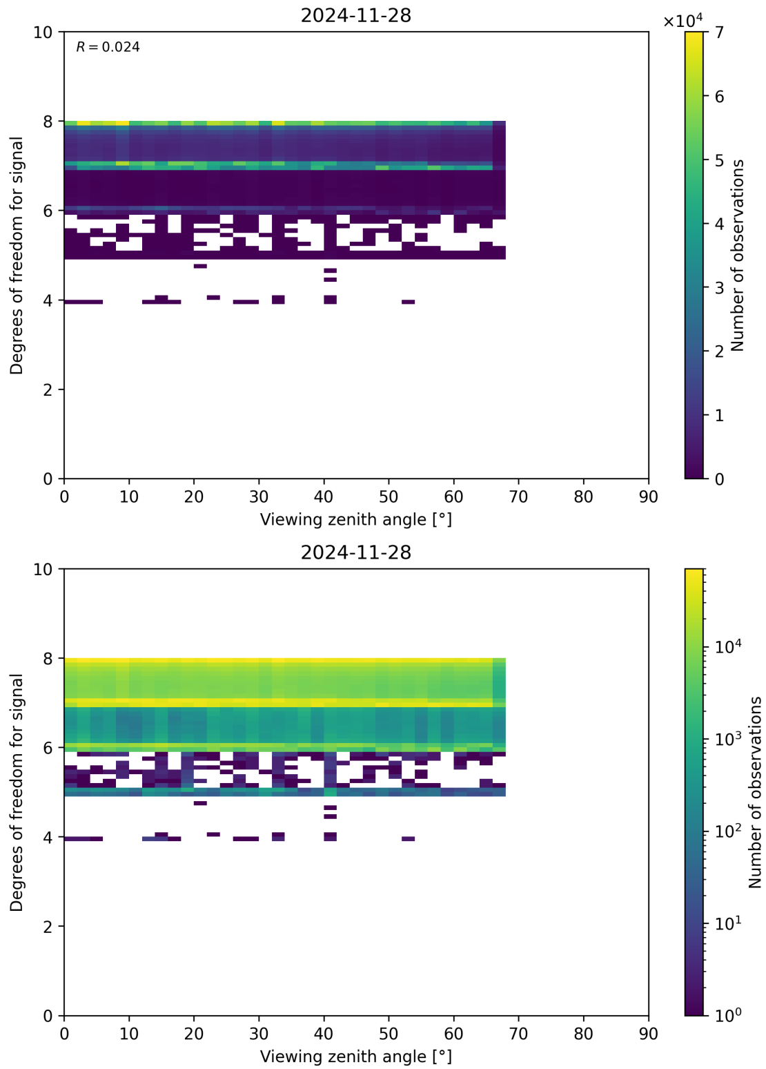
Figure 73: Scatter density plot of “Viewing zenith angle” against “Degrees of freedom for signal” for 2024-11-27 to 2024-11-29.
