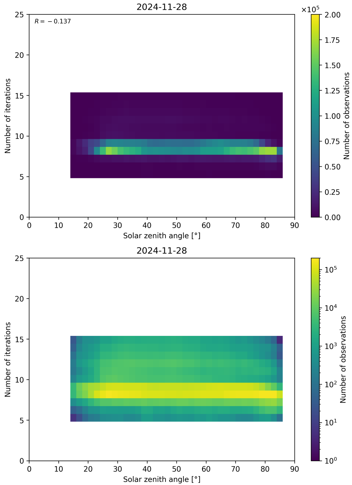
Figure 67: Scatter density plot of “Solar zenith angle” against “Number of iterations” for 2024-11-27 to 2024-11-29.
