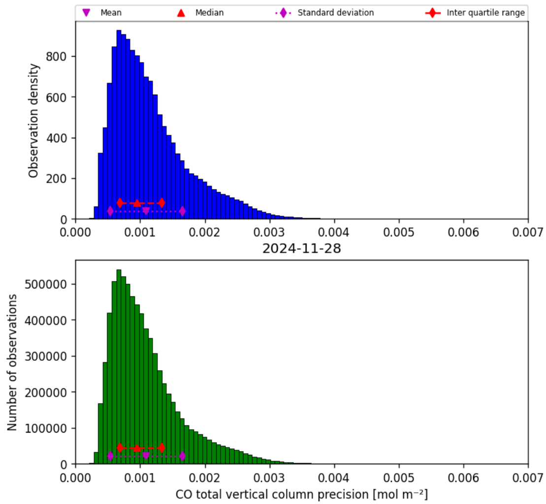
Figure 20: Histogram of “CO total vertical column precision” for 2024-11-27 to 2024-11-29
