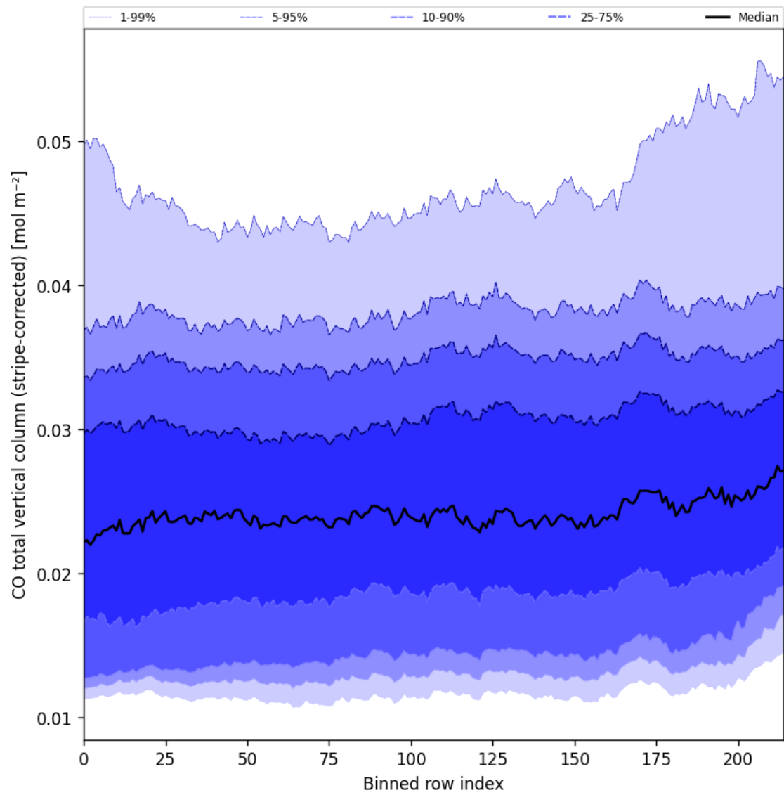
Figure 27: Along track statistics of “CO total vertical column (stripe-corrected)” for 2024-11-27 to 2024-11-29
