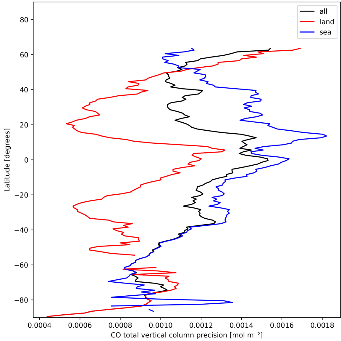
Figure 12: Zonal average of “CO total vertical column precision” for 2024-11-27 to 2024-11-29.
