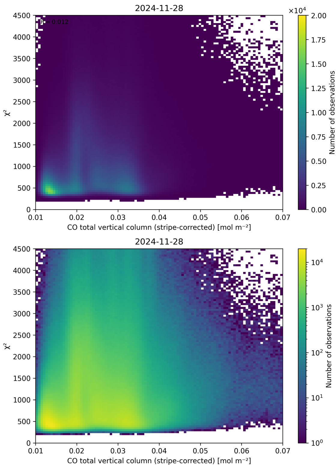
Figure 37: Scatter density plot of “CO total vertical column (stripe-corrected)” against “ \chi^2 ” for 2024-11-27 to 2024-11-29.
