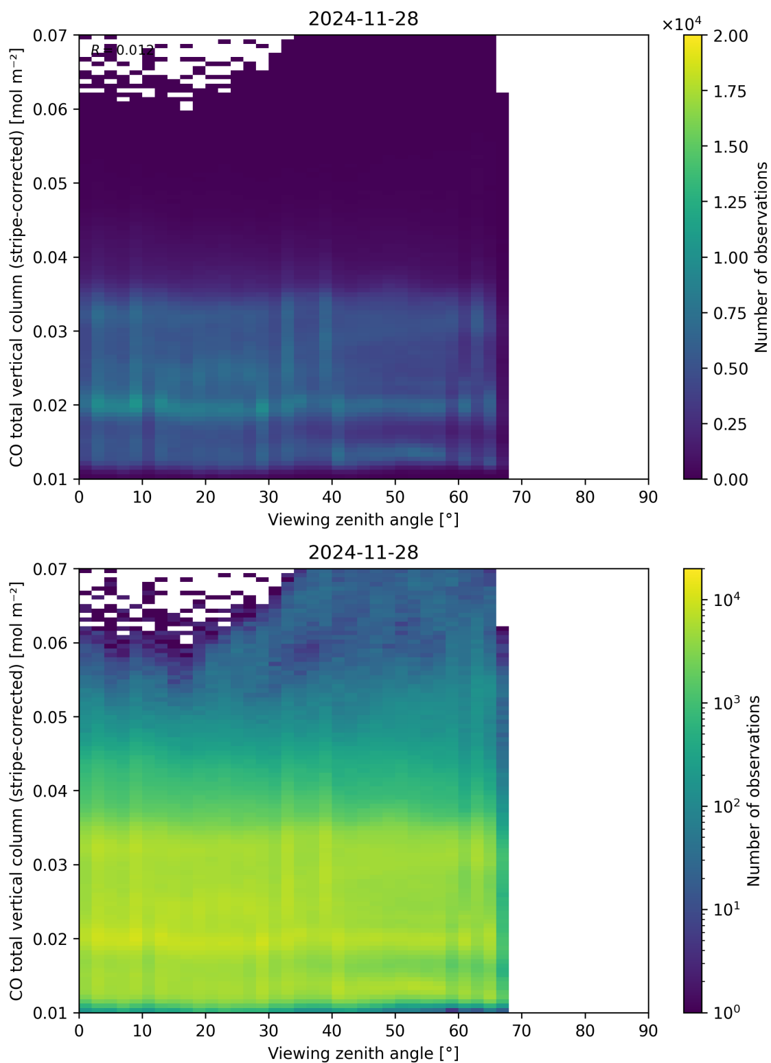
Figure 70: Scatter density plot of “Viewing zenith angle” against “CO total vertical column (stripe-corrected)” for 2024-11-27 to 2024-11-29.
