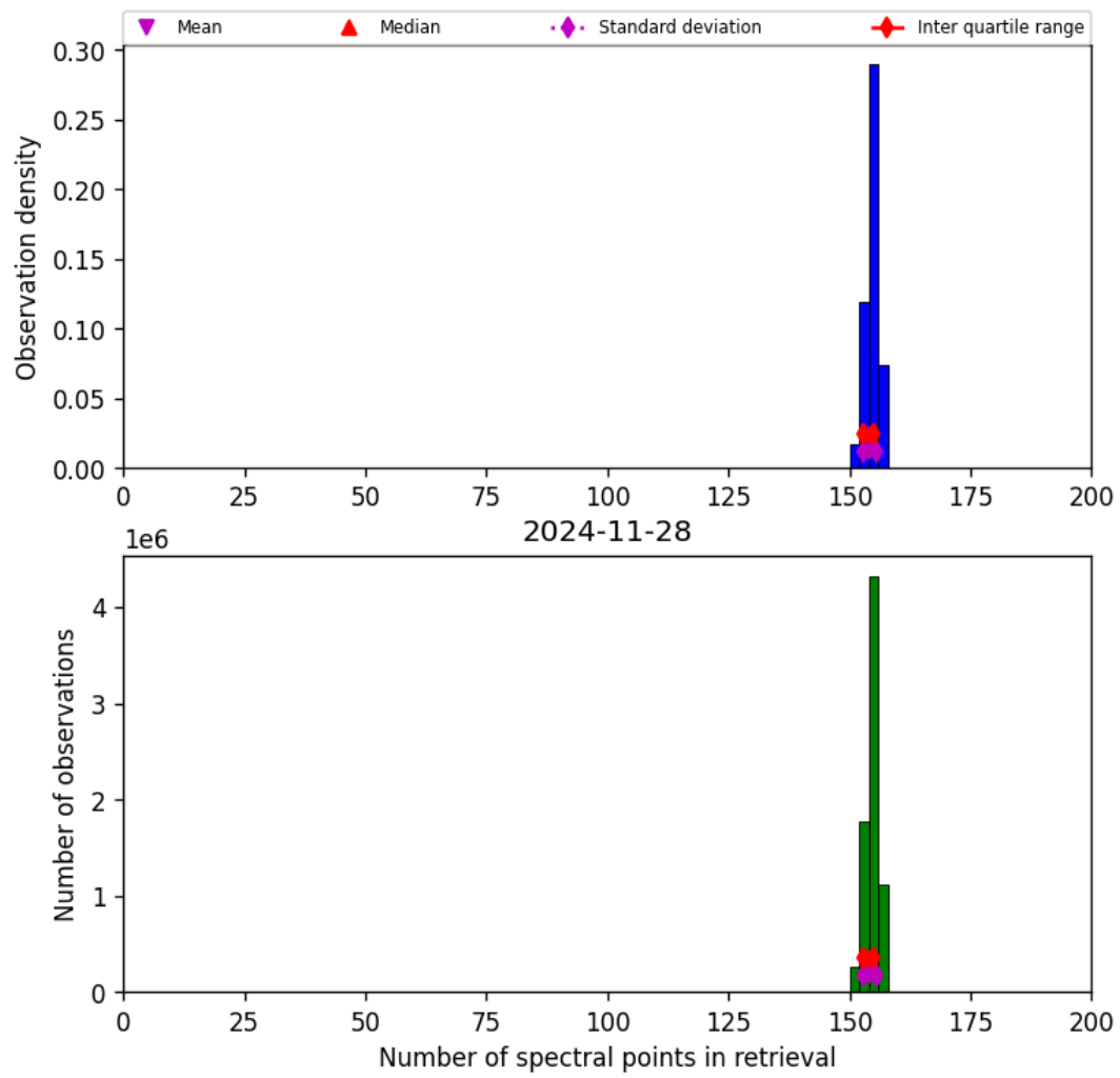
Figure 21: Histogram of “Number of spectral points in retrieval” for 2024-11-27 to 2024-11-29
