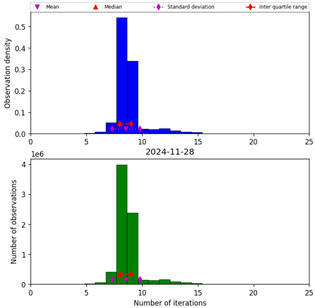
Figure 24: Histogram of “Number of iterations” for 2024-11-27 to 2024-11-29
