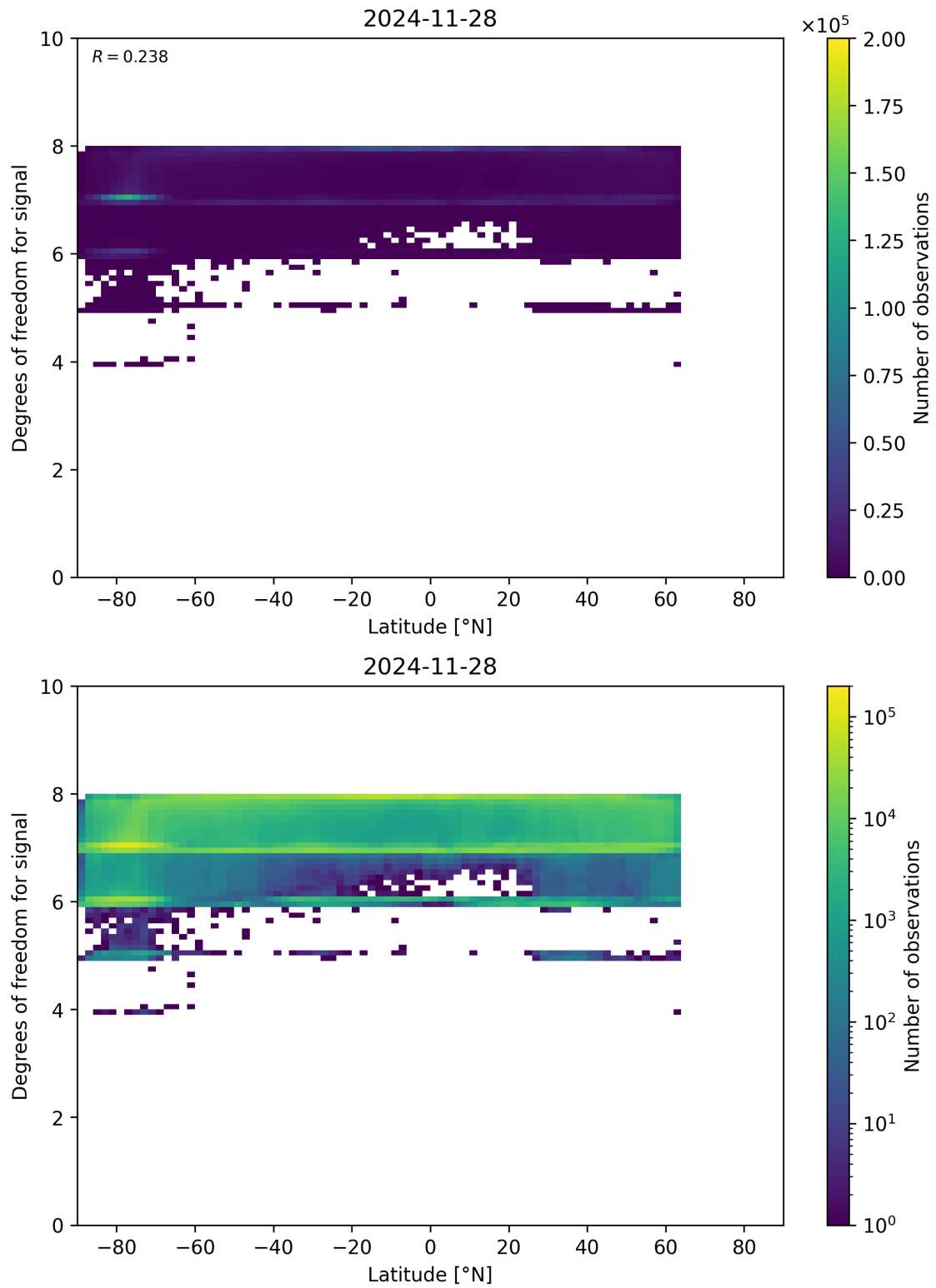
Figure 55: Scatter density plot of “Latitude” against “Degrees of freedom for signal” for 2024-11-27 to 2024-11-29.
