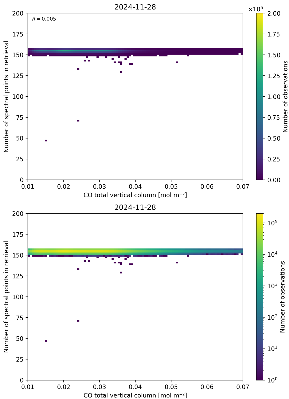
Figure 43: Scatter density plot of “CO total vertical column” against “Number of spectral points in retrieval” for 2024-11-27 to 2024-11-29.
