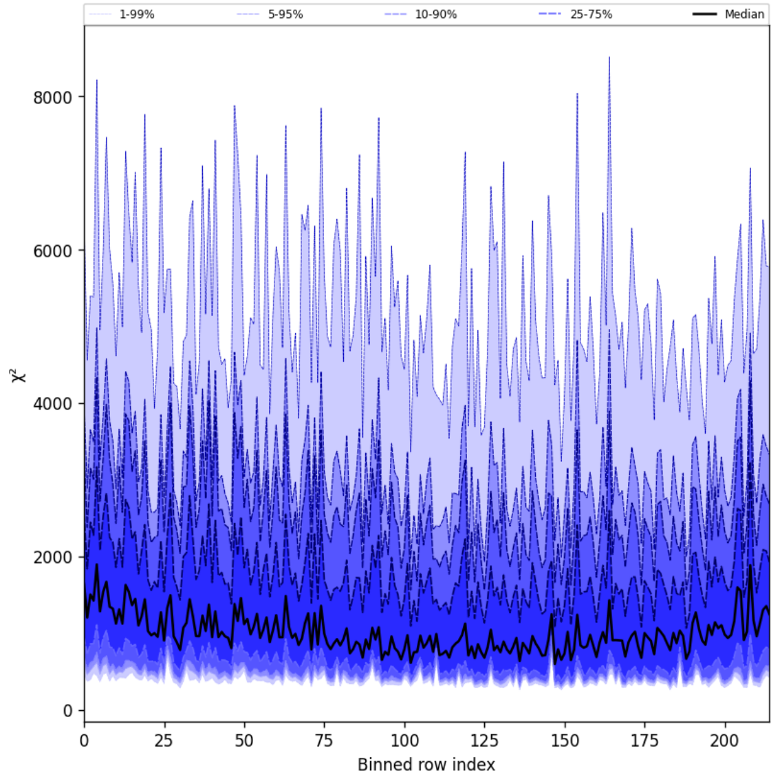
Figure 30: Along track statistics of “ \chi^2 ” for 2024-11-27 to 2024-11-29
