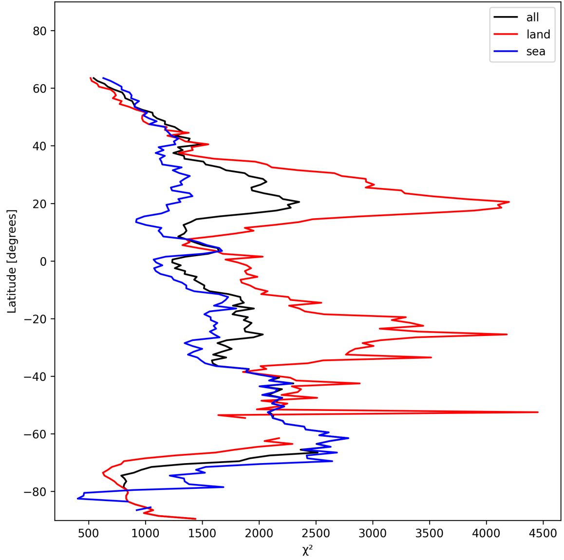
Figure 14: Zonal average of “ \chi^2 ” for 2024-11-27 to 2024-11-29.
