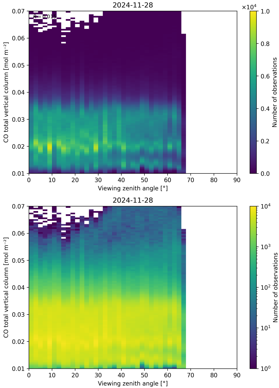
Figure 69: Scatter density plot of “Viewing zenith angle” against “CO total vertical column” for 2024-11-27 to 2024-11-29.
