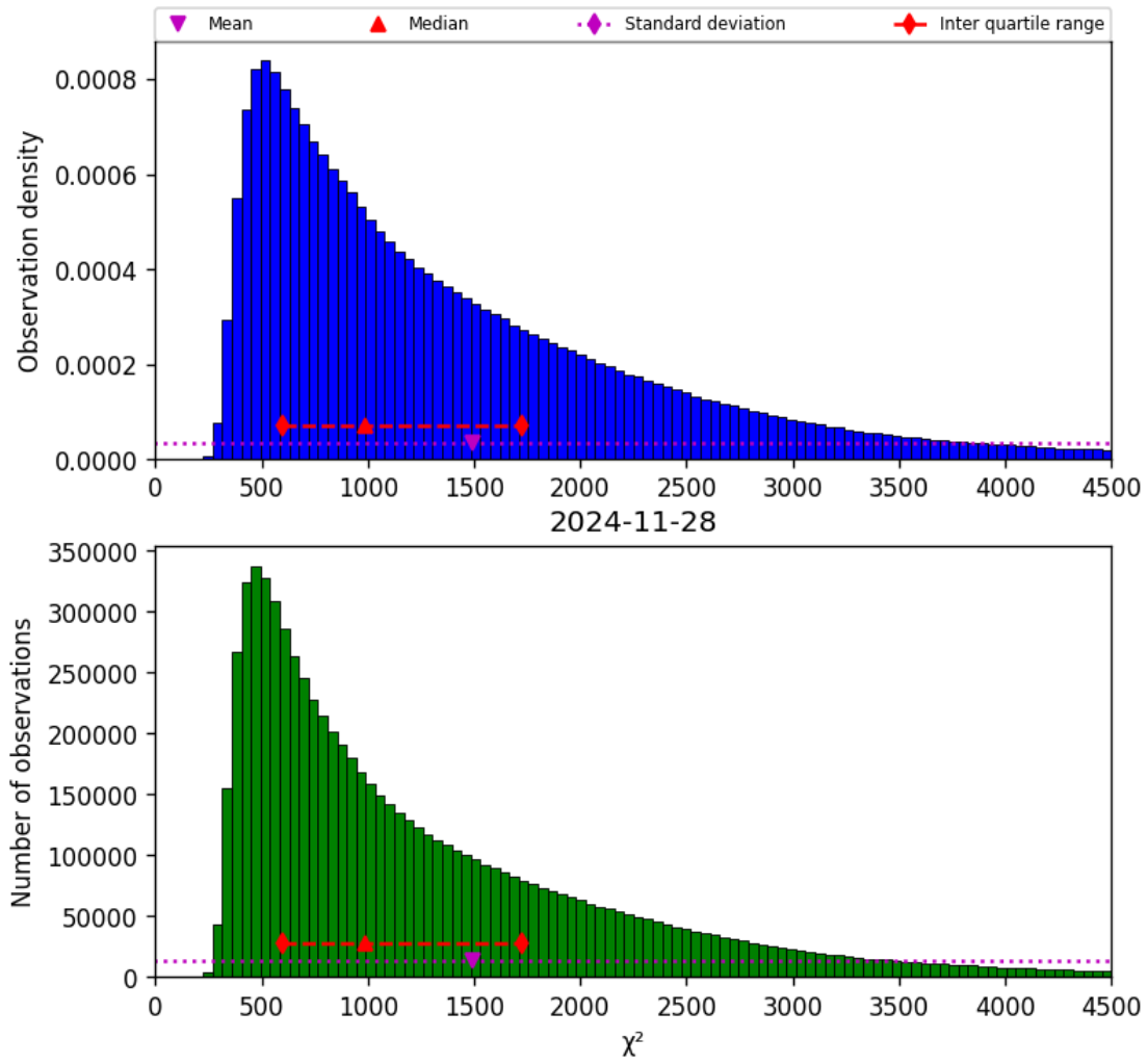
Figure 22: Histogram of “ \chi^2 ” for 2024-11-27 to 2024-11-29
