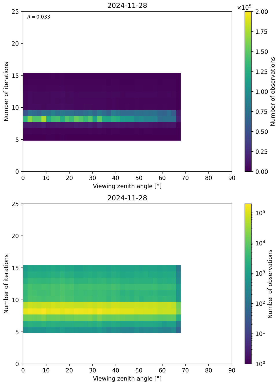
Figure 75: Scatter density plot of “Viewing zenith angle” against “Number of iterations” for 2024-11-27 to 2024-11-29.
