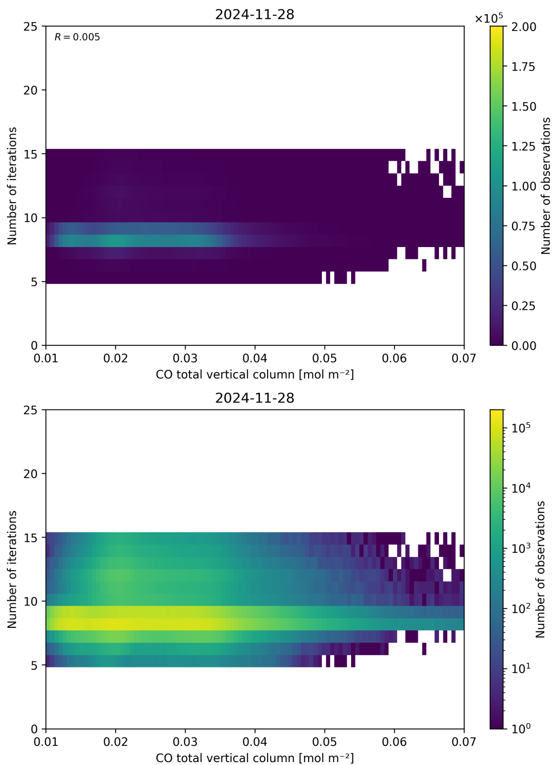
Figure 42: Scatter density plot of “CO total vertical column” against “Number of iterations” for 2024-11-27 to 2024-11-29.
