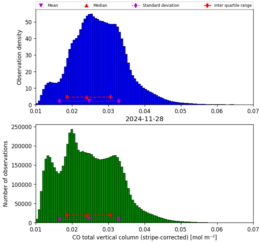
Figure 19: Histogram of “CO total vertical column (stripe-corrected)” for 2024-11-27 to 2024-11-29
