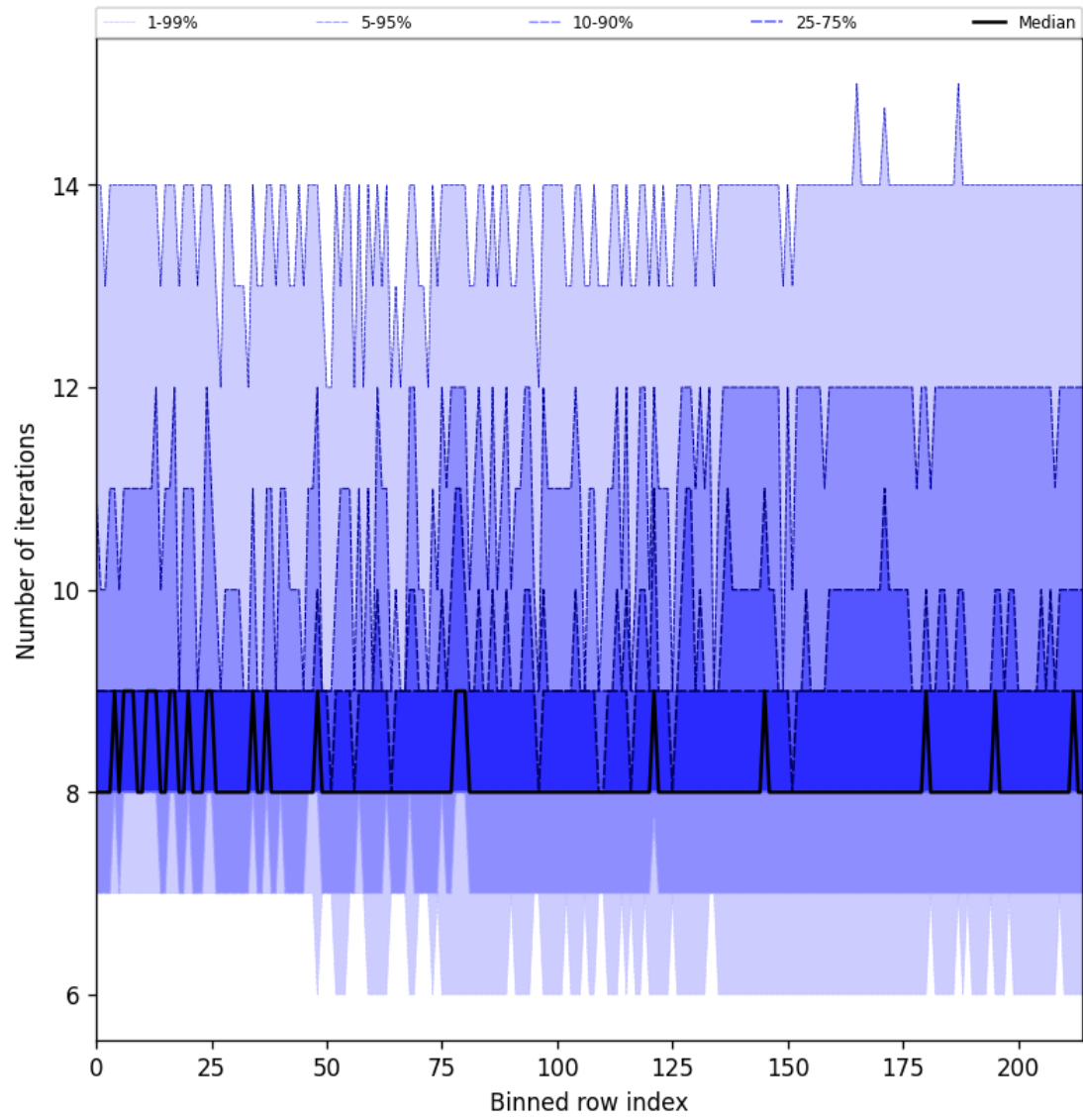
Figure 32: Along track statistics of “Number of iterations” for 2024-11-27 to 2024-11-29
