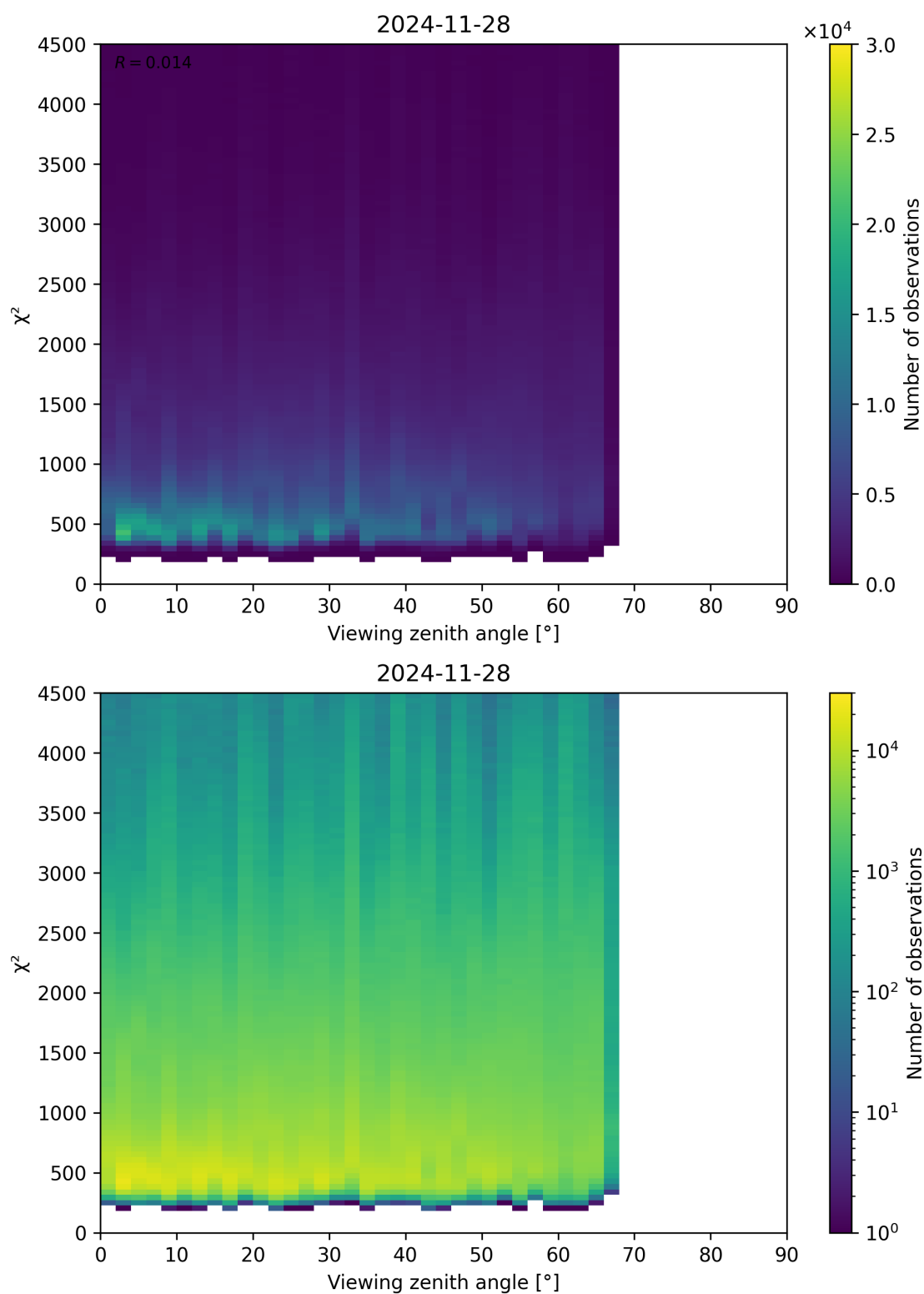
Figure 72: Scatter density plot of “Viewing zenith angle” against “ \chi^2 ” for 2024-11-27 to 2024-11-29.
