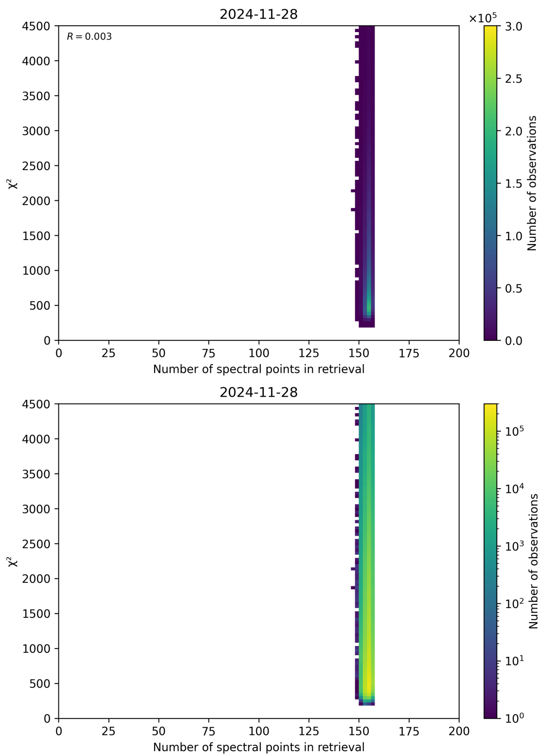
Figure 58: Scatter density plot of “Number of spectral points in retrieval” against “ \chi^2 ” for 2024-11-27 to 2024-11-29.
