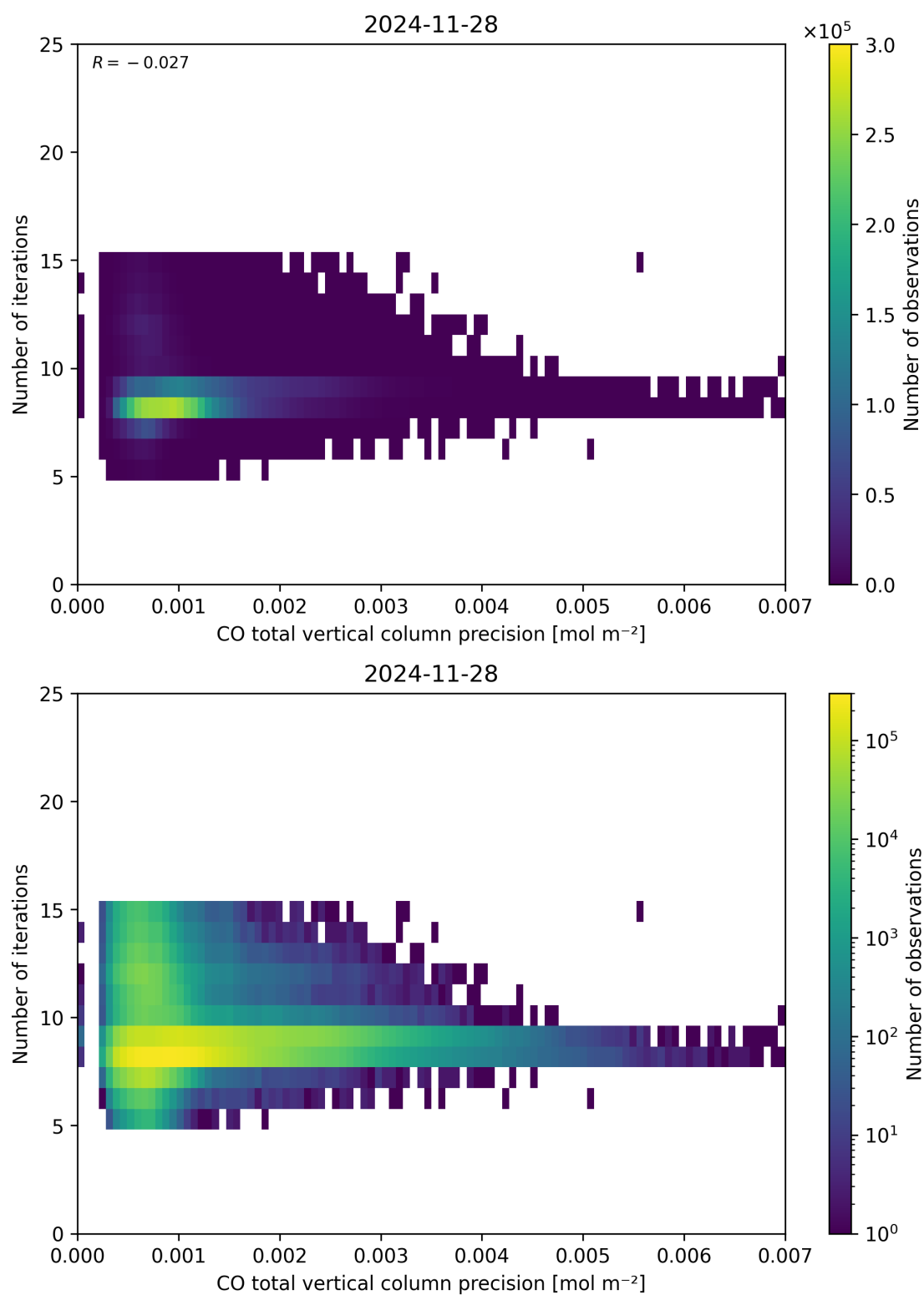
Figure 46: Scatter density plot of “CO total vertical column precision” against “Number of iterations” for 2024-11-27 to 2024-11-29.
