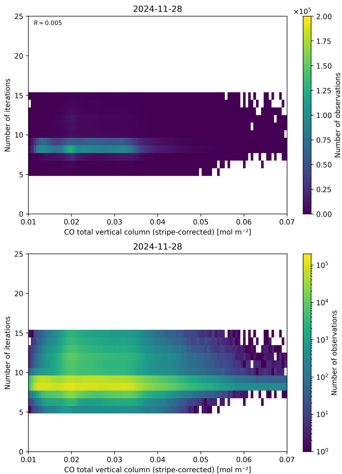
Figure 39: Scatter density plot of “CO total vertical column (stripe-corrected)” against “Number of iterations” for 2024-11-27 to 2024-11-29.
