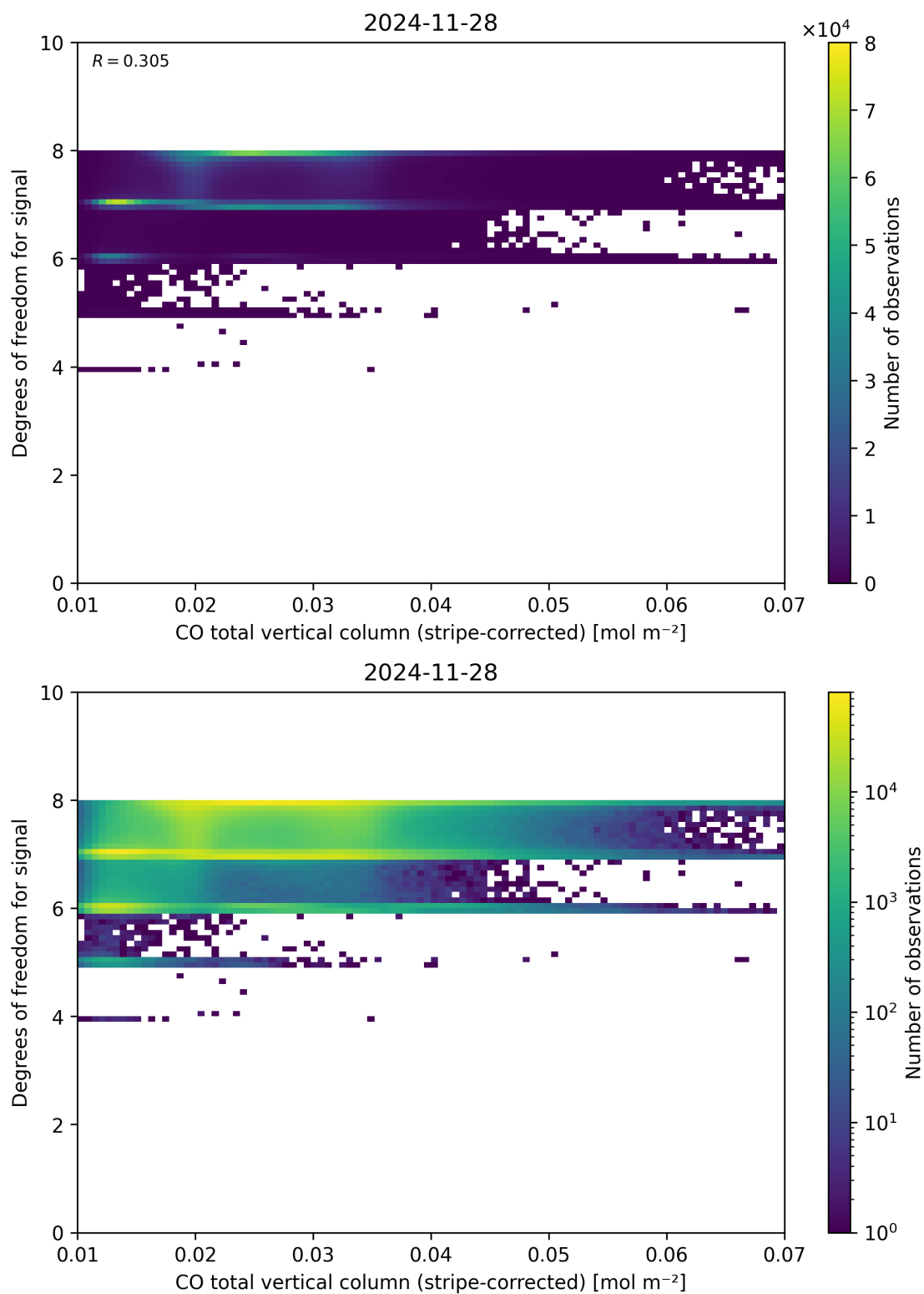
Figure 38: Scatter density plot of “CO total vertical column (stripe-corrected)” against “Degrees of freedom for signal” for 2024-11-27 to 2024-11-29.
