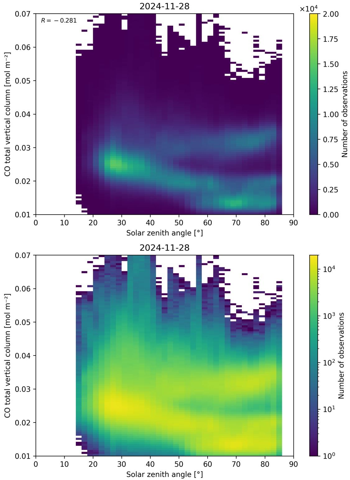
Figure 61: Scatter density plot of “Solar zenith angle” against “CO total vertical column” for 2024-11-27 to 2024-11-29.
