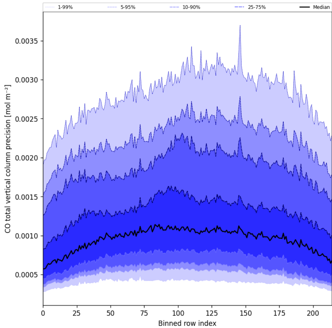
Figure 28: Along track statistics of “CO total vertical column precision” for 2024-11-27 to 2024-11-29
