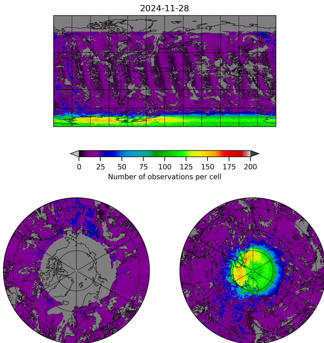
Figure 8: Map of the number of observations for 2024-11-27 to 2024-11-29
