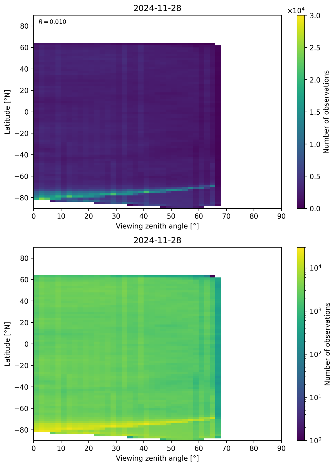
Figure 74: Scatter density plot of “Viewing zenith angle” against “Latitude” for 2024-11-27 to 2024-11-29.
