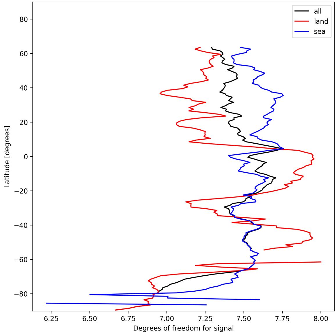
Figure 15: Zonal average of “Degrees of freedom for signal” for 2024-11-27 to 2024-11-29.
