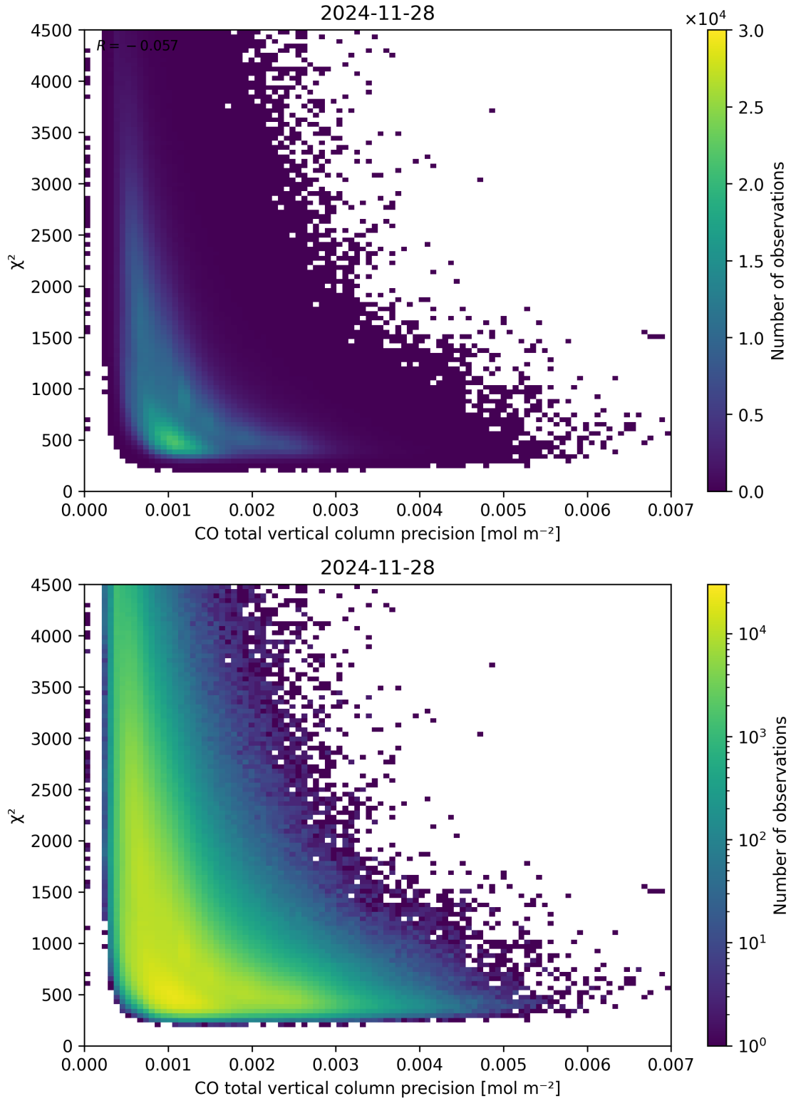
Figure 44: Scatter density plot of “CO total vertical column precision” against “ \chi^2 ” for 2024-11-27 to 2024-11-29.
