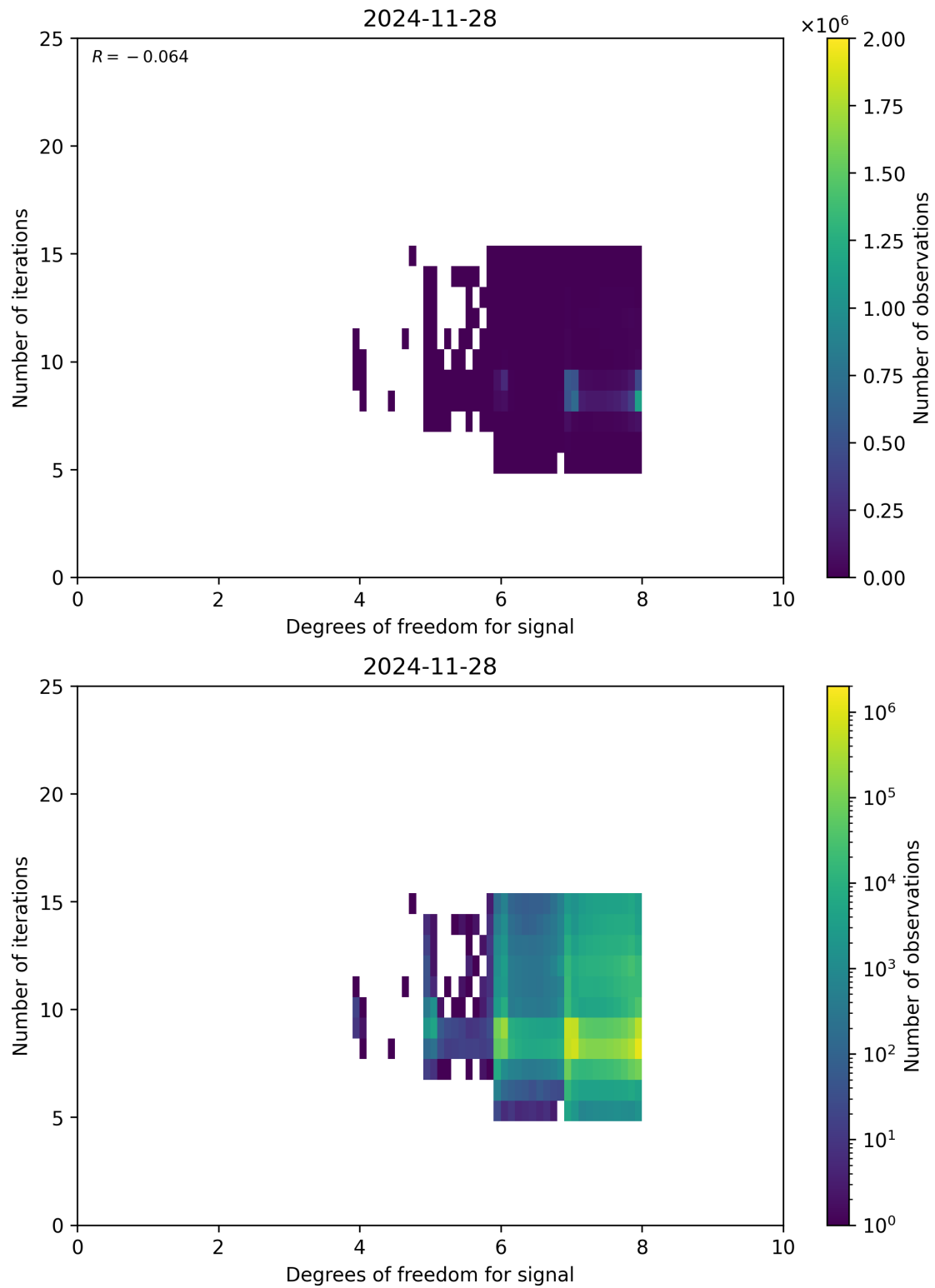
Figure 50: Scatter density plot of “Degrees of freedom for signal” against “Number of iterations” for 2024-11-27 to 2024-11-29.
