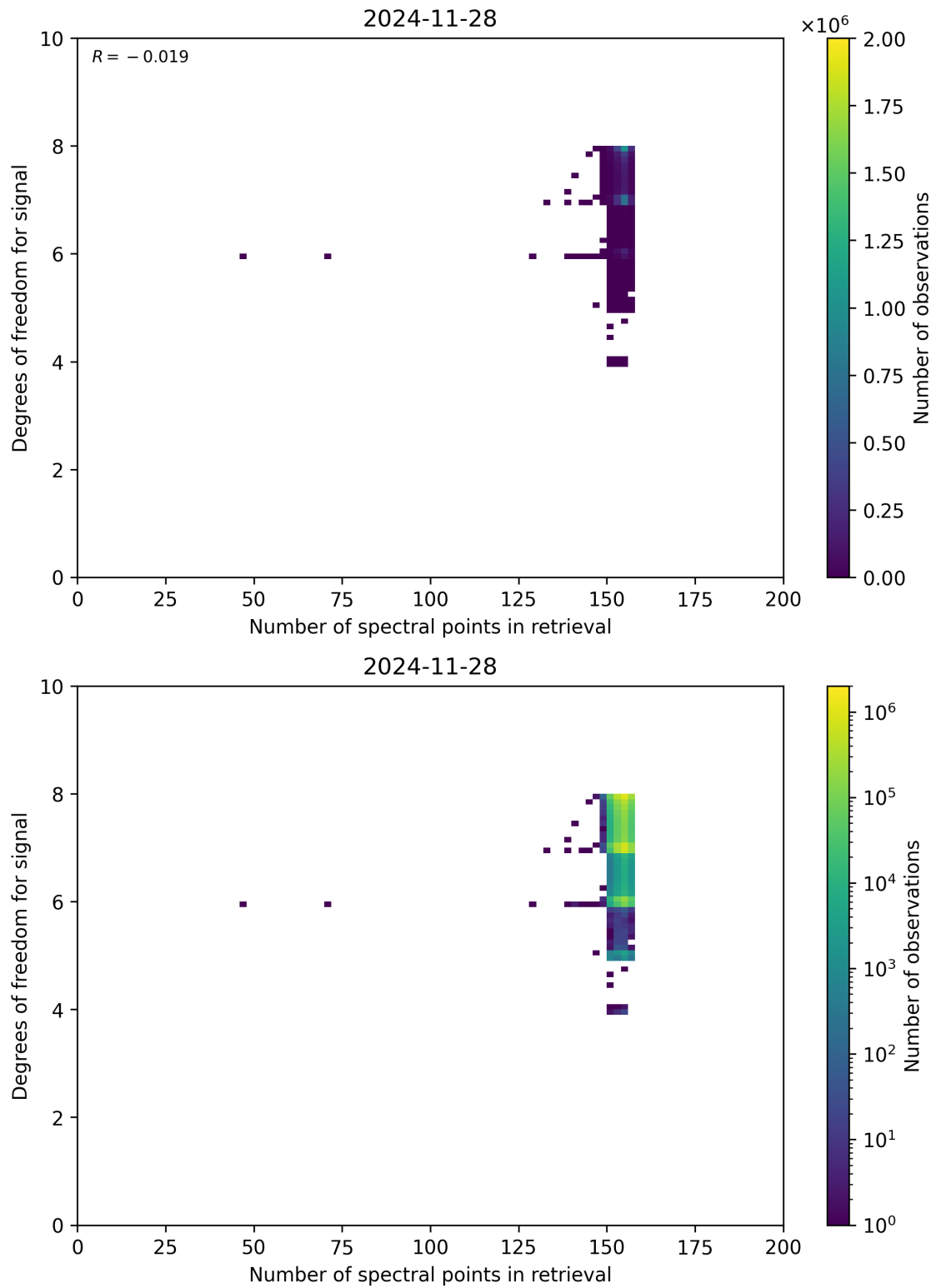
Figure 59: Scatter density plot of “Number of spectral points in retrieval” against “Degrees of freedom for signal” for 2024-11-27 to 2024-11-29.
