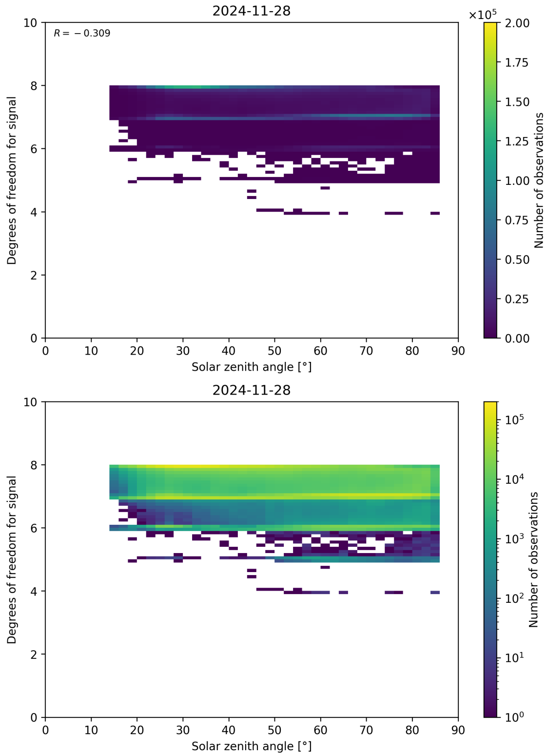
Figure 65: Scatter density plot of “Solar zenith angle” against “Degrees of freedom for signal” for 2024-11-27 to 2024-11-29.
