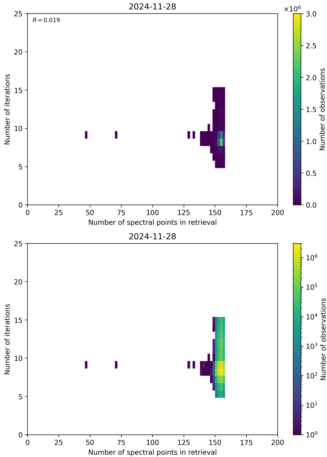
Figure 60: Scatter density plot of “Number of spectral points in retrieval” against “Number of iterations” for 2024-11-27 to 2024-11-29.
