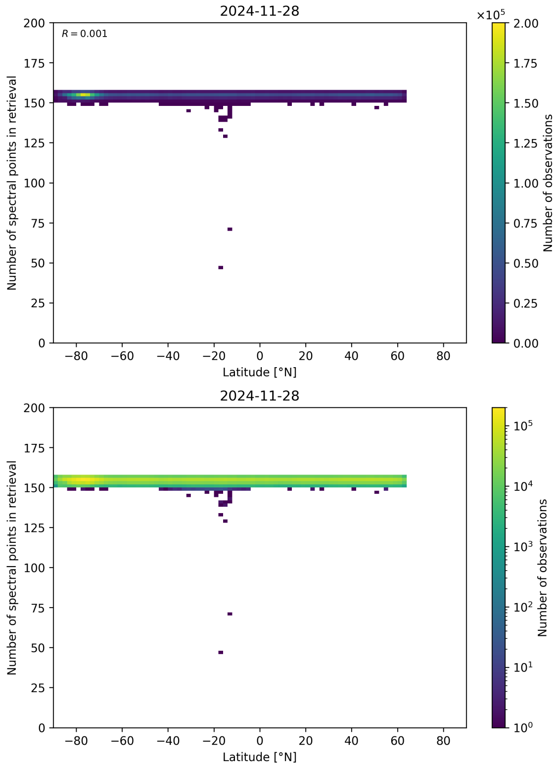
Figure 57: Scatter density plot of “Latitude” against “Number of spectral points in retrieval” for 2024-11-27 to 2024-11-29.
