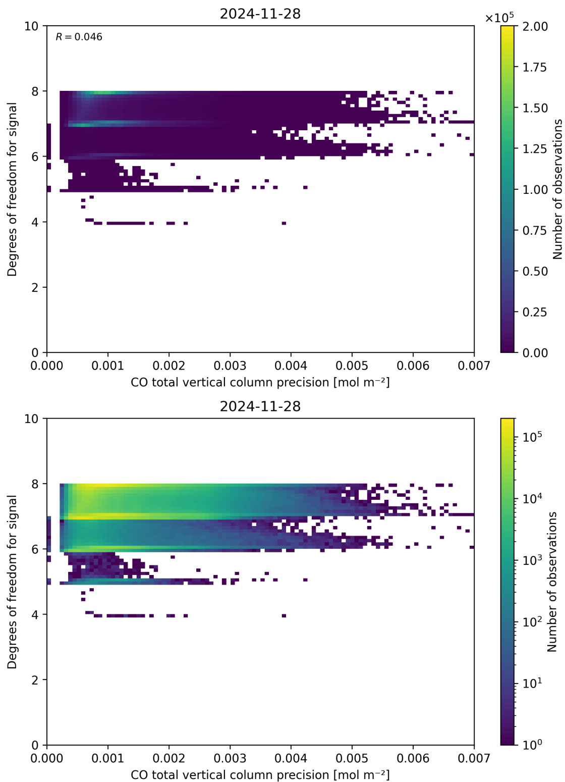
Figure 45: Scatter density plot of “CO total vertical column precision” against “Degrees of freedom for signal” for 2024-11-27 to 2024-11-29.
