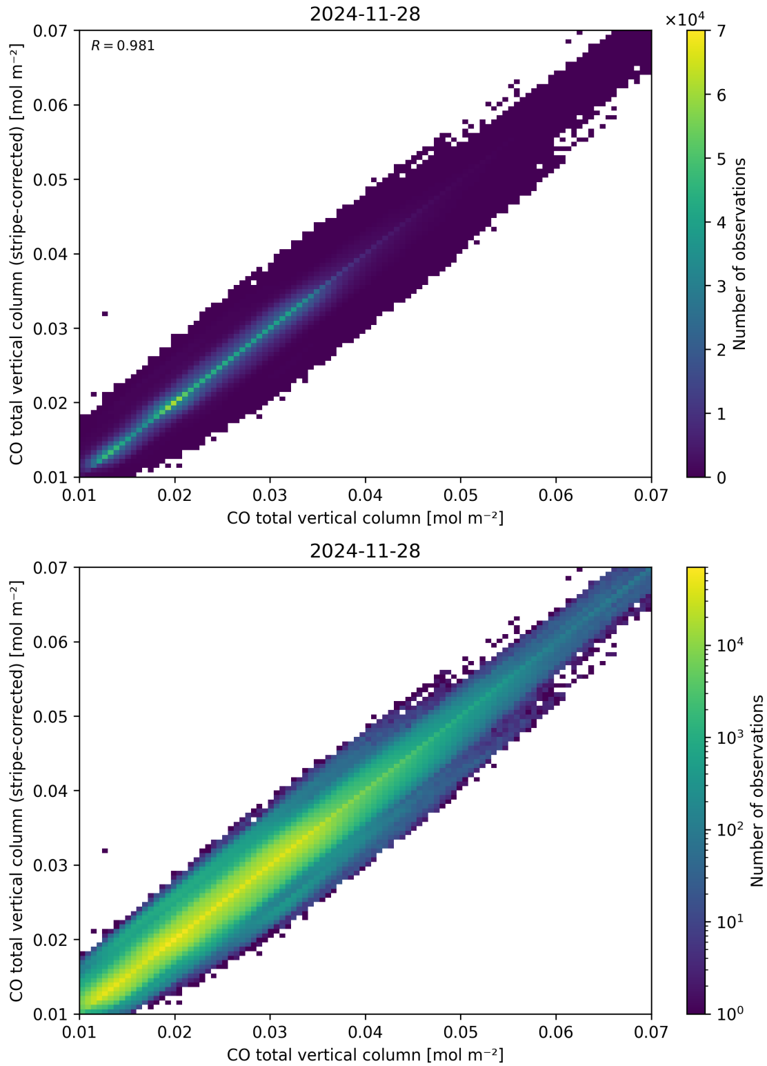
Figure 33: Scatter density plot of “CO total vertical column” against “CO total vertical column (stripe-corrected)” for 2024-11-27 to 2024-11-29.
