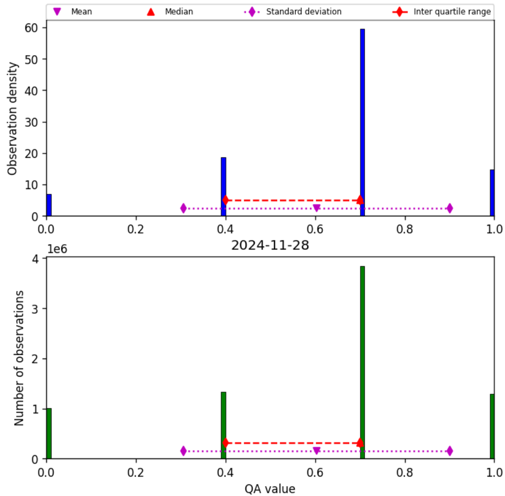
Figure 17: Histogram of “QA value” for 2024-11-27 to 2024-11-29
