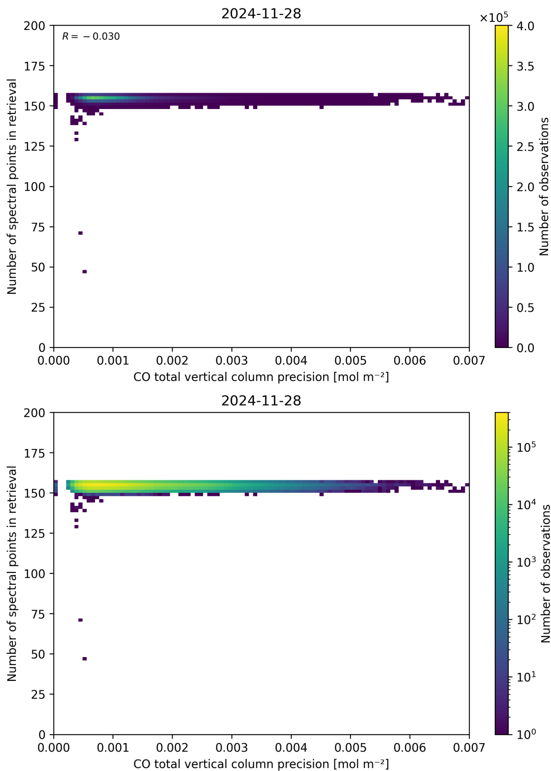
Figure 47: Scatter density plot of “CO total vertical column precision” against “Number of spectral points in retrieval” for 2024-11-27 to 2024-11-29.
