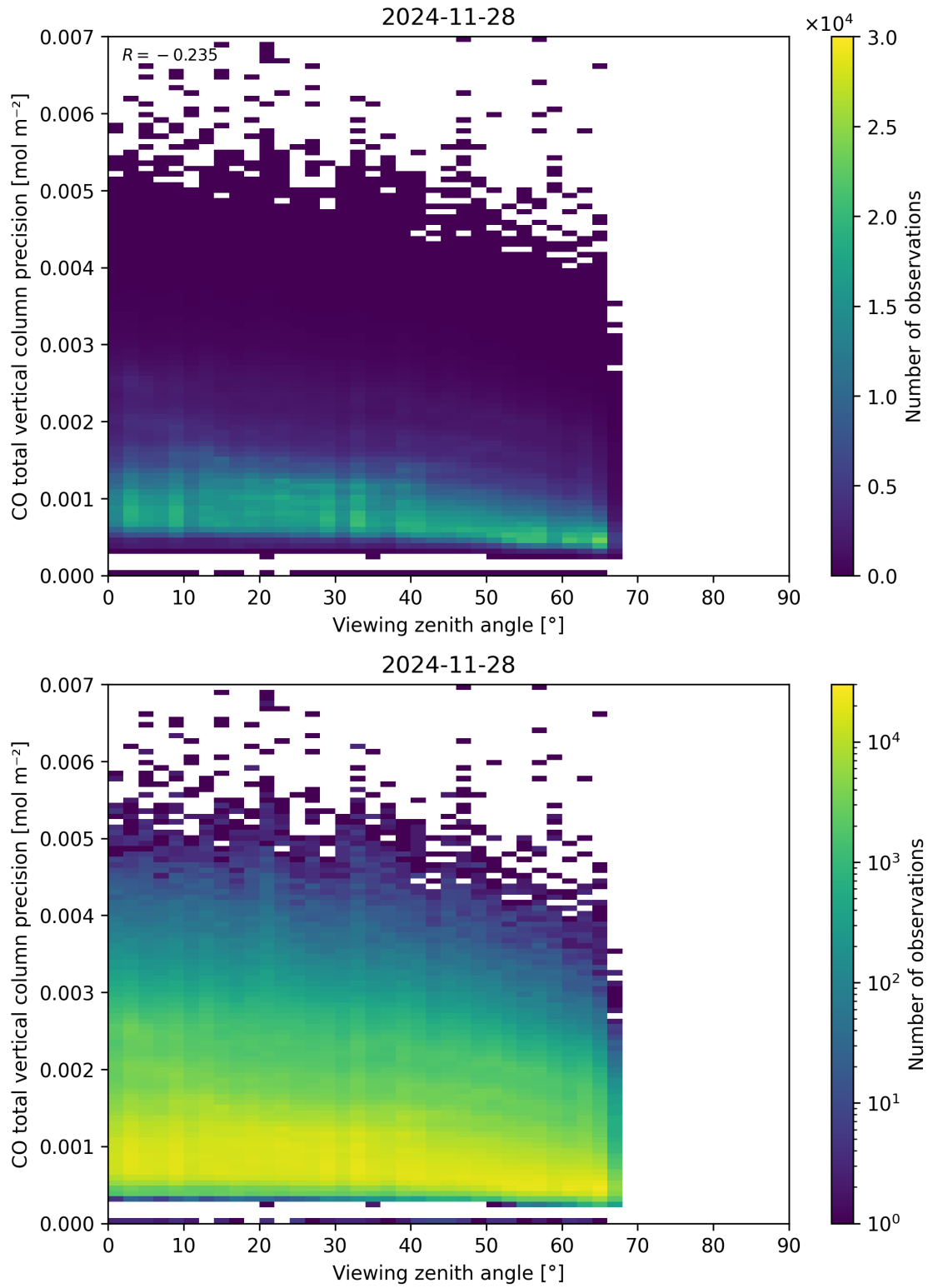
Figure 71: Scatter density plot of “Viewing zenith angle” against “CO total vertical column precision” for 2024-11-27 to 2024-11-29.
