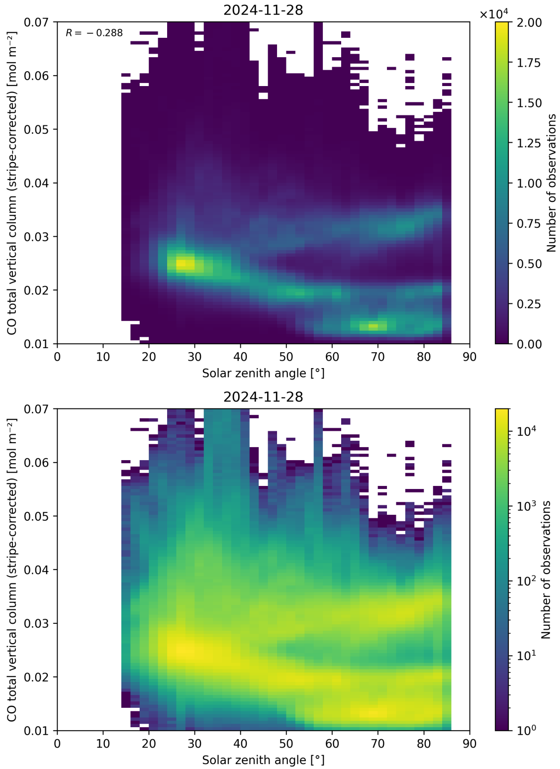
Figure 62: Scatter density plot of “Solar zenith angle” against “CO total vertical column (stripe-corrected)” for 2024-11-27 to 2024-11-29.
