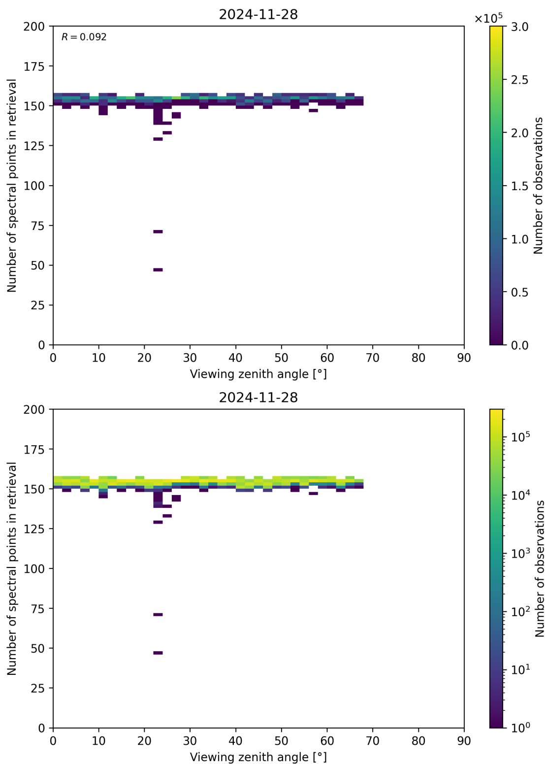
Figure 76: Scatter density plot of “Viewing zenith angle” against “Number of spectral points in retrieval” for 2024-11-27 to 2024-11-29.
