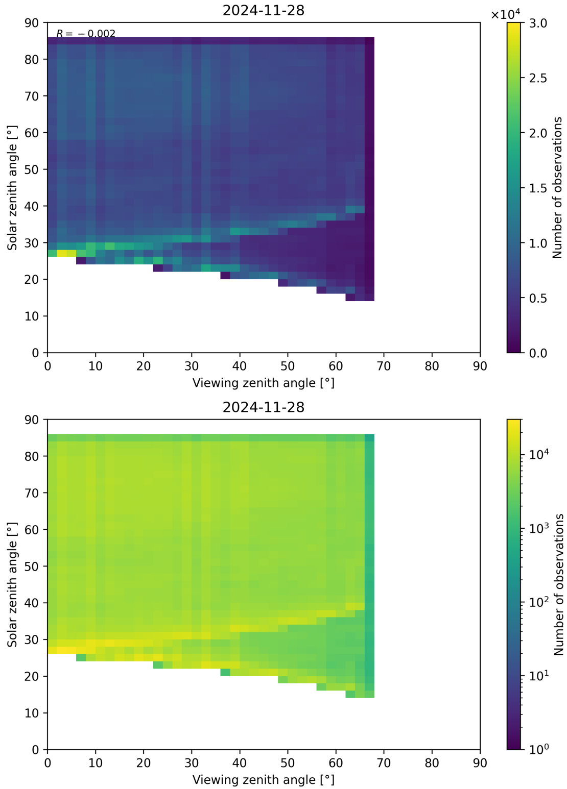
Figure 77: Scatter density plot of “Viewing zenith angle” against “Solar zenith angle” for 2024-11-27 to 2024-11-29.
