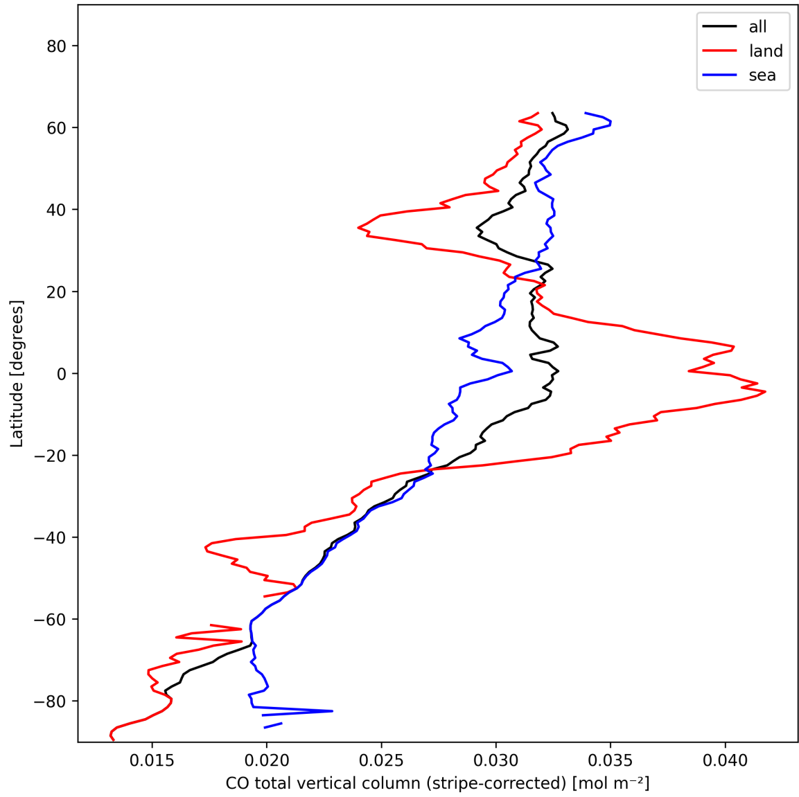
Figure 11: Zonal average of “CO total vertical column (stripe-corrected)” for 2024-11-27 to 2024-11-29.
