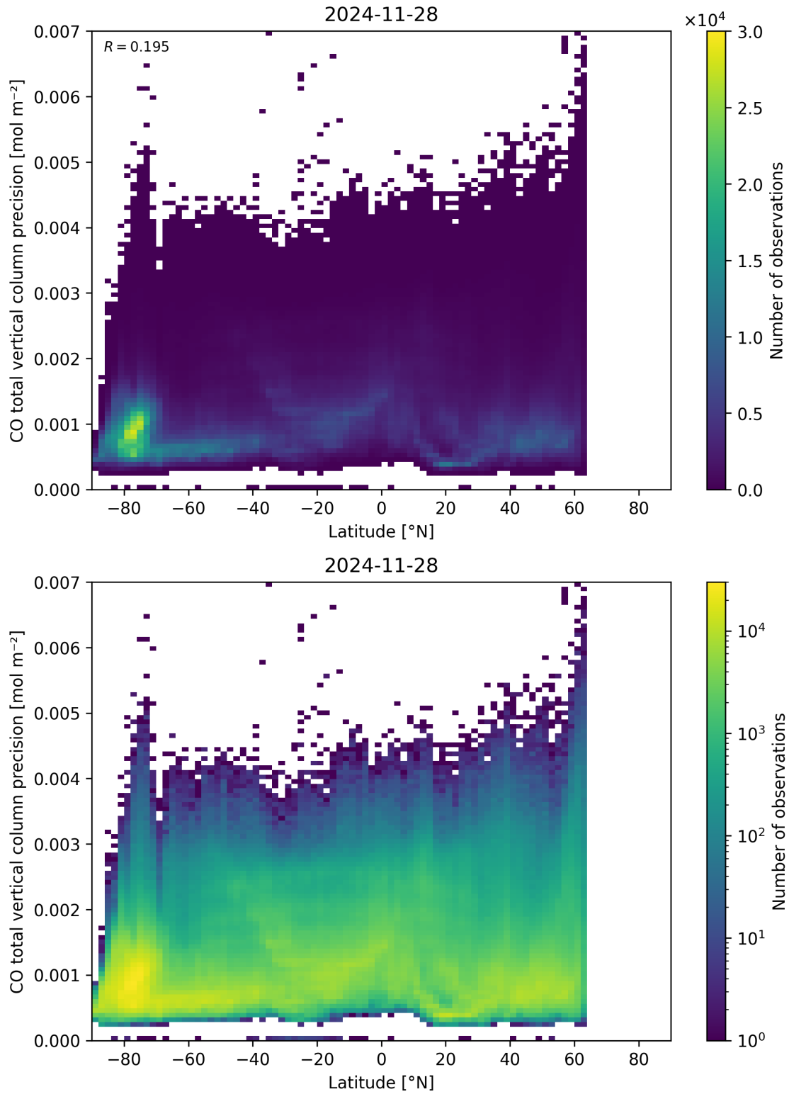
Figure 53: Scatter density plot of “Latitude” against “CO total vertical column precision” for 2024-11-27 to 2024-11-29.
