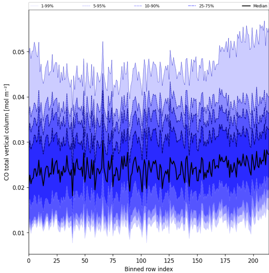
Figure 26: Along track statistics of “CO total vertical column” for 2024-11-27 to 2024-11-29
