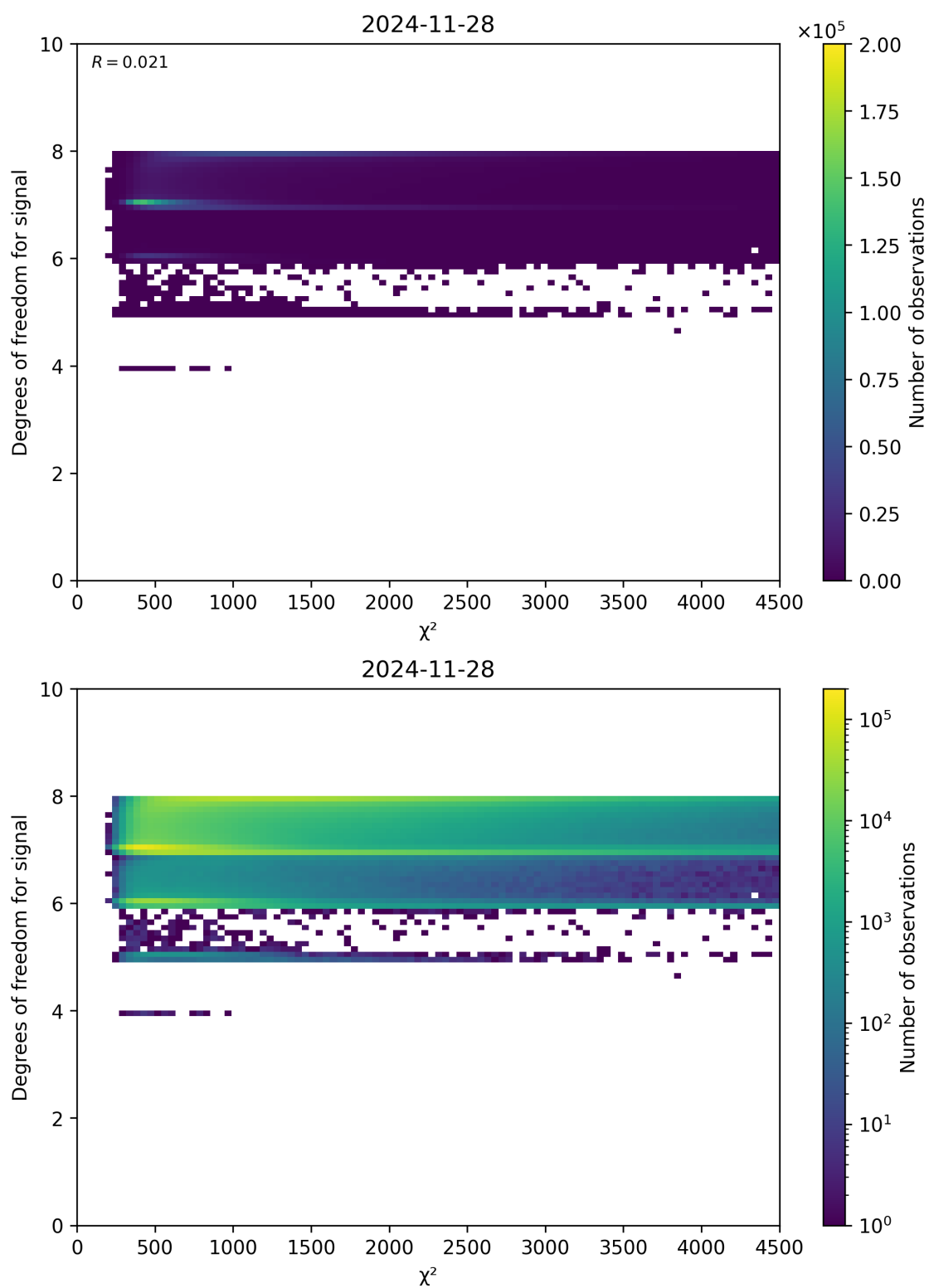
Figure 48: Scatter density plot of “ \chi^2 ” against “Degrees of freedom for signal” for 2024-11-27 to 2024-11-29.
