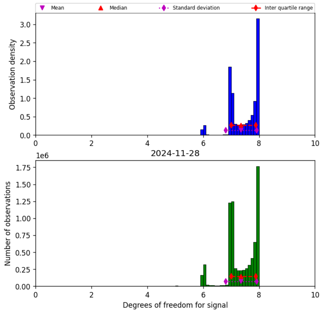
Figure 23: Histogram of “Degrees of freedom for signal” for 2024-11-27 to 2024-11-29
