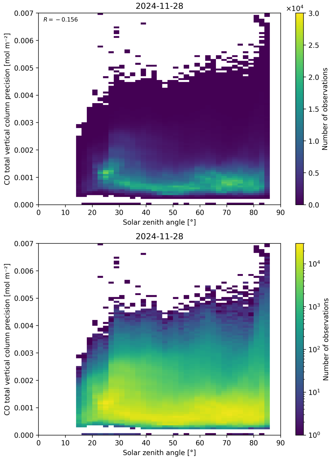
Figure 63: Scatter density plot of “Solar zenith angle” against “CO total vertical column precision” for 2024-11-27 to 2024-11-29.
