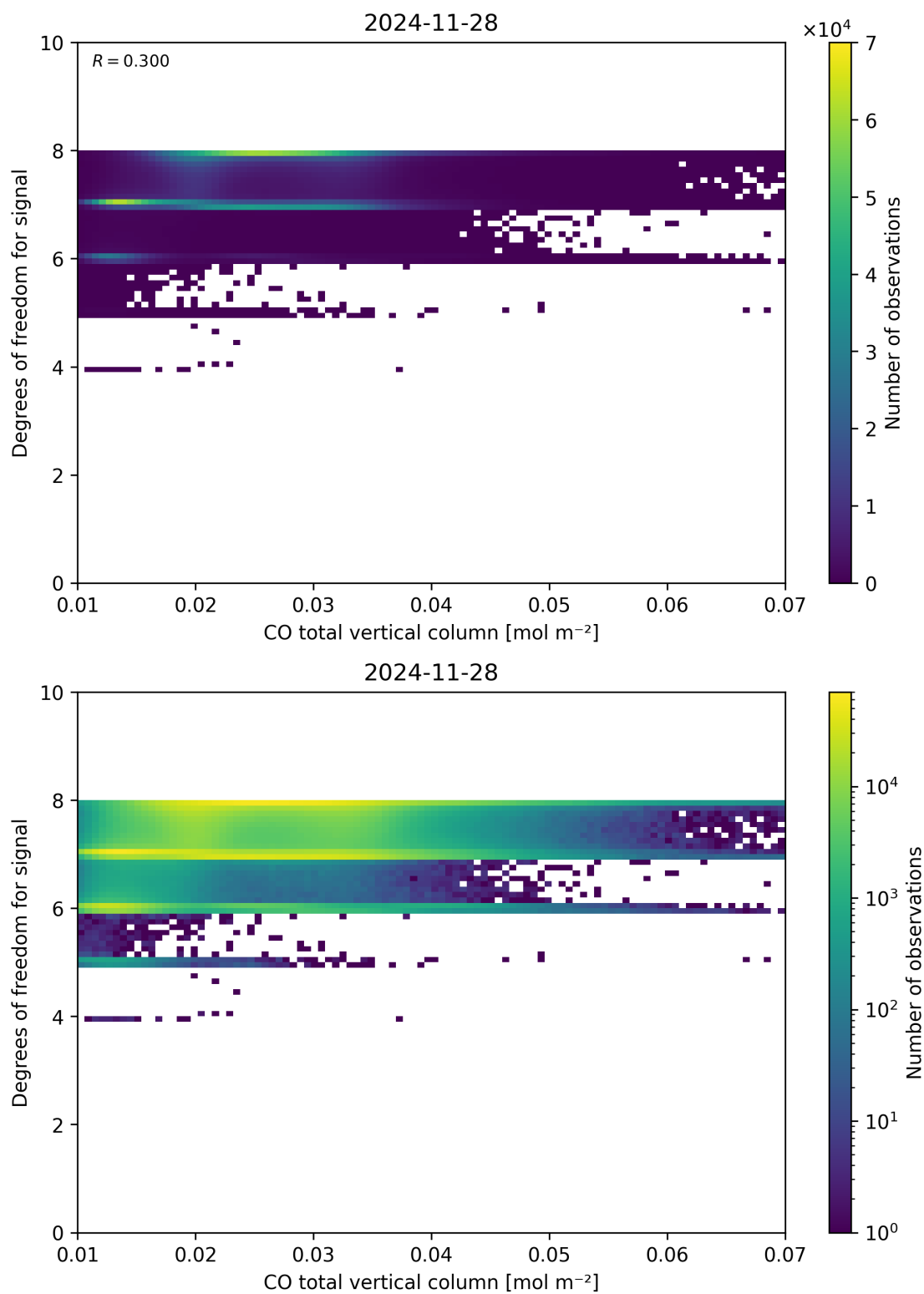
Figure 41: Scatter density plot of “CO total vertical column” against “Degrees of freedom for signal” for 2024-11-27 to 2024-11-29.
