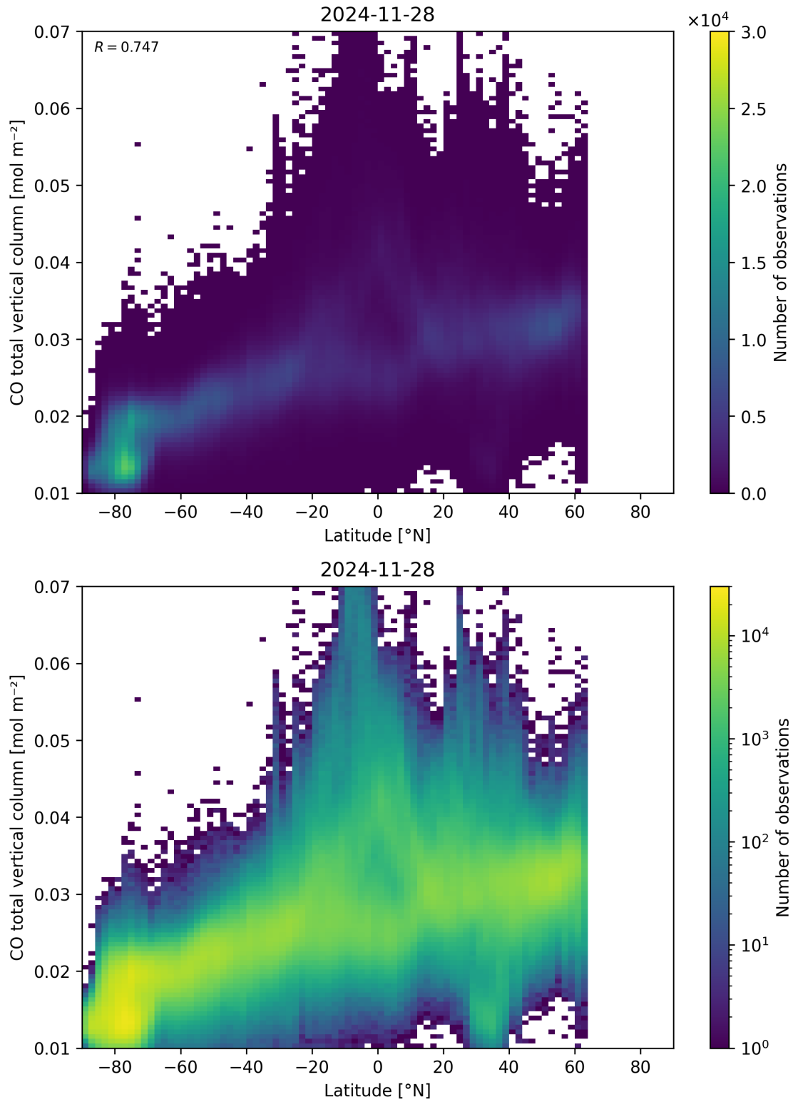
Figure 51: Scatter density plot of “Latitude” against “CO total vertical column” for 2024-11-27 to 2024-11-29.
