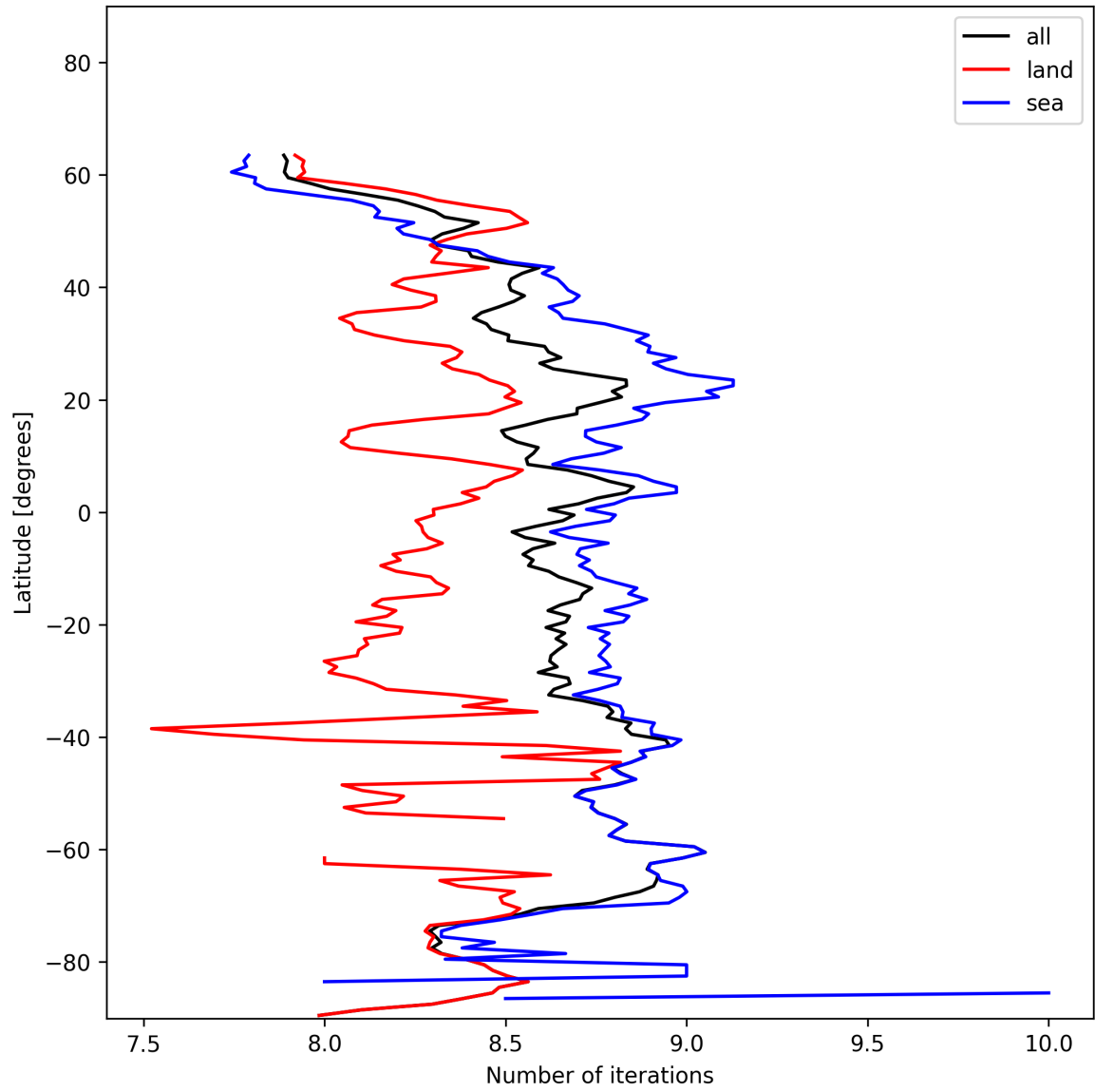
Figure 16: Zonal average of “Number of iterations” for 2024-11-27 to 2024-11-29.
