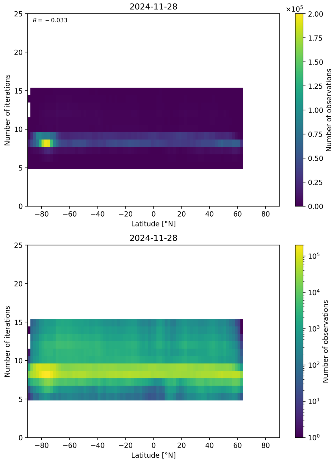
Figure 56: Scatter density plot of “Latitude” against “Number of iterations” for 2024-11-27 to 2024-11-29.
