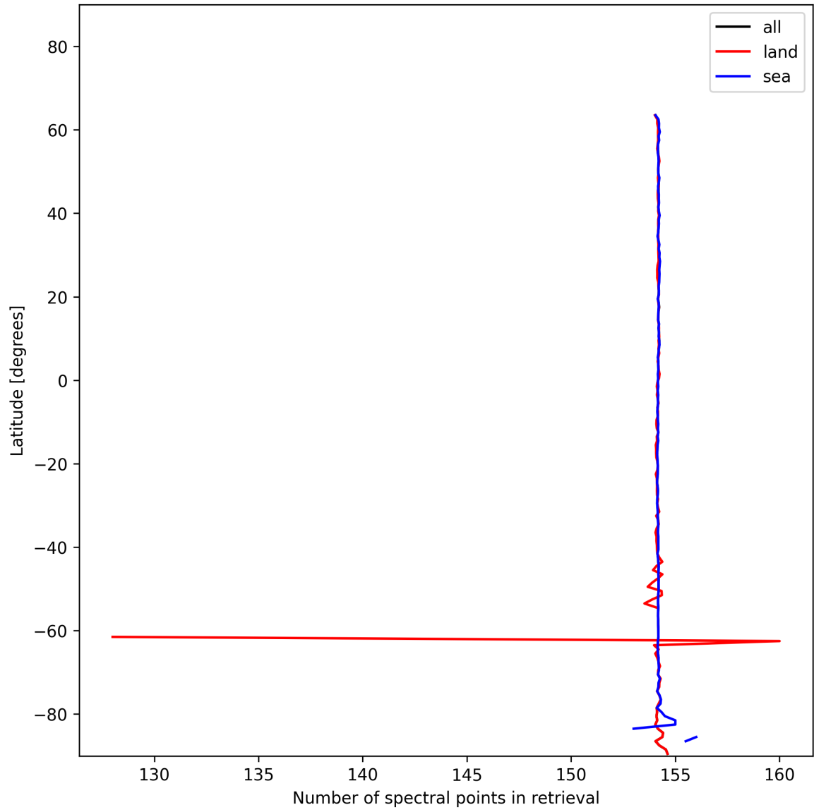
Figure 13: Zonal average of “Number of spectral points in retrieval” for 2024-11-27 to 2024-11-29.
