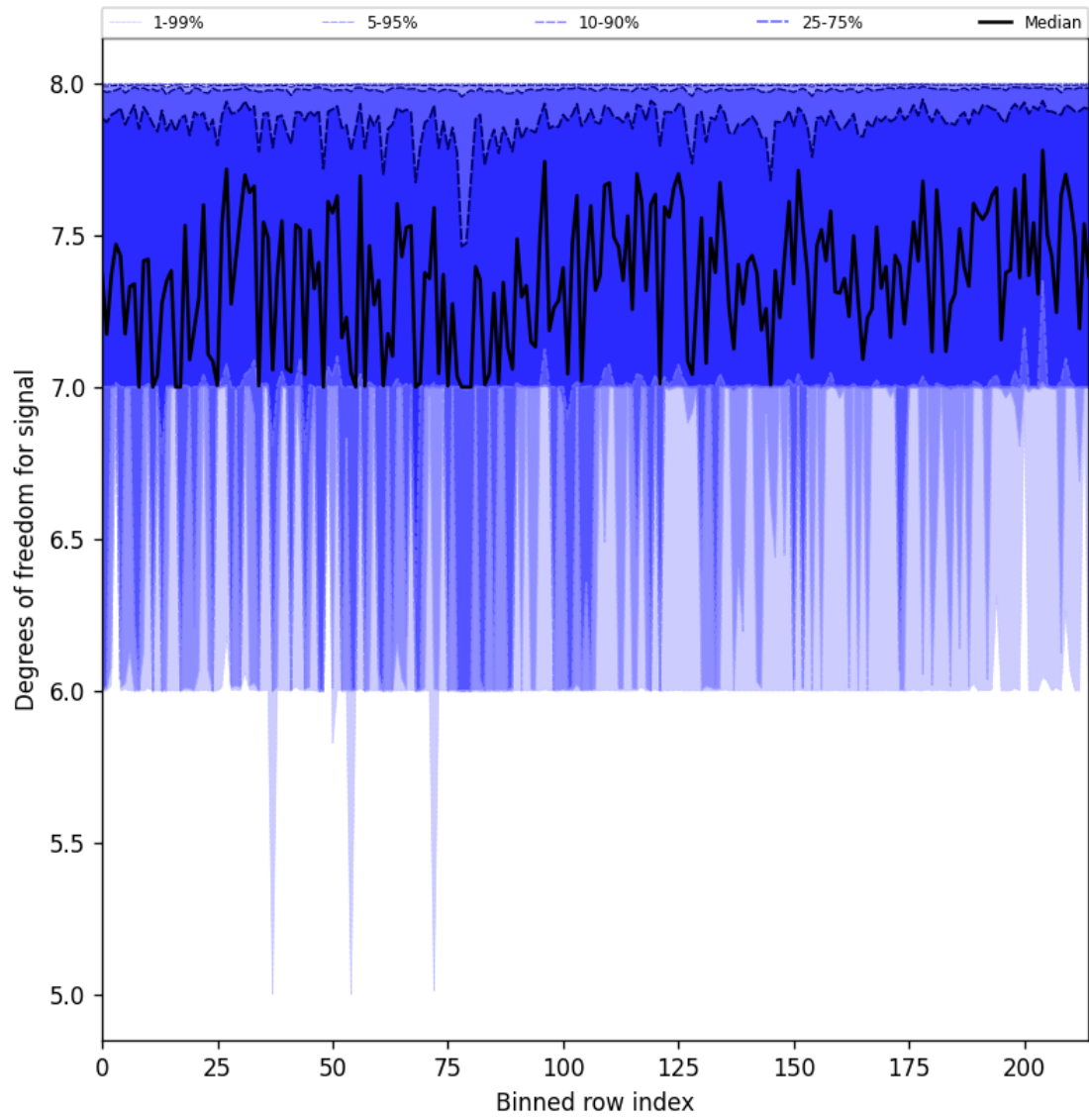
Figure 31: Along track statistics of “Degrees of freedom for signal” for 2024-11-27 to 2024-11-29
