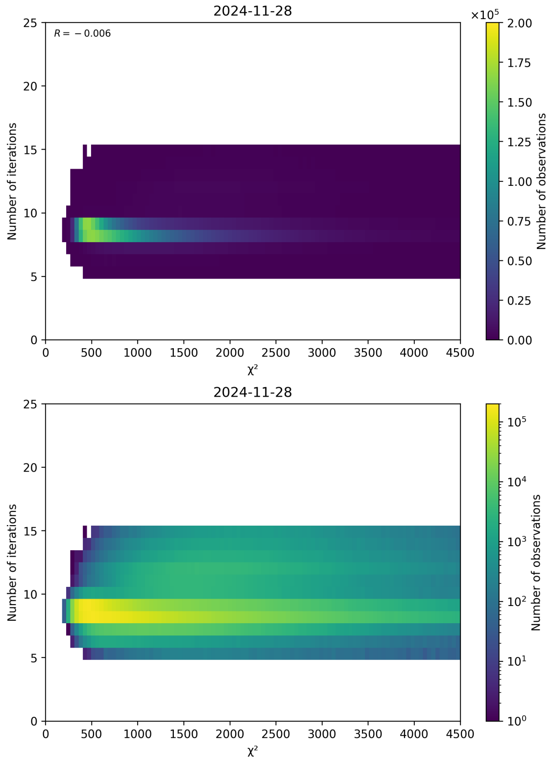
Figure 49: Scatter density plot of “ \chi^2 ” against “Number of iterations” for 2024-11-27 to 2024-11-29.
