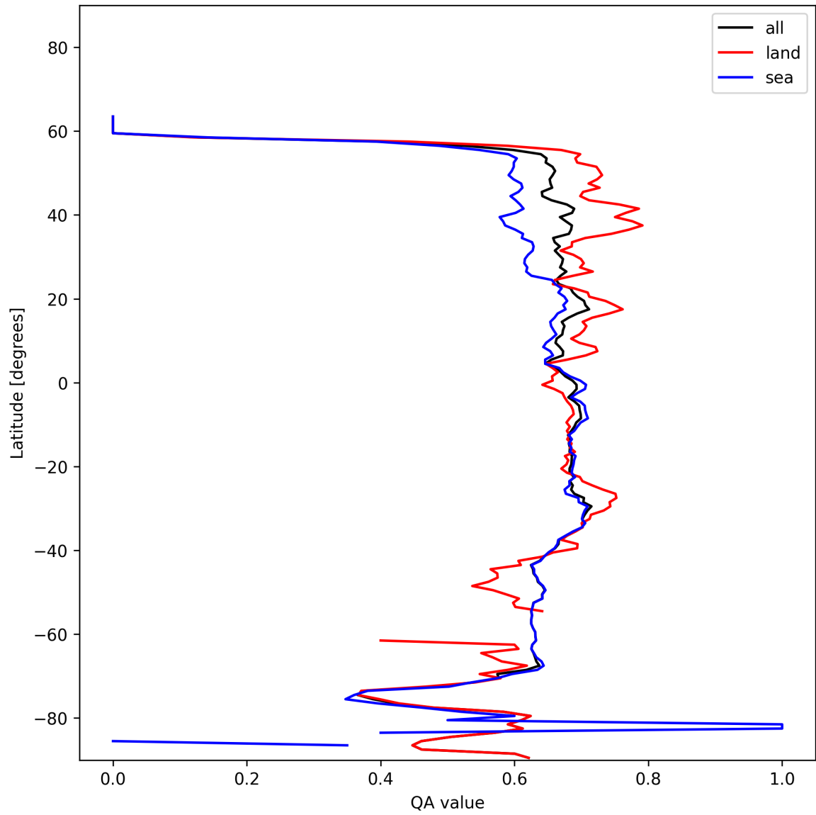
Figure 9: Zonal average of “QA value” for 2024-11-27 to 2024-11-29.
