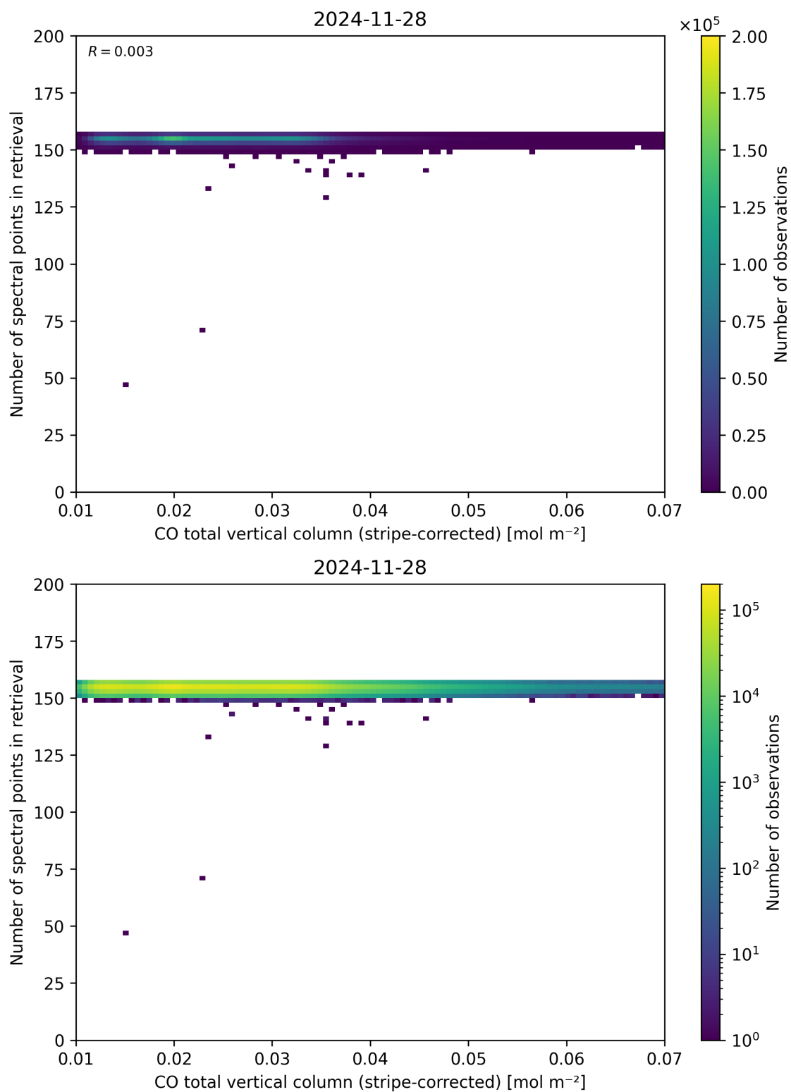
Figure 40: Scatter density plot of “CO total vertical column (stripe-corrected)” against “Number of spectral points in retrieval” for 2024-11-27 to 2024-11-29.
