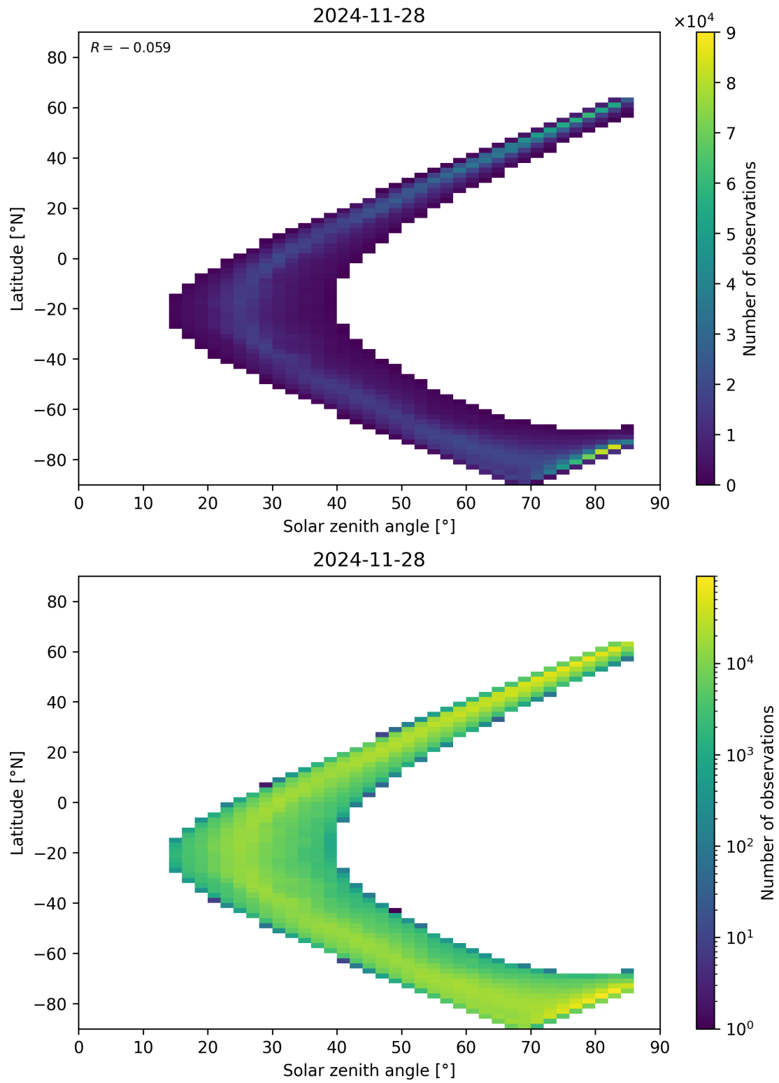
Figure 66: Scatter density plot of “Solar zenith angle” against “Latitude” for 2024-11-27 to 2024-11-29.
