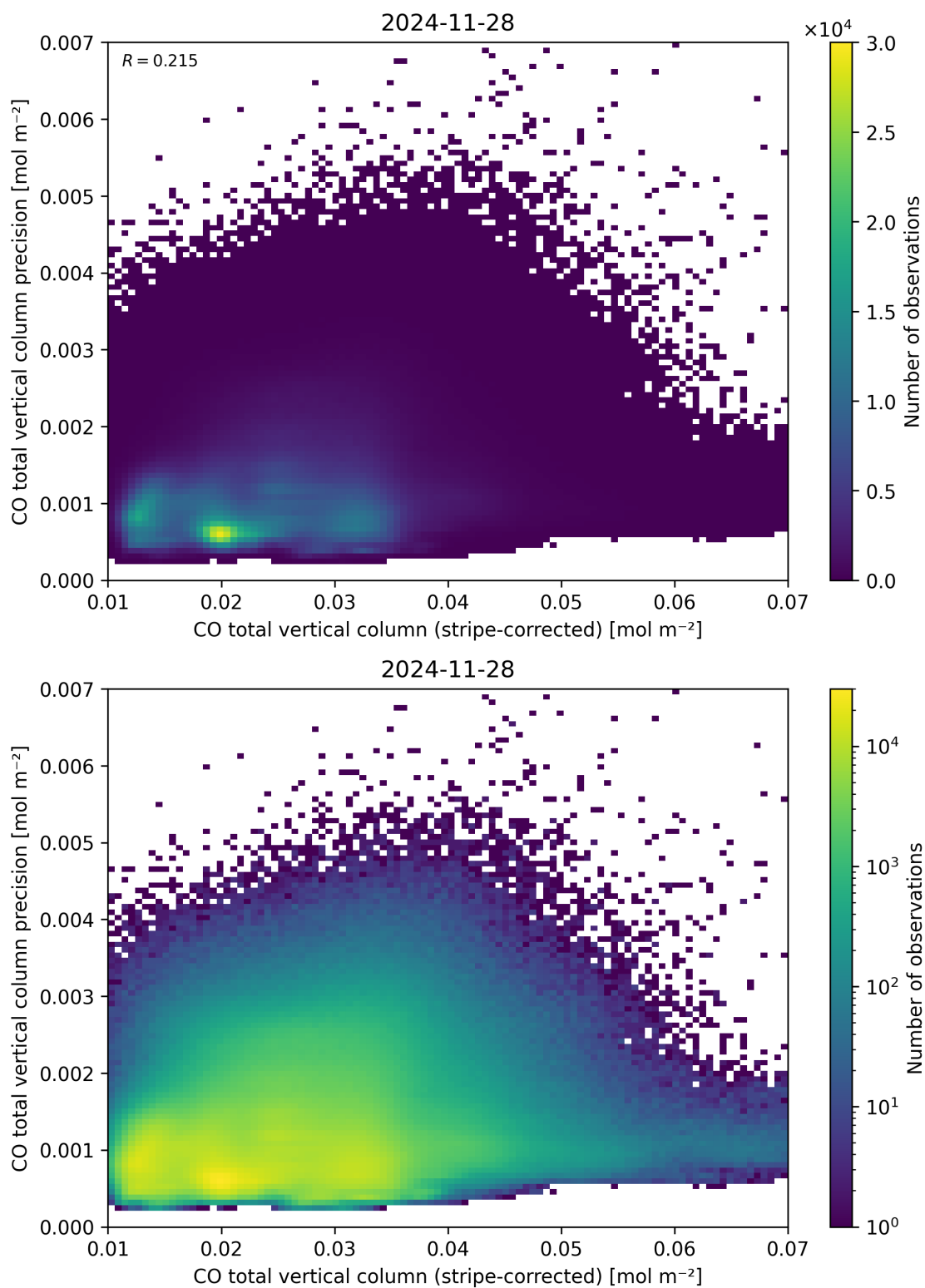
Figure 36: Scatter density plot of “CO total vertical column (stripe-corrected)” against “CO total vertical column precision” for 2024-11-27 to 2024-11-29.
