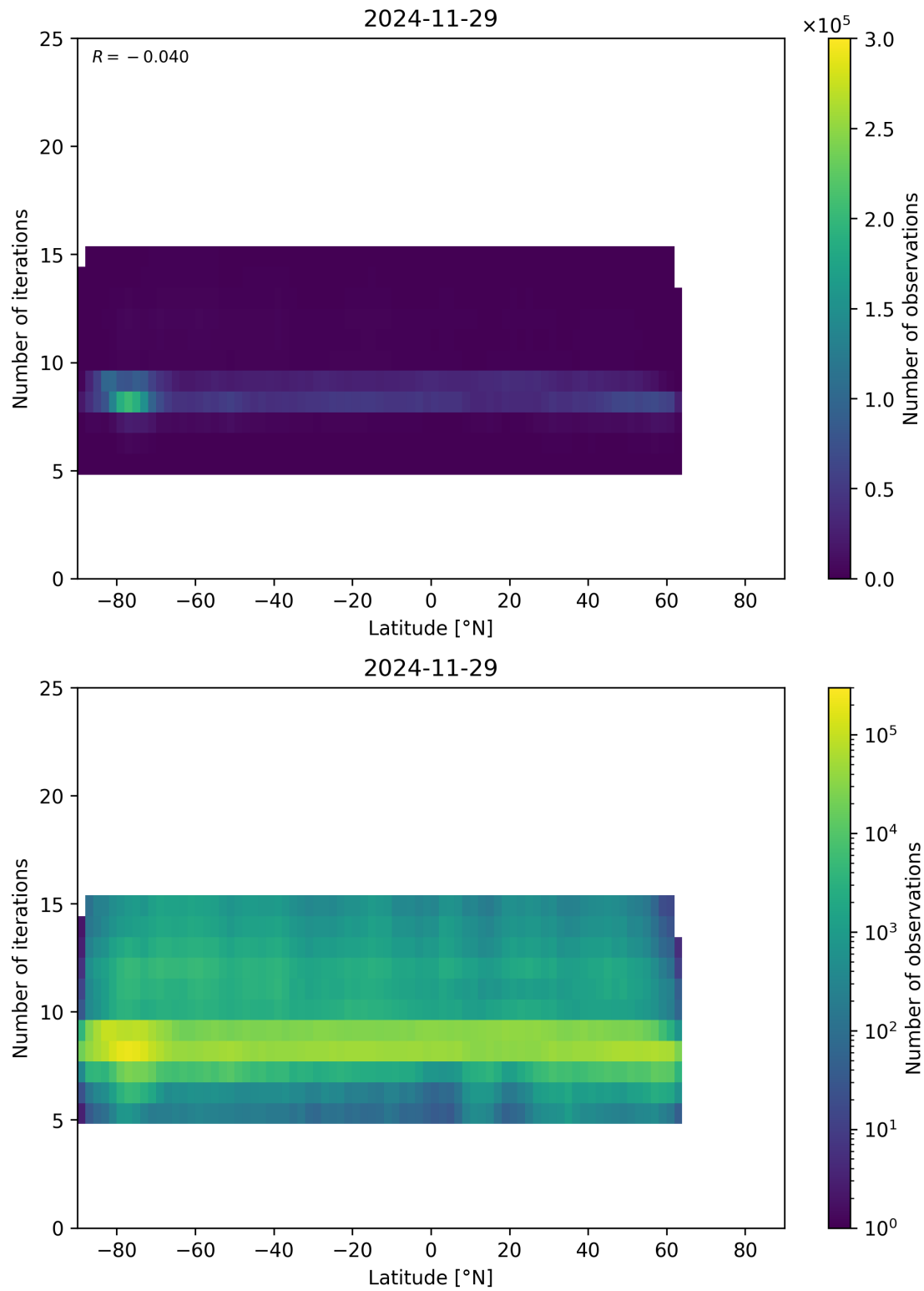
Figure 56: Scatter density plot of “Latitude” against “Number of iterations” for 2024-11-28 to 2024-11-30.
