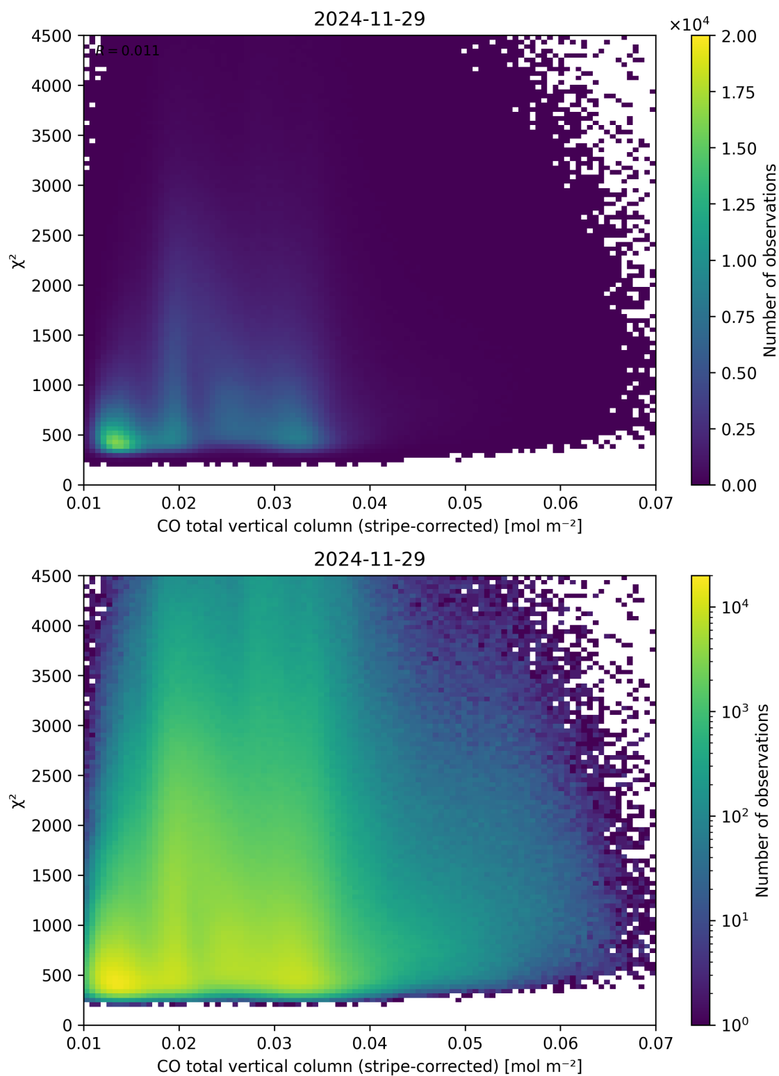
Figure 37: Scatter density plot of “CO total vertical column (stripe-corrected)” against “ \chi^2 ” for 2024-11-28 to 2024-11-30.
