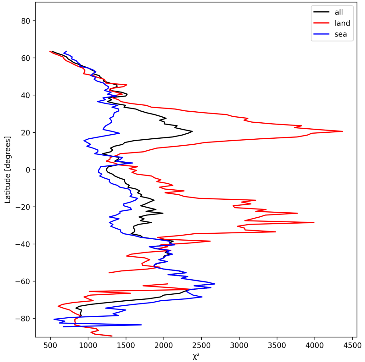
Figure 14: Zonal average of “ \chi^2 ” for 2024-11-28 to 2024-11-30.
