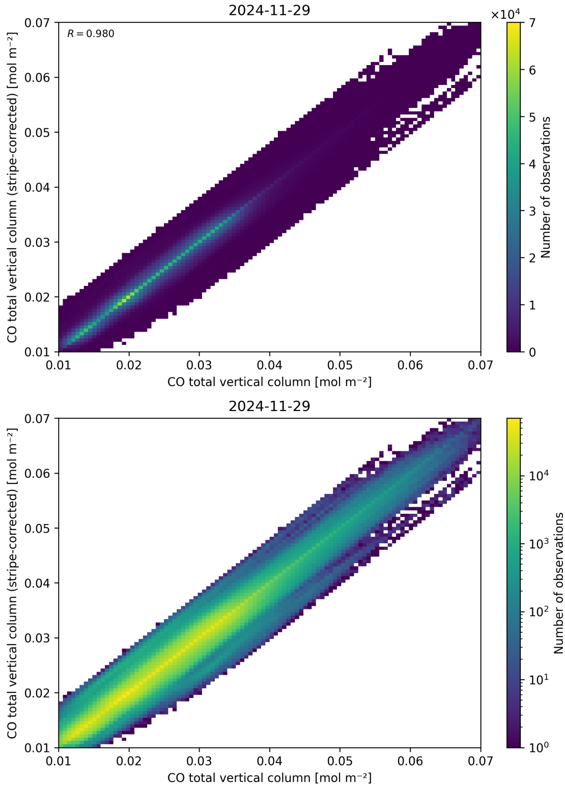
Figure 33: Scatter density plot of “CO total vertical column” against “CO total vertical column (stripe-corrected)” for 2024-11-28 to 2024-11-30.
