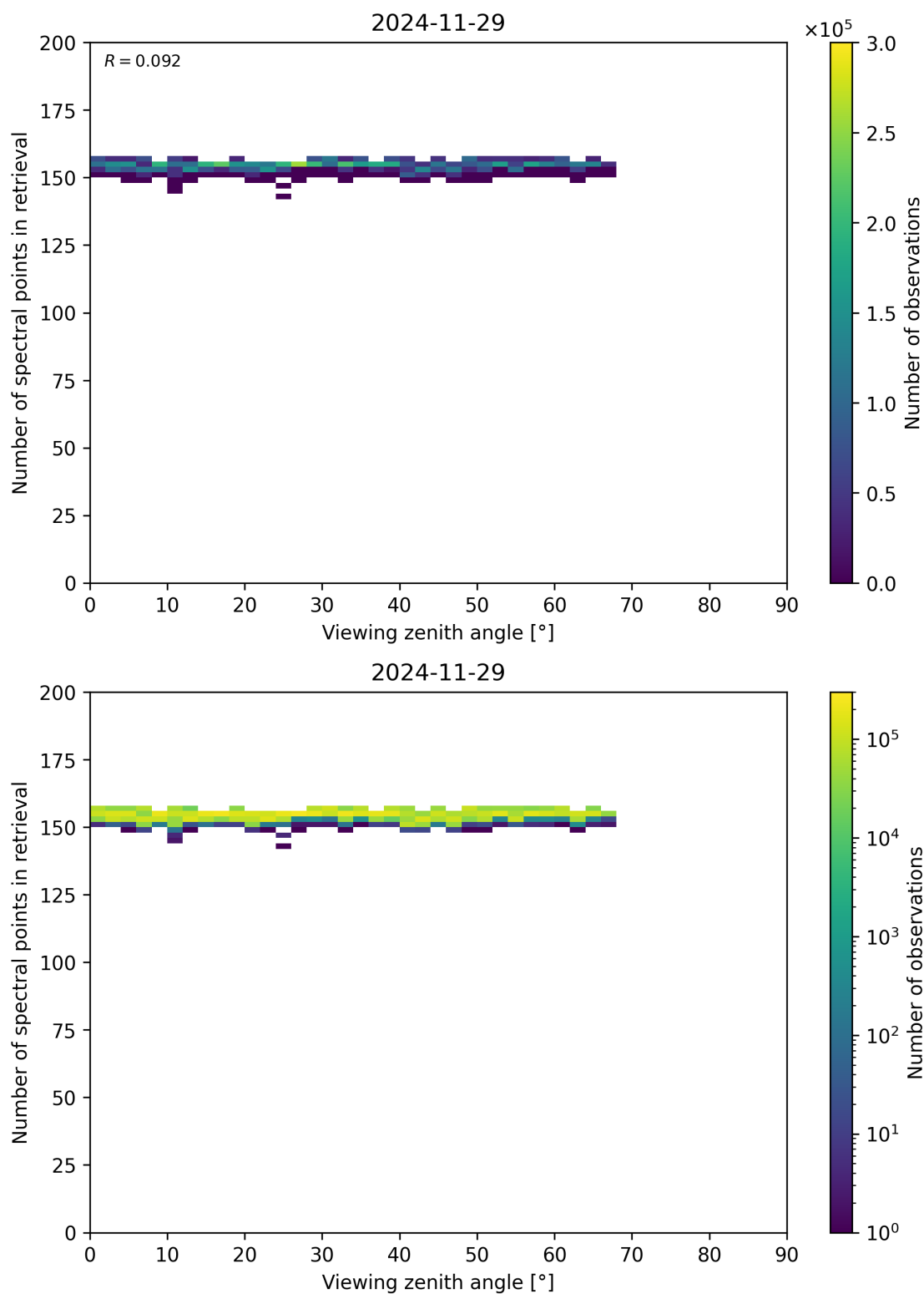
Figure 76: Scatter density plot of “Viewing zenith angle” against “Number of spectral points in retrieval” for 2024-11-28 to 2024-11-30.
