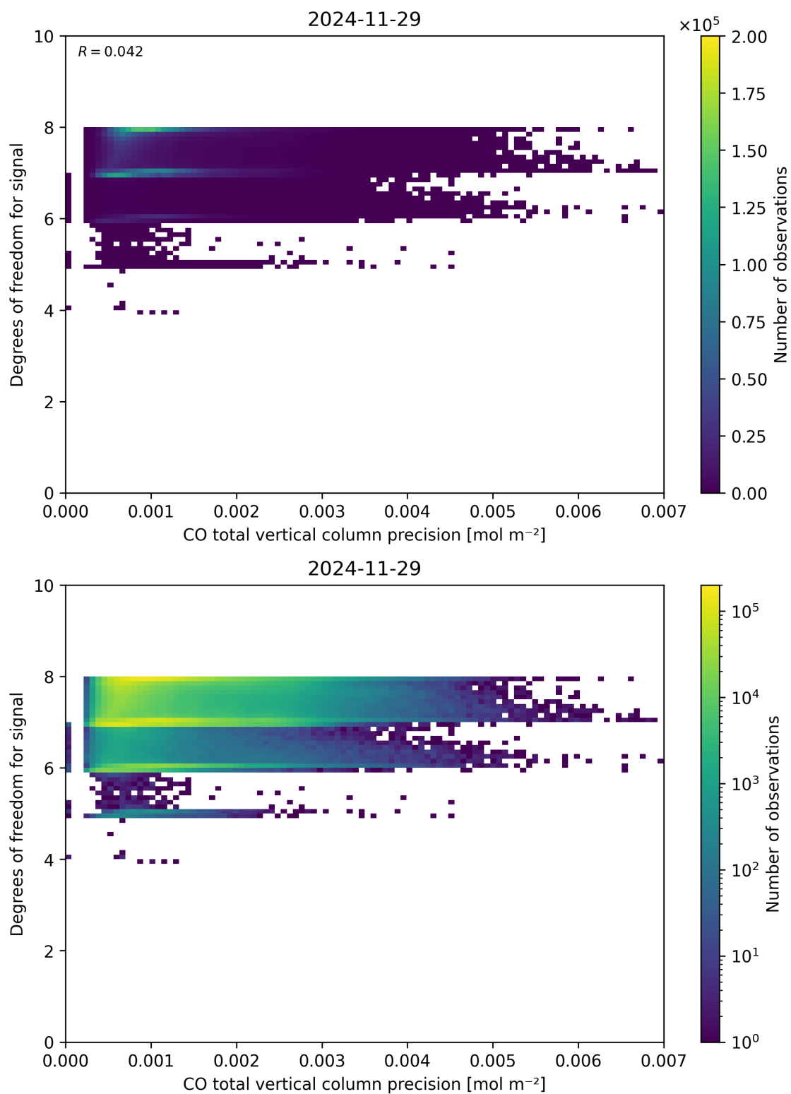
Figure 45: Scatter density plot of “CO total vertical column precision” against “Degrees of freedom for signal” for 2024-11-28 to 2024-11-30.
