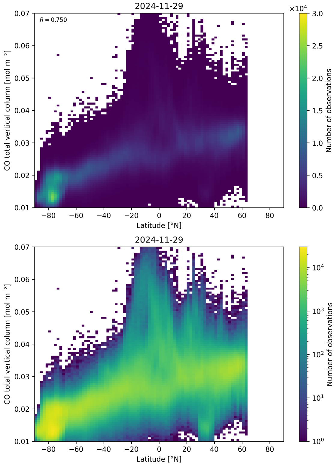
Figure 51: Scatter density plot of “Latitude” against “CO total vertical column” for 2024-11-28 to 2024-11-30.
