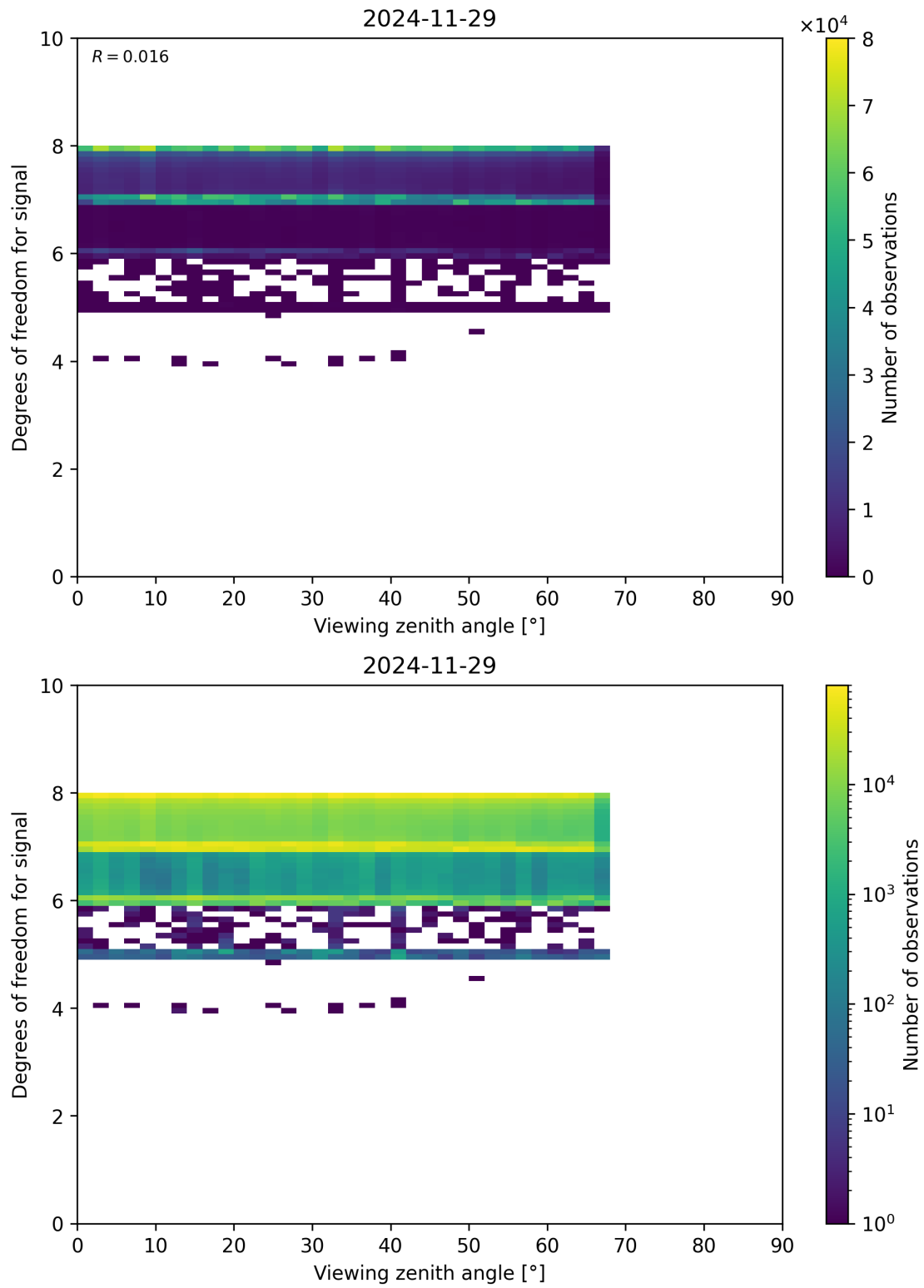
Figure 73: Scatter density plot of “Viewing zenith angle” against “Degrees of freedom for signal” for 2024-11-28 to 2024-11-30.
