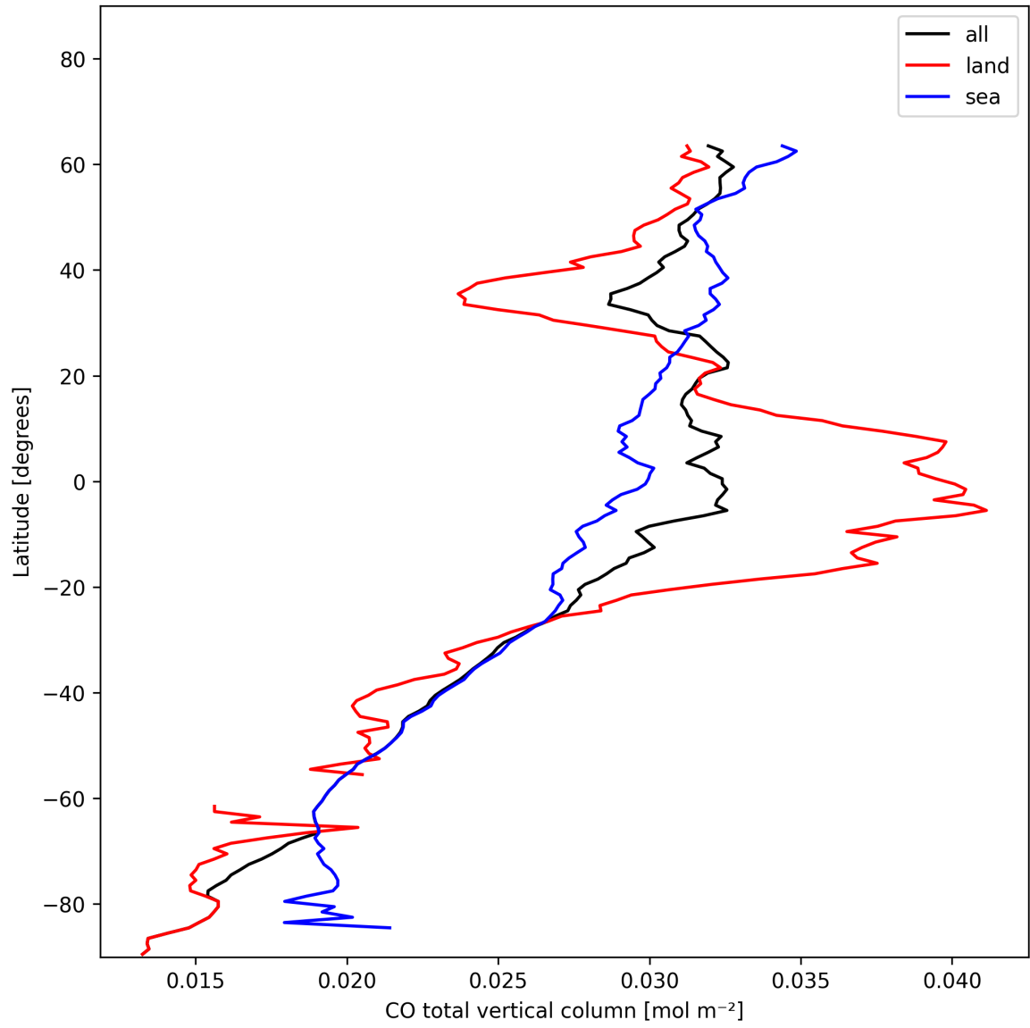
Figure 10: Zonal average of “CO total vertical column” for 2024-11-28 to 2024-11-30.
