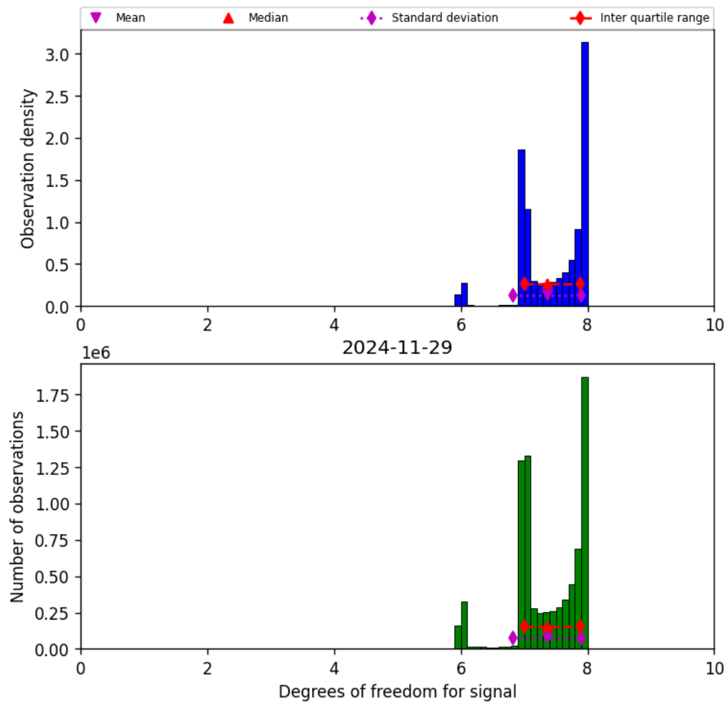
Figure 23: Histogram of “Degrees of freedom for signal” for 2024-11-28 to 2024-11-30
