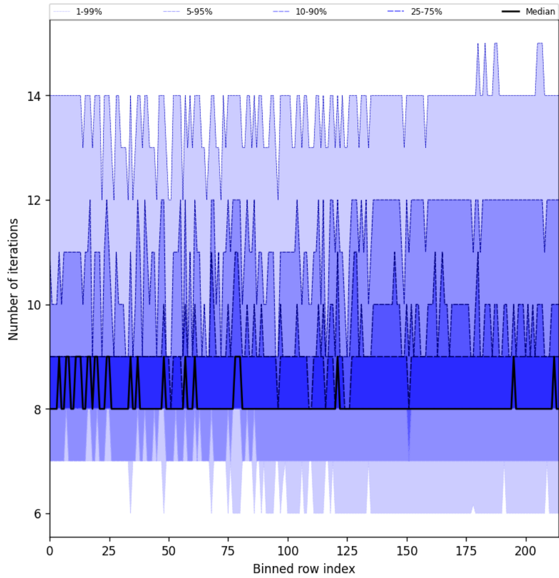
Figure 32: Along track statistics of “Number of iterations” for 2024-11-28 to 2024-11-30
