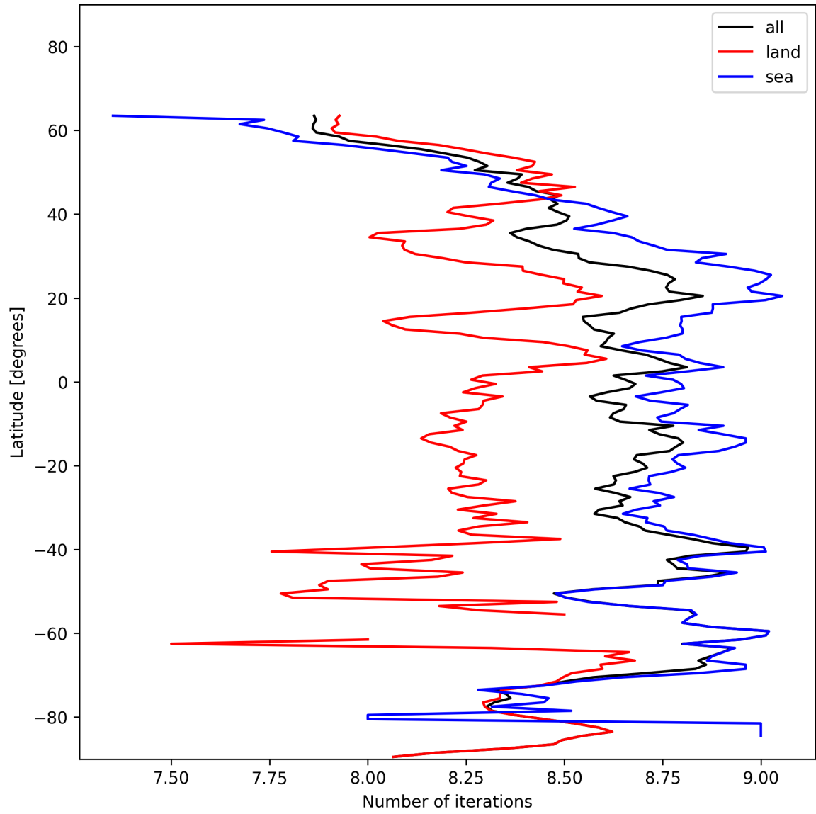
Figure 16: Zonal average of “Number of iterations” for 2024-11-28 to 2024-11-30.
