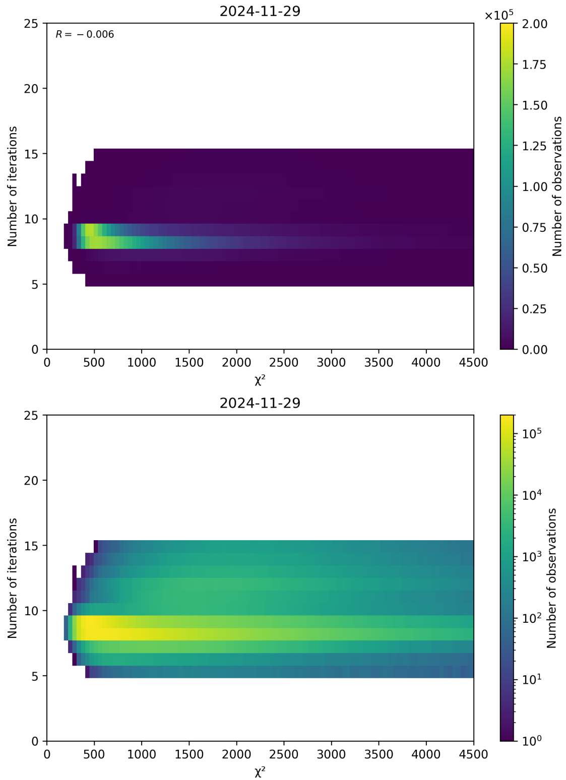
Figure 49: Scatter density plot of “ \chi^2 ” against “Number of iterations” for 2024-11-28 to 2024-11-30.
