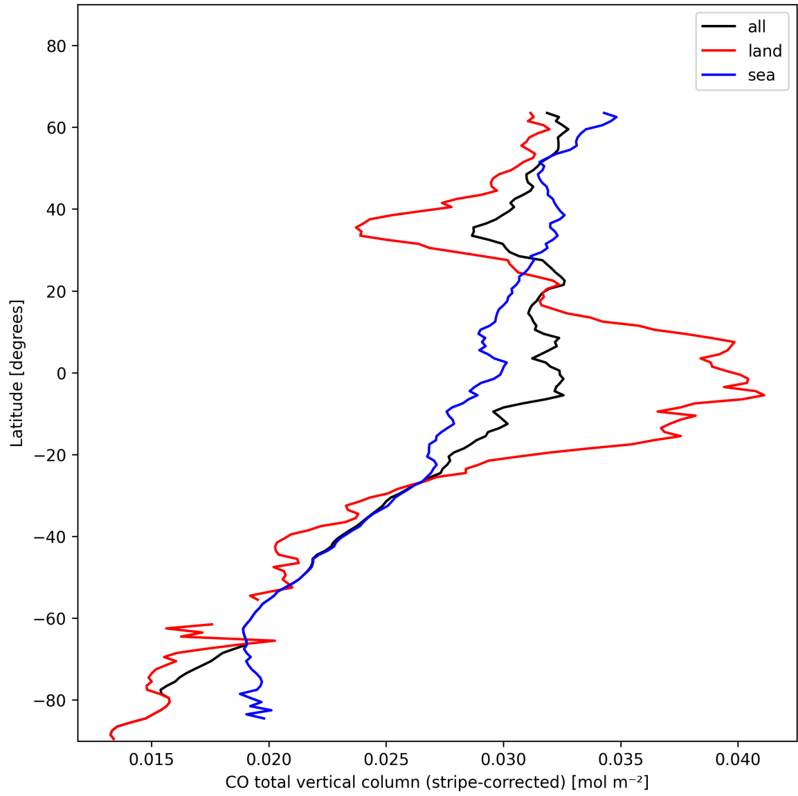
Figure 11: Zonal average of “CO total vertical column (stripe-corrected)” for 2024-11-28 to 2024-11-30.
