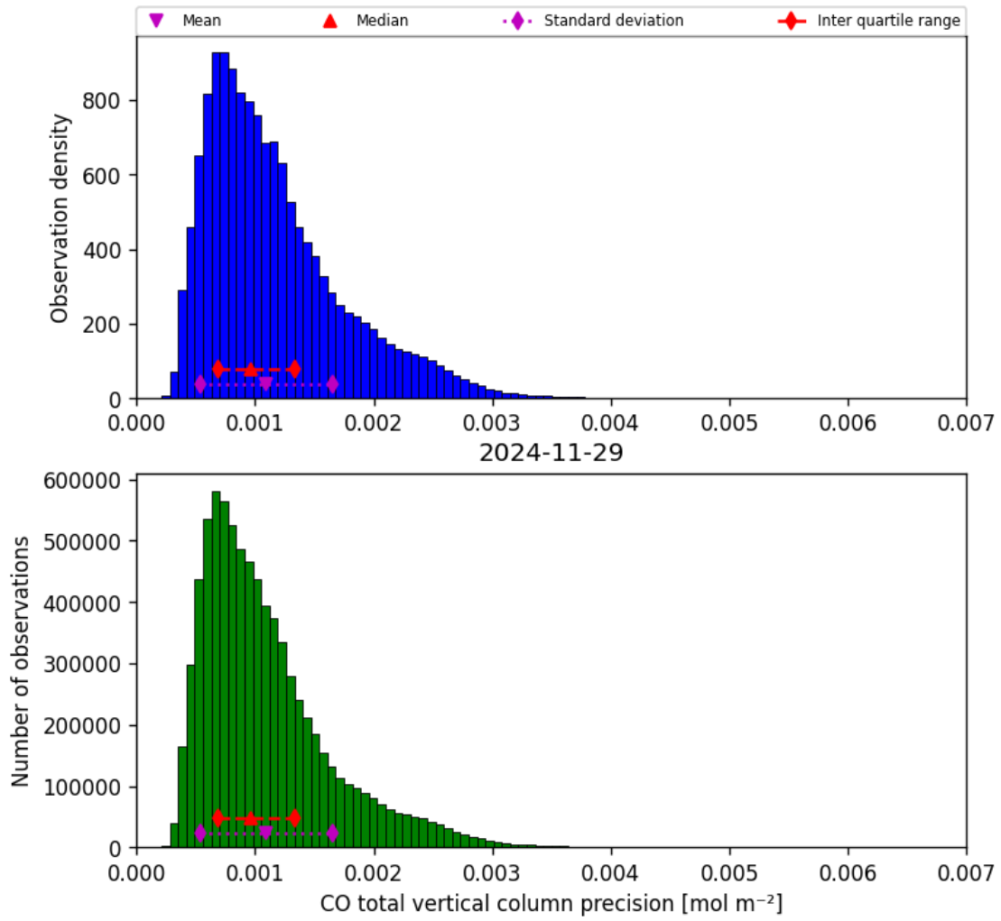
Figure 20: Histogram of “CO total vertical column precision” for 2024-11-28 to 2024-11-30
