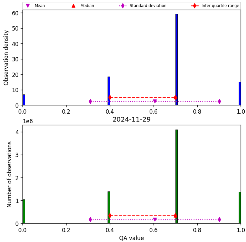
Figure 17: Histogram of “QA value” for 2024-11-28 to 2024-11-30
