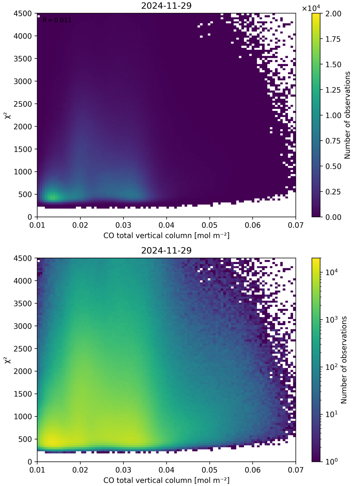
Figure 35: Scatter density plot of “CO total vertical column” against “ \chi^2 ” for 2024-11-28 to 2024-11-30.
