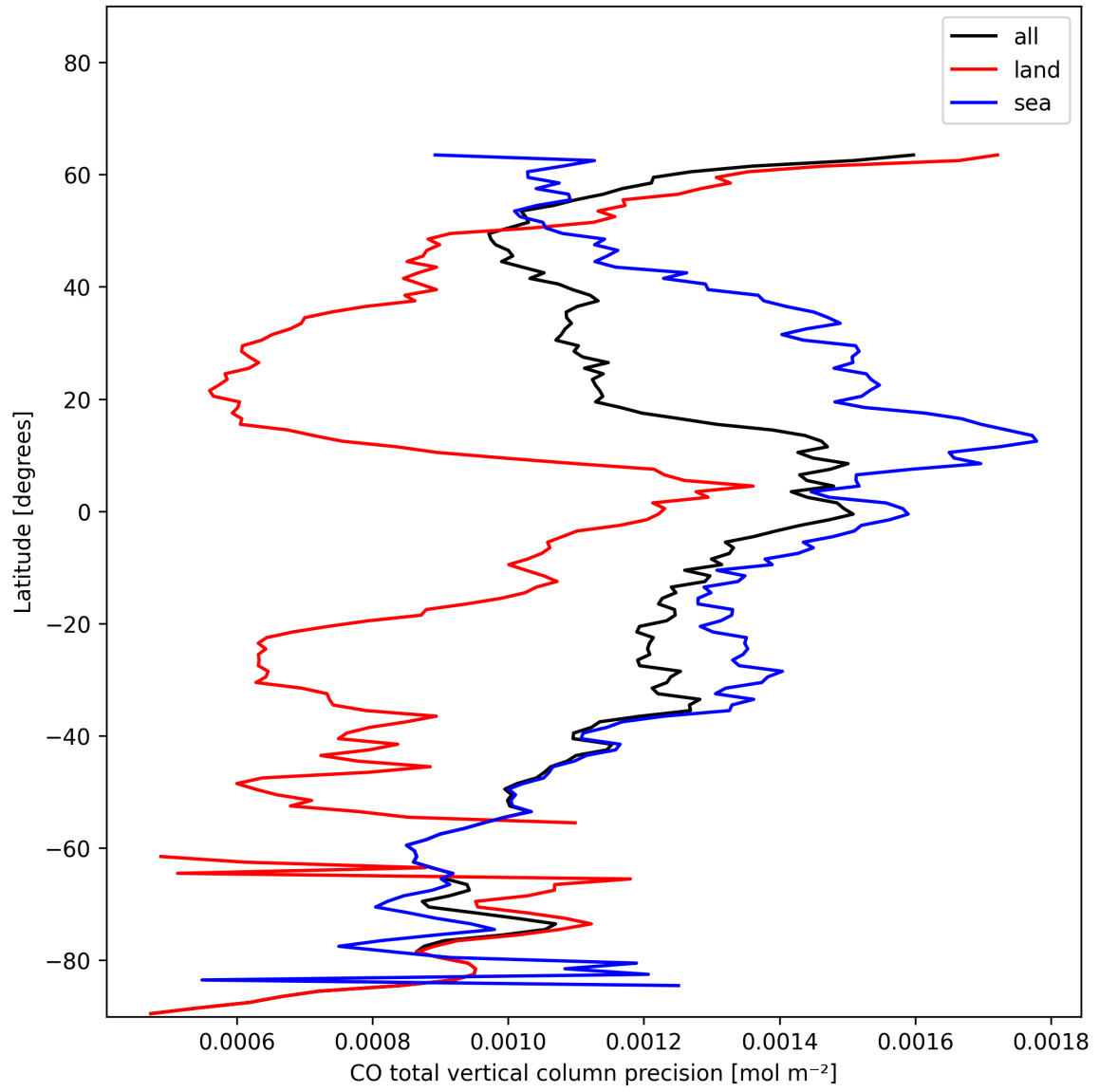
Figure 12: Zonal average of “CO total vertical column precision” for 2024-11-28 to 2024-11-30.
