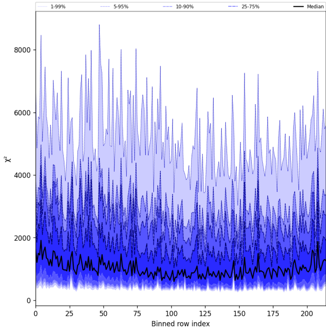
Figure 30: Along track statistics of “ \chi^2 ” for 2024-11-28 to 2024-11-30
