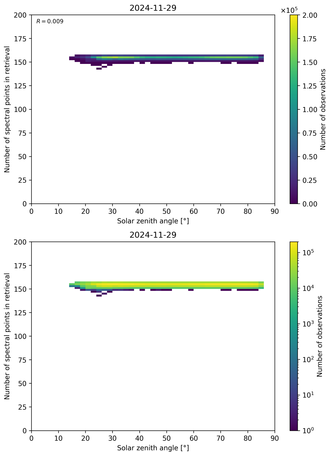
Figure 68: Scatter density plot of “Solar zenith angle” against “Number of spectral points in retrieval” for 2024-11-28 to 2024-11-30.
