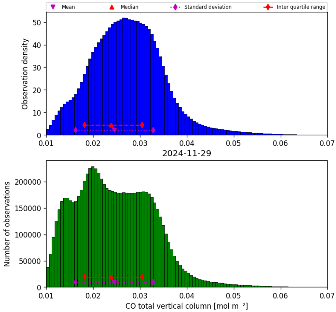
Figure 18: Histogram of “CO total vertical column” for 2024-11-28 to 2024-11-30
