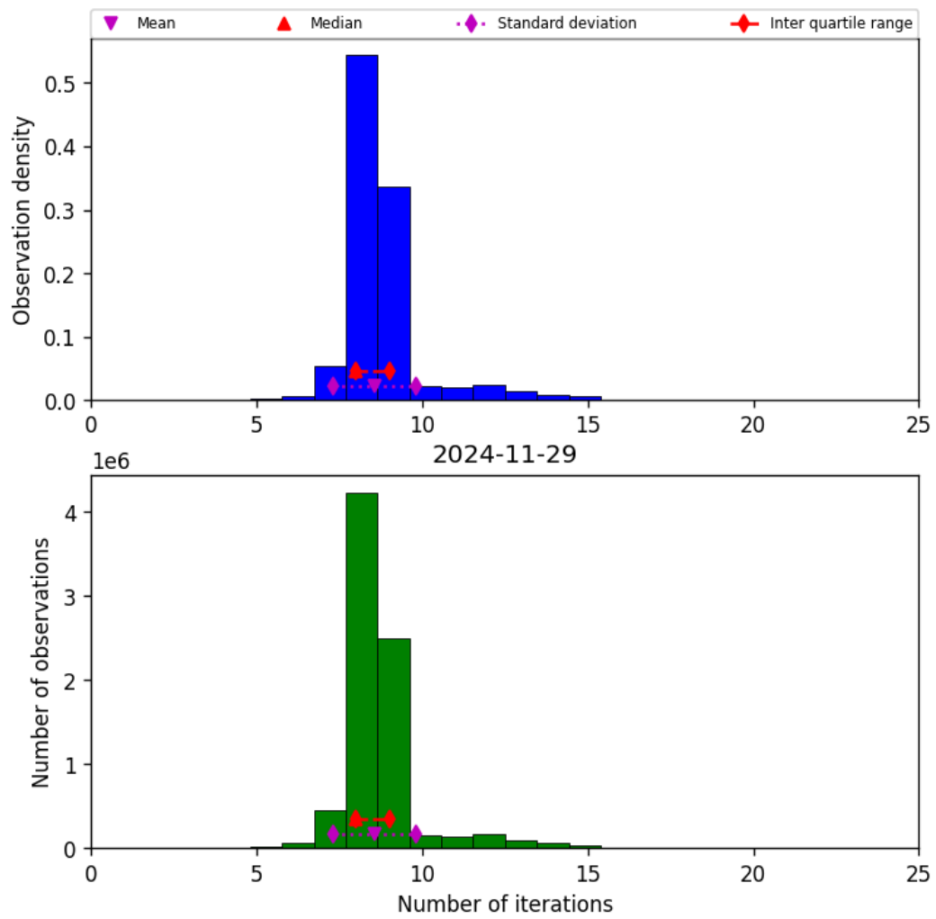
Figure 24: Histogram of “Number of iterations” for 2024-11-28 to 2024-11-30
