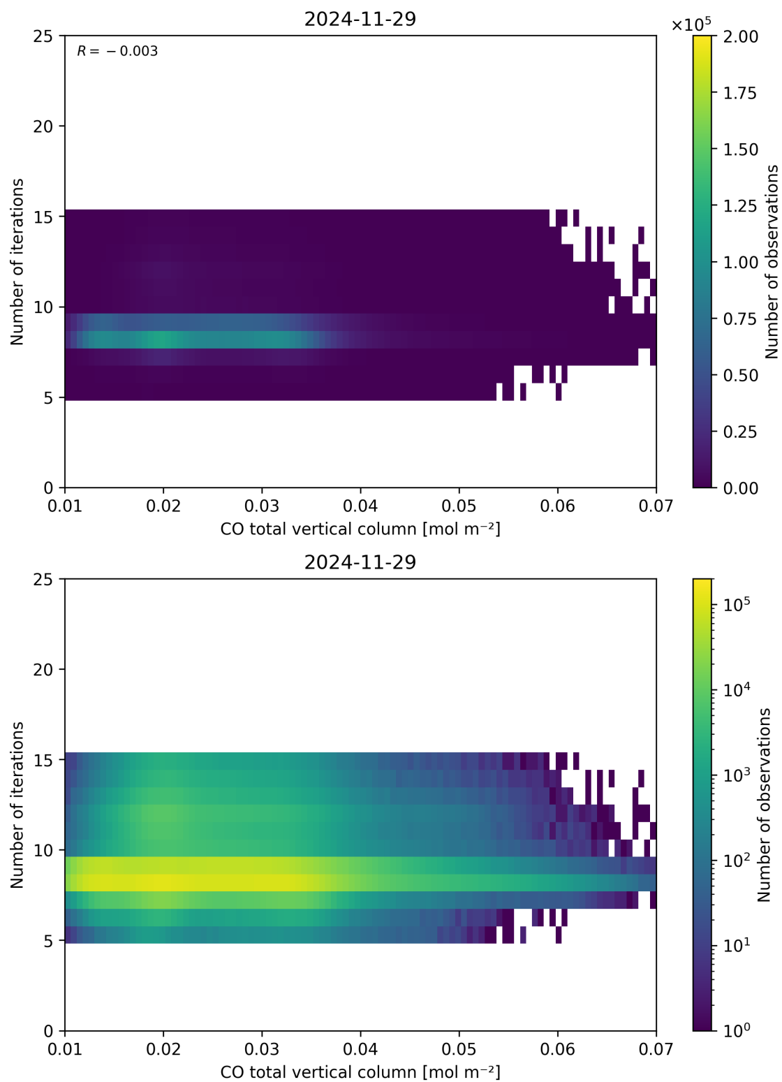
Figure 42: Scatter density plot of “CO total vertical column” against “Number of iterations” for 2024-11-28 to 2024-11-30.
