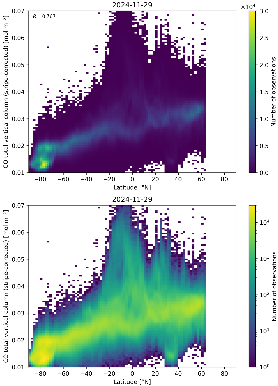
Figure 52: Scatter density plot of “Latitude” against “CO total vertical column (stripe-corrected)” for 2024-11-28 to 2024-11-30.
