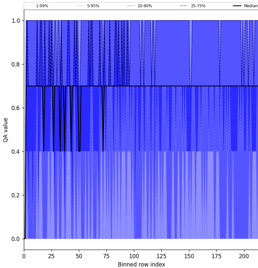
Figure 25: Along track statistics of “QA value” for 2024-11-28 to 2024-11-30
