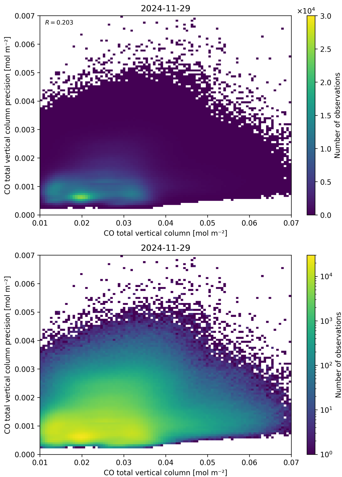
Figure 34: Scatter density plot of “CO total vertical column” against “CO total vertical column precision” for 2024-11-28 to 2024-11-30.
