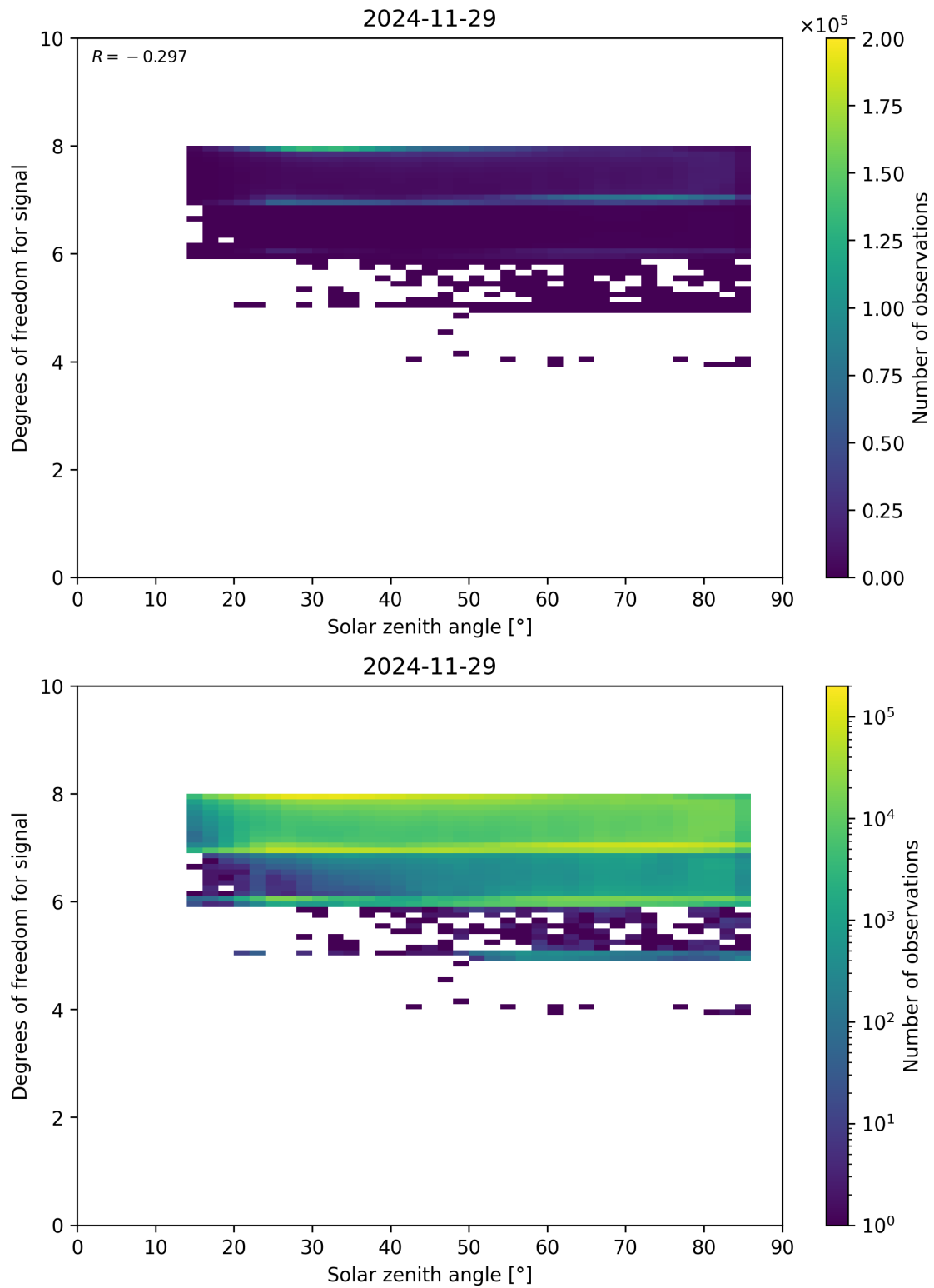
Figure 65: Scatter density plot of “Solar zenith angle” against “Degrees of freedom for signal” for 2024-11-28 to 2024-11-30.
