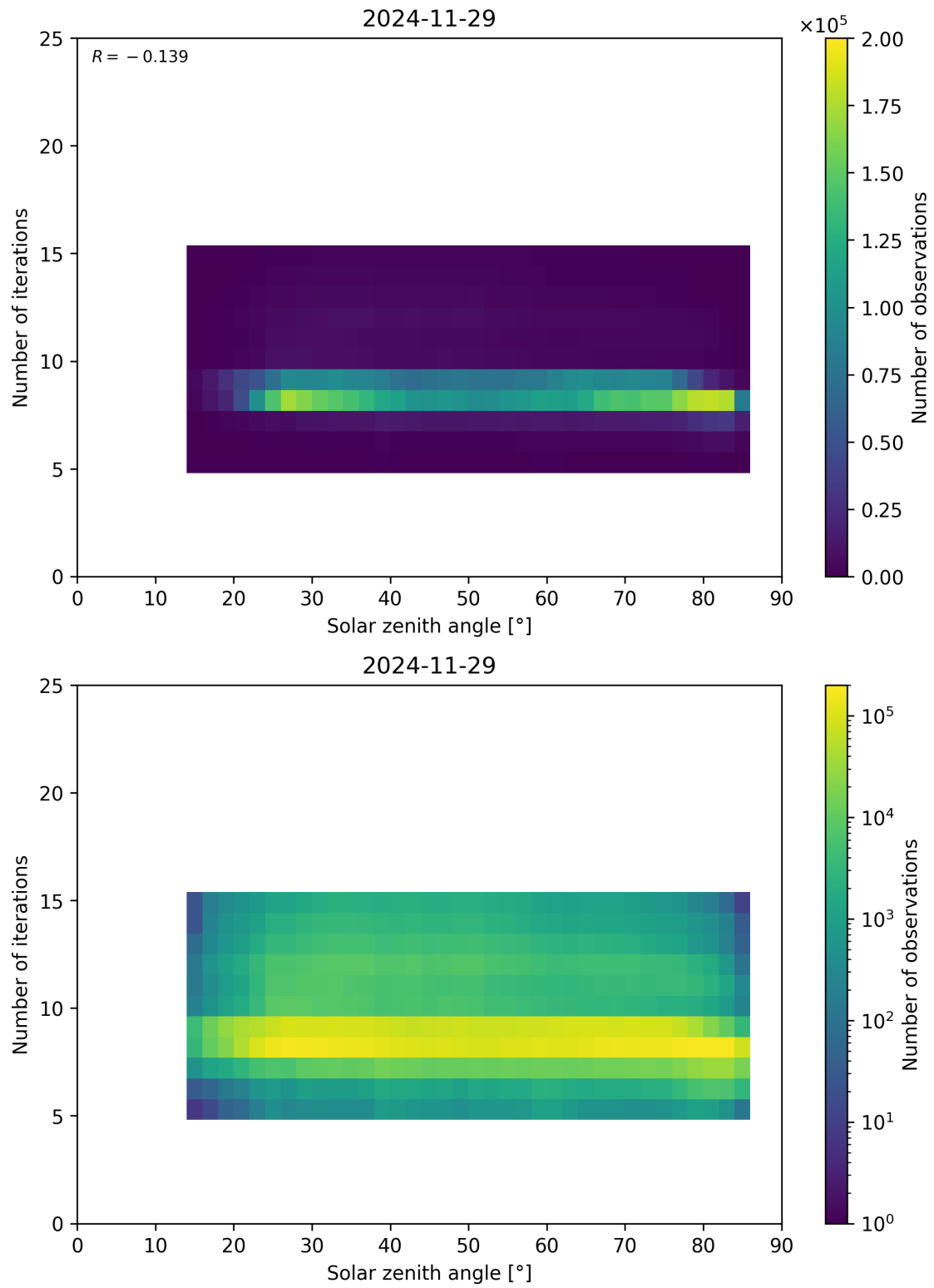
Figure 67: Scatter density plot of “Solar zenith angle” against “Number of iterations” for 2024-11-28 to 2024-11-30.
