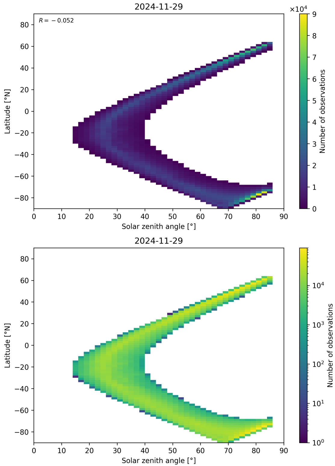
Figure 66: Scatter density plot of “Solar zenith angle” against “Latitude” for 2024-11-28 to 2024-11-30.
