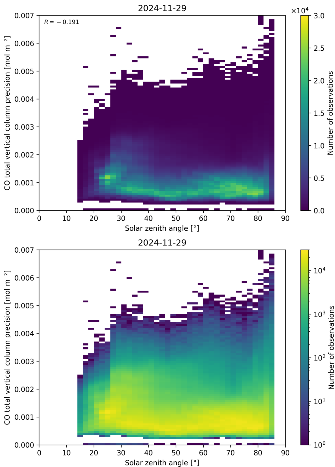
Figure 63: Scatter density plot of “Solar zenith angle” against “CO total vertical column precision” for 2024-11-28 to 2024-11-30.
