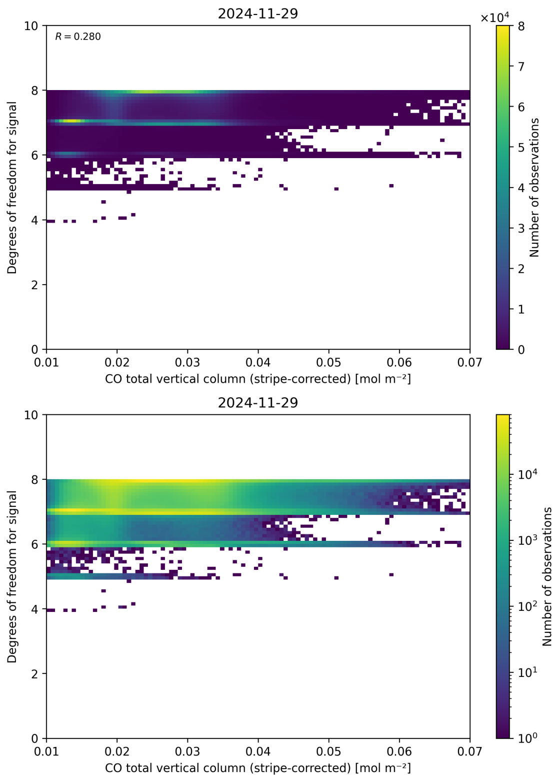
Figure 38: Scatter density plot of “CO total vertical column (stripe-corrected)” against “Degrees of freedom for signal” for 2024-11-28 to 2024-11-30.
