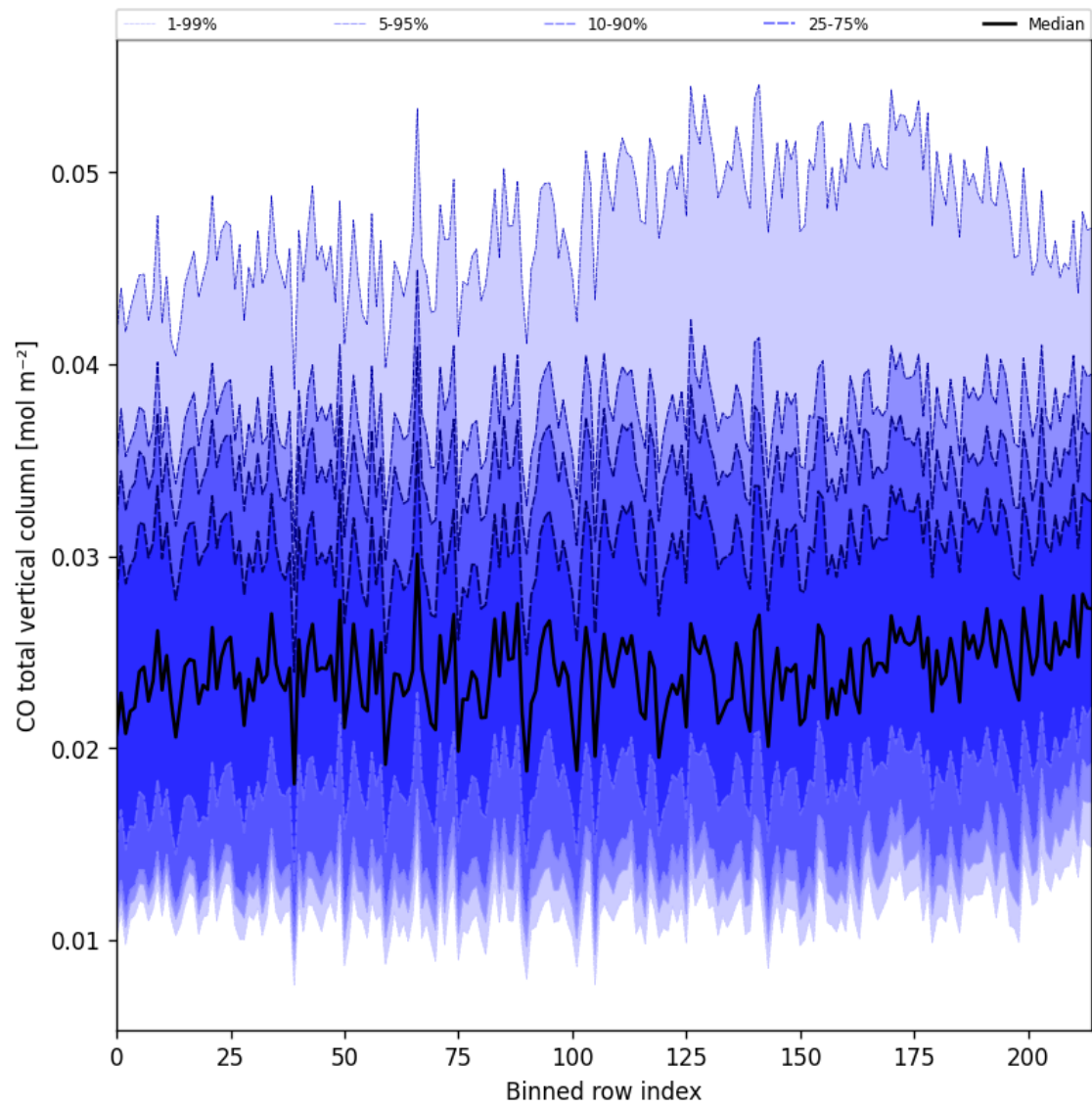
Figure 26: Along track statistics of “CO total vertical column” for 2024-11-28 to 2024-11-30
