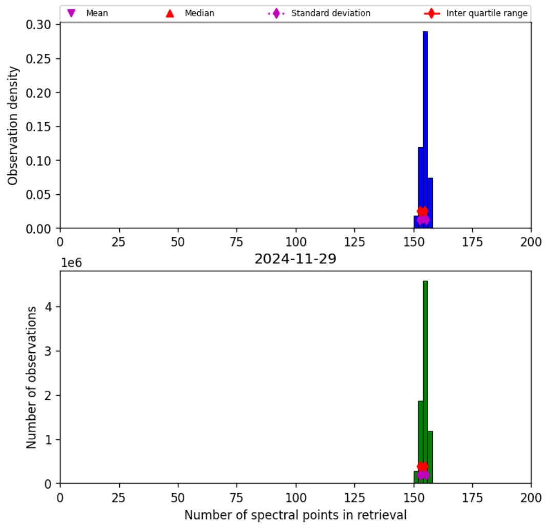
Figure 21: Histogram of “Number of spectral points in retrieval” for 2024-11-28 to 2024-11-30
