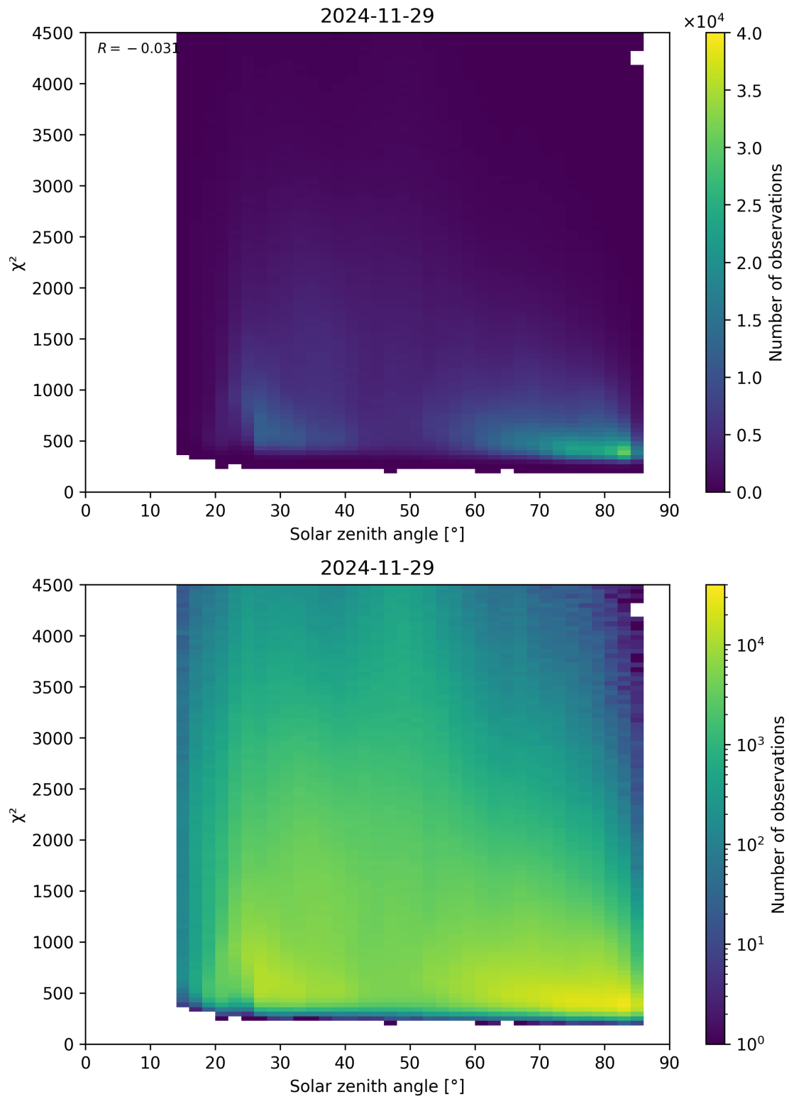
Figure 64: Scatter density plot of “Solar zenith angle” against “ \chi^2 ” for 2024-11-28 to 2024-11-30.
