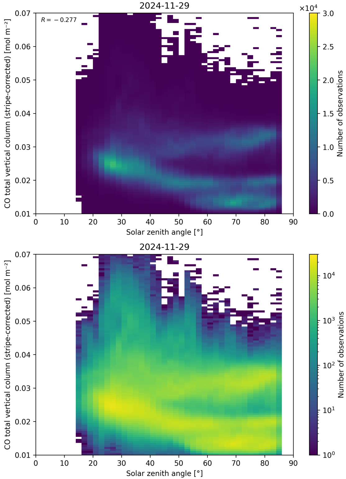
Figure 62: Scatter density plot of “Solar zenith angle” against “CO total vertical column (stripe-corrected)” for 2024-11-28 to 2024-11-30.
