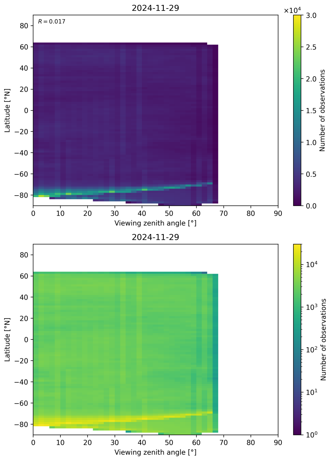
Figure 74: Scatter density plot of “Viewing zenith angle” against “Latitude” for 2024-11-28 to 2024-11-30.
