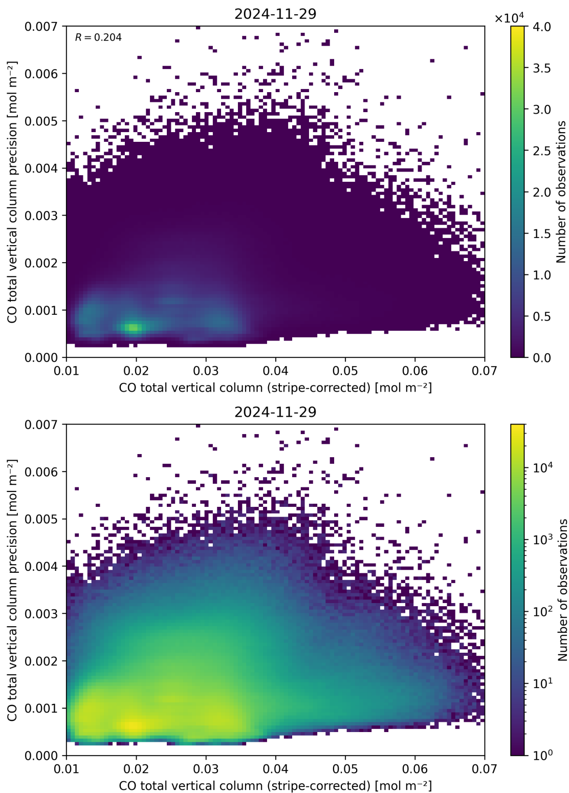
Figure 36: Scatter density plot of “CO total vertical column (stripe-corrected)” against “CO total vertical column precision” for 2024-11-28 to 2024-11-30.
