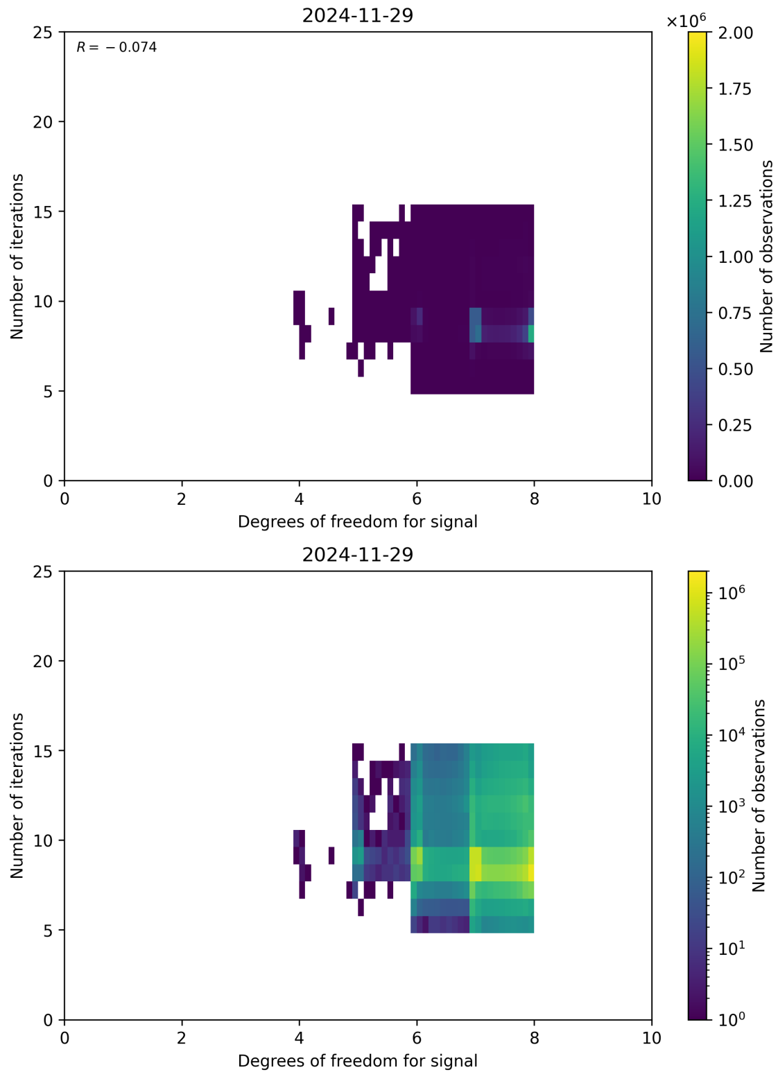
Figure 50: Scatter density plot of “Degrees of freedom for signal” against “Number of iterations” for 2024-11-28 to 2024-11-30.
