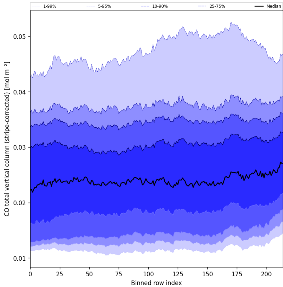
Figure 27: Along track statistics of “CO total vertical column (stripe-corrected)” for 2024-11-28 to 2024-11-30
