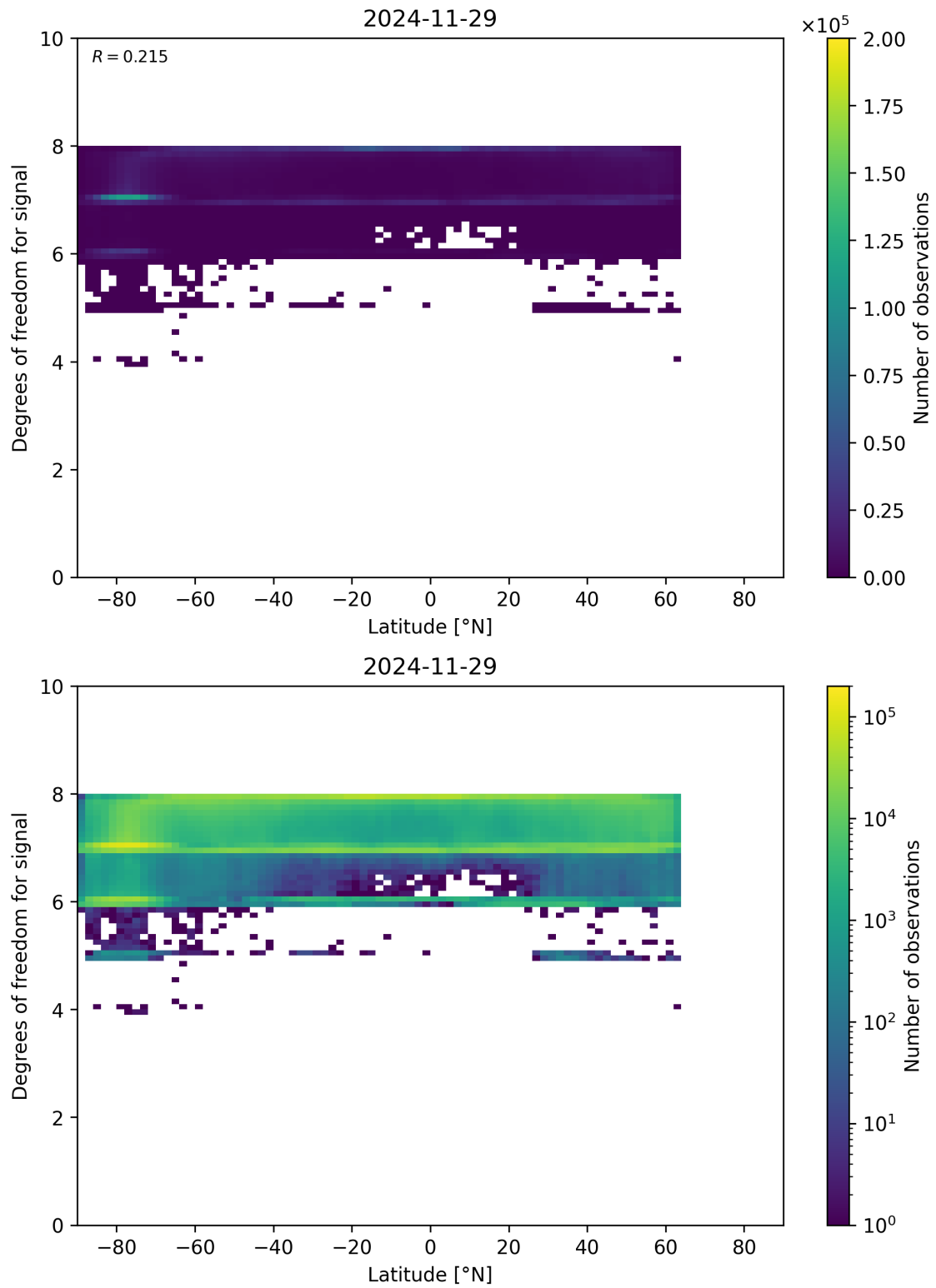
Figure 55: Scatter density plot of “Latitude” against “Degrees of freedom for signal” for 2024-11-28 to 2024-11-30.
