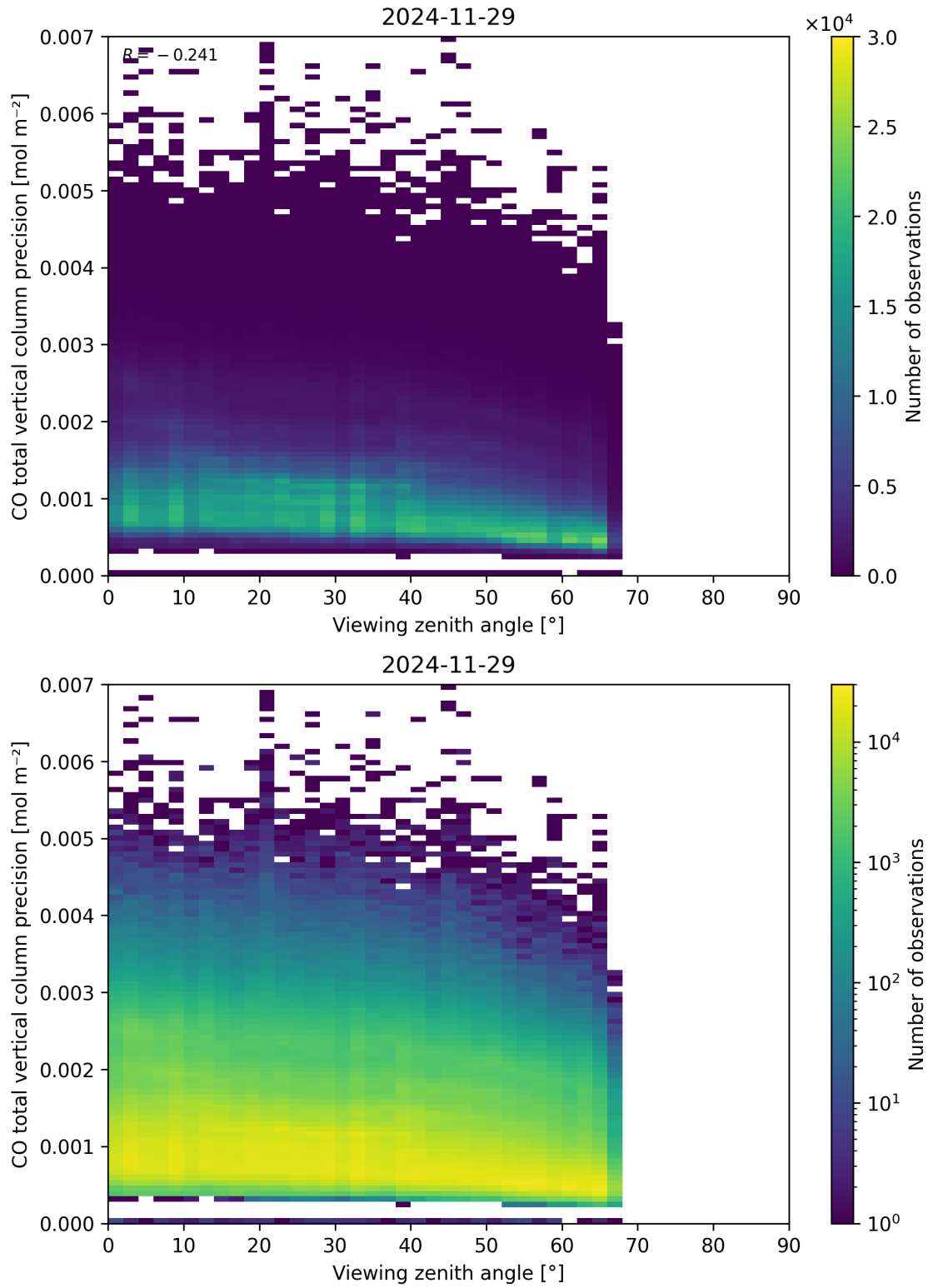
Figure 71: Scatter density plot of “Viewing zenith angle” against “CO total vertical column precision” for 2024-11-28 to 2024-11-30.
