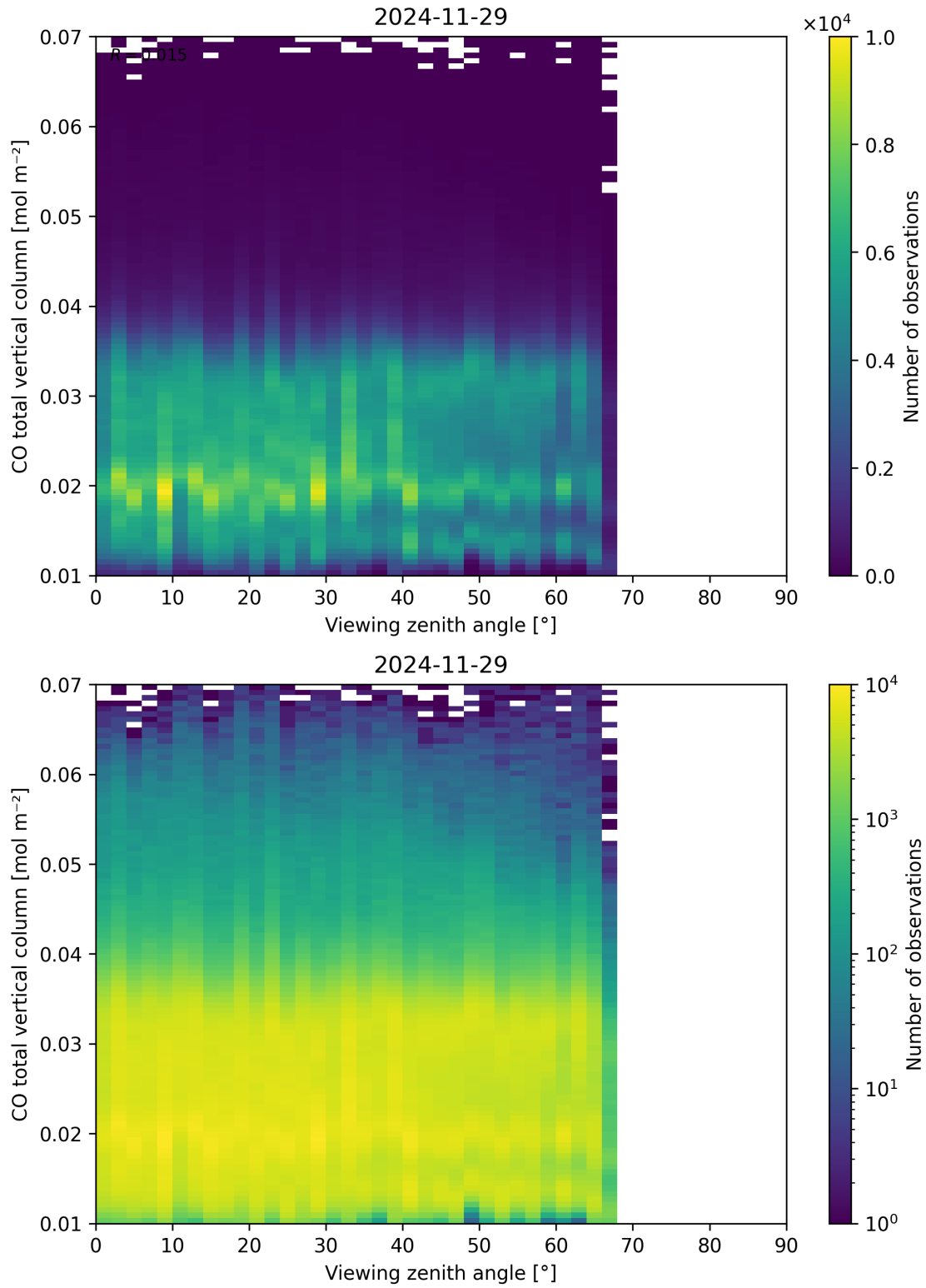
Figure 69: Scatter density plot of “Viewing zenith angle” against “CO total vertical column” for 2024-11-28 to 2024-11-30.
