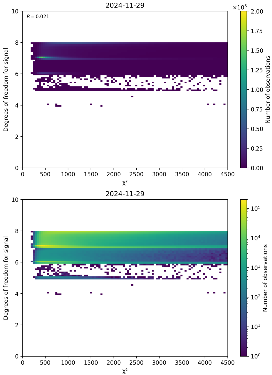
Figure 48: Scatter density plot of “ \chi^2 ” against “Degrees of freedom for signal” for 2024-11-28 to 2024-11-30.
