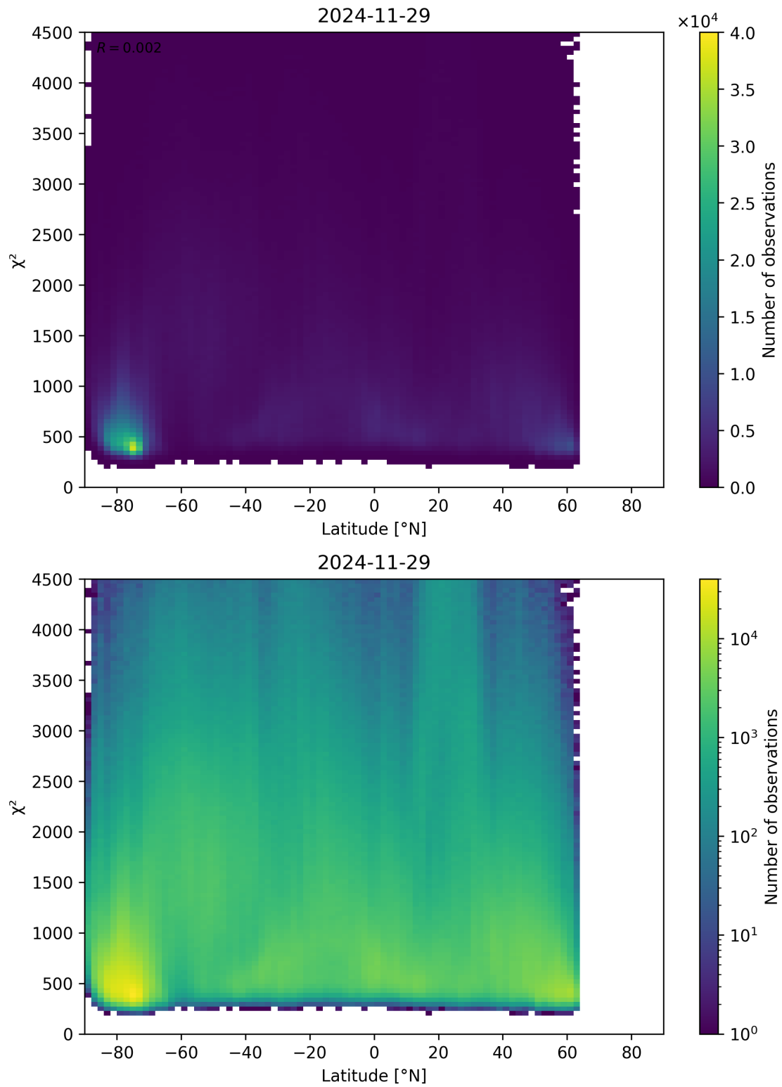
Figure 54: Scatter density plot of “Latitude” against “ \chi^2 ” for 2024-11-28 to 2024-11-30.
