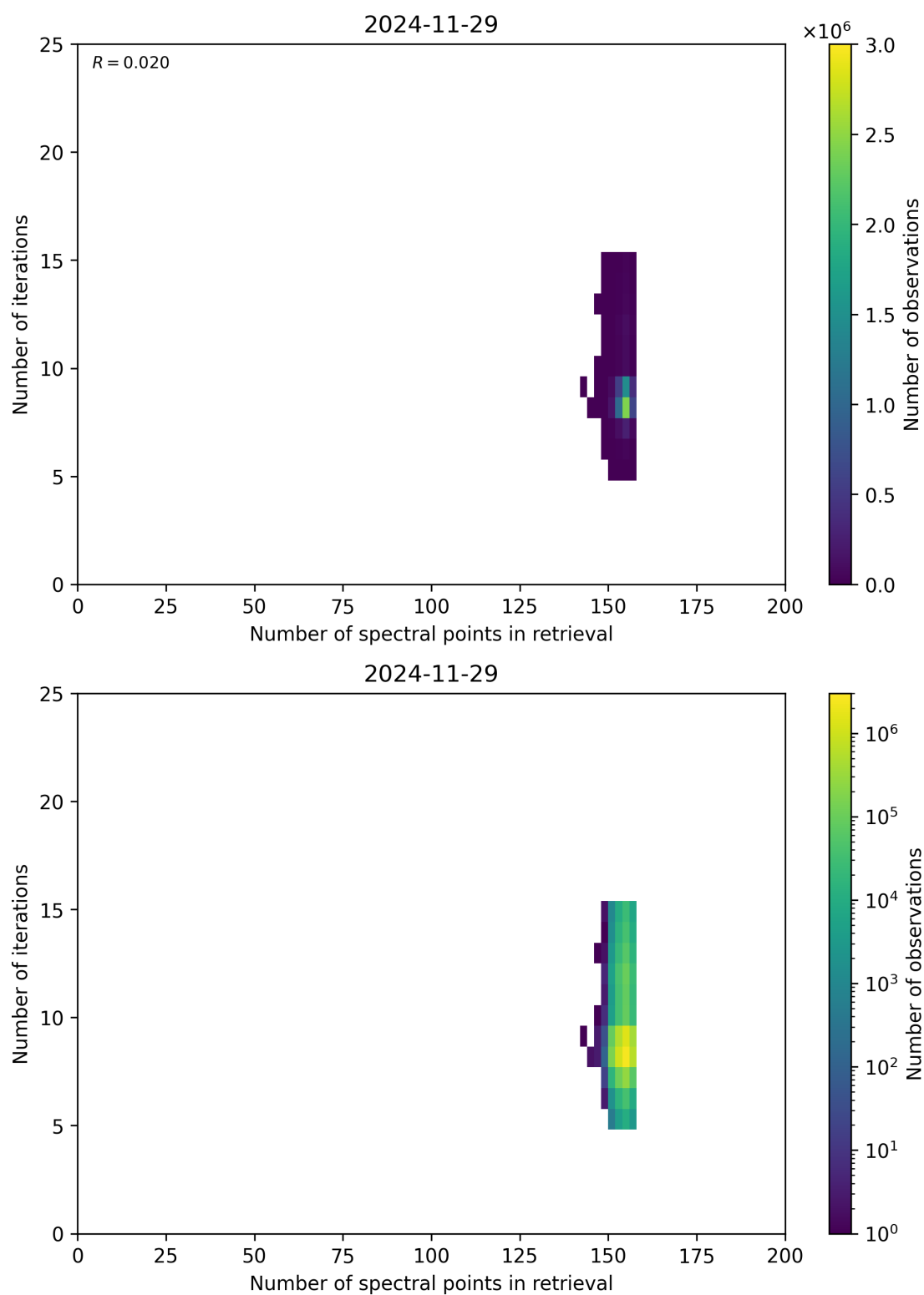
Figure 60: Scatter density plot of “Number of spectral points in retrieval” against “Number of iterations” for 2024-11-28 to 2024-11-30.
