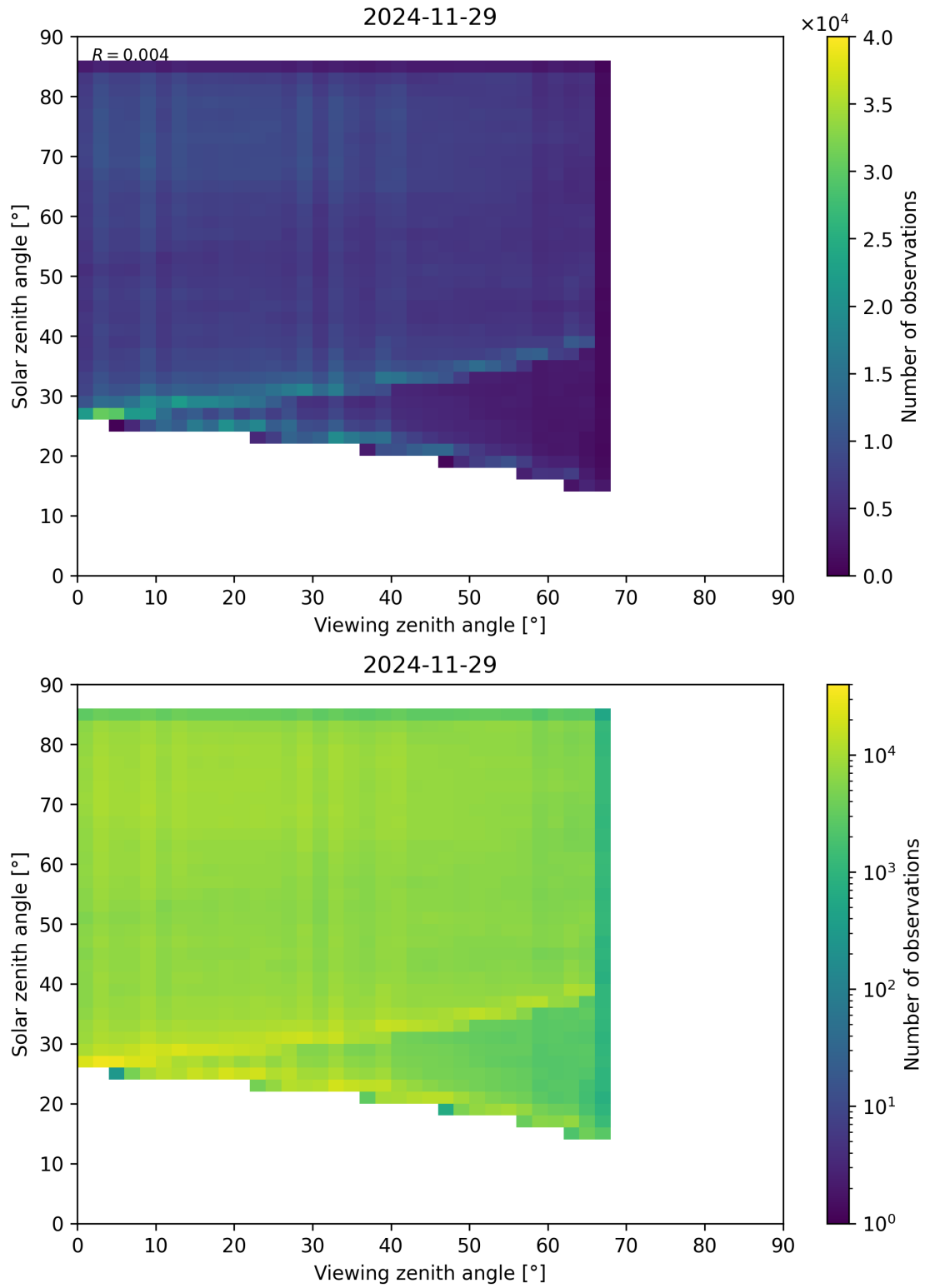
Figure 77: Scatter density plot of “Viewing zenith angle” against “Solar zenith angle” for 2024-11-28 to 2024-11-30.
