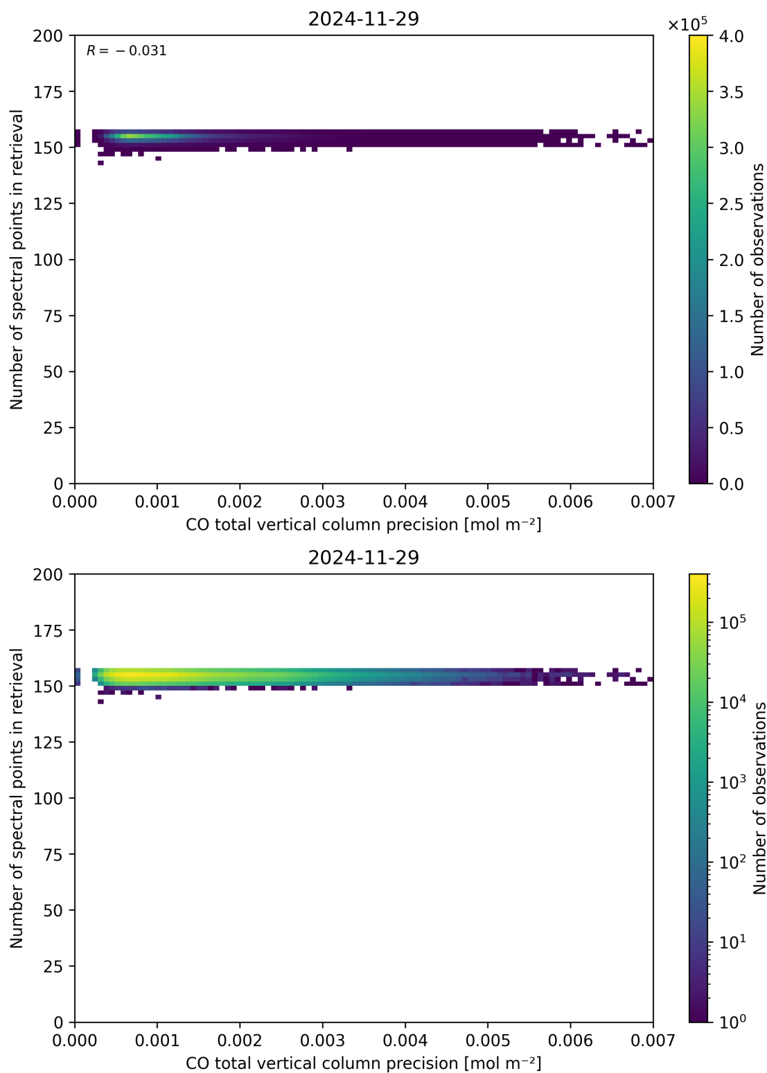
Figure 47: Scatter density plot of “CO total vertical column precision” against “Number of spectral points in retrieval” for 2024-11-28 to 2024-11-30.
