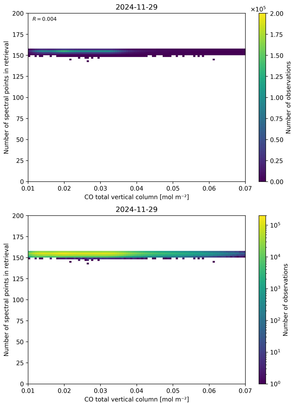
Figure 43: Scatter density plot of “CO total vertical column” against “Number of spectral points in retrieval” for 2024-11-28 to 2024-11-30.
