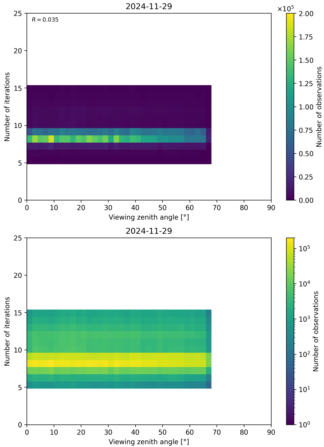
Figure 75: Scatter density plot of “Viewing zenith angle” against “Number of iterations” for 2024-11-28 to 2024-11-30.
