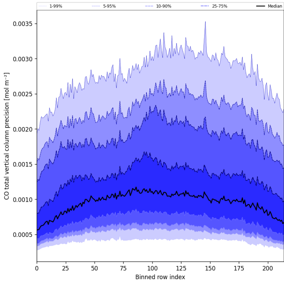
Figure 28: Along track statistics of “CO total vertical column precision” for 2024-11-28 to 2024-11-30
