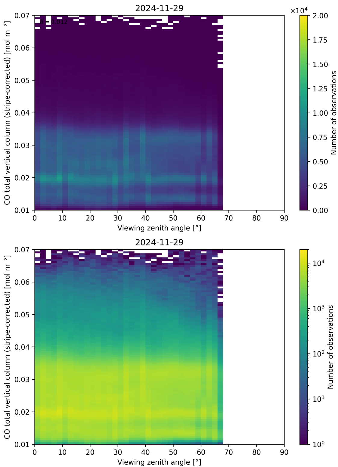
Figure 70: Scatter density plot of “Viewing zenith angle” against “CO total vertical column (stripe-corrected)” for 2024-11-28 to 2024-11-30.
