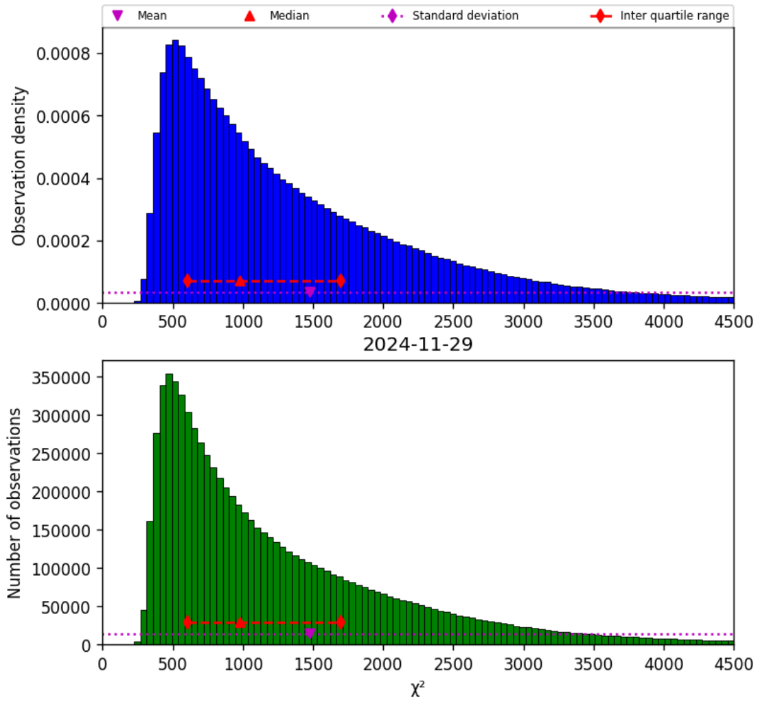
Figure 22: Histogram of “ \chi^2 ” for 2024-11-28 to 2024-11-30
