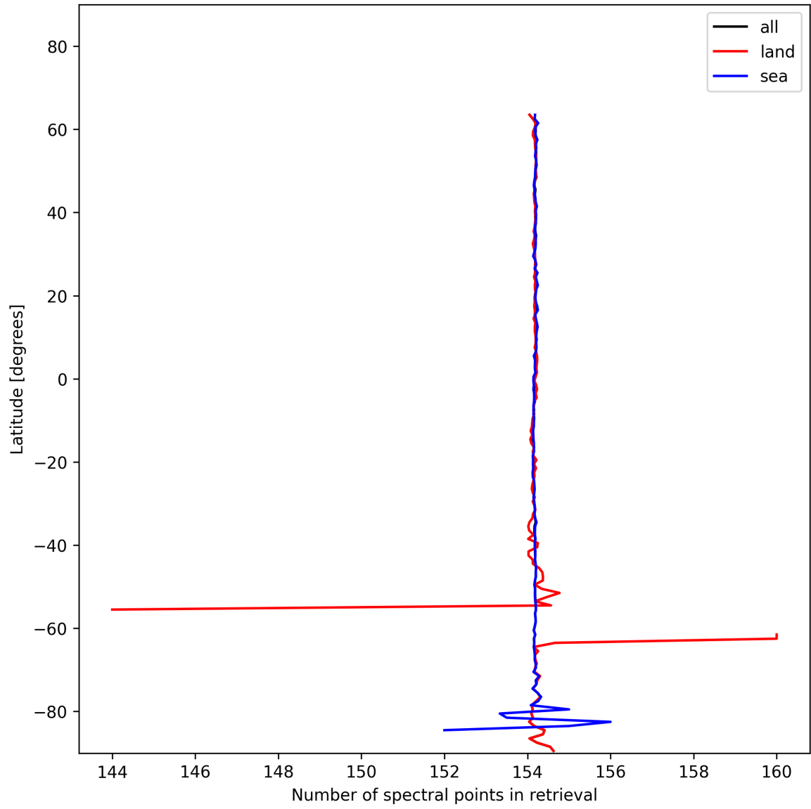
Figure 13: Zonal average of “Number of spectral points in retrieval” for 2024-11-28 to 2024-11-30.
