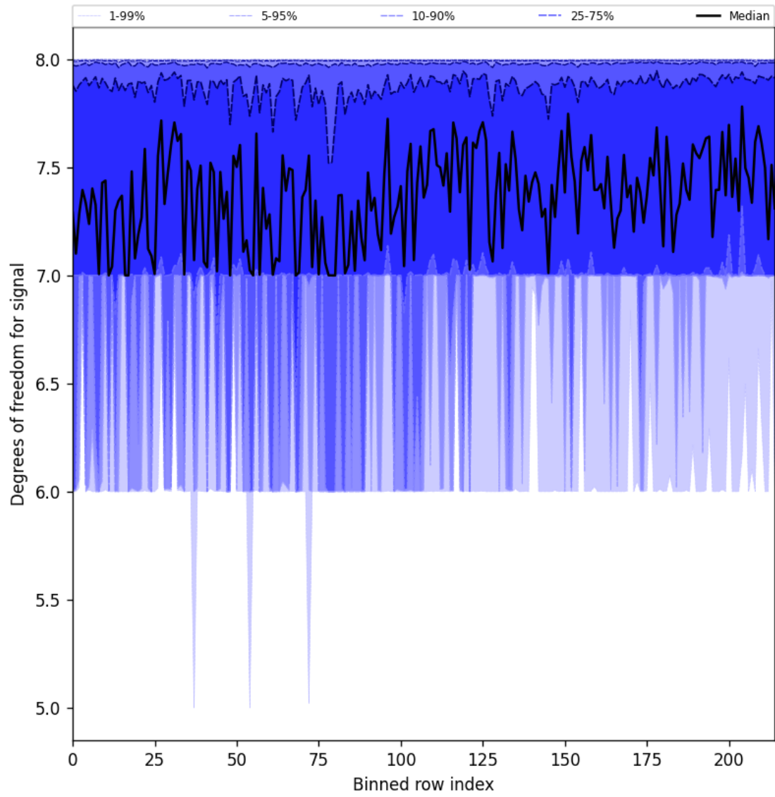
Figure 31: Along track statistics of “Degrees of freedom for signal” for 2024-11-28 to 2024-11-30
