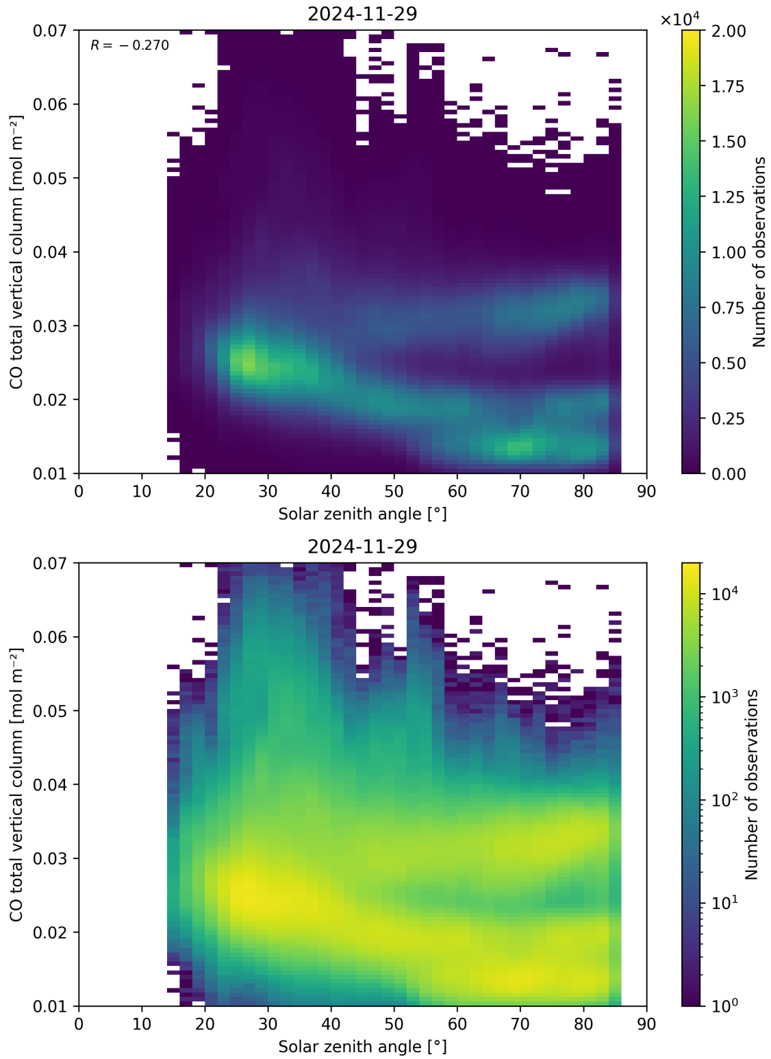
Figure 61: Scatter density plot of “Solar zenith angle” against “CO total vertical column” for 2024-11-28 to 2024-11-30.
