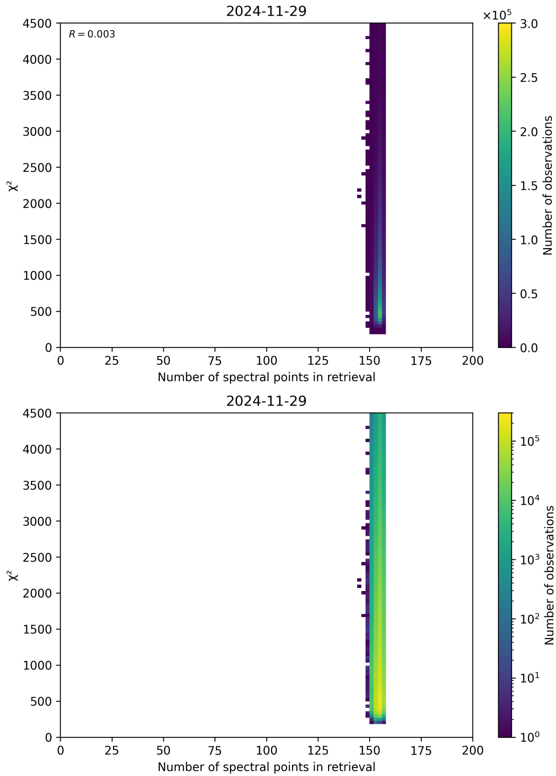
Figure 58: Scatter density plot of “Number of spectral points in retrieval” against “ \chi^2 ” for 2024-11-28 to 2024-11-30.
