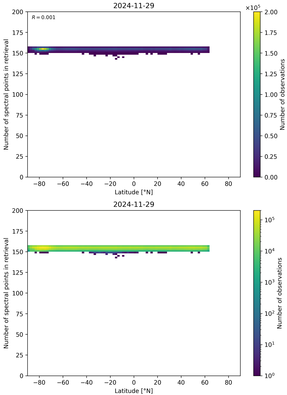
Figure 57: Scatter density plot of “Latitude” against “Number of spectral points in retrieval” for 2024-11-28 to 2024-11-30.
