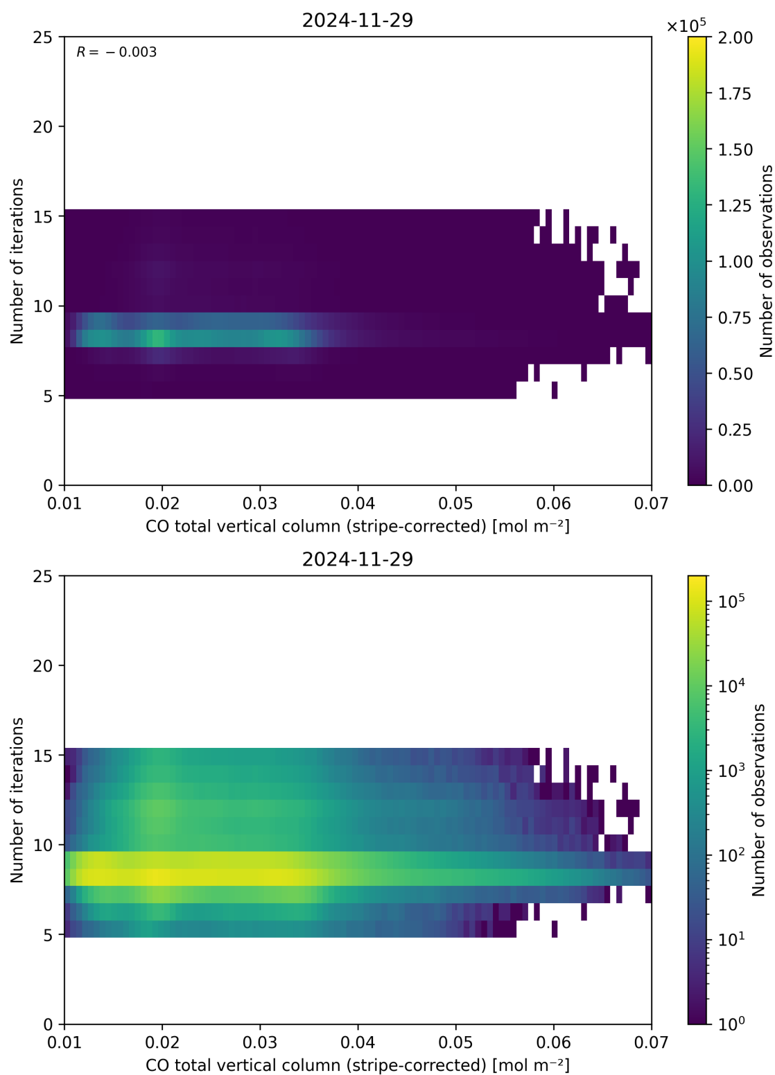
Figure 39: Scatter density plot of “CO total vertical column (stripe-corrected)” against “Number of iterations” for 2024-11-28 to 2024-11-30.
