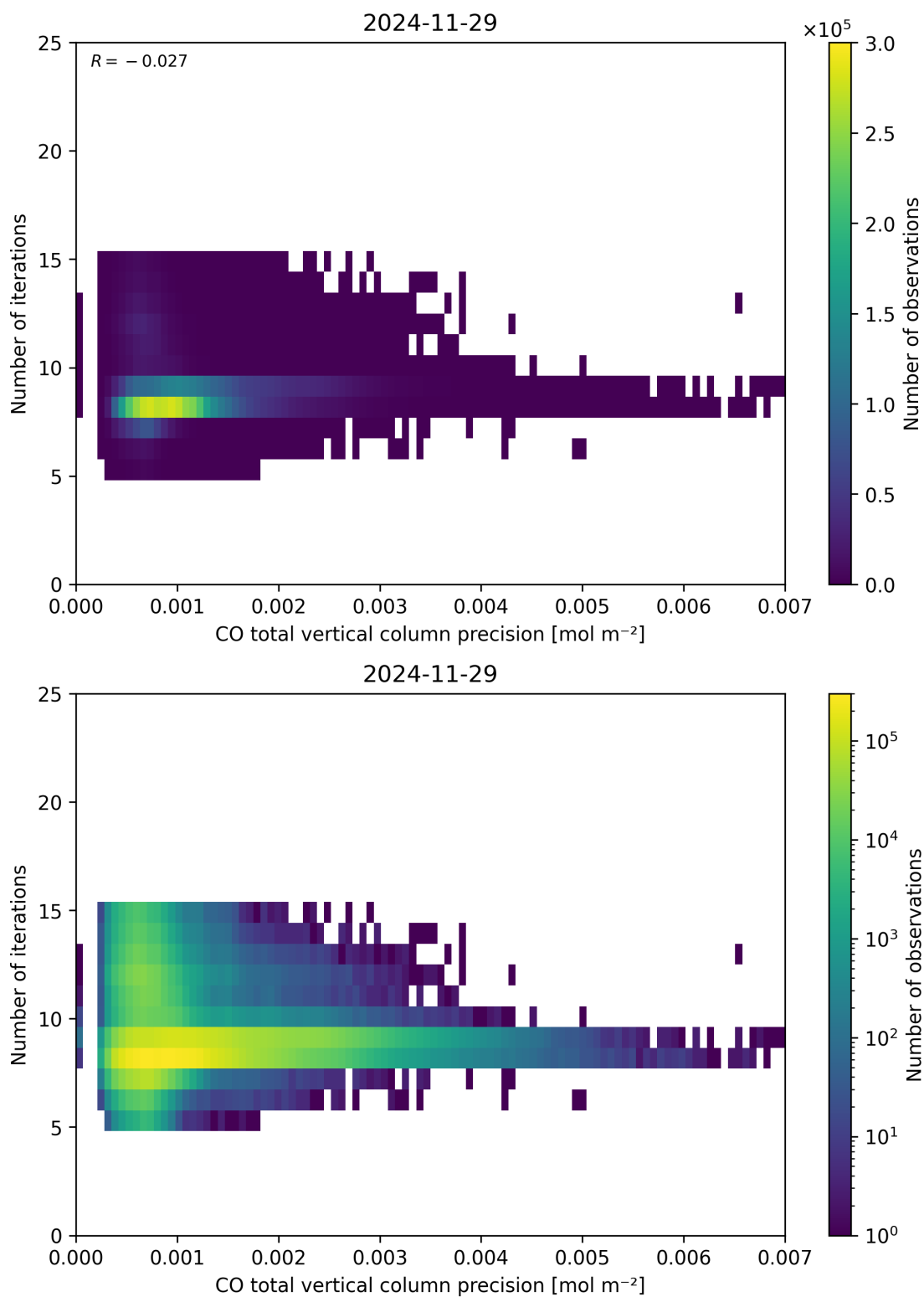
Figure 46: Scatter density plot of “CO total vertical column precision” against “Number of iterations” for 2024-11-28 to 2024-11-30.
