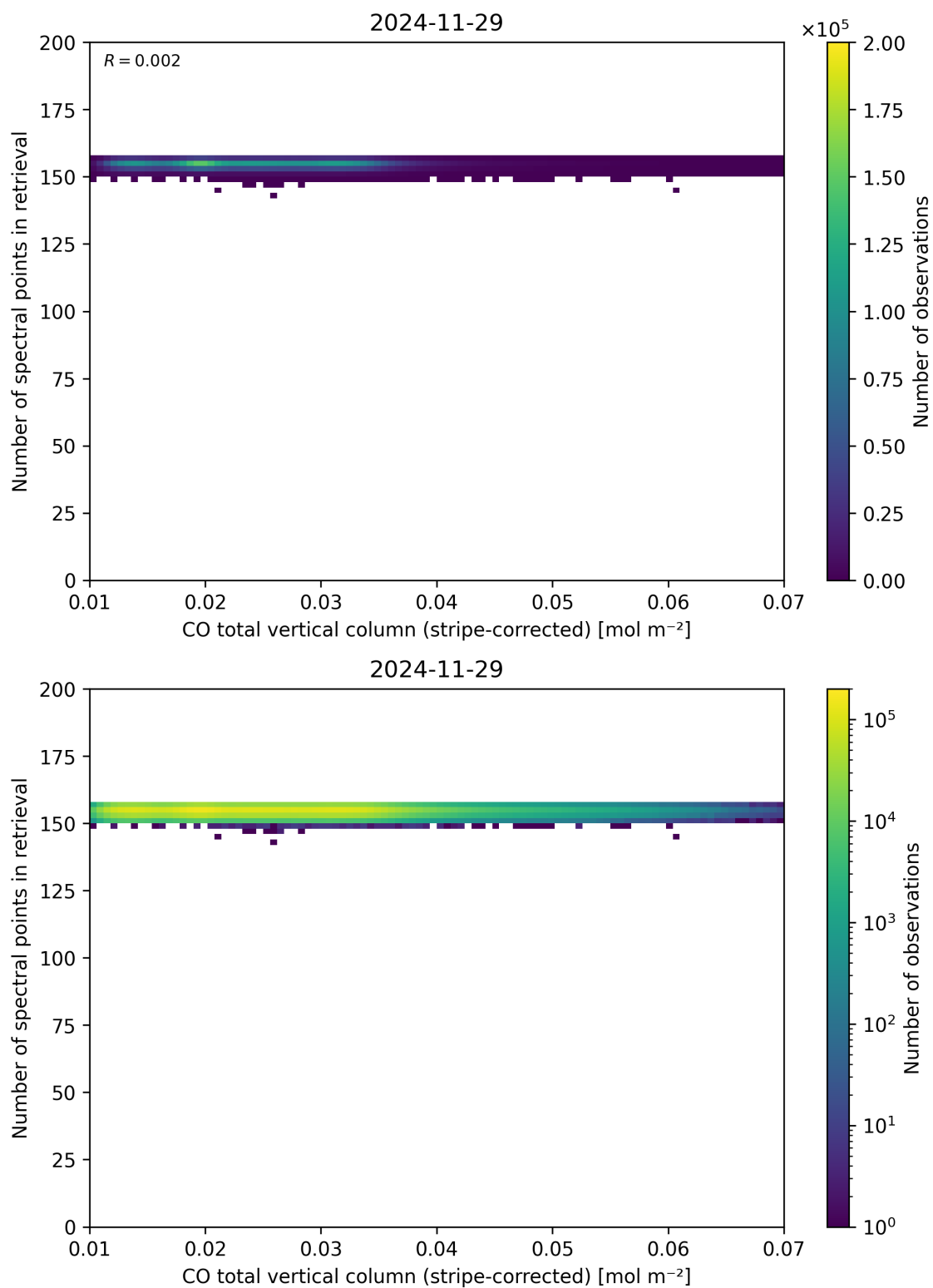
Figure 40: Scatter density plot of “CO total vertical column (stripe-corrected)” against “Number of spectral points in retrieval” for 2024-11-28 to 2024-11-30.
