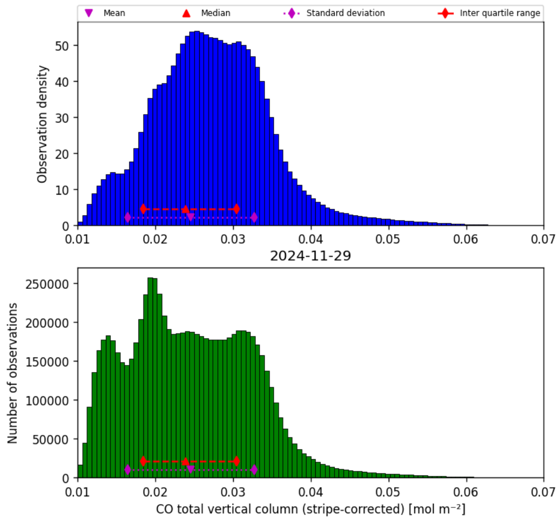
Figure 19: Histogram of “CO total vertical column (stripe-corrected)” for 2024-11-28 to 2024-11-30
