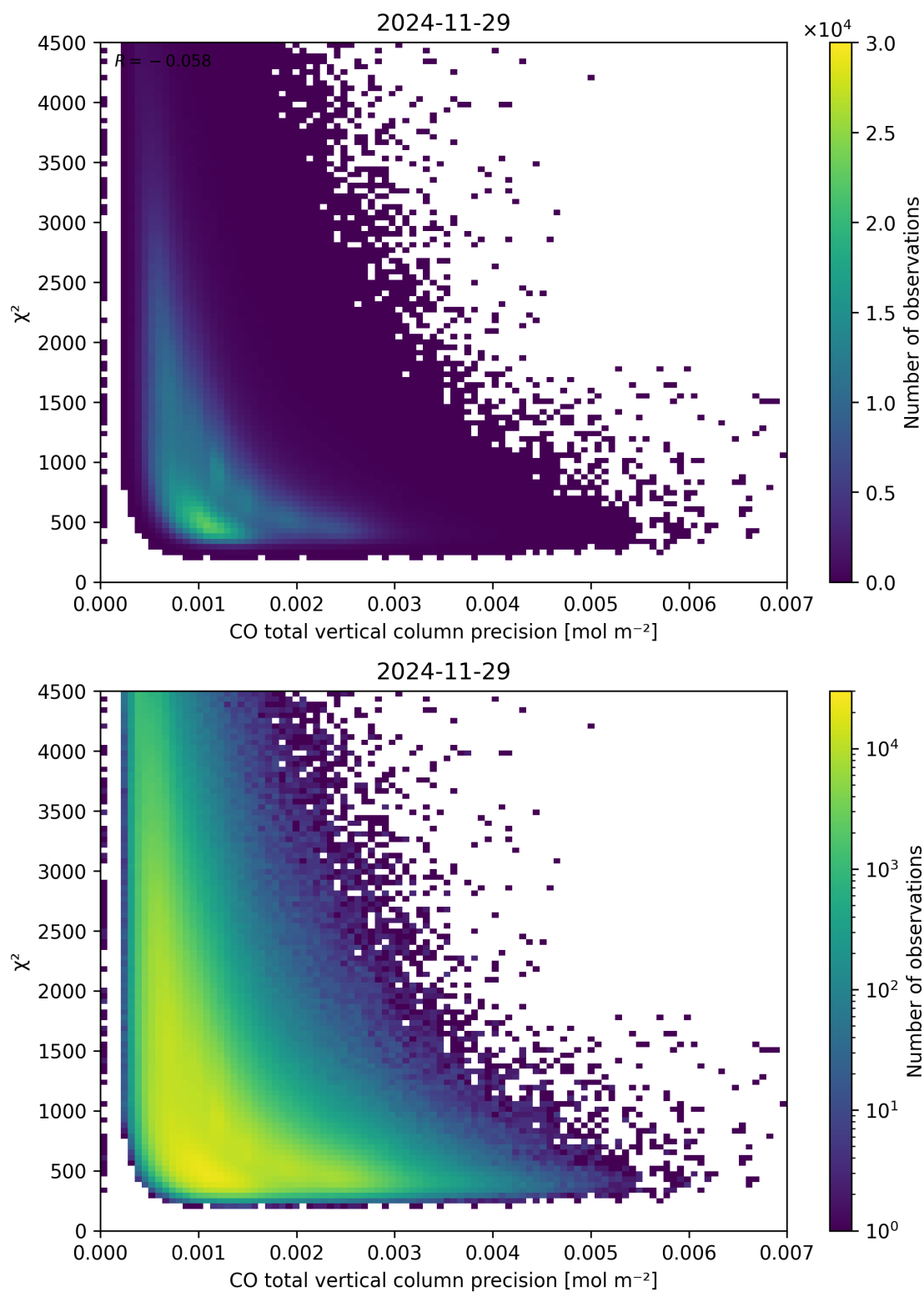
Figure 44: Scatter density plot of “CO total vertical column precision” against “ \chi^2 ” for 2024-11-28 to 2024-11-30.
