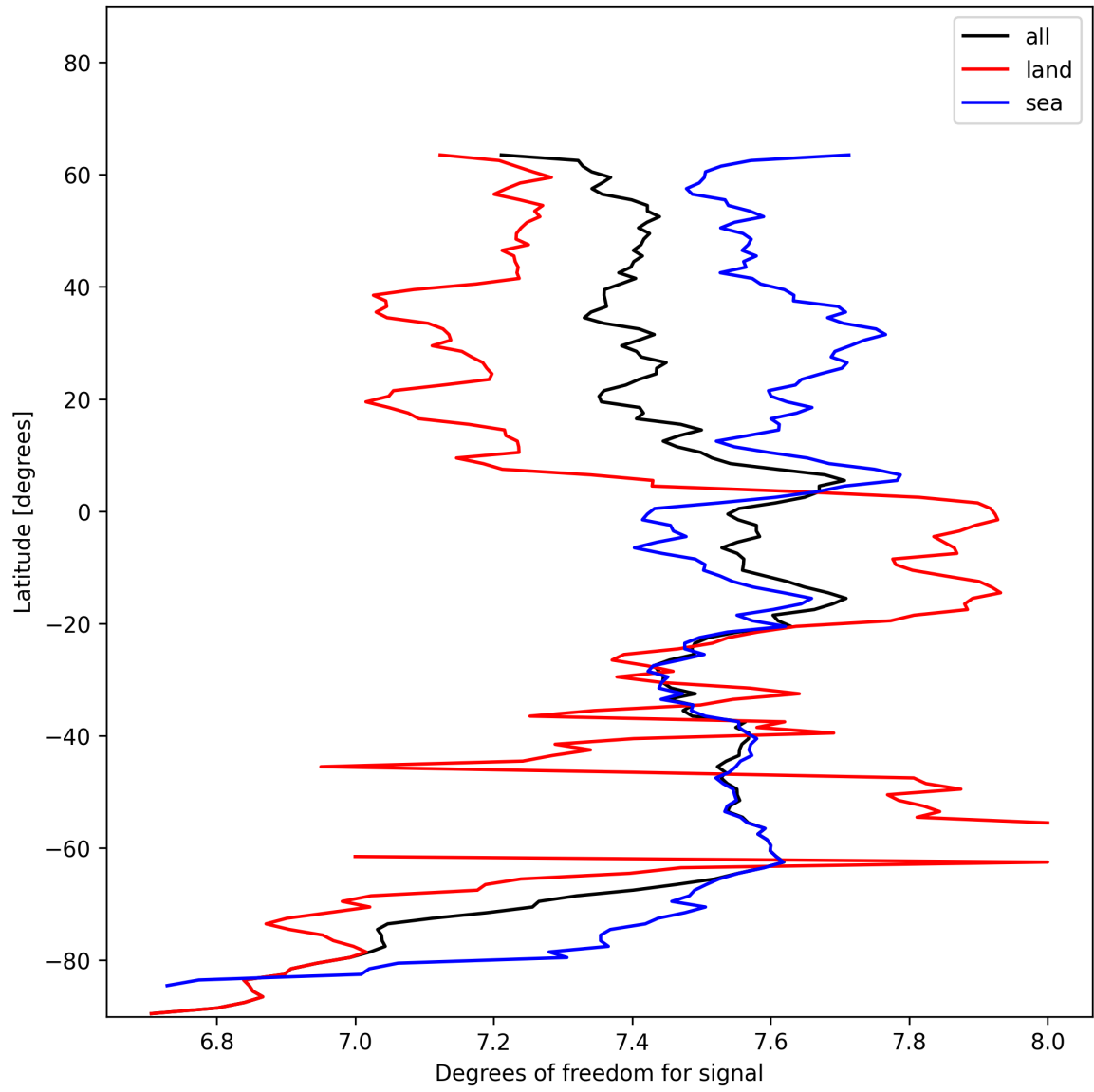
Figure 15: Zonal average of “Degrees of freedom for signal” for 2024-11-28 to 2024-11-30.
