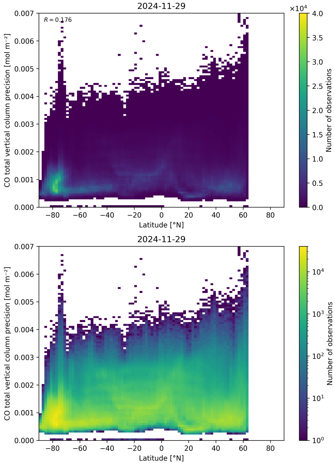
Figure 53: Scatter density plot of “Latitude” against “CO total vertical column precision” for 2024-11-28 to 2024-11-30.
