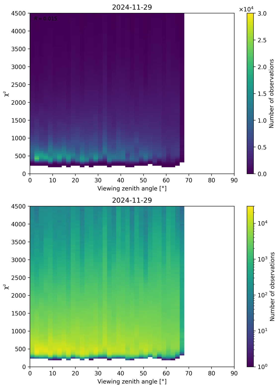
Figure 72: Scatter density plot of “Viewing zenith angle” against “ \chi^2 ” for 2024-11-28 to 2024-11-30.
