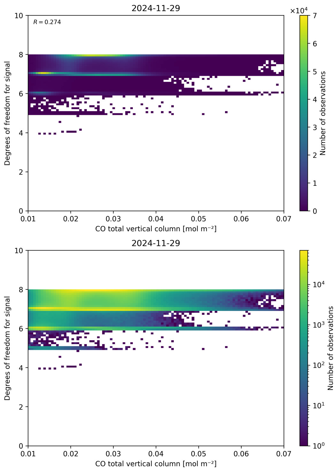
Figure 41: Scatter density plot of “CO total vertical column” against “Degrees of freedom for signal” for 2024-11-28 to 2024-11-30.
