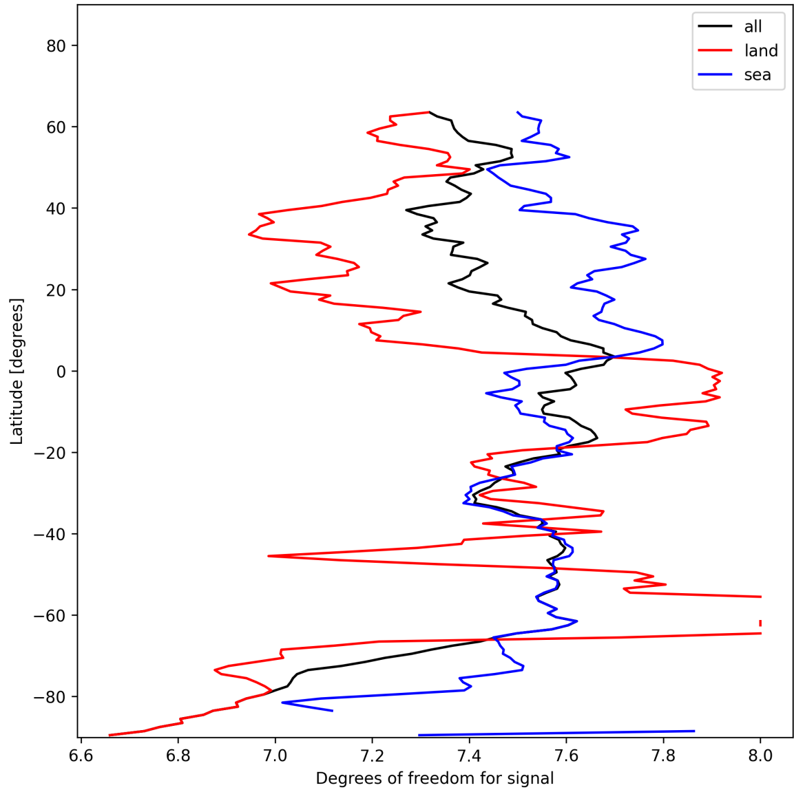
Figure 15: Zonal average of “Degrees of freedom for signal” for 2024-11-30 to 2024-12-01.
