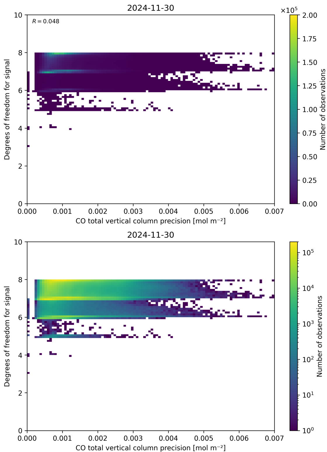
Figure 45: Scatter density plot of “CO total vertical column precision” against “Degrees of freedom for signal” for 2024-11-30 to 2024-12-01.
