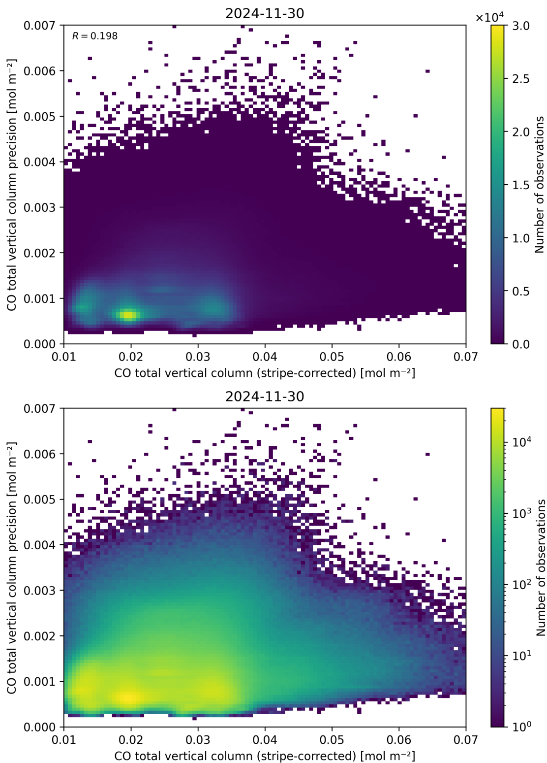
Figure 36: Scatter density plot of “CO total vertical column (stripe-corrected)” against “CO total vertical column precision” for 2024-11-30 to 2024-12-01.
