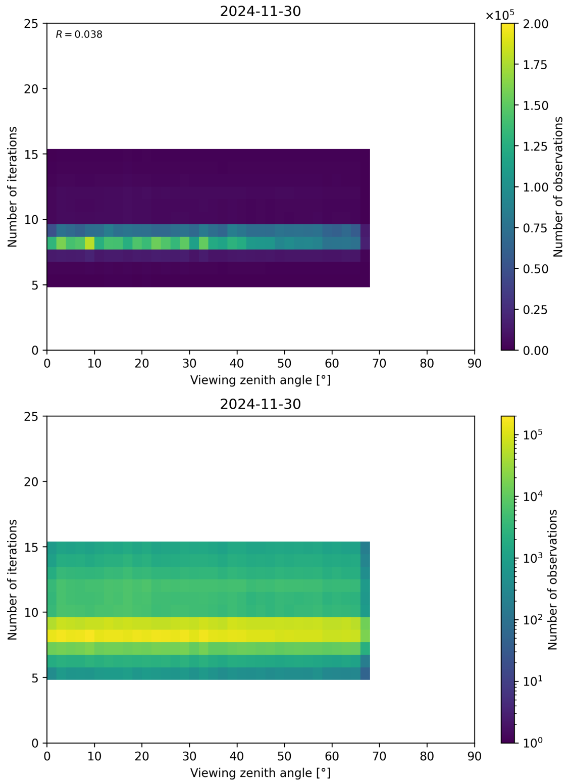
Figure 75: Scatter density plot of “Viewing zenith angle” against “Number of iterations” for 2024-11-30 to 2024-12-01.
