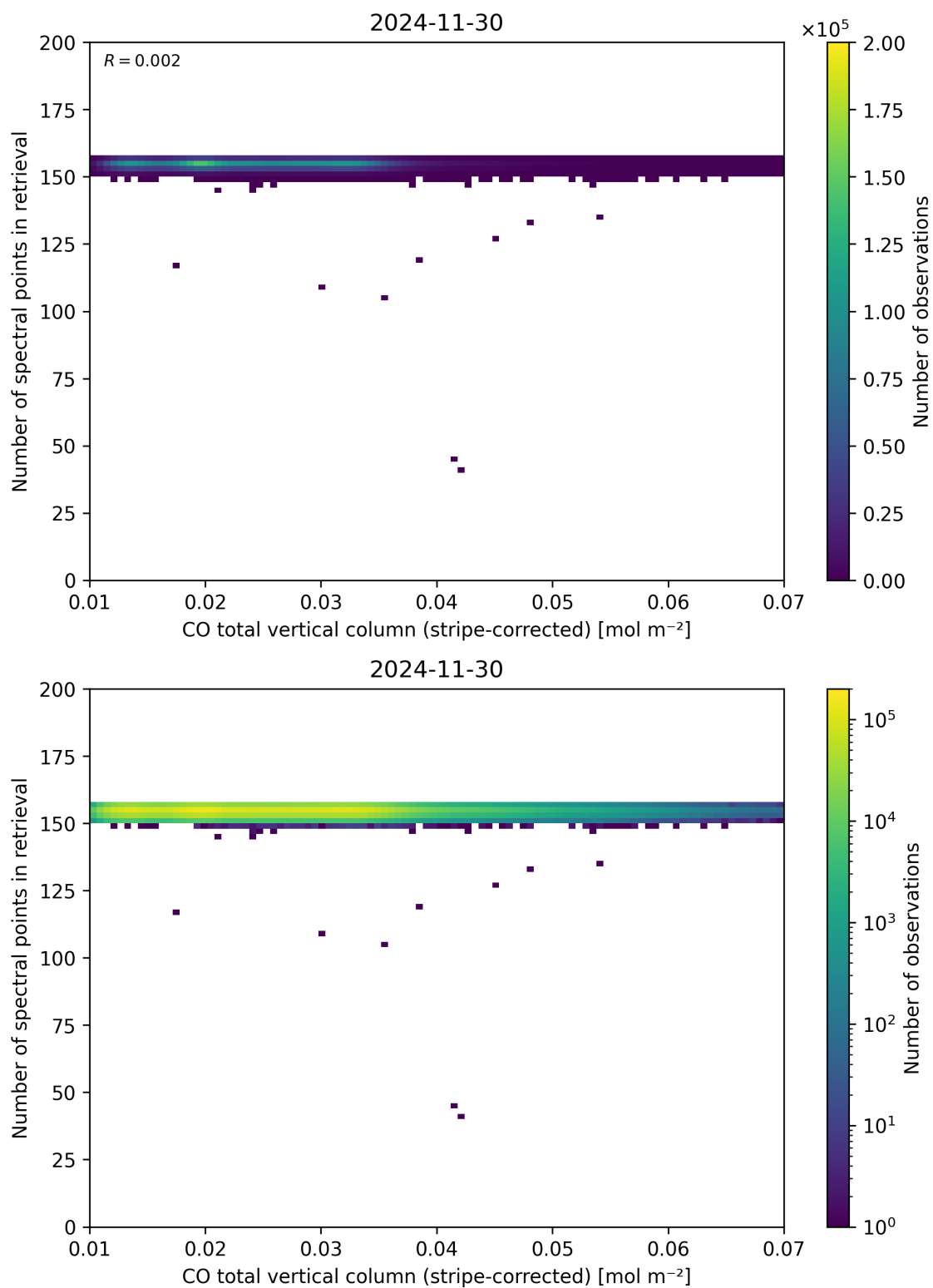
Figure 40: Scatter density plot of “CO total vertical column (stripe-corrected)” against “Number of spectral points in retrieval” for 2024-11-30 to 2024-12-01.
