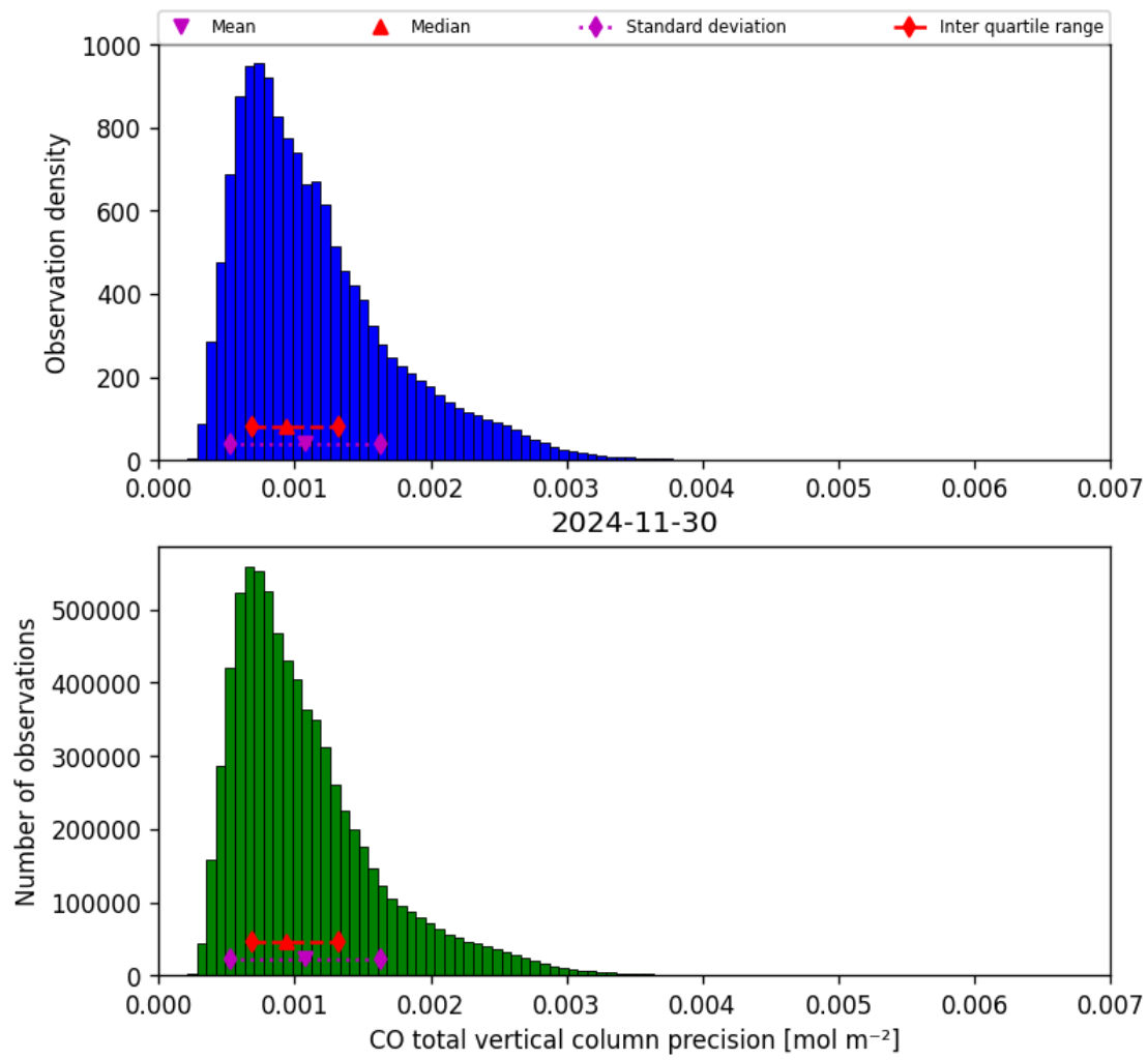
Figure 20: Histogram of “CO total vertical column precision” for 2024-11-30 to 2024-12-01
