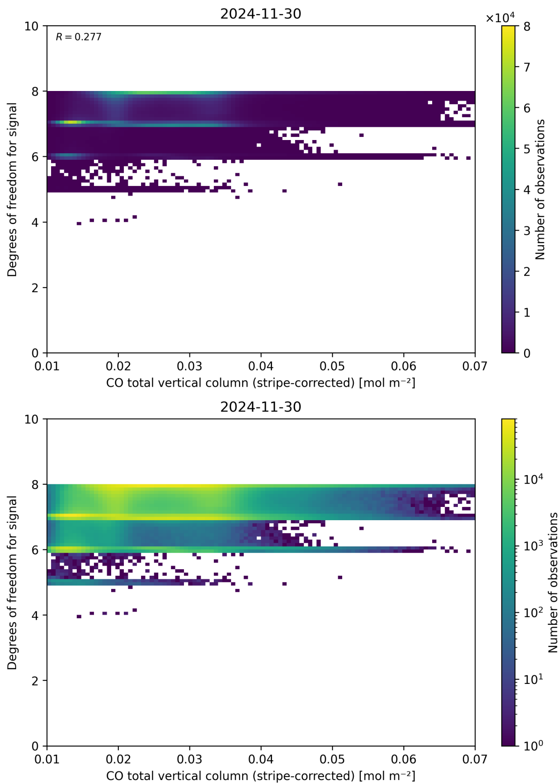
Figure 38: Scatter density plot of “CO total vertical column (stripe-corrected)” against “Degrees of freedom for signal” for 2024-11-30 to 2024-12-01.
