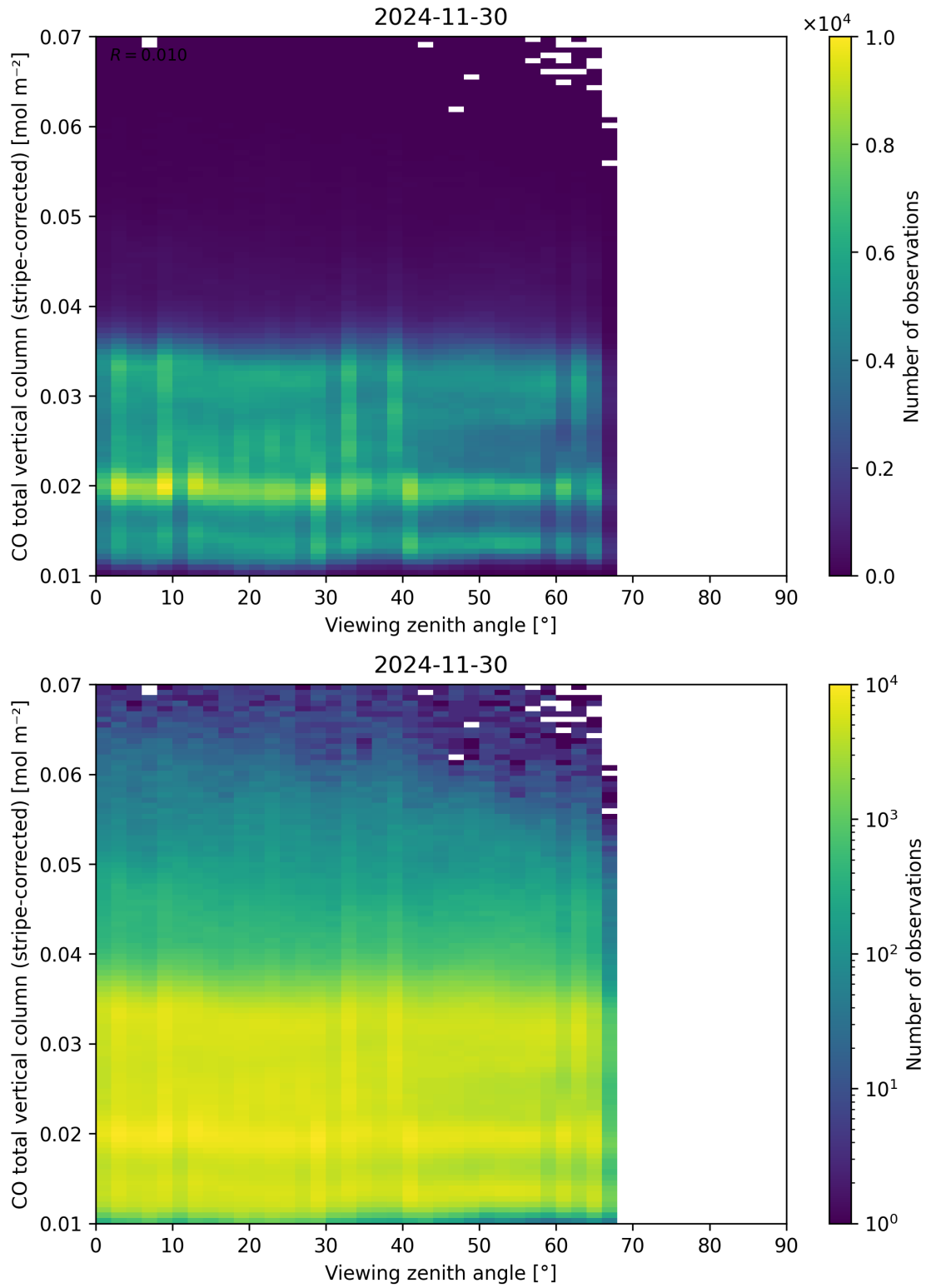
Figure 70: Scatter density plot of “Viewing zenith angle” against “CO total vertical column (stripe-corrected)” for 2024-11-30 to 2024-12-01.
