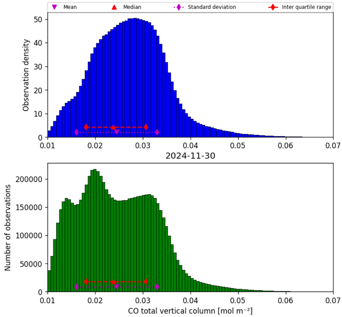
Figure 18: Histogram of “CO total vertical column” for 2024-11-30 to 2024-12-01
