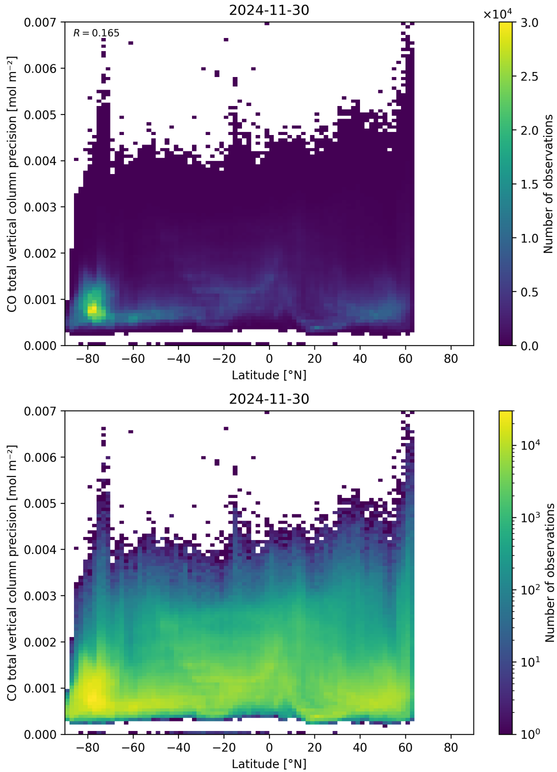
Figure 53: Scatter density plot of “Latitude” against “CO total vertical column precision” for 2024-11-30 to 2024-12-01.
