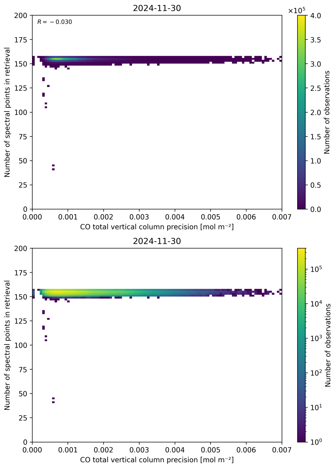
Figure 47: Scatter density plot of “CO total vertical column precision” against “Number of spectral points in retrieval” for 2024-11-30 to 2024-12-01.
