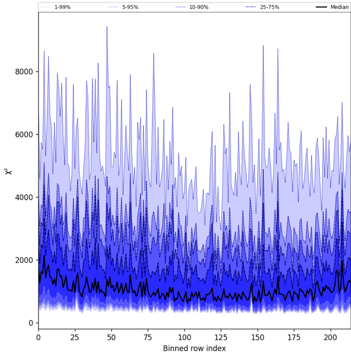
Figure 30: Along track statistics of “ \chi^2 ” for 2024-11-30 to 2024-12-01
