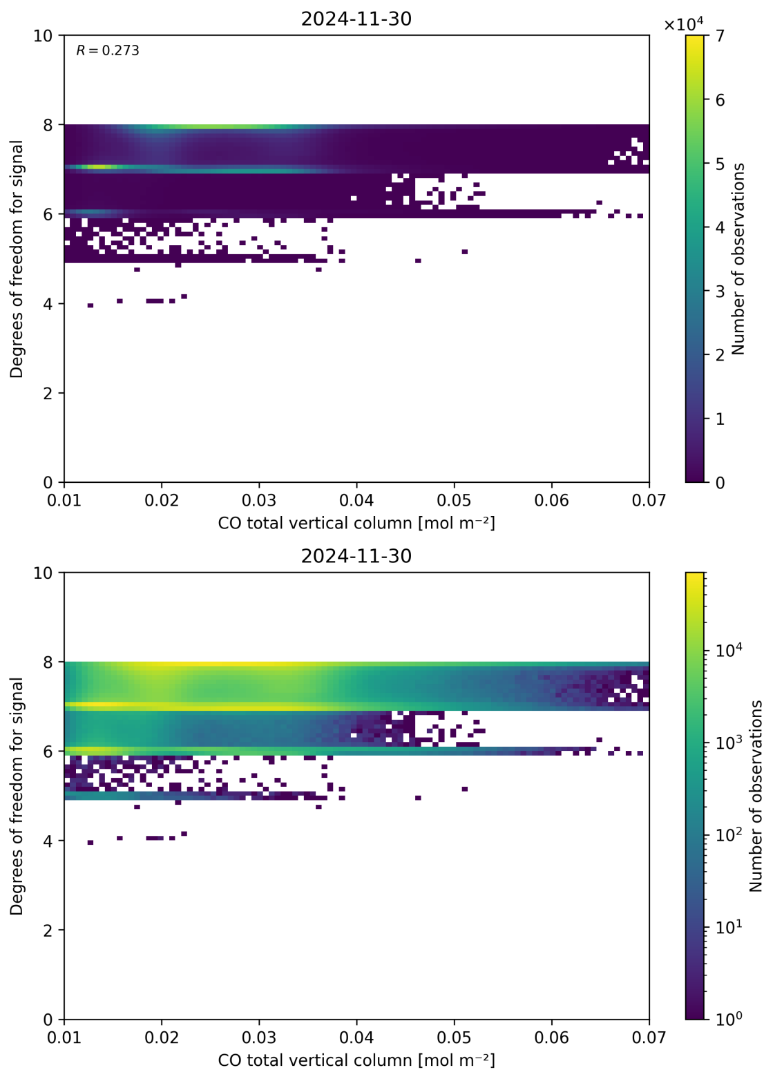
Figure 41: Scatter density plot of “CO total vertical column” against “Degrees of freedom for signal” for 2024-11-30 to 2024-12-01.
