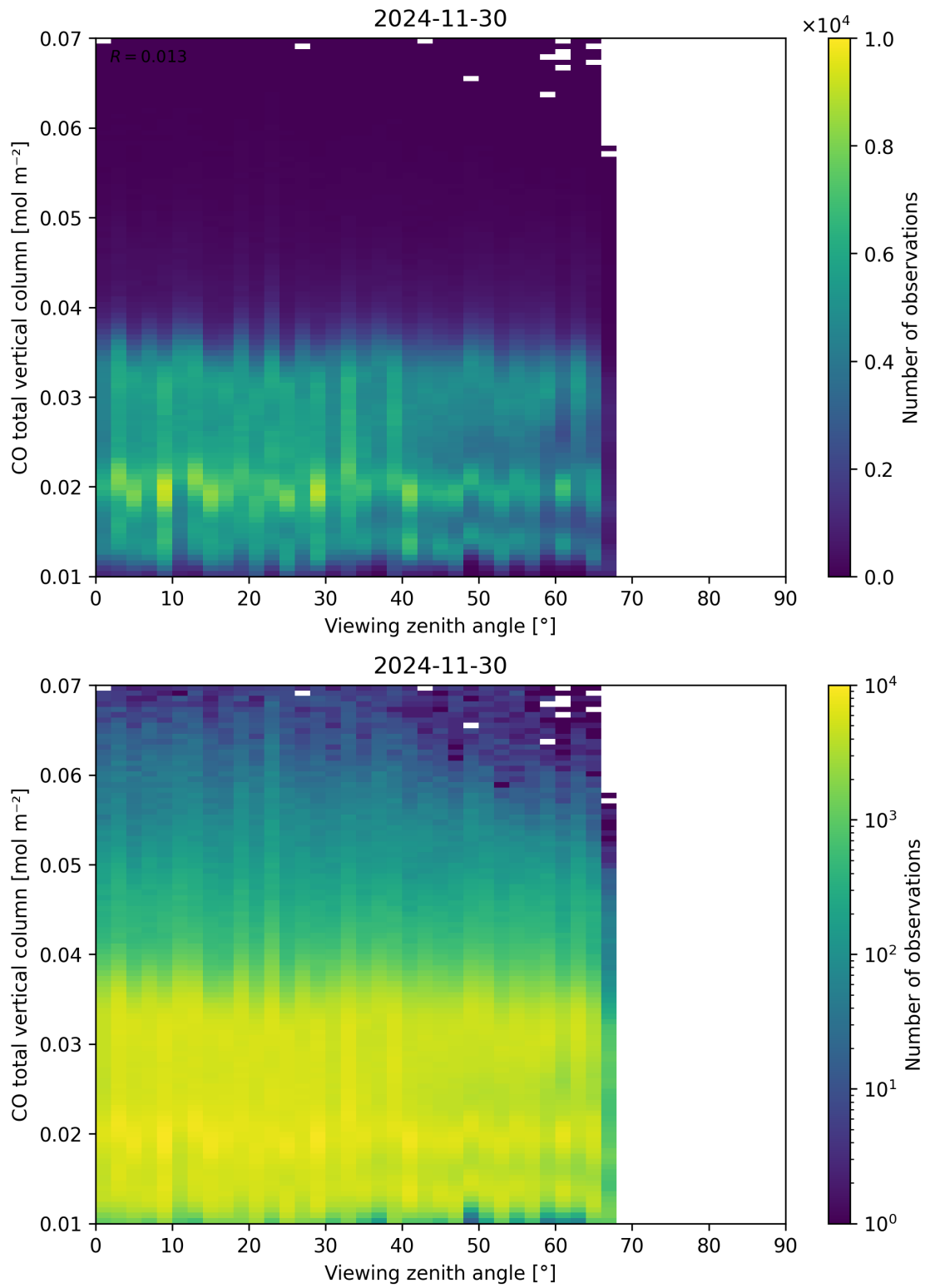
Figure 69: Scatter density plot of “Viewing zenith angle” against “CO total vertical column” for 2024-11-30 to 2024-12-01.
