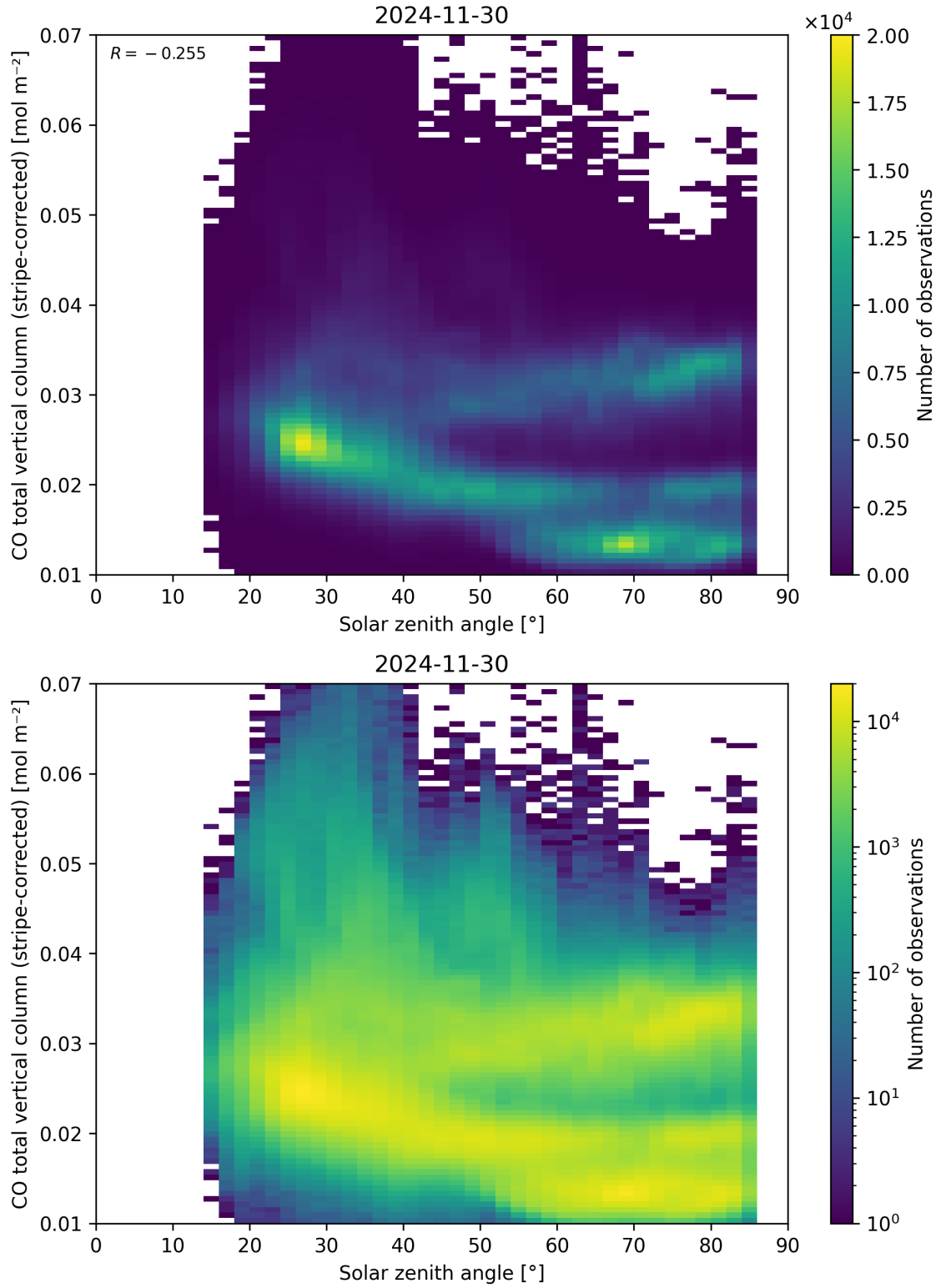
Figure 62: Scatter density plot of “Solar zenith angle” against “CO total vertical column (stripe-corrected)” for 2024-11-30 to 2024-12-01.
