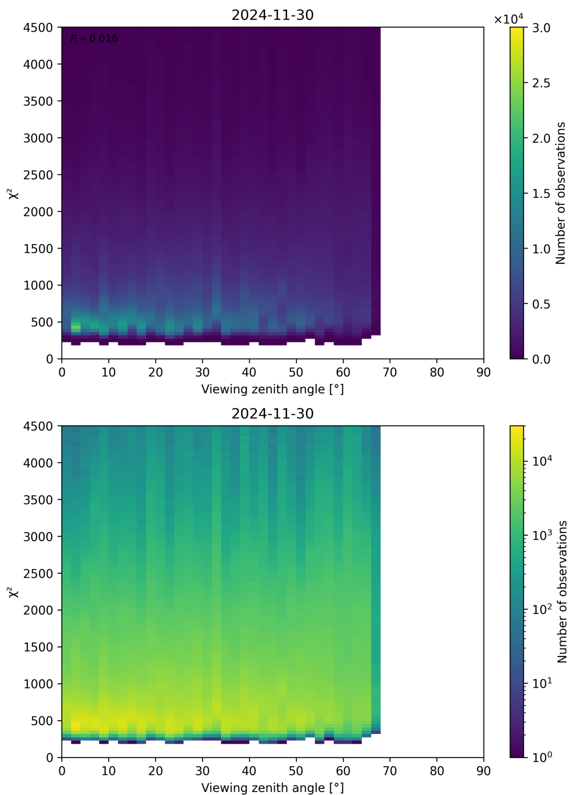
Figure 72: Scatter density plot of “Viewing zenith angle” against “ \chi^2 ” for 2024-11-30 to 2024-12-01.
