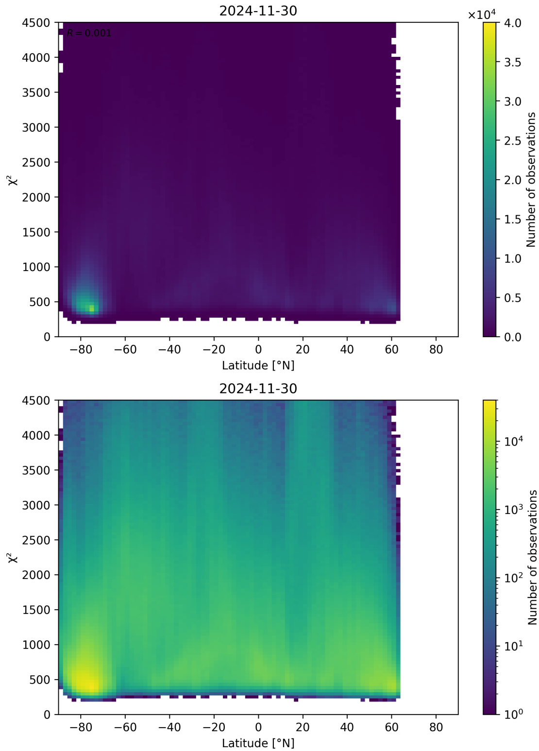
Figure 54: Scatter density plot of “Latitude” against “ \chi^2 ” for 2024-11-30 to 2024-12-01.
