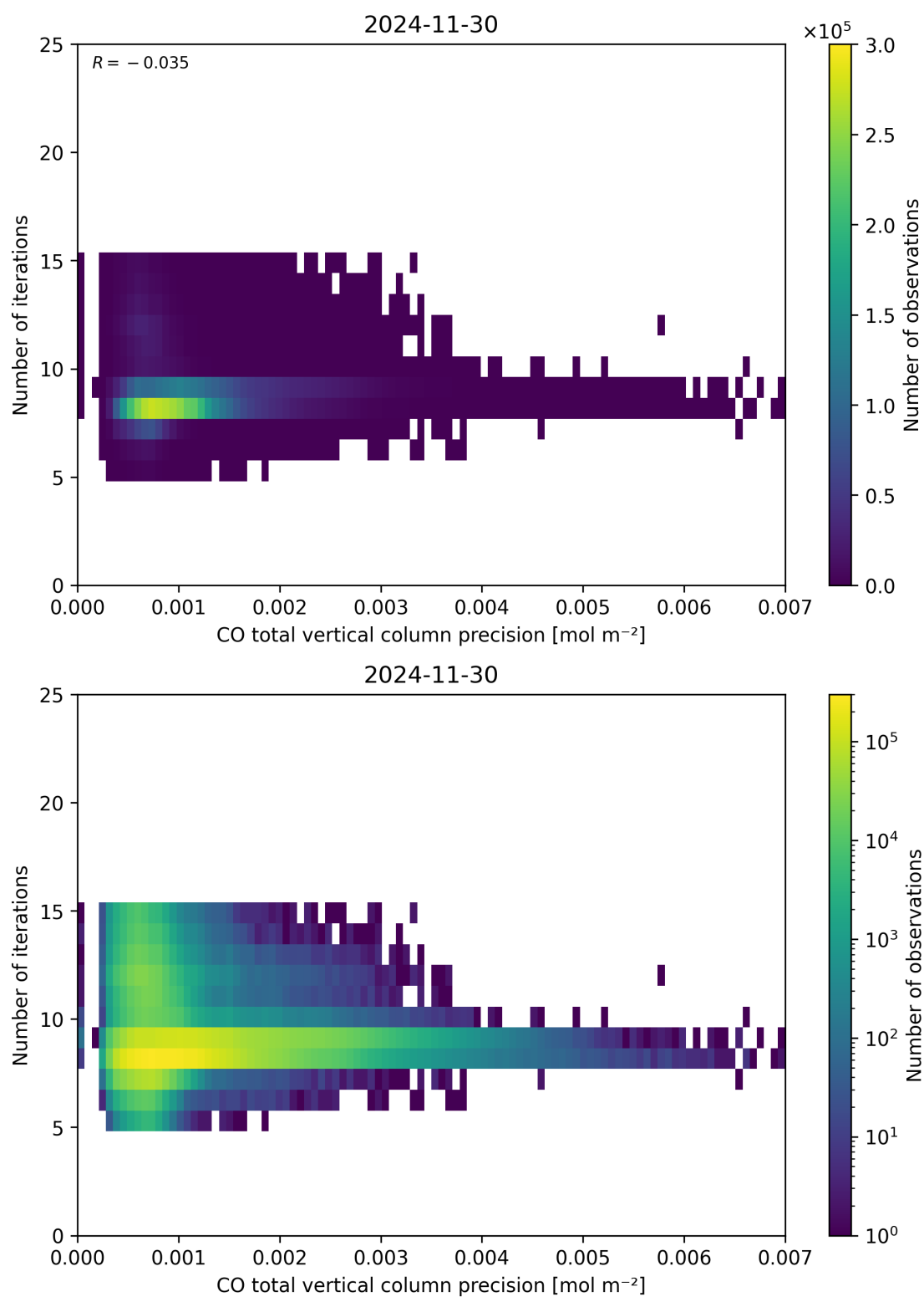
Figure 46: Scatter density plot of “CO total vertical column precision” against “Number of iterations” for 2024-11-30 to 2024-12-01.
