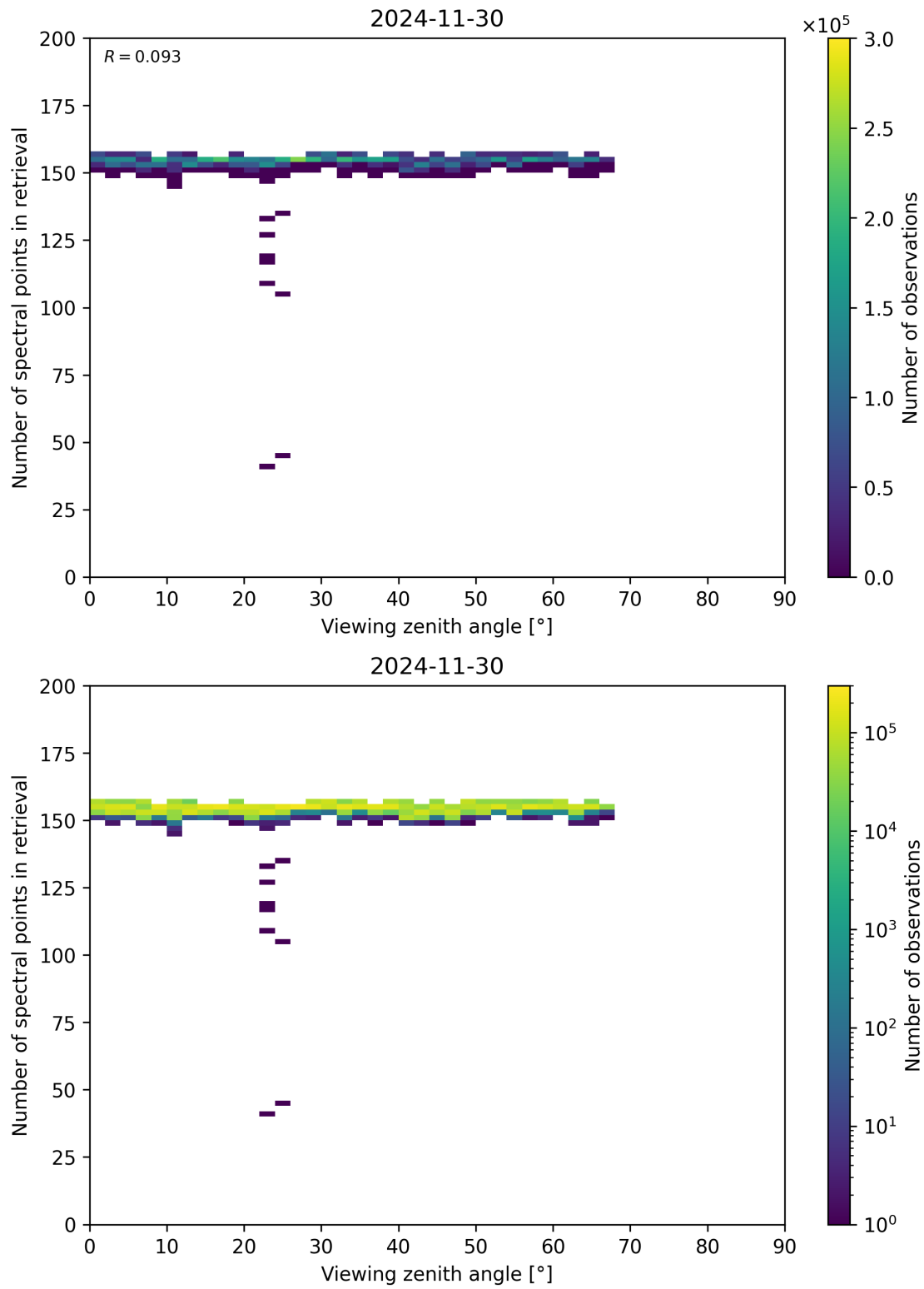
Figure 76: Scatter density plot of “Viewing zenith angle” against “Number of spectral points in retrieval” for 2024-11-30 to 2024-12-01.
