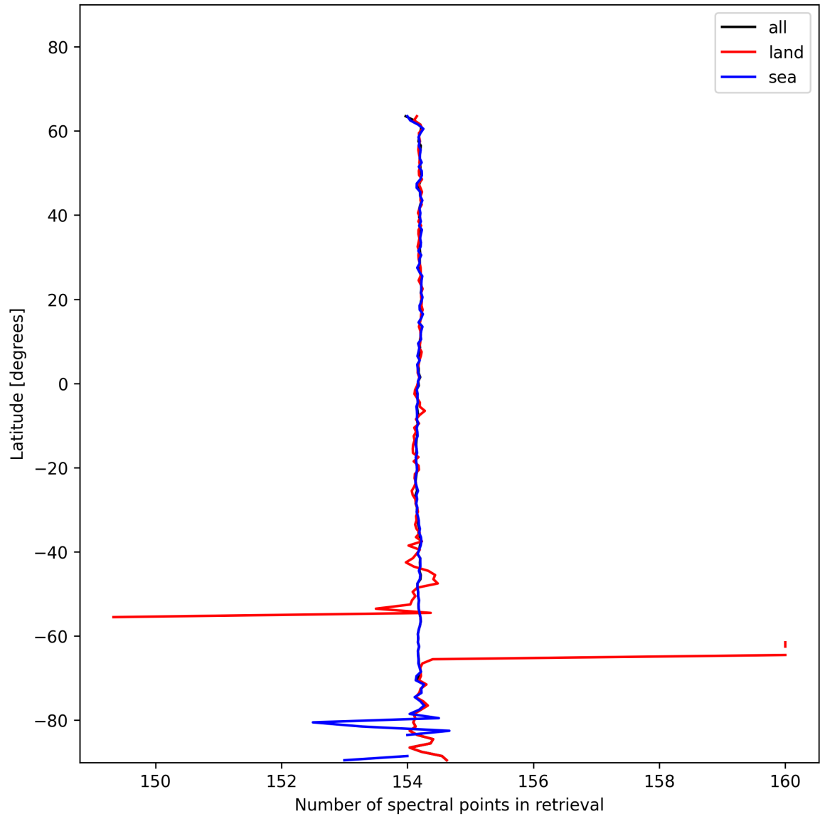
Figure 13: Zonal average of “Number of spectral points in retrieval” for 2024-11-30 to 2024-12-01.
