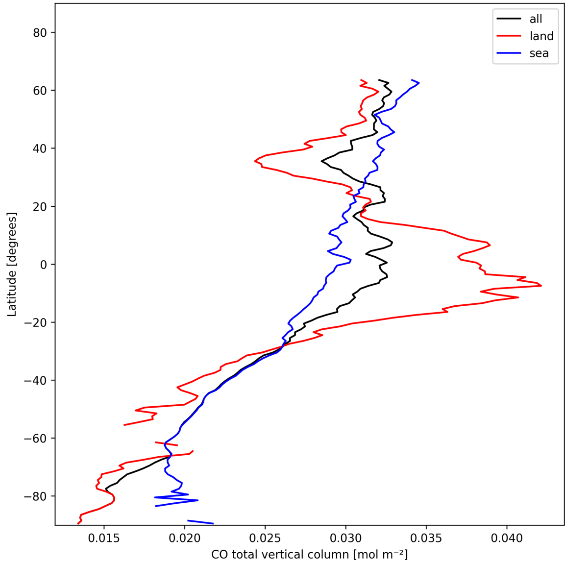
Figure 10: Zonal average of “CO total vertical column” for 2024-11-30 to 2024-12-01.
