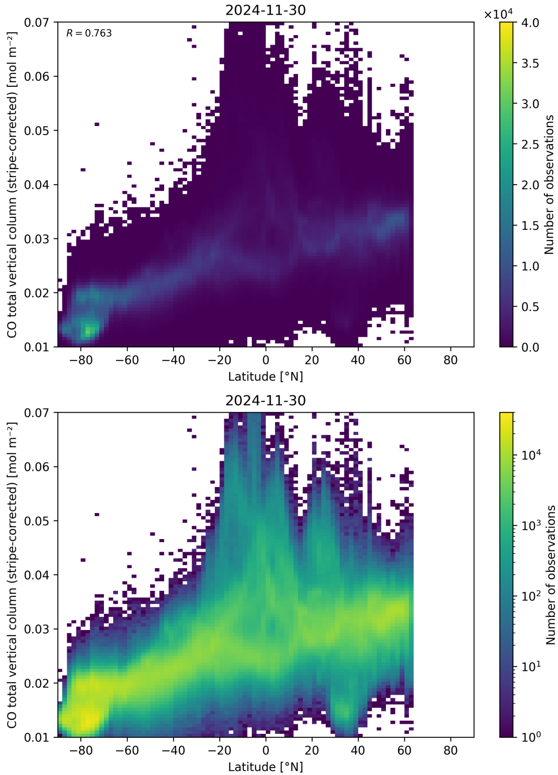
Figure 52: Scatter density plot of “Latitude” against “CO total vertical column (stripe-corrected)” for 2024-11-30 to 2024-12-01.
