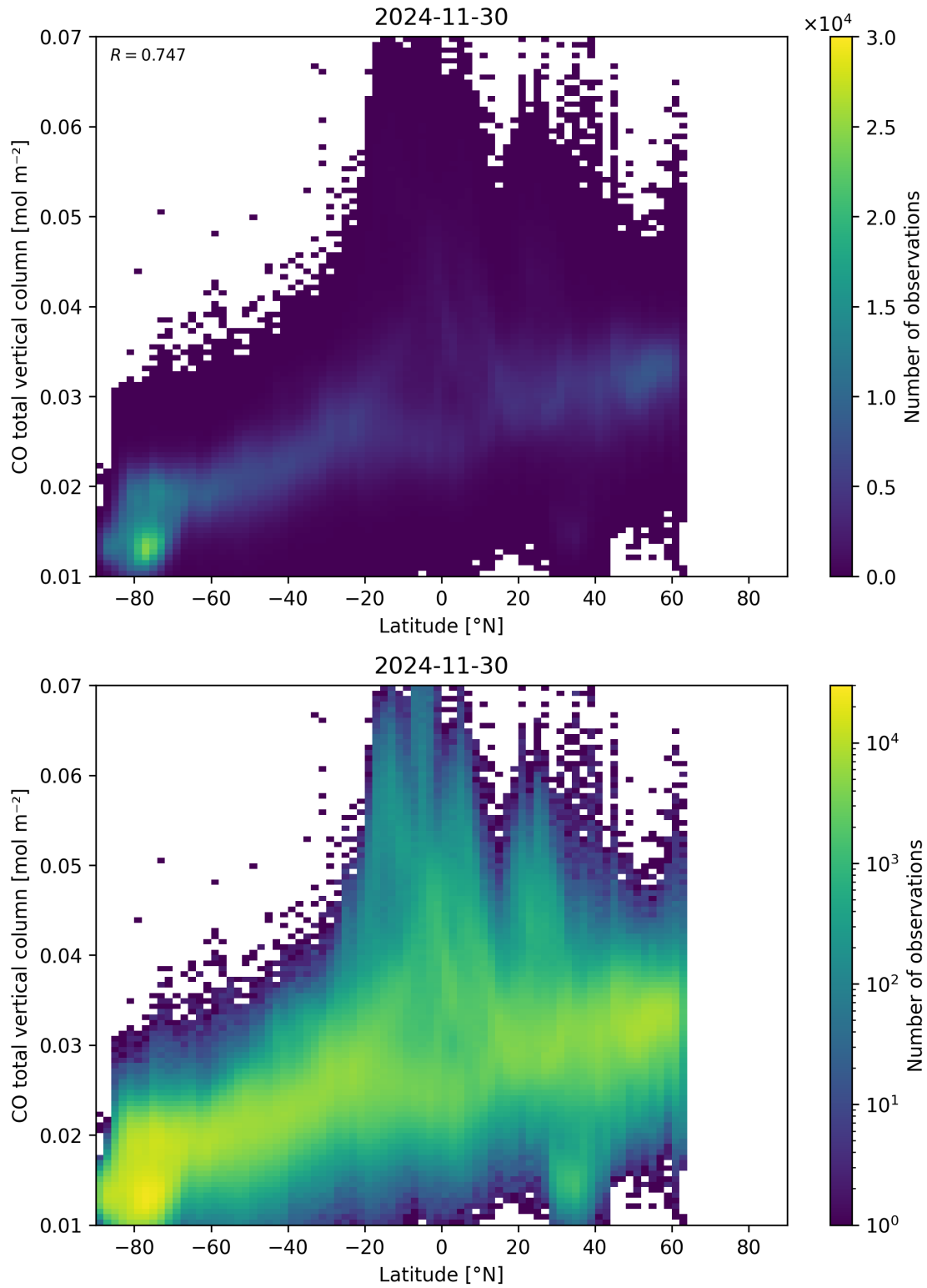
Figure 51: Scatter density plot of “Latitude” against “CO total vertical column” for 2024-11-30 to 2024-12-01.
