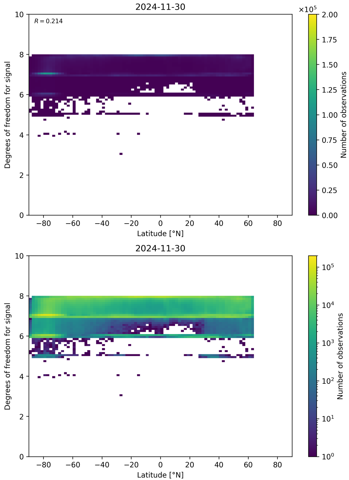
Figure 55: Scatter density plot of “Latitude” against “Degrees of freedom for signal” for 2024-11-30 to 2024-12-01.
