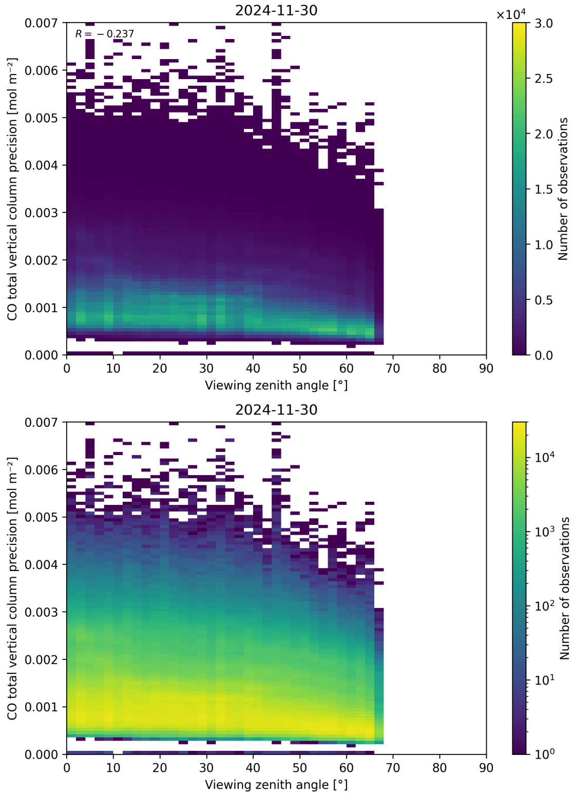
Figure 71: Scatter density plot of “Viewing zenith angle” against “CO total vertical column precision” for 2024-11-30 to 2024-12-01.
