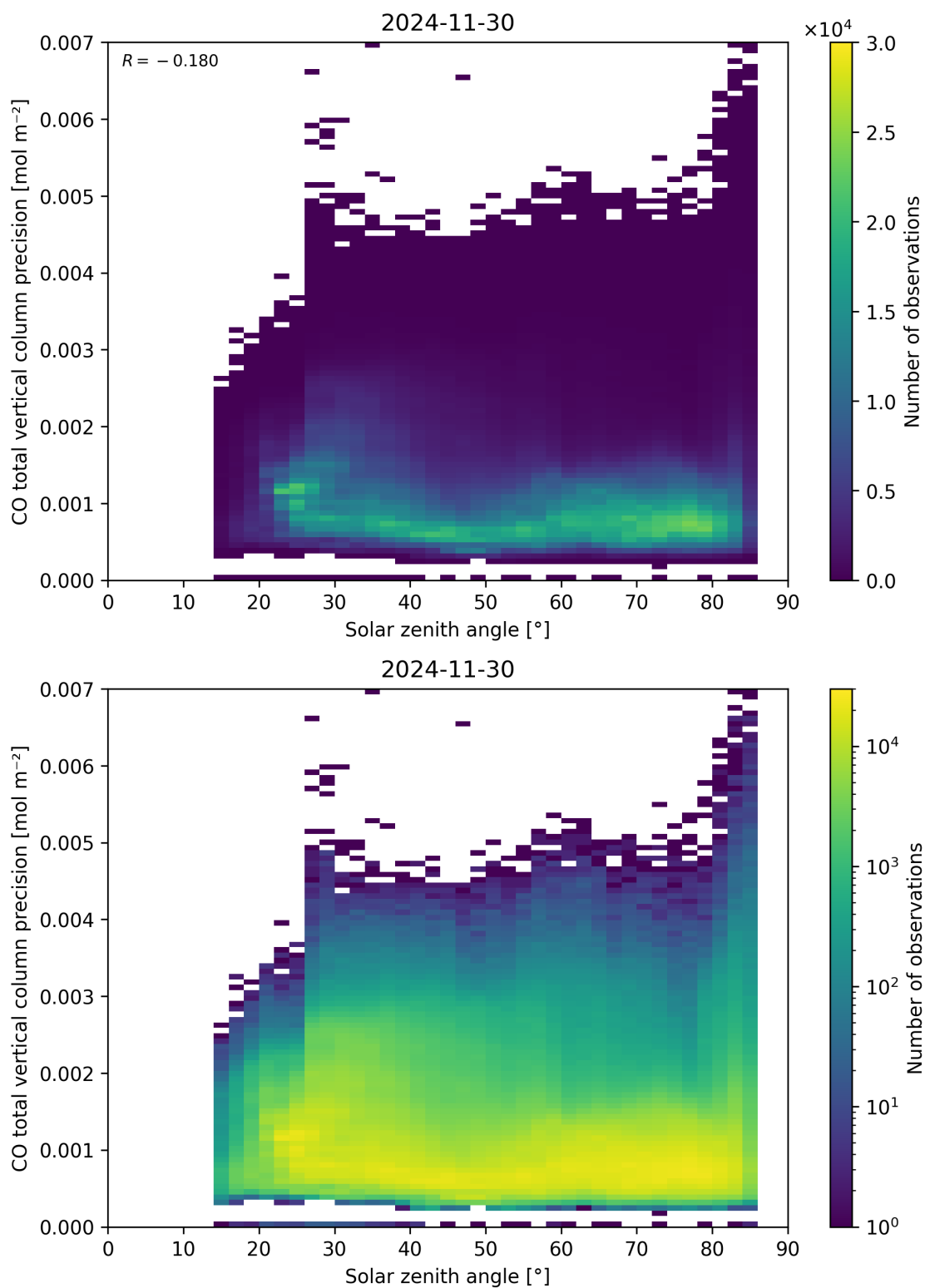
Figure 63: Scatter density plot of “Solar zenith angle” against “CO total vertical column precision” for 2024-11-30 to 2024-12-01.
