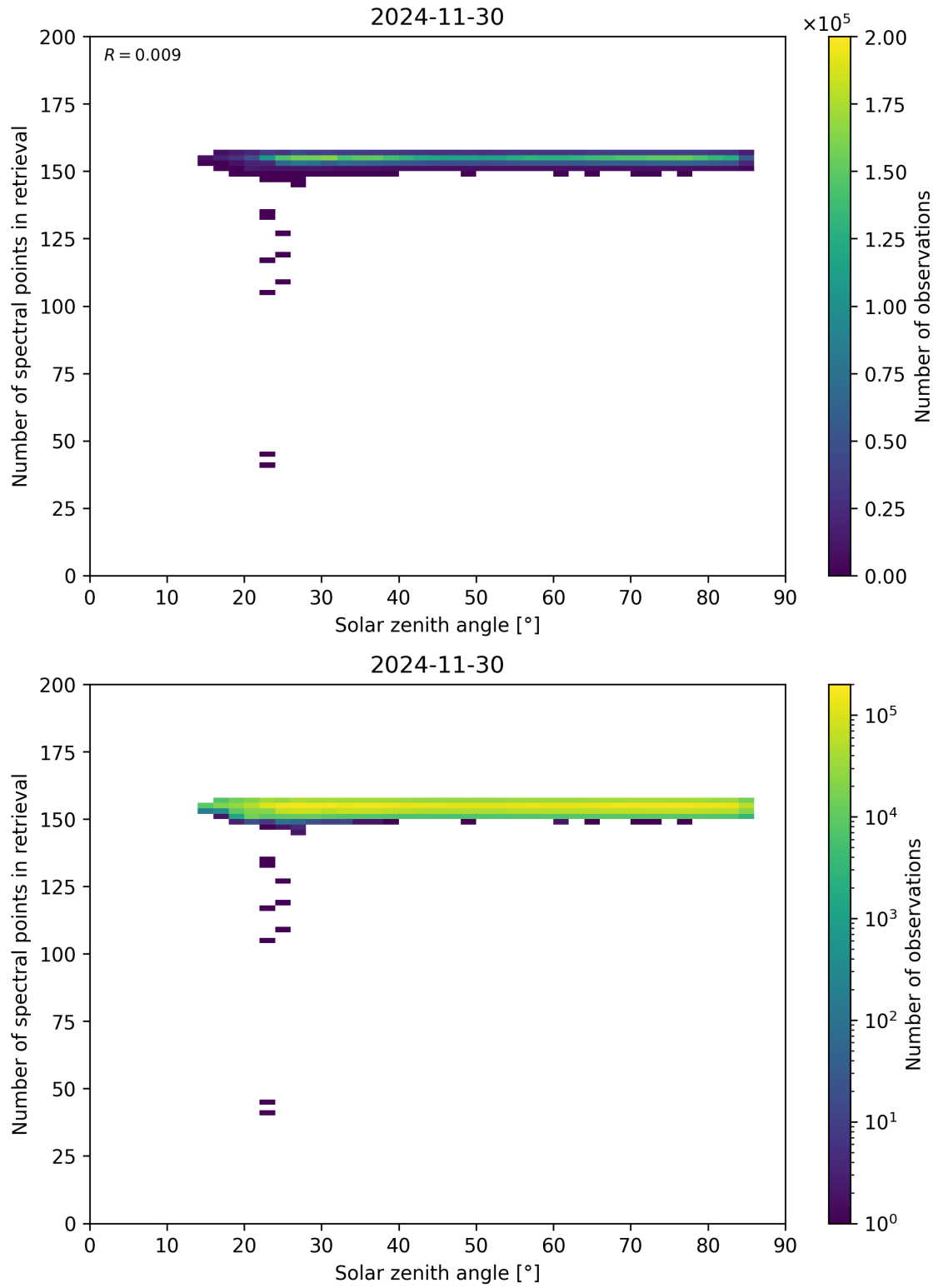
Figure 68: Scatter density plot of “Solar zenith angle” against “Number of spectral points in retrieval” for 2024-11-30 to 2024-12-01.
