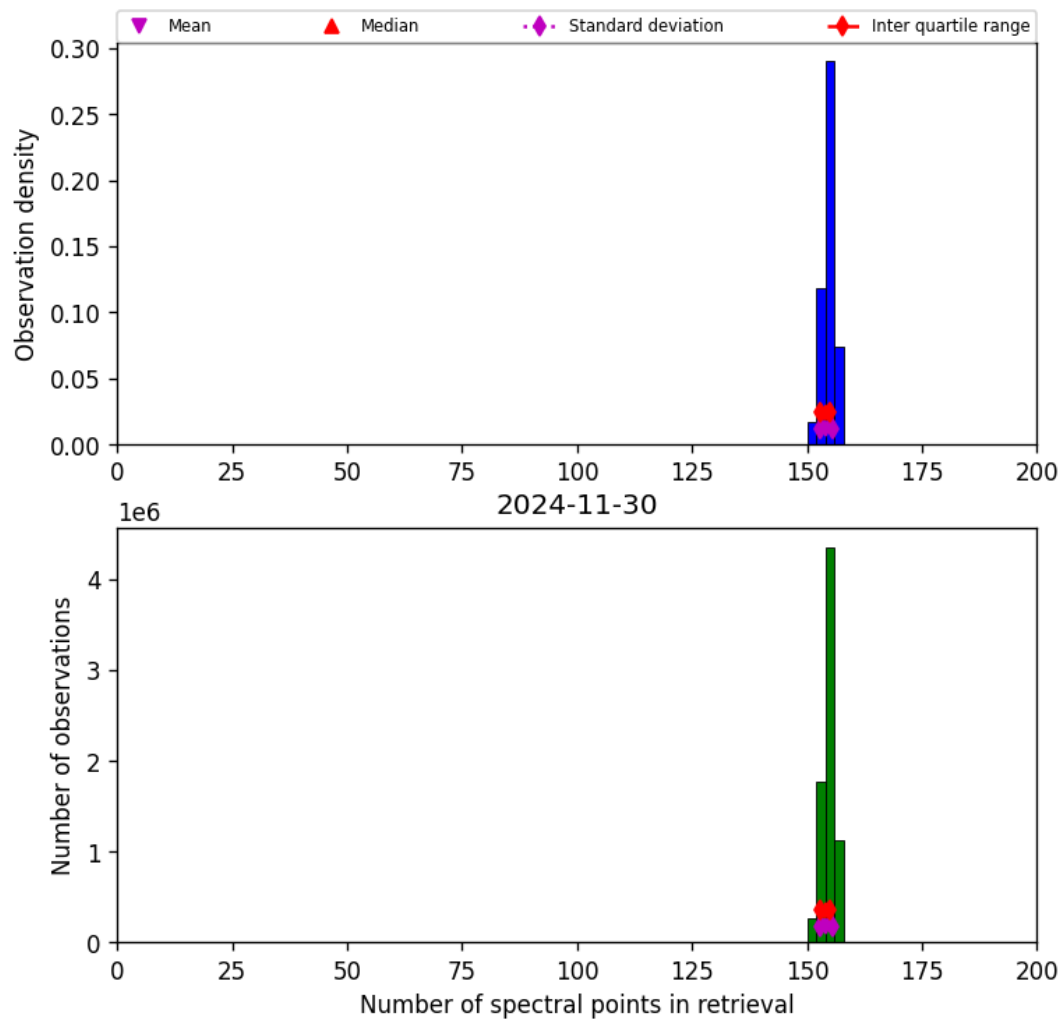
Figure 21: Histogram of “Number of spectral points in retrieval” for 2024-11-30 to 2024-12-01
