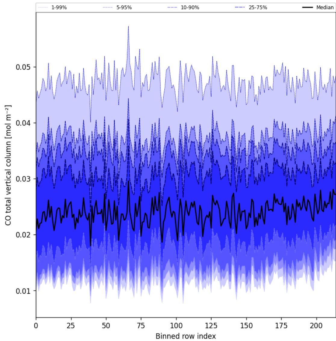
Figure 26: Along track statistics of “CO total vertical column” for 2024-11-30 to 2024-12-01
