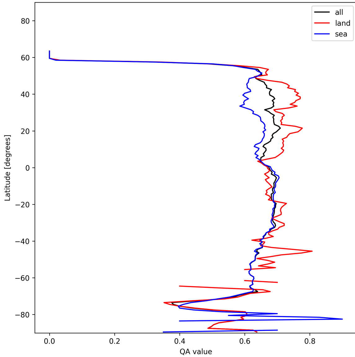
Figure 9: Zonal average of “QA value” for 2024-11-30 to 2024-12-01.
