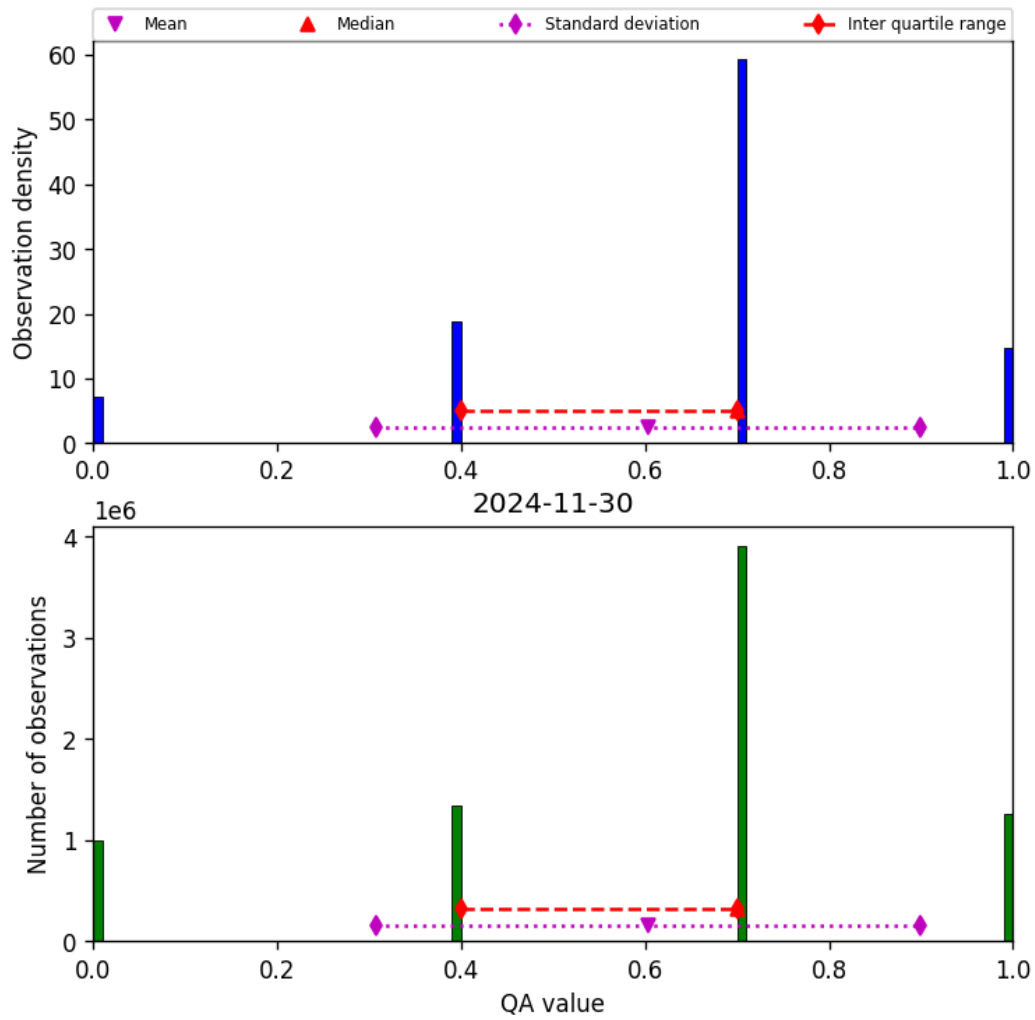
Figure 17: Histogram of “QA value” for 2024-11-30 to 2024-12-01
