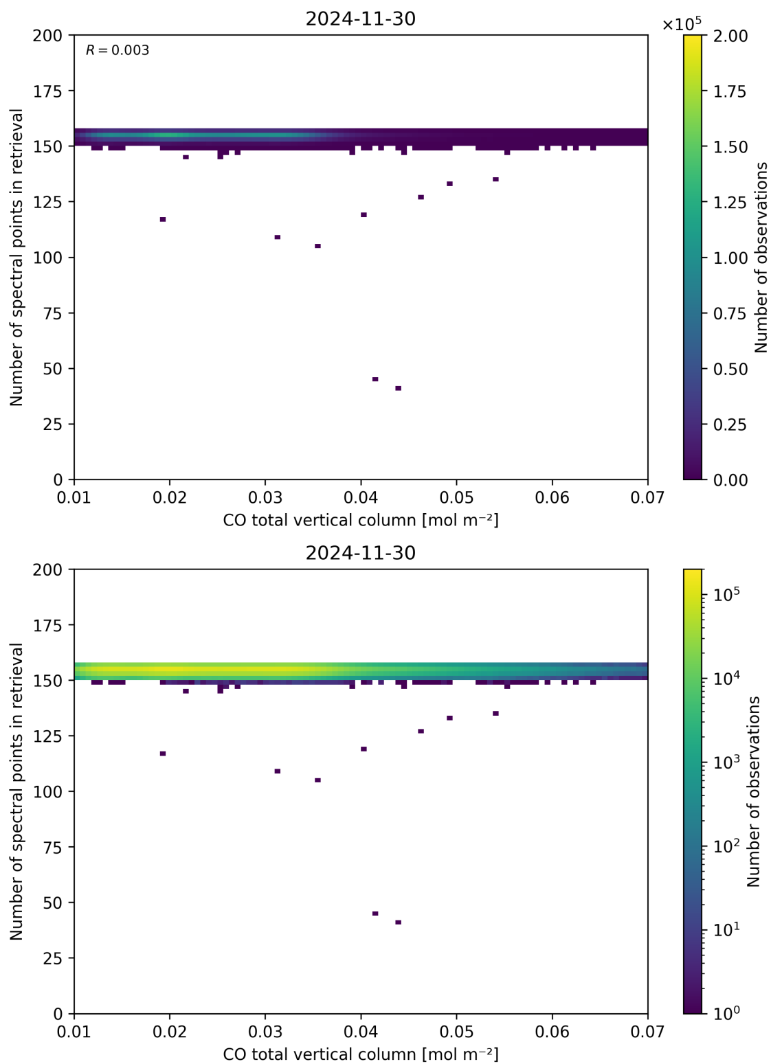
Figure 43: Scatter density plot of “CO total vertical column” against “Number of spectral points in retrieval” for 2024-11-30 to 2024-12-01.
