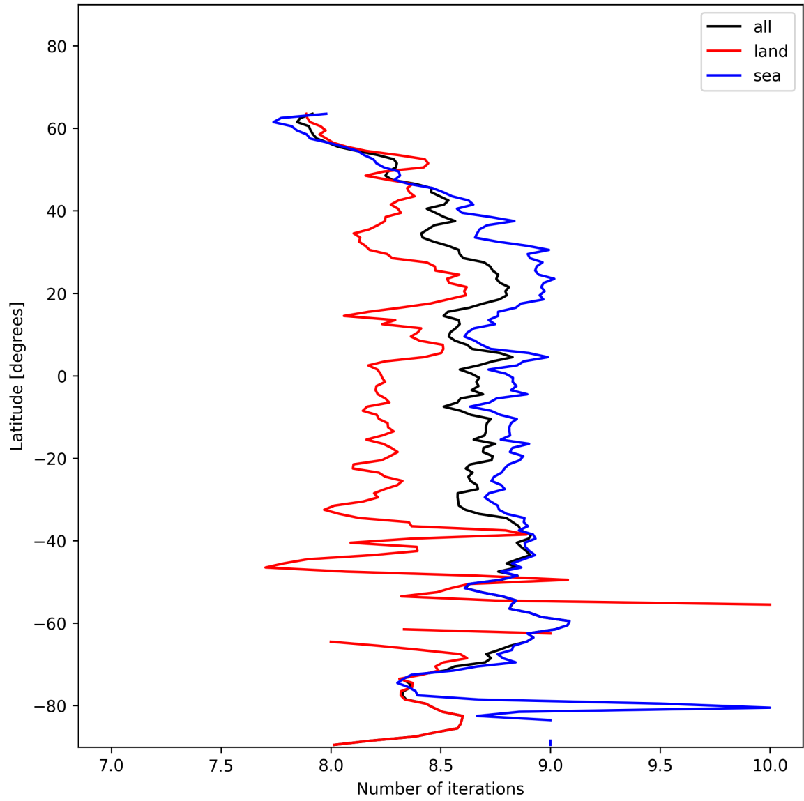
Figure 16: Zonal average of “Number of iterations” for 2024-11-30 to 2024-12-01.
