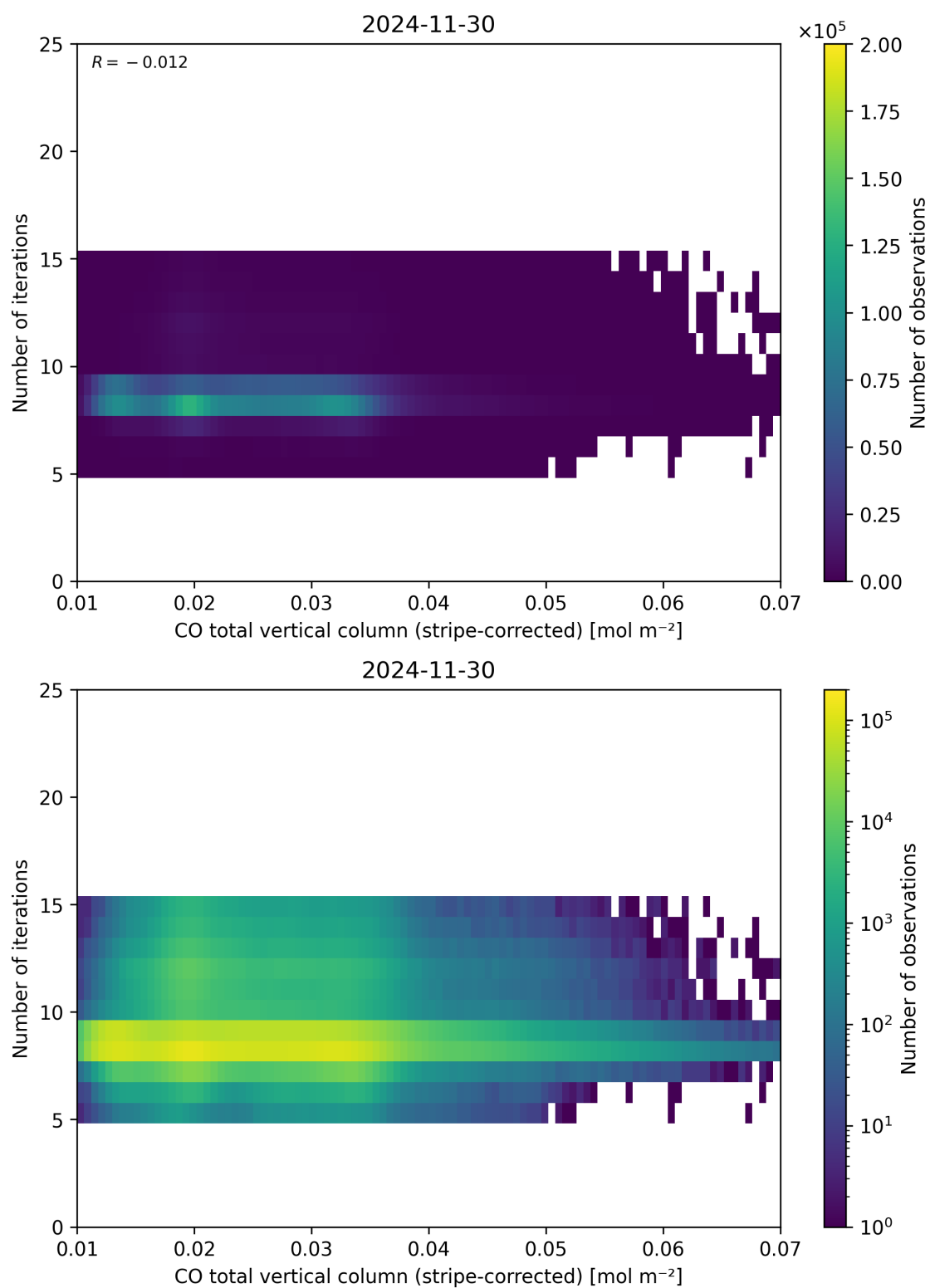
Figure 39: Scatter density plot of “CO total vertical column (stripe-corrected)” against “Number of iterations” for 2024-11-30 to 2024-12-01.
