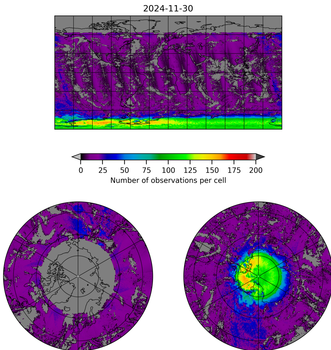
Figure 8: Map of the number of observations for 2024-11-30 to 2024-12-01
