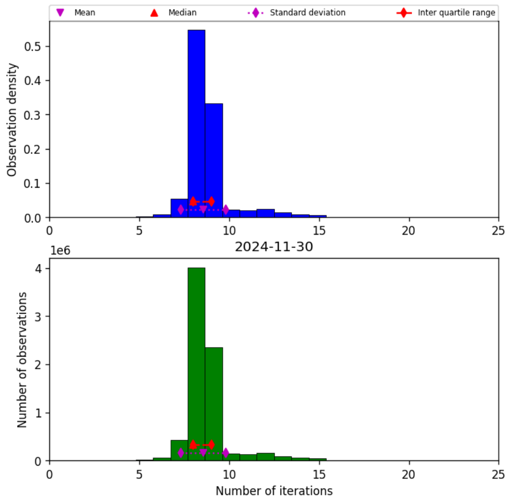
Figure 24: Histogram of “Number of iterations” for 2024-11-30 to 2024-12-01
