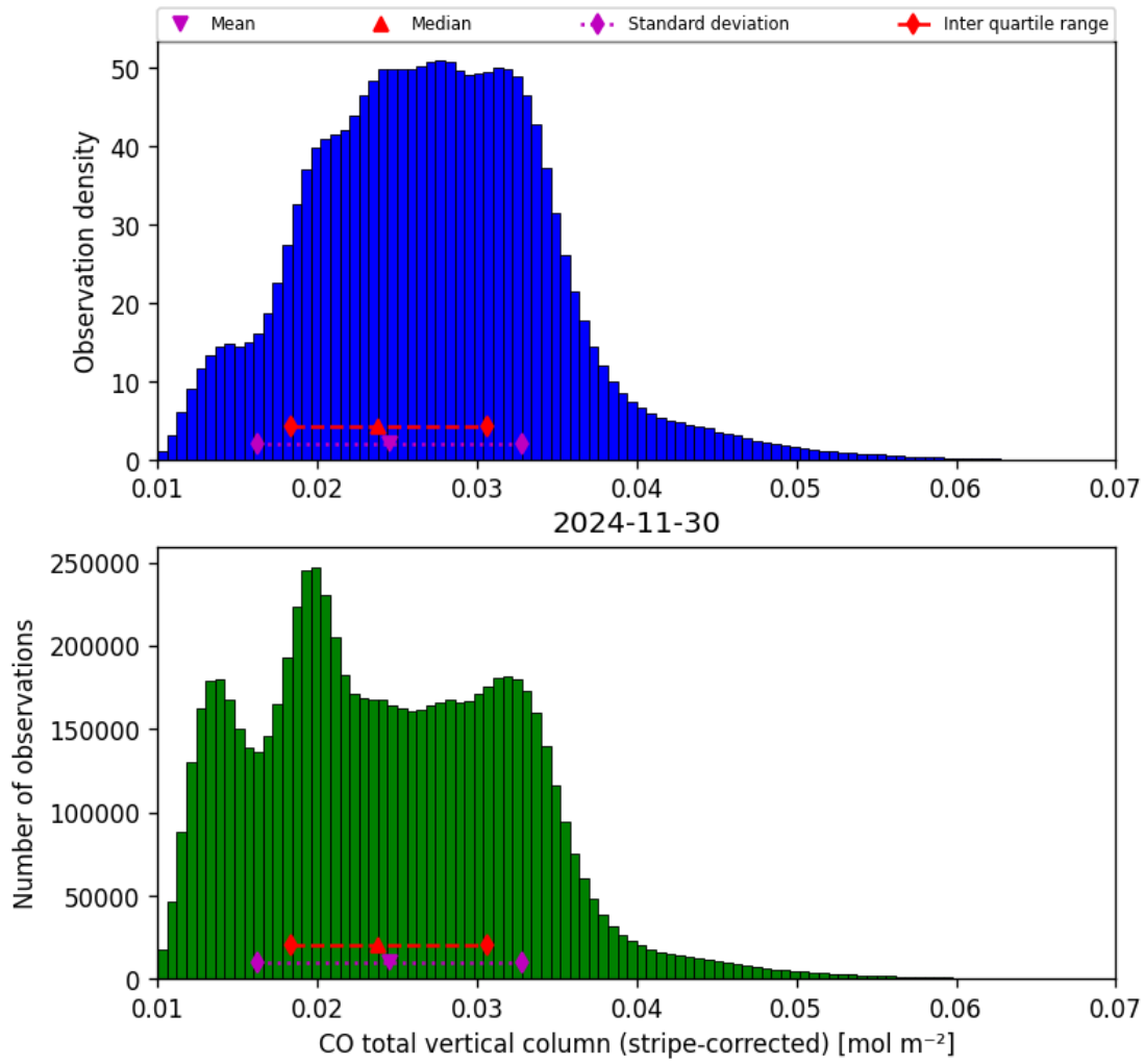
Figure 19: Histogram of “CO total vertical column (stripe-corrected)” for 2024-11-30 to 2024-12-01
