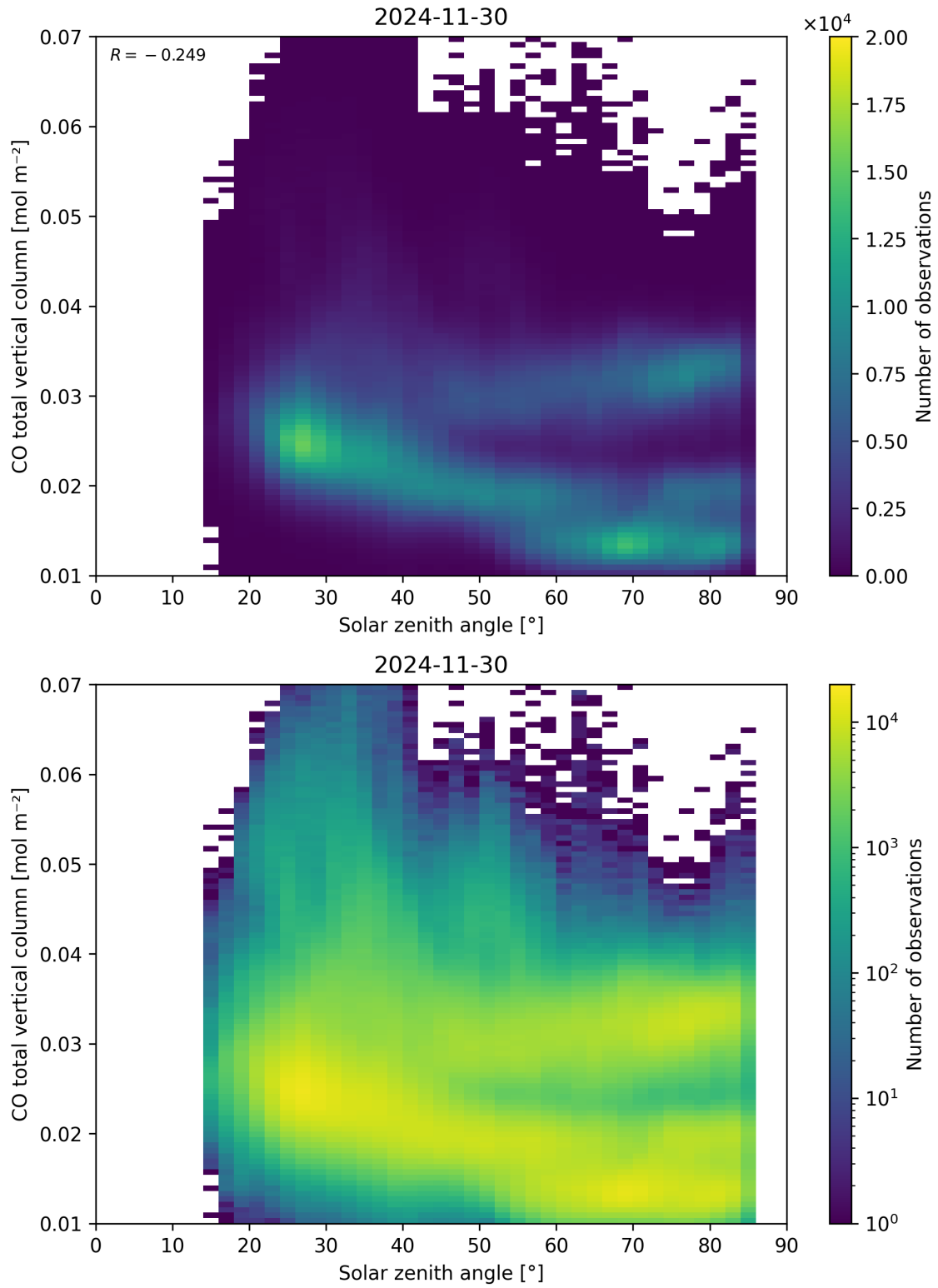
Figure 61: Scatter density plot of “Solar zenith angle” against “CO total vertical column” for 2024-11-30 to 2024-12-01.
