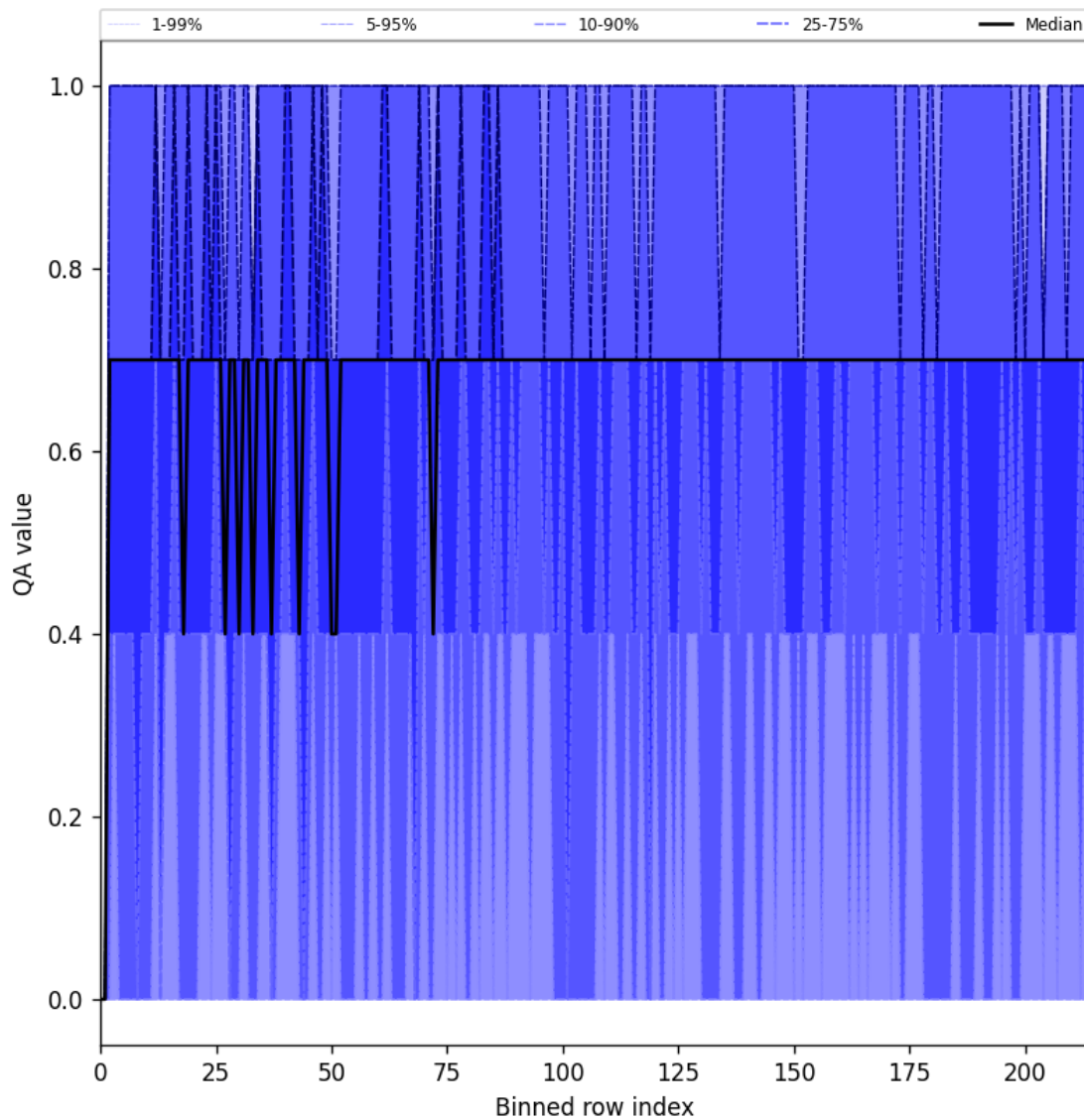
Figure 25: Along track statistics of “QA value” for 2024-11-30 to 2024-12-01
