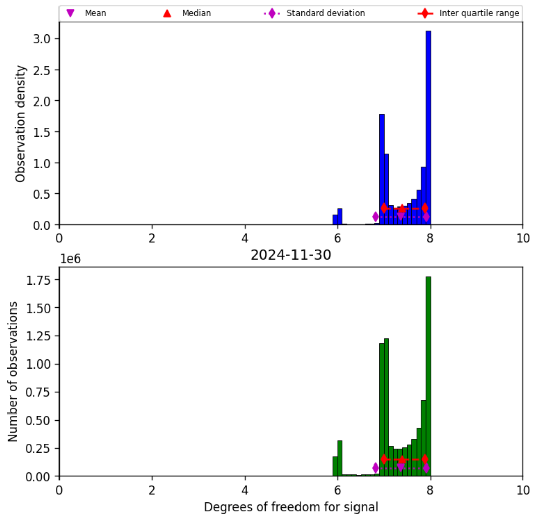
Figure 23: Histogram of “Degrees of freedom for signal” for 2024-11-30 to 2024-12-01
