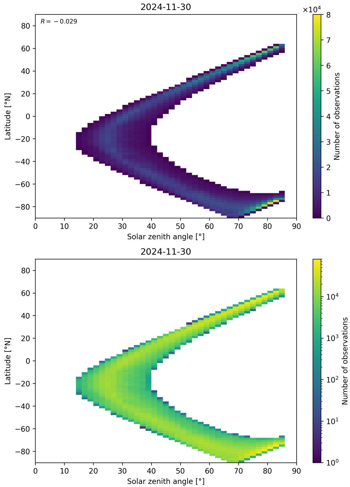
Figure 66: Scatter density plot of “Solar zenith angle” against “Latitude” for 2024-11-30 to 2024-12-01.
