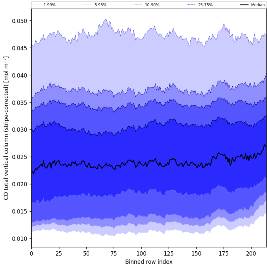
Figure 27: Along track statistics of “CO total vertical column (stripe-corrected)” for 2024-11-30 to 2024-12-01
