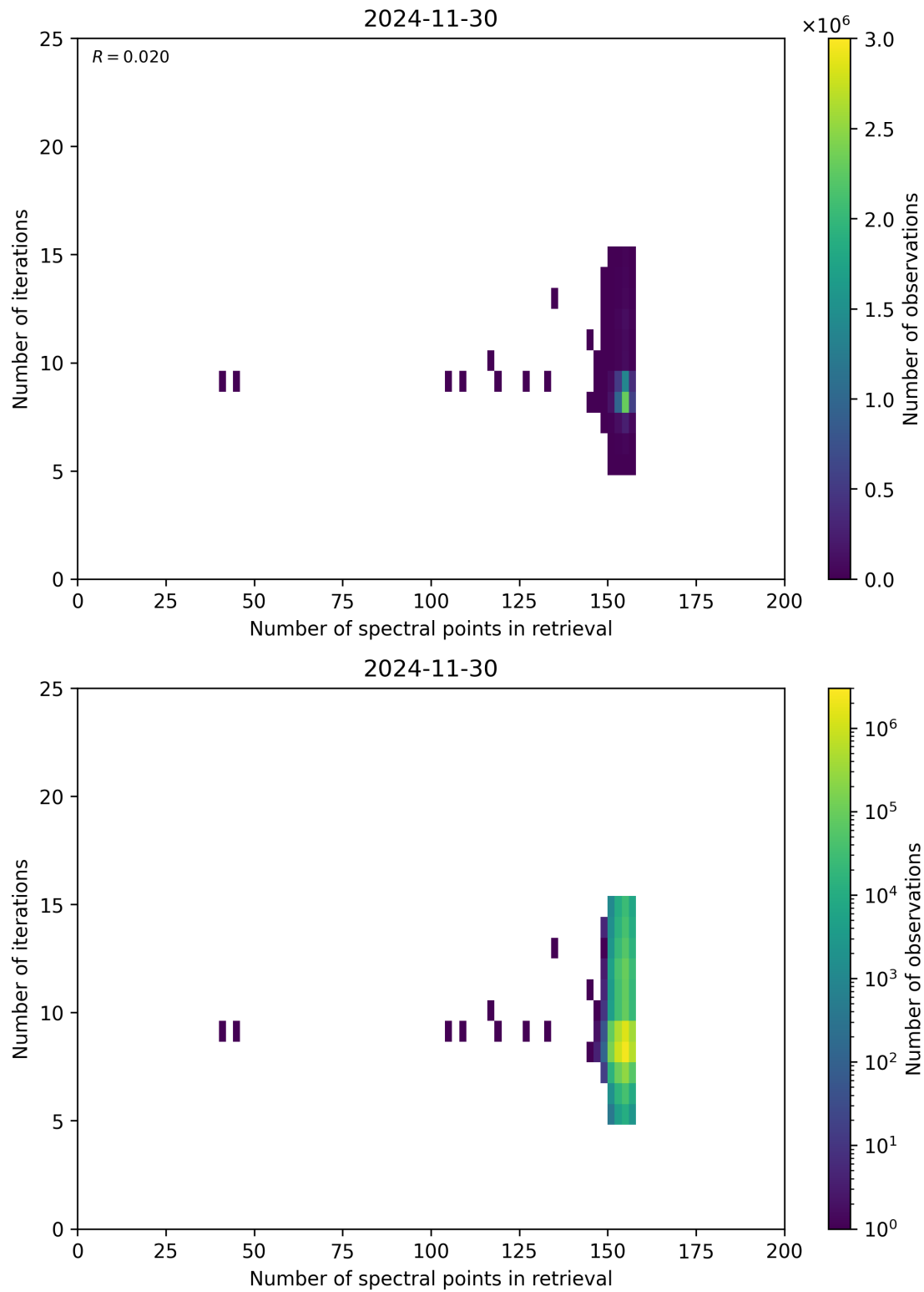
Figure 60: Scatter density plot of “Number of spectral points in retrieval” against “Number of iterations” for 2024-11-30 to 2024-12-01.
