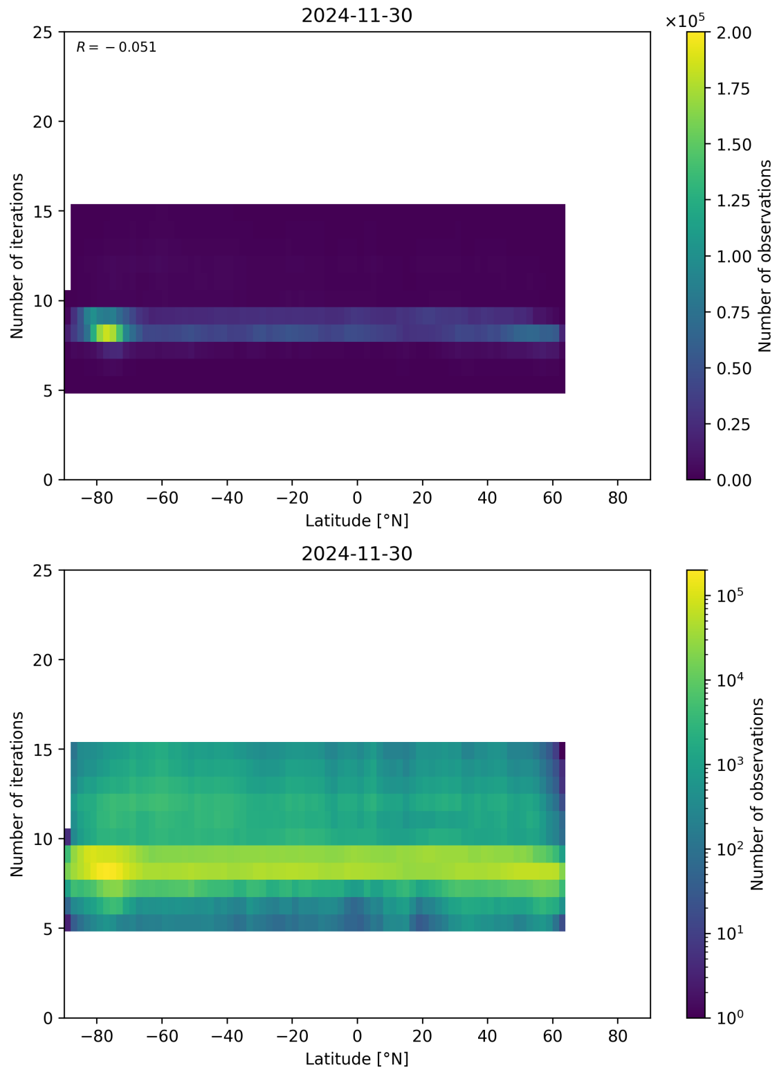
Figure 56: Scatter density plot of “Latitude” against “Number of iterations” for 2024-11-30 to 2024-12-01.
