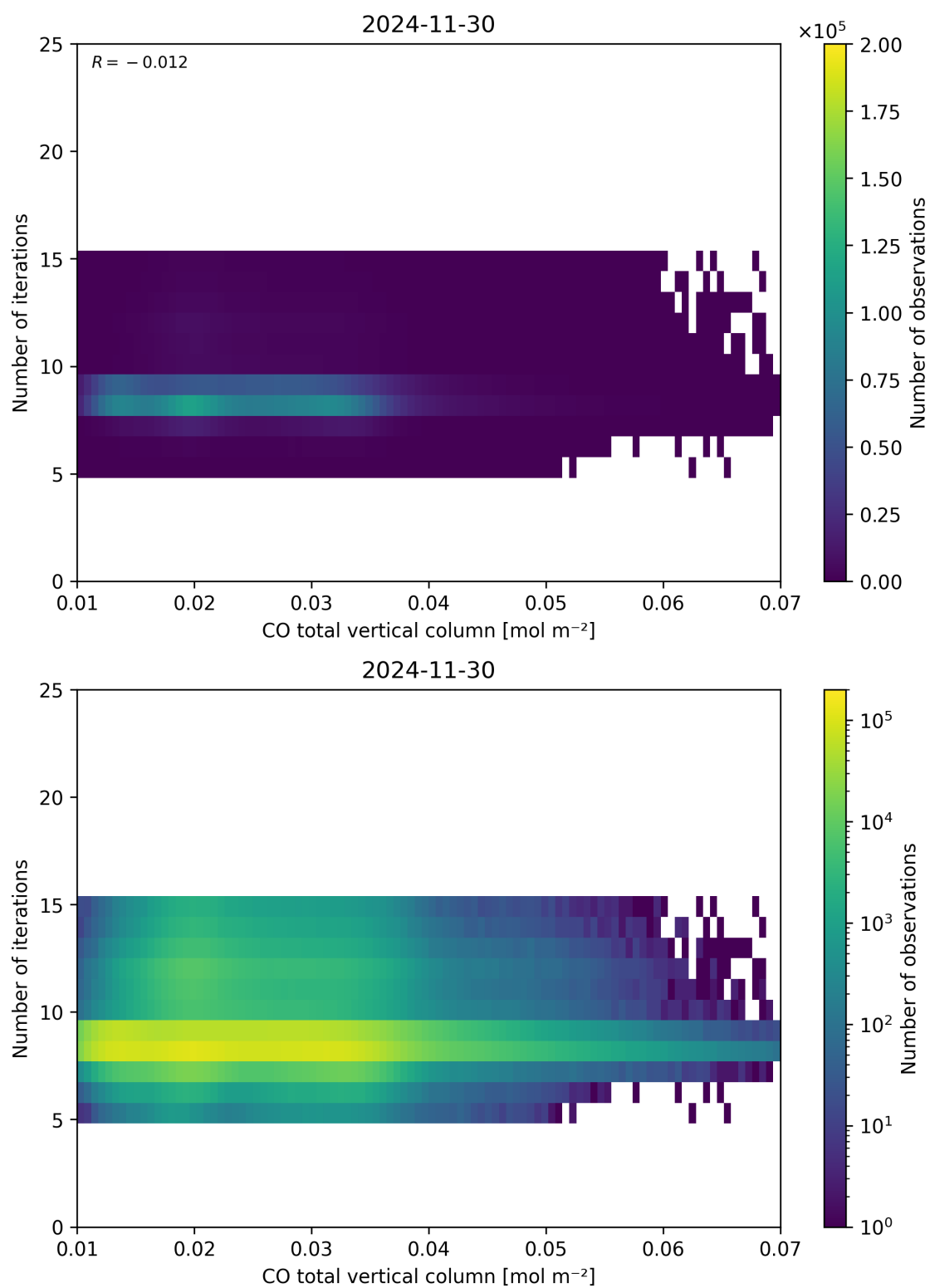
Figure 42: Scatter density plot of “CO total vertical column” against “Number of iterations” for 2024-11-30 to 2024-12-01.
