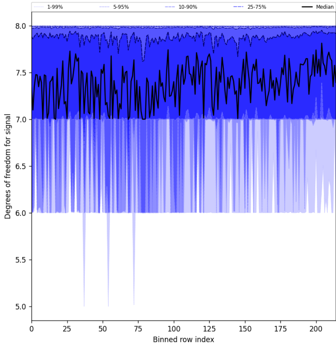
Figure 31: Along track statistics of “Degrees of freedom for signal” for 2024-11-30 to 2024-12-01
