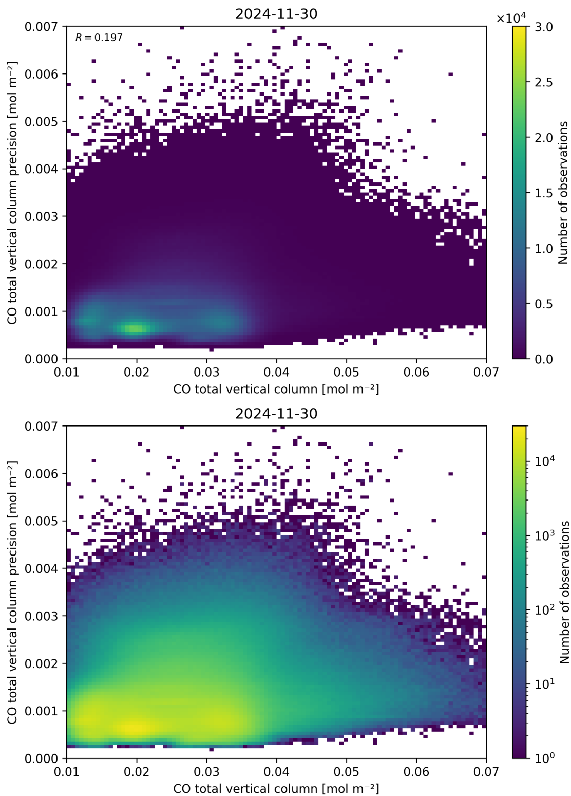
Figure 34: Scatter density plot of “CO total vertical column” against “CO total vertical column precision” for 2024-11-30 to 2024-12-01.
