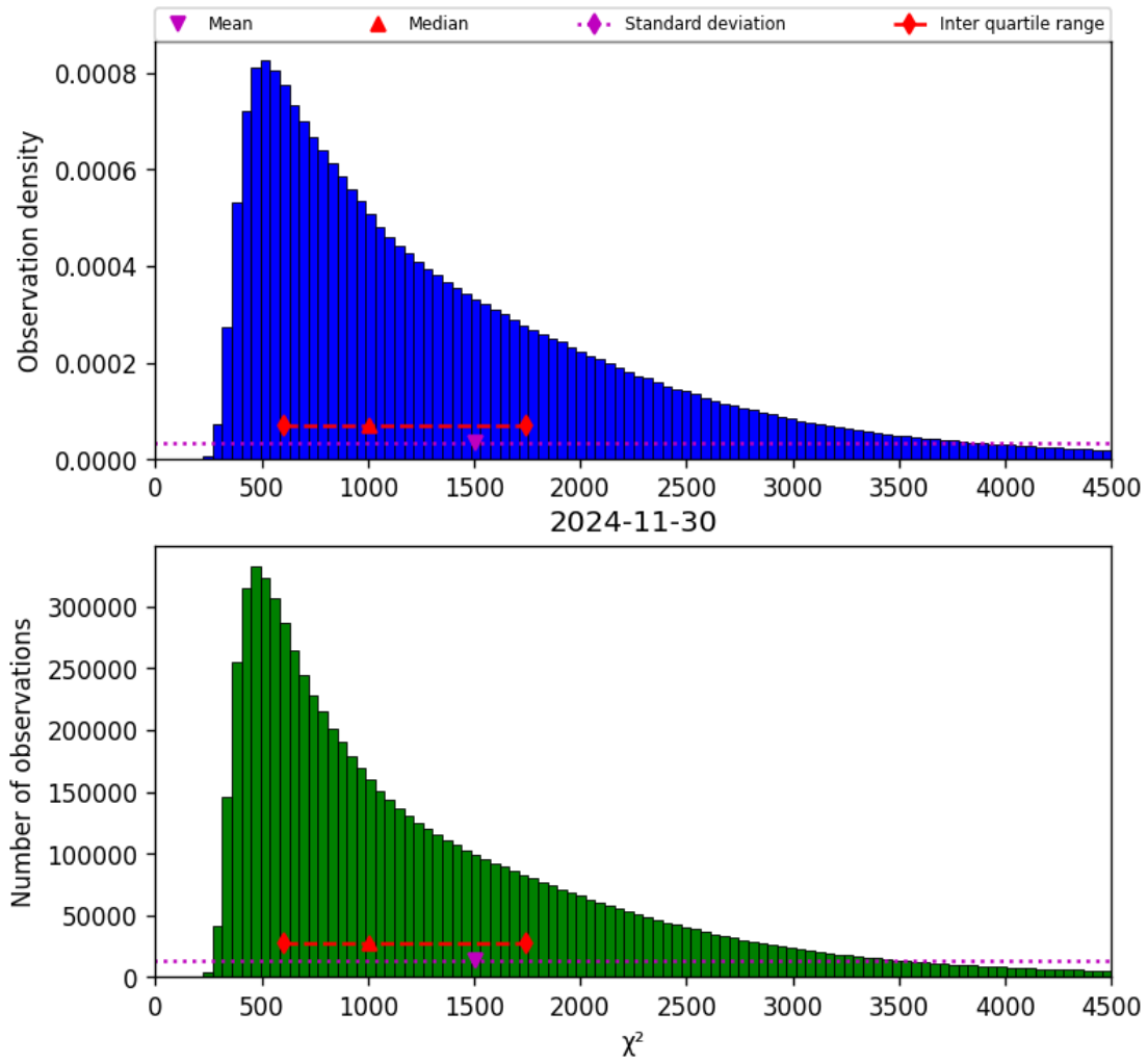
Figure 22: Histogram of " \chi^2 " for 2024-11-30 to 2024-12-01
