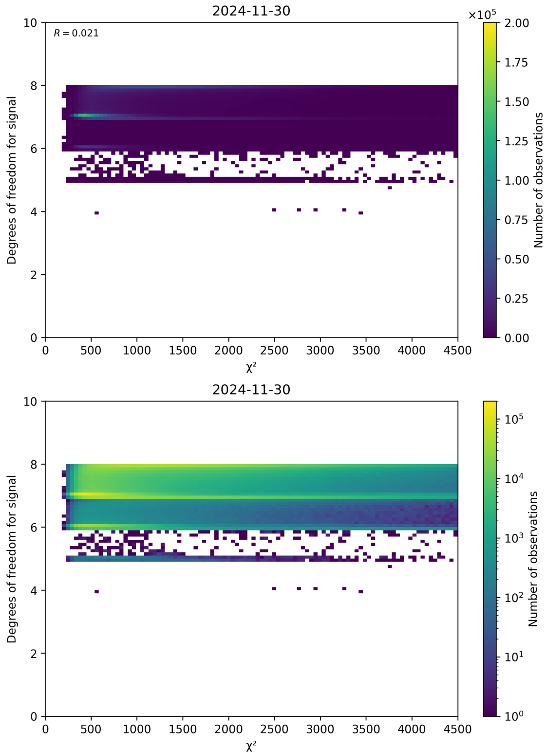
Figure 48: Scatter density plot of “ \chi^2 ” against “Degrees of freedom for signal” for 2024-11-30 to 2024-12-01.
