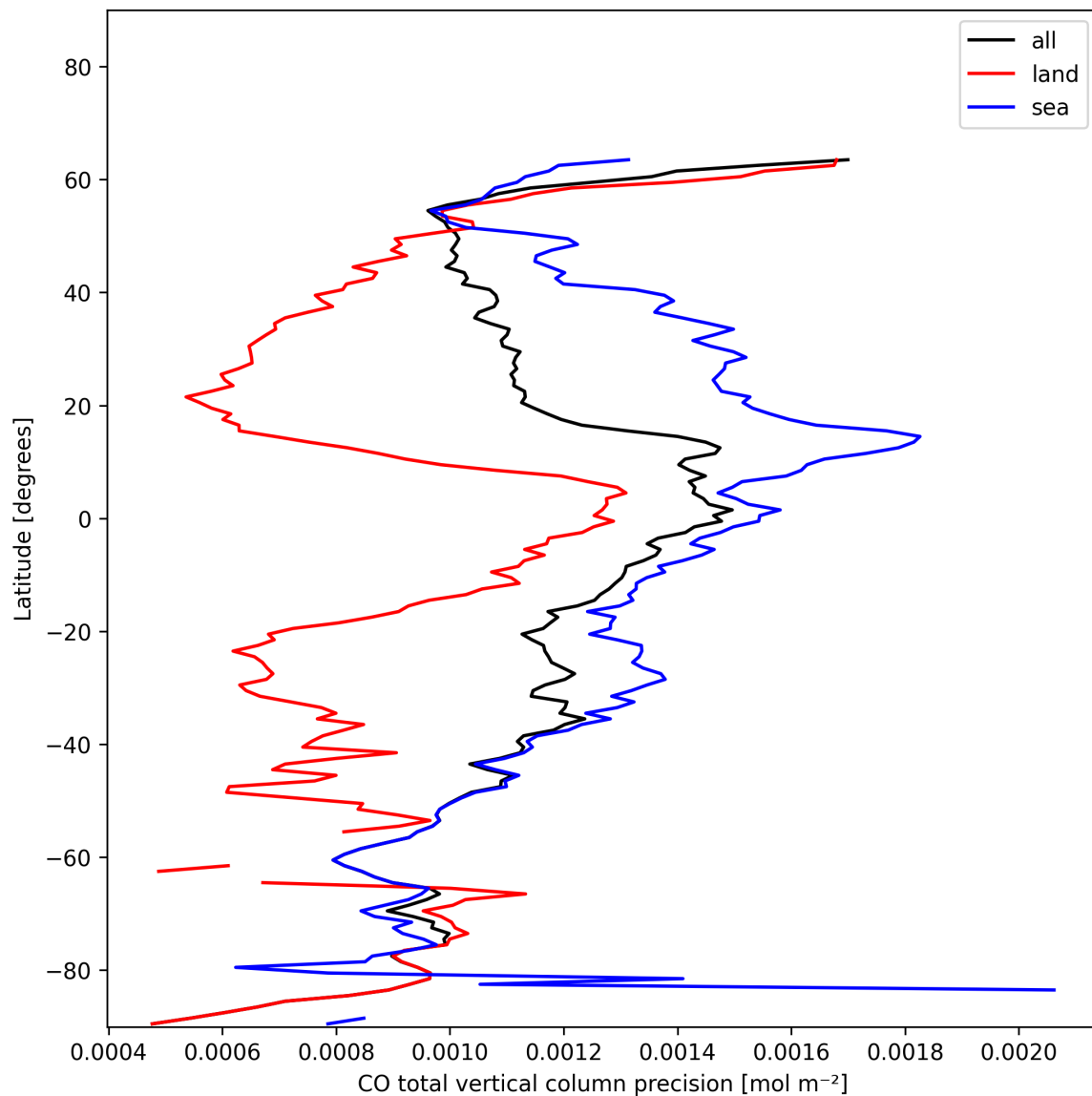
Figure 12: Zonal average of “CO total vertical column precision” for 2024-11-30 to 2024-12-01.
