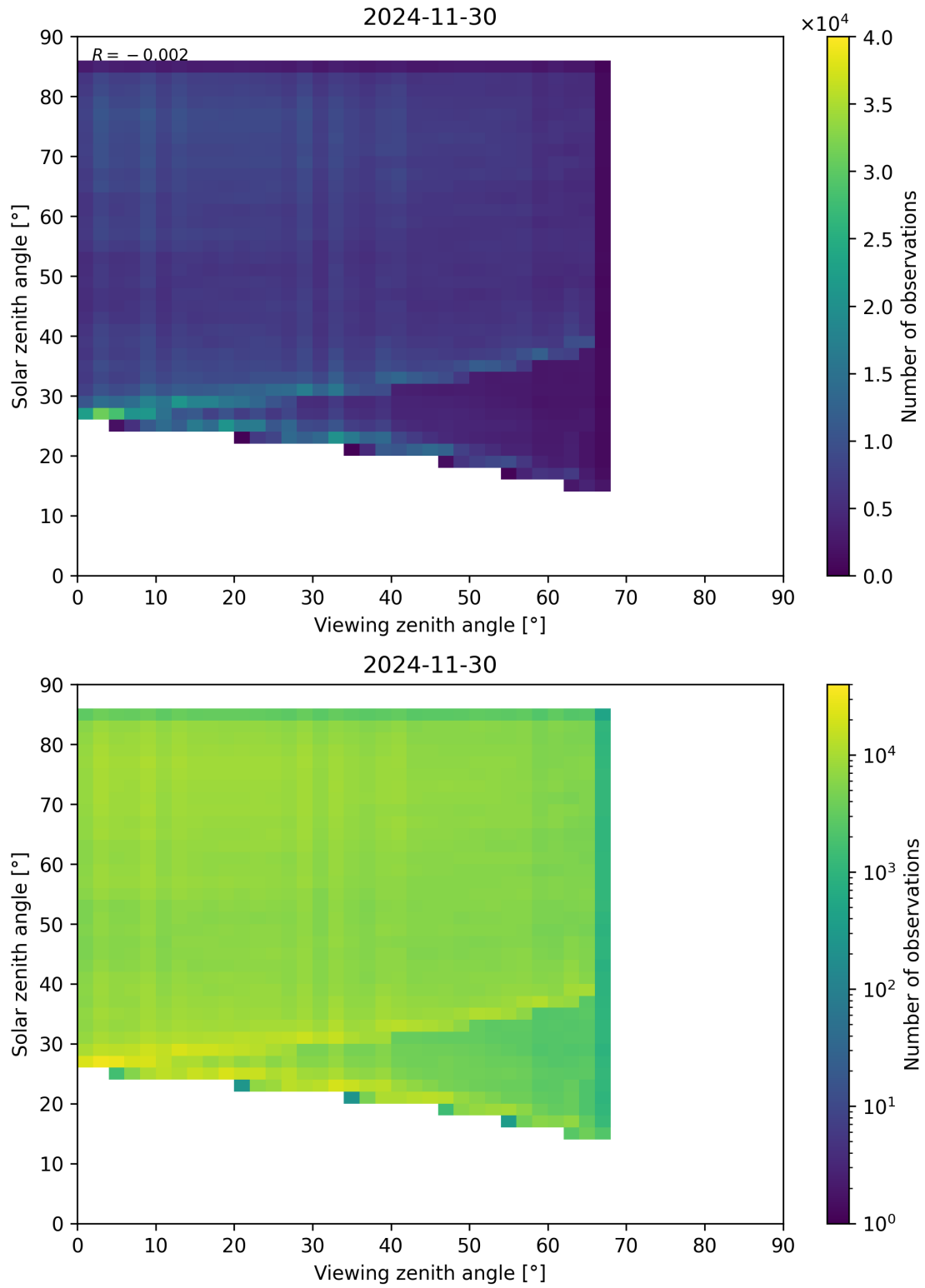
Figure 77: Scatter density plot of “Viewing zenith angle” against “Solar zenith angle” for 2024-11-30 to 2024-12-01.
