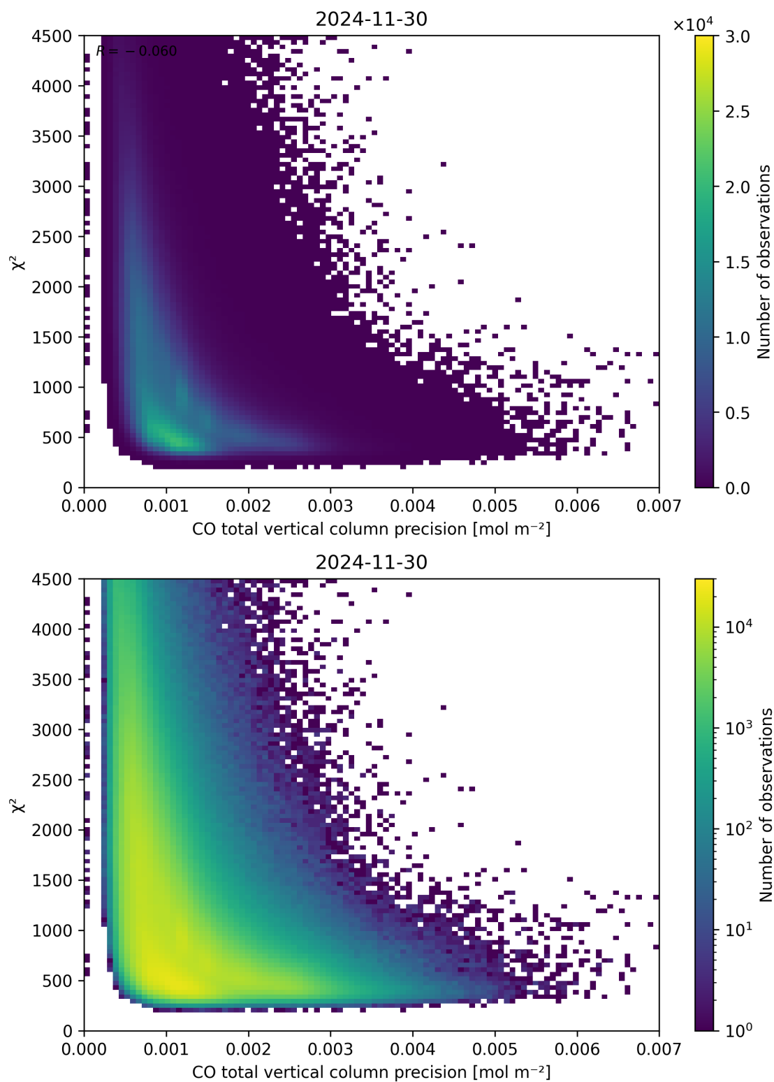
Figure 44: Scatter density plot of “CO total vertical column precision” against “ \chi^2 ” for 2024-11-30 to 2024-12-01.
