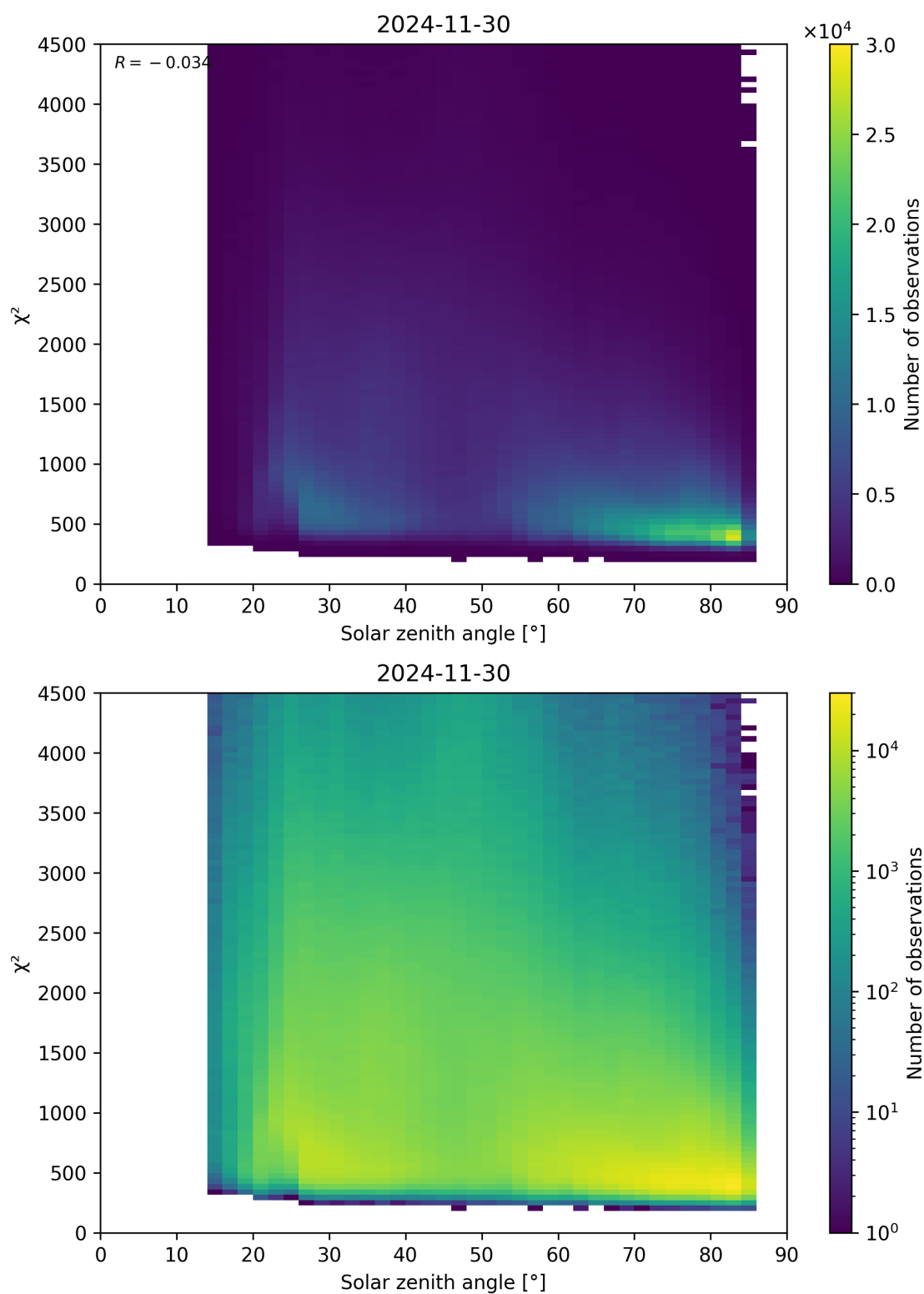
Figure 64: Scatter density plot of “Solar zenith angle” against “ \chi^2 ” for 2024-11-30 to 2024-12-01.
