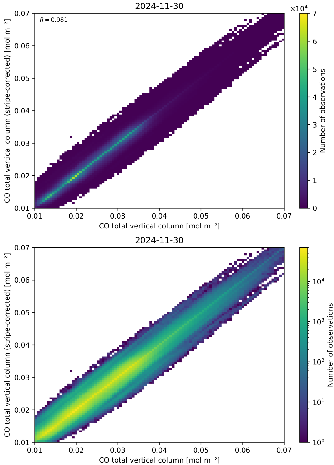
Figure 33: Scatter density plot of “CO total vertical column” against “CO total vertical column (stripe-corrected)” for 2024-11-30 to 2024-12-01.
