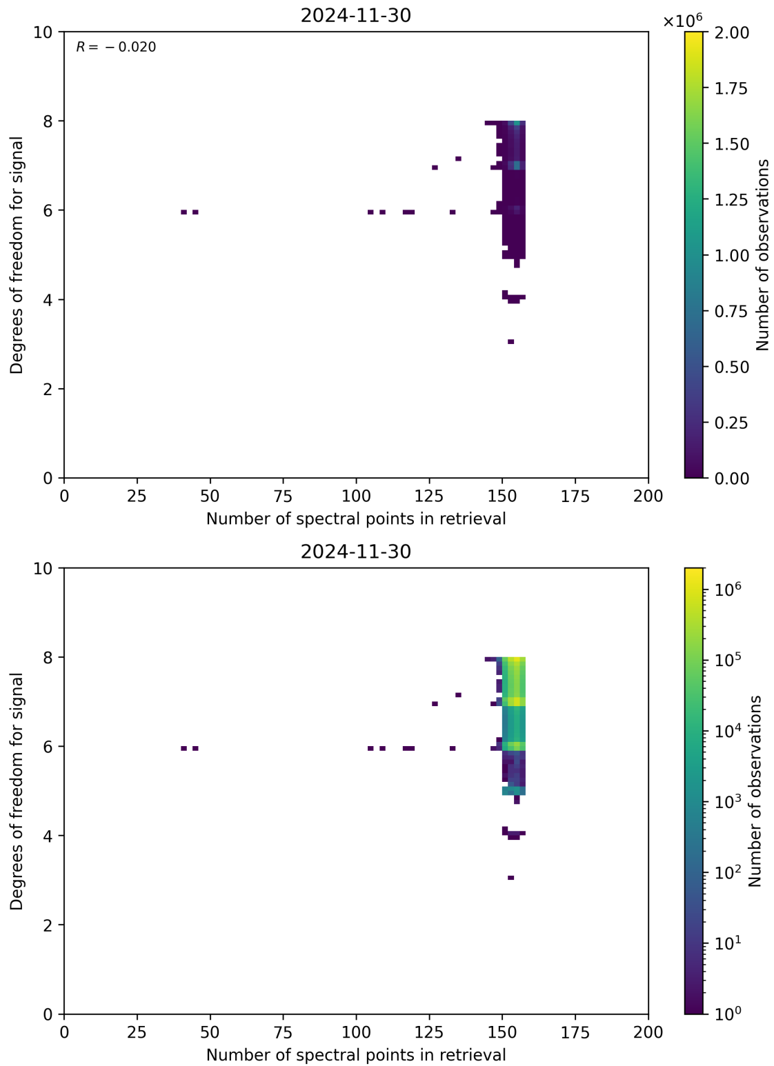
Figure 59: Scatter density plot of “Number of spectral points in retrieval” against “Degrees of freedom for signal” for 2024-11-30 to 2024-12-01.
