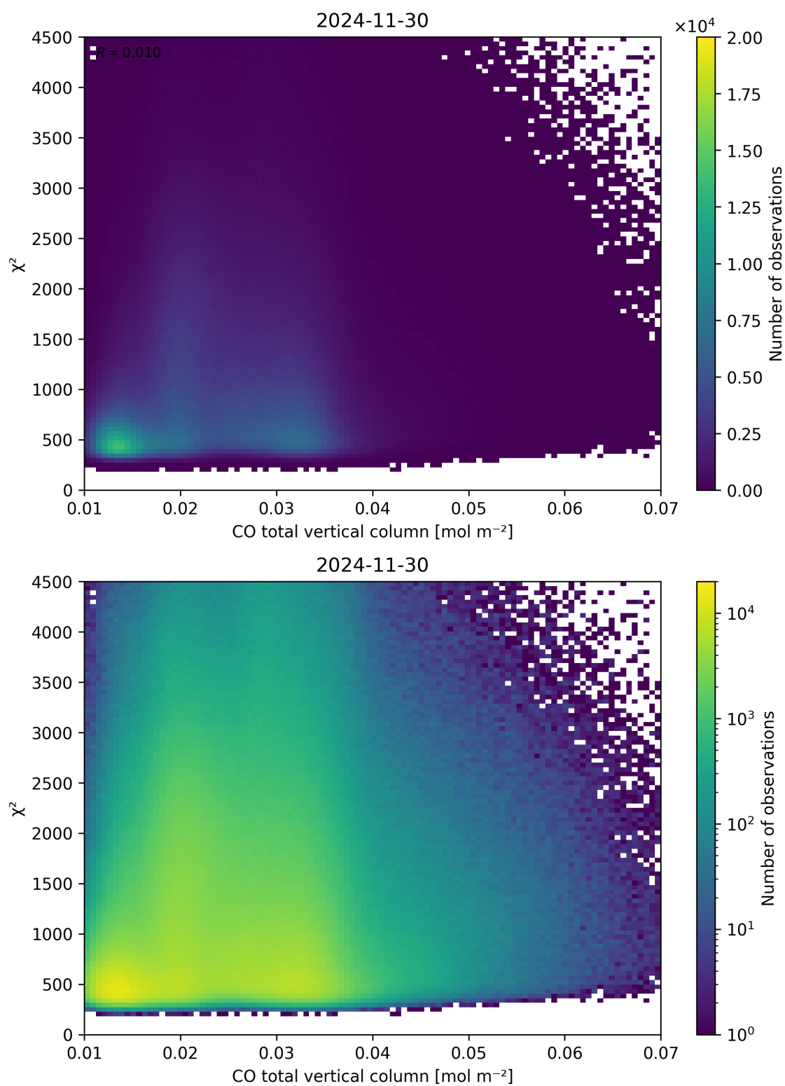
Figure 35: Scatter density plot of “CO total vertical column” against “ \chi^2 ” for 2024-11-30 to 2024-12-01.
