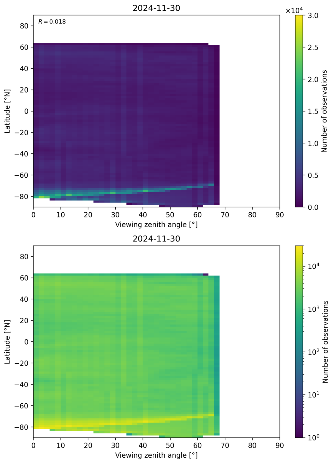
Figure 74: Scatter density plot of “Viewing zenith angle” against “Latitude” for 2024-11-30 to 2024-12-01.
