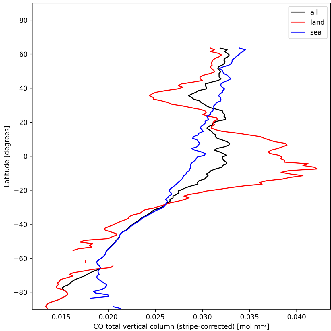
Figure 11: Zonal average of “CO total vertical column (stripe-corrected)” for 2024-11-30 to 2024-12-01.
