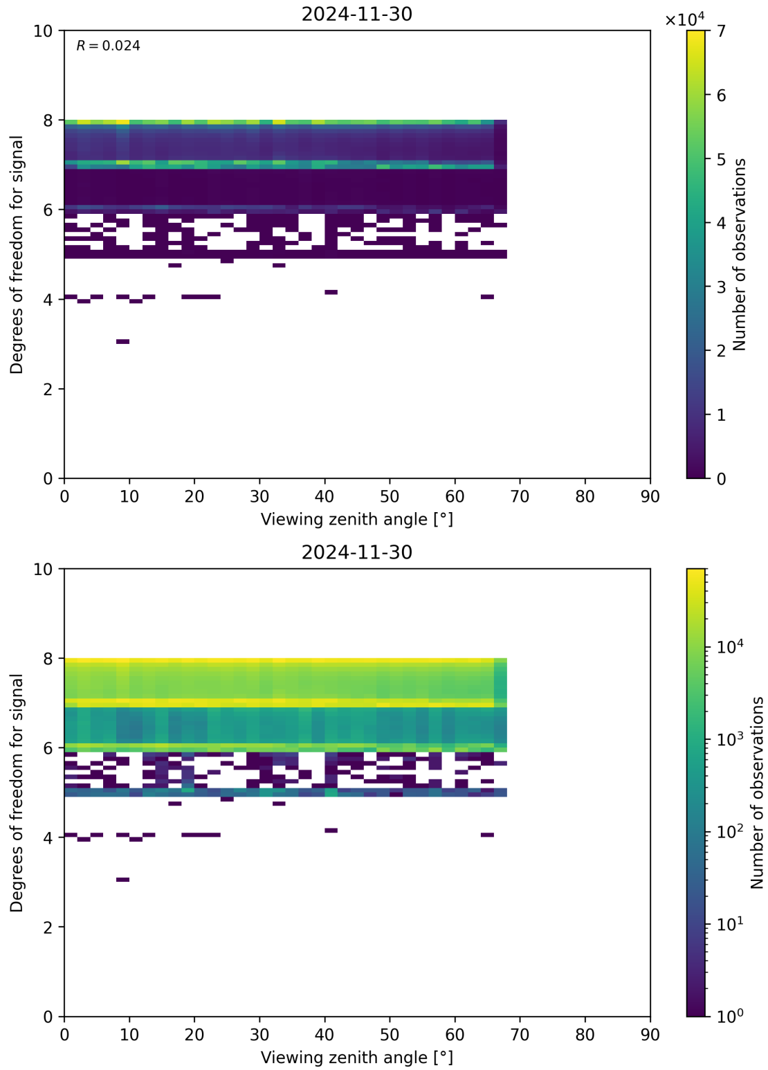
Figure 73: Scatter density plot of “Viewing zenith angle” against “Degrees of freedom for signal” for 2024-11-30 to 2024-12-01.
