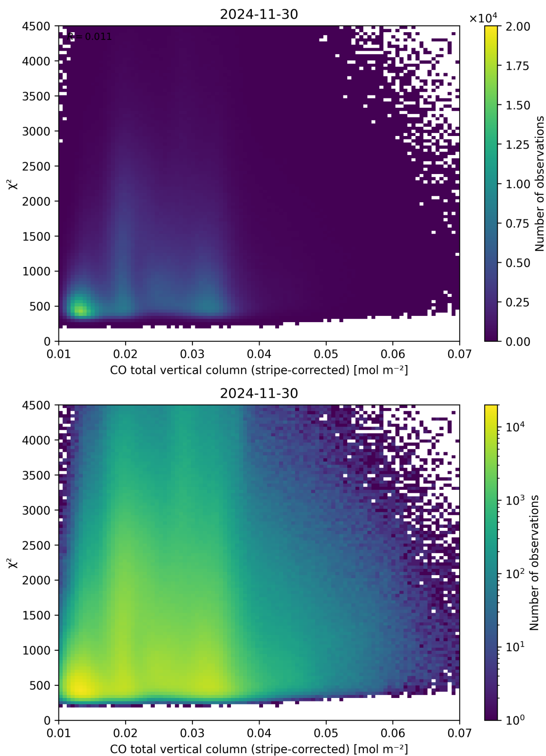
Figure 37: Scatter density plot of “CO total vertical column (stripe-corrected)” against “ \chi^2 ” for 2024-11-30 to 2024-12-01.
