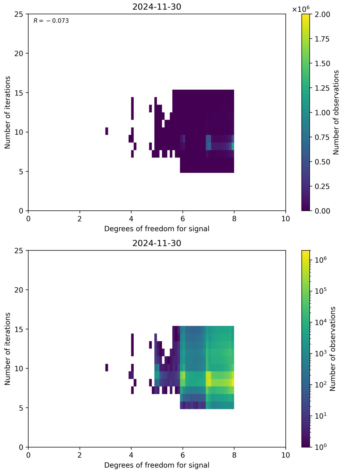
Figure 50: Scatter density plot of “Degrees of freedom for signal” against “Number of iterations” for 2024-11-30 to 2024-12-01.
