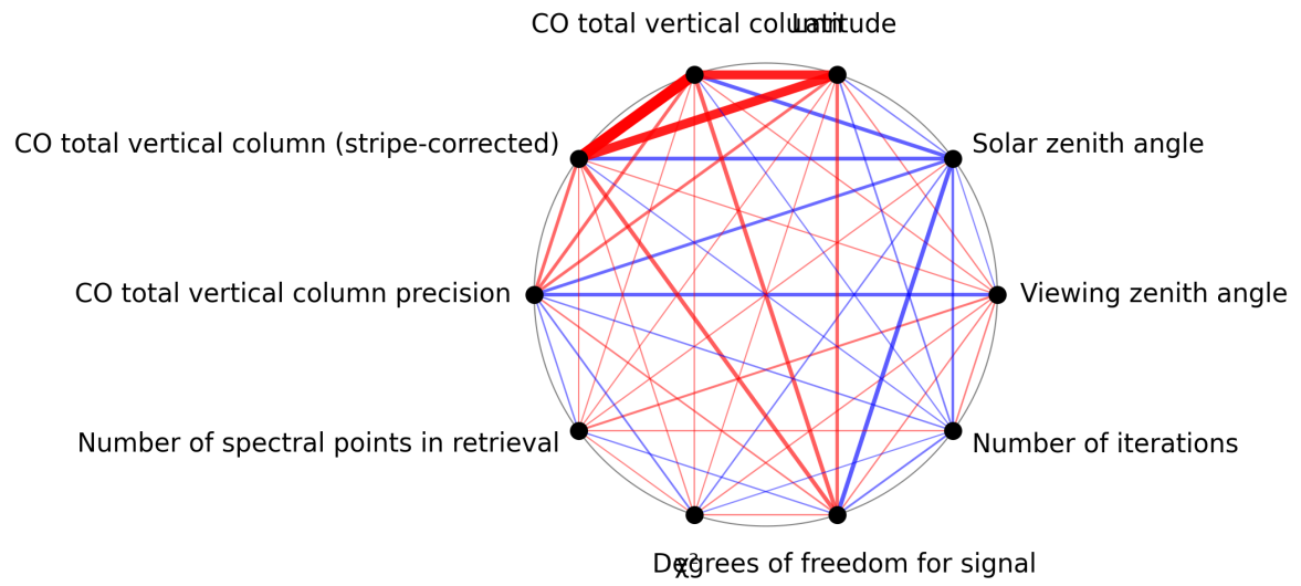
Figure 1: Map of correlation graph for 2024-11-30 to 2024-12-01.
