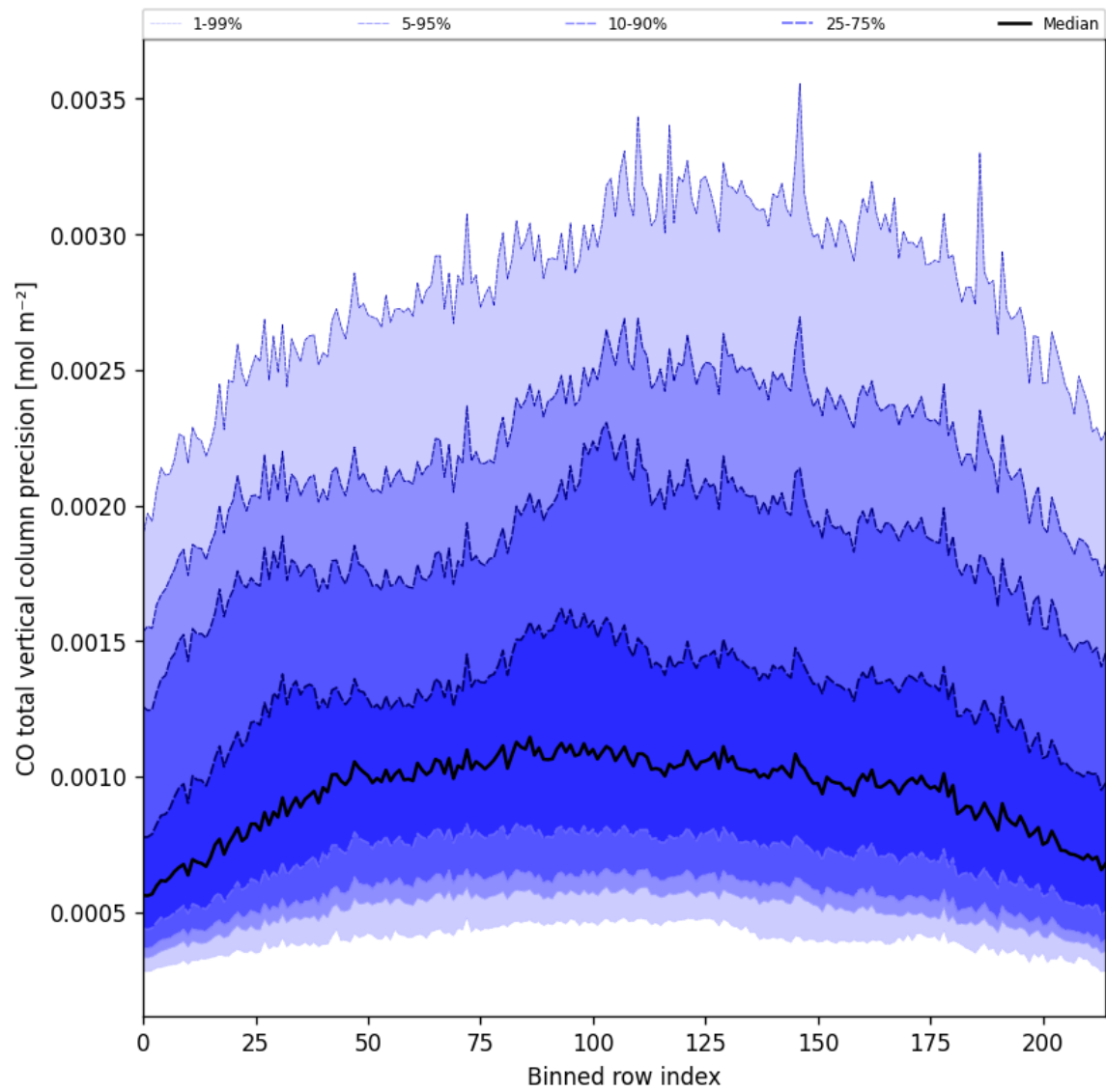
Figure 28: Along track statistics of “CO total vertical column precision” for 2024-11-30 to 2024-12-01
