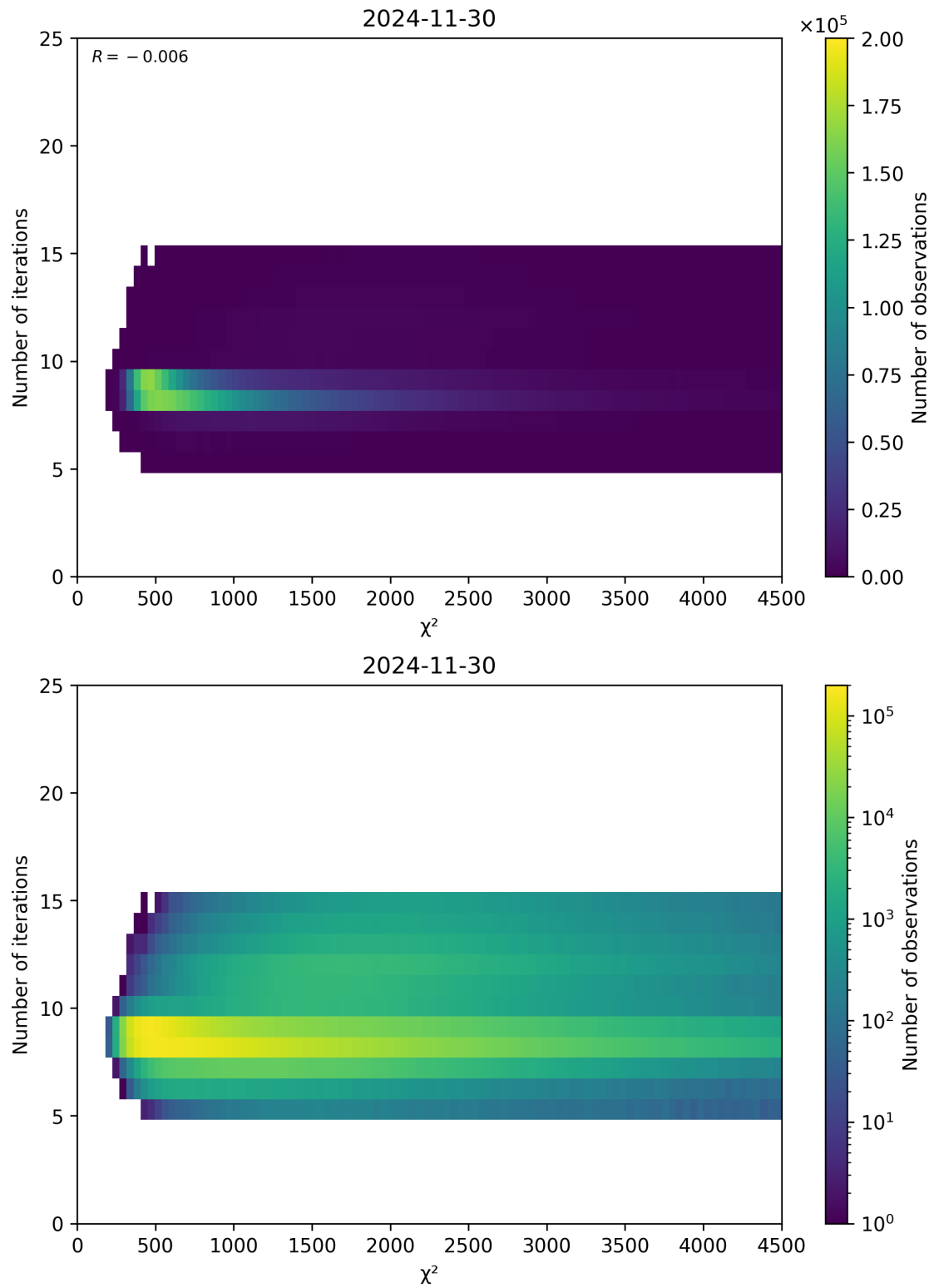
Figure 49: Scatter density plot of “ \chi^2 ” against “Number of iterations” for 2024-11-30 to 2024-12-01.
