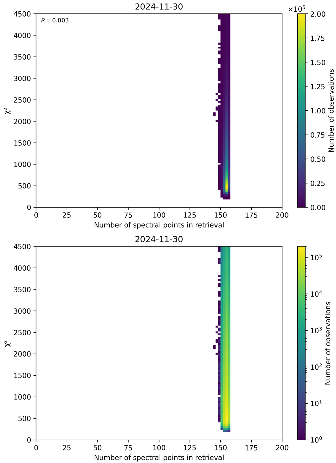
Figure 58: Scatter density plot of “Number of spectral points in retrieval” against “ \chi^2 ” for 2024-11-30 to 2024-12-01.
