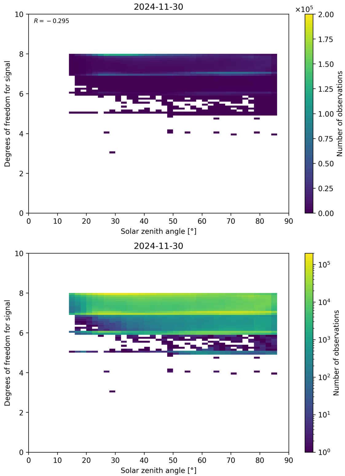
Figure 65: Scatter density plot of “Solar zenith angle” against “Degrees of freedom for signal” for 2024-11-30 to 2024-12-01.
