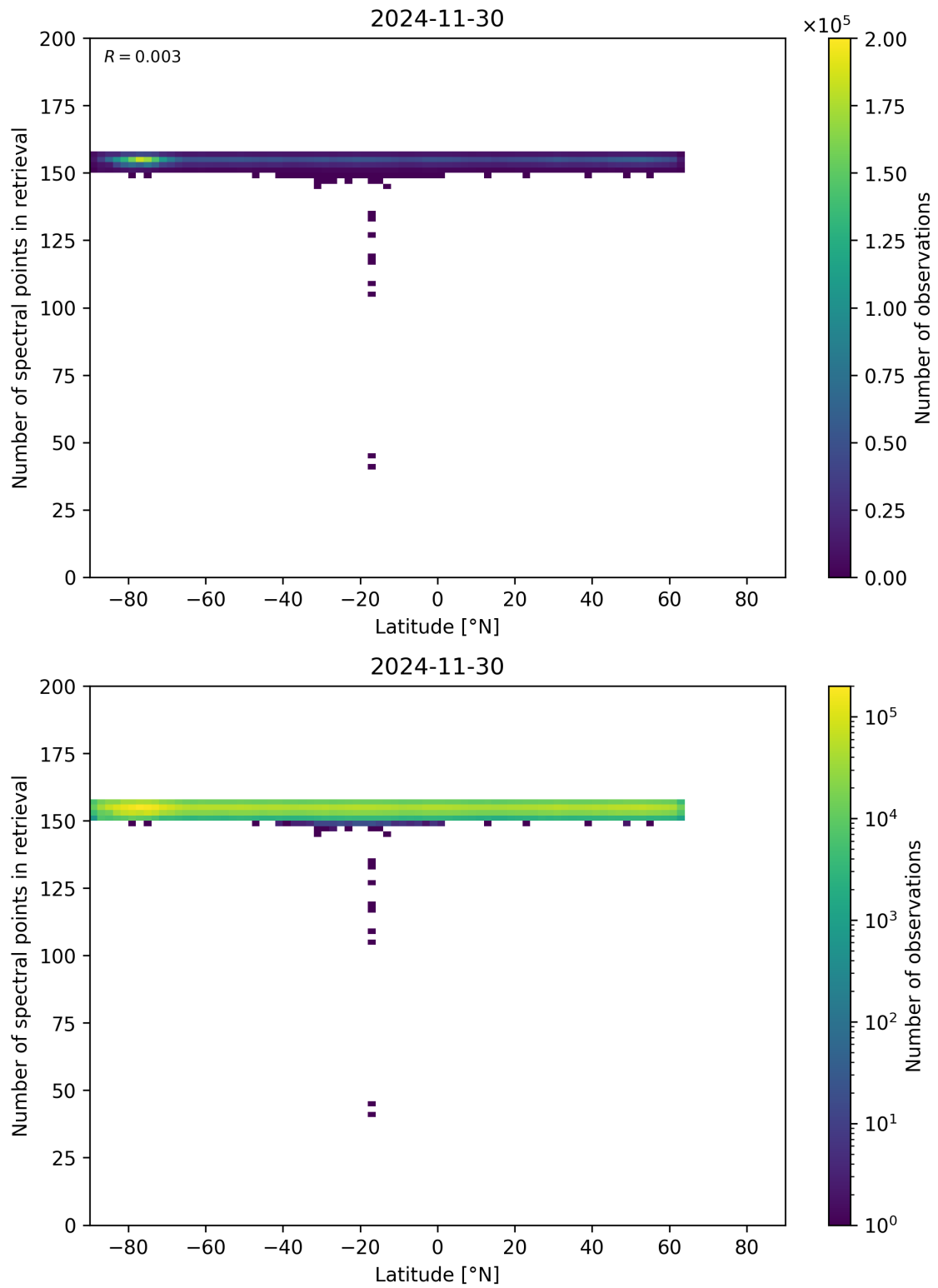
Figure 57: Scatter density plot of “Latitude” against “Number of spectral points in retrieval” for 2024-11-30 to 2024-12-01.
