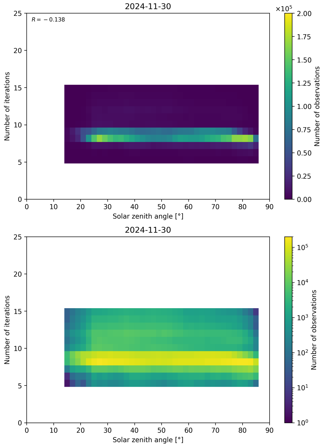
Figure 67: Scatter density plot of “Solar zenith angle” against “Number of iterations” for 2024-11-30 to 2024-12-01.
