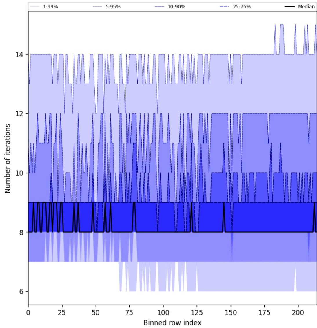
Figure 32: Along track statistics of “Number of iterations” for 2024-11-30 to 2024-12-01
