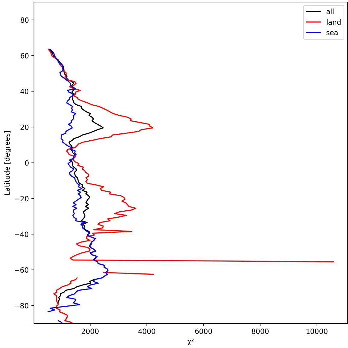
Figure 14: Zonal average of “ \chi^2 ” for 2024-11-30 to 2024-12-01.
