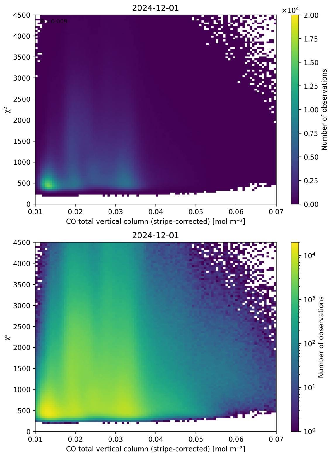
Figure 37: Scatter density plot of “CO total vertical column (stripe-corrected)” against “ \chi^2 ” for 2024-11-30 to 2024-12-02.
