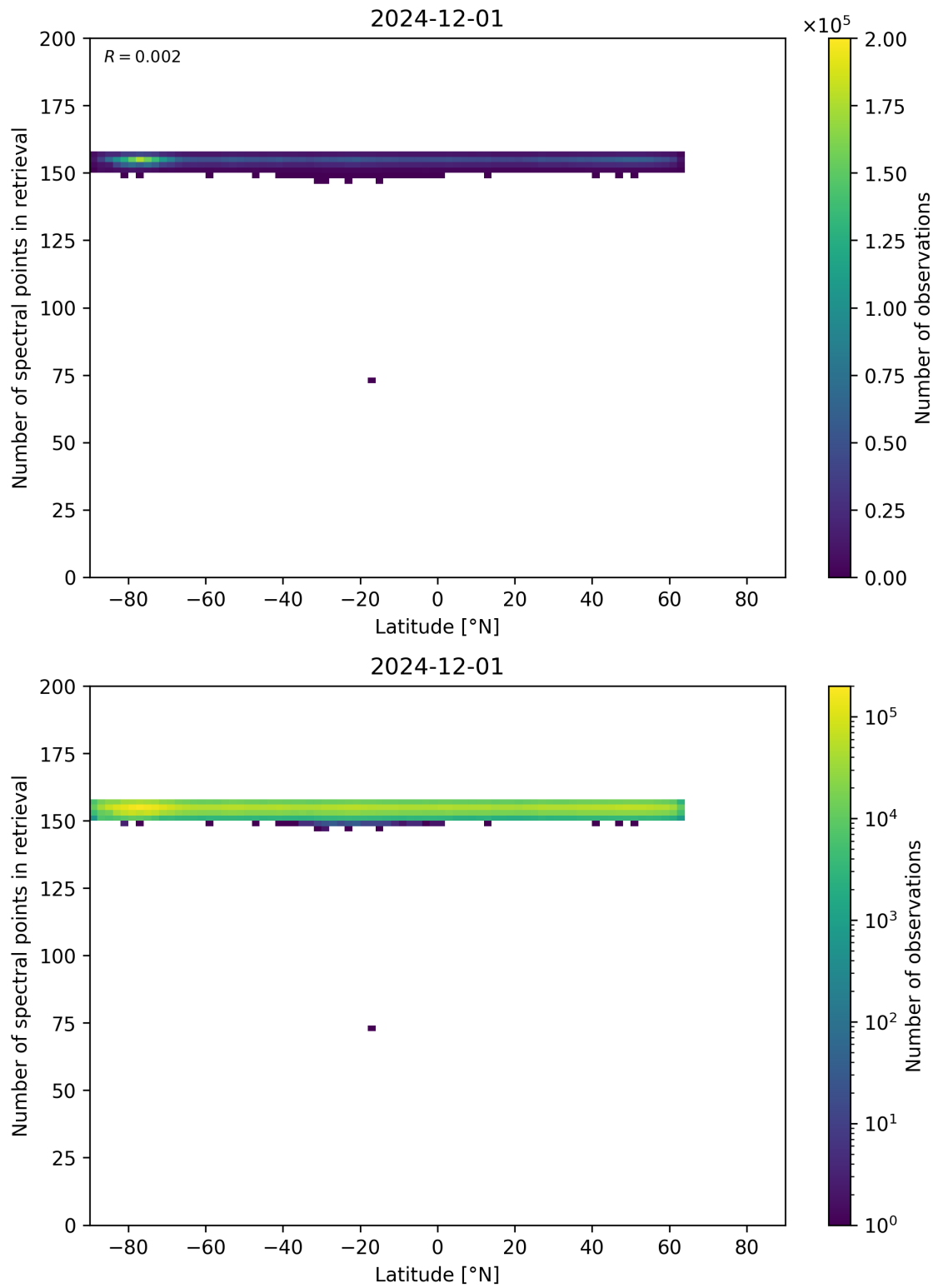
Figure 57: Scatter density plot of “Latitude” against “Number of spectral points in retrieval” for 2024-11-30 to 2024-12-02.
