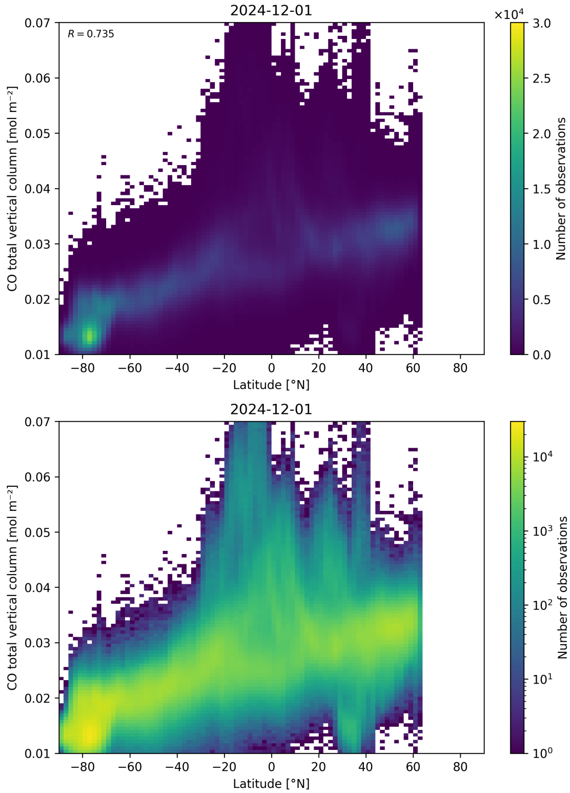
Figure 51: Scatter density plot of “Latitude” against “CO total vertical column” for 2024-11-30 to 2024-12-02.
