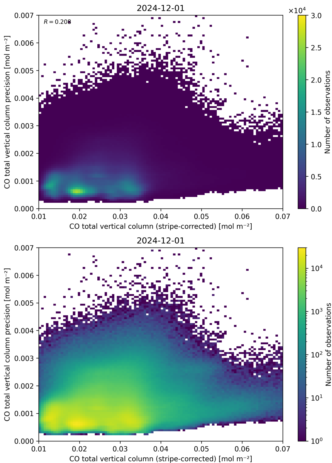
Figure 36: Scatter density plot of “CO total vertical column (stripe-corrected)” against “CO total vertical column precision” for 2024-11-30 to 2024-12-02.
