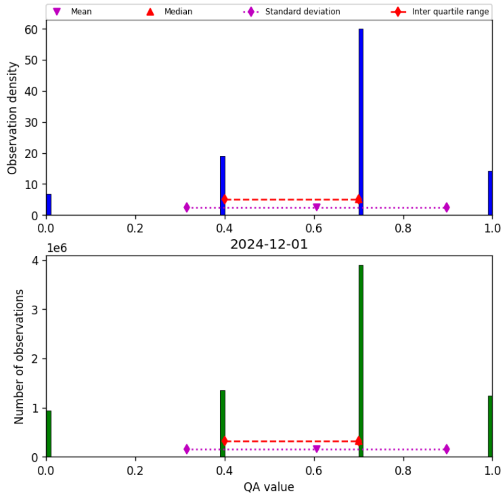
Figure 17: Histogram of “QA value” for 2024-11-30 to 2024-12-02
