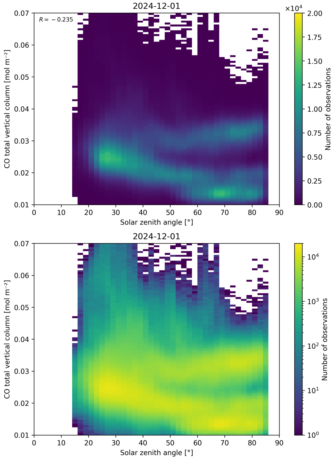
Figure 61: Scatter density plot of “Solar zenith angle” against “CO total vertical column” for 2024-11-30 to 2024-12-02.
