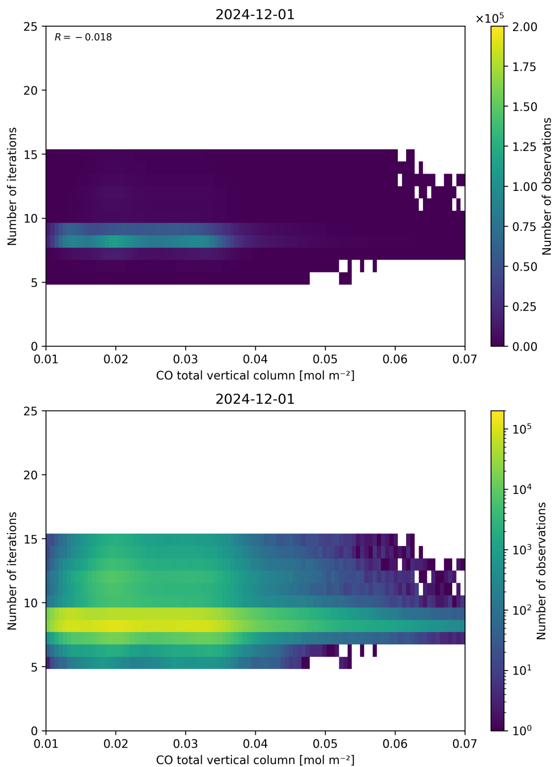
Figure 42: Scatter density plot of “CO total vertical column” against “Number of iterations” for 2024-11-30 to 2024-12-02.
