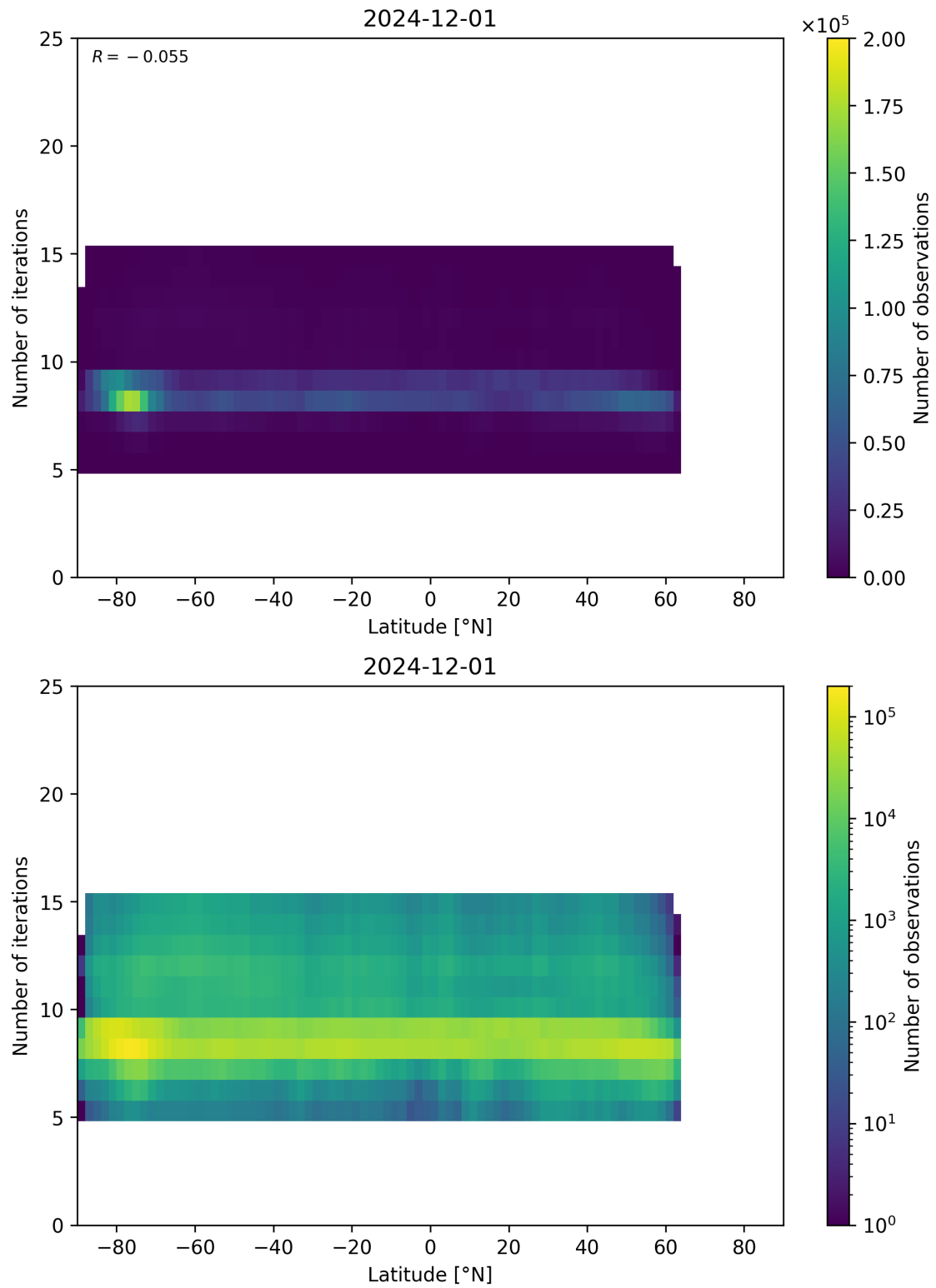
Figure 56: Scatter density plot of “Latitude” against “Number of iterations” for 2024-11-30 to 2024-12-02.
