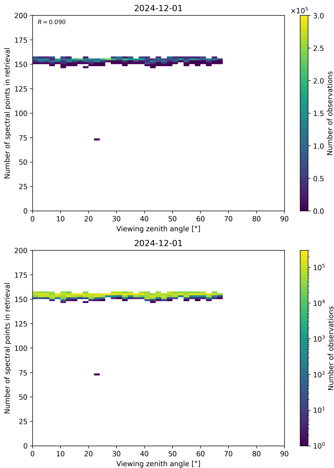
Figure 76: Scatter density plot of “Viewing zenith angle” against “Number of spectral points in retrieval” for 2024-11-30 to 2024-12-02.
