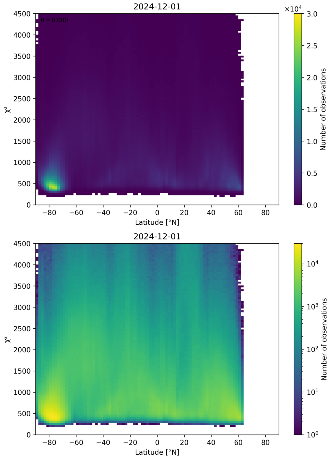
Figure 54: Scatter density plot of “Latitude” against “ \chi^2 ” for 2024-11-30 to 2024-12-02.
