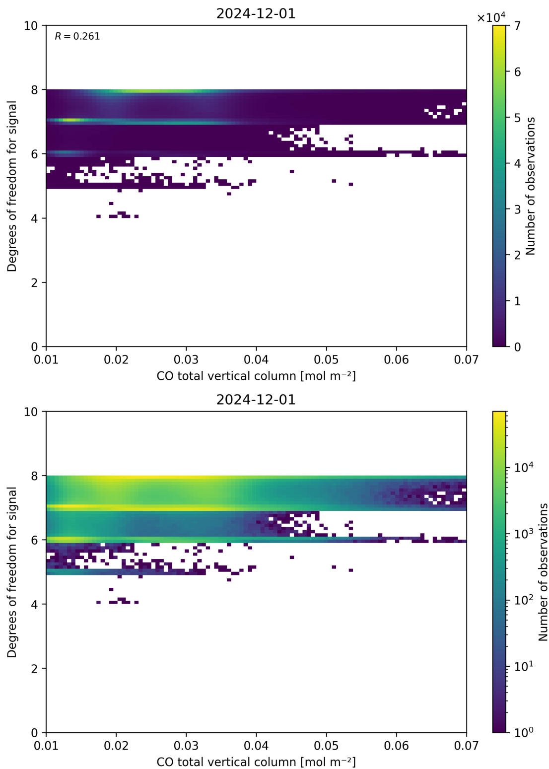
Figure 41: Scatter density plot of “CO total vertical column” against “Degrees of freedom for signal” for 2024-11-30 to 2024-12-02.
