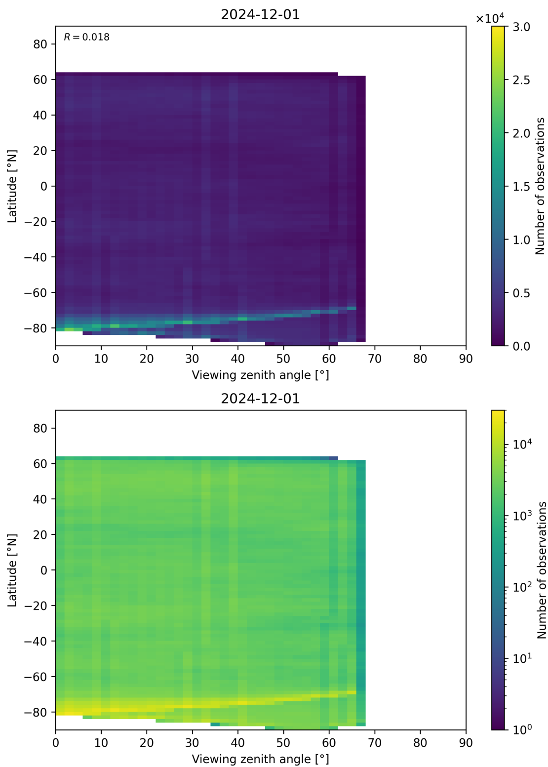
Figure 74: Scatter density plot of “Viewing zenith angle” against “Latitude” for 2024-11-30 to 2024-12-02.
