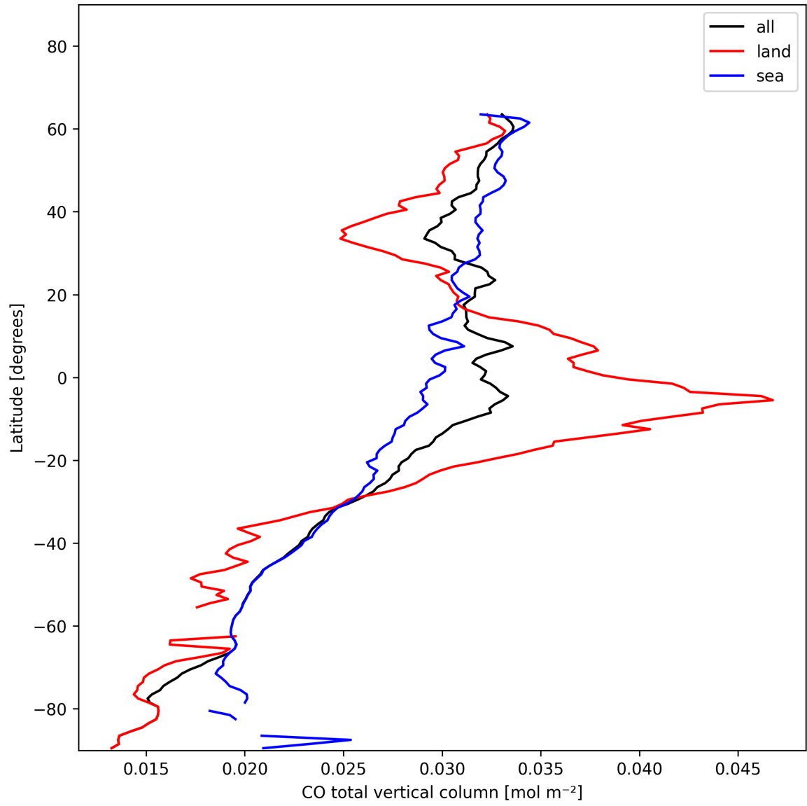
Figure 10: Zonal average of “CO total vertical column” for 2024-11-30 to 2024-12-02.
