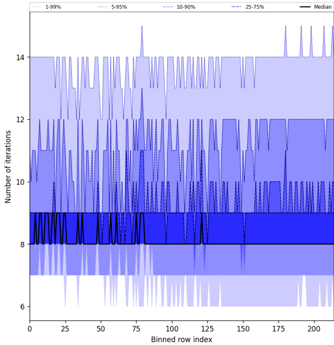
Figure 32: Along track statistics of “Number of iterations” for 2024-11-30 to 2024-12-02
