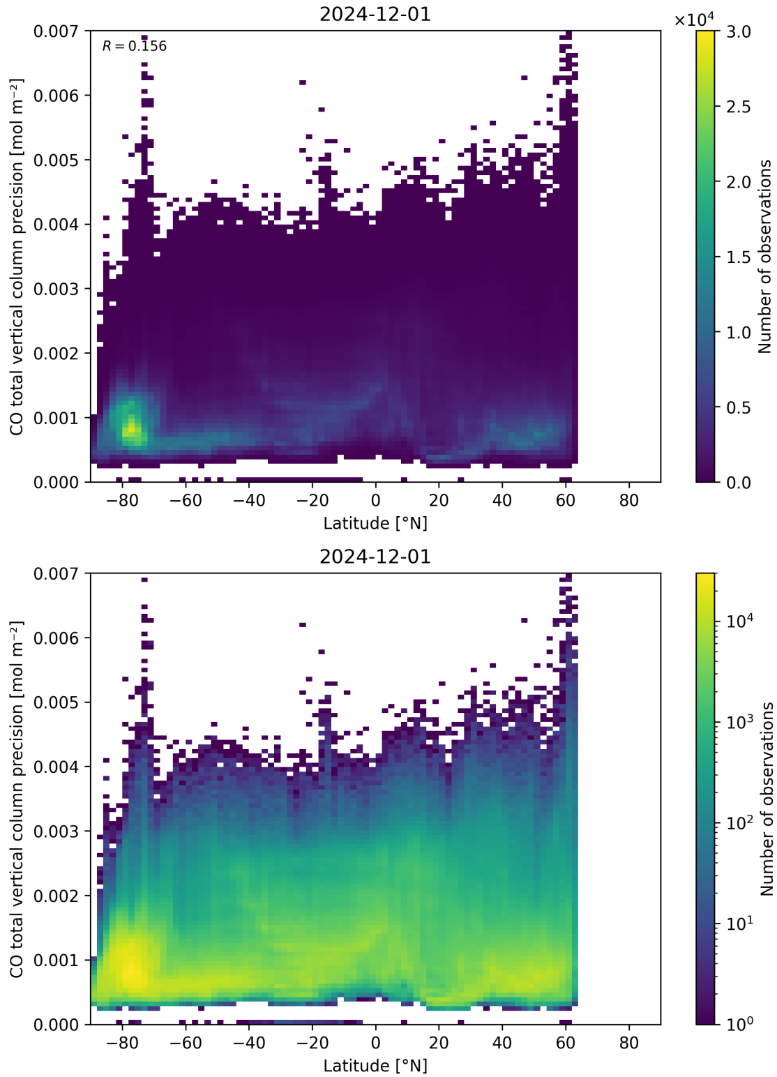
Figure 53: Scatter density plot of “Latitude” against “CO total vertical column precision” for 2024-11-30 to 2024-12-02.
