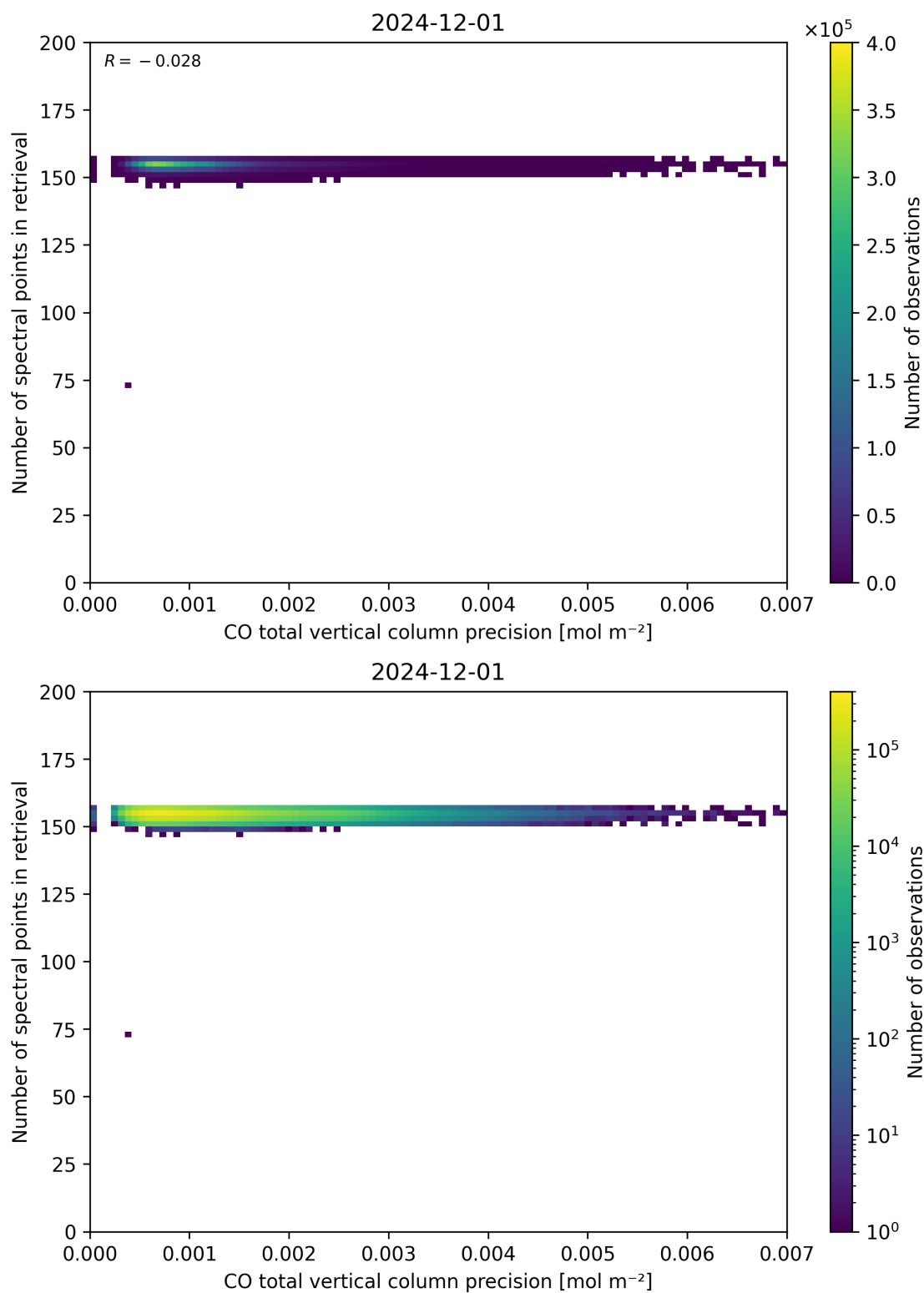
Figure 47: Scatter density plot of “CO total vertical column precision” against “Number of spectral points in retrieval” for 2024-11-30 to 2024-12-02.
