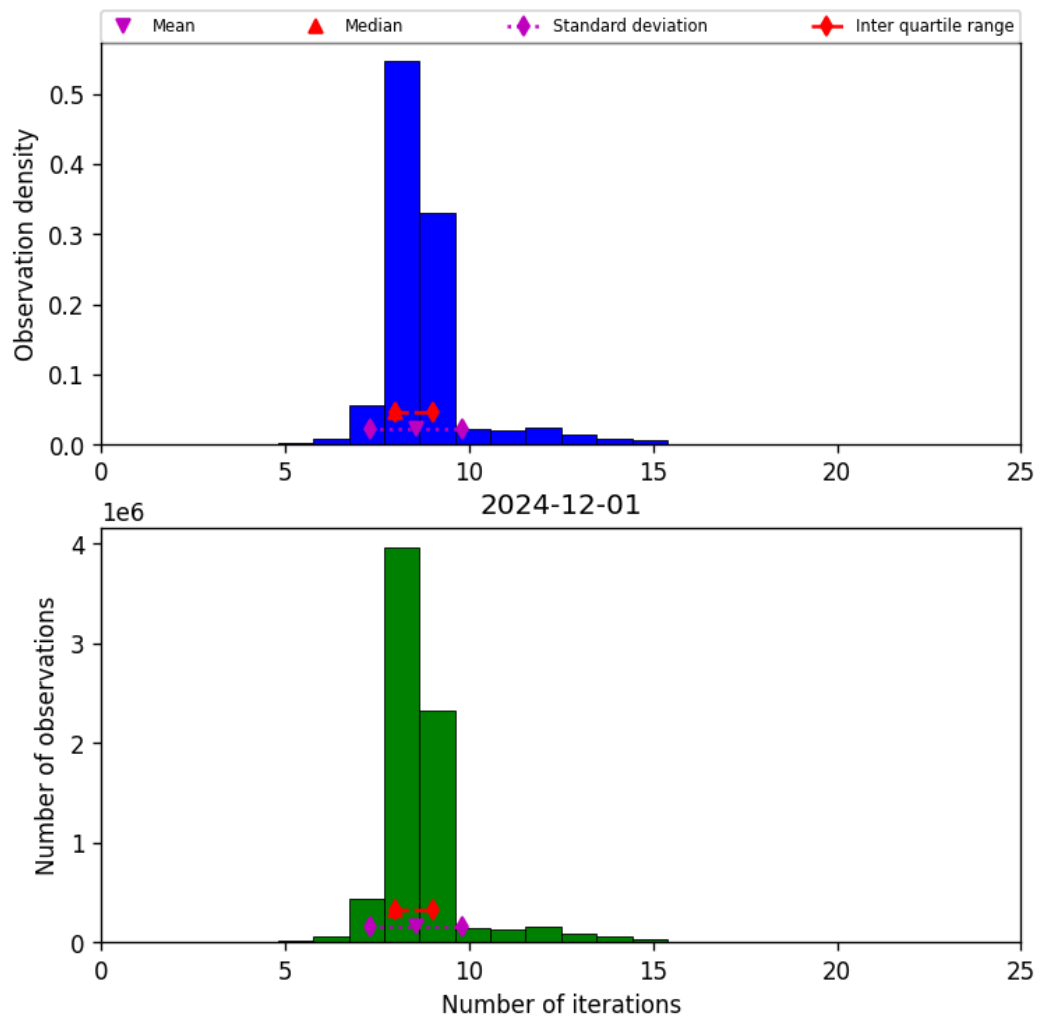
Figure 24: Histogram of “Number of iterations” for 2024-11-30 to 2024-12-02
