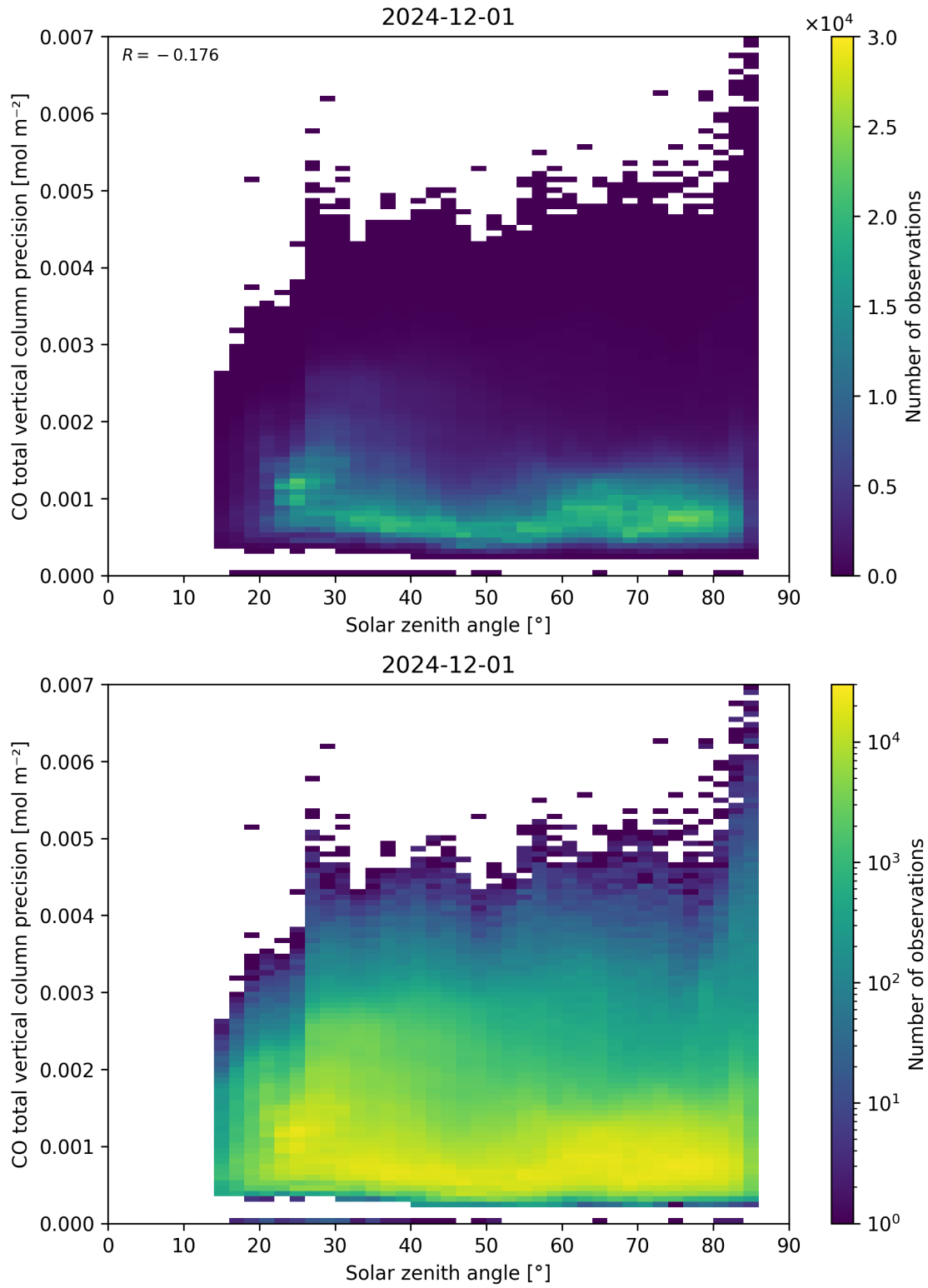
Figure 63: Scatter density plot of “Solar zenith angle” against “CO total vertical column precision” for 2024-11-30 to 2024-12-02.
