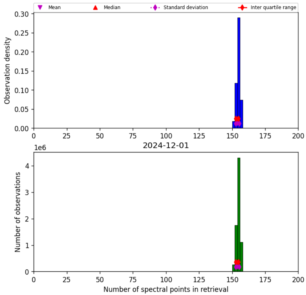
Figure 21: Histogram of “Number of spectral points in retrieval” for 2024-11-30 to 2024-12-02
