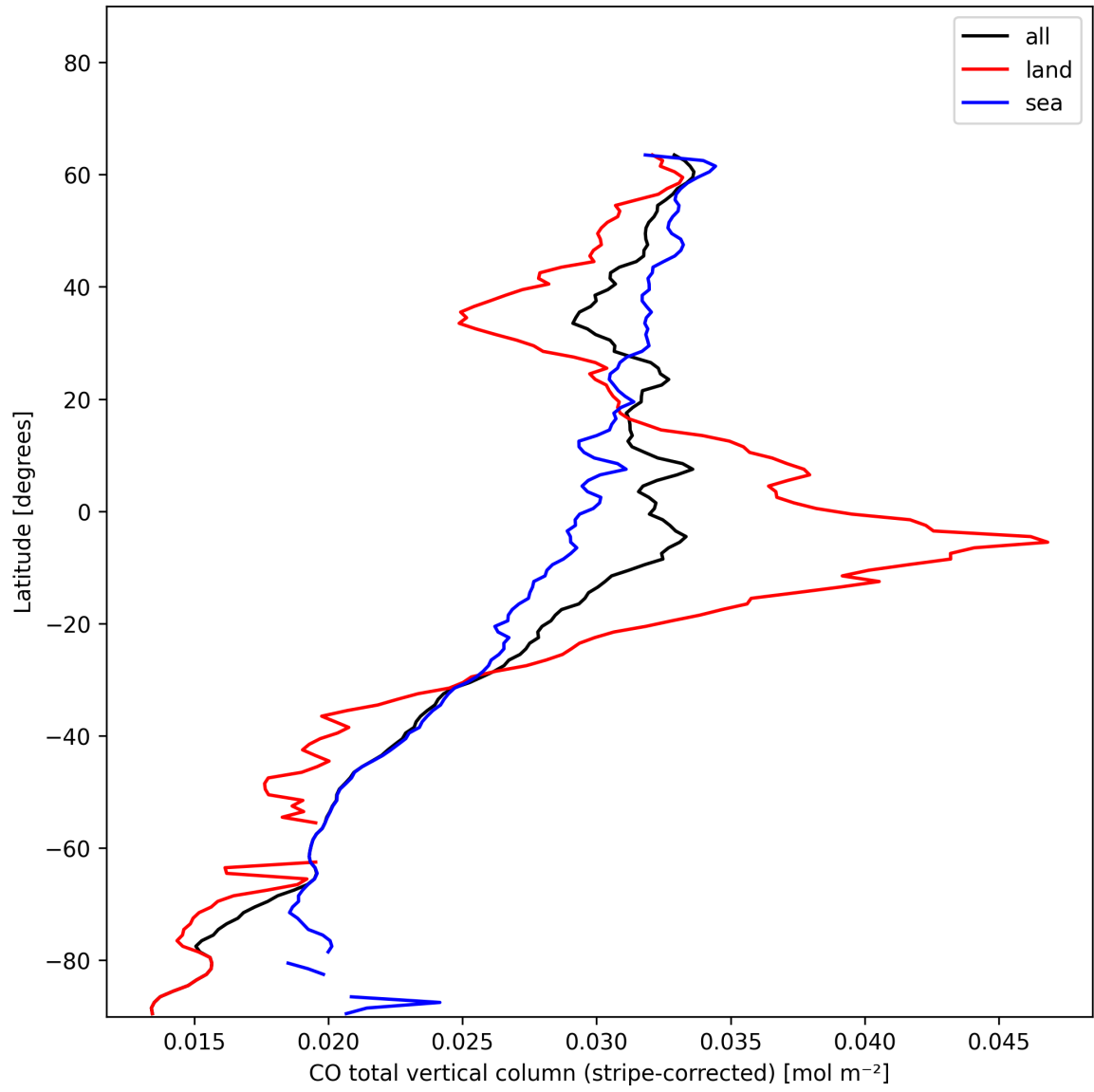
Figure 11: Zonal average of “CO total vertical column (stripe-corrected)” for 2024-11-30 to 2024-12-02.
