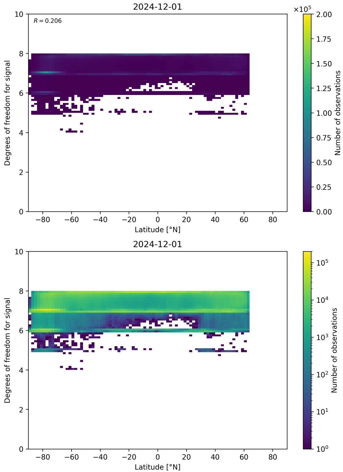
Figure 55: Scatter density plot of “Latitude” against “Degrees of freedom for signal” for 2024-11-30 to 2024-12-02.
