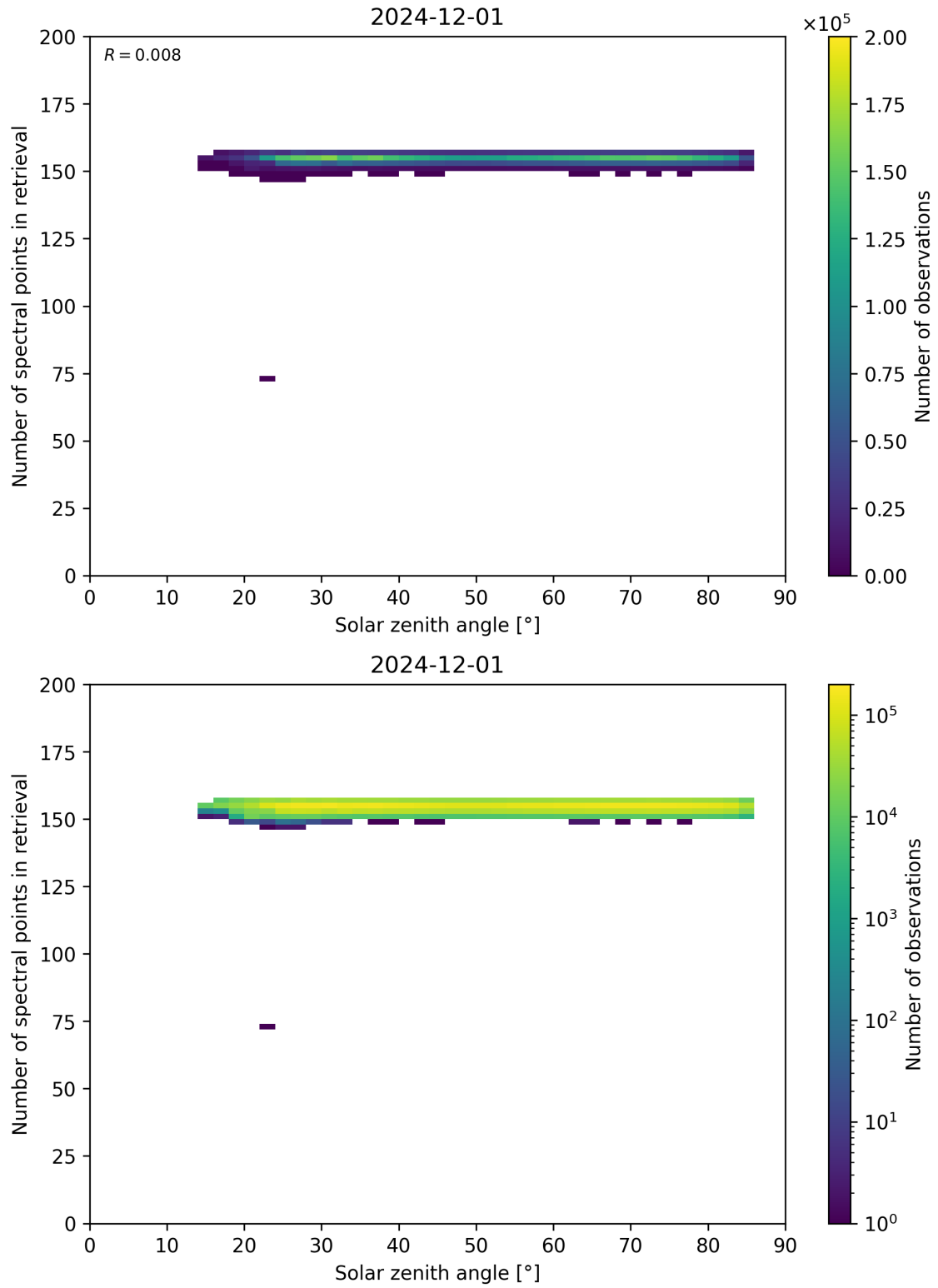
Figure 68: Scatter density plot of “Solar zenith angle” against “Number of spectral points in retrieval” for 2024-11-30 to 2024-12-02.
