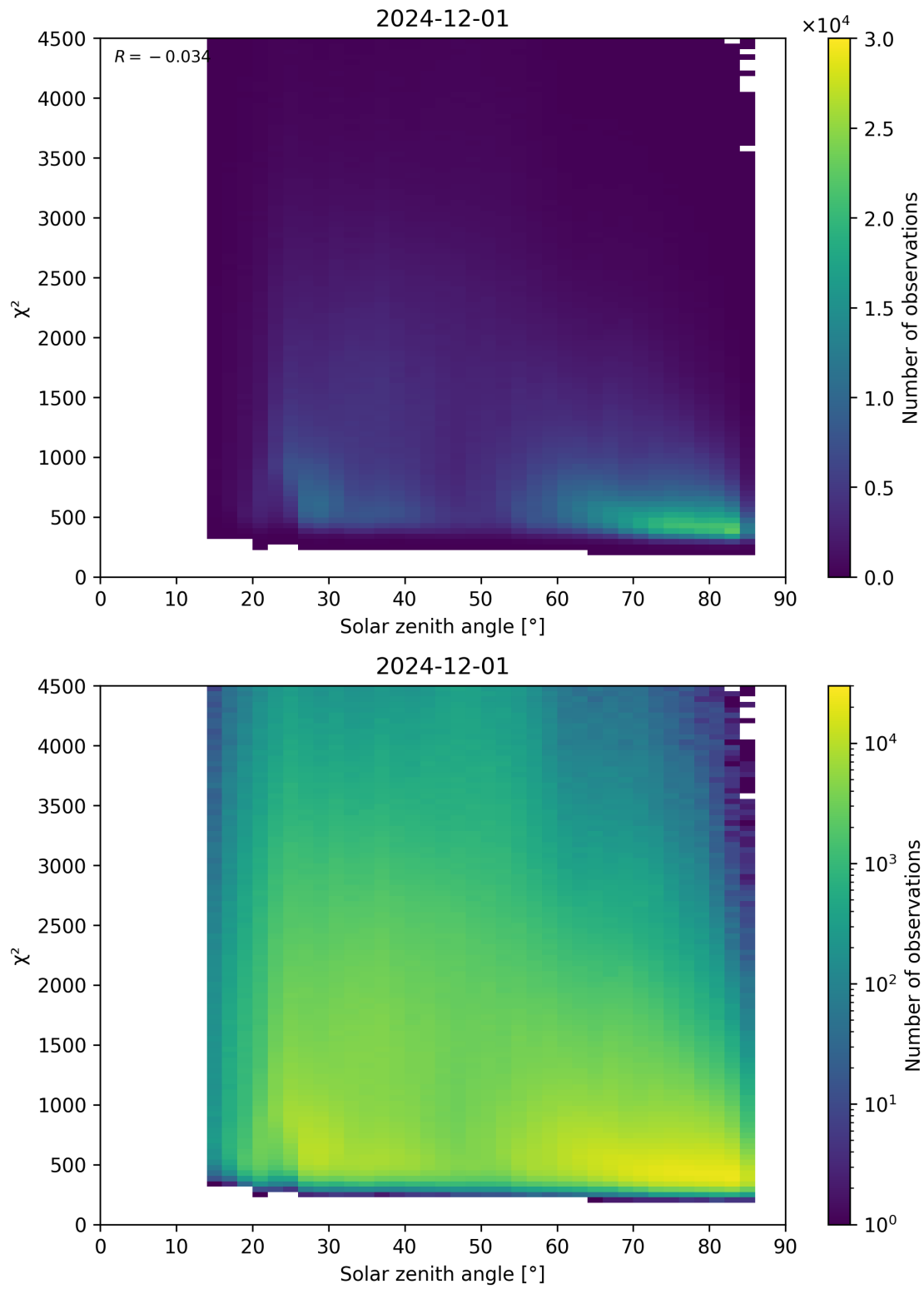
Figure 64: Scatter density plot of “Solar zenith angle” against “ \chi^2 ” for 2024-11-30 to 2024-12-02.
