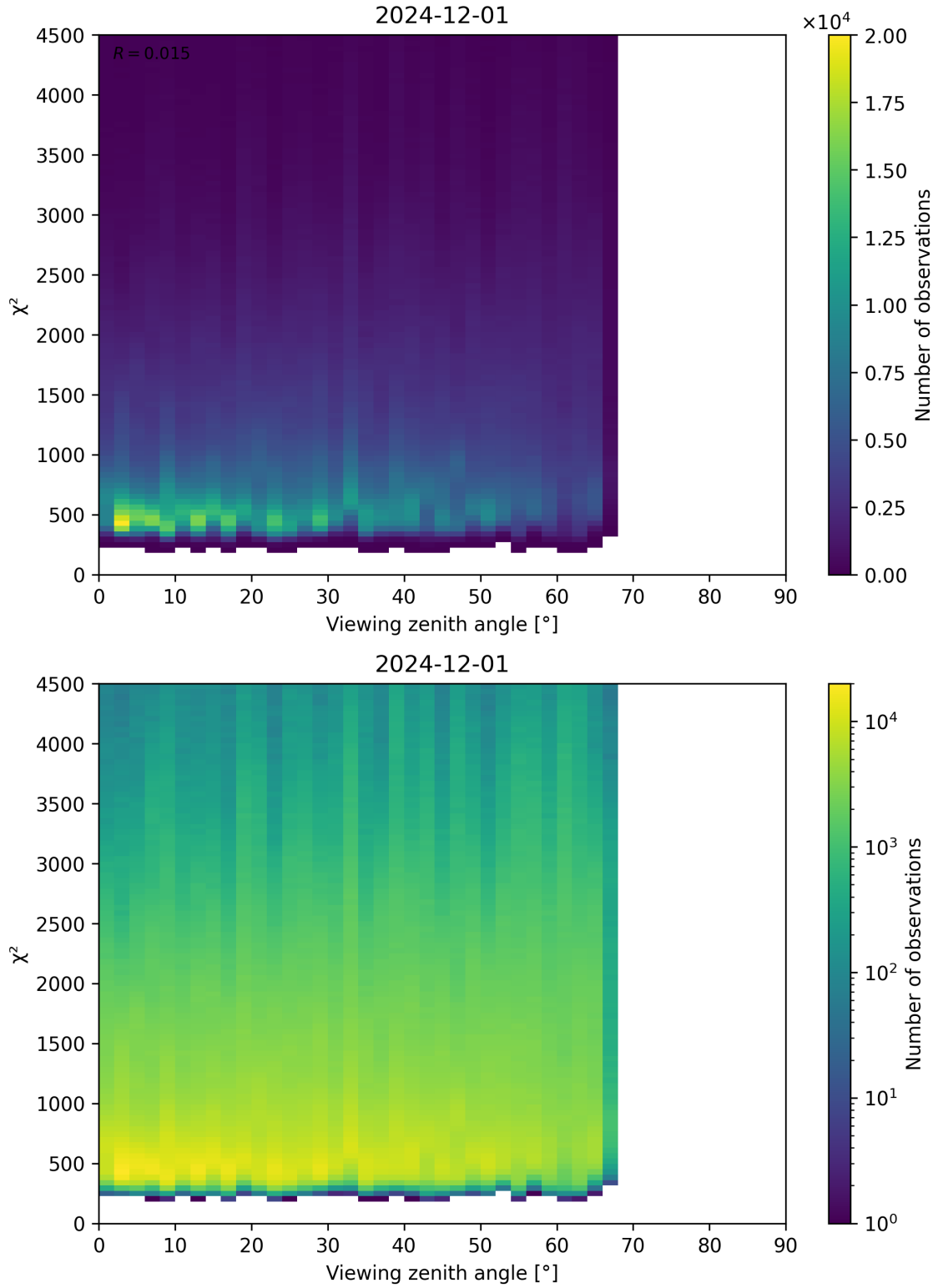
Figure 72: Scatter density plot of “Viewing zenith angle” against “ \chi^2 ” for 2024-11-30 to 2024-12-02.
