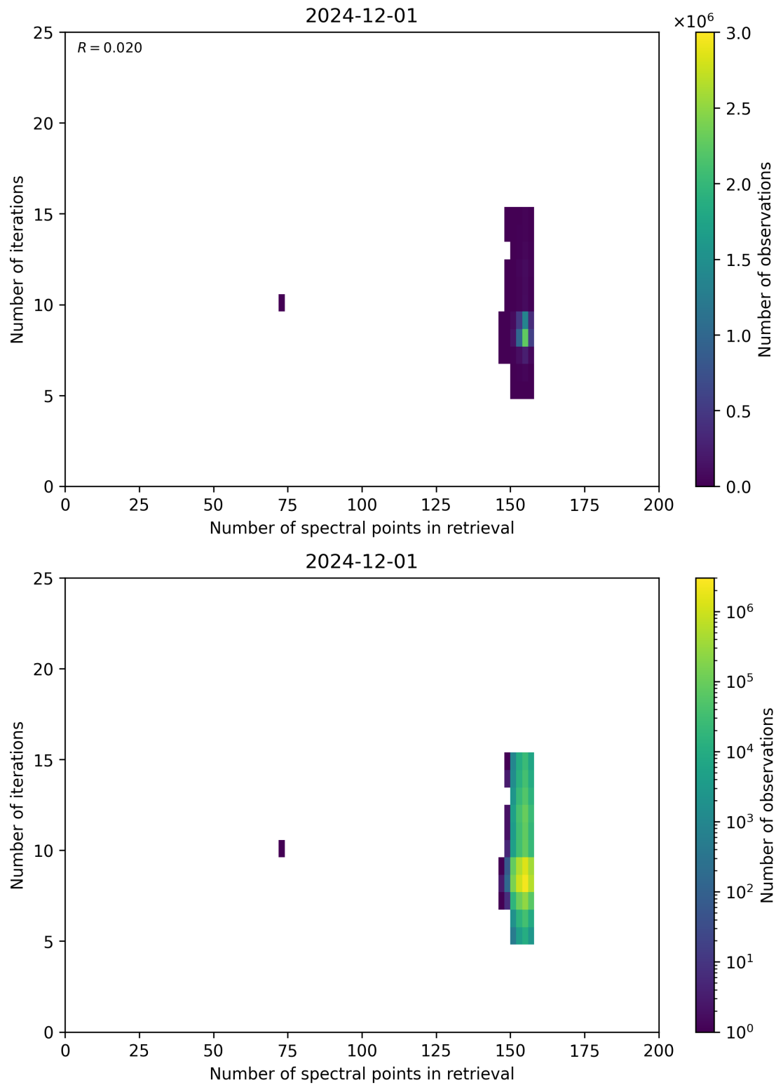
Figure 60: Scatter density plot of “Number of spectral points in retrieval” against “Number of iterations” for 2024-11-30 to 2024-12-02.
