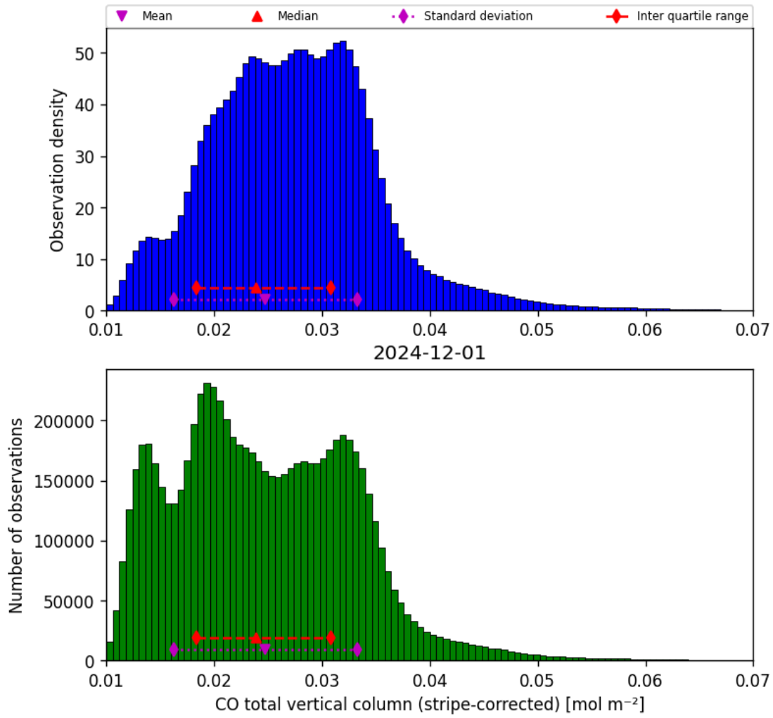
Figure 19: Histogram of “CO total vertical column (stripe-corrected)” for 2024-11-30 to 2024-12-02
