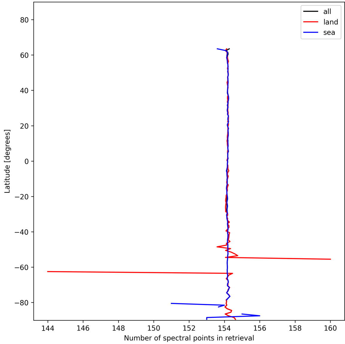
Figure 13: Zonal average of “Number of spectral points in retrieval” for 2024-11-30 to 2024-12-02.
