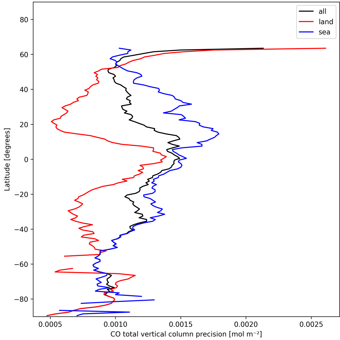
Figure 12: Zonal average of “CO total vertical column precision” for 2024-11-30 to 2024-12-02.
