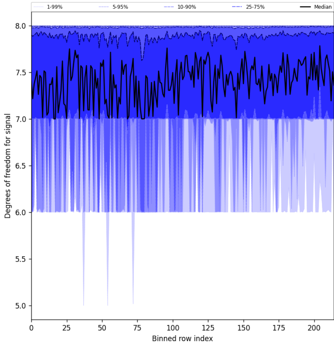
Figure 31: Along track statistics of “Degrees of freedom for signal” for 2024-11-30 to 2024-12-02
