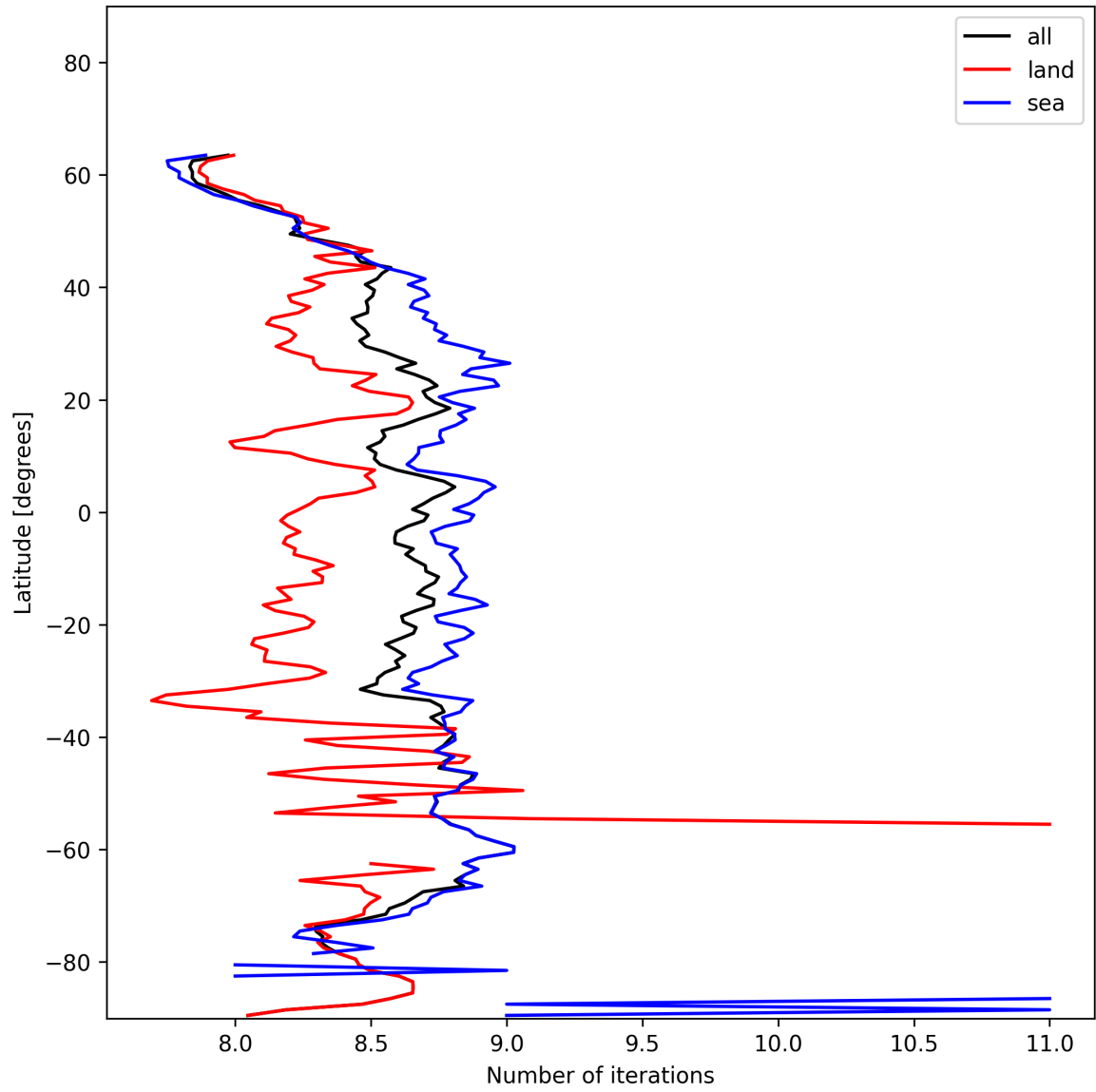
Figure 16: Zonal average of “Number of iterations” for 2024-11-30 to 2024-12-02.
