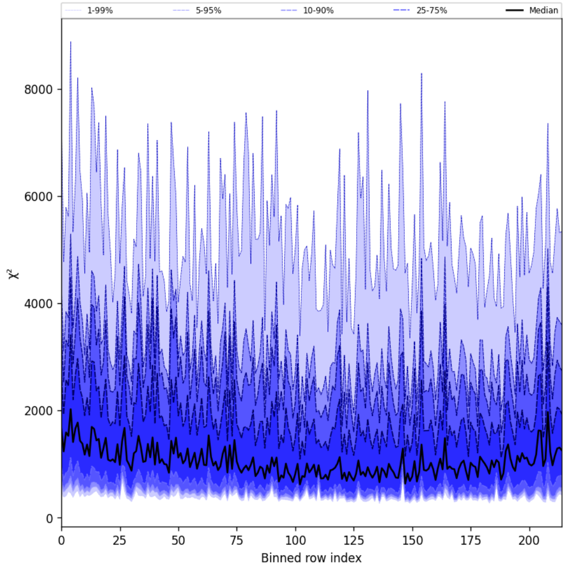
Figure 30: Along track statistics of “ \chi^2 ” for 2024-11-30 to 2024-12-02
