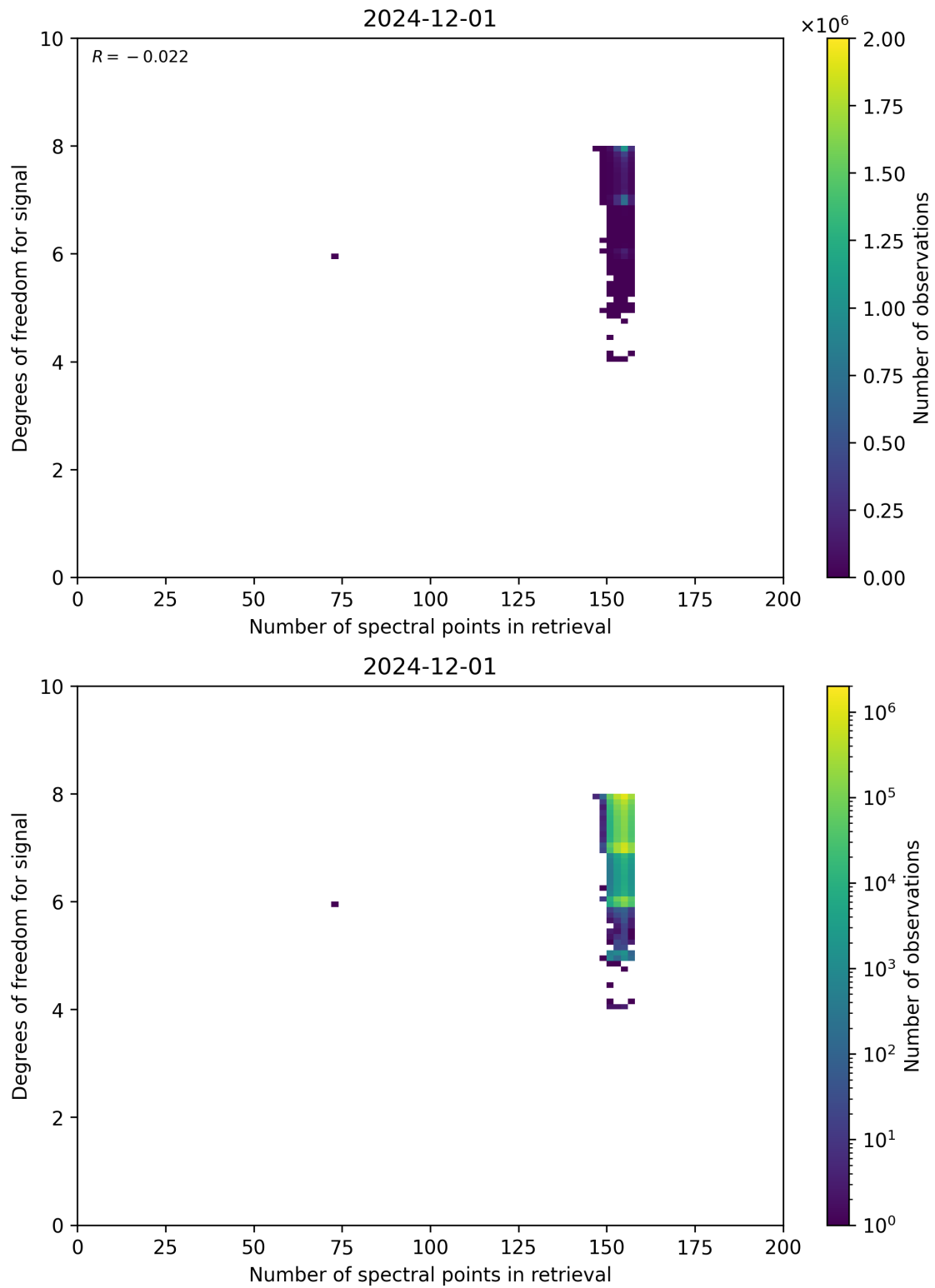
Figure 59: Scatter density plot of “Number of spectral points in retrieval” against “Degrees of freedom for signal” for 2024-11-30 to 2024-12-02.
