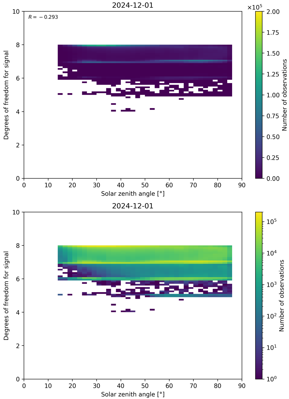
Figure 65: Scatter density plot of “Solar zenith angle” against “Degrees of freedom for signal” for 2024-11-30 to 2024-12-02.
