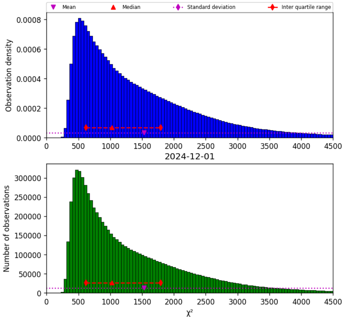
Figure 22: Histogram of “ \chi^2 ” for 2024-11-30 to 2024-12-02
