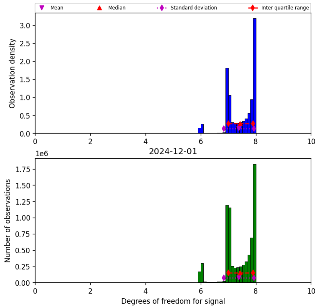
Figure 23: Histogram of “Degrees of freedom for signal” for 2024-11-30 to 2024-12-02
