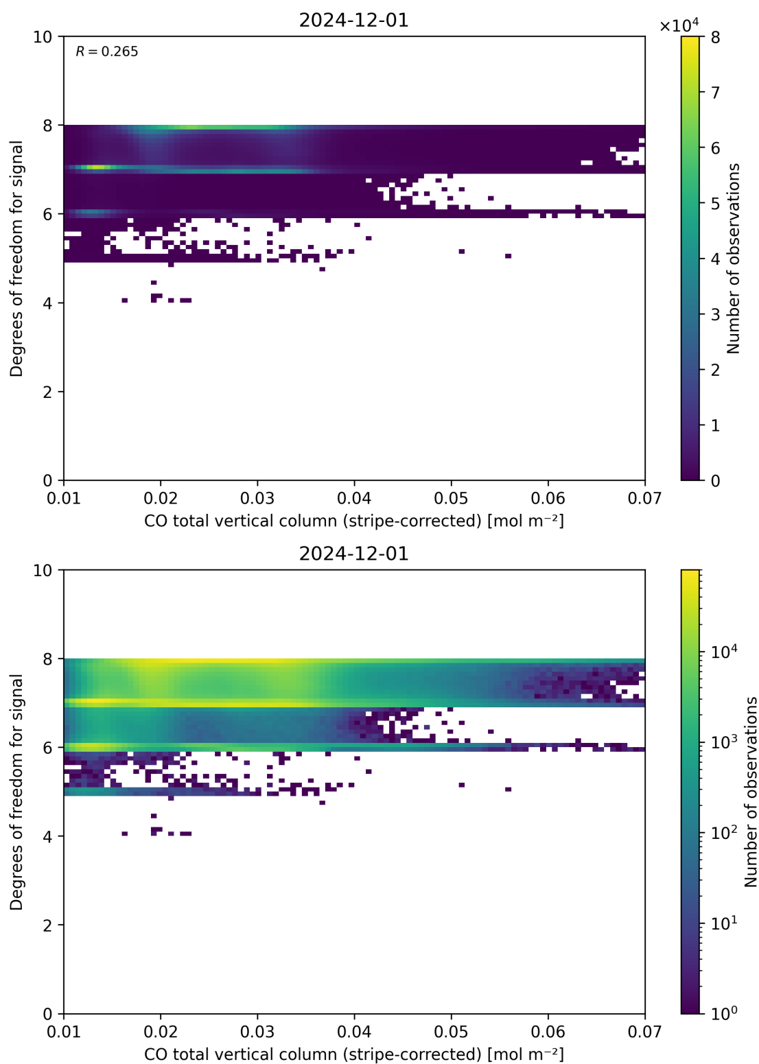
Figure 38: Scatter density plot of “CO total vertical column (stripe-corrected)” against “Degrees of freedom for signal” for 2024-11-30 to 2024-12-02.
