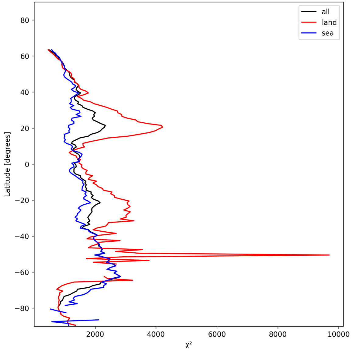
Figure 14: Zonal average of “ \chi^2 ” for 2024-11-30 to 2024-12-02.
