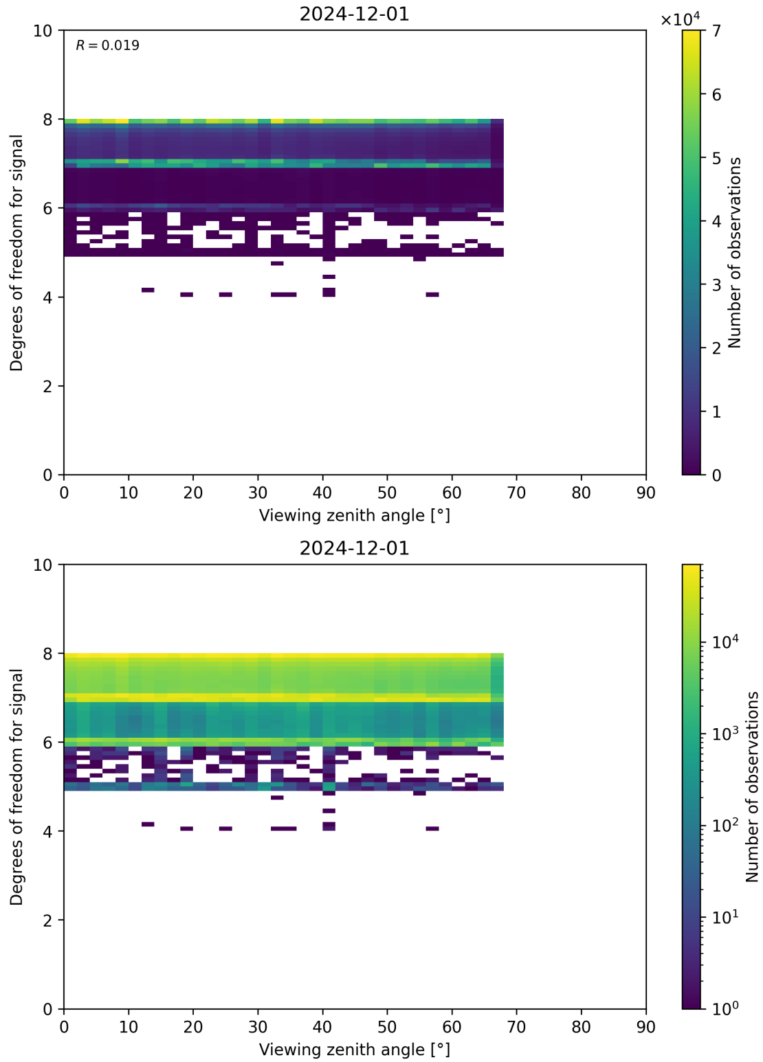
Figure 73: Scatter density plot of “Viewing zenith angle” against “Degrees of freedom for signal” for 2024-11-30 to 2024-12-02.
