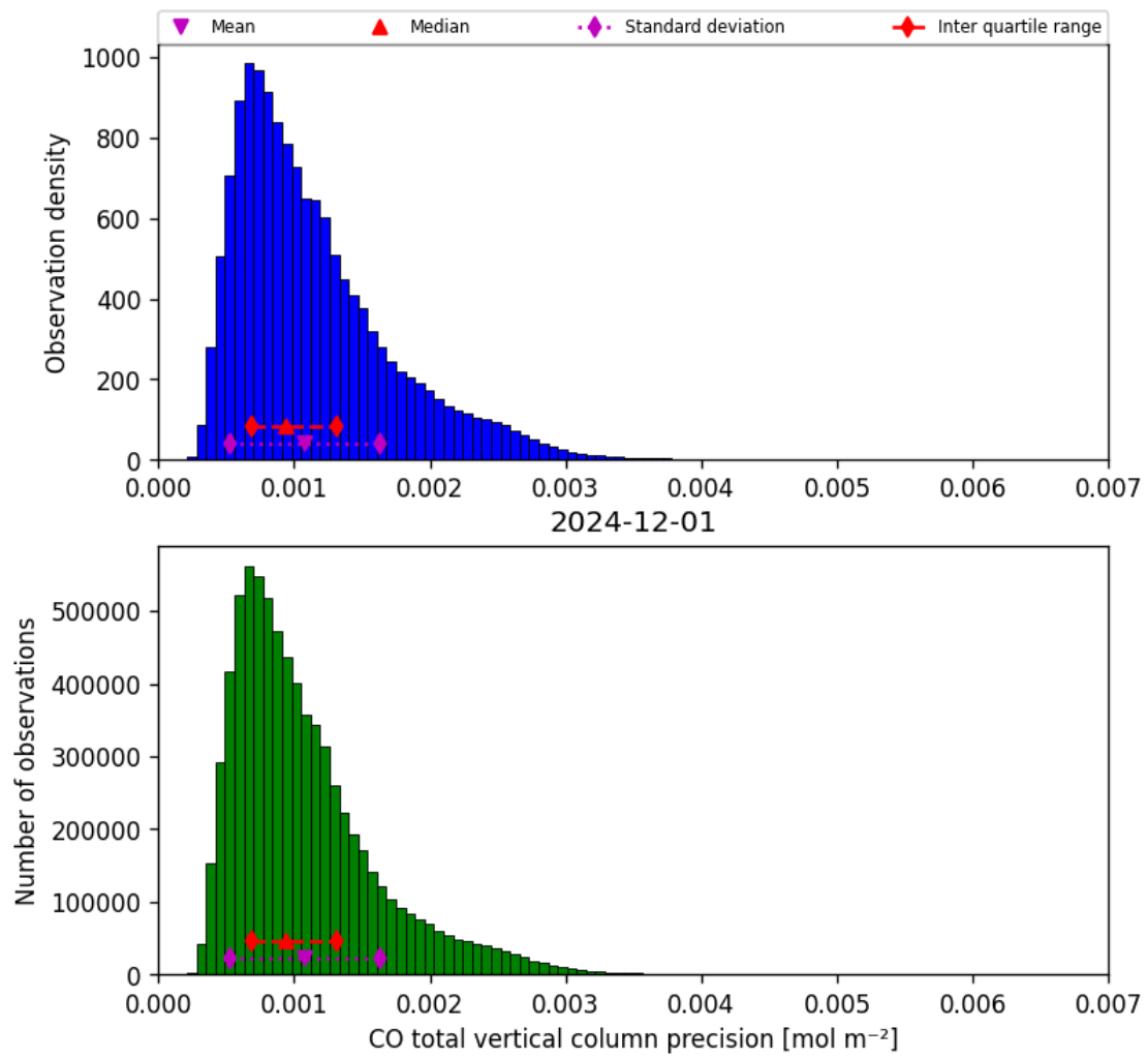
Figure 20: Histogram of “CO total vertical column precision” for 2024-11-30 to 2024-12-02
