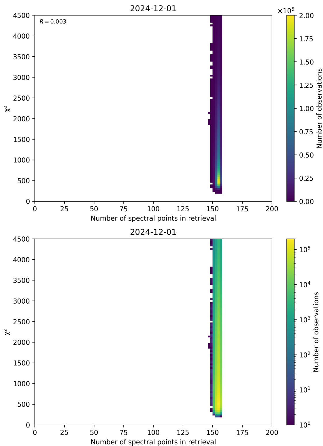
Figure 58: Scatter density plot of “Number of spectral points in retrieval” against “ \chi^2 ” for 2024-11-30 to 2024-12-02.
