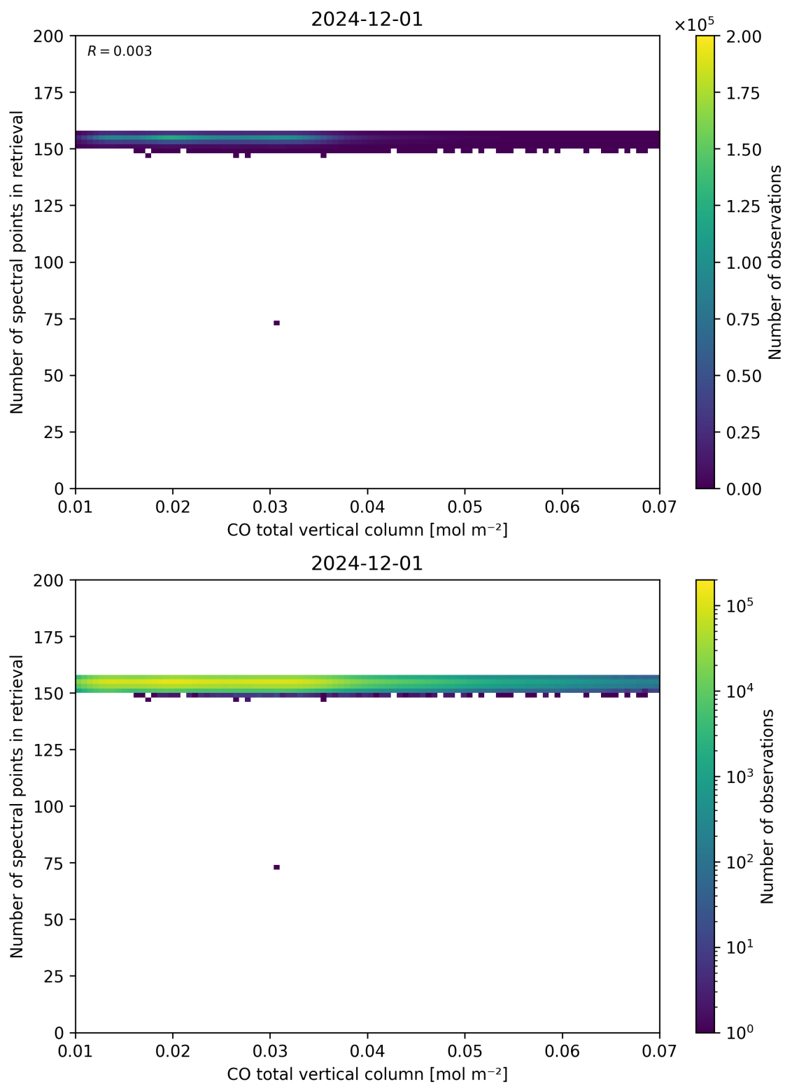
Figure 43: Scatter density plot of “CO total vertical column” against “Number of spectral points in retrieval” for 2024-11-30 to 2024-12-02.
