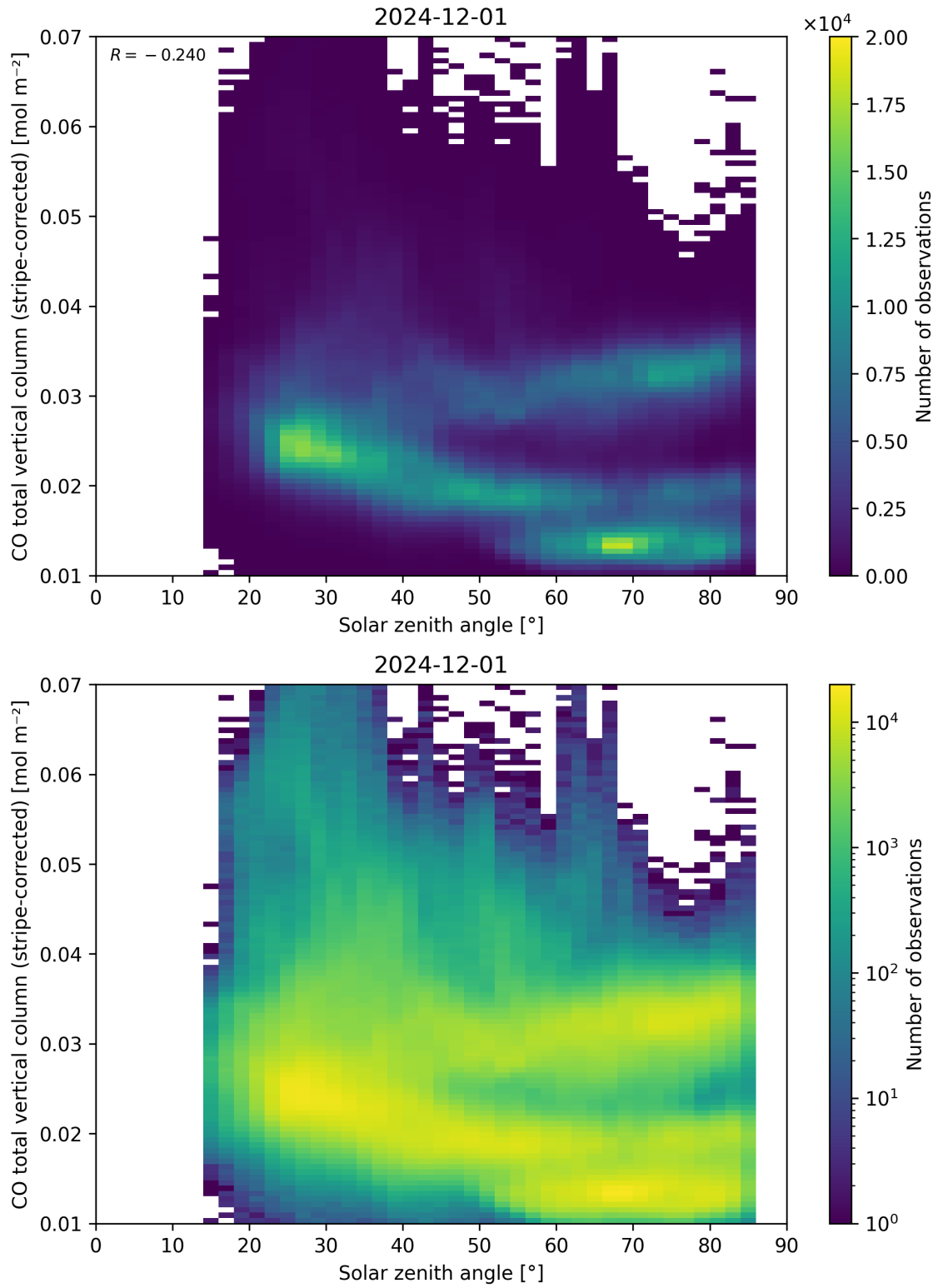
Figure 62: Scatter density plot of “Solar zenith angle” against “CO total vertical column (stripe-corrected)” for 2024-11-30 to 2024-12-02.
