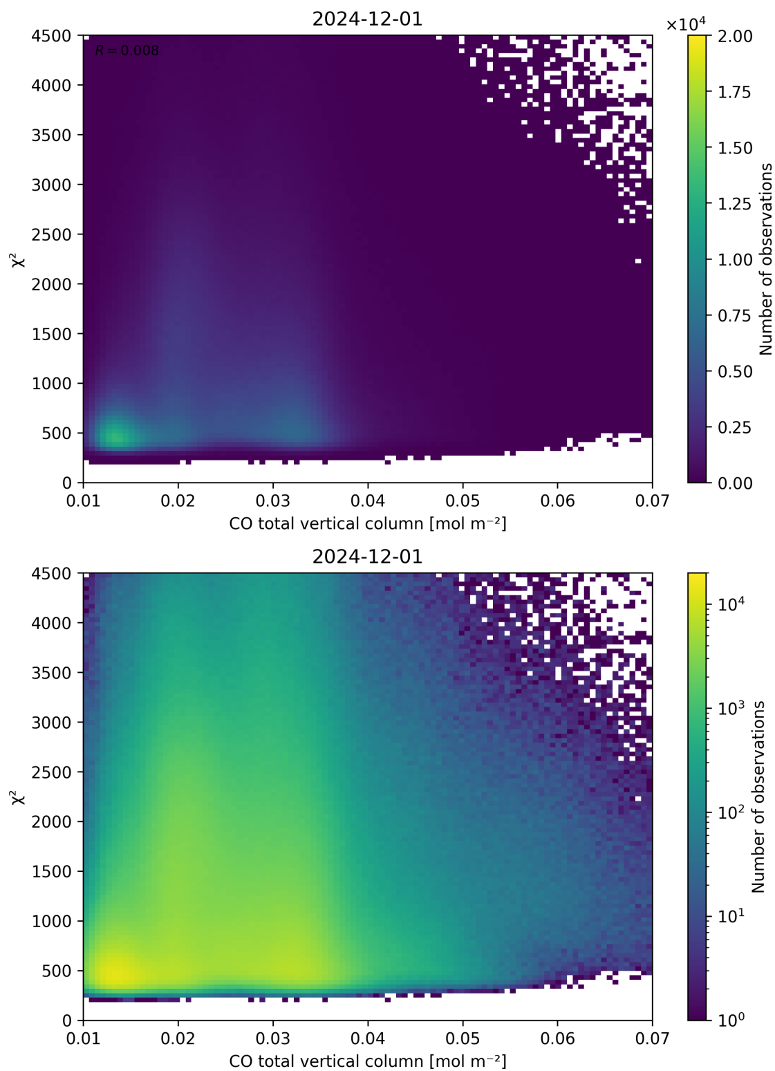
Figure 35: Scatter density plot of “CO total vertical column” against “ \chi^2 ” for 2024-11-30 to 2024-12-02.
