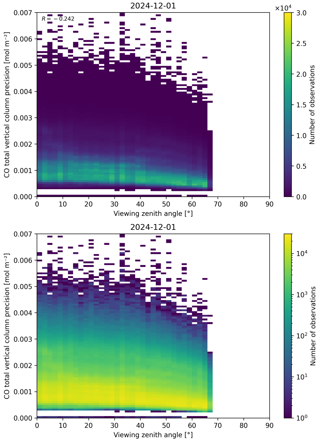
Figure 71: Scatter density plot of “Viewing zenith angle” against “CO total vertical column precision” for 2024-11-30 to 2024-12-02.
