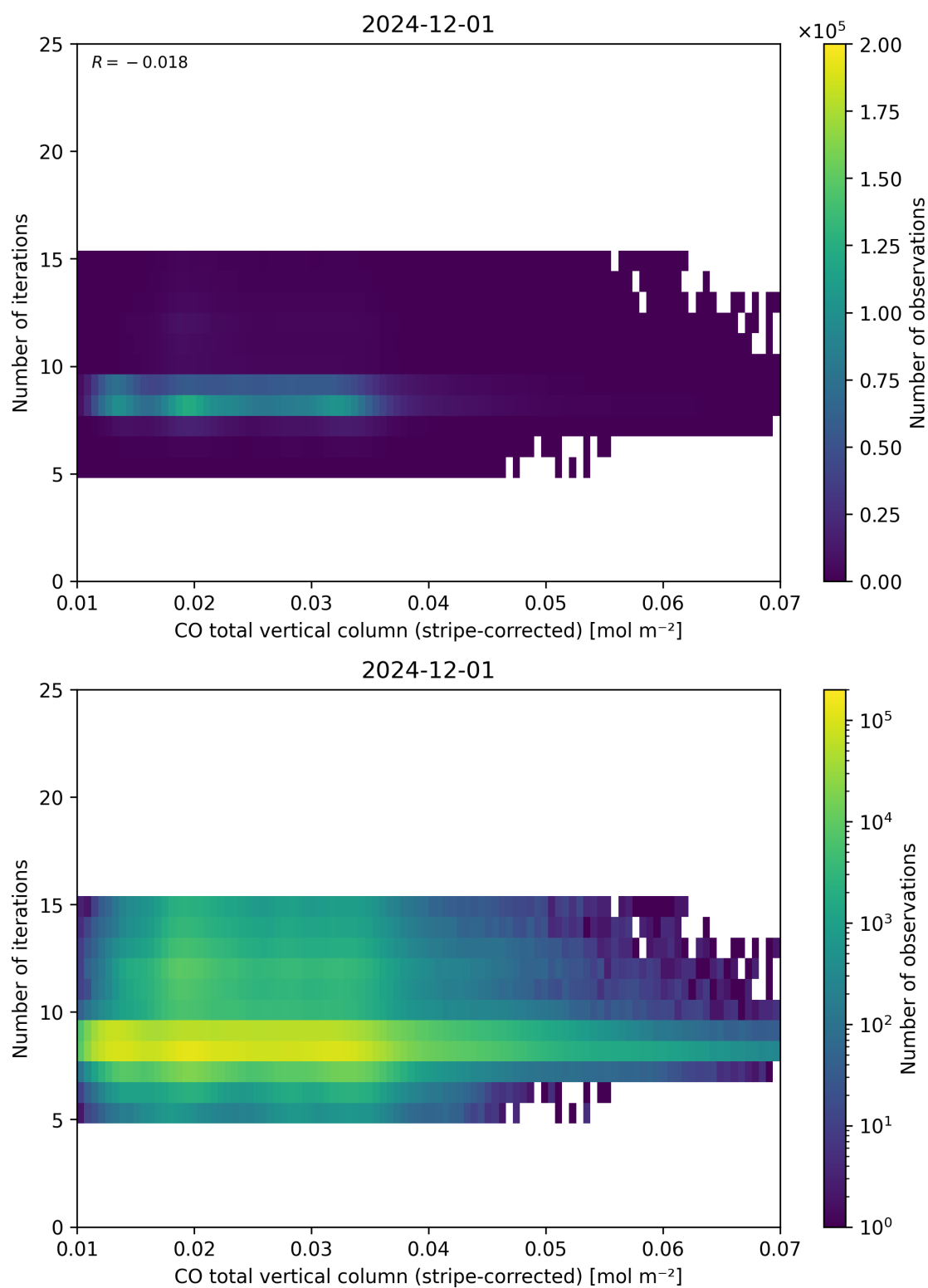
Figure 39: Scatter density plot of “CO total vertical column (stripe-corrected)” against “Number of iterations” for 2024-11-30 to 2024-12-02.
