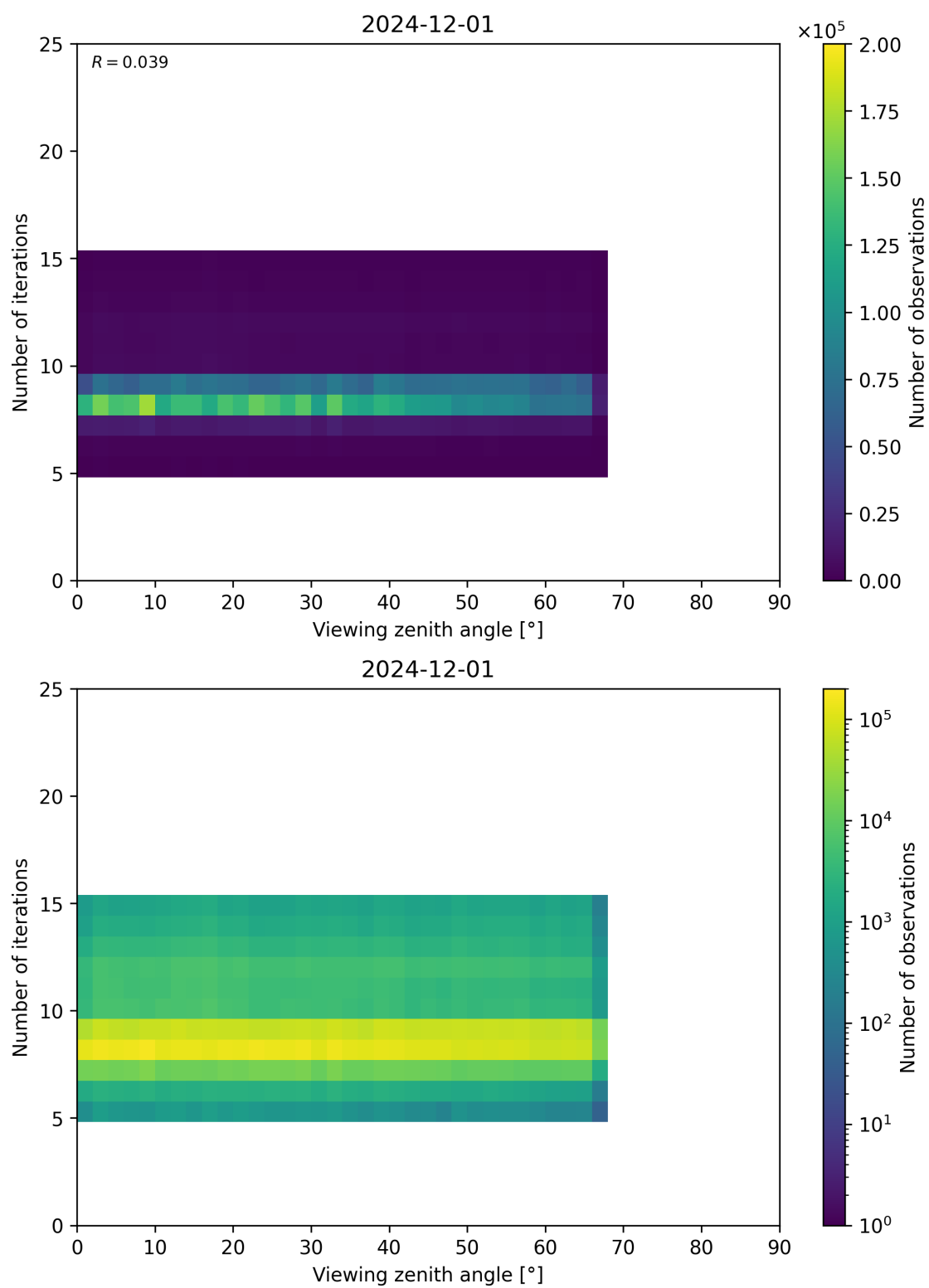
Figure 75: Scatter density plot of “Viewing zenith angle” against “Number of iterations” for 2024-11-30 to 2024-12-02.
