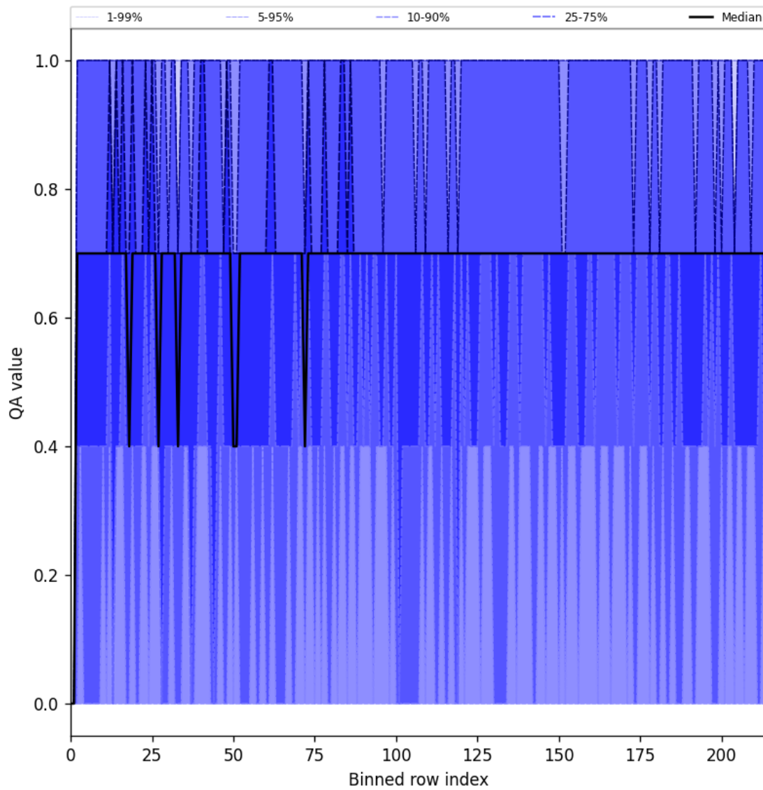
Figure 25: Along track statistics of "QA value" for 2024-11-30 to 2024-12-02
