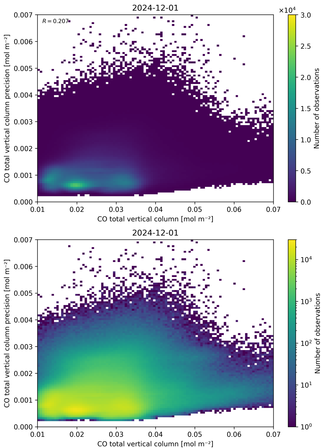
Figure 34: Scatter density plot of “CO total vertical column” against “CO total vertical column precision” for 2024-11-30 to 2024-12-02.
