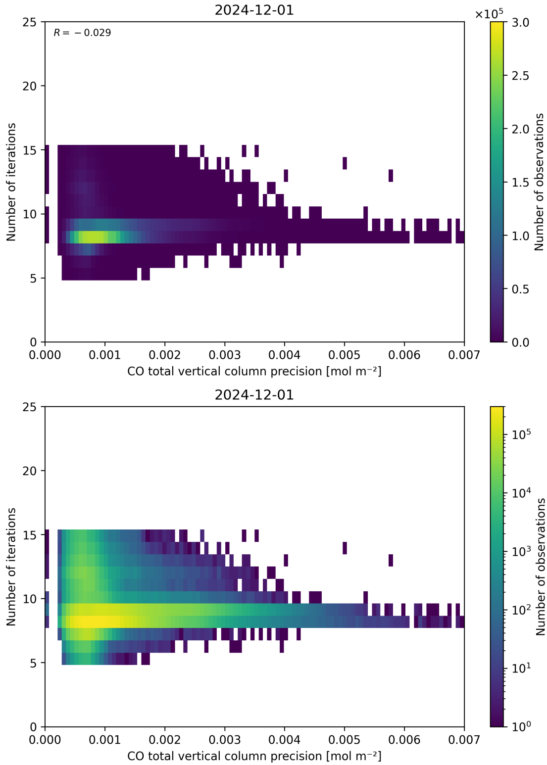
Figure 46: Scatter density plot of “CO total vertical column precision” against “Number of iterations” for 2024-11-30 to 2024-12-02.
