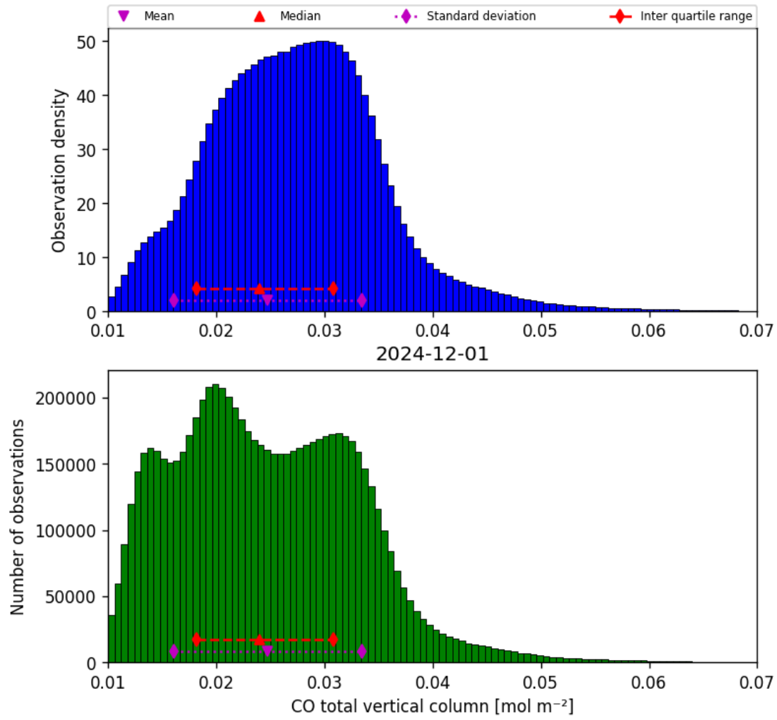
Figure 18: Histogram of “CO total vertical column” for 2024-11-30 to 2024-12-02
