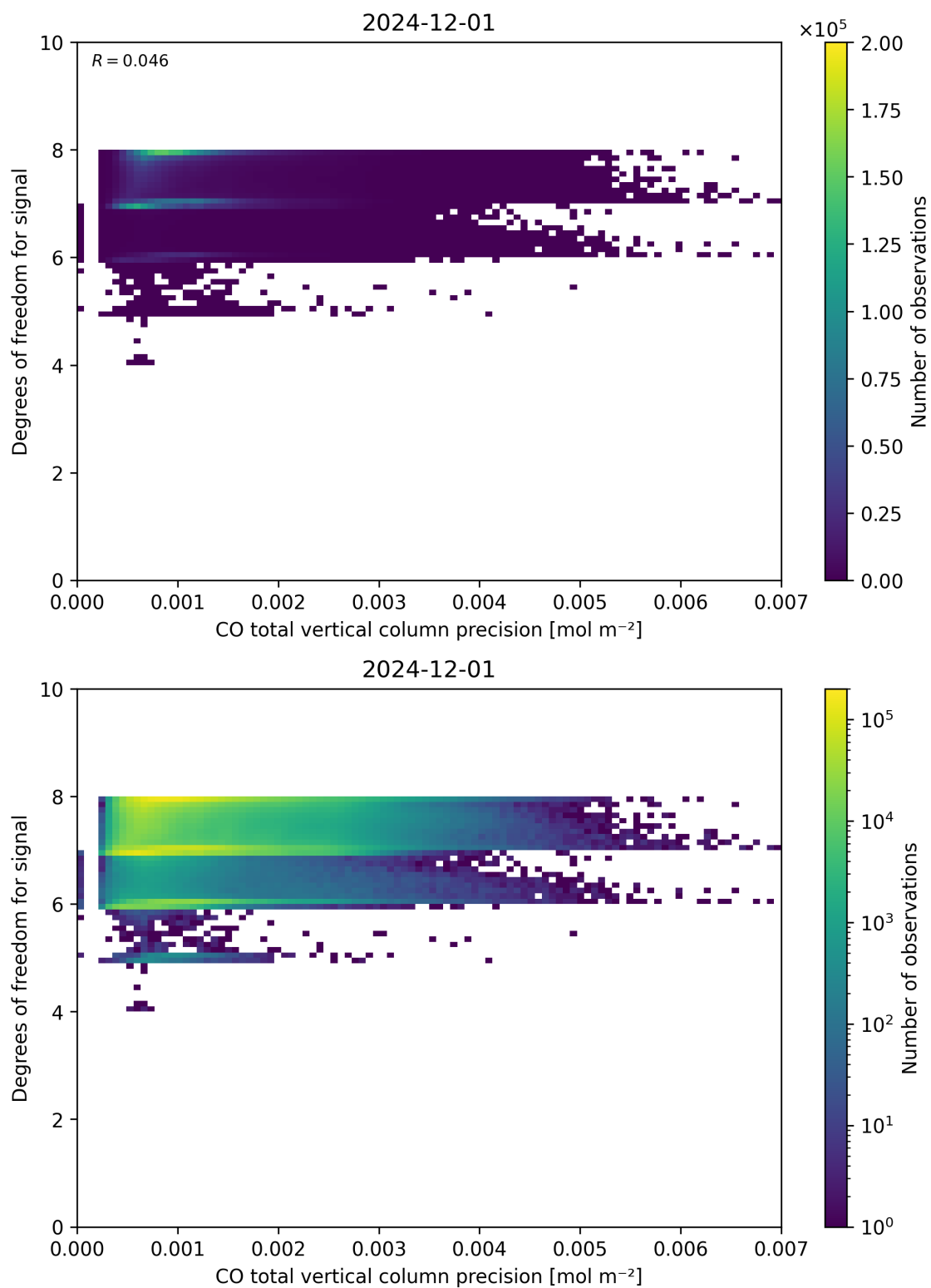
Figure 45: Scatter density plot of “CO total vertical column precision” against “Degrees of freedom for signal” for 2024-11-30 to 2024-12-02.
