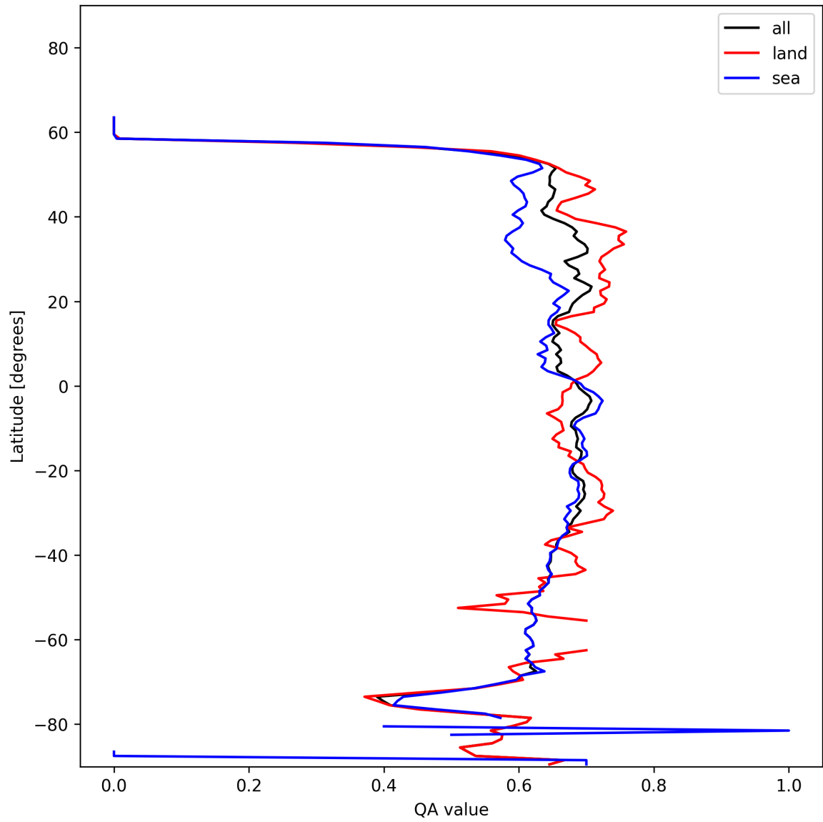
Figure 9: Zonal average of “QA value” for 2024-11-30 to 2024-12-02.
