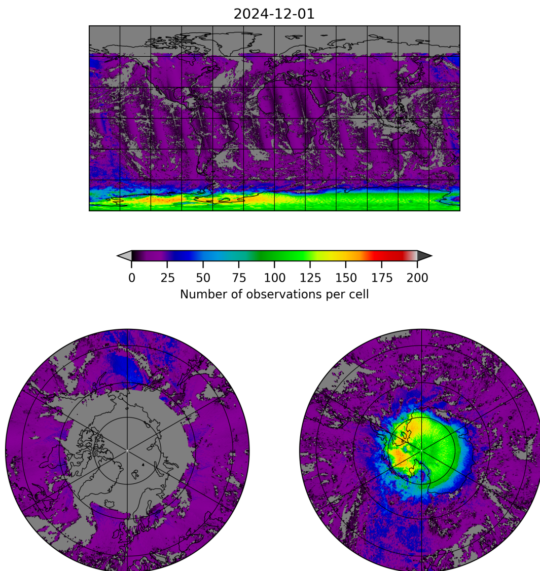
Figure 8: Map of the number of observations for 2024-11-30 to 2024-12-02
