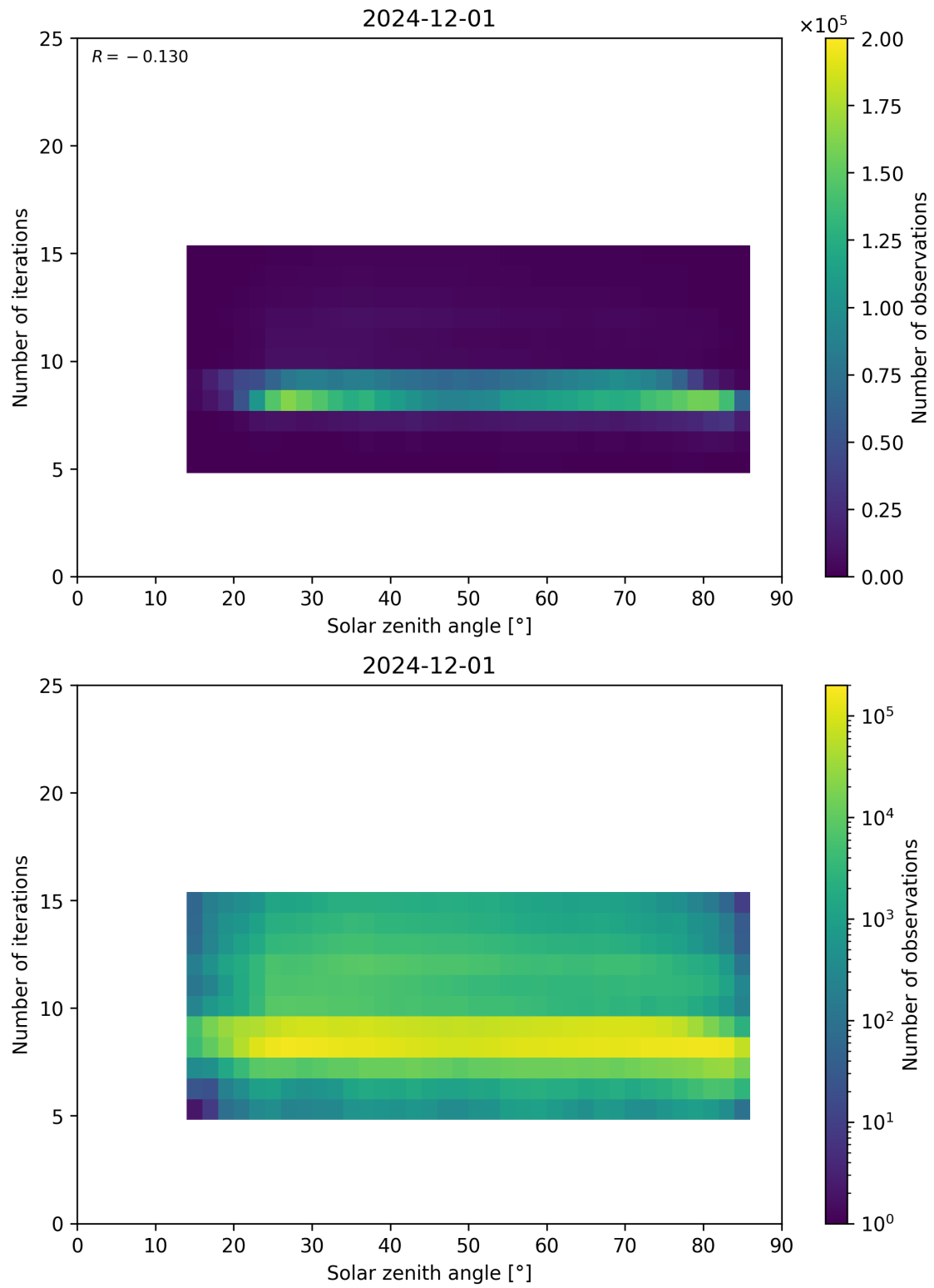
Figure 67: Scatter density plot of “Solar zenith angle” against “Number of iterations” for 2024-11-30 to 2024-12-02.
