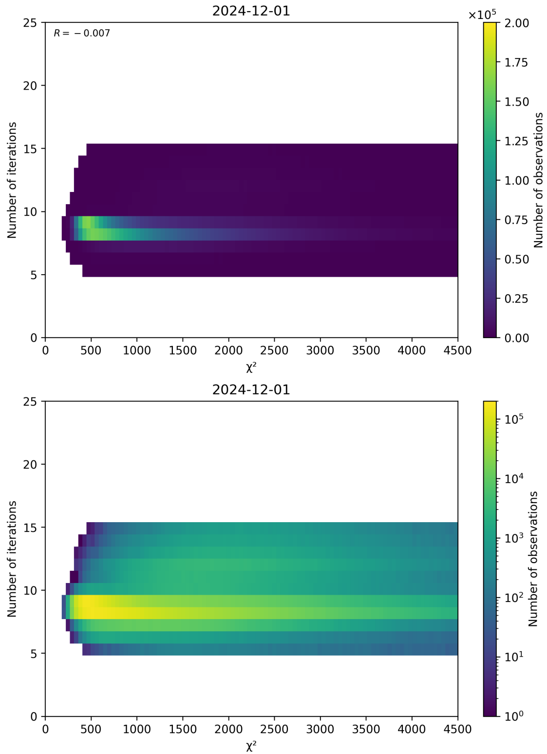
Figure 49: Scatter density plot of “ \chi^2 ” against “Number of iterations” for 2024-11-30 to 2024-12-02.
