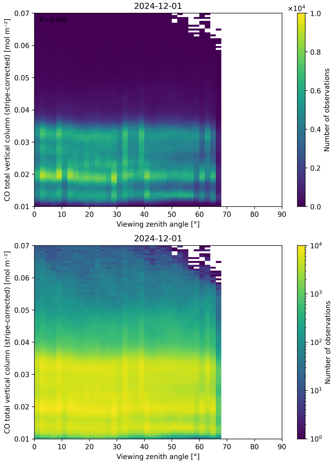
Figure 70: Scatter density plot of “Viewing zenith angle” against “CO total vertical column (stripe-corrected)” for 2024-11-30 to 2024-12-02.
