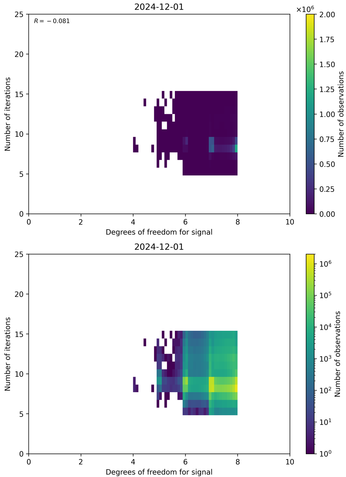
Figure 50: Scatter density plot of “Degrees of freedom for signal” against “Number of iterations” for 2024-11-30 to 2024-12-02.
