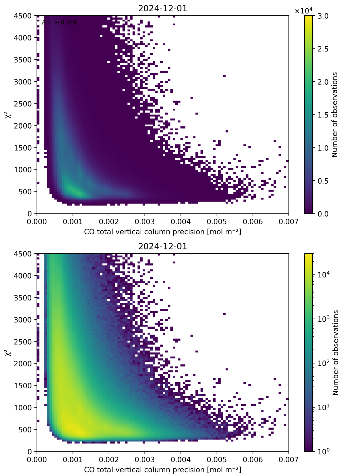
Figure 44: Scatter density plot of “CO total vertical column precision” against “ \chi^2 ” for 2024-11-30 to 2024-12-02.
