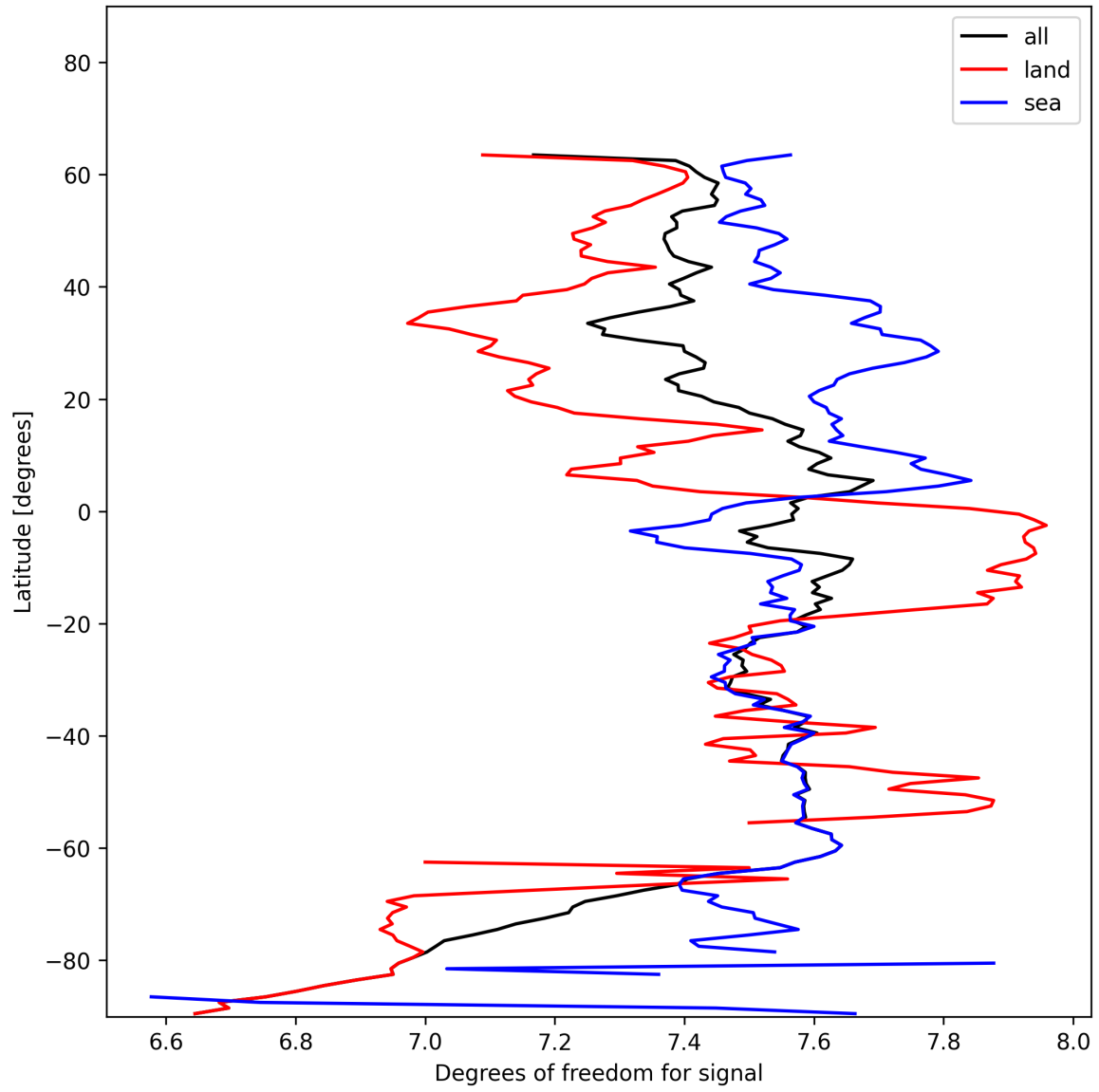
Figure 15: Zonal average of “Degrees of freedom for signal” for 2024-11-30 to 2024-12-02.
