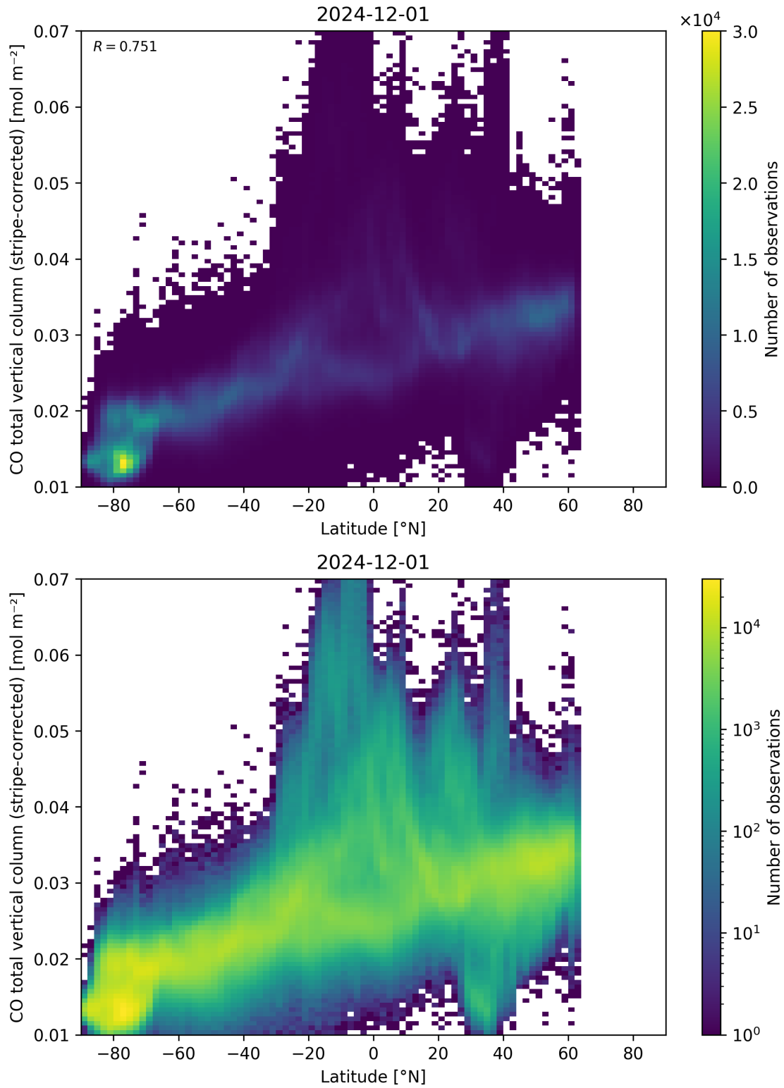
Figure 52: Scatter density plot of “Latitude” against “CO total vertical column (stripe-corrected)” for 2024-11-30 to 2024-12-02.
