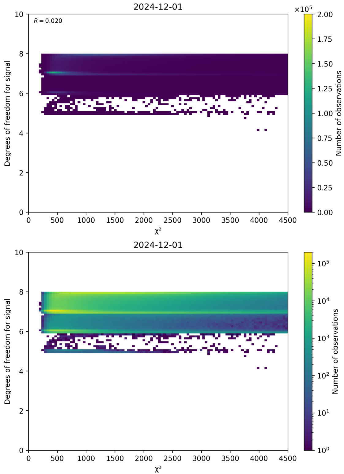
Figure 48: Scatter density plot of “ \chi^2 ” against “Degrees of freedom for signal” for 2024-11-30 to 2024-12-02.
