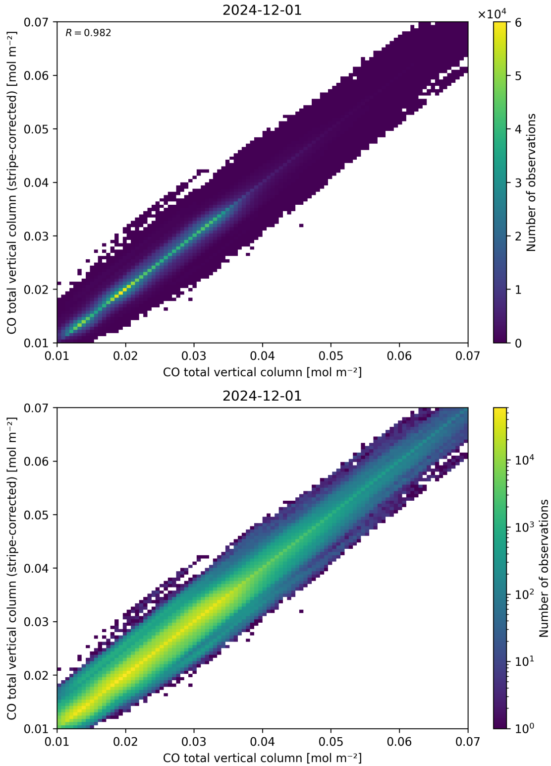
Figure 33: Scatter density plot of “CO total vertical column” against “CO total vertical column (stripe-corrected)” for 2024-11-30 to 2024-12-02.
