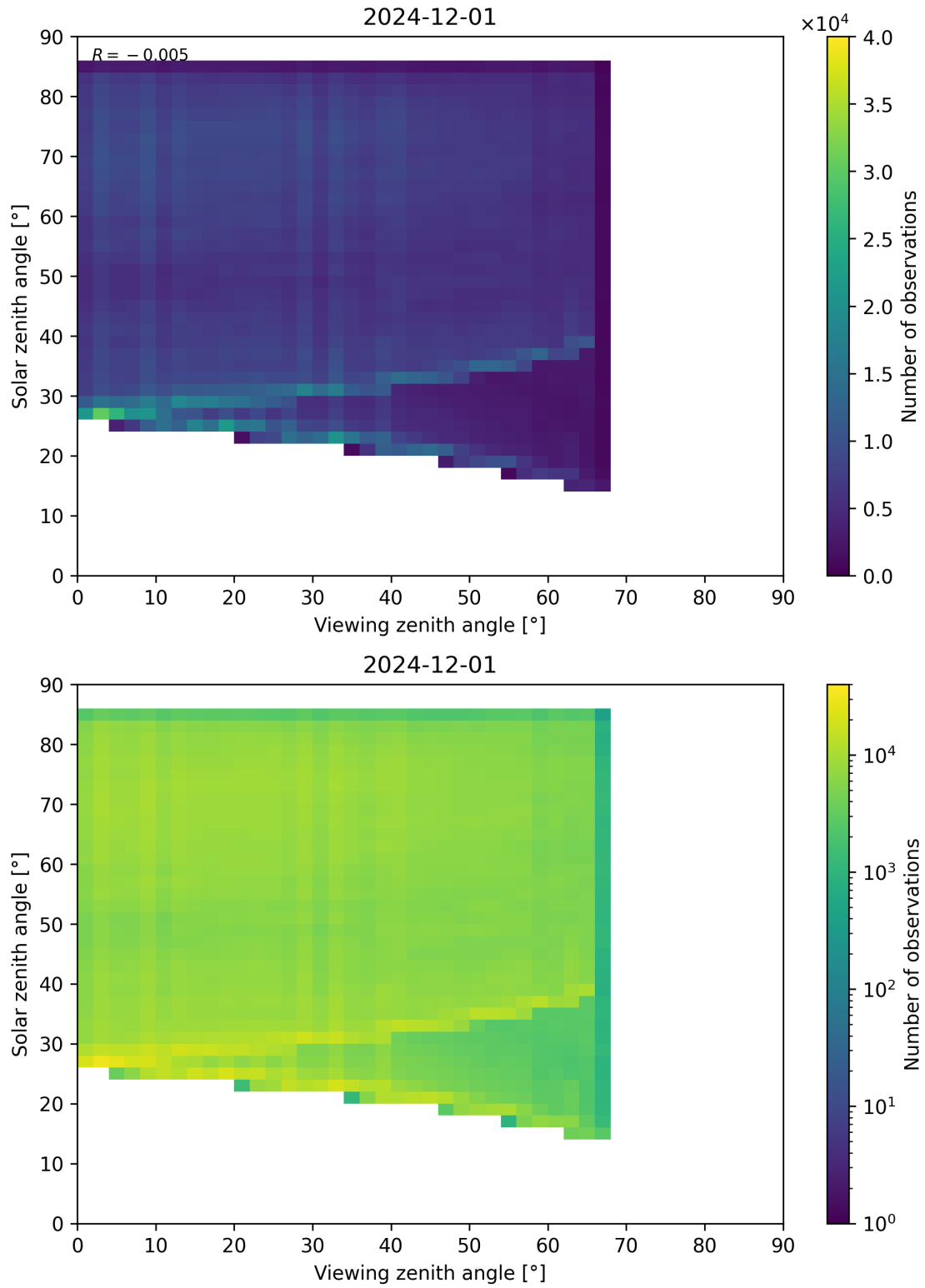
Figure 77: Scatter density plot of “Viewing zenith angle” against “Solar zenith angle” for 2024-11-30 to 2024-12-02.
