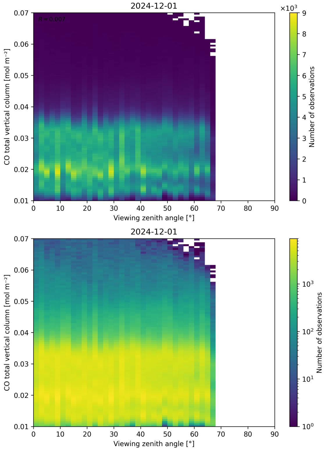
Figure 69: Scatter density plot of “Viewing zenith angle” against “CO total vertical column” for 2024-11-30 to 2024-12-02.
