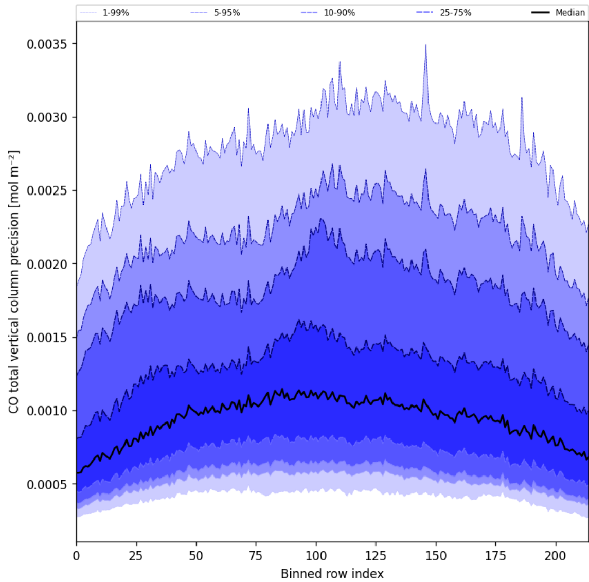
Figure 28: Along track statistics of “CO total vertical column precision” for 2024-11-30 to 2024-12-02
