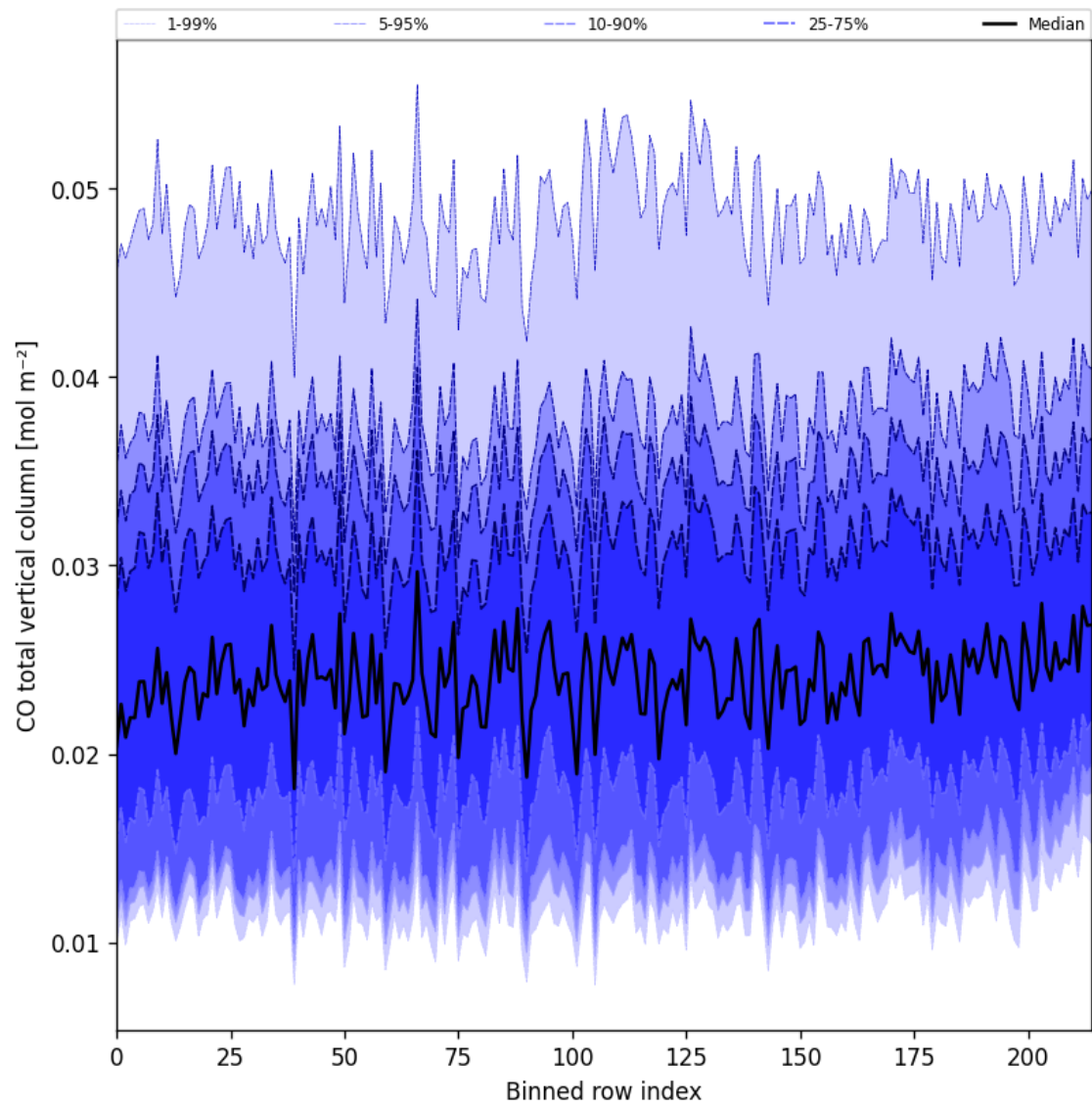
Figure 26: Along track statistics of “CO total vertical column” for 2024-11-30 to 2024-12-02
