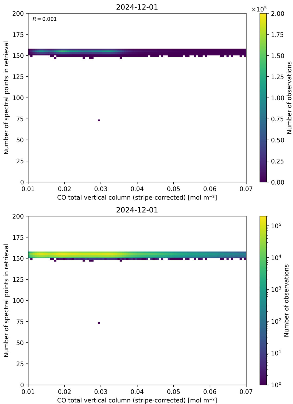
Figure 40: Scatter density plot of “CO total vertical column (stripe-corrected)” against “Number of spectral points in retrieval” for 2024-11-30 to 2024-12-02.
