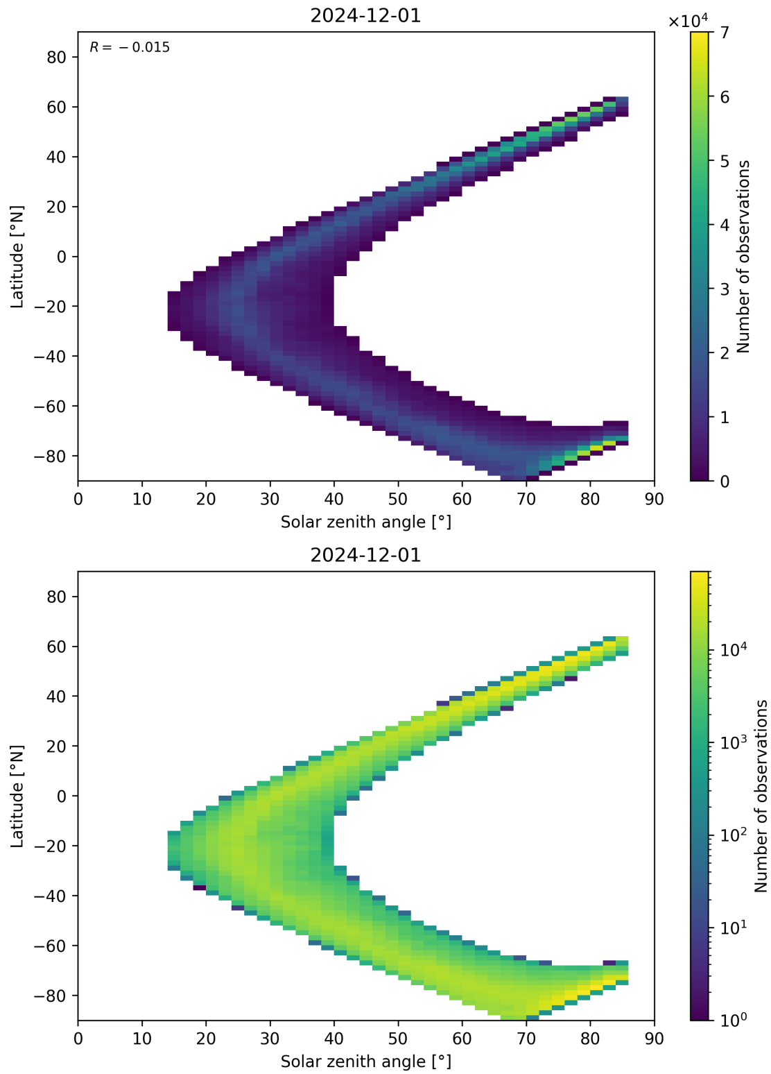
Figure 66: Scatter density plot of “Solar zenith angle” against “Latitude” for 2024-11-30 to 2024-12-02.
