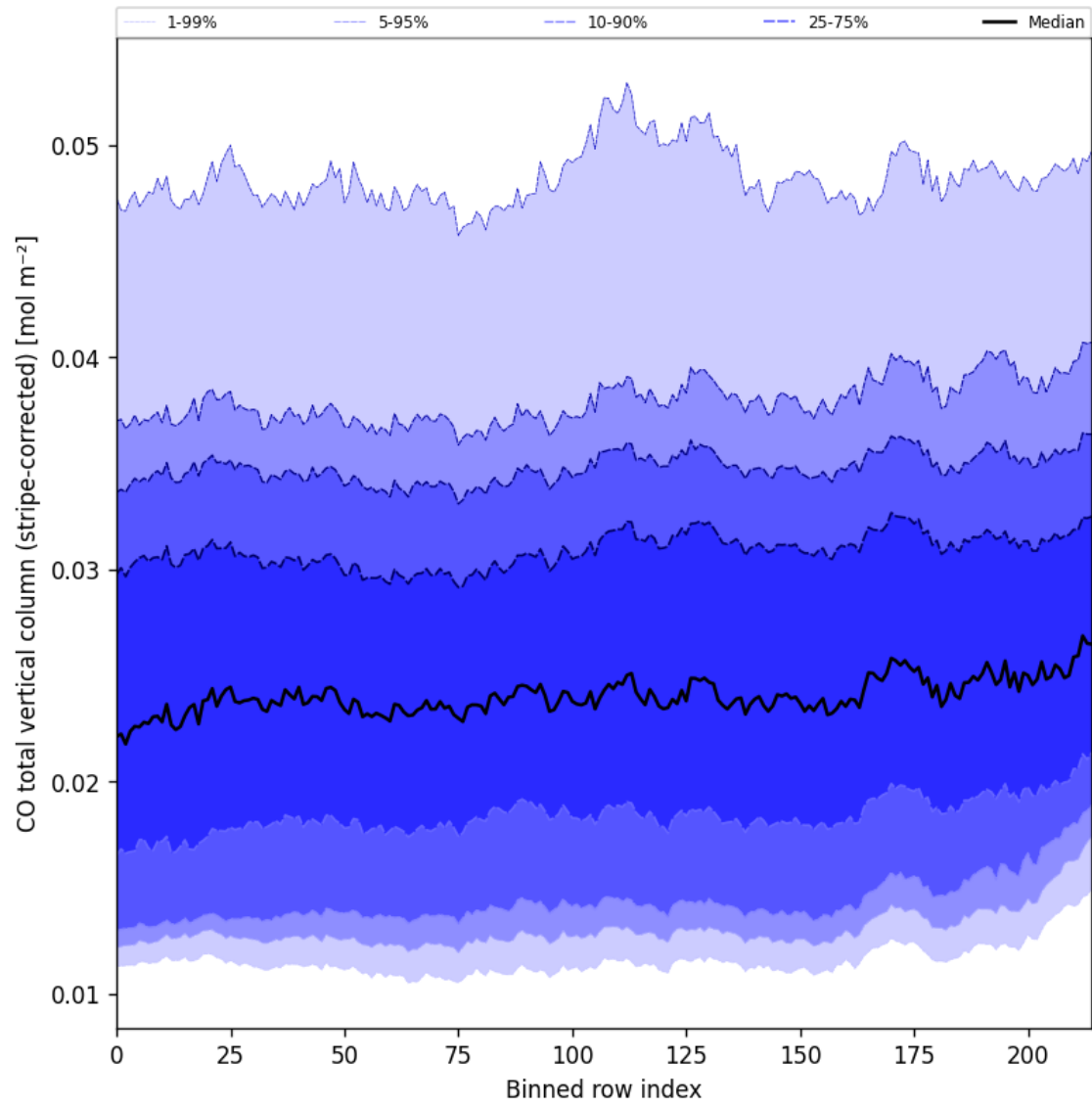
Figure 27: Along track statistics of “CO total vertical column (stripe-corrected)” for 2024-11-30 to 2024-12-02
