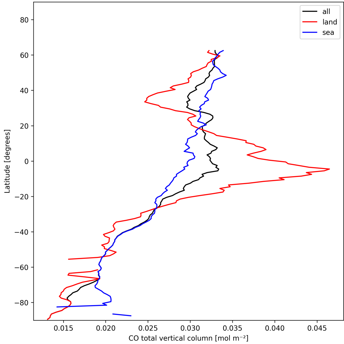
Figure 10: Zonal average of “CO total vertical column” for 2024-12-01 to 2024-12-03.
