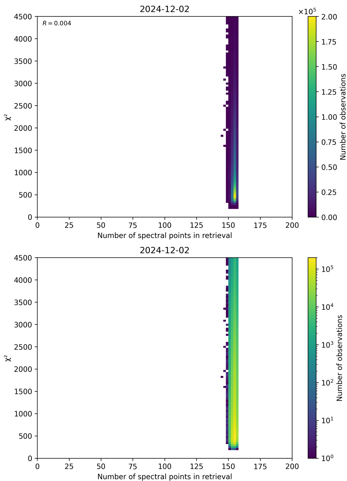
Figure 58: Scatter density plot of “Number of spectral points in retrieval” against “ \chi^2 ” for 2024-12-01 to 2024-12-03.
