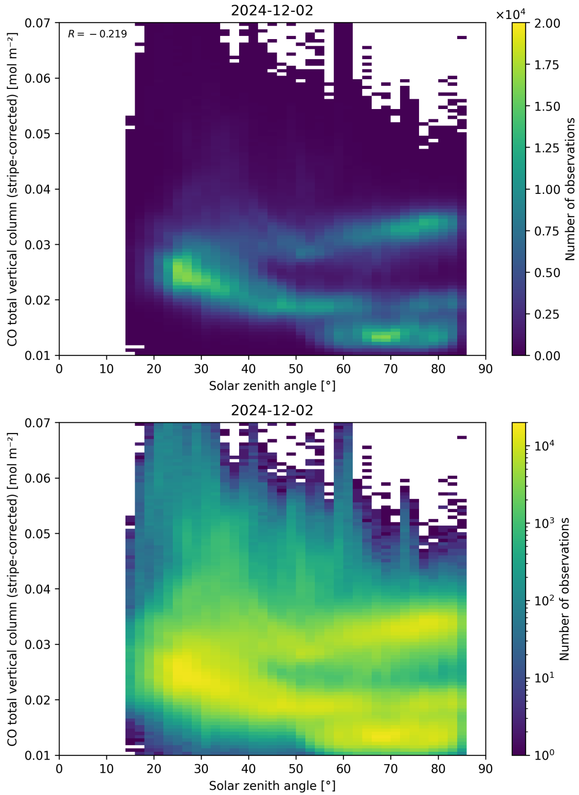
Figure 62: Scatter density plot of “Solar zenith angle” against “CO total vertical column (stripe-corrected)” for 2024-12-01 to 2024-12-03.
