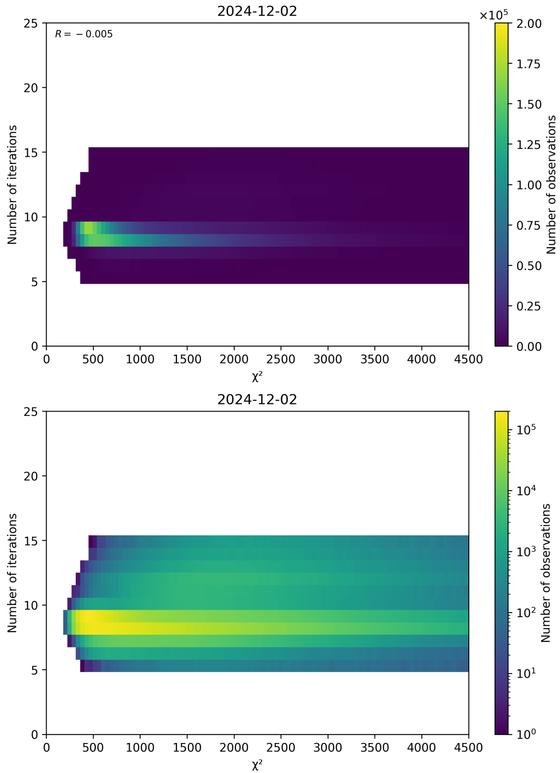
Figure 49: Scatter density plot of “ \chi^2 ” against “Number of iterations” for 2024-12-01 to 2024-12-03.
