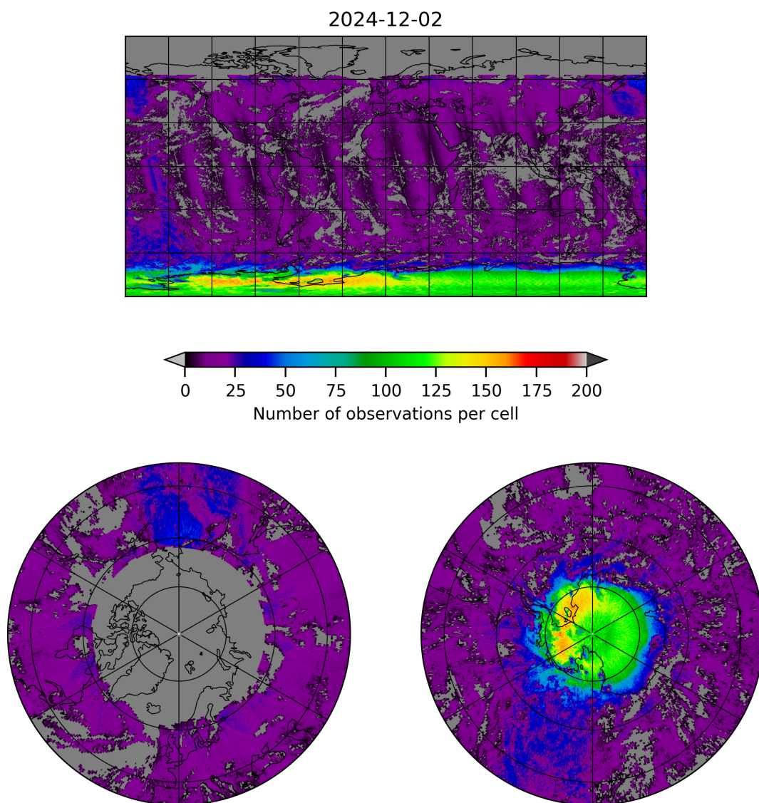
Figure 8: Map of the number of observations for 2024-12-01 to 2024-12-03
