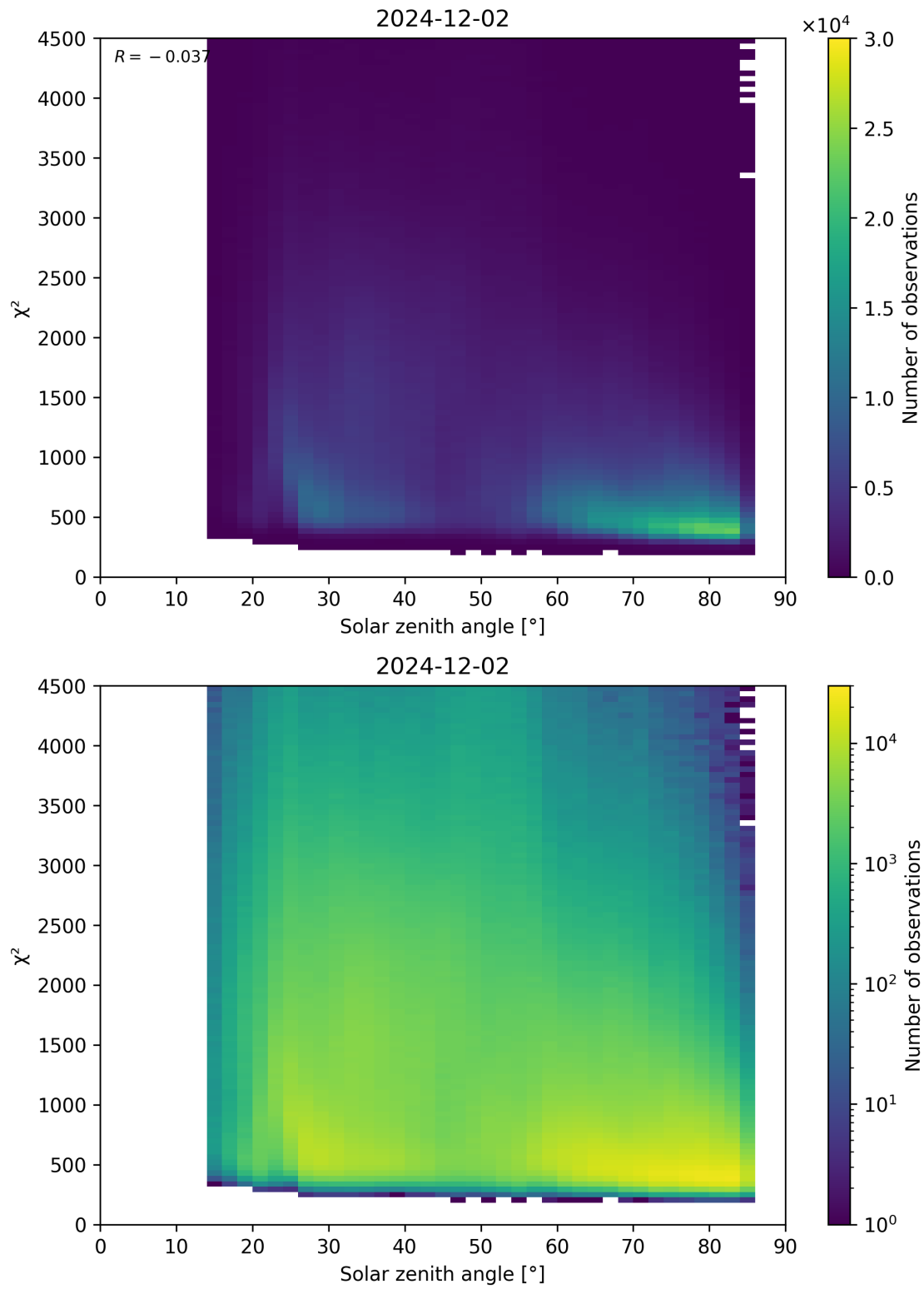
Figure 64: Scatter density plot of “Solar zenith angle” against “ \chi^2 ” for 2024-12-01 to 2024-12-03.
