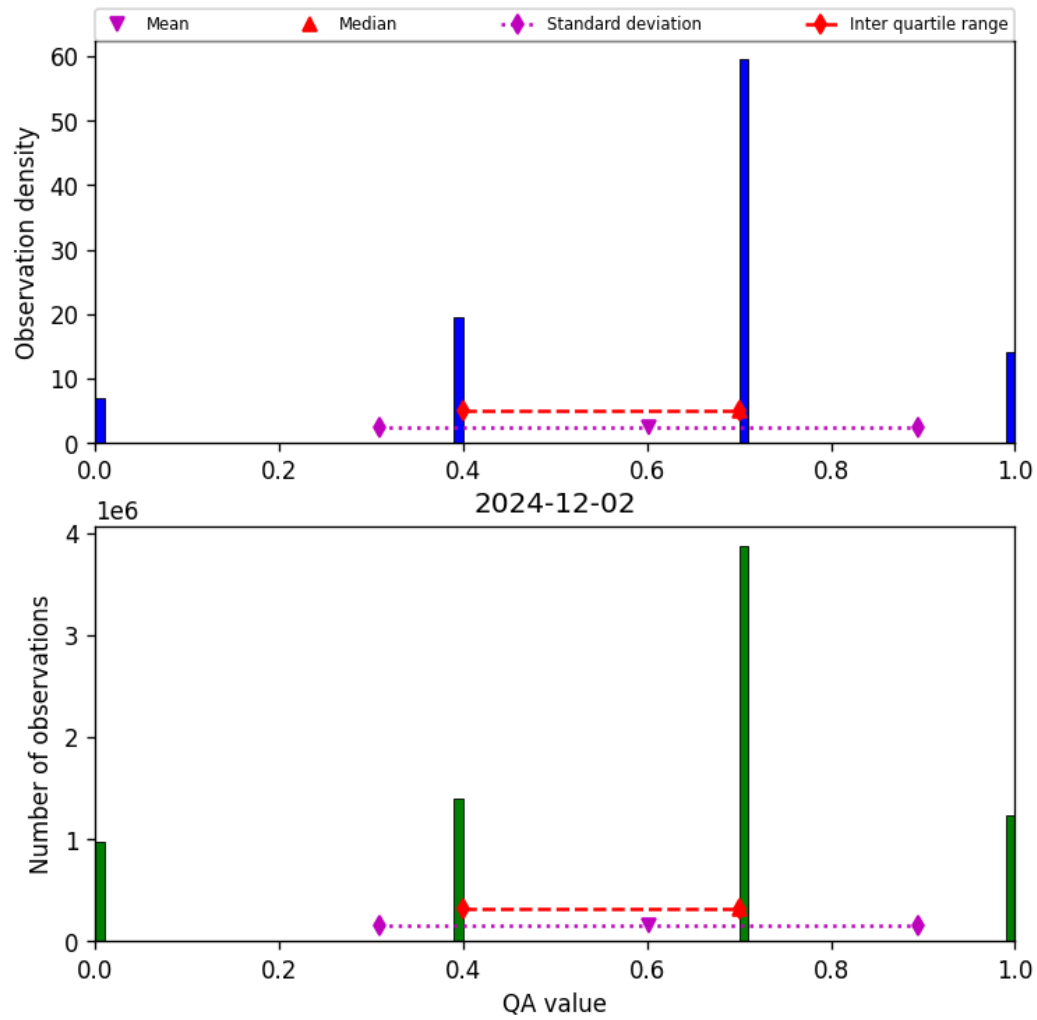
Figure 17: Histogram of “QA value” for 2024-12-01 to 2024-12-03
