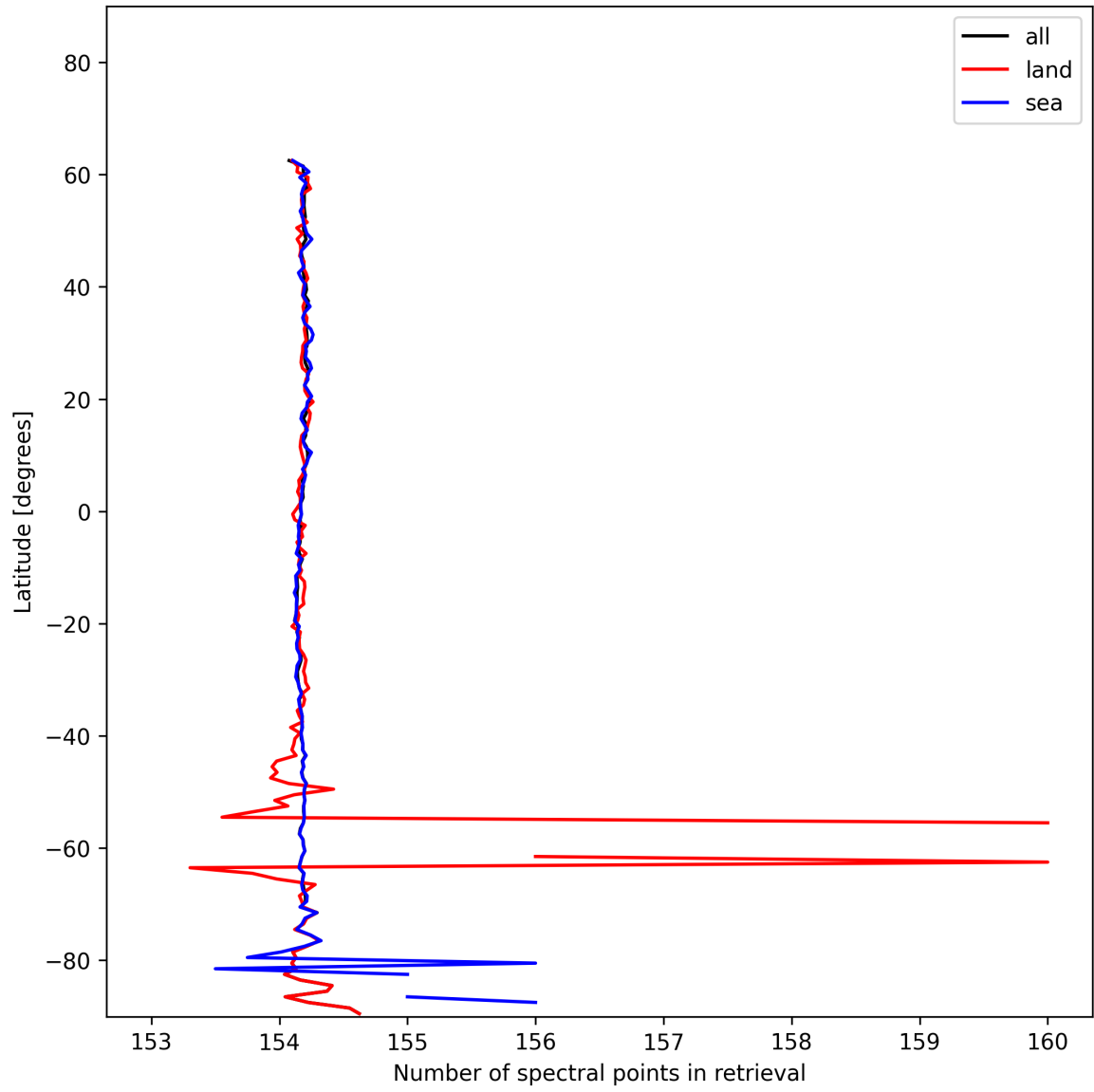
Figure 13: Zonal average of “Number of spectral points in retrieval” for 2024-12-01 to 2024-12-03.
