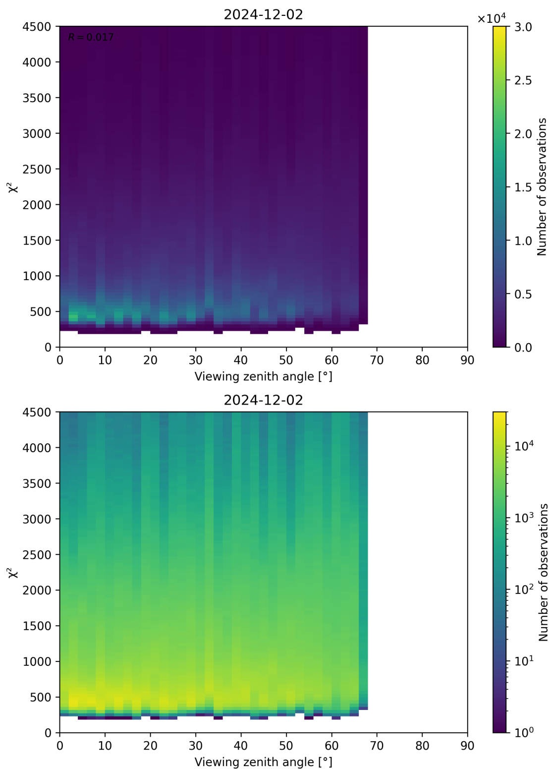
Figure 72: Scatter density plot of “Viewing zenith angle” against “ \chi^2 ” for 2024-12-01 to 2024-12-03.
