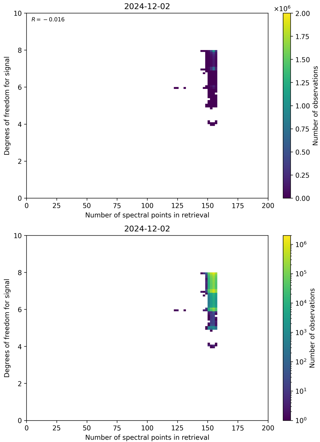
Figure 59: Scatter density plot of “Number of spectral points in retrieval” against “Degrees of freedom for signal” for 2024-12-01 to 2024-12-03.
