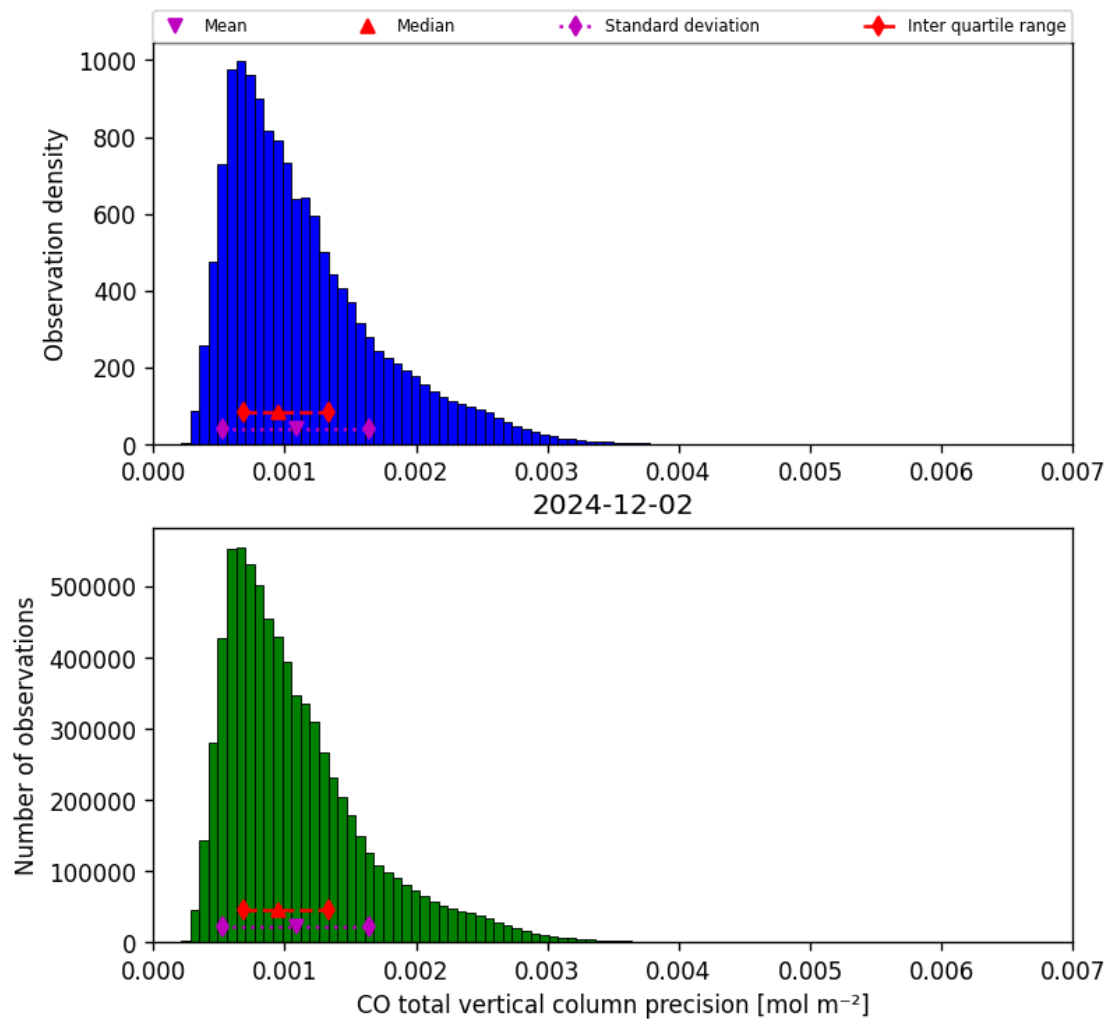
Figure 20: Histogram of “CO total vertical column precision” for 2024-12-01 to 2024-12-03
