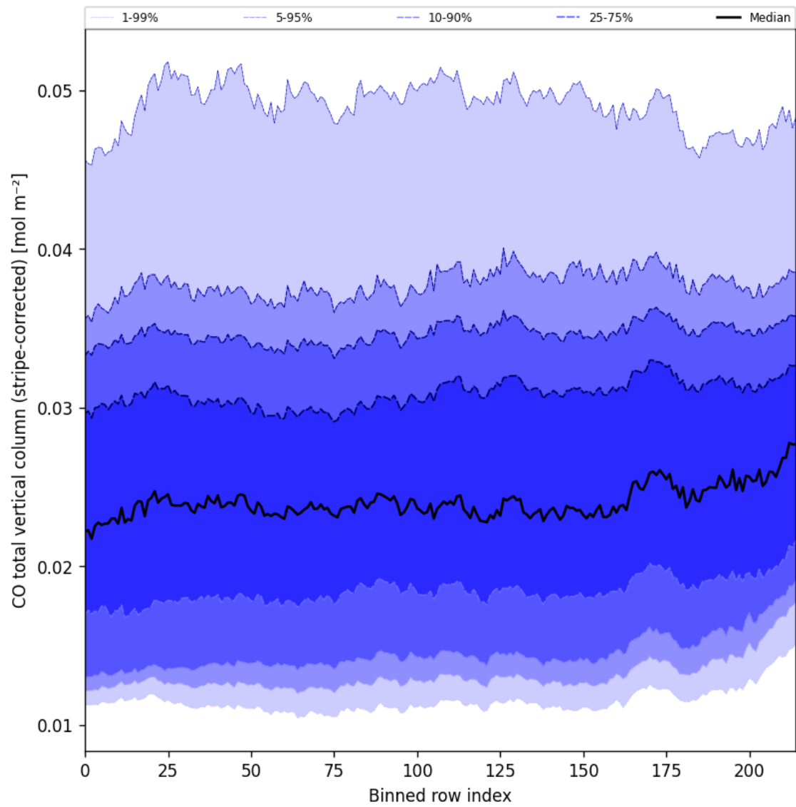
Figure 27: Along track statistics of “CO total vertical column (stripe-corrected)” for 2024-12-01 to 2024-12-03
