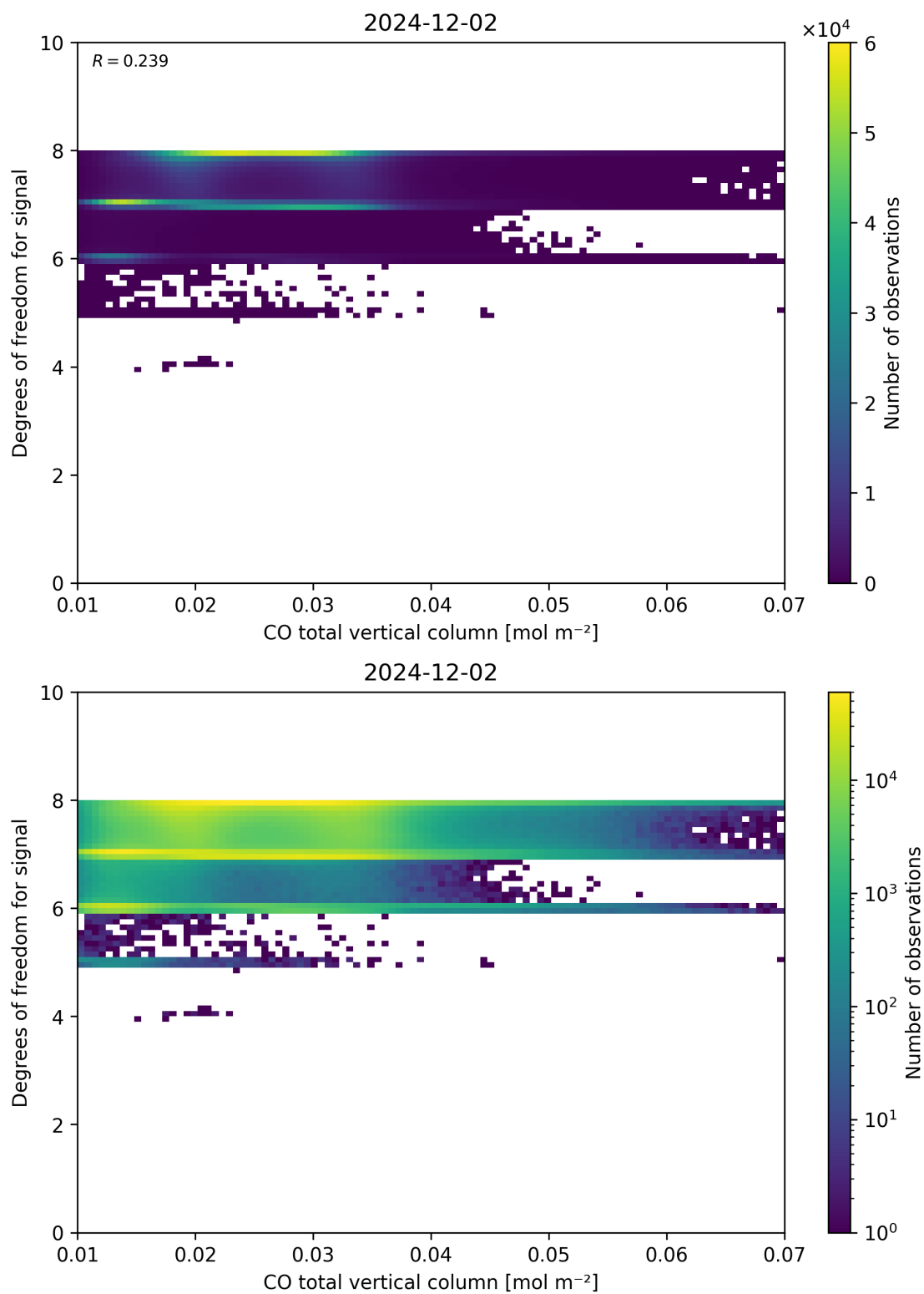
Figure 41: Scatter density plot of “CO total vertical column” against “Degrees of freedom for signal” for 2024-12-01 to 2024-12-03.
