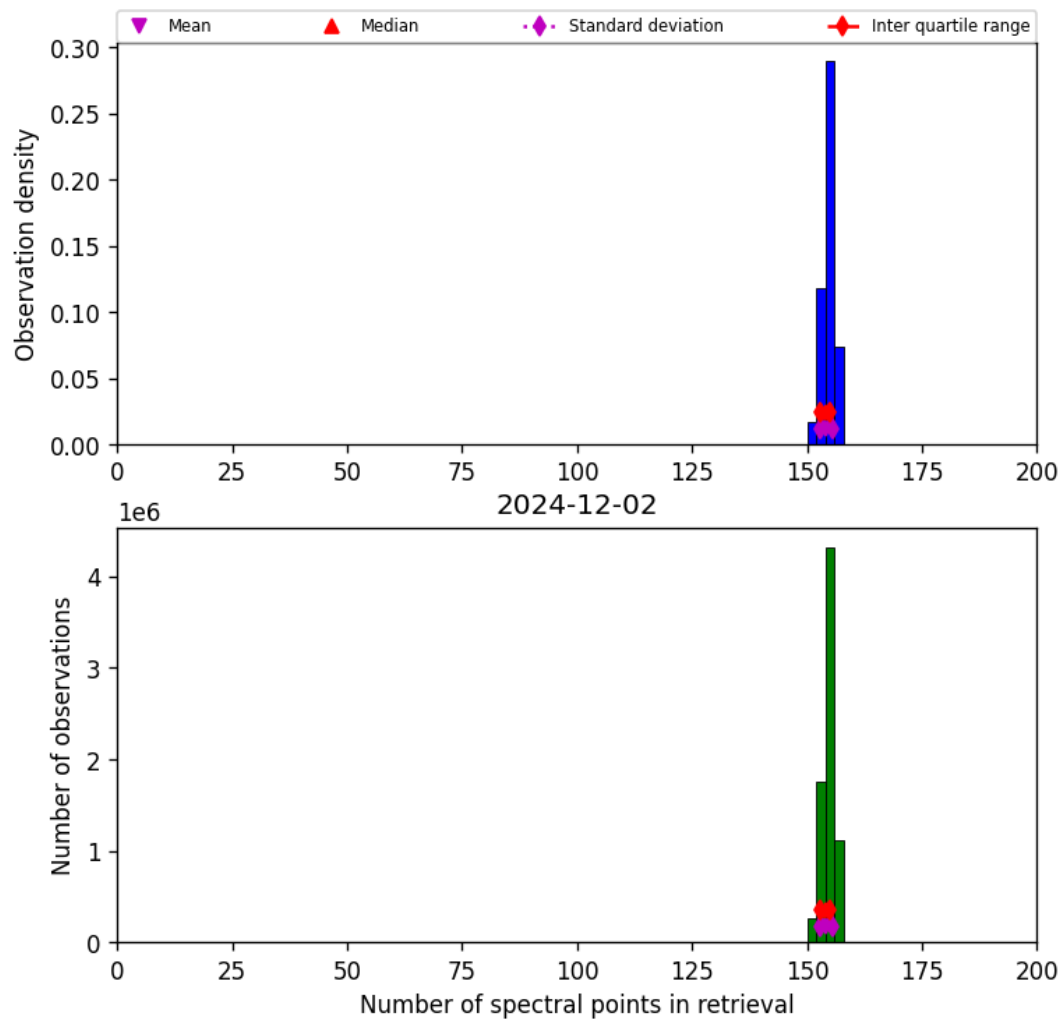
Figure 21: Histogram of “Number of spectral points in retrieval” for 2024-12-01 to 2024-12-03
