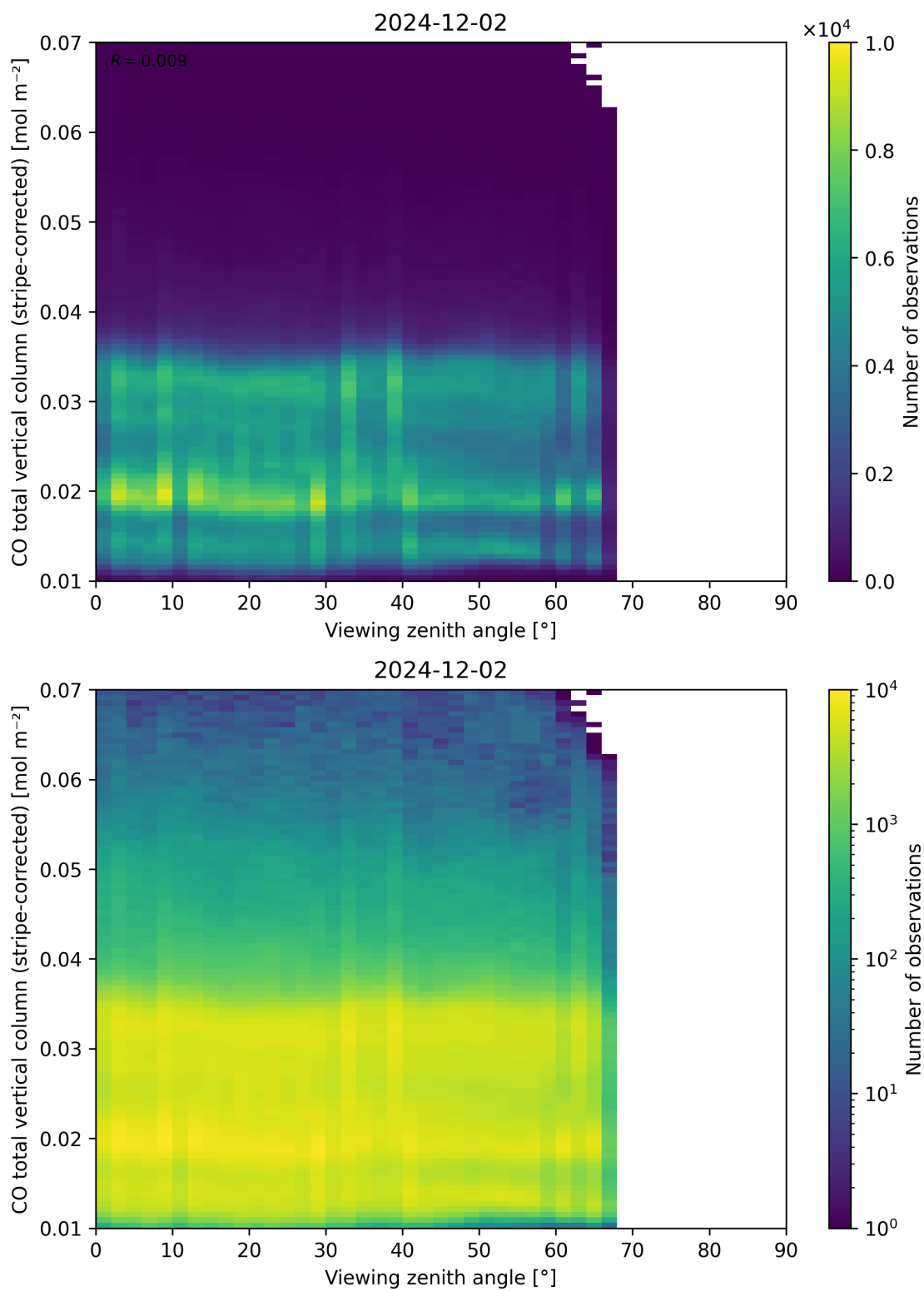
Figure 70: Scatter density plot of “Viewing zenith angle” against “CO total vertical column (stripe-corrected)” for 2024-12-01 to 2024-12-03.
