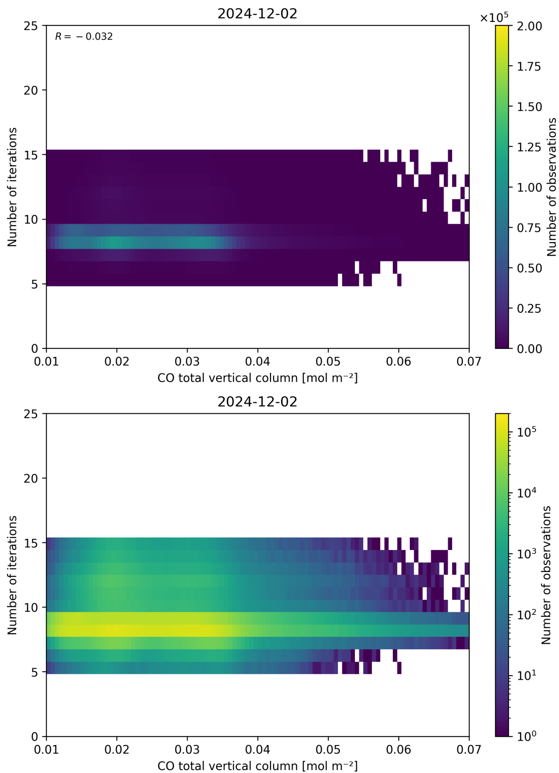
Figure 42: Scatter density plot of “CO total vertical column” against “Number of iterations” for 2024-12-01 to 2024-12-03.
