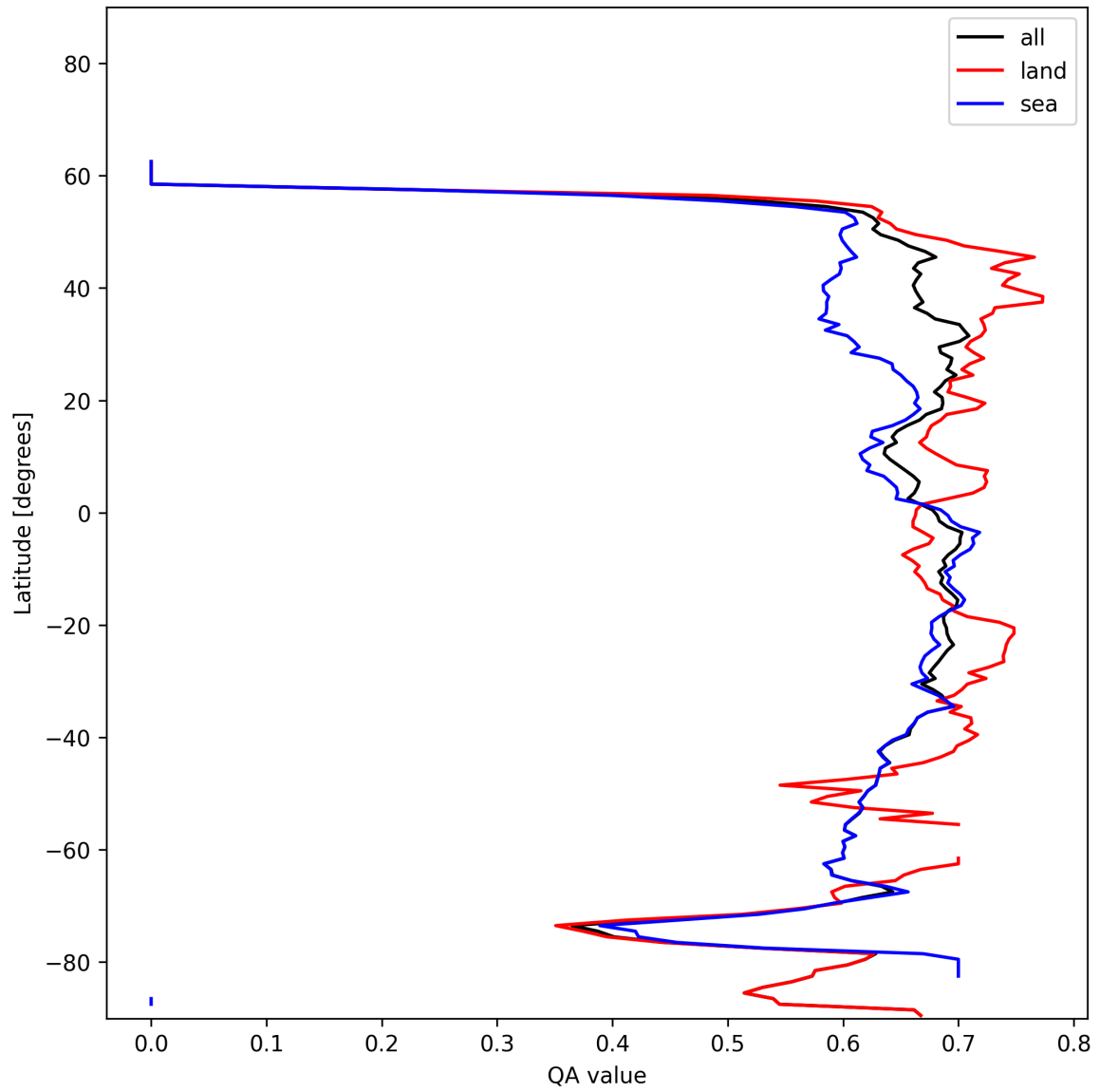
Figure 9: Zonal average of “QA value” for 2024-12-01 to 2024-12-03.
