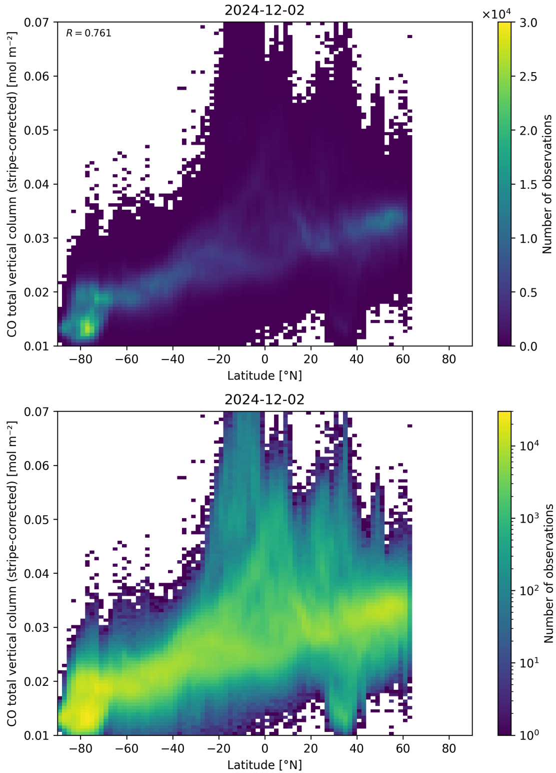
Figure 52: Scatter density plot of “Latitude” against “CO total vertical column (stripe-corrected)” for 2024-12-01 to 2024-12-03.
