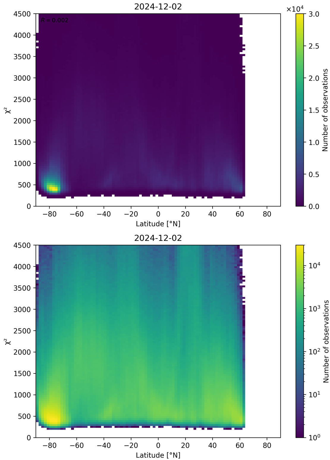
Figure 54: Scatter density plot of “Latitude” against “ \chi^2 ” for 2024-12-01 to 2024-12-03.
