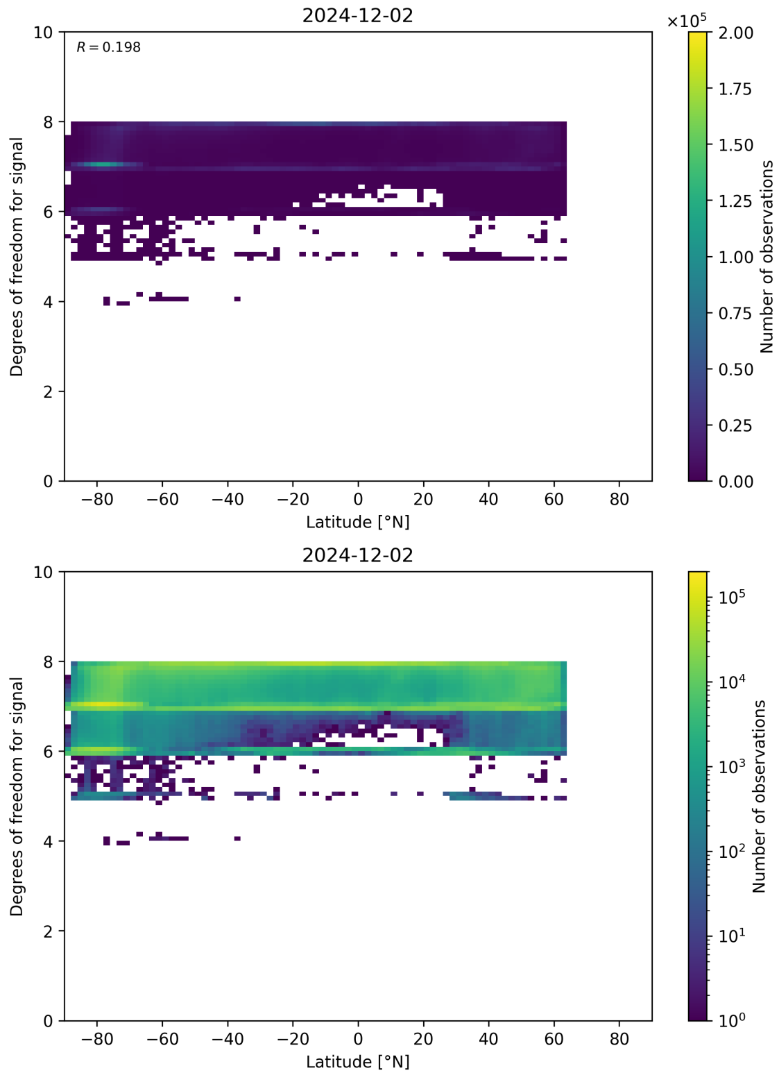
Figure 55: Scatter density plot of “Latitude” against “Degrees of freedom for signal” for 2024-12-01 to 2024-12-03.
