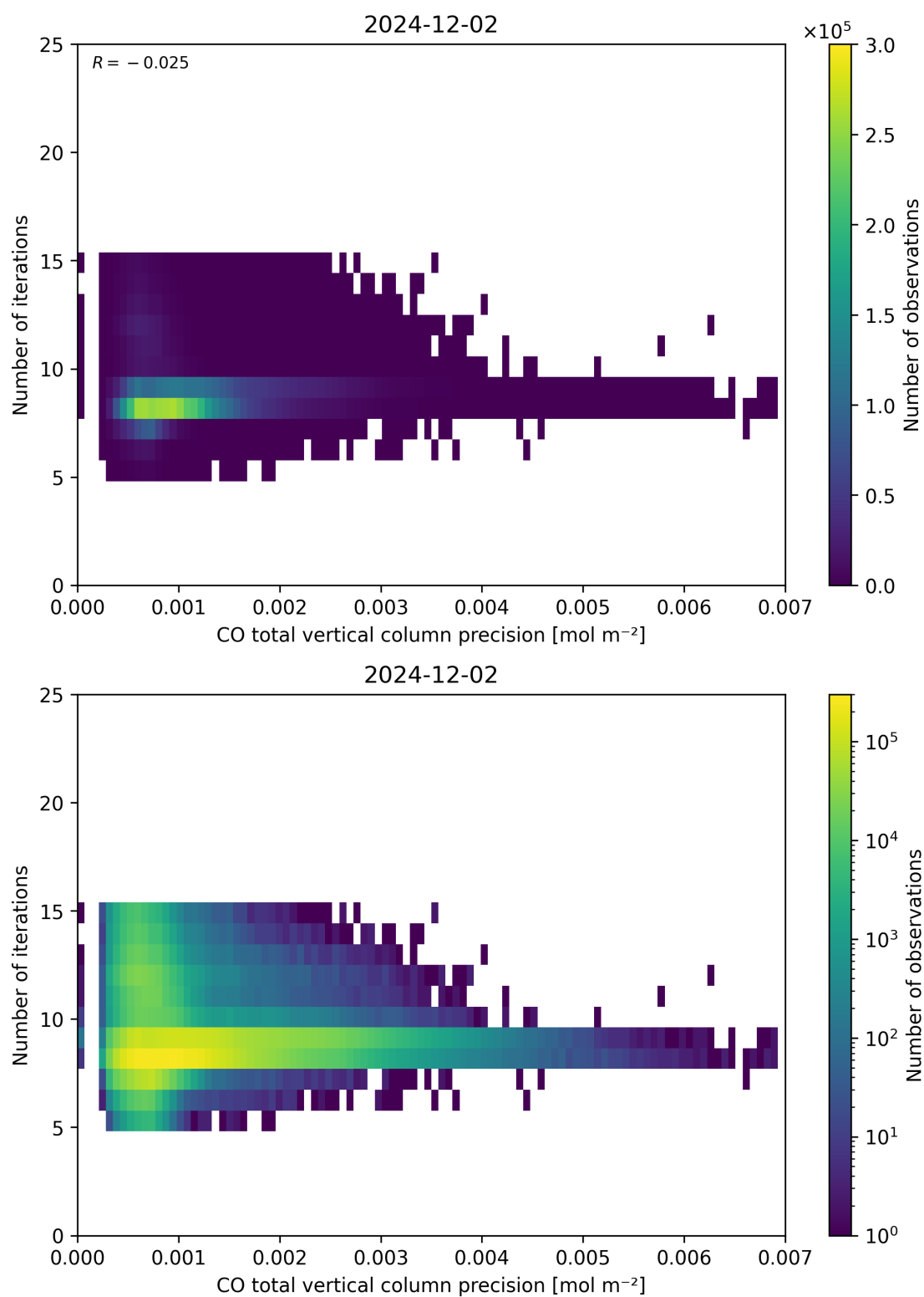
Figure 46: Scatter density plot of “CO total vertical column precision” against “Number of iterations” for 2024-12-01 to 2024-12-03.
