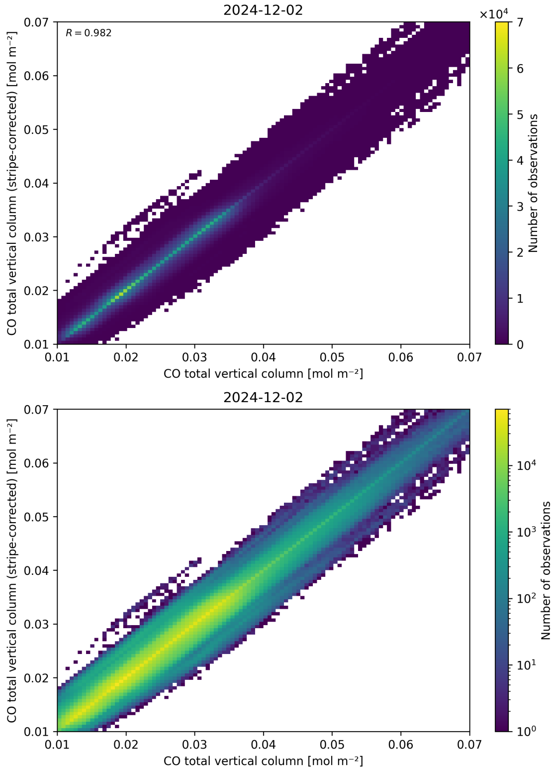
Figure 33: Scatter density plot of “CO total vertical column” against “CO total vertical column (stripe-corrected)” for 2024-12-01 to 2024-12-03.
