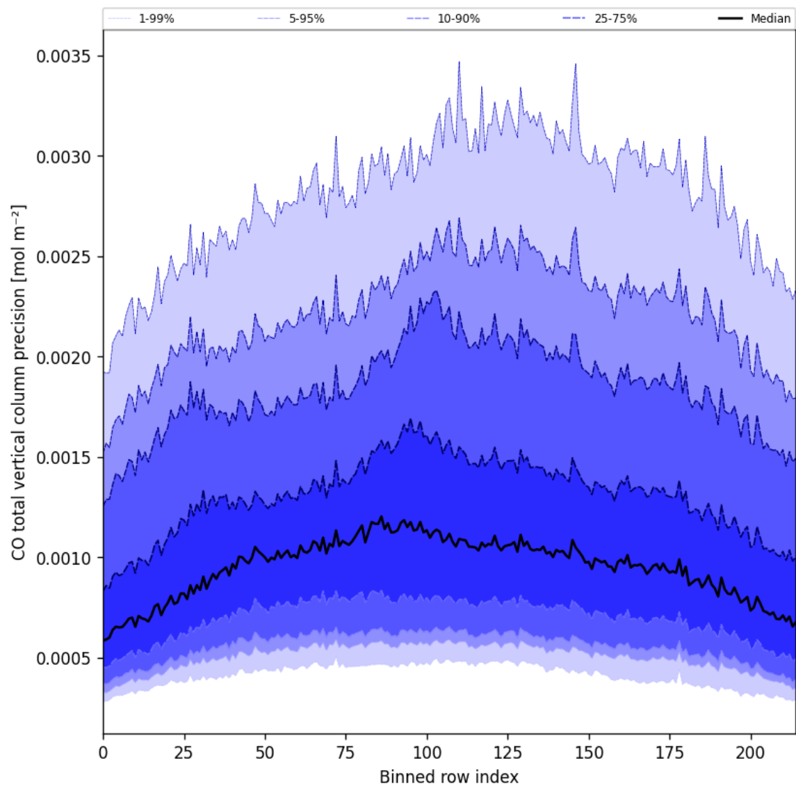
Figure 28: Along track statistics of “CO total vertical column precision” for 2024-12-01 to 2024-12-03
