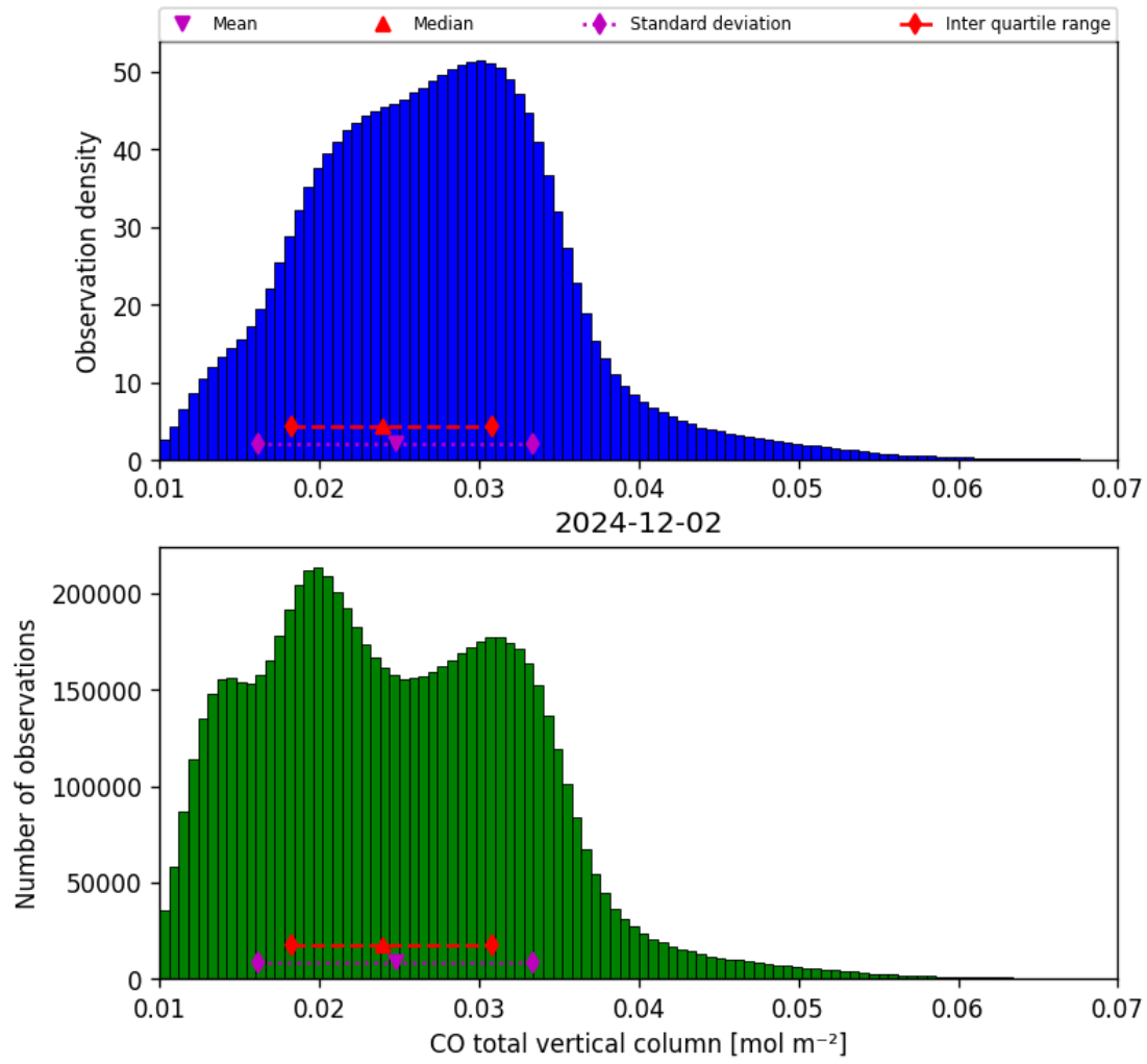
Figure 18: Histogram of “CO total vertical column” for 2024-12-01 to 2024-12-03
