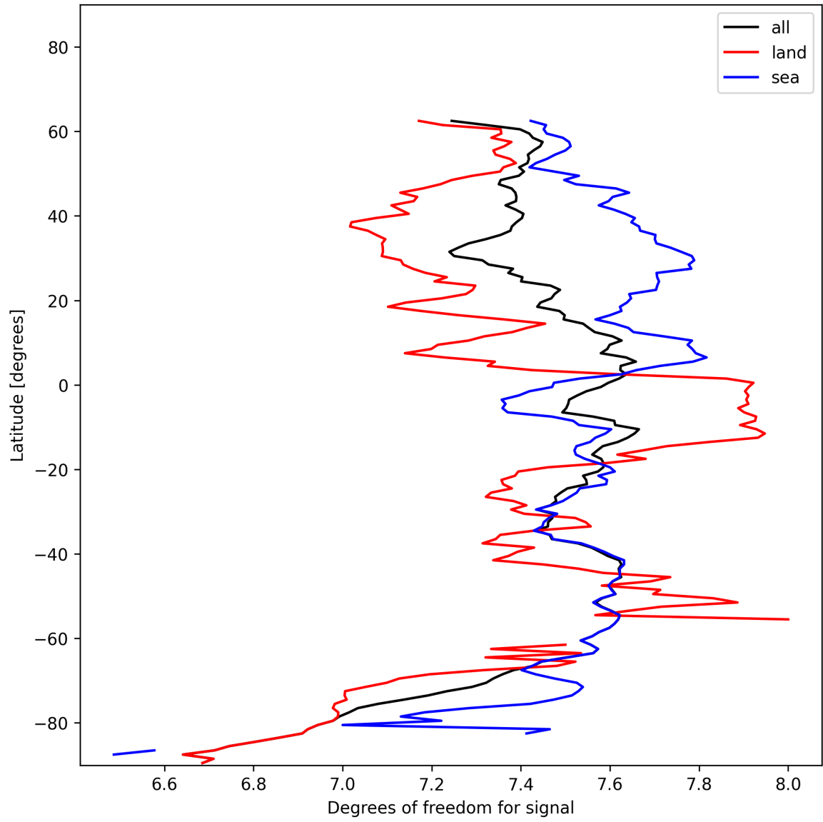
Figure 15: Zonal average of “Degrees of freedom for signal” for 2024-12-01 to 2024-12-03.
