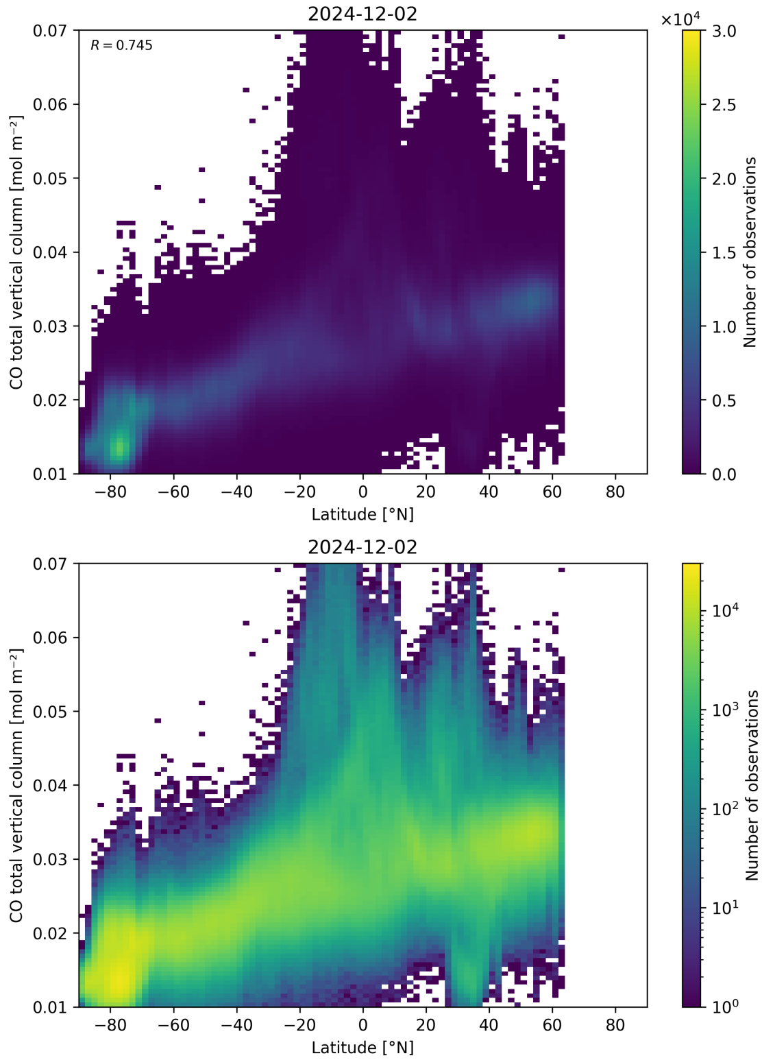
Figure 51: Scatter density plot of “Latitude” against “CO total vertical column” for 2024-12-01 to 2024-12-03.
