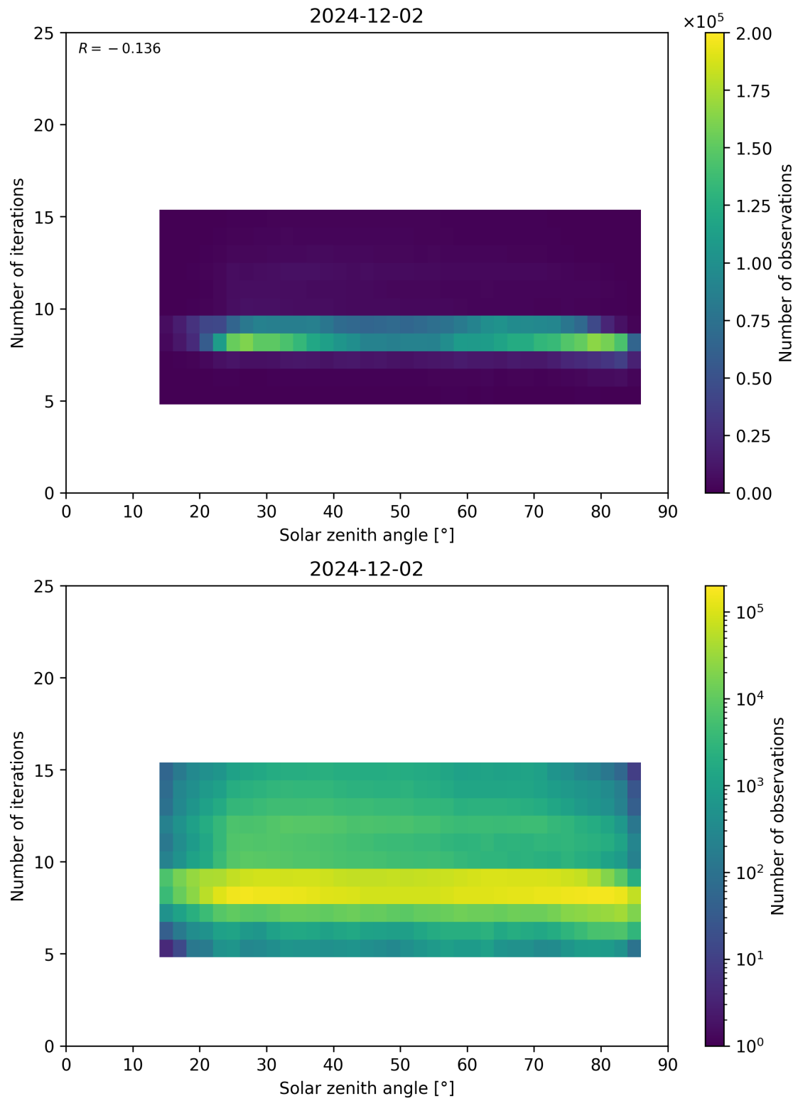
Figure 67: Scatter density plot of “Solar zenith angle” against “Number of iterations” for 2024-12-01 to 2024-12-03.
