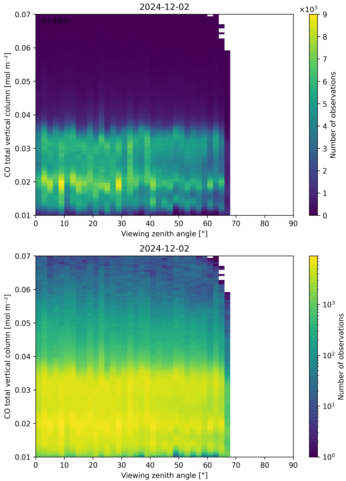
Figure 69: Scatter density plot of “Viewing zenith angle” against “CO total vertical column” for 2024-12-01 to 2024-12-03.
