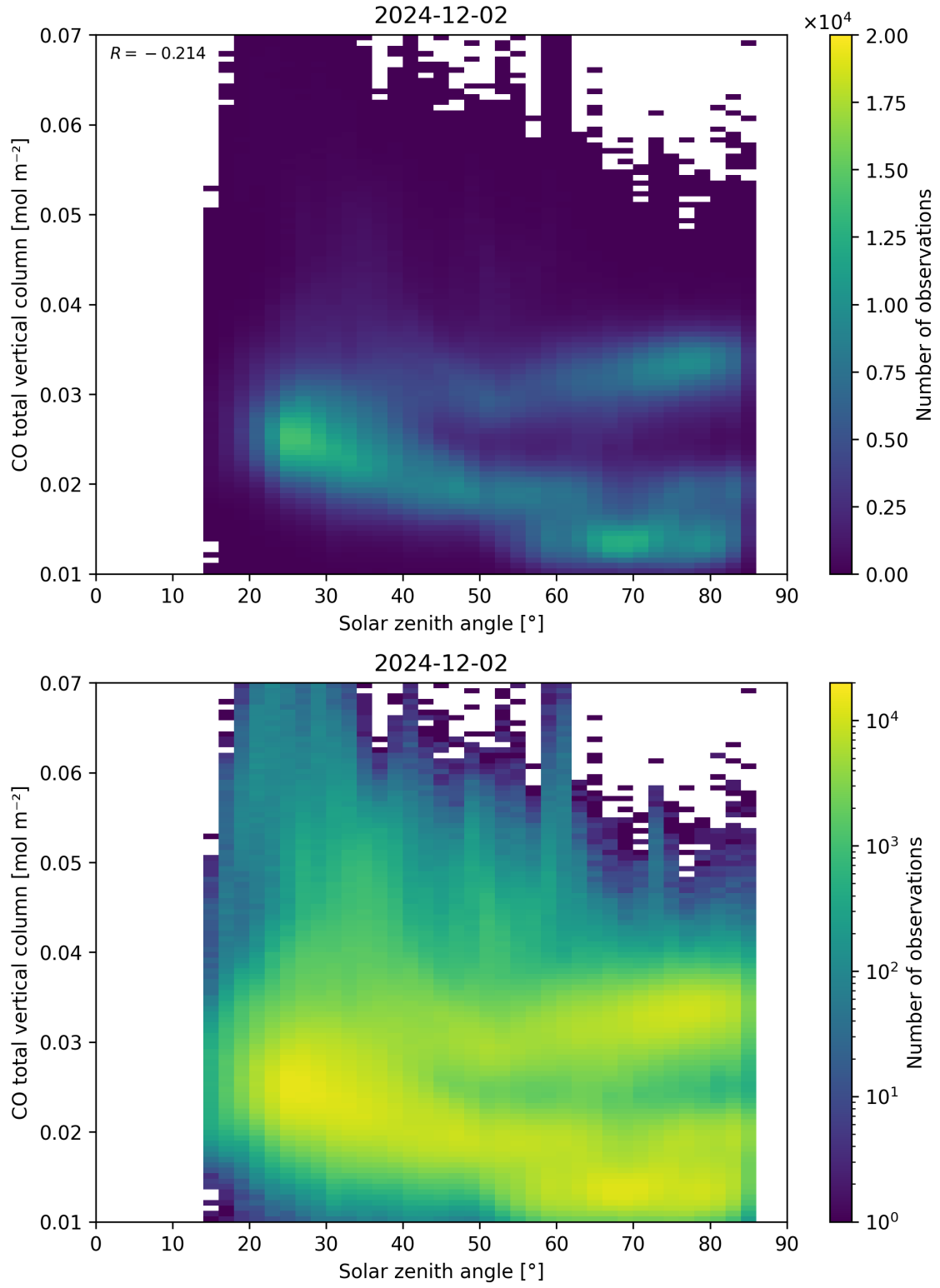
Figure 61: Scatter density plot of “Solar zenith angle” against “CO total vertical column” for 2024-12-01 to 2024-12-03.
