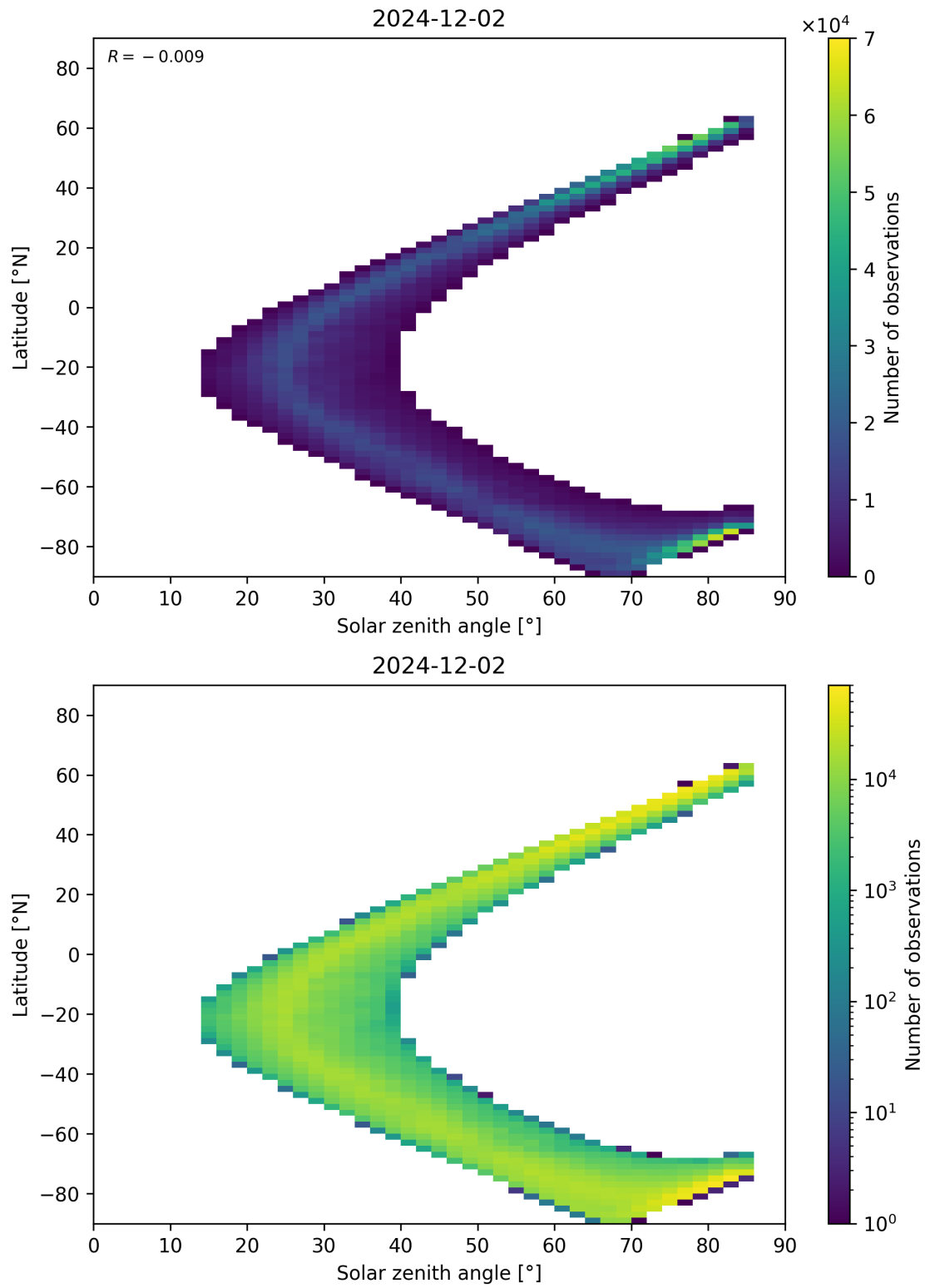
Figure 66: Scatter density plot of “Solar zenith angle” against “Latitude” for 2024-12-01 to 2024-12-03.
