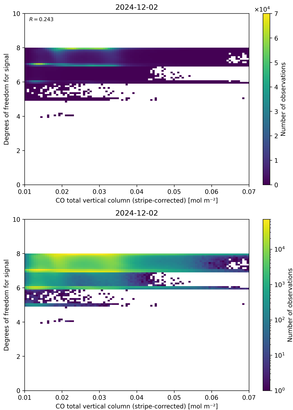
Figure 38: Scatter density plot of “CO total vertical column (stripe-corrected)” against “Degrees of freedom for signal” for 2024-12-01 to 2024-12-03.
