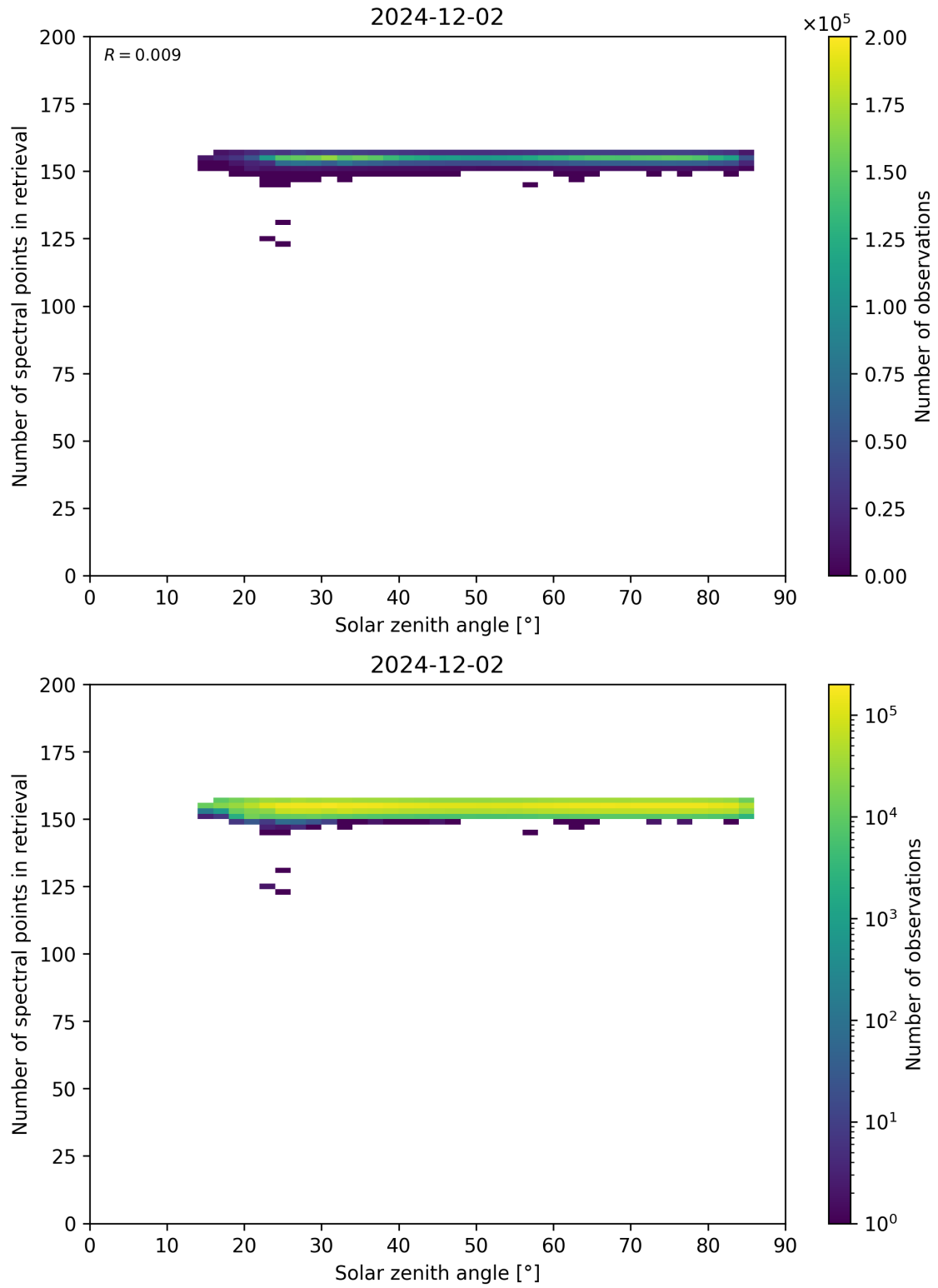
Figure 68: Scatter density plot of “Solar zenith angle” against “Number of spectral points in retrieval” for 2024-12-01 to 2024-12-03.
