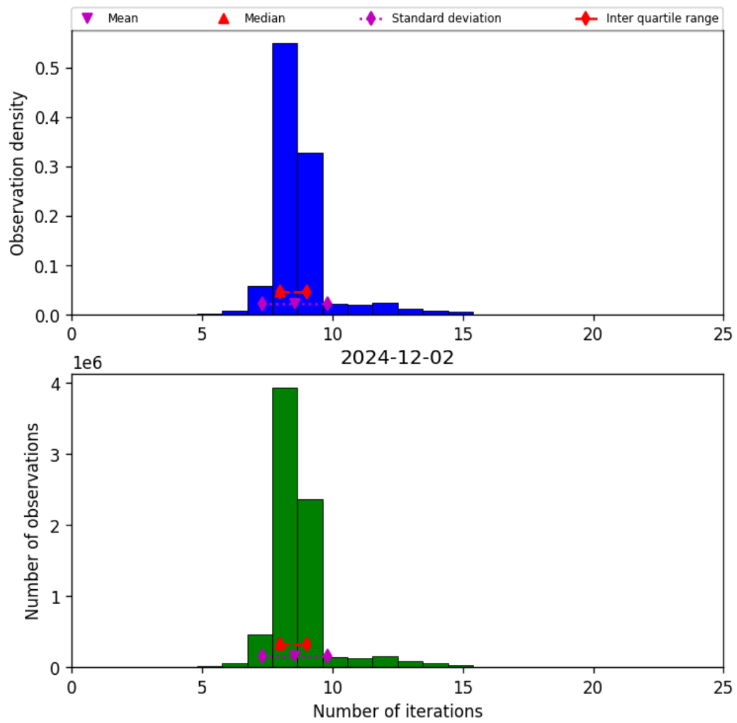
Figure 24: Histogram of “Number of iterations” for 2024-12-01 to 2024-12-03
