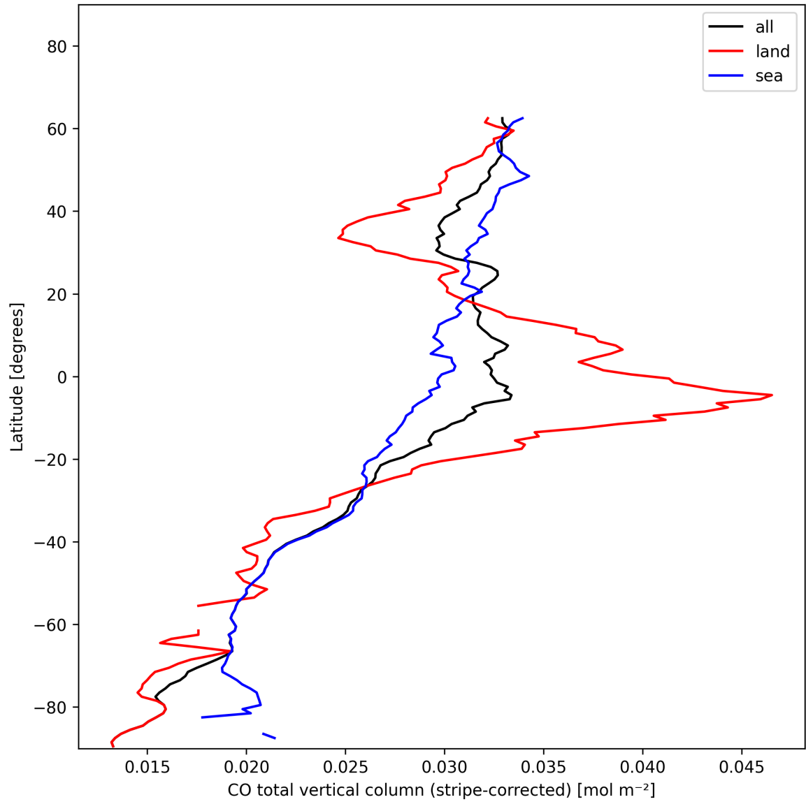
Figure 11: Zonal average of “CO total vertical column (stripe-corrected)” for 2024-12-01 to 2024-12-03.
