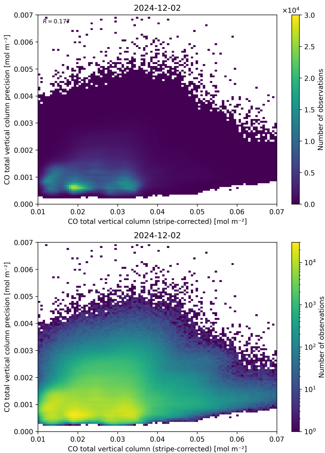
Figure 36: Scatter density plot of “CO total vertical column (stripe-corrected)” against “CO total vertical column precision” for 2024-12-01 to 2024-12-03.
