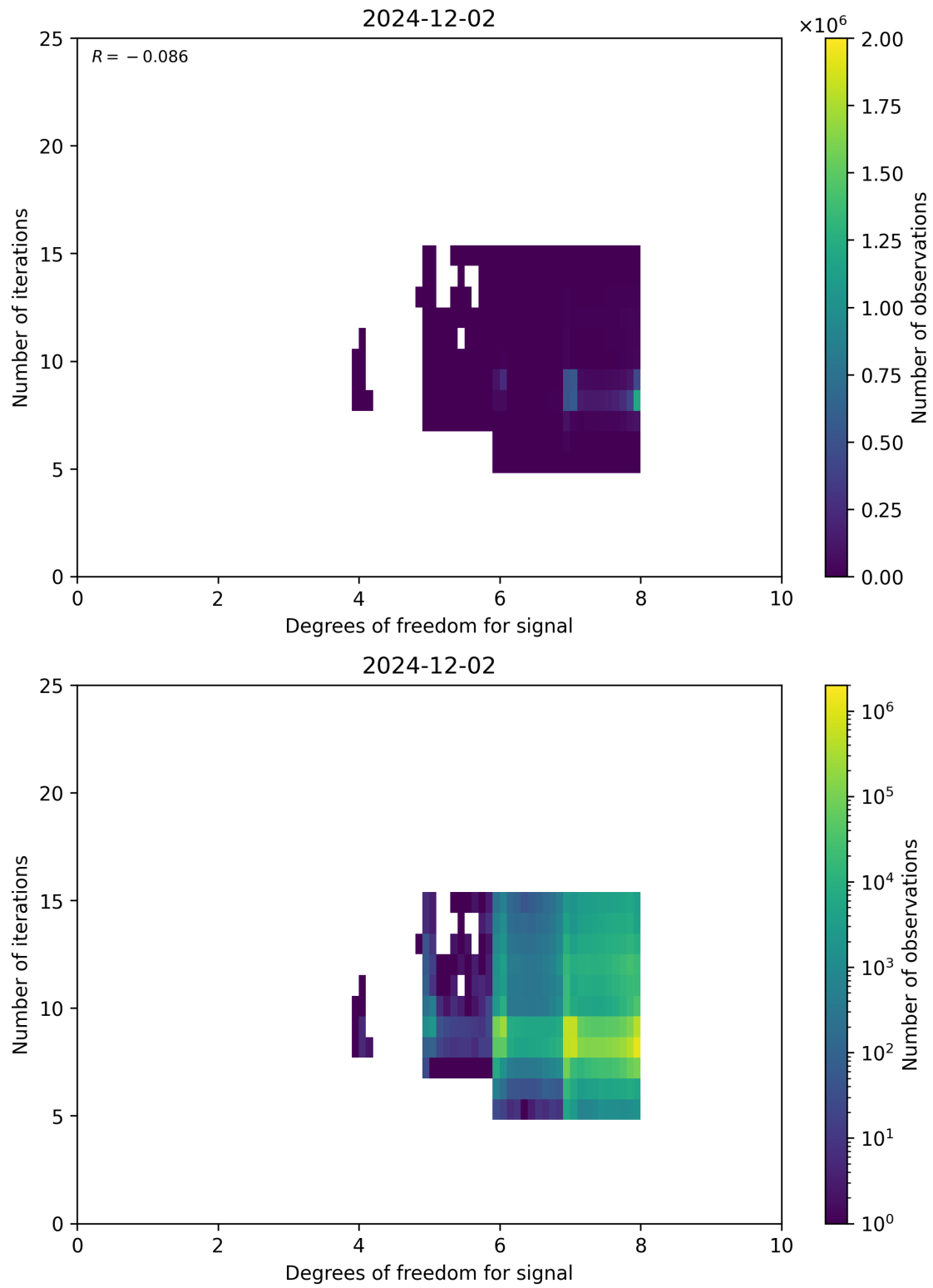
Figure 50: Scatter density plot of “Degrees of freedom for signal” against “Number of iterations” for 2024-12-01 to 2024-12-03.
