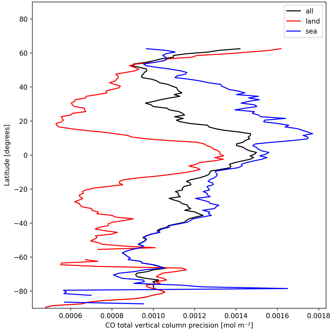
Figure 12: Zonal average of “CO total vertical column precision” for 2024-12-01 to 2024-12-03.
