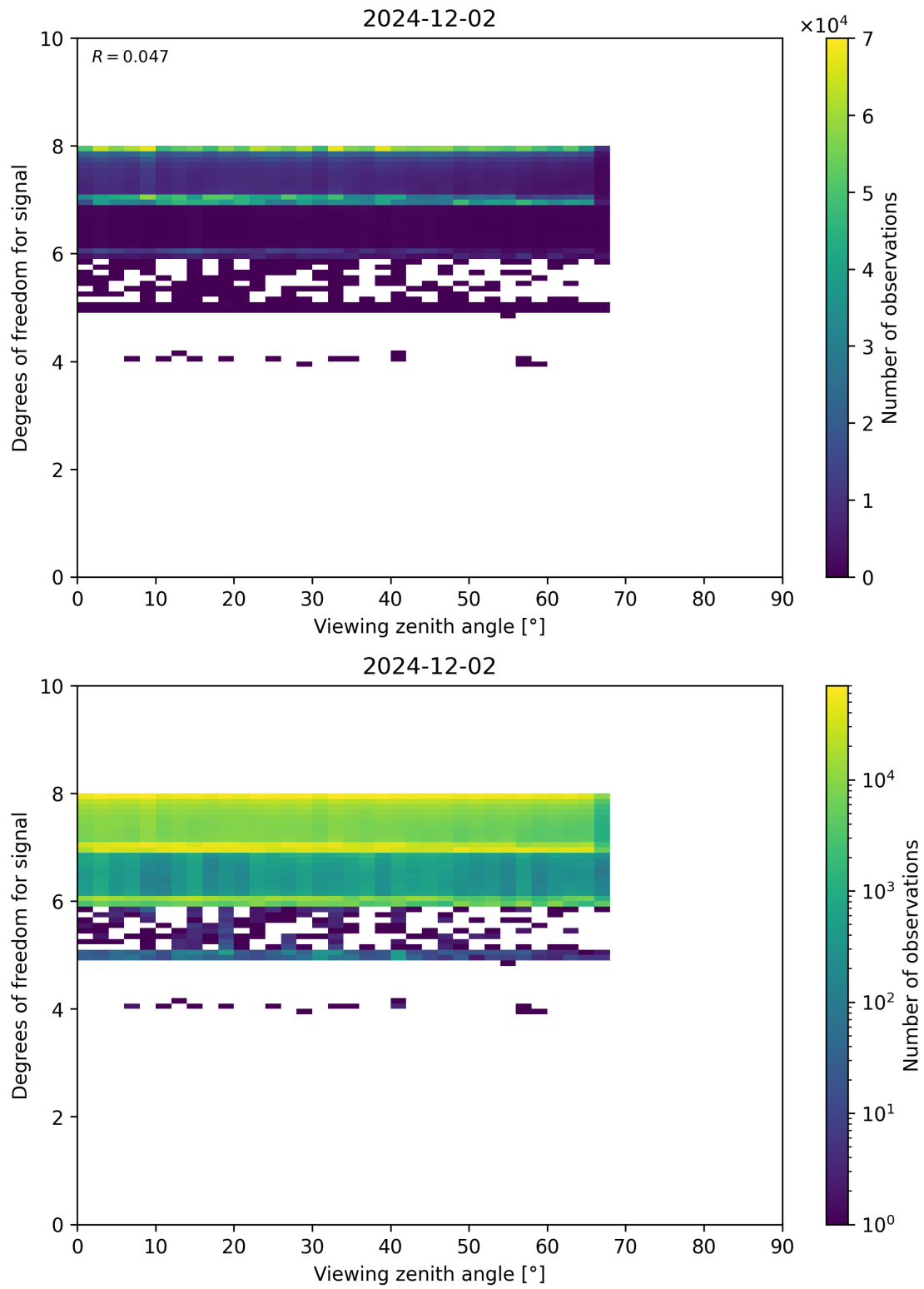
Figure 73: Scatter density plot of “Viewing zenith angle” against “Degrees of freedom for signal” for 2024-12-01 to 2024-12-03.
