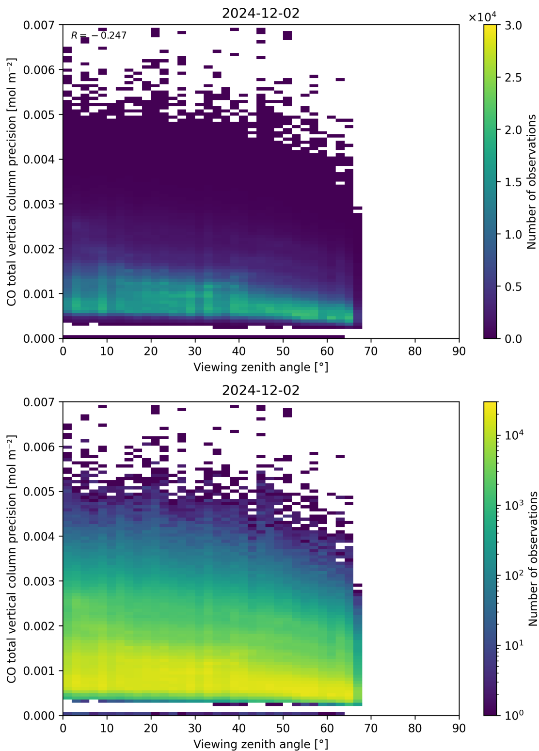
Figure 71: Scatter density plot of “Viewing zenith angle” against “CO total vertical column precision” for 2024-12-01 to 2024-12-03.
