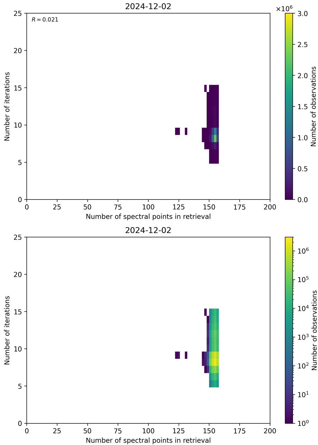
Figure 60: Scatter density plot of “Number of spectral points in retrieval” against “Number of iterations” for 2024-12-01 to 2024-12-03.
