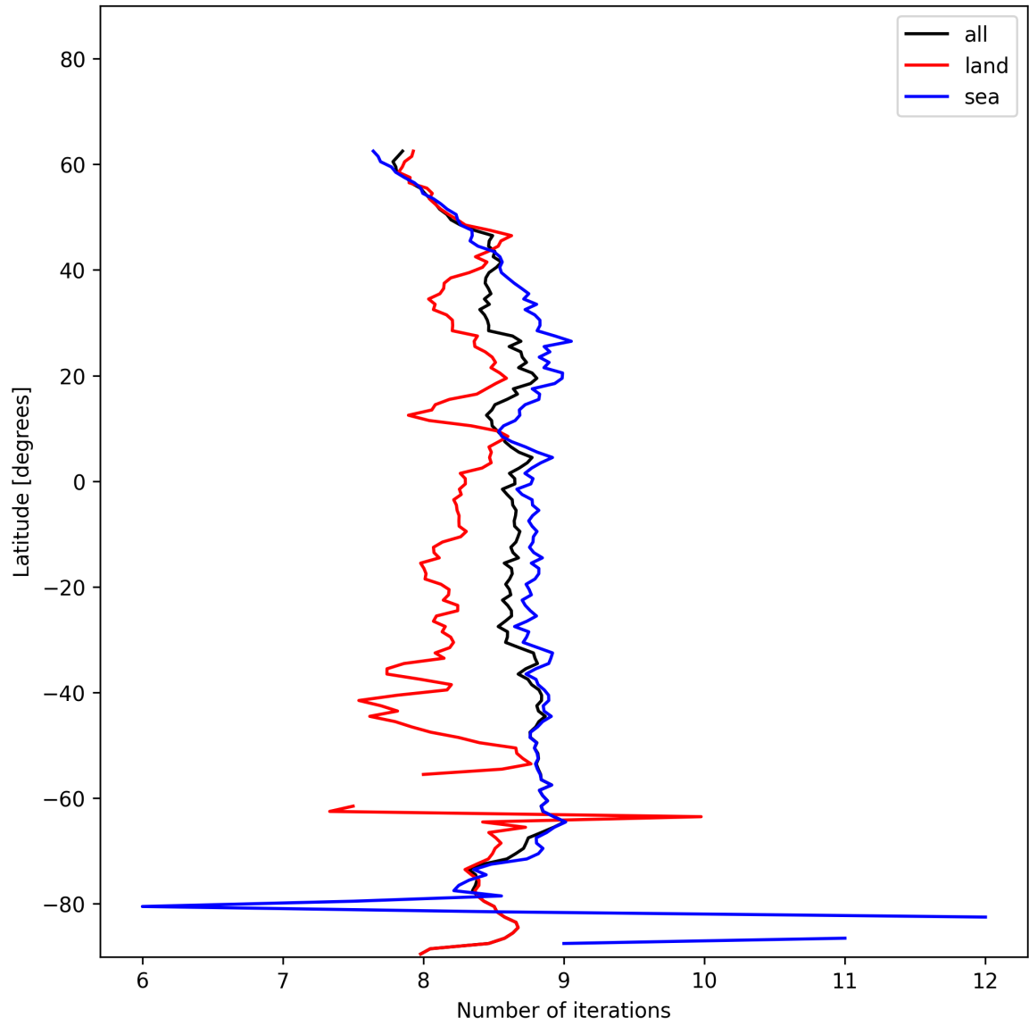
Figure 16: Zonal average of “Number of iterations” for 2024-12-01 to 2024-12-03.
