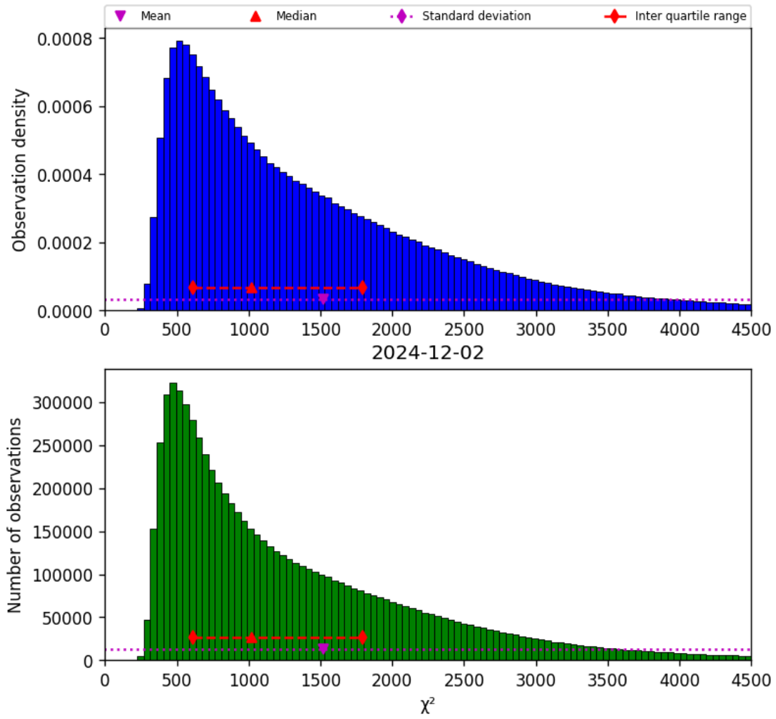
Figure 22: Histogram of “ \chi^2 ” for 2024-12-01 to 2024-12-03
