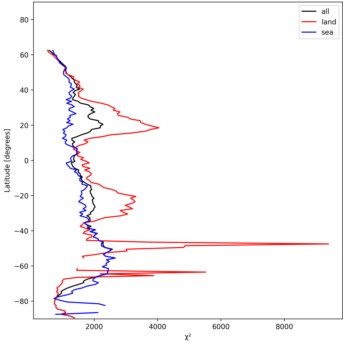
Figure 14: Zonal average of “ \chi^2 ” for 2024-12-01 to 2024-12-03.
