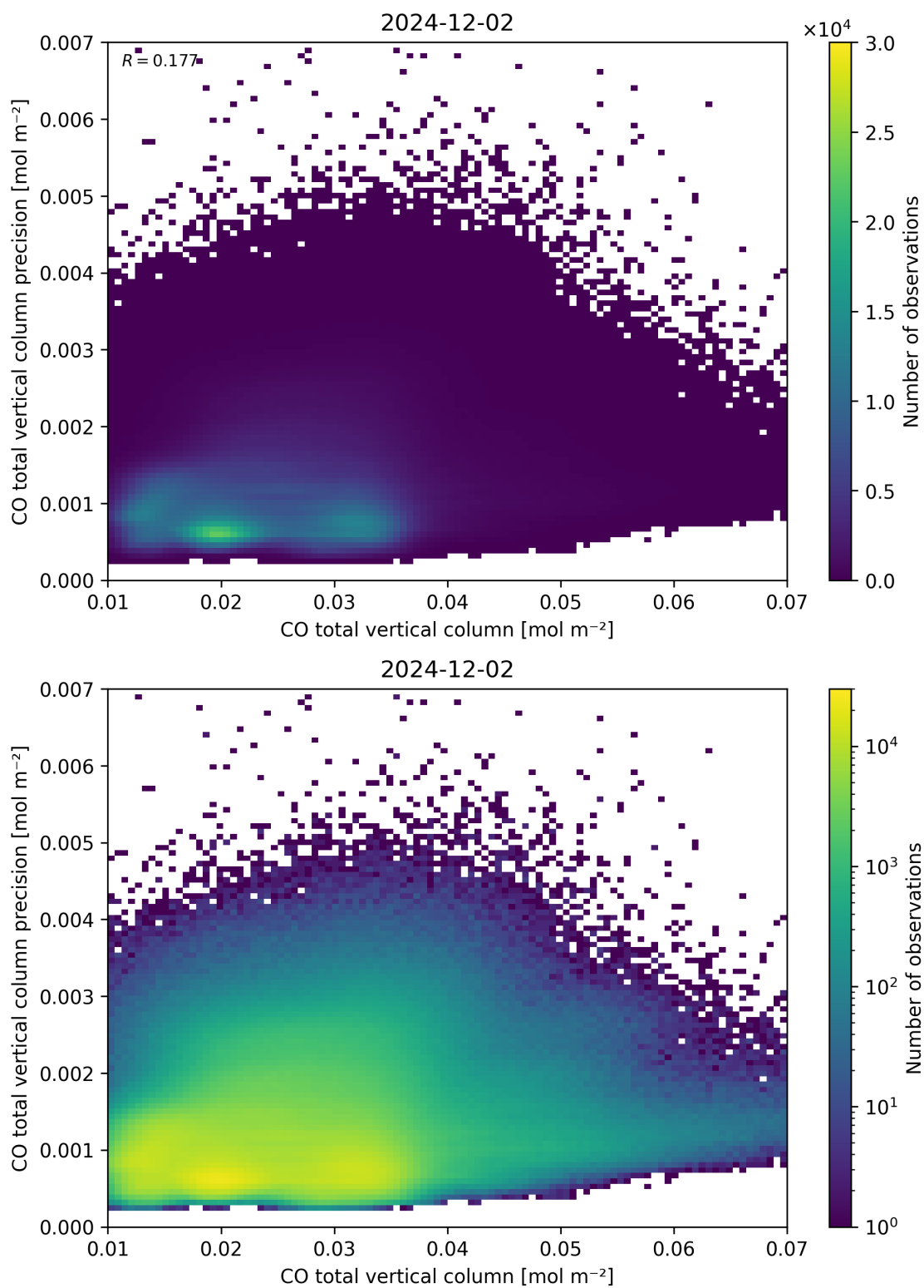
Figure 34: Scatter density plot of “CO total vertical column” against “CO total vertical column precision” for 2024-12-01 to 2024-12-03.
