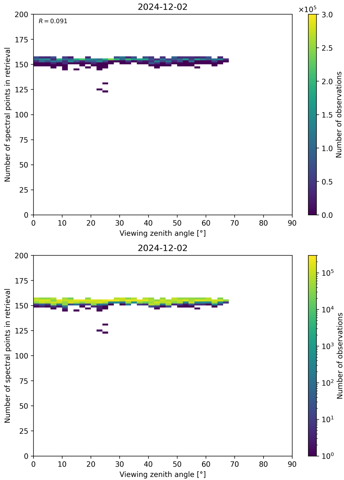
Figure 76: Scatter density plot of “Viewing zenith angle” against “Number of spectral points in retrieval” for 2024-12-01 to 2024-12-03.
