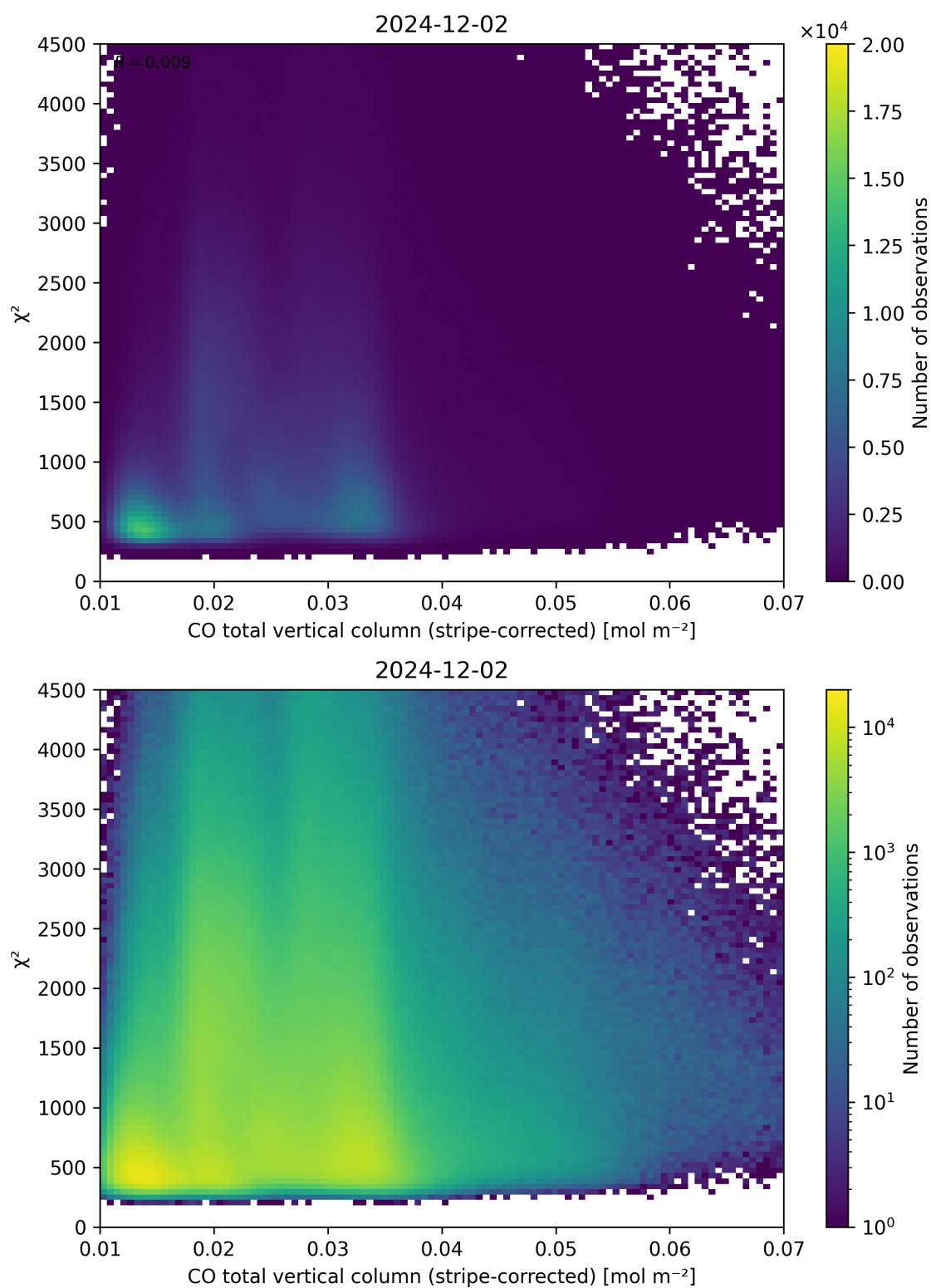
Figure 37: Scatter density plot of “CO total vertical column (stripe-corrected)” against “ \chi^2 ” for 2024-12-01 to 2024-12-03.
