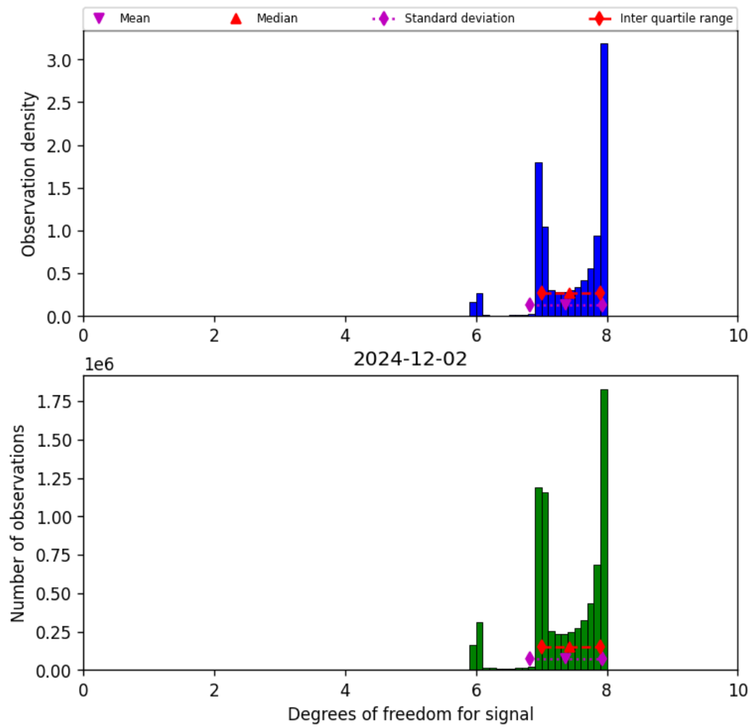
Figure 23: Histogram of “Degrees of freedom for signal” for 2024-12-01 to 2024-12-03
