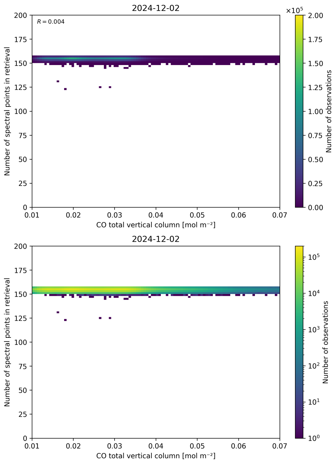
Figure 43: Scatter density plot of “CO total vertical column” against “Number of spectral points in retrieval” for 2024-12-01 to 2024-12-03.
