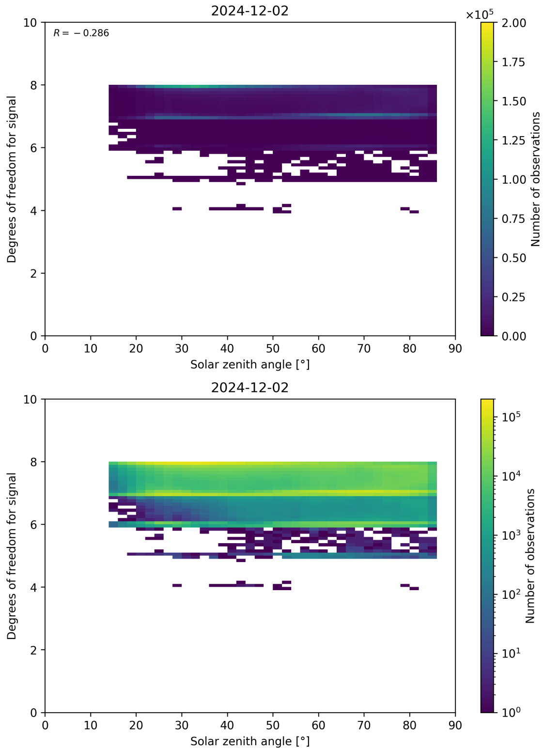
Figure 65: Scatter density plot of “Solar zenith angle” against “Degrees of freedom for signal” for 2024-12-01 to 2024-12-03.
