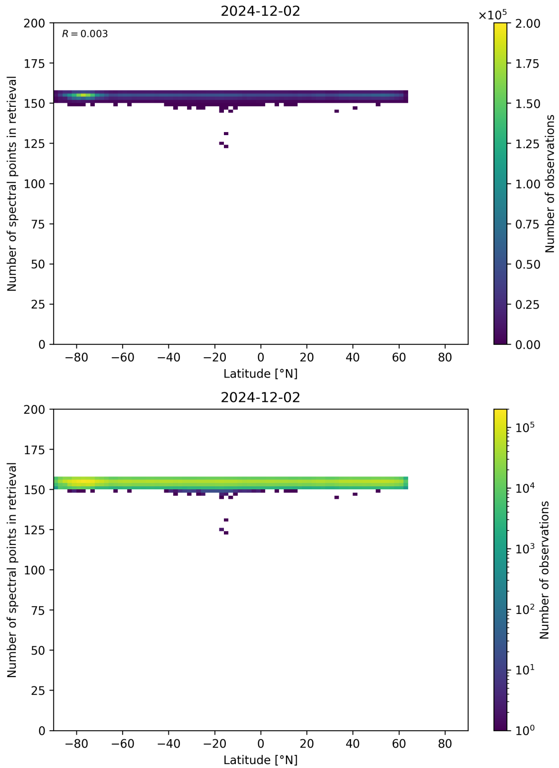
Figure 57: Scatter density plot of “Latitude” against “Number of spectral points in retrieval” for 2024-12-01 to 2024-12-03.
