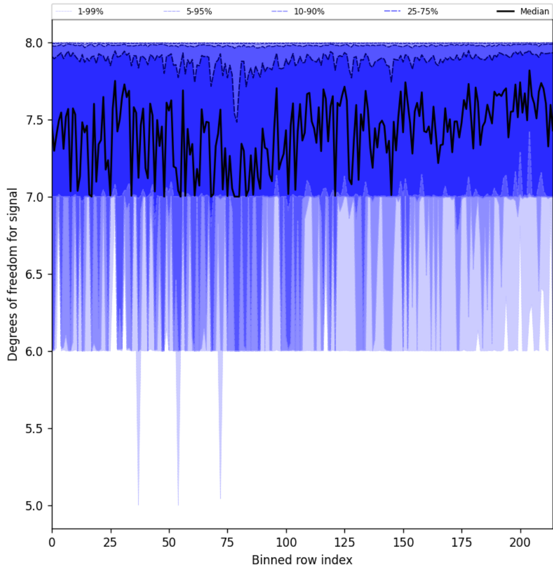
Figure 31: Along track statistics of “Degrees of freedom for signal” for 2024-12-01 to 2024-12-03
