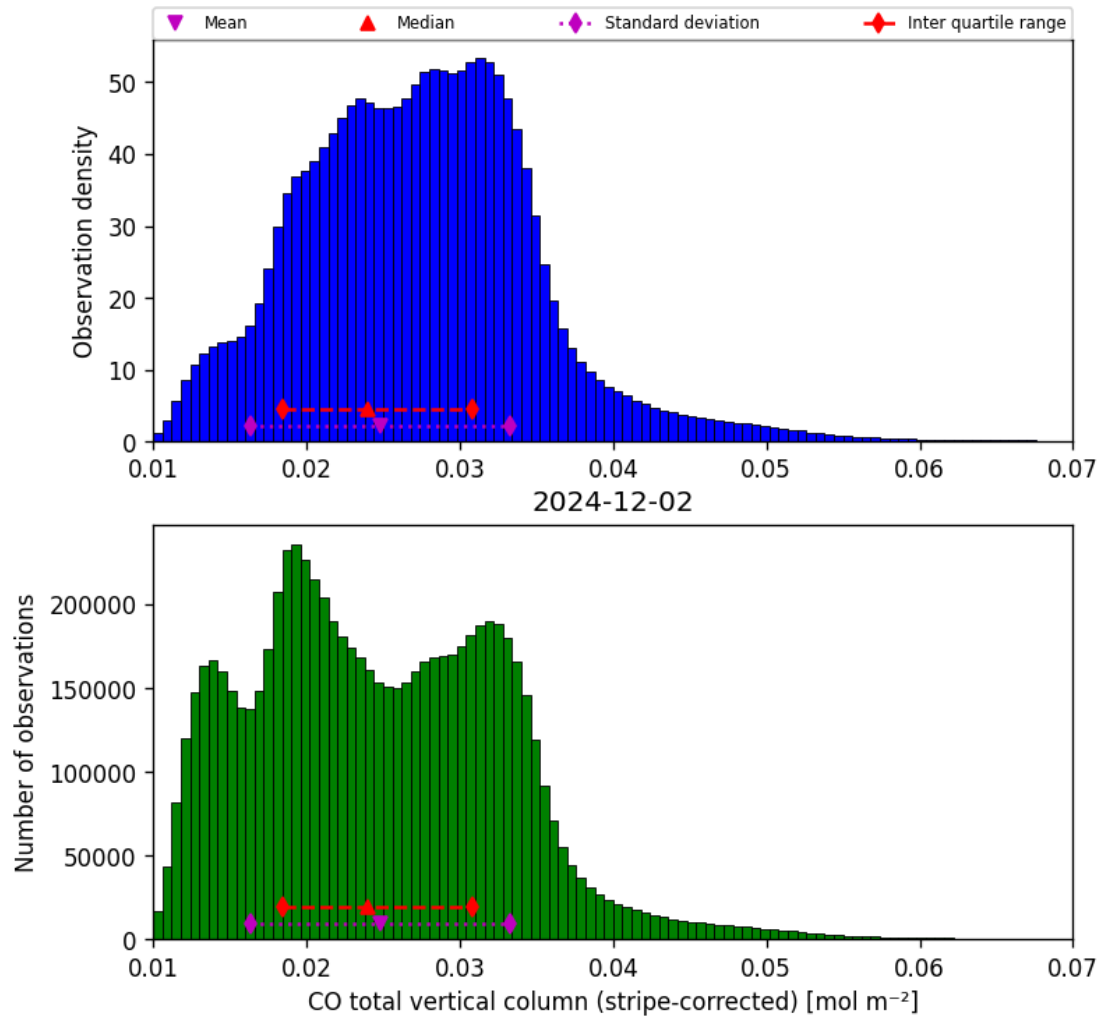
Figure 19: Histogram of “CO total vertical column (stripe-corrected)” for 2024-12-01 to 2024-12-03
