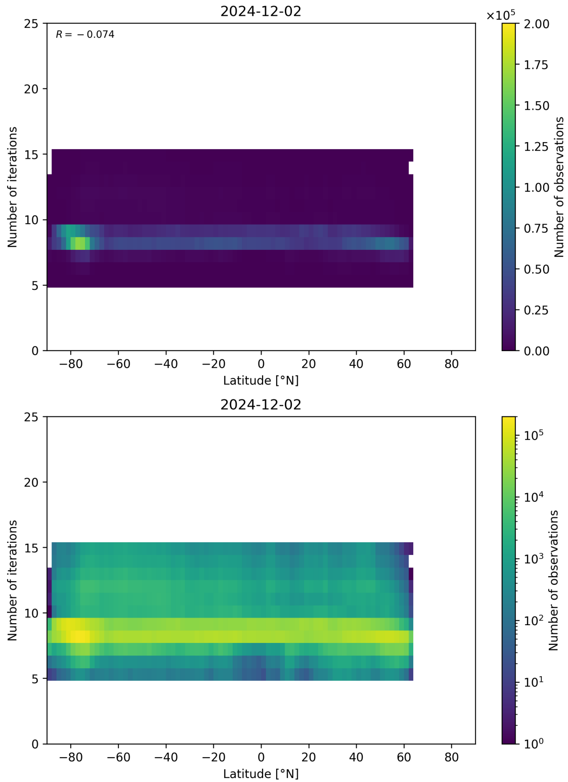
Figure 56: Scatter density plot of “Latitude” against “Number of iterations” for 2024-12-01 to 2024-12-03.
