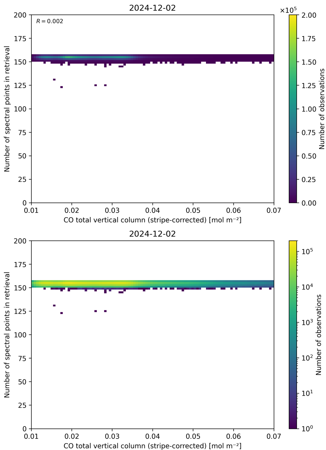
Figure 40: Scatter density plot of “CO total vertical column (stripe-corrected)” against “Number of spectral points in retrieval” for 2024-12-01 to 2024-12-03.
