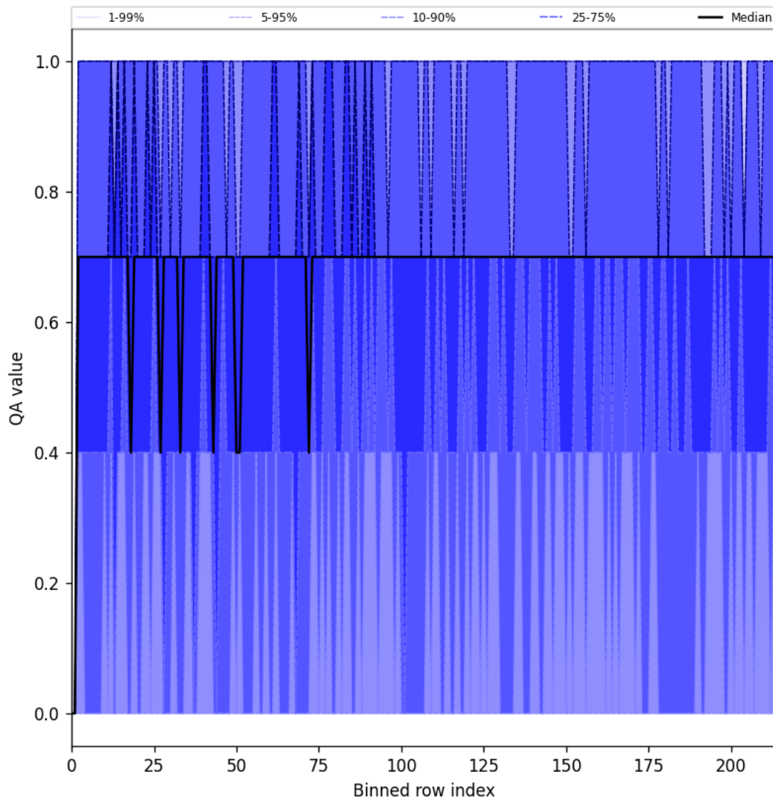
Figure 25: Along track statistics of “QA value” for 2024-12-01 to 2024-12-03
