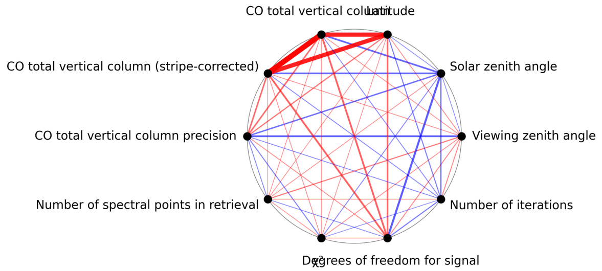
Figure 1: Map of correlation graph for 2024-12-01 to 2024-12-03.
