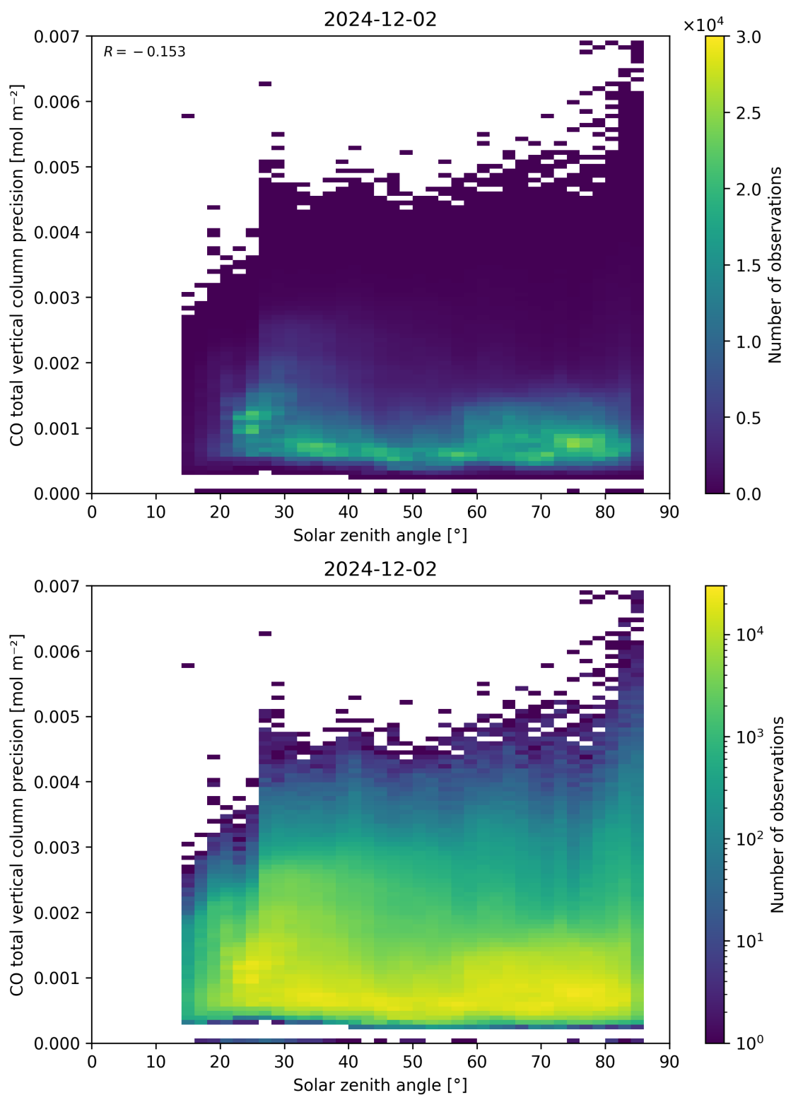
Figure 63: Scatter density plot of “Solar zenith angle” against “CO total vertical column precision” for 2024-12-01 to 2024-12-03.
