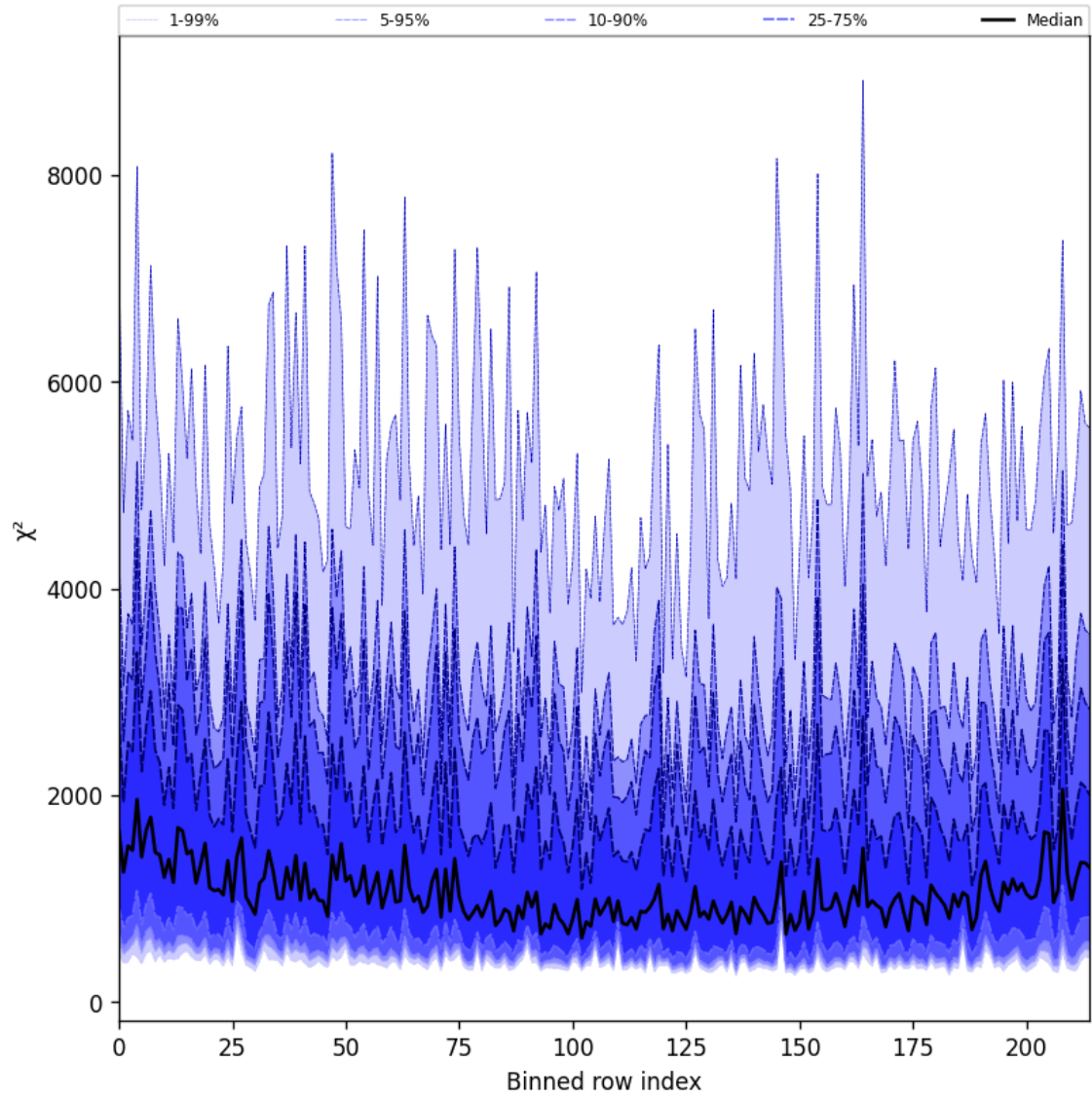
Figure 30: Along track statistics of “ \chi^2 ” for 2024-12-01 to 2024-12-03
