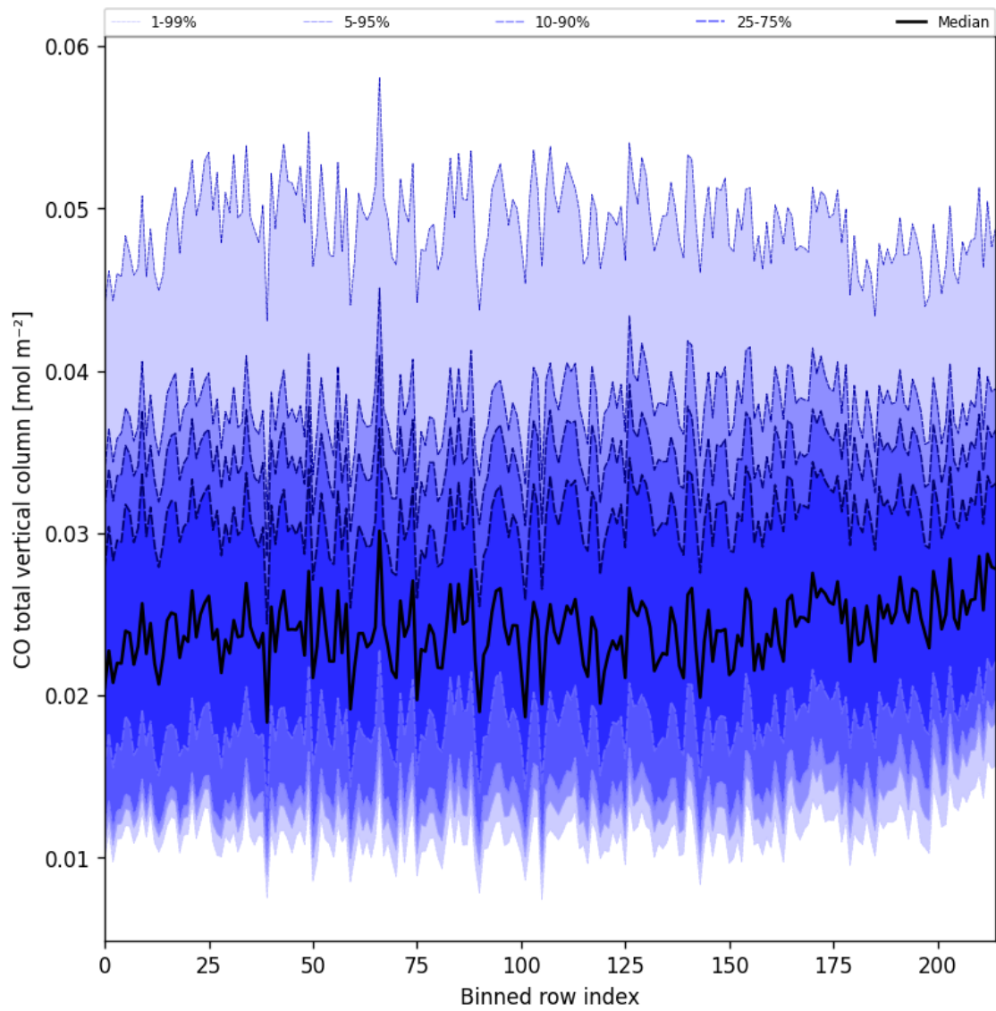
Figure 26: Along track statistics of “CO total vertical column” for 2024-12-01 to 2024-12-03
