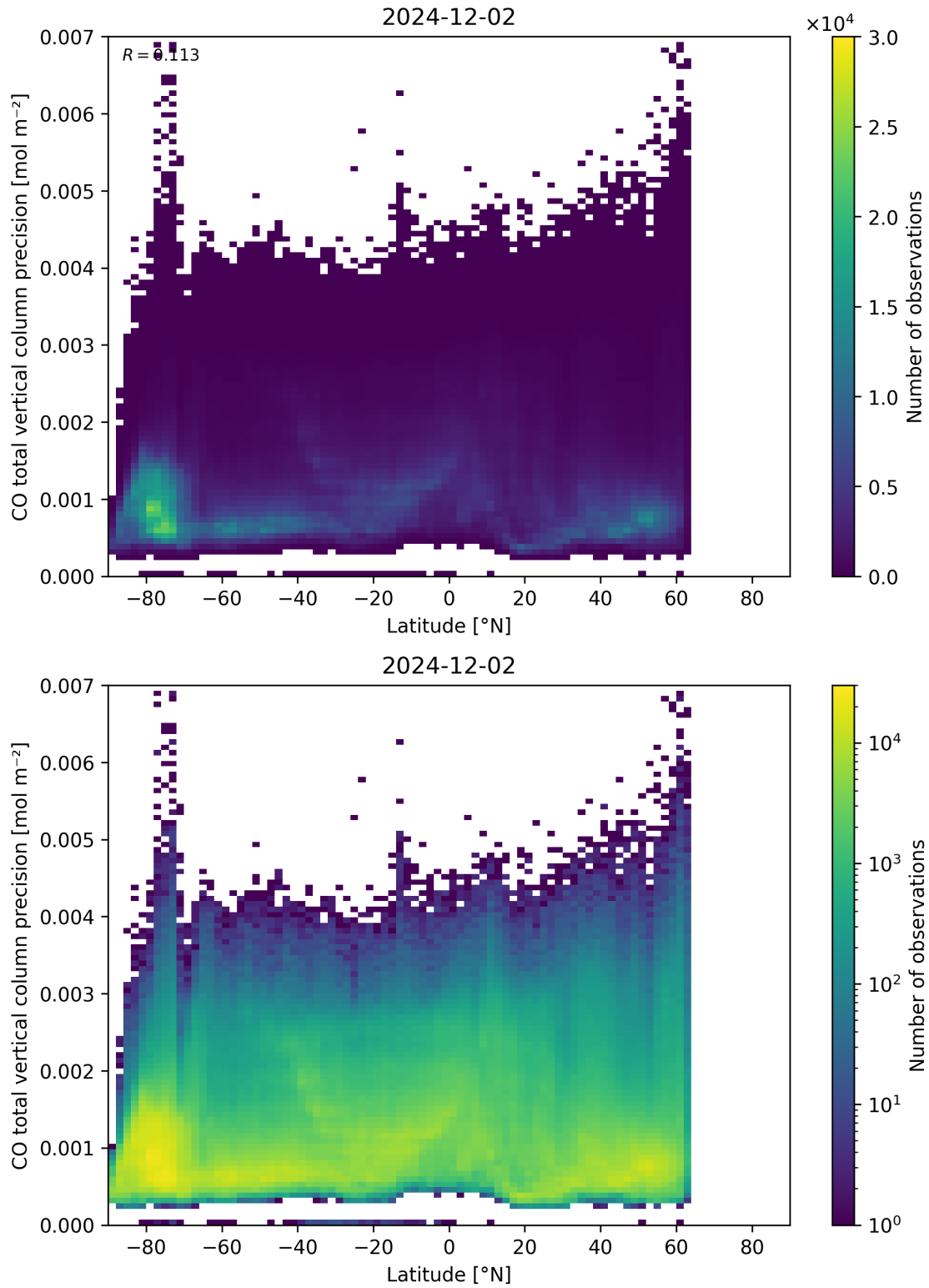
Figure 53: Scatter density plot of “Latitude” against “CO total vertical column precision” for 2024-12-01 to 2024-12-03.
