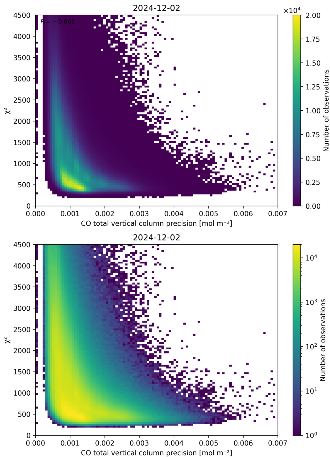
Figure 44: Scatter density plot of “CO total vertical column precision” against “ \chi^2 ” for 2024-12-01 to 2024-12-03.
