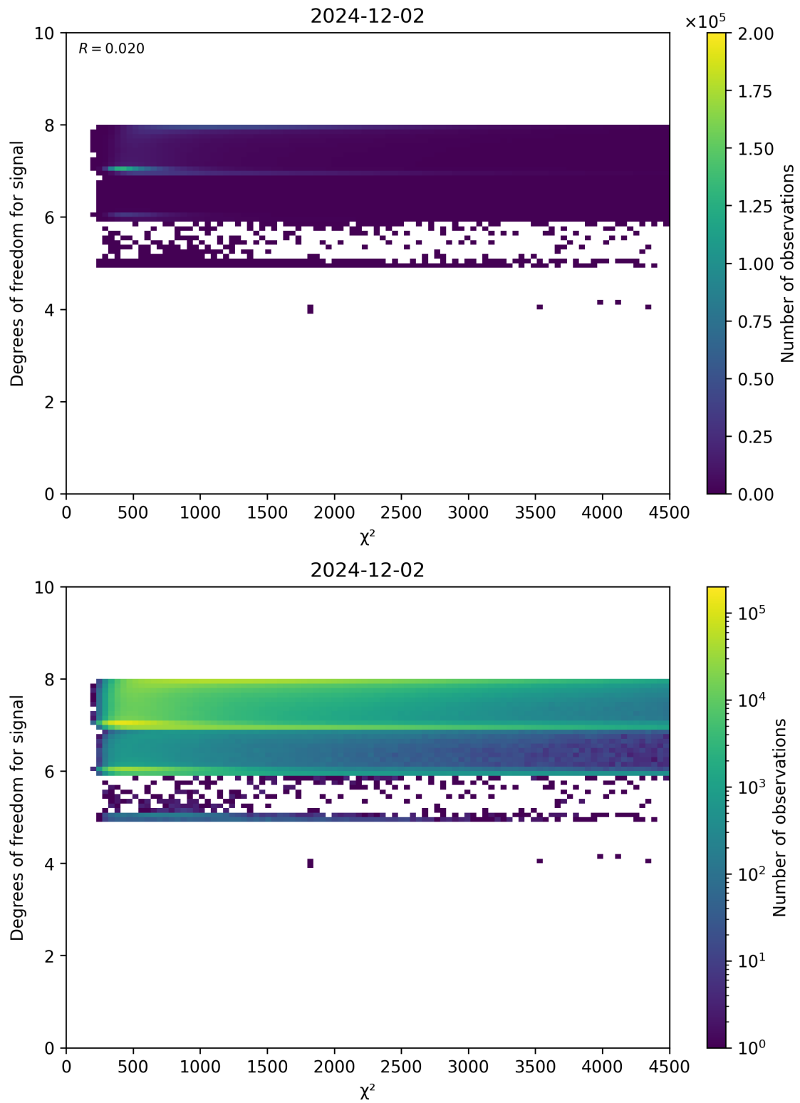
Figure 48: Scatter density plot of “ \chi^2 ” against “Degrees of freedom for signal” for 2024-12-01 to 2024-12-03.
