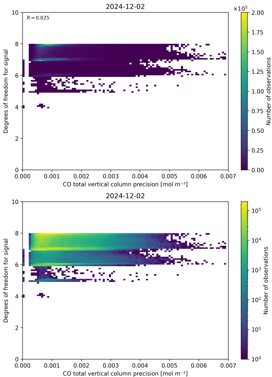
Figure 45: Scatter density plot of “CO total vertical column precision” against “Degrees of freedom for signal” for 2024-12-01 to 2024-12-03.
