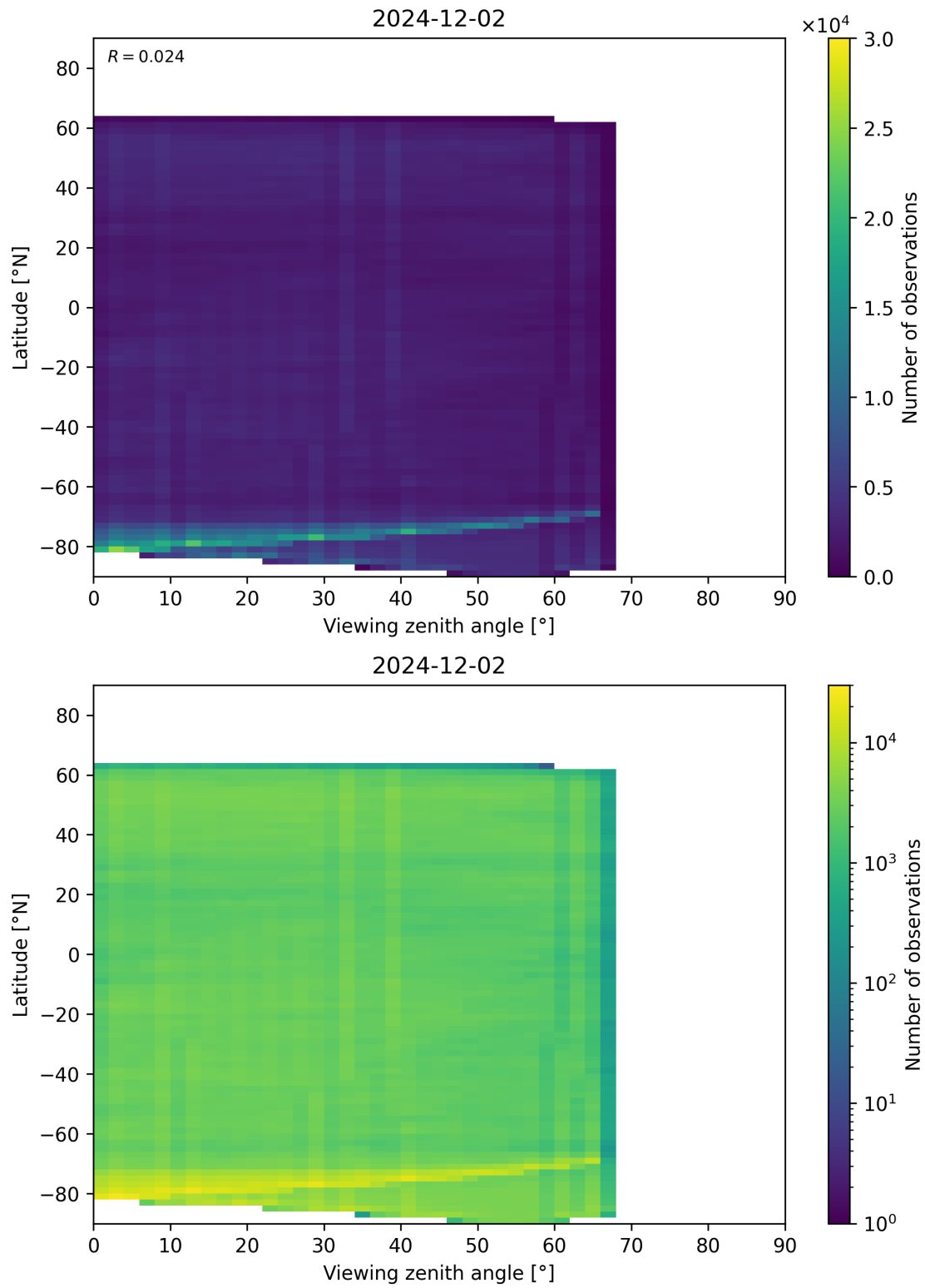
Figure 74: Scatter density plot of “Viewing zenith angle” against “Latitude” for 2024-12-01 to 2024-12-03.
