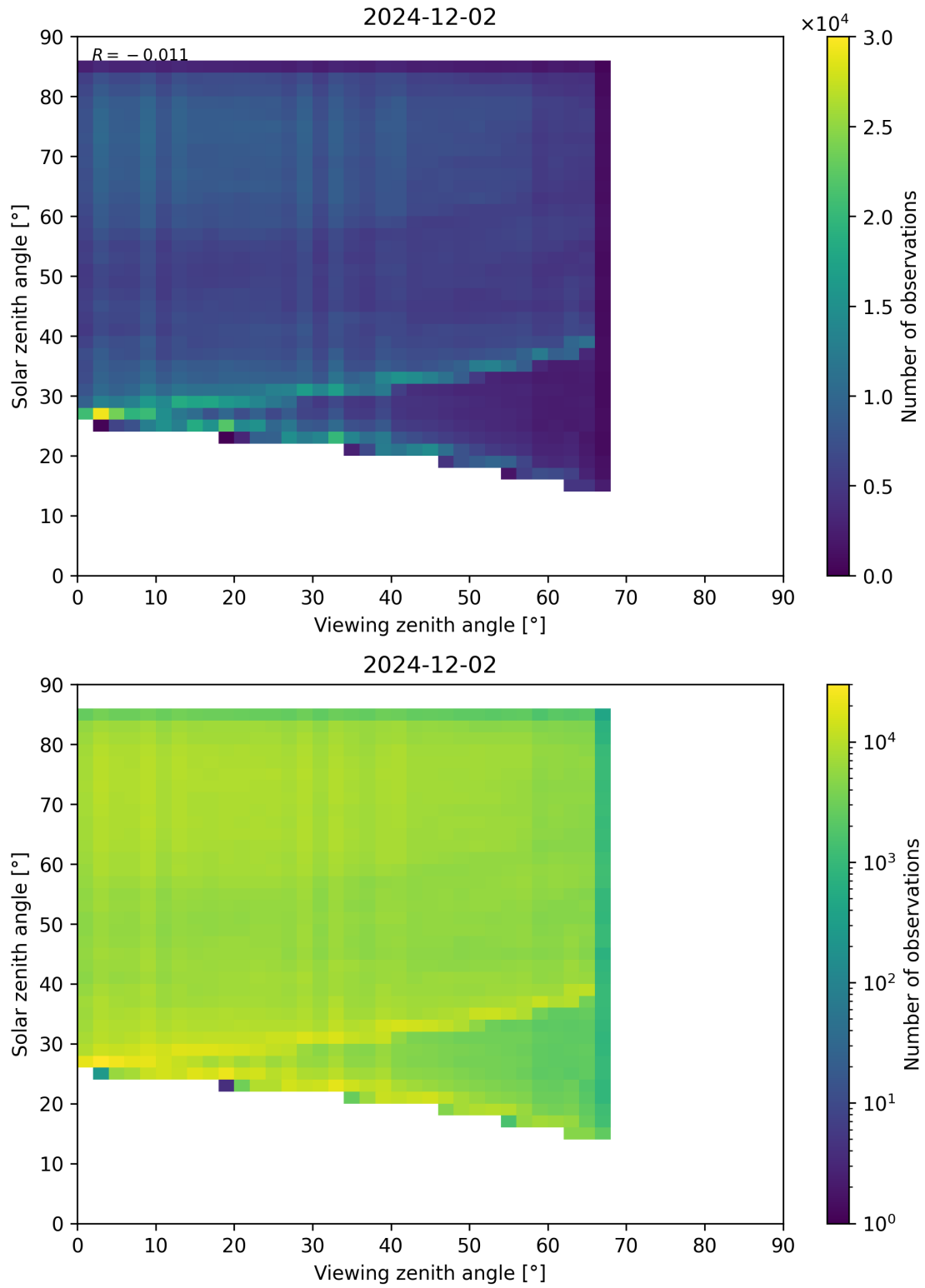
Figure 77: Scatter density plot of “Viewing zenith angle” against “Solar zenith angle” for 2024-12-01 to 2024-12-03.
