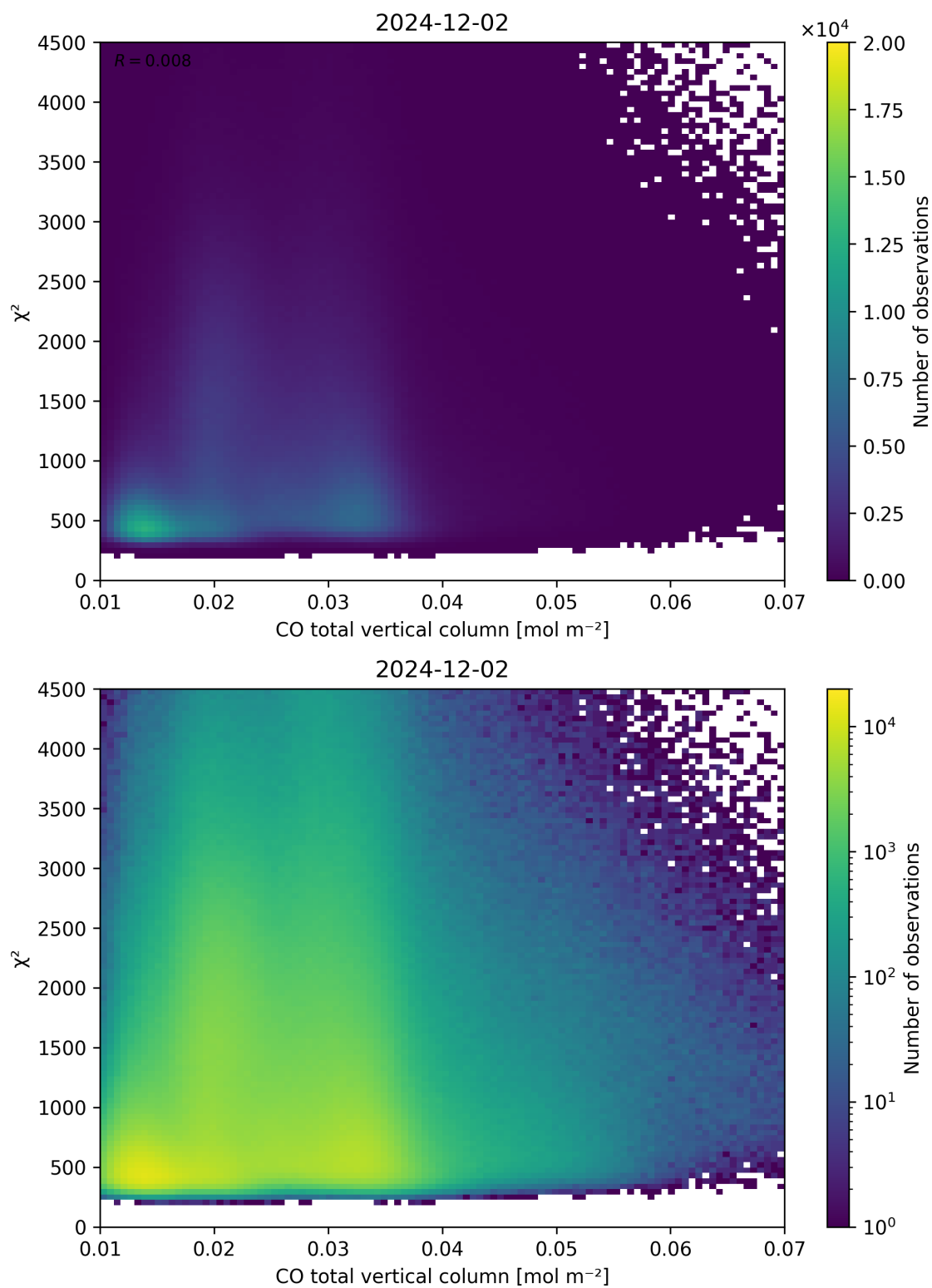
Figure 35: Scatter density plot of “CO total vertical column” against “ \chi^2 ” for 2024-12-01 to 2024-12-03.
