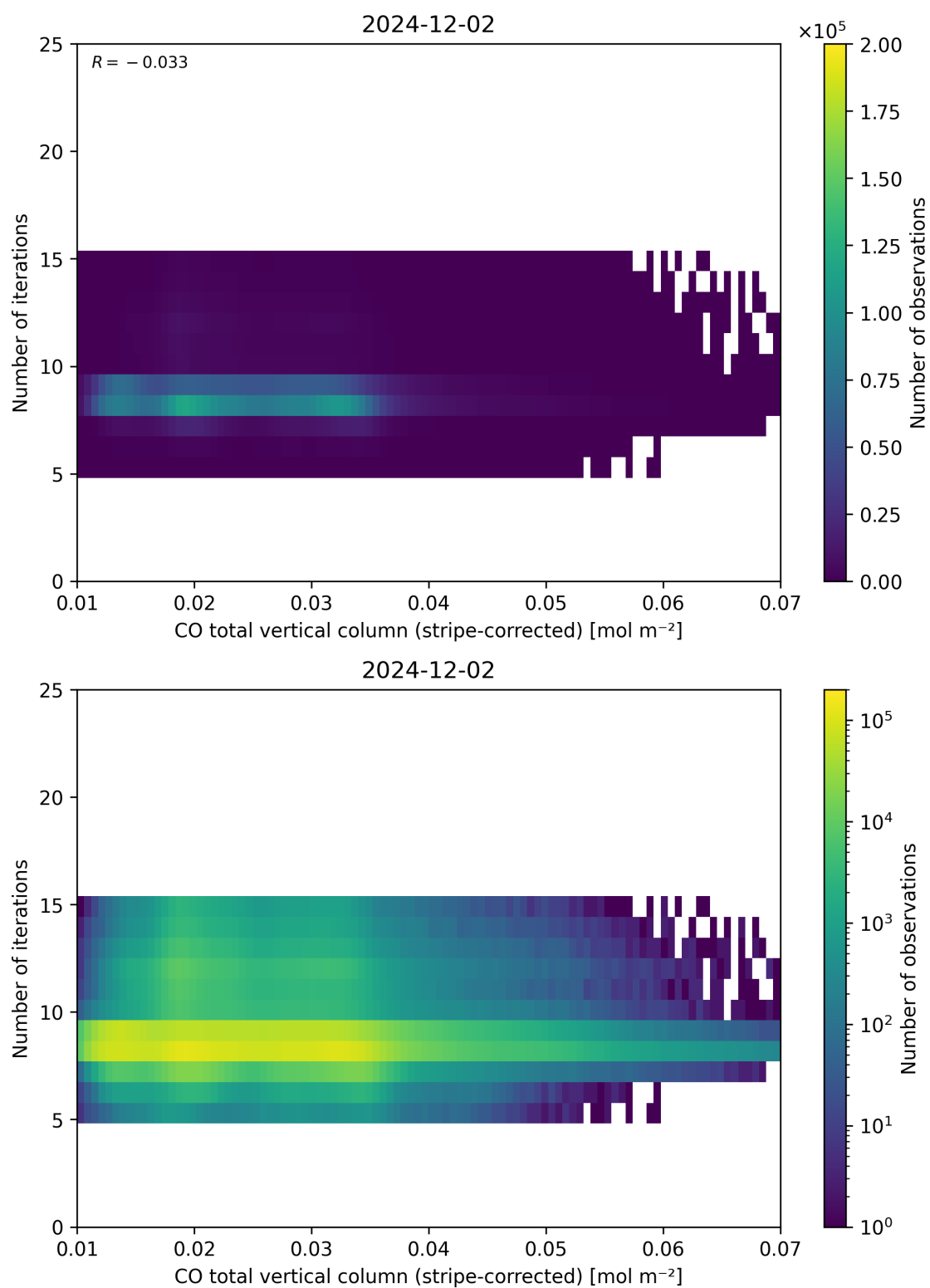
Figure 39: Scatter density plot of “CO total vertical column (stripe-corrected)” against “Number of iterations” for 2024-12-01 to 2024-12-03.
