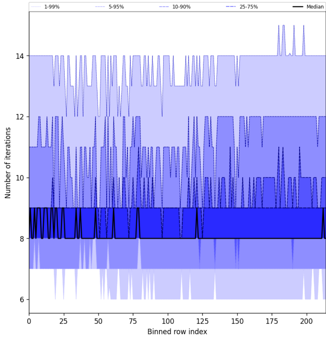
Figure 32: Along track statistics of “Number of iterations” for 2024-12-01 to 2024-12-03
