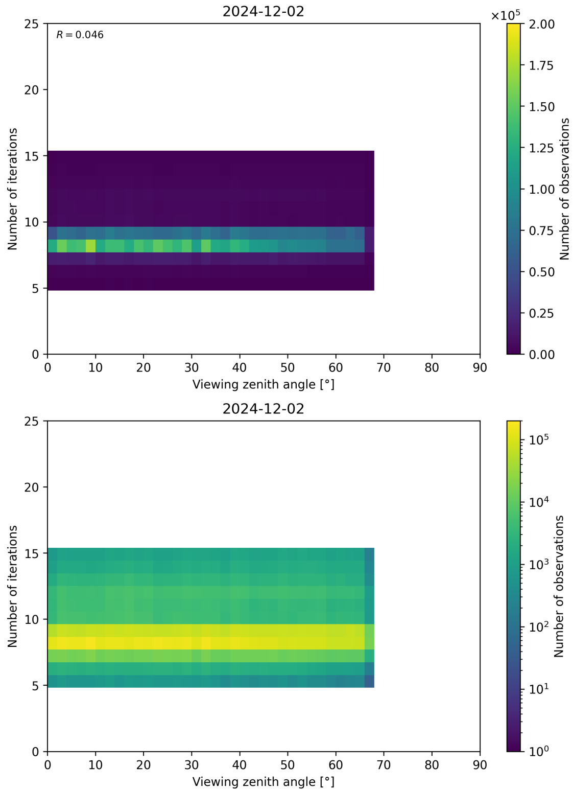
Figure 75: Scatter density plot of “Viewing zenith angle” against “Number of iterations” for 2024-12-01 to 2024-12-03.
