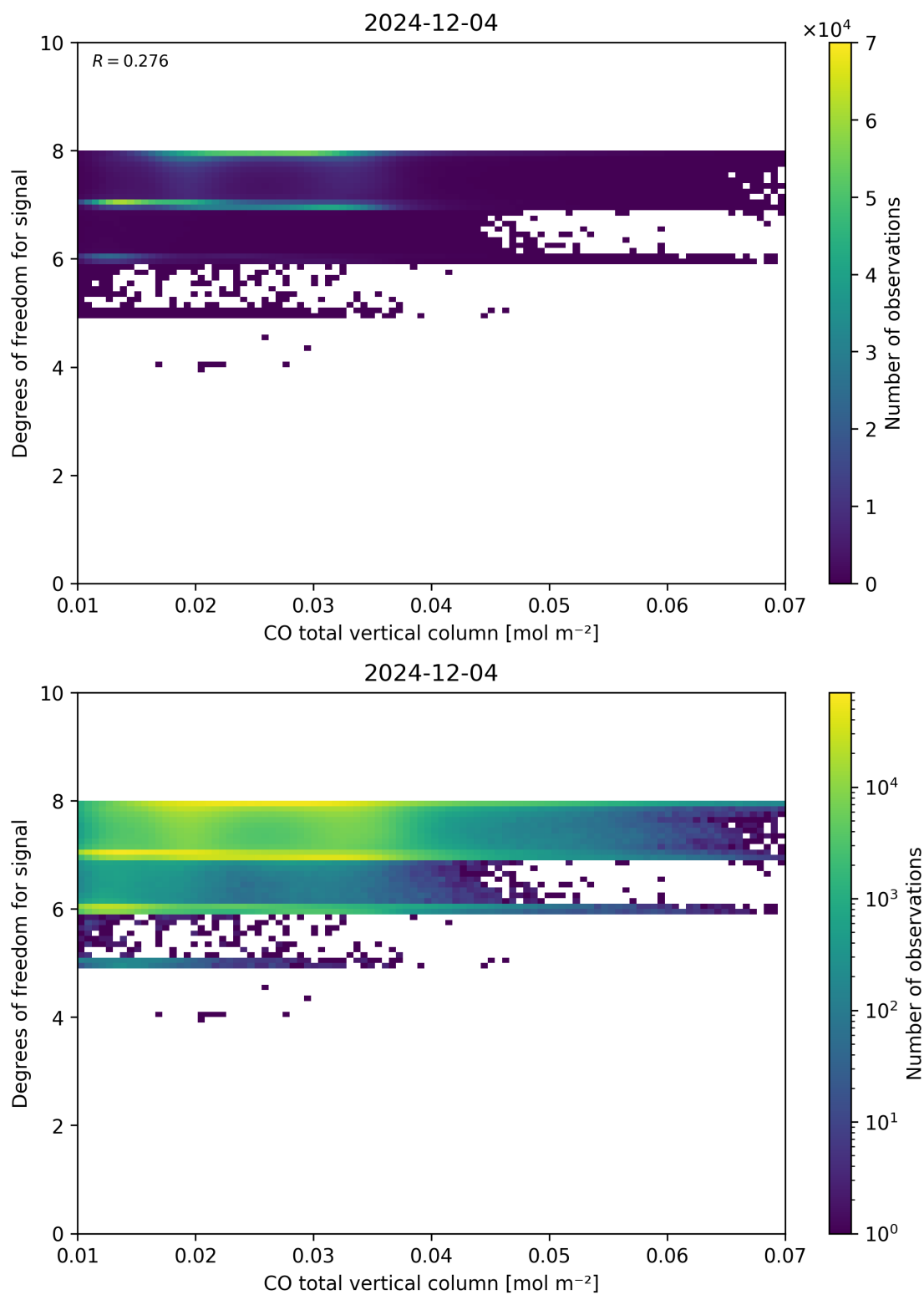
Figure 41: Scatter density plot of “CO total vertical column” against “Degrees of freedom for signal” for 2024-12-03 to 2024-12-05.
