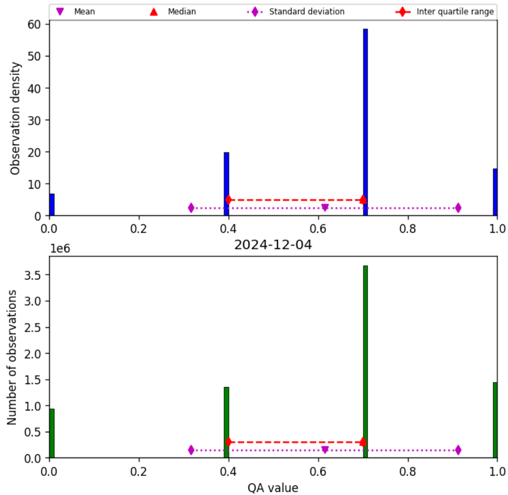
Figure 17: Histogram of “QA value” for 2024-12-03 to 2024-12-05
