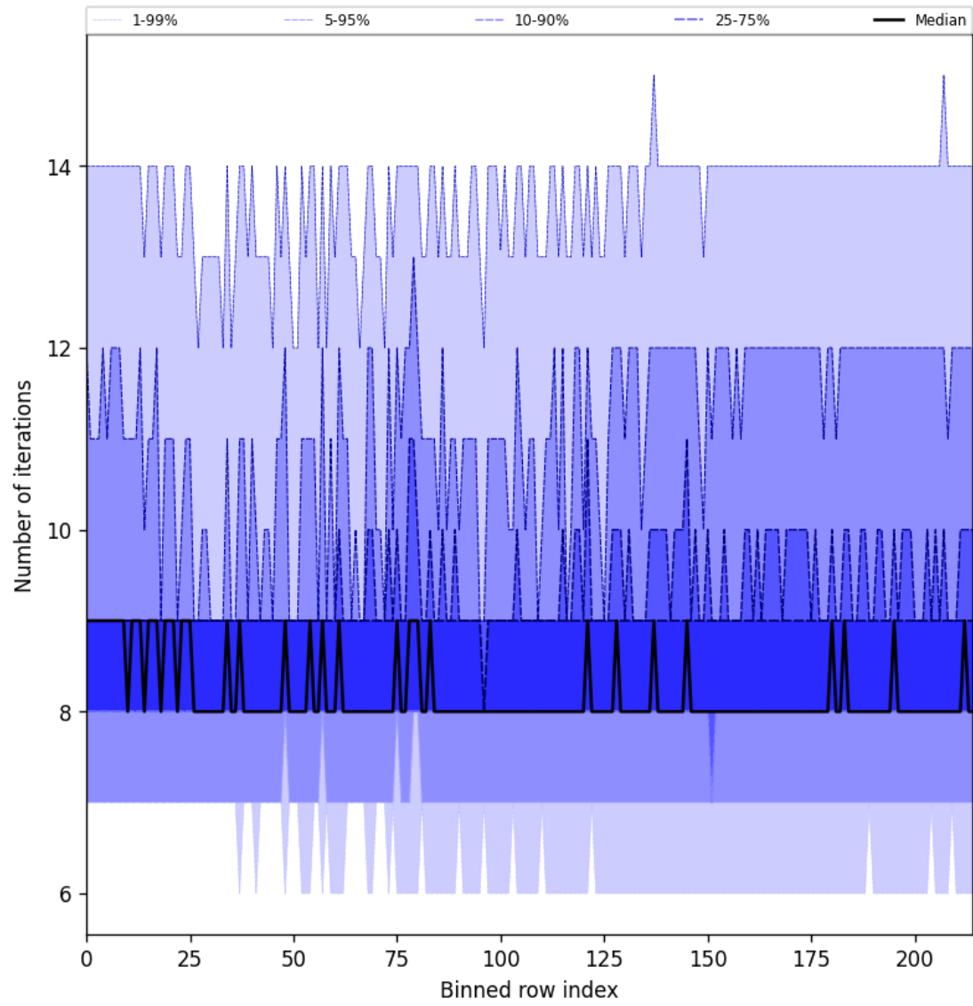
Figure 32: Along track statistics of “Number of iterations” for 2024-12-03 to 2024-12-05
