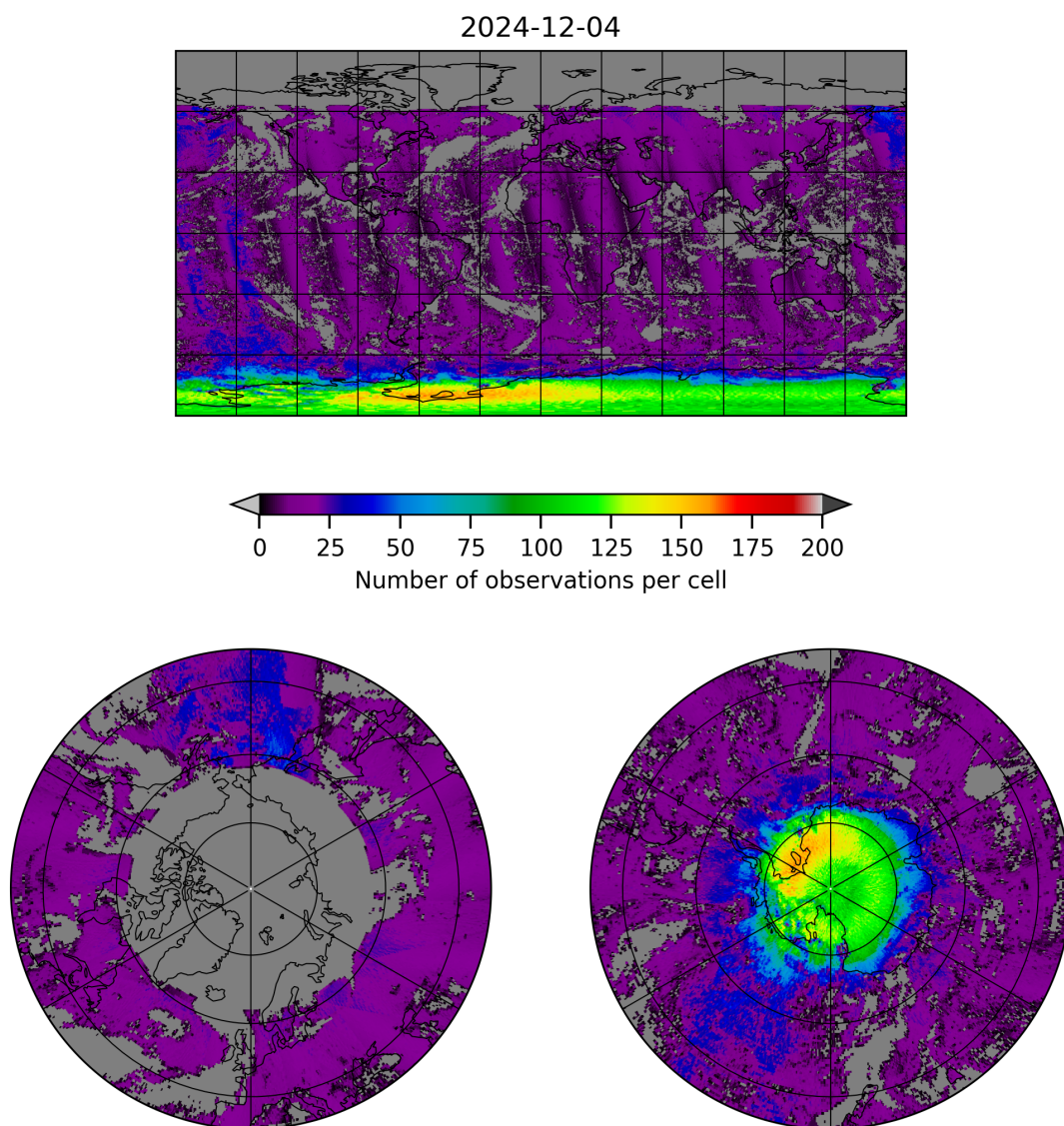
Figure 8: Map of the number of observations for 2024-12-03 to 2024-12-05
