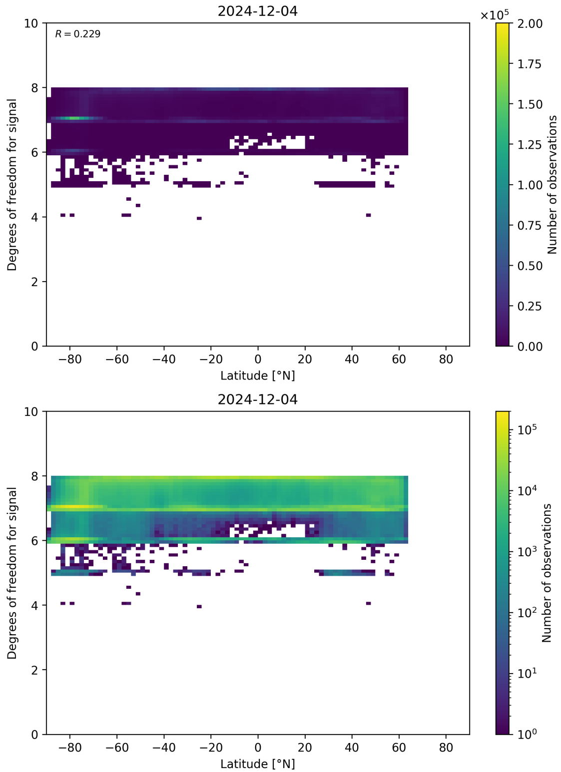
Figure 55: Scatter density plot of “Latitude” against “Degrees of freedom for signal” for 2024-12-03 to 2024-12-05.
