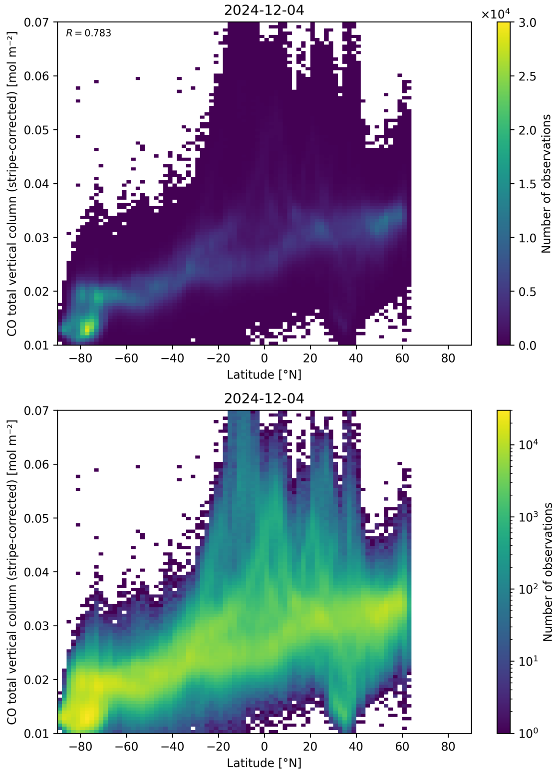
Figure 52: Scatter density plot of “Latitude” against “CO total vertical column (stripe-corrected)” for 2024-12-03 to 2024-12-05.
