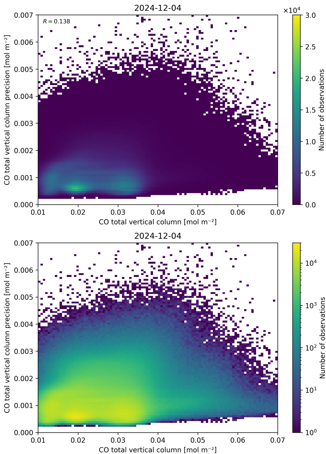
Figure 34: Scatter density plot of “CO total vertical column” against “CO total vertical column precision” for 2024-12-03 to 2024-12-05.
