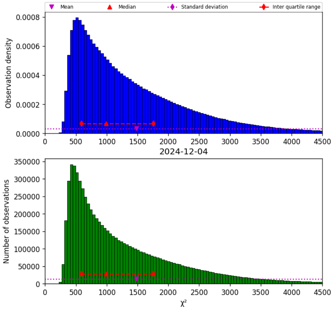
Figure 22: Histogram of “ \chi^2 ” for 2024-12-03 to 2024-12-05
