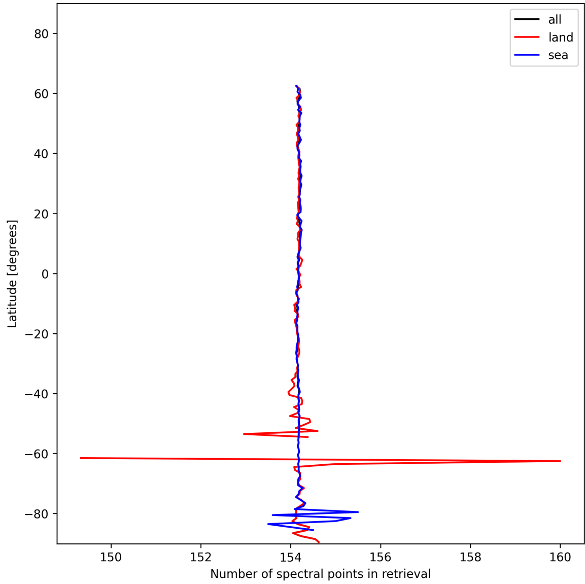
Figure 13: Zonal average of “Number of spectral points in retrieval” for 2024-12-03 to 2024-12-05.
