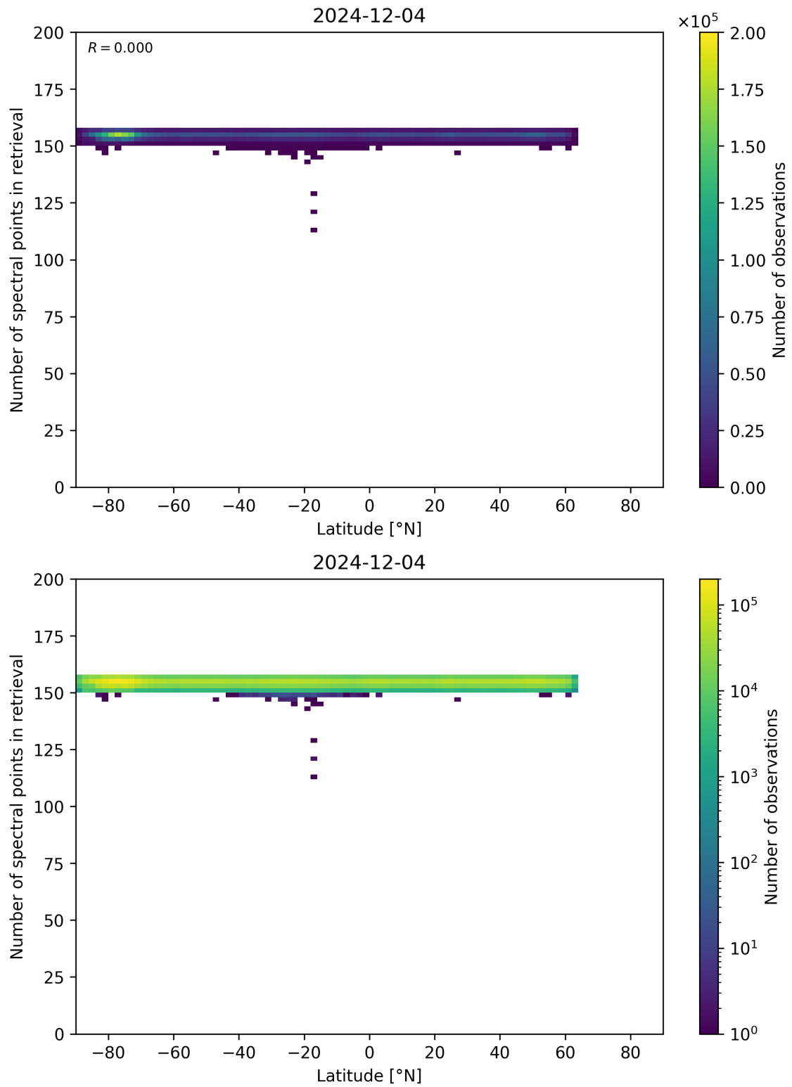
Figure 57: Scatter density plot of “Latitude” against “Number of spectral points in retrieval” for 2024-12-03 to 2024-12-05.
