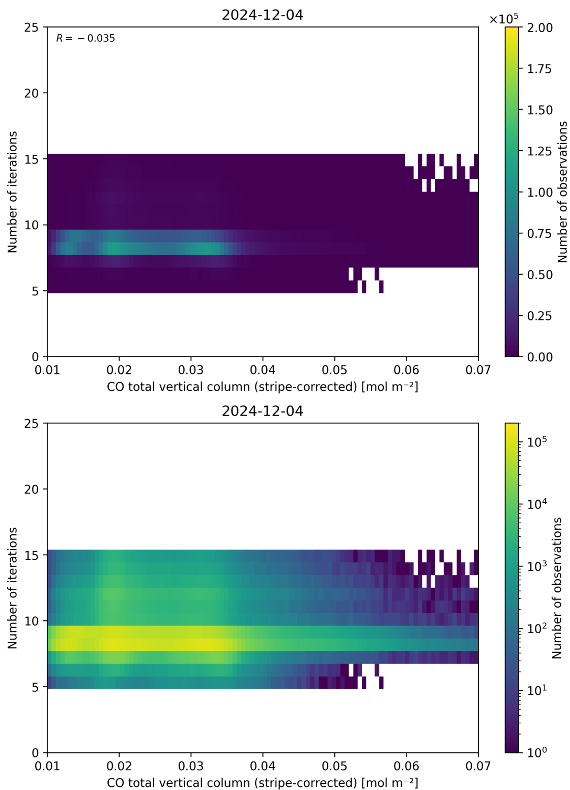
Figure 39: Scatter density plot of “CO total vertical column (stripe-corrected)” against “Number of iterations” for 2024-12-03 to 2024-12-05.
