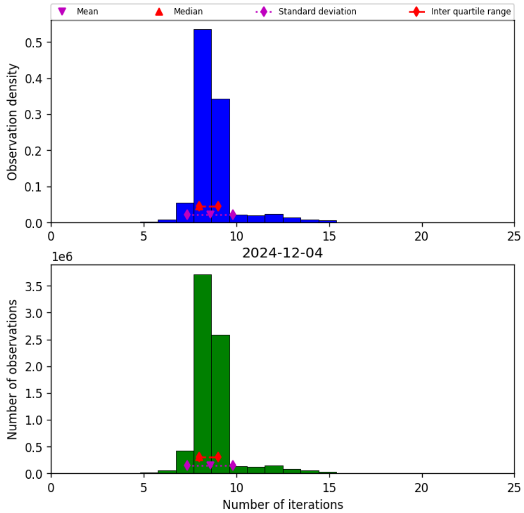
Figure 24: Histogram of “Number of iterations” for 2024-12-03 to 2024-12-05
