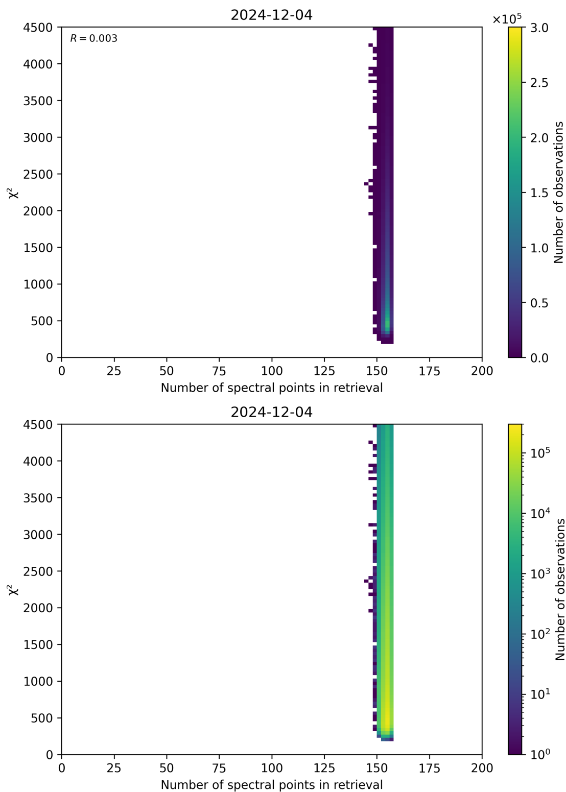
Figure 58: Scatter density plot of “Number of spectral points in retrieval” against “ \chi^2 ” for 2024-12-03 to 2024-12-05.
