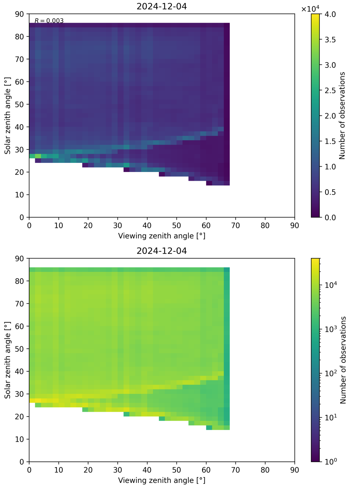
Figure 77: Scatter density plot of “Viewing zenith angle” against “Solar zenith angle” for 2024-12-03 to 2024-12-05.
