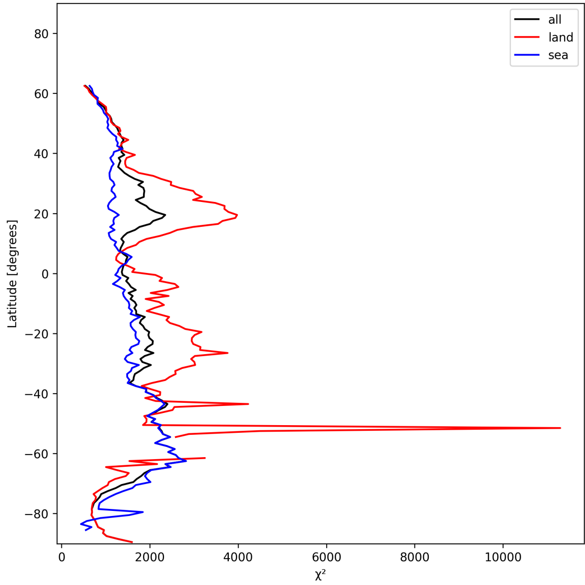
Figure 14: Zonal average of “ \chi^2 ” for 2024-12-03 to 2024-12-05.
