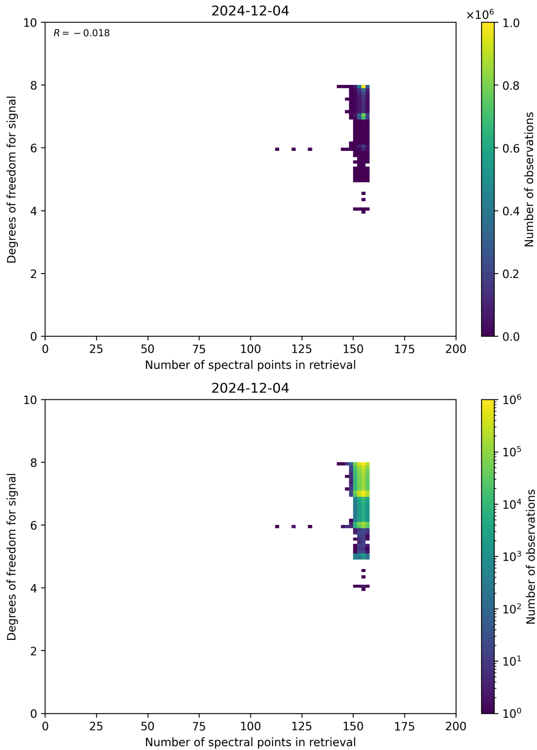
Figure 59: Scatter density plot of “Number of spectral points in retrieval” against “Degrees of freedom for signal” for 2024-12-03 to 2024-12-05.
