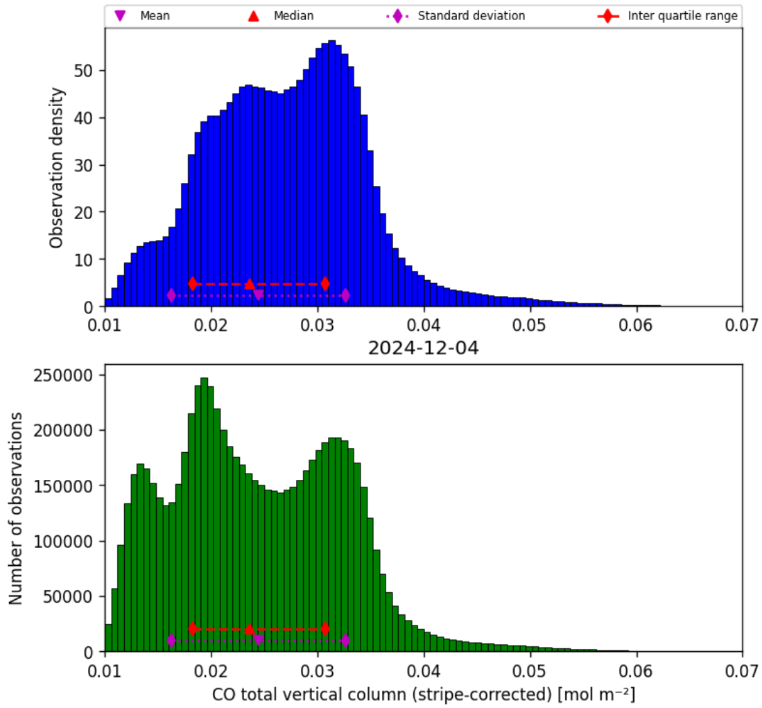
Figure 19: Histogram of “CO total vertical column (stripe-corrected)” for 2024-12-03 to 2024-12-05
