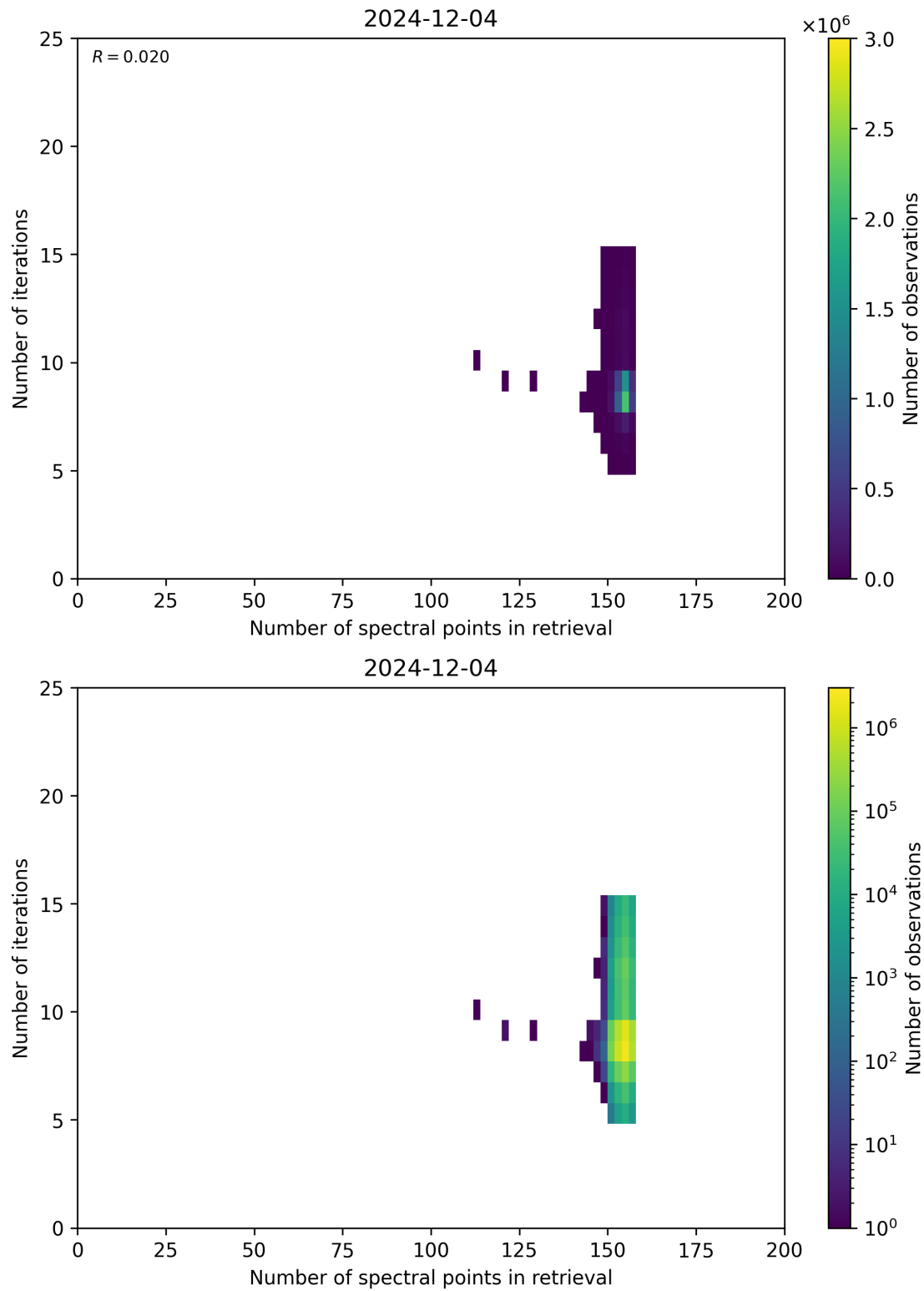
Figure 60: Scatter density plot of “Number of spectral points in retrieval” against “Number of iterations” for 2024-12-03 to 2024-12-05.
