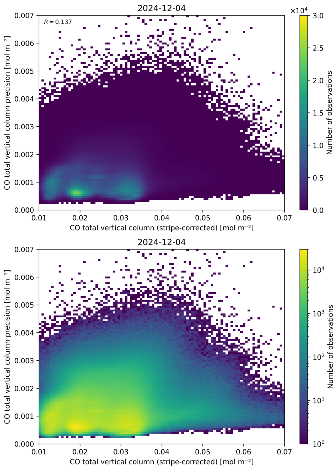
Figure 36: Scatter density plot of “CO total vertical column (stripe-corrected)” against “CO total vertical column precision” for 2024-12-03 to 2024-12-05.
