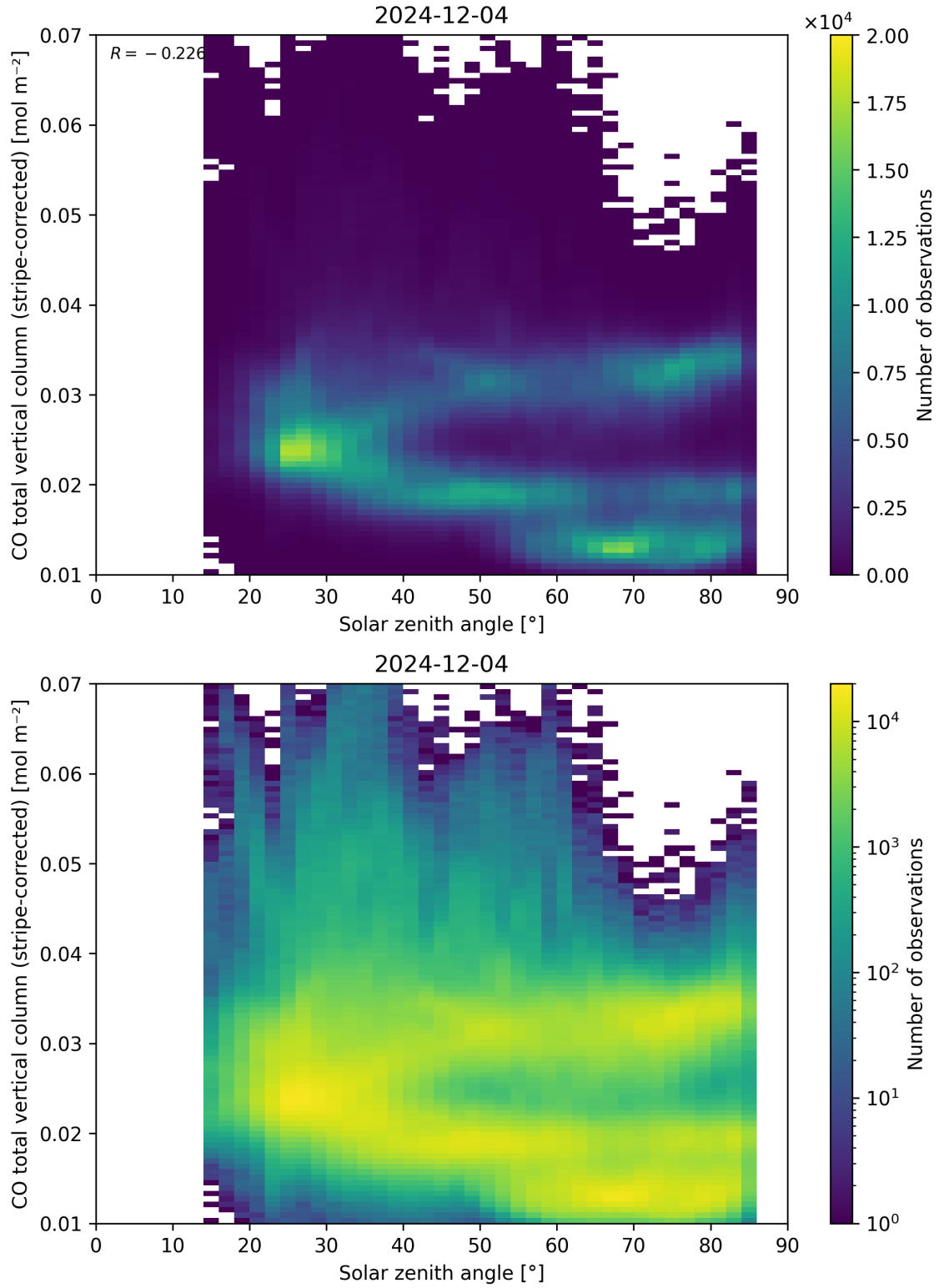
Figure 62: Scatter density plot of “Solar zenith angle” against “CO total vertical column (stripe-corrected)” for 2024-12-03 to 2024-12-05.
