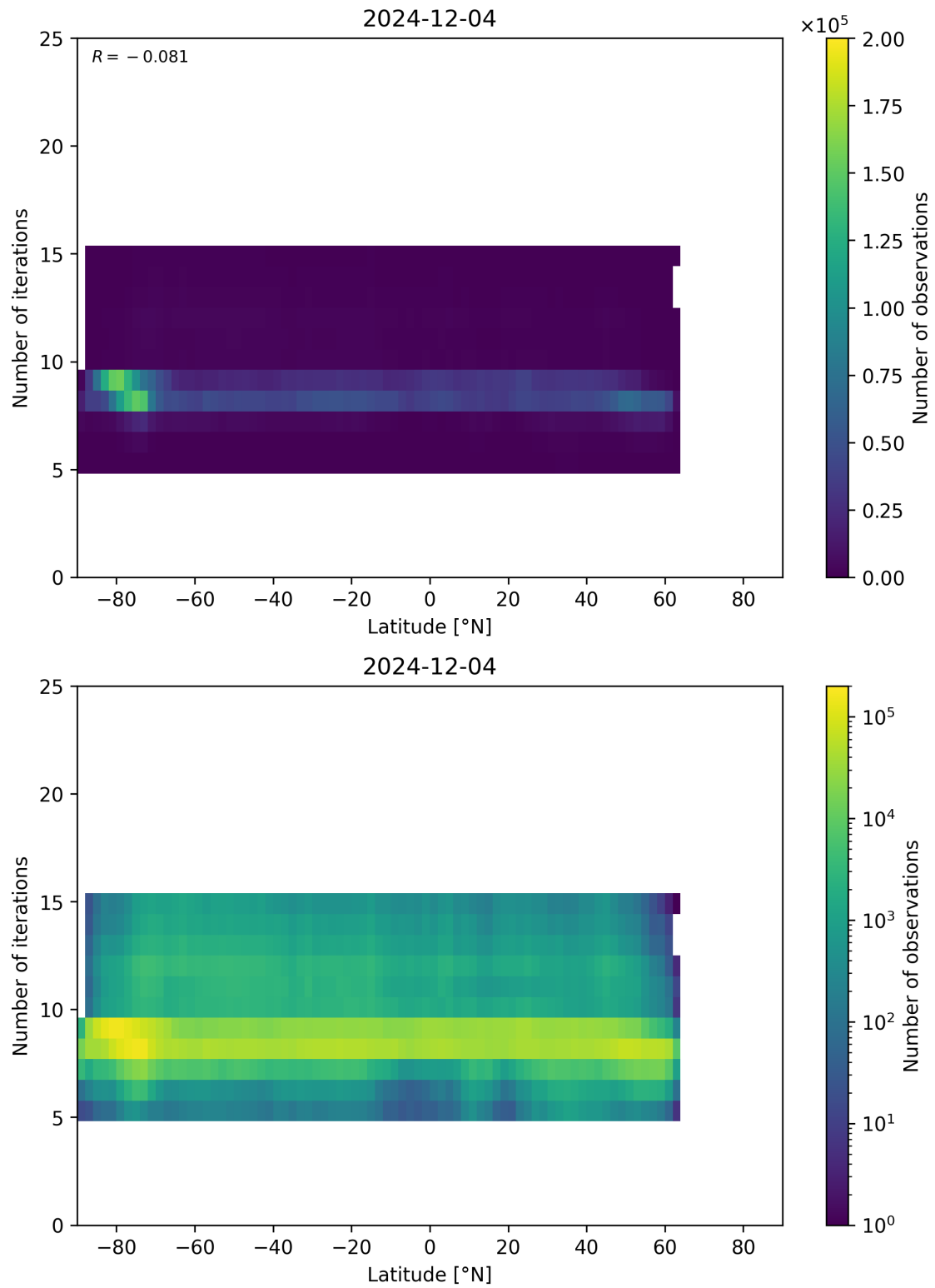
Figure 56: Scatter density plot of “Latitude” against “Number of iterations” for 2024-12-03 to 2024-12-05.
