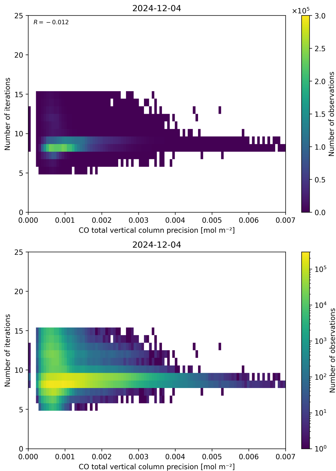
Figure 46: Scatter density plot of “CO total vertical column precision” against “Number of iterations” for 2024-12-03 to 2024-12-05.
