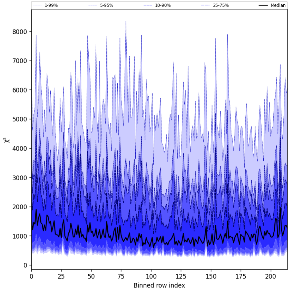
Figure 30: Along track statistics of “ \chi^2 ” for 2024-12-03 to 2024-12-05
