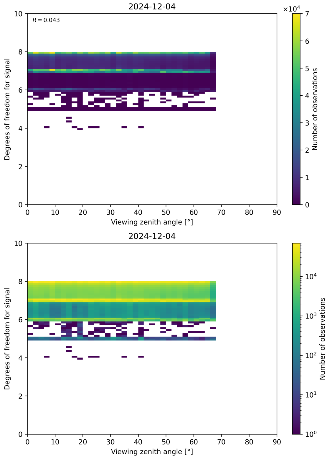
Figure 73: Scatter density plot of “Viewing zenith angle” against “Degrees of freedom for signal” for 2024-12-03 to 2024-12-05.
