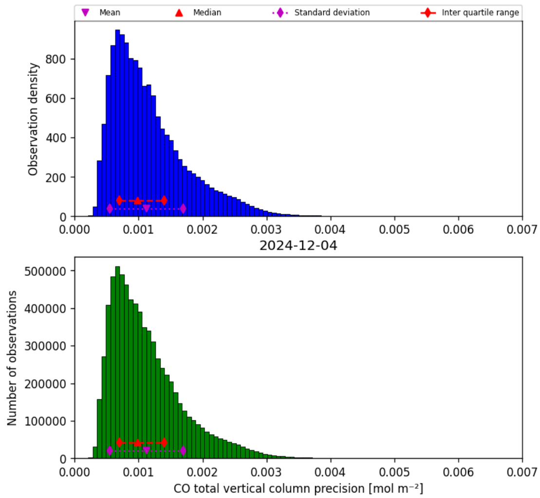
Figure 20: Histogram of “CO total vertical column precision” for 2024-12-03 to 2024-12-05
