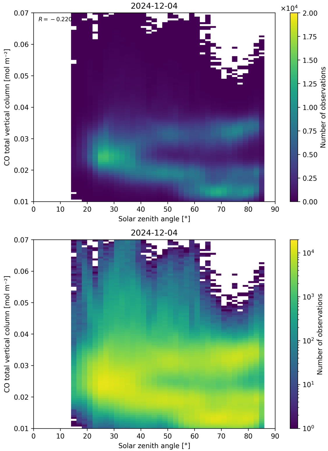
Figure 61: Scatter density plot of “Solar zenith angle” against “CO total vertical column” for 2024-12-03 to 2024-12-05.
