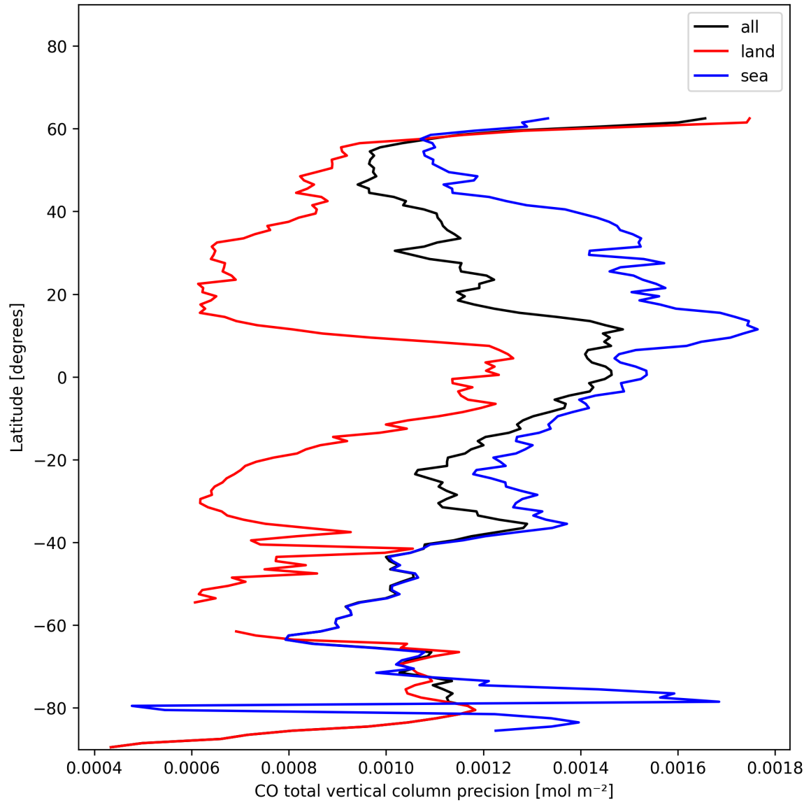
Figure 12: Zonal average of “CO total vertical column precision” for 2024-12-03 to 2024-12-05.
