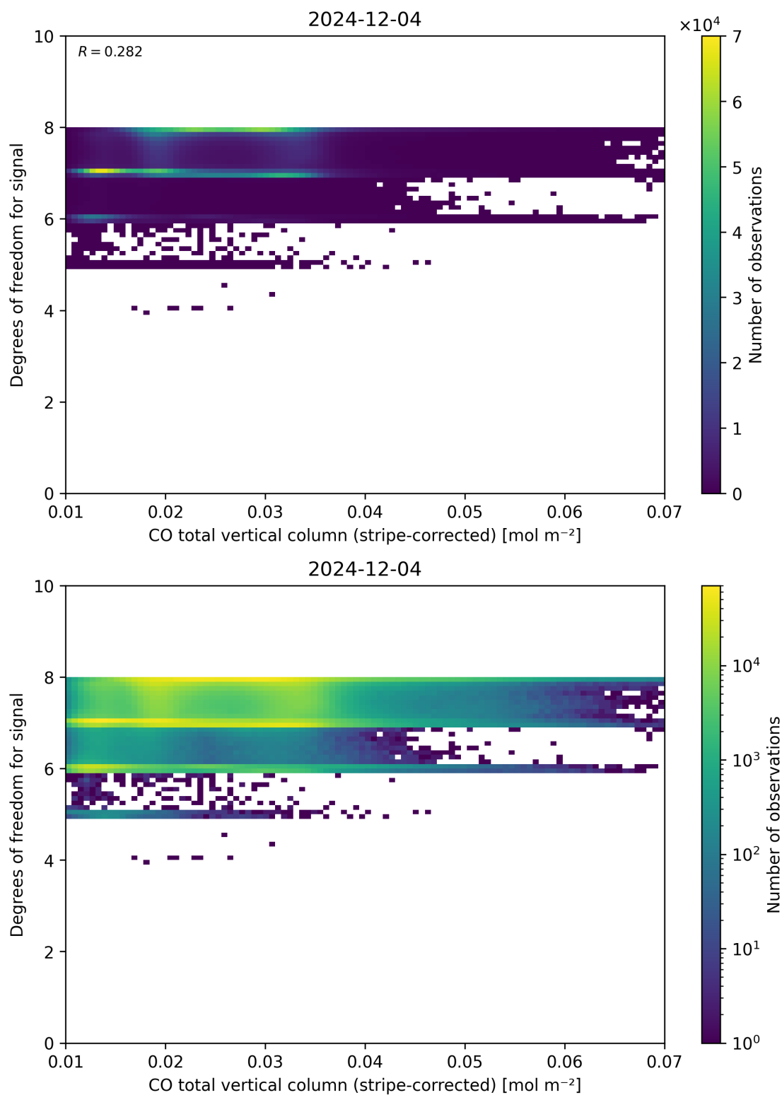
Figure 38: Scatter density plot of “CO total vertical column (stripe-corrected)” against “Degrees of freedom for signal” for 2024-12-03 to 2024-12-05.
