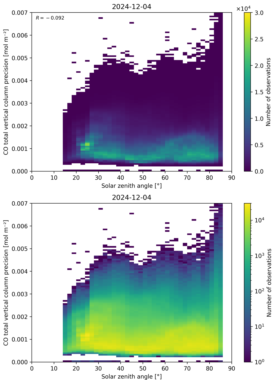
Figure 63: Scatter density plot of “Solar zenith angle” against “CO total vertical column precision” for 2024-12-03 to 2024-12-05.
