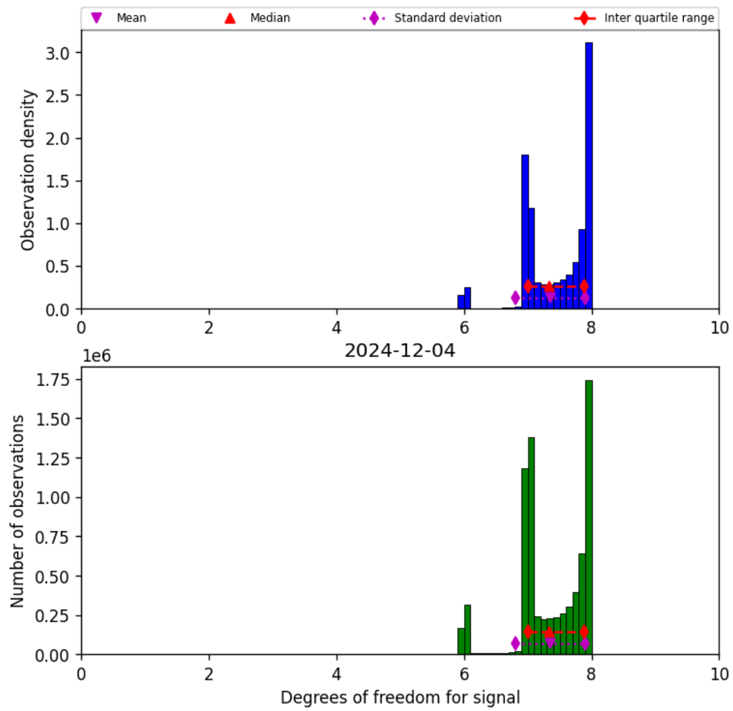
Figure 23: Histogram of “Degrees of freedom for signal” for 2024-12-03 to 2024-12-05
