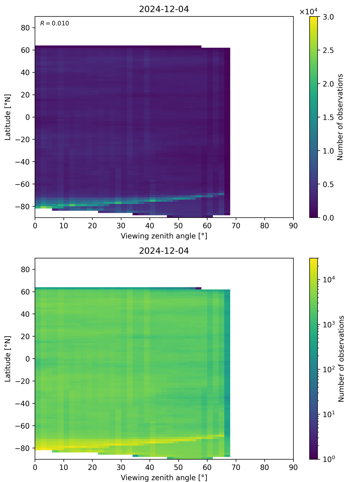
Figure 74: Scatter density plot of “Viewing zenith angle” against “Latitude” for 2024-12-03 to 2024-12-05.
