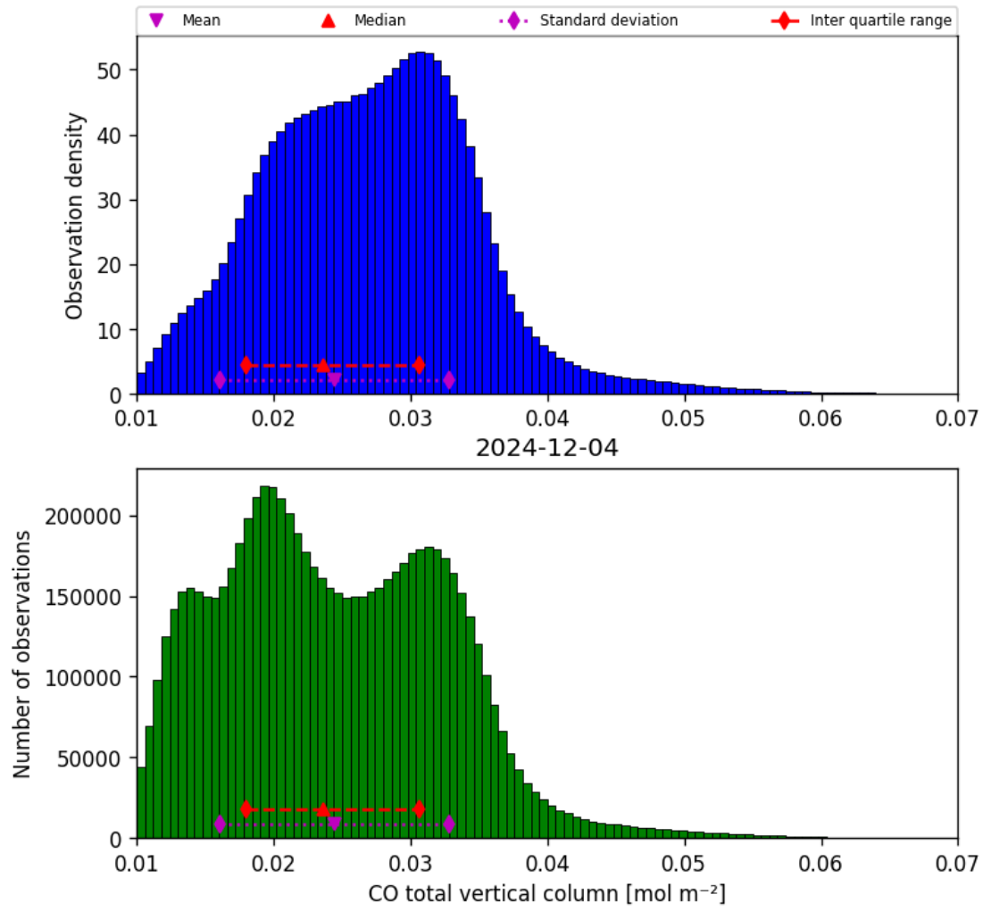
Figure 18: Histogram of “CO total vertical column” for 2024-12-03 to 2024-12-05
