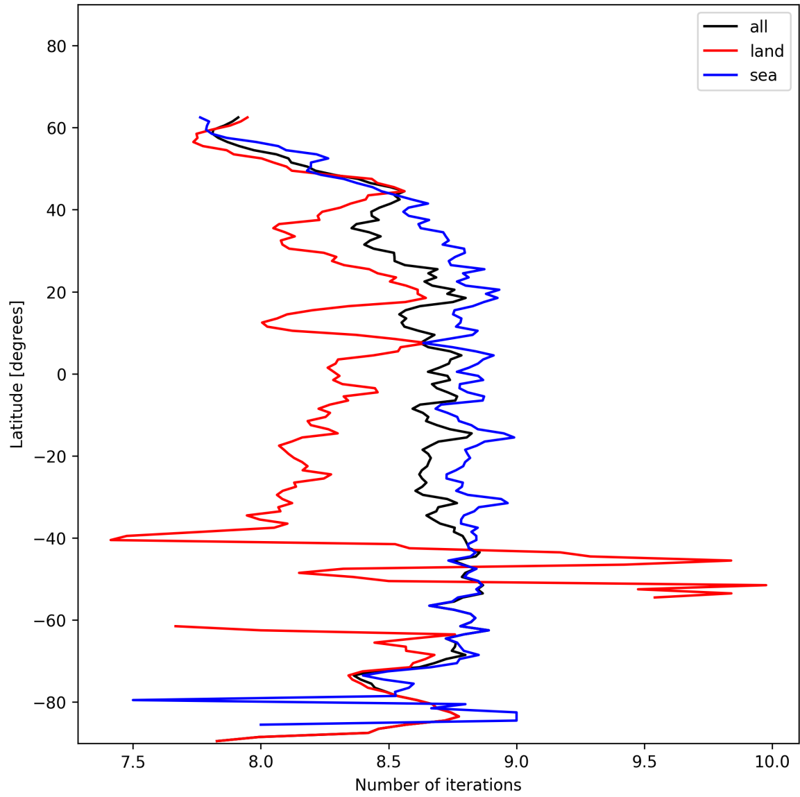
Figure 16: Zonal average of “Number of iterations” for 2024-12-03 to 2024-12-05.
