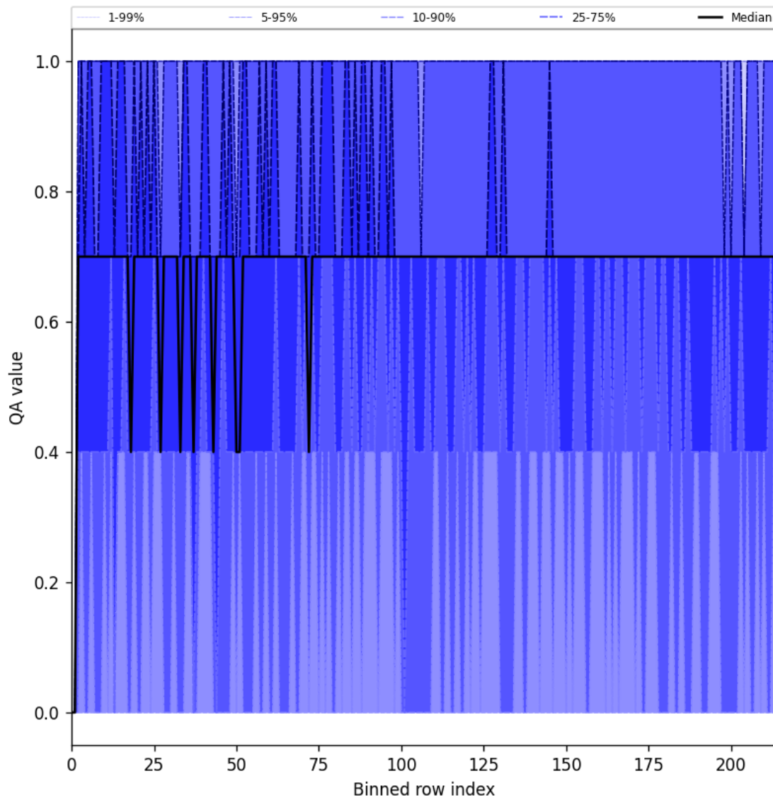
Figure 25: Along track statistics of “QA value” for 2024-12-03 to 2024-12-05
