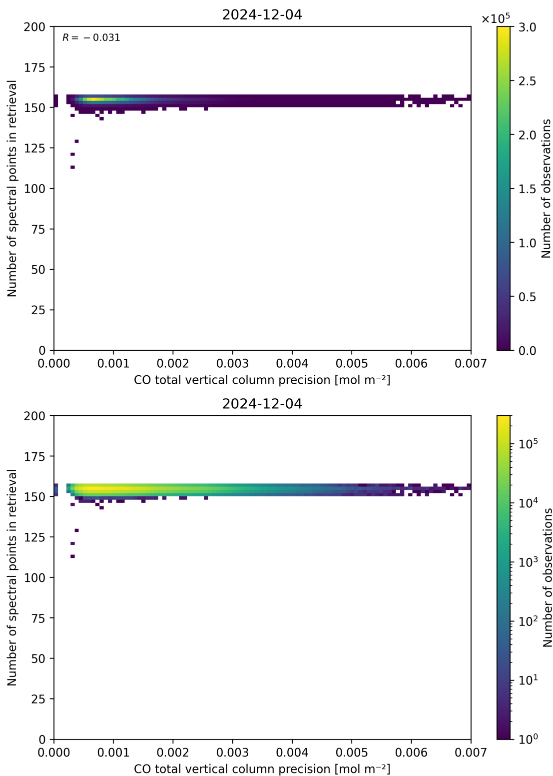
Figure 47: Scatter density plot of “CO total vertical column precision” against “Number of spectral points in retrieval” for 2024-12-03 to 2024-12-05.
