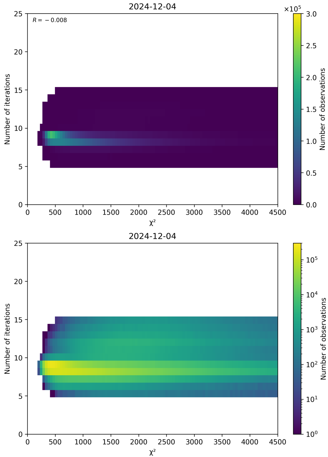
Figure 49: Scatter density plot of “ \chi^2 ” against “Number of iterations” for 2024-12-03 to 2024-12-05.
