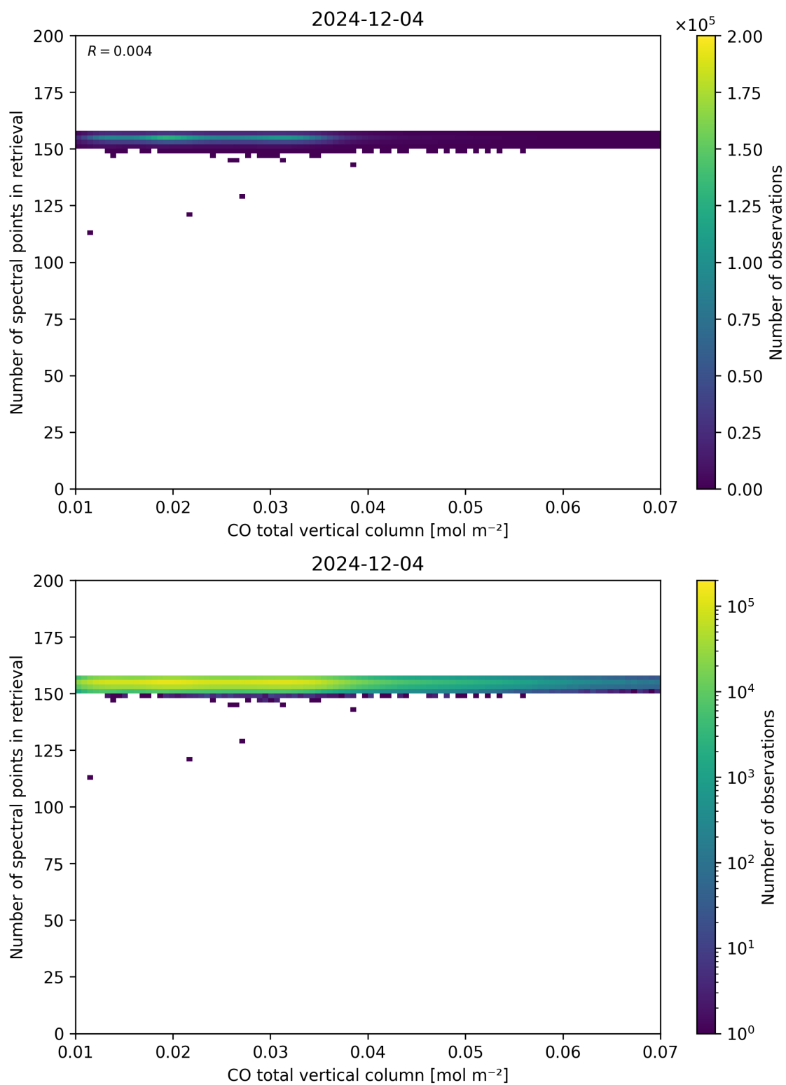
Figure 43: Scatter density plot of “CO total vertical column” against “Number of spectral points in retrieval” for 2024-12-03 to 2024-12-05.
