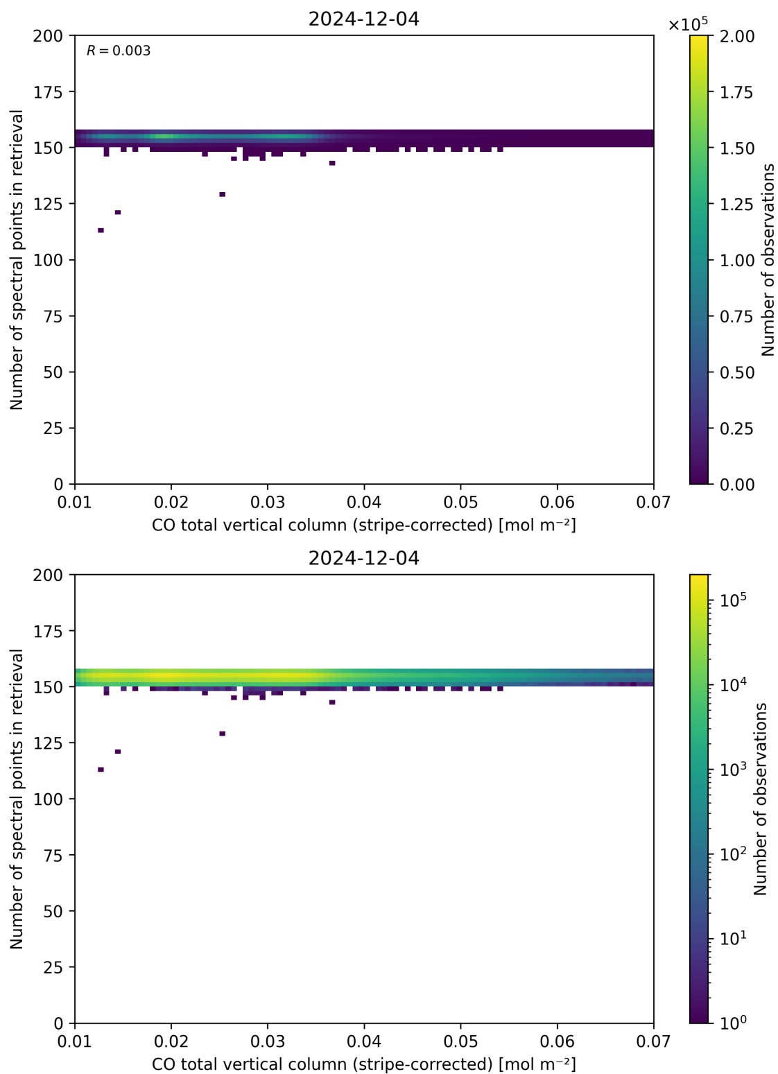
Figure 40: Scatter density plot of “CO total vertical column (stripe-corrected)” against “Number of spectral points in retrieval” for 2024-12-03 to 2024-12-05.
