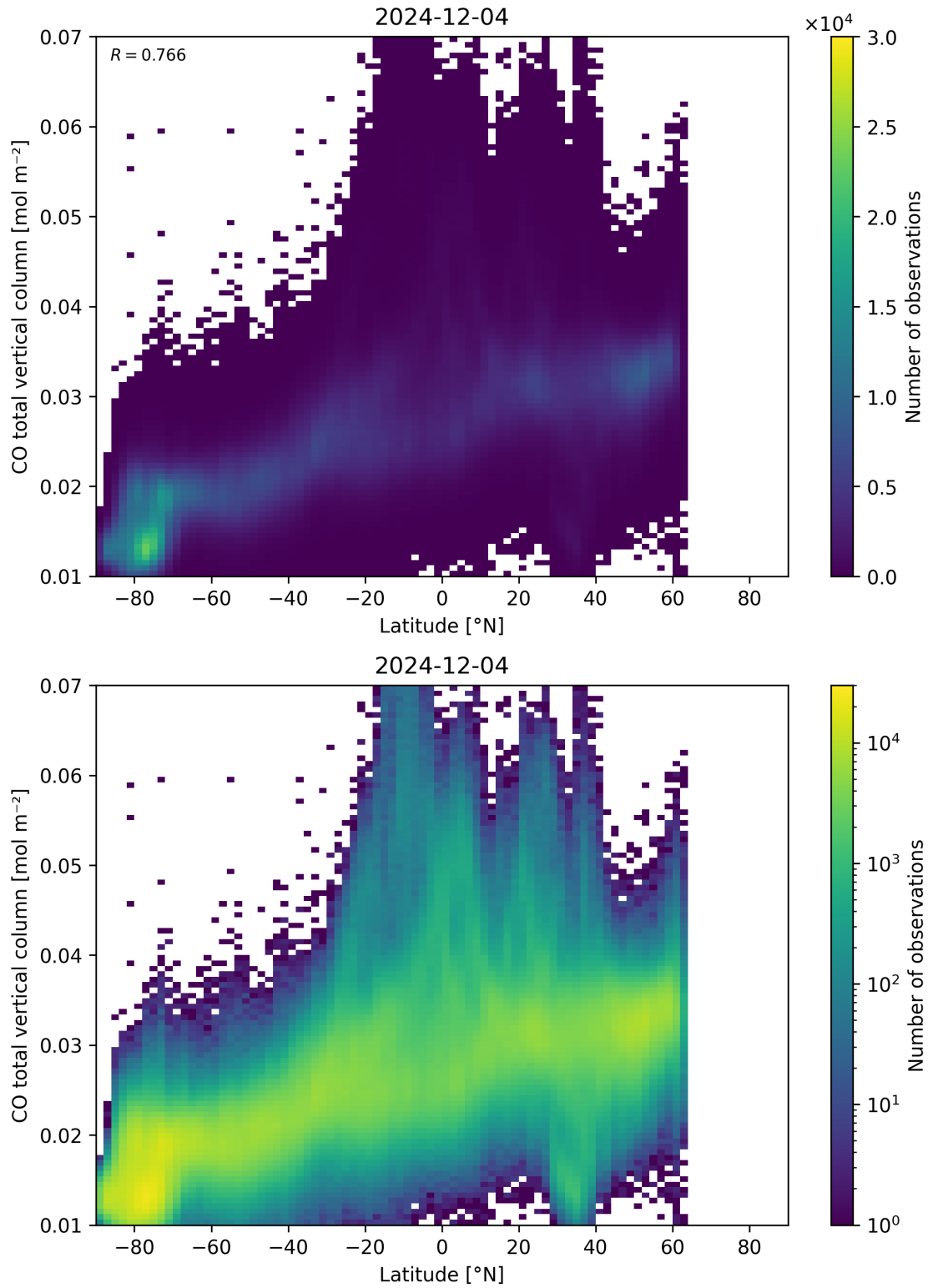
Figure 51: Scatter density plot of “Latitude” against “CO total vertical column” for 2024-12-03 to 2024-12-05.
