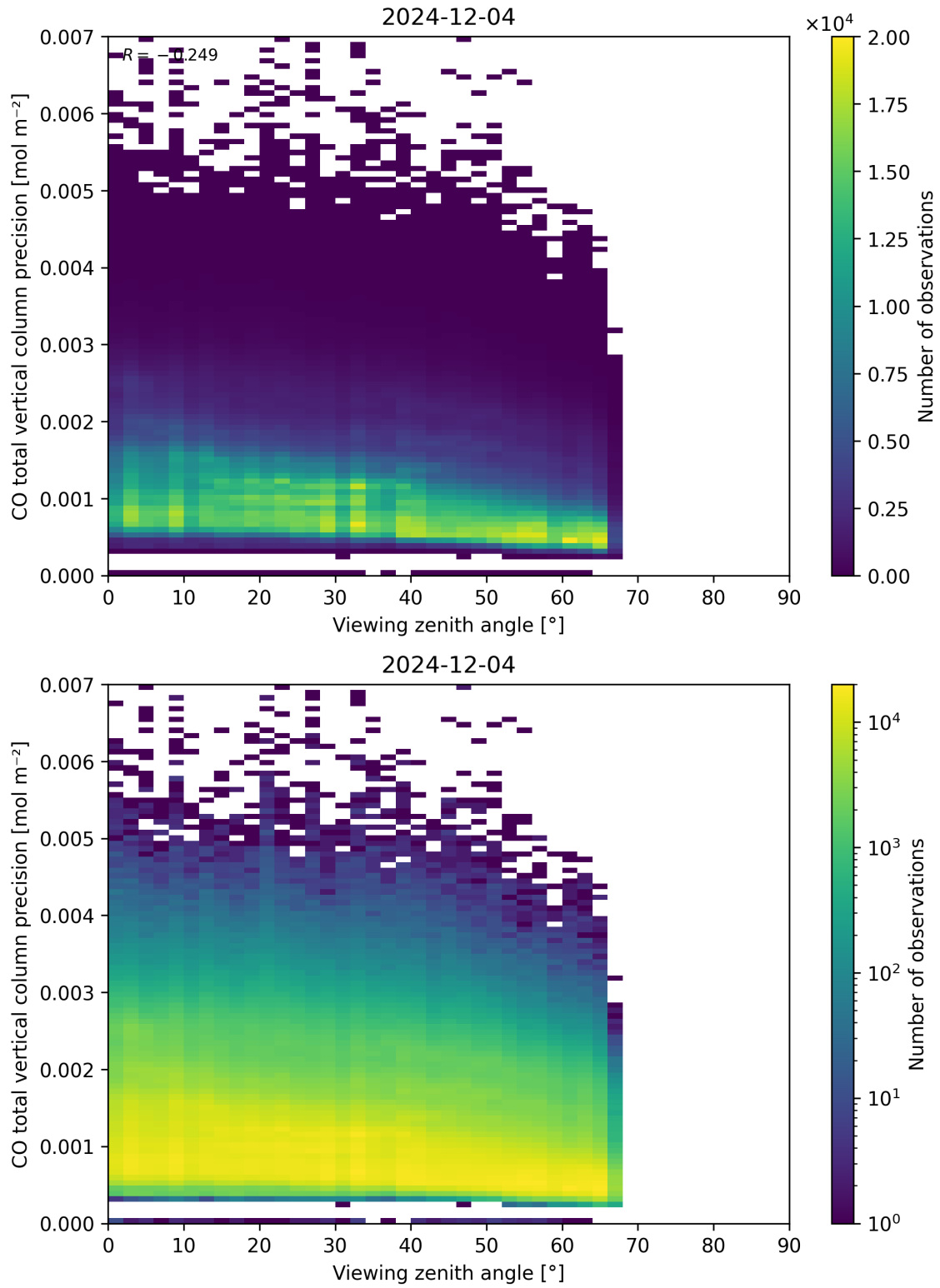
Figure 71: Scatter density plot of “Viewing zenith angle” against “CO total vertical column precision” for 2024-12-03 to 2024-12-05.
