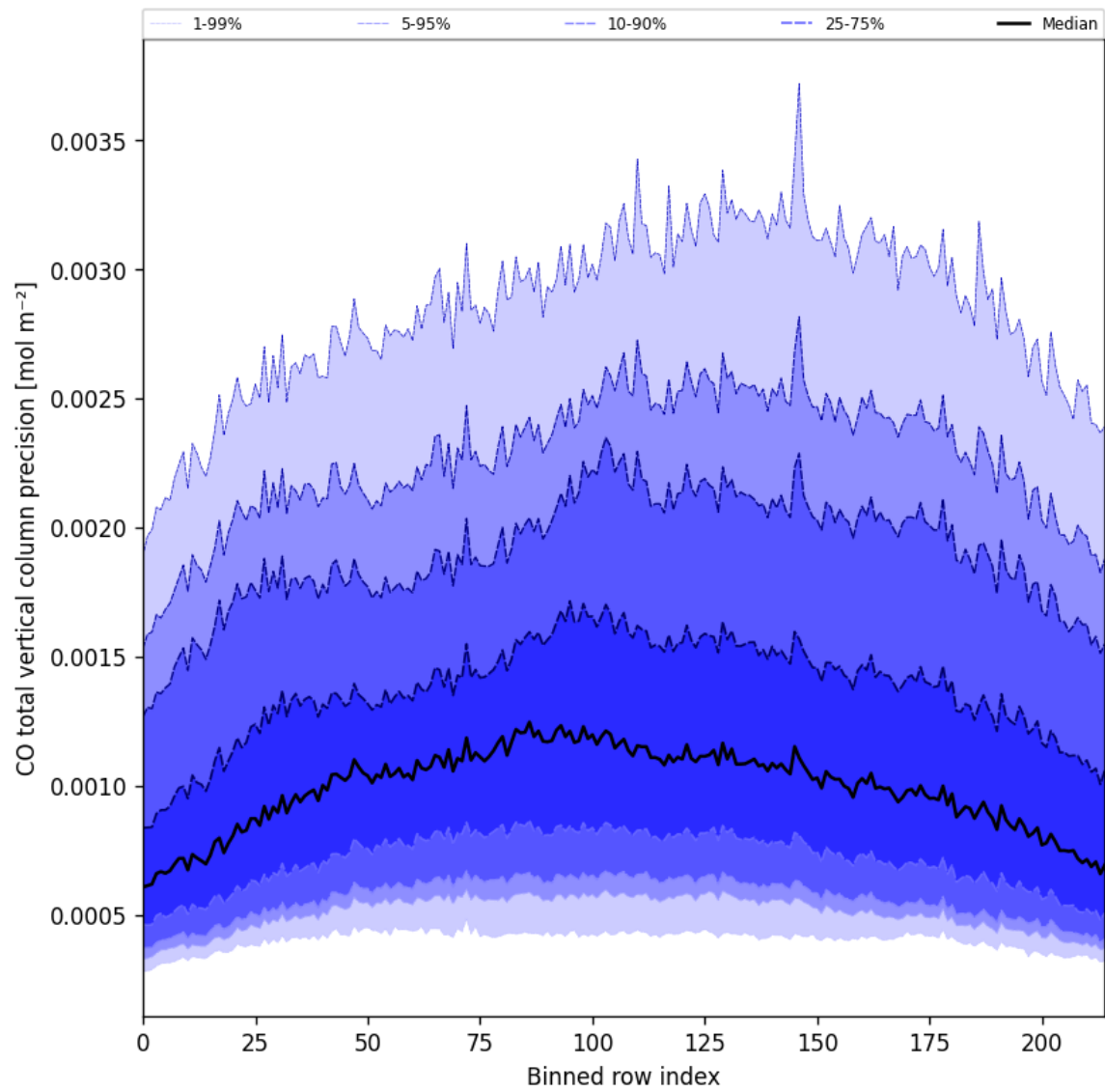
Figure 28: Along track statistics of “CO total vertical column precision” for 2024-12-03 to 2024-12-05
