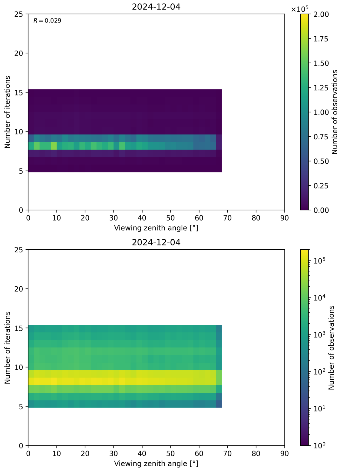
Figure 75: Scatter density plot of “Viewing zenith angle” against “Number of iterations” for 2024-12-03 to 2024-12-05.
