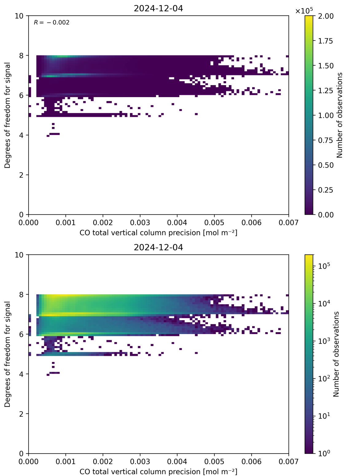
Figure 45: Scatter density plot of “CO total vertical column precision” against “Degrees of freedom for signal” for 2024-12-03 to 2024-12-05.
