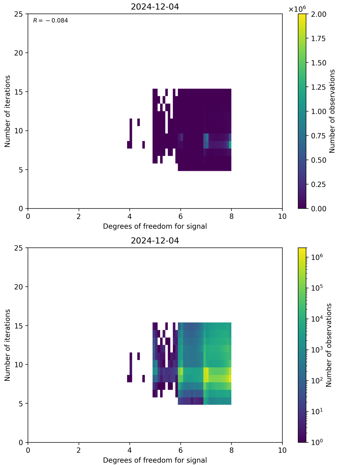
Figure 50: Scatter density plot of “Degrees of freedom for signal” against “Number of iterations” for 2024-12-03 to 2024-12-05.
