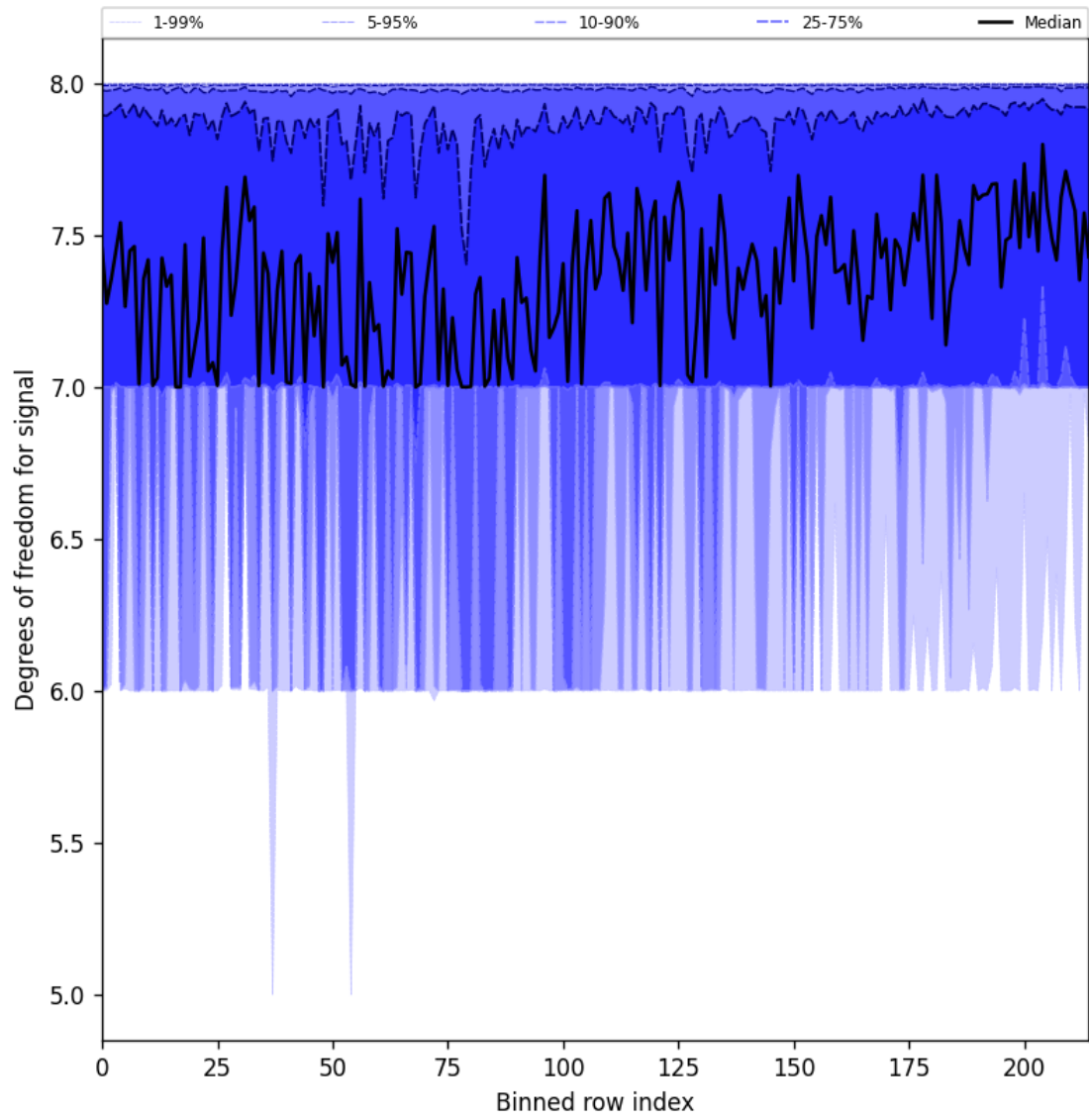
Figure 31: Along track statistics of “Degrees of freedom for signal” for 2024-12-03 to 2024-12-05
