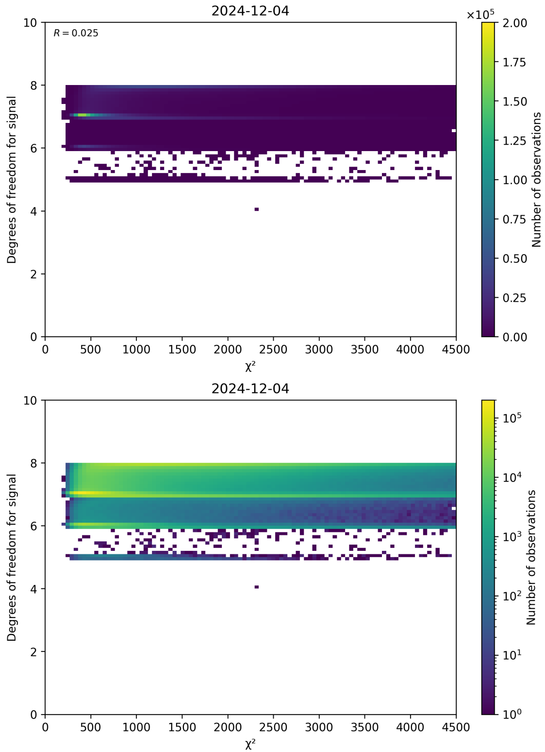
Figure 48: Scatter density plot of “ \chi^2 ” against “Degrees of freedom for signal” for 2024-12-03 to 2024-12-05.
