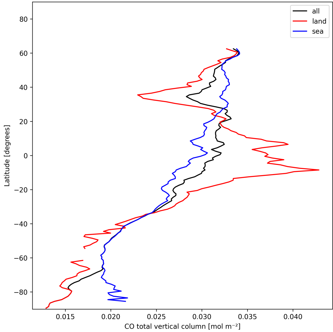
Figure 10: Zonal average of “CO total vertical column” for 2024-12-03 to 2024-12-05.
