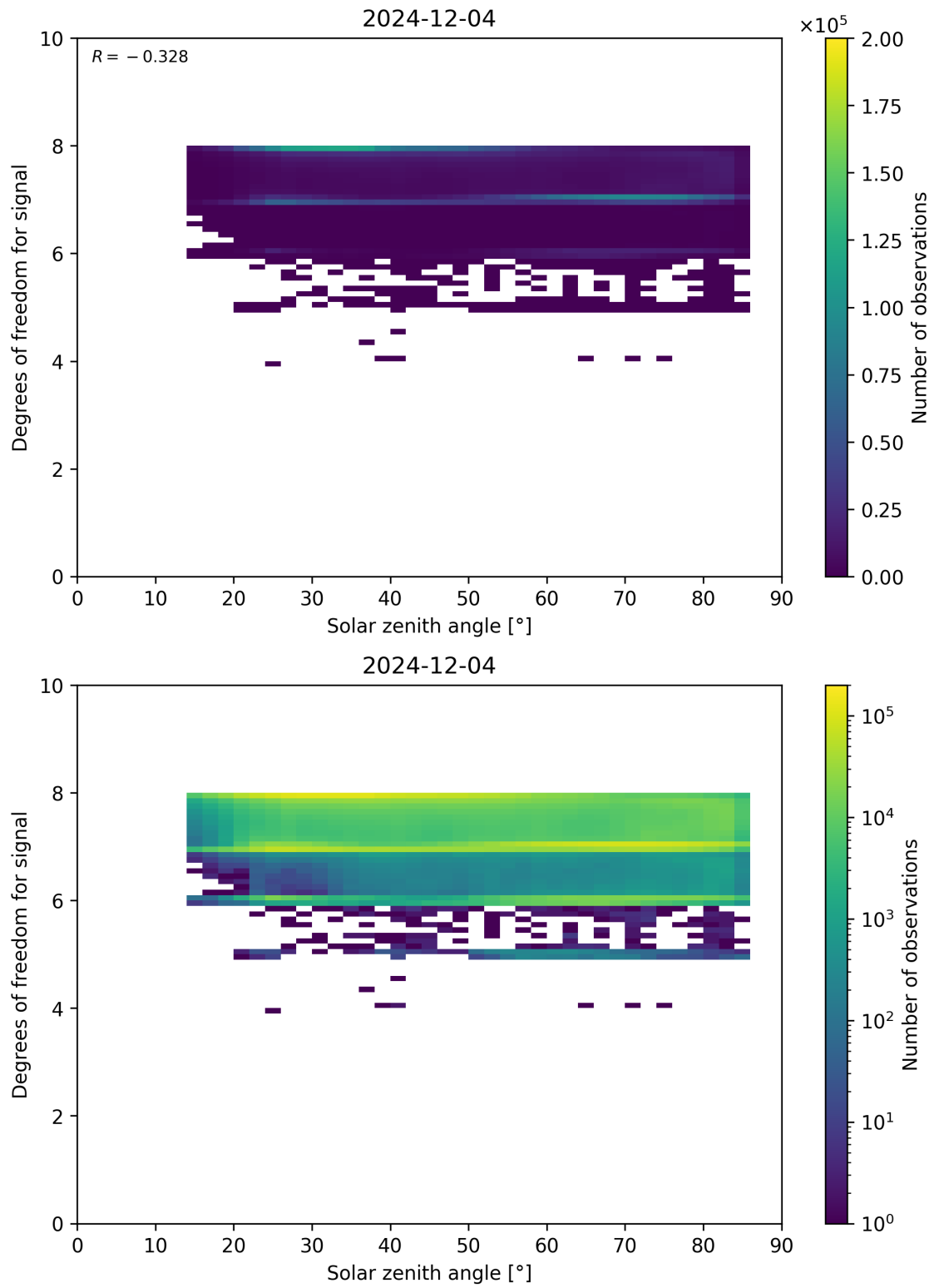
Figure 65: Scatter density plot of “Solar zenith angle” against “Degrees of freedom for signal” for 2024-12-03 to 2024-12-05.
