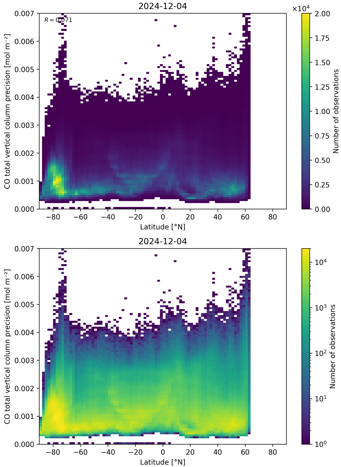
Figure 53: Scatter density plot of “Latitude” against “CO total vertical column precision” for 2024-12-03 to 2024-12-05.
