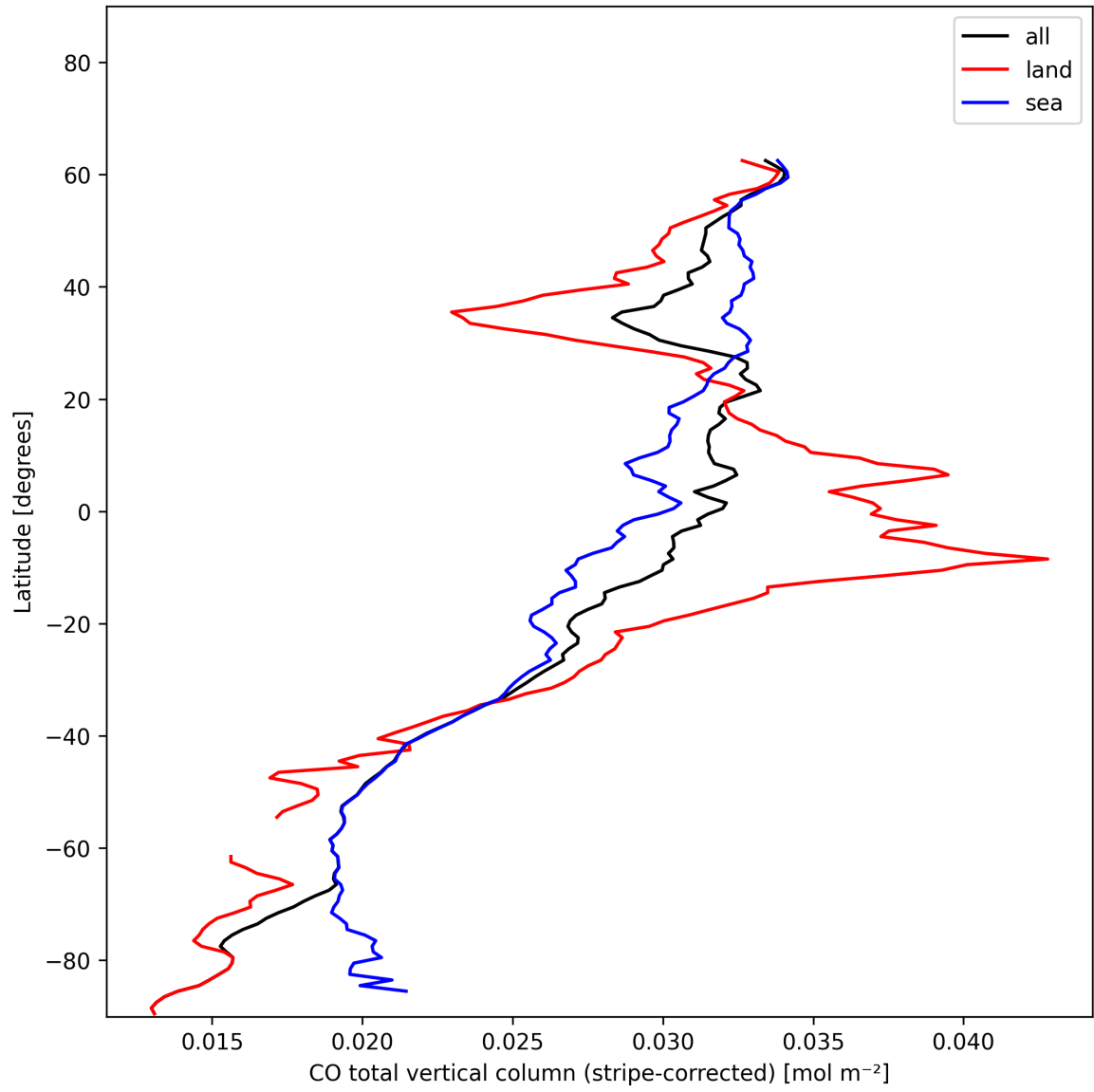
Figure 11: Zonal average of “CO total vertical column (stripe-corrected)” for 2024-12-03 to 2024-12-05.
