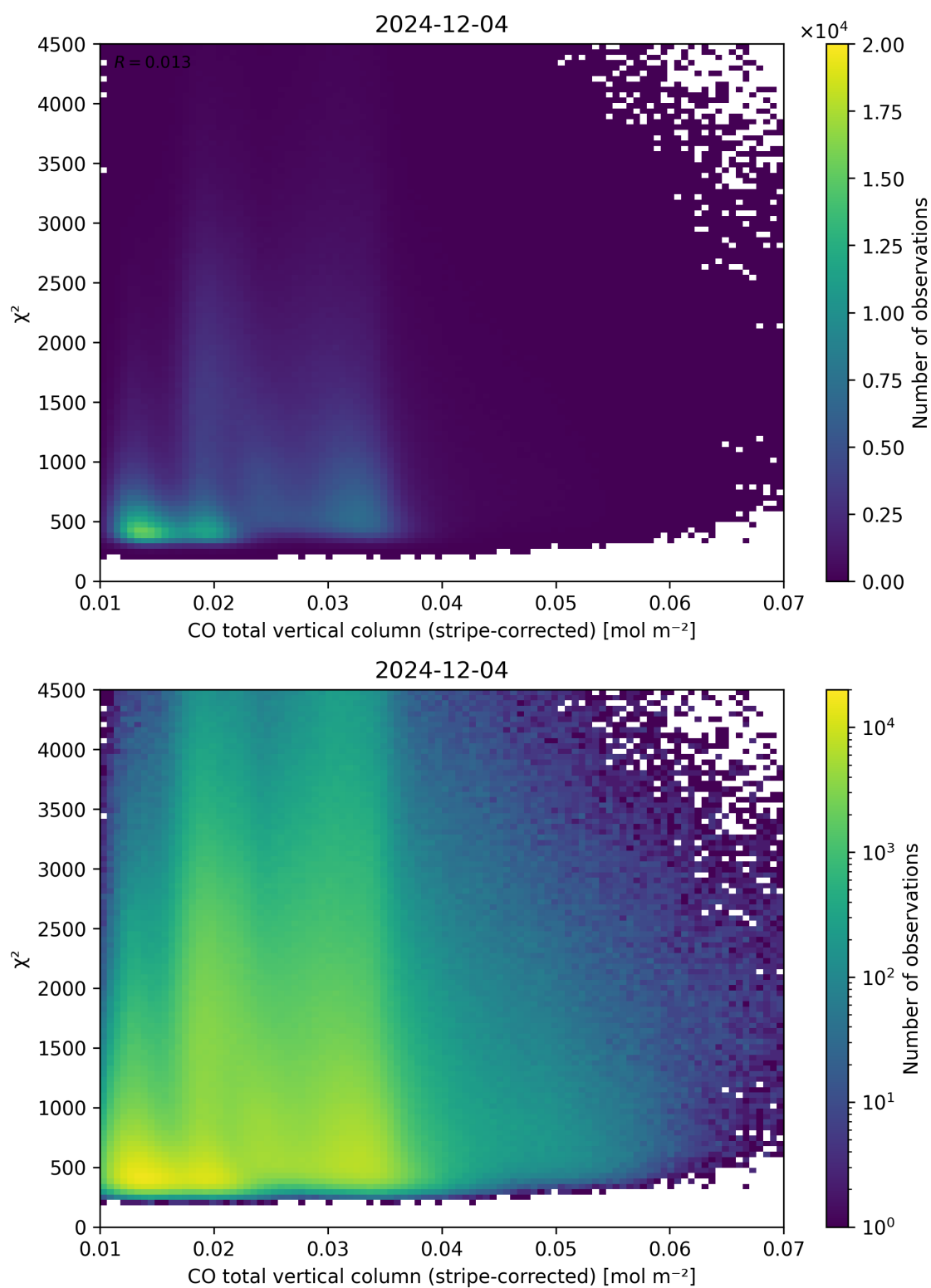
Figure 37: Scatter density plot of “CO total vertical column (stripe-corrected)” against “ \chi^2 ” for 2024-12-03 to 2024-12-05.
