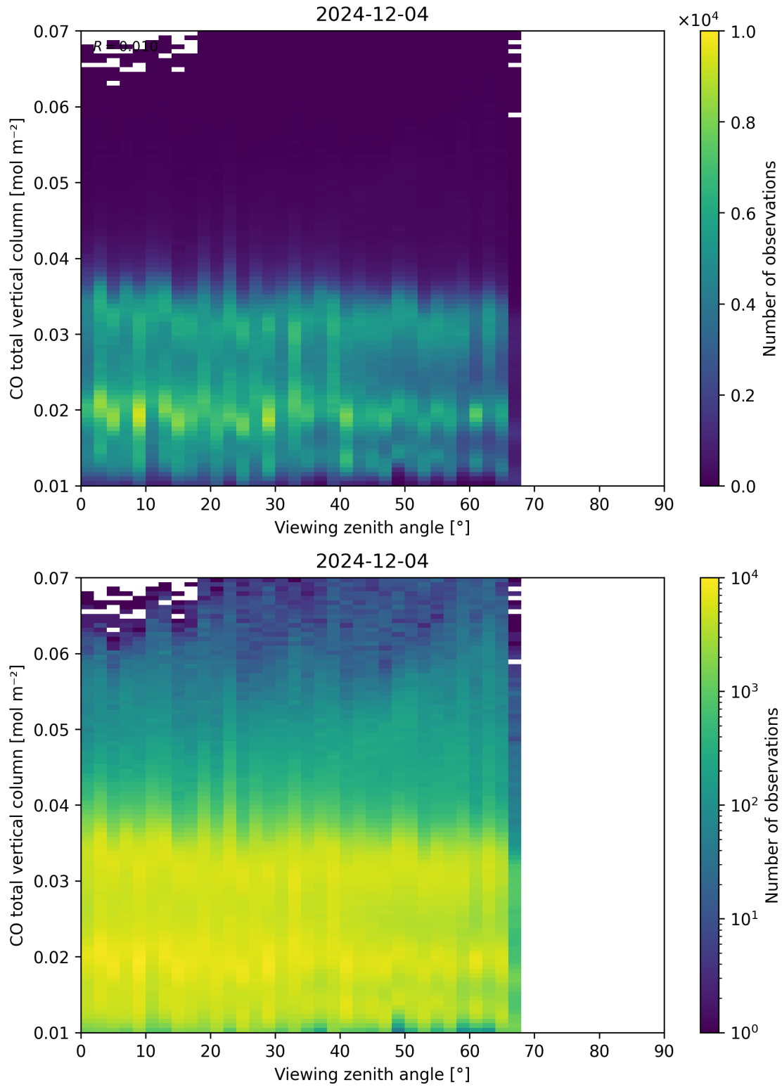
Figure 69: Scatter density plot of “Viewing zenith angle” against “CO total vertical column” for 2024-12-03 to 2024-12-05.
