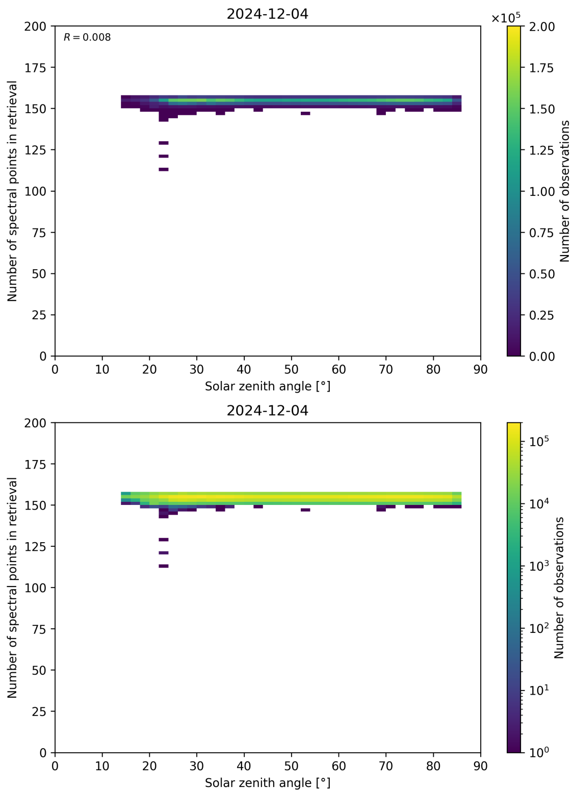
Figure 68: Scatter density plot of “Solar zenith angle” against “Number of spectral points in retrieval” for 2024-12-03 to 2024-12-05.
