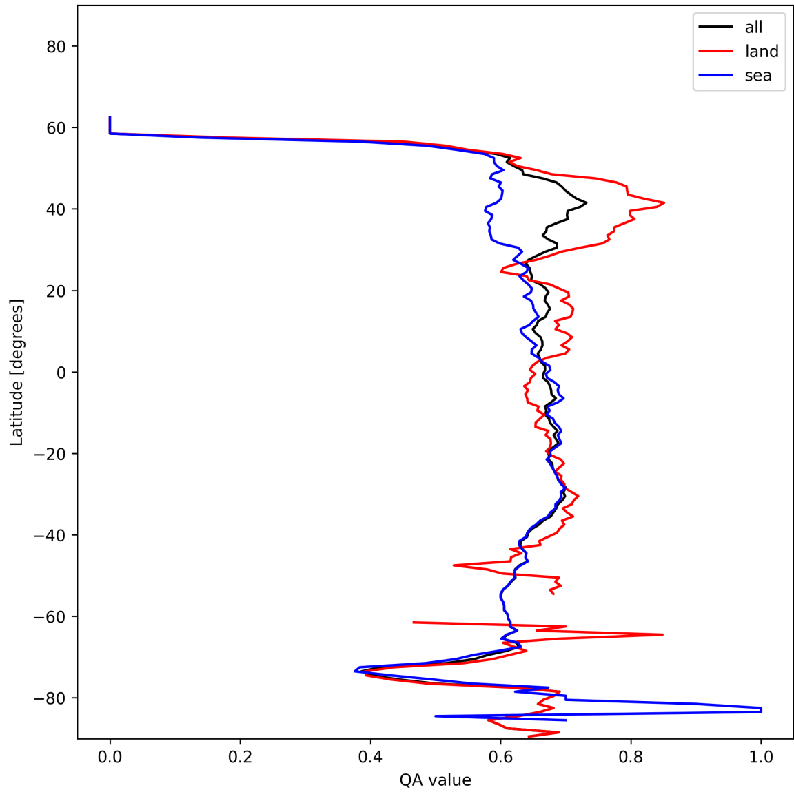
Figure 9: Zonal average of “QA value” for 2024-12-03 to 2024-12-05.
