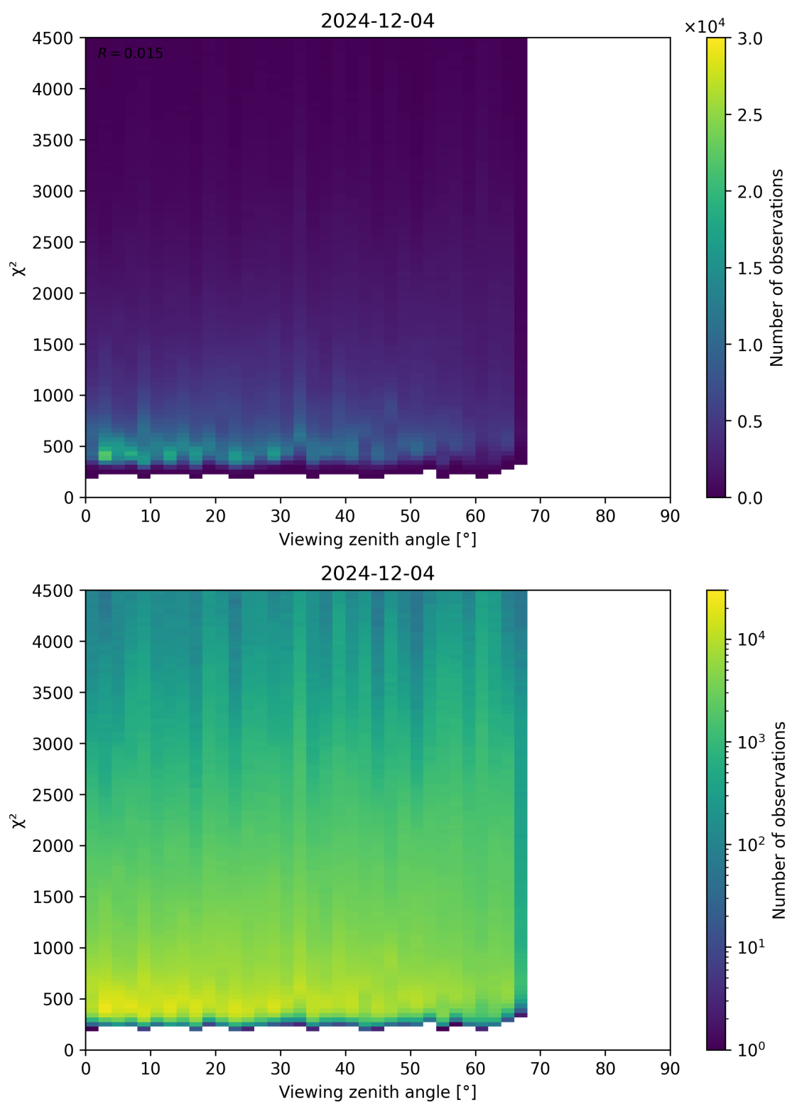
Figure 72: Scatter density plot of “Viewing zenith angle” against “ \chi^2 ” for 2024-12-03 to 2024-12-05.
