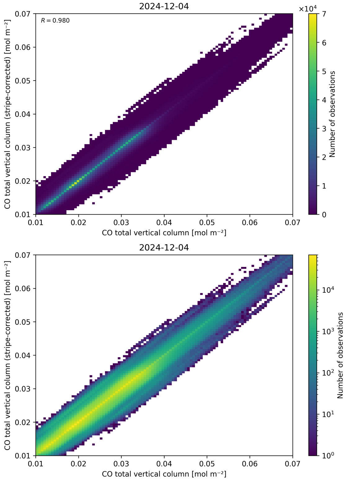
Figure 33: Scatter density plot of “CO total vertical column” against “CO total vertical column (stripe-corrected)” for 2024-12-03 to 2024-12-05.
