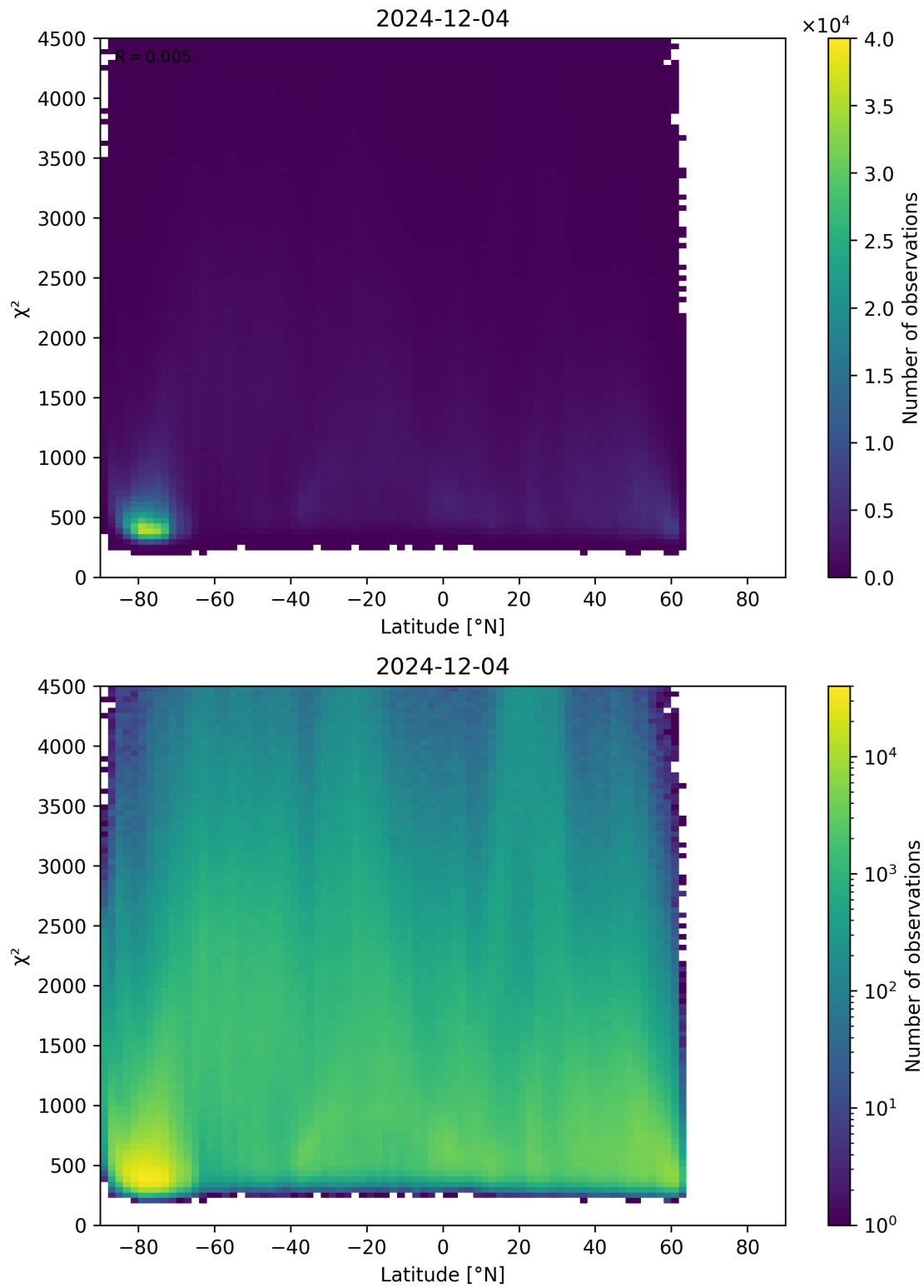
Figure 54: Scatter density plot of “Latitude” against “ \chi^2 ” for 2024-12-03 to 2024-12-05.
