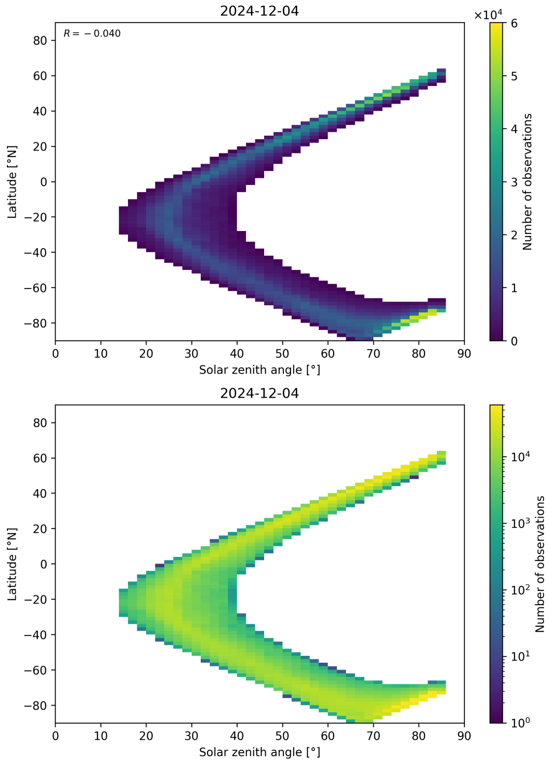
Figure 66: Scatter density plot of “Solar zenith angle” against “Latitude” for 2024-12-03 to 2024-12-05.
