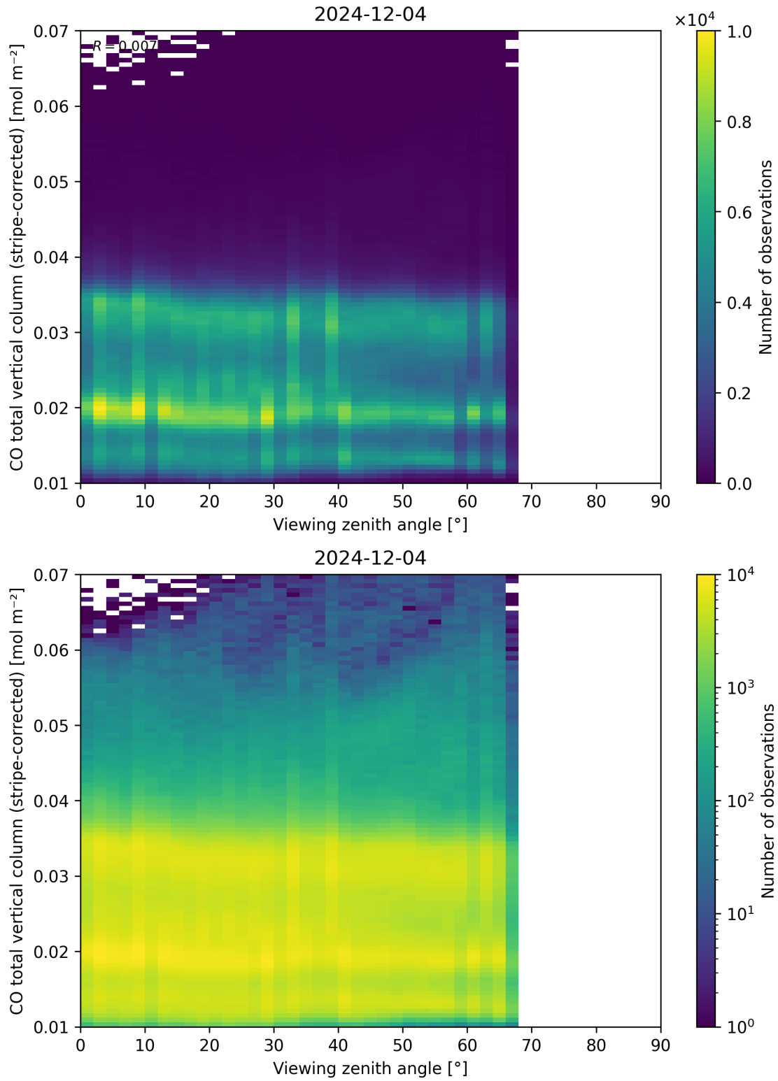
Figure 70: Scatter density plot of “Viewing zenith angle” against “CO total vertical column (stripe-corrected)” for 2024-12-03 to 2024-12-05.
