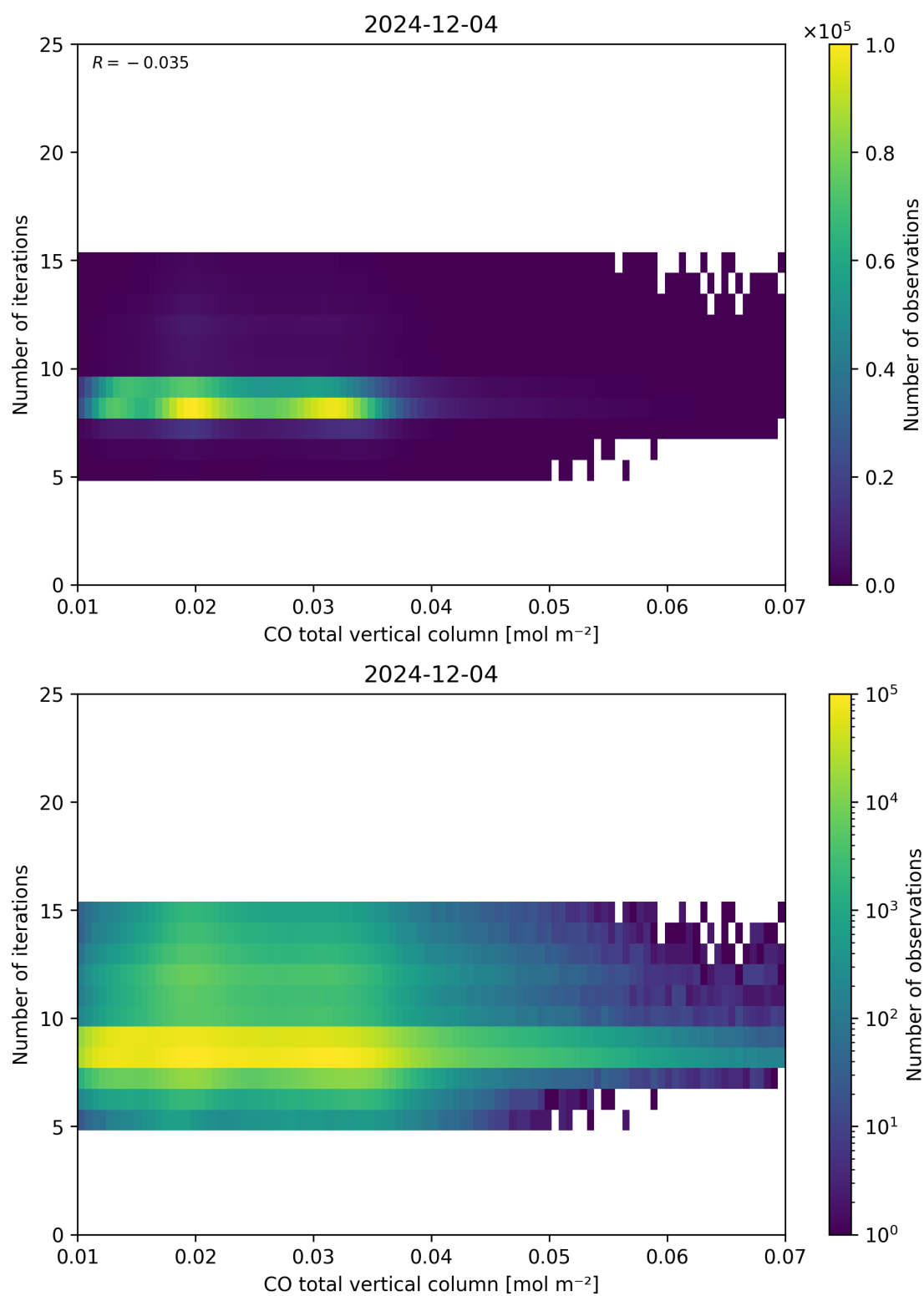
Figure 42: Scatter density plot of “CO total vertical column” against “Number of iterations” for 2024-12-03 to 2024-12-05.
