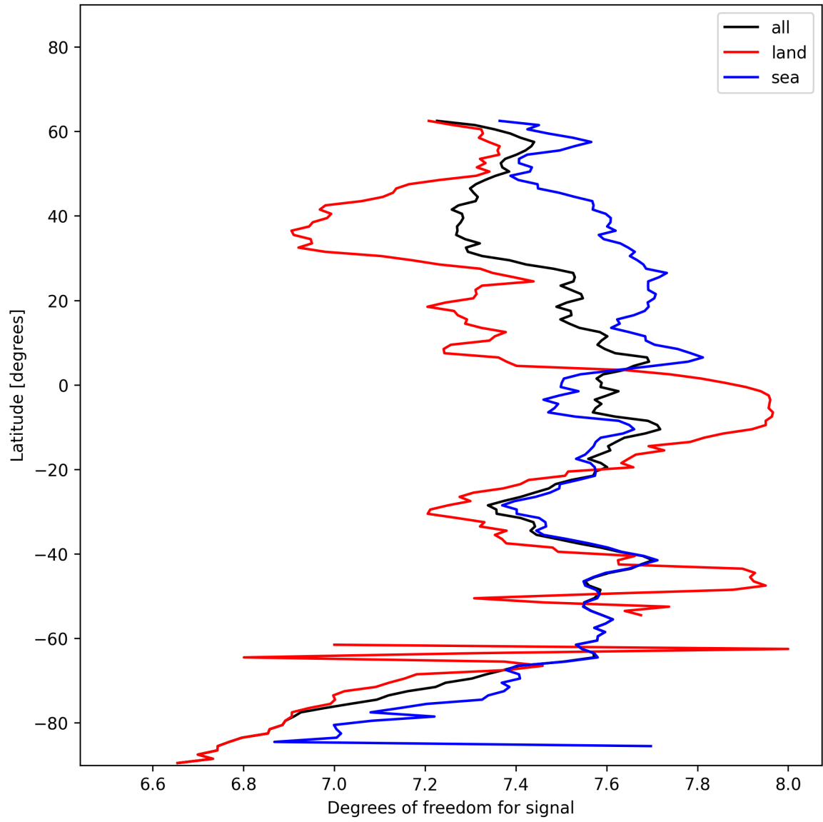
Figure 15: Zonal average of “Degrees of freedom for signal” for 2024-12-03 to 2024-12-05.
