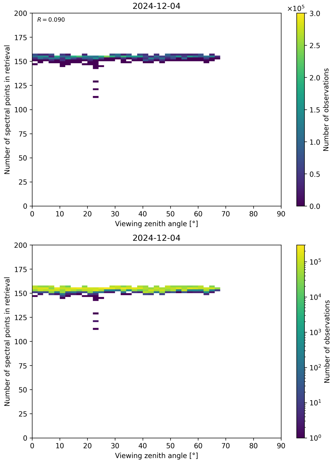
Figure 76: Scatter density plot of “Viewing zenith angle” against “Number of spectral points in retrieval” for 2024-12-03 to 2024-12-05.
