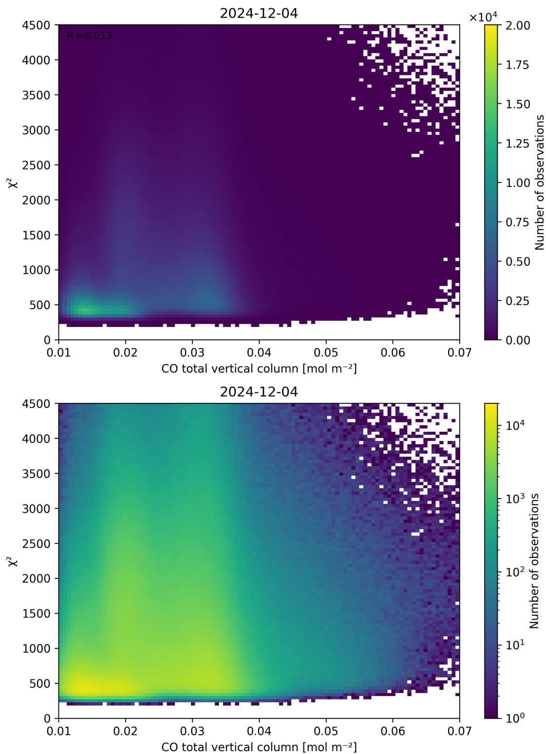
Figure 35: Scatter density plot of “CO total vertical column” against “ \chi^2 ” for 2024-12-03 to 2024-12-05.
