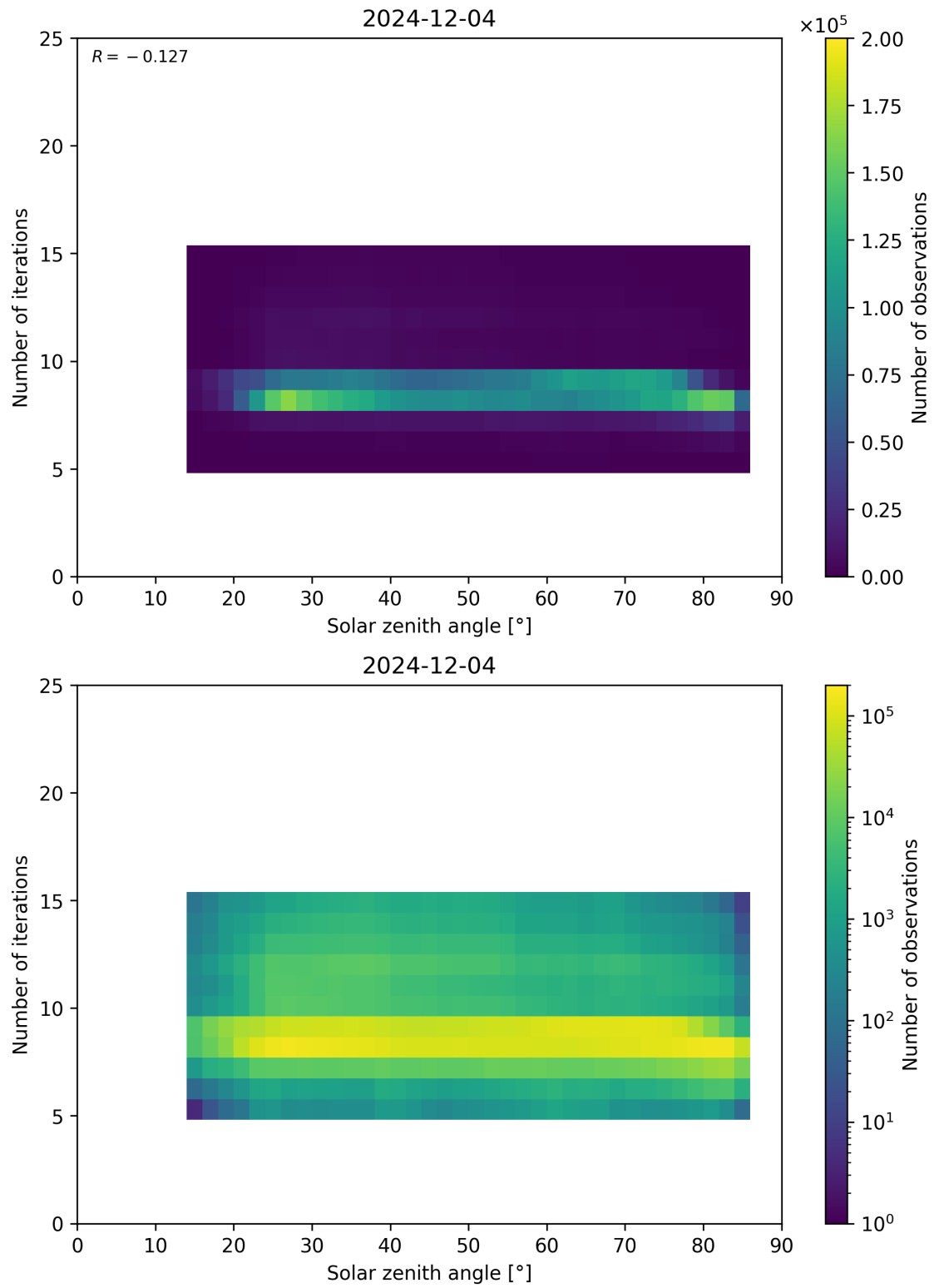
Figure 67: Scatter density plot of “Solar zenith angle” against “Number of iterations” for 2024-12-03 to 2024-12-05.
