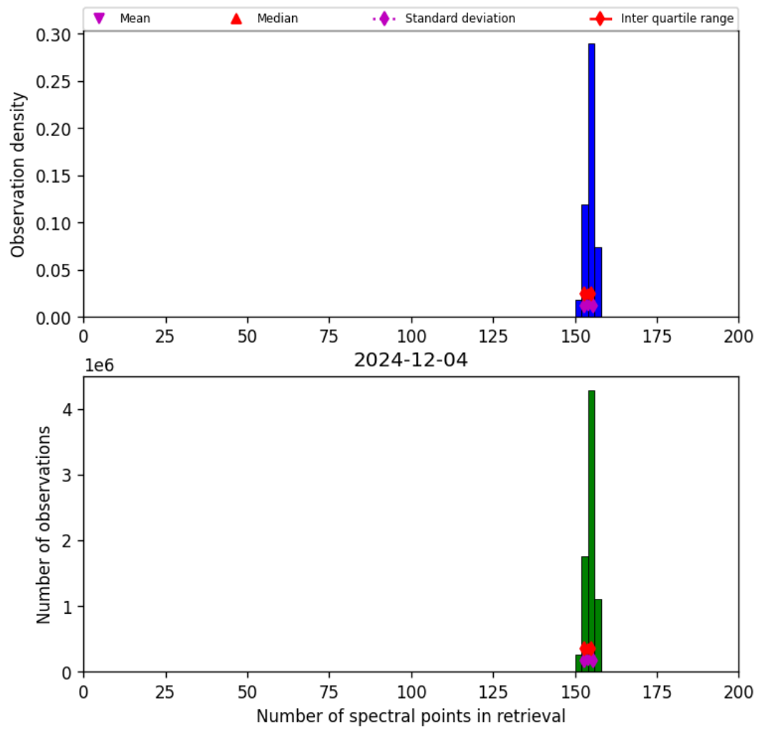
Figure 21: Histogram of “Number of spectral points in retrieval” for 2024-12-03 to 2024-12-05
