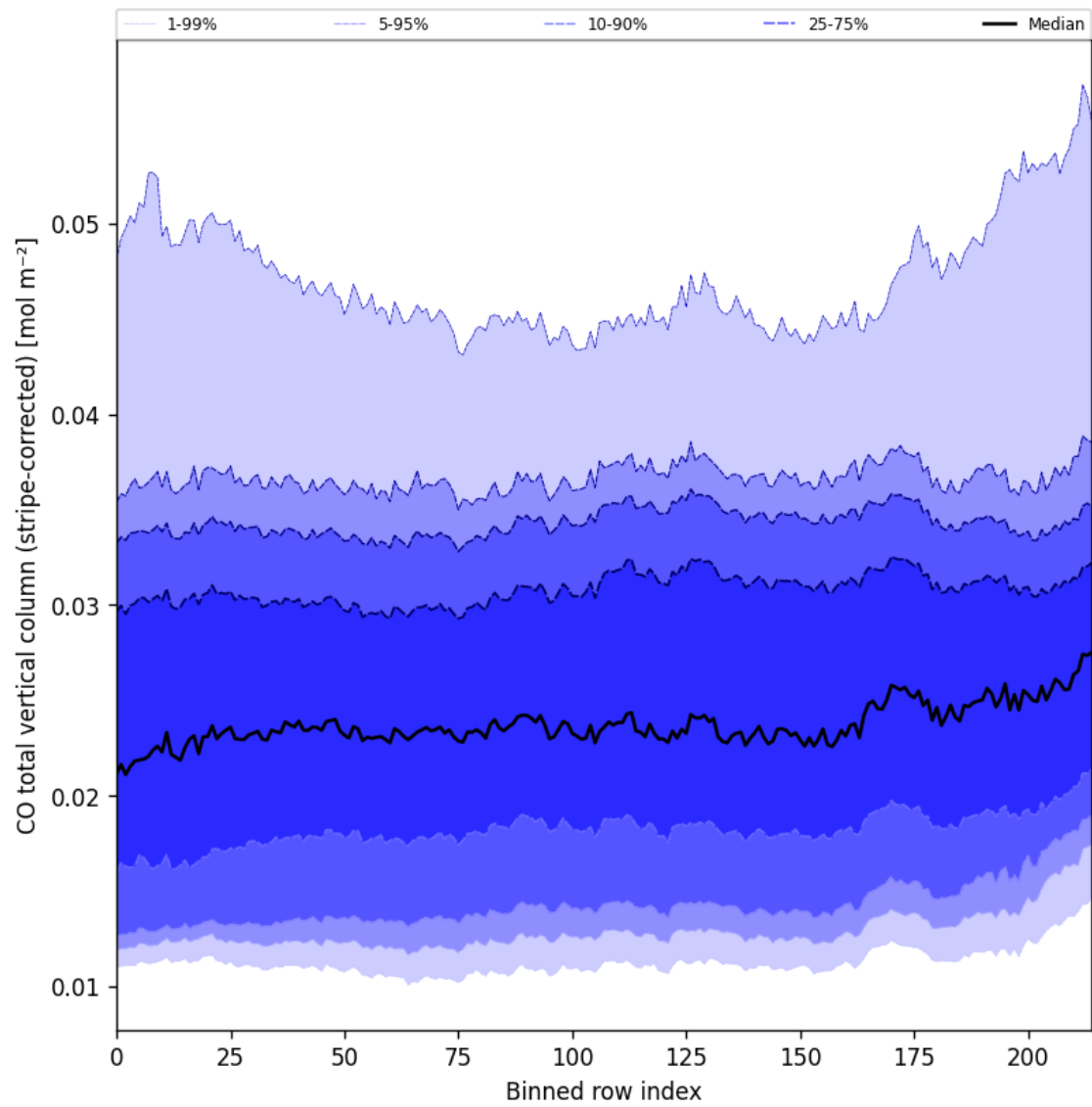
Figure 27: Along track statistics of “CO total vertical column (stripe-corrected)” for 2024-12-03 to 2024-12-05
