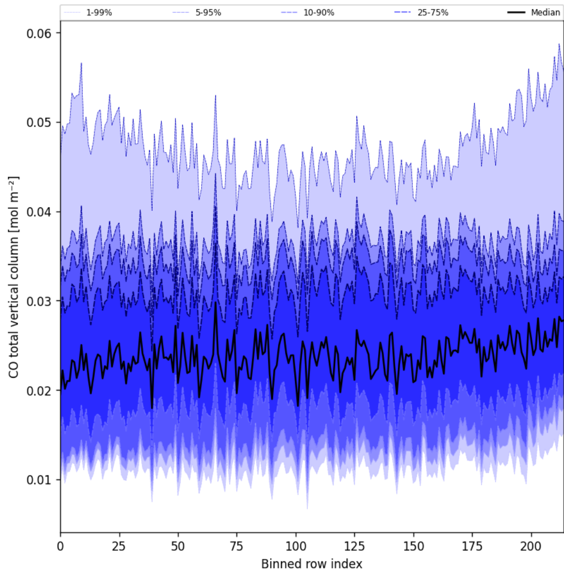
Figure 26: Along track statistics of “CO total vertical column” for 2024-12-03 to 2024-12-05
