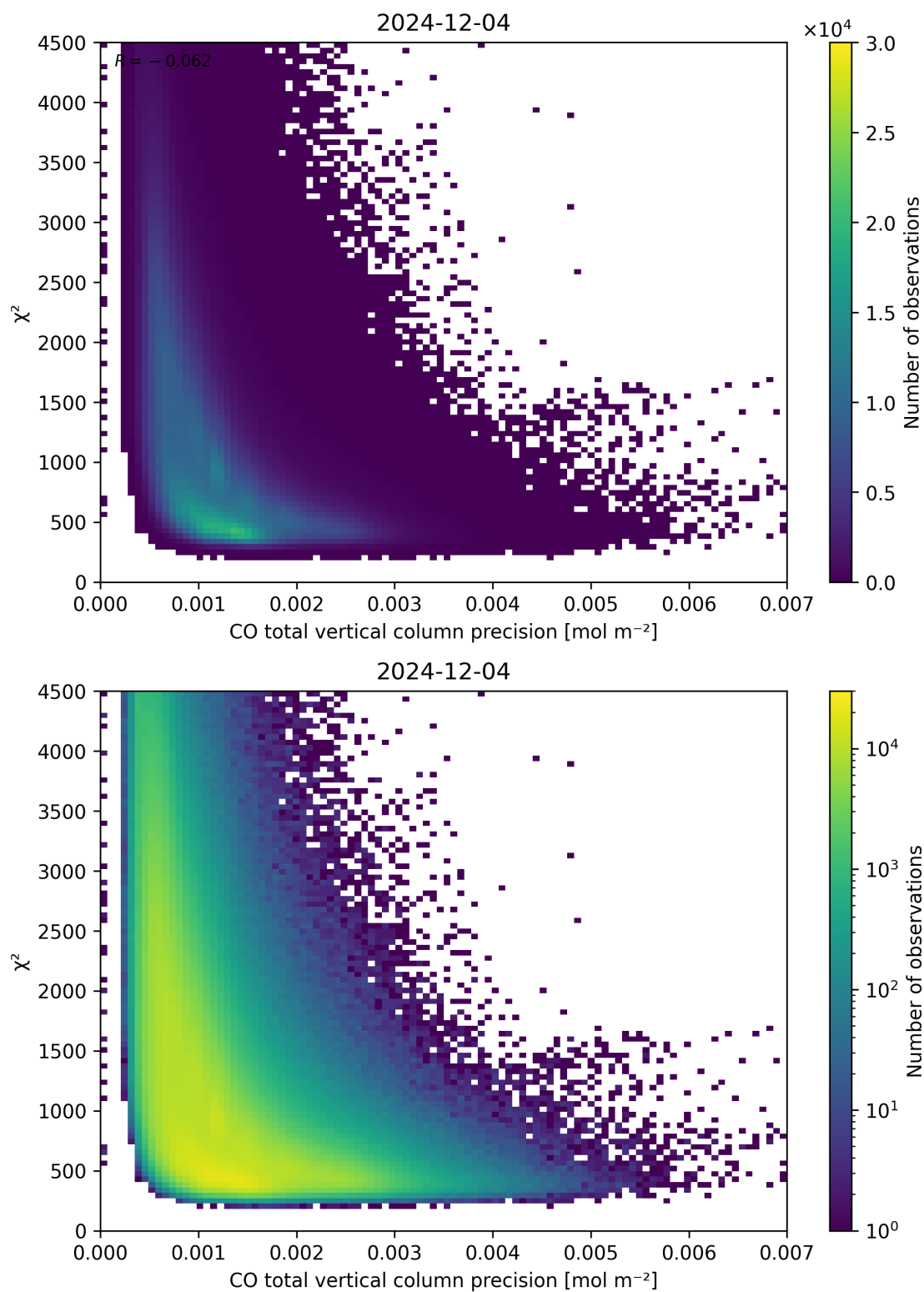
Figure 44: Scatter density plot of “CO total vertical column precision” against “ \chi^2 ” for 2024-12-03 to 2024-12-05.
