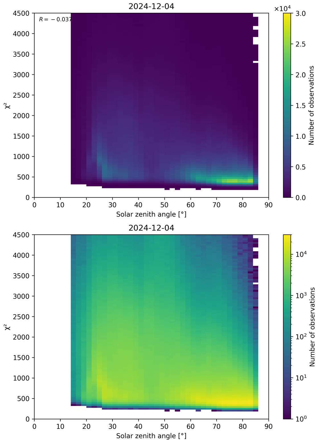
Figure 64: Scatter density plot of “Solar zenith angle” against “ \chi^2 ” for 2024-12-03 to 2024-12-05.
