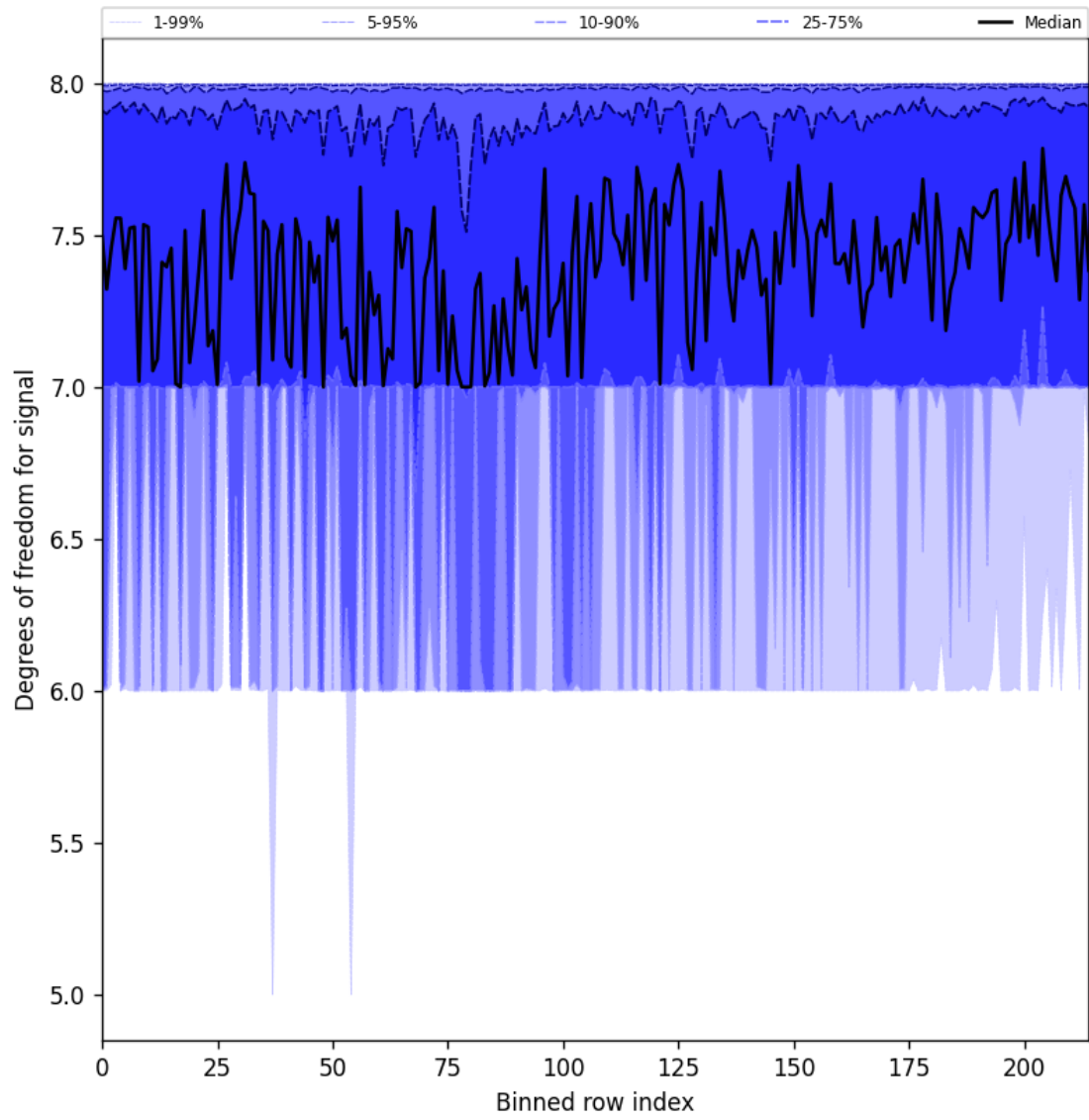
Figure 31: Along track statistics of “Degrees of freedom for signal” for 2024-12-04 to 2024-12-06
