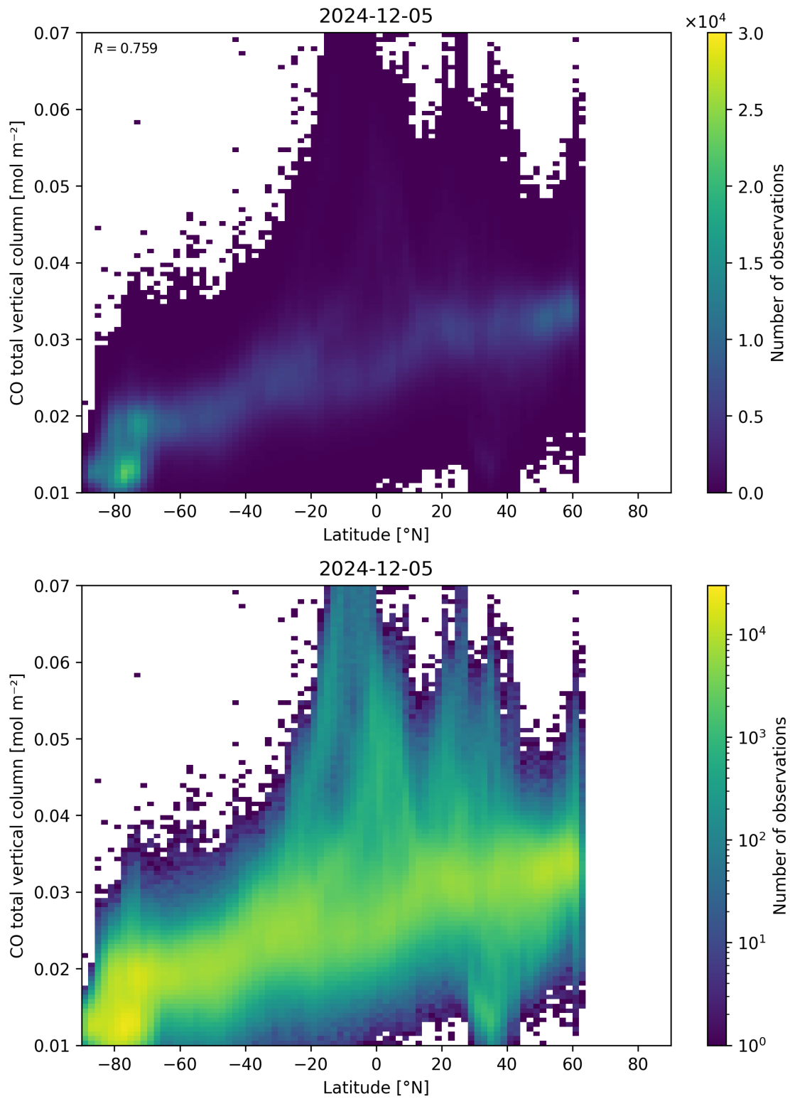
Figure 51: Scatter density plot of “Latitude” against “CO total vertical column” for 2024-12-04 to 2024-12-06.
