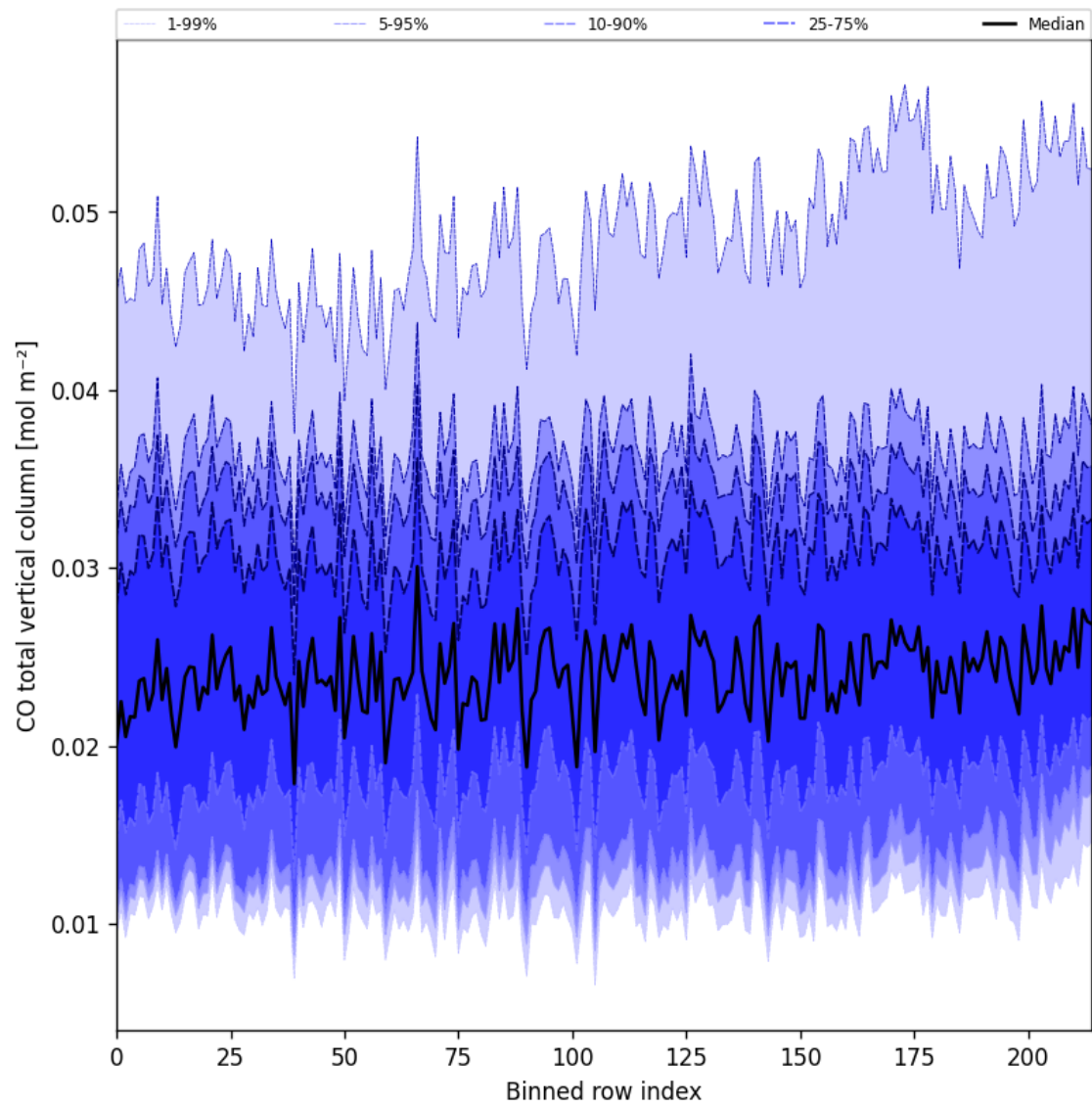
Figure 26: Along track statistics of “CO total vertical column” for 2024-12-04 to 2024-12-06
