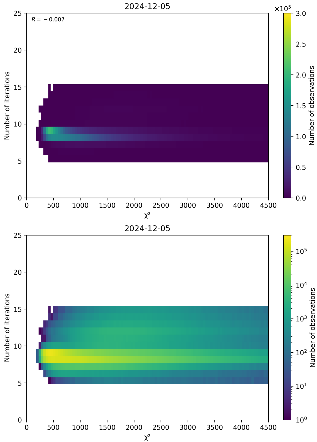
Figure 49: Scatter density plot of “ \chi^2 ” against “Number of iterations” for 2024-12-04 to 2024-12-06.
