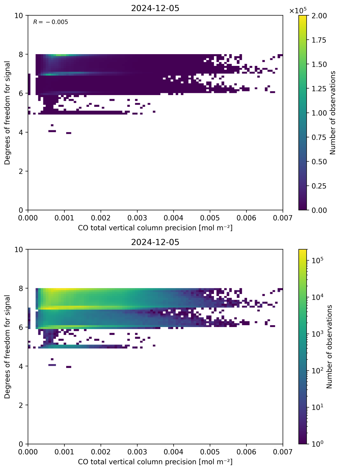
Figure 45: Scatter density plot of “CO total vertical column precision” against “Degrees of freedom for signal” for 2024-12-04 to 2024-12-06.
