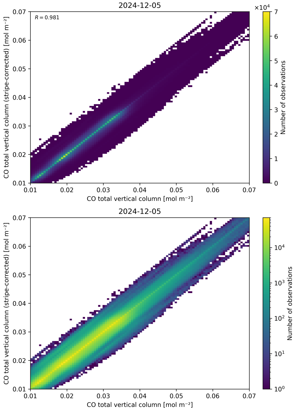
Figure 33: Scatter density plot of “CO total vertical column” against “CO total vertical column (stripe-corrected)” for 2024-12-04 to 2024-12-06.
