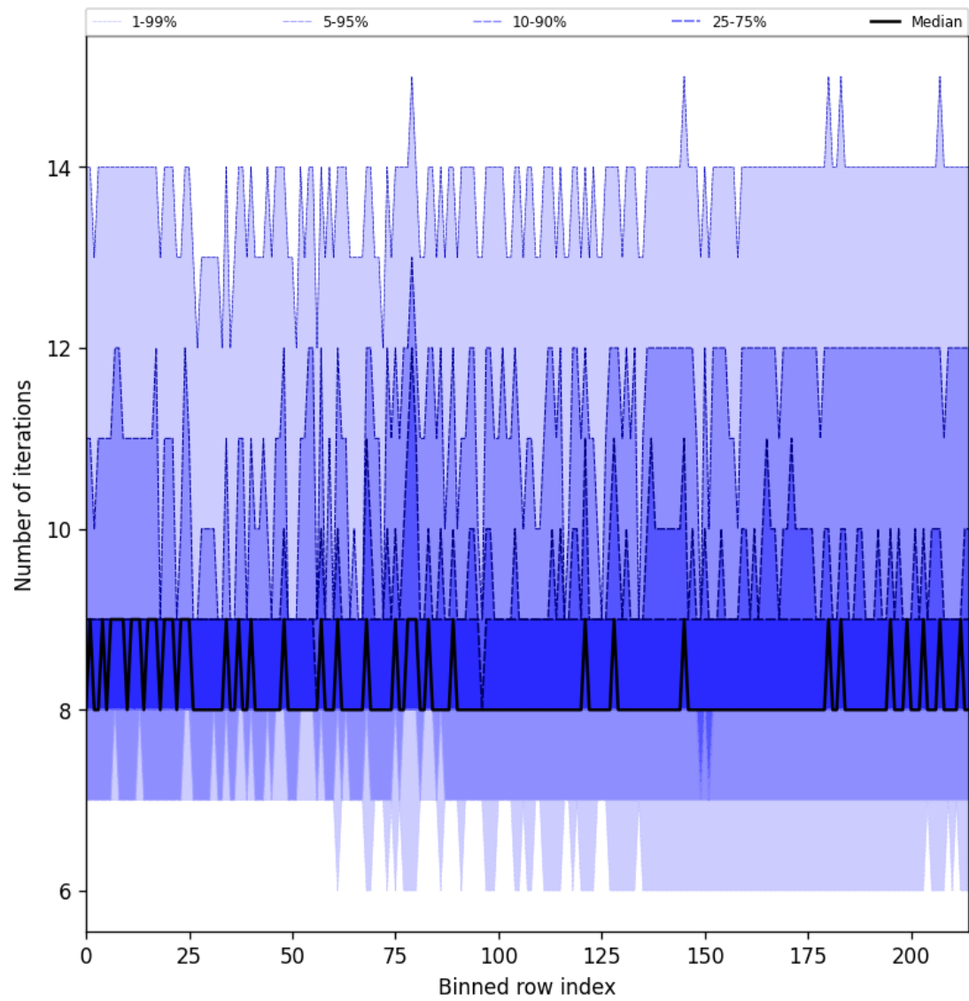
Figure 32: Along track statistics of “Number of iterations” for 2024-12-04 to 2024-12-06
