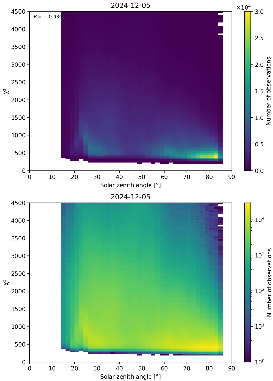
Figure 64: Scatter density plot of “Solar zenith angle” against “ \chi^2 ” for 2024-12-04 to 2024-12-06.
