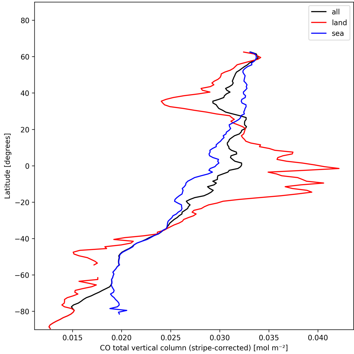
Figure 11: Zonal average of “CO total vertical column (stripe-corrected)” for 2024-12-04 to 2024-12-06.
