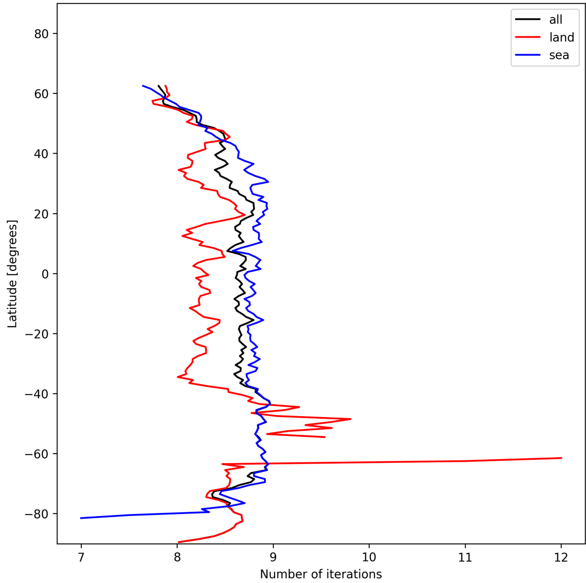
Figure 16: Zonal average of “Number of iterations” for 2024-12-04 to 2024-12-06.
