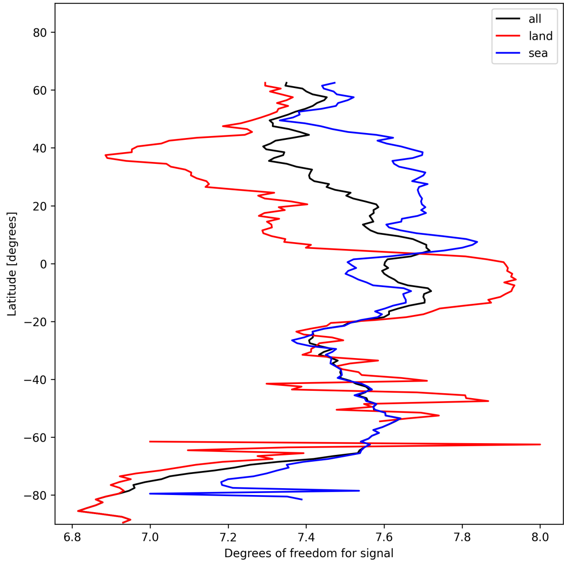
Figure 15: Zonal average of “Degrees of freedom for signal” for 2024-12-04 to 2024-12-06.
