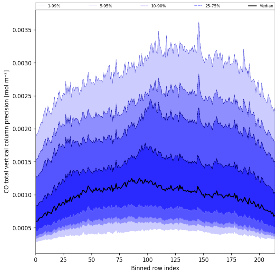
Figure 28: Along track statistics of “CO total vertical column precision” for 2024-12-04 to 2024-12-06
