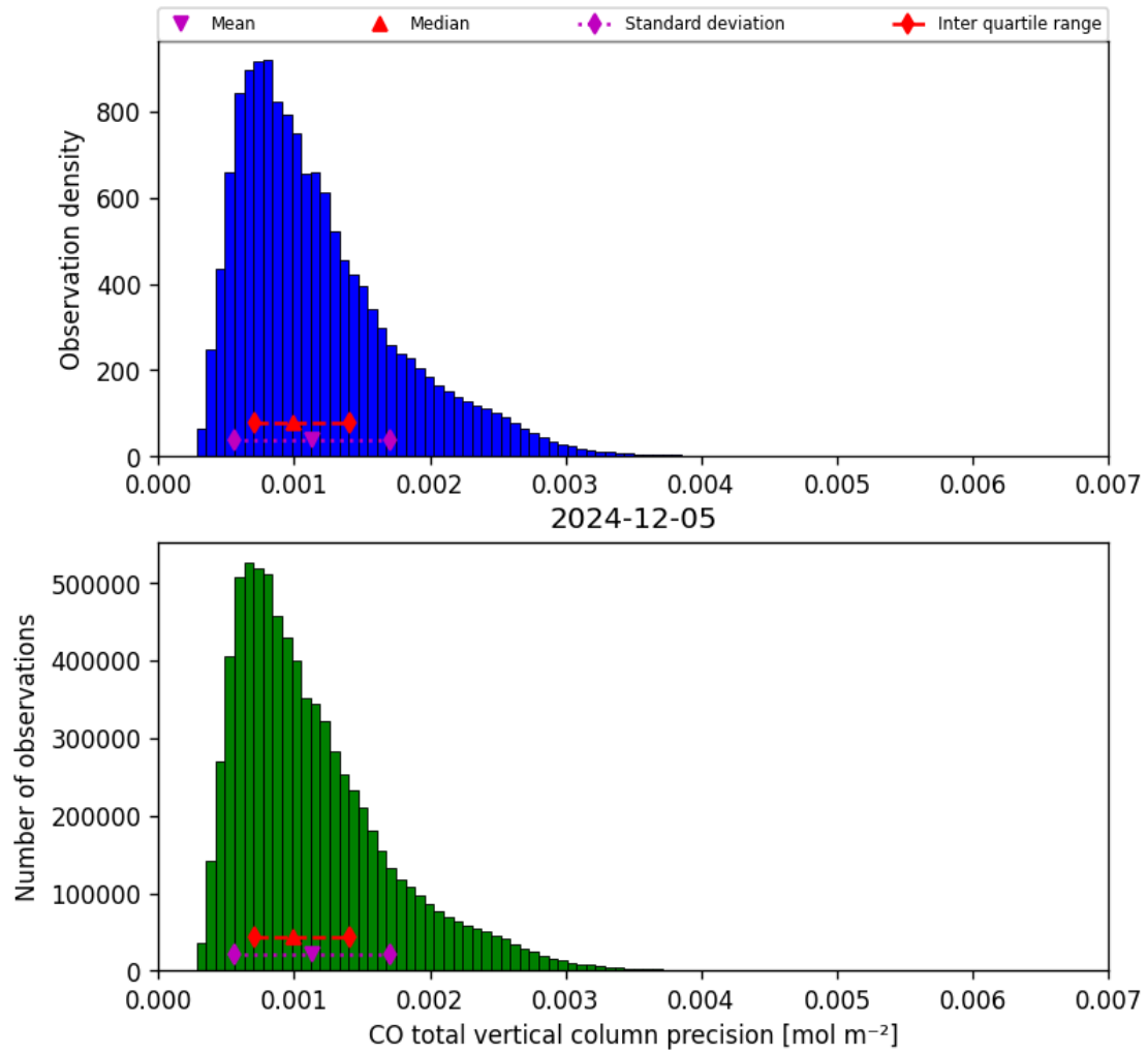
Figure 20: Histogram of “CO total vertical column precision” for 2024-12-04 to 2024-12-06
