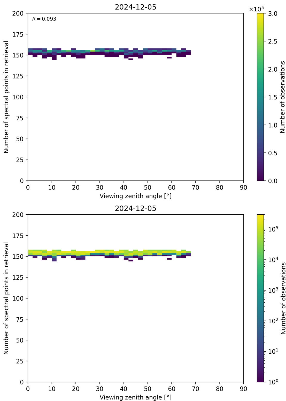
Figure 76: Scatter density plot of “Viewing zenith angle” against “Number of spectral points in retrieval” for 2024-12-04 to 2024-12-06.
