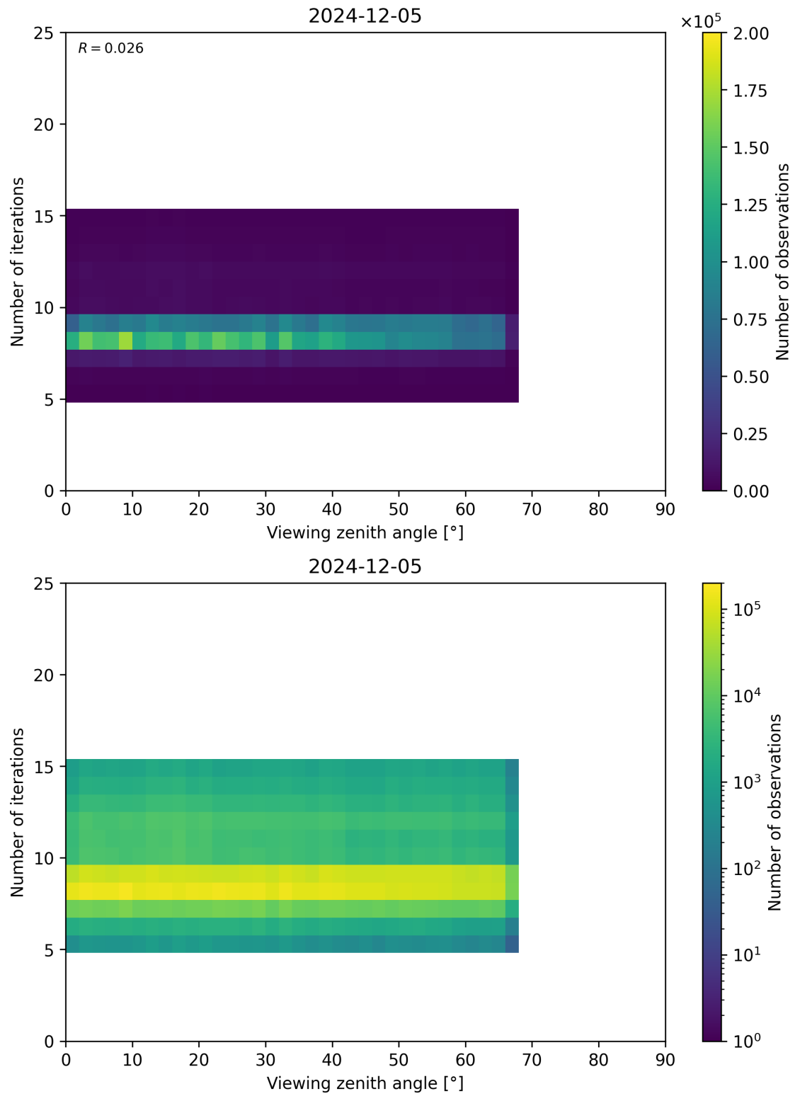
Figure 75: Scatter density plot of “Viewing zenith angle” against “Number of iterations” for 2024-12-04 to 2024-12-06.
