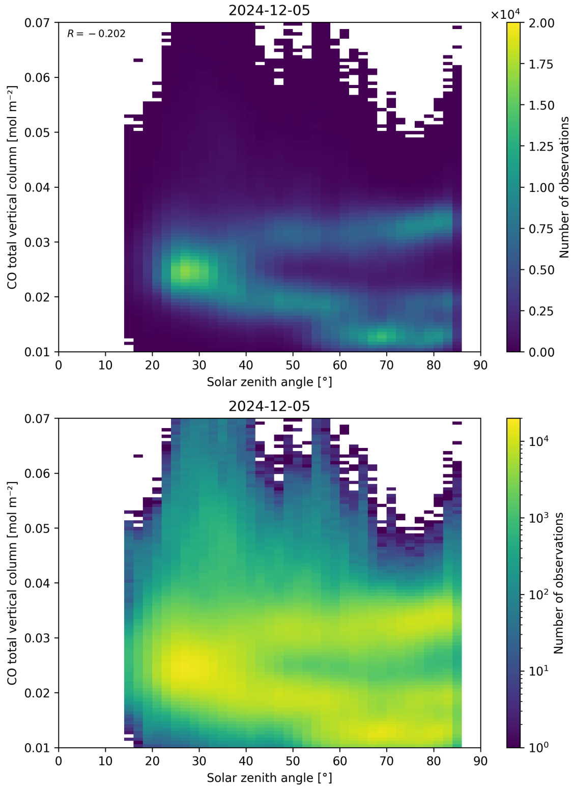
Figure 61: Scatter density plot of “Solar zenith angle” against “CO total vertical column” for 2024-12-04 to 2024-12-06.
