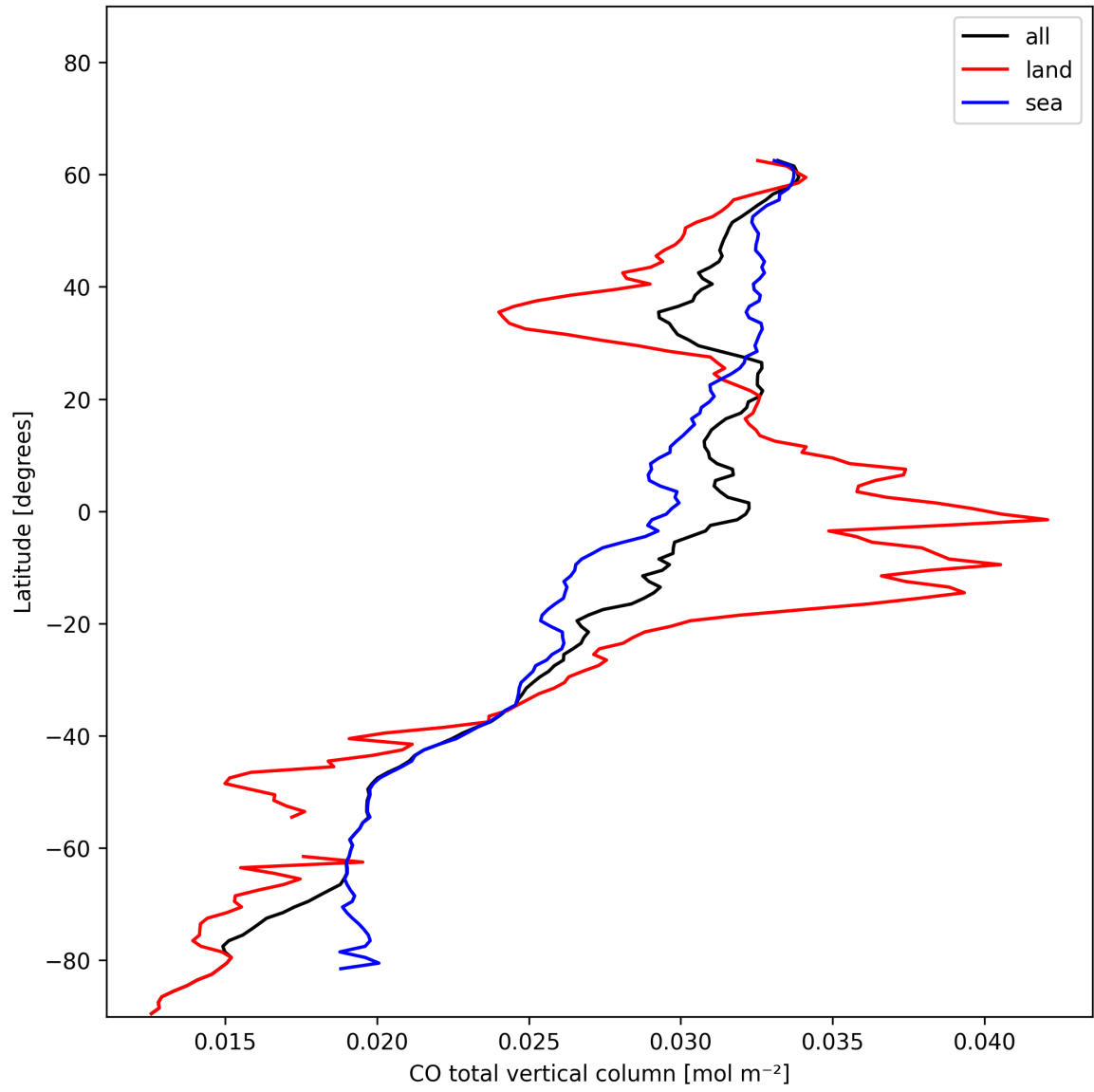
Figure 10: Zonal average of “CO total vertical column” for 2024-12-04 to 2024-12-06.
