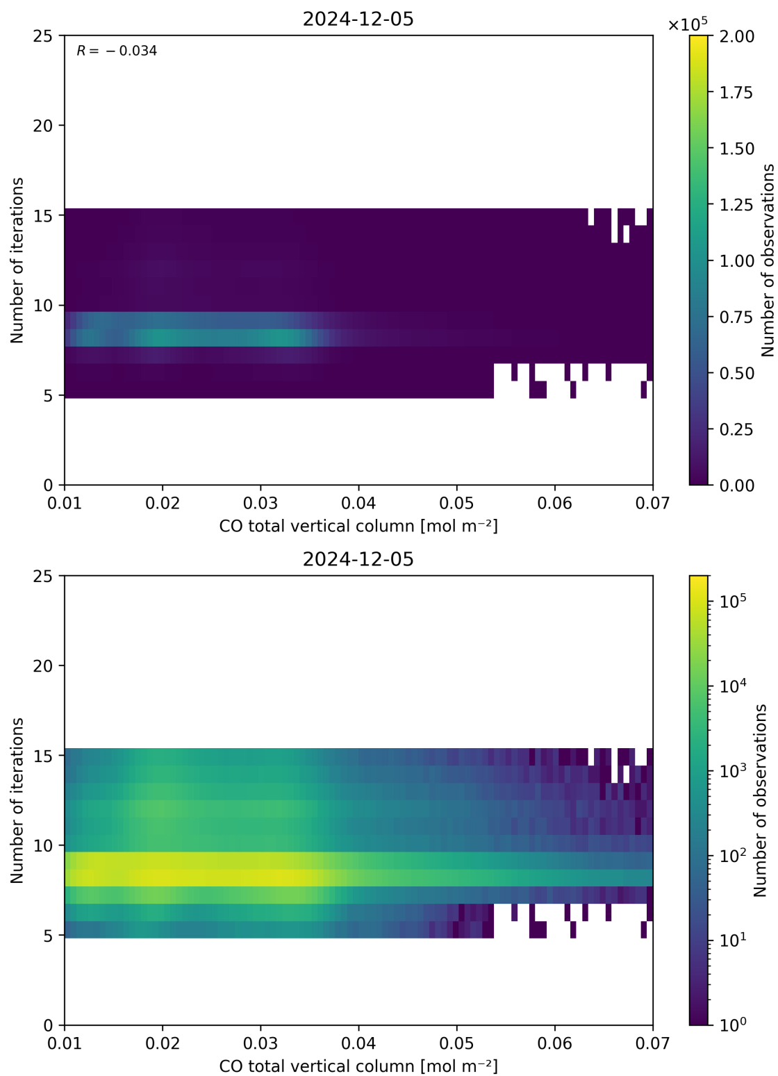
Figure 42: Scatter density plot of “CO total vertical column” against “Number of iterations” for 2024-12-04 to 2024-12-06.
