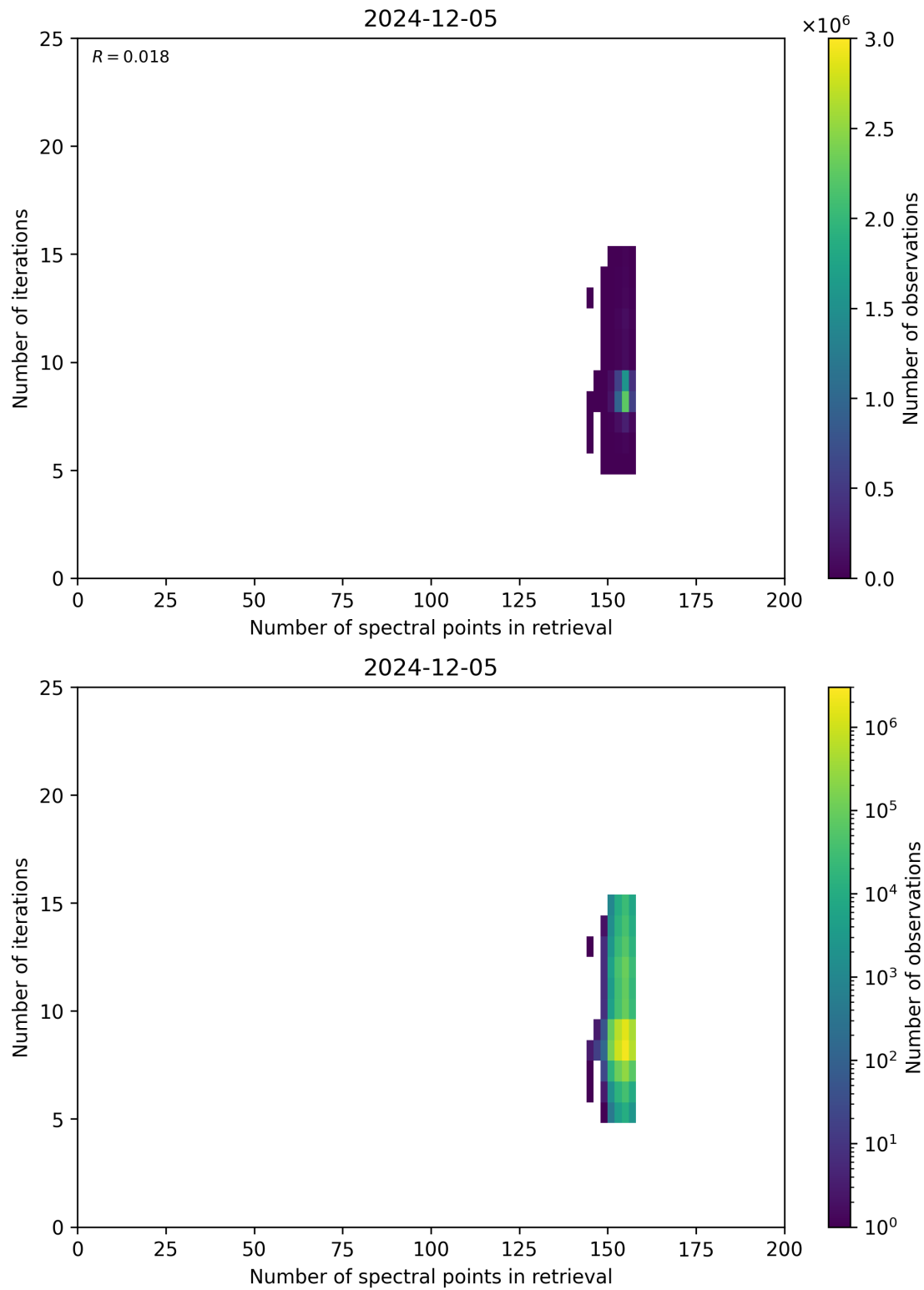
Figure 60: Scatter density plot of “Number of spectral points in retrieval” against “Number of iterations” for 2024-12-04 to 2024-12-06.
