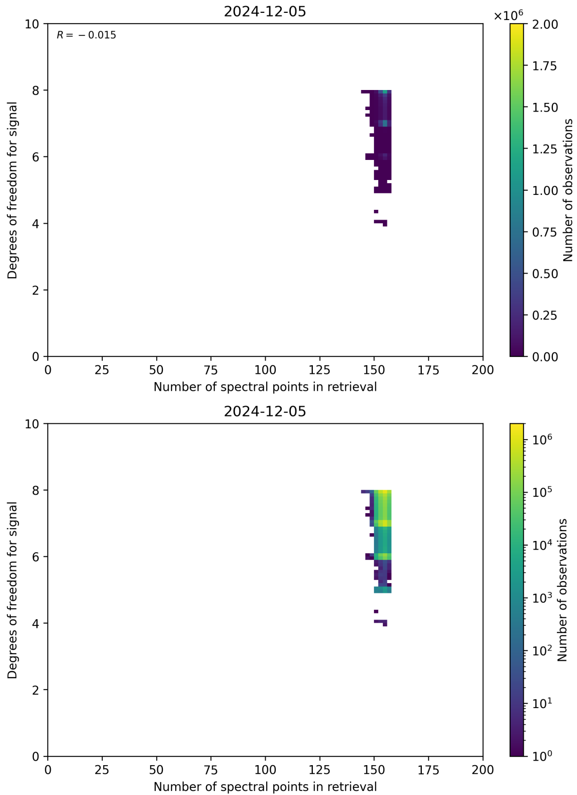
Figure 59: Scatter density plot of “Number of spectral points in retrieval” against “Degrees of freedom for signal” for 2024-12-04 to 2024-12-06.
