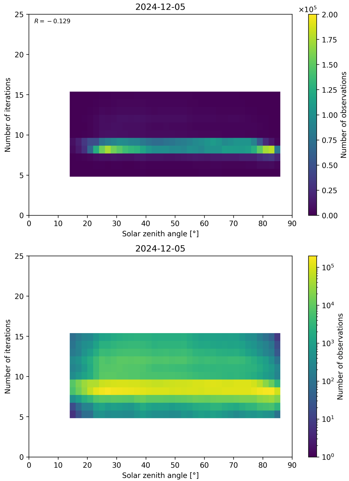
Figure 67: Scatter density plot of “Solar zenith angle” against “Number of iterations” for 2024-12-04 to 2024-12-06.
