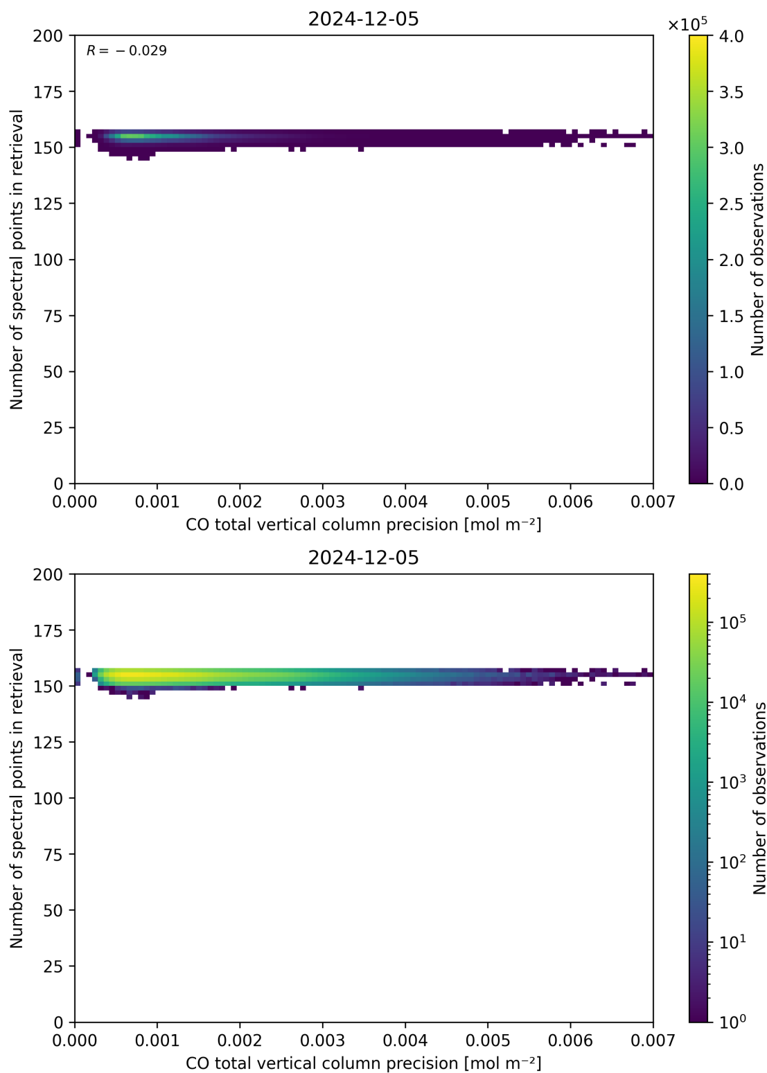
Figure 47: Scatter density plot of “CO total vertical column precision” against “Number of spectral points in retrieval” for 2024-12-04 to 2024-12-06.
