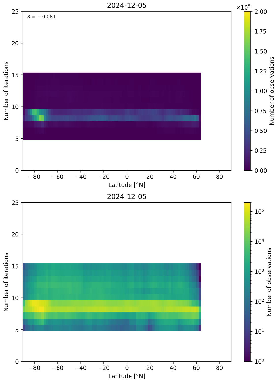
Figure 56: Scatter density plot of “Latitude” against “Number of iterations” for 2024-12-04 to 2024-12-06.
