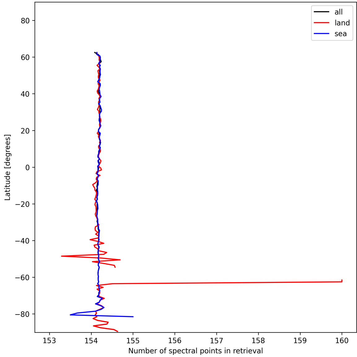
Figure 13: Zonal average of “Number of spectral points in retrieval” for 2024-12-04 to 2024-12-06.
