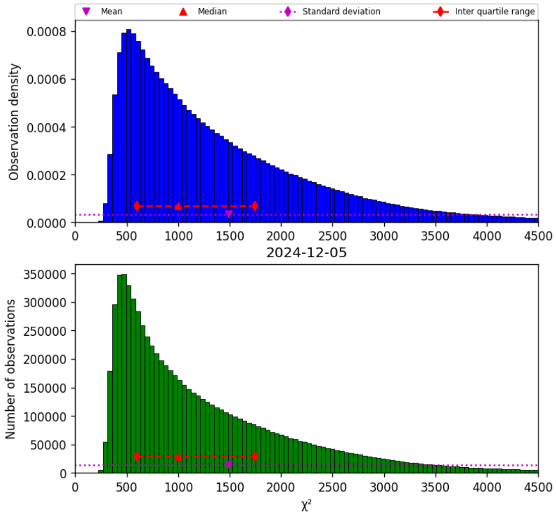
Figure 22: Histogram of “ \chi^2 ” for 2024-12-04 to 2024-12-06
