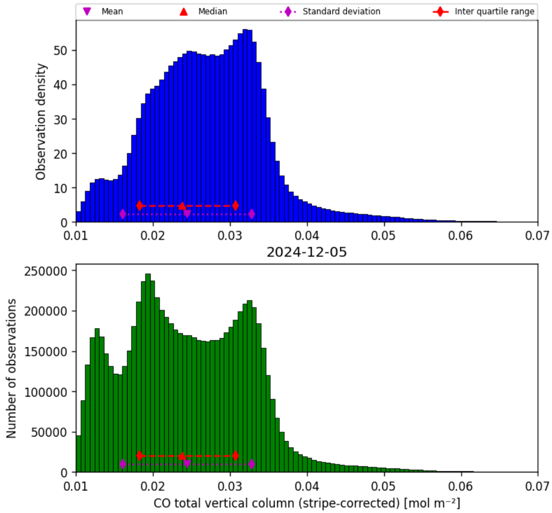
Figure 19: Histogram of “CO total vertical column (stripe-corrected)” for 2024-12-04 to 2024-12-06
