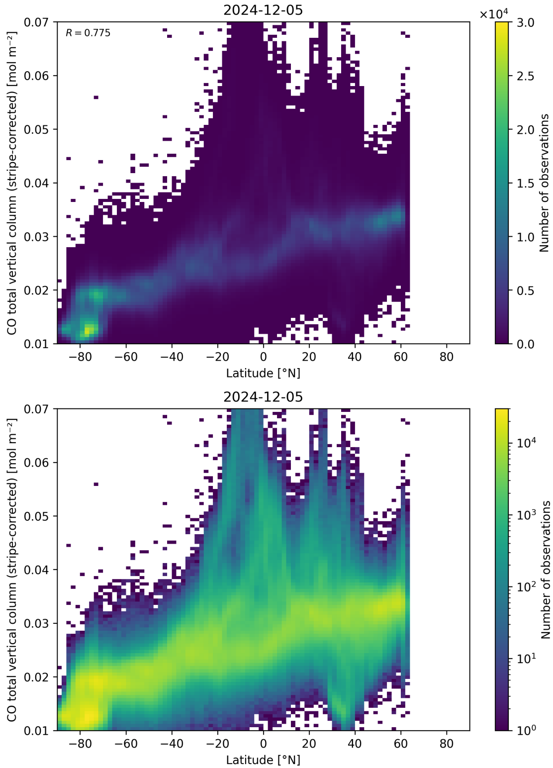
Figure 52: Scatter density plot of “Latitude” against “CO total vertical column (stripe-corrected)” for 2024-12-04 to 2024-12-06.
