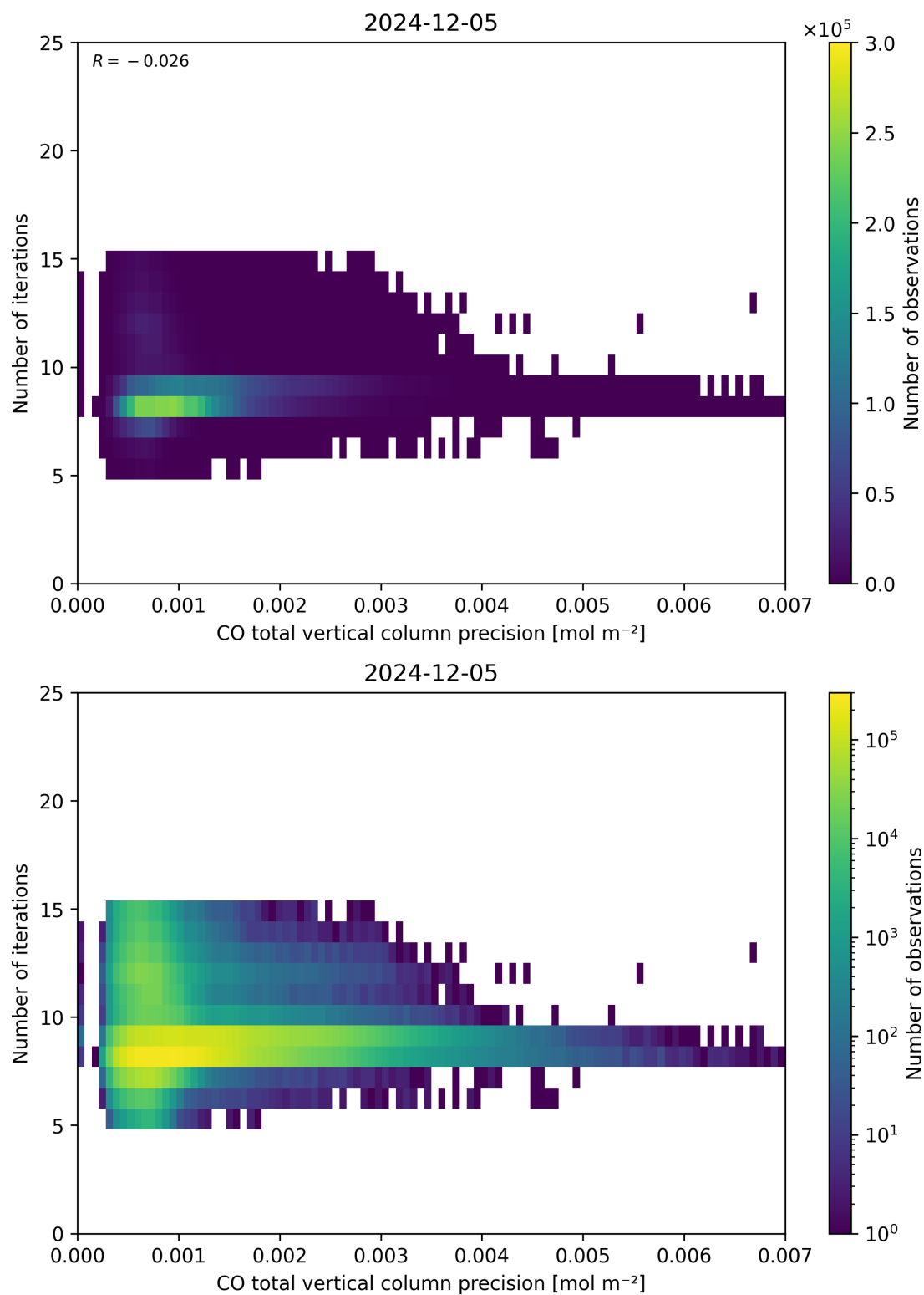
Figure 46: Scatter density plot of “CO total vertical column precision” against “Number of iterations” for 2024-12-04 to 2024-12-06.
