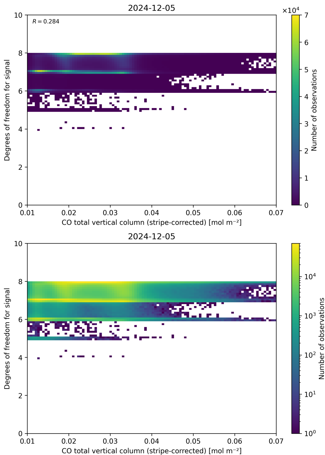
Figure 38: Scatter density plot of “CO total vertical column (stripe-corrected)” against “Degrees of freedom for signal” for 2024-12-04 to 2024-12-06.
