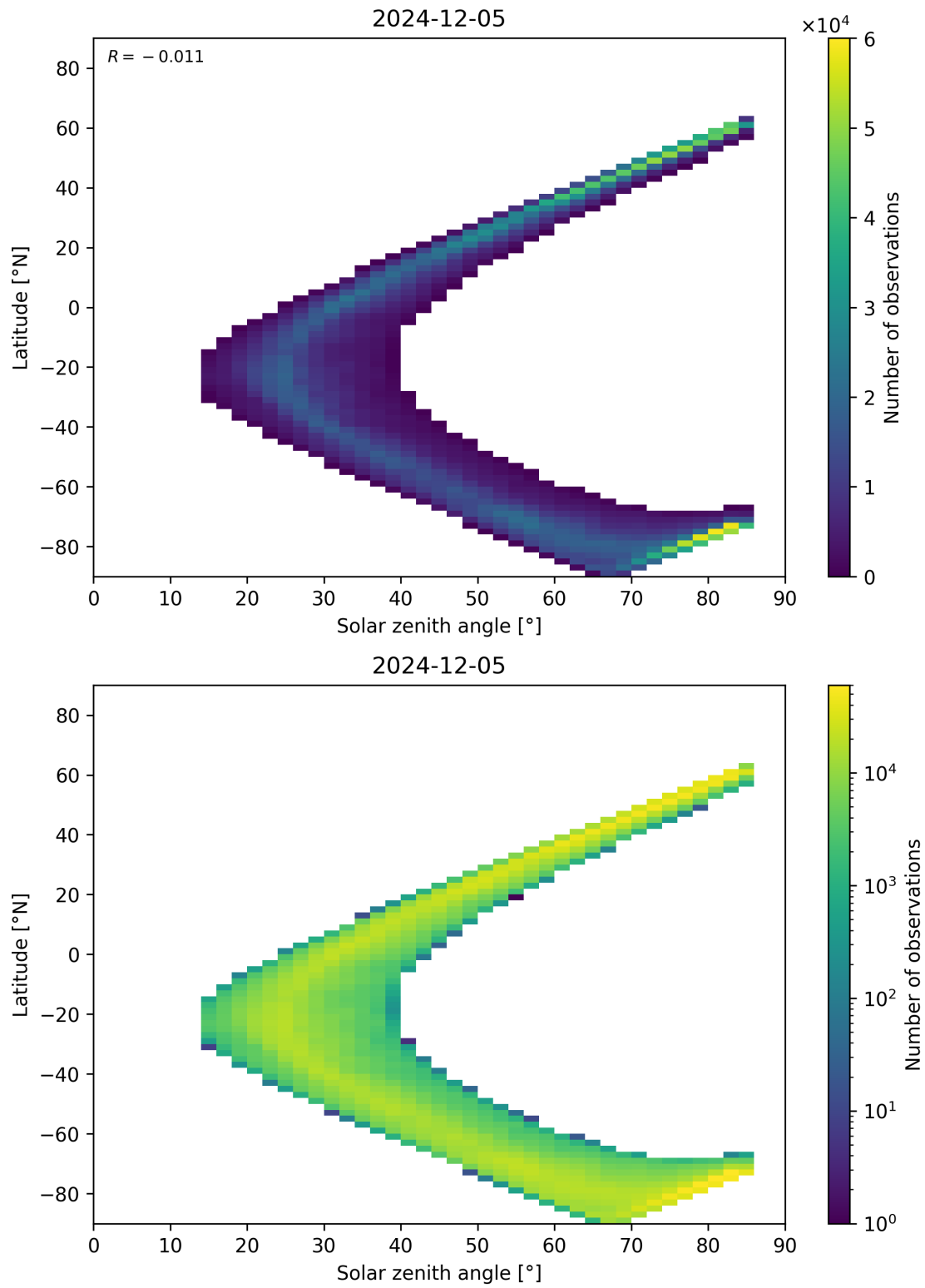
Figure 66: Scatter density plot of “Solar zenith angle” against “Latitude” for 2024-12-04 to 2024-12-06.
