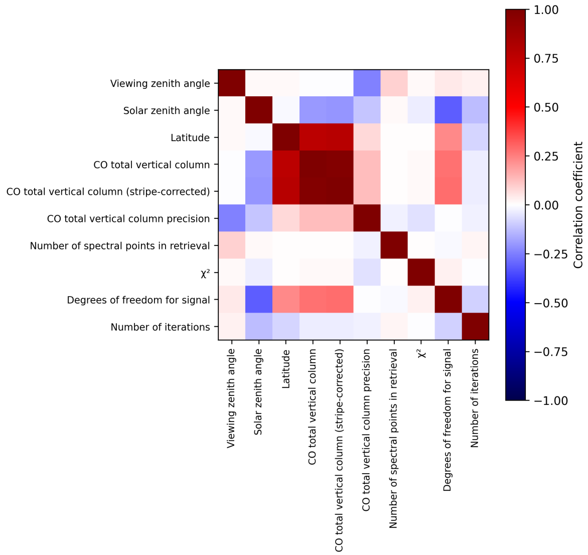
Figure 2: Map of correlation matrix for 2024-12-04 to 2024-12-06.
