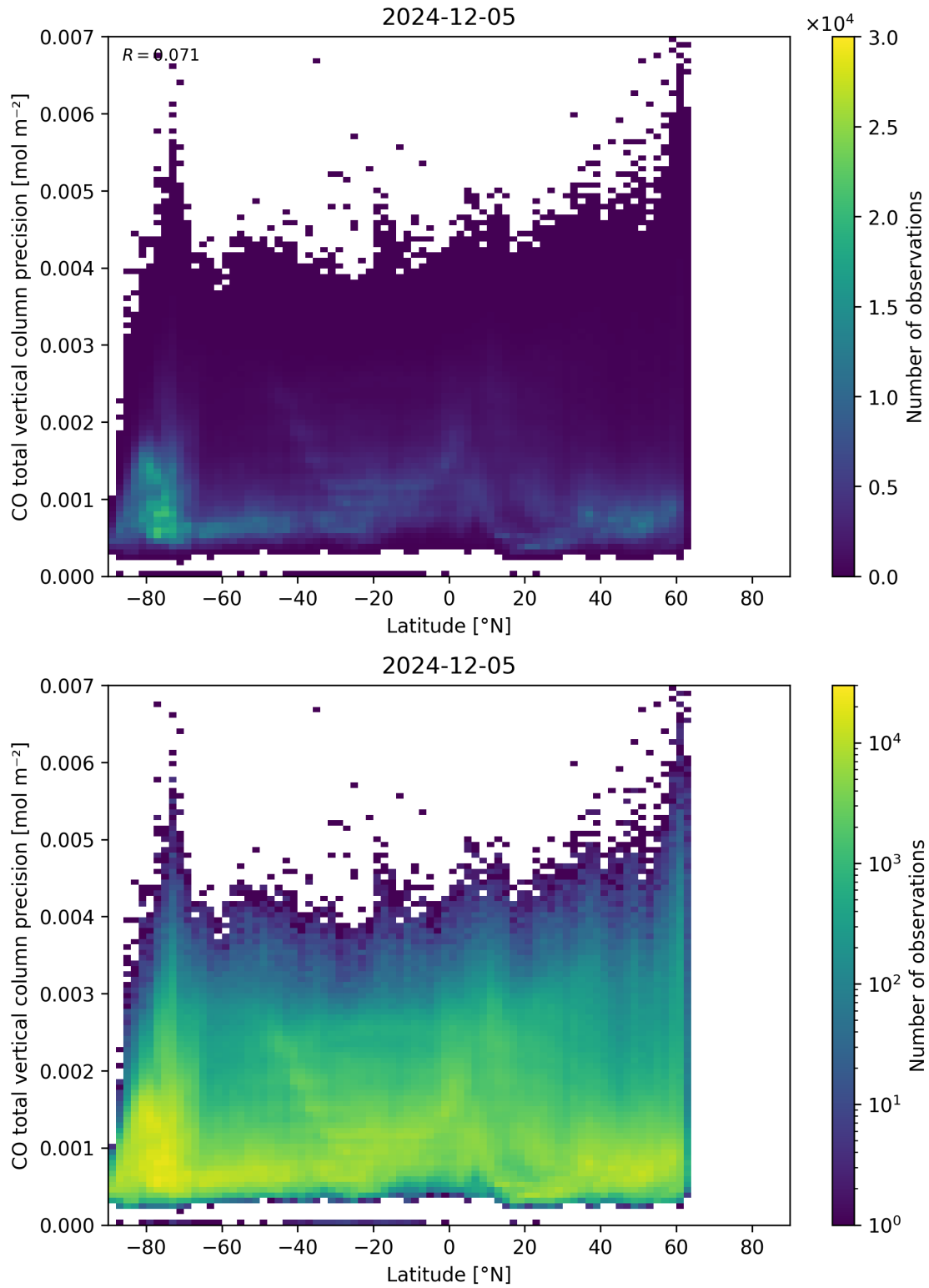
Figure 53: Scatter density plot of “Latitude” against “CO total vertical column precision” for 2024-12-04 to 2024-12-06.
