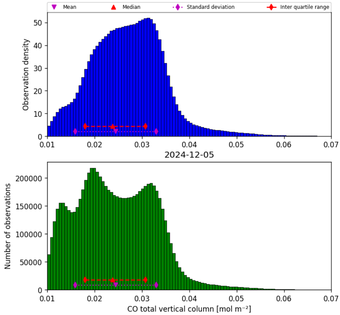
Figure 18: Histogram of “CO total vertical column” for 2024-12-04 to 2024-12-06
