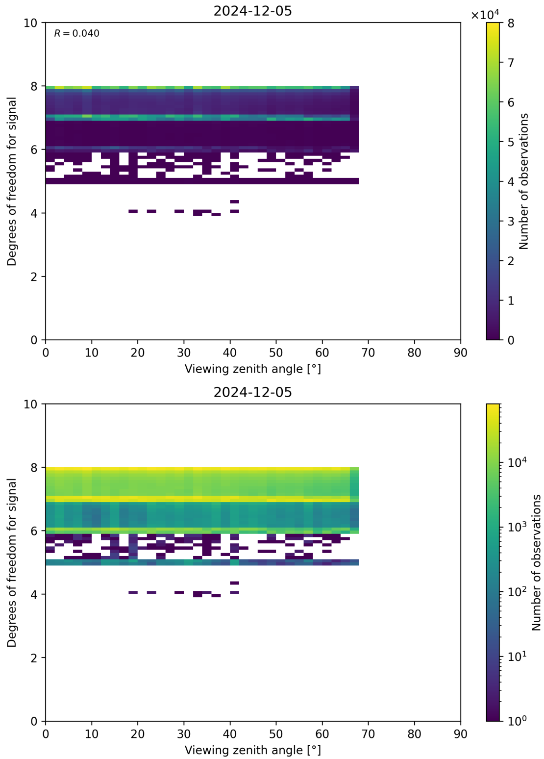
Figure 73: Scatter density plot of “Viewing zenith angle” against “Degrees of freedom for signal” for 2024-12-04 to 2024-12-06.
