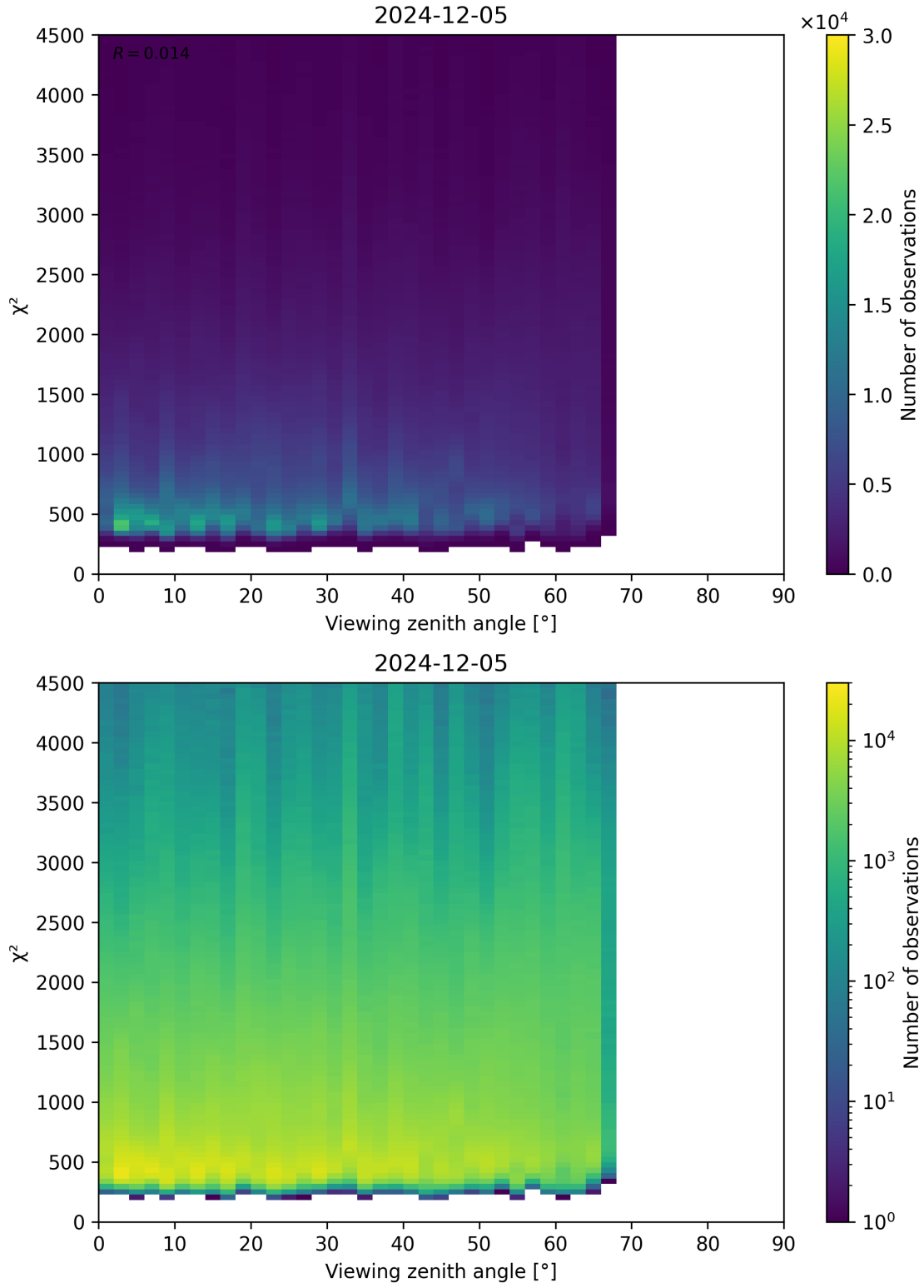
Figure 72: Scatter density plot of “Viewing zenith angle” against “ \chi^2 ” for 2024-12-04 to 2024-12-06.
