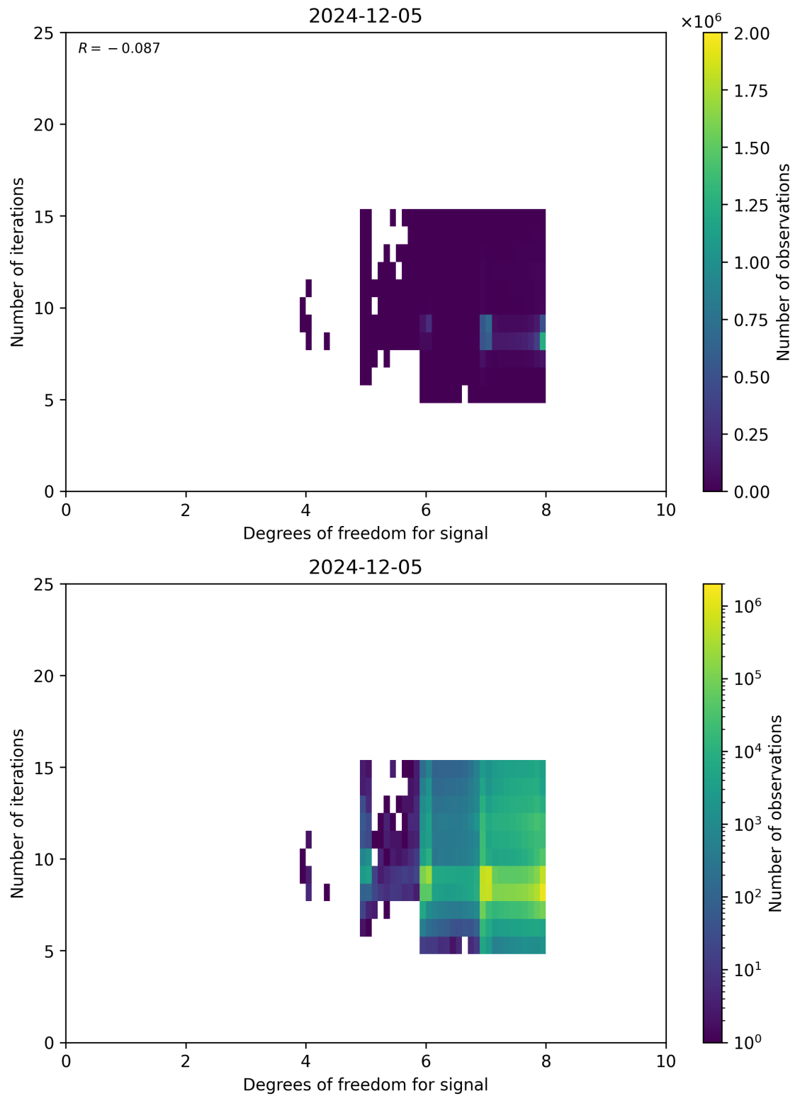
Figure 50: Scatter density plot of “Degrees of freedom for signal” against “Number of iterations” for 2024-12-04 to 2024-12-06.
