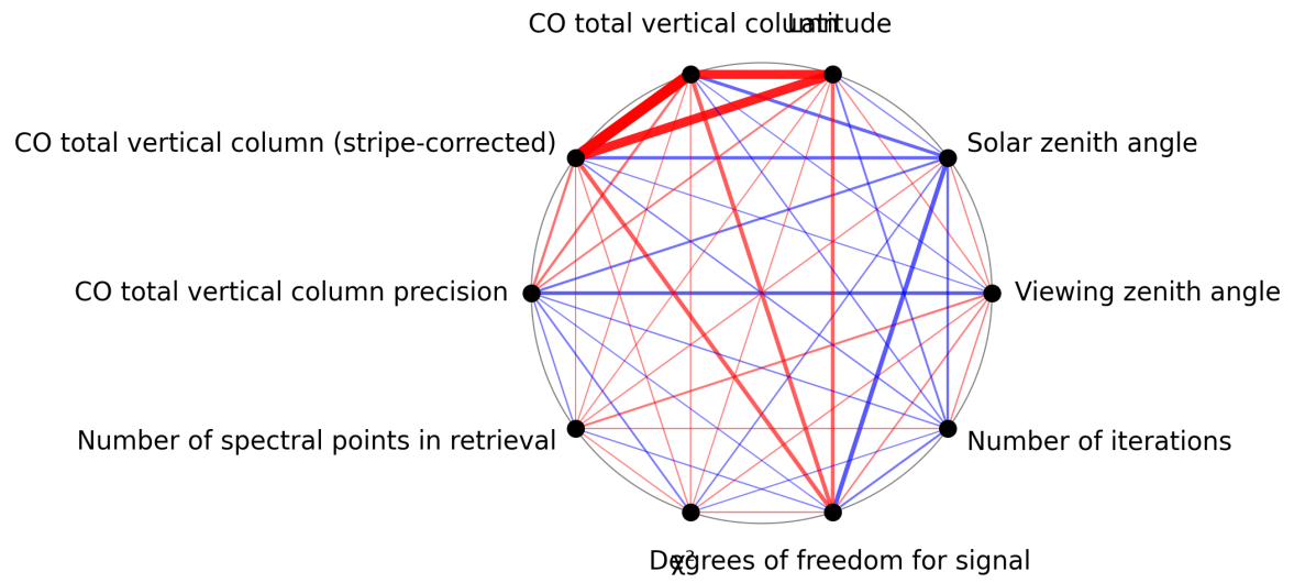
Figure 1: Map of correlation graph for 2024-12-04 to 2024-12-06.
