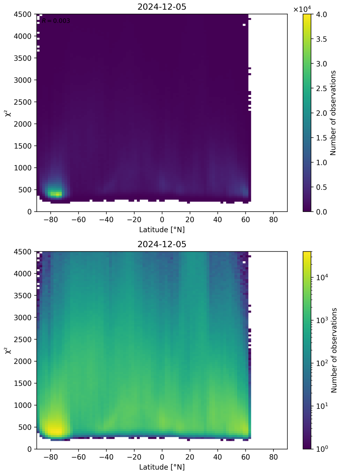
Figure 54: Scatter density plot of “Latitude” against “ \chi^2 ” for 2024-12-04 to 2024-12-06.
