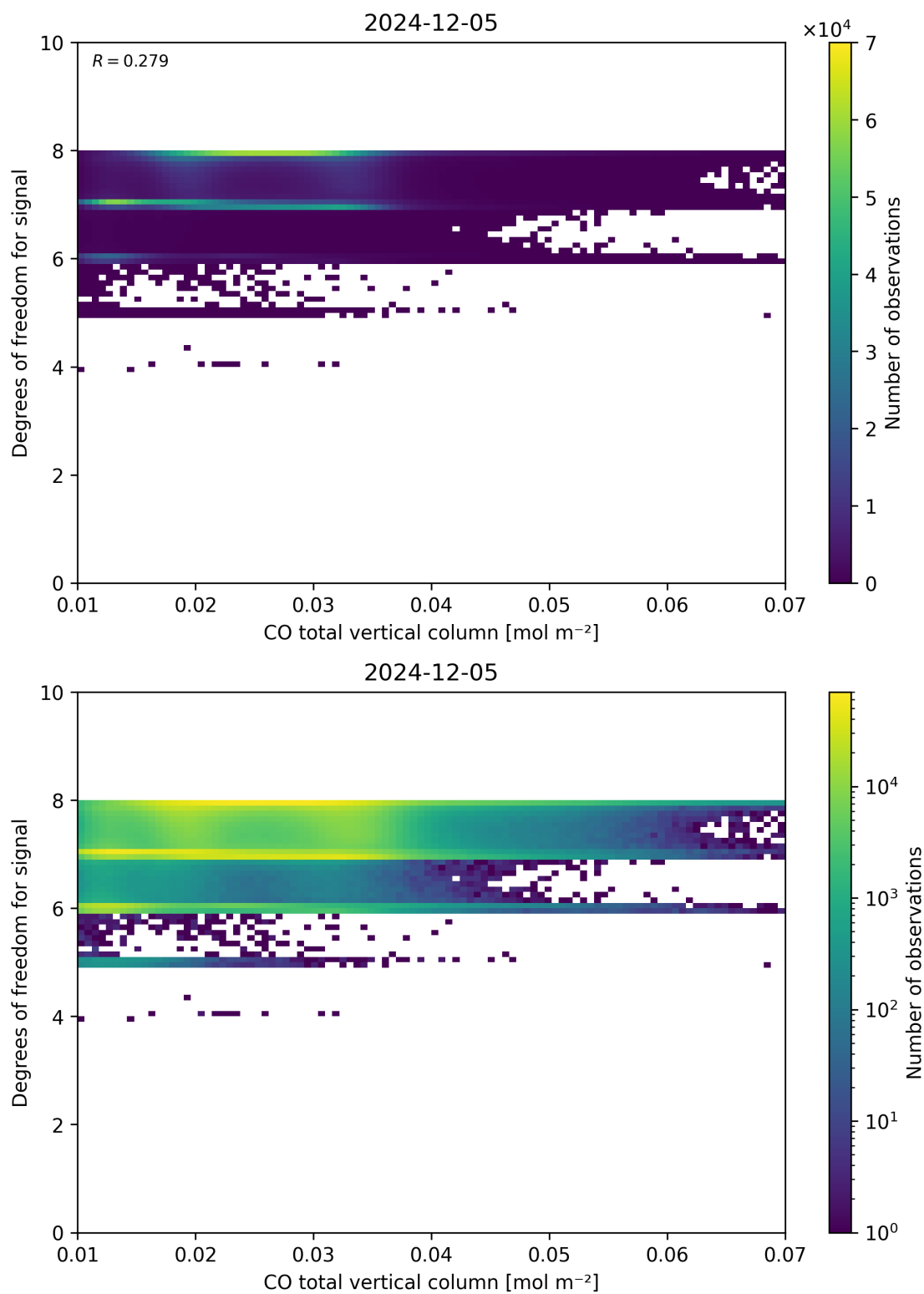
Figure 41: Scatter density plot of “CO total vertical column” against “Degrees of freedom for signal” for 2024-12-04 to 2024-12-06.
