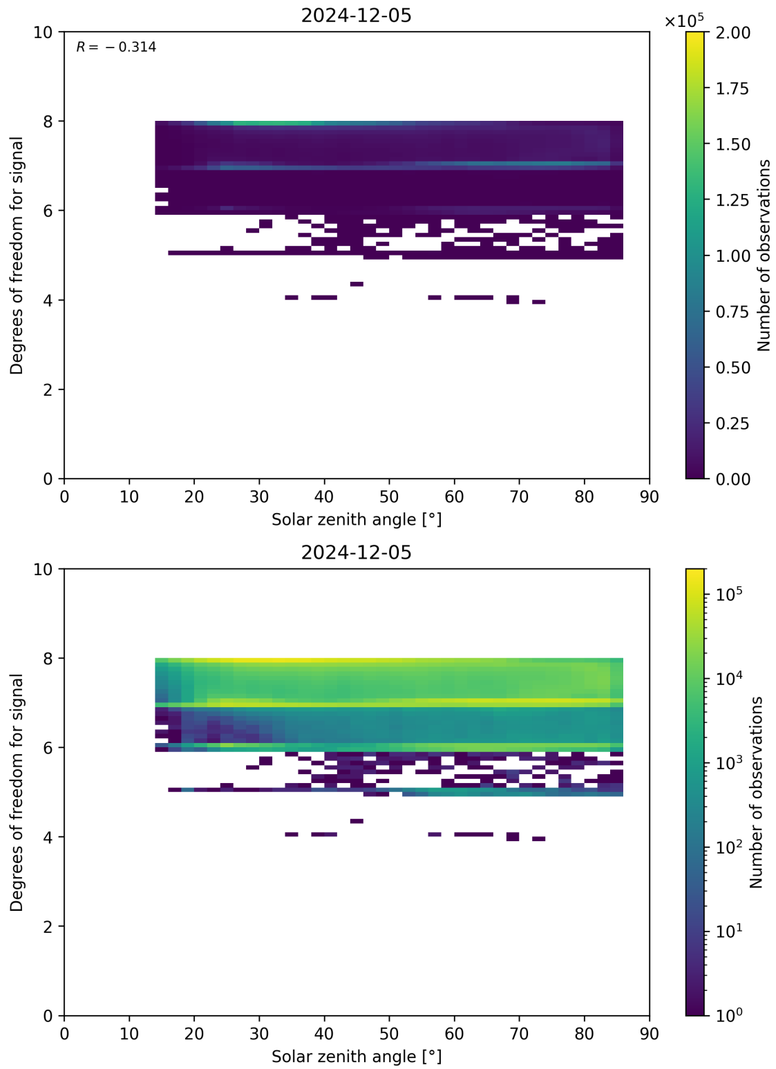
Figure 65: Scatter density plot of “Solar zenith angle” against “Degrees of freedom for signal” for 2024-12-04 to 2024-12-06.
