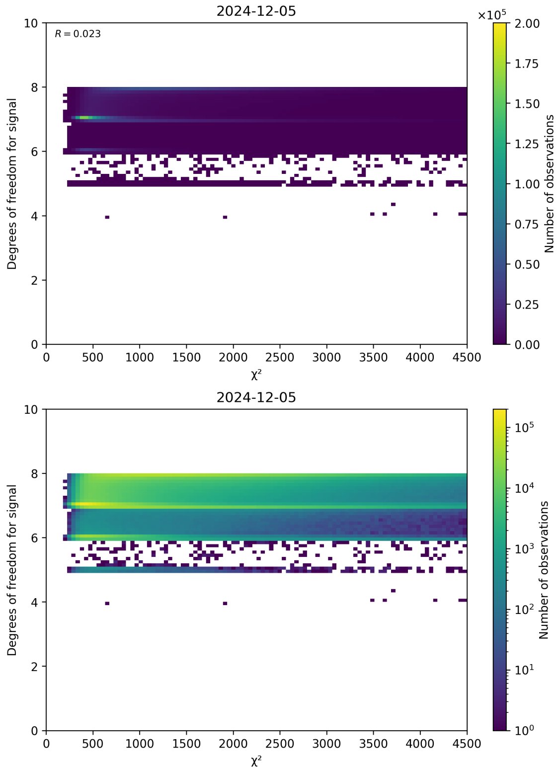
Figure 48: Scatter density plot of “ \chi^2 ” against “Degrees of freedom for signal” for 2024-12-04 to 2024-12-06.
