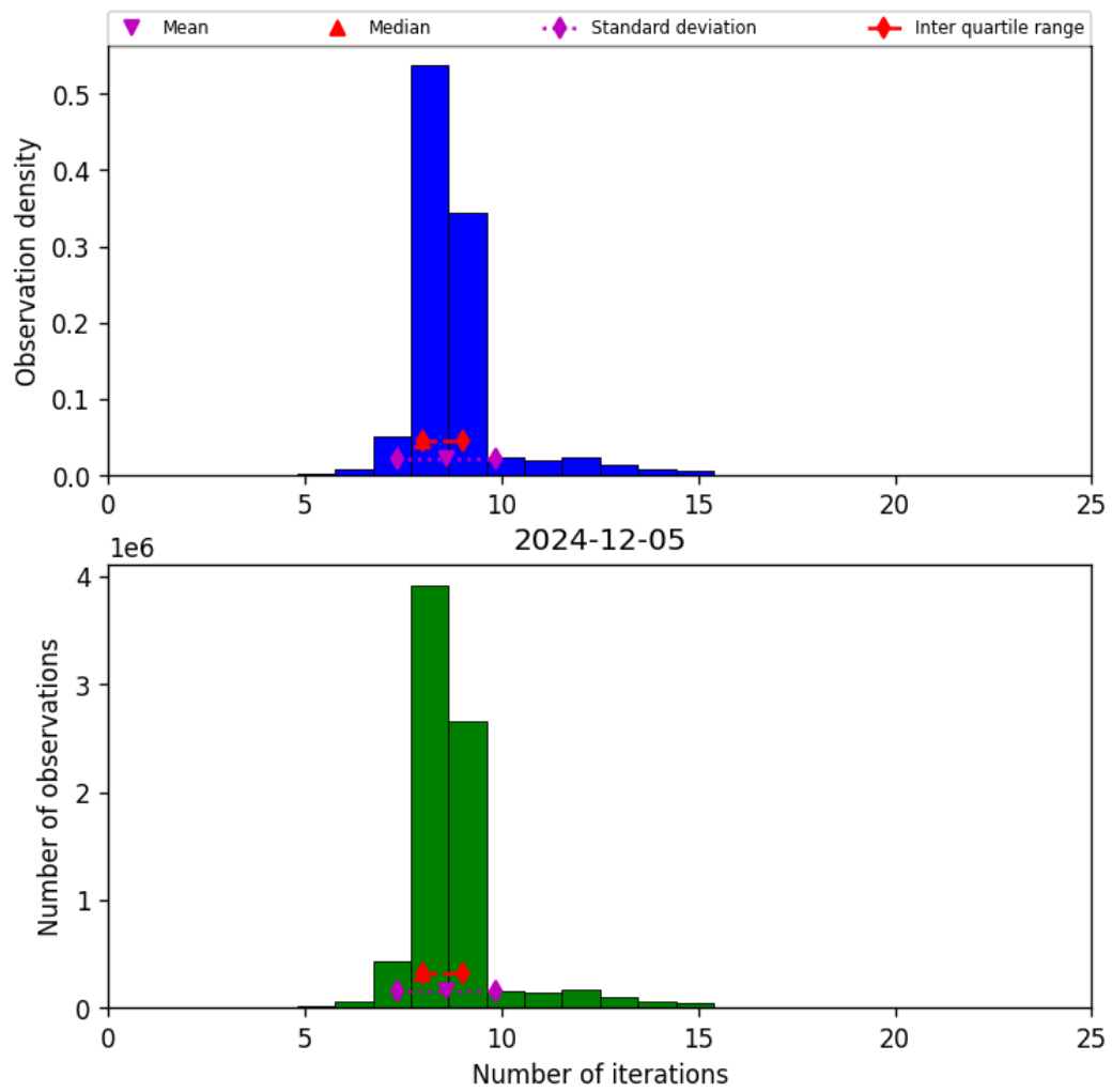
Figure 24: Histogram of “Number of iterations” for 2024-12-04 to 2024-12-06
