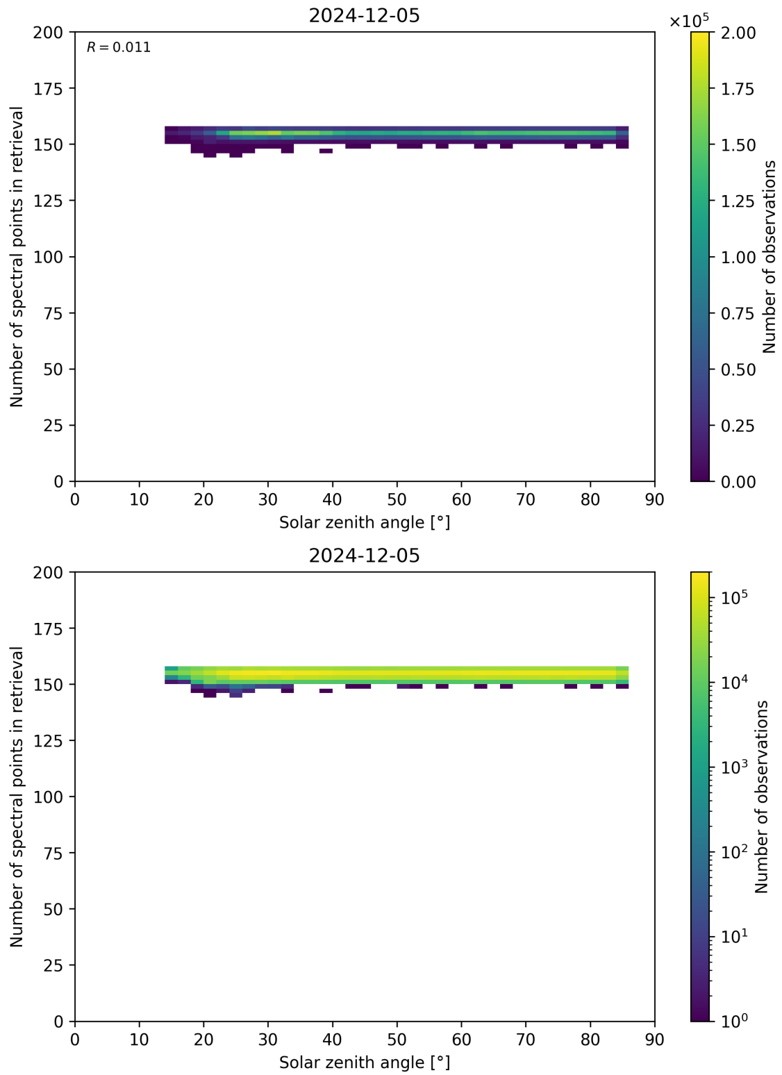
Figure 68: Scatter density plot of “Solar zenith angle” against “Number of spectral points in retrieval” for 2024-12-04 to 2024-12-06.
