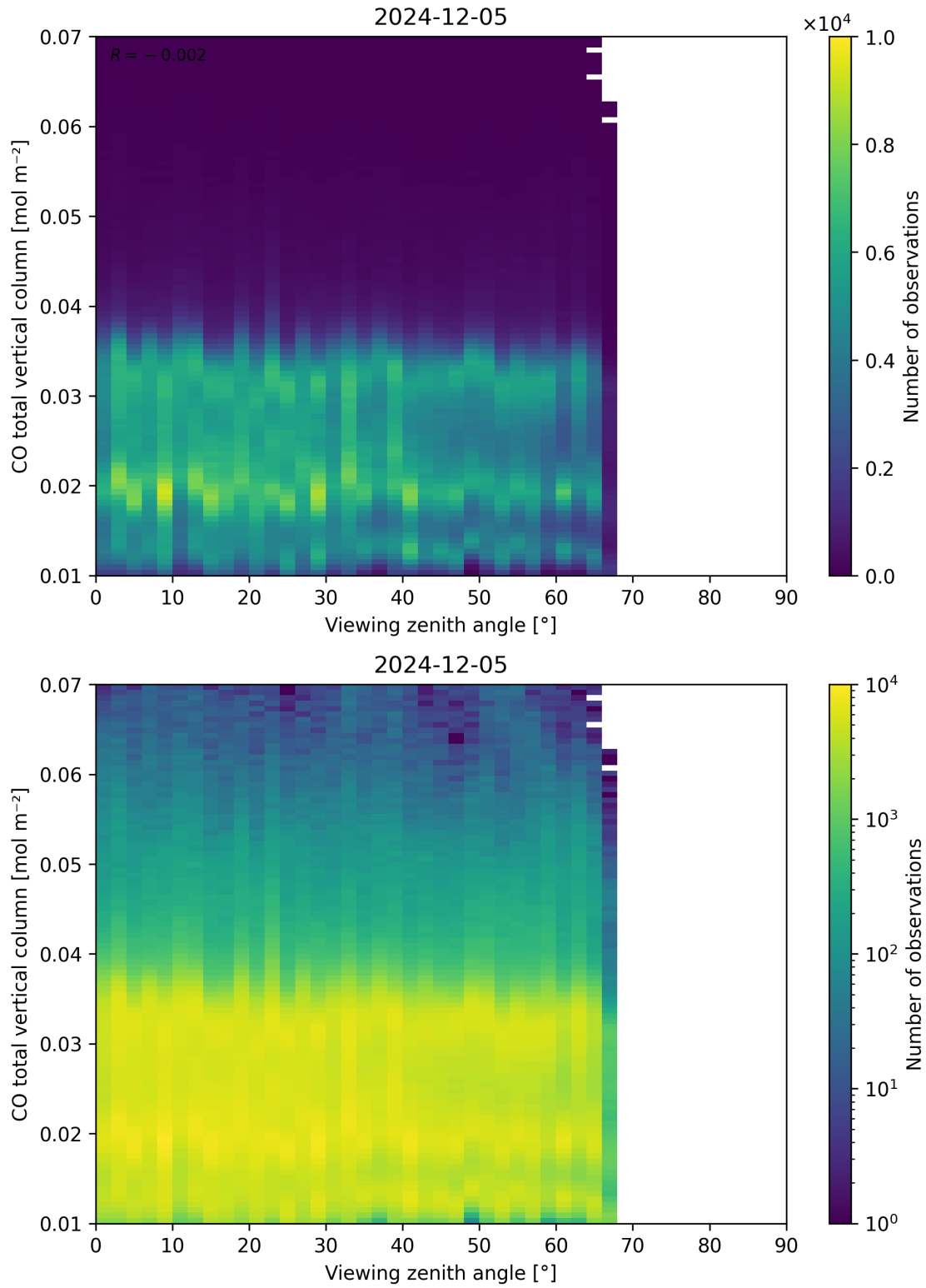
Figure 69: Scatter density plot of “Viewing zenith angle” against “CO total vertical column” for 2024-12-04 to 2024-12-06.
