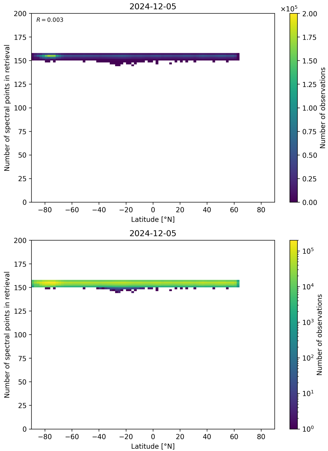
Figure 57: Scatter density plot of “Latitude” against “Number of spectral points in retrieval” for 2024-12-04 to 2024-12-06.
