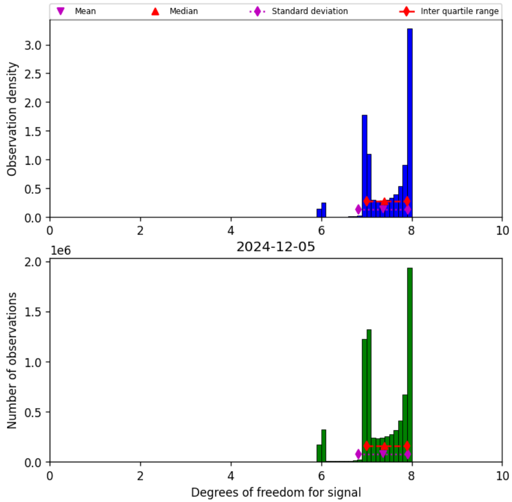
Figure 23: Histogram of “Degrees of freedom for signal” for 2024-12-04 to 2024-12-06
