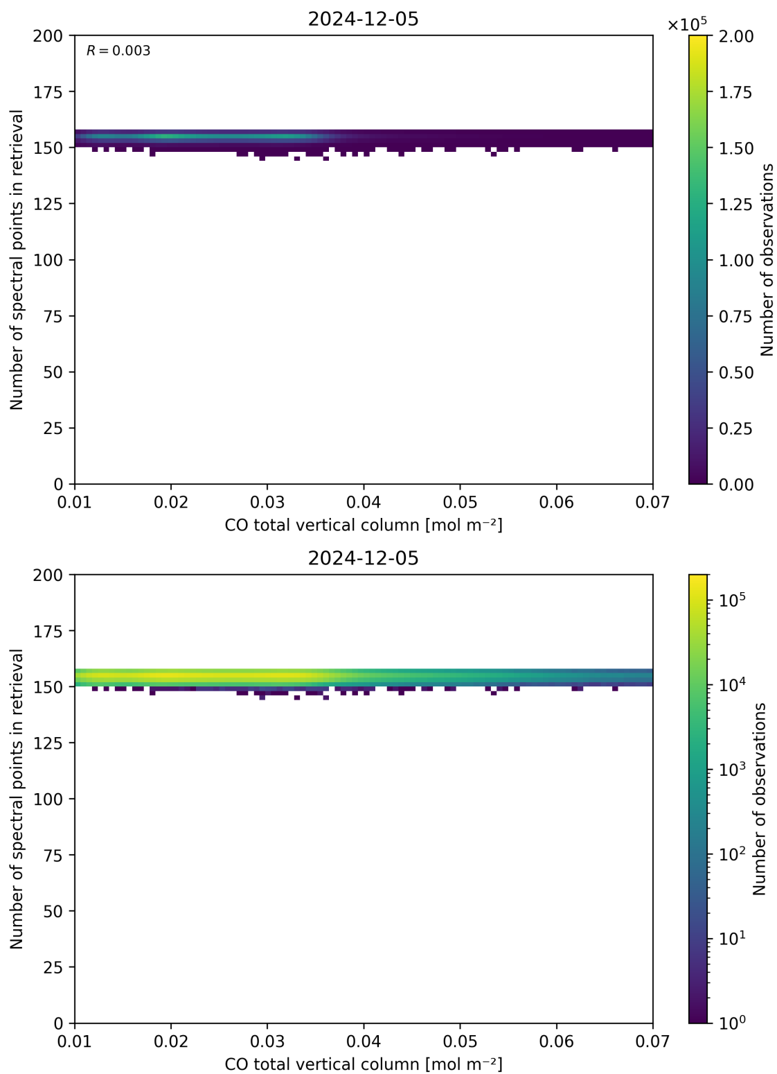
Figure 43: Scatter density plot of “CO total vertical column” against “Number of spectral points in retrieval” for 2024-12-04 to 2024-12-06.
