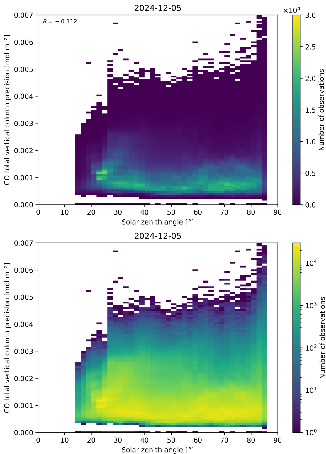
Figure 63: Scatter density plot of “Solar zenith angle” against “CO total vertical column precision” for 2024-12-04 to 2024-12-06.
