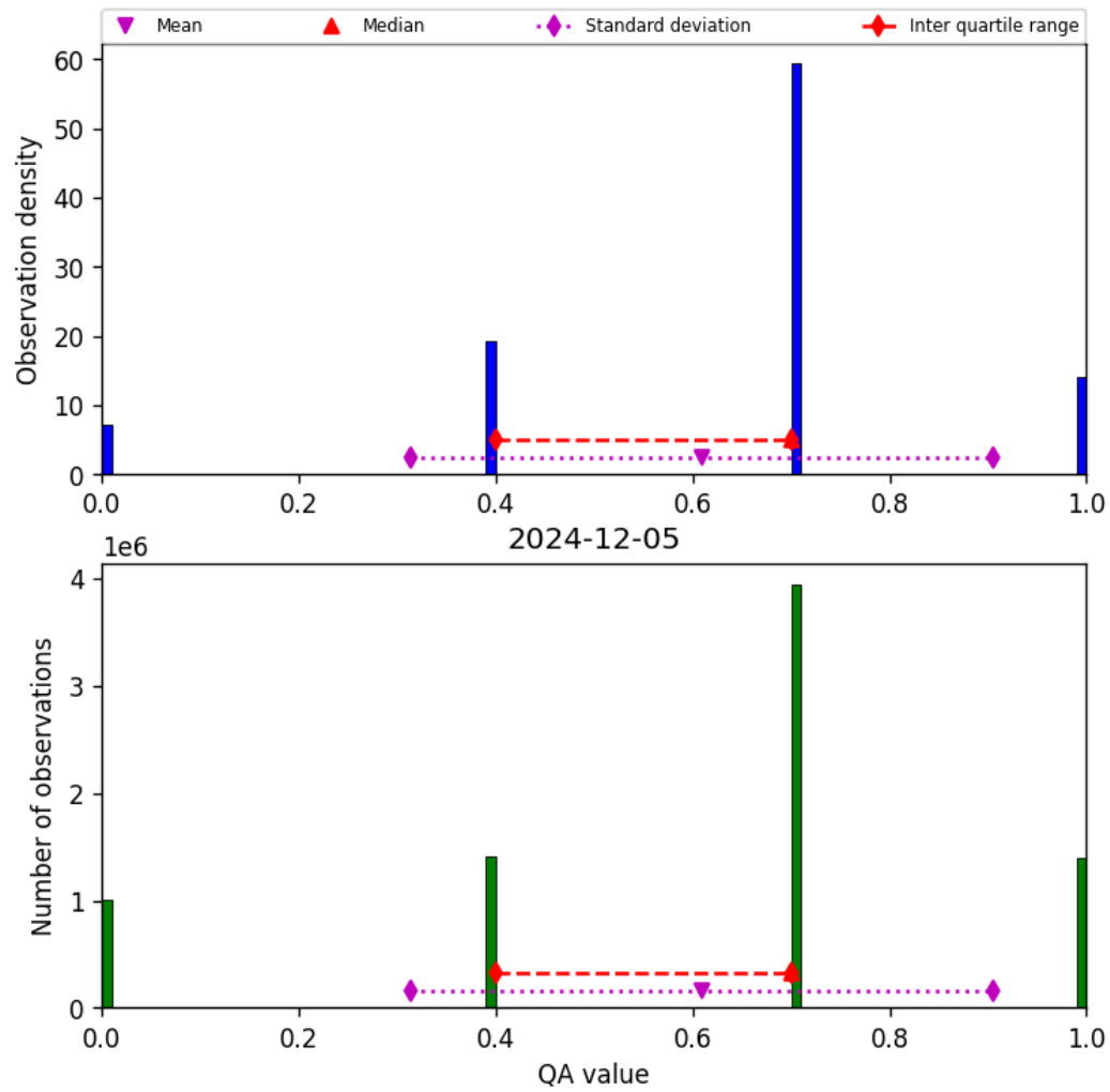
Figure 17: Histogram of “QA value” for 2024-12-04 to 2024-12-06
