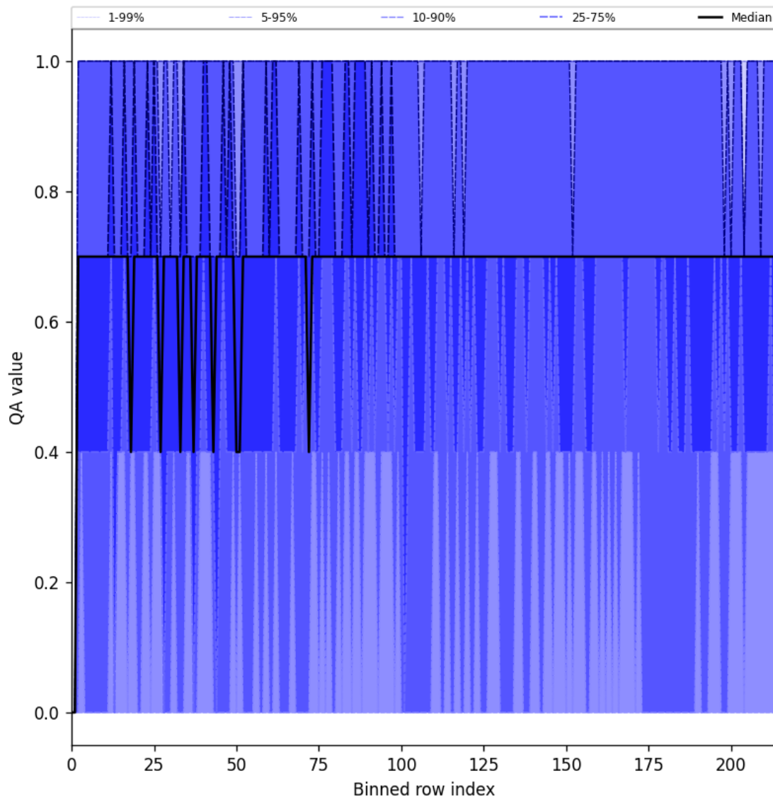
Figure 25: Along track statistics of “QA value” for 2024-12-04 to 2024-12-06
