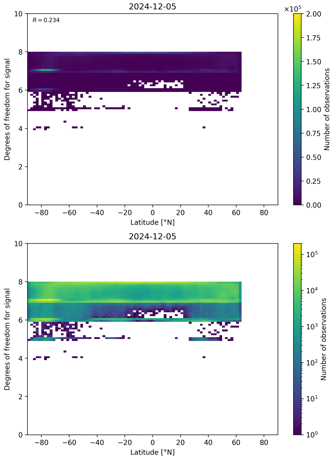
Figure 55: Scatter density plot of “Latitude” against “Degrees of freedom for signal” for 2024-12-04 to 2024-12-06.
