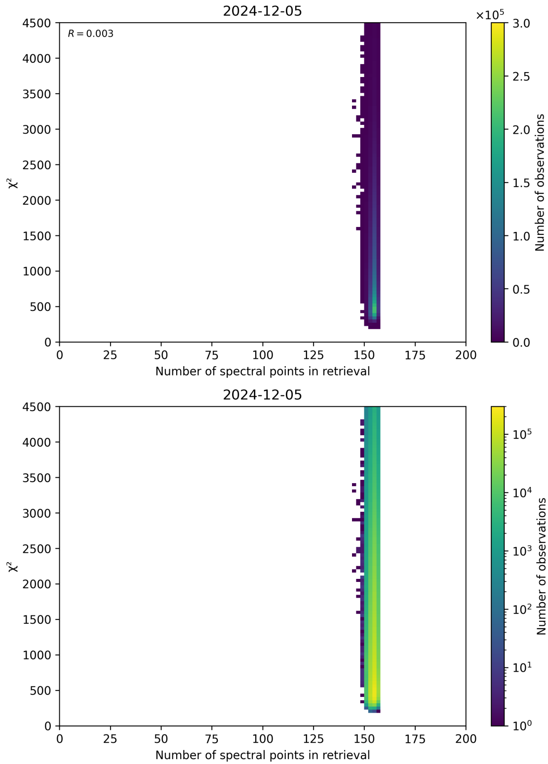
Figure 58: Scatter density plot of “Number of spectral points in retrieval” against “ \chi^2 ” for 2024-12-04 to 2024-12-06.
