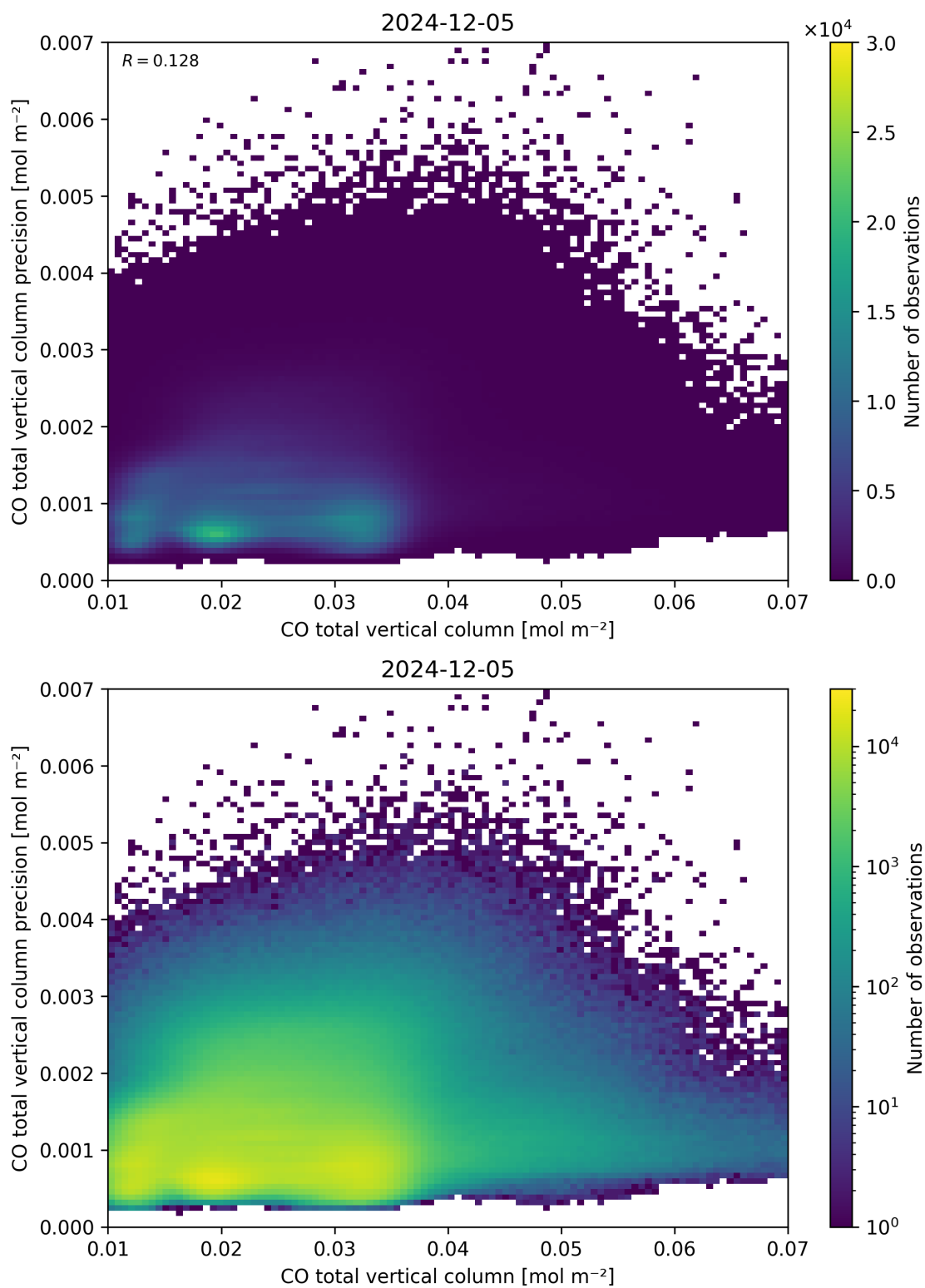
Figure 34: Scatter density plot of “CO total vertical column” against “CO total vertical column precision” for 2024-12-04 to 2024-12-06.
