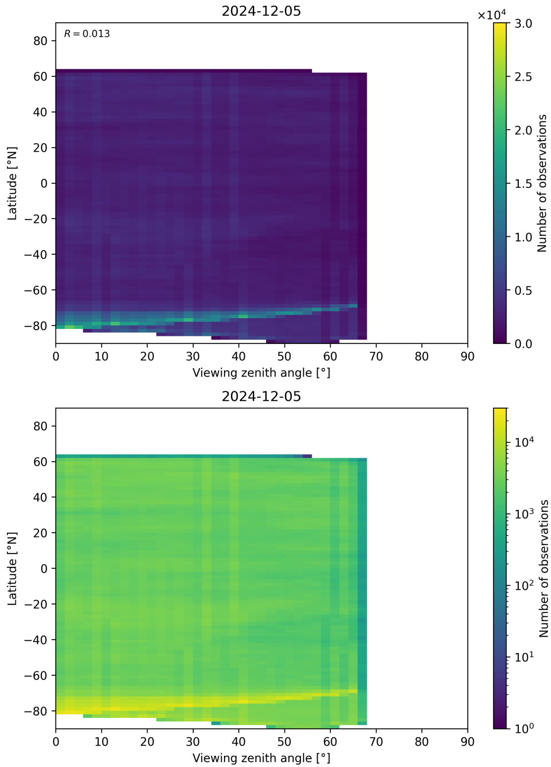
Figure 74: Scatter density plot of “Viewing zenith angle” against “Latitude” for 2024-12-04 to 2024-12-06.
