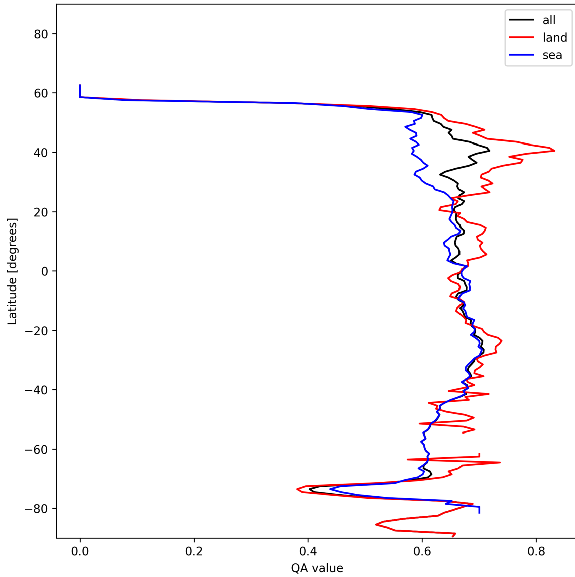
Figure 9: Zonal average of “QA value” for 2024-12-04 to 2024-12-06.
