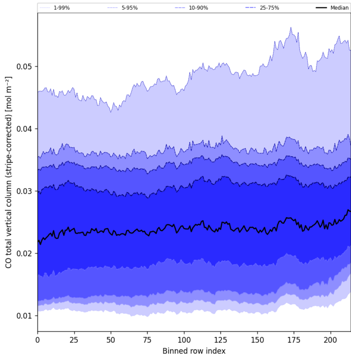
Figure 27: Along track statistics of “CO total vertical column (stripe-corrected)” for 2024-12-04 to 2024-12-06
