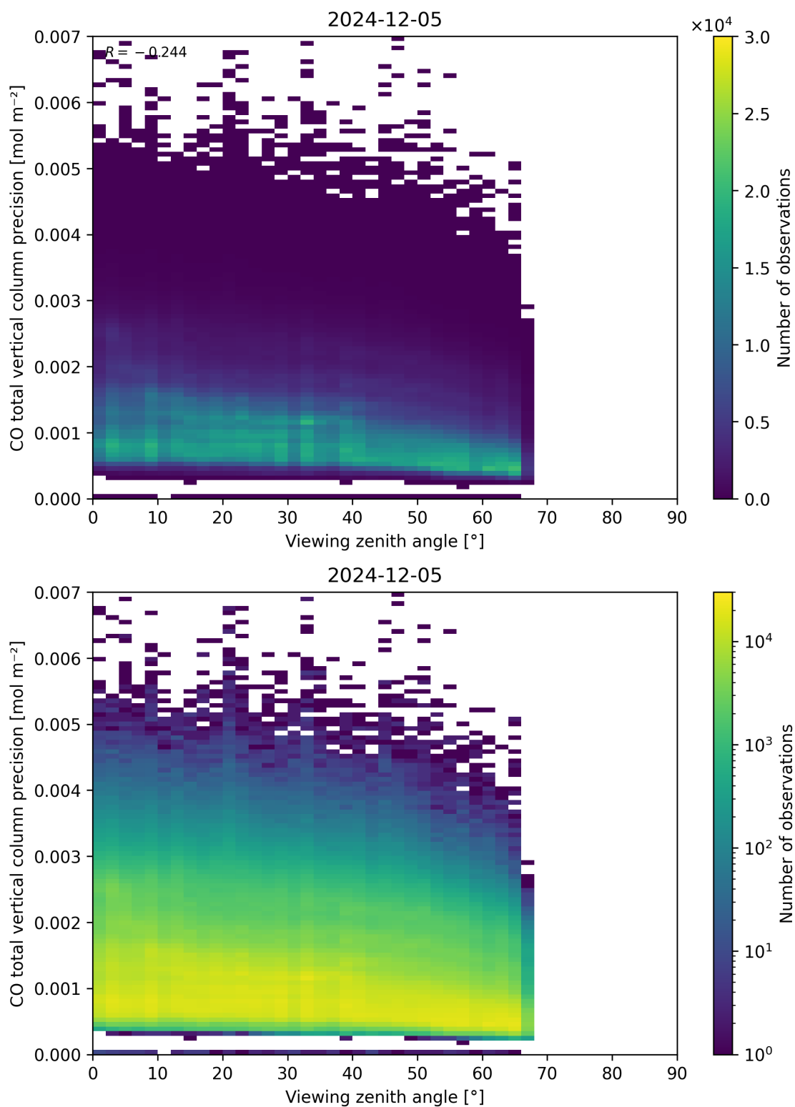
Figure 71: Scatter density plot of “Viewing zenith angle” against “CO total vertical column precision” for 2024-12-04 to 2024-12-06.
