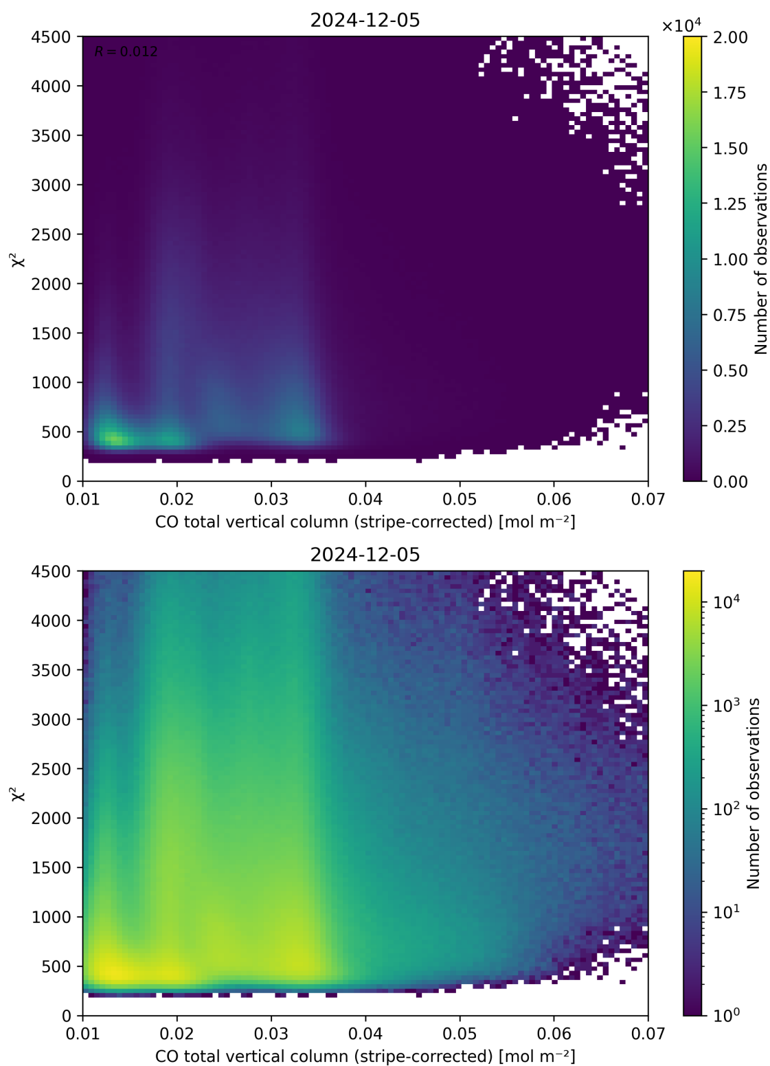
Figure 37: Scatter density plot of “CO total vertical column (stripe-corrected)” against “ \chi^2 ” for 2024-12-04 to 2024-12-06.
