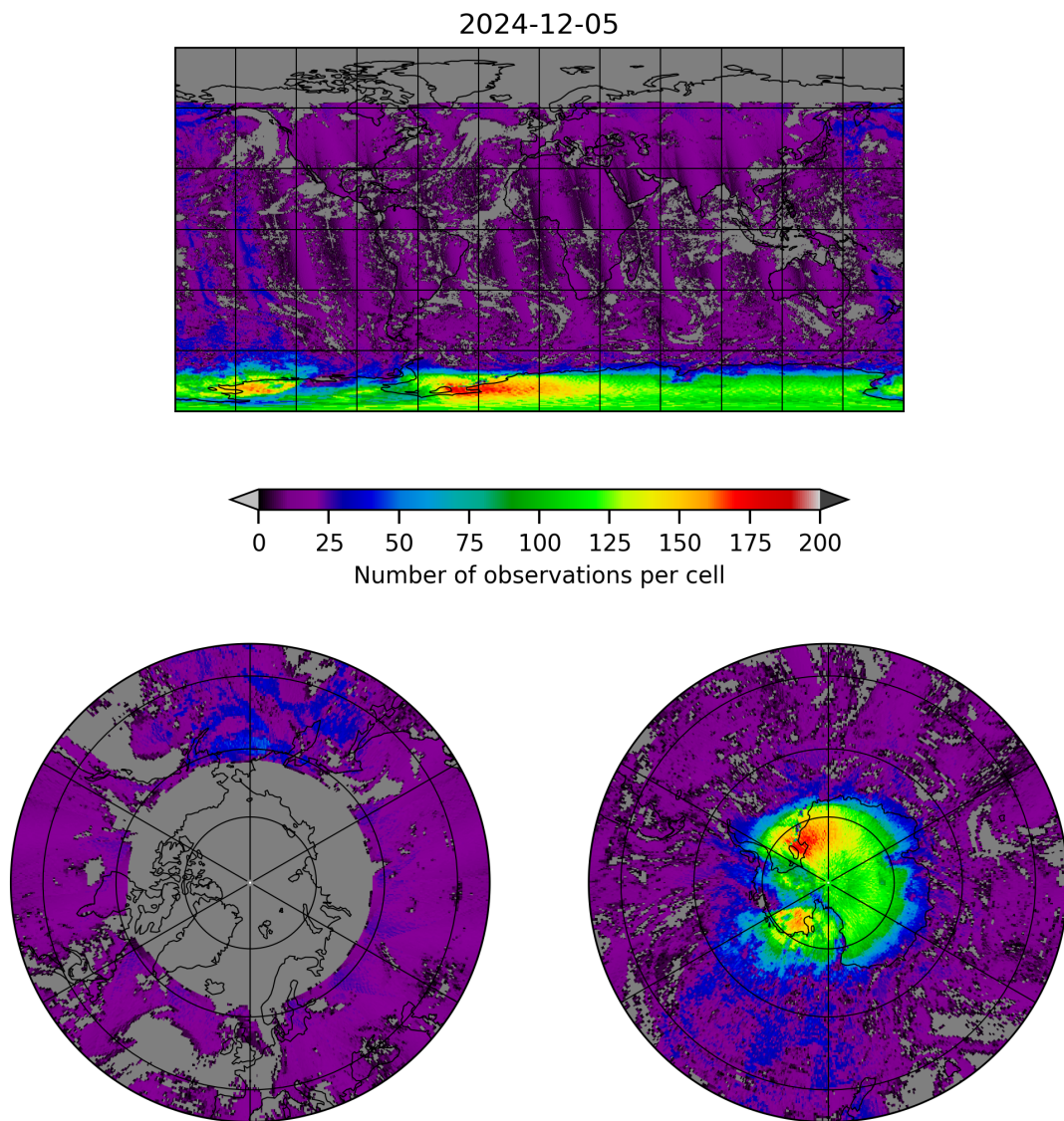
Figure 8: Map of the number of observations for 2024-12-04 to 2024-12-06
