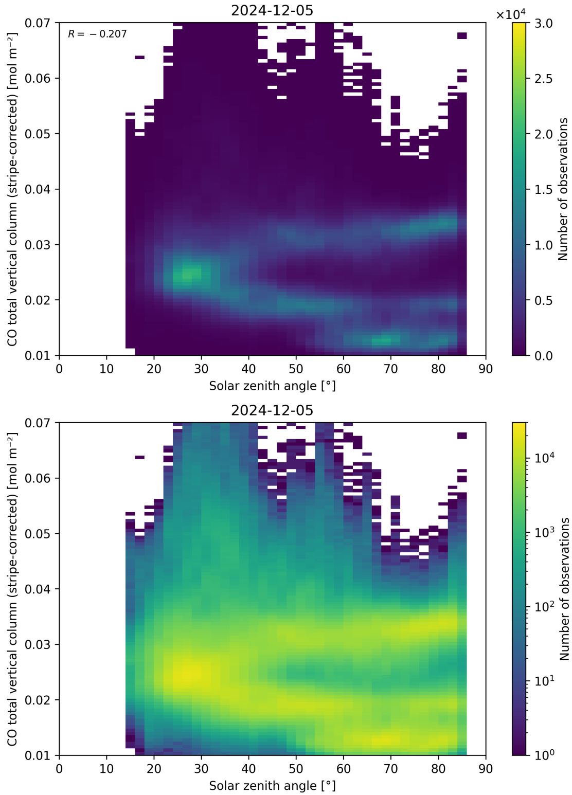
Figure 62: Scatter density plot of “Solar zenith angle” against “CO total vertical column (stripe-corrected)” for 2024-12-04 to 2024-12-06.
