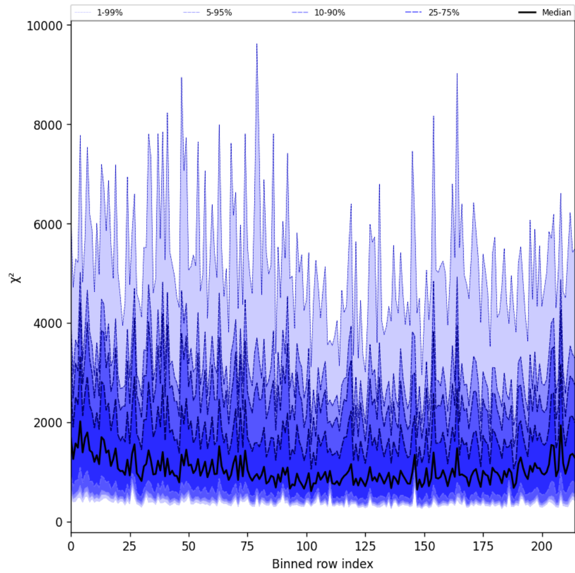
Figure 30: Along track statistics of “ \chi^2 ” for 2024-12-04 to 2024-12-06
