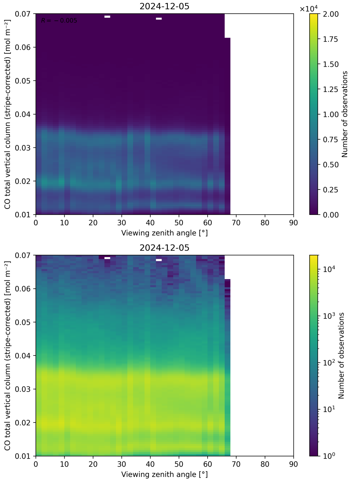
Figure 70: Scatter density plot of “Viewing zenith angle” against “CO total vertical column (stripe-corrected)” for 2024-12-04 to 2024-12-06.
