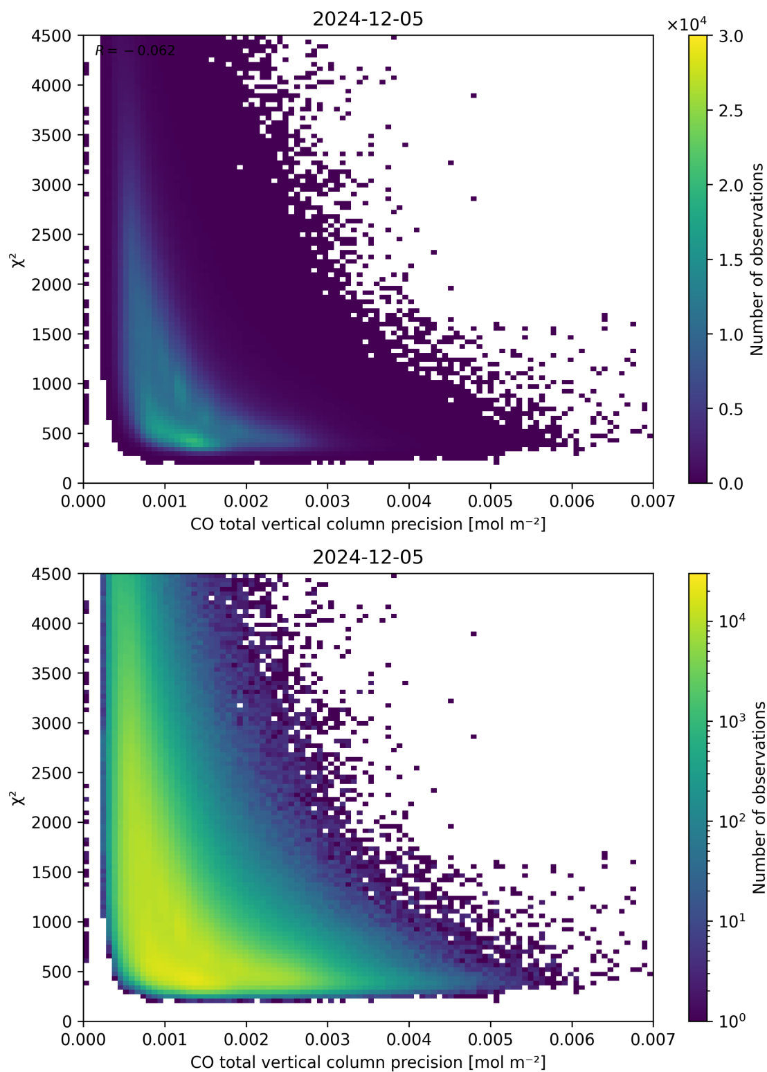
Figure 44: Scatter density plot of “CO total vertical column precision” against “ \chi^2 ” for 2024-12-04 to 2024-12-06.
