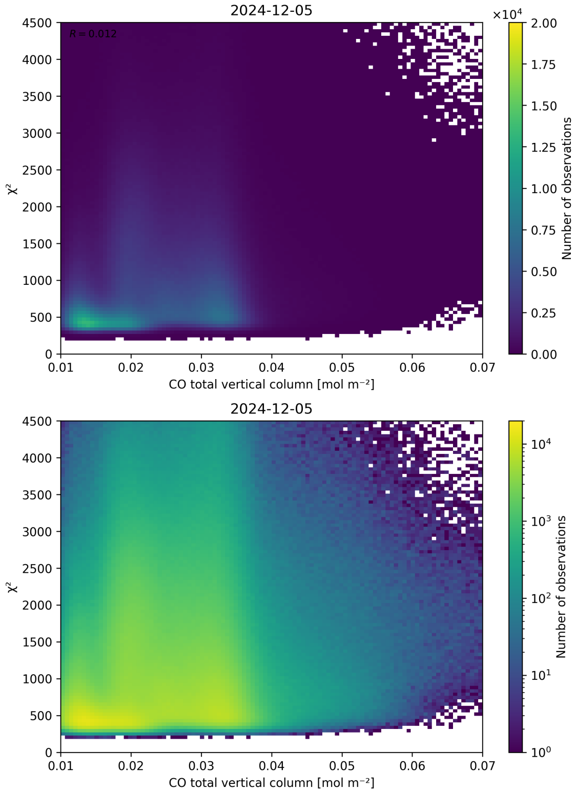
Figure 35: Scatter density plot of “CO total vertical column” against “ \chi^2 ” for 2024-12-04 to 2024-12-06.
