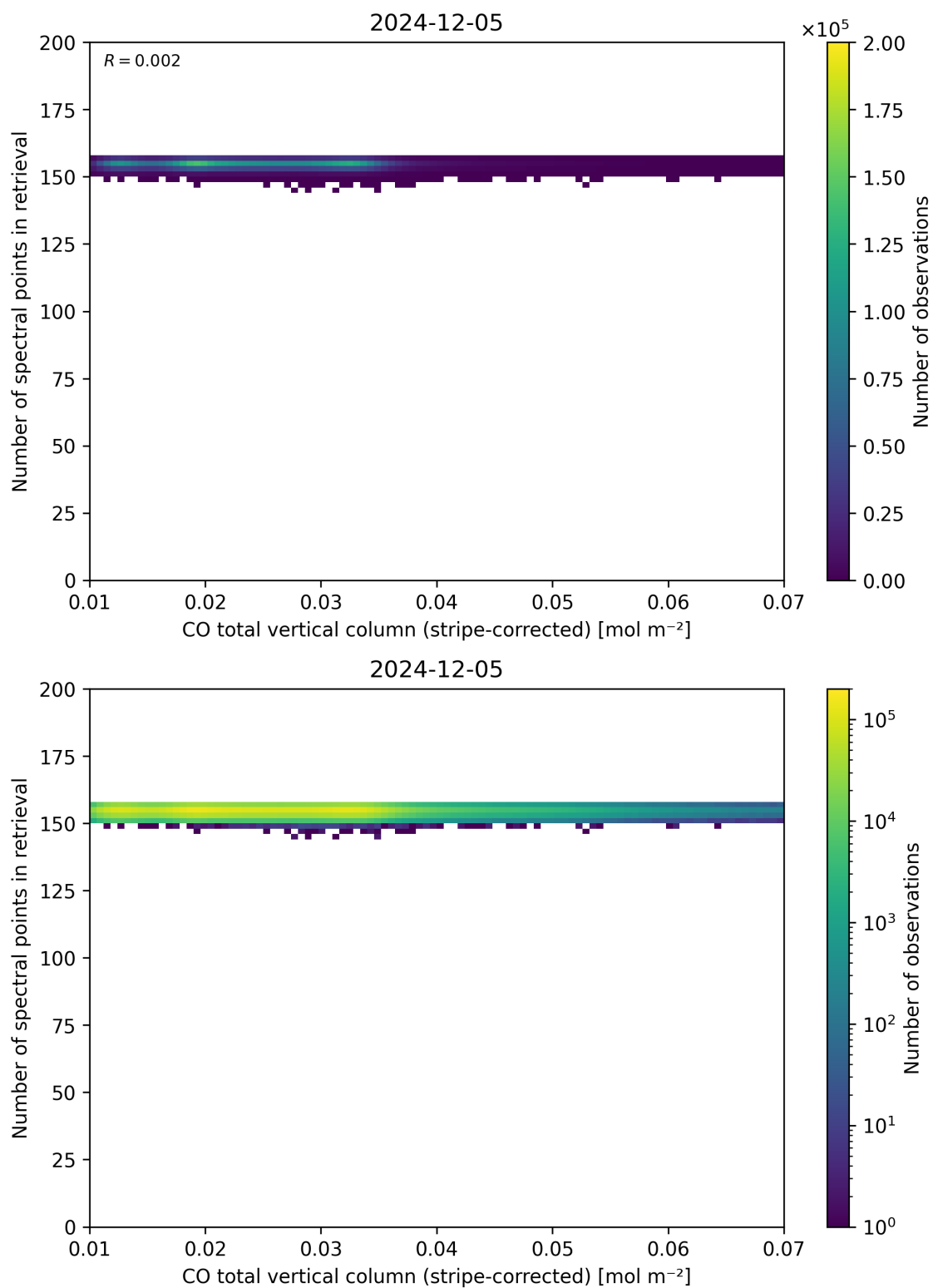
Figure 40: Scatter density plot of “CO total vertical column (stripe-corrected)” against “Number of spectral points in retrieval” for 2024-12-04 to 2024-12-06.
