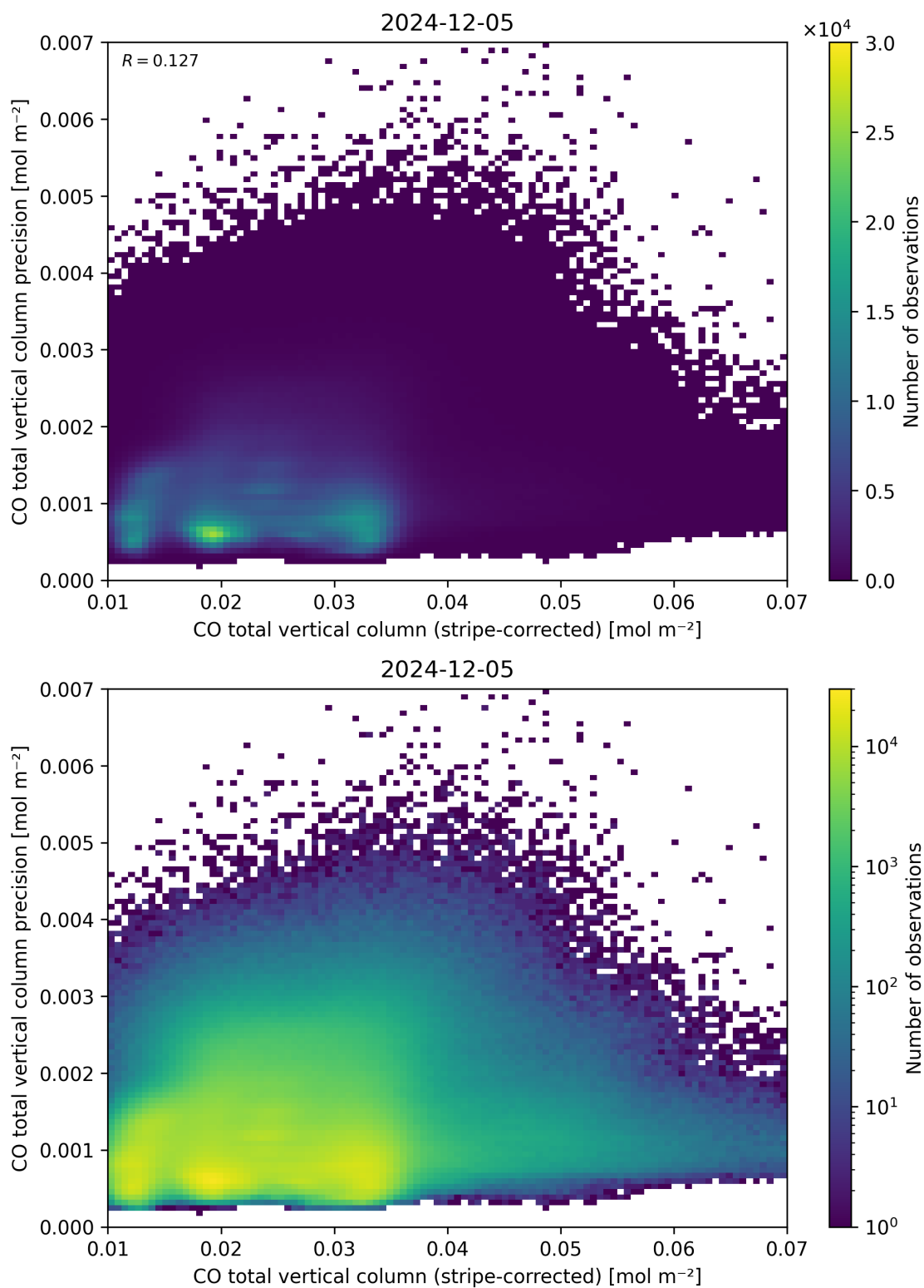
Figure 36: Scatter density plot of “CO total vertical column (stripe-corrected)” against “CO total vertical column precision” for 2024-12-04 to 2024-12-06.
