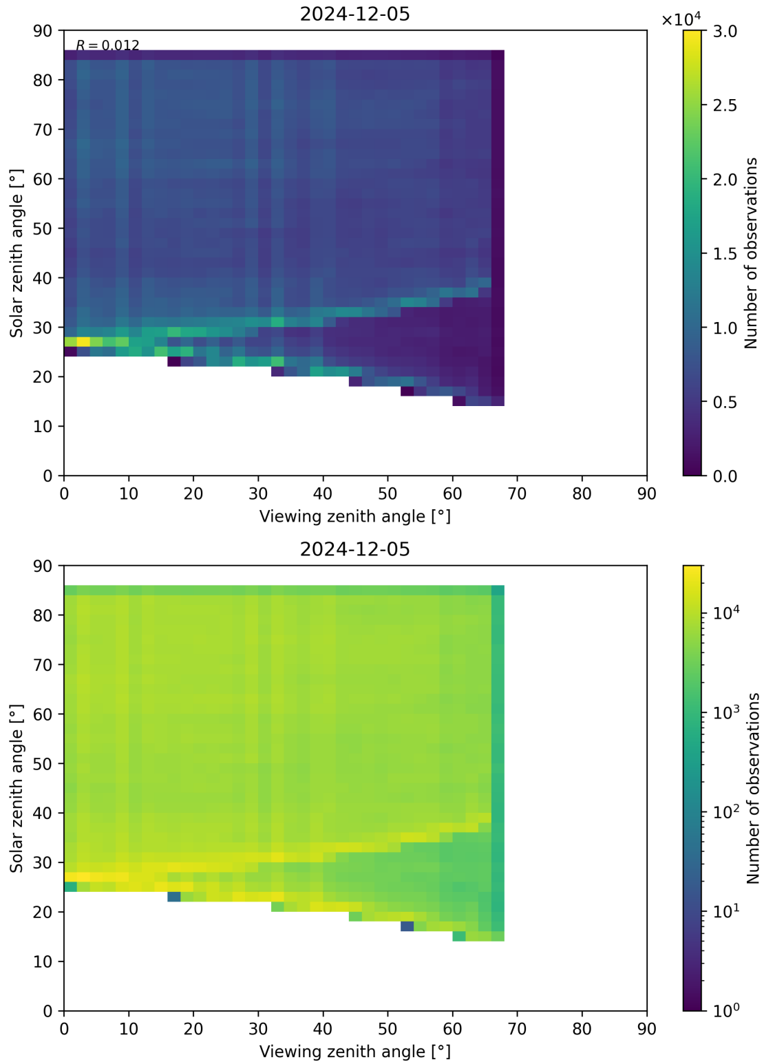
Figure 77: Scatter density plot of “Viewing zenith angle” against “Solar zenith angle” for 2024-12-04 to 2024-12-06.
