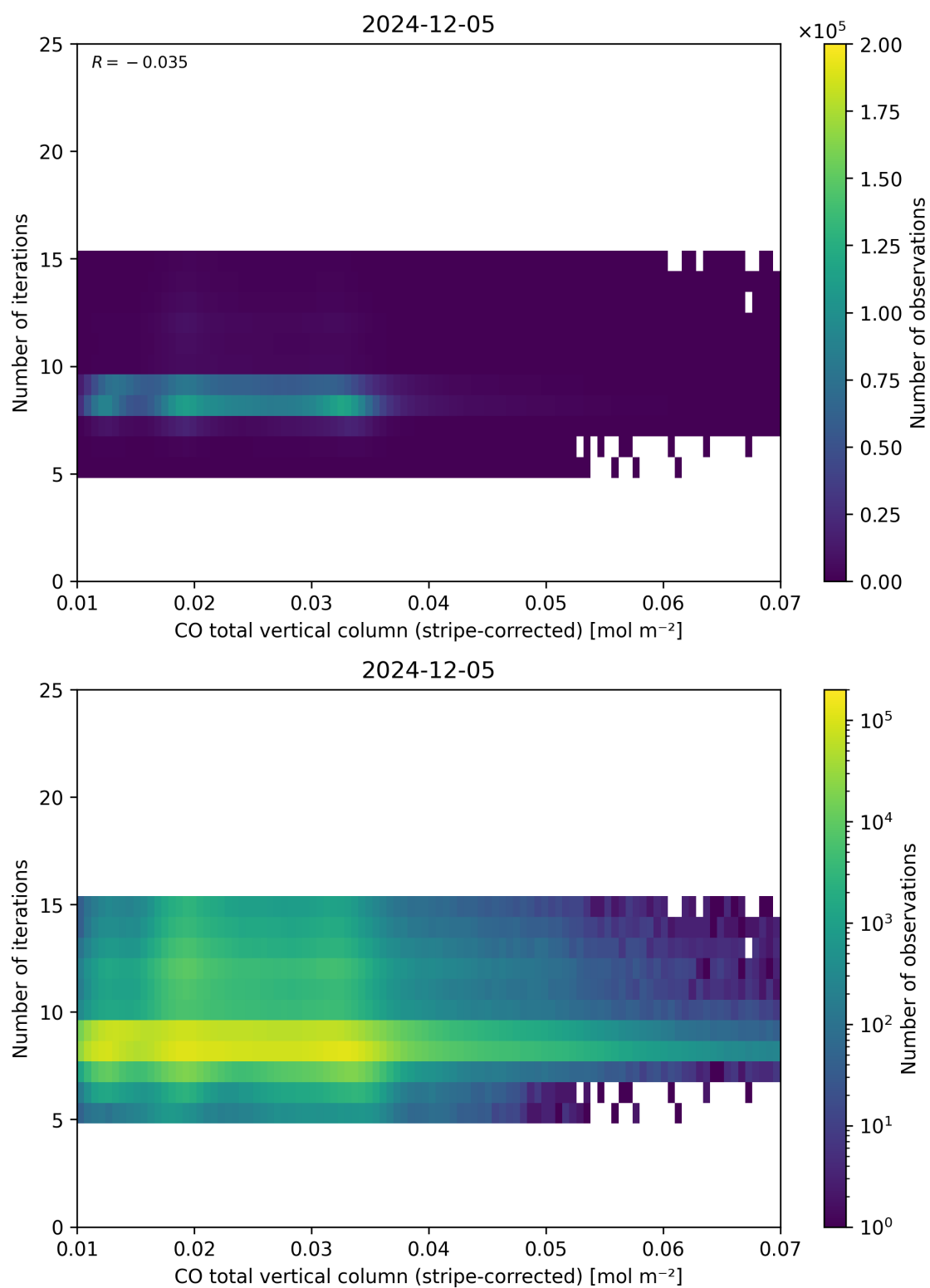
Figure 39: Scatter density plot of “CO total vertical column (stripe-corrected)” against “Number of iterations” for 2024-12-04 to 2024-12-06.
