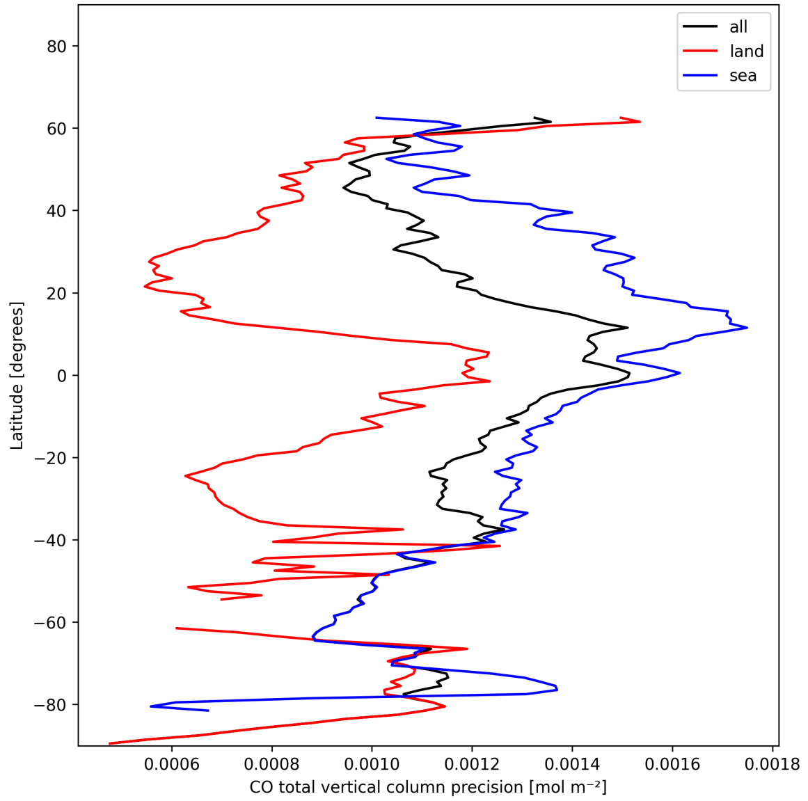
Figure 12: Zonal average of “CO total vertical column precision” for 2024-12-04 to 2024-12-06.
