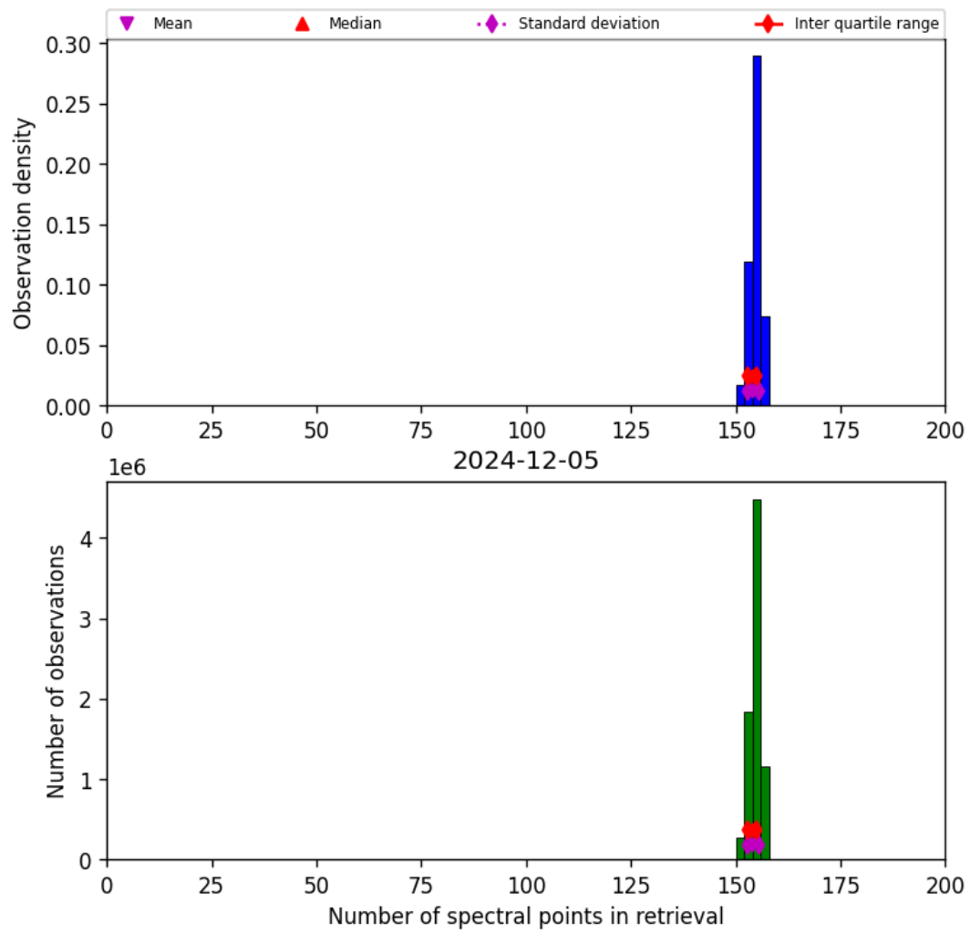
Figure 21: Histogram of “Number of spectral points in retrieval” for 2024-12-04 to 2024-12-06
