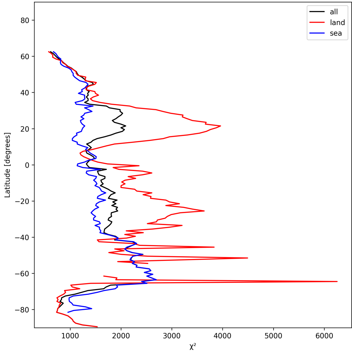
Figure 14: Zonal average of “ \chi^2 ” for 2024-12-04 to 2024-12-06.
