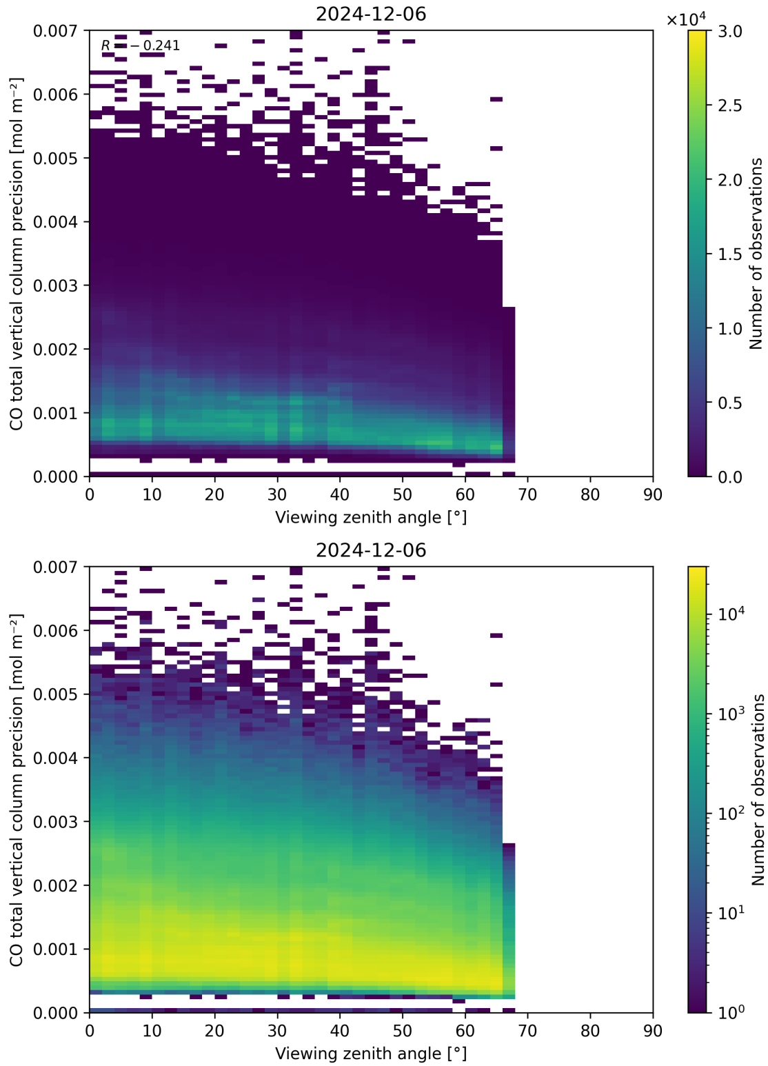
Figure 71: Scatter density plot of “Viewing zenith angle” against “CO total vertical column precision” for 2024-12-06 to 2024-12-07.
