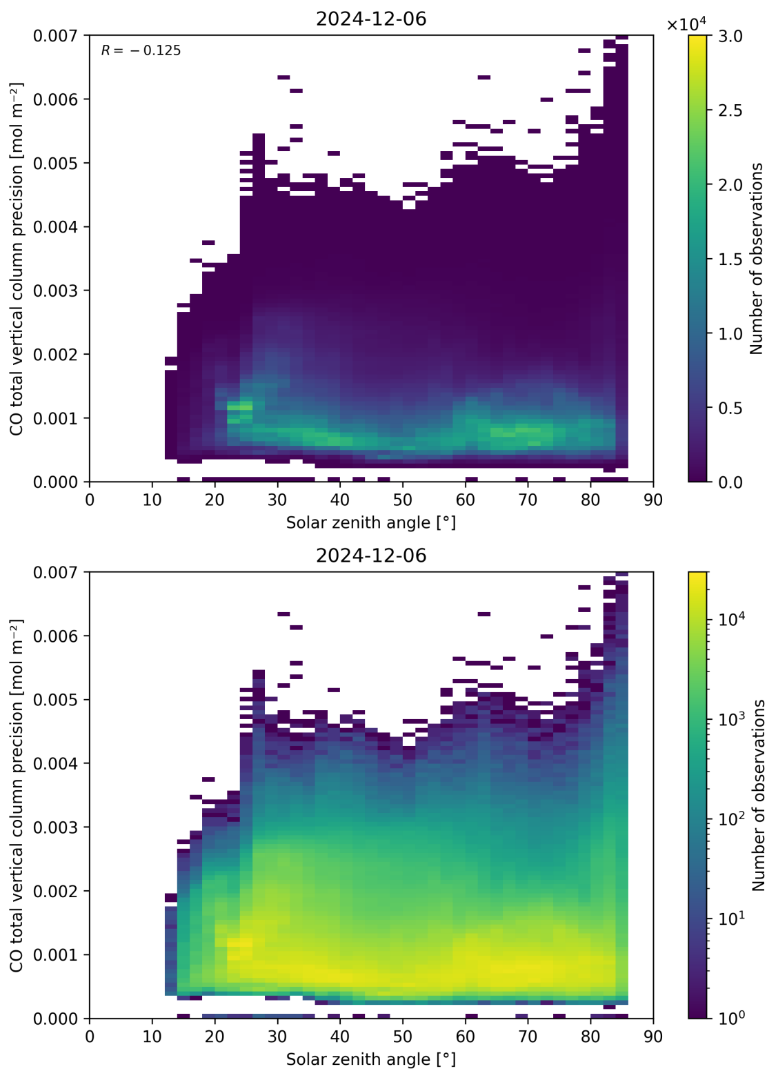
Figure 63: Scatter density plot of “Solar zenith angle” against “CO total vertical column precision” for 2024-12-06 to 2024-12-07.
