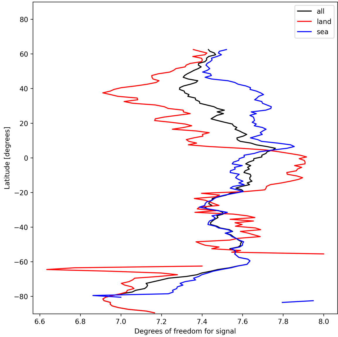
Figure 15: Zonal average of “Degrees of freedom for signal” for 2024-12-06 to 2024-12-07.
