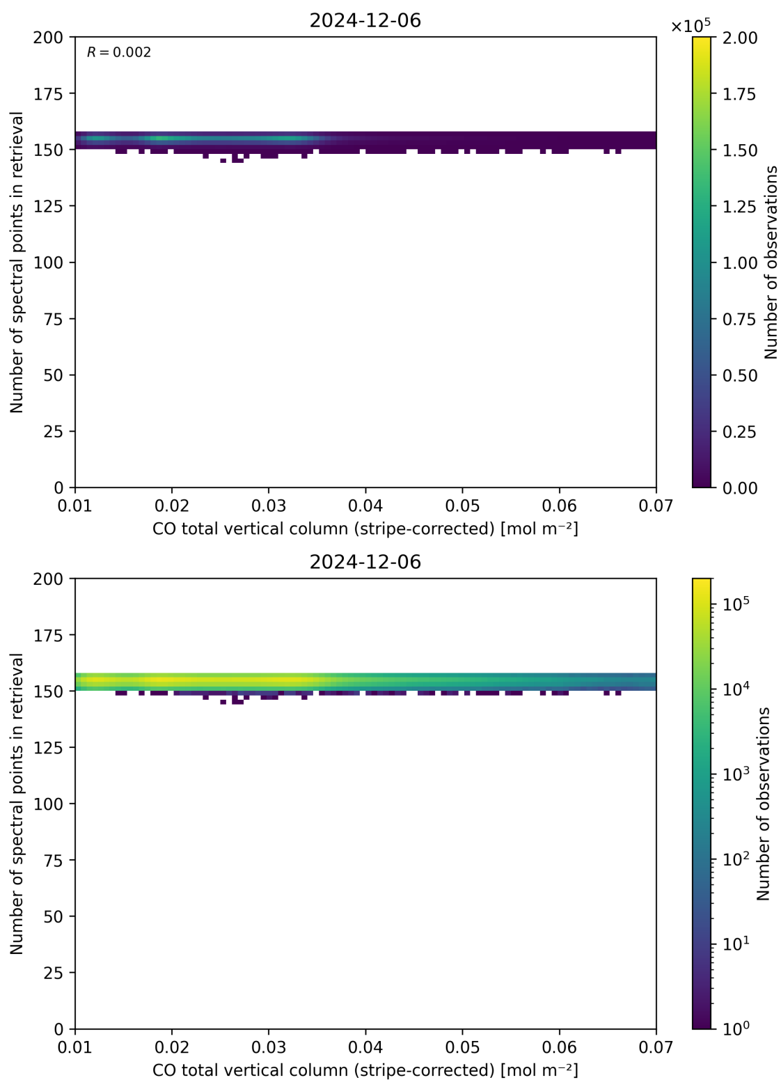
Figure 40: Scatter density plot of “CO total vertical column (stripe-corrected)” against “Number of spectral points in retrieval” for 2024-12-06 to 2024-12-07.
