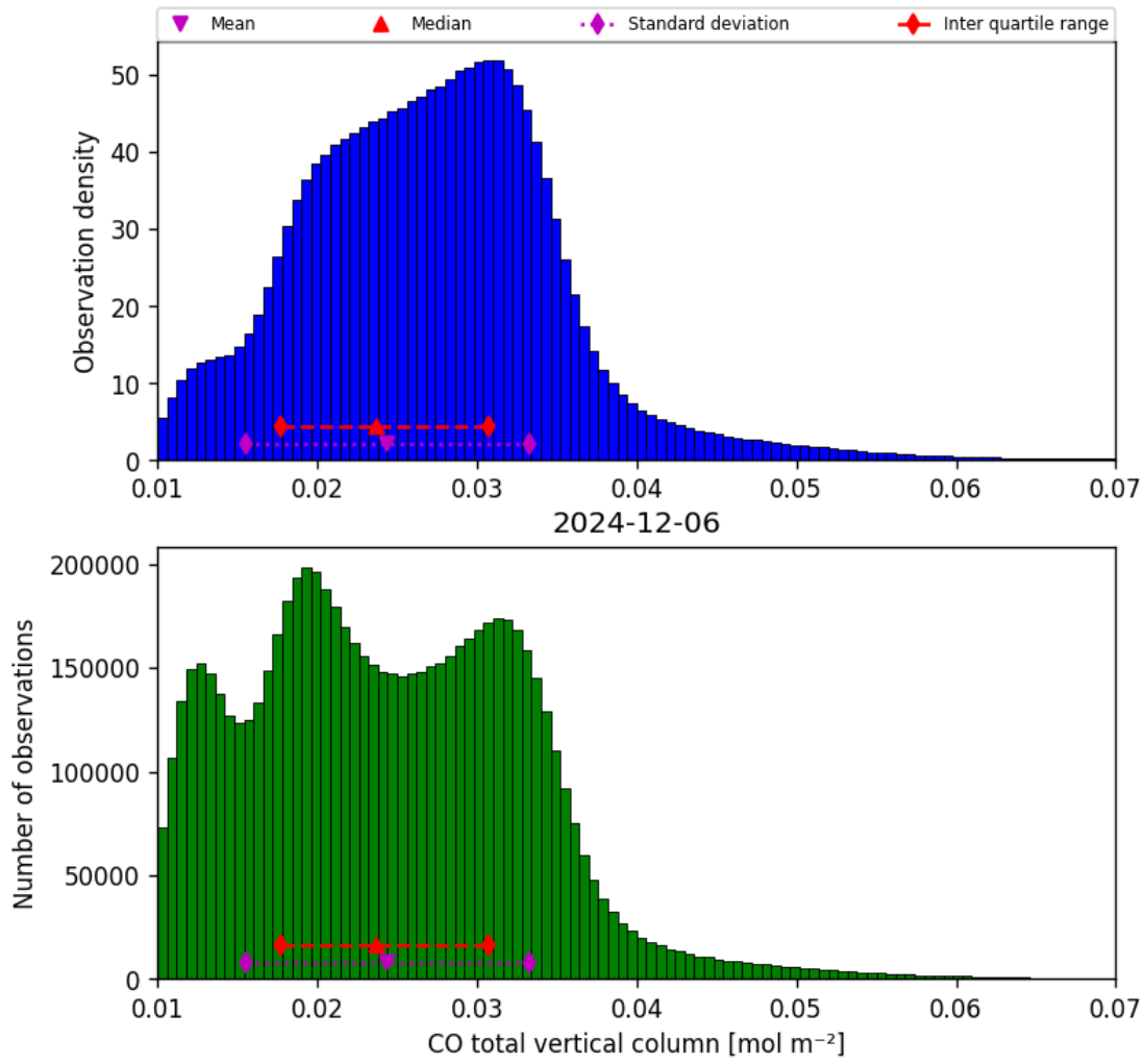
Figure 18: Histogram of “CO total vertical column” for 2024-12-06 to 2024-12-07
