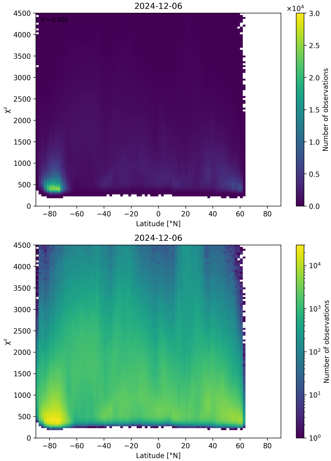
Figure 54: Scatter density plot of “Latitude” against “ \chi^2 ” for 2024-12-06 to 2024-12-07.
