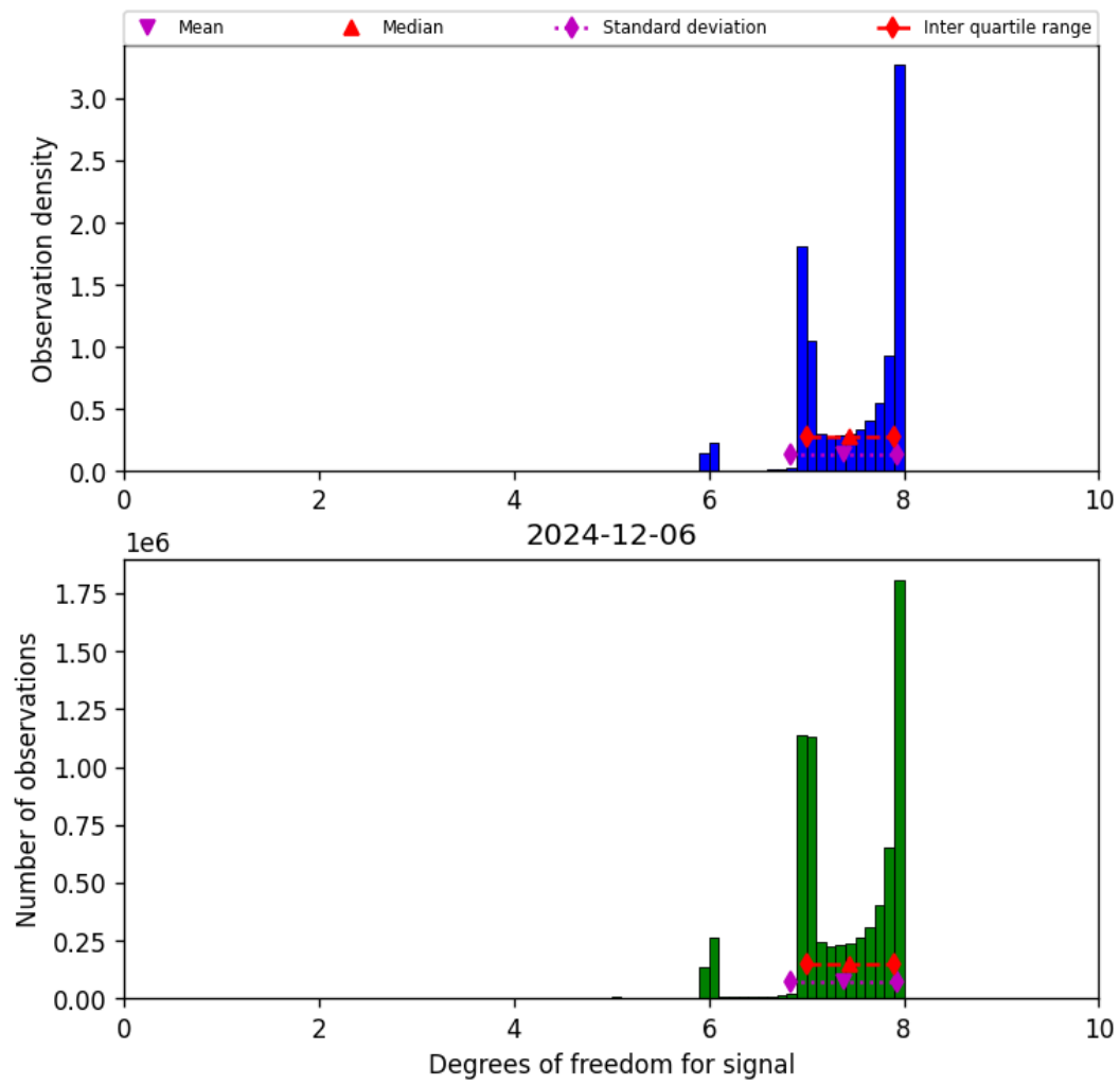
Figure 23: Histogram of “Degrees of freedom for signal” for 2024-12-06 to 2024-12-07
