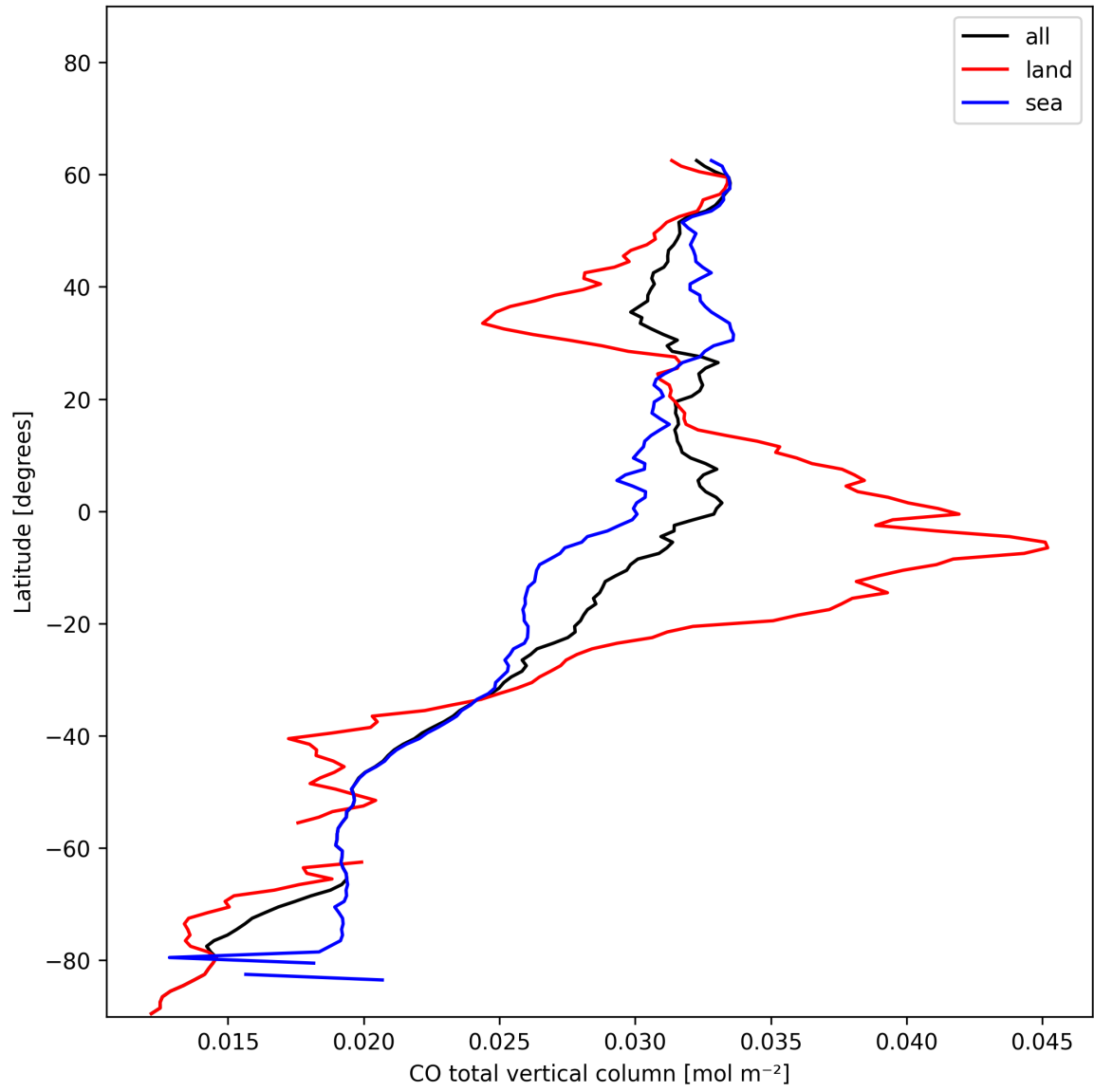
Figure 10: Zonal average of “CO total vertical column” for 2024-12-06 to 2024-12-07.
