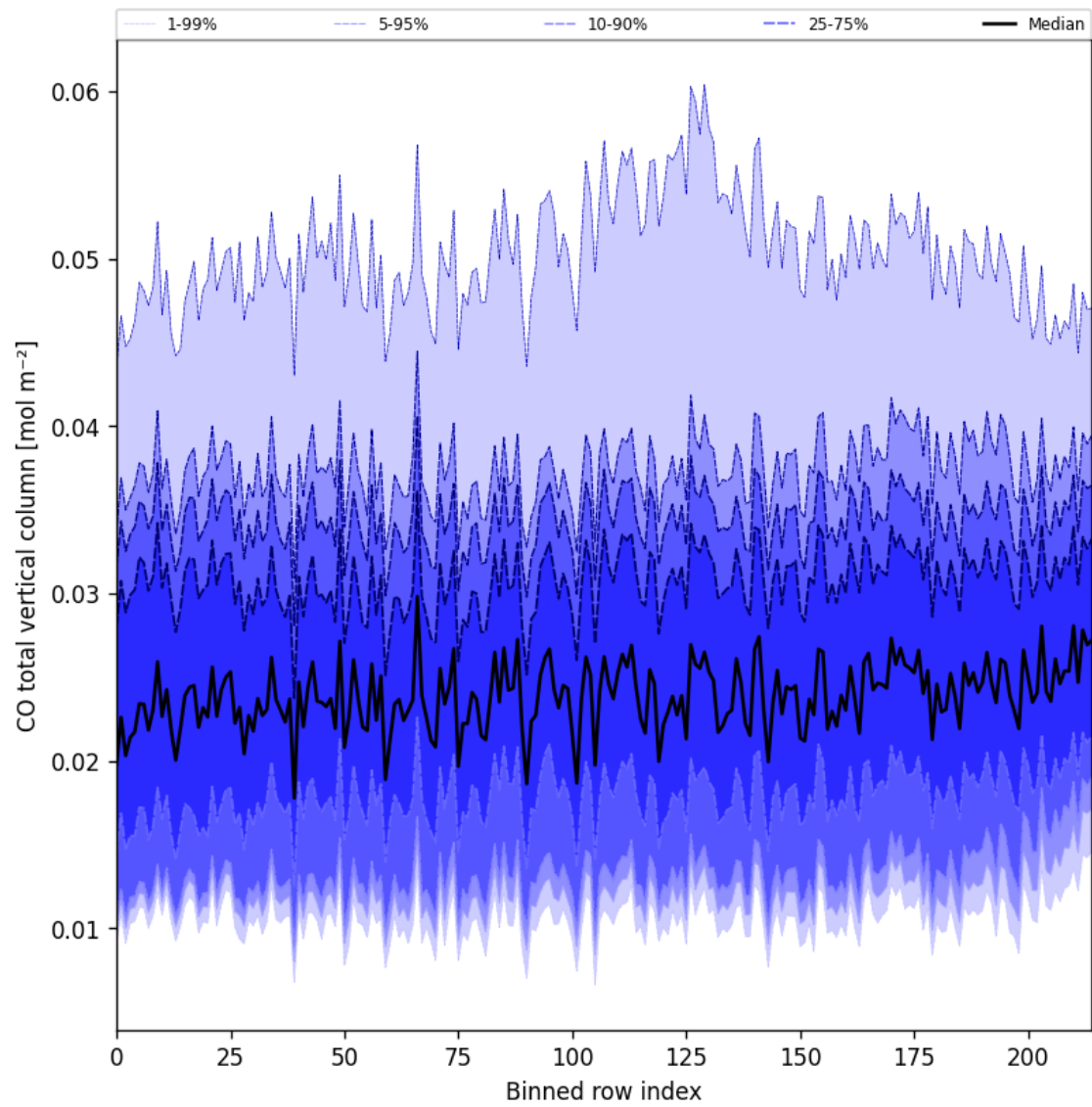
Figure 26: Along track statistics of “CO total vertical column” for 2024-12-06 to 2024-12-07
