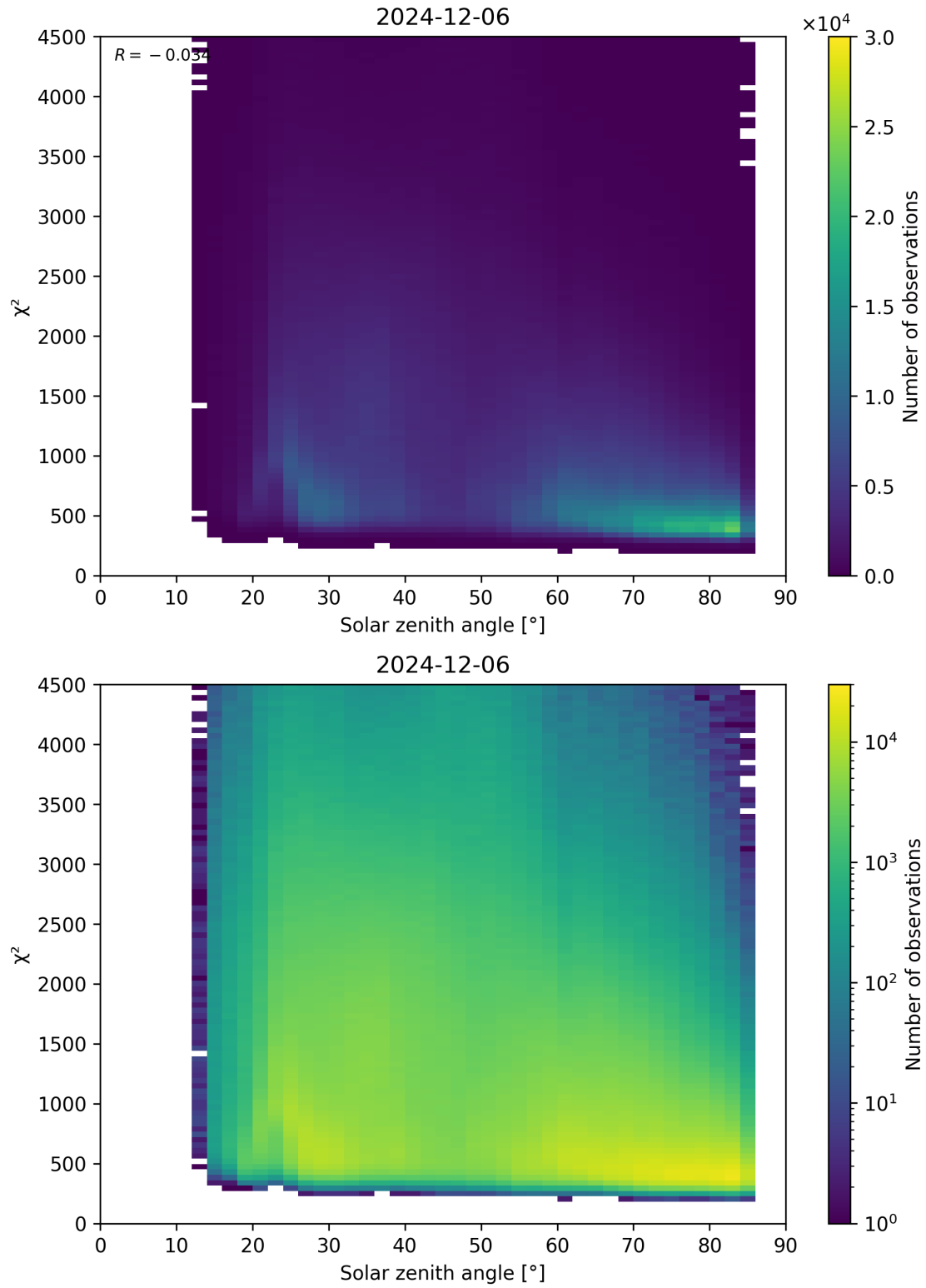
Figure 64: Scatter density plot of “Solar zenith angle” against “ \chi^2 ” for 2024-12-06 to 2024-12-07.
