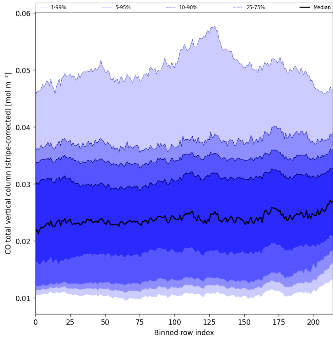
Figure 27: Along track statistics of “CO total vertical column (stripe-corrected)” for 2024-12-06 to 2024-12-07
