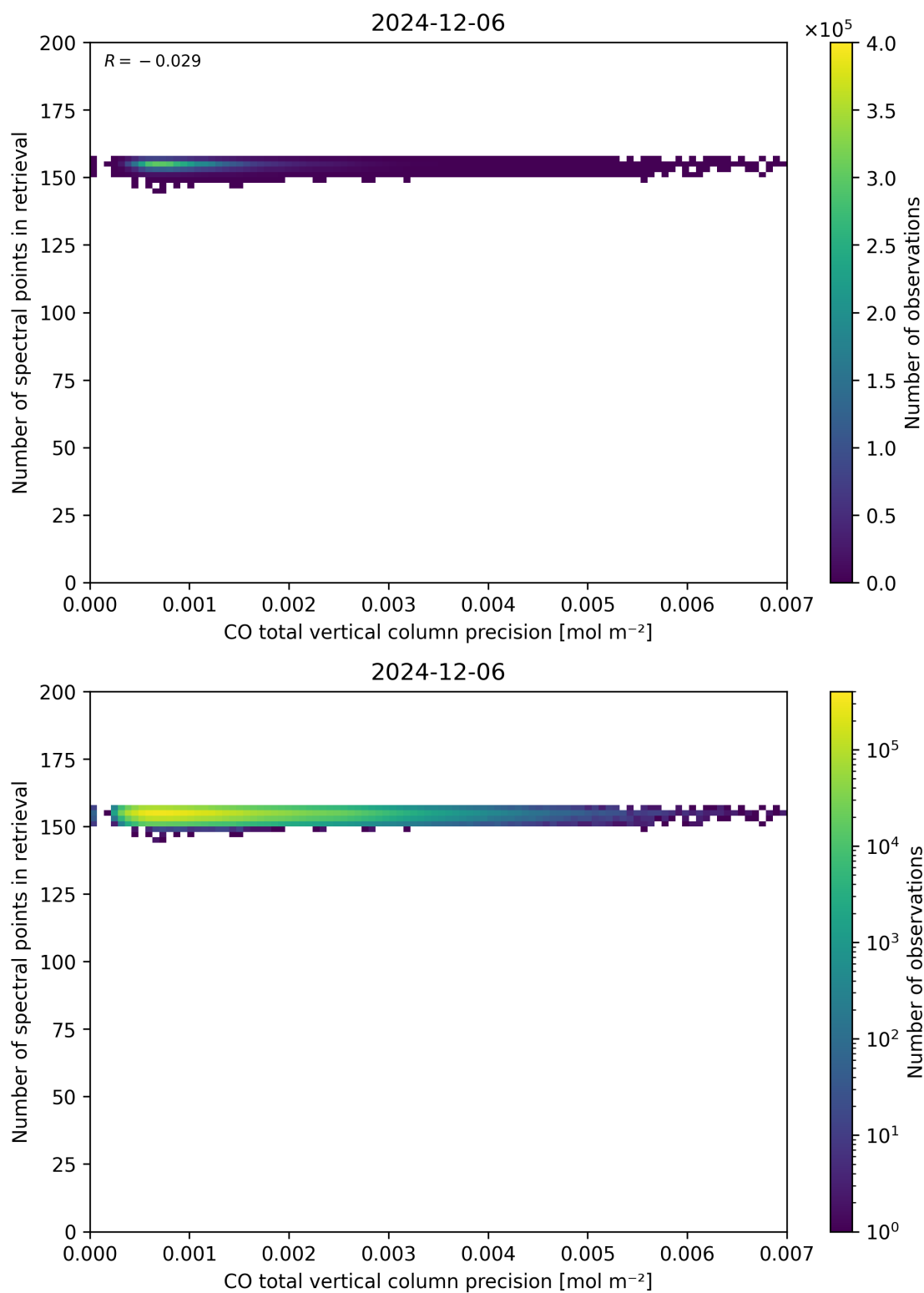
Figure 47: Scatter density plot of “CO total vertical column precision” against “Number of spectral points in retrieval” for 2024-12-06 to 2024-12-07.
