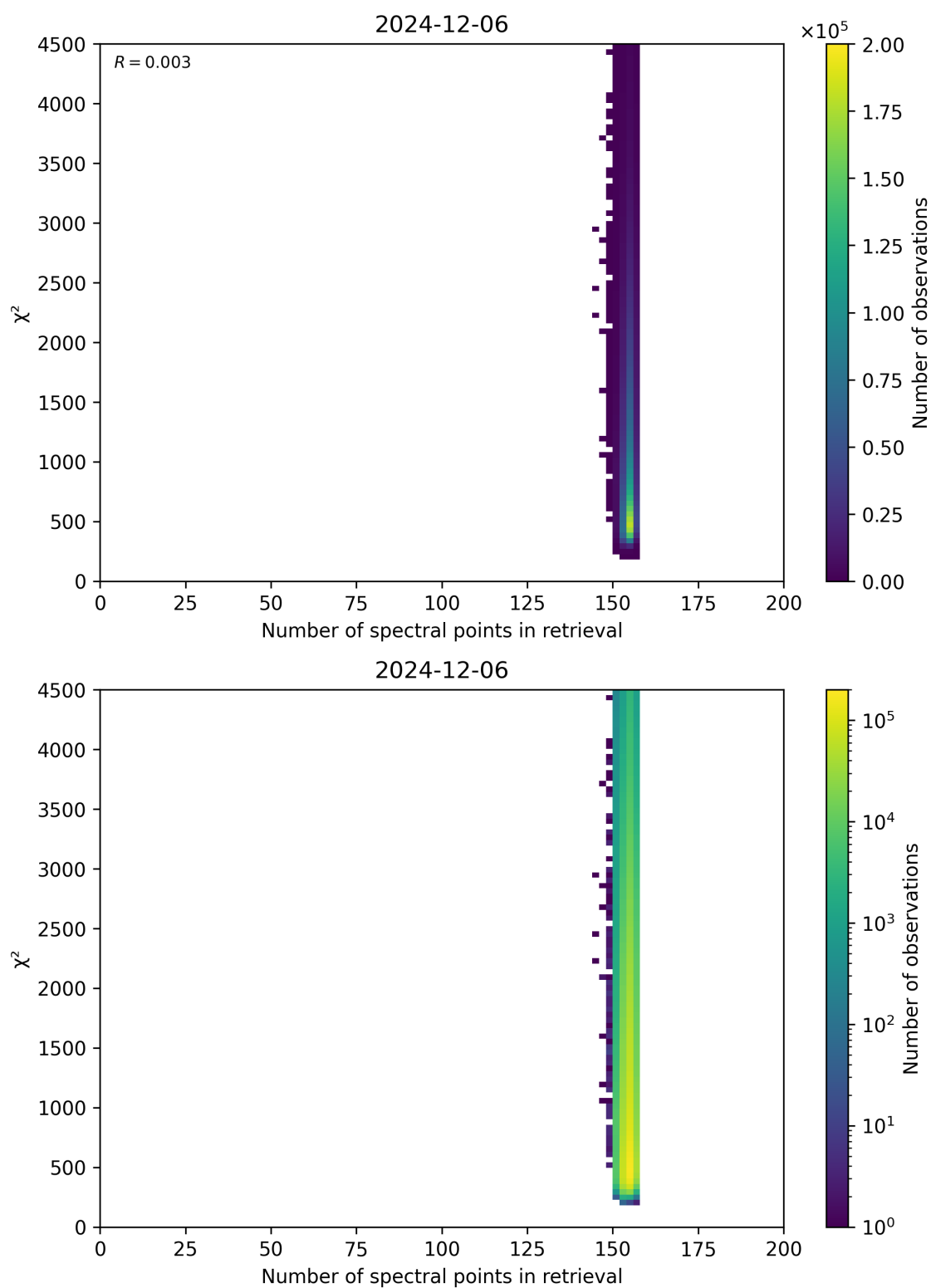
Figure 58: Scatter density plot of “Number of spectral points in retrieval” against “ \chi^2 ” for 2024-12-06 to 2024-12-07.
