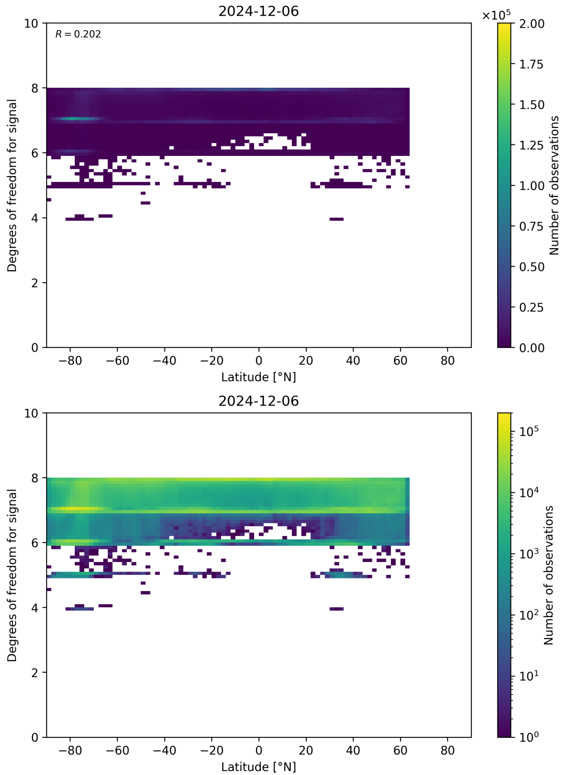
Figure 55: Scatter density plot of “Latitude” against “Degrees of freedom for signal” for 2024-12-06 to 2024-12-07.
