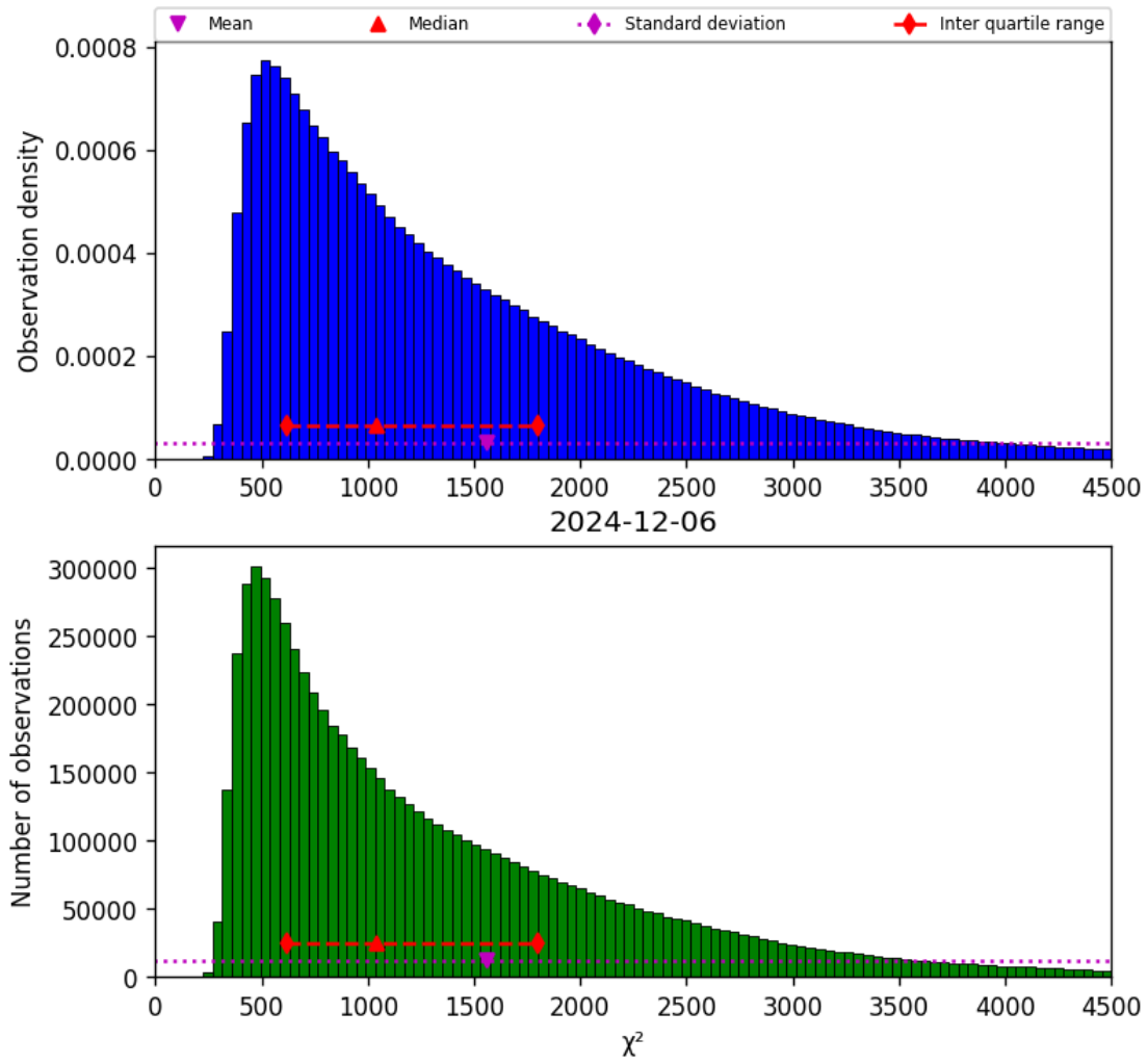
Figure 22: Histogram of “ \chi^2 ” for 2024-12-06 to 2024-12-07
