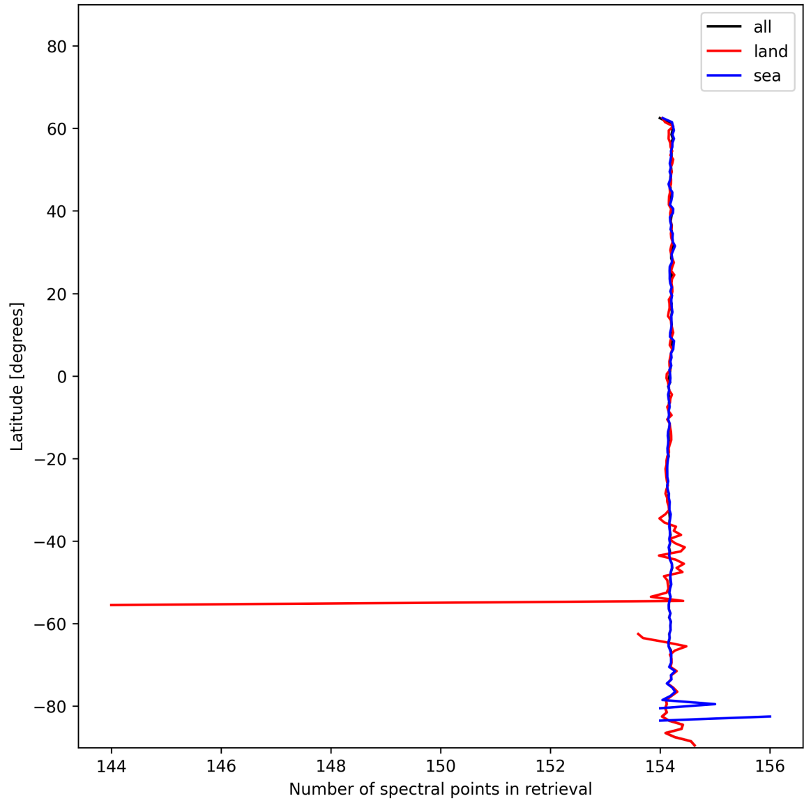
Figure 13: Zonal average of “Number of spectral points in retrieval” for 2024-12-06 to 2024-12-07.
