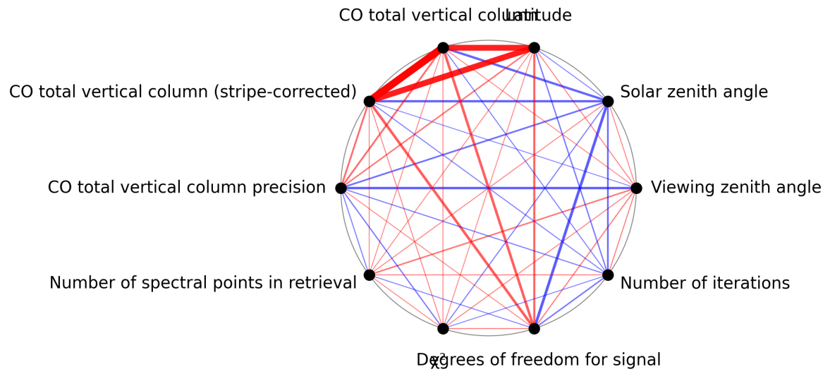
Figure 1: Map of correlation graph for 2024-12-06 to 2024-12-07.
