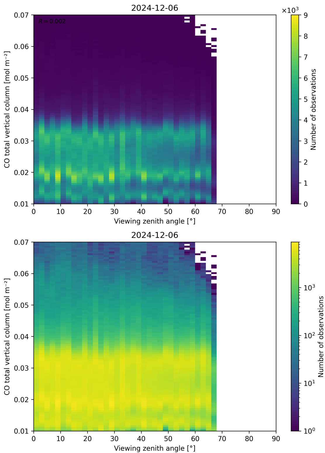
Figure 69: Scatter density plot of “Viewing zenith angle” against “CO total vertical column” for 2024-12-06 to 2024-12-07.
