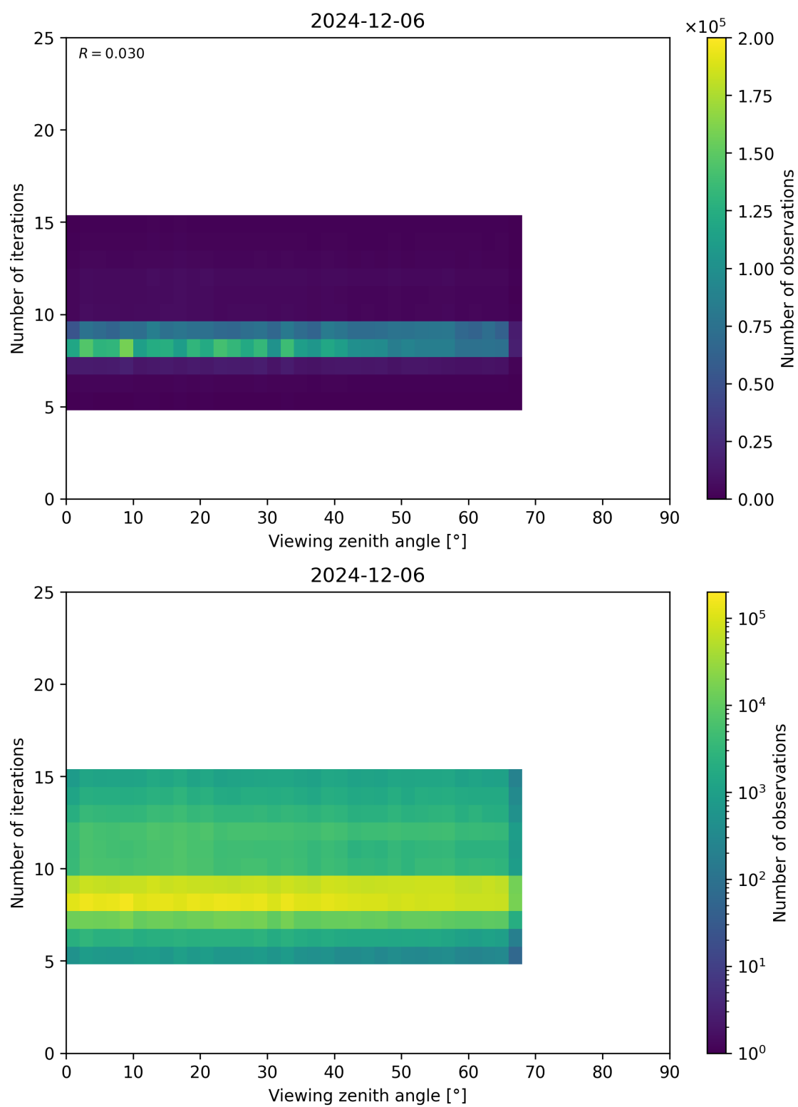
Figure 75: Scatter density plot of “Viewing zenith angle” against “Number of iterations” for 2024-12-06 to 2024-12-07.
