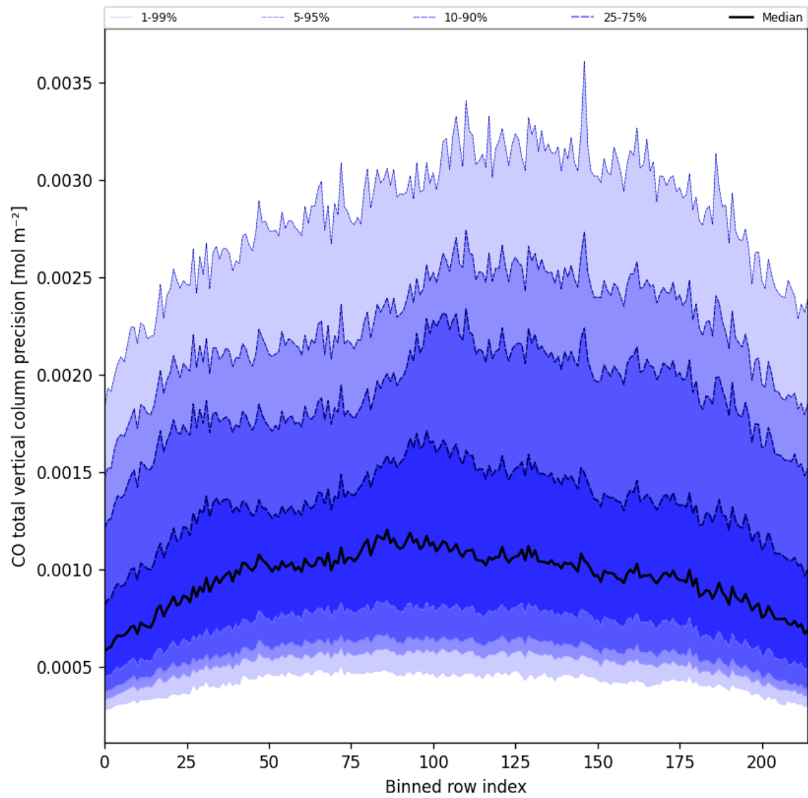
Figure 28: Along track statistics of “CO total vertical column precision” for 2024-12-06 to 2024-12-07
