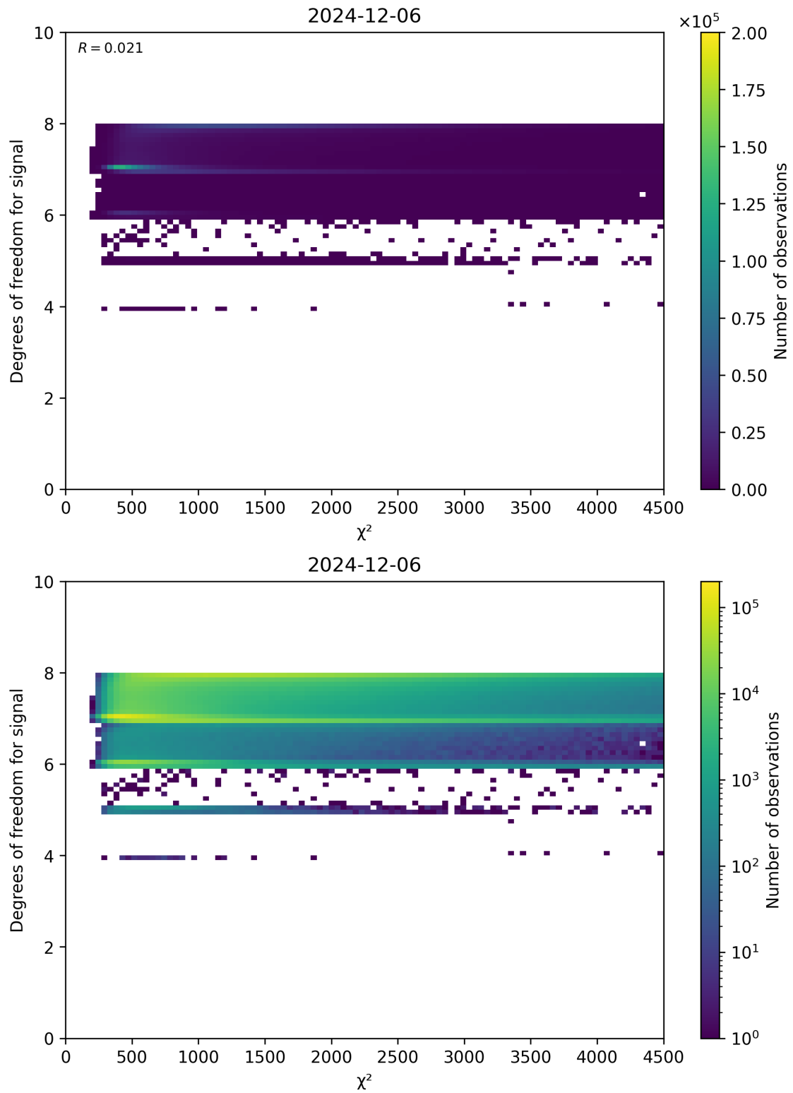
Figure 48: Scatter density plot of “ \chi^2 ” against “Degrees of freedom for signal” for 2024-12-06 to 2024-12-07.
