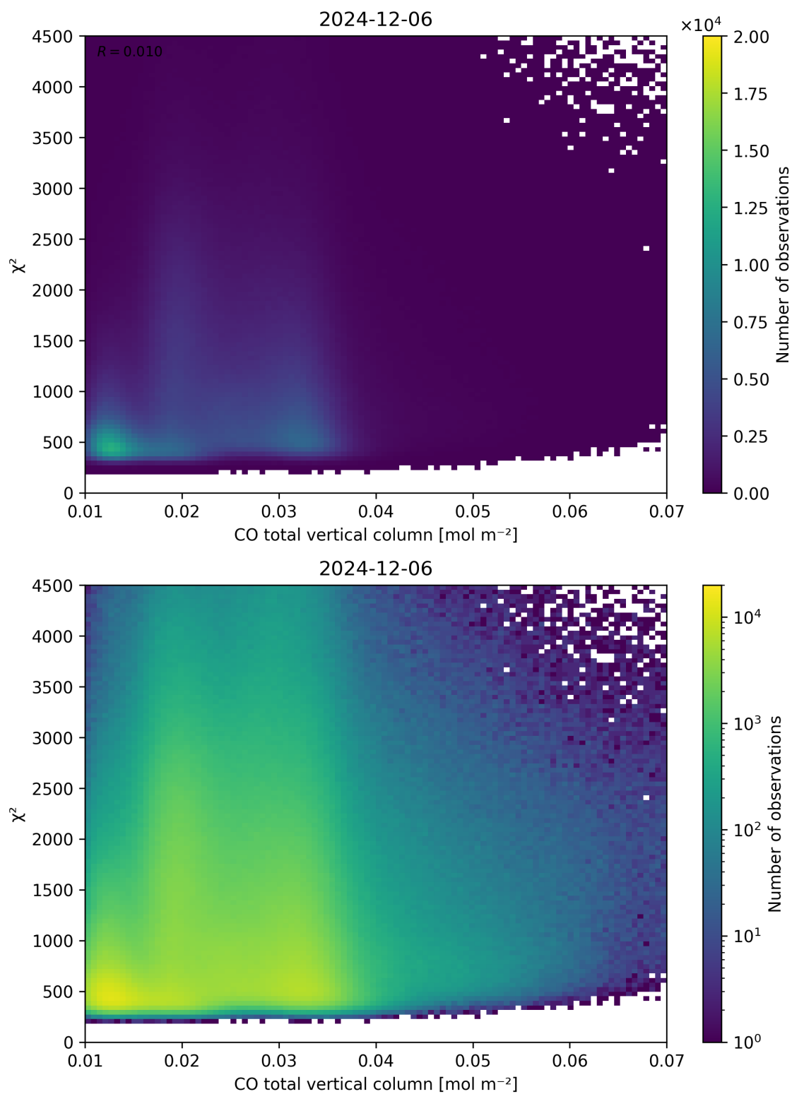
Figure 35: Scatter density plot of “CO total vertical column” against “ \chi^2 ” for 2024-12-06 to 2024-12-07.
