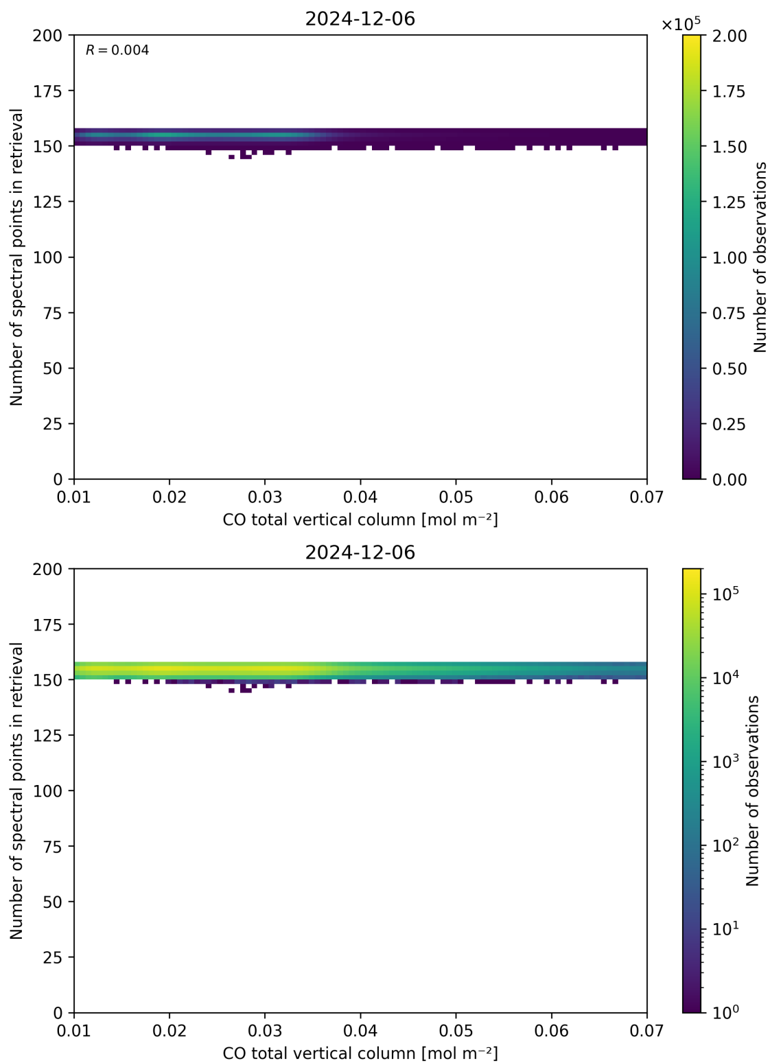
Figure 43: Scatter density plot of “CO total vertical column” against “Number of spectral points in retrieval” for 2024-12-06 to 2024-12-07.
