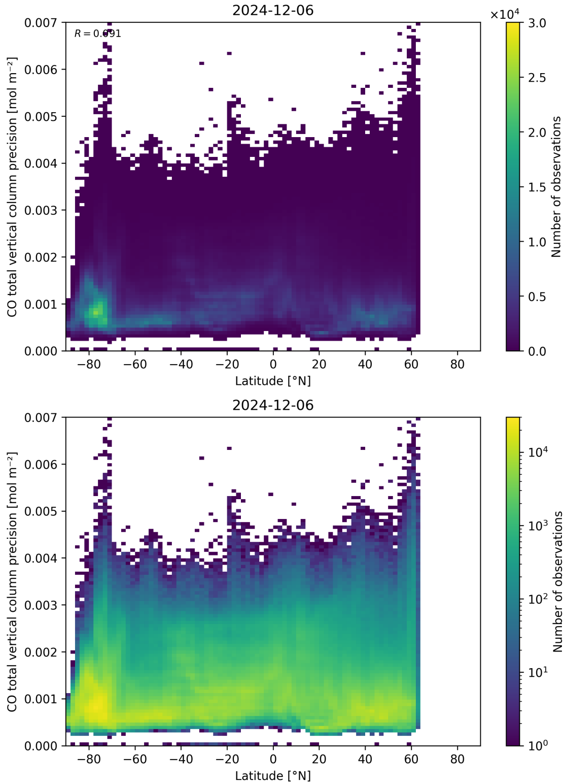
Figure 53: Scatter density plot of “Latitude” against “CO total vertical column precision” for 2024-12-06 to 2024-12-07.
