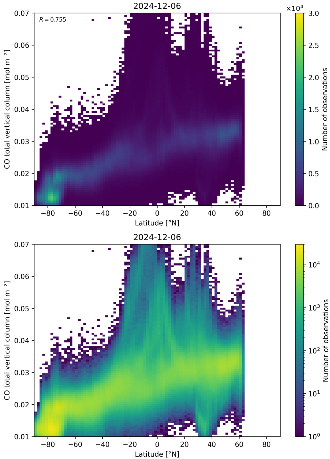
Figure 51: Scatter density plot of “Latitude” against “CO total vertical column” for 2024-12-06 to 2024-12-07.
