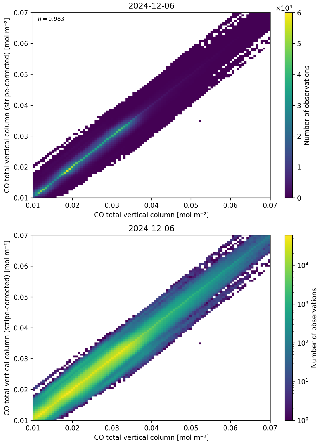
Figure 33: Scatter density plot of “CO total vertical column” against “CO total vertical column (stripe-corrected)” for 2024-12-06 to 2024-12-07.
