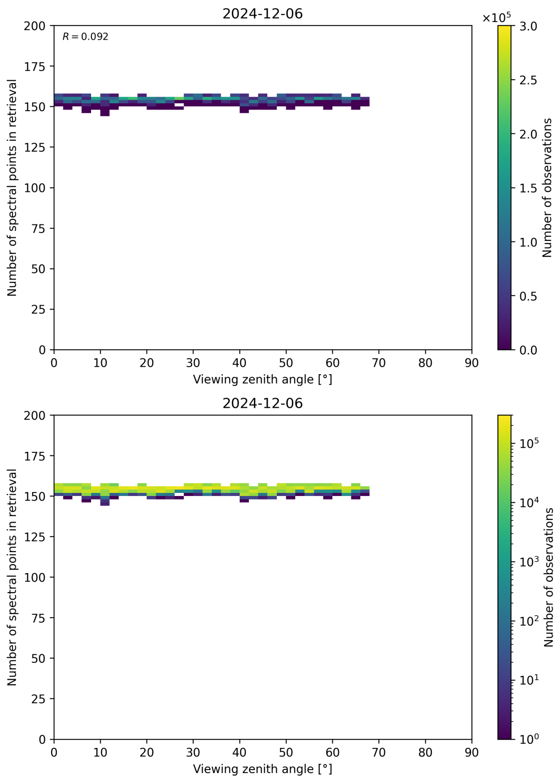
Figure 76: Scatter density plot of “Viewing zenith angle” against “Number of spectral points in retrieval” for 2024-12-06 to 2024-12-07.
