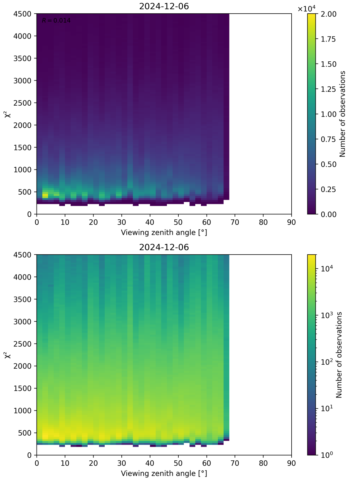
Figure 72: Scatter density plot of “Viewing zenith angle” against “ \chi^2 ” for 2024-12-06 to 2024-12-07.
