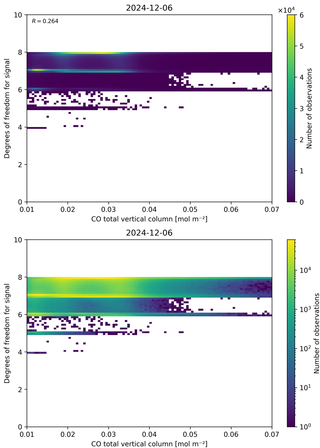
Figure 41: Scatter density plot of “CO total vertical column” against “Degrees of freedom for signal” for 2024-12-06 to 2024-12-07.
