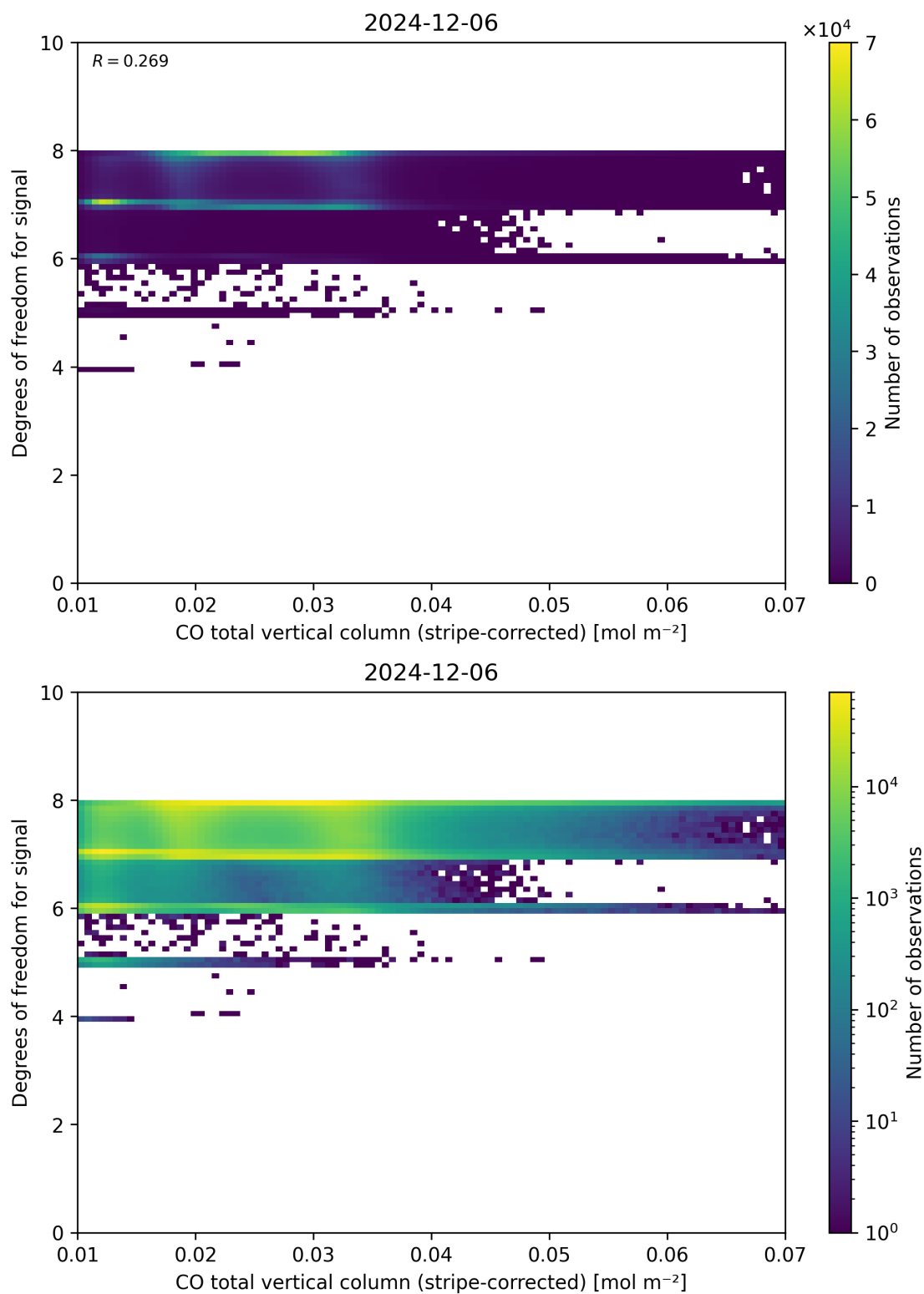
Figure 38: Scatter density plot of “CO total vertical column (stripe-corrected)” against “Degrees of freedom for signal” for 2024-12-06 to 2024-12-07.
