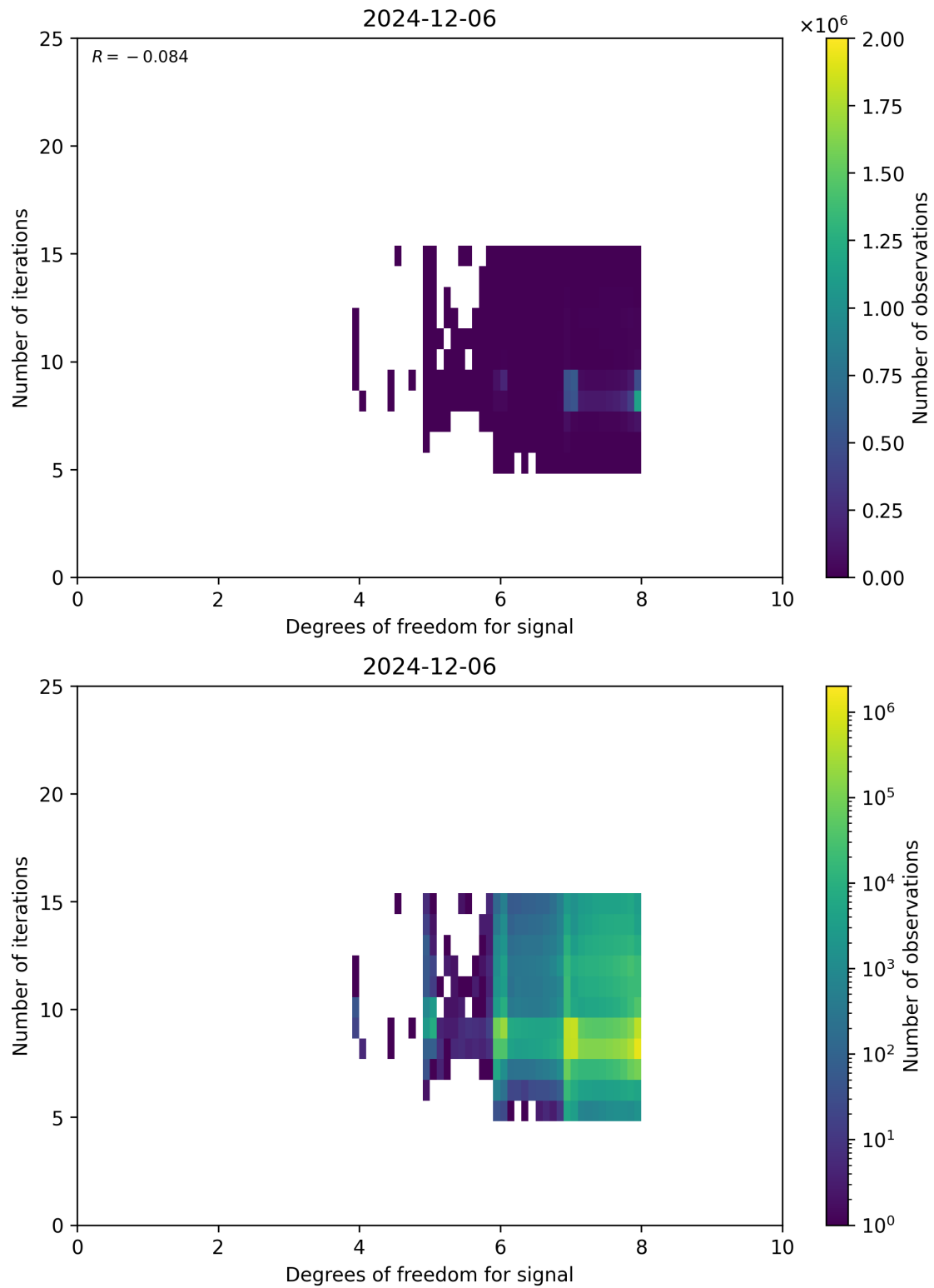
Figure 50: Scatter density plot of “Degrees of freedom for signal” against “Number of iterations” for 2024-12-06 to 2024-12-07.
