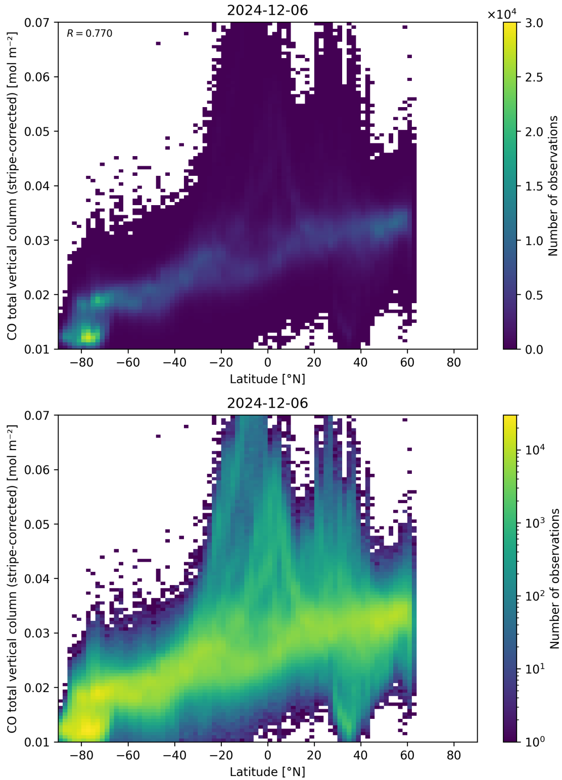
Figure 52: Scatter density plot of “Latitude” against “CO total vertical column (stripe-corrected)” for 2024-12-06 to 2024-12-07.
