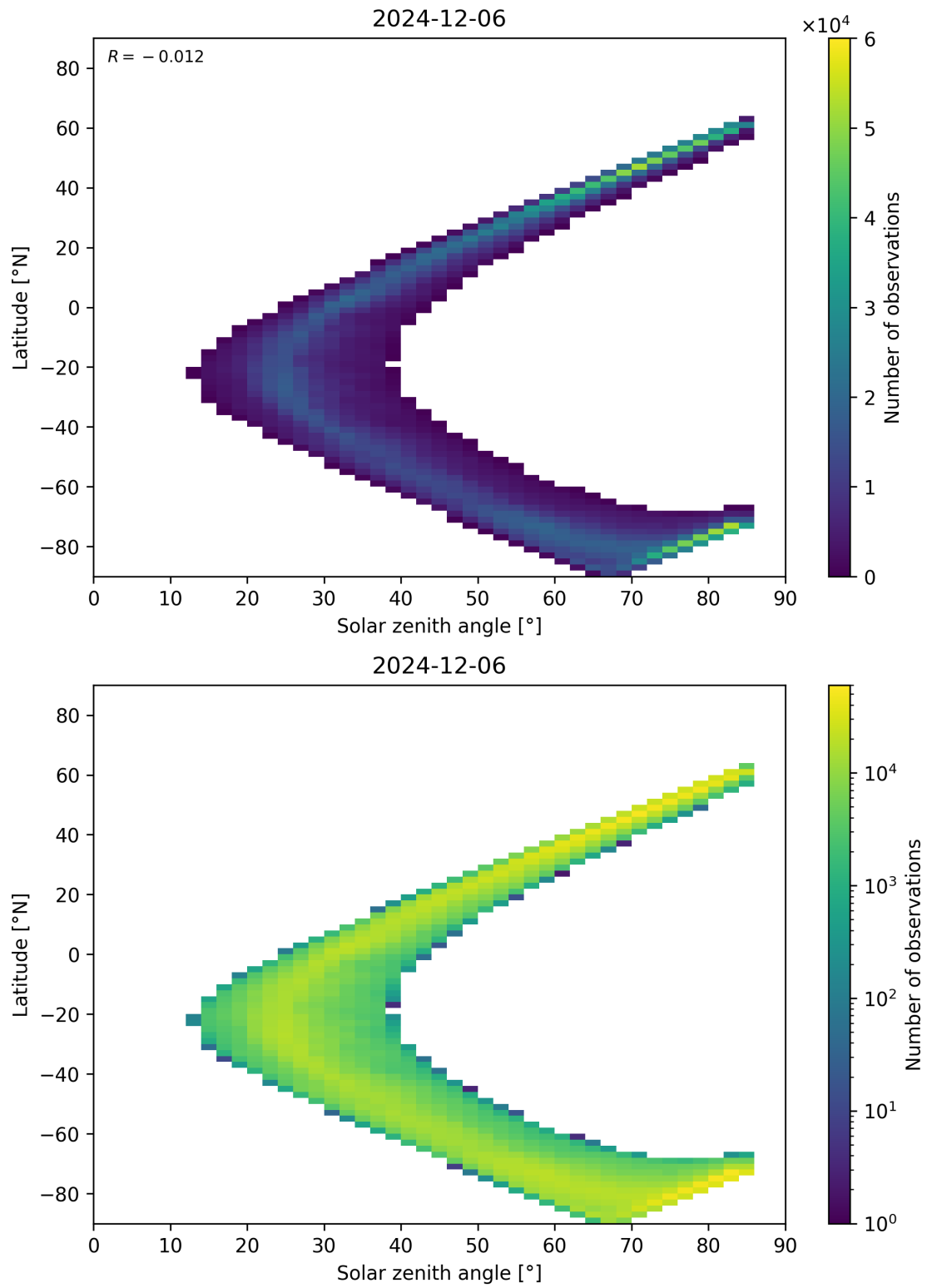
Figure 66: Scatter density plot of “Solar zenith angle” against “Latitude” for 2024-12-06 to 2024-12-07.
