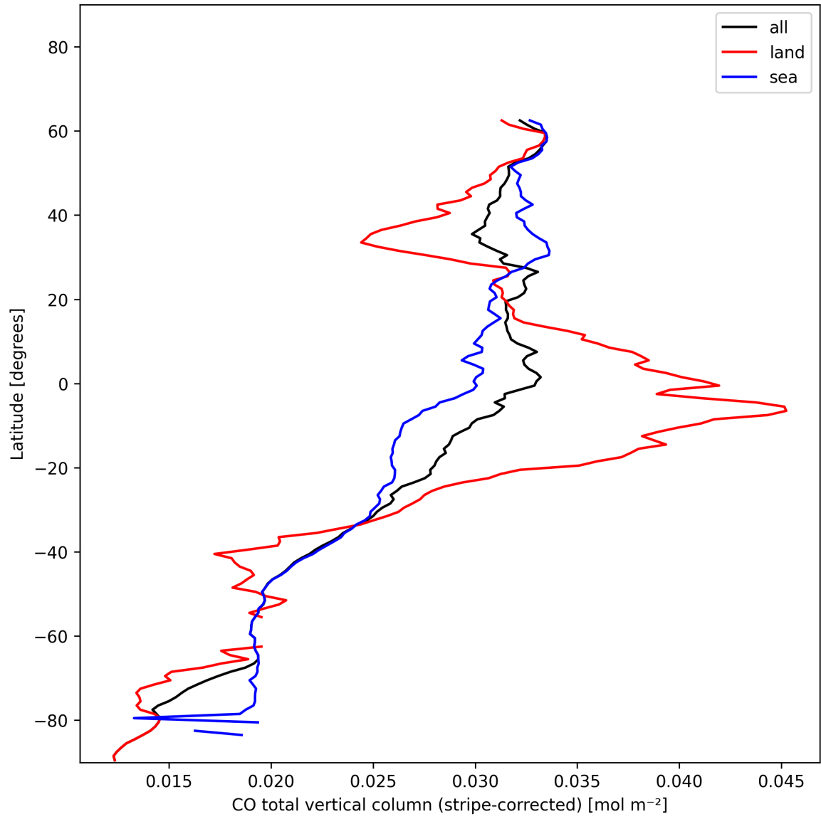
Figure 11: Zonal average of “CO total vertical column (stripe-corrected)” for 2024-12-06 to 2024-12-07.
