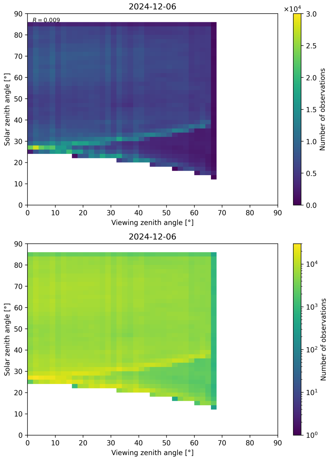
Figure 77: Scatter density plot of “Viewing zenith angle” against “Solar zenith angle” for 2024-12-06 to 2024-12-07.
