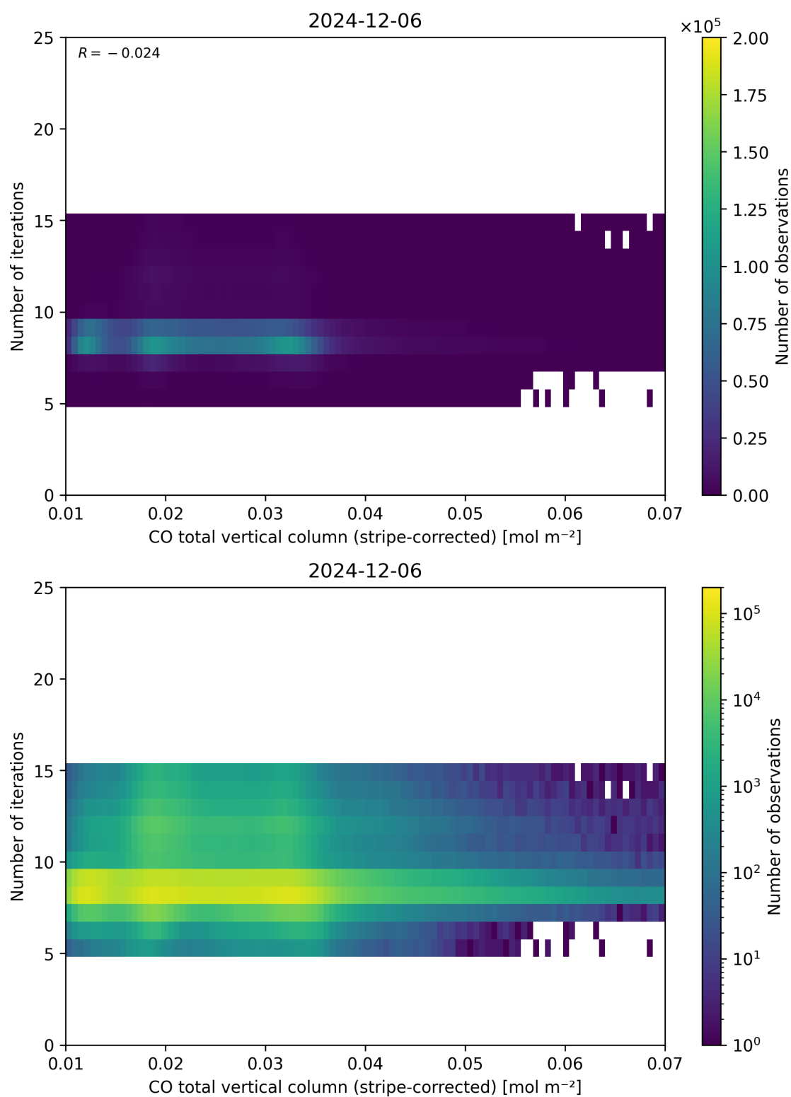
Figure 39: Scatter density plot of “CO total vertical column (stripe-corrected)” against “Number of iterations” for 2024-12-06 to 2024-12-07.
