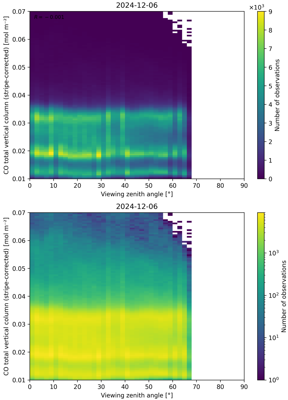
Figure 70: Scatter density plot of “Viewing zenith angle” against “CO total vertical column (stripe-corrected)” for 2024-12-06 to 2024-12-07.
