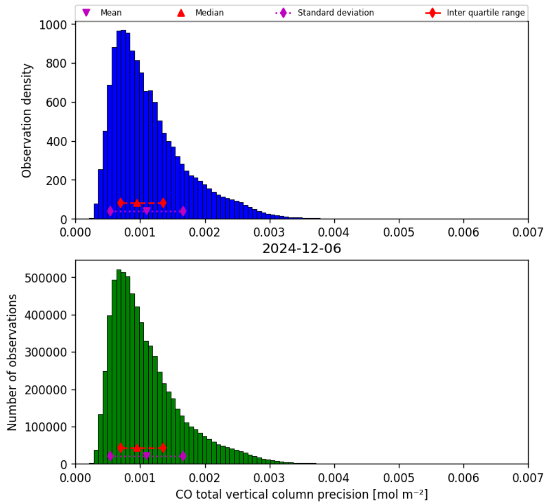
Figure 20: Histogram of “CO total vertical column precision” for 2024-12-06 to 2024-12-07
