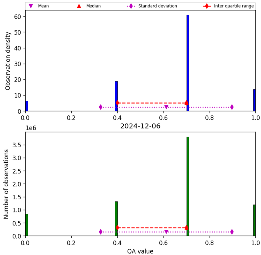
Figure 17: Histogram of “QA value” for 2024-12-06 to 2024-12-07
