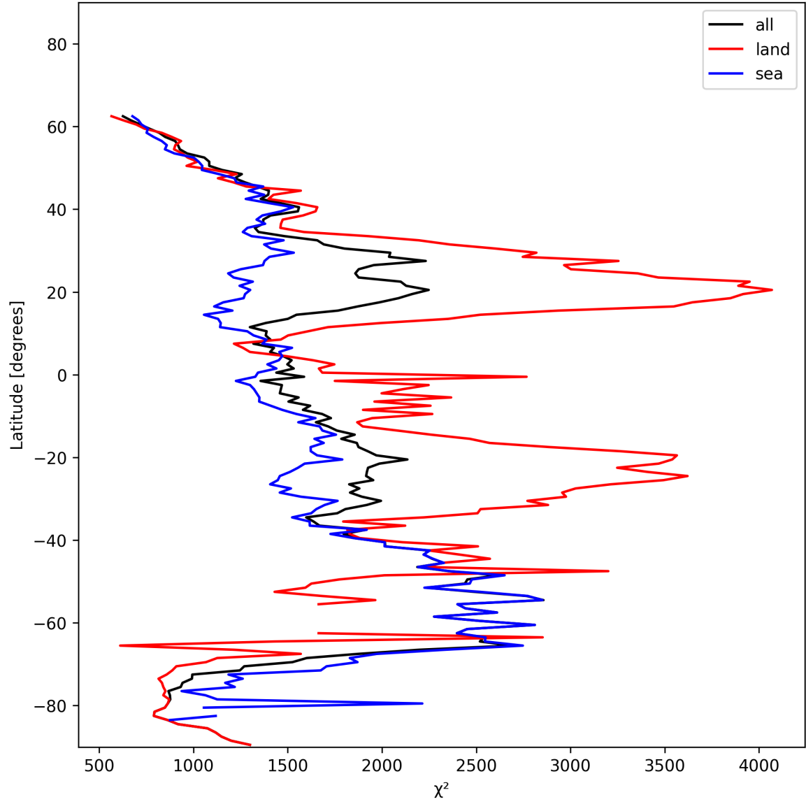
Figure 14: Zonal average of “ \chi^2 ” for 2024-12-06 to 2024-12-07.
