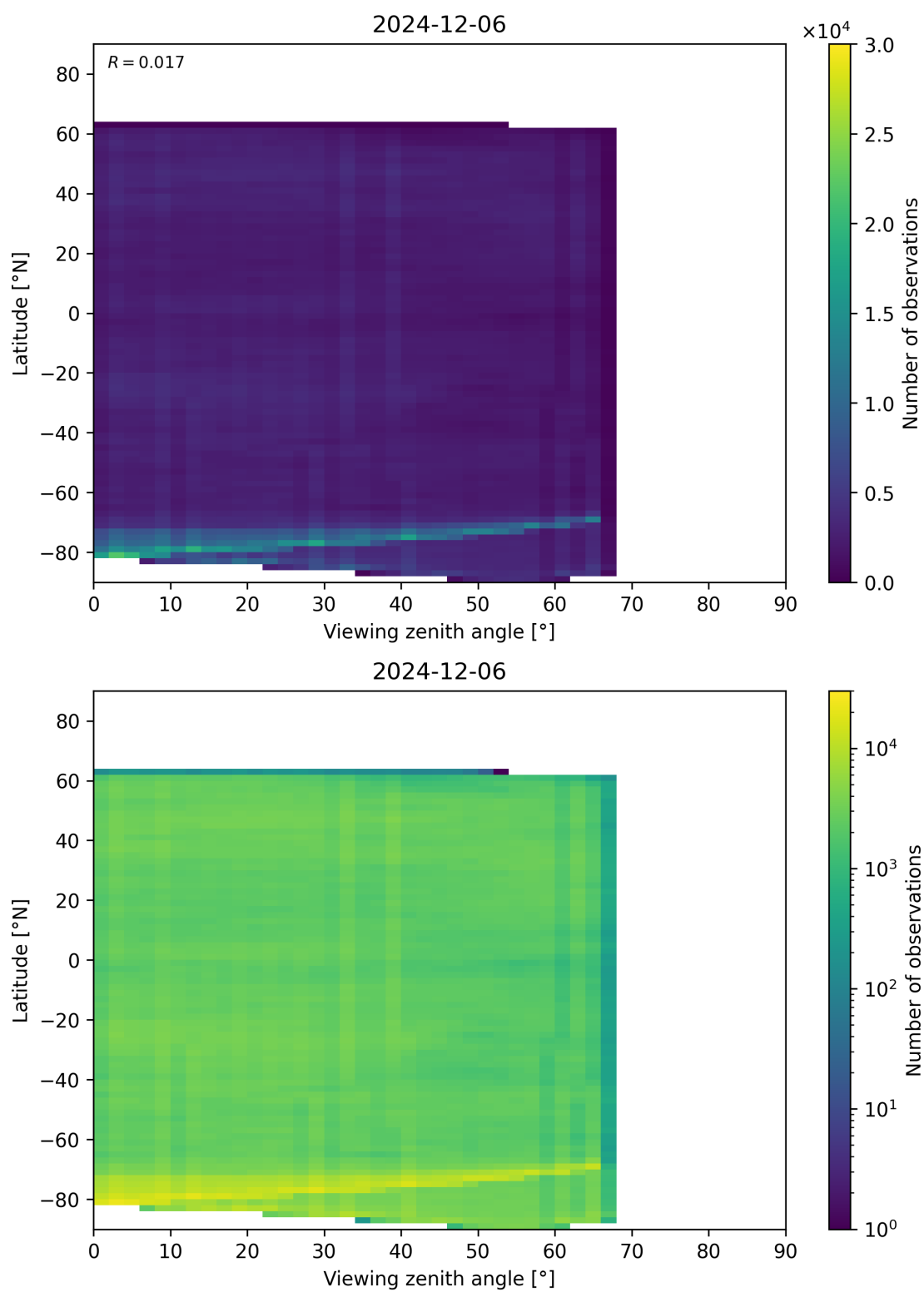
Figure 74: Scatter density plot of “Viewing zenith angle” against “Latitude” for 2024-12-06 to 2024-12-07.
