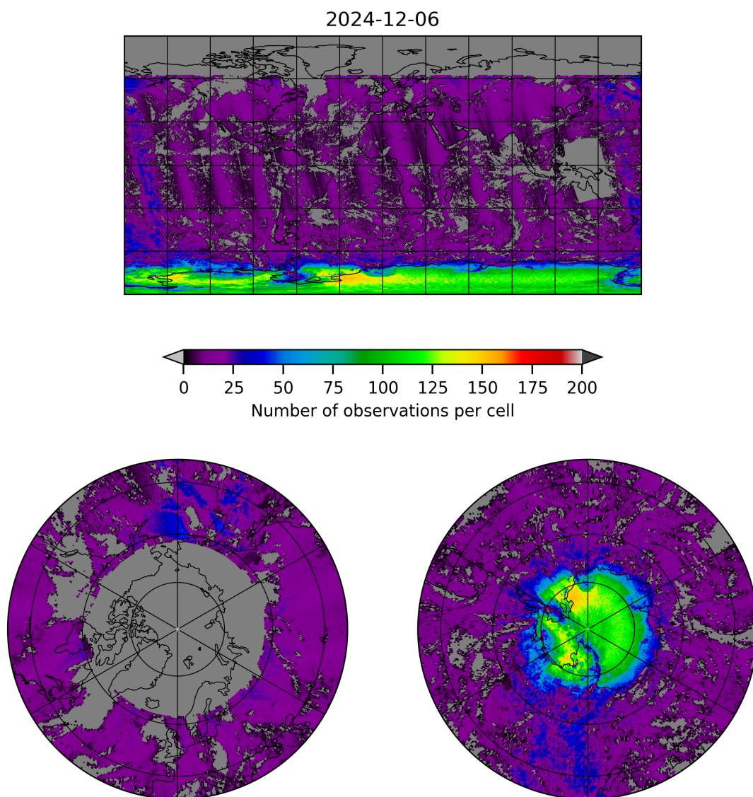
Figure 8: Map of the number of observations for 2024-12-06 to 2024-12-07
