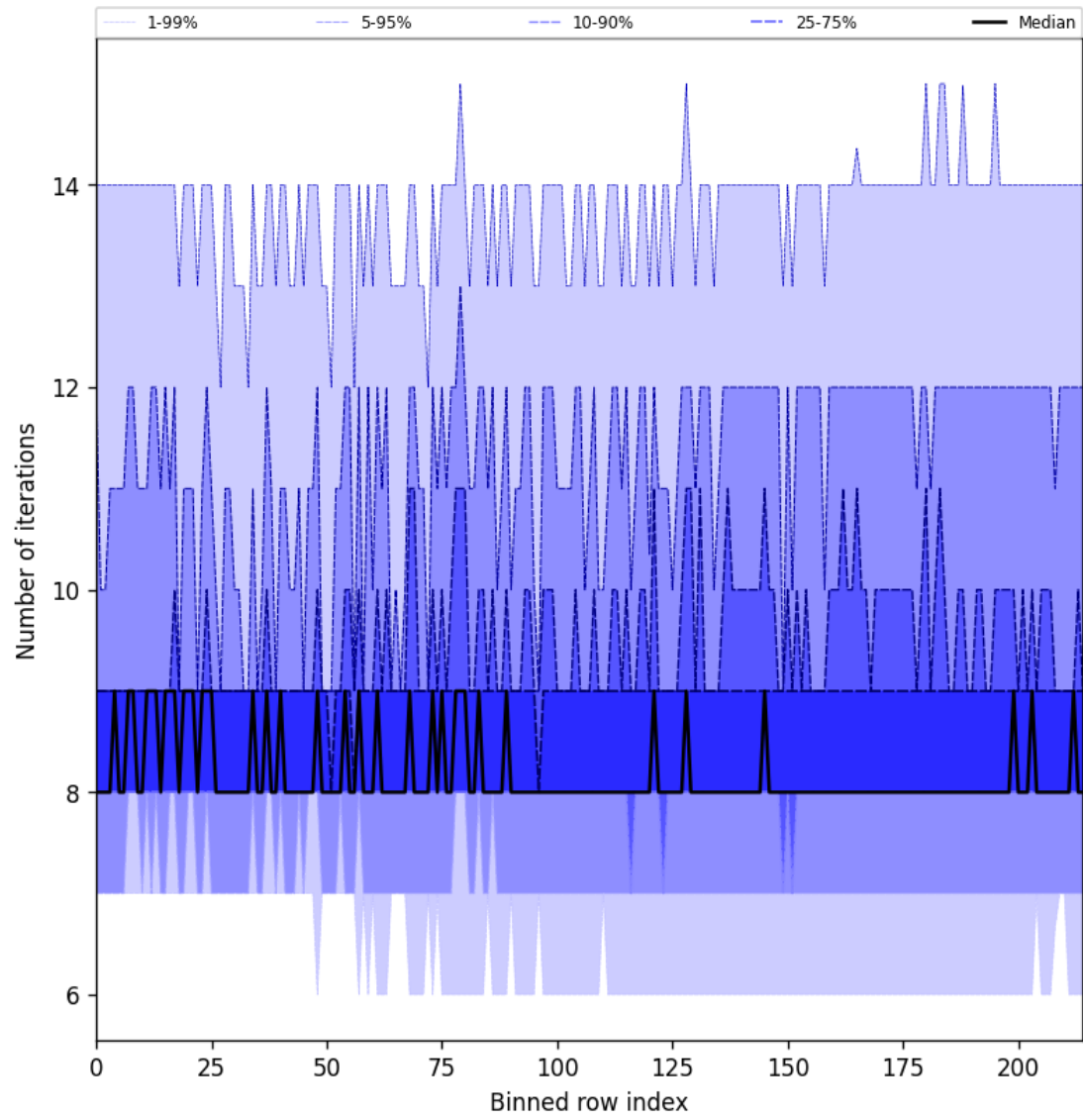
Figure 32: Along track statistics of “Number of iterations” for 2024-12-06 to 2024-12-07
