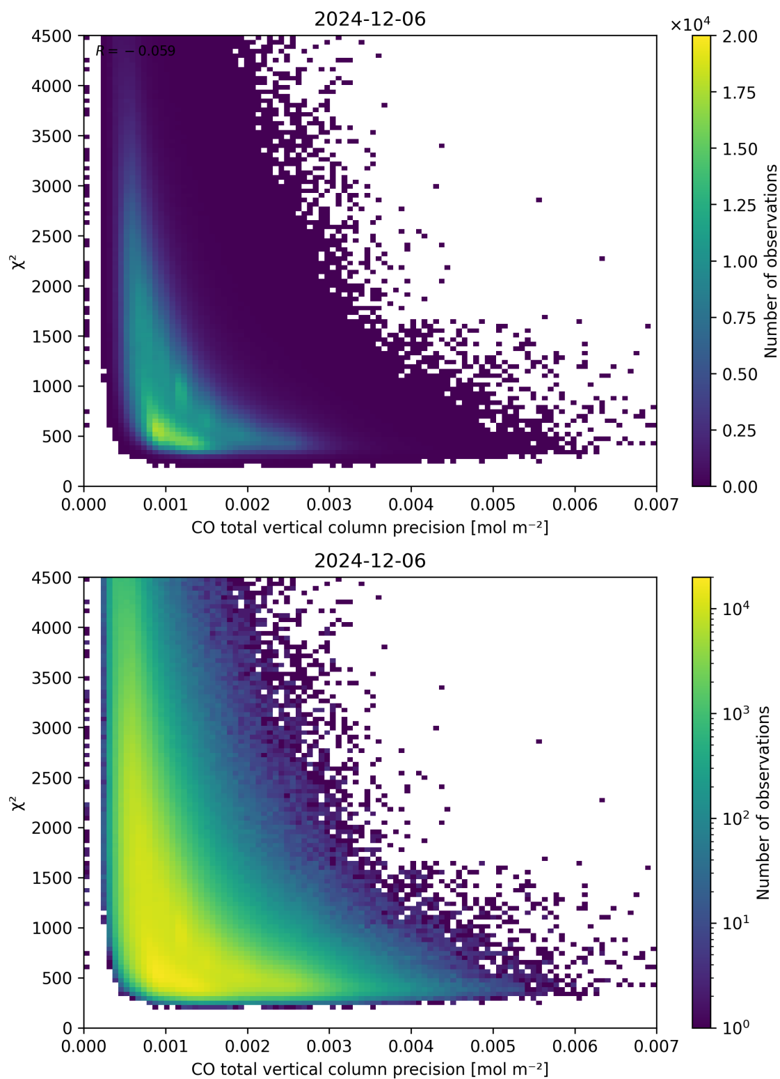
Figure 44: Scatter density plot of “CO total vertical column precision” against “ \chi^2 ” for 2024-12-06 to 2024-12-07.
