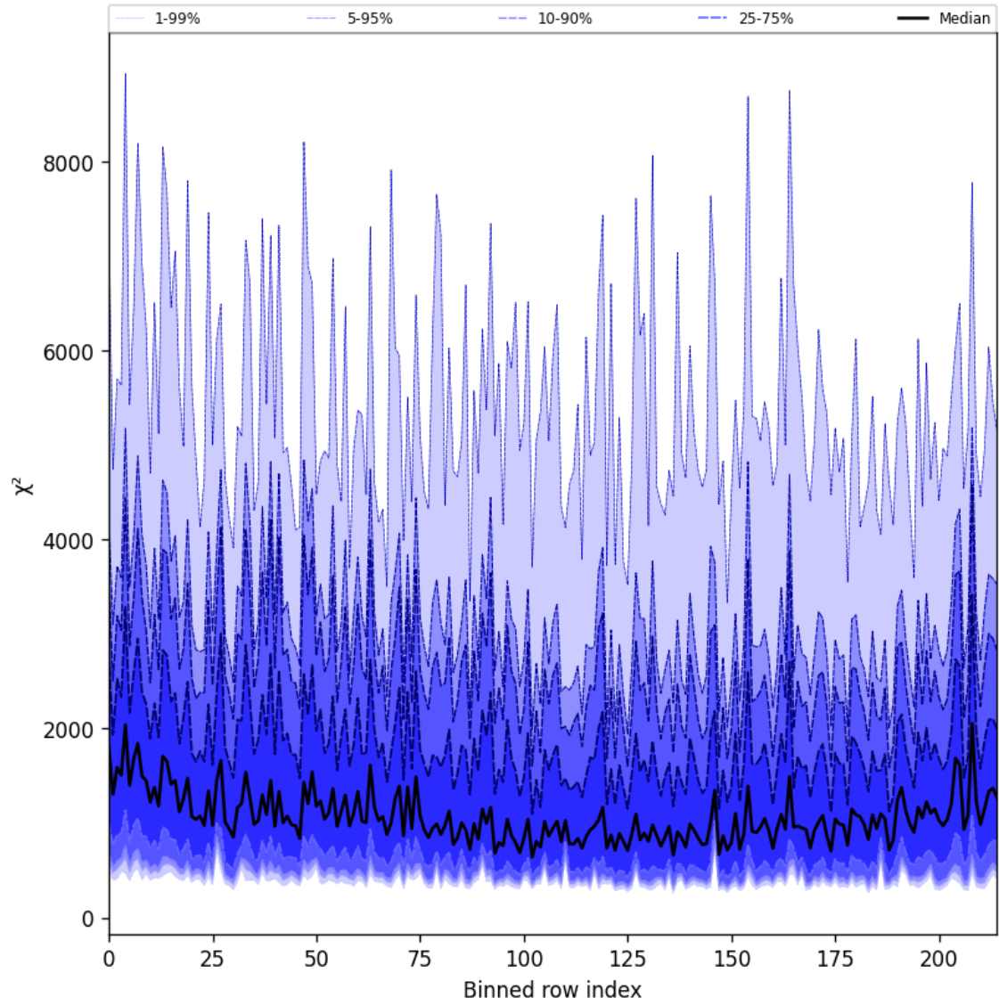
Figure 30: Along track statistics of “ \chi^2 ” for 2024-12-06 to 2024-12-07
