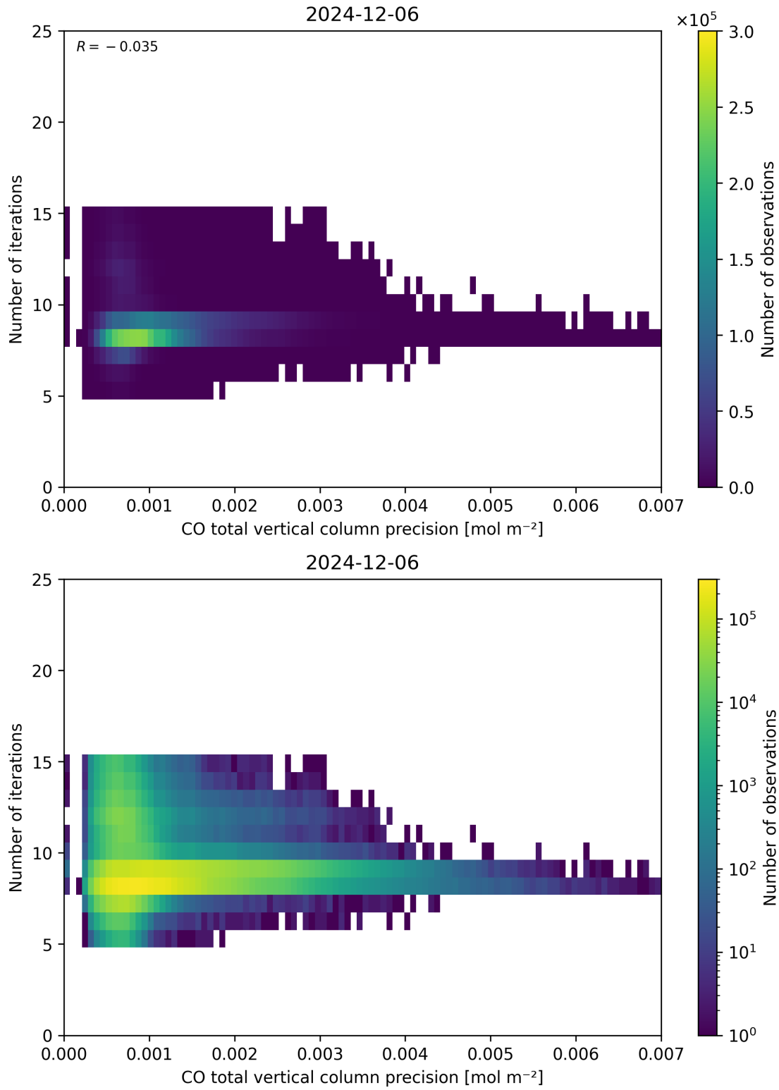
Figure 46: Scatter density plot of “CO total vertical column precision” against “Number of iterations” for 2024-12-06 to 2024-12-07.
