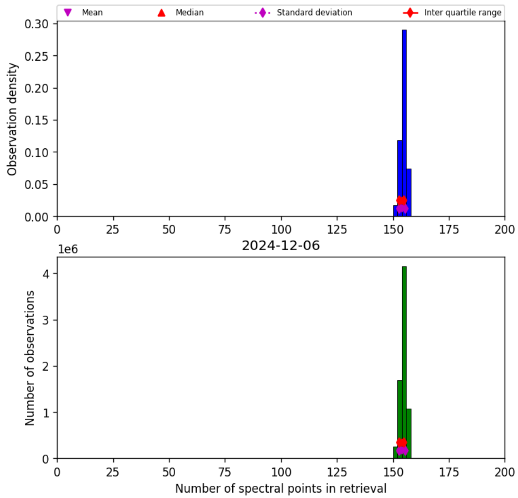
Figure 21: Histogram of “Number of spectral points in retrieval” for 2024-12-06 to 2024-12-07
