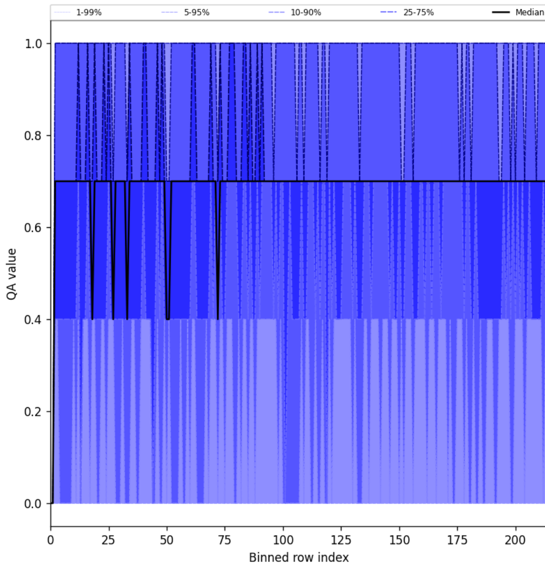
Figure 25: Along track statistics of “QA value” for 2024-12-06 to 2024-12-07
