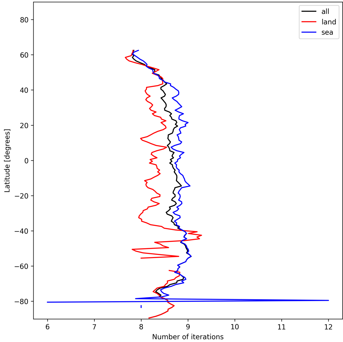
Figure 16: Zonal average of “Number of iterations” for 2024-12-06 to 2024-12-07.
