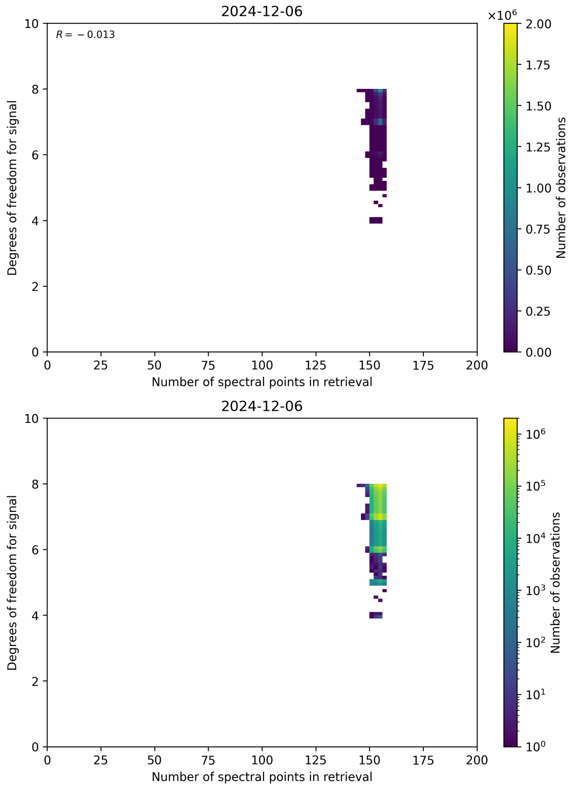
Figure 59: Scatter density plot of “Number of spectral points in retrieval” against “Degrees of freedom for signal” for 2024-12-06 to 2024-12-07.
