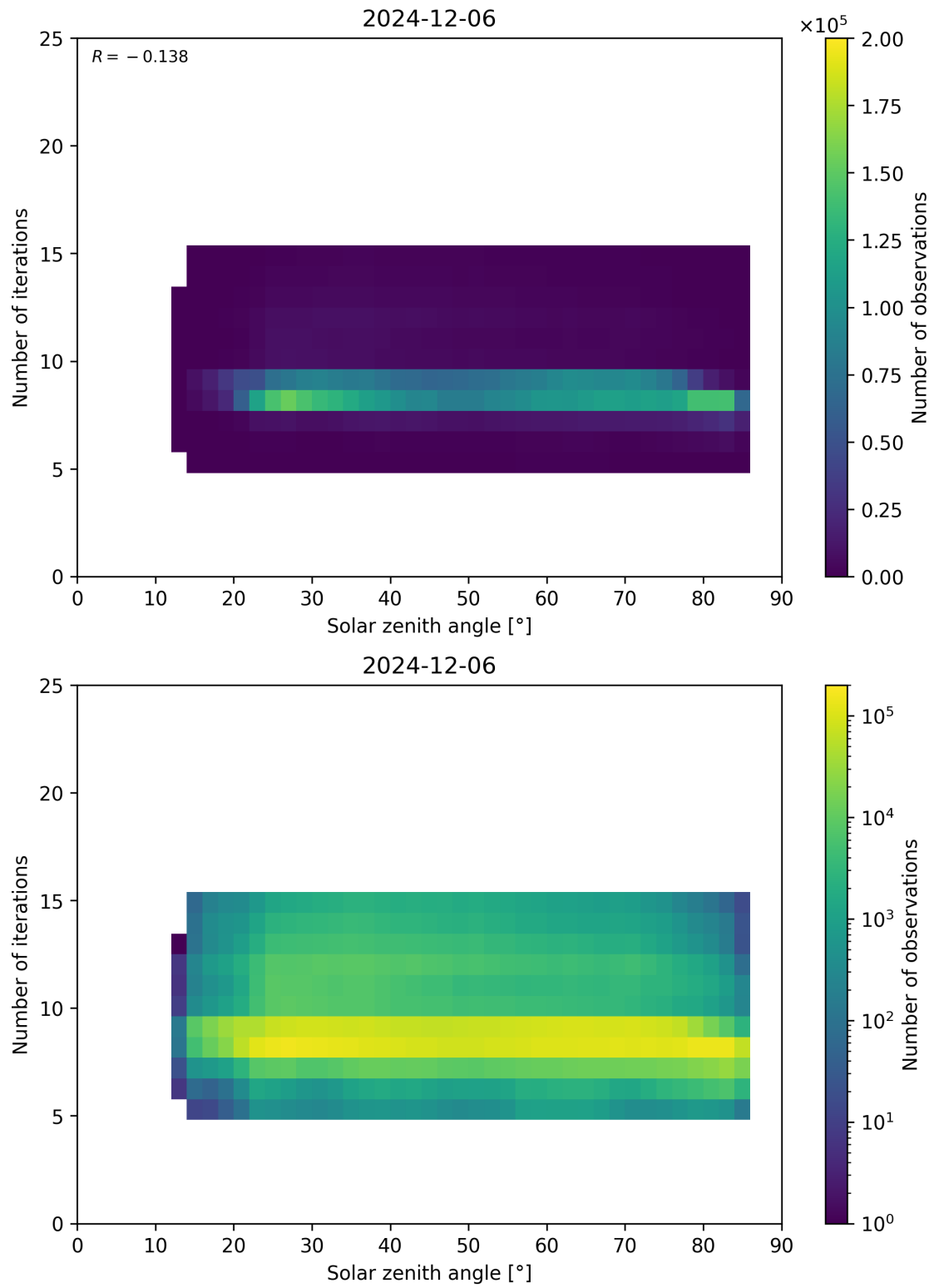
Figure 67: Scatter density plot of “Solar zenith angle” against “Number of iterations” for 2024-12-06 to 2024-12-07.
