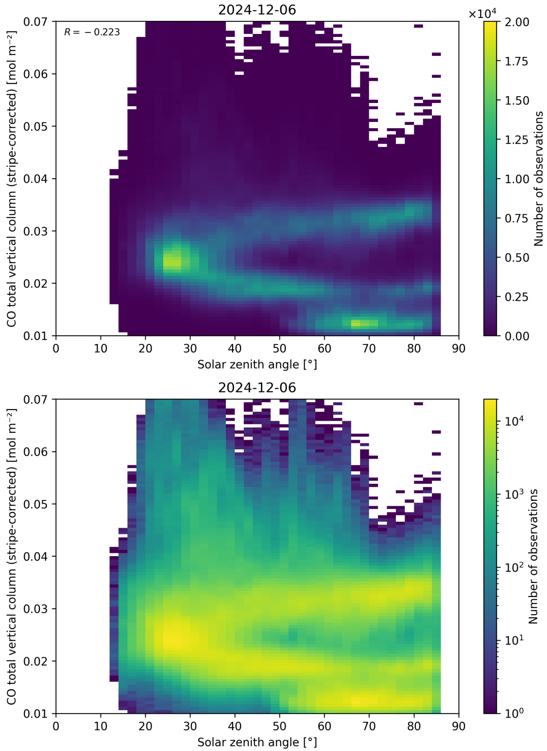
Figure 62: Scatter density plot of “Solar zenith angle” against “CO total vertical column (stripe-corrected)” for 2024-12-06 to 2024-12-07.
