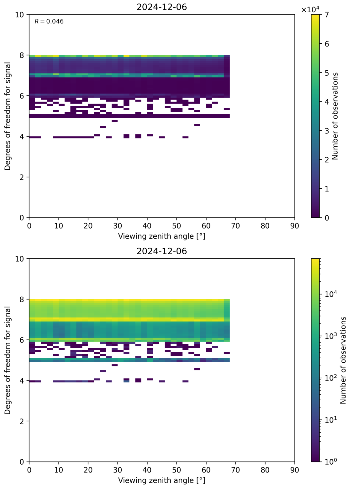
Figure 73: Scatter density plot of “Viewing zenith angle” against “Degrees of freedom for signal” for 2024-12-06 to 2024-12-07.
