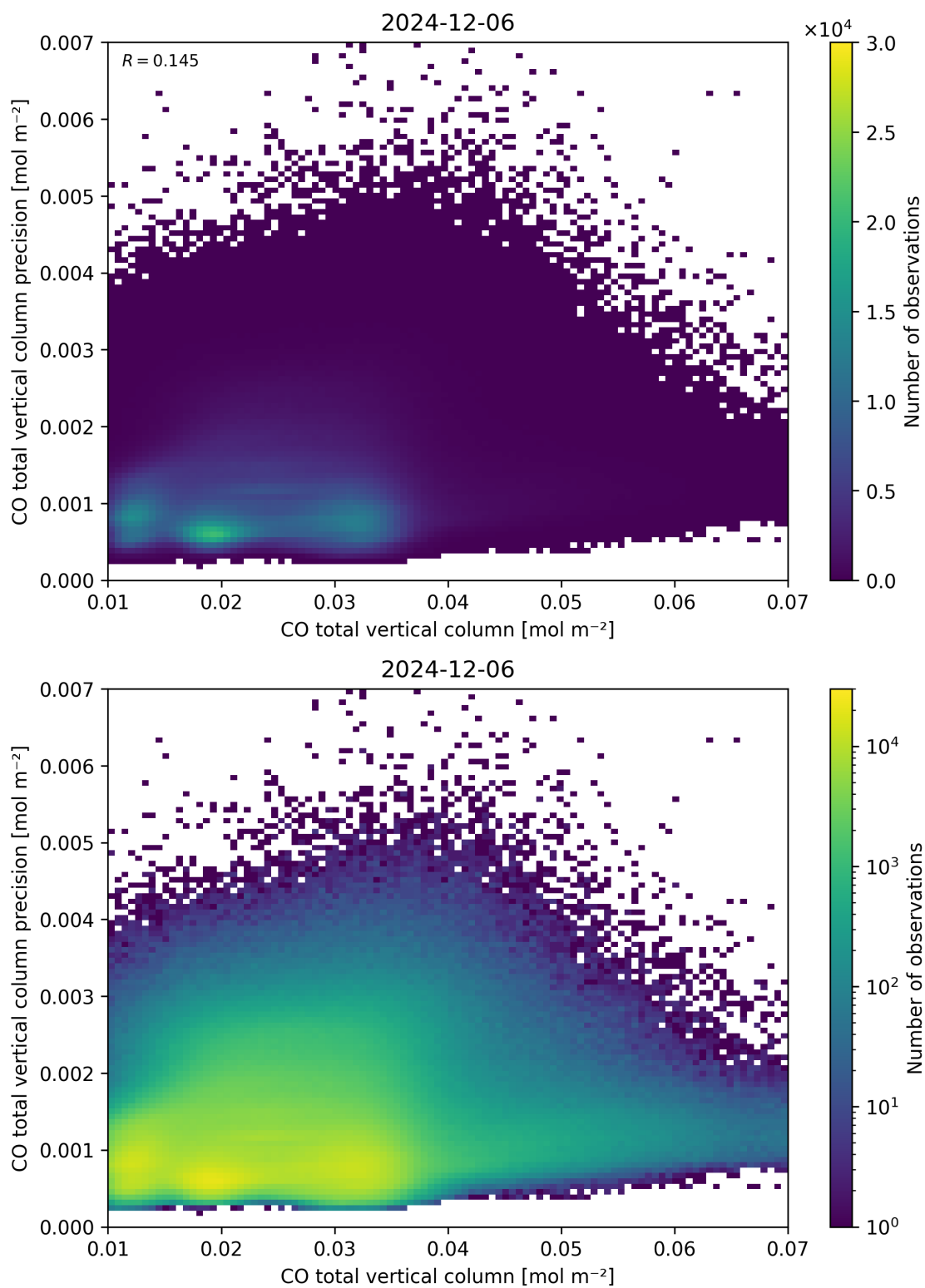
Figure 34: Scatter density plot of “CO total vertical column” against “CO total vertical column precision” for 2024-12-06 to 2024-12-07.
