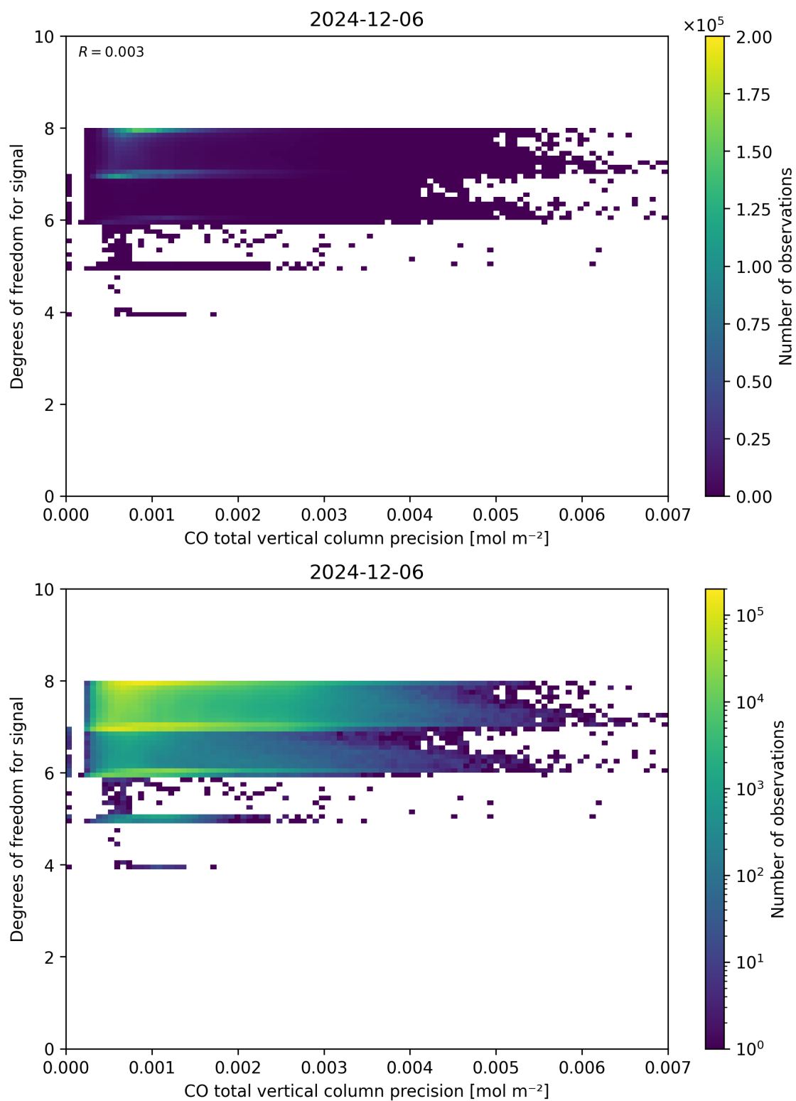
Figure 45: Scatter density plot of “CO total vertical column precision” against “Degrees of freedom for signal” for 2024-12-06 to 2024-12-07.
