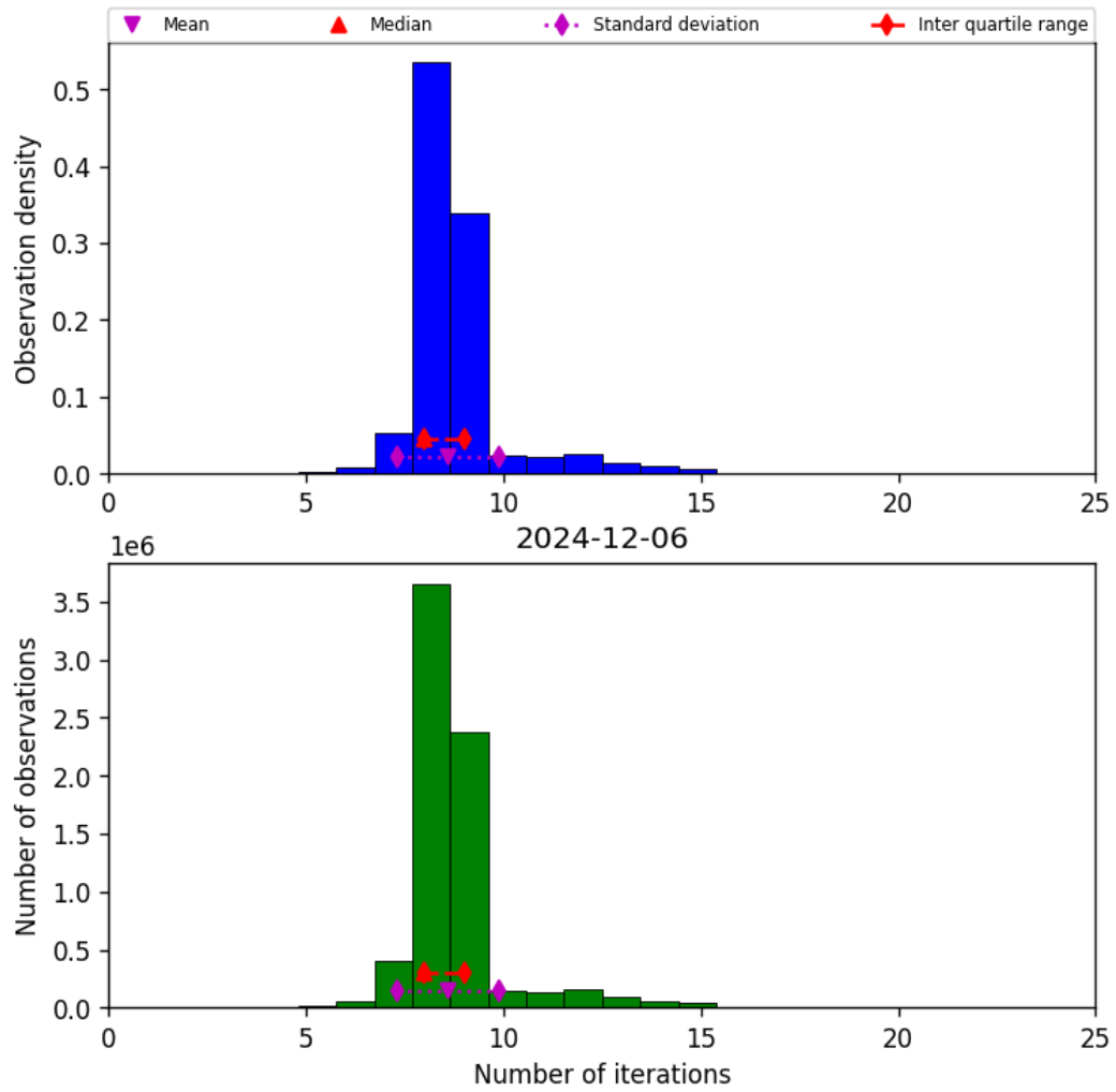
Figure 24: Histogram of “Number of iterations” for 2024-12-06 to 2024-12-07
