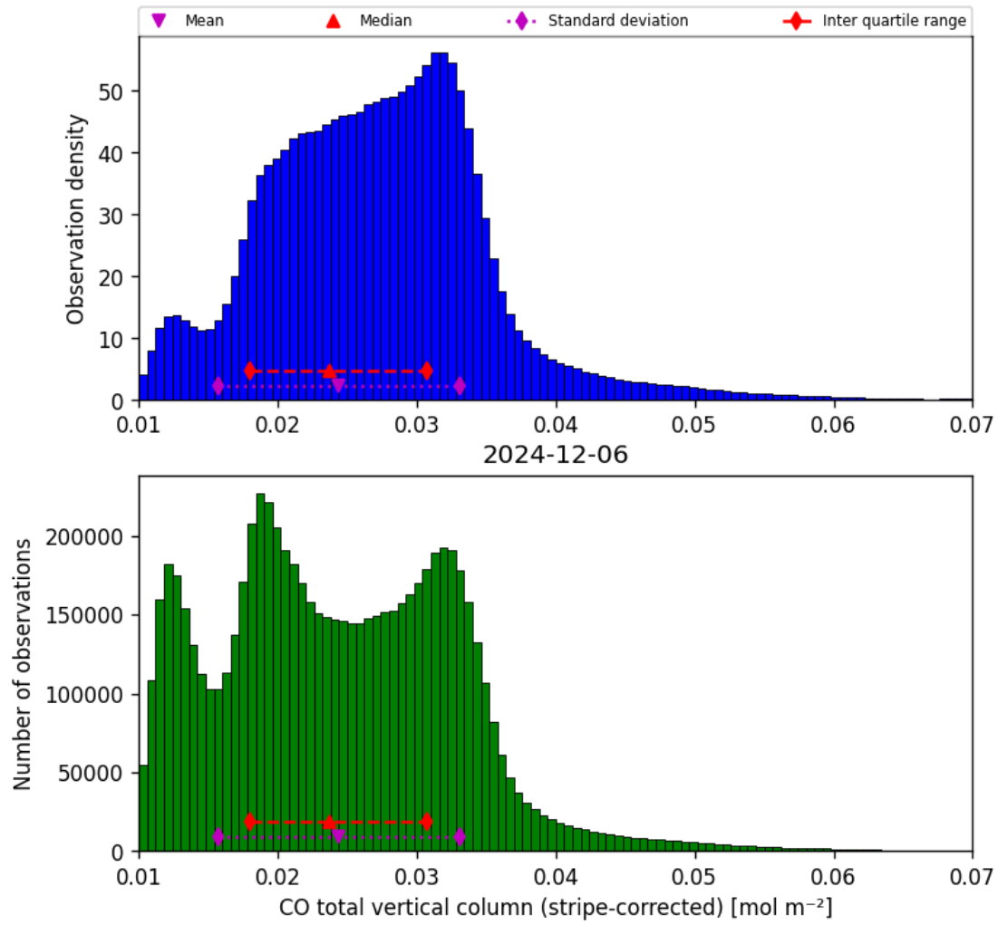
Figure 19: Histogram of “CO total vertical column (stripe-corrected)” for 2024-12-06 to 2024-12-07
