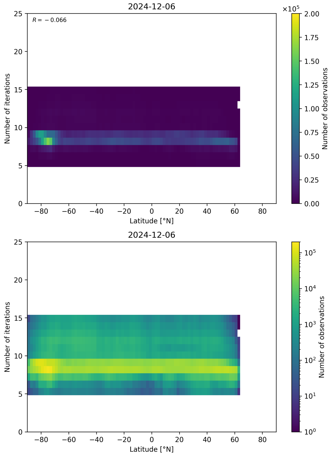
Figure 56: Scatter density plot of “Latitude” against “Number of iterations” for 2024-12-06 to 2024-12-07.
