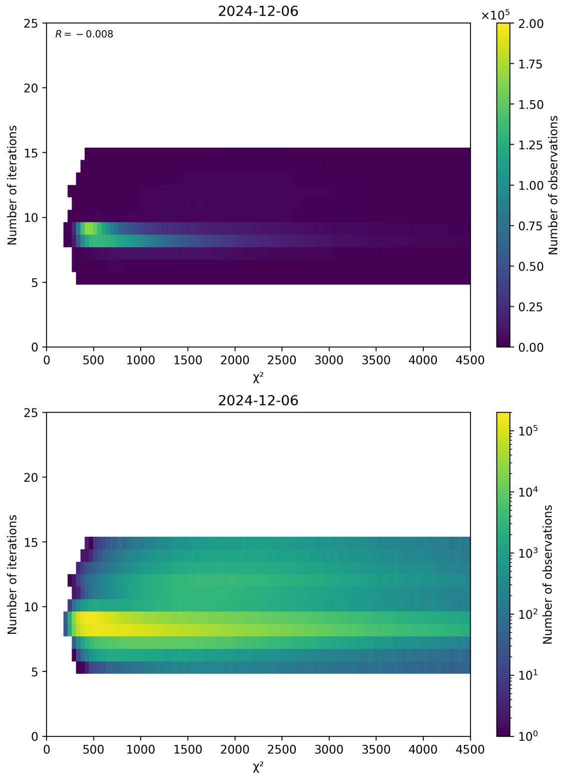
Figure 49: Scatter density plot of “ \chi^2 ” against “Number of iterations” for 2024-12-06 to 2024-12-07.
