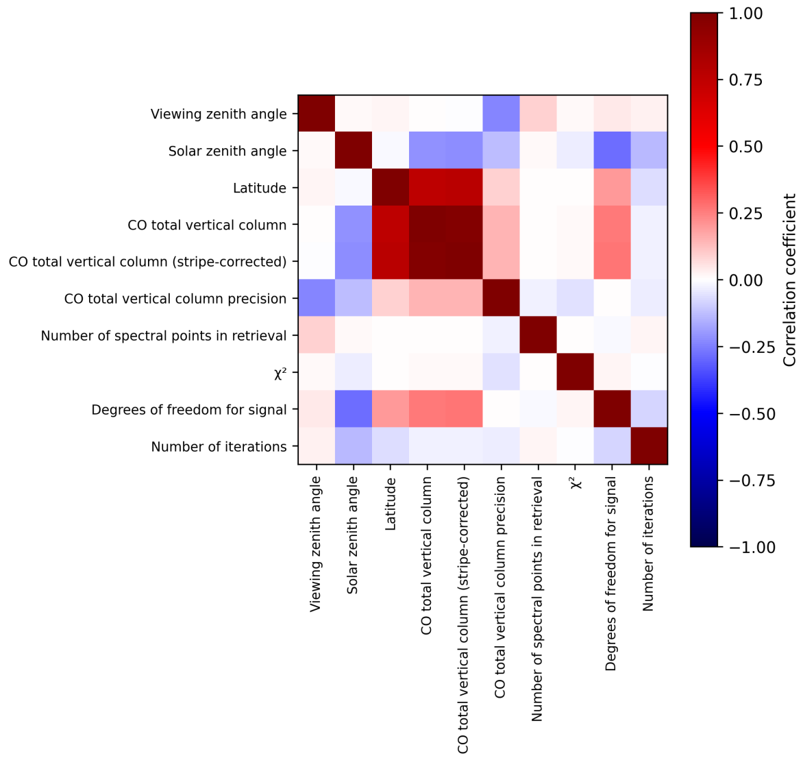
Figure 2: Map of correlation matrix for 2024-12-06 to 2024-12-07.
