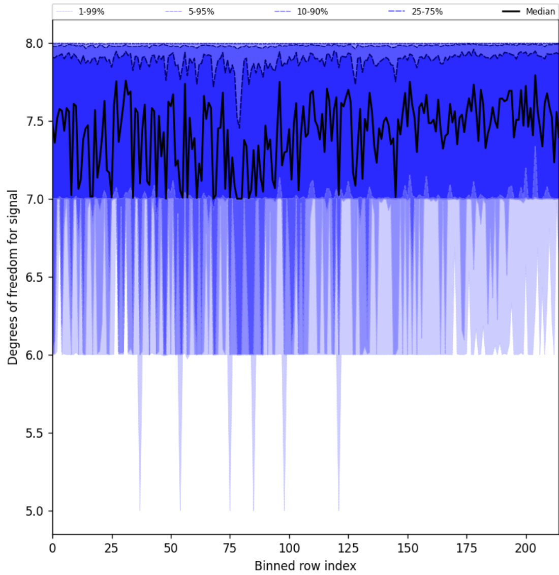
Figure 31: Along track statistics of “Degrees of freedom for signal” for 2024-12-06 to 2024-12-07
