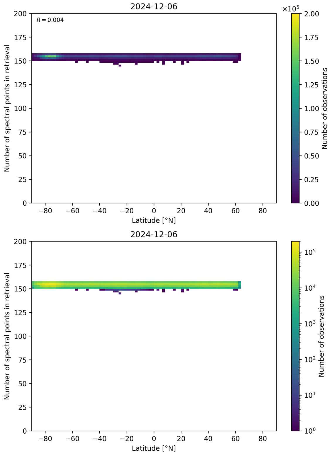
Figure 57: Scatter density plot of “Latitude” against “Number of spectral points in retrieval” for 2024-12-06 to 2024-12-07.
