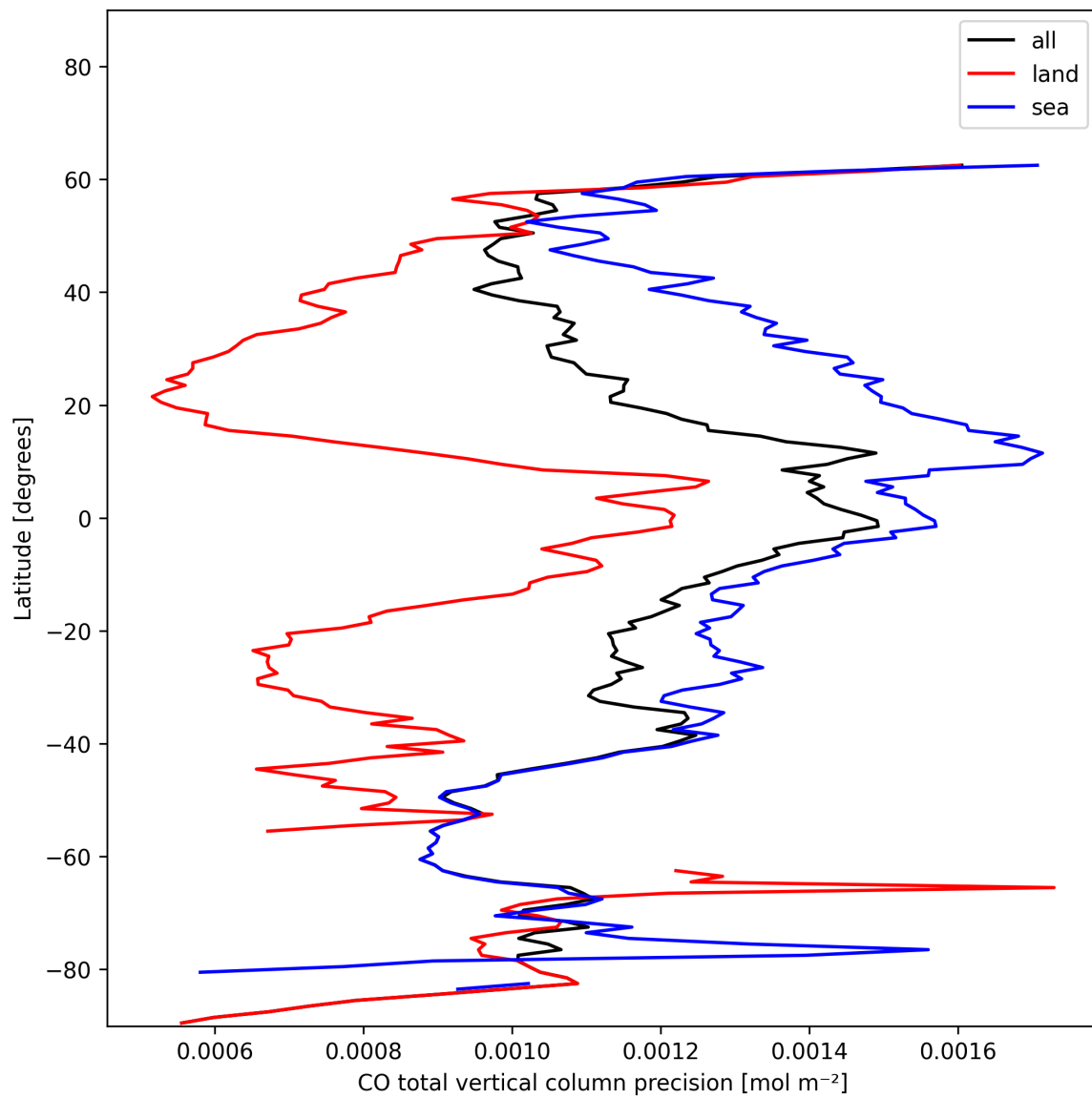
Figure 12: Zonal average of “CO total vertical column precision” for 2024-12-06 to 2024-12-07.
