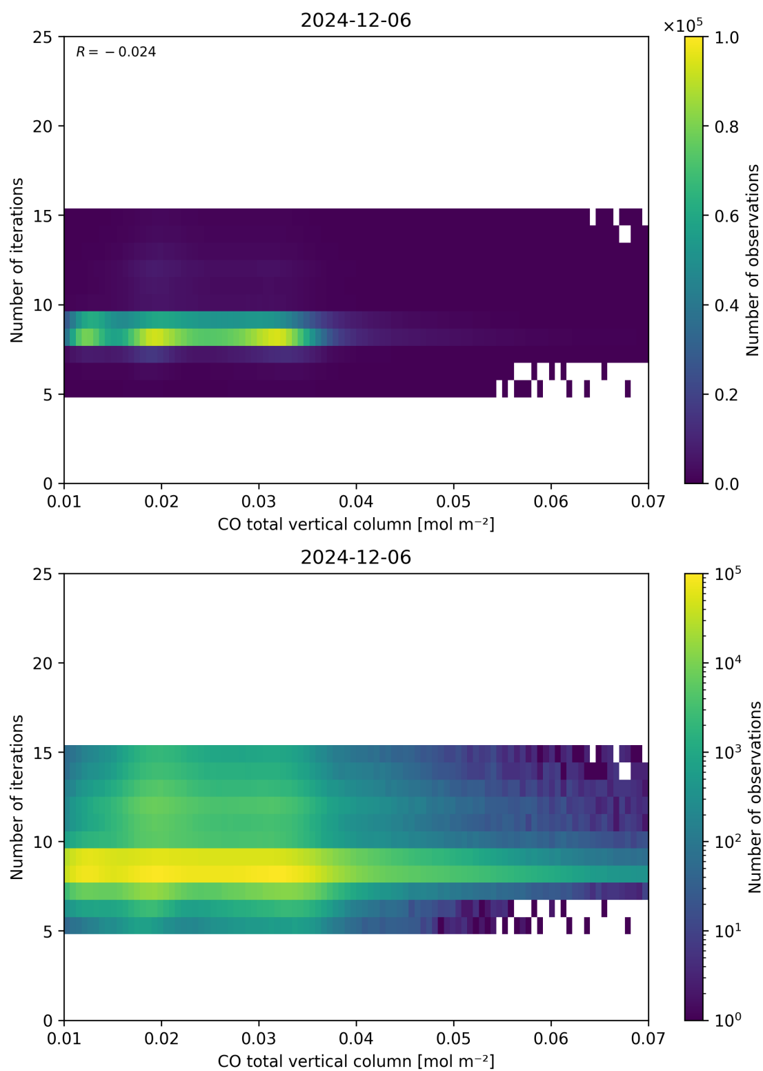
Figure 42: Scatter density plot of “CO total vertical column” against “Number of iterations” for 2024-12-06 to 2024-12-07.
