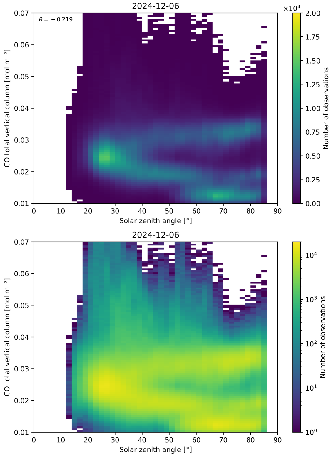
Figure 61: Scatter density plot of “Solar zenith angle” against “CO total vertical column” for 2024-12-06 to 2024-12-07.
