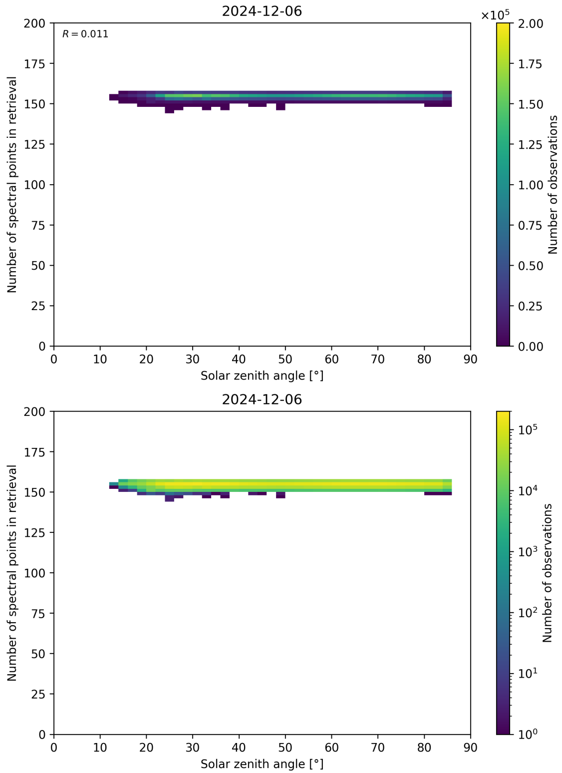
Figure 68: Scatter density plot of “Solar zenith angle” against “Number of spectral points in retrieval” for 2024-12-06 to 2024-12-07.
