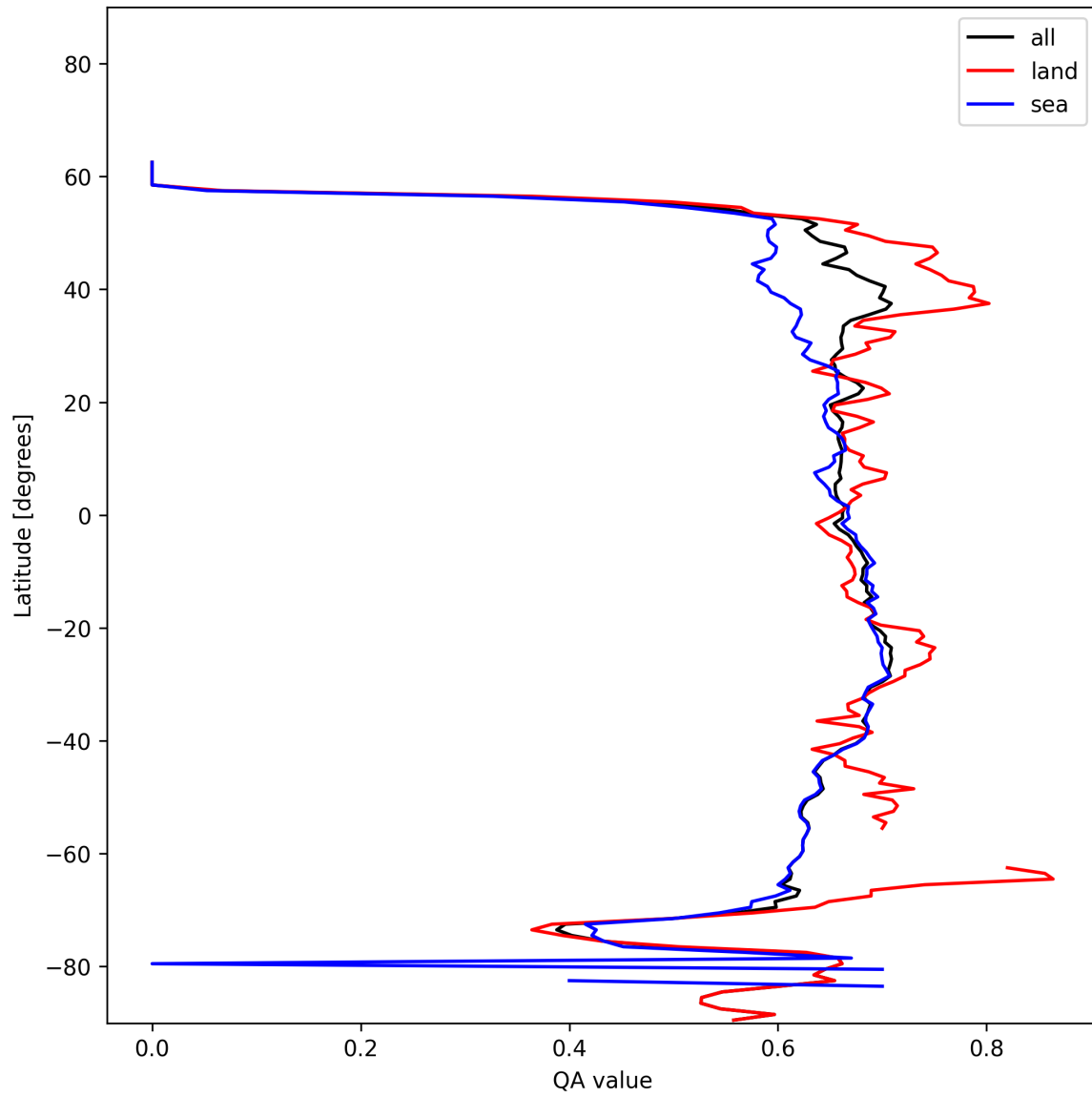
Figure 9: Zonal average of “QA value” for 2024-12-06 to 2024-12-07.
