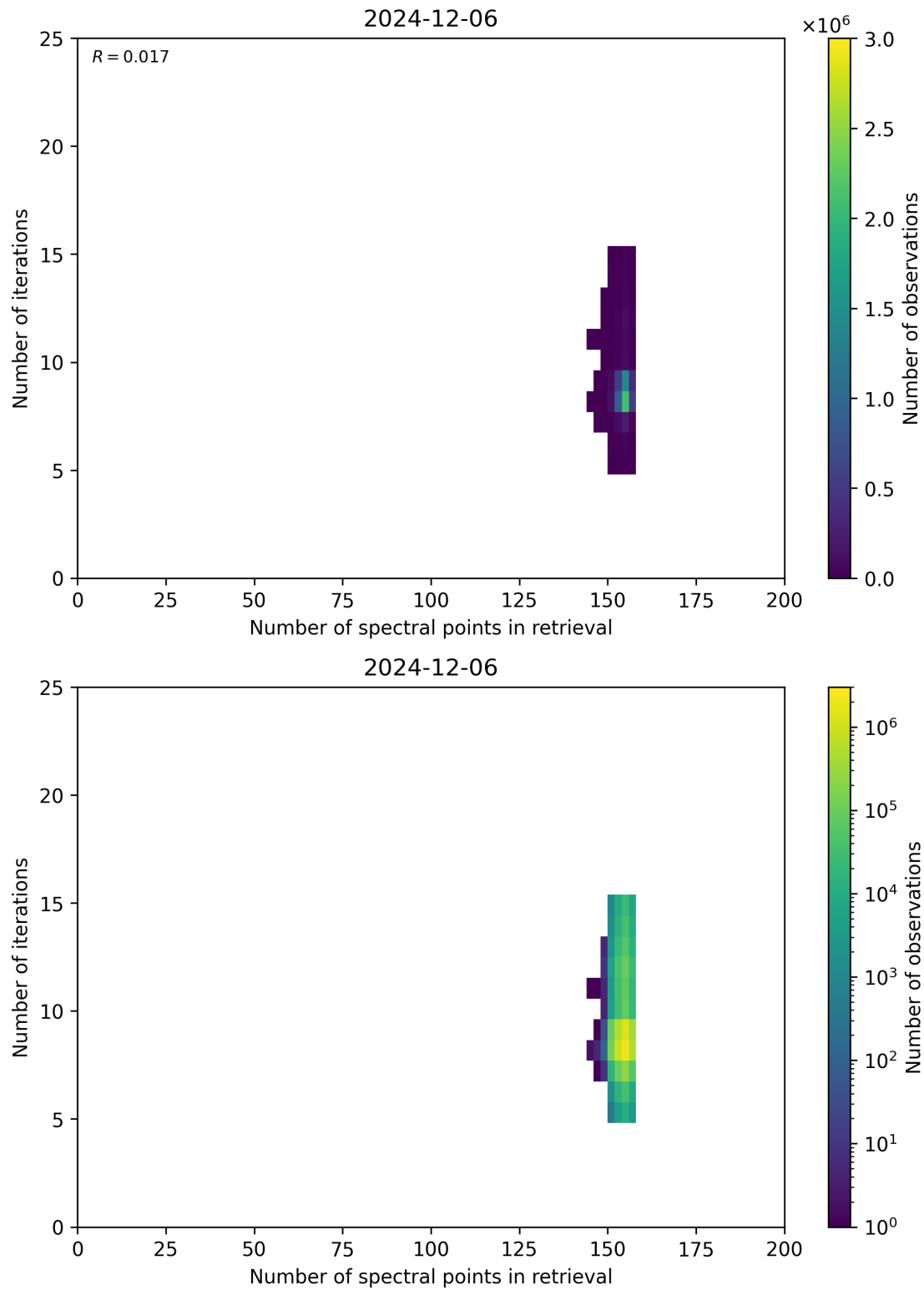
Figure 60: Scatter density plot of “Number of spectral points in retrieval” against “Number of iterations” for 2024-12-06 to 2024-12-07.
