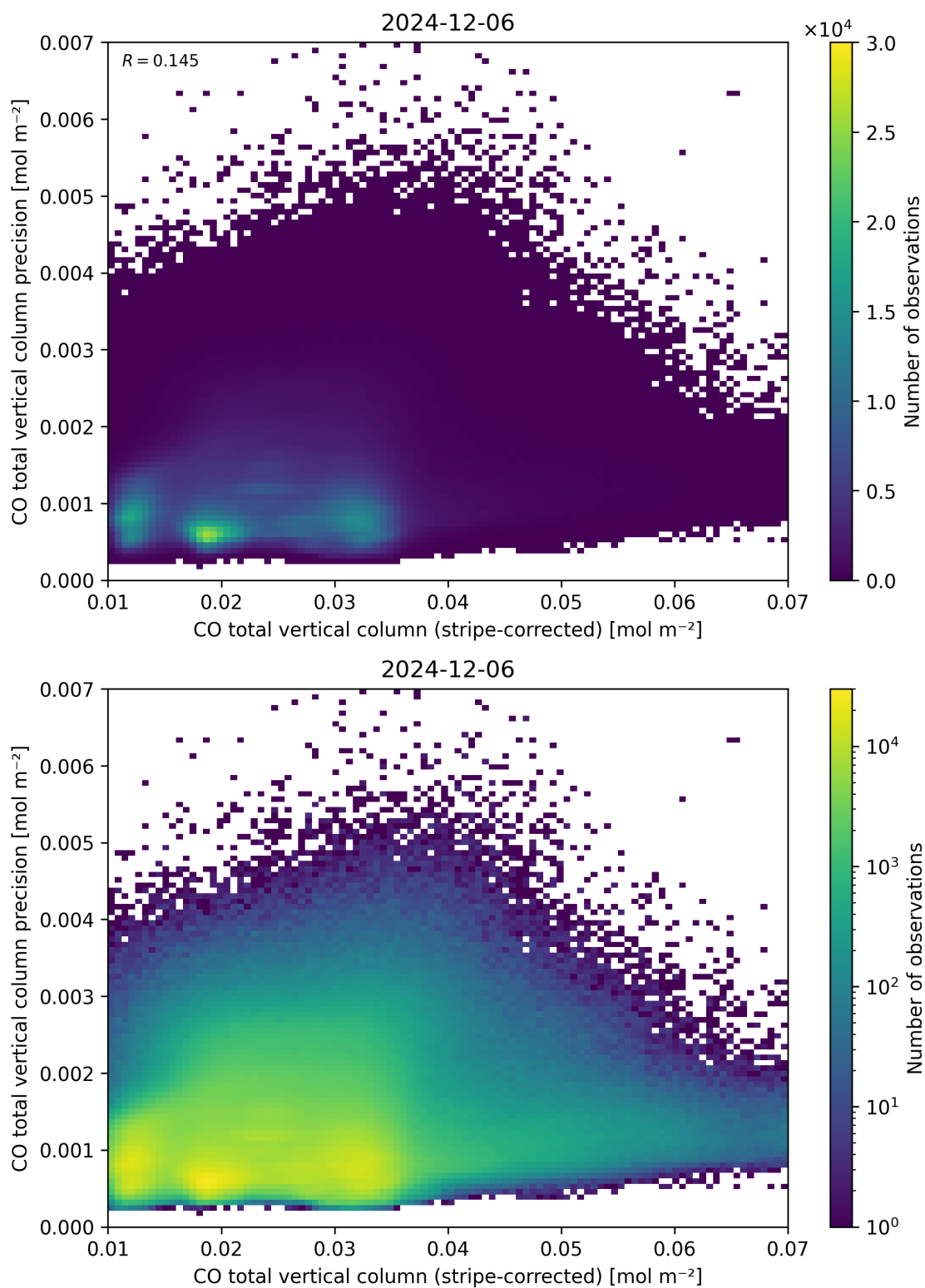
Figure 36: Scatter density plot of “CO total vertical column (stripe-corrected)” against “CO total vertical column precision” for 2024-12-06 to 2024-12-07.
