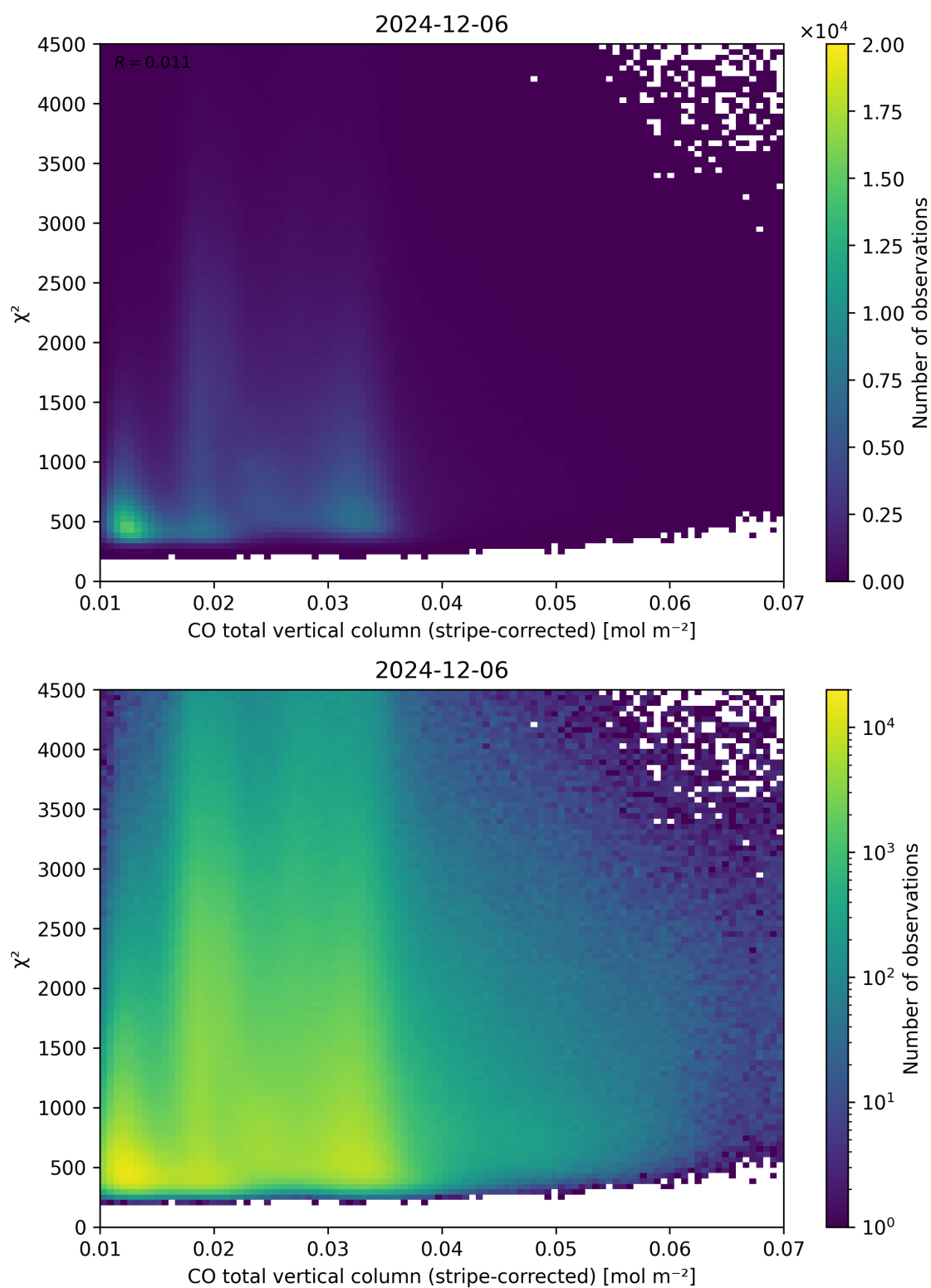
Figure 37: Scatter density plot of “CO total vertical column (stripe-corrected)” against “ \chi^2 ” for 2024-12-06 to 2024-12-07.
