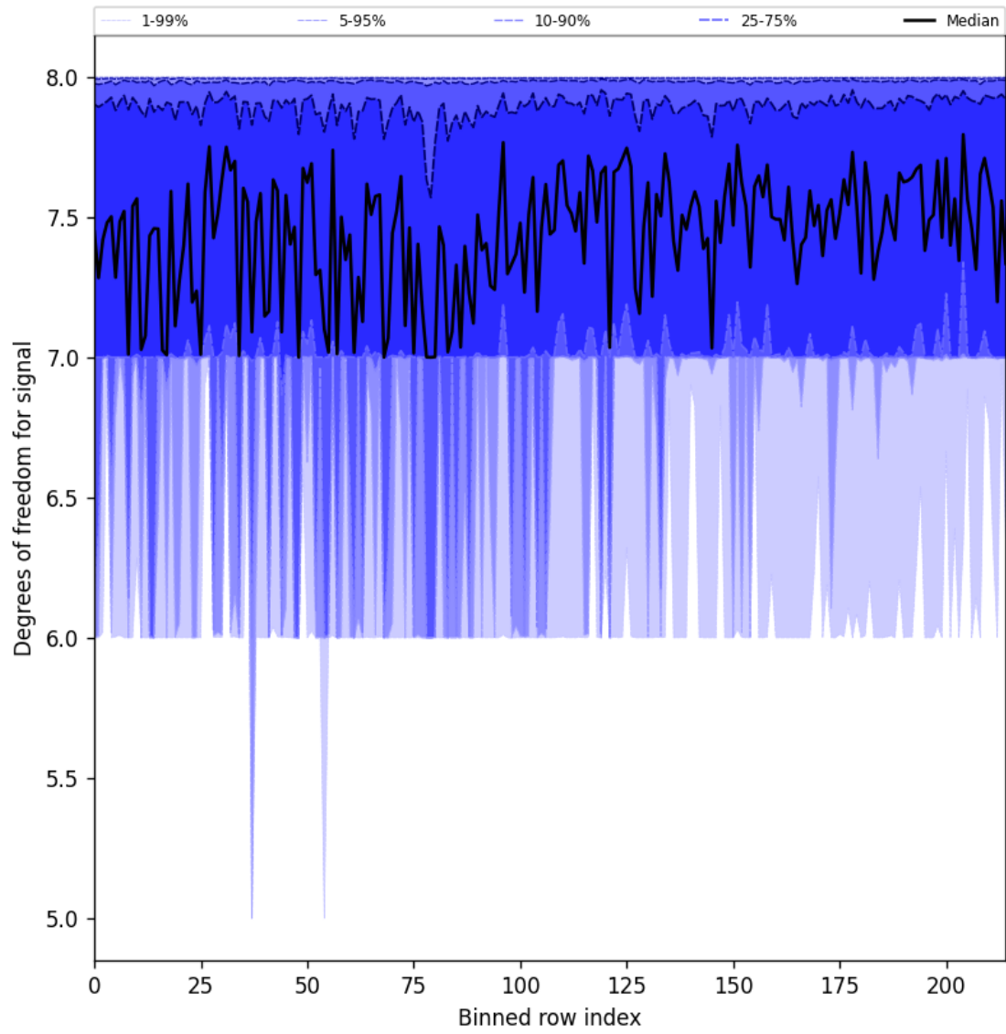
Figure 31: Along track statistics of “Degrees of freedom for signal” for 2024-12-06 to 2024-12-08
