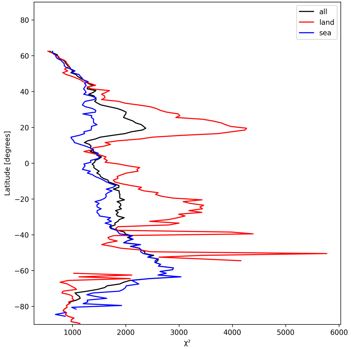
Figure 14: Zonal average of “ \chi^2 ” for 2024-12-06 to 2024-12-08.
