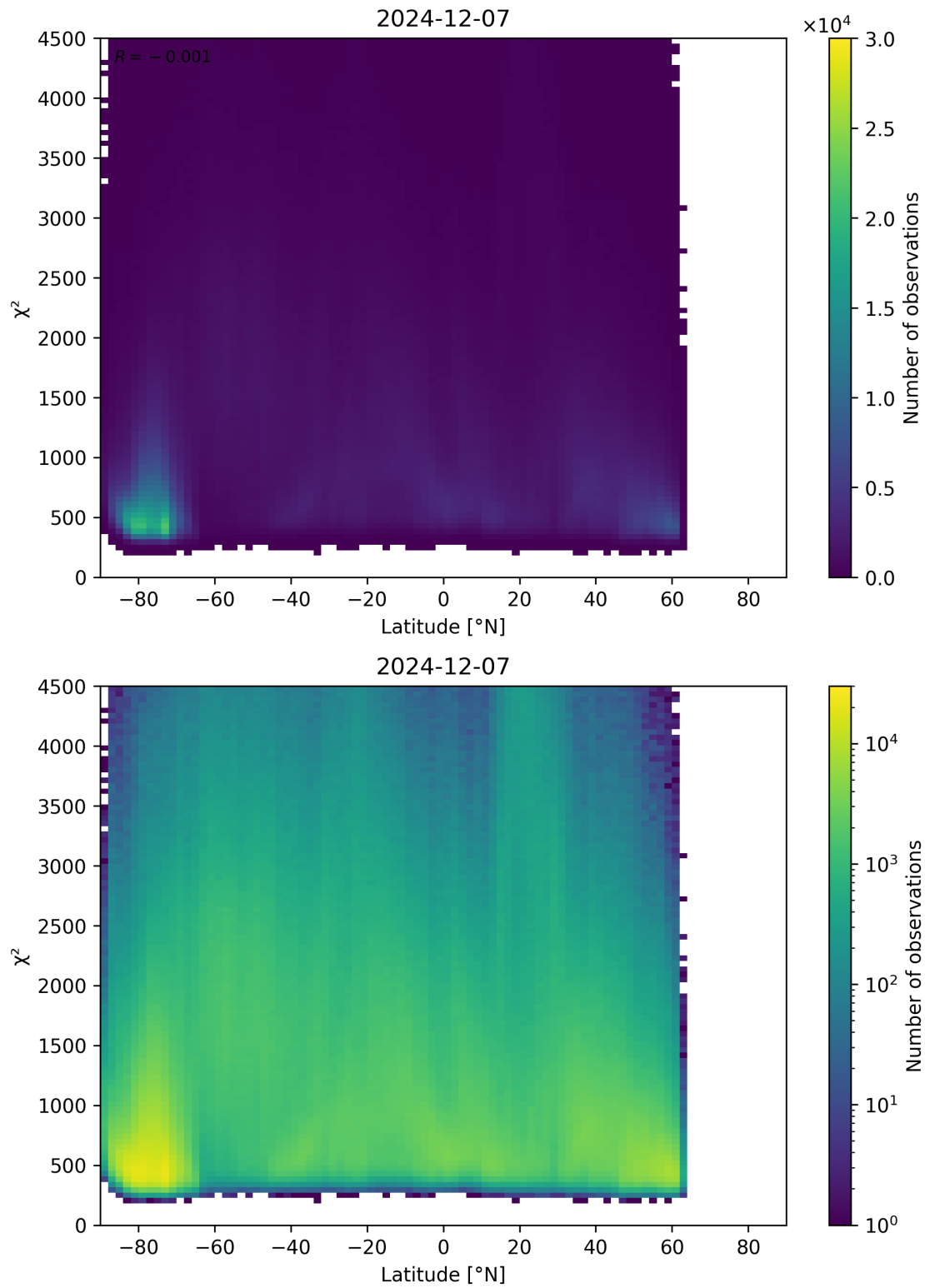
Figure 54: Scatter density plot of “Latitude” against “ \chi^2 ” for 2024-12-06 to 2024-12-08.
