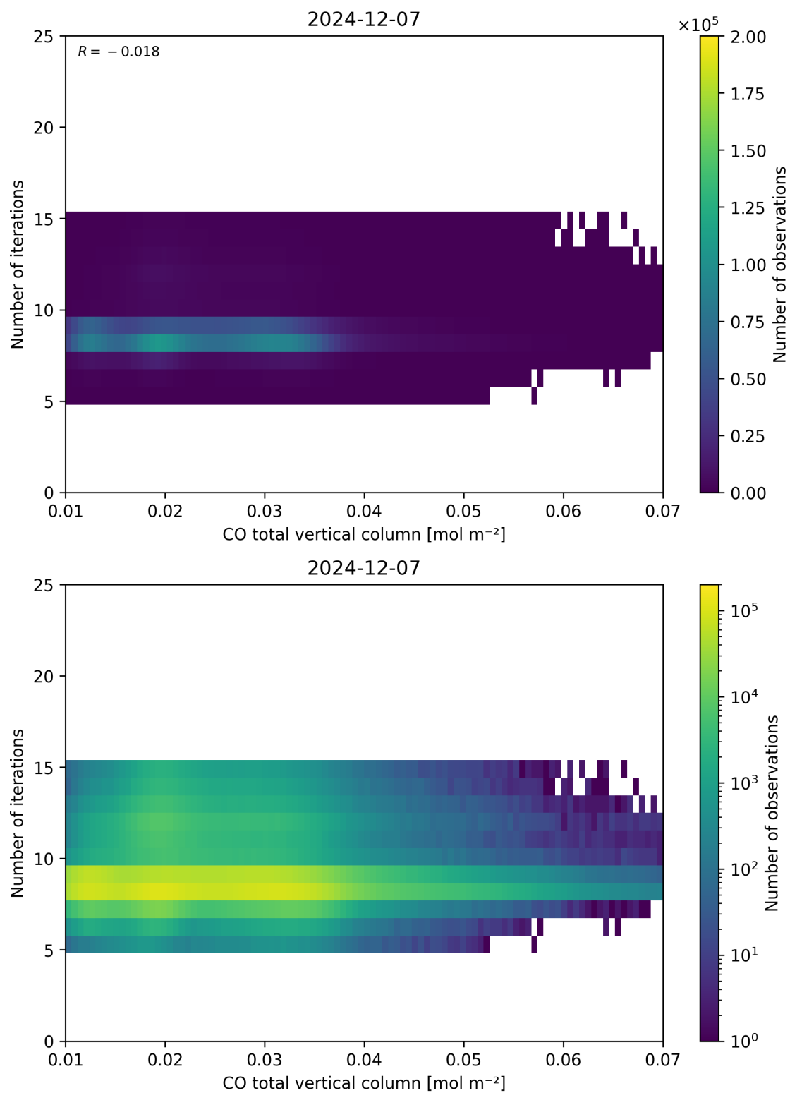
Figure 42: Scatter density plot of “CO total vertical column” against “Number of iterations” for 2024-12-06 to 2024-12-08.
