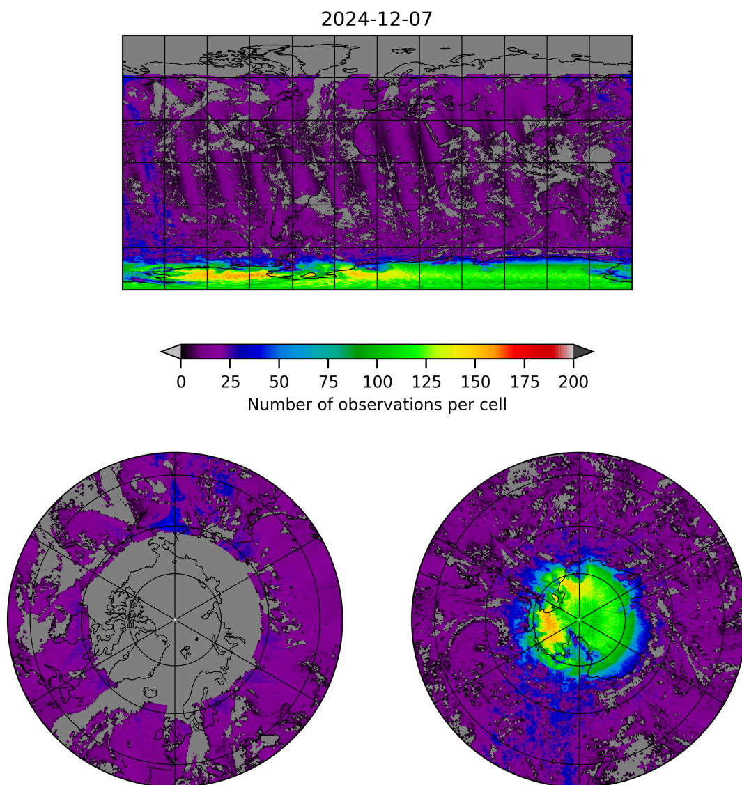
Figure 8: Map of the number of observations for 2024-12-06 to 2024-12-08
