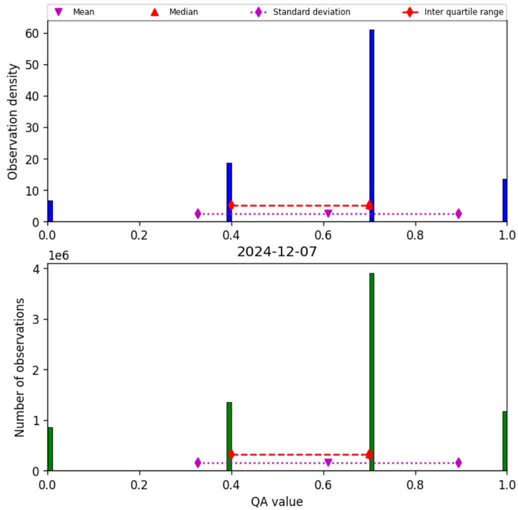
Figure 17: Histogram of “QA value” for 2024-12-06 to 2024-12-08
