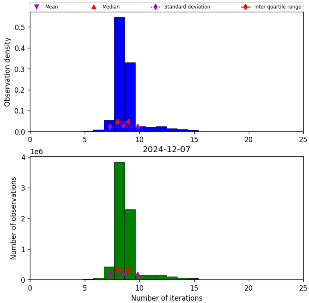
Figure 24: Histogram of “Number of iterations” for 2024-12-06 to 2024-12-08
