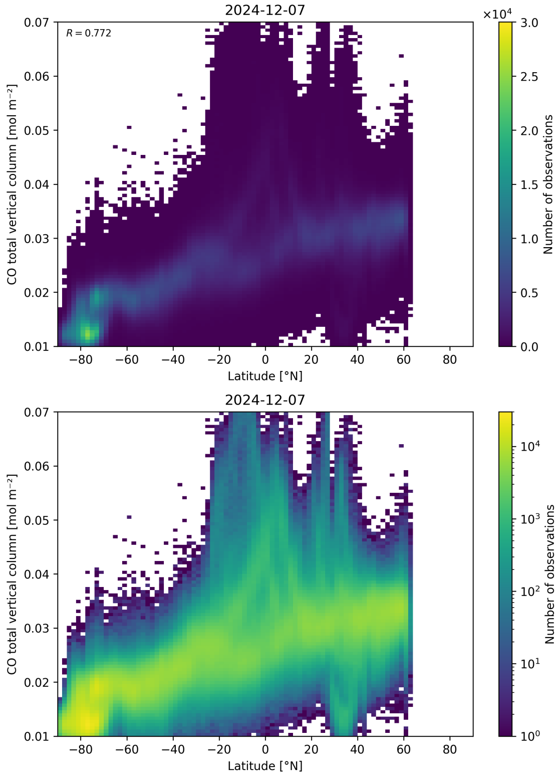
Figure 51: Scatter density plot of “Latitude” against “CO total vertical column” for 2024-12-06 to 2024-12-08.
