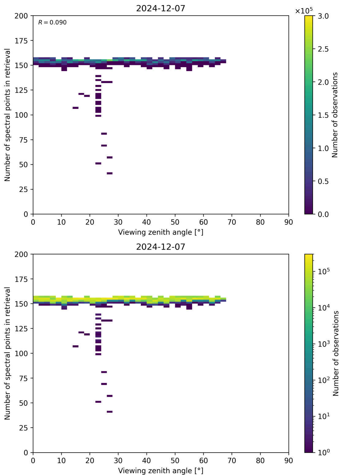
Figure 76: Scatter density plot of “Viewing zenith angle” against “Number of spectral points in retrieval” for 2024-12-06 to 2024-12-08.
