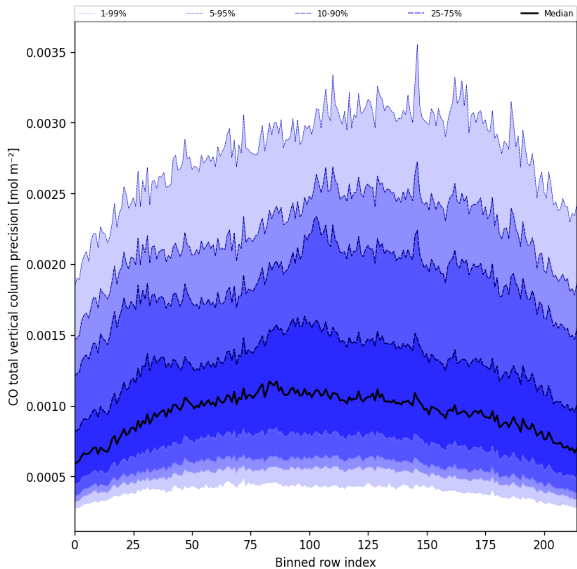
Figure 28: Along track statistics of “CO total vertical column precision” for 2024-12-06 to 2024-12-08
