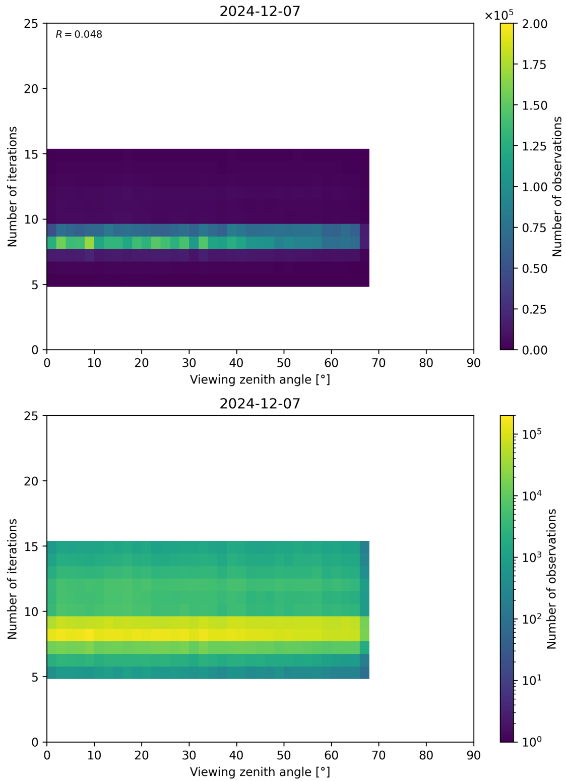
Figure 75: Scatter density plot of “Viewing zenith angle” against “Number of iterations” for 2024-12-06 to 2024-12-08.
