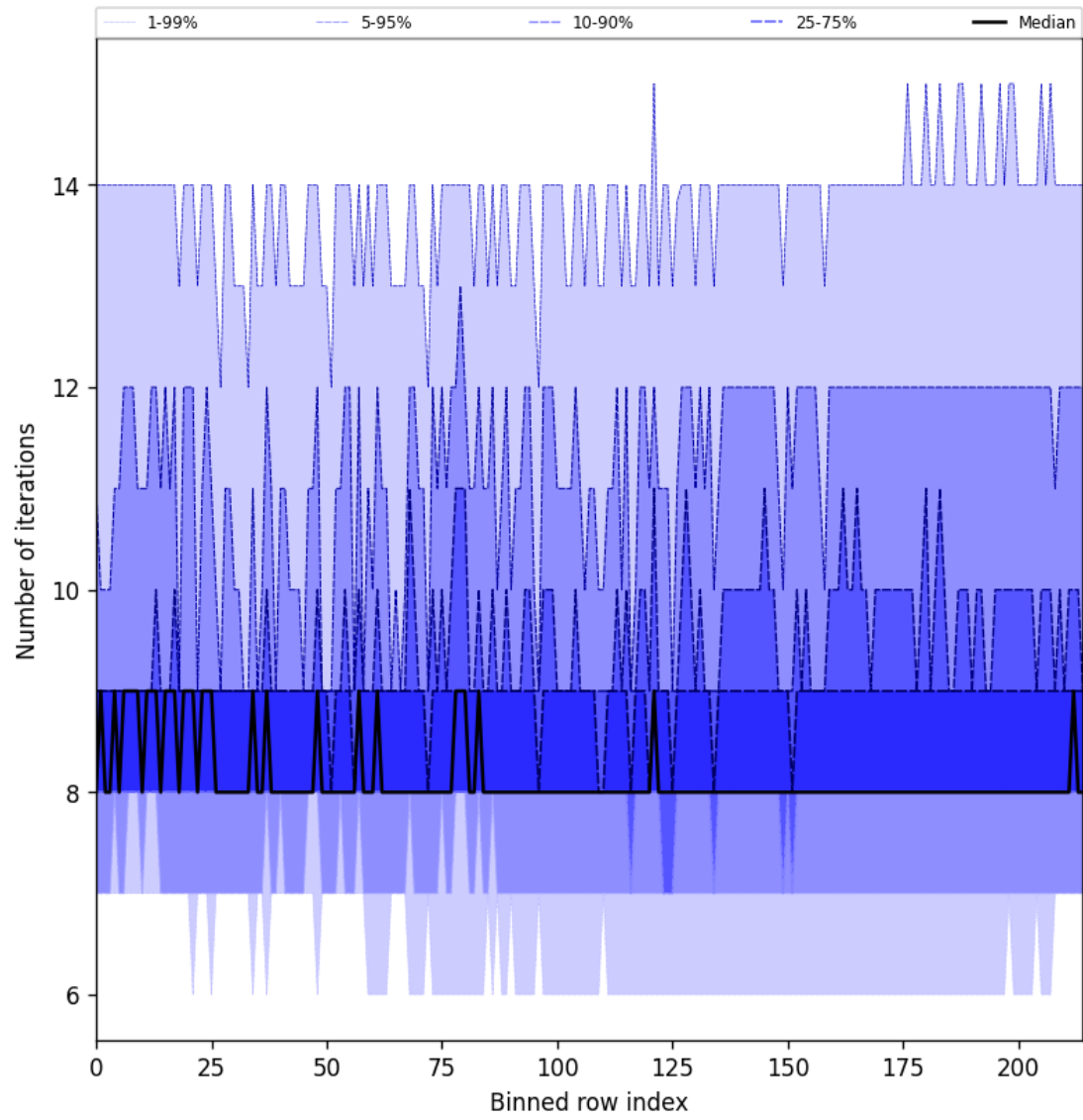
Figure 32: Along track statistics of “Number of iterations” for 2024-12-06 to 2024-12-08
