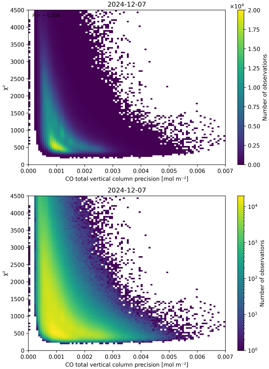
Figure 44: Scatter density plot of “CO total vertical column precision” against “ \chi^2 ” for 2024-12-06 to 2024-12-08.
