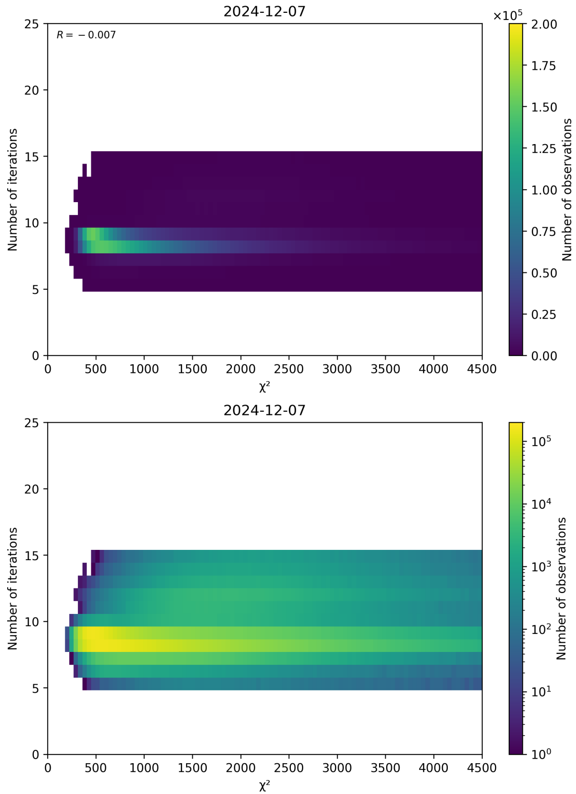
Figure 49: Scatter density plot of “ \chi^2 ” against “Number of iterations” for 2024-12-06 to 2024-12-08.
