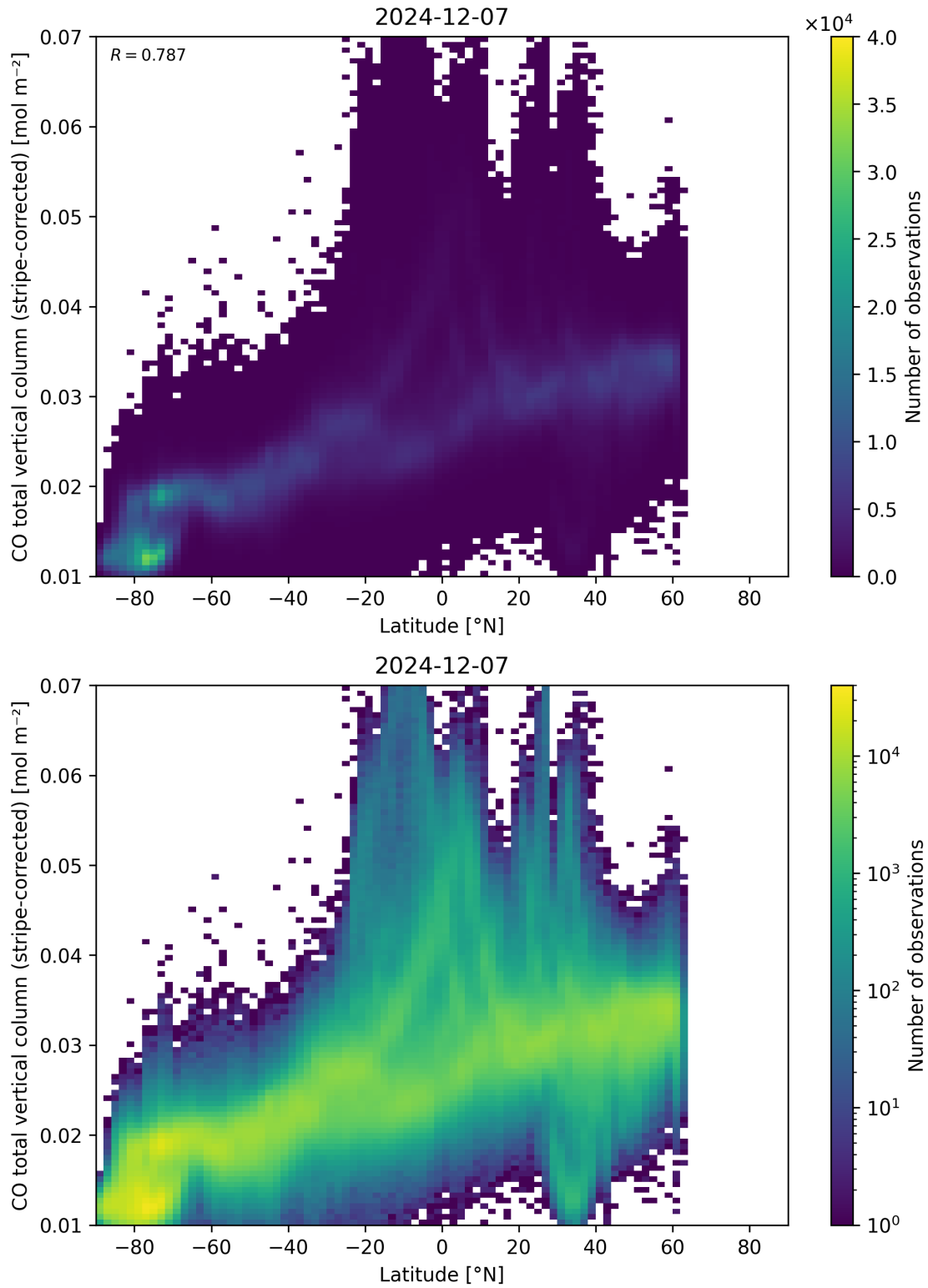
Figure 52: Scatter density plot of “Latitude” against “CO total vertical column (stripe-corrected)” for 2024-12-06 to 2024-12-08.
