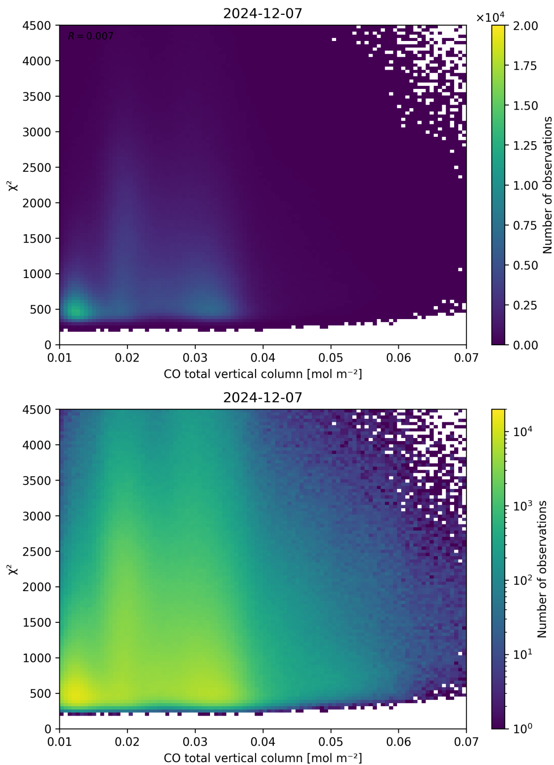
Figure 35: Scatter density plot of “CO total vertical column” against “ \chi^2 ” for 2024-12-06 to 2024-12-08.
