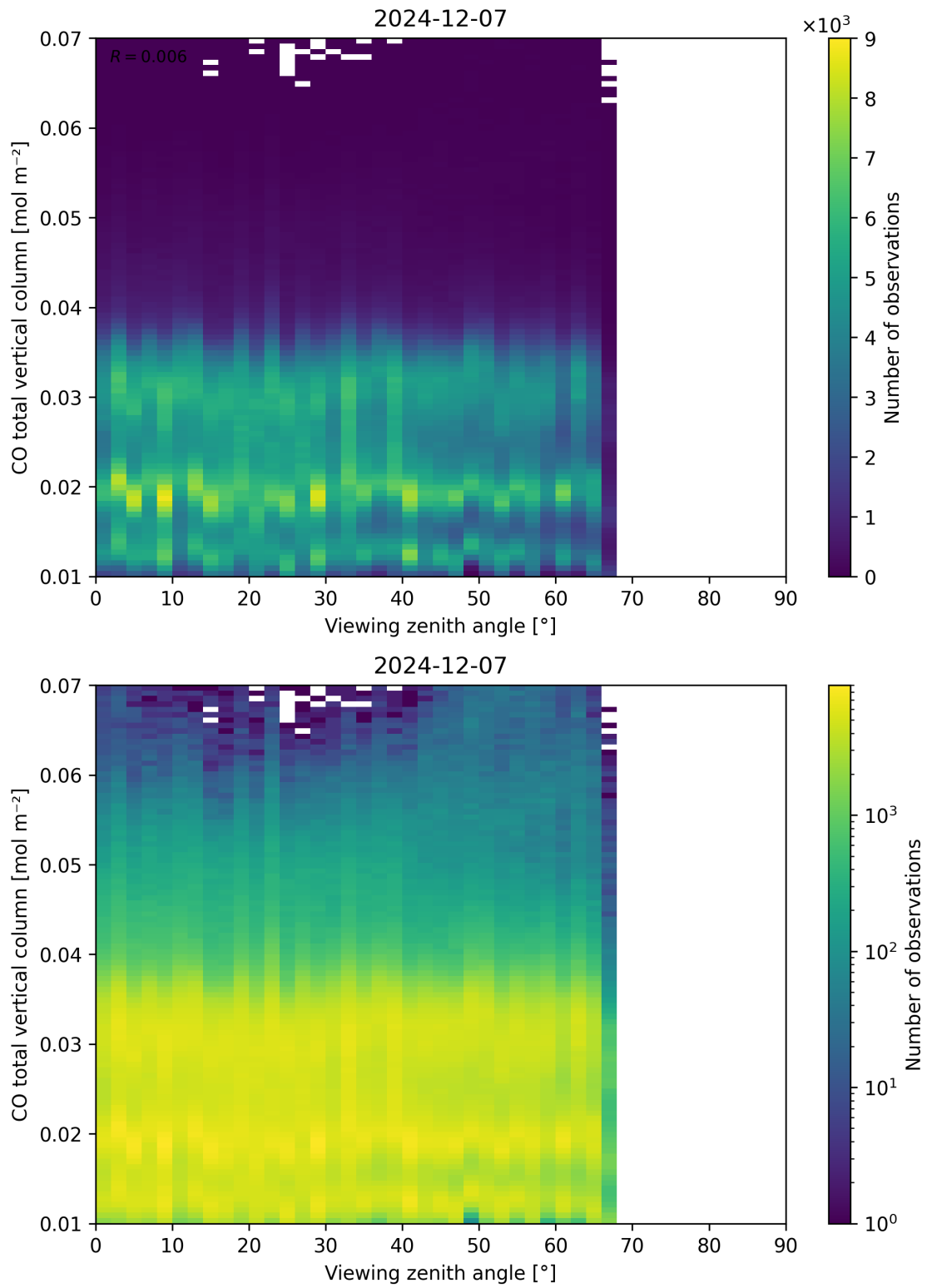
Figure 69: Scatter density plot of “Viewing zenith angle” against “CO total vertical column” for 2024-12-06 to 2024-12-08.
