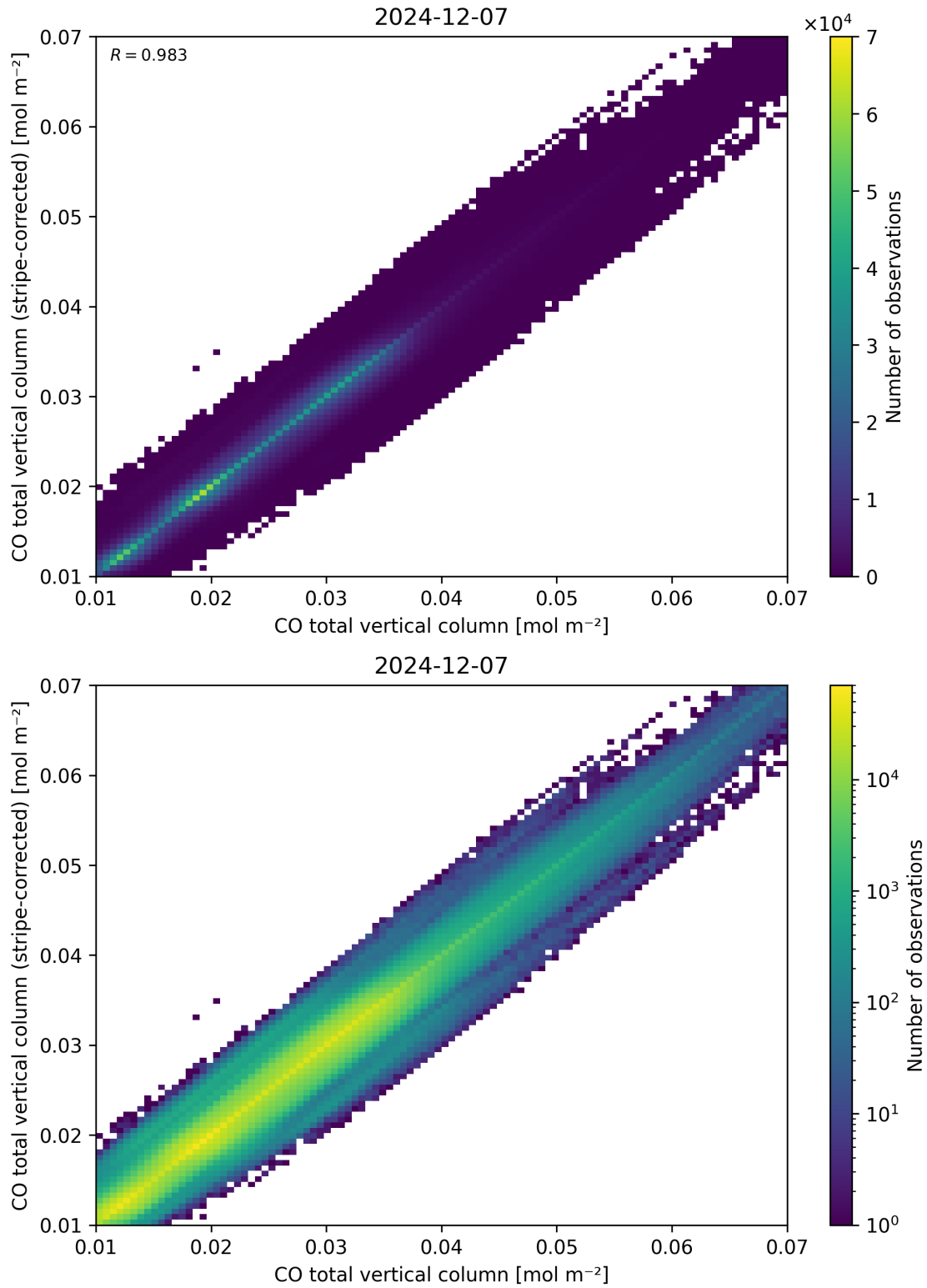
Figure 33: Scatter density plot of “CO total vertical column” against “CO total vertical column (stripe-corrected)” for 2024-12-06 to 2024-12-08.
