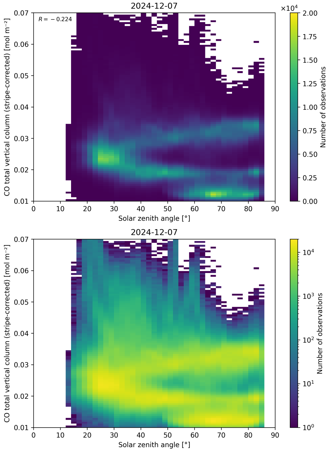
Figure 62: Scatter density plot of “Solar zenith angle” against “CO total vertical column (stripe-corrected)” for 2024-12-06 to 2024-12-08.
