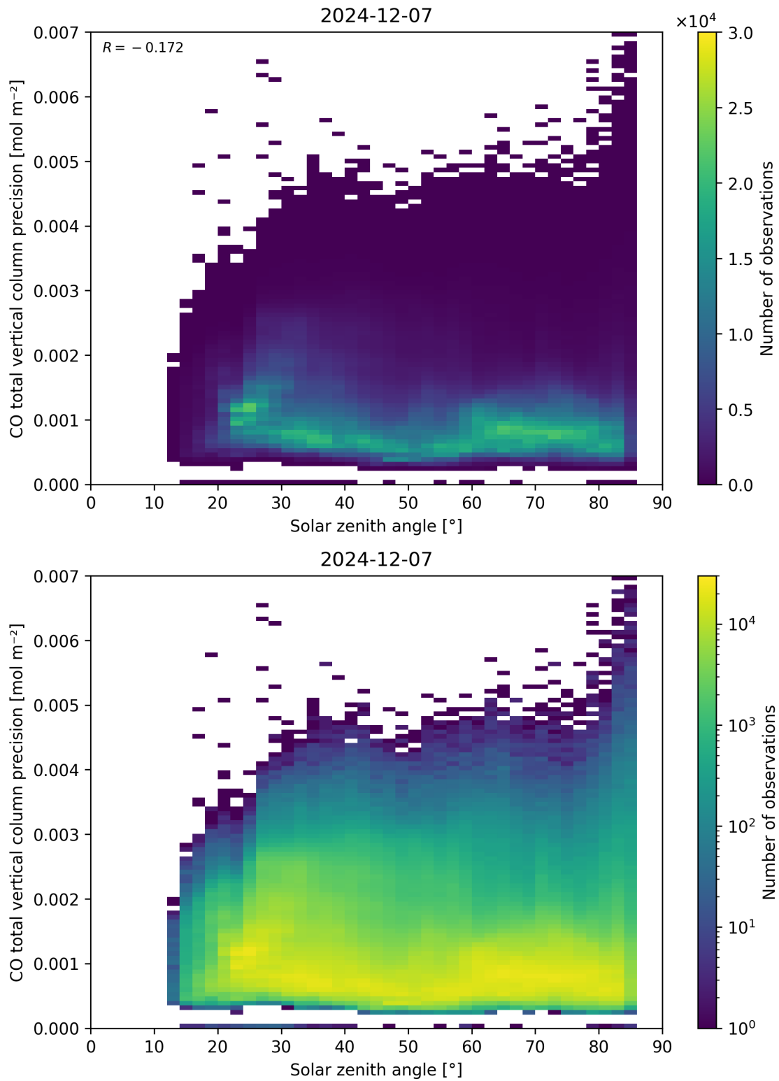
Figure 63: Scatter density plot of “Solar zenith angle” against “CO total vertical column precision” for 2024-12-06 to 2024-12-08.
