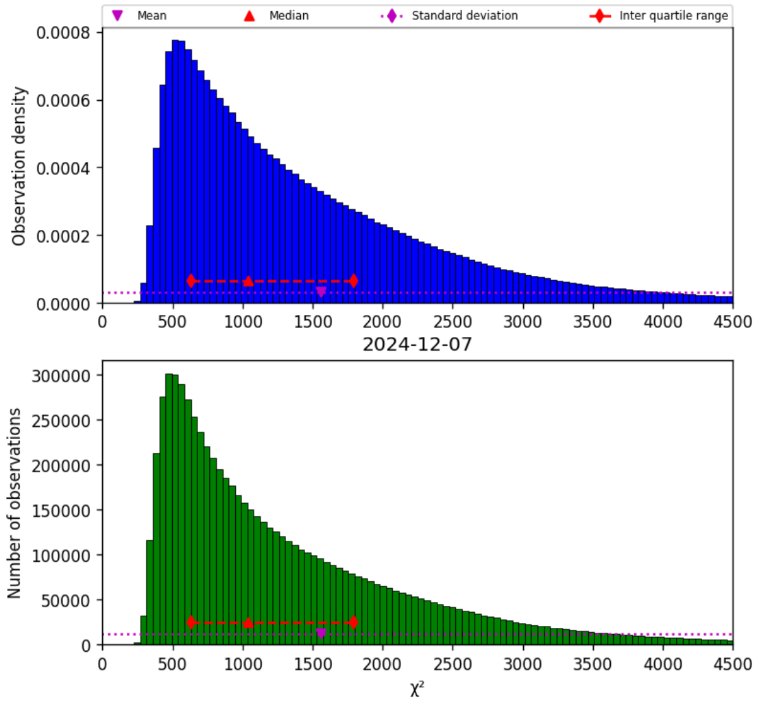
Figure 22: Histogram of “ \chi^2 ” for 2024-12-06 to 2024-12-08
