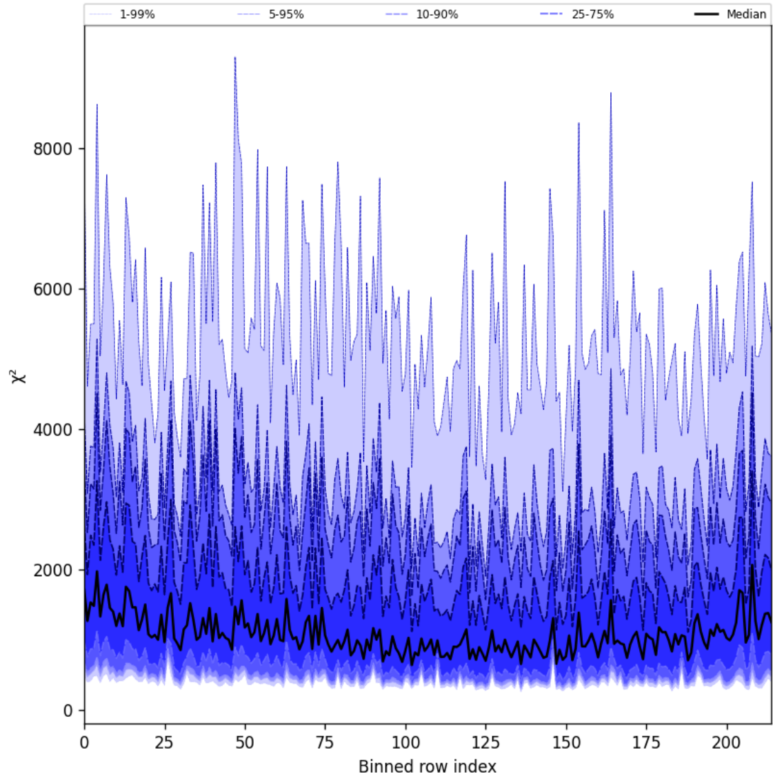
Figure 30: Along track statistics of “ \chi^2 ” for 2024-12-06 to 2024-12-08
