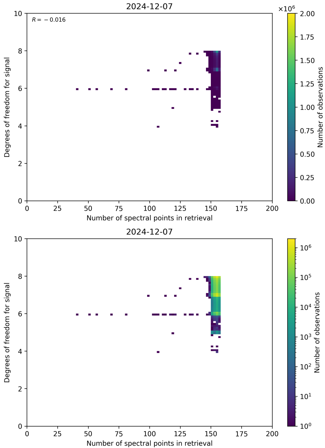
Figure 59: Scatter density plot of “Number of spectral points in retrieval” against “Degrees of freedom for signal” for 2024-12-06 to 2024-12-08.
