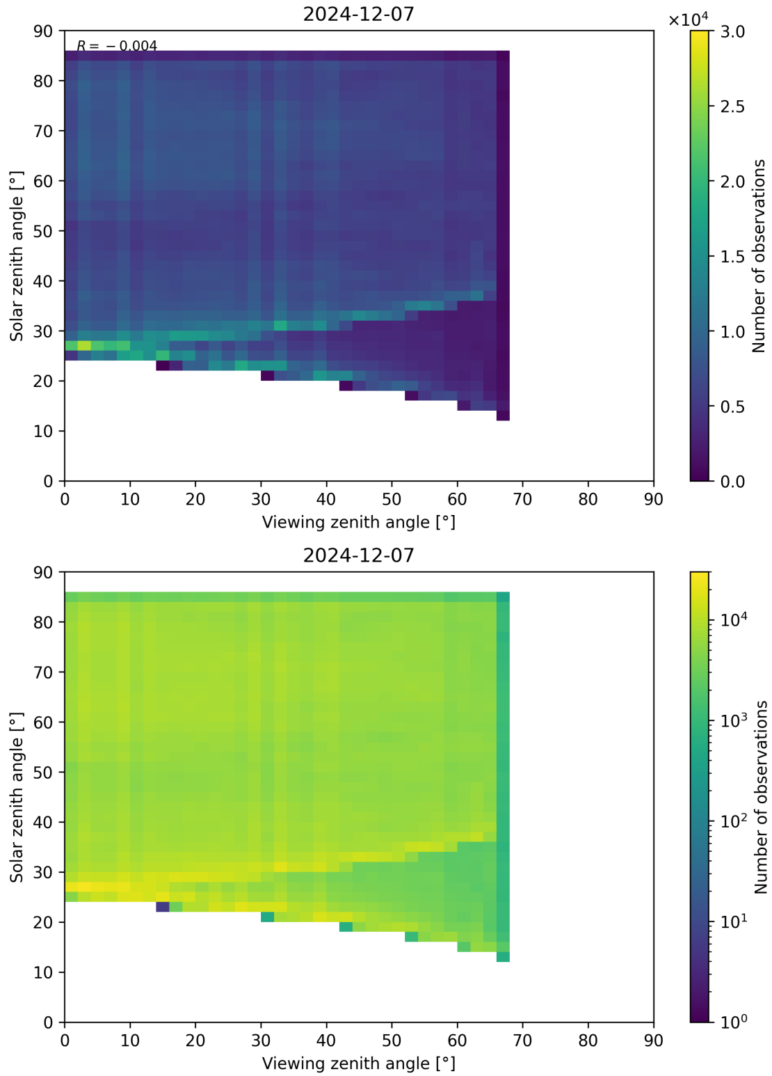
Figure 77: Scatter density plot of “Viewing zenith angle” against “Solar zenith angle” for 2024-12-06 to 2024-12-08.
