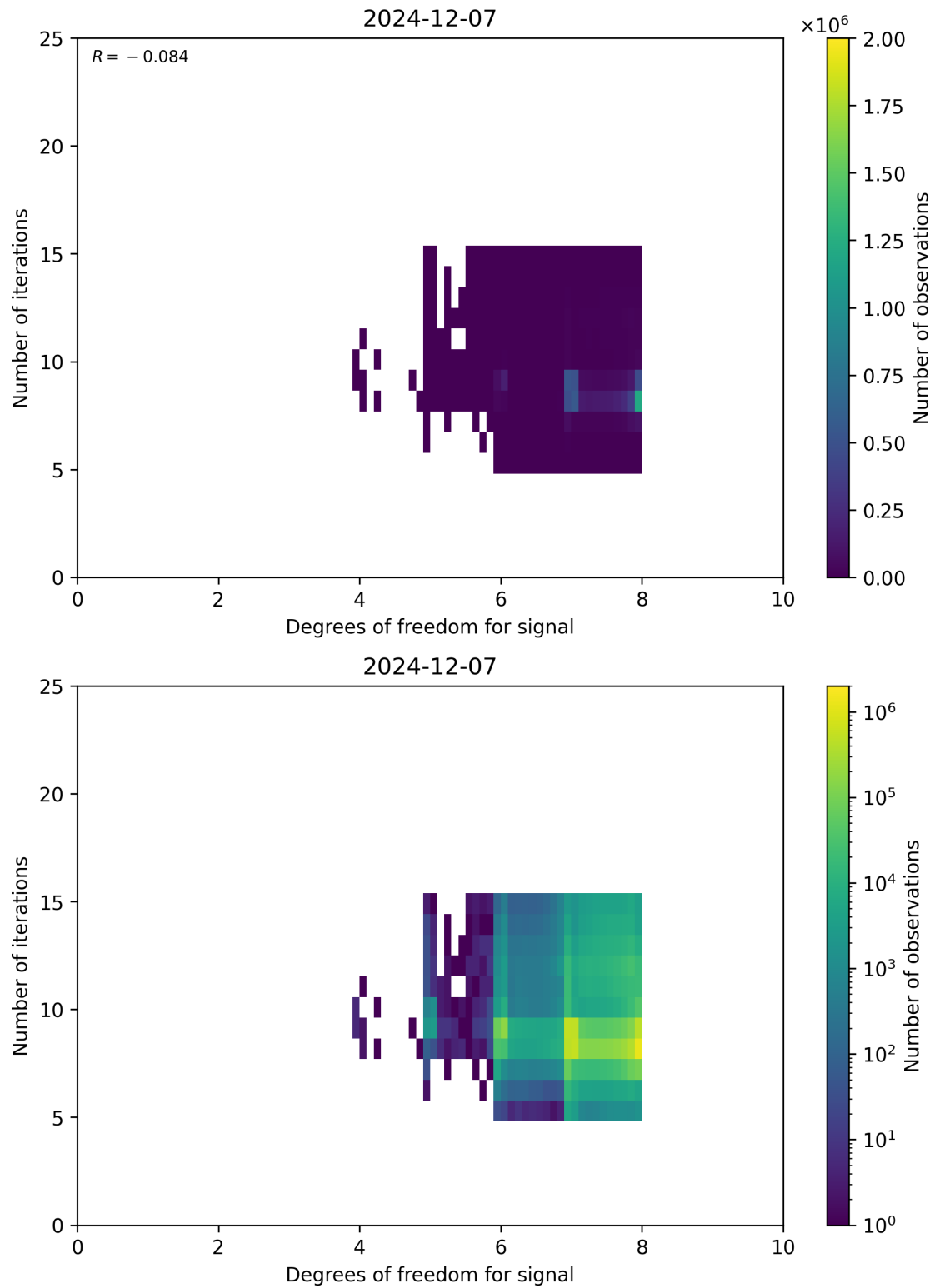
Figure 50: Scatter density plot of “Degrees of freedom for signal” against “Number of iterations” for 2024-12-06 to 2024-12-08.
