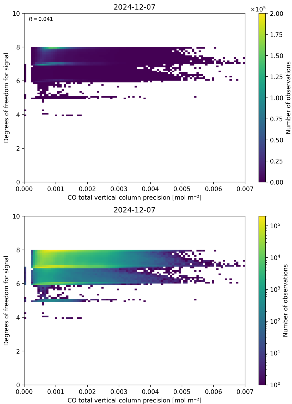
Figure 45: Scatter density plot of “CO total vertical column precision” against “Degrees of freedom for signal” for 2024-12-06 to 2024-12-08.
