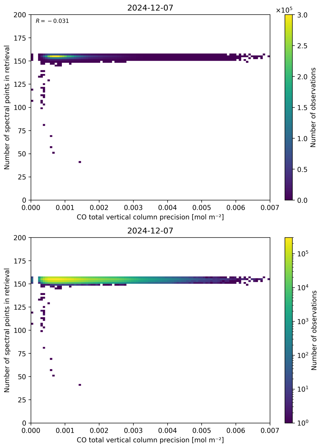
Figure 47: Scatter density plot of “CO total vertical column precision” against “Number of spectral points in retrieval” for 2024-12-06 to 2024-12-08.
