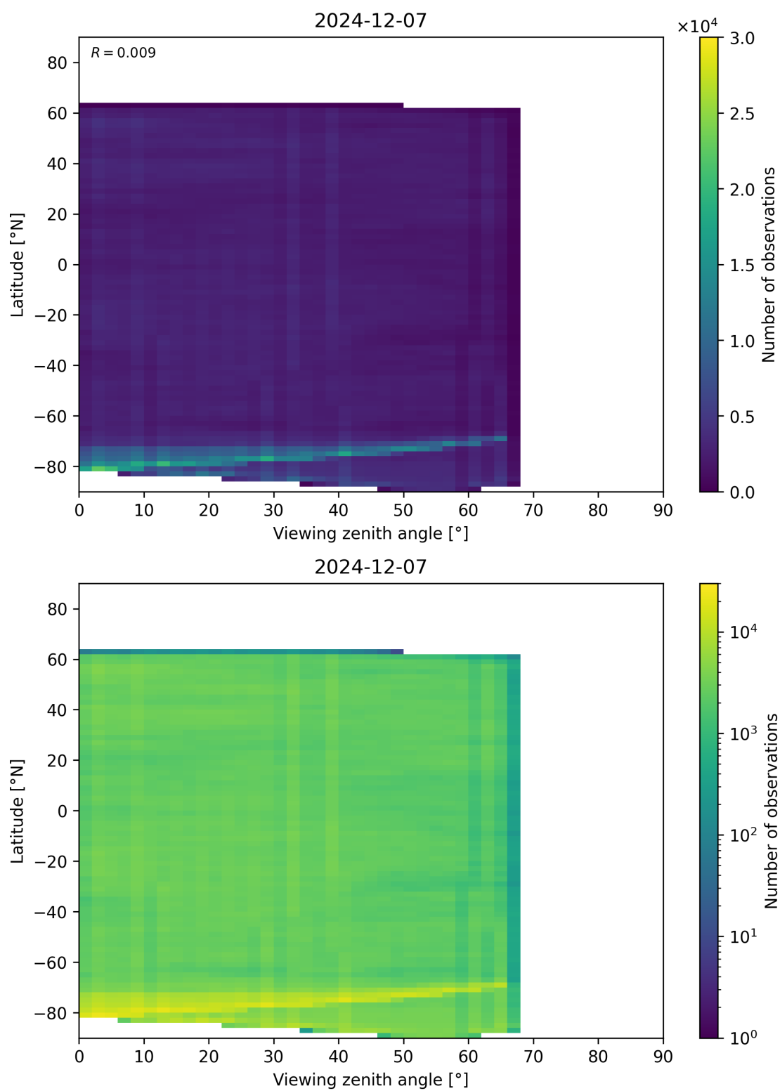
Figure 74: Scatter density plot of “Viewing zenith angle” against “Latitude” for 2024-12-06 to 2024-12-08.
