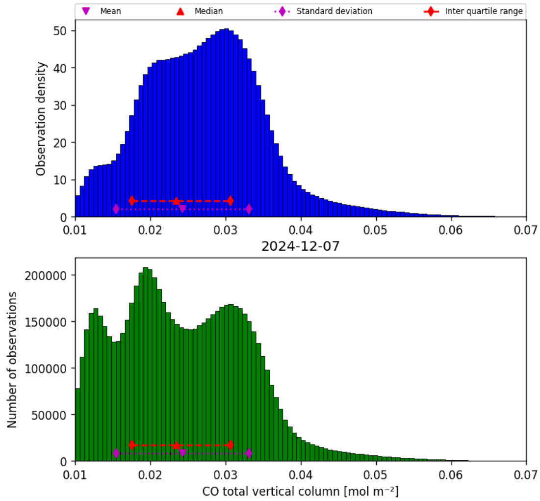
Figure 18: Histogram of “CO total vertical column” for 2024-12-06 to 2024-12-08
