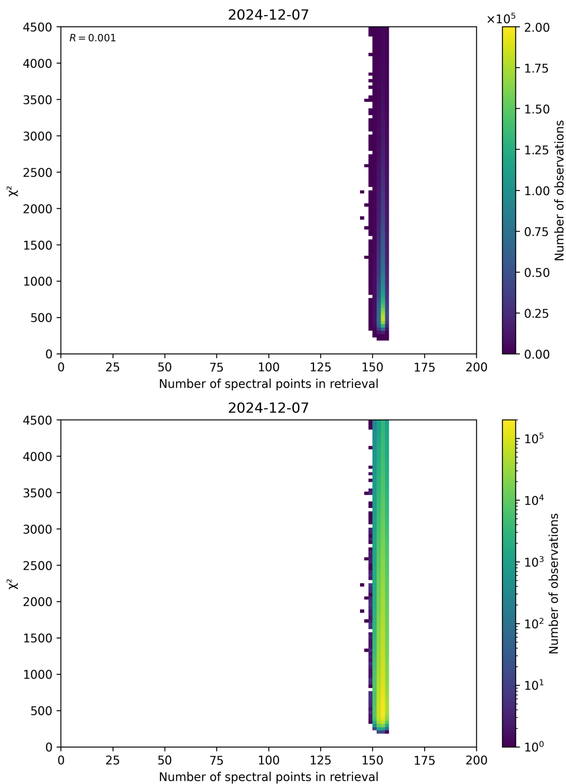
Figure 58: Scatter density plot of “Number of spectral points in retrieval” against “ \chi^2 ” for 2024-12-06 to 2024-12-08.
