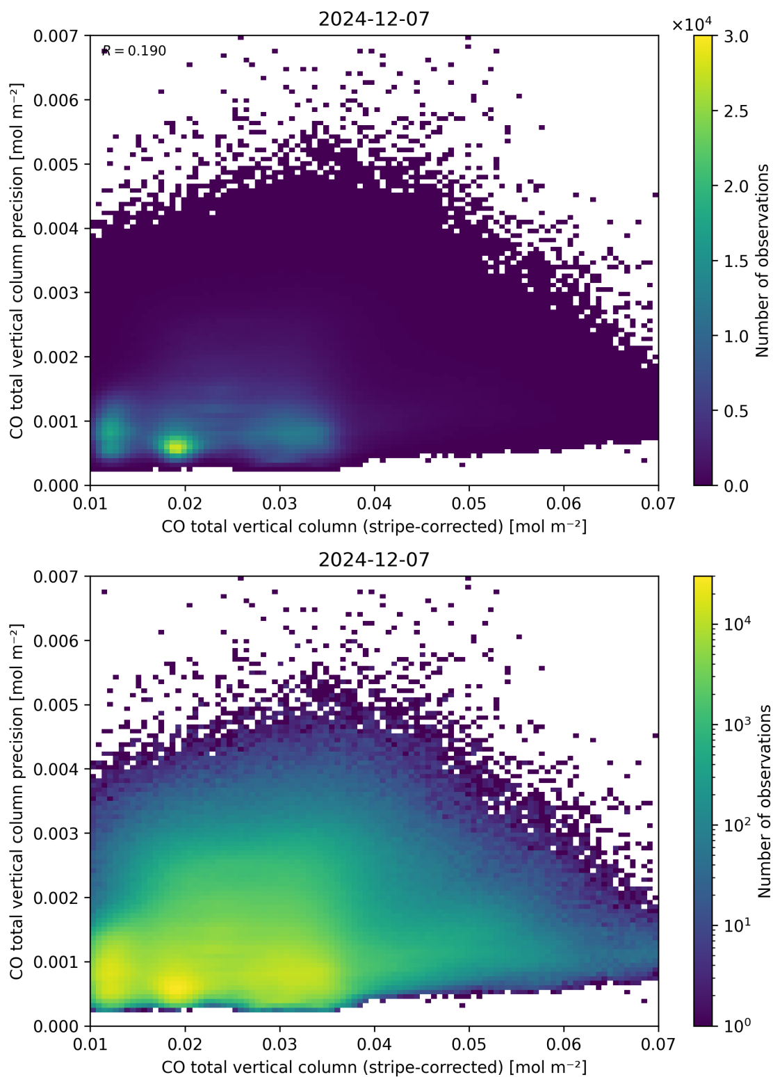
Figure 36: Scatter density plot of “CO total vertical column (stripe-corrected)” against “CO total vertical column precision” for 2024-12-06 to 2024-12-08.
