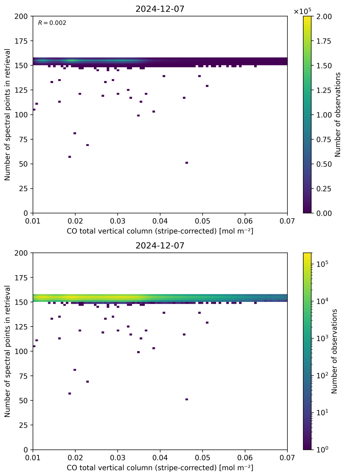
Figure 40: Scatter density plot of “CO total vertical column (stripe-corrected)” against “Number of spectral points in retrieval” for 2024-12-06 to 2024-12-08.
