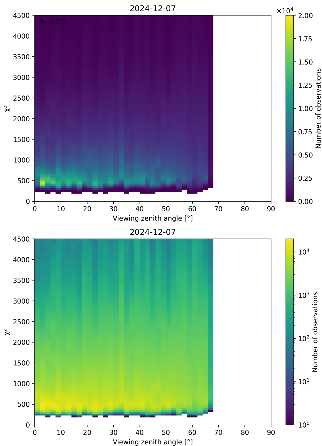
Figure 72: Scatter density plot of “Viewing zenith angle” against “ \chi^2 ” for 2024-12-06 to 2024-12-08.
