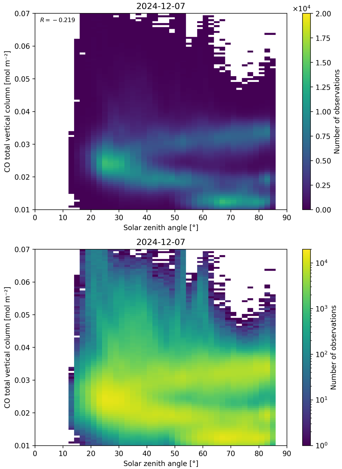
Figure 61: Scatter density plot of “Solar zenith angle” against “CO total vertical column” for 2024-12-06 to 2024-12-08.
