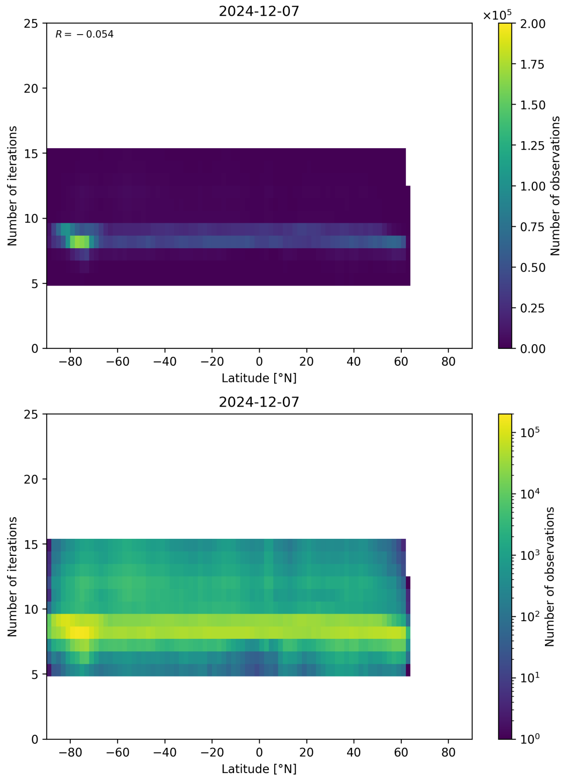
Figure 56: Scatter density plot of “Latitude” against “Number of iterations” for 2024-12-06 to 2024-12-08.
