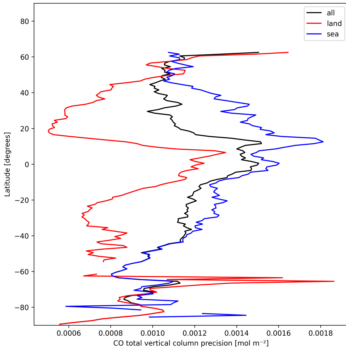
Figure 12: Zonal average of “CO total vertical column precision” for 2024-12-06 to 2024-12-08.
