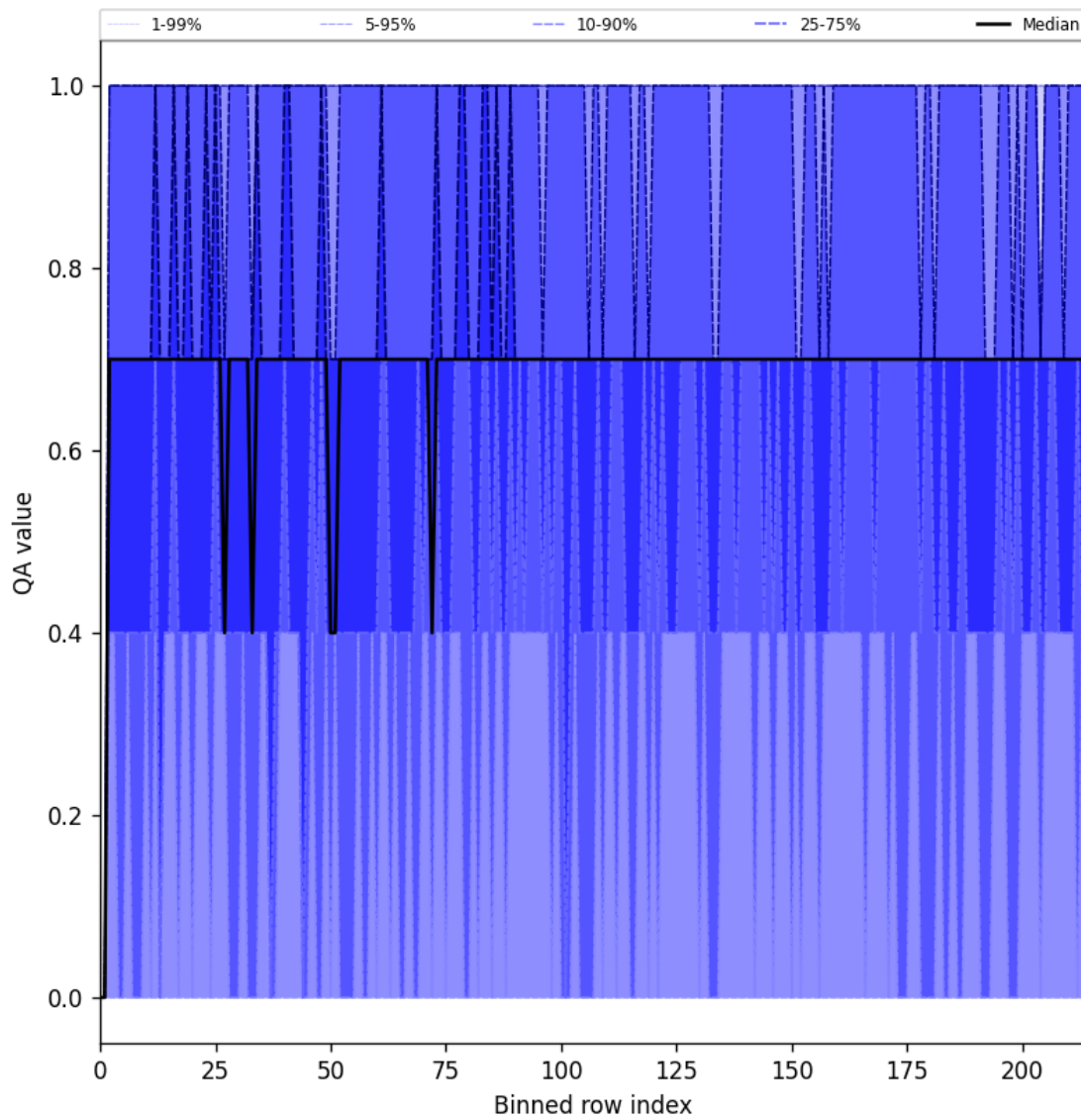
Figure 25: Along track statistics of “QA value” for 2024-12-06 to 2024-12-08
