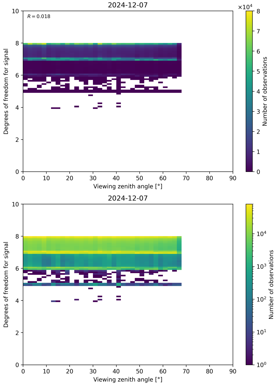
Figure 73: Scatter density plot of “Viewing zenith angle” against “Degrees of freedom for signal” for 2024-12-06 to 2024-12-08.
