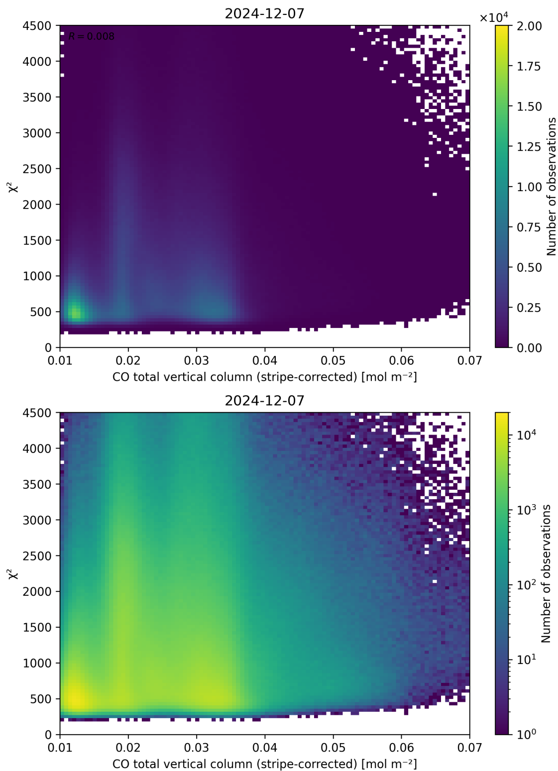
Figure 37: Scatter density plot of “CO total vertical column (stripe-corrected)” against “ \chi^2 ” for 2024-12-06 to 2024-12-08.
