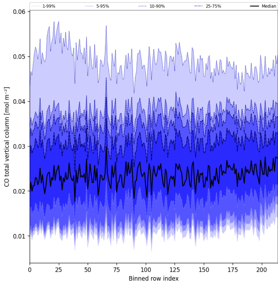
Figure 26: Along track statistics of “CO total vertical column” for 2024-12-06 to 2024-12-08
