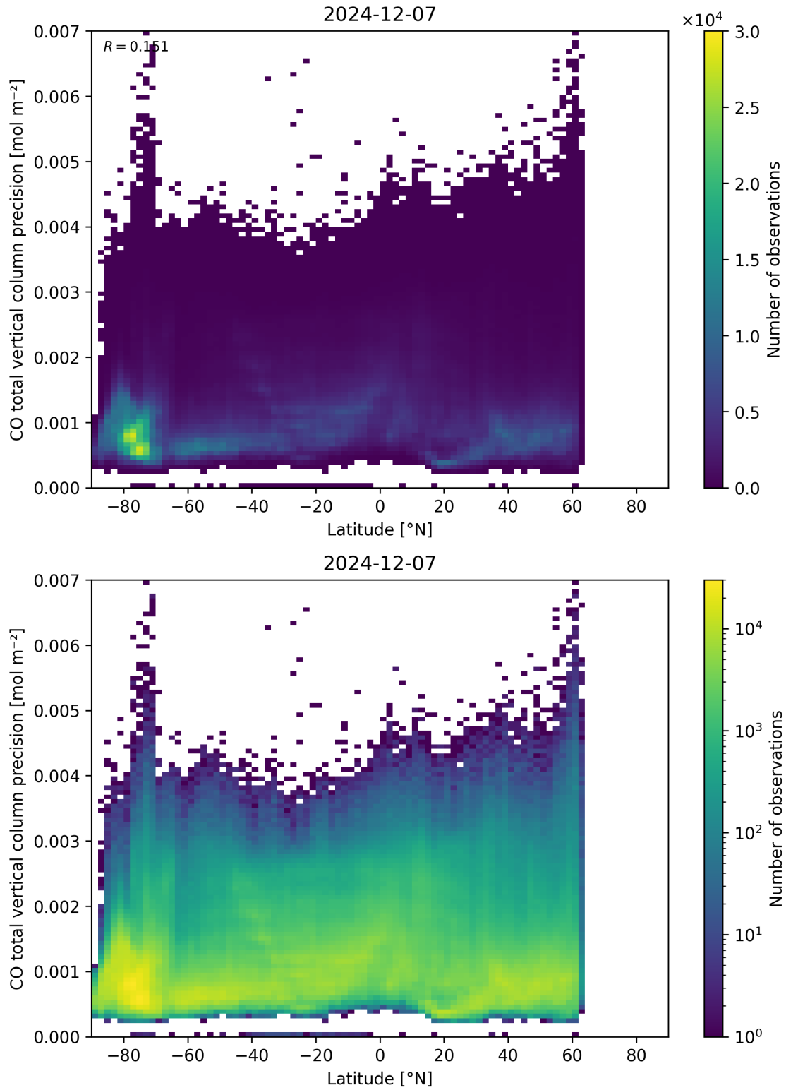
Figure 53: Scatter density plot of “Latitude” against “CO total vertical column precision” for 2024-12-06 to 2024-12-08.
