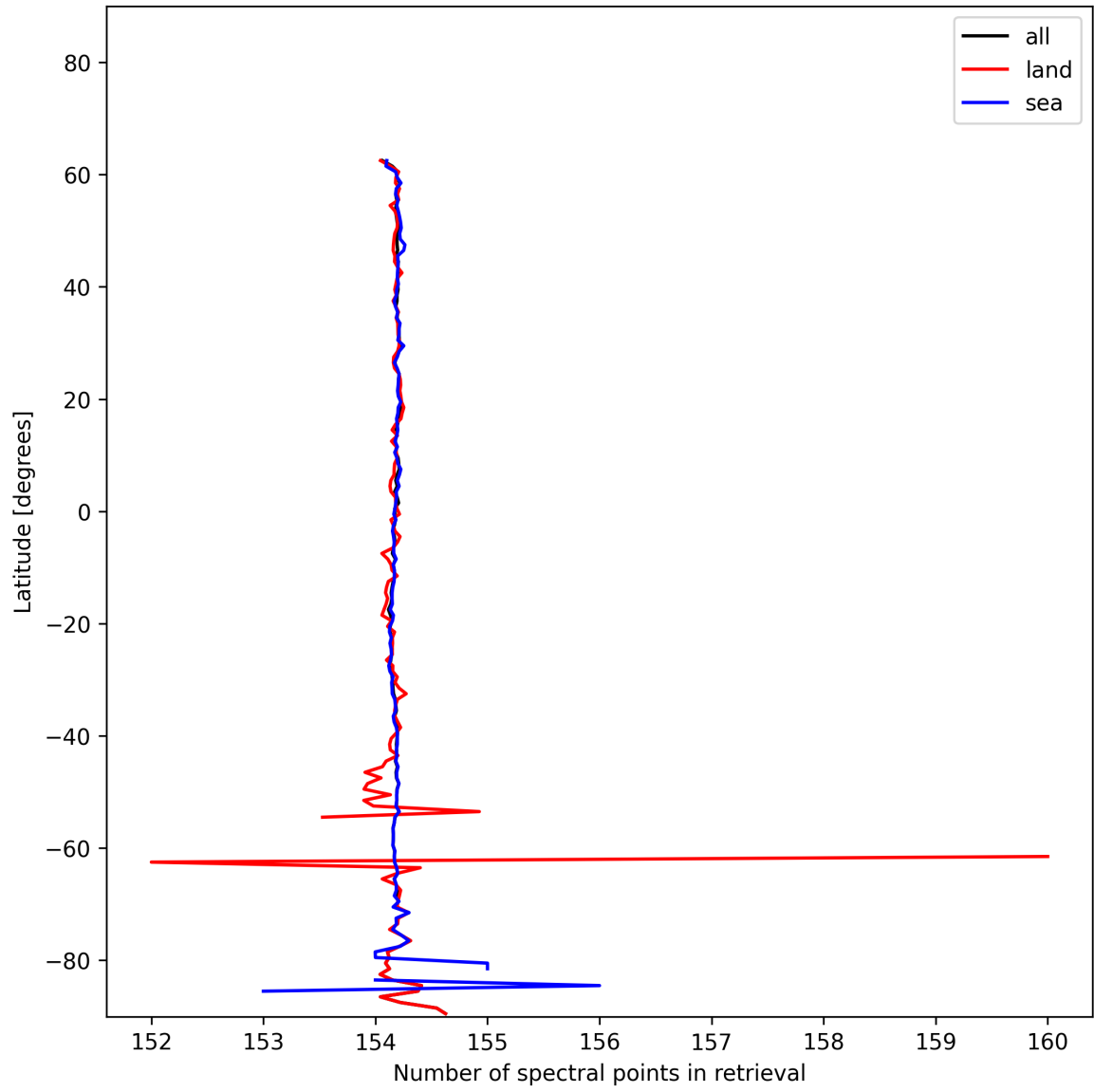
Figure 13: Zonal average of “Number of spectral points in retrieval” for 2024-12-06 to 2024-12-08.
