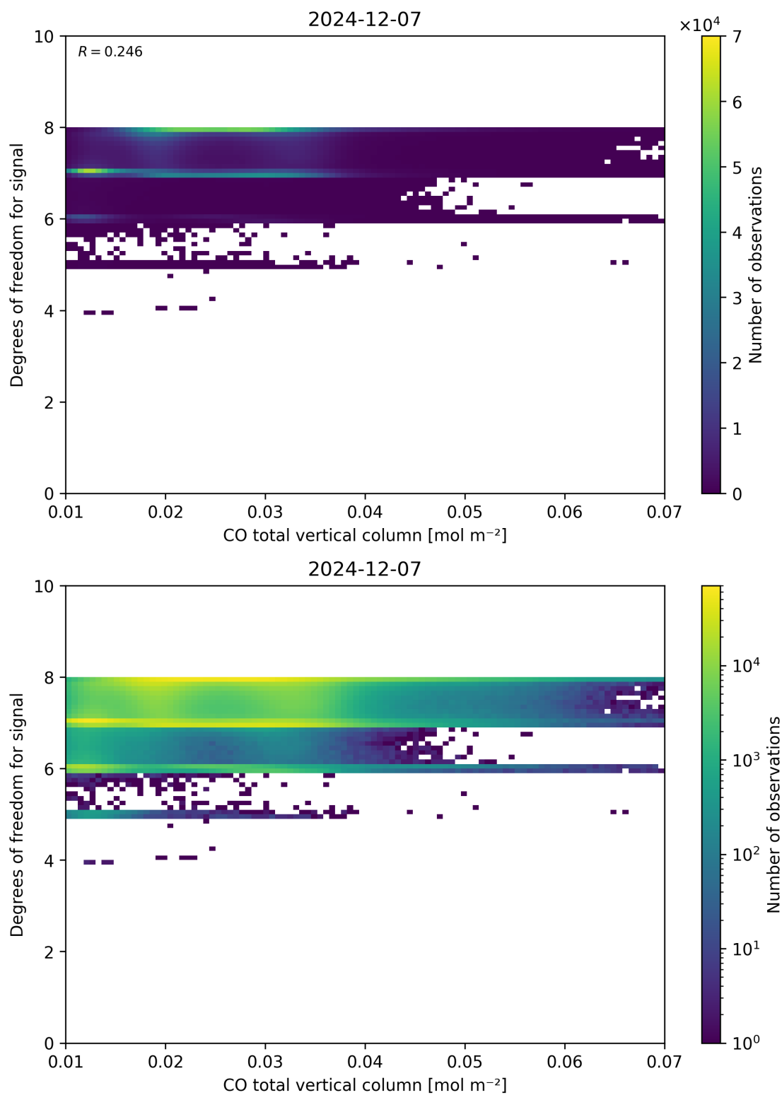
Figure 41: Scatter density plot of “CO total vertical column” against “Degrees of freedom for signal” for 2024-12-06 to 2024-12-08.
