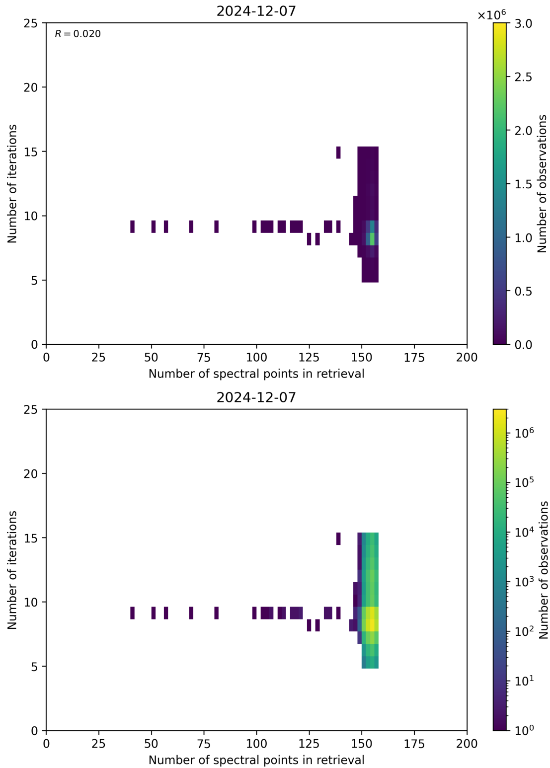
Figure 60: Scatter density plot of “Number of spectral points in retrieval” against “Number of iterations” for 2024-12-06 to 2024-12-08.
