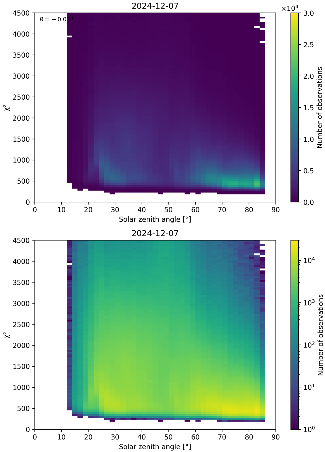
Figure 64: Scatter density plot of “Solar zenith angle” against “ \chi^2 ” for 2024-12-06 to 2024-12-08.
