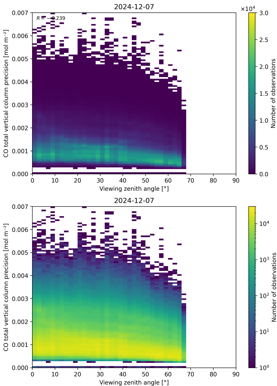
Figure 71: Scatter density plot of “Viewing zenith angle” against “CO total vertical column precision” for 2024-12-06 to 2024-12-08.
