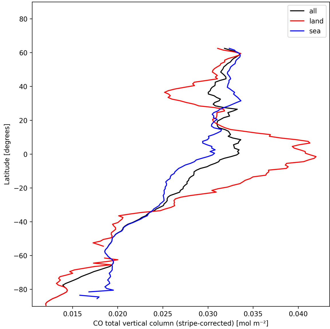
Figure 11: Zonal average of “CO total vertical column (stripe-corrected)” for 2024-12-06 to 2024-12-08.
