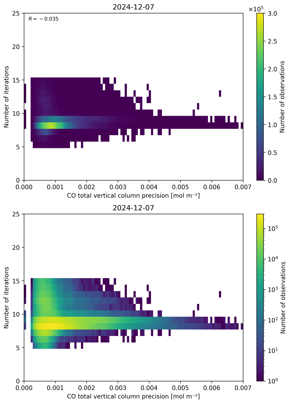
Figure 46: Scatter density plot of “CO total vertical column precision” against “Number of iterations” for 2024-12-06 to 2024-12-08.
