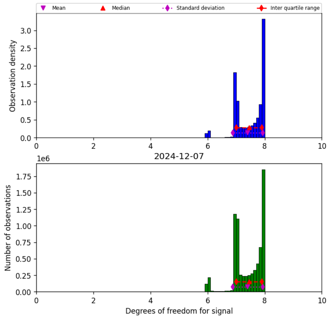
Figure 23: Histogram of “Degrees of freedom for signal” for 2024-12-06 to 2024-12-08
