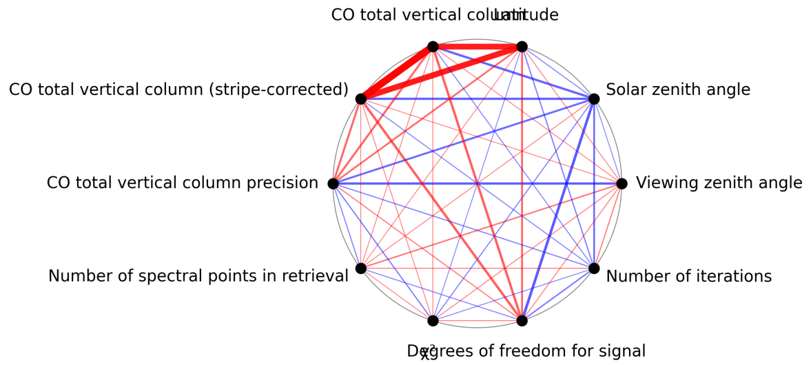
Figure 1: Map of correlation graph for 2024-12-06 to 2024-12-08.
