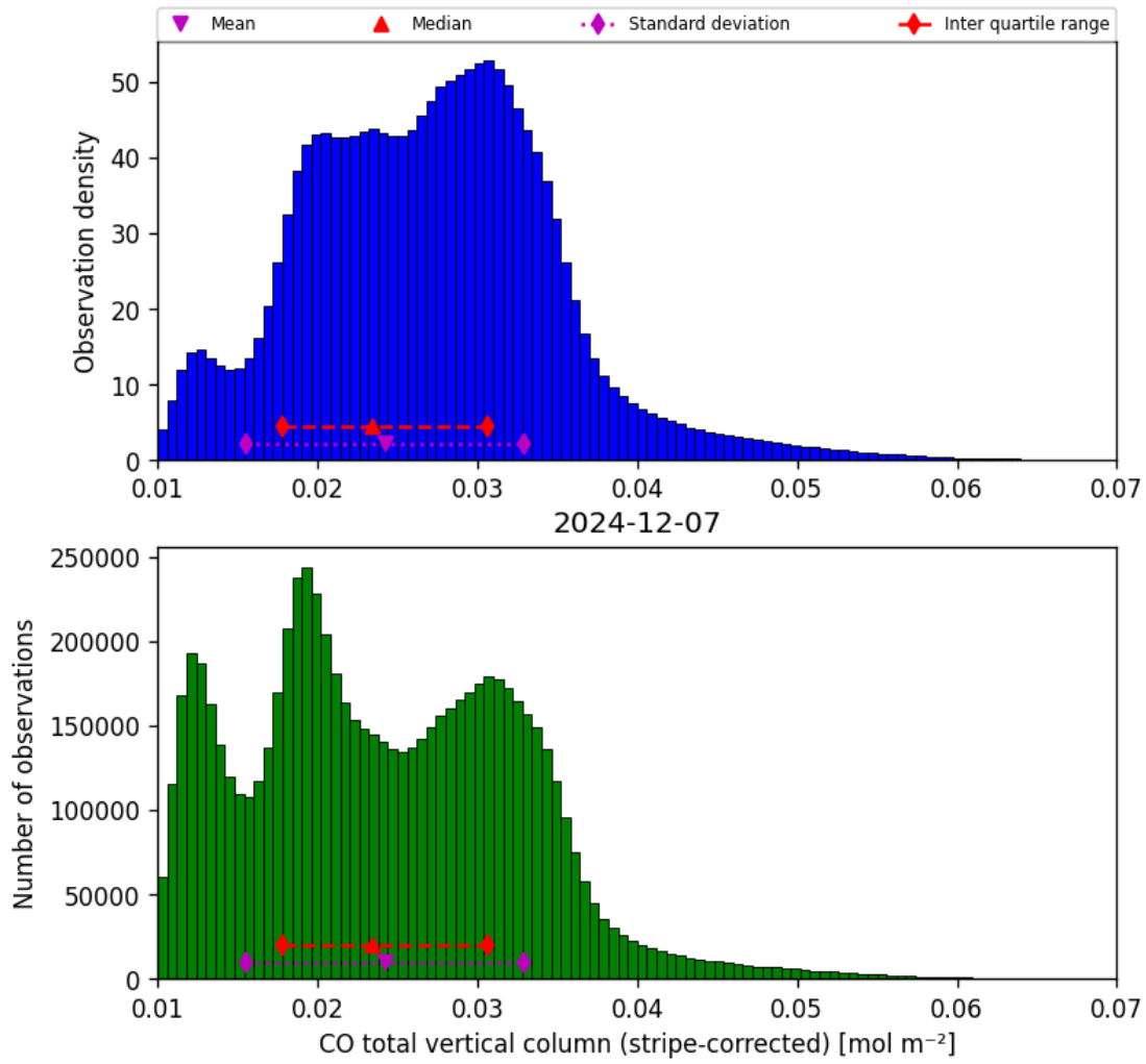
Figure 19: Histogram of “CO total vertical column (stripe-corrected)” for 2024-12-06 to 2024-12-08
