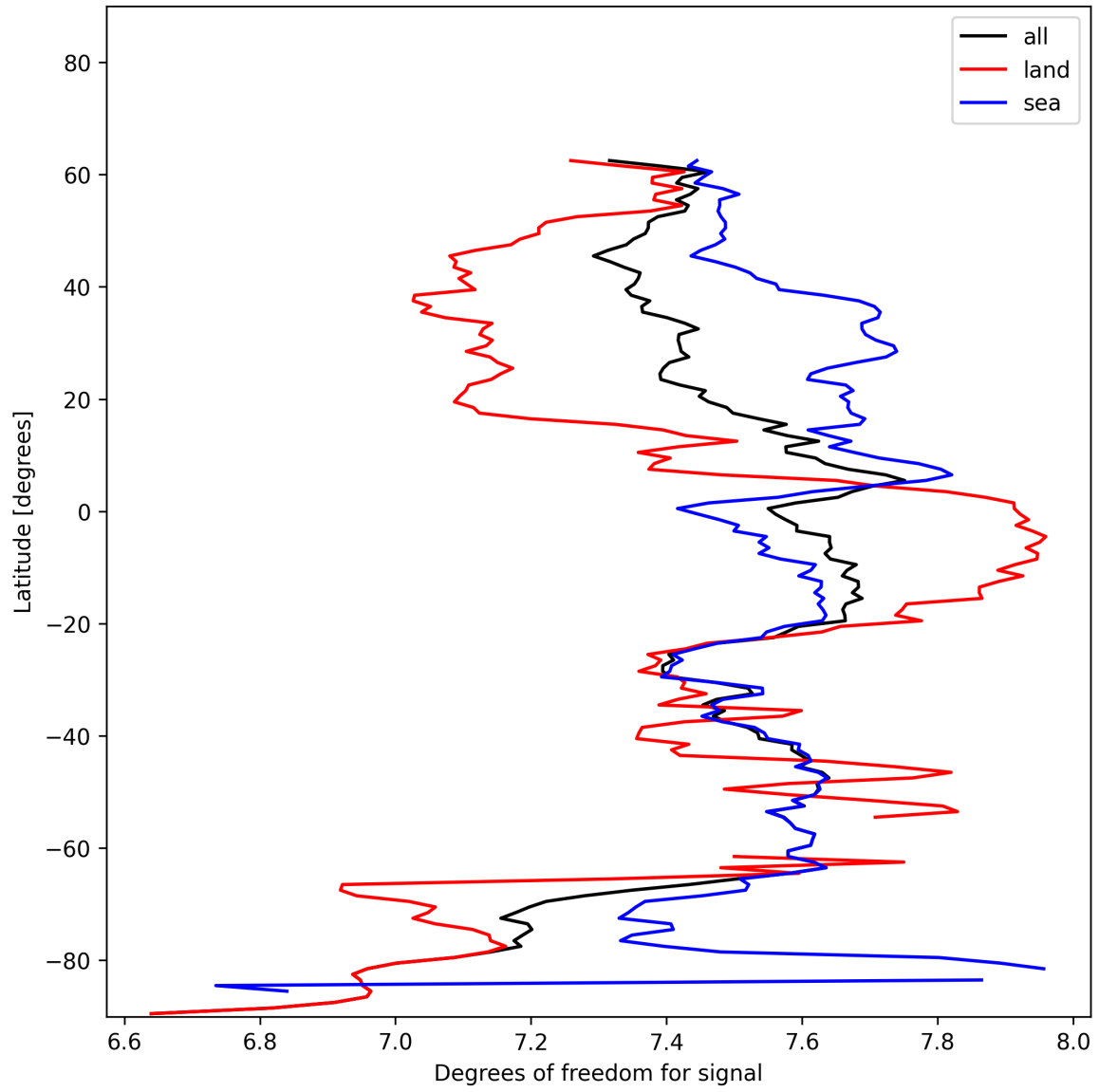
Figure 15: Zonal average of “Degrees of freedom for signal” for 2024-12-06 to 2024-12-08.
