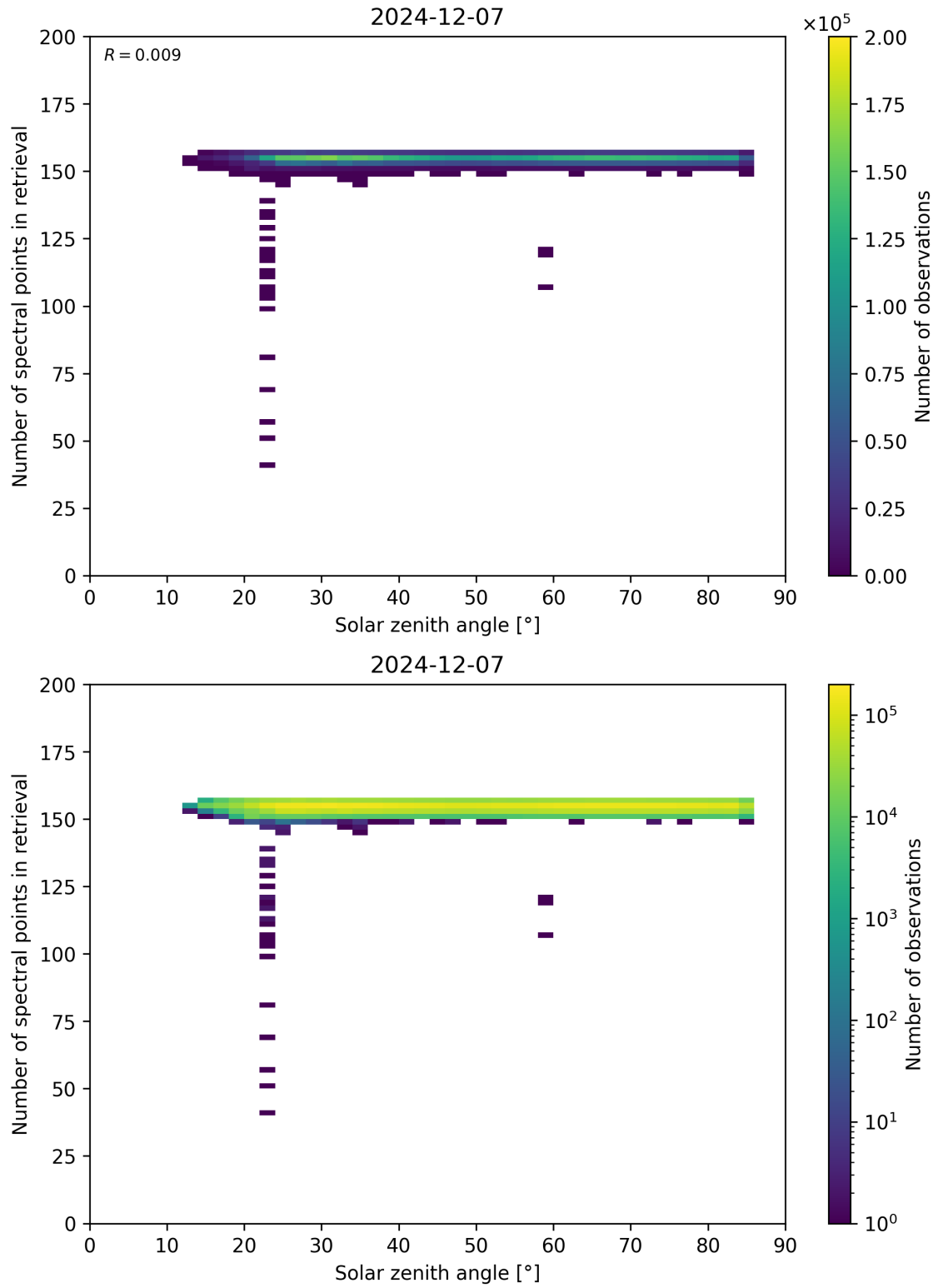
Figure 68: Scatter density plot of “Solar zenith angle” against “Number of spectral points in retrieval” for 2024-12-06 to 2024-12-08.
