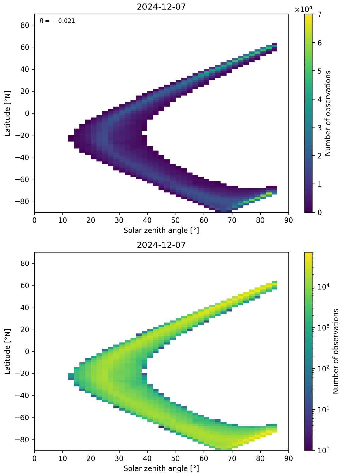
Figure 66: Scatter density plot of “Solar zenith angle” against “Latitude” for 2024-12-06 to 2024-12-08.
