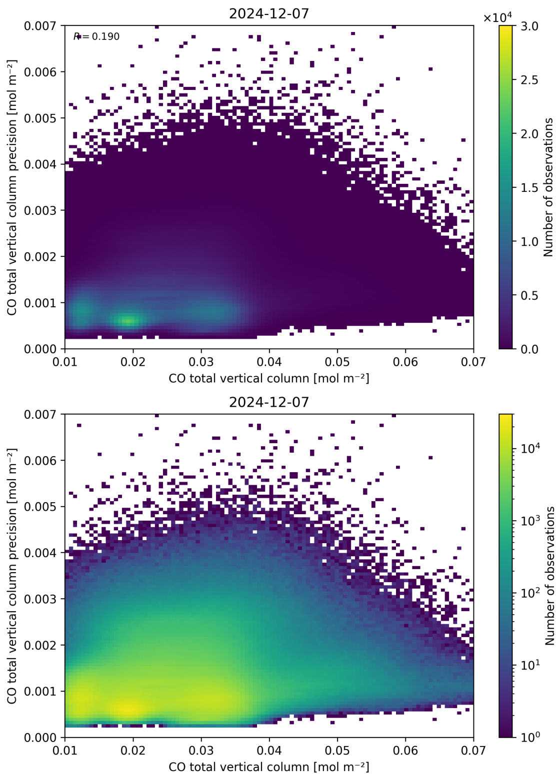
Figure 34: Scatter density plot of “CO total vertical column” against “CO total vertical column precision” for 2024-12-06 to 2024-12-08.
