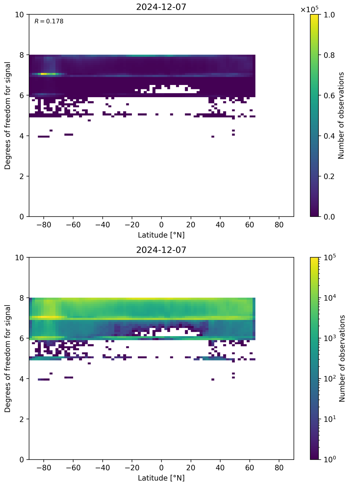
Figure 55: Scatter density plot of “Latitude” against “Degrees of freedom for signal” for 2024-12-06 to 2024-12-08.
