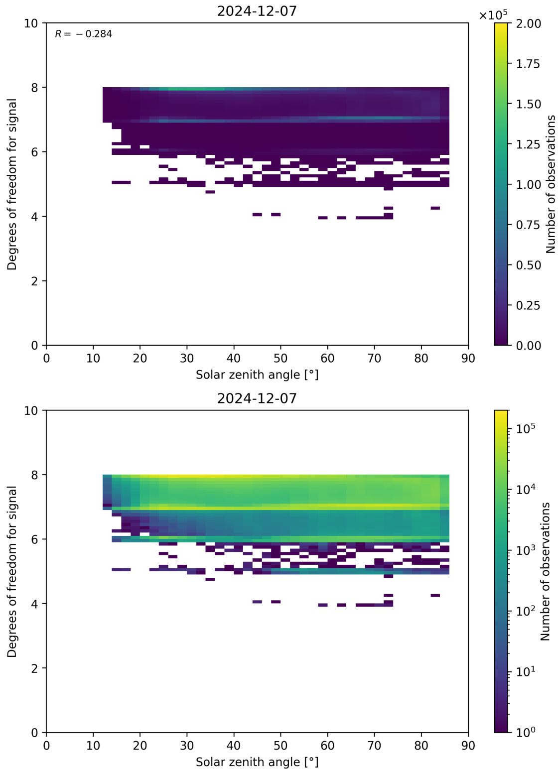
Figure 65: Scatter density plot of “Solar zenith angle” against “Degrees of freedom for signal” for 2024-12-06 to 2024-12-08.
