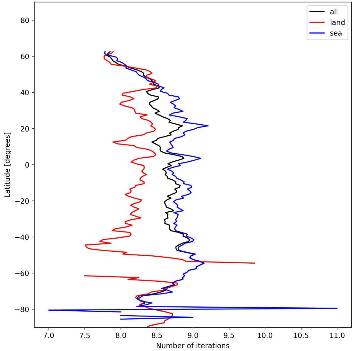
Figure 16: Zonal average of “Number of iterations” for 2024-12-06 to 2024-12-08.
