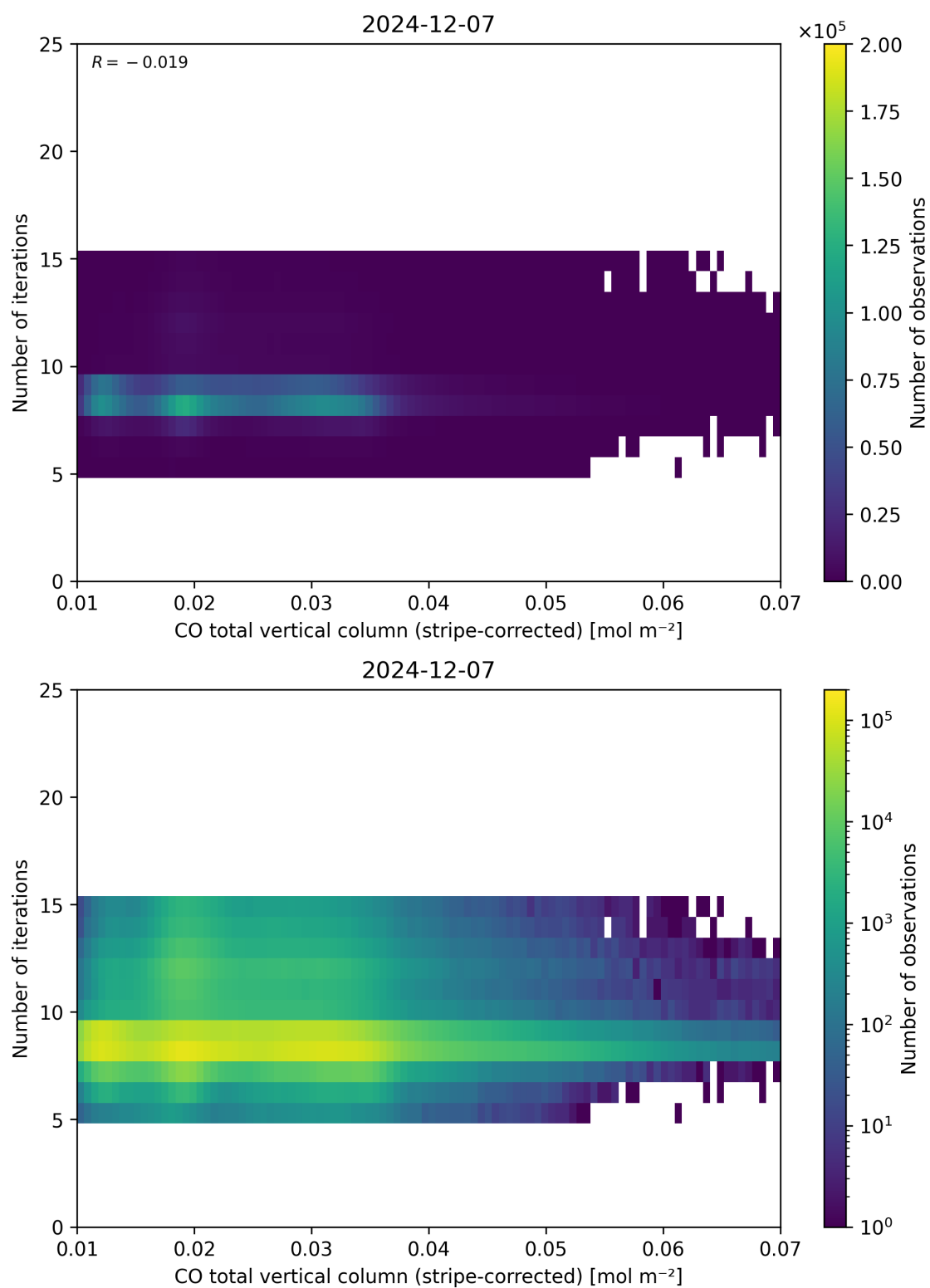
Figure 39: Scatter density plot of “CO total vertical column (stripe-corrected)” against “Number of iterations” for 2024-12-06 to 2024-12-08.
