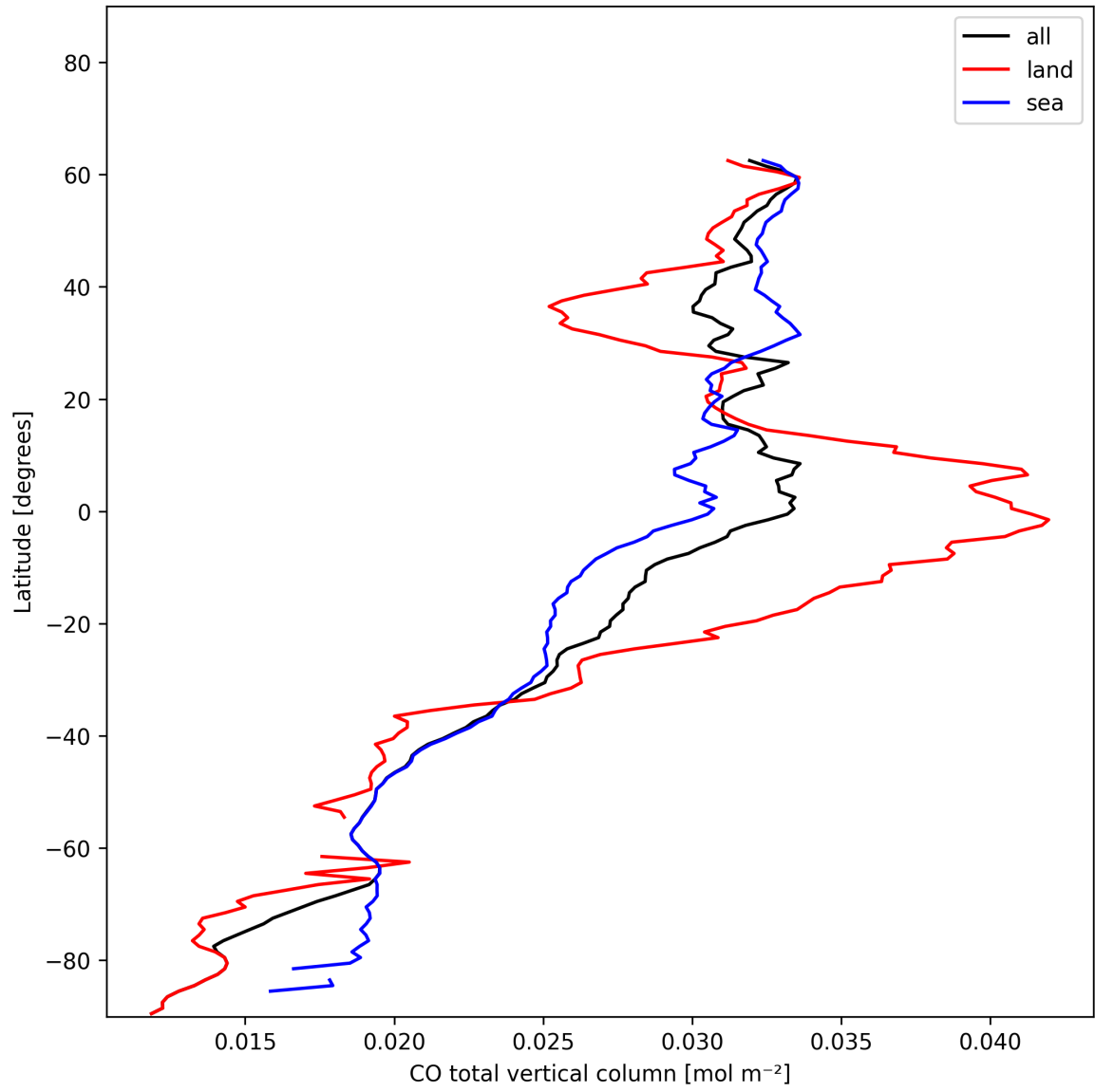
Figure 10: Zonal average of “CO total vertical column” for 2024-12-06 to 2024-12-08.
