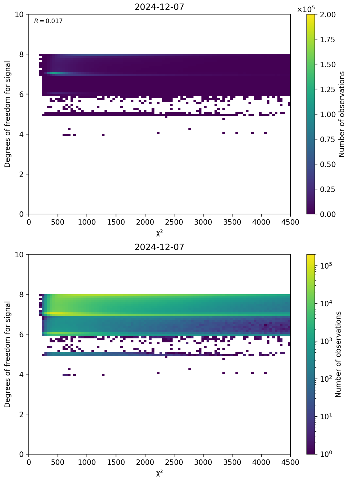
Figure 48: Scatter density plot of “ \chi^2 ” against “Degrees of freedom for signal” for 2024-12-06 to 2024-12-08.
