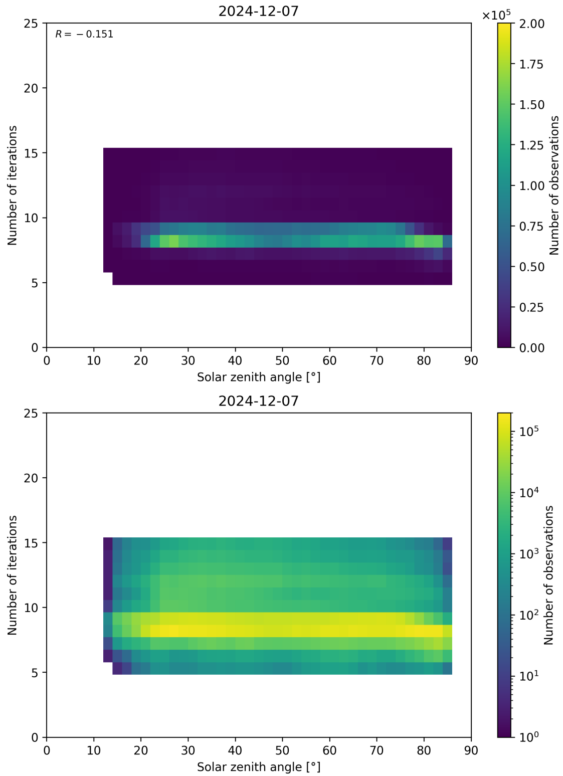
Figure 67: Scatter density plot of “Solar zenith angle” against “Number of iterations” for 2024-12-06 to 2024-12-08.
