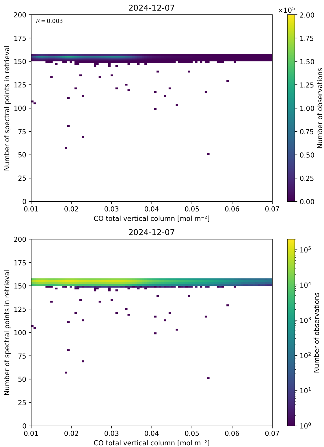
Figure 43: Scatter density plot of “CO total vertical column” against “Number of spectral points in retrieval” for 2024-12-06 to 2024-12-08.
