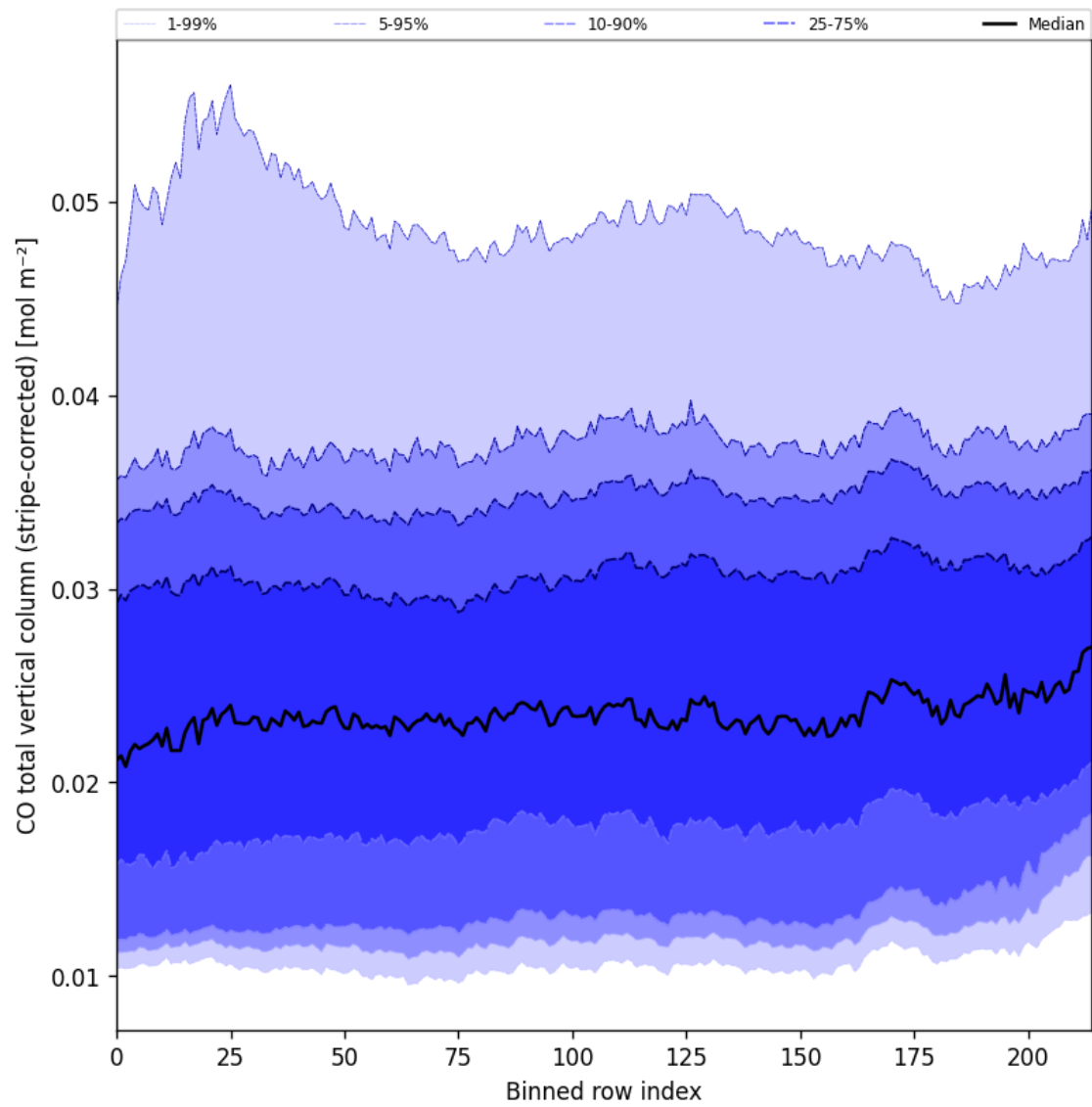
Figure 27: Along track statistics of “CO total vertical column (stripe-corrected)” for 2024-12-06 to 2024-12-08
