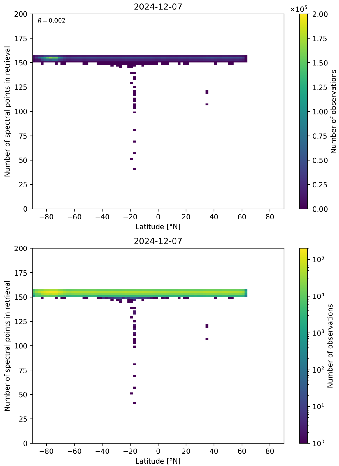
Figure 57: Scatter density plot of “Latitude” against “Number of spectral points in retrieval” for 2024-12-06 to 2024-12-08.
