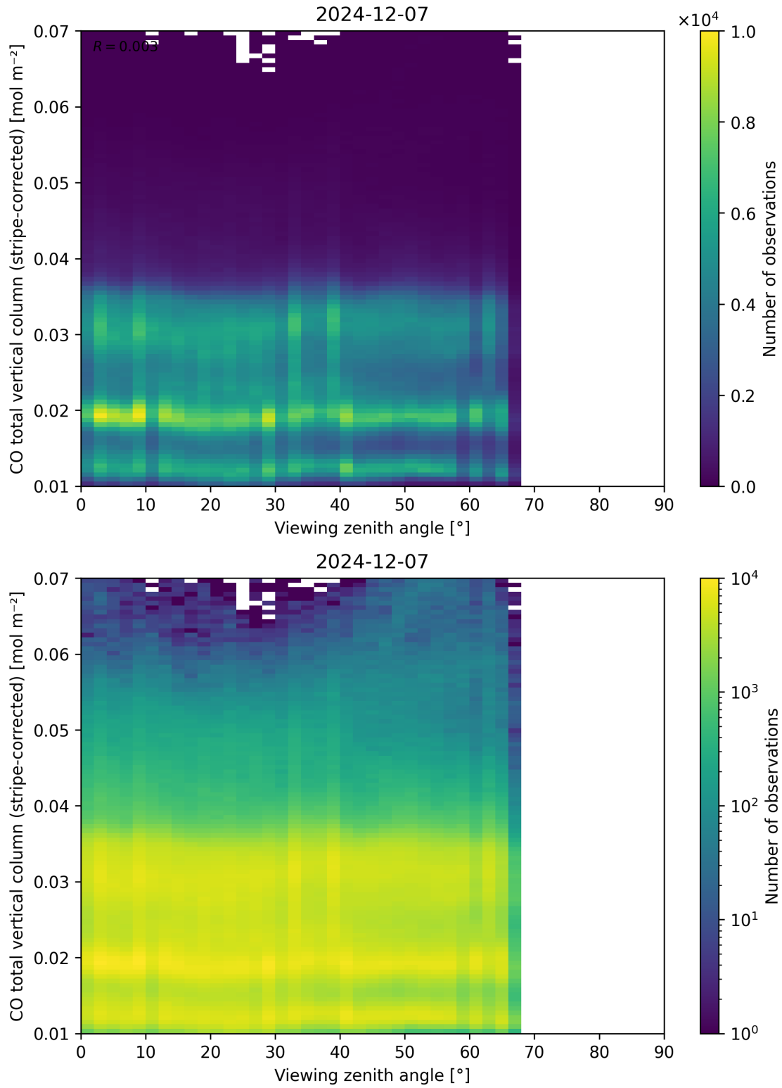
Figure 70: Scatter density plot of “Viewing zenith angle” against “CO total vertical column (stripe-corrected)” for 2024-12-06 to 2024-12-08.
