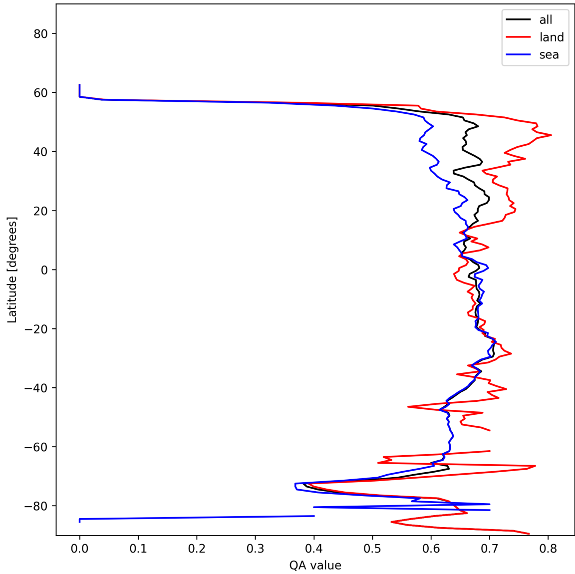
Figure 9: Zonal average of “QA value” for 2024-12-06 to 2024-12-08.
