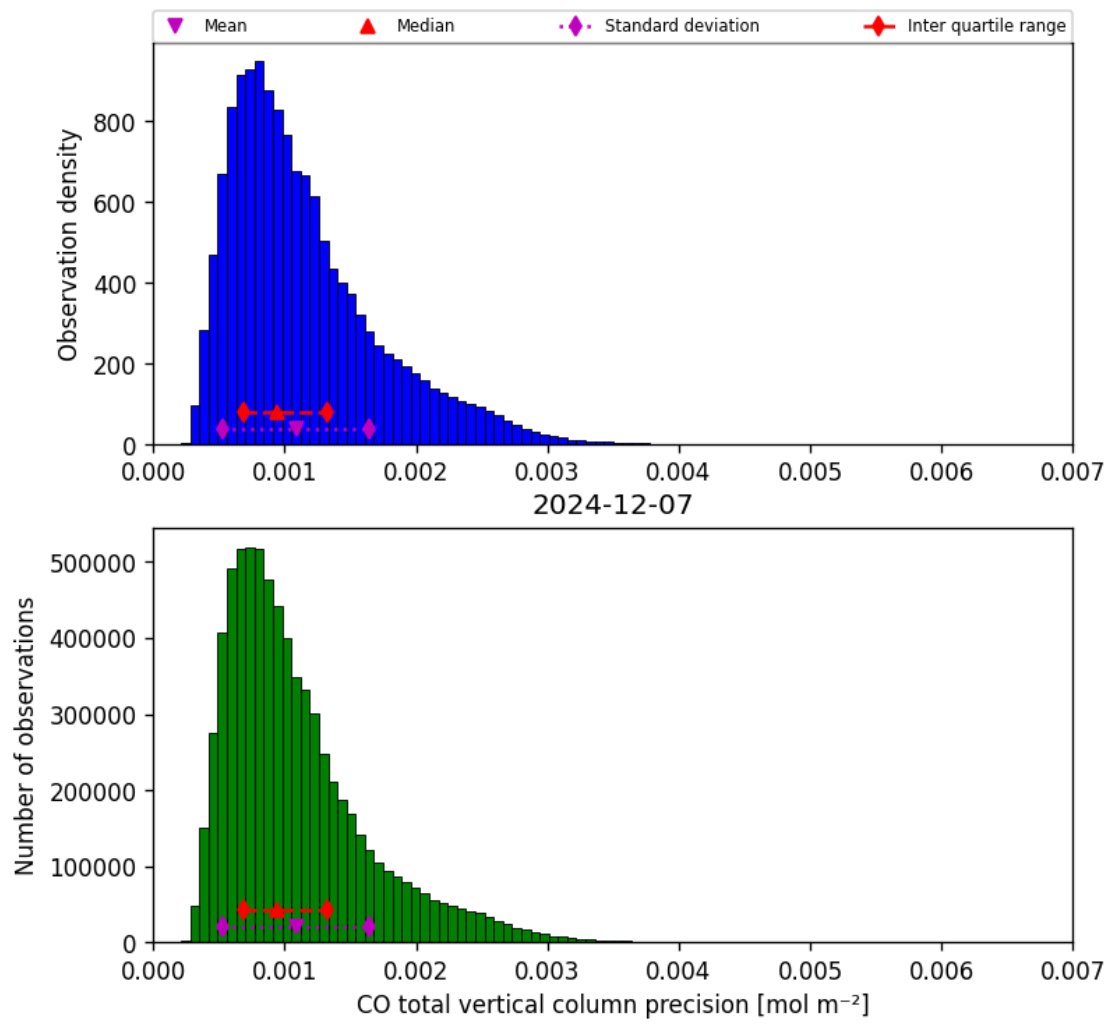
Figure 20: Histogram of “CO total vertical column precision” for 2024-12-06 to 2024-12-08
