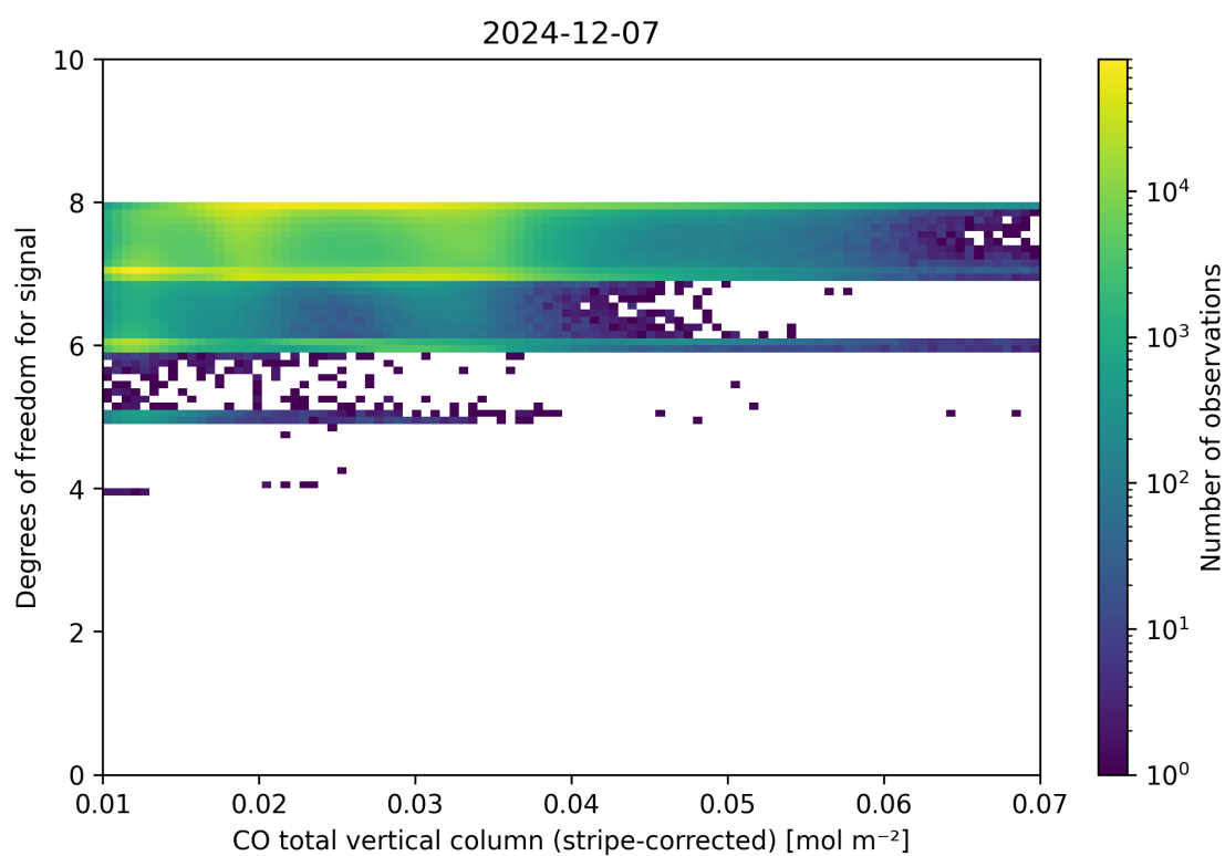
Figure 38: Scatter density plot of “CO total vertical column (stripe-corrected)” against “Degrees of freedom for signal” for 2024-12-06 to 2024-12-08.
