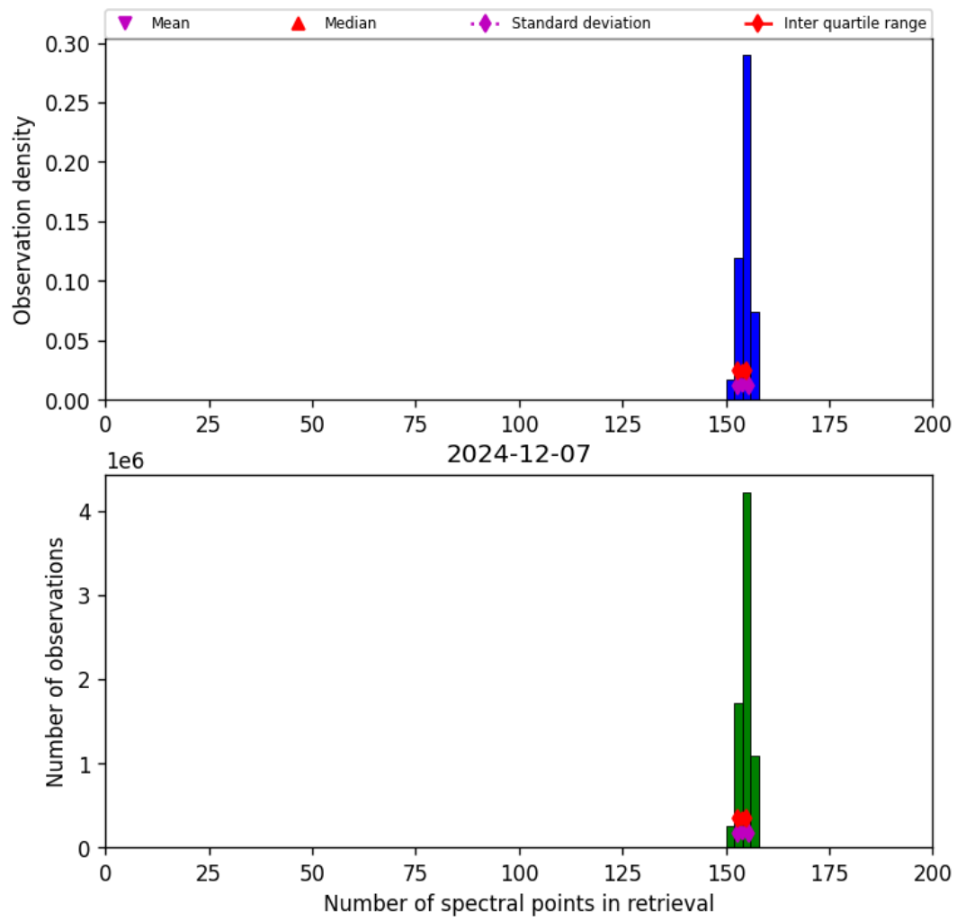
Figure 21: Histogram of “Number of spectral points in retrieval” for 2024-12-06 to 2024-12-08
