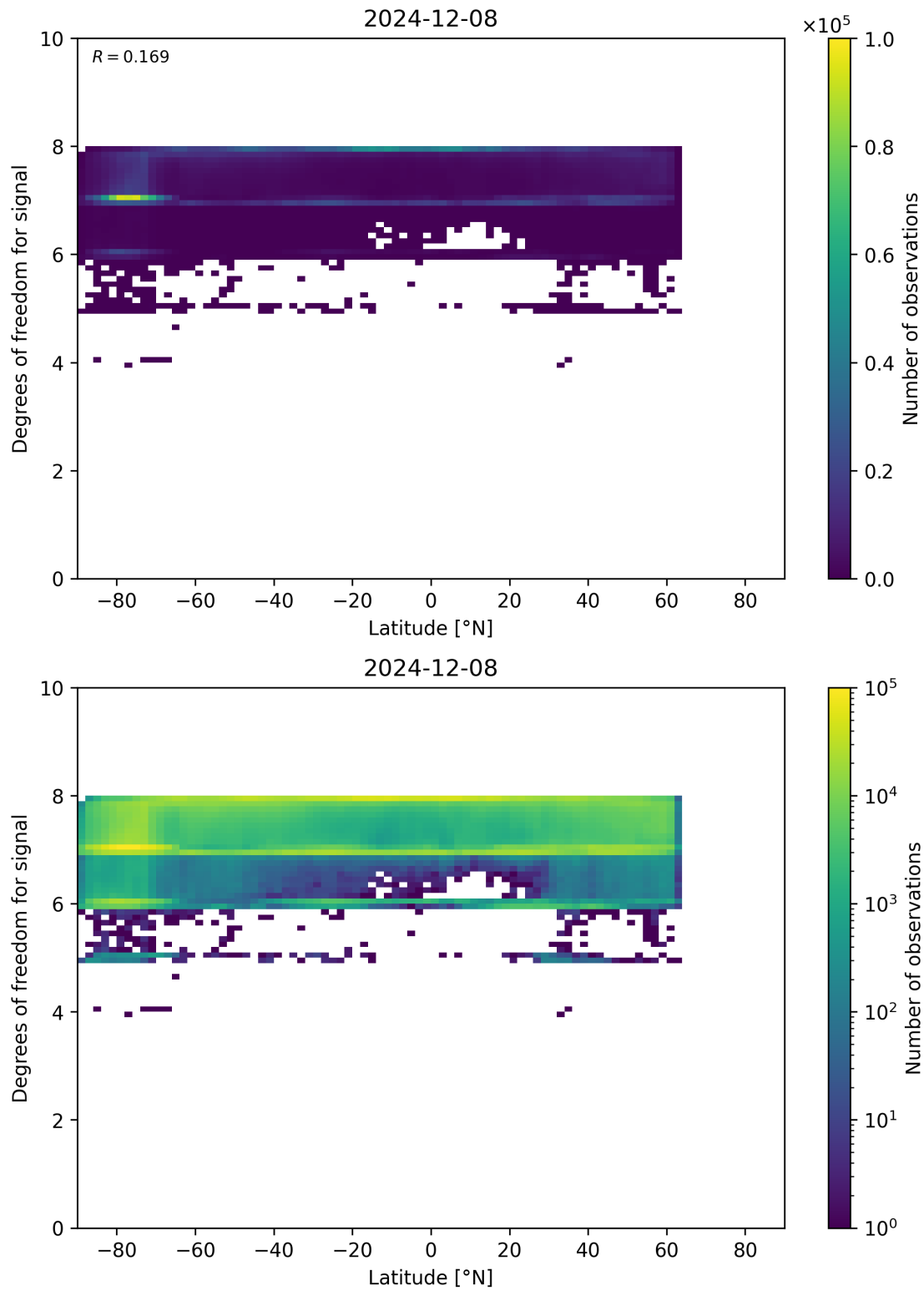
Figure 55: Scatter density plot of “Latitude” against “Degrees of freedom for signal” for 2024-12-07 to 2024-12-09.
