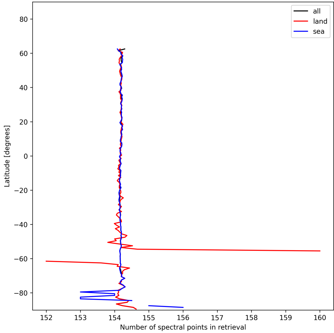
Figure 13: Zonal average of “Number of spectral points in retrieval” for 2024-12-07 to 2024-12-09.
