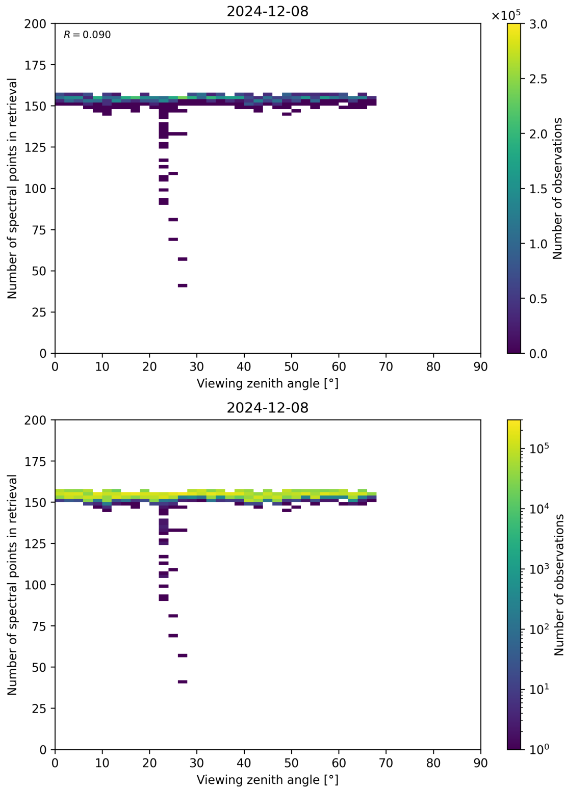
Figure 76: Scatter density plot of “Viewing zenith angle” against “Number of spectral points in retrieval” for 2024-12-07 to 2024-12-09.
