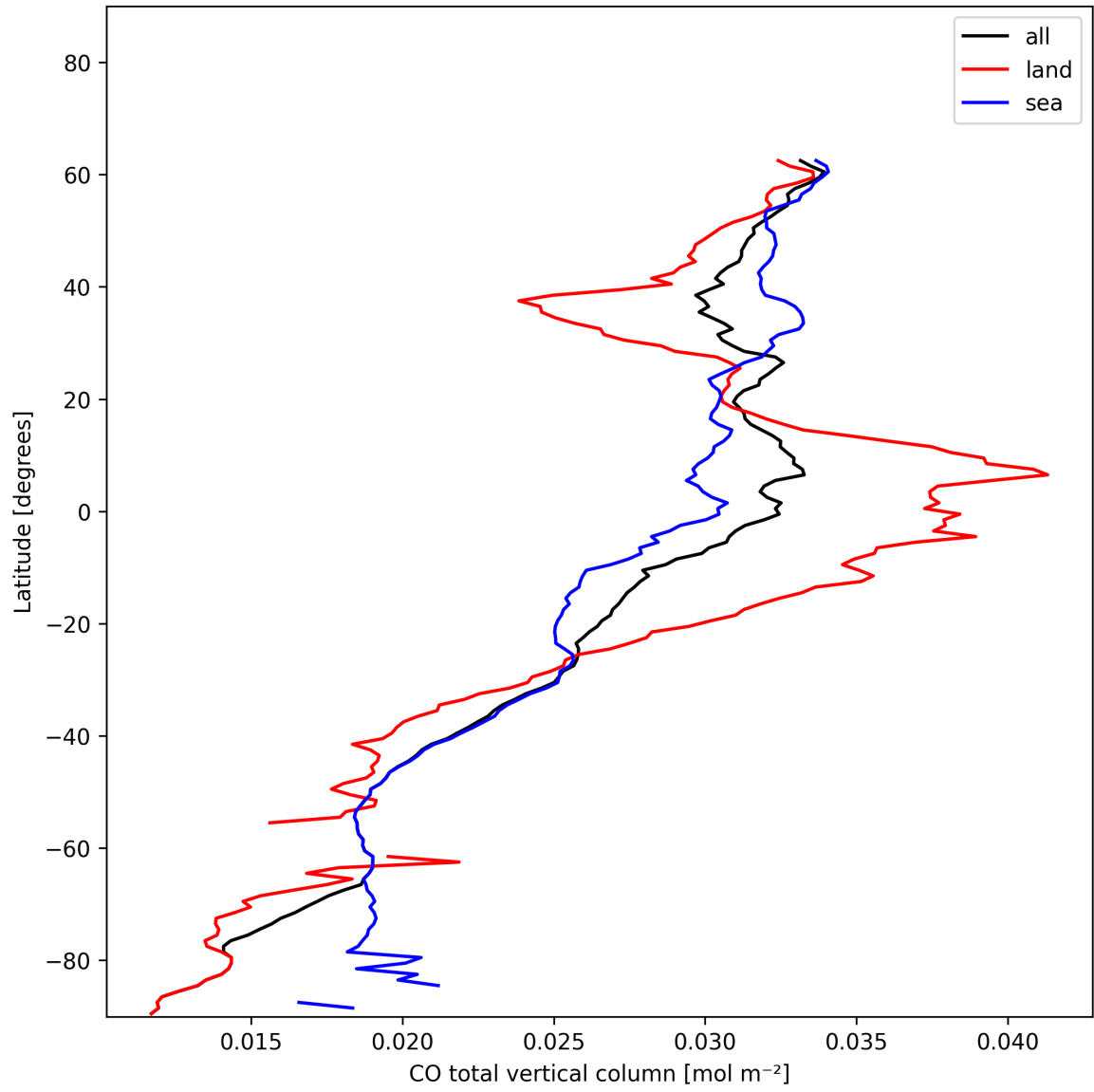
Figure 10: Zonal average of “CO total vertical column” for 2024-12-07 to 2024-12-09.
