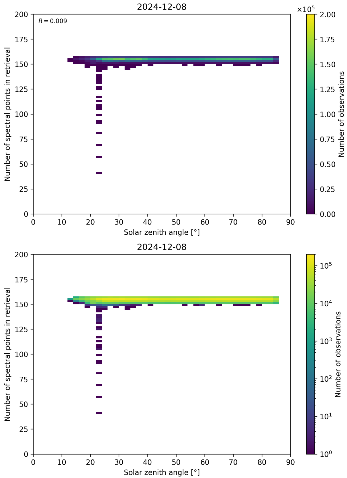
Figure 68: Scatter density plot of “Solar zenith angle” against “Number of spectral points in retrieval” for 2024-12-07 to 2024-12-09.
