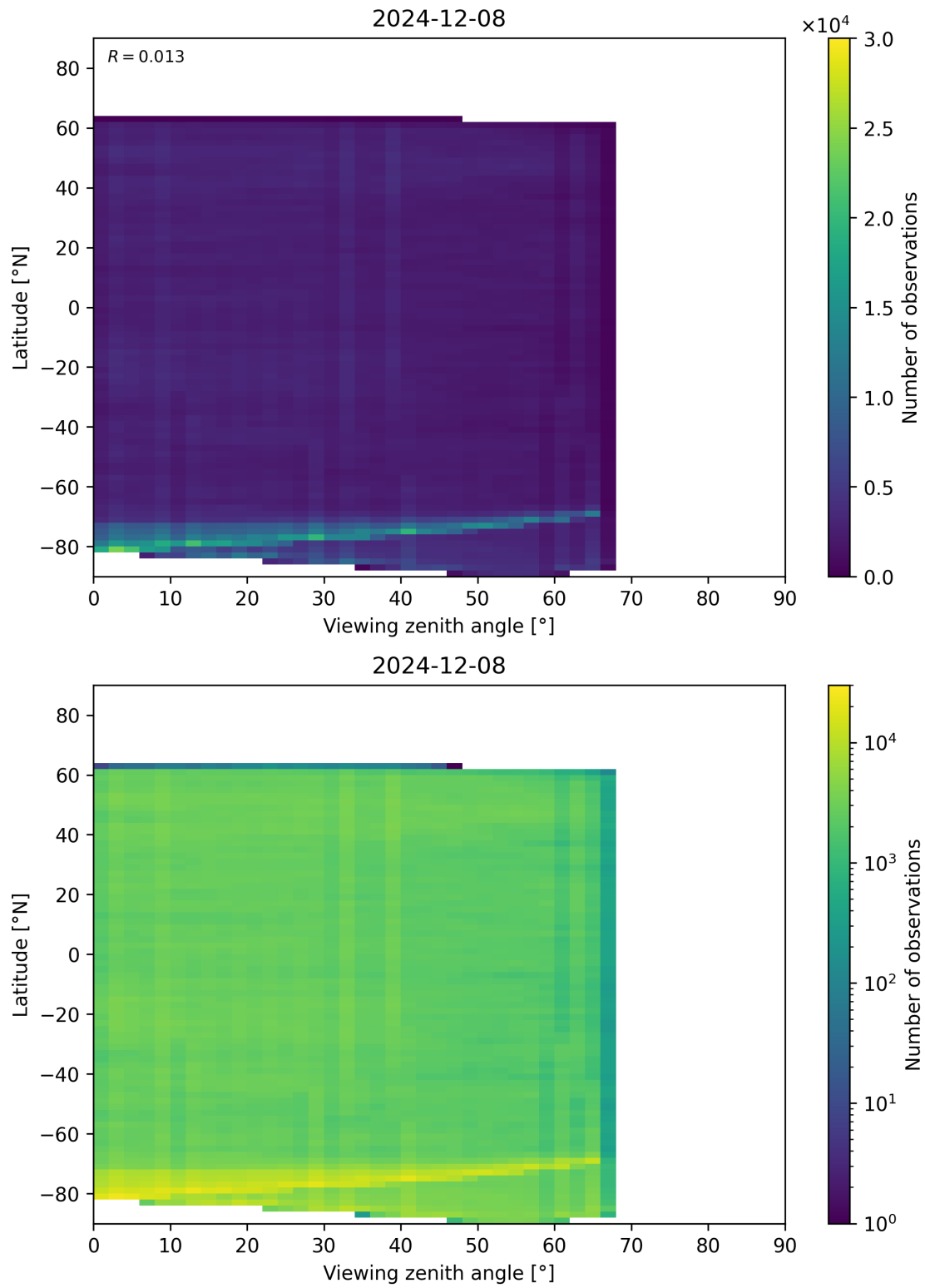
Figure 74: Scatter density plot of “Viewing zenith angle” against “Latitude” for 2024-12-07 to 2024-12-09.
