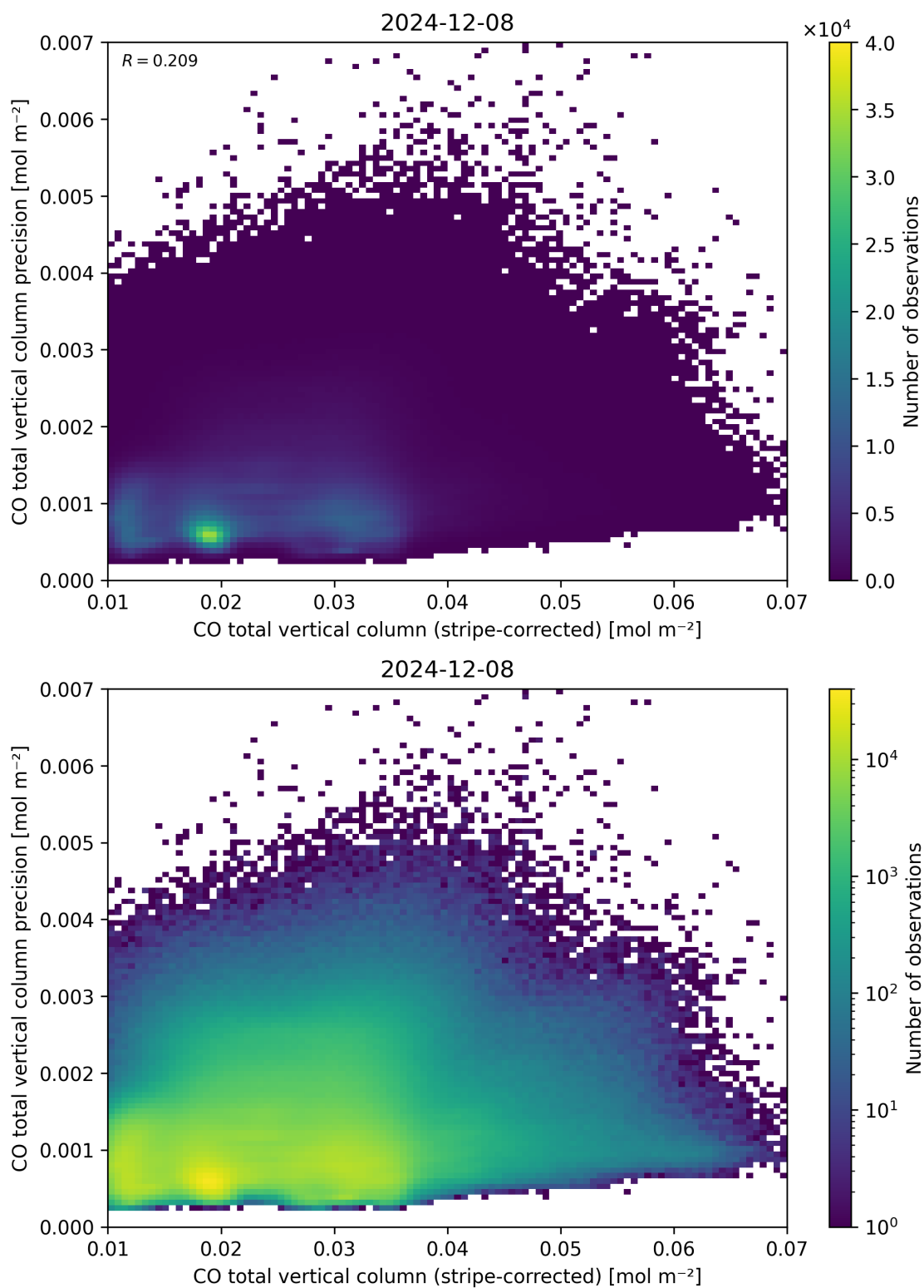
Figure 36: Scatter density plot of “CO total vertical column (stripe-corrected)” against “CO total vertical column precision” for 2024-12-07 to 2024-12-09.
