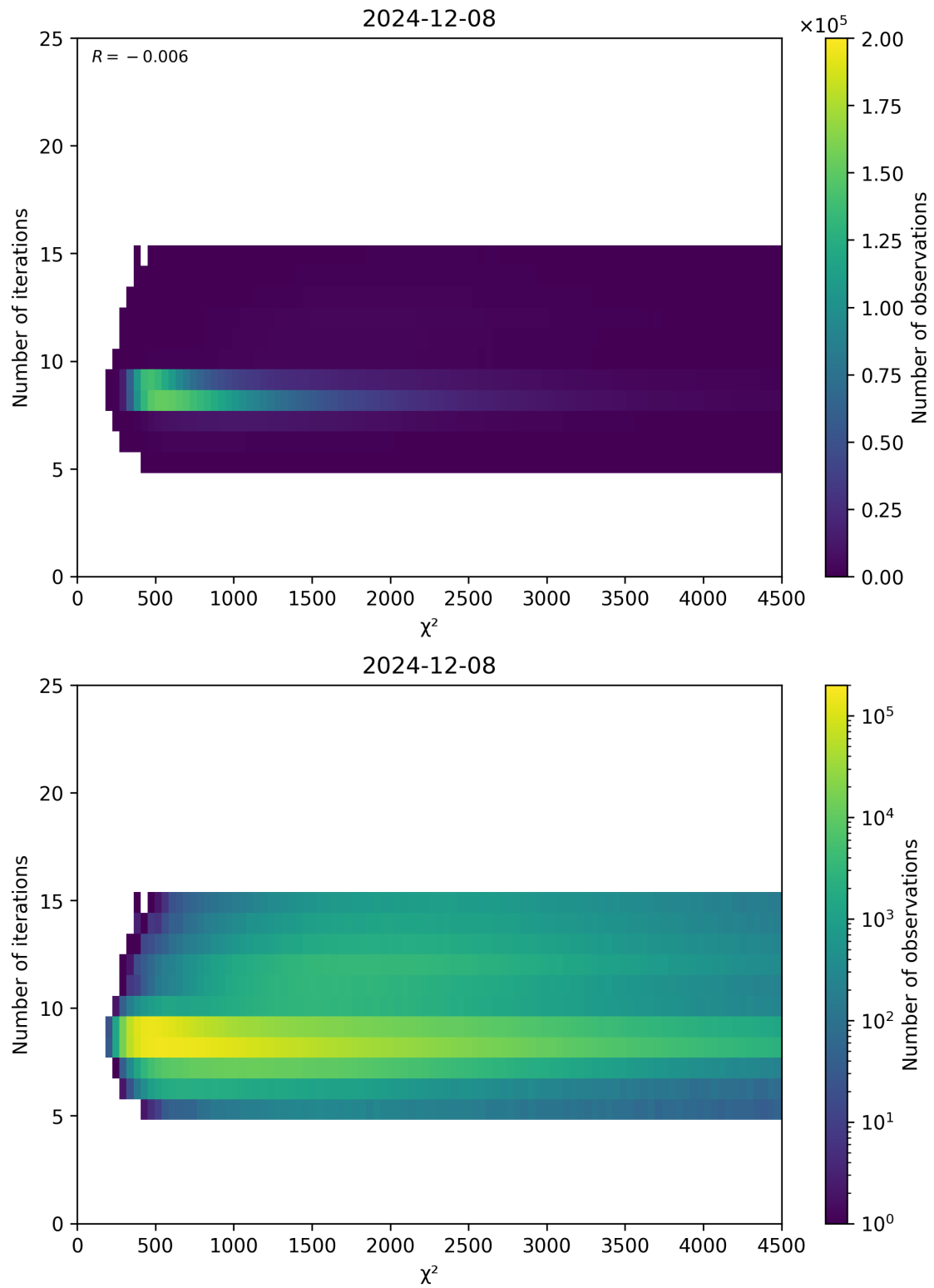
Figure 49: Scatter density plot of “ \chi^2 ” against “Number of iterations” for 2024-12-07 to 2024-12-09.
