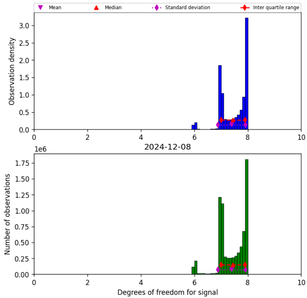
Figure 23: Histogram of “Degrees of freedom for signal” for 2024-12-07 to 2024-12-09
