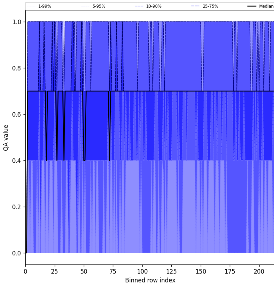
Figure 25: Along track statistics of “QA value” for 2024-12-07 to 2024-12-09
