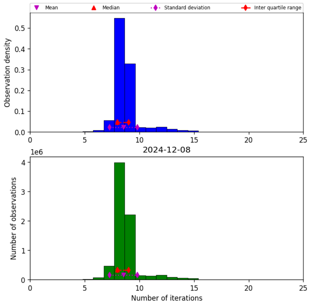
Figure 24: Histogram of “Number of iterations” for 2024-12-07 to 2024-12-09
