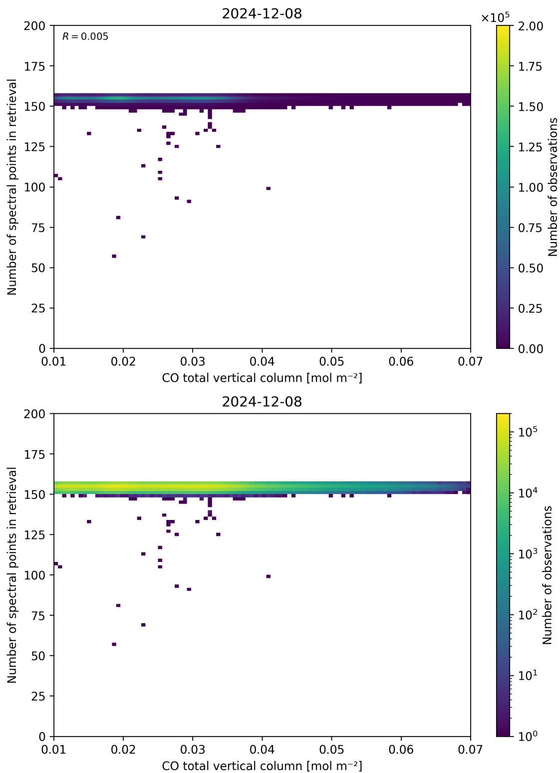
Figure 43: Scatter density plot of “CO total vertical column” against “Number of spectral points in retrieval” for 2024-12-07 to 2024-12-09.
