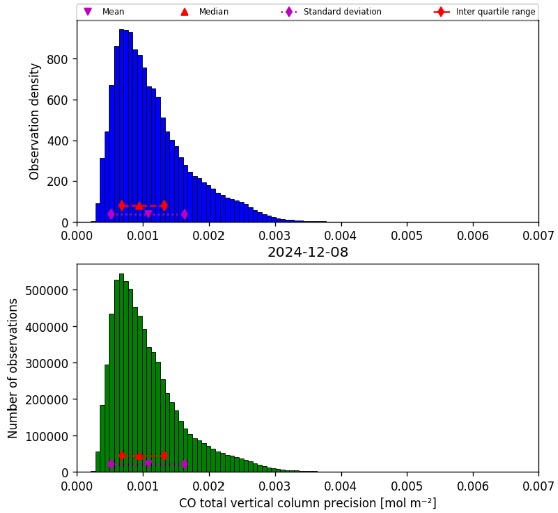
Figure 20: Histogram of “CO total vertical column precision” for 2024-12-07 to 2024-12-09
