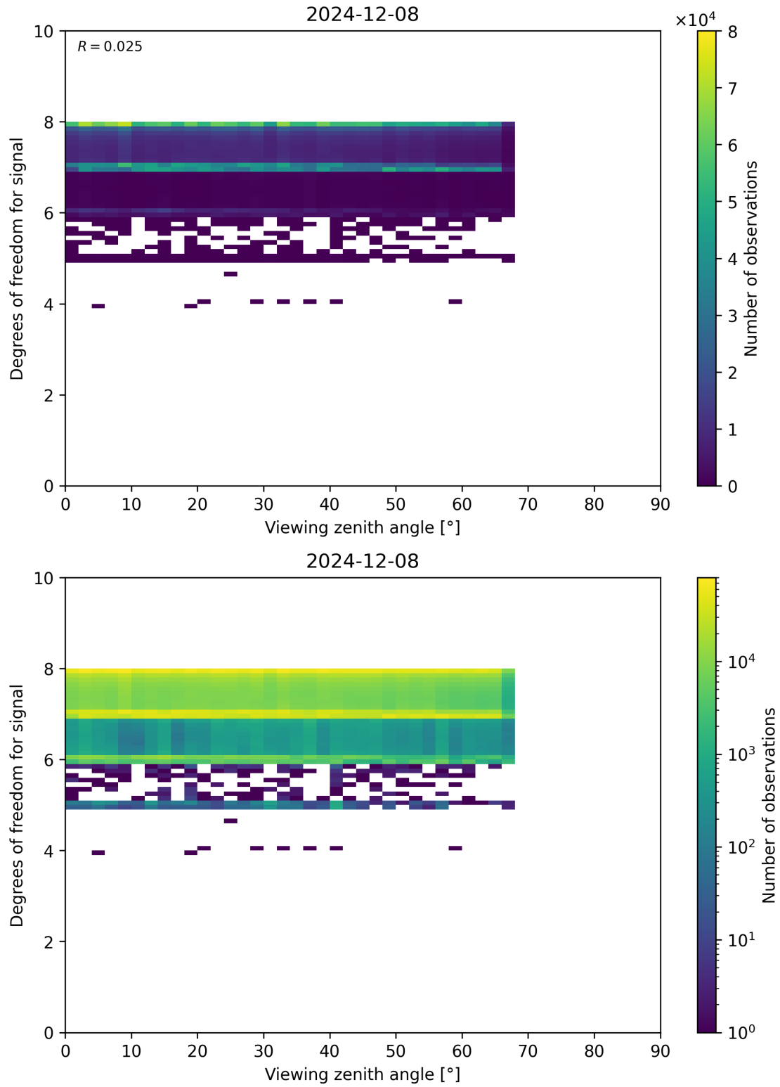
Figure 73: Scatter density plot of “Viewing zenith angle” against “Degrees of freedom for signal” for 2024-12-07 to 2024-12-09.
