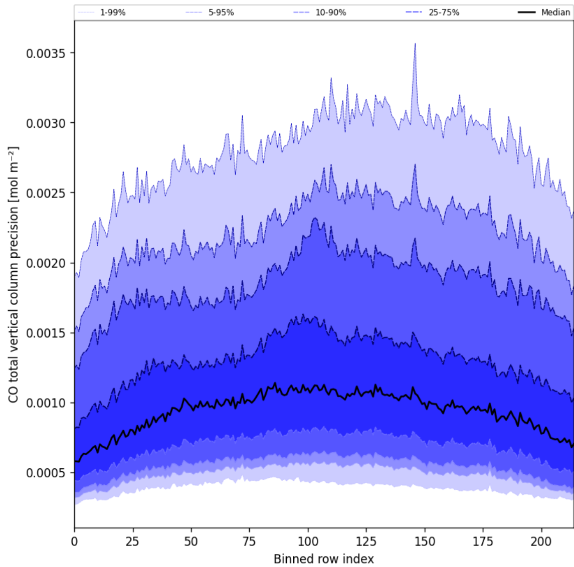
Figure 28: Along track statistics of “CO total vertical column precision” for 2024-12-07 to 2024-12-09
