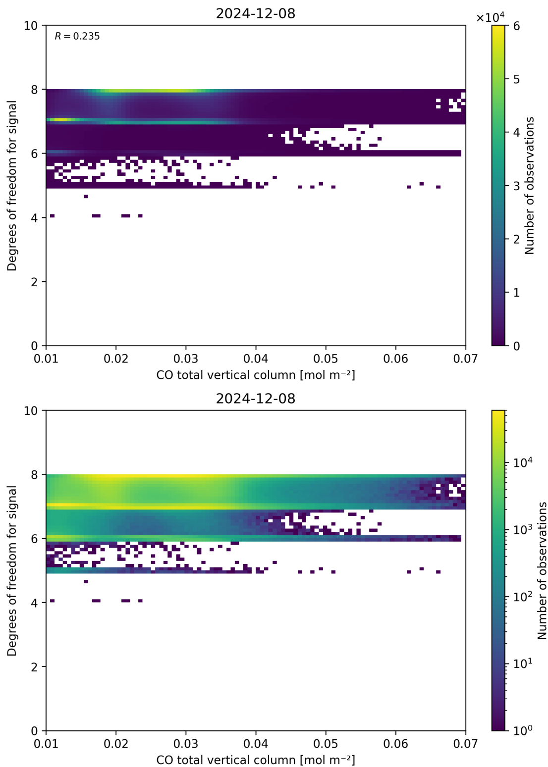
Figure 41: Scatter density plot of “CO total vertical column” against “Degrees of freedom for signal” for 2024-12-07 to 2024-12-09.
