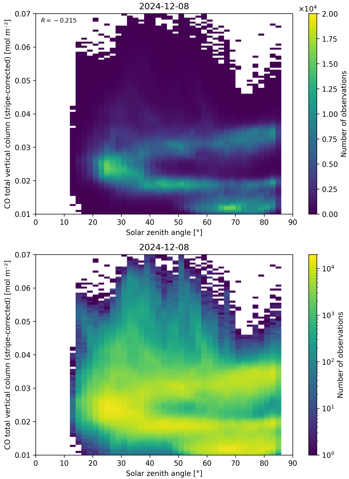
Figure 62: Scatter density plot of “Solar zenith angle” against “CO total vertical column (stripe-corrected)” for 2024-12-07 to 2024-12-09.
