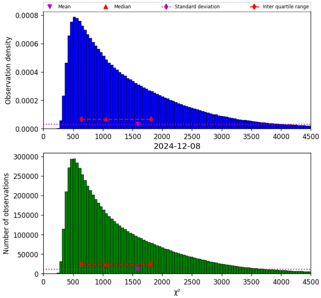
Figure 22: Histogram of " \chi^2 " for 2024-12-07 to 2024-12-09
