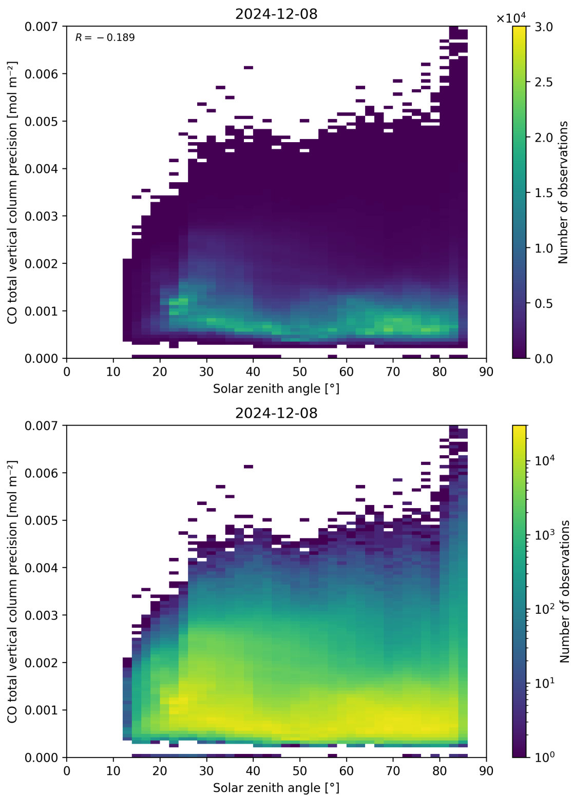
Figure 63: Scatter density plot of “Solar zenith angle” against “CO total vertical column precision” for 2024-12-07 to 2024-12-09.
