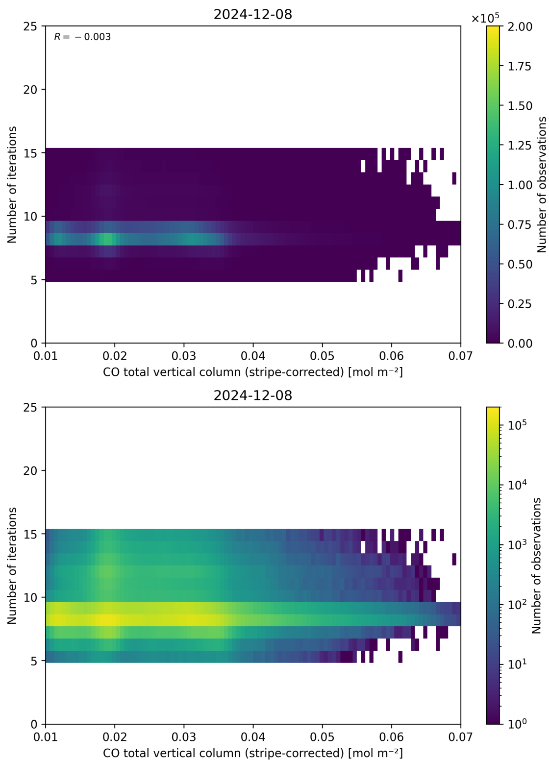
Figure 39: Scatter density plot of “CO total vertical column (stripe-corrected)” against “Number of iterations” for 2024-12-07 to 2024-12-09.
