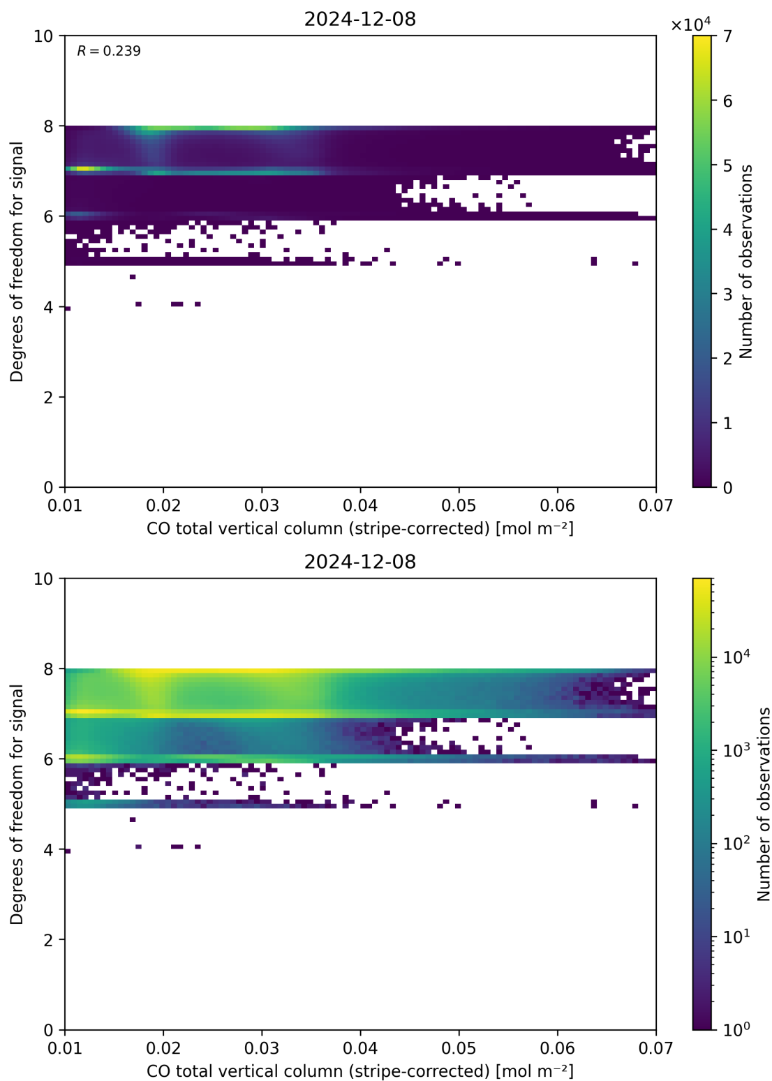
Figure 38: Scatter density plot of “CO total vertical column (stripe-corrected)” against “Degrees of freedom for signal” for 2024-12-07 to 2024-12-09.
