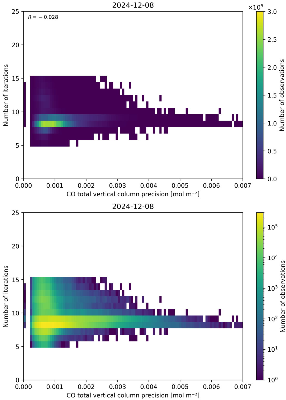
Figure 46: Scatter density plot of “CO total vertical column precision” against “Number of iterations” for 2024-12-07 to 2024-12-09.
