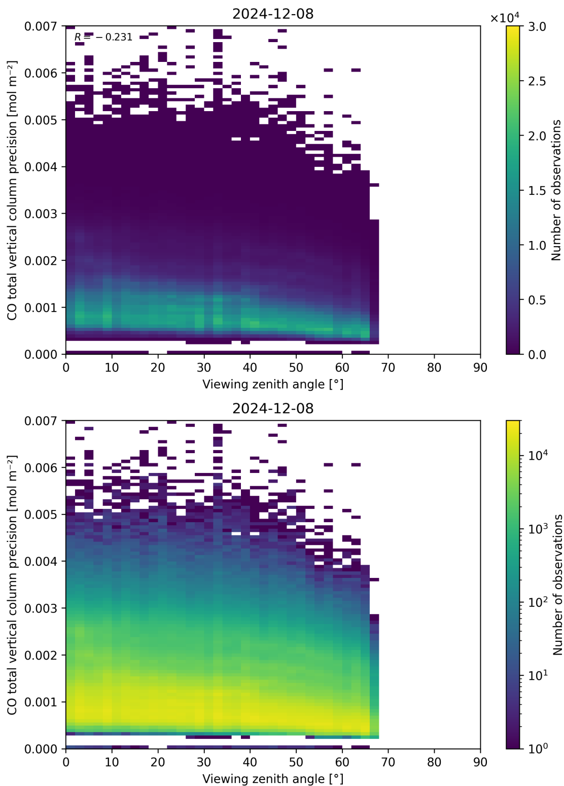
Figure 71: Scatter density plot of “Viewing zenith angle” against “CO total vertical column precision” for 2024-12-07 to 2024-12-09.
