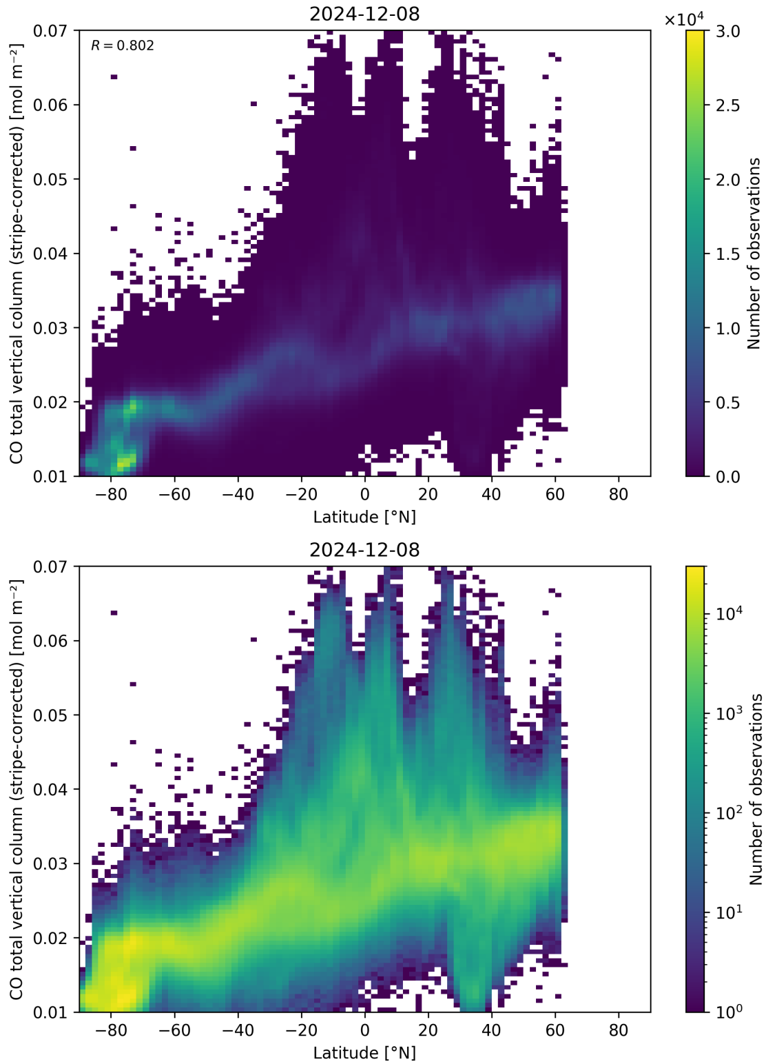
Figure 52: Scatter density plot of “Latitude” against “CO total vertical column (stripe-corrected)” for 2024-12-07 to 2024-12-09.
