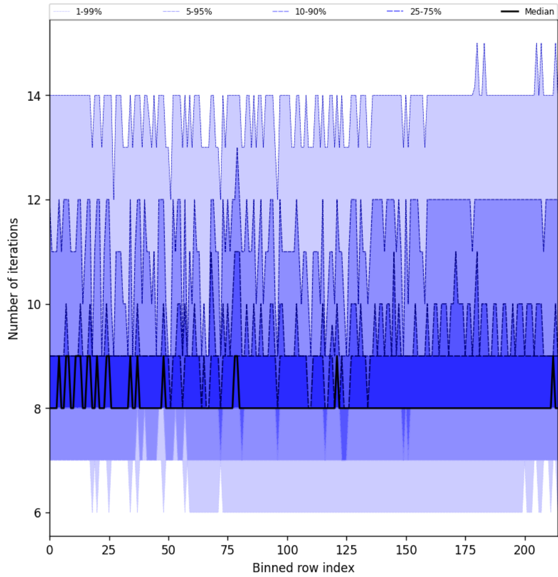
Figure 32: Along track statistics of “Number of iterations” for 2024-12-07 to 2024-12-09
