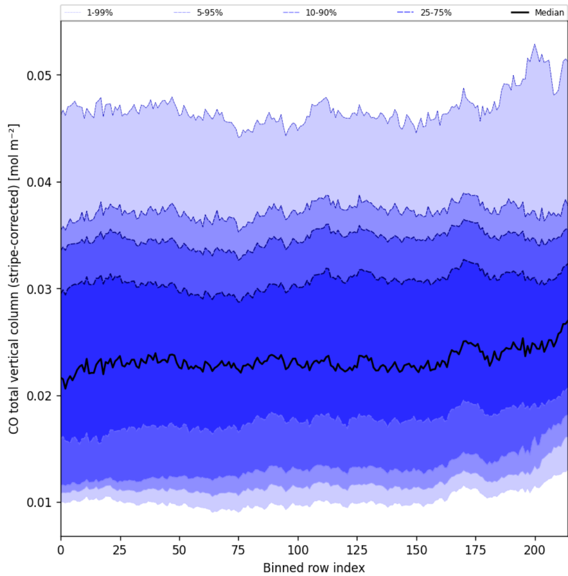
Figure 27: Along track statistics of “CO total vertical column (stripe-corrected)” for 2024-12-07 to 2024-12-09
