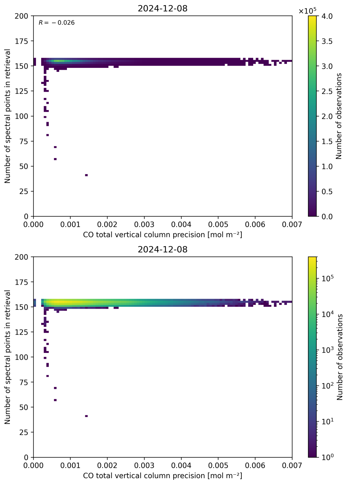
Figure 47: Scatter density plot of “CO total vertical column precision” against “Number of spectral points in retrieval” for 2024-12-07 to 2024-12-09.
