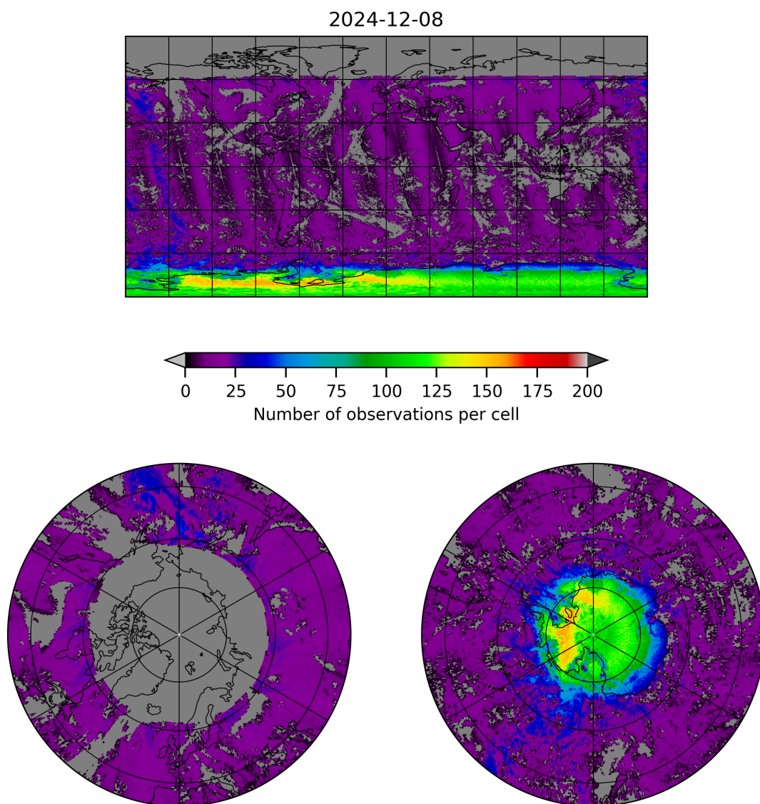
Figure 8: Map of the number of observations for 2024-12-07 to 2024-12-09
