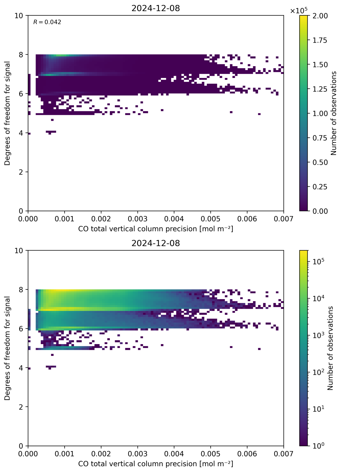
Figure 45: Scatter density plot of “CO total vertical column precision” against “Degrees of freedom for signal” for 2024-12-07 to 2024-12-09.
