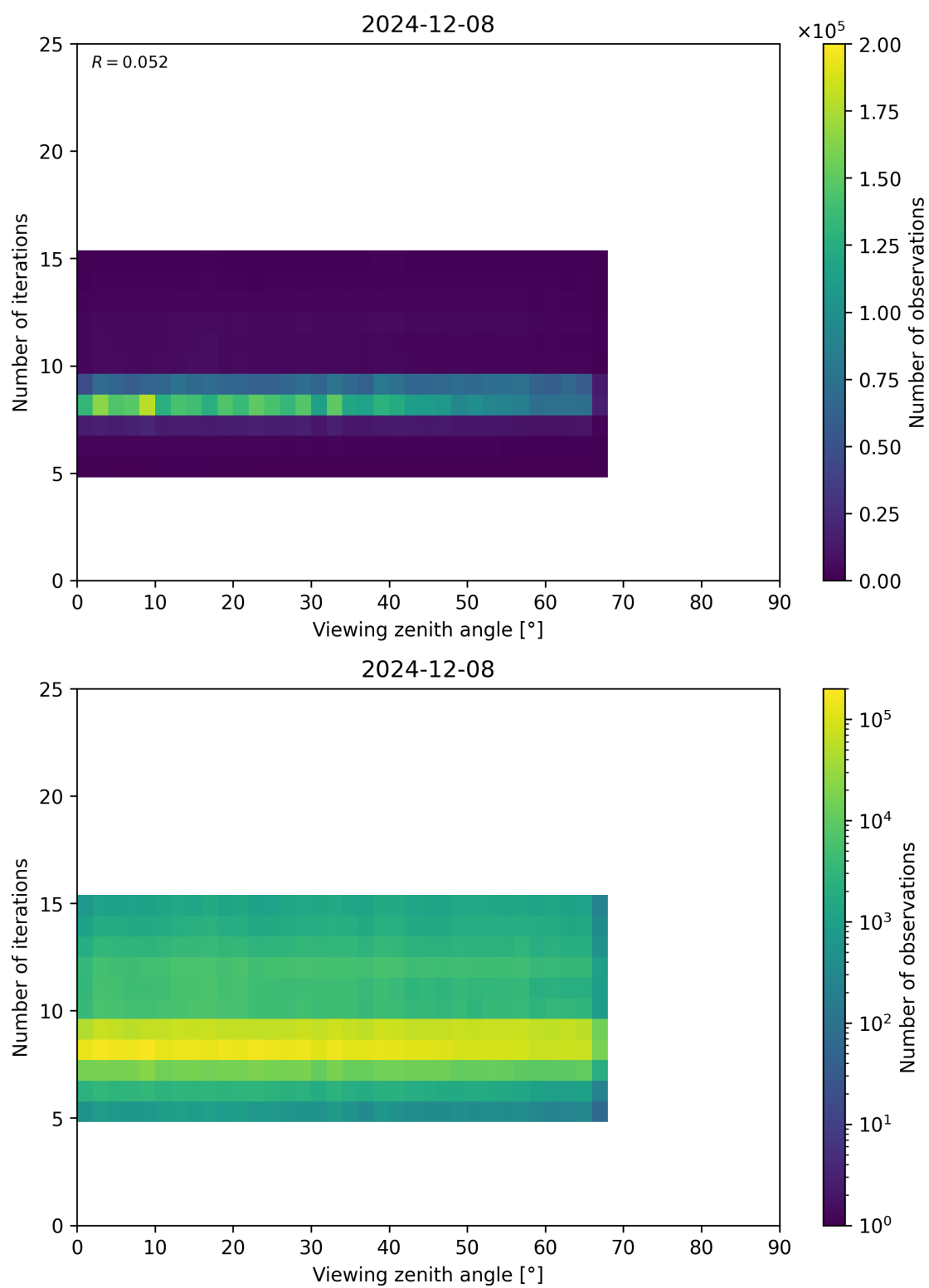
Figure 75: Scatter density plot of “Viewing zenith angle” against “Number of iterations” for 2024-12-07 to 2024-12-09.
