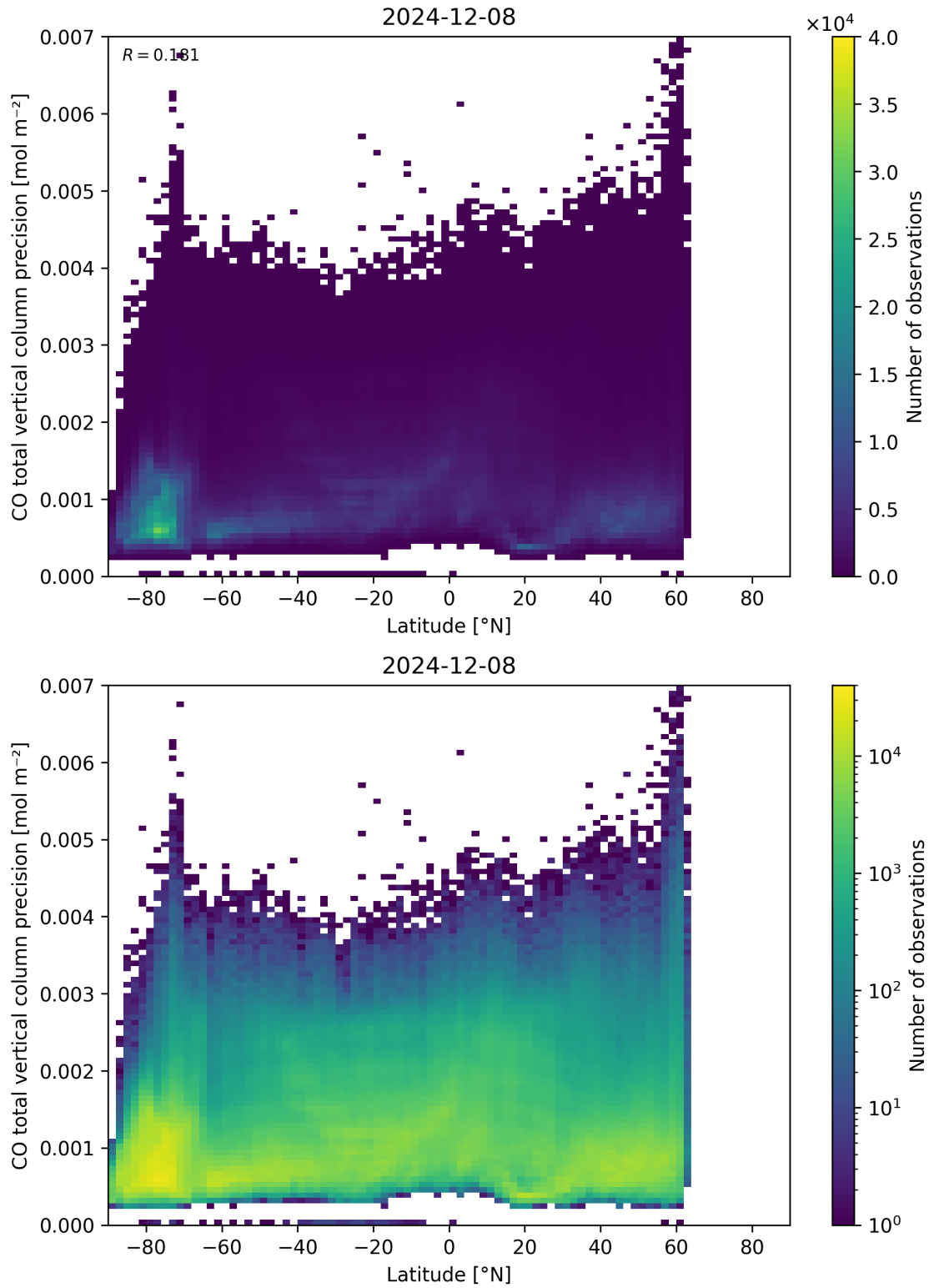
Figure 53: Scatter density plot of “Latitude” against “CO total vertical column precision” for 2024-12-07 to 2024-12-09.
