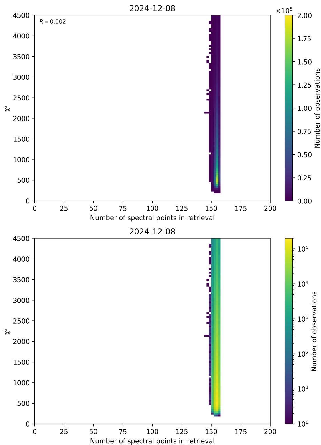
Figure 58: Scatter density plot of “Number of spectral points in retrieval” against “ \chi^2 ” for 2024-12-07 to 2024-12-09.
