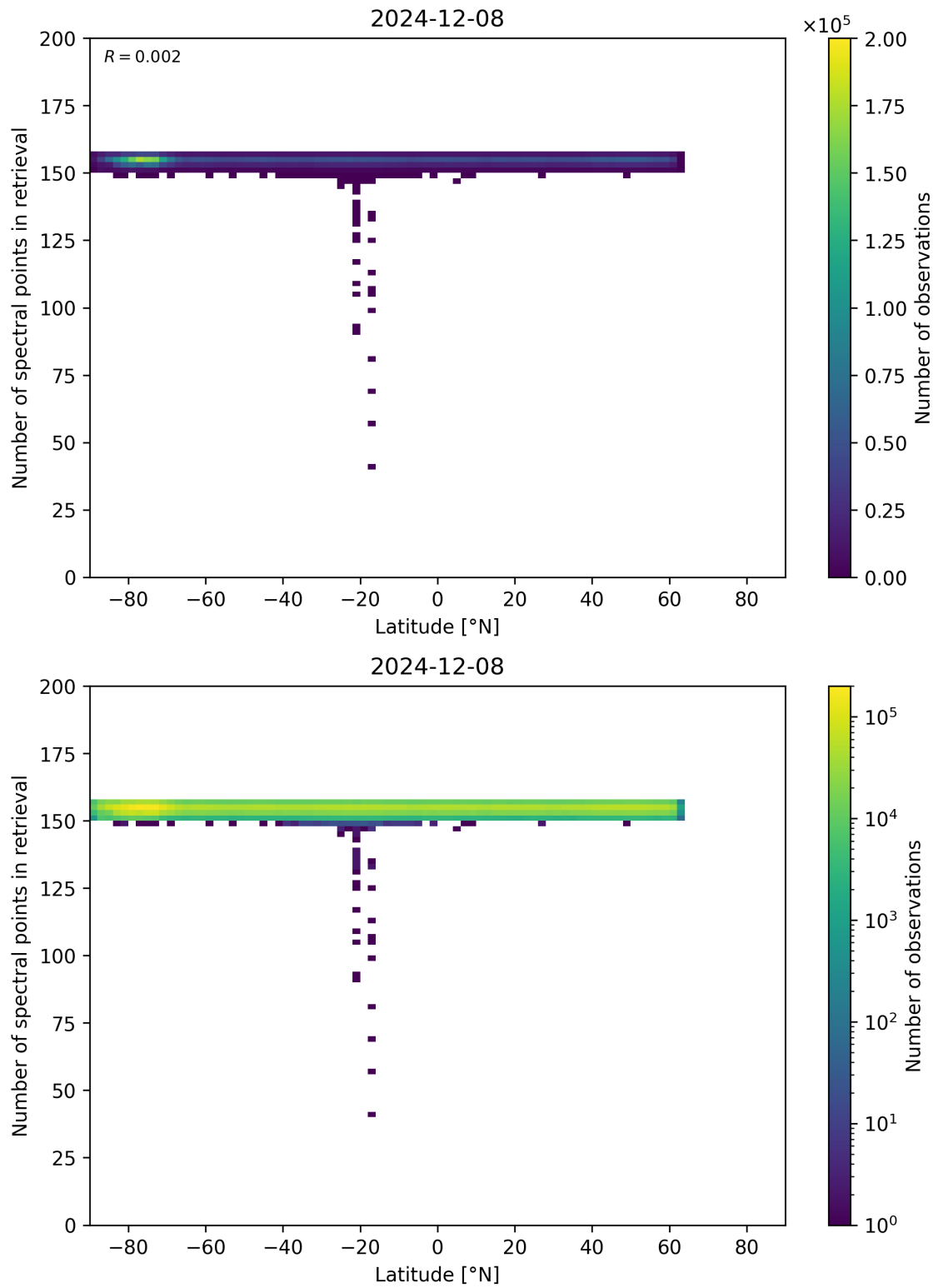
Figure 57: Scatter density plot of “Latitude” against “Number of spectral points in retrieval” for 2024-12-07 to 2024-12-09.
