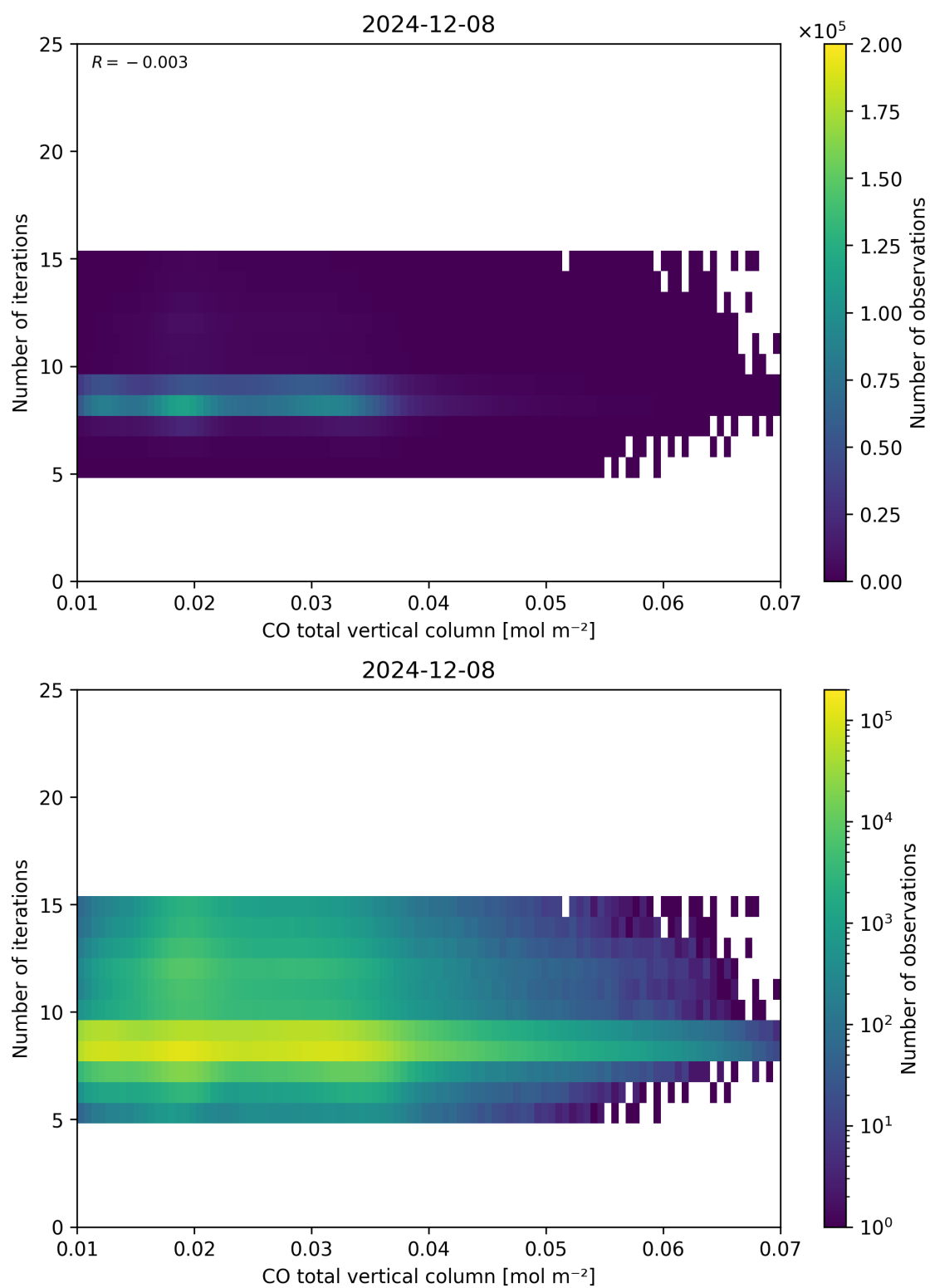
Figure 42: Scatter density plot of “CO total vertical column” against “Number of iterations” for 2024-12-07 to 2024-12-09.
