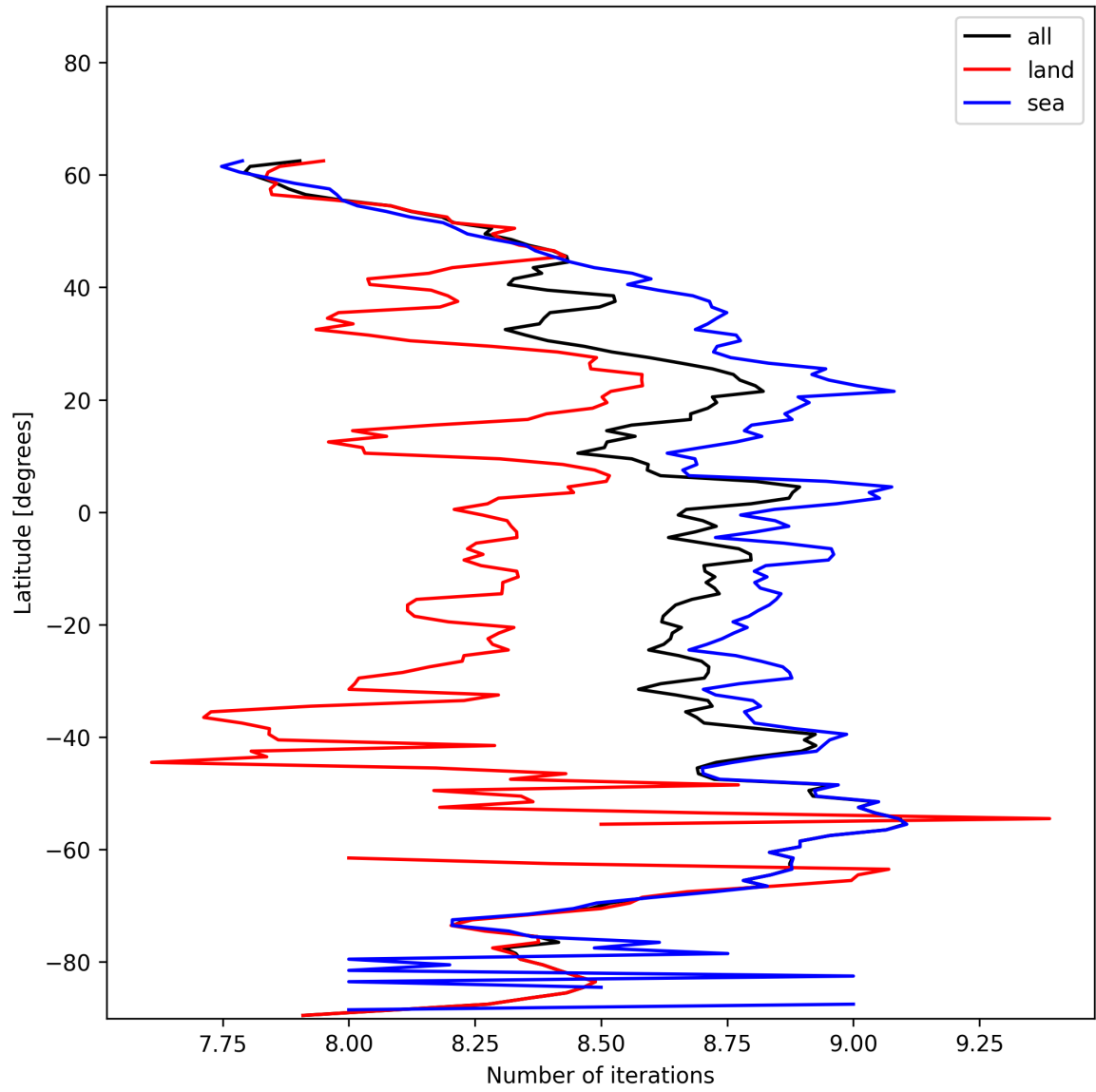
Figure 16: Zonal average of “Number of iterations” for 2024-12-07 to 2024-12-09.
