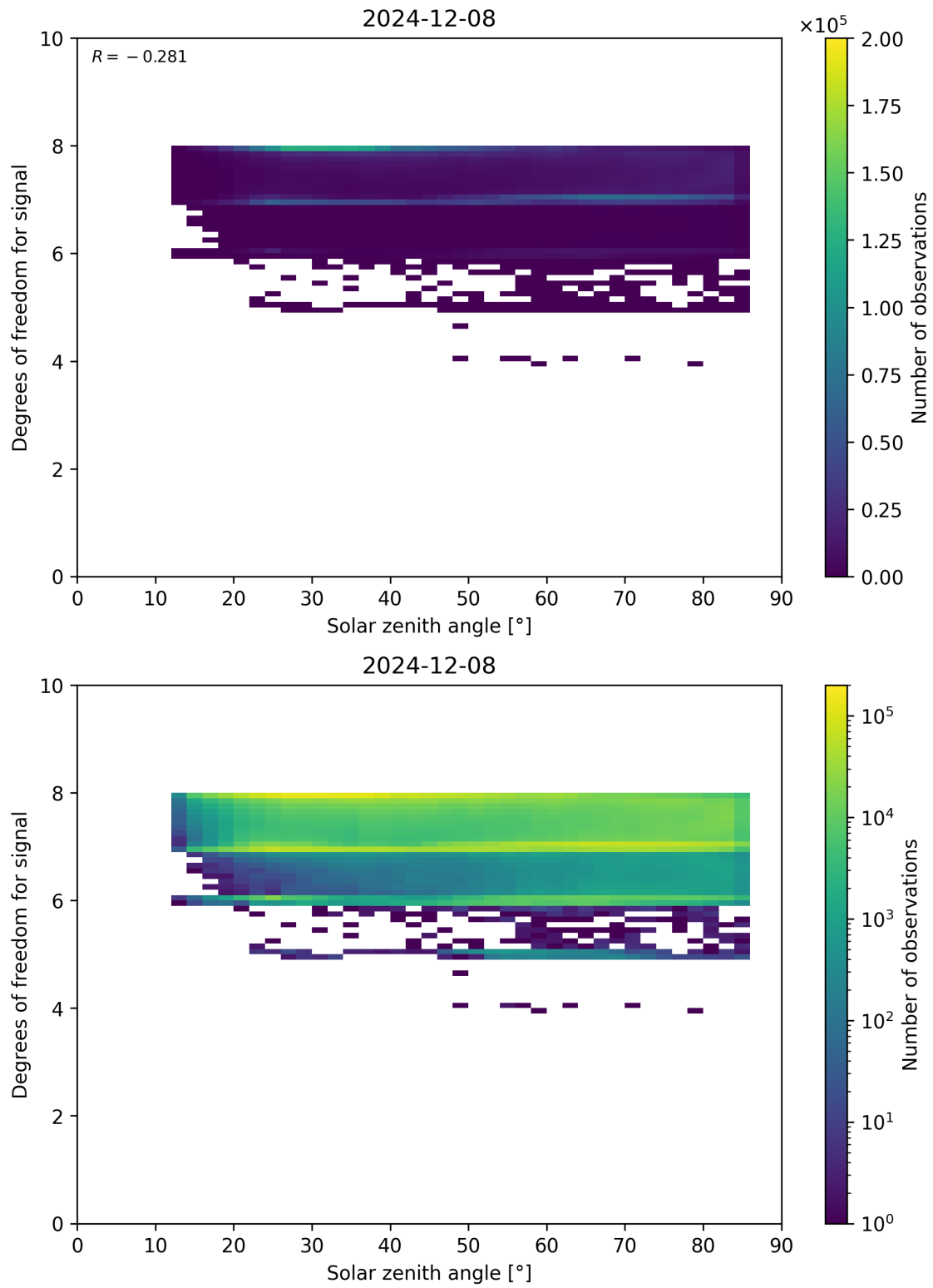
Figure 65: Scatter density plot of “Solar zenith angle” against “Degrees of freedom for signal” for 2024-12-07 to 2024-12-09.
