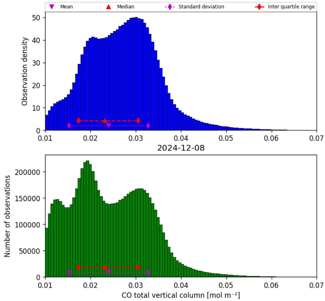
Figure 18: Histogram of “CO total vertical column” for 2024-12-07 to 2024-12-09
