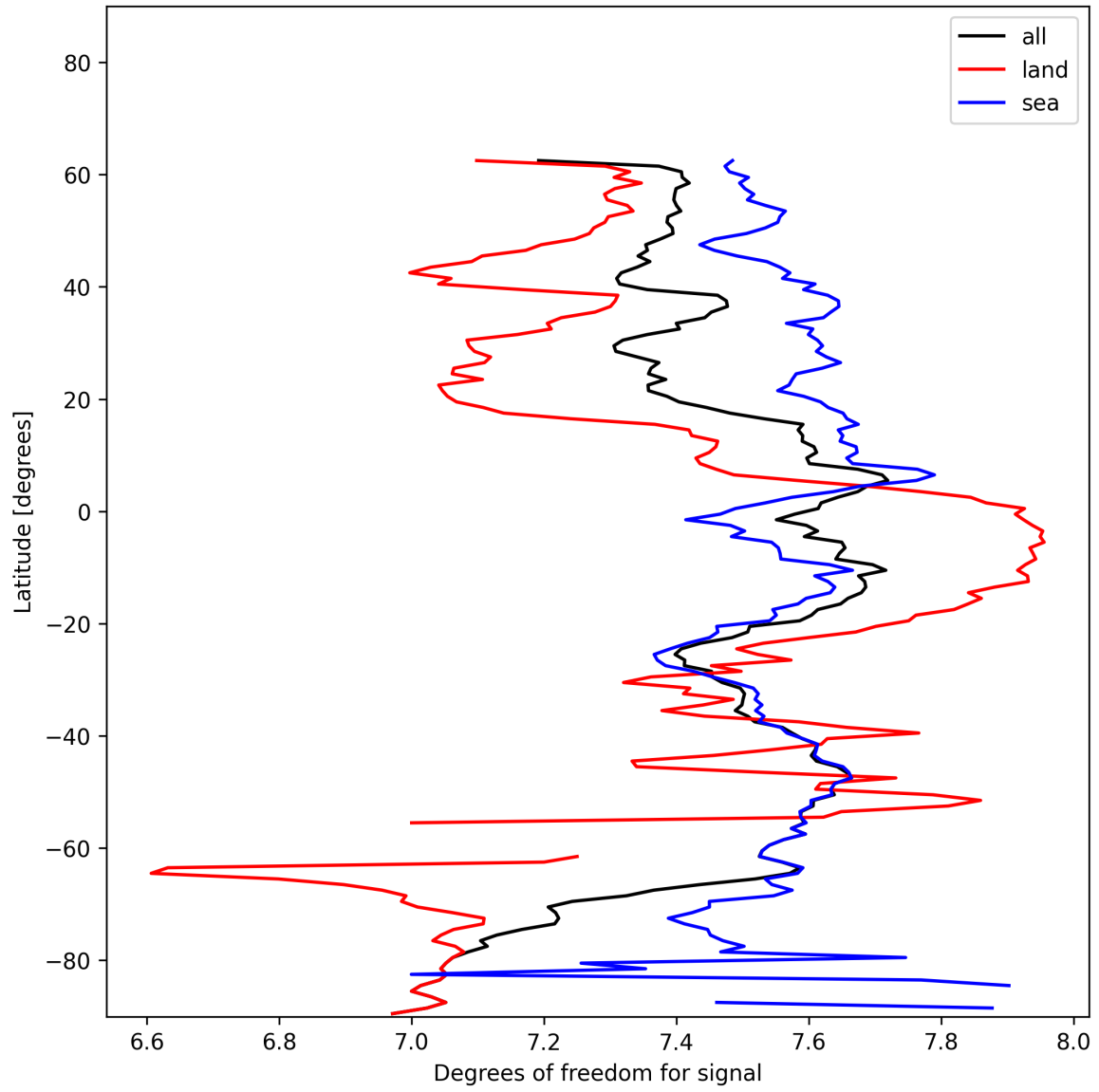
Figure 15: Zonal average of “Degrees of freedom for signal” for 2024-12-07 to 2024-12-09.
