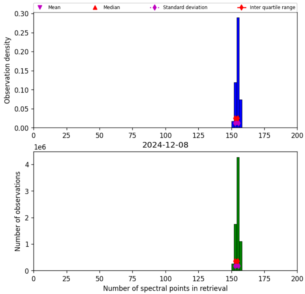
Figure 21: Histogram of “Number of spectral points in retrieval” for 2024-12-07 to 2024-12-09
