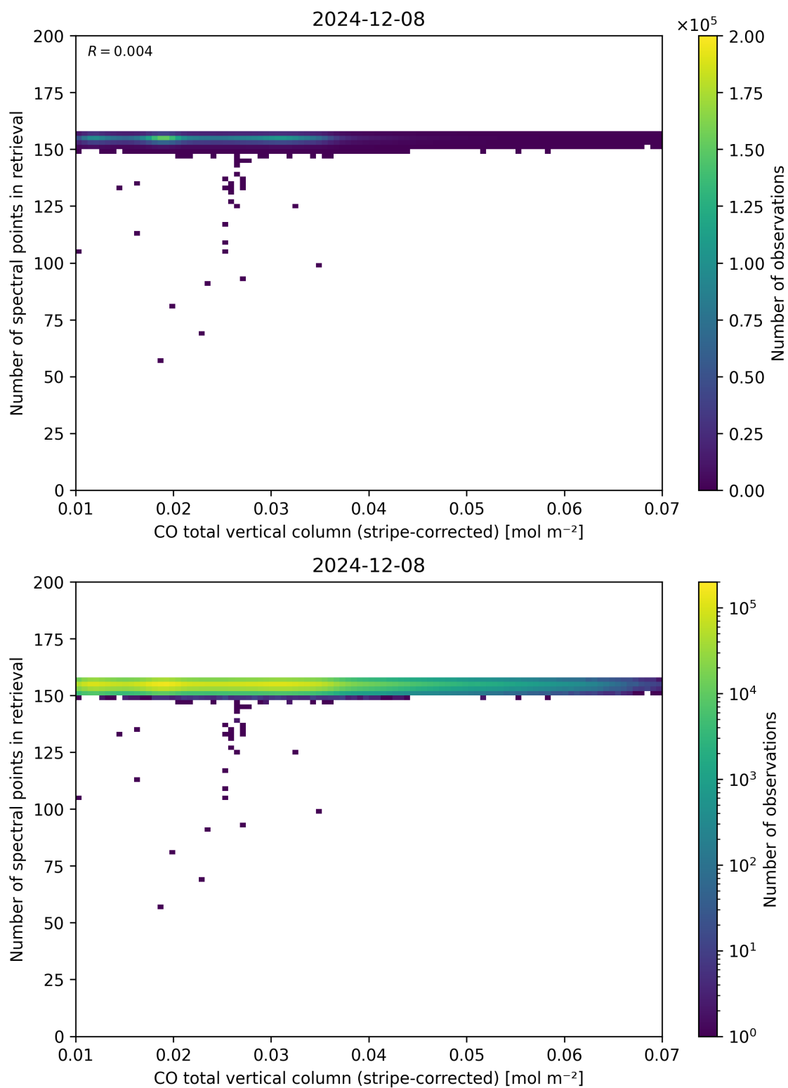
Figure 40: Scatter density plot of “CO total vertical column (stripe-corrected)” against “Number of spectral points in retrieval” for 2024-12-07 to 2024-12-09.
