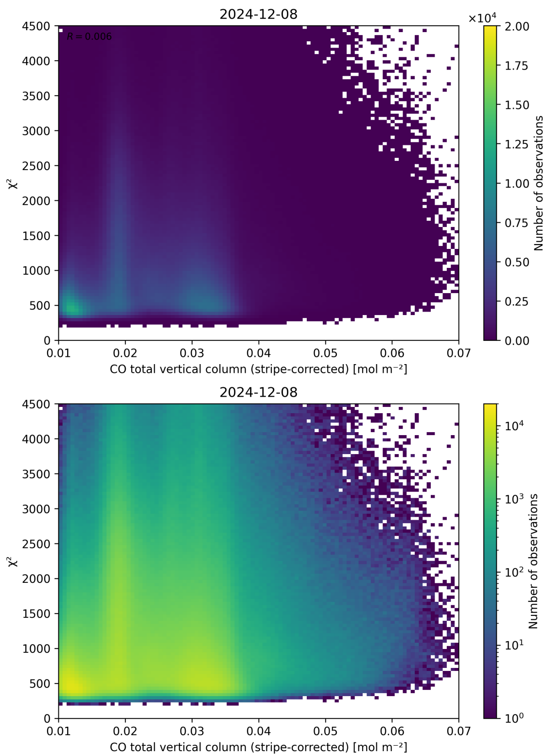
Figure 37: Scatter density plot of “CO total vertical column (stripe-corrected)” against “ \chi^2 ” for 2024-12-07 to 2024-12-09.
