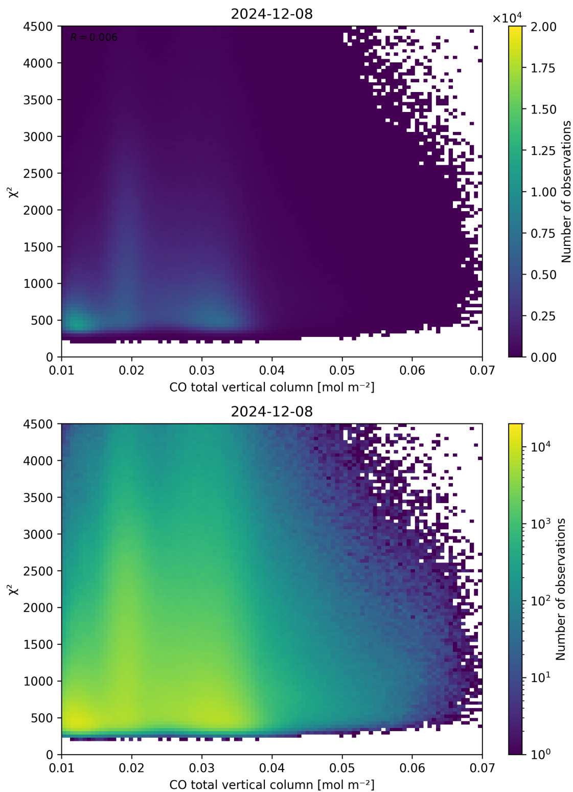
Figure 35: Scatter density plot of “CO total vertical column” against “ \chi^2 ” for 2024-12-07 to 2024-12-09.
