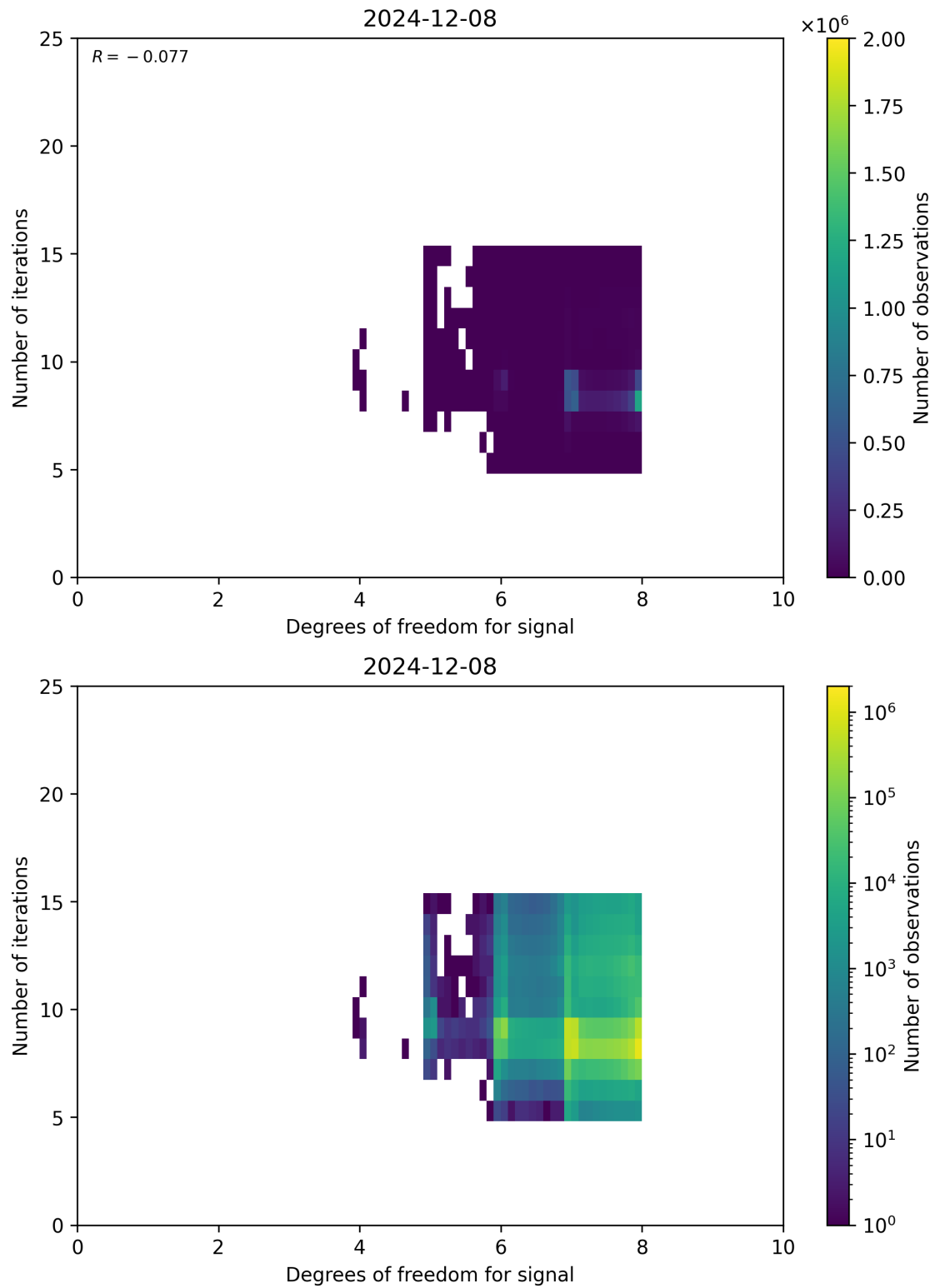
Figure 50: Scatter density plot of “Degrees of freedom for signal” against “Number of iterations” for 2024-12-07 to 2024-12-09.
