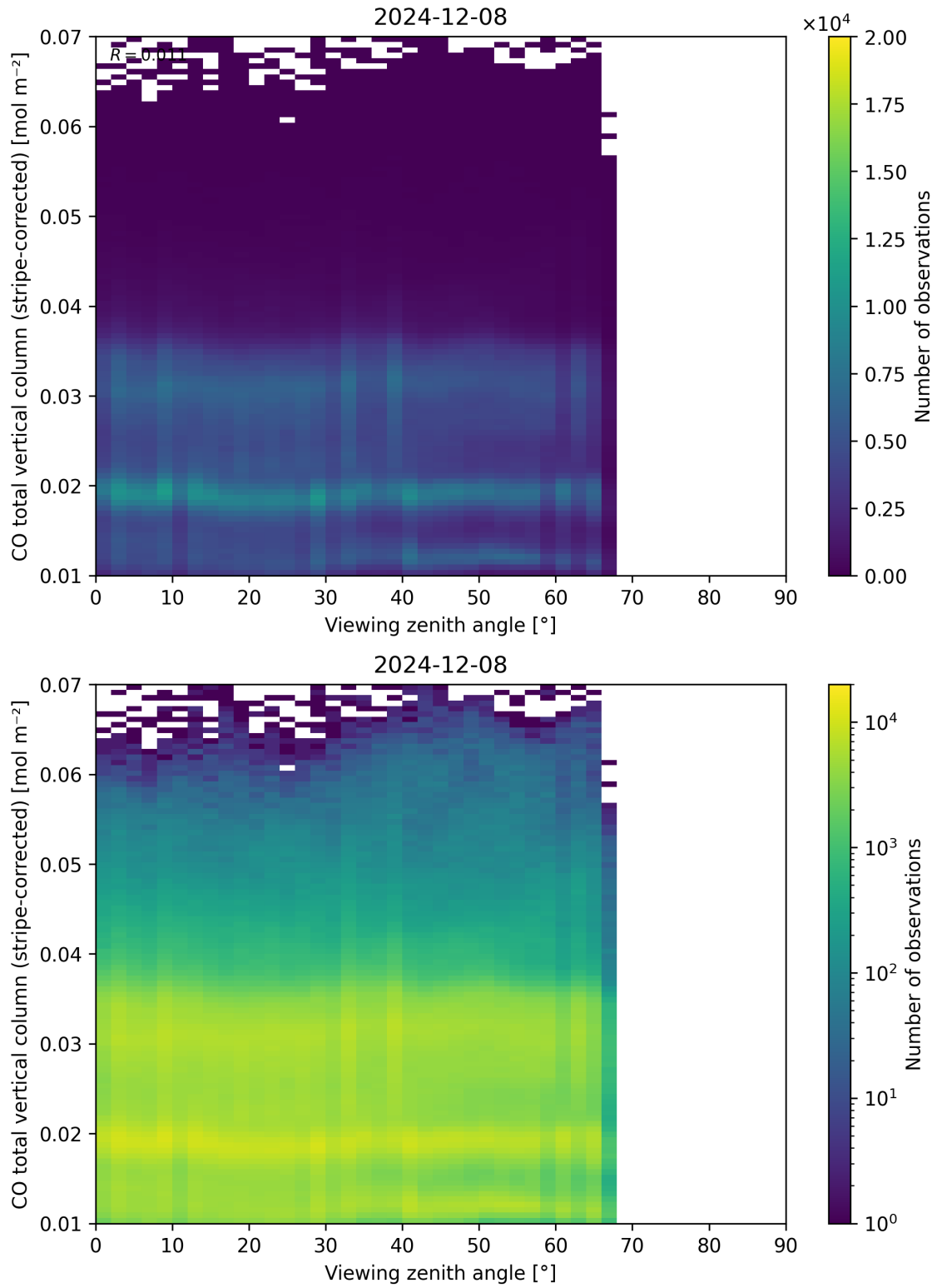
Figure 70: Scatter density plot of “Viewing zenith angle” against “CO total vertical column (stripe-corrected)” for 2024-12-07 to 2024-12-09.
