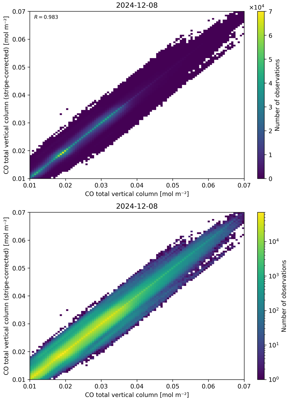
Figure 33: Scatter density plot of “CO total vertical column” against “CO total vertical column (stripe-corrected)” for 2024-12-07 to 2024-12-09.
