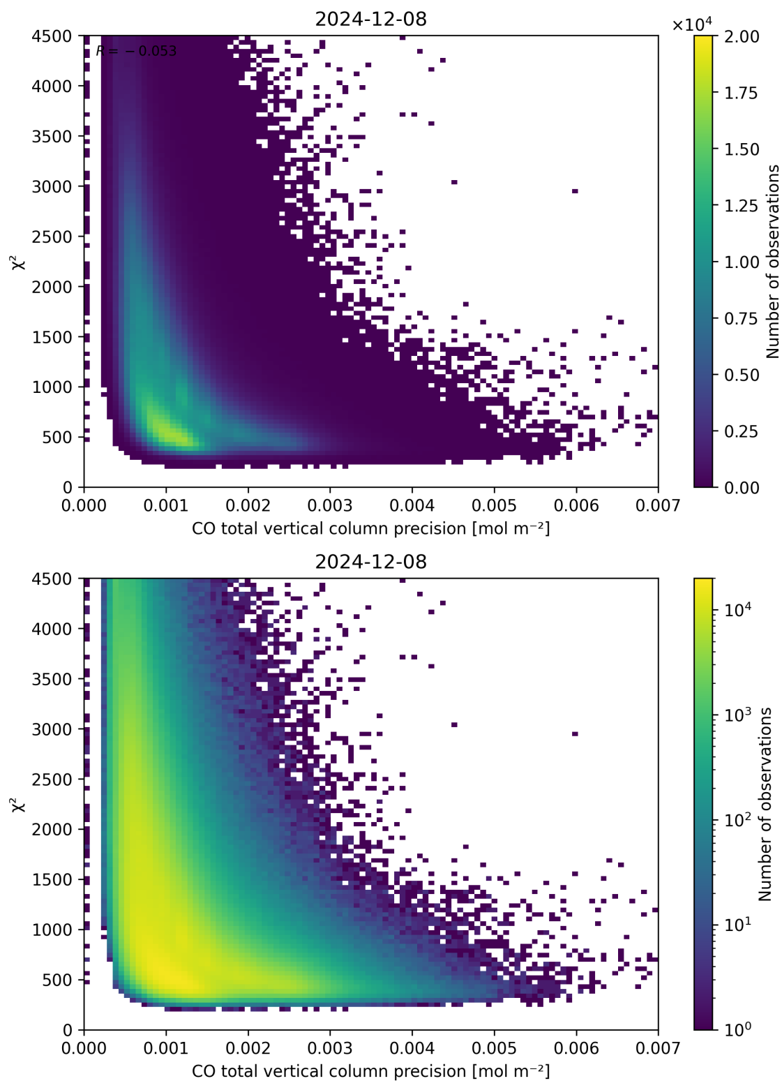
Figure 44: Scatter density plot of “CO total vertical column precision” against “ \chi^2 ” for 2024-12-07 to 2024-12-09.
