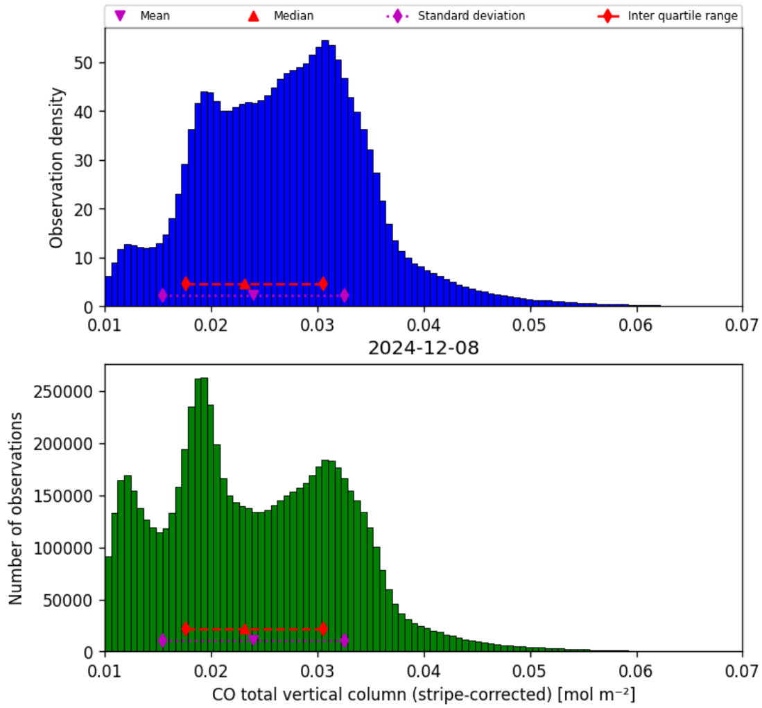
Figure 19: Histogram of “CO total vertical column (stripe-corrected)” for 2024-12-07 to 2024-12-09
