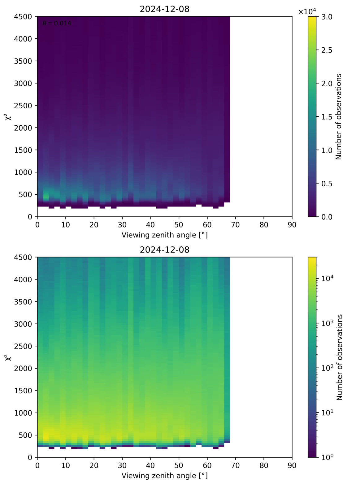
Figure 72: Scatter density plot of “Viewing zenith angle” against “ \chi^2 ” for 2024-12-07 to 2024-12-09.
