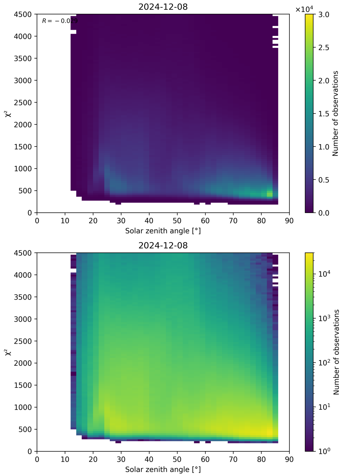
Figure 64: Scatter density plot of “Solar zenith angle” against “ \chi^2 ” for 2024-12-07 to 2024-12-09.
