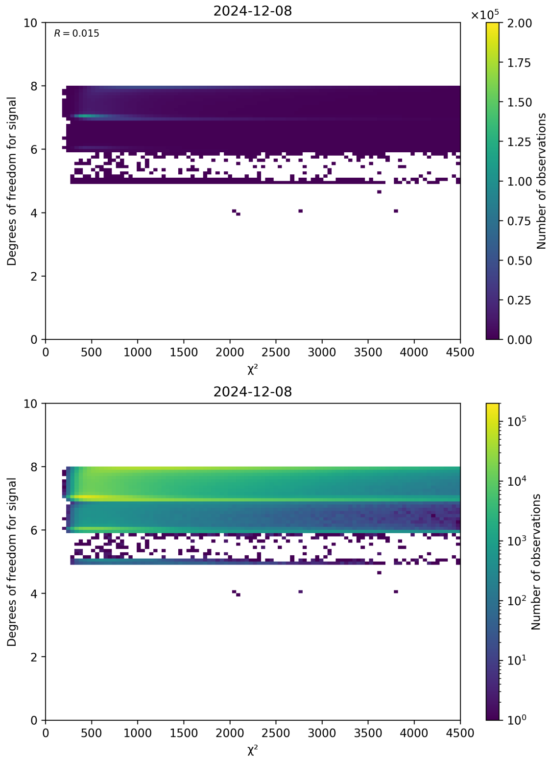
Figure 48: Scatter density plot of “ \chi^2 ” against “Degrees of freedom for signal” for 2024-12-07 to 2024-12-09.
