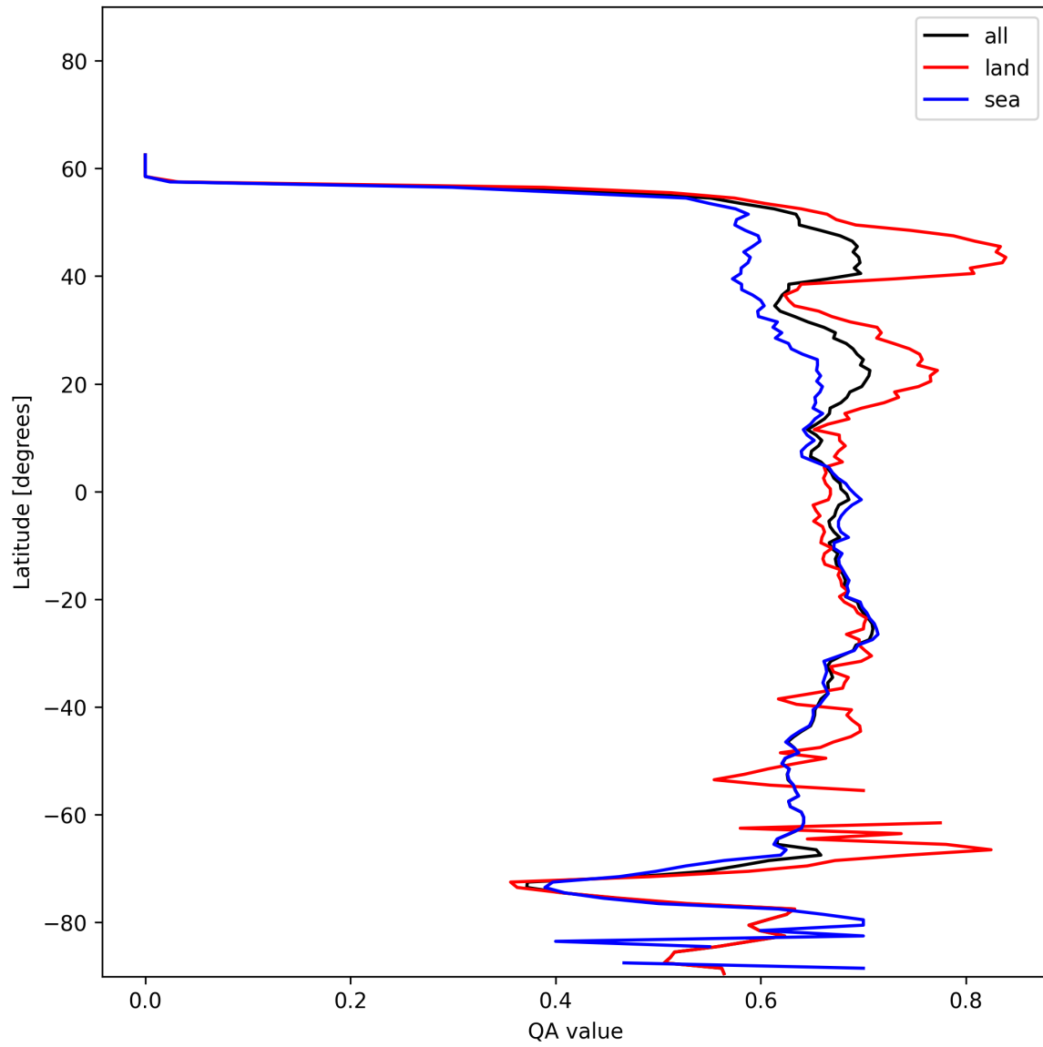
Figure 9: Zonal average of “QA value” for 2024-12-07 to 2024-12-09.
