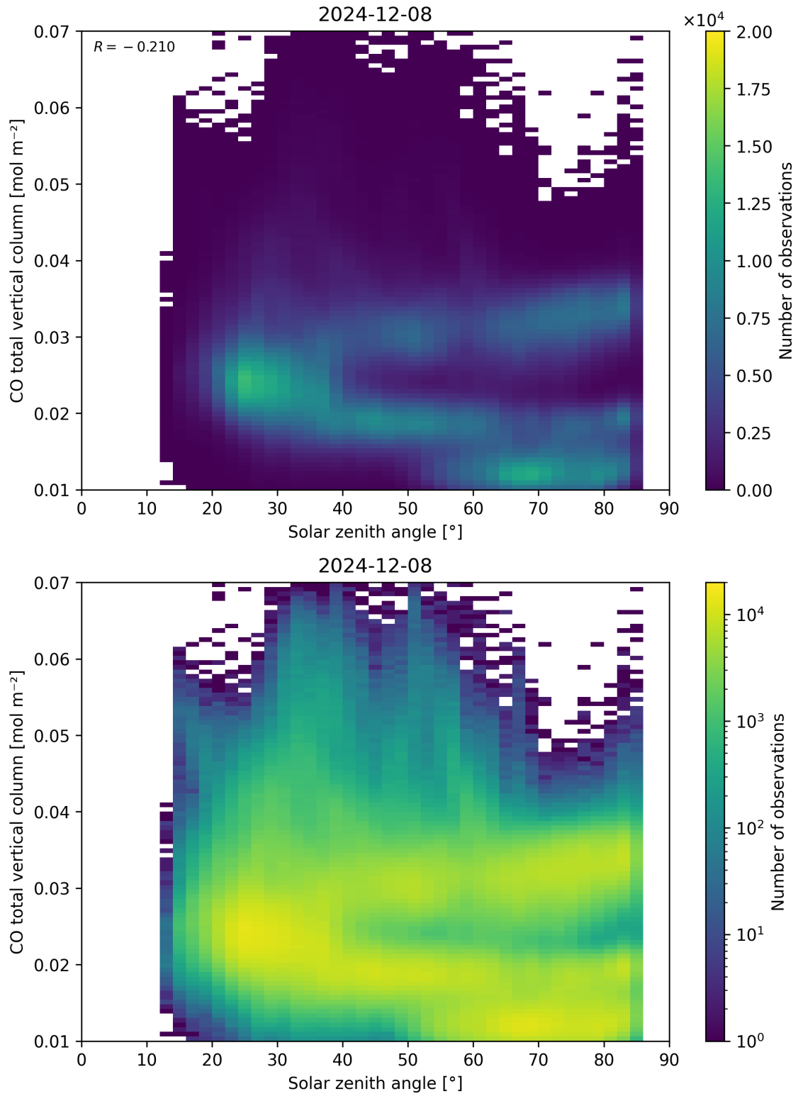
Figure 61: Scatter density plot of “Solar zenith angle” against “CO total vertical column” for 2024-12-07 to 2024-12-09.
