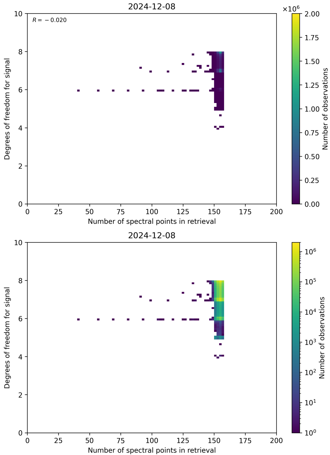
Figure 59: Scatter density plot of “Number of spectral points in retrieval” against “Degrees of freedom for signal” for 2024-12-07 to 2024-12-09.
