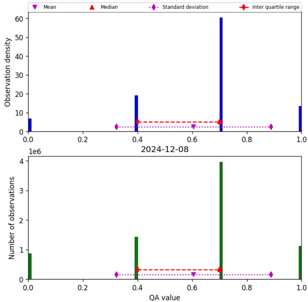
Figure 17: Histogram of “QA value” for 2024-12-07 to 2024-12-09
