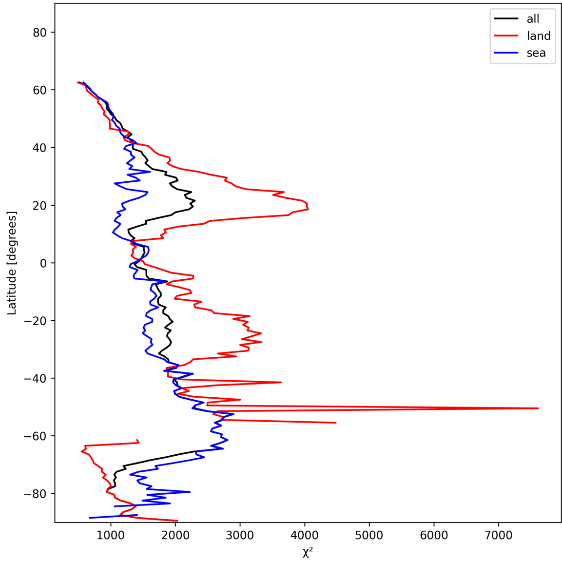
Figure 14: Zonal average of “ \chi^2 ” for 2024-12-07 to 2024-12-09.
