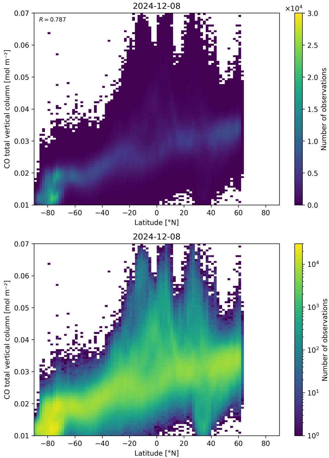
Figure 51: Scatter density plot of “Latitude” against “CO total vertical column” for 2024-12-07 to 2024-12-09.
