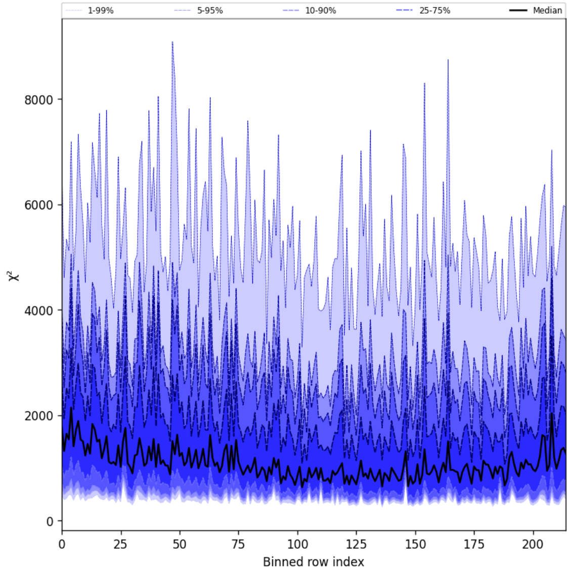
Figure 30: Along track statistics of “ \chi^2 ” for 2024-12-07 to 2024-12-09
