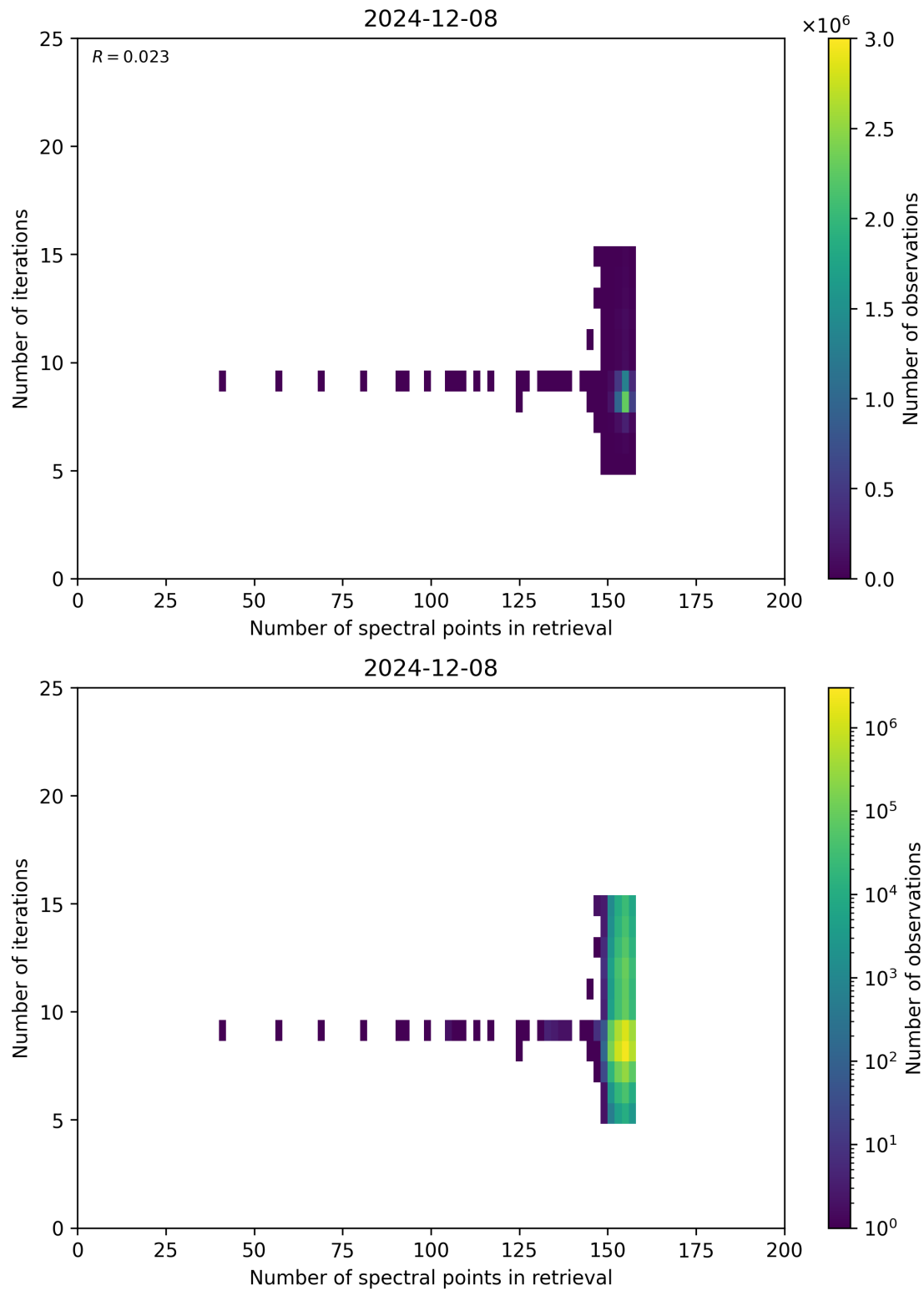
Figure 60: Scatter density plot of “Number of spectral points in retrieval” against “Number of iterations” for 2024-12-07 to 2024-12-09.
