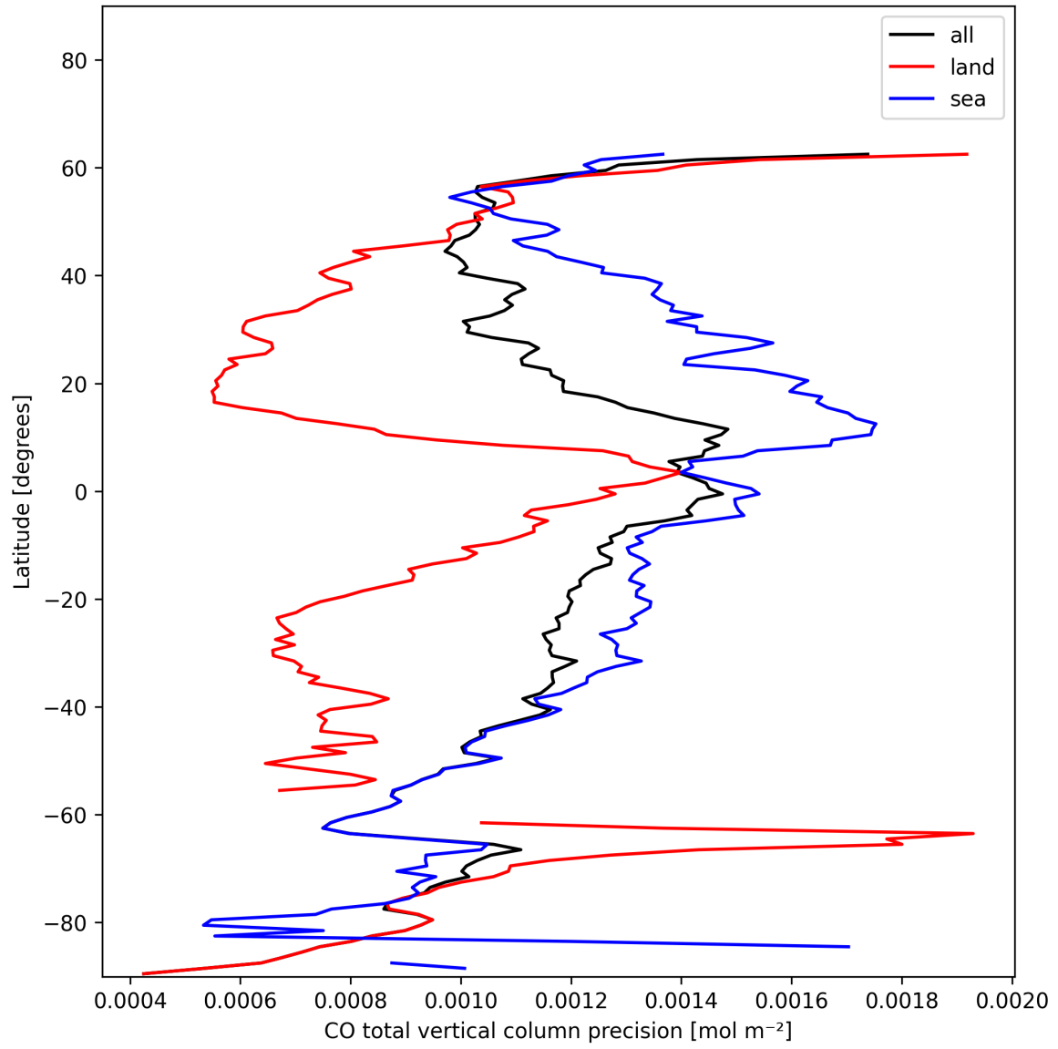
Figure 12: Zonal average of “CO total vertical column precision” for 2024-12-07 to 2024-12-09.
