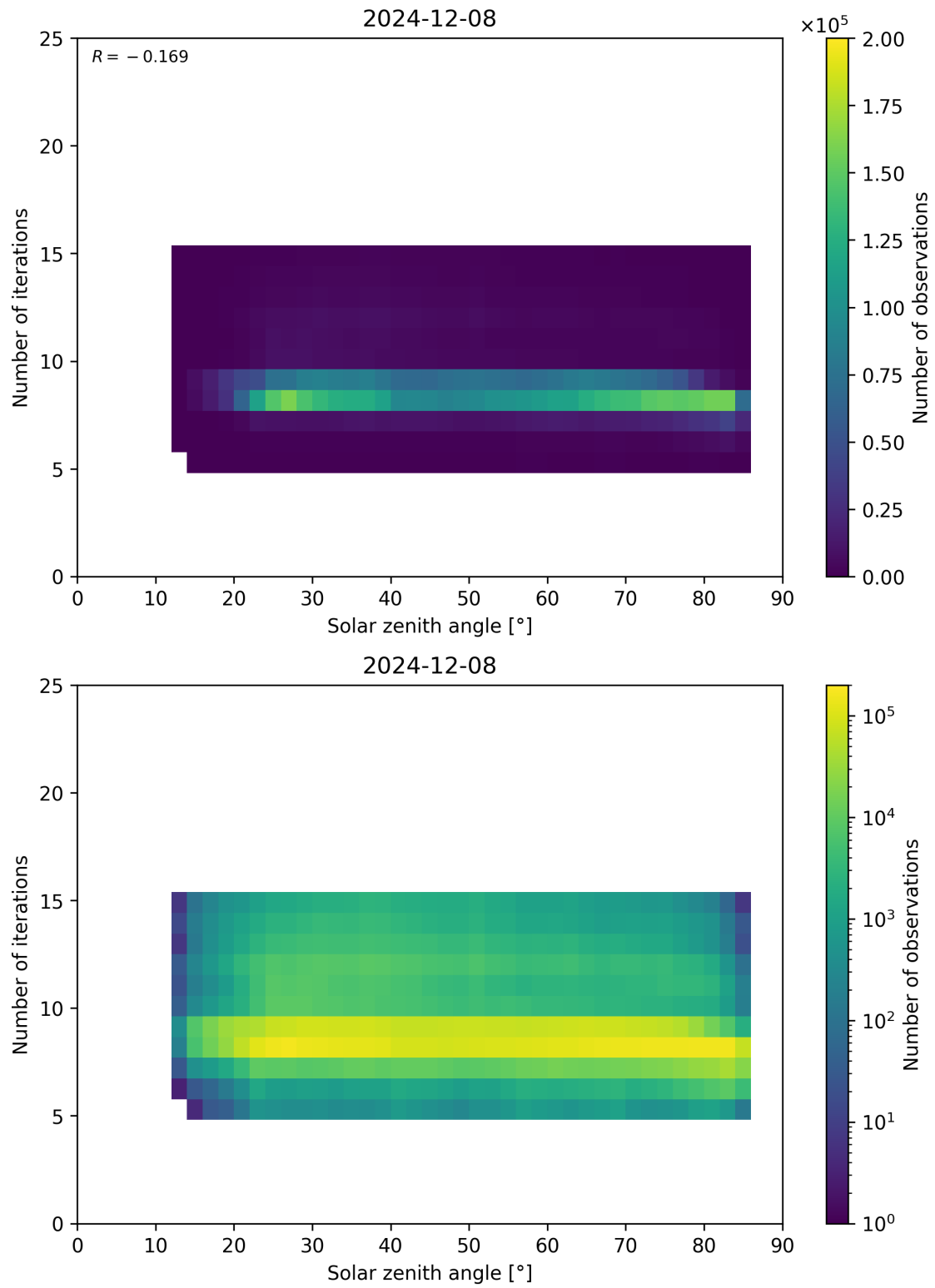
Figure 67: Scatter density plot of “Solar zenith angle” against “Number of iterations” for 2024-12-07 to 2024-12-09.
