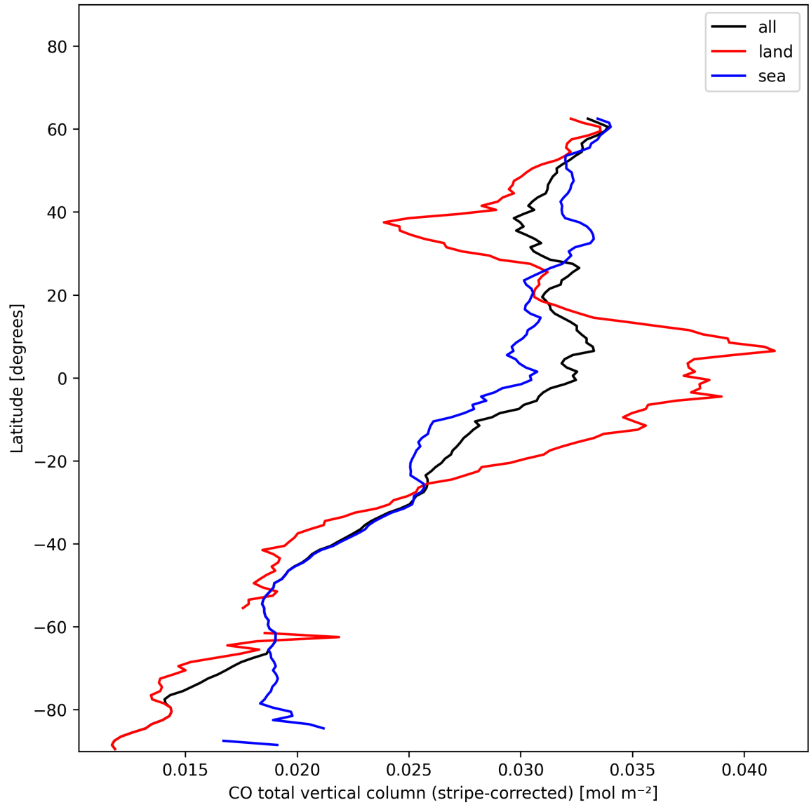
Figure 11: Zonal average of “CO total vertical column (stripe-corrected)” for 2024-12-07 to 2024-12-09.
