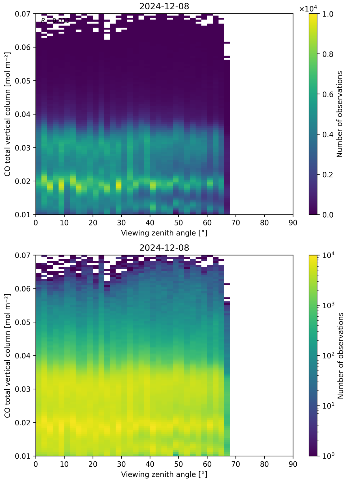
Figure 69: Scatter density plot of “Viewing zenith angle” against “CO total vertical column” for 2024-12-07 to 2024-12-09.
