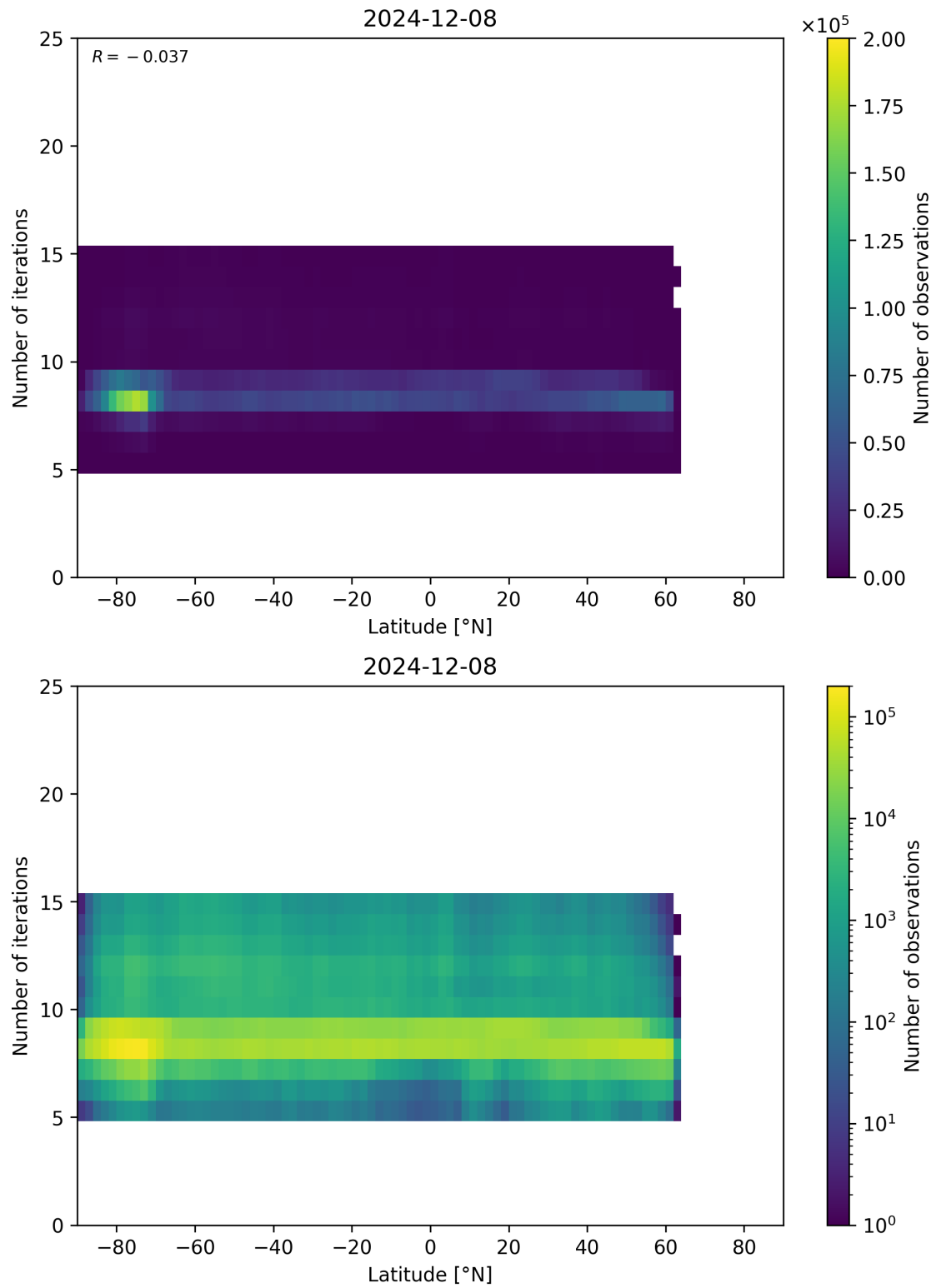
Figure 56: Scatter density plot of “Latitude” against “Number of iterations” for 2024-12-07 to 2024-12-09.
