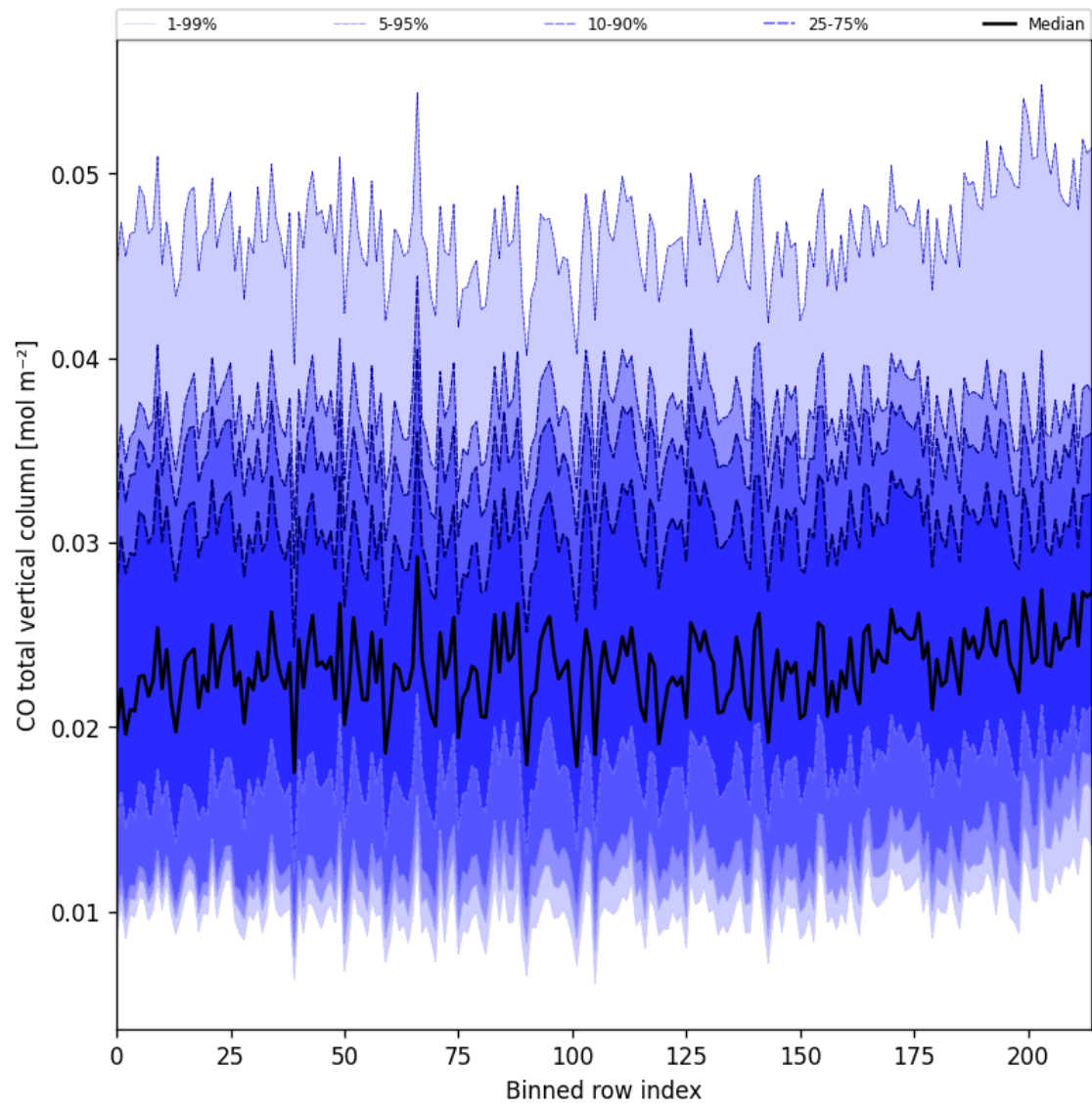
Figure 26: Along track statistics of “CO total vertical column” for 2024-12-07 to 2024-12-09
