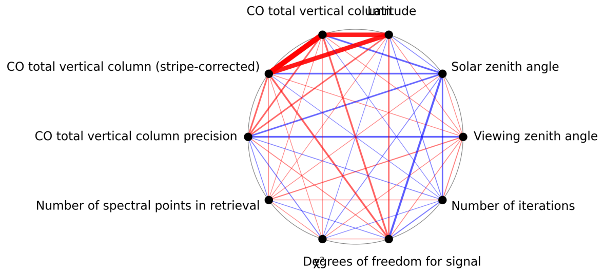
Figure 1: Map of correlation graph for 2024-12-07 to 2024-12-09.
