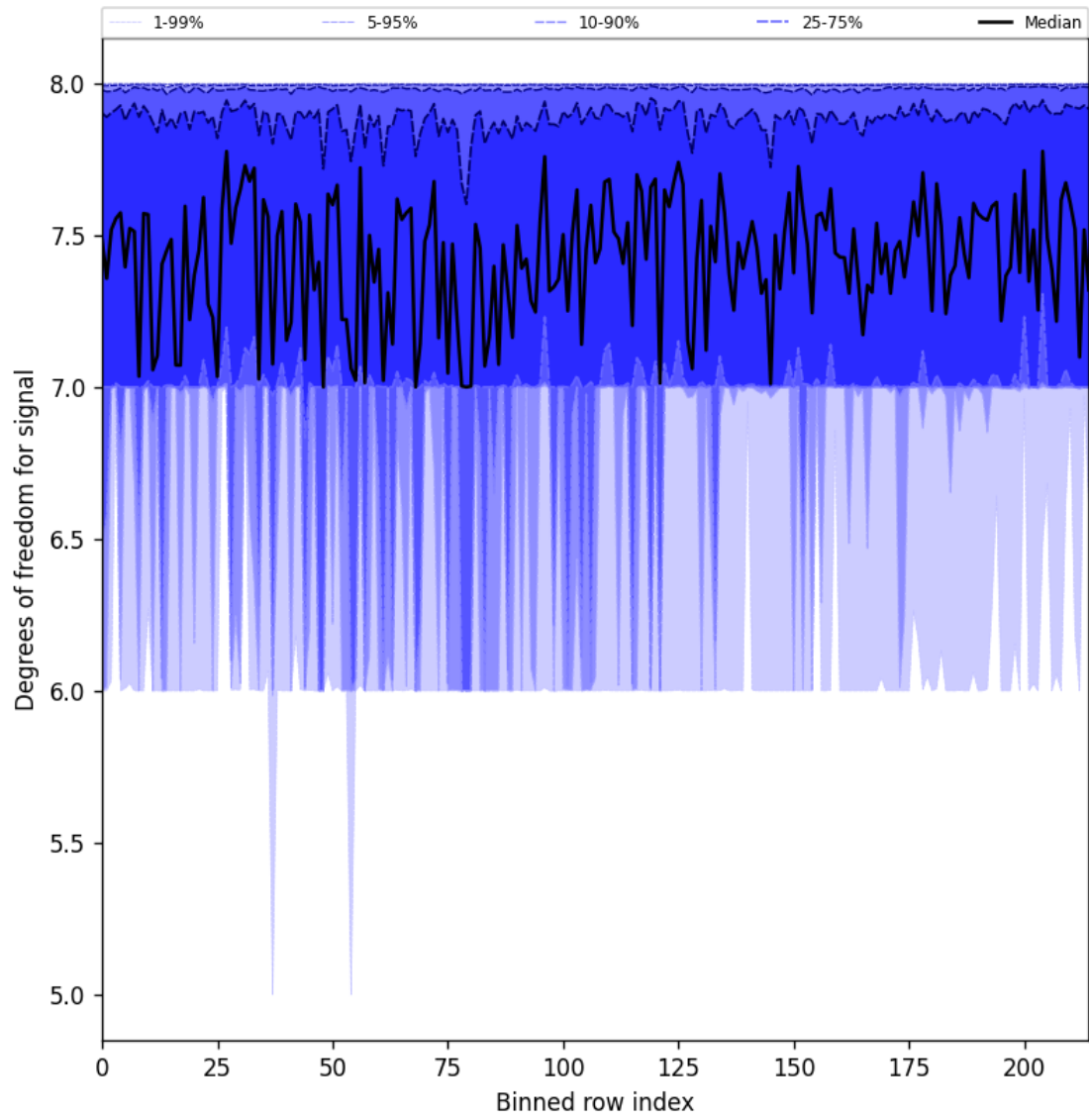
Figure 31: Along track statistics of “Degrees of freedom for signal” for 2024-12-07 to 2024-12-09
