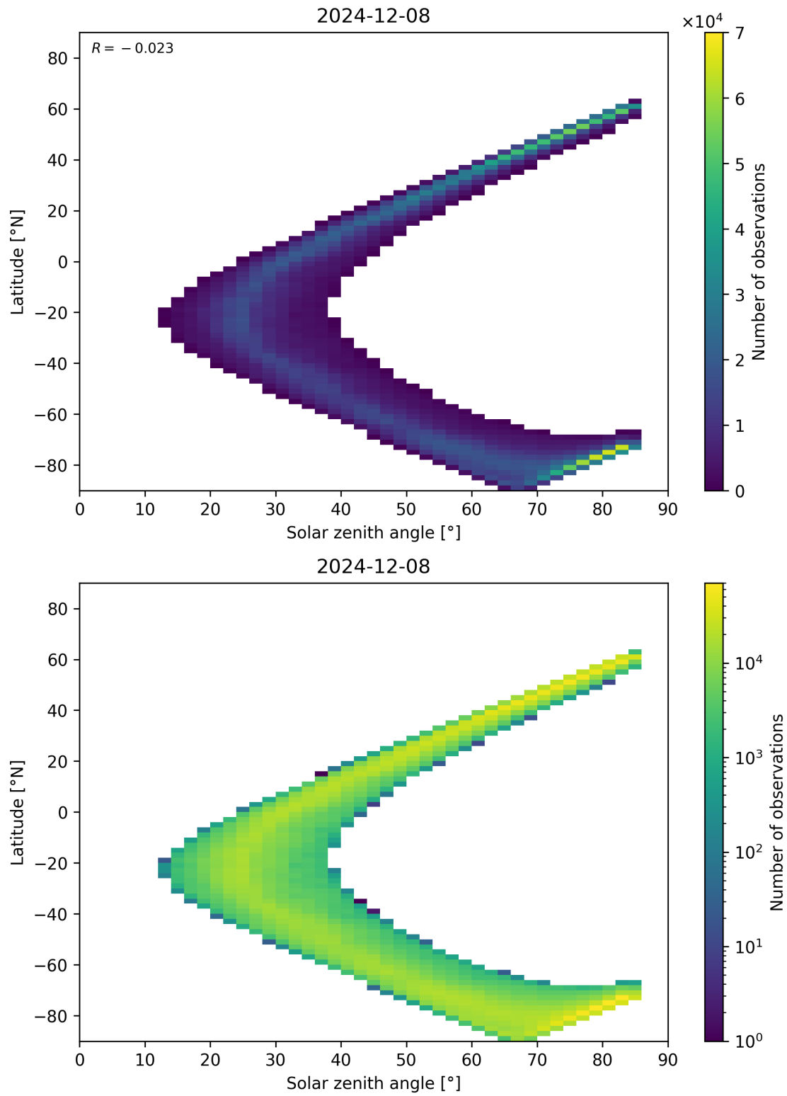
Figure 66: Scatter density plot of “Solar zenith angle” against “Latitude” for 2024-12-07 to 2024-12-09.
