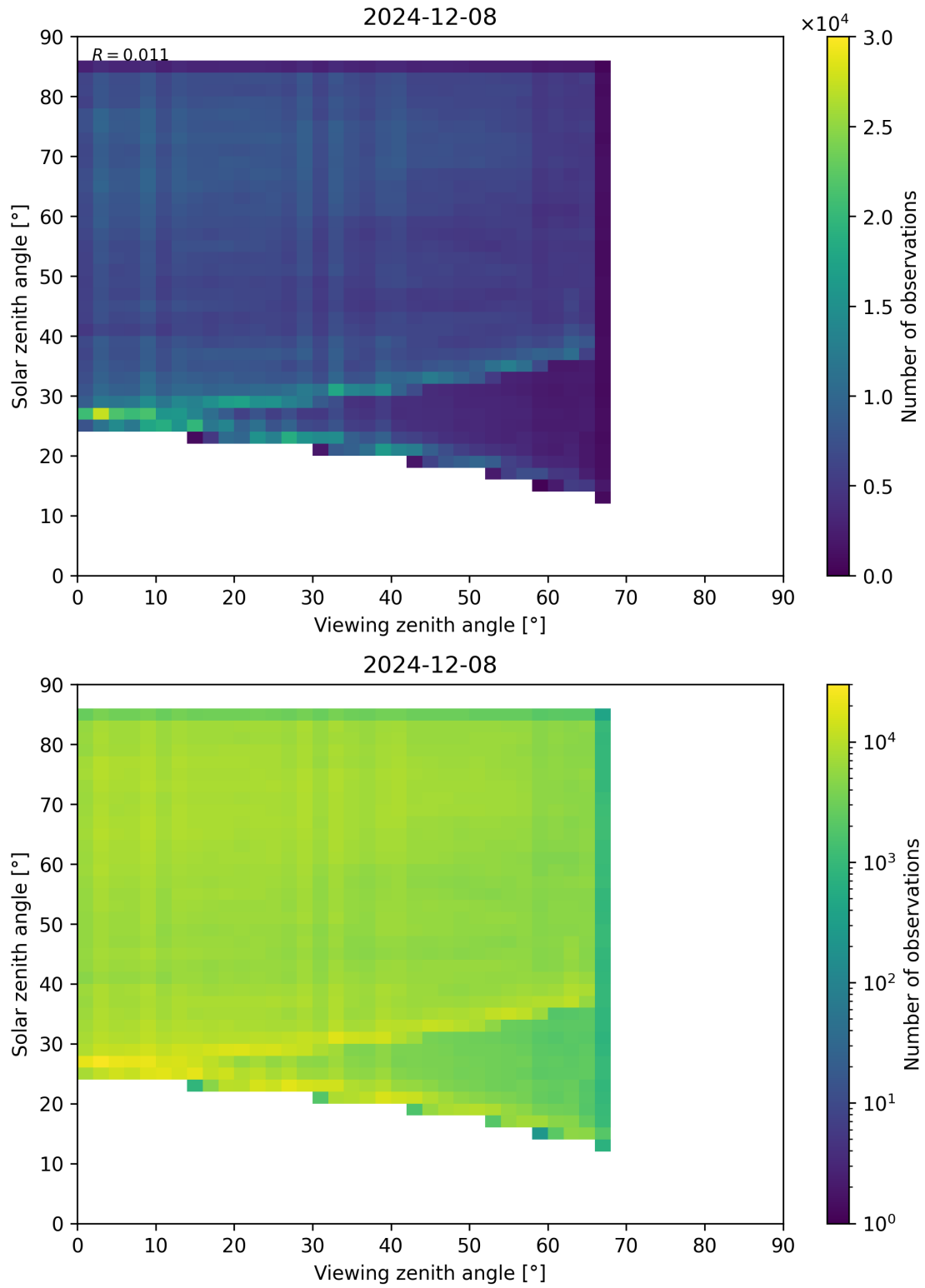
Figure 77: Scatter density plot of “Viewing zenith angle” against “Solar zenith angle” for 2024-12-07 to 2024-12-09.
