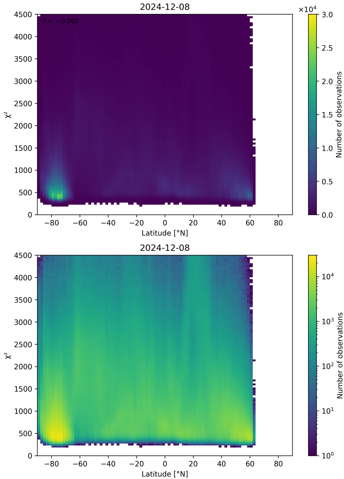
Figure 54: Scatter density plot of “Latitude” against “ \chi^2 ” for 2024-12-07 to 2024-12-09.
