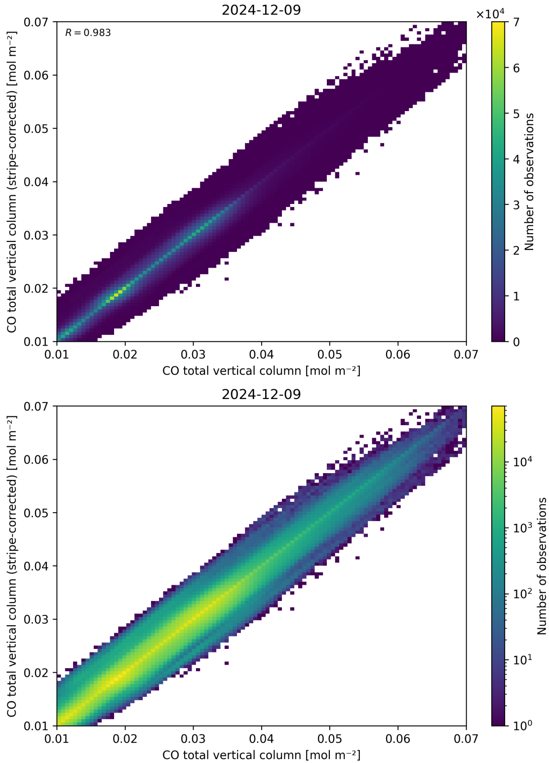
Figure 33: Scatter density plot of “CO total vertical column” against “CO total vertical column (stripe-corrected)” for 2024-12-08 to 2024-12-10.
