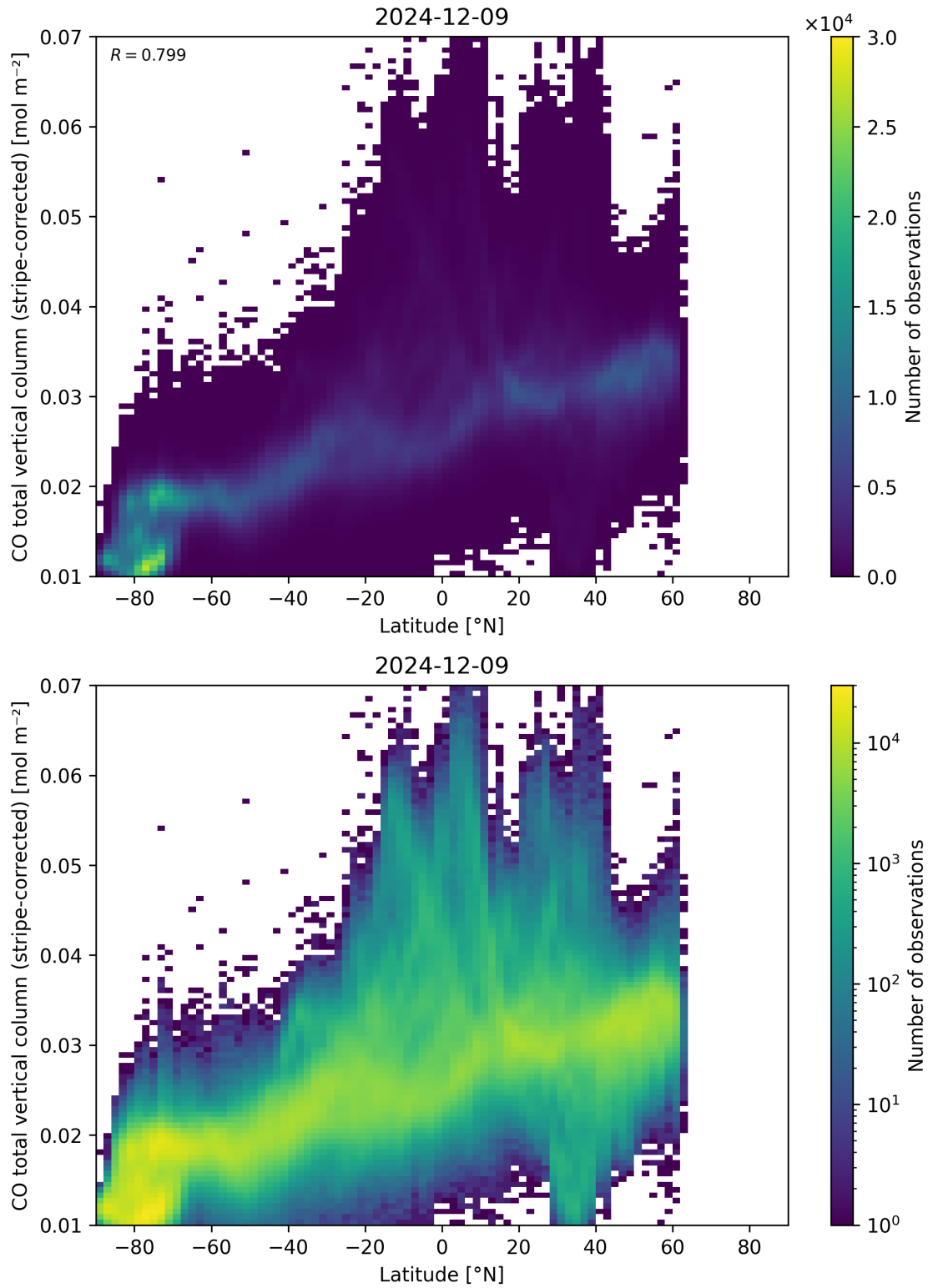
Figure 52: Scatter density plot of “Latitude” against “CO total vertical column (stripe-corrected)” for 2024-12-08 to 2024-12-10.
