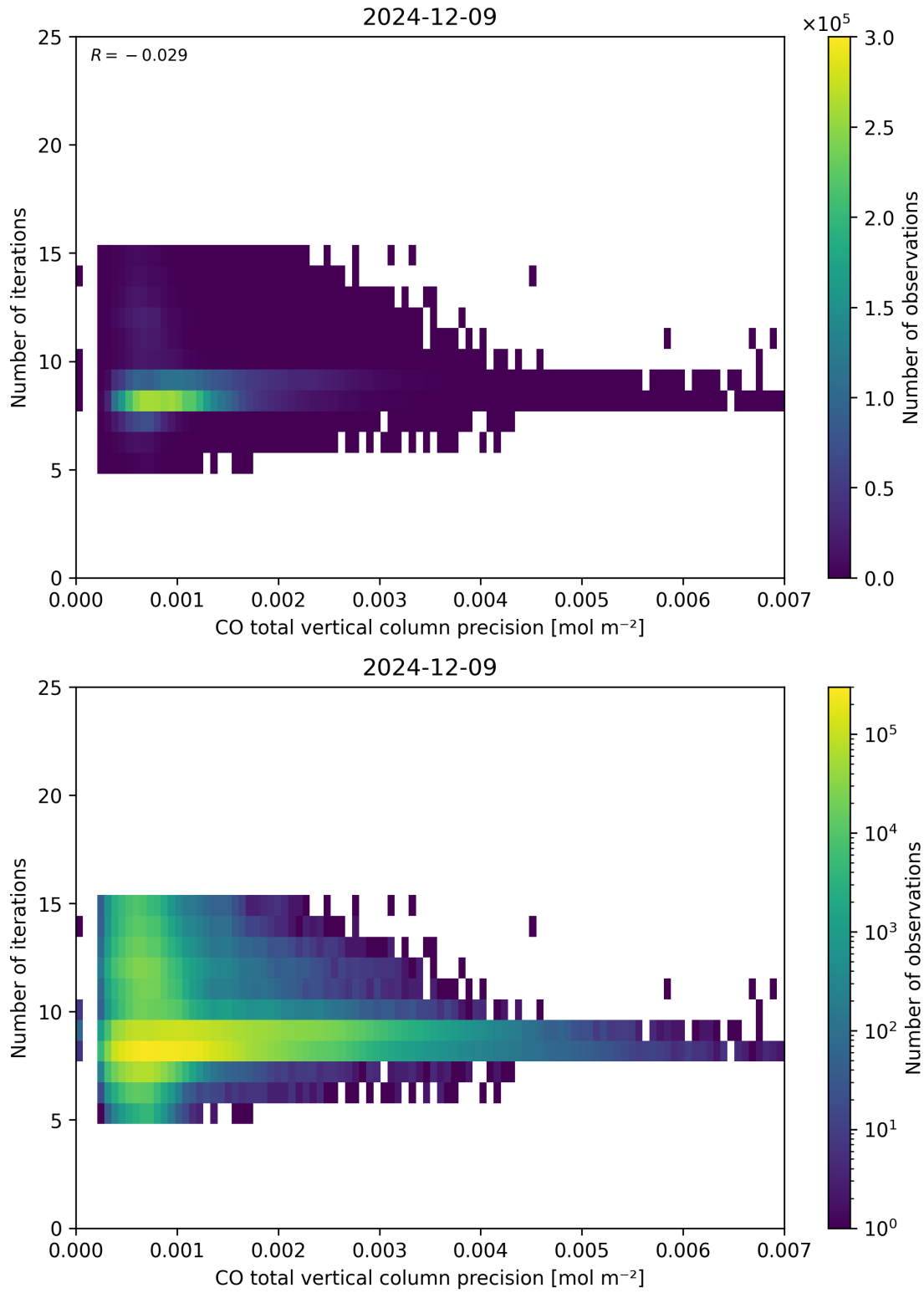
Figure 46: Scatter density plot of “CO total vertical column precision” against “Number of iterations” for 2024-12-08 to 2024-12-10.
