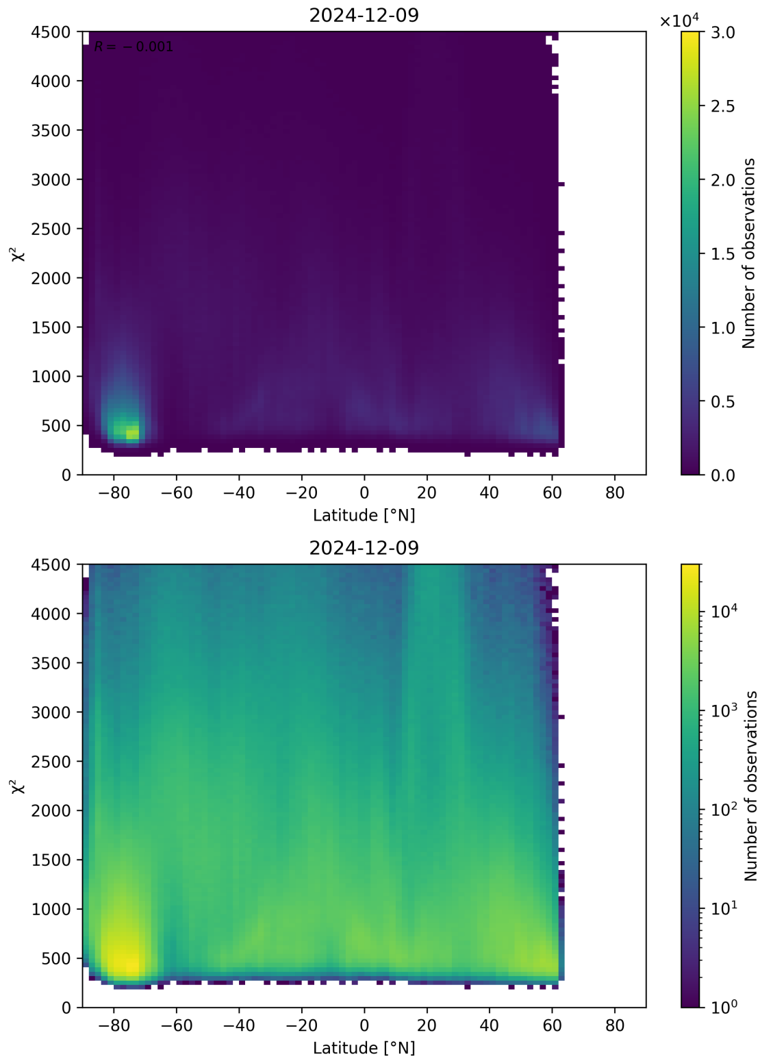
Figure 54: Scatter density plot of “Latitude” against “ \chi^2 ” for 2024-12-08 to 2024-12-10.
