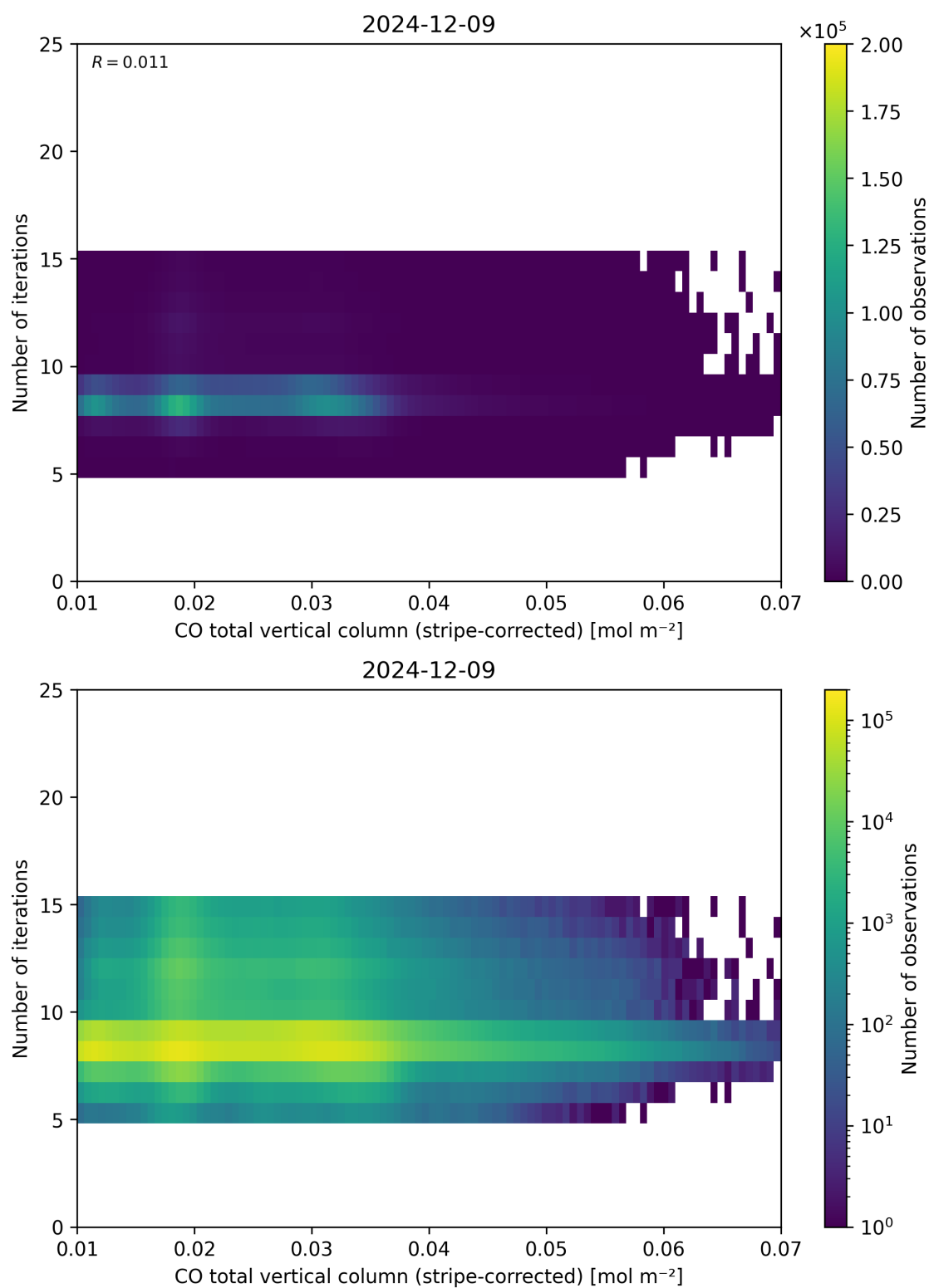
Figure 39: Scatter density plot of “CO total vertical column (stripe-corrected)” against “Number of iterations” for 2024-12-08 to 2024-12-10.
