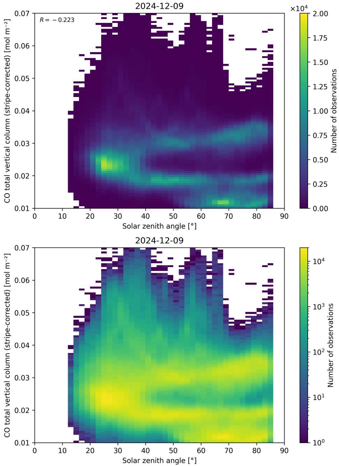
Figure 62: Scatter density plot of “Solar zenith angle” against “CO total vertical column (stripe-corrected)” for 2024-12-08 to 2024-12-10.
