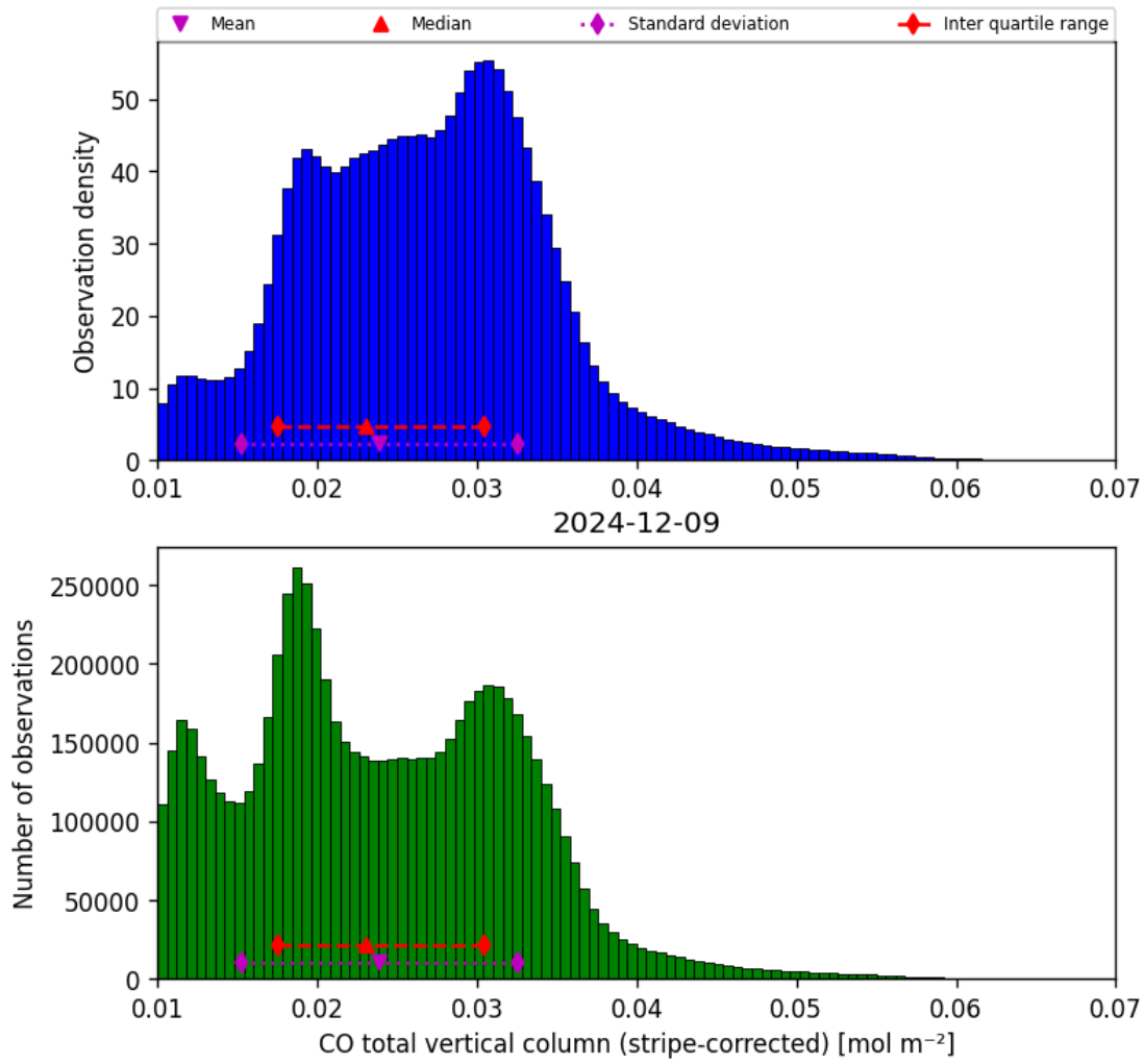
Figure 19: Histogram of “CO total vertical column (stripe-corrected)” for 2024-12-08 to 2024-12-10
