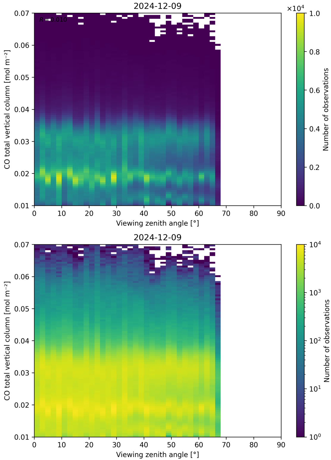
Figure 69: Scatter density plot of “Viewing zenith angle” against “CO total vertical column” for 2024-12-08 to 2024-12-10.
