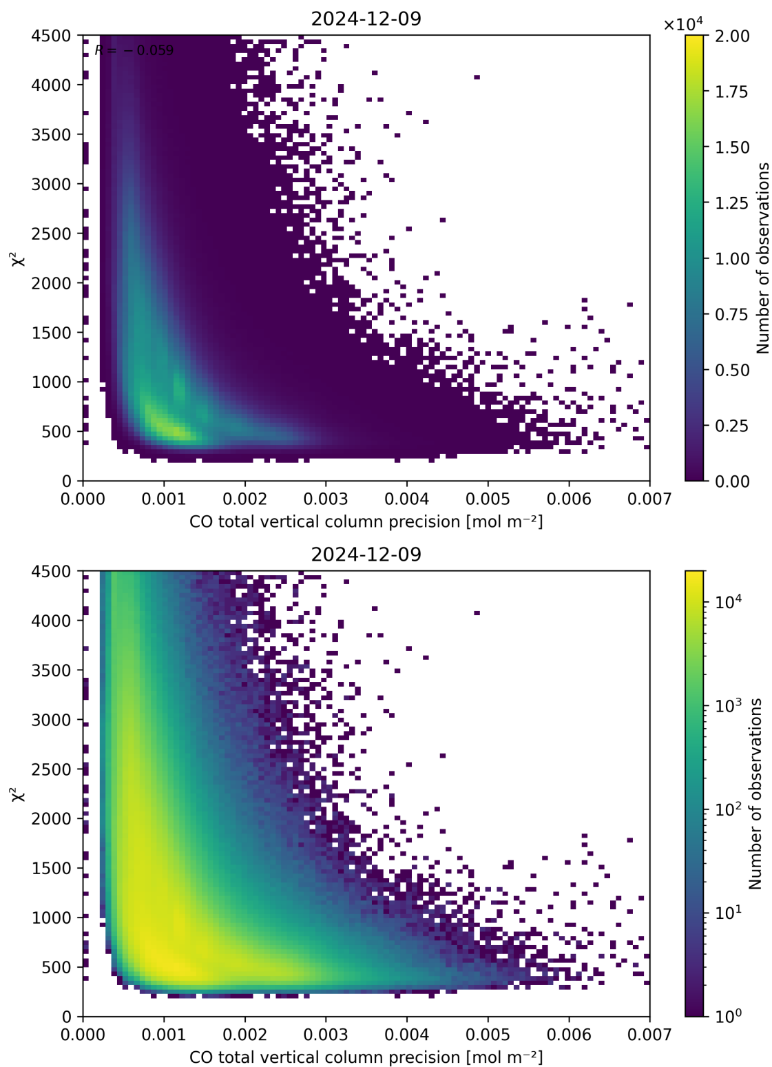
Figure 44: Scatter density plot of “CO total vertical column precision” against “ \chi^2 ” for 2024-12-08 to 2024-12-10.
