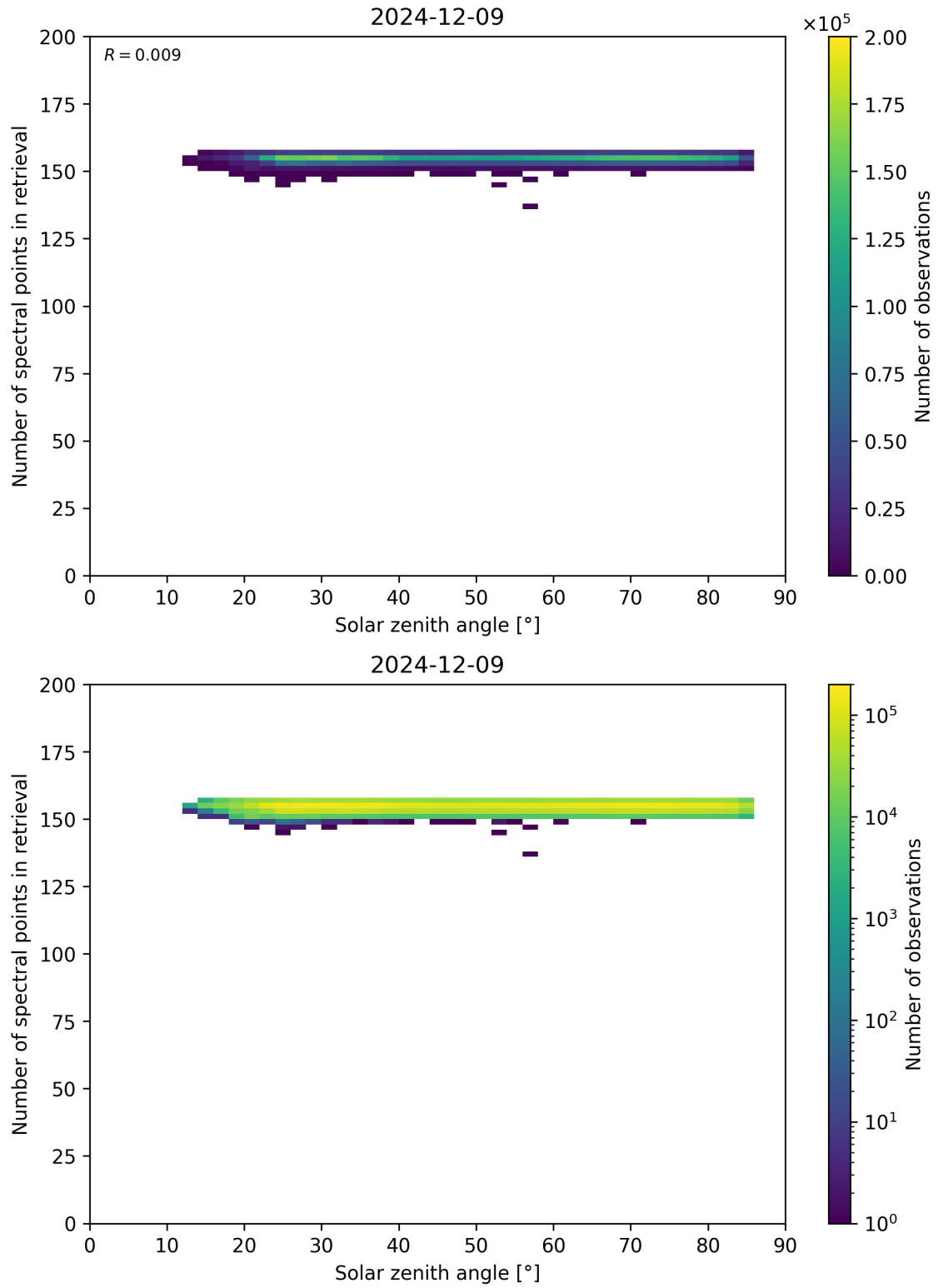
Figure 68: Scatter density plot of “Solar zenith angle” against “Number of spectral points in retrieval” for 2024-12-08 to 2024-12-10.
