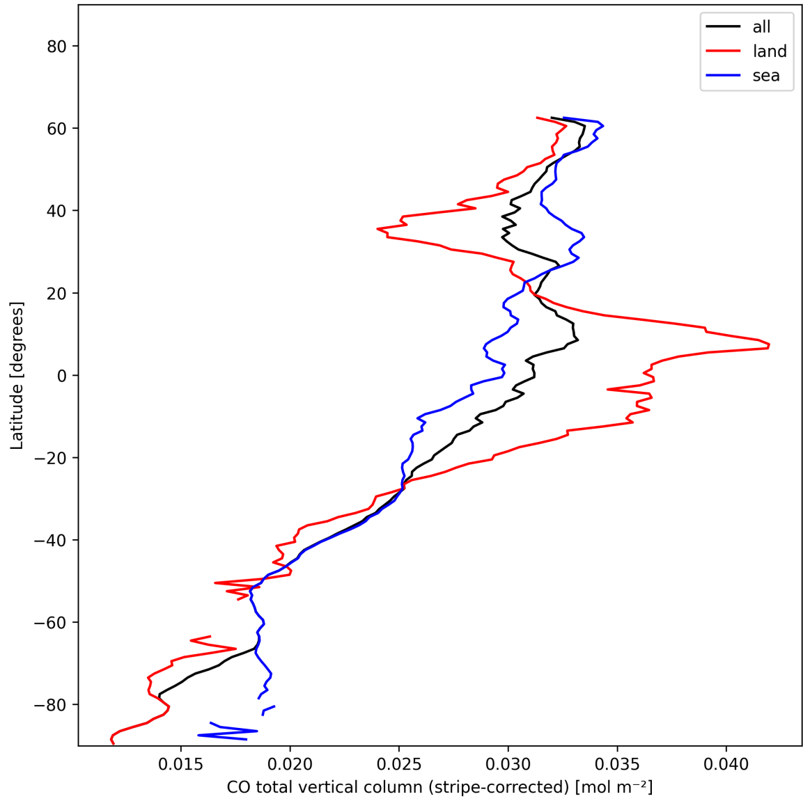
Figure 11: Zonal average of “CO total vertical column (stripe-corrected)” for 2024-12-08 to 2024-12-10.
