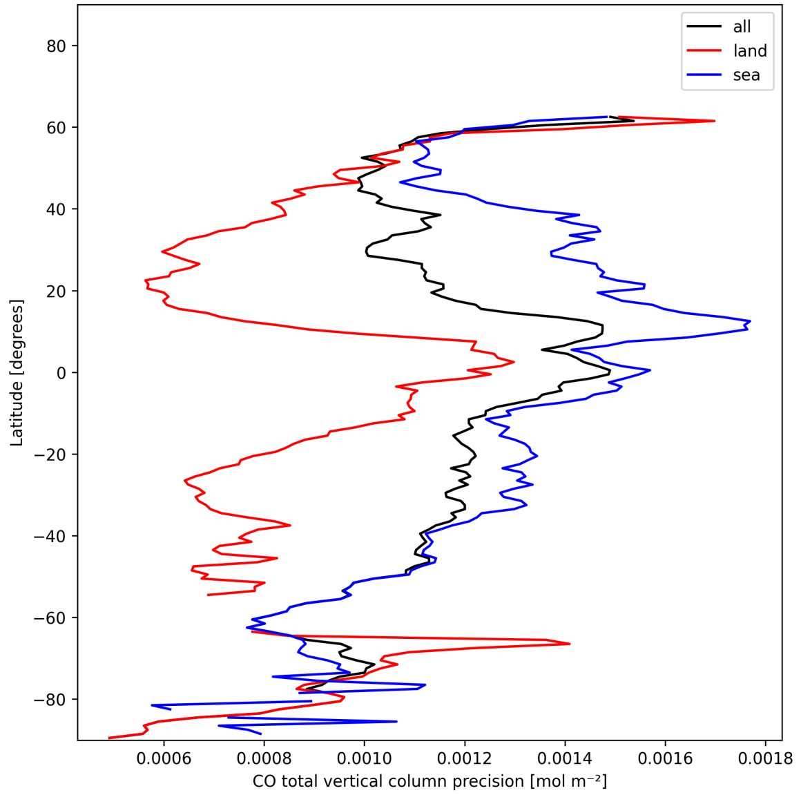
Figure 12: Zonal average of “CO total vertical column precision” for 2024-12-08 to 2024-12-10.
