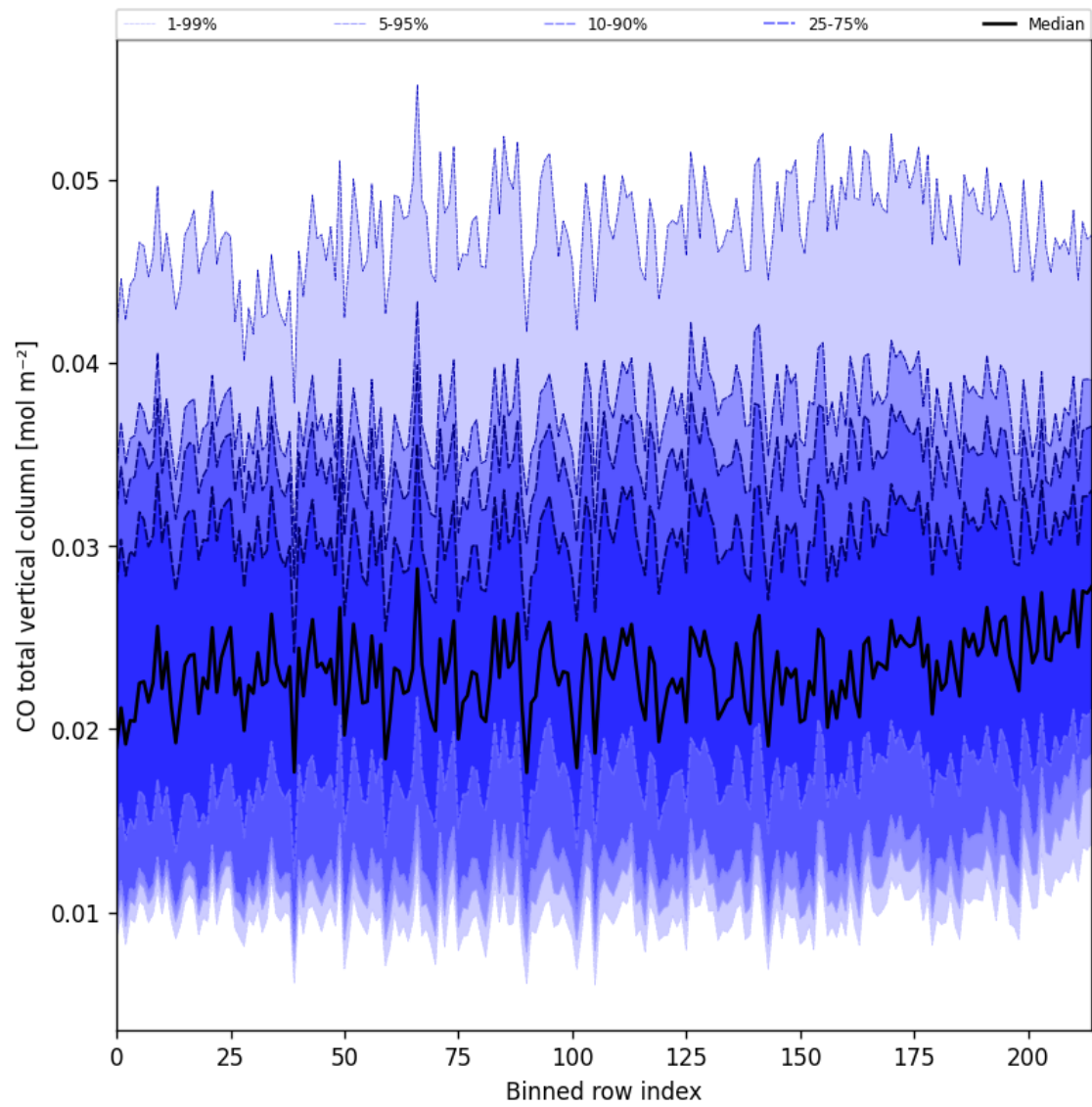
Figure 26: Along track statistics of “CO total vertical column” for 2024-12-08 to 2024-12-10
