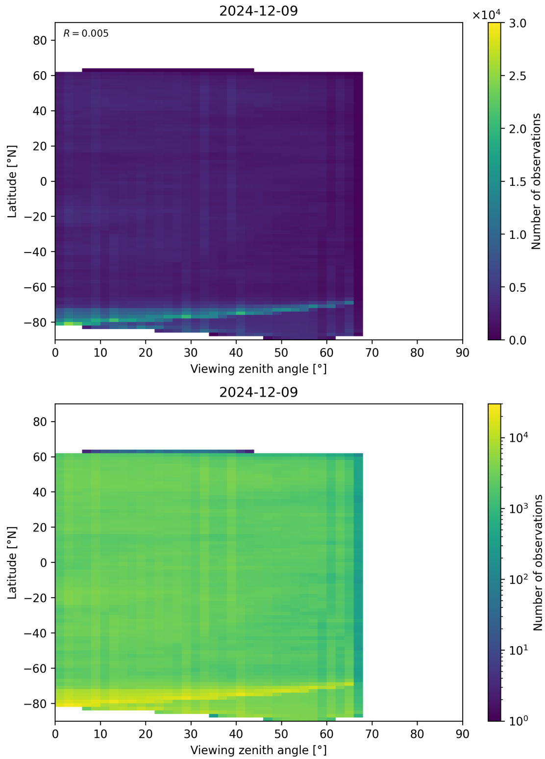
Figure 74: Scatter density plot of “Viewing zenith angle” against “Latitude” for 2024-12-08 to 2024-12-10.
