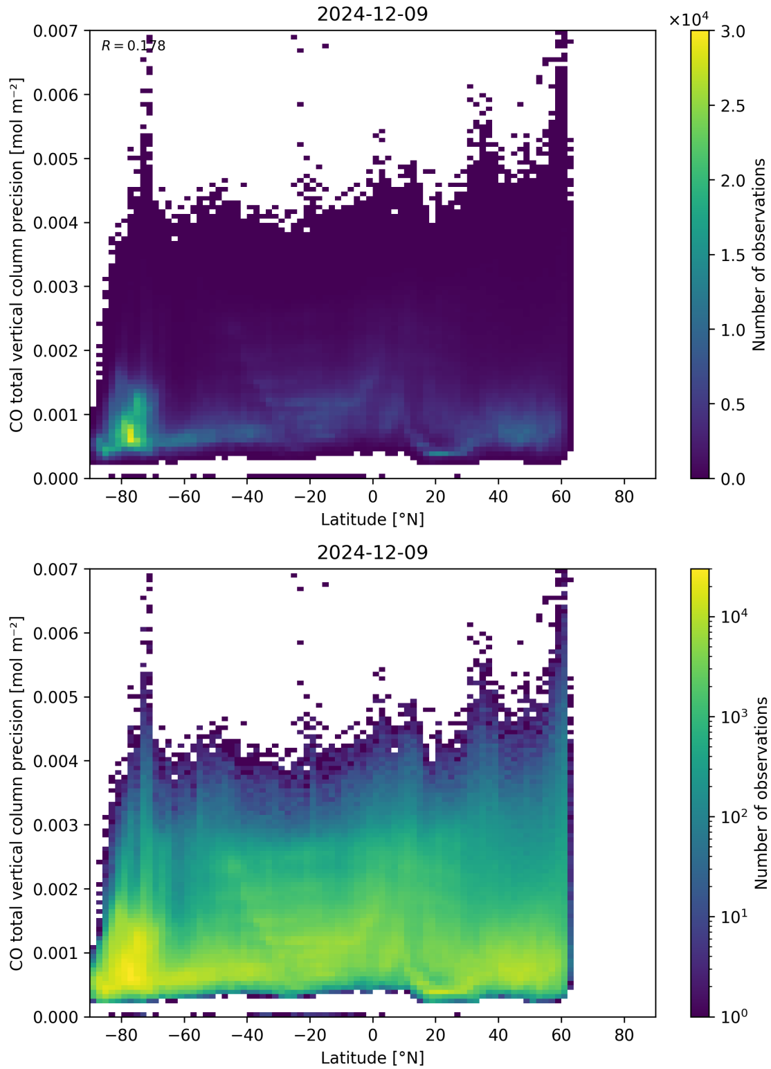
Figure 53: Scatter density plot of “Latitude” against “CO total vertical column precision” for 2024-12-08 to 2024-12-10.
