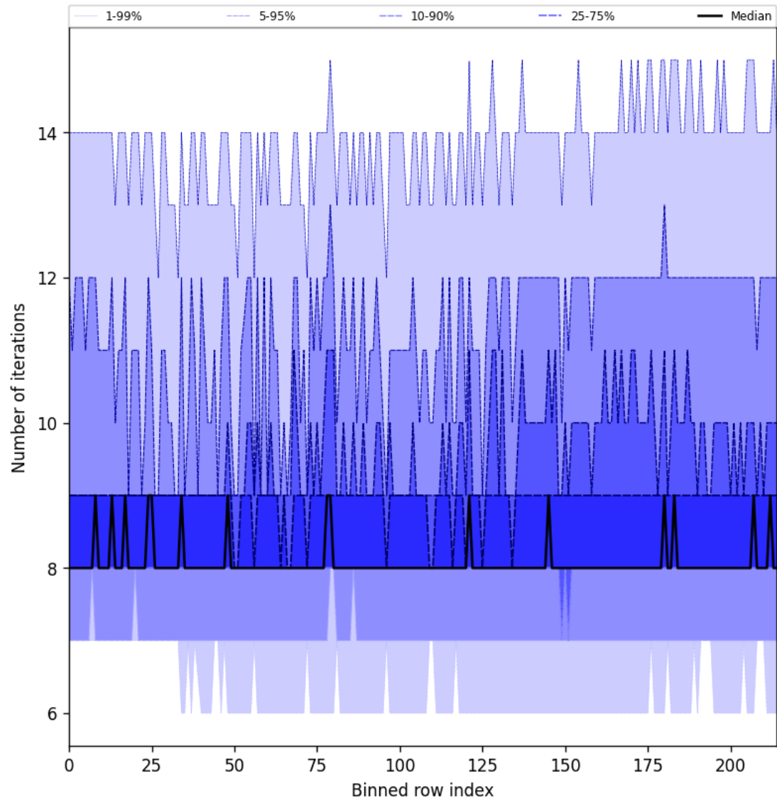
Figure 32: Along track statistics of “Number of iterations” for 2024-12-08 to 2024-12-10
