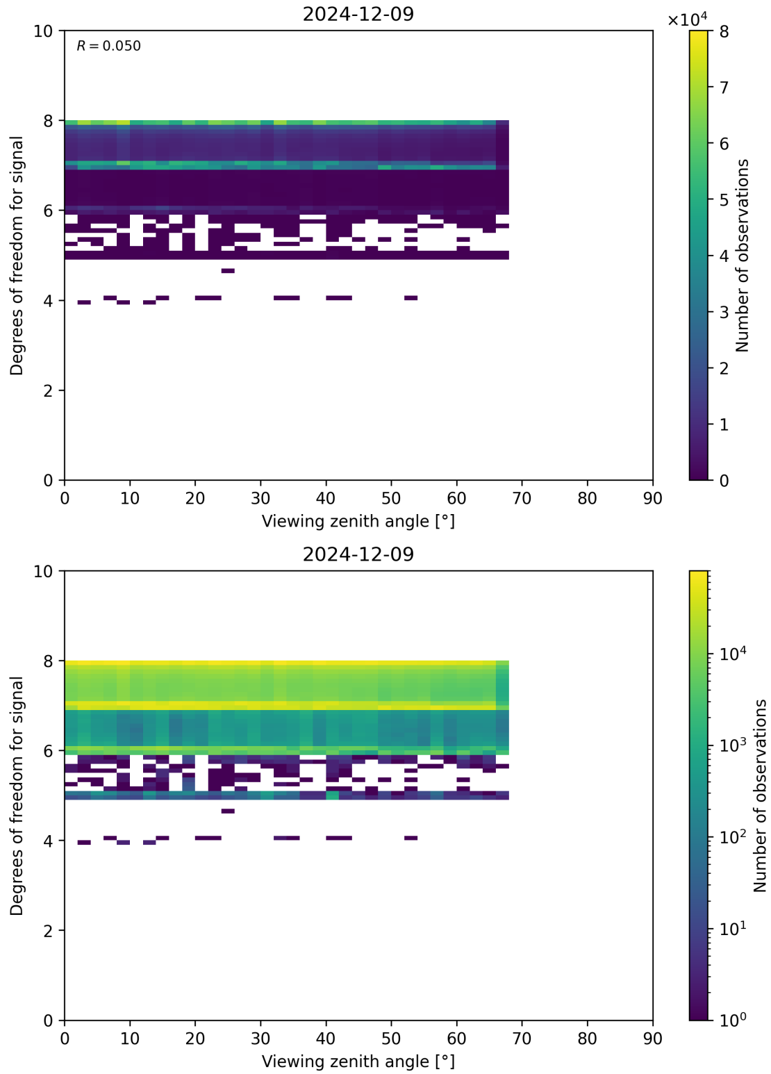
Figure 73: Scatter density plot of “Viewing zenith angle” against “Degrees of freedom for signal” for 2024-12-08 to 2024-12-10.
