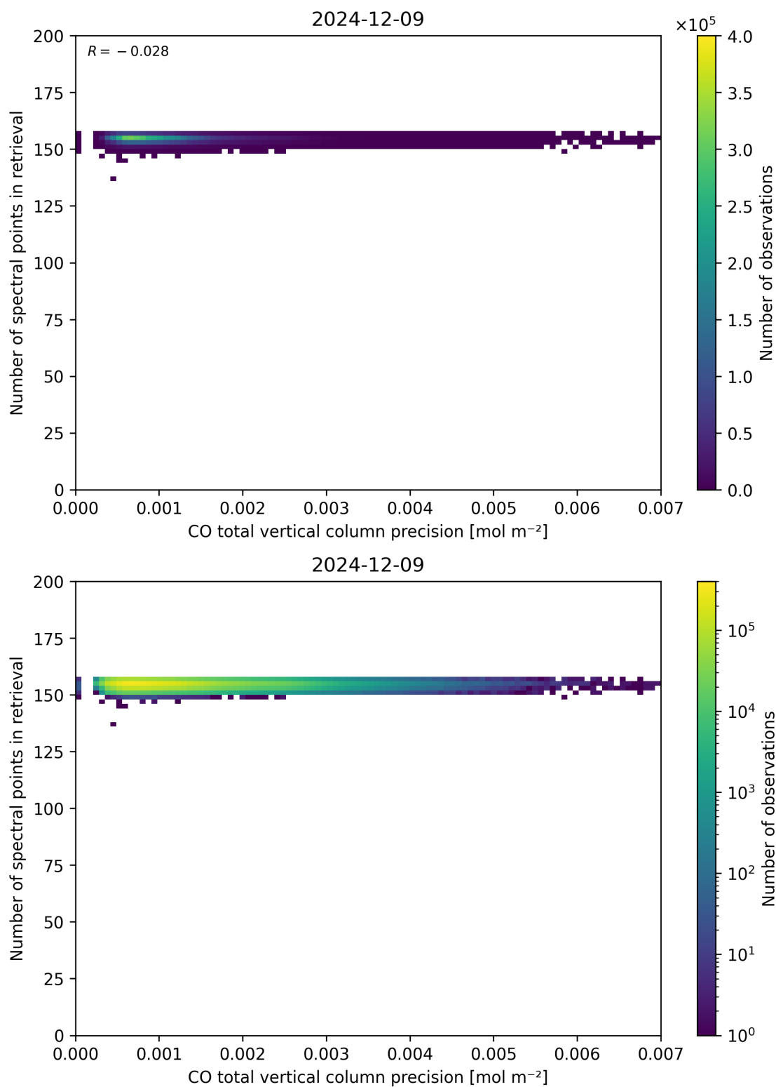
Figure 47: Scatter density plot of “CO total vertical column precision” against “Number of spectral points in retrieval” for 2024-12-08 to 2024-12-10.
