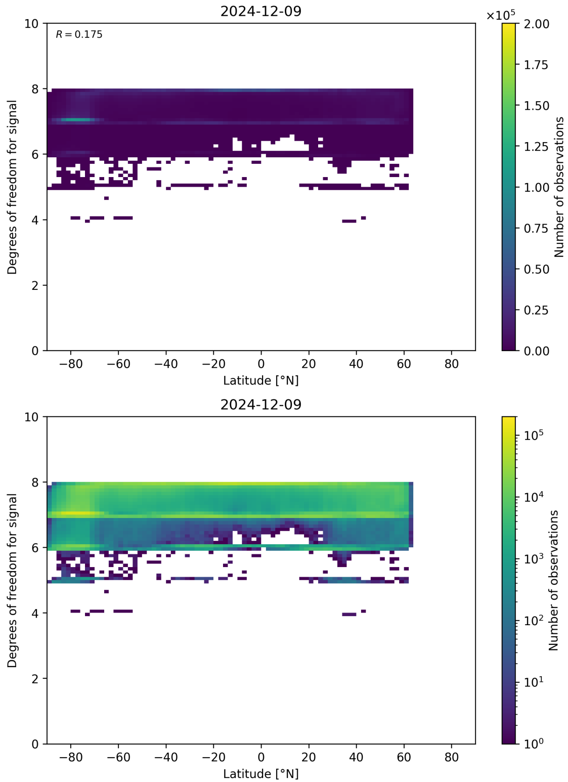
Figure 55: Scatter density plot of “Latitude” against “Degrees of freedom for signal” for 2024-12-08 to 2024-12-10.
