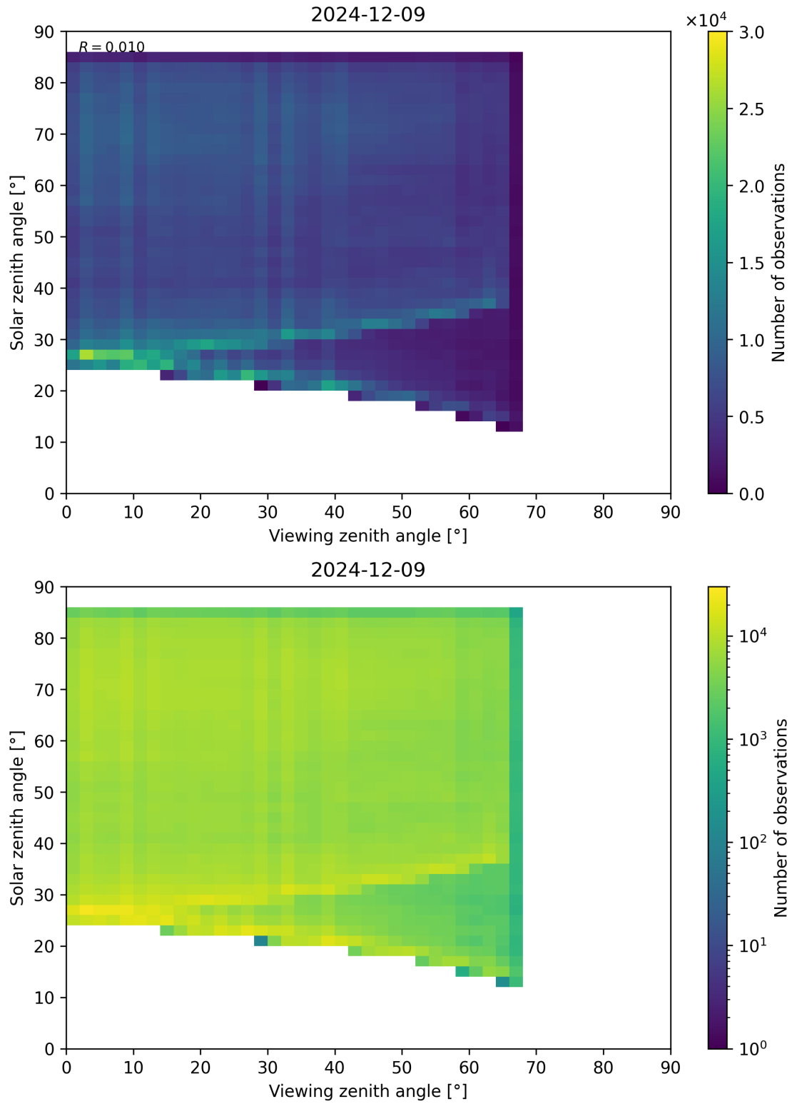
Figure 77: Scatter density plot of “Viewing zenith angle” against “Solar zenith angle” for 2024-12-08 to 2024-12-10.
