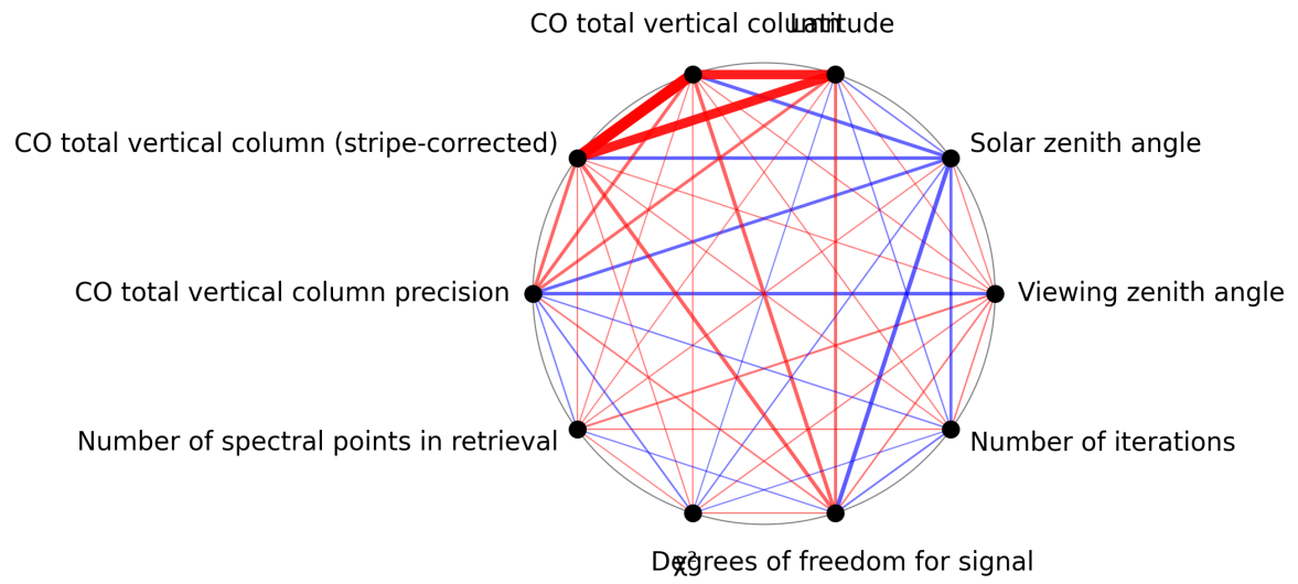
Figure 1: Map of correlation graph for 2024-12-08 to 2024-12-10.
