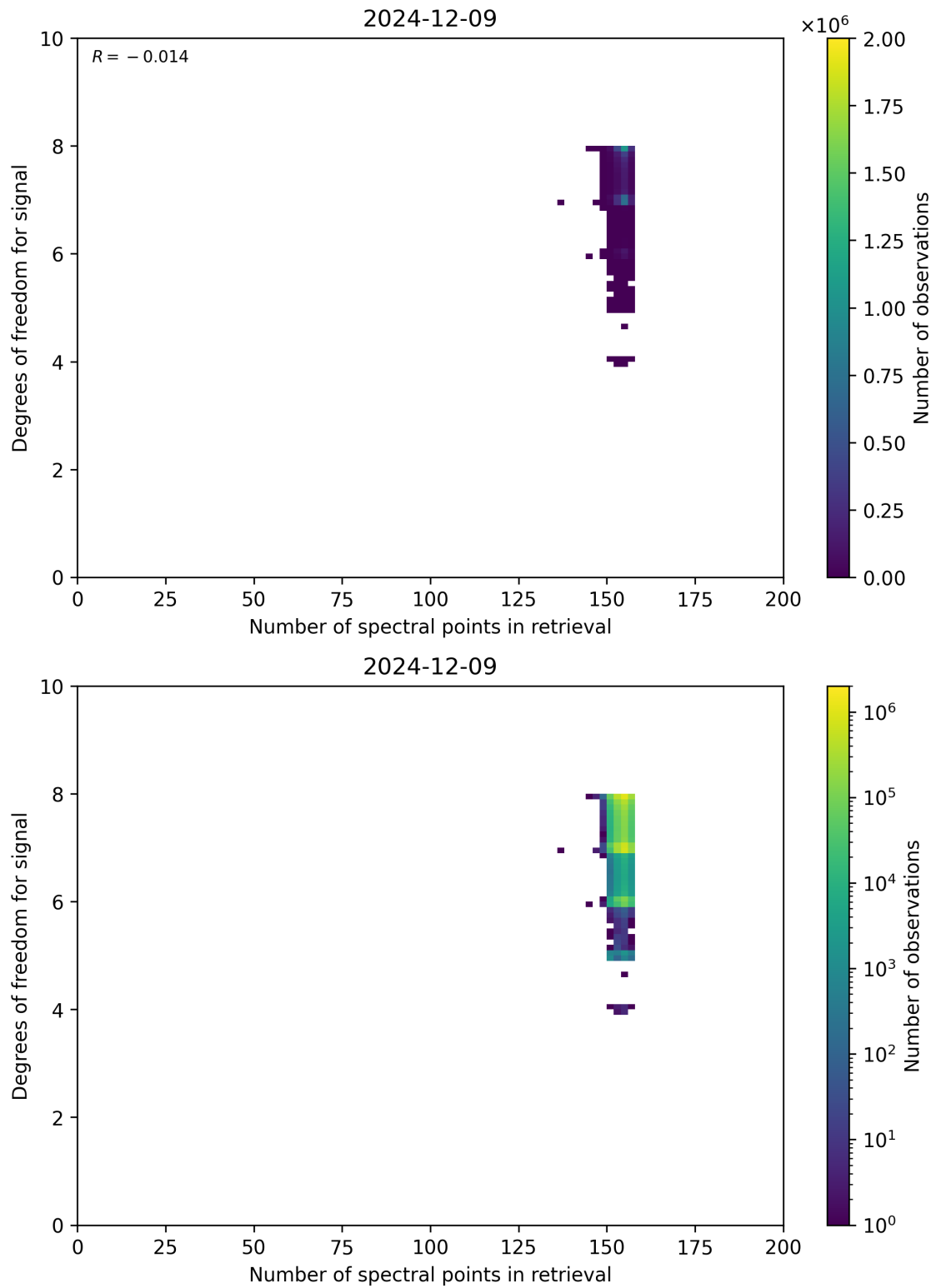
Figure 59: Scatter density plot of “Number of spectral points in retrieval” against “Degrees of freedom for signal” for 2024-12-08 to 2024-12-10.
