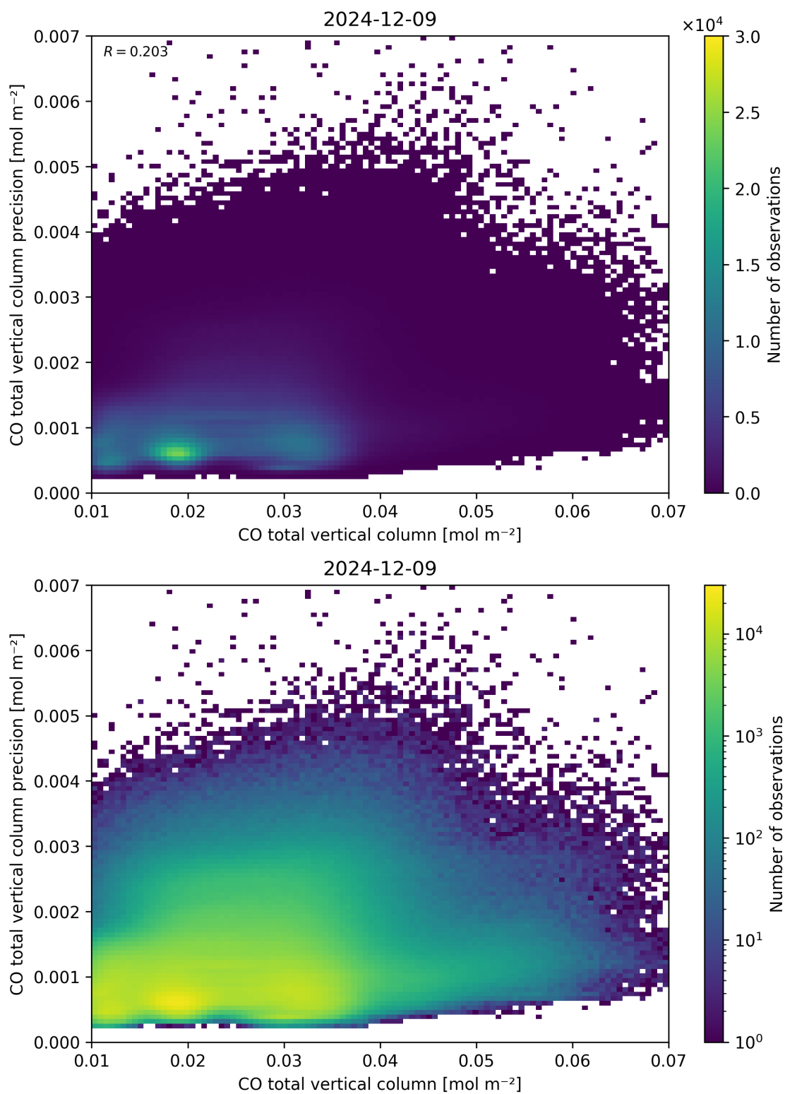
Figure 34: Scatter density plot of “CO total vertical column” against “CO total vertical column precision” for 2024-12-08 to 2024-12-10.
