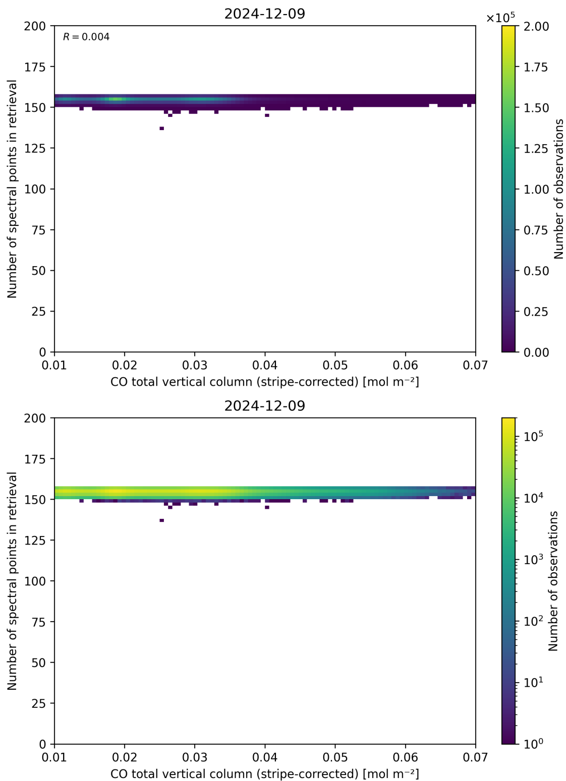
Figure 40: Scatter density plot of “CO total vertical column (stripe-corrected)” against “Number of spectral points in retrieval” for 2024-12-08 to 2024-12-10.
