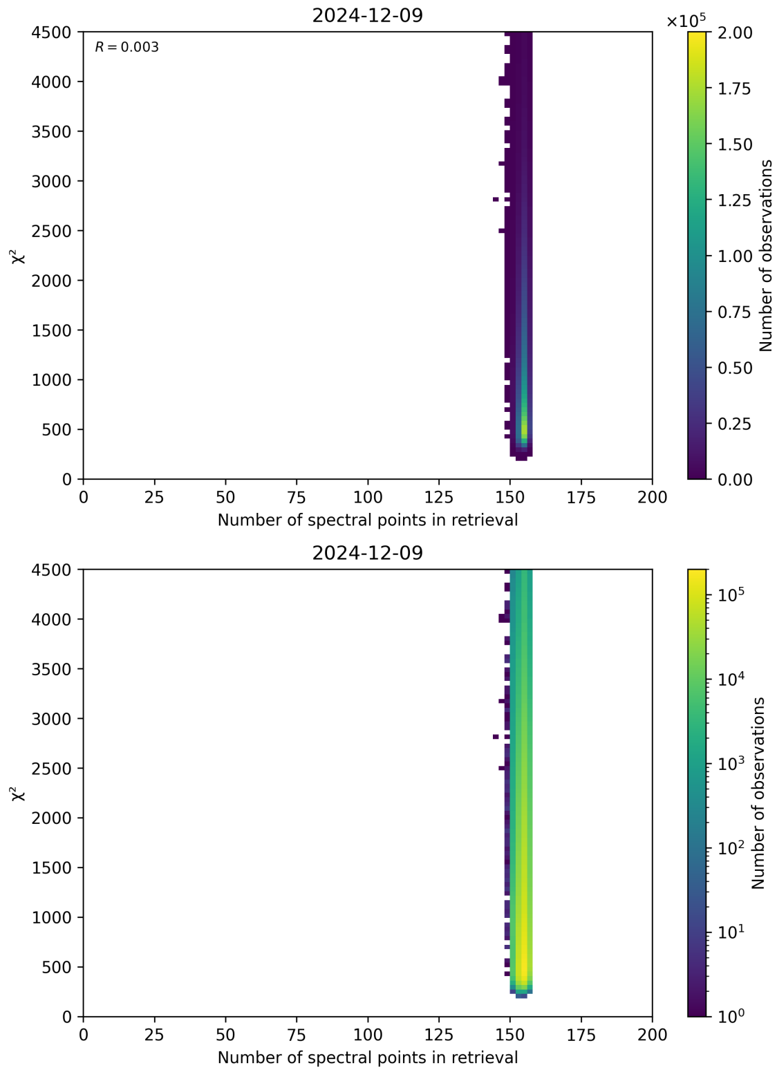
Figure 58: Scatter density plot of “Number of spectral points in retrieval” against “ \chi^2 ” for 2024-12-08 to 2024-12-10.
