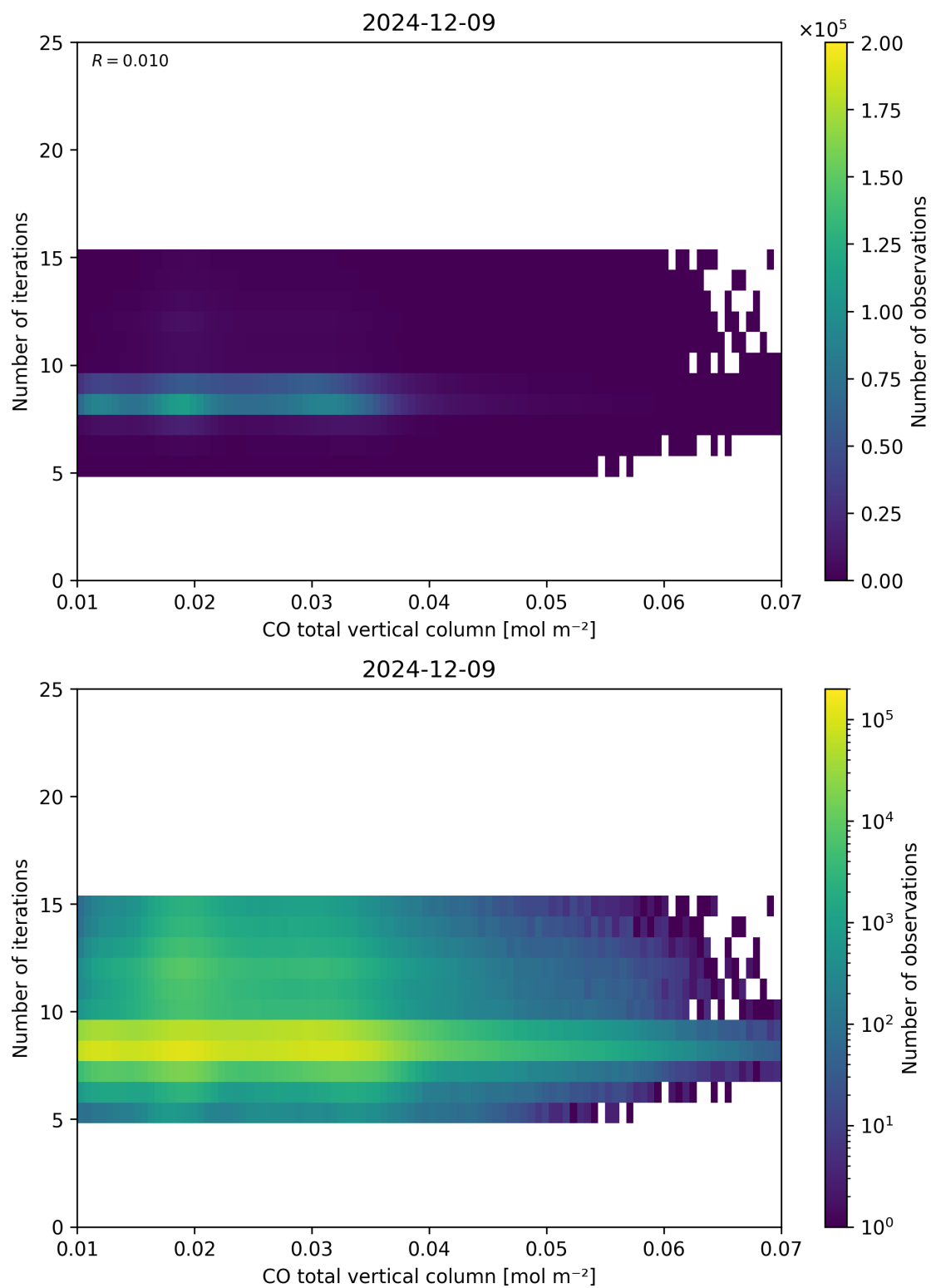
Figure 42: Scatter density plot of “CO total vertical column” against “Number of iterations” for 2024-12-08 to 2024-12-10.
