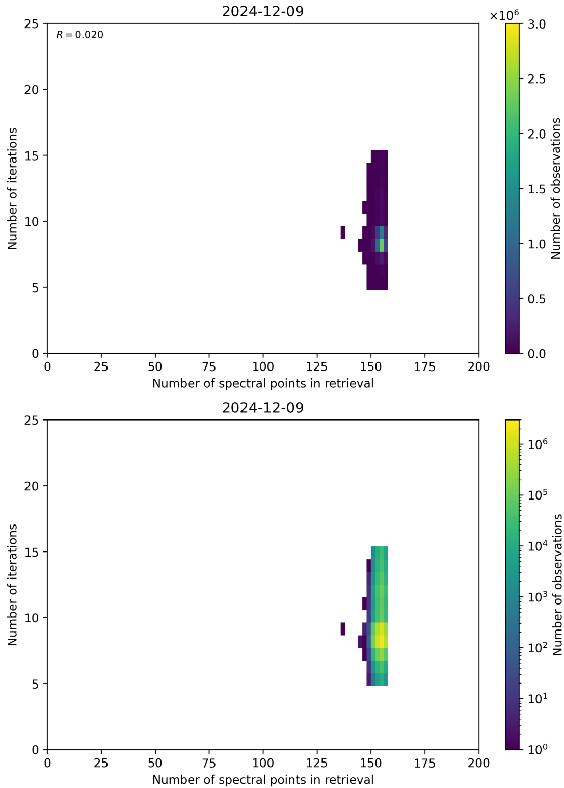
Figure 60: Scatter density plot of “Number of spectral points in retrieval” against “Number of iterations” for 2024-12-08 to 2024-12-10.
