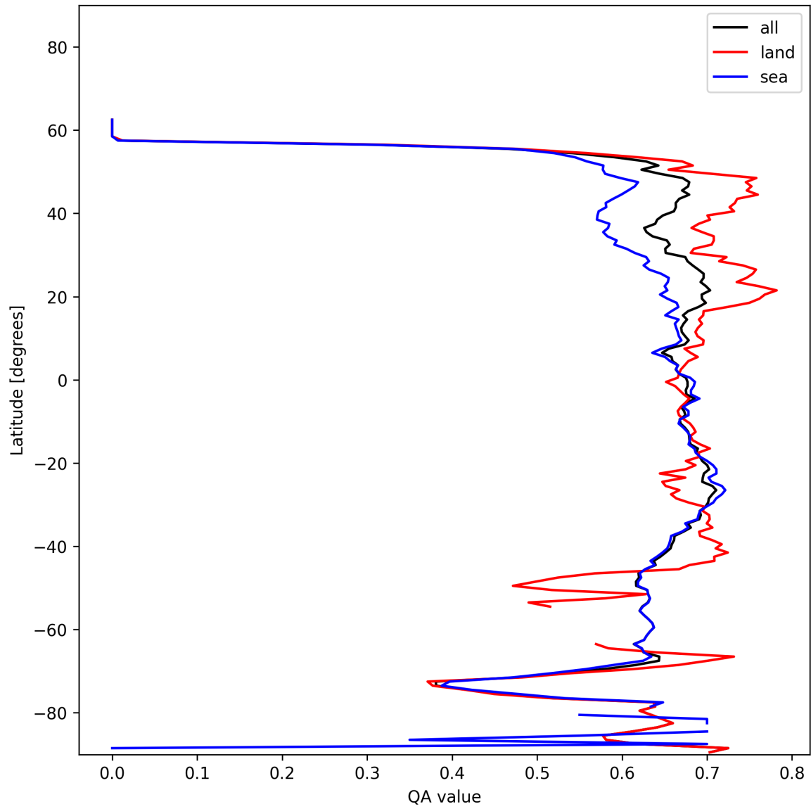
Figure 9: Zonal average of “QA value” for 2024-12-08 to 2024-12-10.
