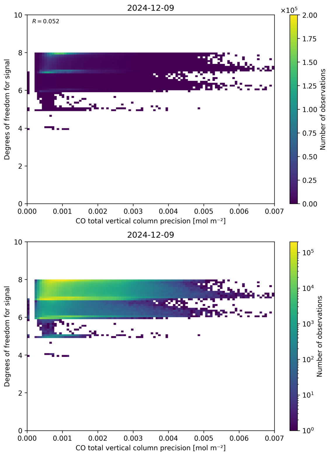
Figure 45: Scatter density plot of “CO total vertical column precision” against “Degrees of freedom for signal” for 2024-12-08 to 2024-12-10.
