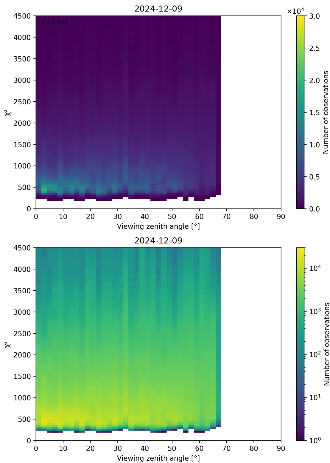
Figure 72: Scatter density plot of “Viewing zenith angle” against “ \chi^2 ” for 2024-12-08 to 2024-12-10.
