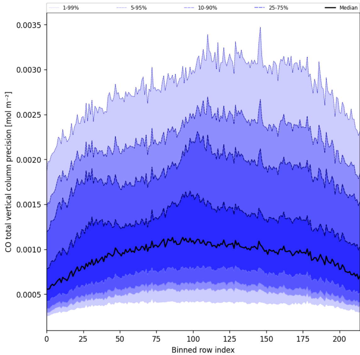
Figure 28: Along track statistics of “CO total vertical column precision” for 2024-12-08 to 2024-12-10
