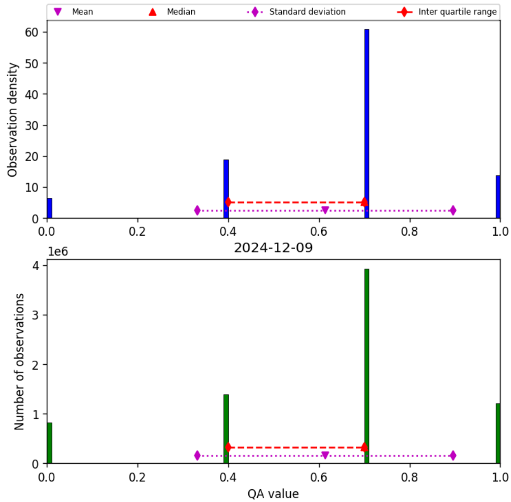
Figure 17: Histogram of “QA value” for 2024-12-08 to 2024-12-10
