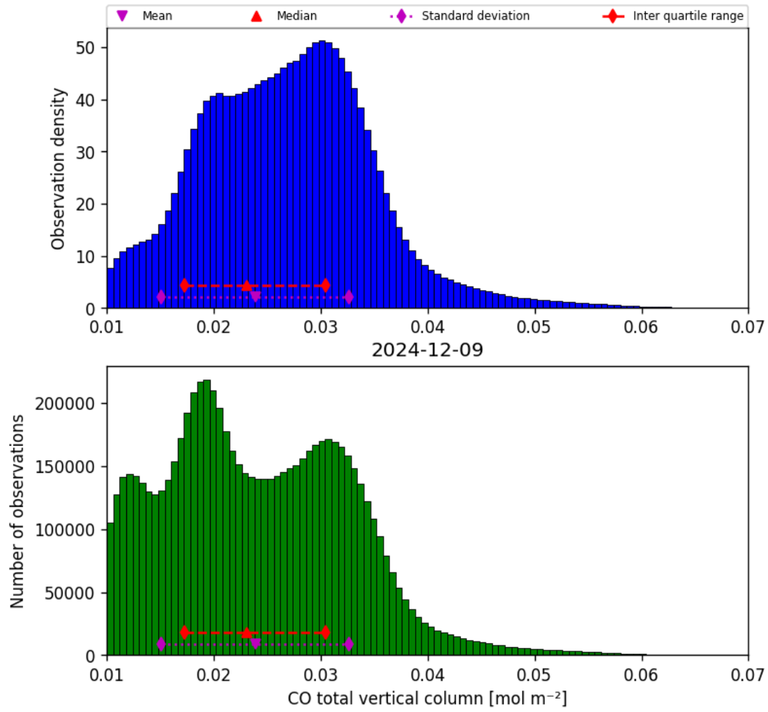
Figure 18: Histogram of “CO total vertical column” for 2024-12-08 to 2024-12-10
