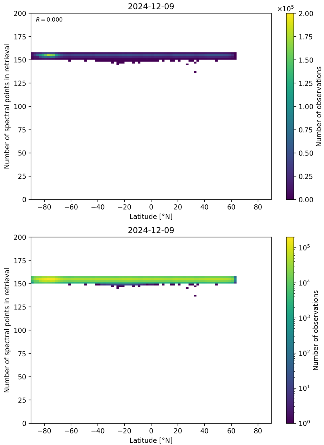
Figure 57: Scatter density plot of “Latitude” against “Number of spectral points in retrieval” for 2024-12-08 to 2024-12-10.
