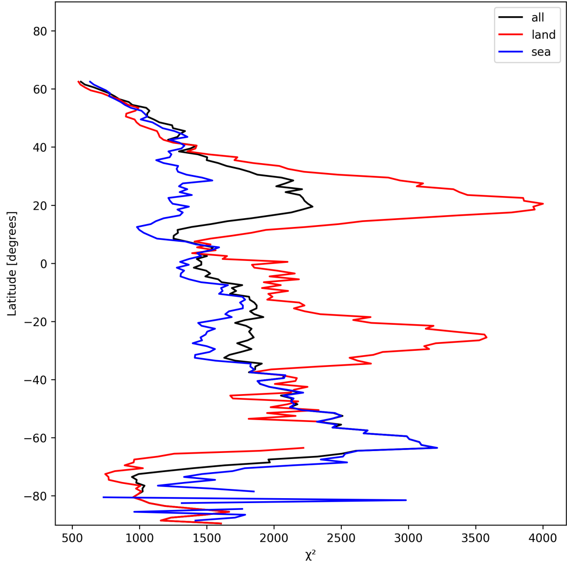
Figure 14: Zonal average of “ \chi^2 ” for 2024-12-08 to 2024-12-10.
