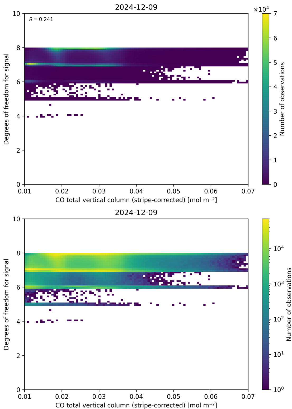
Figure 38: Scatter density plot of “CO total vertical column (stripe-corrected)” against “Degrees of freedom for signal” for 2024-12-08 to 2024-12-10.
