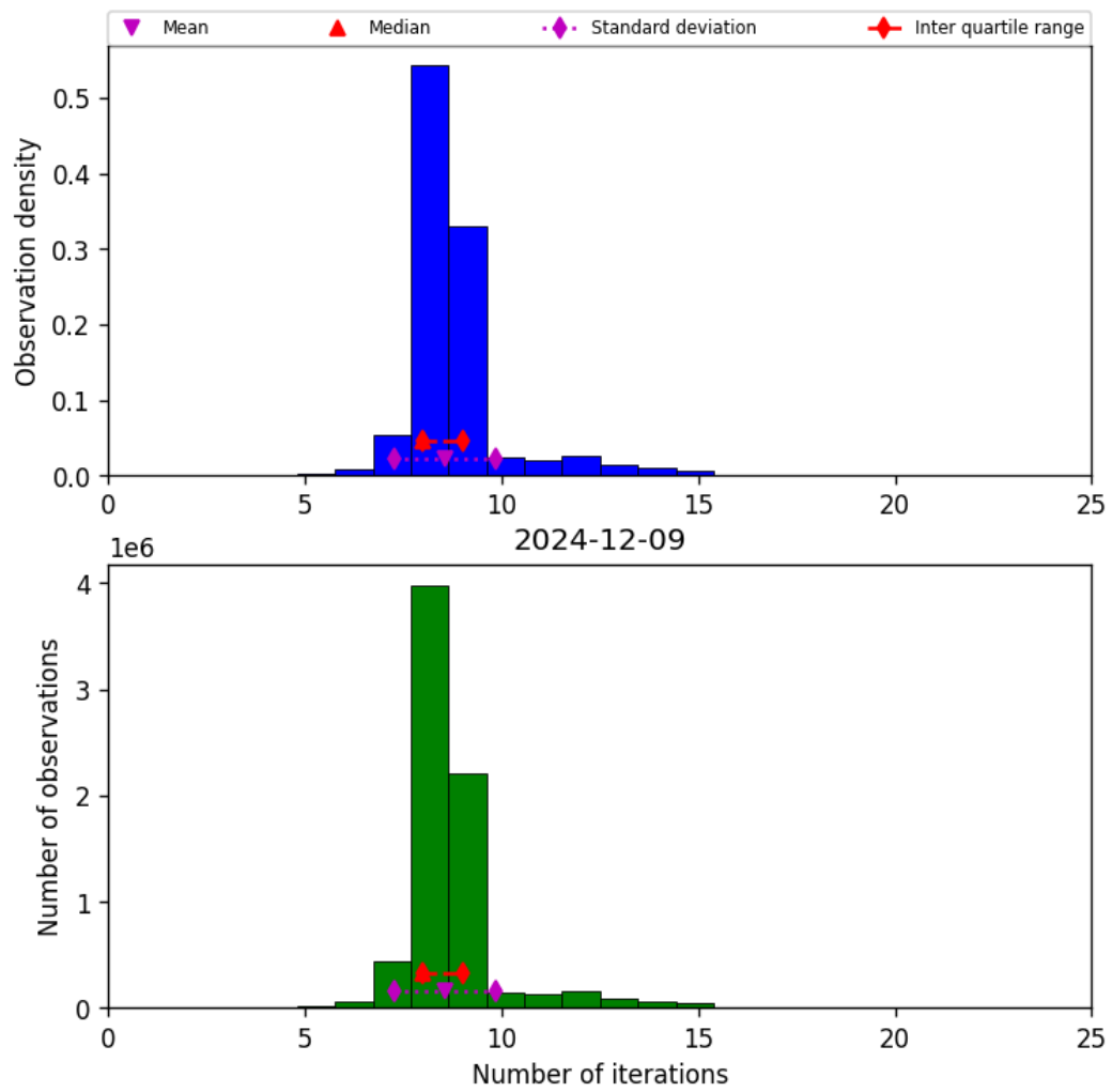
Figure 24: Histogram of “Number of iterations” for 2024-12-08 to 2024-12-10
