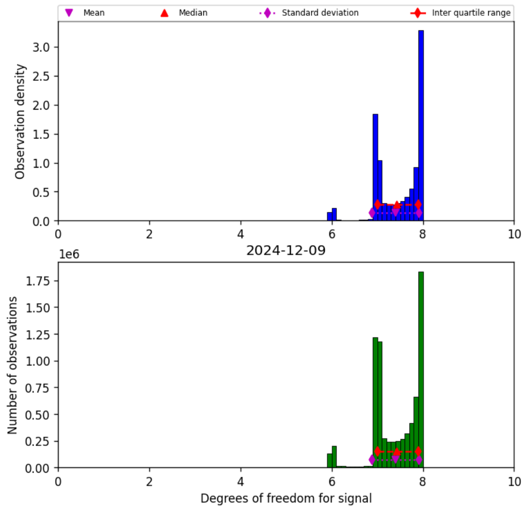
Figure 23: Histogram of “Degrees of freedom for signal” for 2024-12-08 to 2024-12-10
