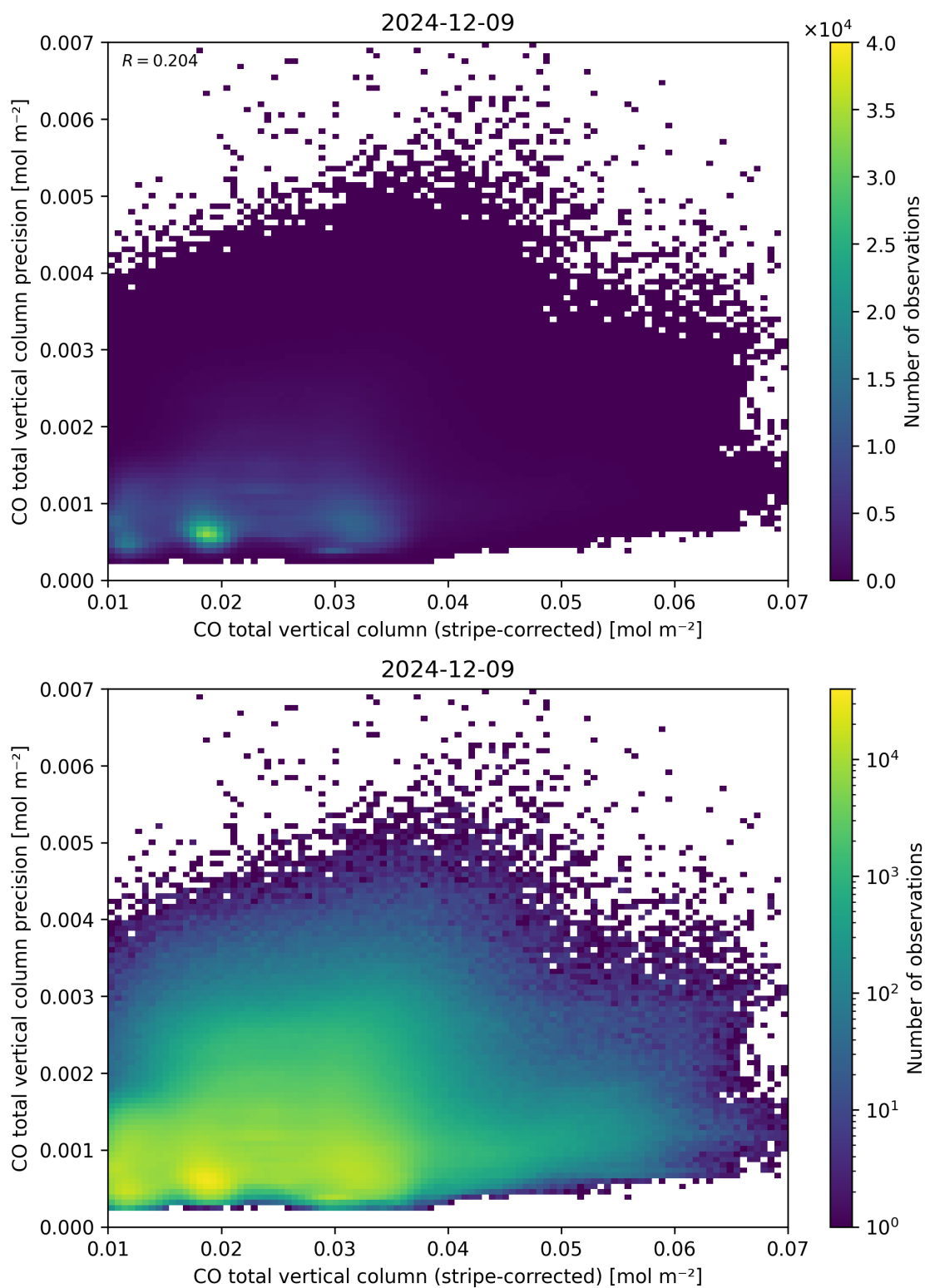
Figure 36: Scatter density plot of “CO total vertical column (stripe-corrected)” against “CO total vertical column precision” for 2024-12-08 to 2024-12-10.
