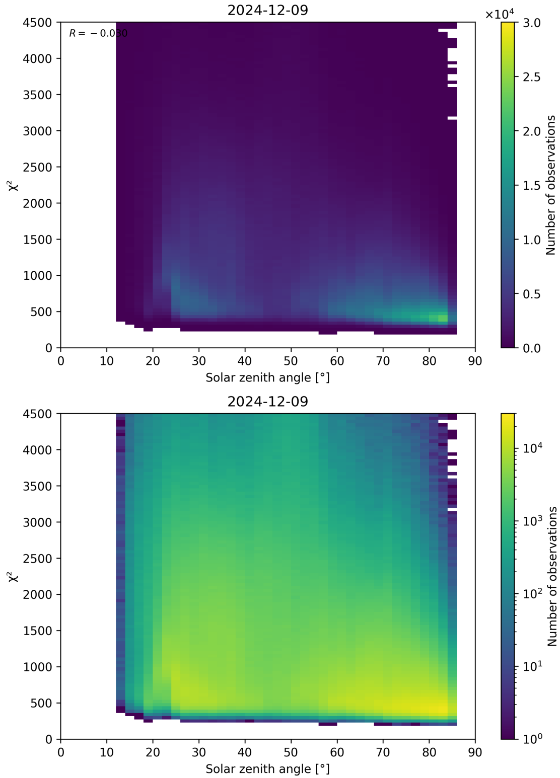
Figure 64: Scatter density plot of “Solar zenith angle” against “ \chi^2 ” for 2024-12-08 to 2024-12-10.
