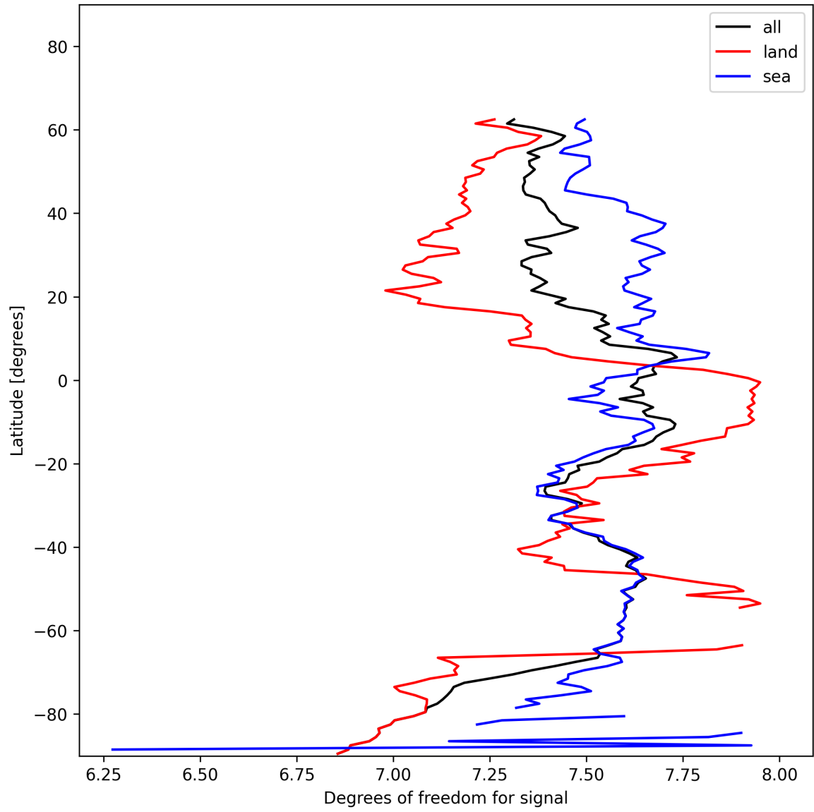
Figure 15: Zonal average of “Degrees of freedom for signal” for 2024-12-08 to 2024-12-10.
