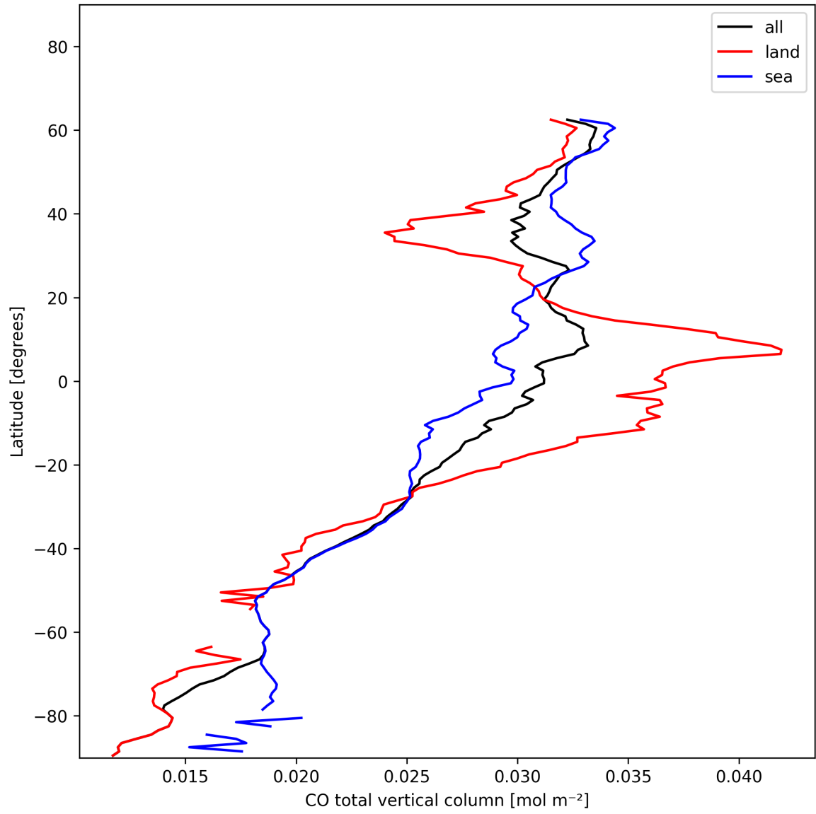
Figure 10: Zonal average of “CO total vertical column” for 2024-12-08 to 2024-12-10.
