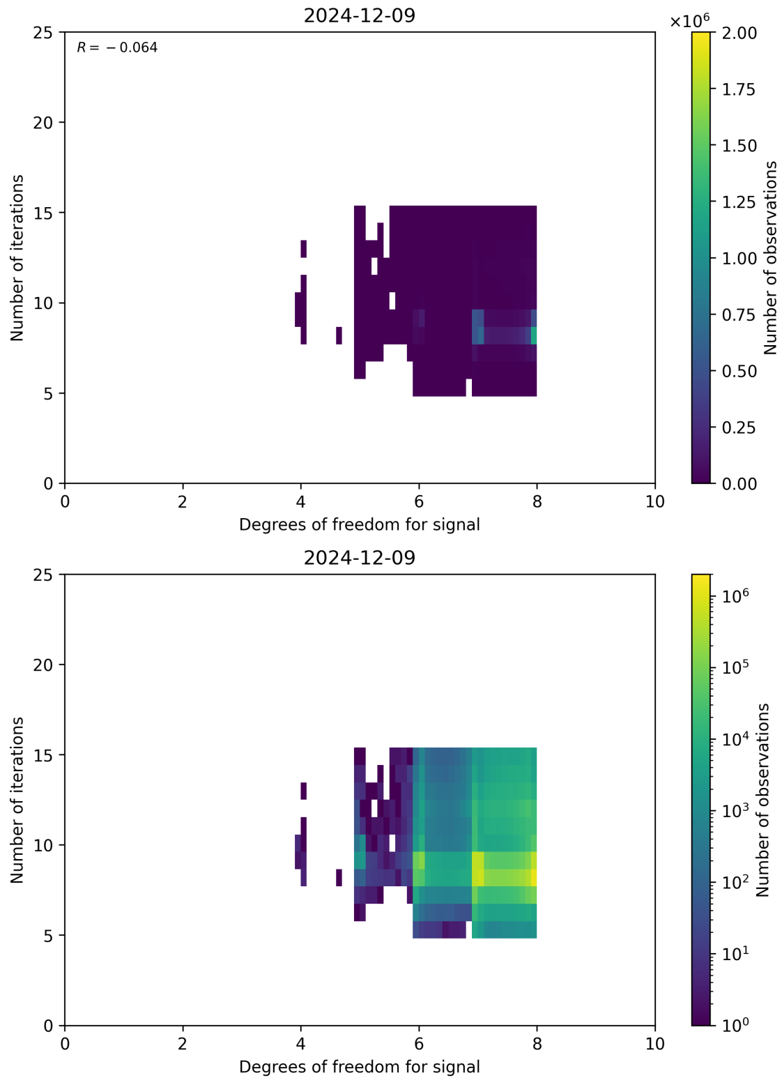
Figure 50: Scatter density plot of “Degrees of freedom for signal” against “Number of iterations” for 2024-12-08 to 2024-12-10.
