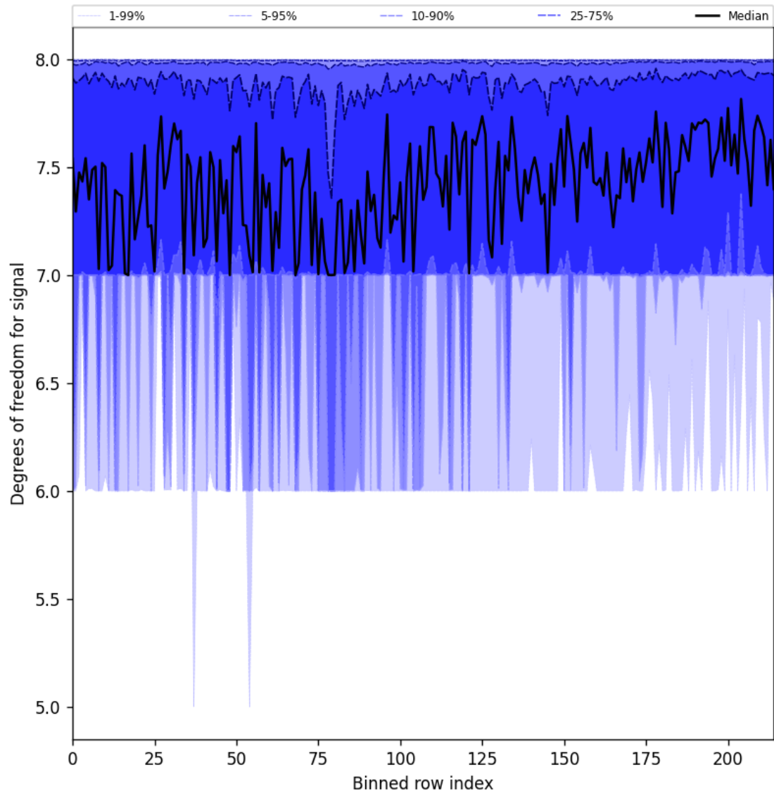
Figure 31: Along track statistics of “Degrees of freedom for signal” for 2024-12-08 to 2024-12-10
