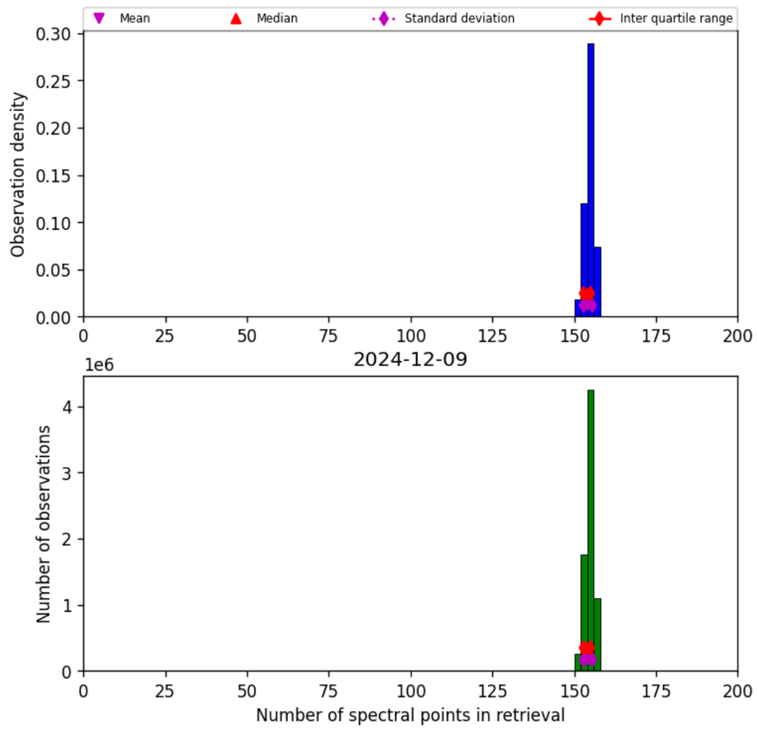
Figure 21: Histogram of “Number of spectral points in retrieval” for 2024-12-08 to 2024-12-10
