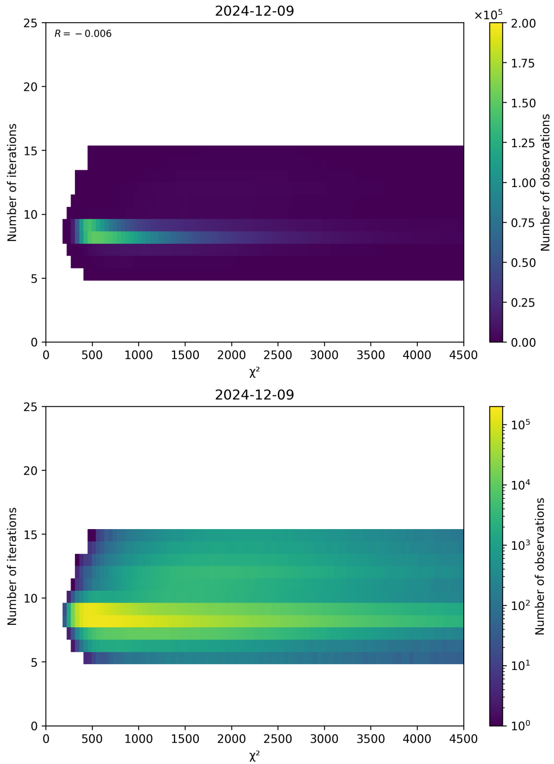
Figure 49: Scatter density plot of “ \chi^2 ” against “Number of iterations” for 2024-12-08 to 2024-12-10.
