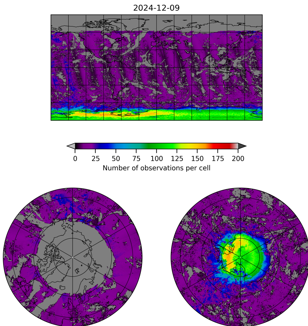
Figure 8: Map of the number of observations for 2024-12-08 to 2024-12-10
