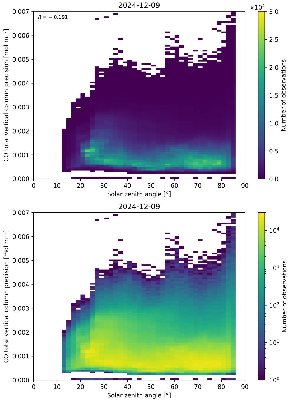
Figure 63: Scatter density plot of “Solar zenith angle” against “CO total vertical column precision” for 2024-12-08 to 2024-12-10.
