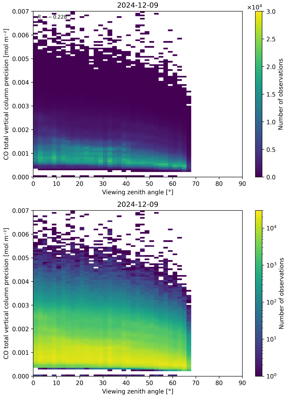
Figure 71: Scatter density plot of “Viewing zenith angle” against “CO total vertical column precision” for 2024-12-08 to 2024-12-10.
