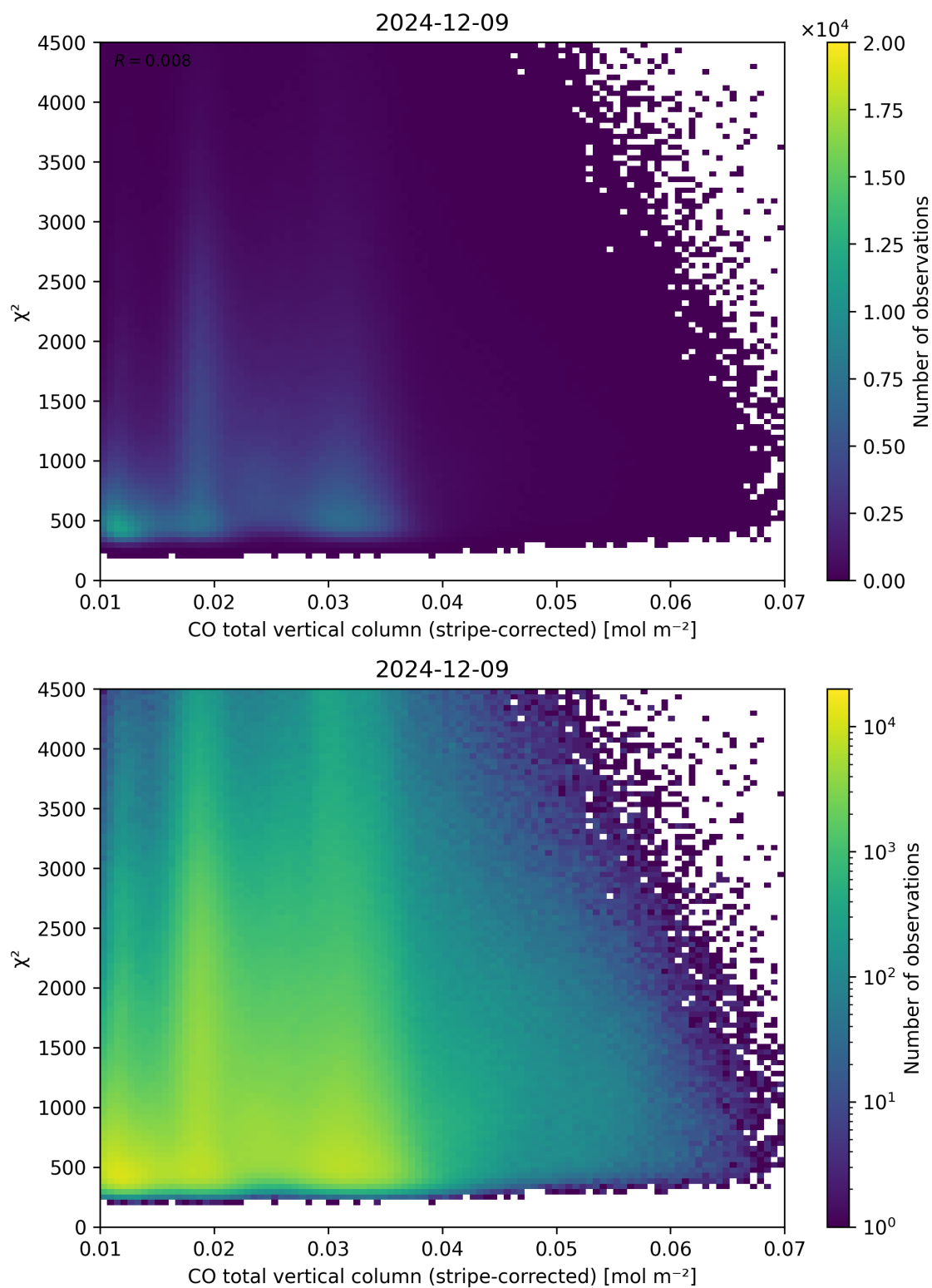
Figure 37: Scatter density plot of “CO total vertical column (stripe-corrected)” against “ \chi^2 ” for 2024-12-08 to 2024-12-10.
