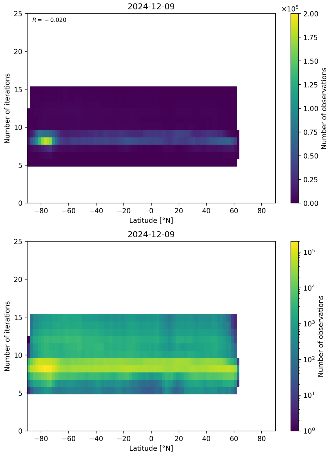
Figure 56: Scatter density plot of “Latitude” against “Number of iterations” for 2024-12-08 to 2024-12-10.
