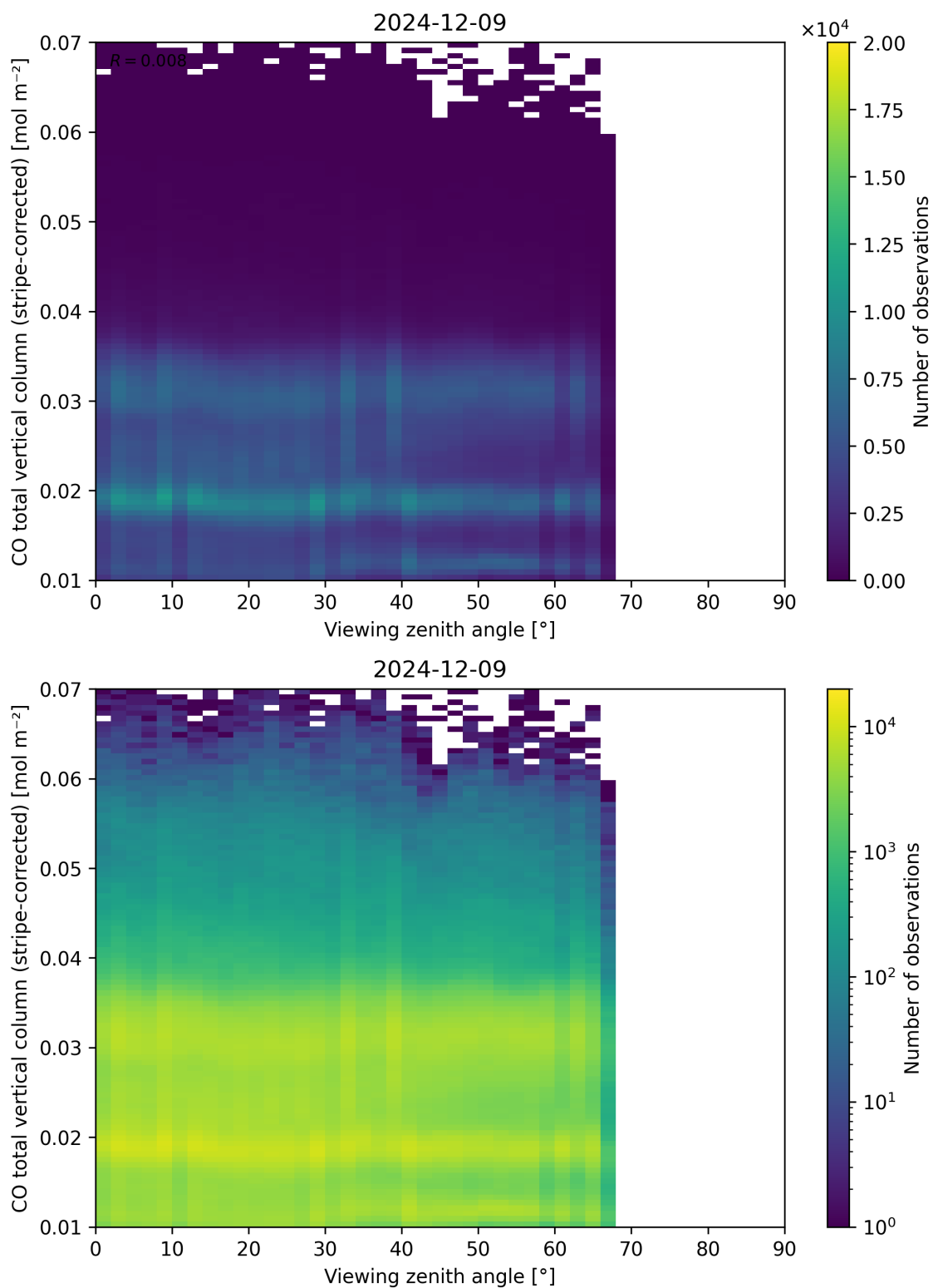
Figure 70: Scatter density plot of “Viewing zenith angle” against “CO total vertical column (stripe-corrected)” for 2024-12-08 to 2024-12-10.
