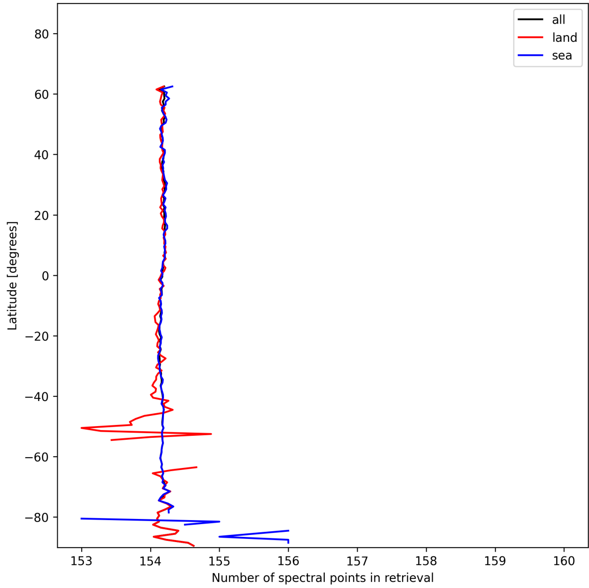
Figure 13: Zonal average of “Number of spectral points in retrieval” for 2024-12-08 to 2024-12-10.
