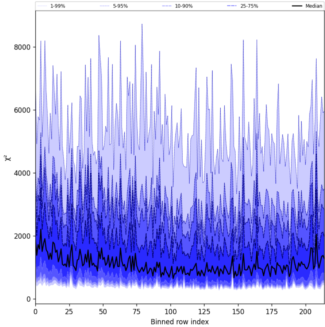
Figure 30: Along track statistics of “ \chi^2 ” for 2024-12-08 to 2024-12-10
