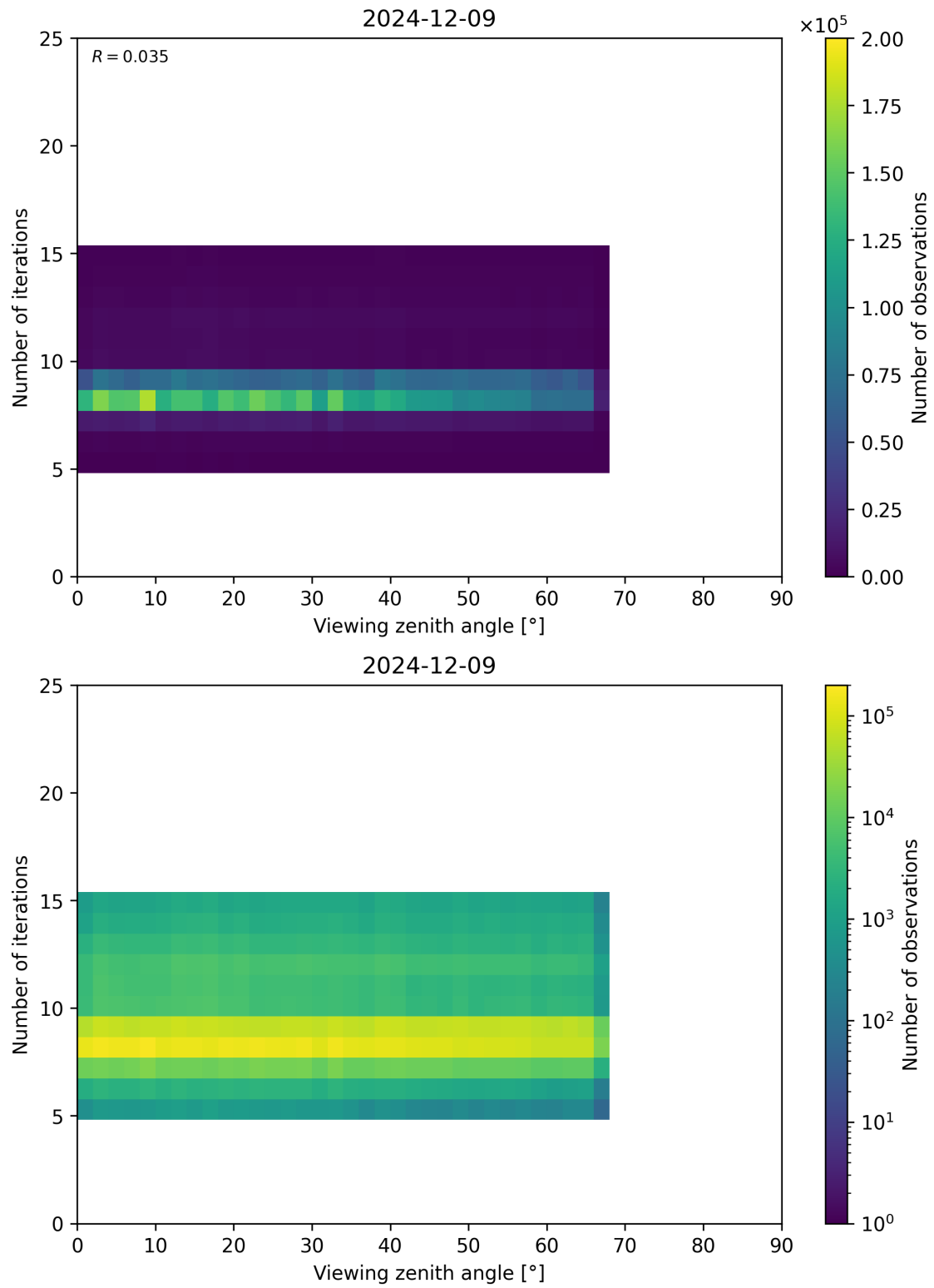
Figure 75: Scatter density plot of “Viewing zenith angle” against “Number of iterations” for 2024-12-08 to 2024-12-10.
