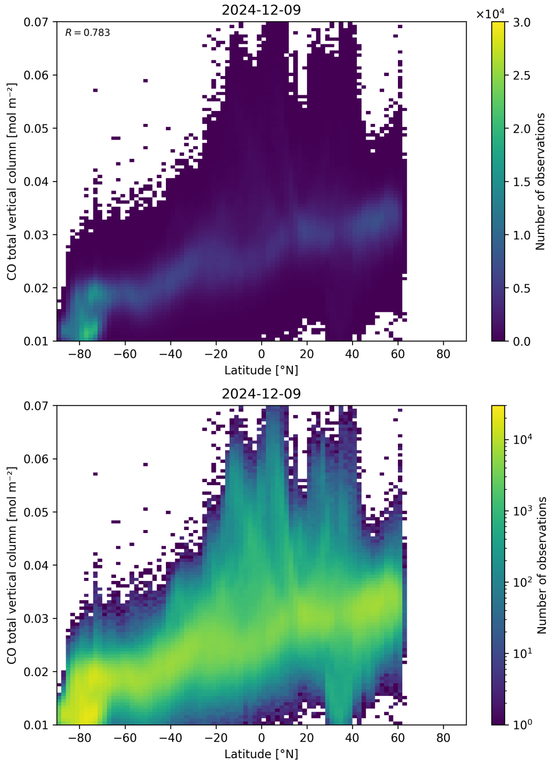
Figure 51: Scatter density plot of “Latitude” against “CO total vertical column” for 2024-12-08 to 2024-12-10.
