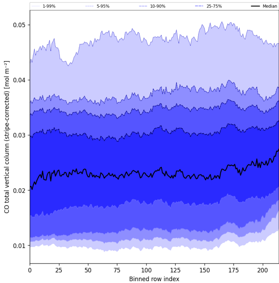
Figure 27: Along track statistics of “CO total vertical column (stripe-corrected)” for 2024-12-08 to 2024-12-10
