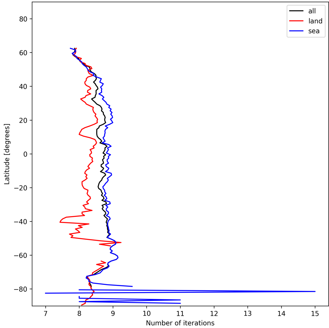
Figure 16: Zonal average of “Number of iterations” for 2024-12-08 to 2024-12-10.
