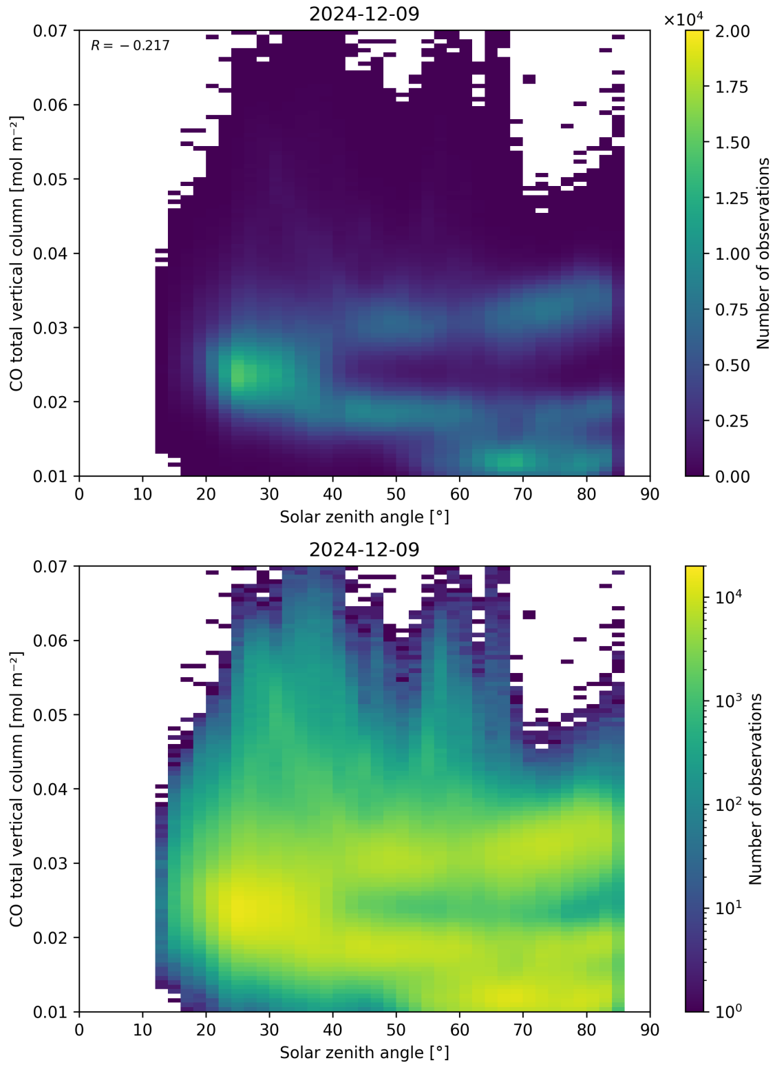
Figure 61: Scatter density plot of “Solar zenith angle” against “CO total vertical column” for 2024-12-08 to 2024-12-10.
