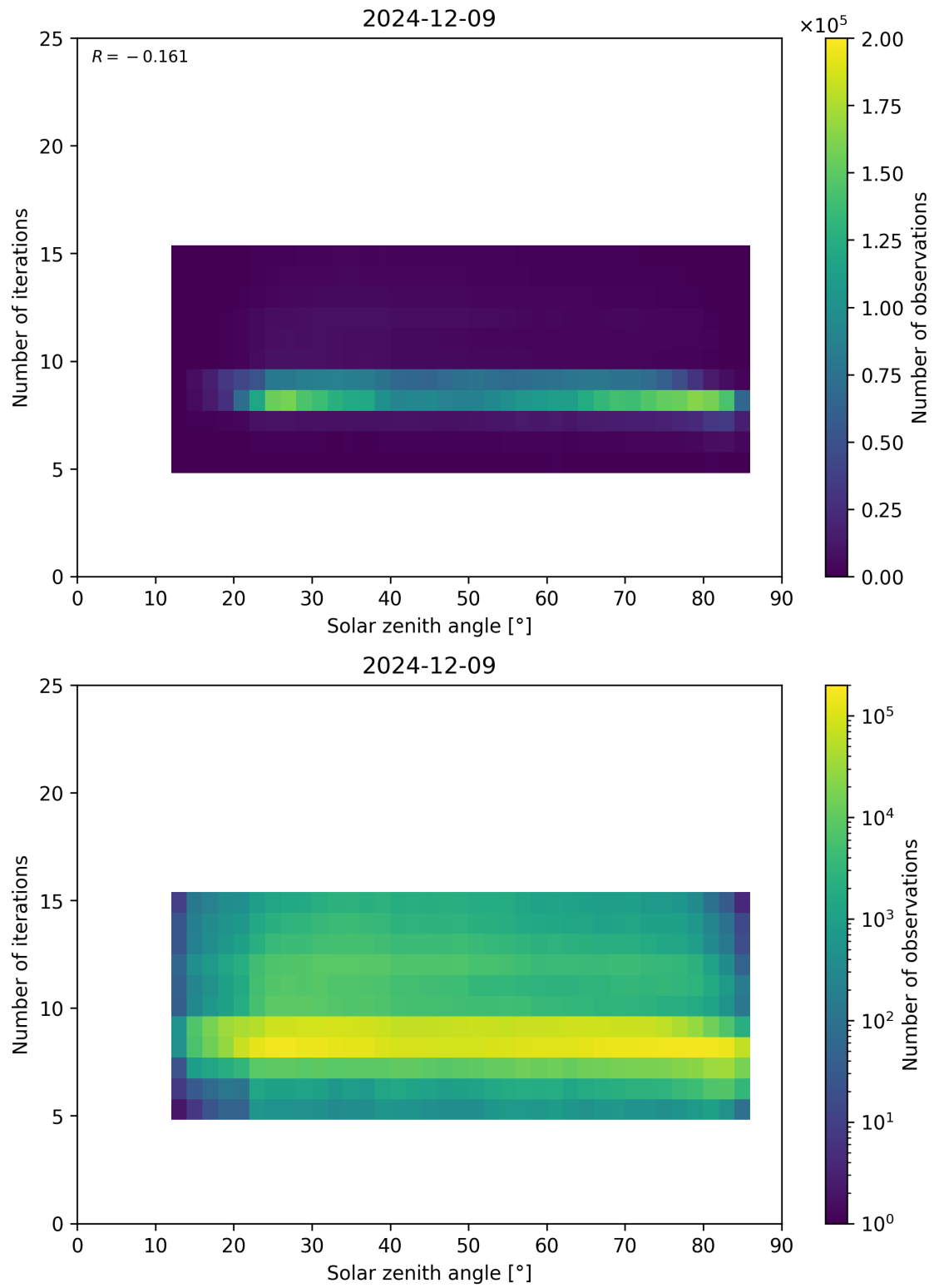
Figure 67: Scatter density plot of “Solar zenith angle” against “Number of iterations” for 2024-12-08 to 2024-12-10.
