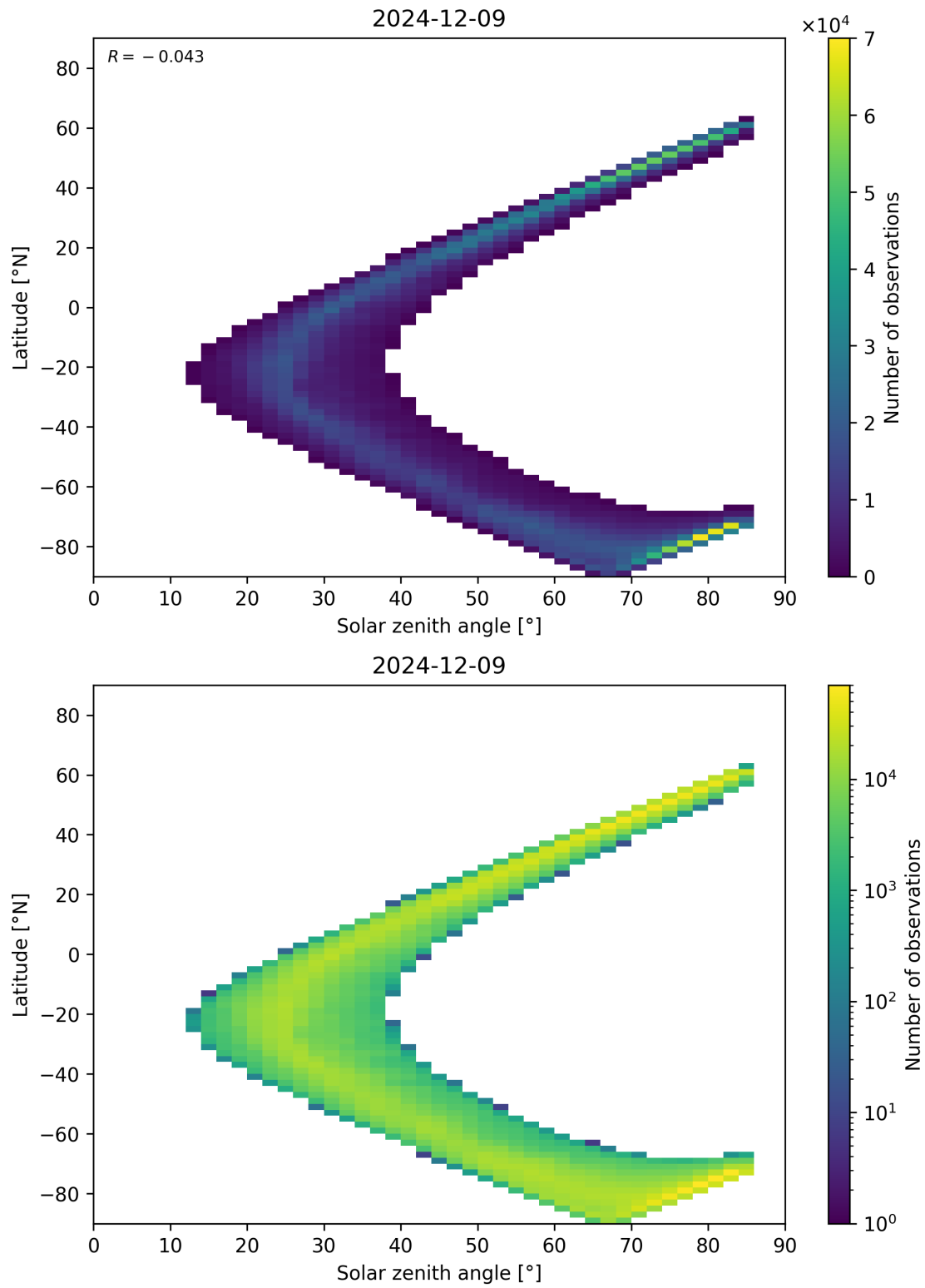
Figure 66: Scatter density plot of “Solar zenith angle” against “Latitude” for 2024-12-08 to 2024-12-10.
