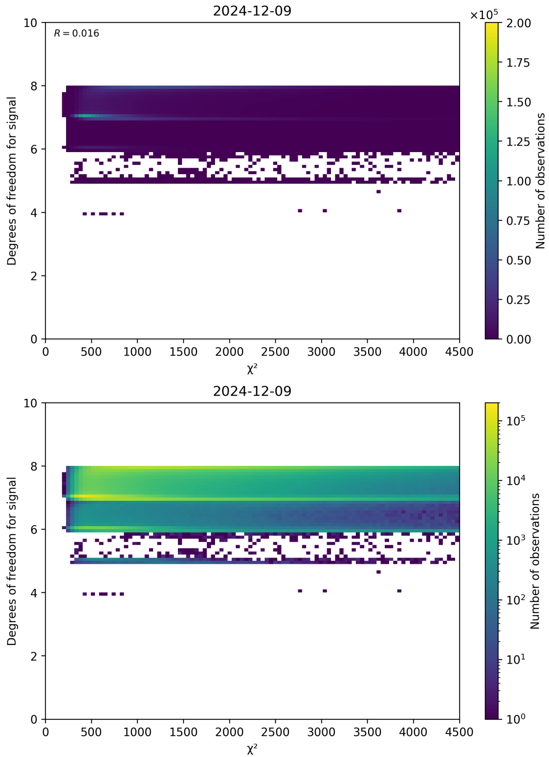
Figure 48: Scatter density plot of “ \chi^2 ” against “Degrees of freedom for signal” for 2024-12-08 to 2024-12-10.
