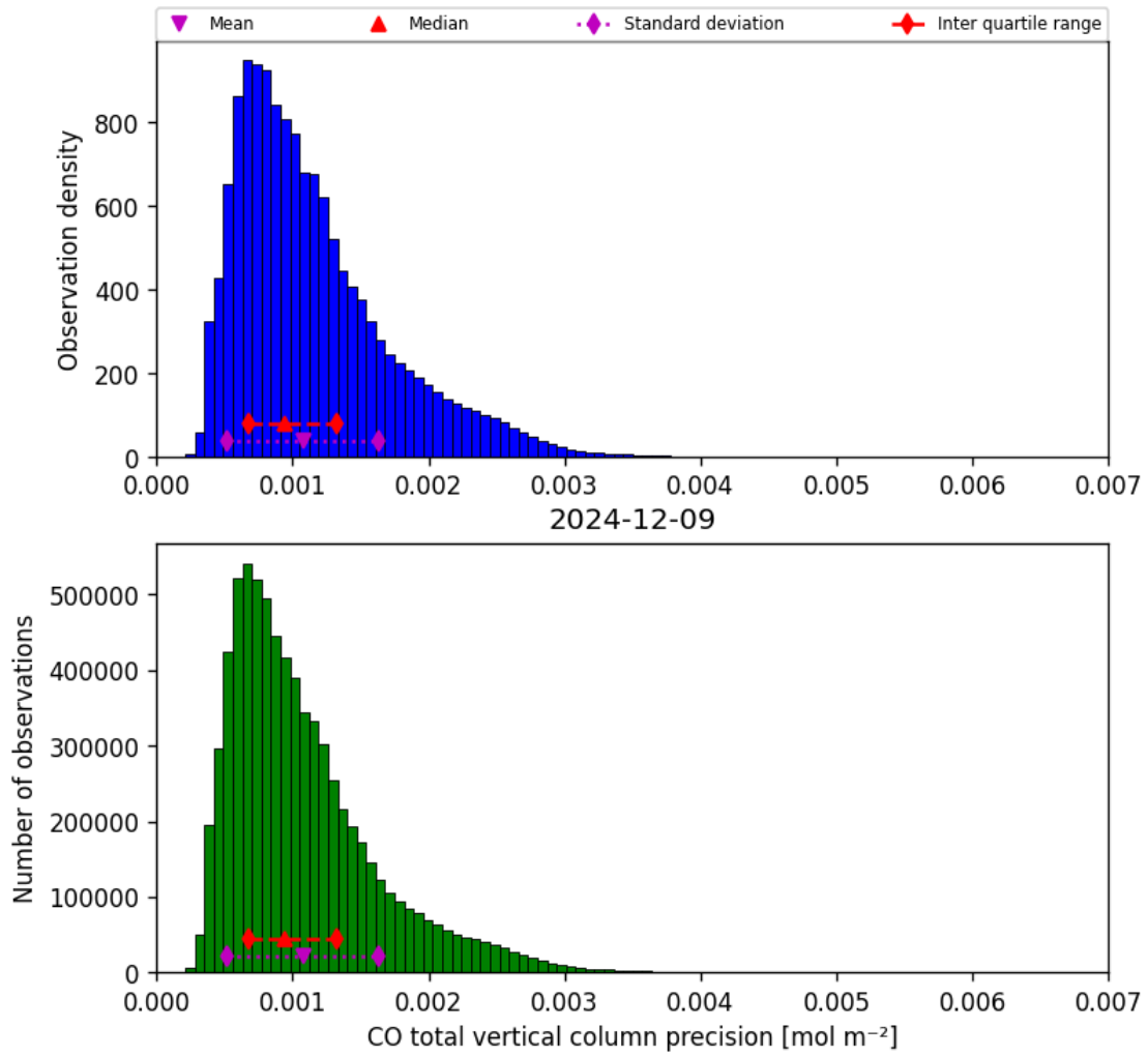
Figure 20: Histogram of “CO total vertical column precision” for 2024-12-08 to 2024-12-10
