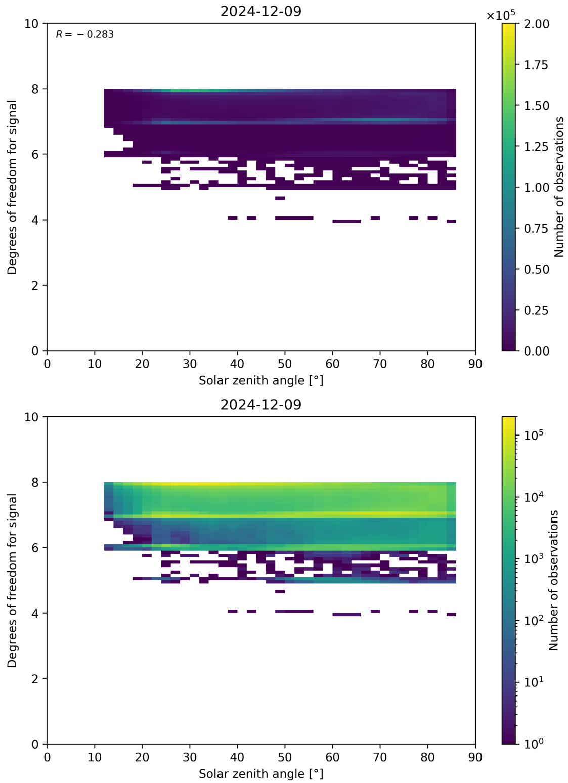
Figure 65: Scatter density plot of “Solar zenith angle” against “Degrees of freedom for signal” for 2024-12-08 to 2024-12-10.
