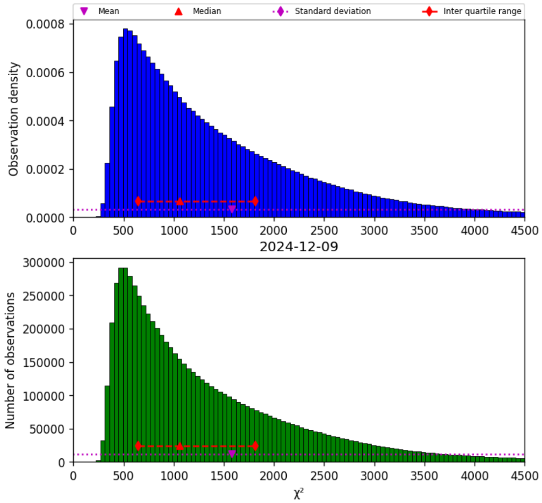
Figure 22: Histogram of “ \chi^2 ” for 2024-12-08 to 2024-12-10
