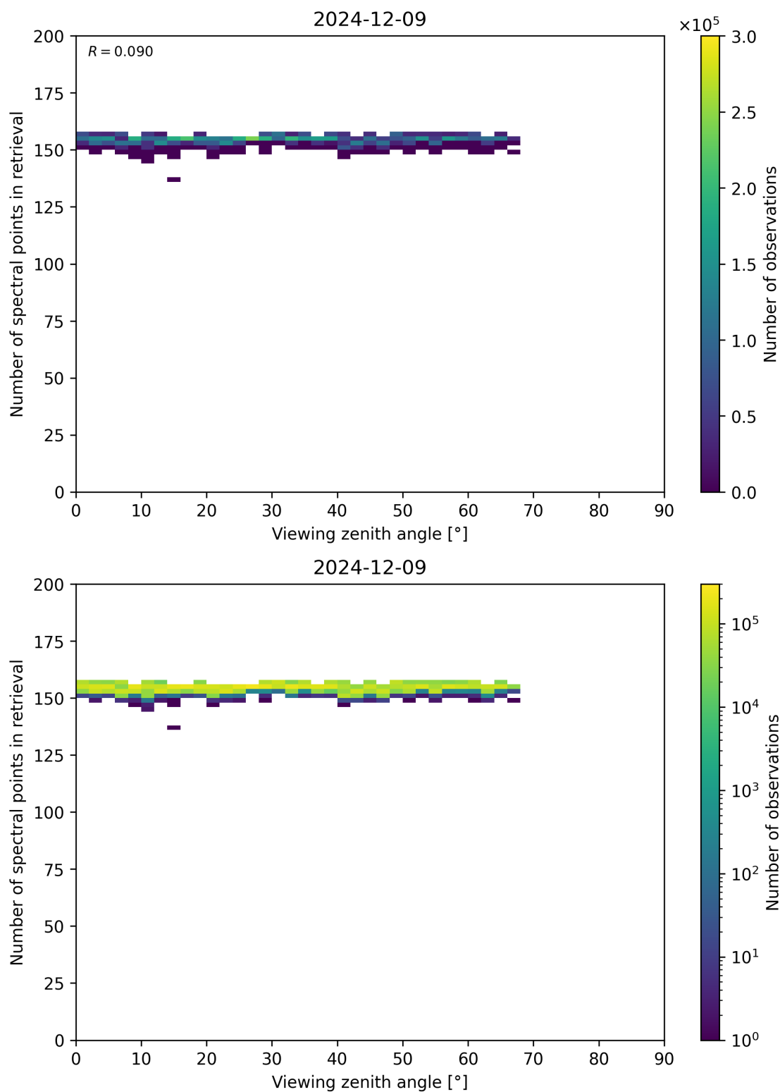
Figure 76: Scatter density plot of “Viewing zenith angle” against “Number of spectral points in retrieval” for 2024-12-08 to 2024-12-10.
