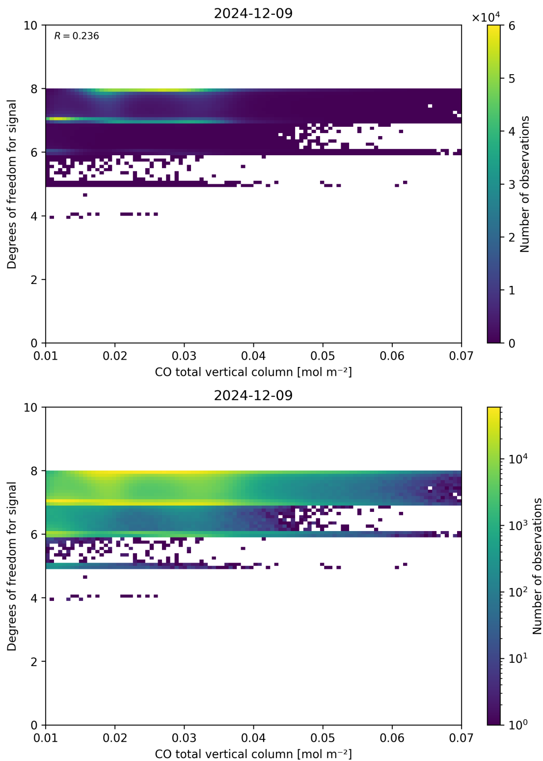
Figure 41: Scatter density plot of “CO total vertical column” against “Degrees of freedom for signal” for 2024-12-08 to 2024-12-10.
