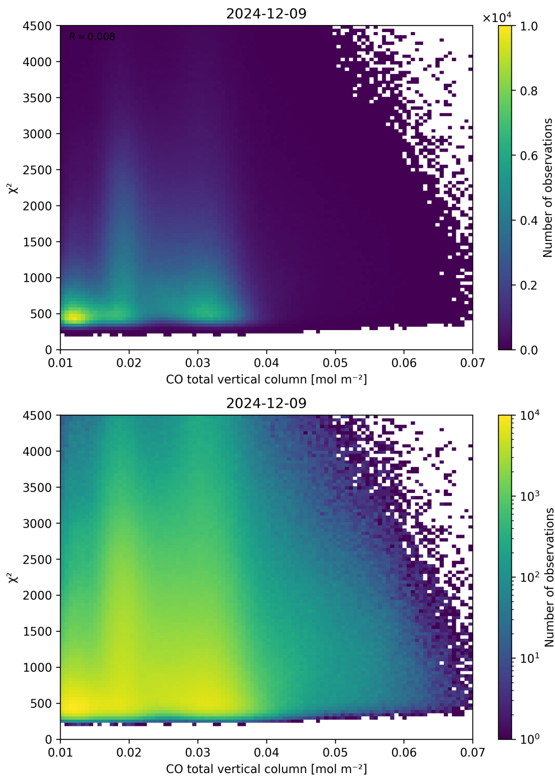
Figure 35: Scatter density plot of “CO total vertical column” against “ \chi^2 ” for 2024-12-08 to 2024-12-10.
