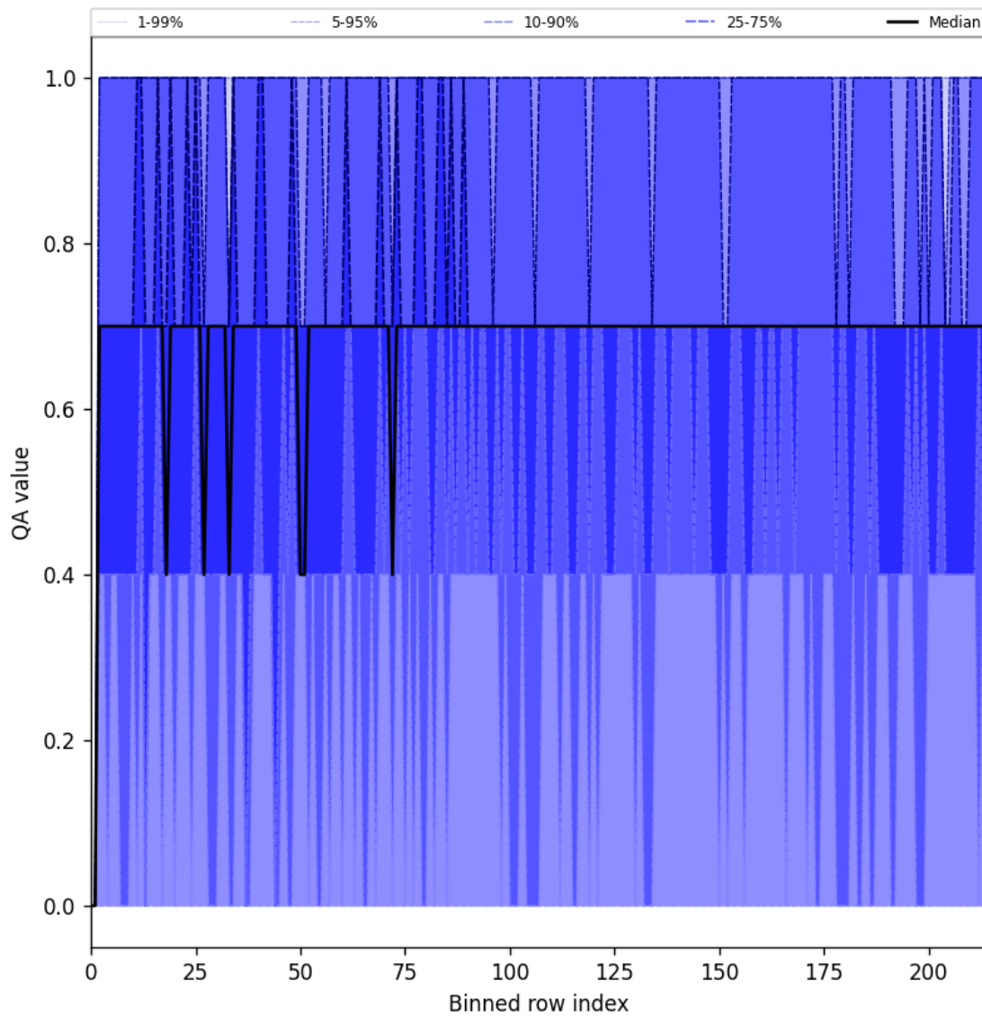
Figure 25: Along track statistics of “QA value” for 2024-12-08 to 2024-12-10
