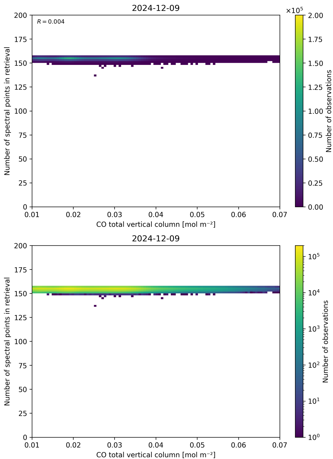
Figure 43: Scatter density plot of “CO total vertical column” against “Number of spectral points in retrieval” for 2024-12-08 to 2024-12-10.
