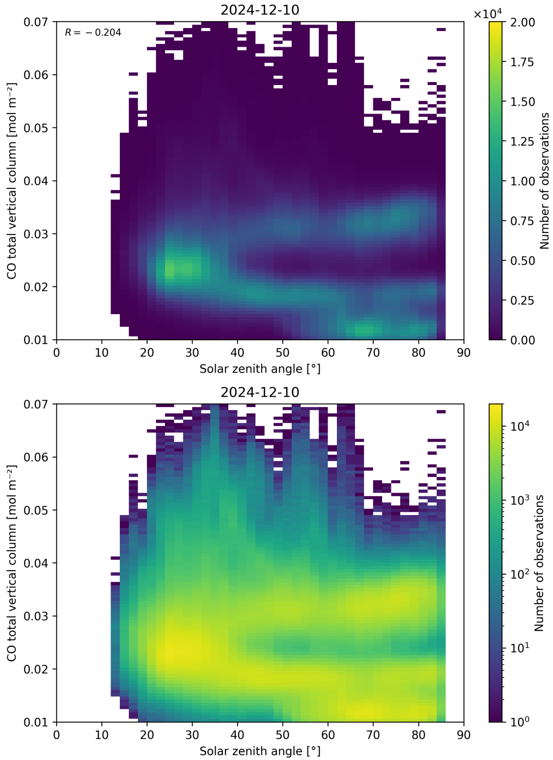
Figure 61: Scatter density plot of “Solar zenith angle” against “CO total vertical column” for 2024-12-09 to 2024-12-11.
