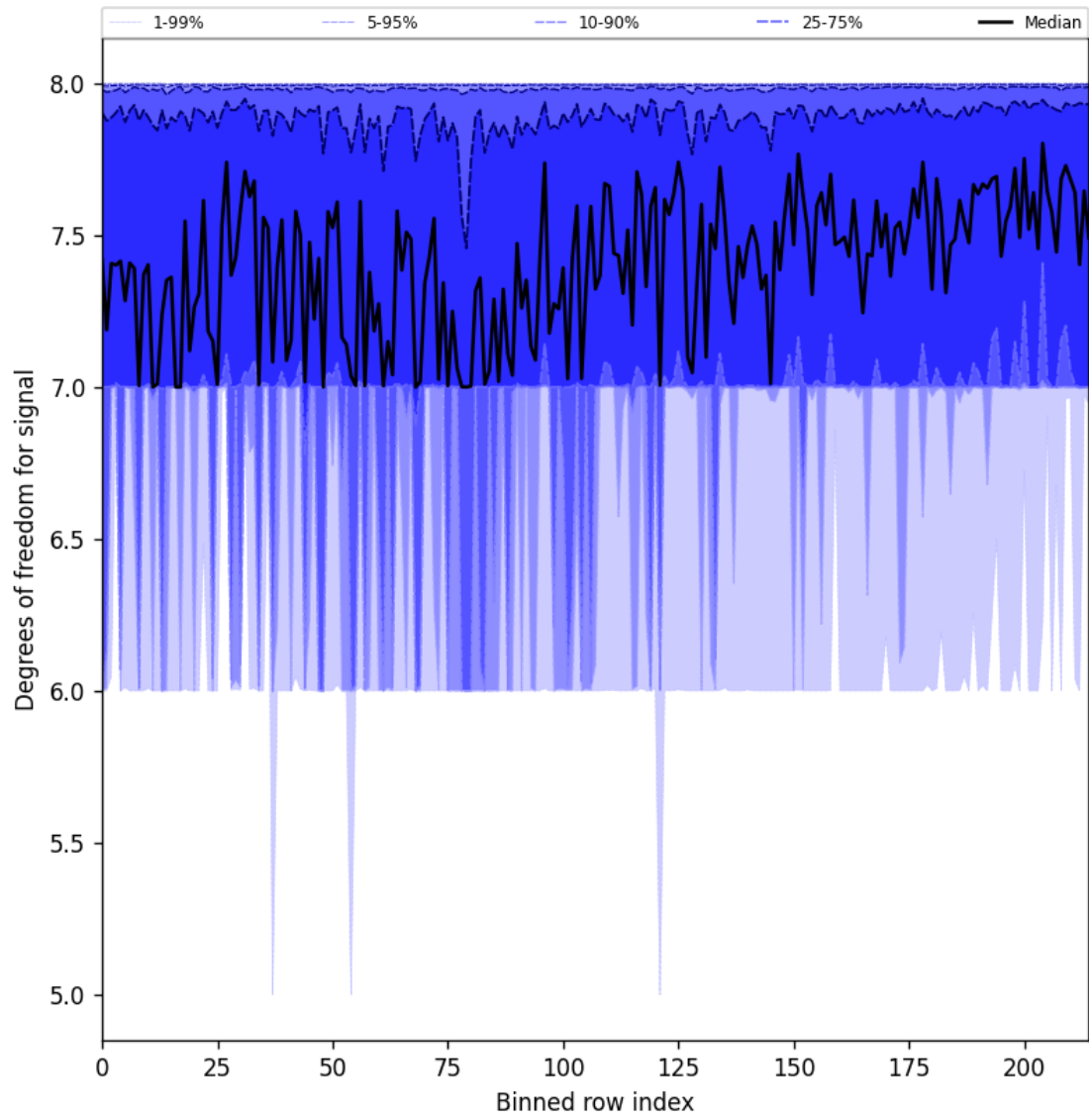
Figure 31: Along track statistics of “Degrees of freedom for signal” for 2024-12-09 to 2024-12-11
