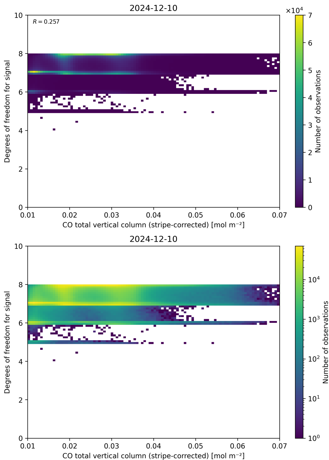
Figure 38: Scatter density plot of “CO total vertical column (stripe-corrected)” against “Degrees of freedom for signal” for 2024-12-09 to 2024-12-11.
