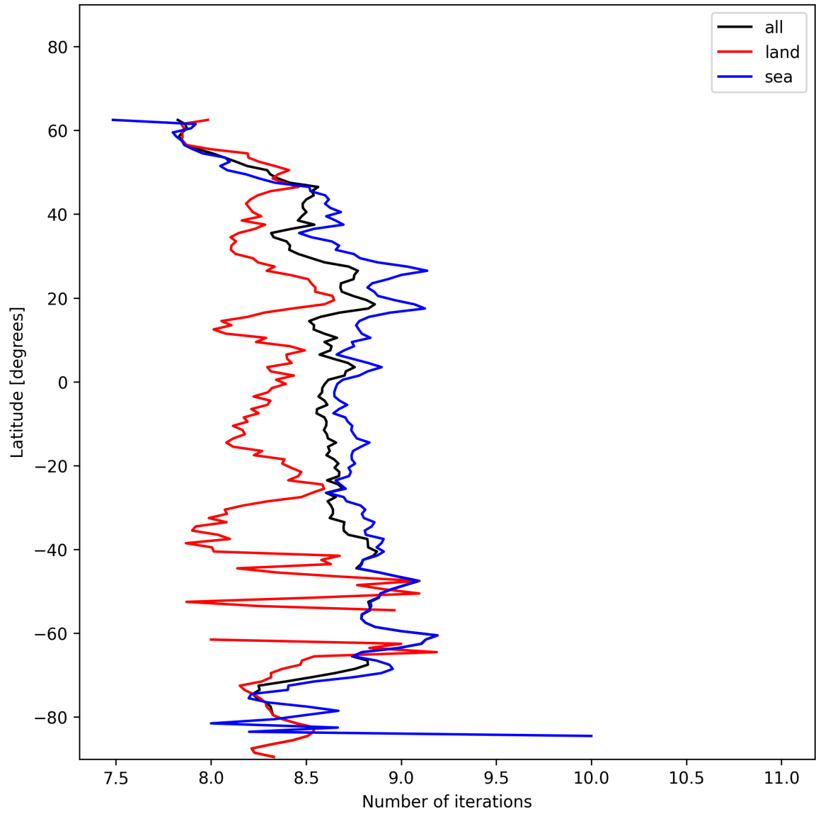
Figure 16: Zonal average of “Number of iterations” for 2024-12-09 to 2024-12-11.
