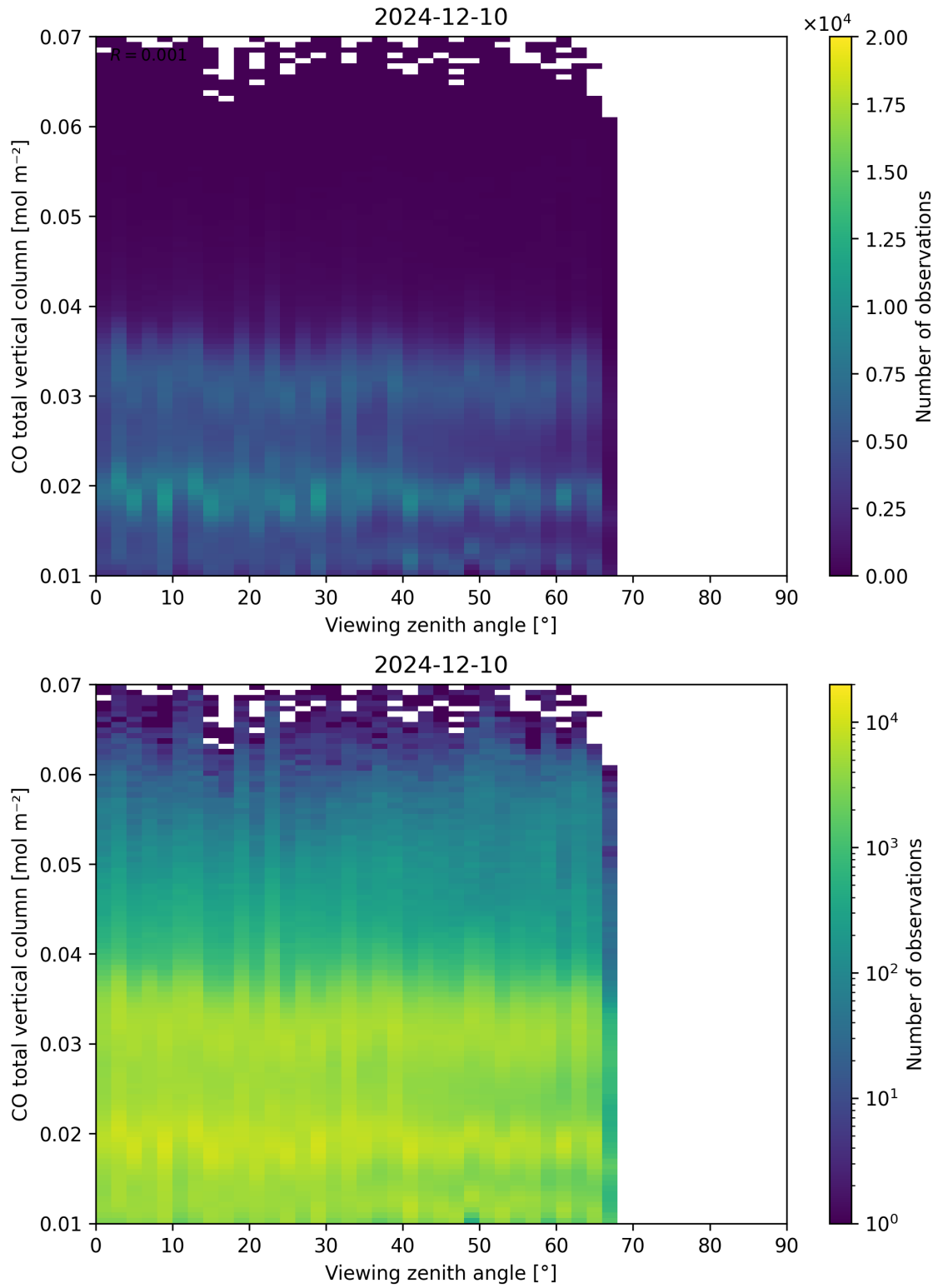
Figure 69: Scatter density plot of “Viewing zenith angle” against “CO total vertical column” for 2024-12-09 to 2024-12-11.
