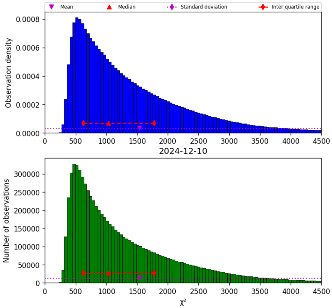
Figure 22: Histogram of “ \chi^2 ” for 2024-12-09 to 2024-12-11
