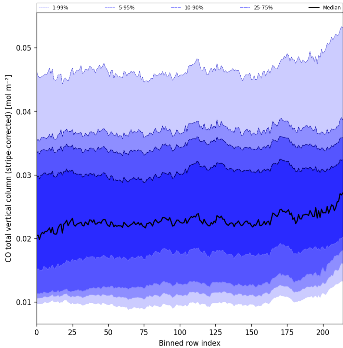
Figure 27: Along track statistics of “CO total vertical column (stripe-corrected)” for 2024-12-09 to 2024-12-11
