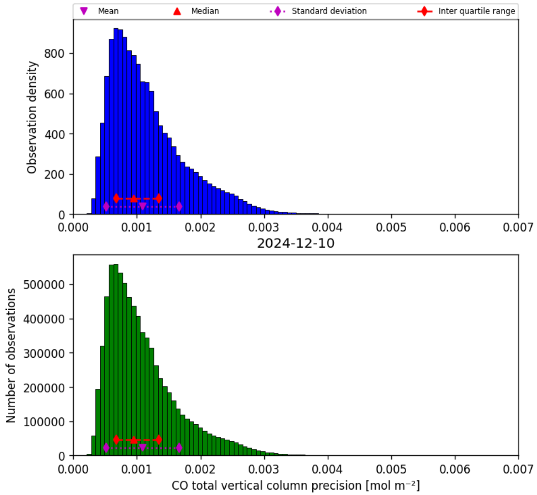
Figure 20: Histogram of “CO total vertical column precision” for 2024-12-09 to 2024-12-11
