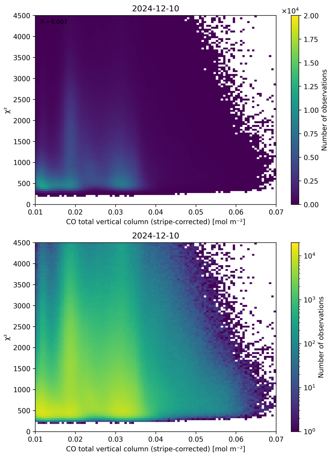
Figure 37: Scatter density plot of “CO total vertical column (stripe-corrected)” against “ \chi^2 ” for 2024-12-09 to 2024-12-11.
