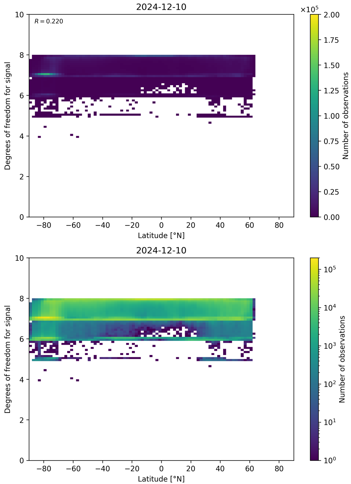
Figure 55: Scatter density plot of “Latitude” against “Degrees of freedom for signal” for 2024-12-09 to 2024-12-11.
