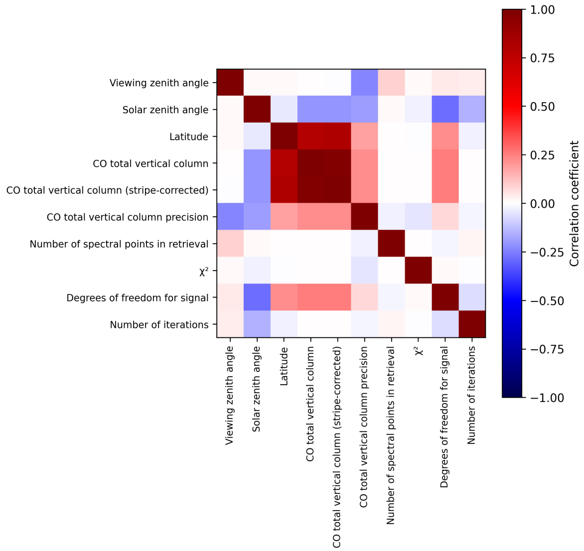
Figure 2: Map of correlation matrix for 2024-12-09 to 2024-12-11.
