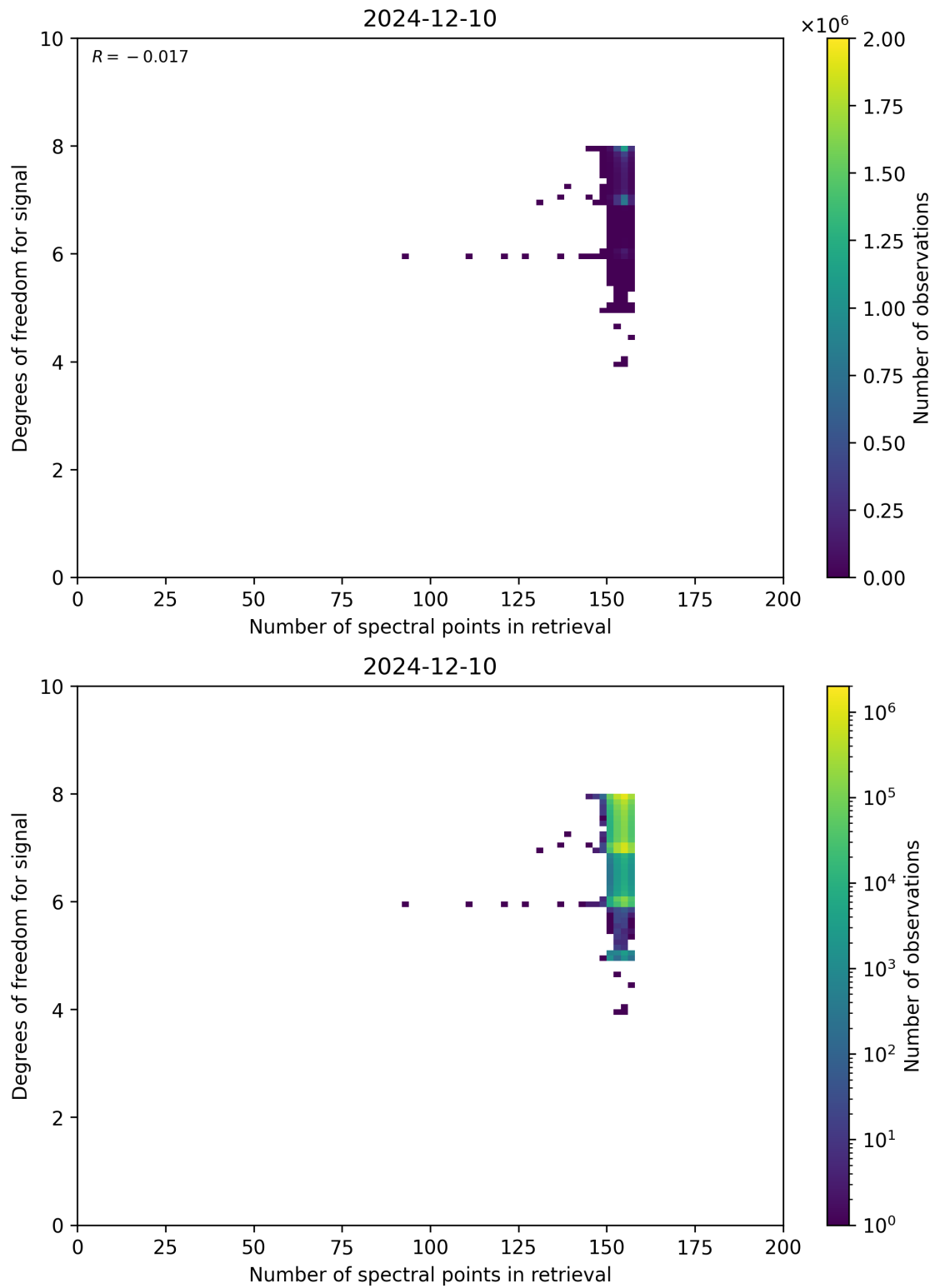
Figure 59: Scatter density plot of “Number of spectral points in retrieval” against “Degrees of freedom for signal” for 2024-12-09 to 2024-12-11.
