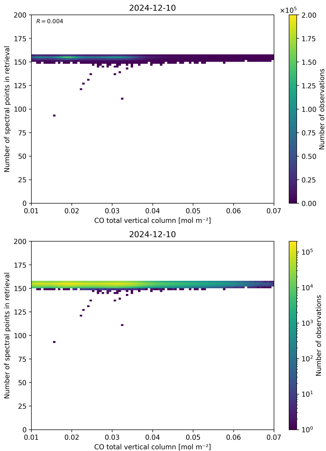
Figure 43: Scatter density plot of “CO total vertical column” against “Number of spectral points in retrieval” for 2024-12-09 to 2024-12-11.
