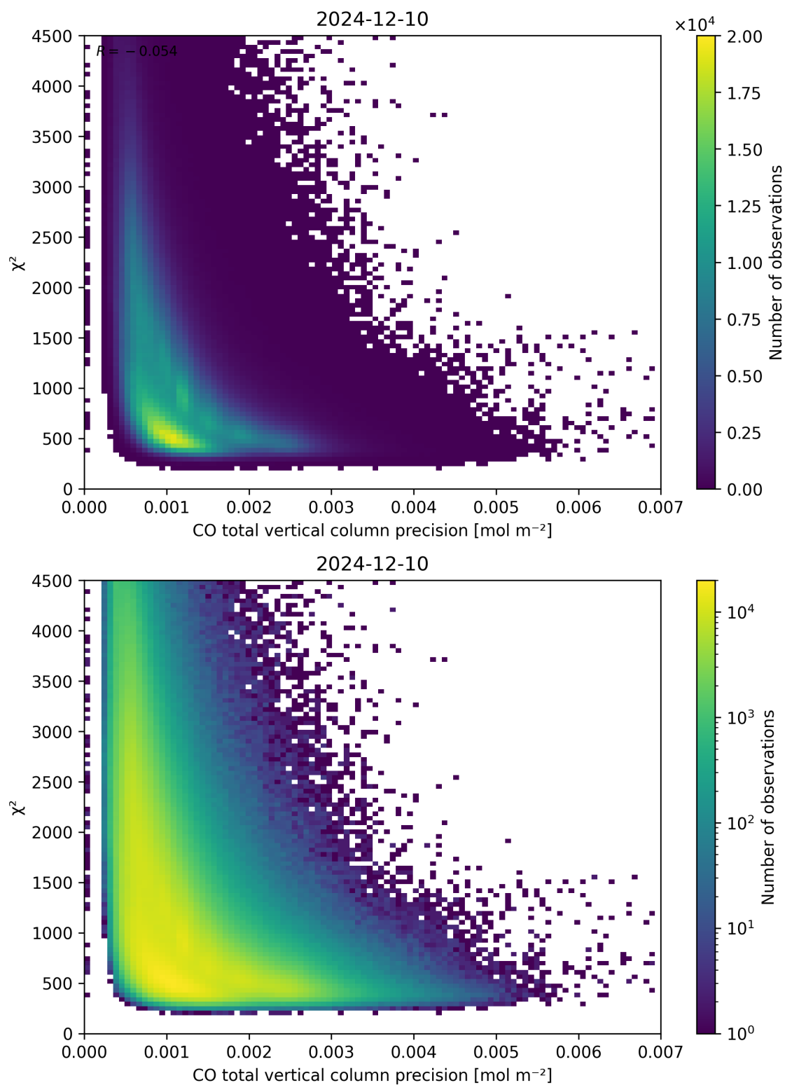
Figure 44: Scatter density plot of “CO total vertical column precision” against “ \chi^2 ” for 2024-12-09 to 2024-12-11.
