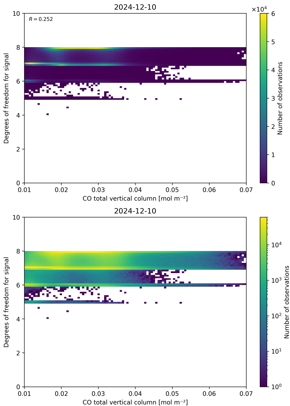
Figure 41: Scatter density plot of “CO total vertical column” against “Degrees of freedom for signal” for 2024-12-09 to 2024-12-11.
