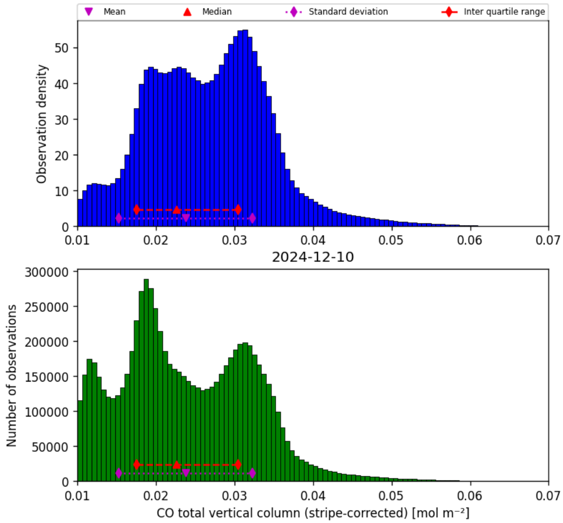
Figure 19: Histogram of “CO total vertical column (stripe-corrected)” for 2024-12-09 to 2024-12-11
