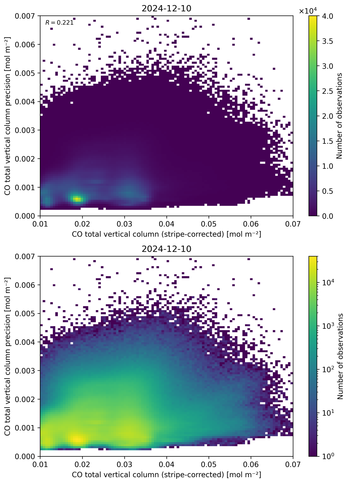
Figure 36: Scatter density plot of “CO total vertical column (stripe-corrected)” against “CO total vertical column precision” for 2024-12-09 to 2024-12-11.
