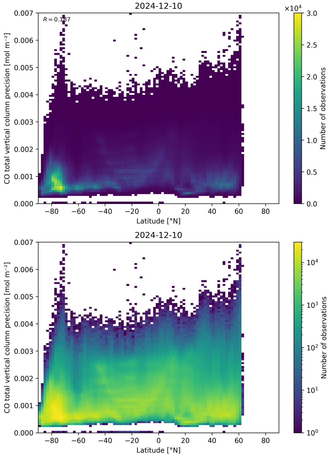
Figure 53: Scatter density plot of “Latitude” against “CO total vertical column precision” for 2024-12-09 to 2024-12-11.
