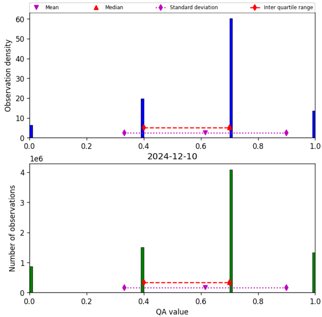
Figure 17: Histogram of “QA value” for 2024-12-09 to 2024-12-11
