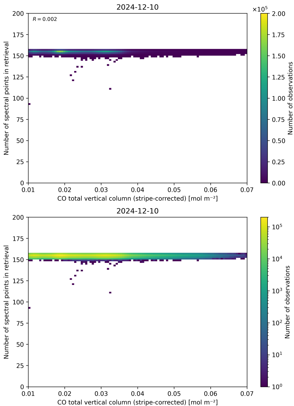
Figure 40: Scatter density plot of “CO total vertical column (stripe-corrected)” against “Number of spectral points in retrieval” for 2024-12-09 to 2024-12-11.
