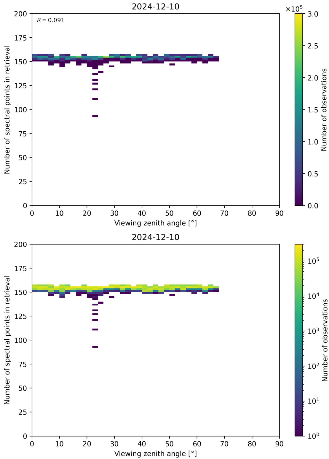
Figure 76: Scatter density plot of “Viewing zenith angle” against “Number of spectral points in retrieval” for 2024-12-09 to 2024-12-11.
