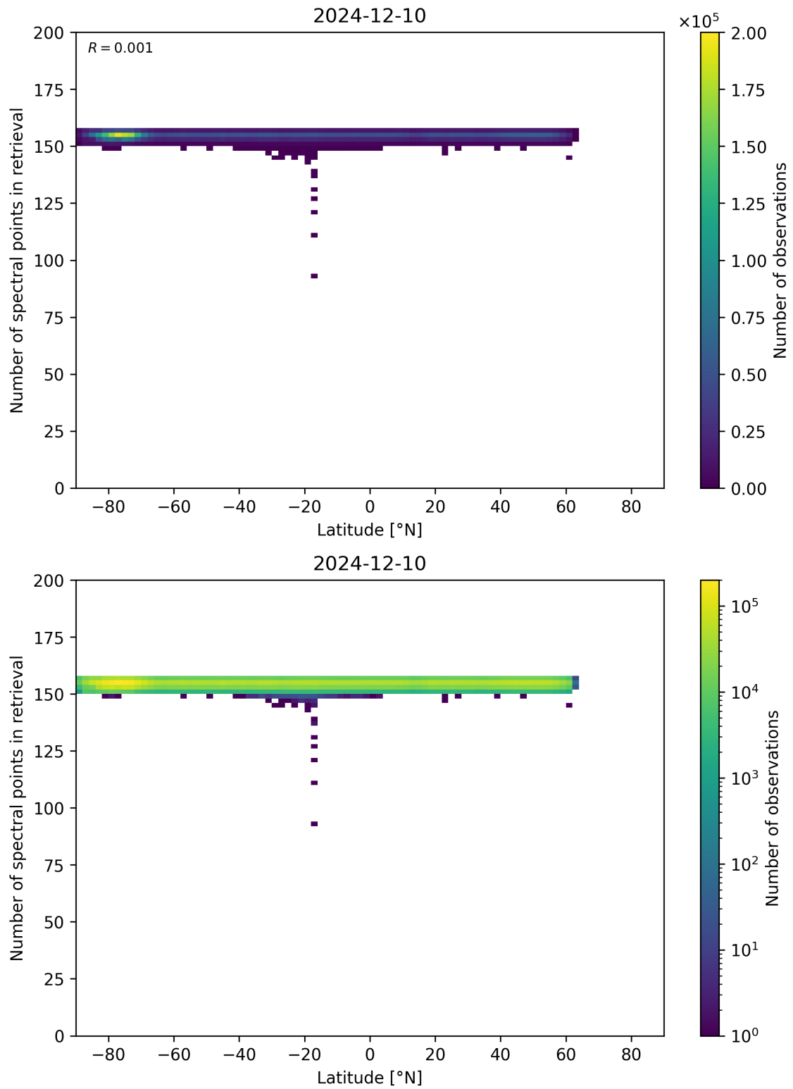
Figure 57: Scatter density plot of “Latitude” against “Number of spectral points in retrieval” for 2024-12-09 to 2024-12-11.
