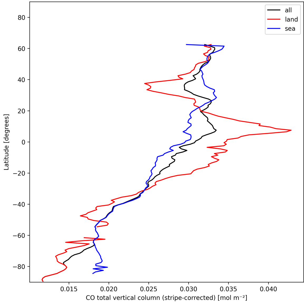
Figure 11: Zonal average of “CO total vertical column (stripe-corrected)” for 2024-12-09 to 2024-12-11.
