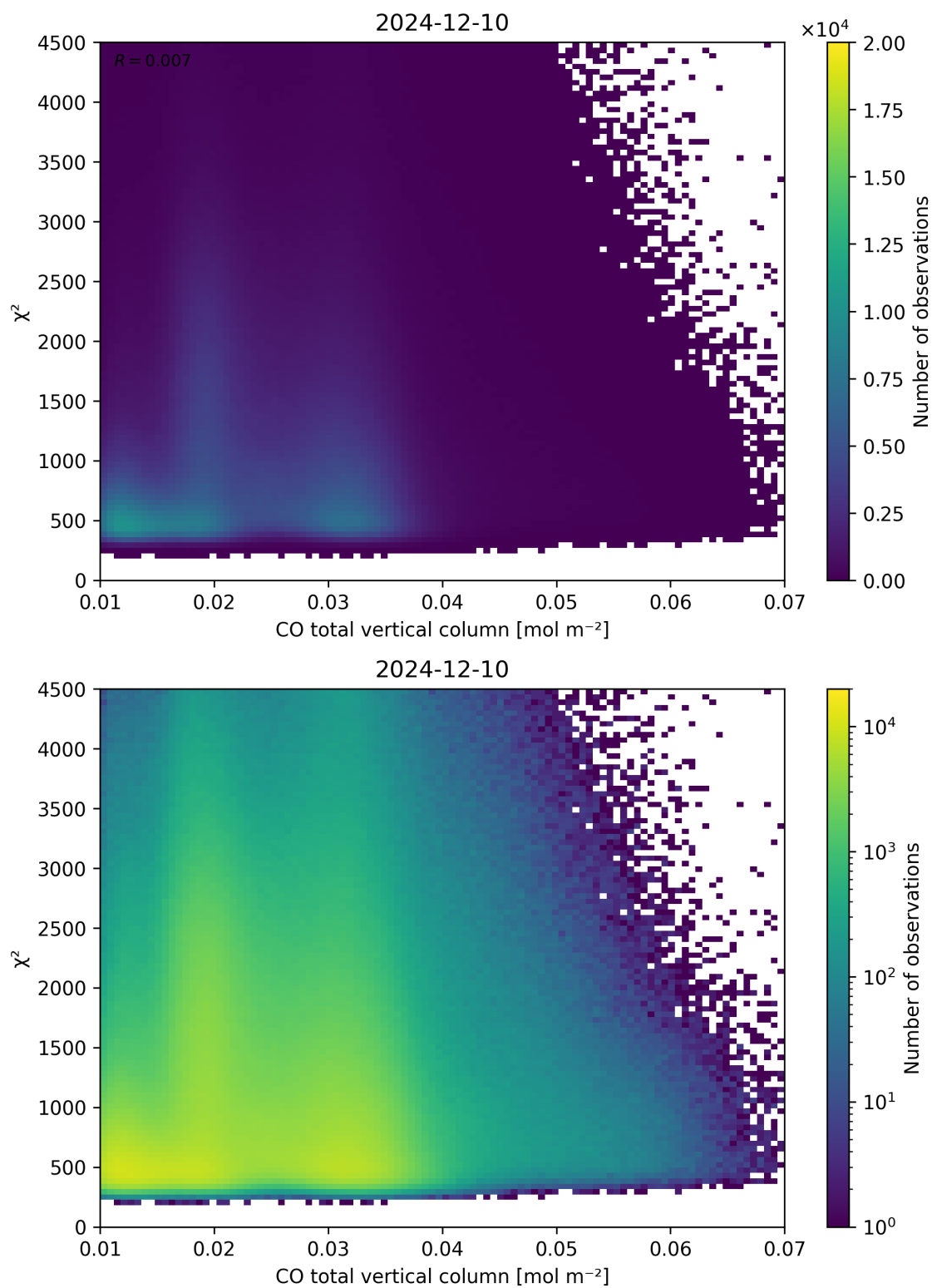
Figure 35: Scatter density plot of “CO total vertical column” against “ \chi^2 ” for 2024-12-09 to 2024-12-11.
