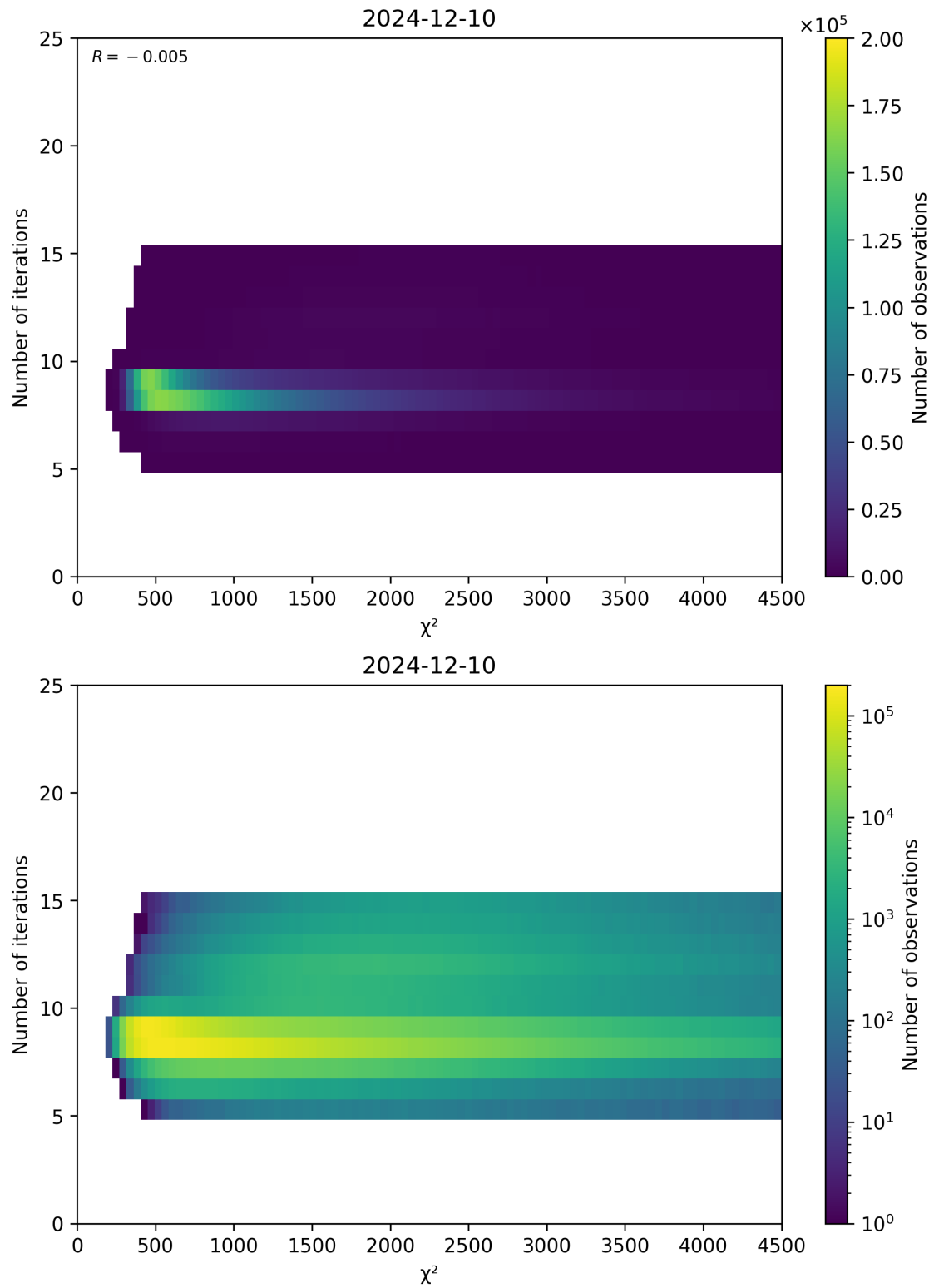
Figure 49: Scatter density plot of “ \chi^2 ” against “Number of iterations” for 2024-12-09 to 2024-12-11.
