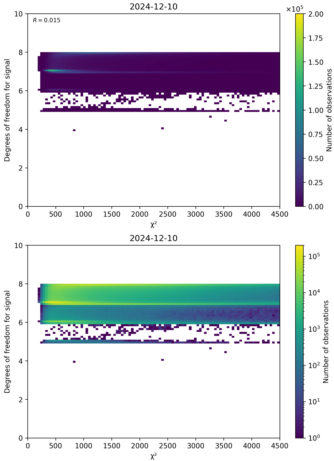
Figure 48: Scatter density plot of “ \chi^2 ” against “Degrees of freedom for signal” for 2024-12-09 to 2024-12-11.
