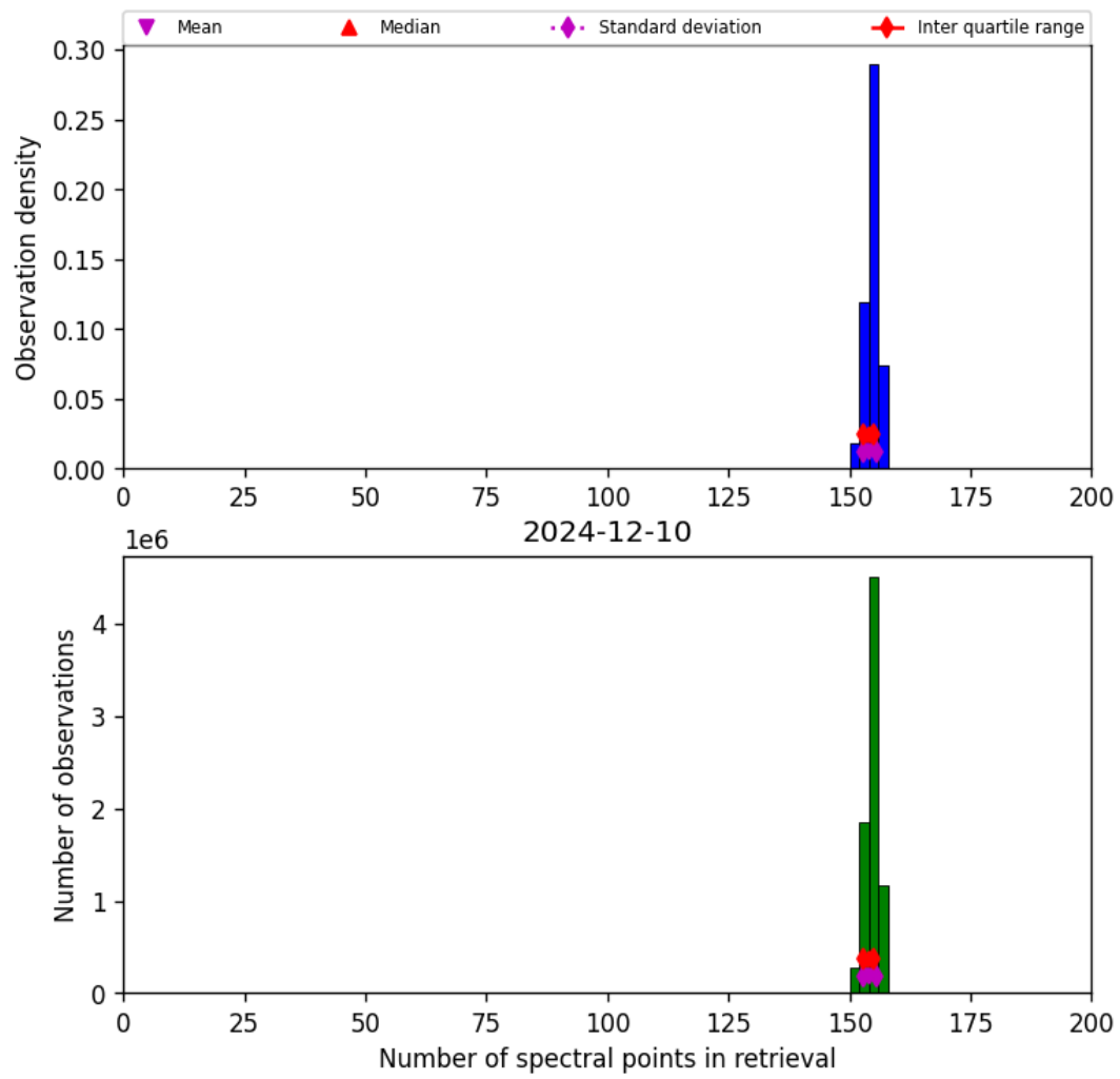
Figure 21: Histogram of “Number of spectral points in retrieval” for 2024-12-09 to 2024-12-11
