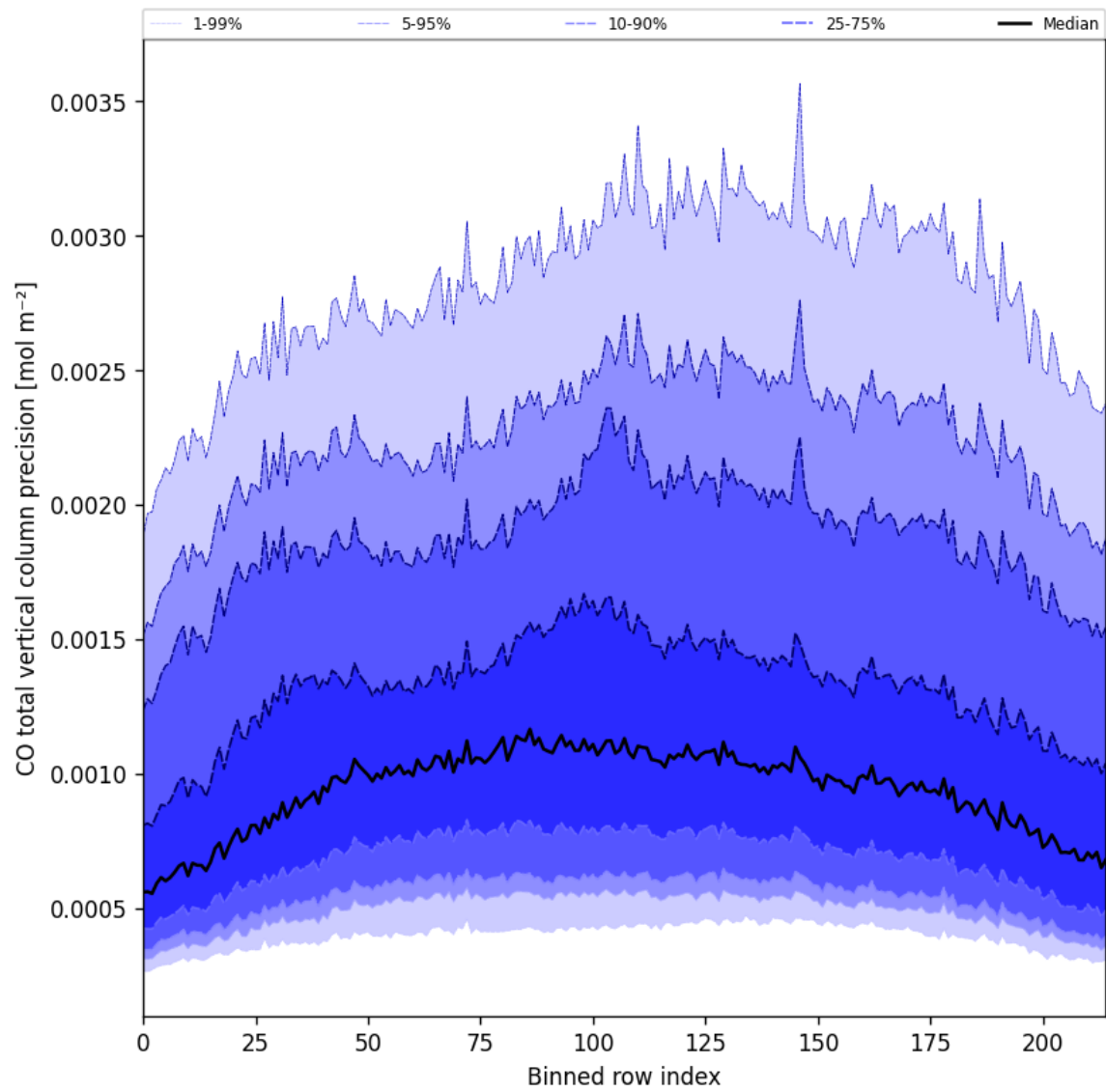
Figure 28: Along track statistics of “CO total vertical column precision” for 2024-12-09 to 2024-12-11
