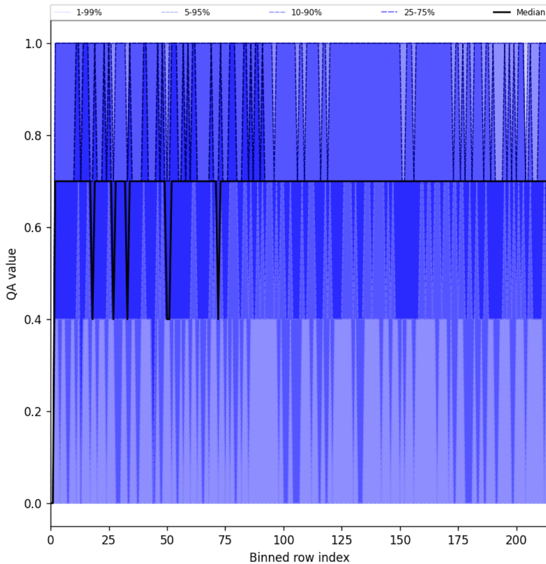
Figure 25: Along track statistics of “QA value” for 2024-12-09 to 2024-12-11
