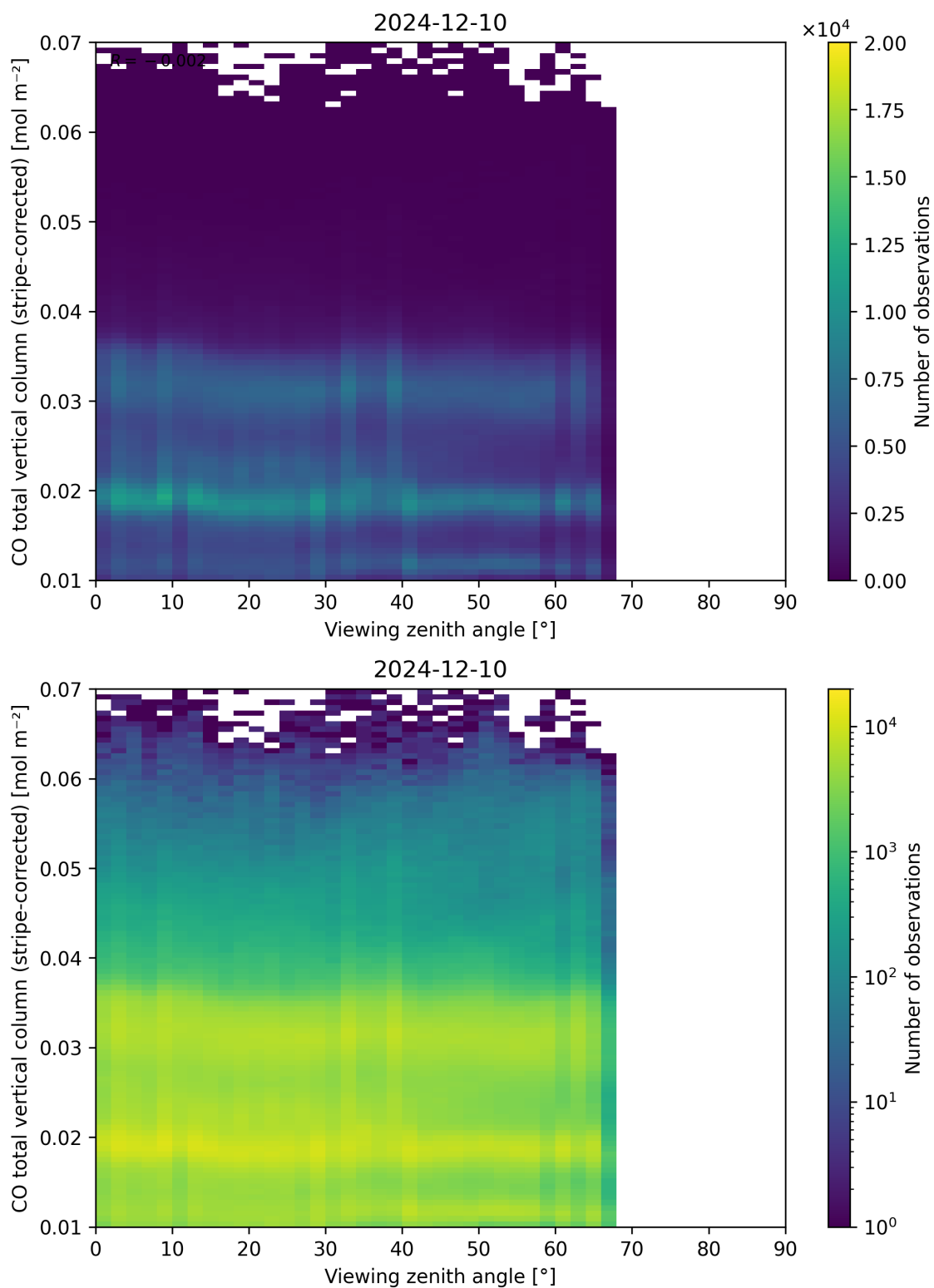
Figure 70: Scatter density plot of “Viewing zenith angle” against “CO total vertical column (stripe-corrected)” for 2024-12-09 to 2024-12-11.
