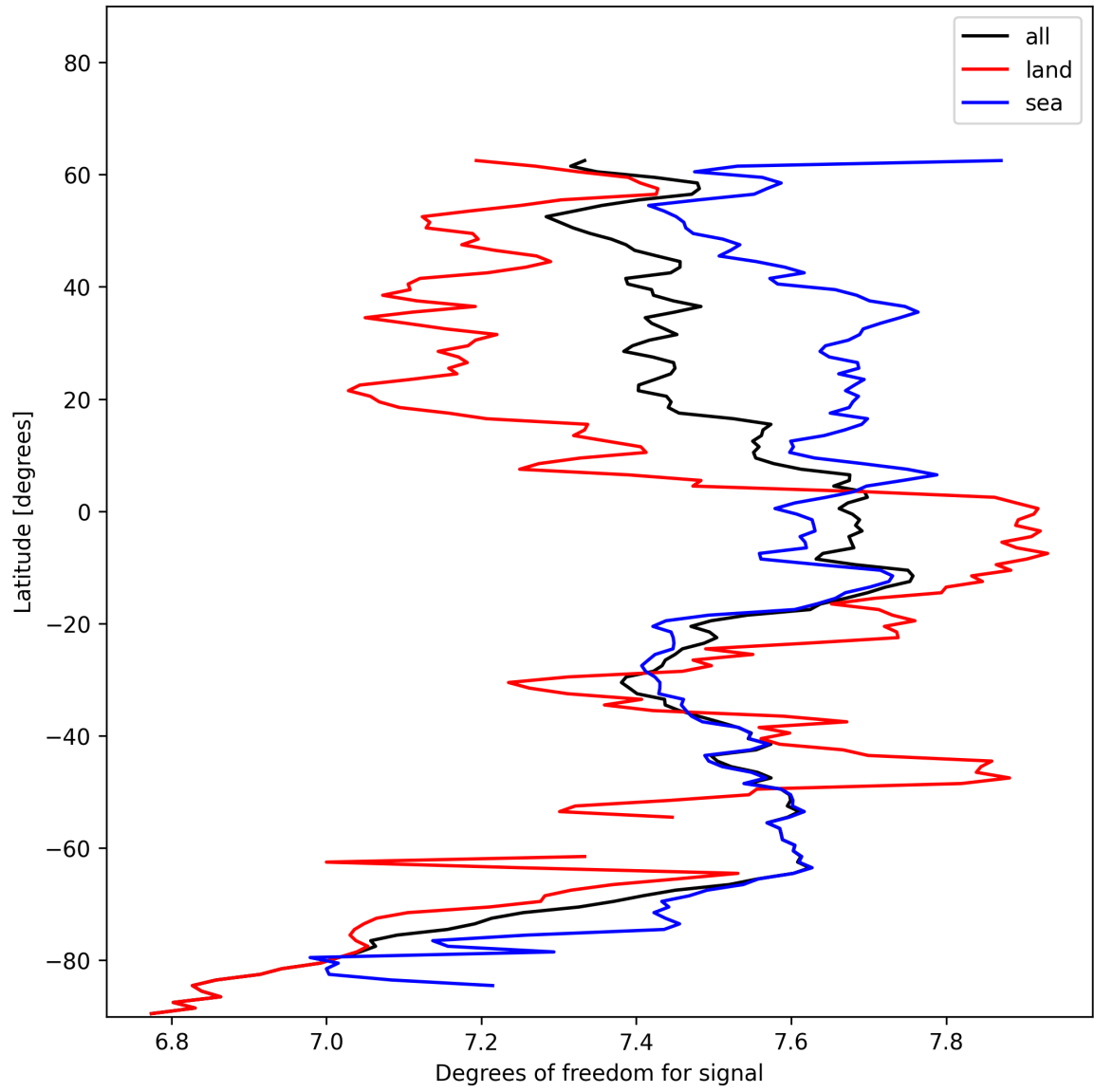
Figure 15: Zonal average of “Degrees of freedom for signal” for 2024-12-09 to 2024-12-11.
