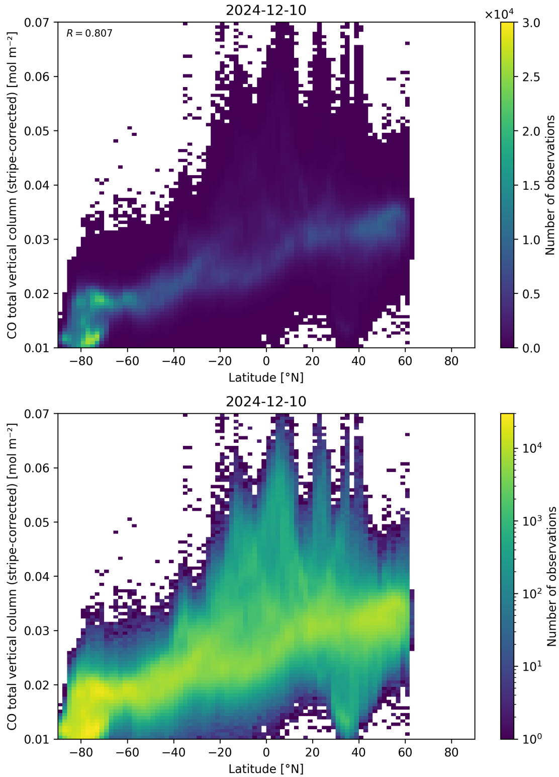
Figure 52: Scatter density plot of “Latitude” against “CO total vertical column (stripe-corrected)” for 2024-12-09 to 2024-12-11.
