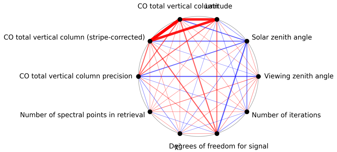
Figure 1: Map of correlation graph for 2024-12-09 to 2024-12-11.
