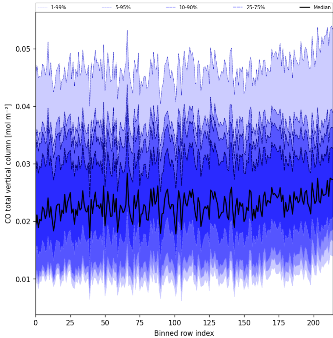
Figure 26: Along track statistics of “CO total vertical column” for 2024-12-09 to 2024-12-11
