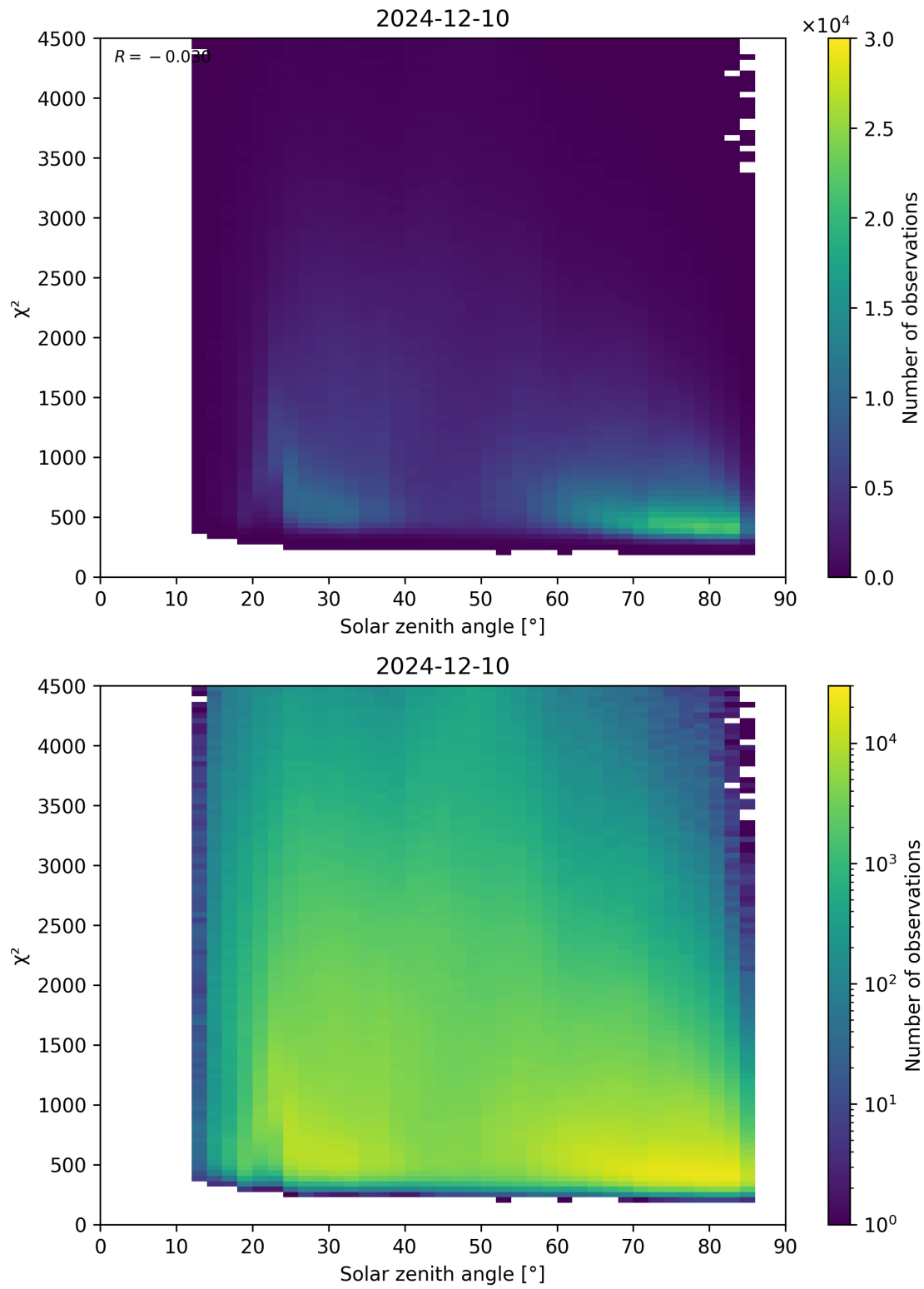
Figure 64: Scatter density plot of “Solar zenith angle” against “ \chi^2 ” for 2024-12-09 to 2024-12-11.
