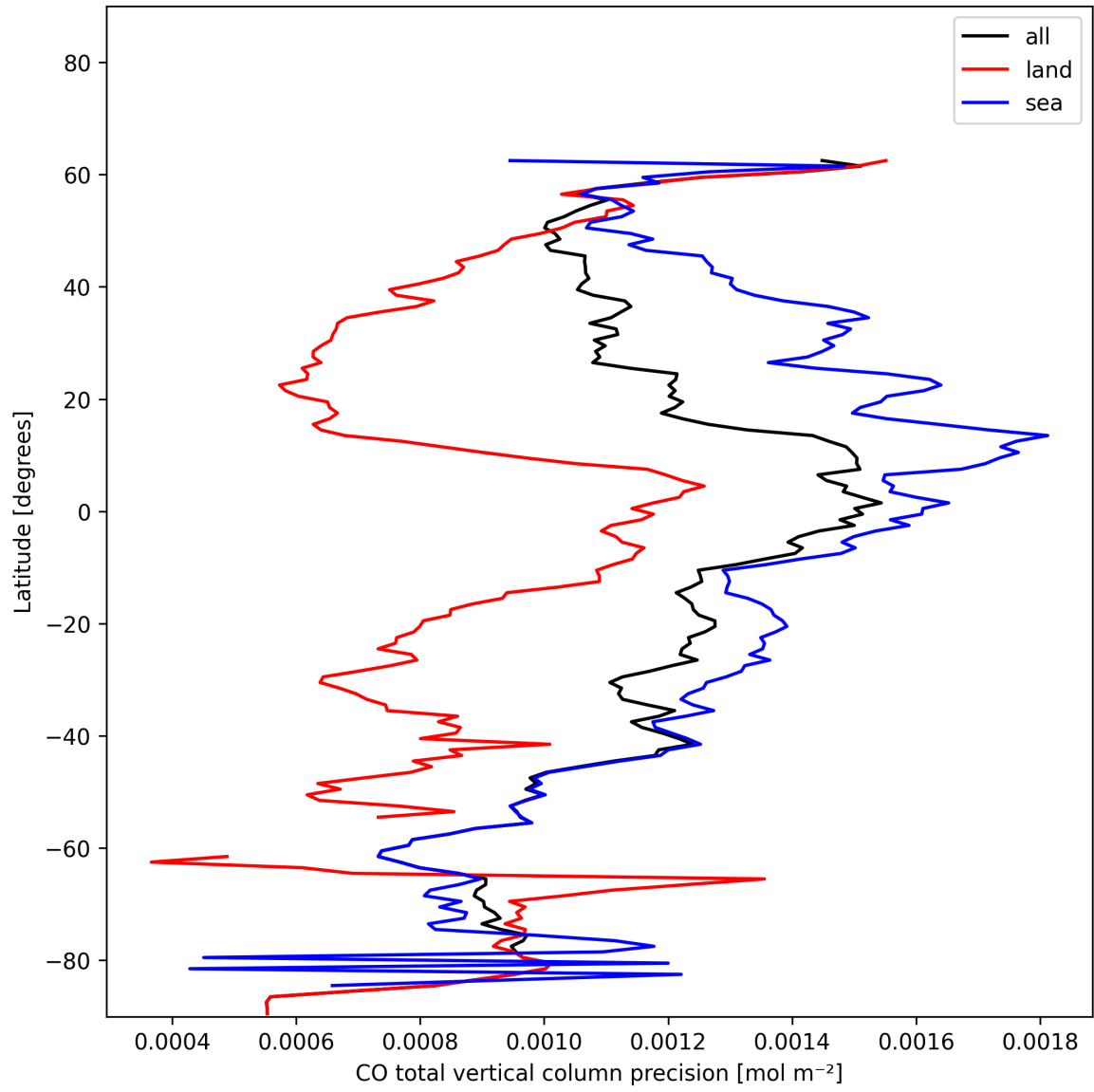
Figure 12: Zonal average of “CO total vertical column precision” for 2024-12-09 to 2024-12-11.
