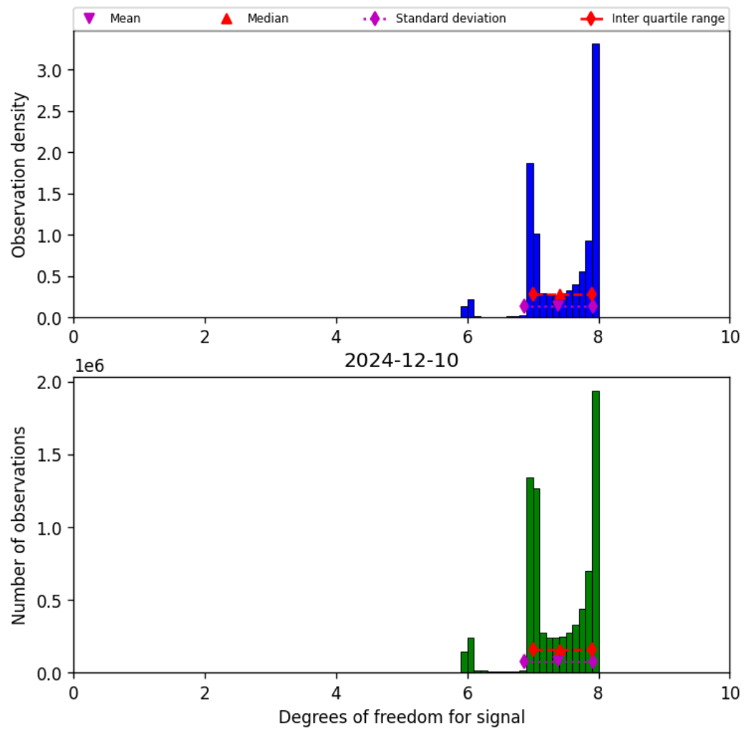
Figure 23: Histogram of “Degrees of freedom for signal” for 2024-12-09 to 2024-12-11
