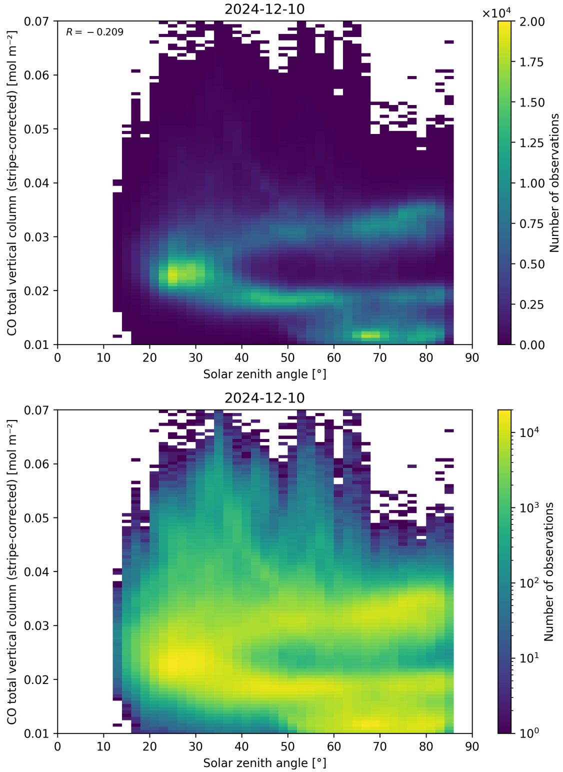
Figure 62: Scatter density plot of “Solar zenith angle” against “CO total vertical column (stripe-corrected)” for 2024-12-09 to 2024-12-11.
