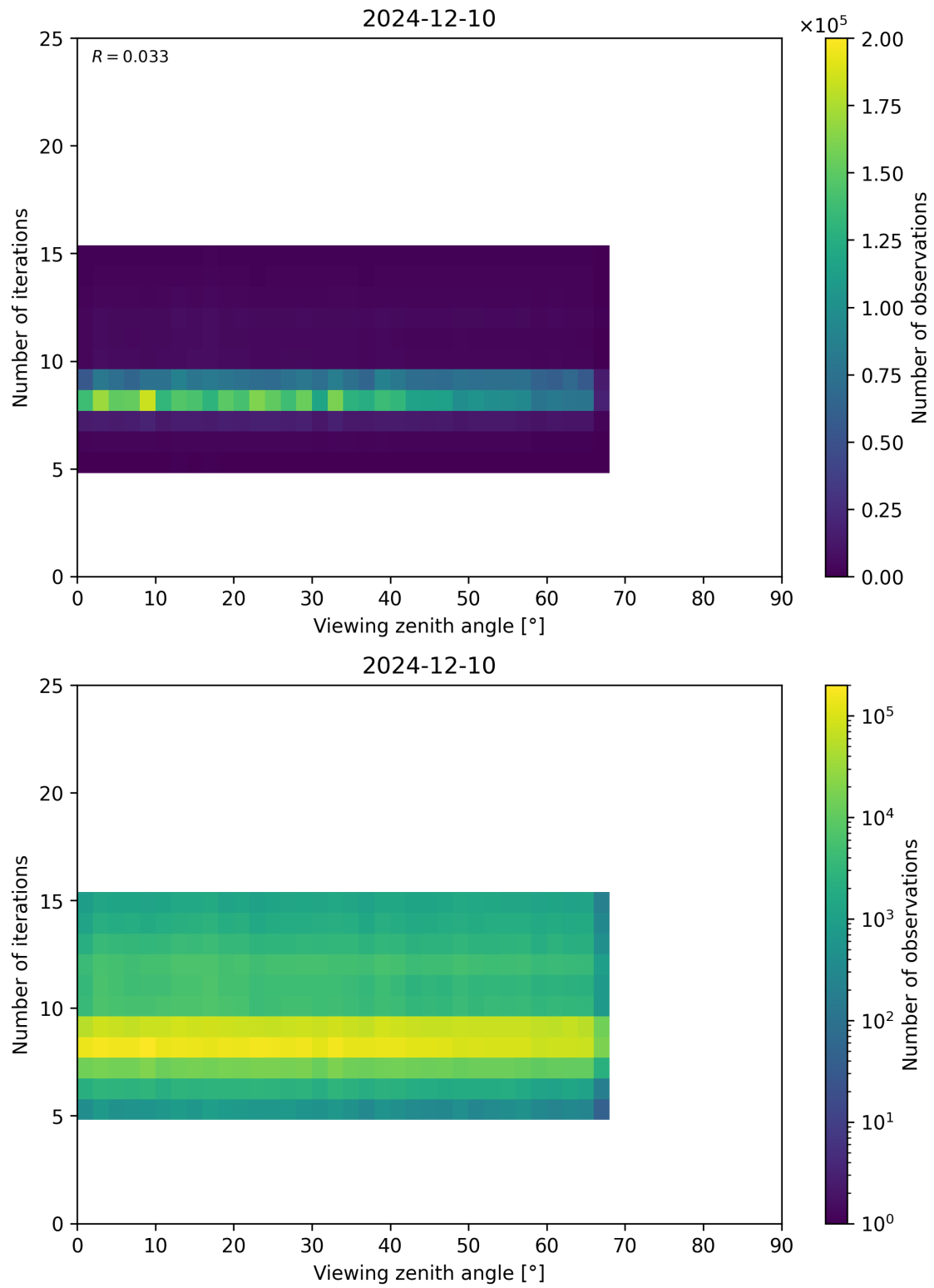
Figure 75: Scatter density plot of “Viewing zenith angle” against “Number of iterations” for 2024-12-09 to 2024-12-11.
