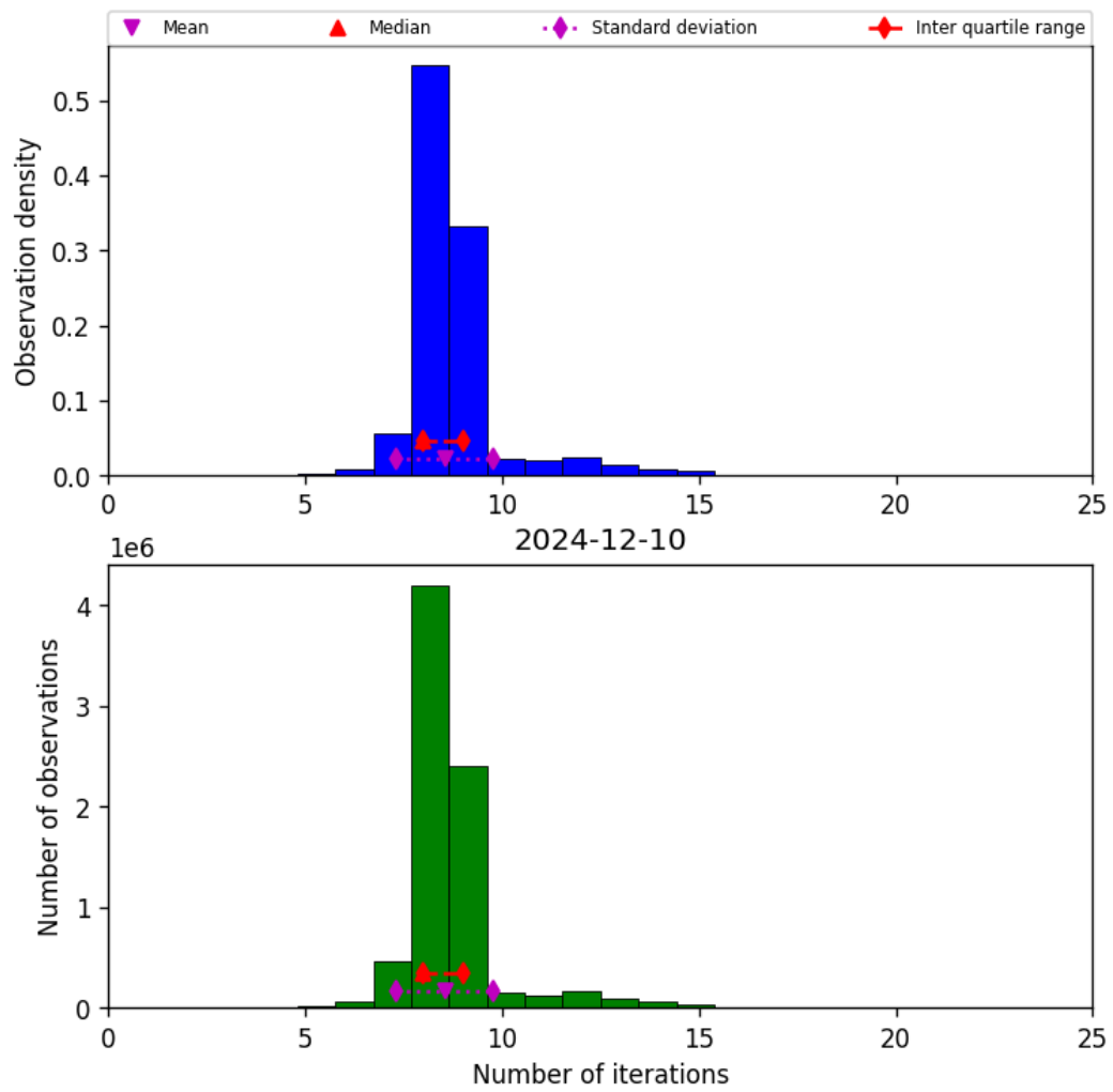
Figure 24: Histogram of “Number of iterations” for 2024-12-09 to 2024-12-11
