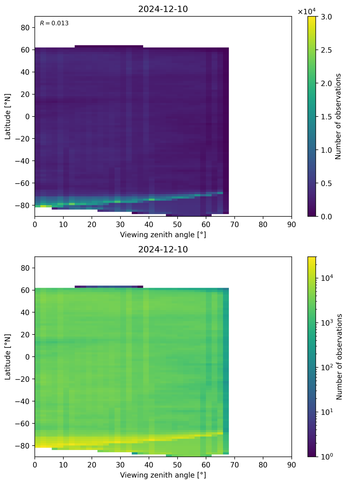
Figure 74: Scatter density plot of “Viewing zenith angle” against “Latitude” for 2024-12-09 to 2024-12-11.
