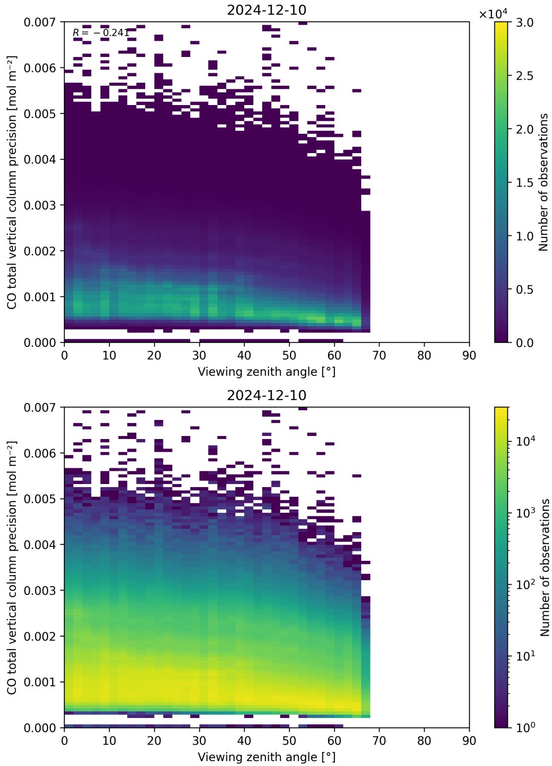
Figure 71: Scatter density plot of “Viewing zenith angle” against “CO total vertical column precision” for 2024-12-09 to 2024-12-11.
