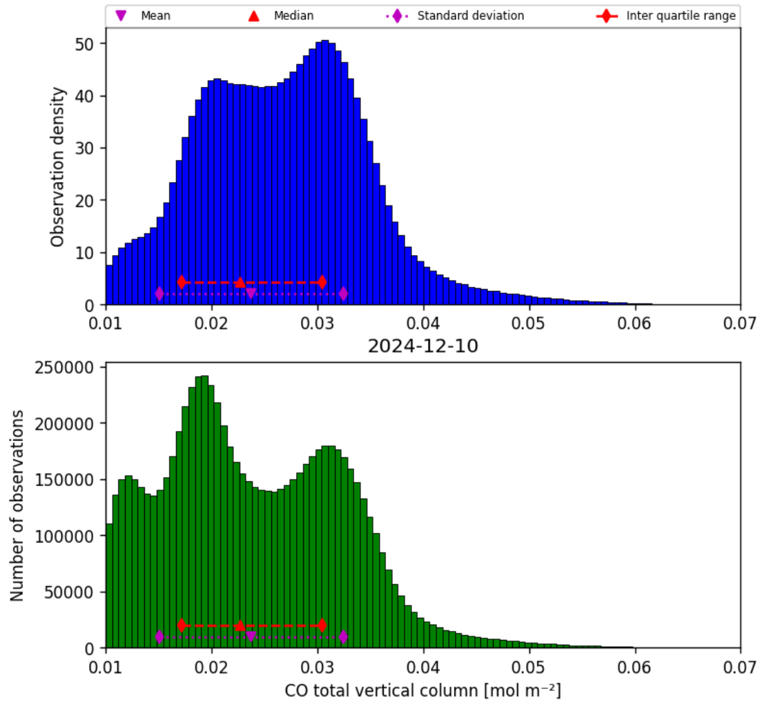
Figure 18: Histogram of “CO total vertical column” for 2024-12-09 to 2024-12-11
