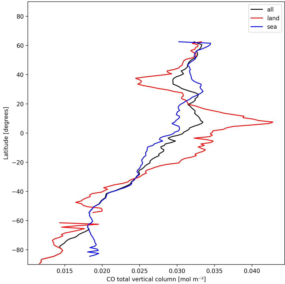
Figure 10: Zonal average of “CO total vertical column” for 2024-12-09 to 2024-12-11.
