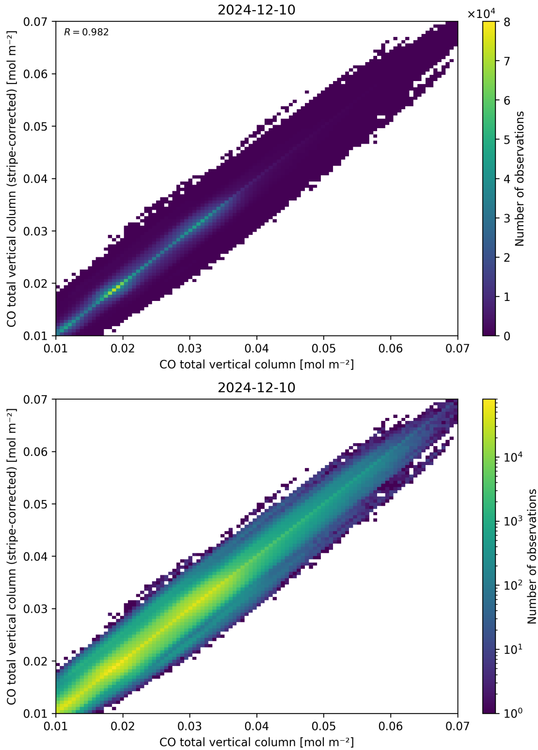
Figure 33: Scatter density plot of “CO total vertical column” against “CO total vertical column (stripe-corrected)” for 2024-12-09 to 2024-12-11.
