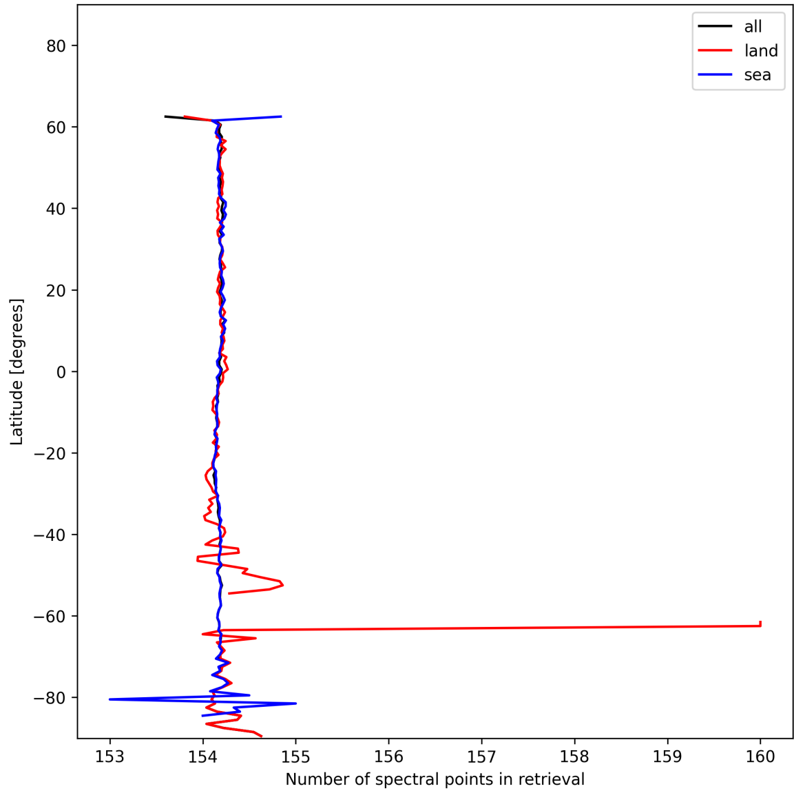
Figure 13: Zonal average of “Number of spectral points in retrieval” for 2024-12-09 to 2024-12-11.
