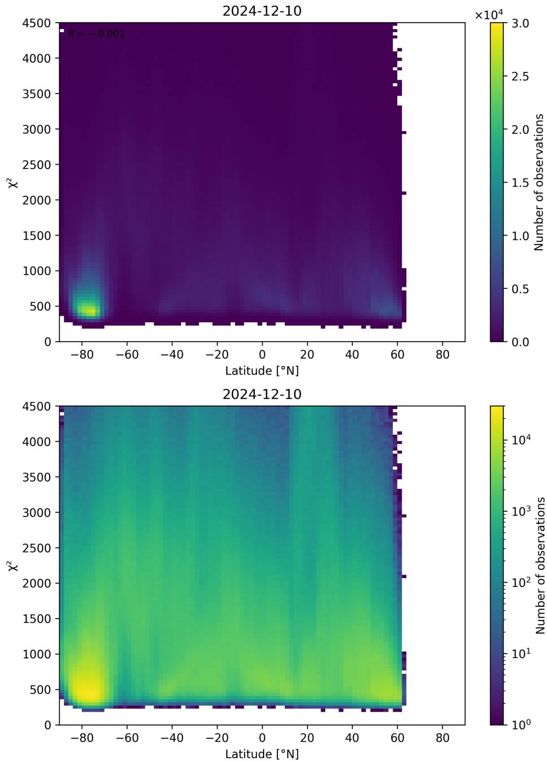
Figure 54: Scatter density plot of “Latitude” against “ \chi^2 ” for 2024-12-09 to 2024-12-11.
