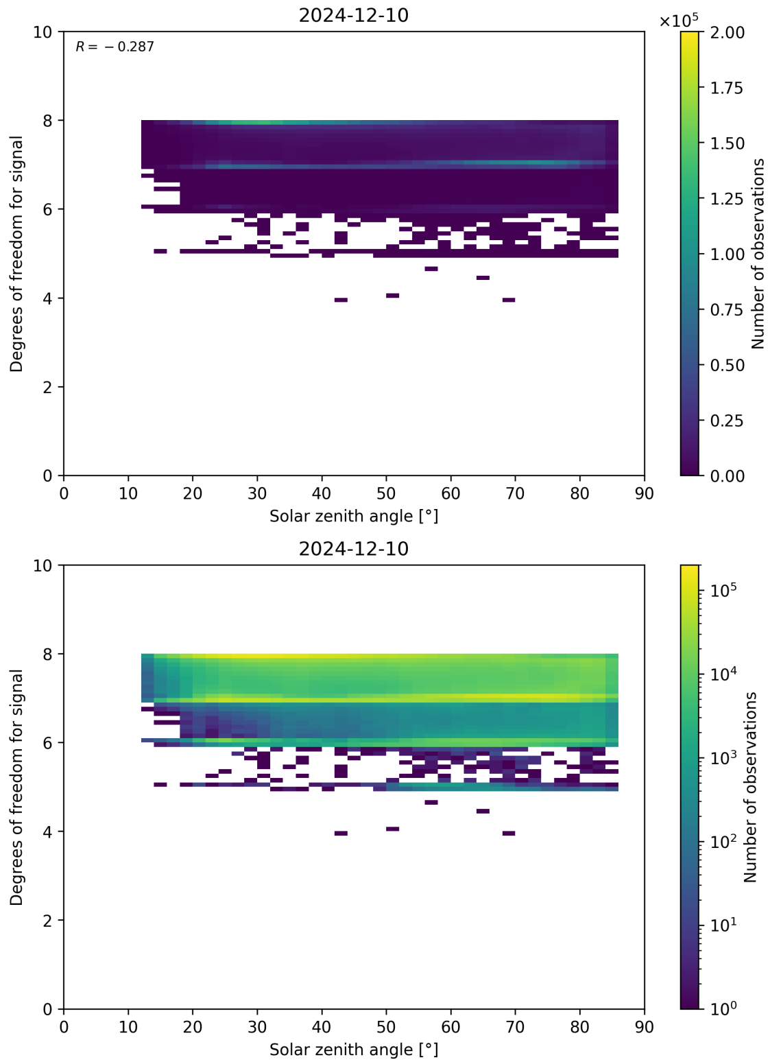
Figure 65: Scatter density plot of “Solar zenith angle” against “Degrees of freedom for signal” for 2024-12-09 to 2024-12-11.
