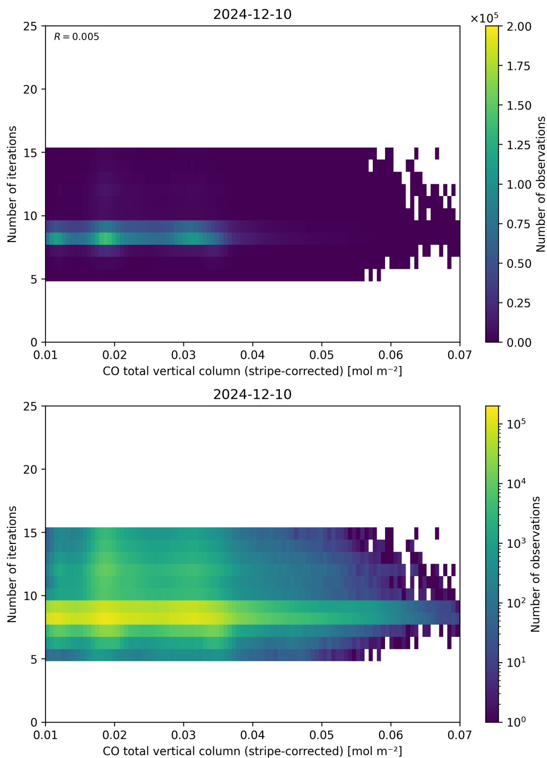
Figure 39: Scatter density plot of “CO total vertical column (stripe-corrected)” against “Number of iterations” for 2024-12-09 to 2024-12-11.
