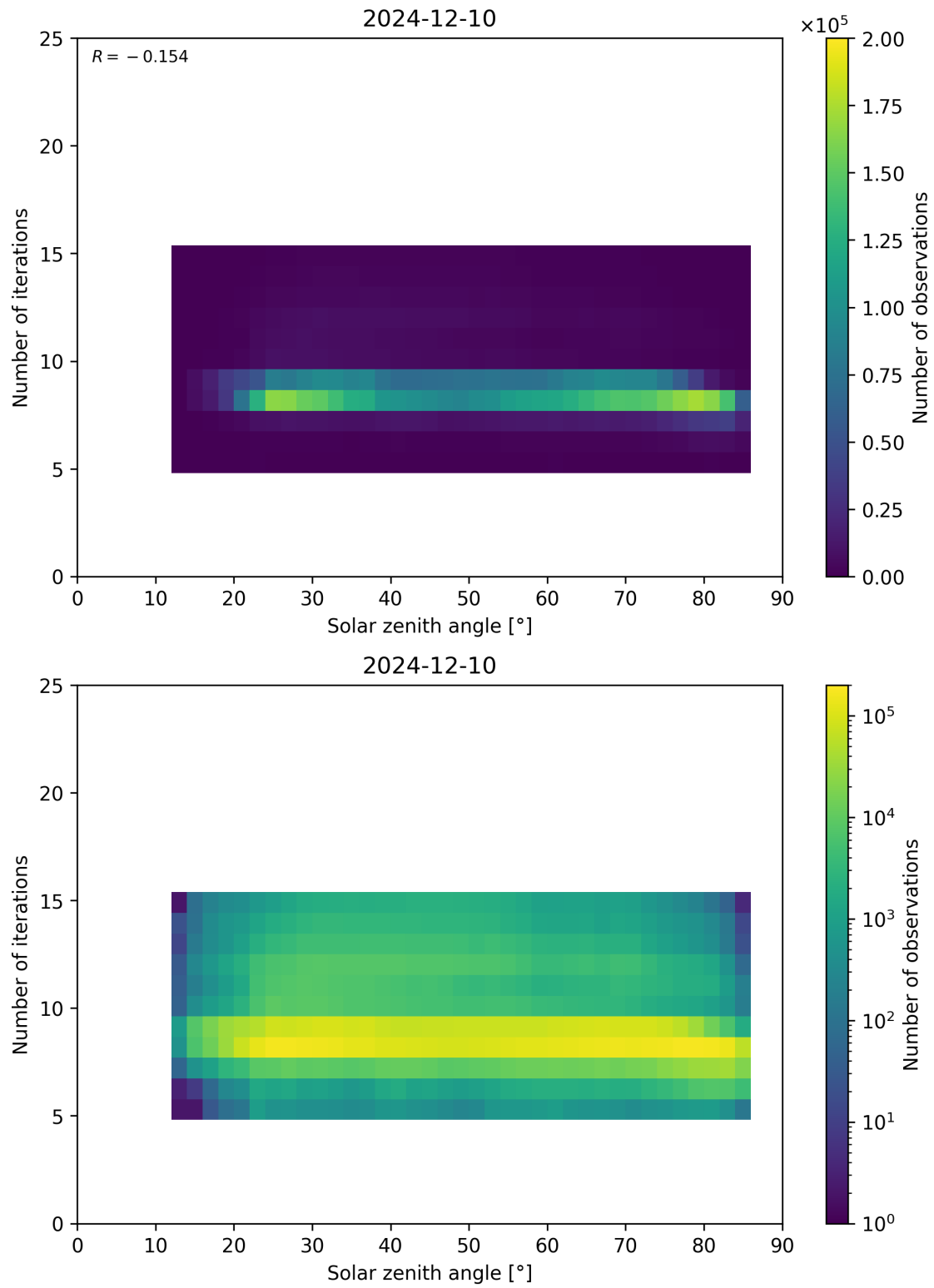
Figure 67: Scatter density plot of “Solar zenith angle” against “Number of iterations” for 2024-12-09 to 2024-12-11.
