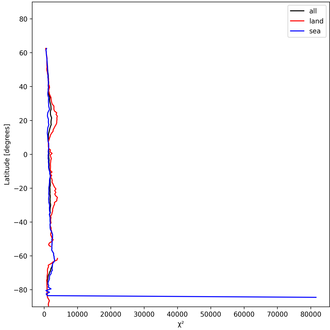
Figure 14: Zonal average of “ \chi^2 ” for 2024-12-09 to 2024-12-11.
