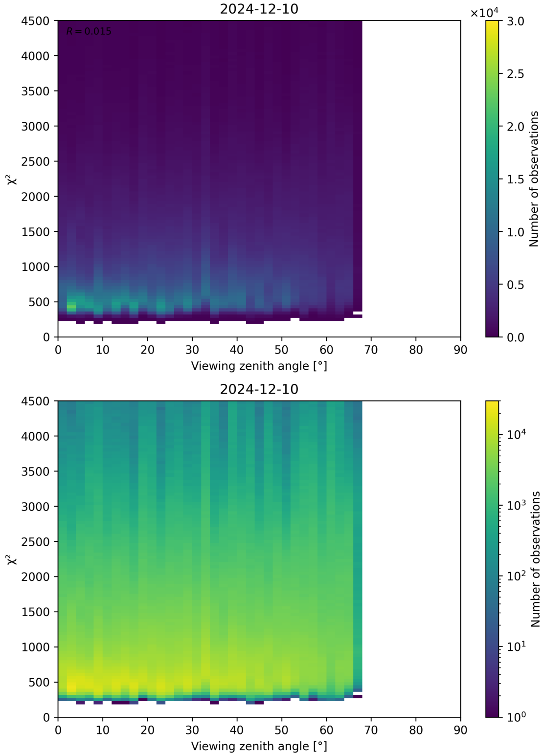
Figure 72: Scatter density plot of “Viewing zenith angle” against “ \chi^2 ” for 2024-12-09 to 2024-12-11.
