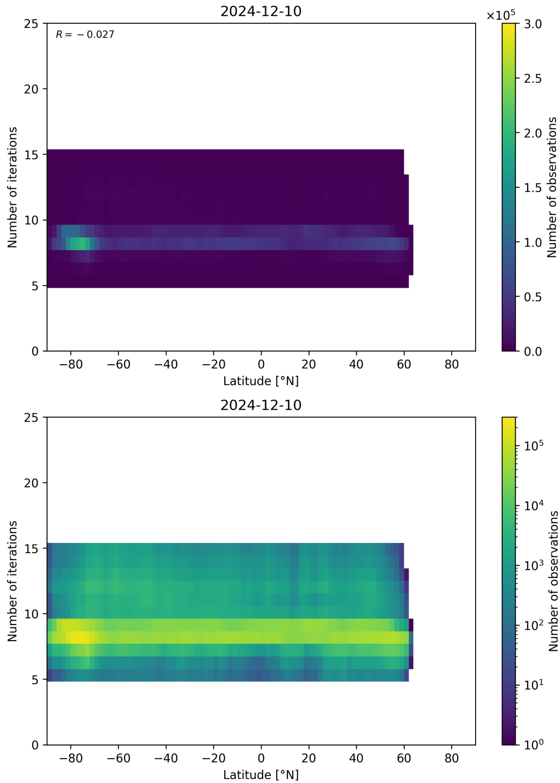
Figure 56: Scatter density plot of “Latitude” against “Number of iterations” for 2024-12-09 to 2024-12-11.
