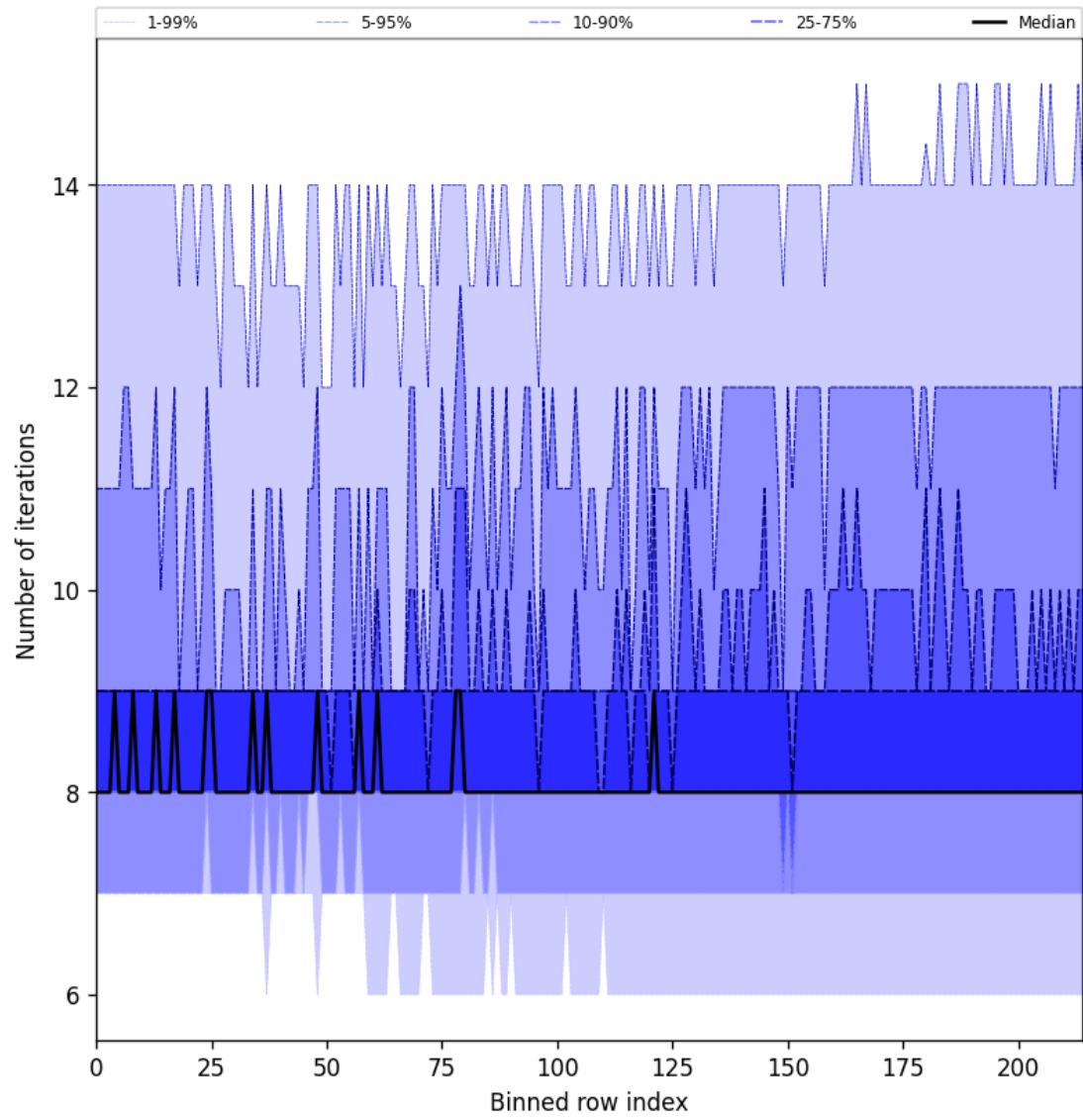
Figure 32: Along track statistics of “Number of iterations” for 2024-12-09 to 2024-12-11
