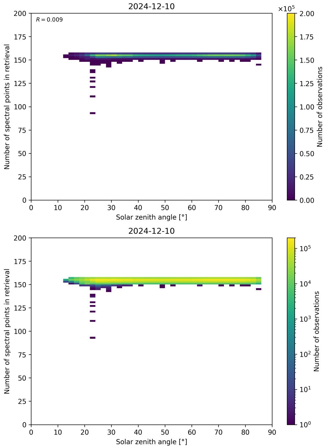
Figure 68: Scatter density plot of “Solar zenith angle” against “Number of spectral points in retrieval” for 2024-12-09 to 2024-12-11.
