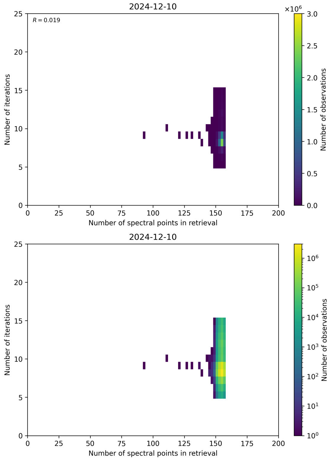
Figure 60: Scatter density plot of “Number of spectral points in retrieval” against “Number of iterations” for 2024-12-09 to 2024-12-11.
