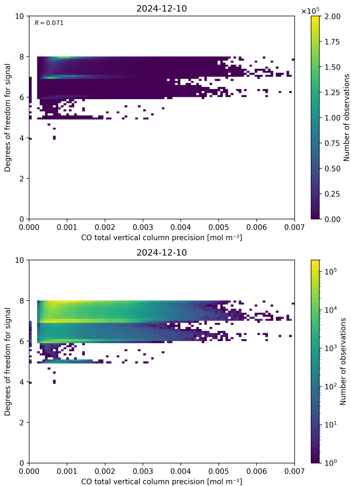
Figure 45: Scatter density plot of “CO total vertical column precision” against “Degrees of freedom for signal” for 2024-12-09 to 2024-12-11.
