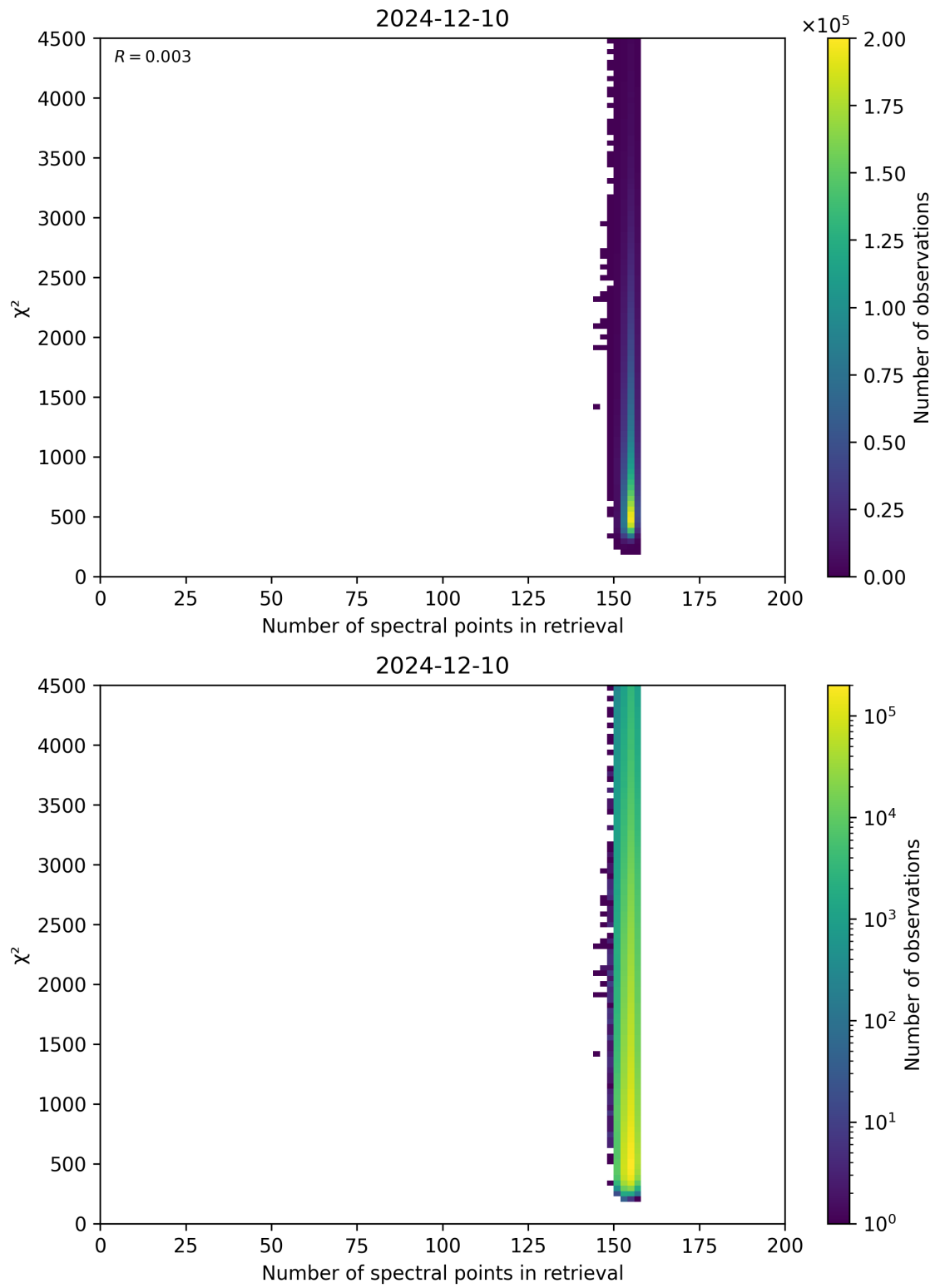
Figure 58: Scatter density plot of “Number of spectral points in retrieval” against “ \chi^2 ” for 2024-12-09 to 2024-12-11.
