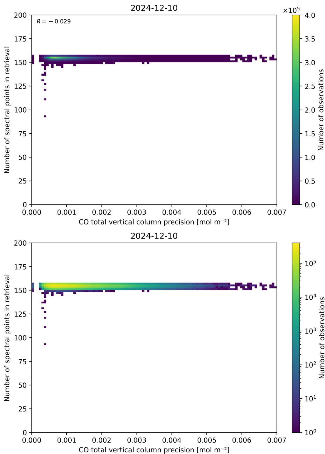
Figure 47: Scatter density plot of “CO total vertical column precision” against “Number of spectral points in retrieval” for 2024-12-09 to 2024-12-11.
