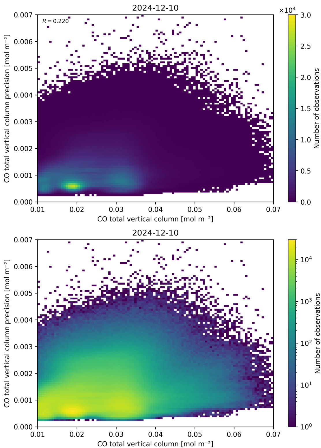
Figure 34: Scatter density plot of “CO total vertical column” against “CO total vertical column precision” for 2024-12-09 to 2024-12-11.
