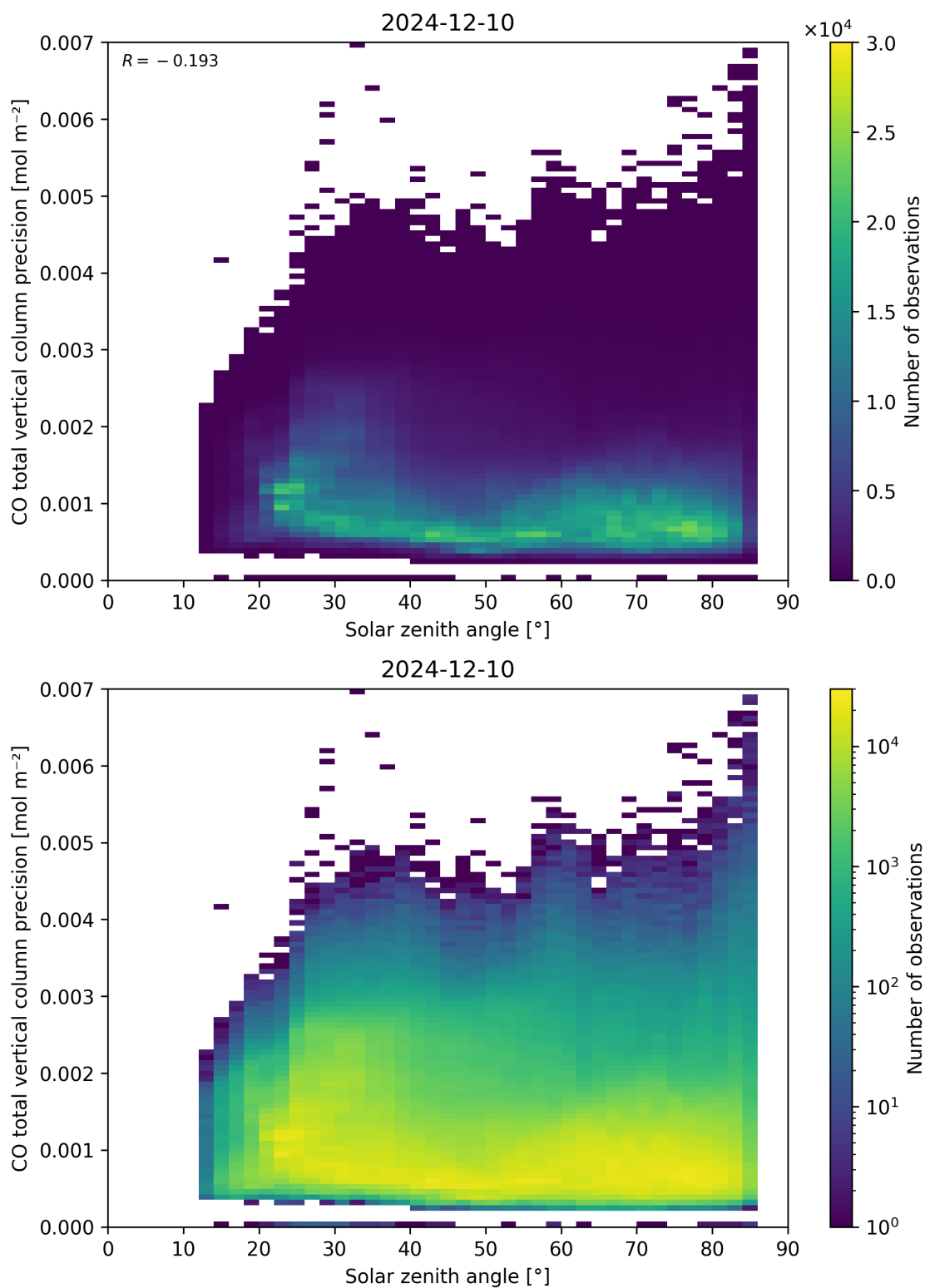
Figure 63: Scatter density plot of “Solar zenith angle” against “CO total vertical column precision” for 2024-12-09 to 2024-12-11.
