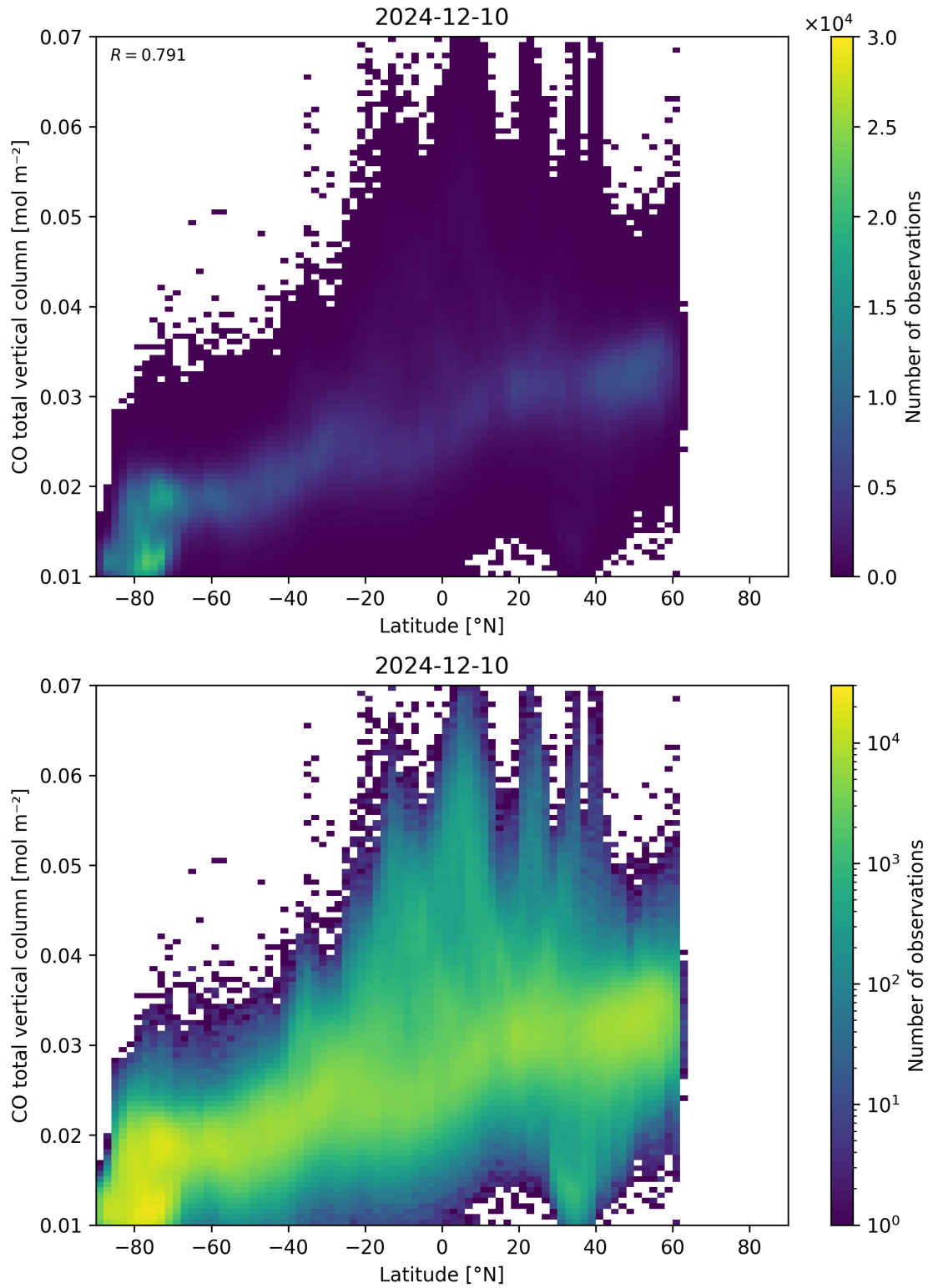
Figure 51: Scatter density plot of “Latitude” against “CO total vertical column” for 2024-12-09 to 2024-12-11.
