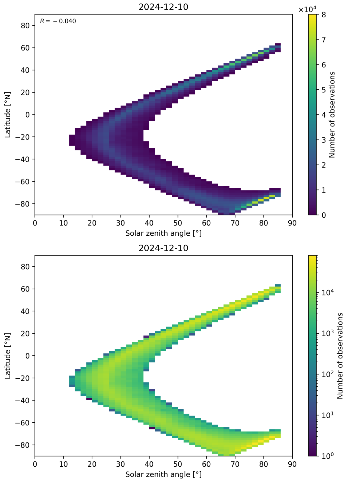
Figure 66: Scatter density plot of “Solar zenith angle” against “Latitude” for 2024-12-09 to 2024-12-11.
