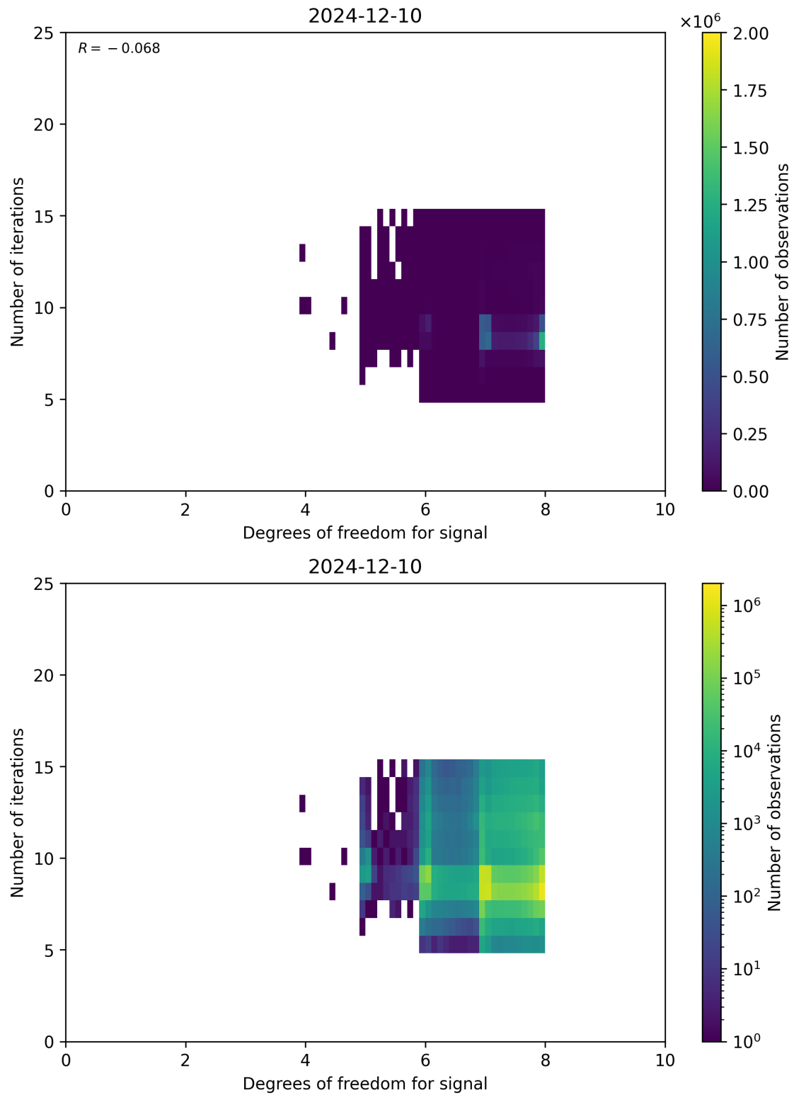
Figure 50: Scatter density plot of “Degrees of freedom for signal” against “Number of iterations” for 2024-12-09 to 2024-12-11.
