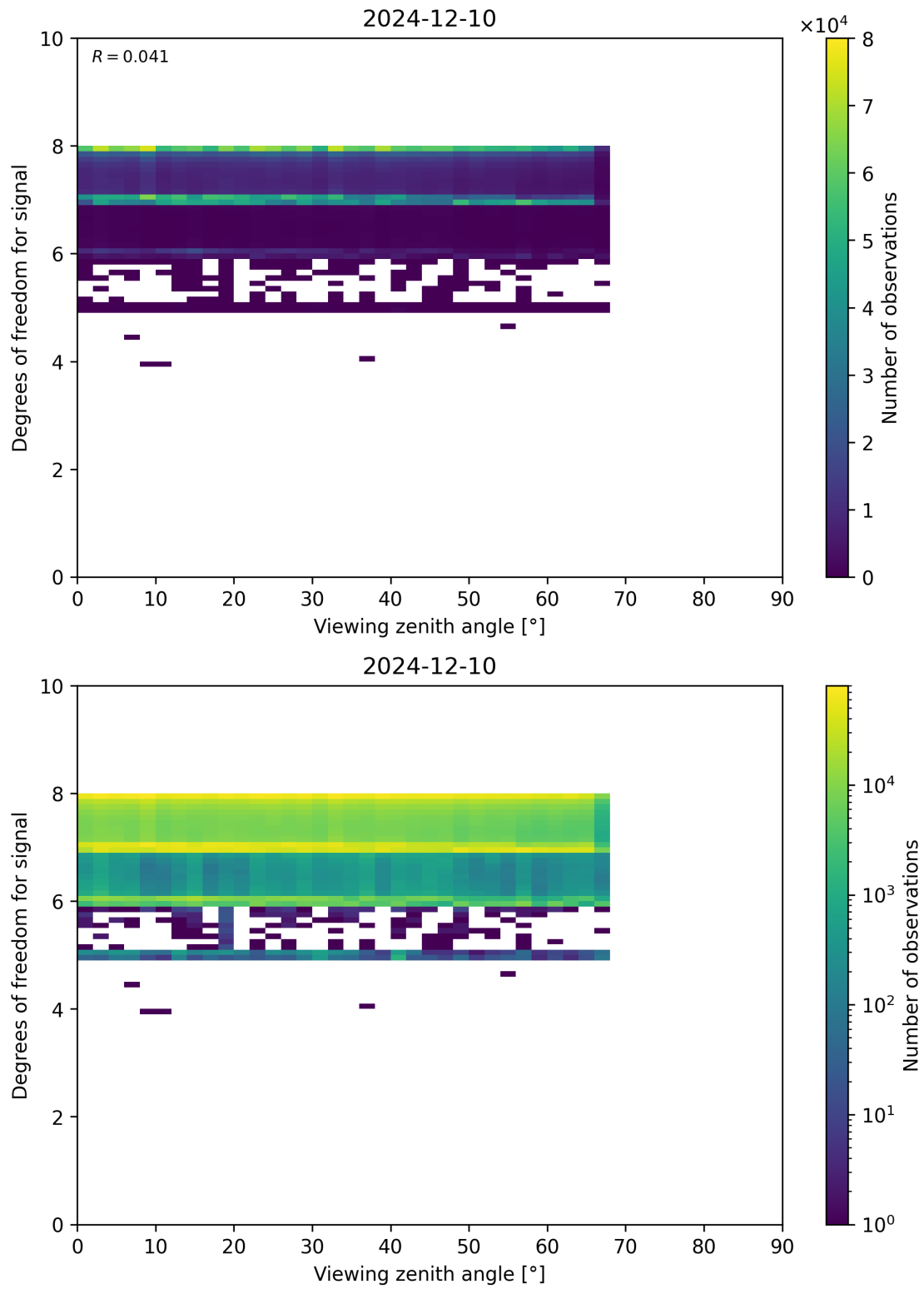
Figure 73: Scatter density plot of “Viewing zenith angle” against “Degrees of freedom for signal” for 2024-12-09 to 2024-12-11.
