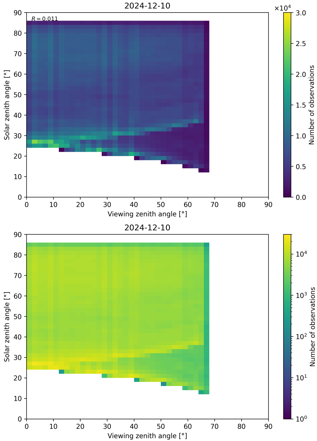
Figure 77: Scatter density plot of “Viewing zenith angle” against “Solar zenith angle” for 2024-12-09 to 2024-12-11.
