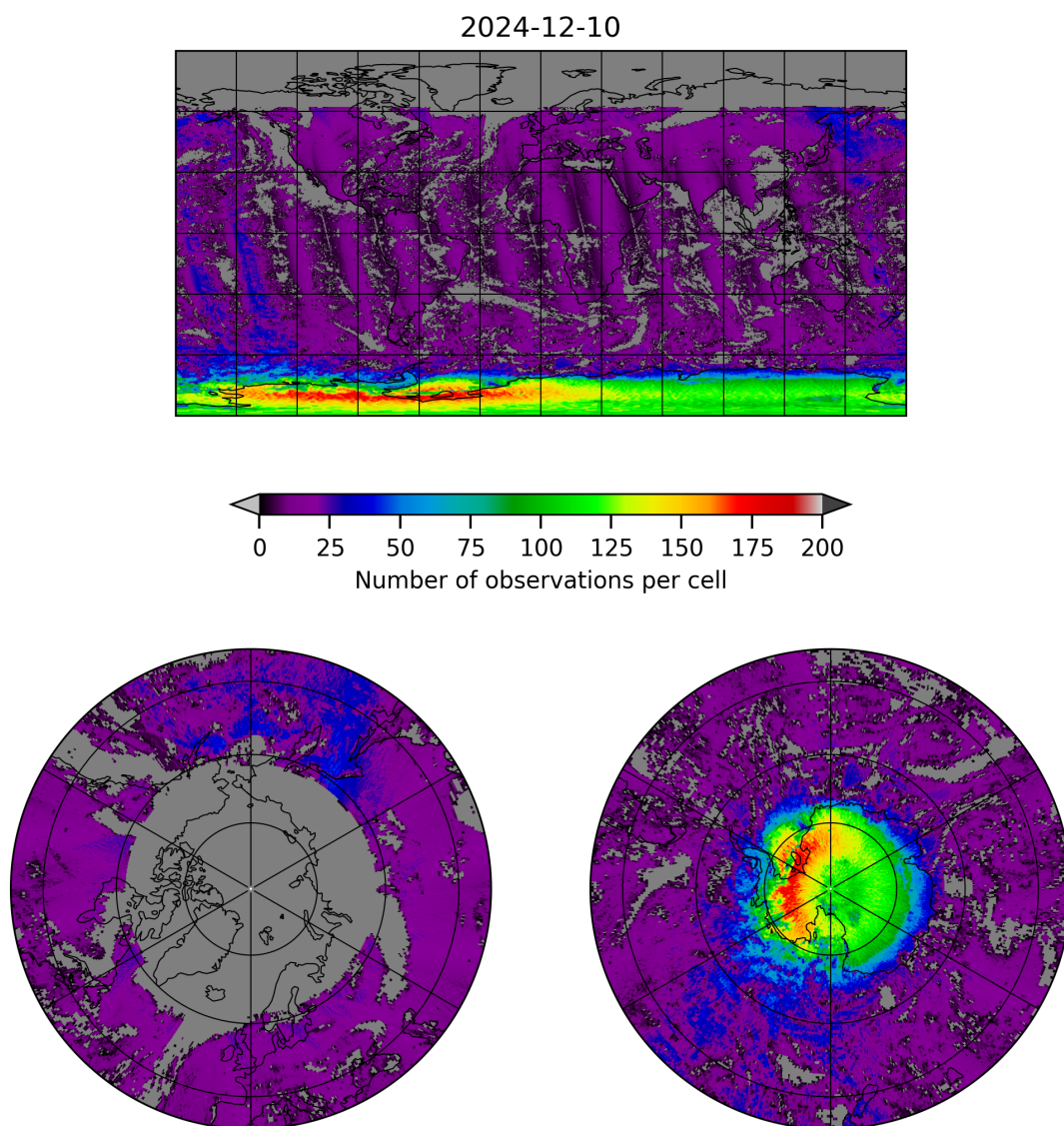
Figure 8: Map of the number of observations for 2024-12-09 to 2024-12-11
