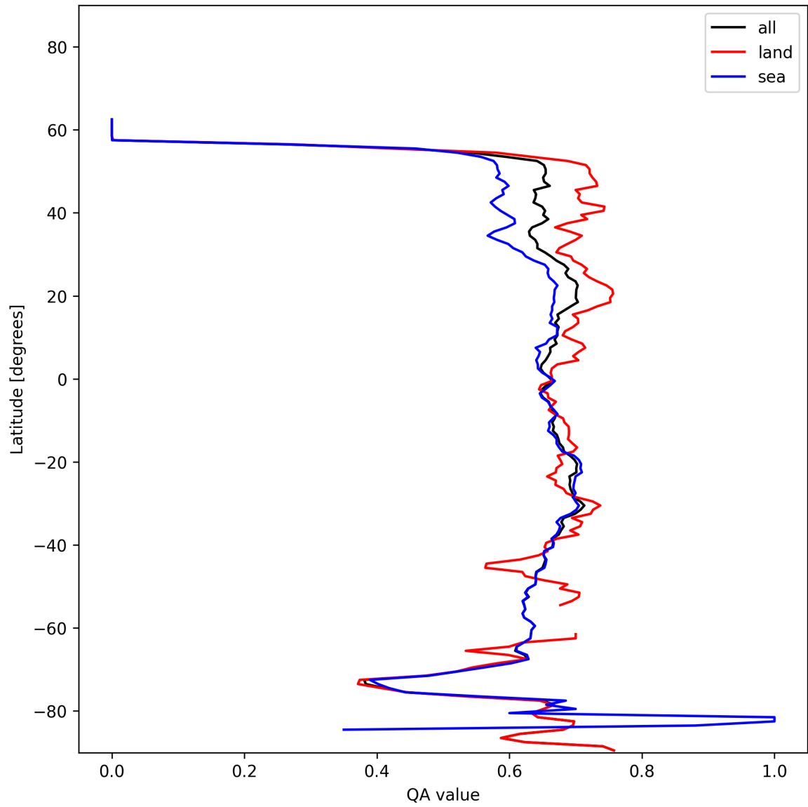
Figure 9: Zonal average of “QA value” for 2024-12-09 to 2024-12-11.
