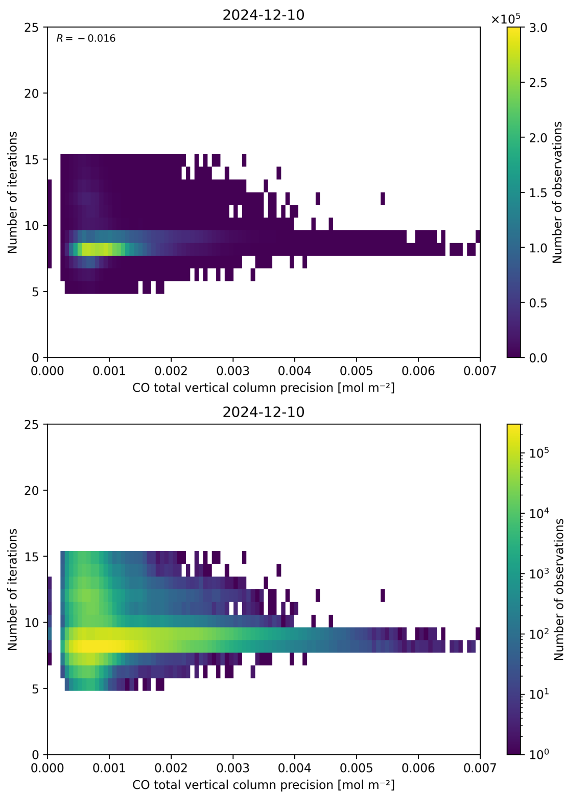
Figure 46: Scatter density plot of “CO total vertical column precision” against “Number of iterations” for 2024-12-09 to 2024-12-11.
