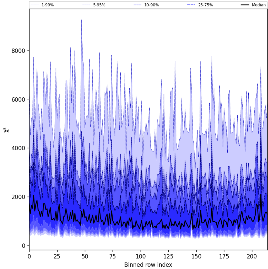
Figure 30: Along track statistics of “ \chi^2 ” for 2024-12-09 to 2024-12-11
