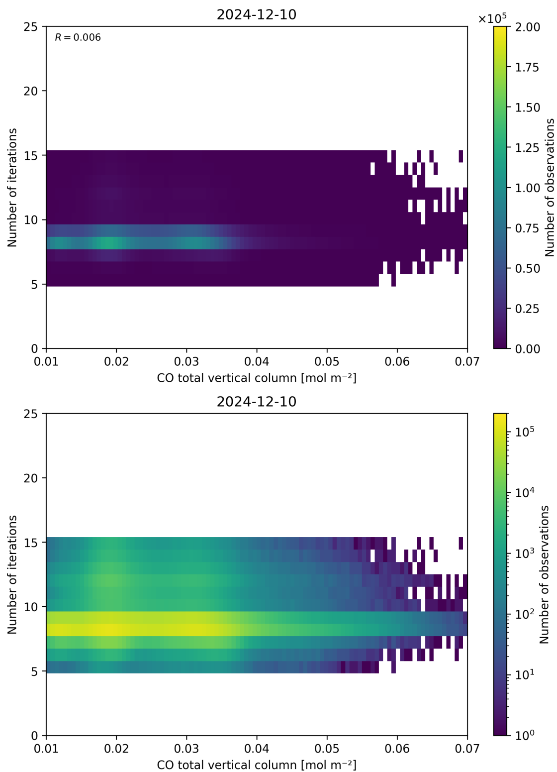
Figure 42: Scatter density plot of “CO total vertical column” against “Number of iterations” for 2024-12-09 to 2024-12-11.
