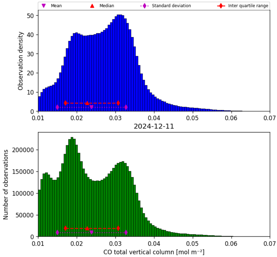
Figure 18: Histogram of “CO total vertical column” for 2024-12-11 to 2024-12-12
