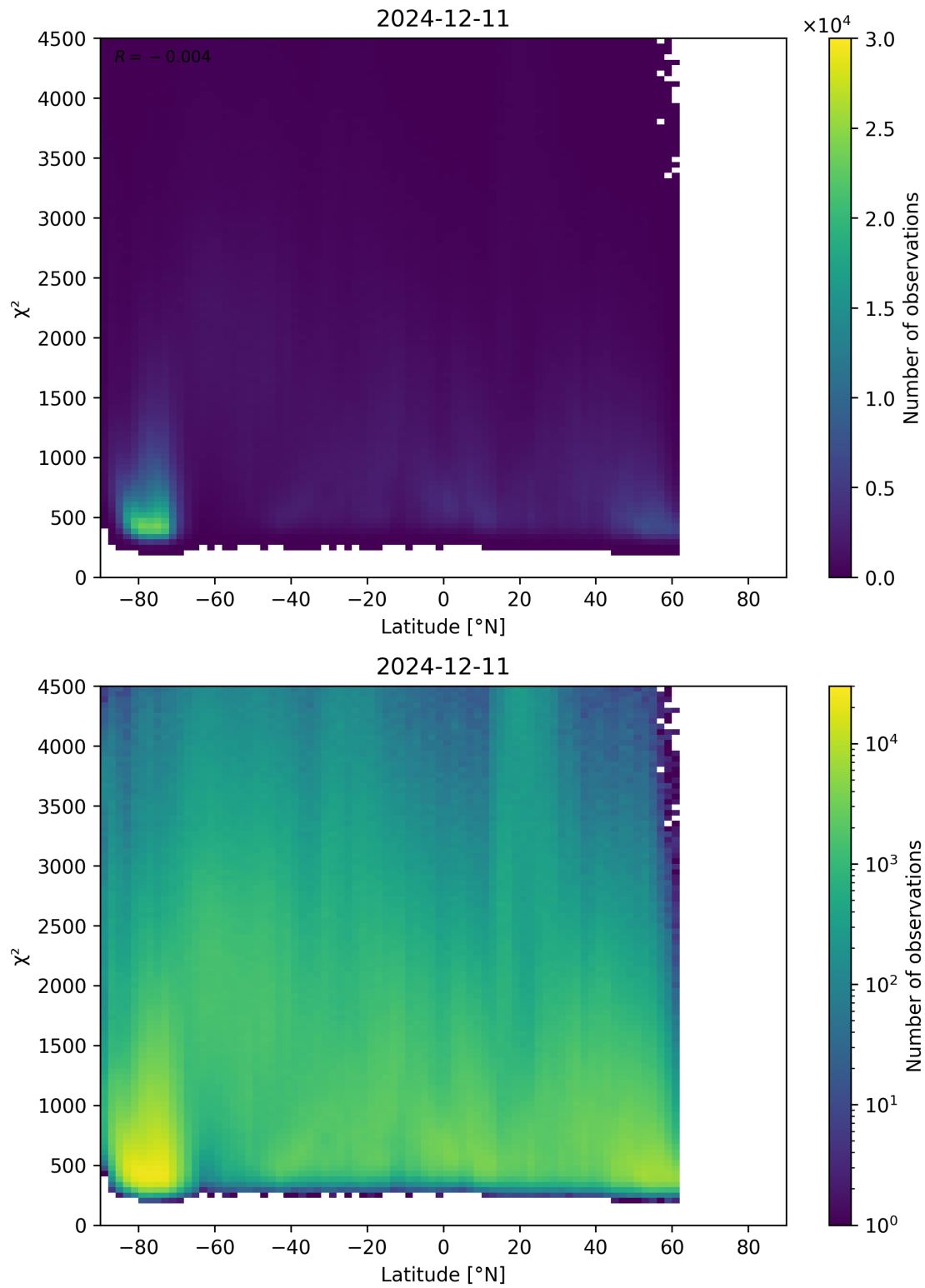
Figure 54: Scatter density plot of “Latitude” against “ \chi^2 ” for 2024-12-11 to 2024-12-12.
