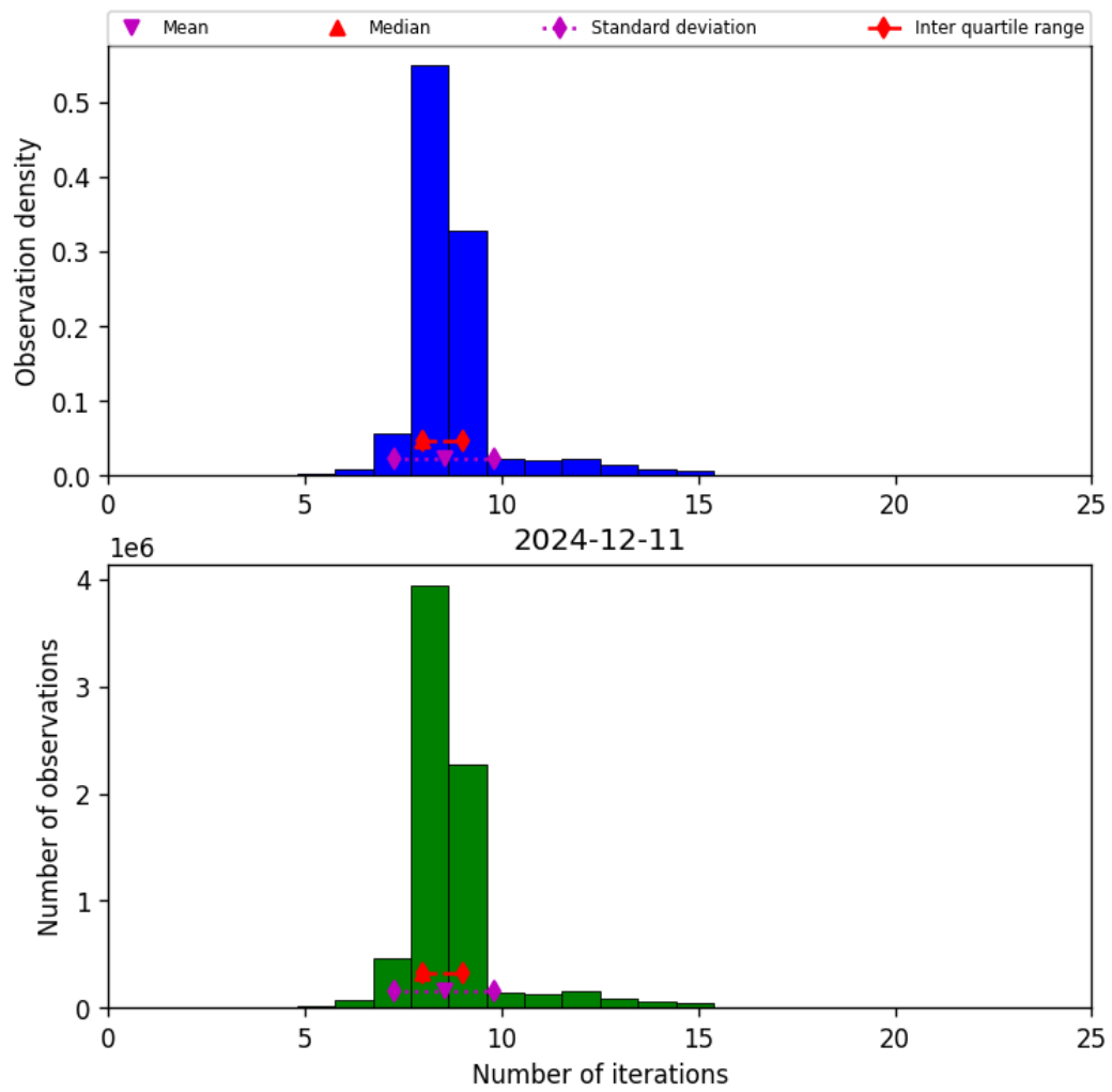
Figure 24: Histogram of “Number of iterations” for 2024-12-11 to 2024-12-12
