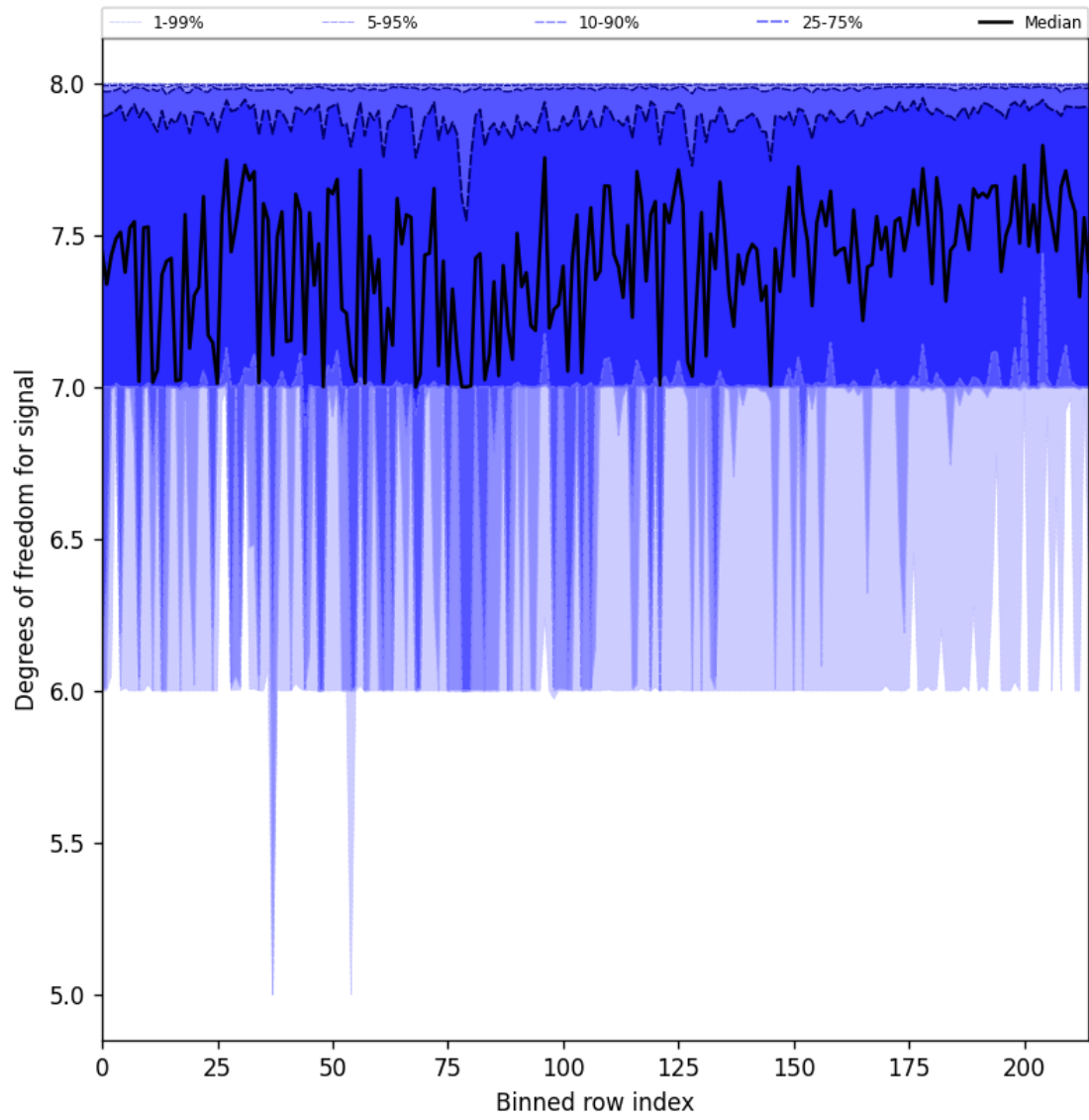
Figure 31: Along track statistics of “Degrees of freedom for signal” for 2024-12-11 to 2024-12-12
