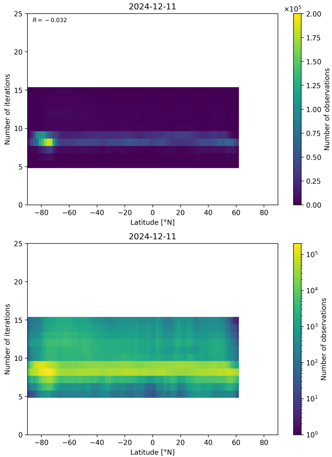
Figure 56: Scatter density plot of “Latitude” against “Number of iterations” for 2024-12-11 to 2024-12-12.
