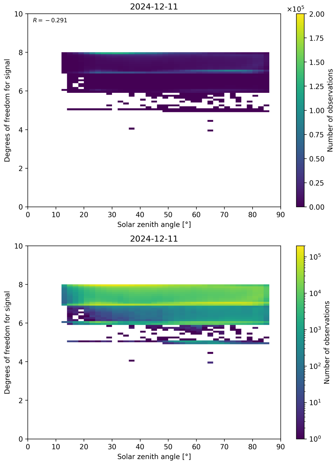
Figure 65: Scatter density plot of “Solar zenith angle” against “Degrees of freedom for signal” for 2024-12-11 to 2024-12-12.
