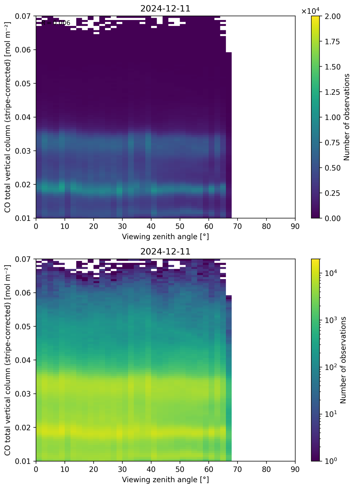
Figure 70: Scatter density plot of “Viewing zenith angle” against “CO total vertical column (stripe-corrected)” for 2024-12-11 to 2024-12-12.
