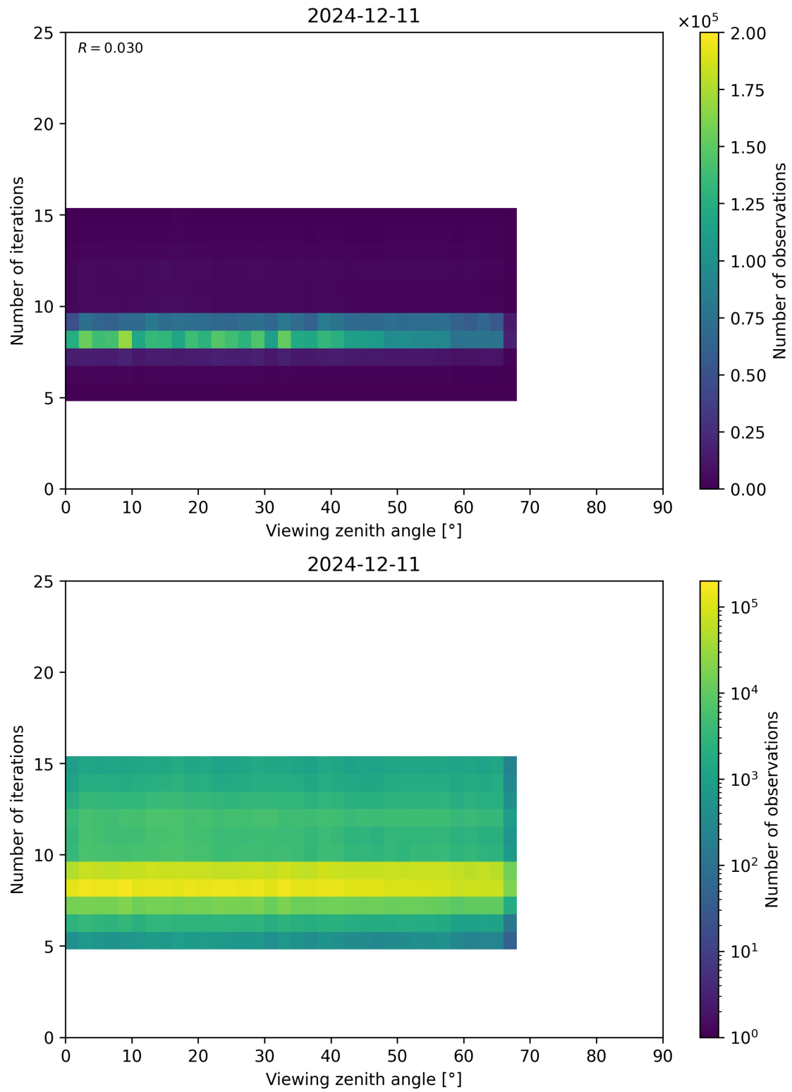
Figure 75: Scatter density plot of “Viewing zenith angle” against “Number of iterations” for 2024-12-11 to 2024-12-12.
