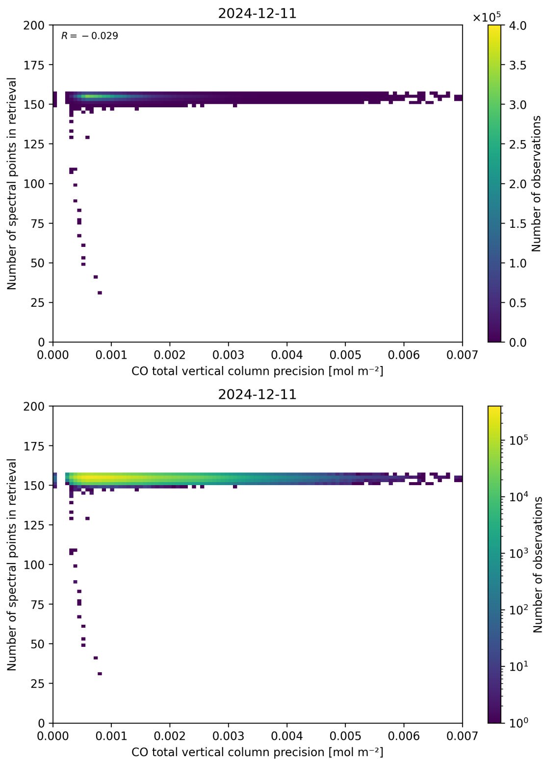
Figure 47: Scatter density plot of “CO total vertical column precision” against “Number of spectral points in retrieval” for 2024-12-11 to 2024-12-12.
