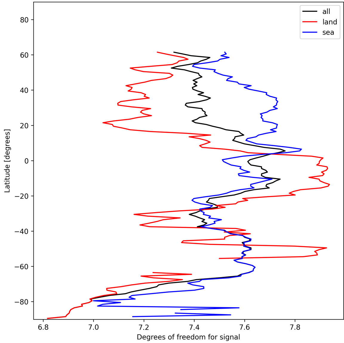
Figure 15: Zonal average of “Degrees of freedom for signal” for 2024-12-11 to 2024-12-12.
