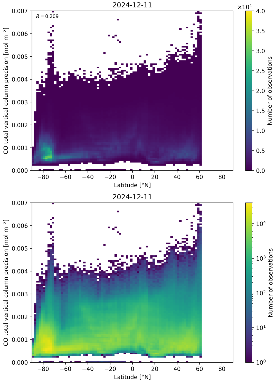
Figure 53: Scatter density plot of “Latitude” against “CO total vertical column precision” for 2024-12-11 to 2024-12-12.
