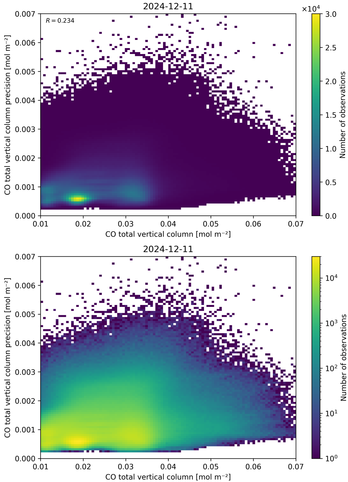
Figure 34: Scatter density plot of “CO total vertical column” against “CO total vertical column precision” for 2024-12-11 to 2024-12-12.
