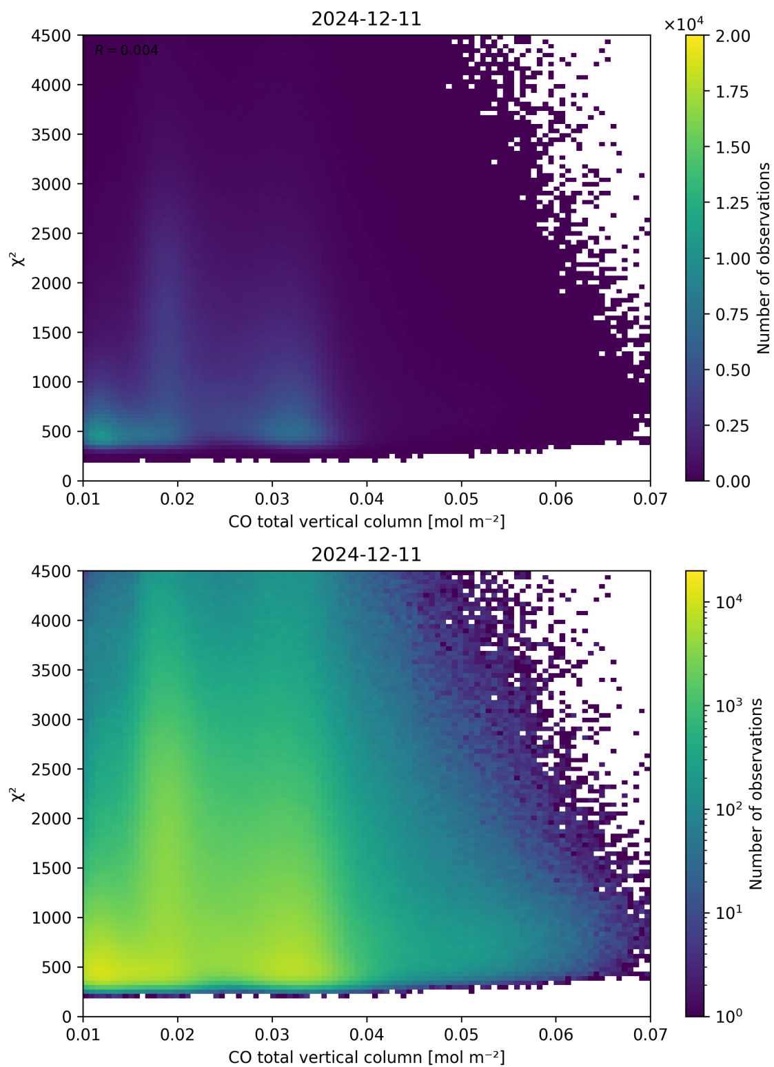
Figure 35: Scatter density plot of “CO total vertical column” against “ \chi^2 ” for 2024-12-11 to 2024-12-12.
