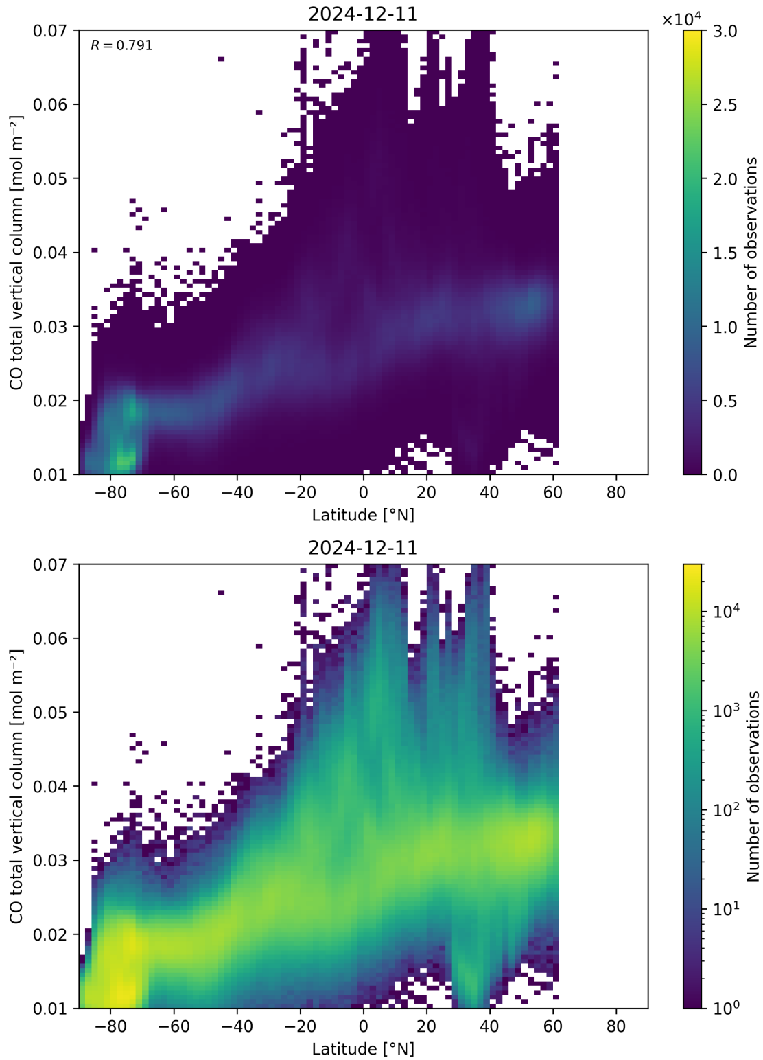
Figure 51: Scatter density plot of “Latitude” against “CO total vertical column” for 2024-12-11 to 2024-12-12.
