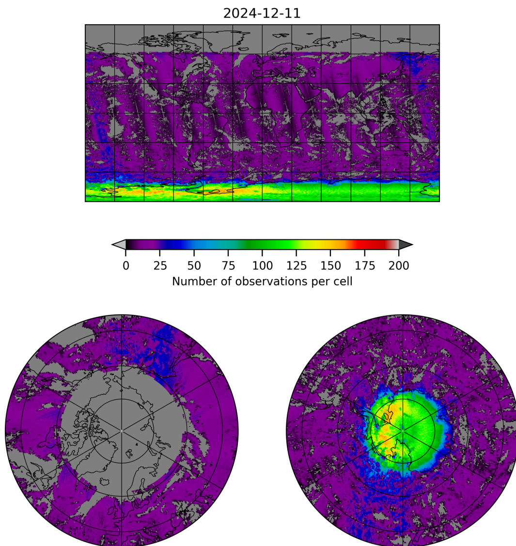
Figure 8: Map of the number of observations for 2024-12-11 to 2024-12-12
