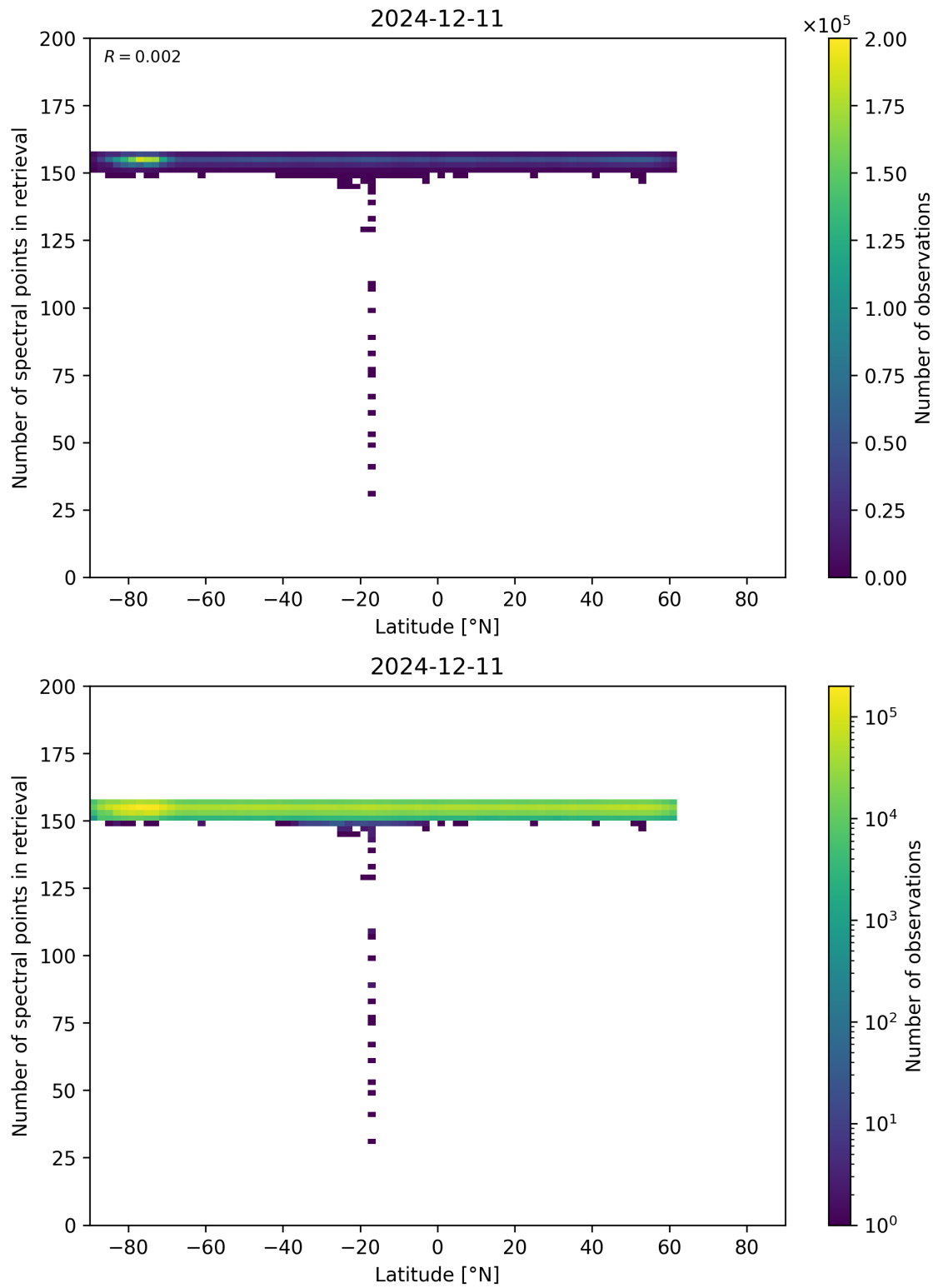
Figure 57: Scatter density plot of “Latitude” against “Number of spectral points in retrieval” for 2024-12-11 to 2024-12-12.
