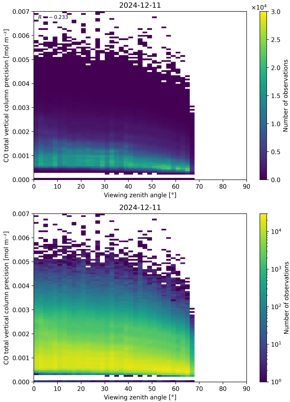
Figure 71: Scatter density plot of “Viewing zenith angle” against “CO total vertical column precision” for 2024-12-11 to 2024-12-12.
