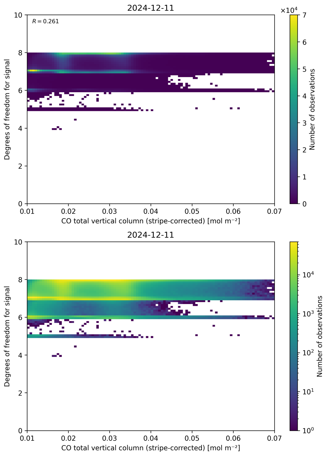
Figure 38: Scatter density plot of “CO total vertical column (stripe-corrected)” against “Degrees of freedom for signal” for 2024-12-11 to 2024-12-12.
