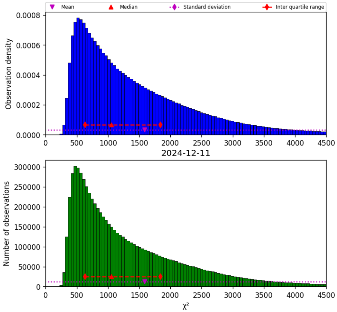
Figure 22: Histogram of “ \chi^2 ” for 2024-12-11 to 2024-12-12
