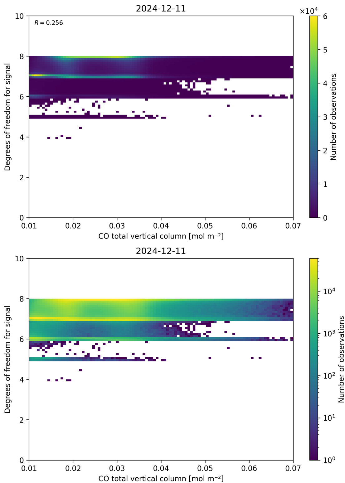
Figure 41: Scatter density plot of “CO total vertical column” against “Degrees of freedom for signal” for 2024-12-11 to 2024-12-12.
