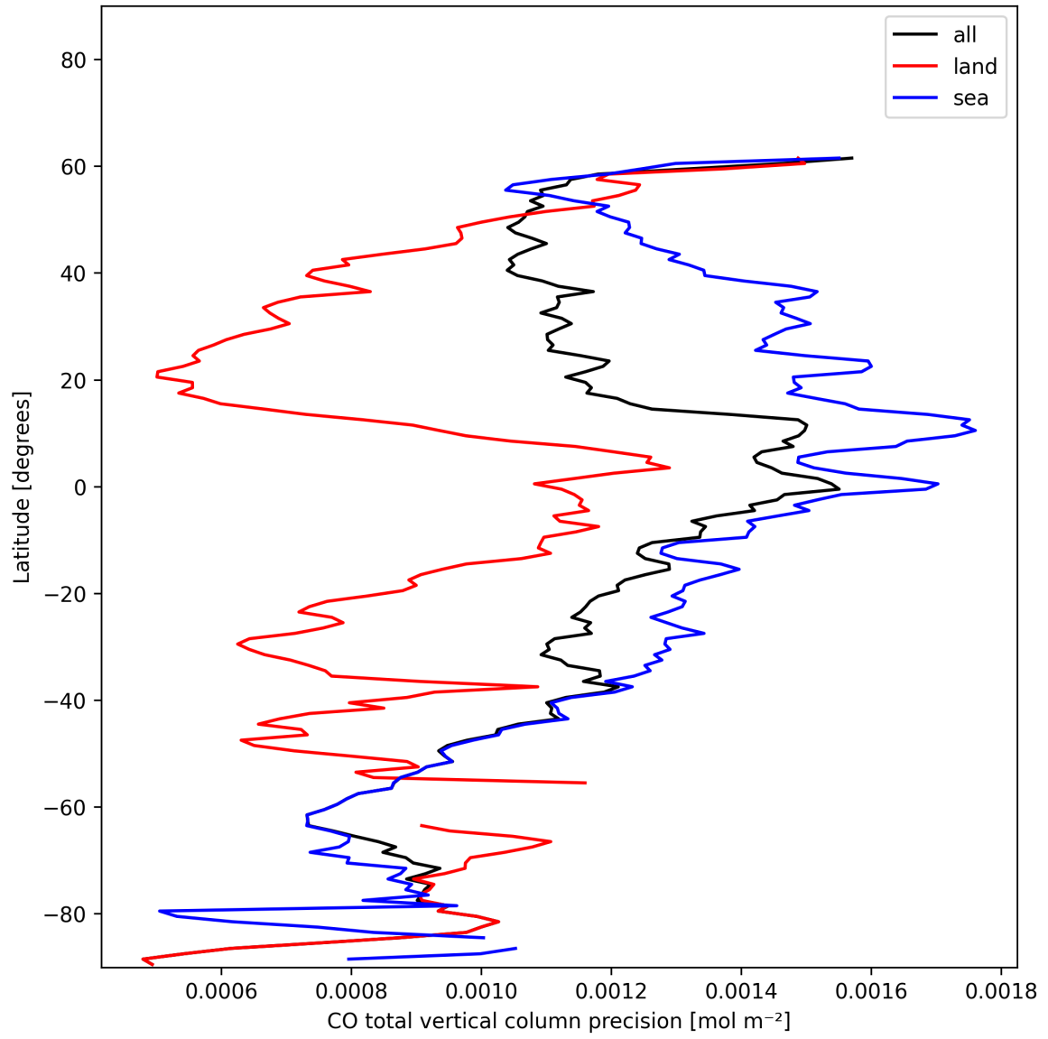
Figure 12: Zonal average of “CO total vertical column precision” for 2024-12-11 to 2024-12-12.
