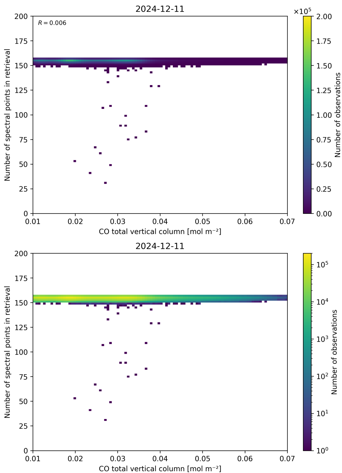
Figure 43: Scatter density plot of “CO total vertical column” against “Number of spectral points in retrieval” for 2024-12-11 to 2024-12-12.
