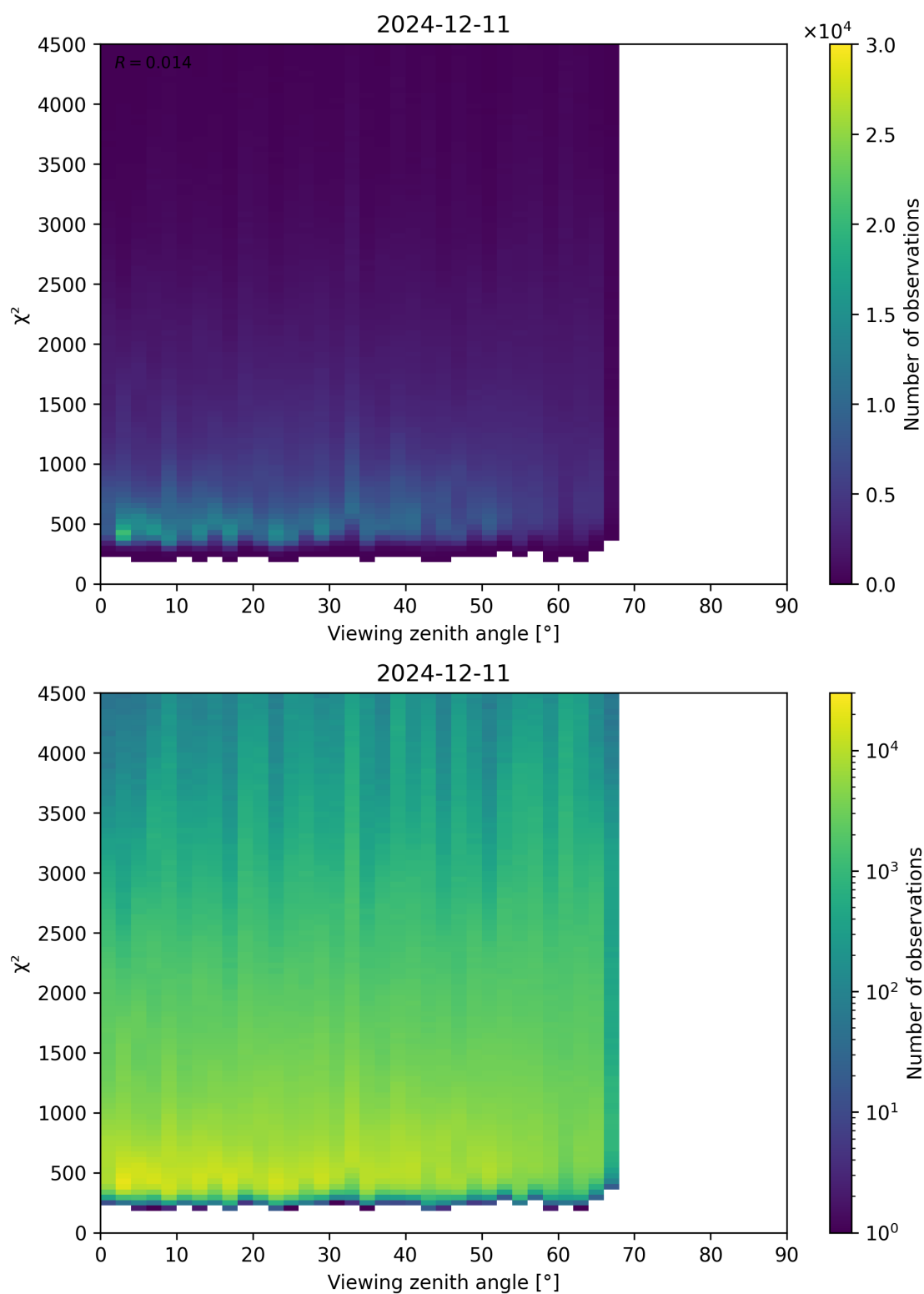
Figure 72: Scatter density plot of “Viewing zenith angle” against “ \chi^2 ” for 2024-12-11 to 2024-12-12.
