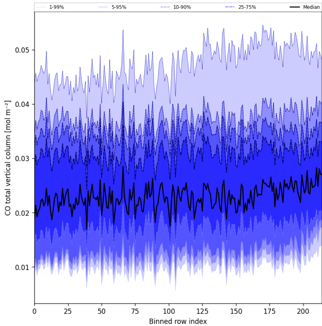
Figure 26: Along track statistics of “CO total vertical column” for 2024-12-11 to 2024-12-12
