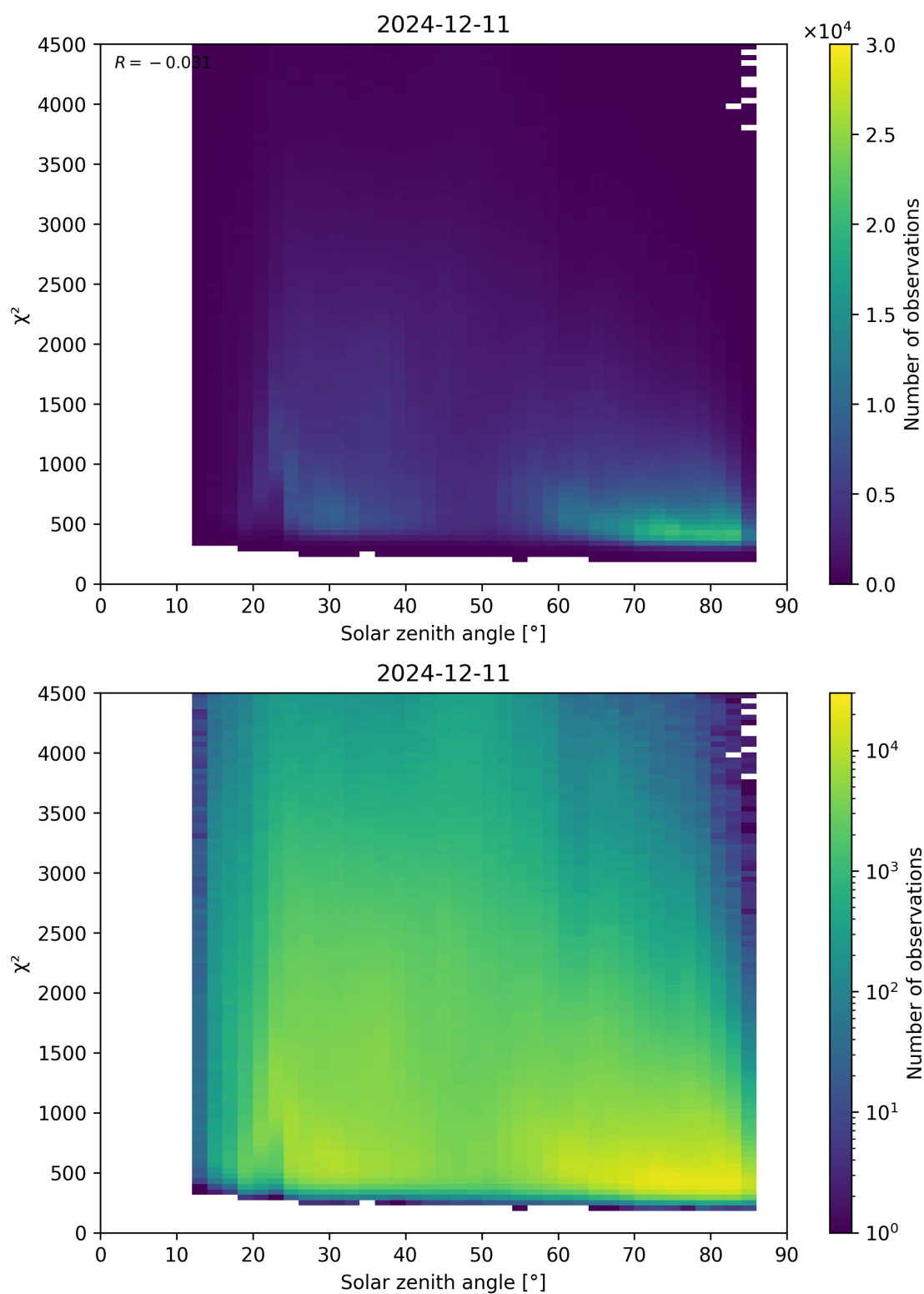
Figure 64: Scatter density plot of “Solar zenith angle” against “ \chi^2 ” for 2024-12-11 to 2024-12-12.
