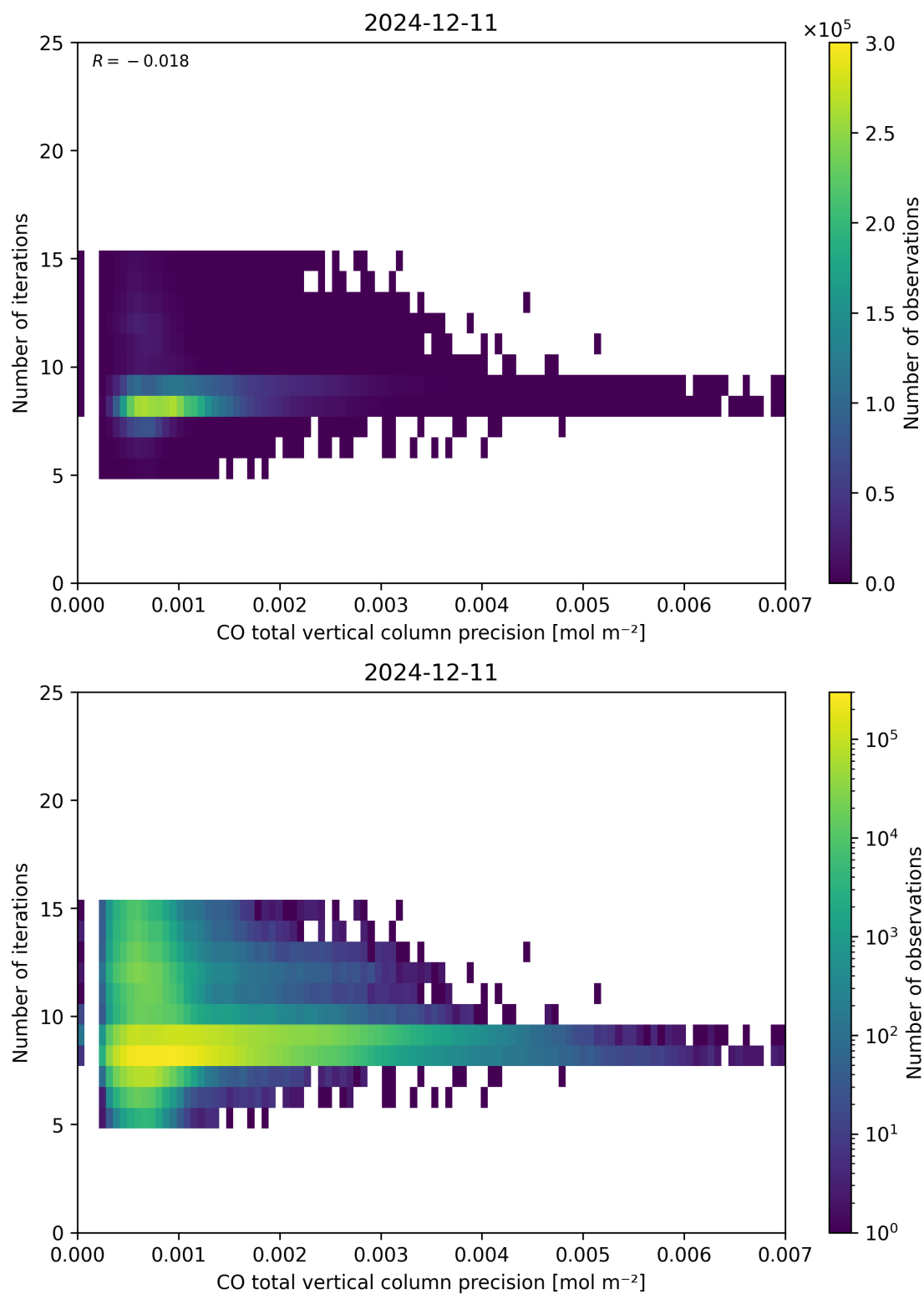
Figure 46: Scatter density plot of “CO total vertical column precision” against “Number of iterations” for 2024-12-11 to 2024-12-12.
