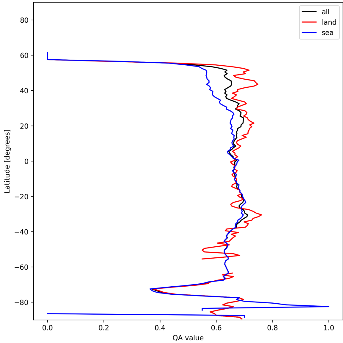
Figure 9: Zonal average of “QA value” for 2024-12-11 to 2024-12-12.
