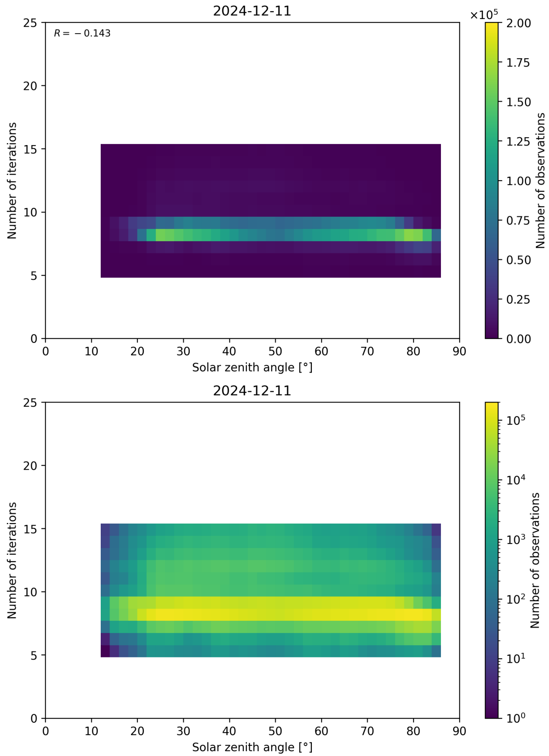
Figure 67: Scatter density plot of “Solar zenith angle” against “Number of iterations” for 2024-12-11 to 2024-12-12.
