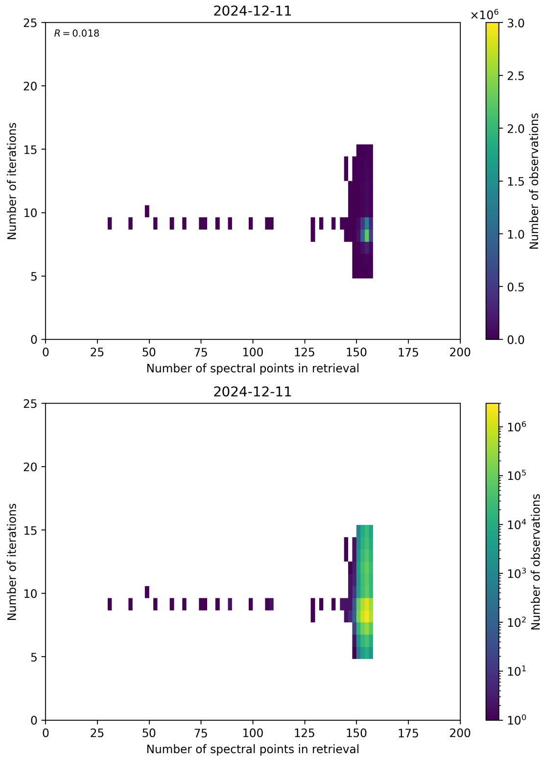
Figure 60: Scatter density plot of “Number of spectral points in retrieval” against “Number of iterations” for 2024-12-11 to 2024-12-12.
