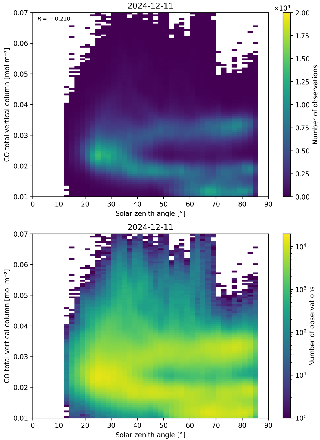
Figure 61: Scatter density plot of “Solar zenith angle” against “CO total vertical column” for 2024-12-11 to 2024-12-12.
