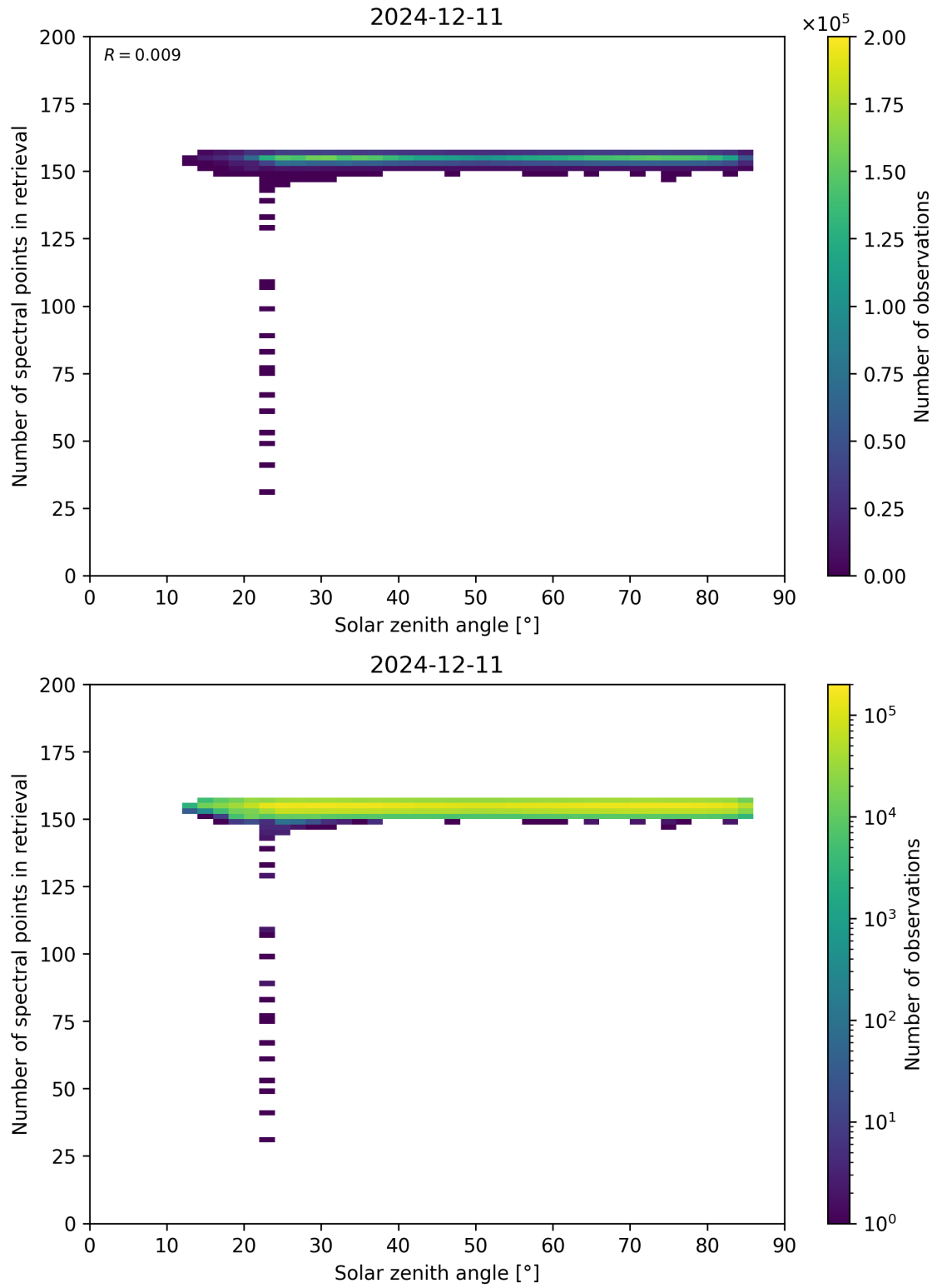
Figure 68: Scatter density plot of “Solar zenith angle” against “Number of spectral points in retrieval” for 2024-12-11 to 2024-12-12.
