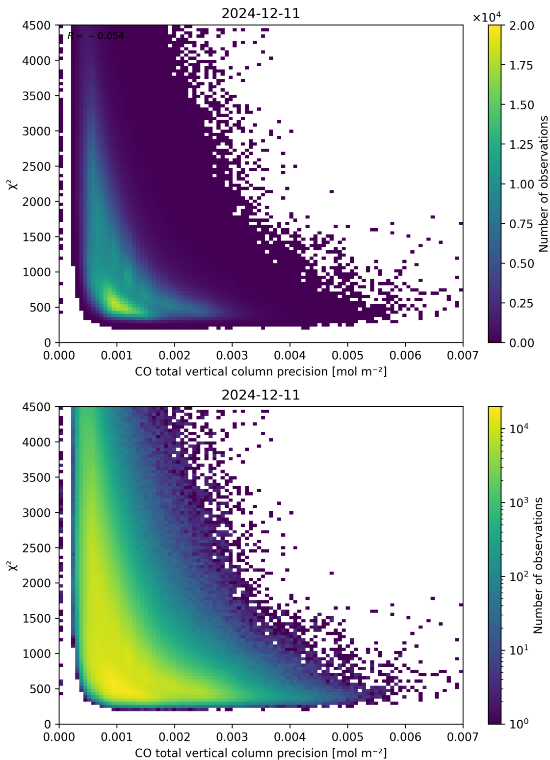
Figure 44: Scatter density plot of “CO total vertical column precision” against “ \chi^2 ” for 2024-12-11 to 2024-12-12.
