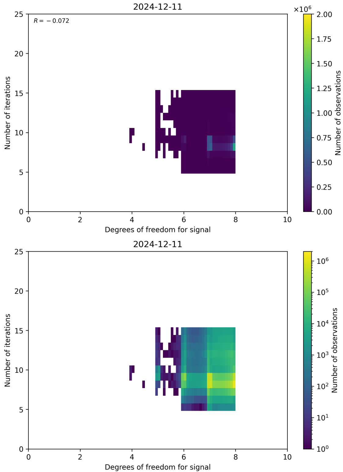
Figure 50: Scatter density plot of “Degrees of freedom for signal” against “Number of iterations” for 2024-12-11 to 2024-12-12.
