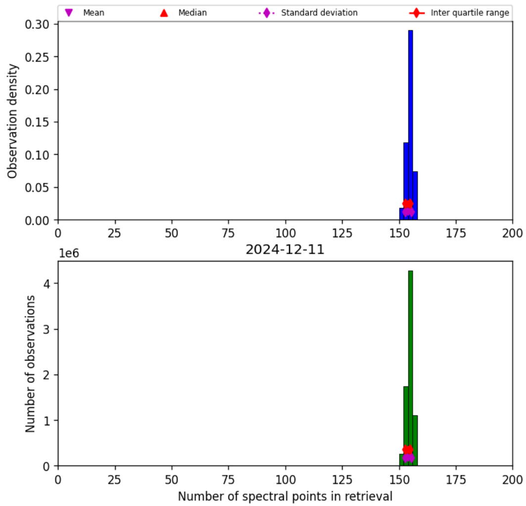
Figure 21: Histogram of “Number of spectral points in retrieval” for 2024-12-11 to 2024-12-12
