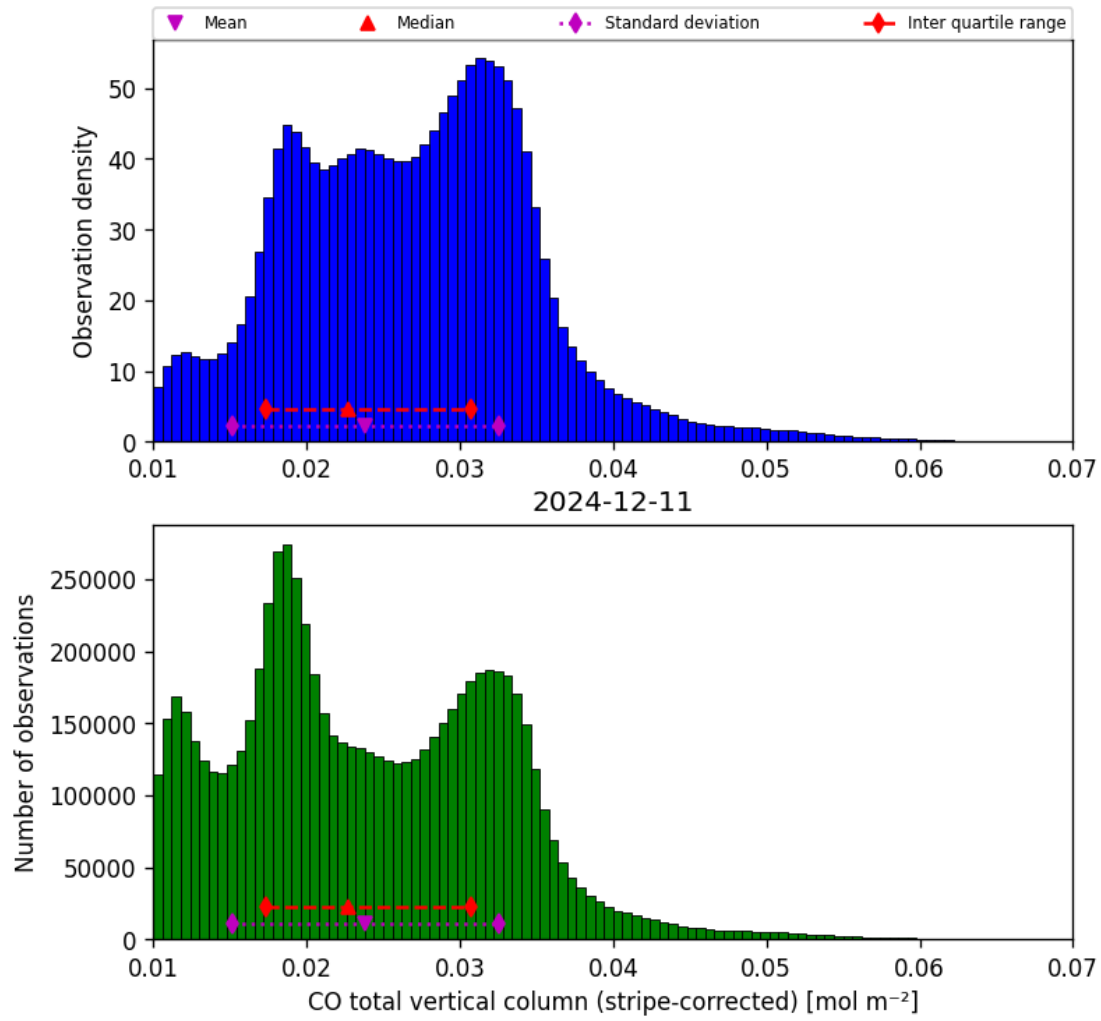
Figure 19: Histogram of “CO total vertical column (stripe-corrected)” for 2024-12-11 to 2024-12-12
