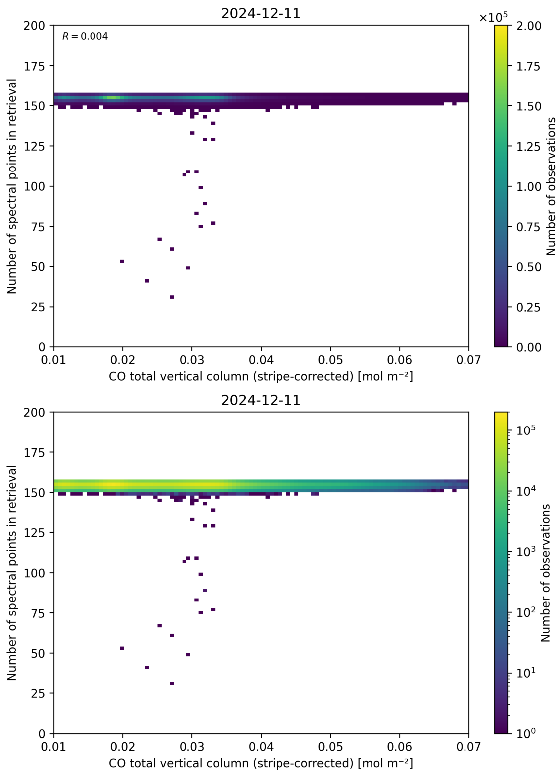
Figure 40: Scatter density plot of “CO total vertical column (stripe-corrected)” against “Number of spectral points in retrieval” for 2024-12-11 to 2024-12-12.
