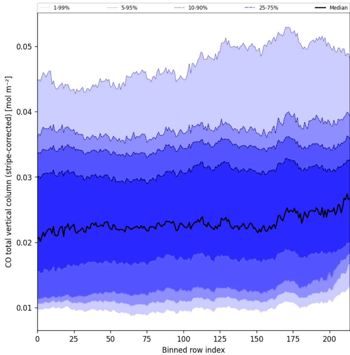
Figure 27: Along track statistics of “CO total vertical column (stripe-corrected)” for 2024-12-11 to 2024-12-12
