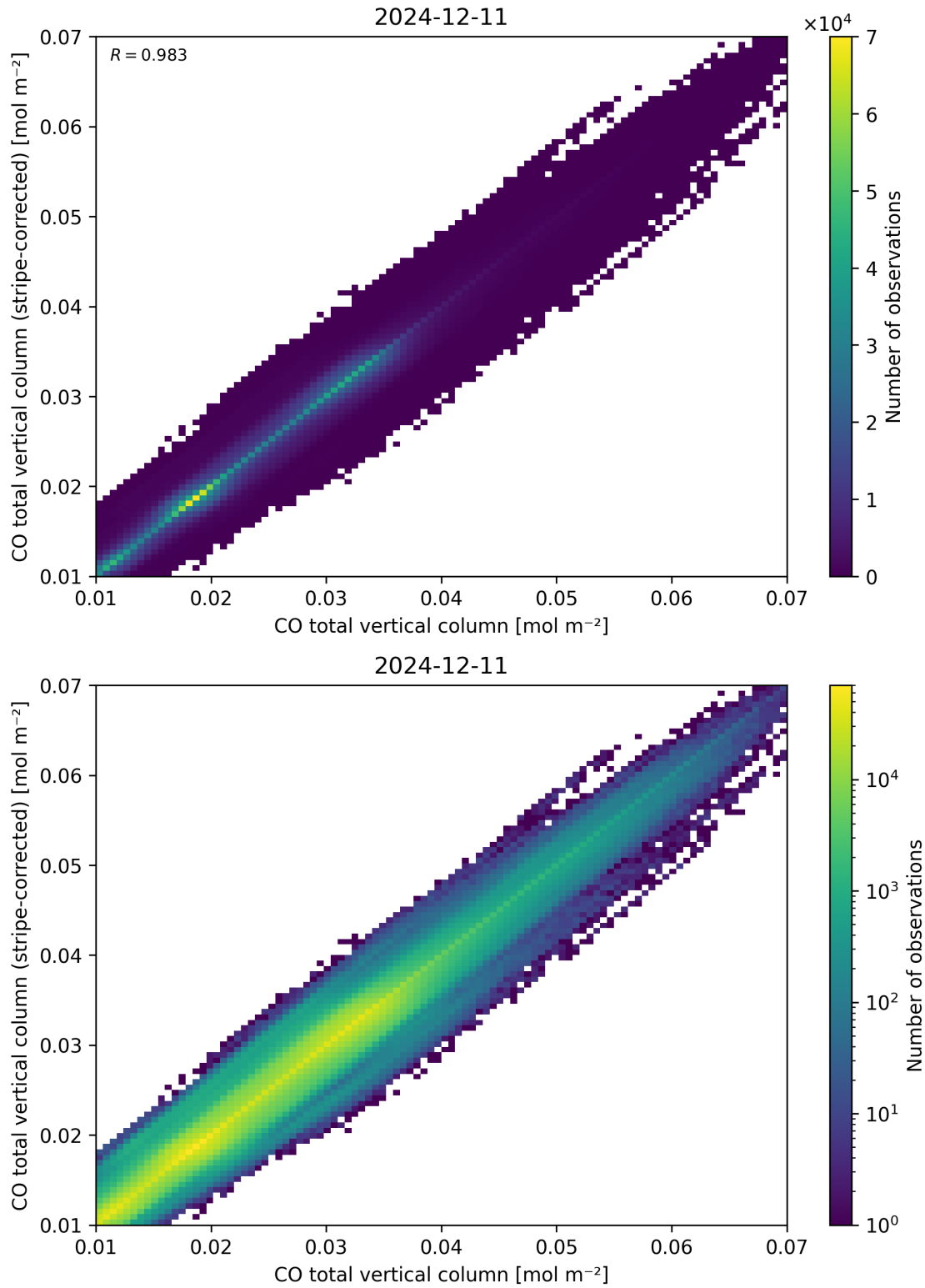
Figure 33: Scatter density plot of “CO total vertical column” against “CO total vertical column (stripe-corrected)” for 2024-12-11 to 2024-12-12.
