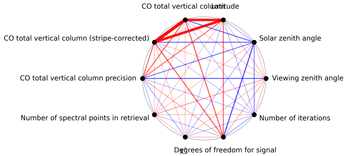
Figure 1: Map of correlation graph for 2024-12-11 to 2024-12-12.
