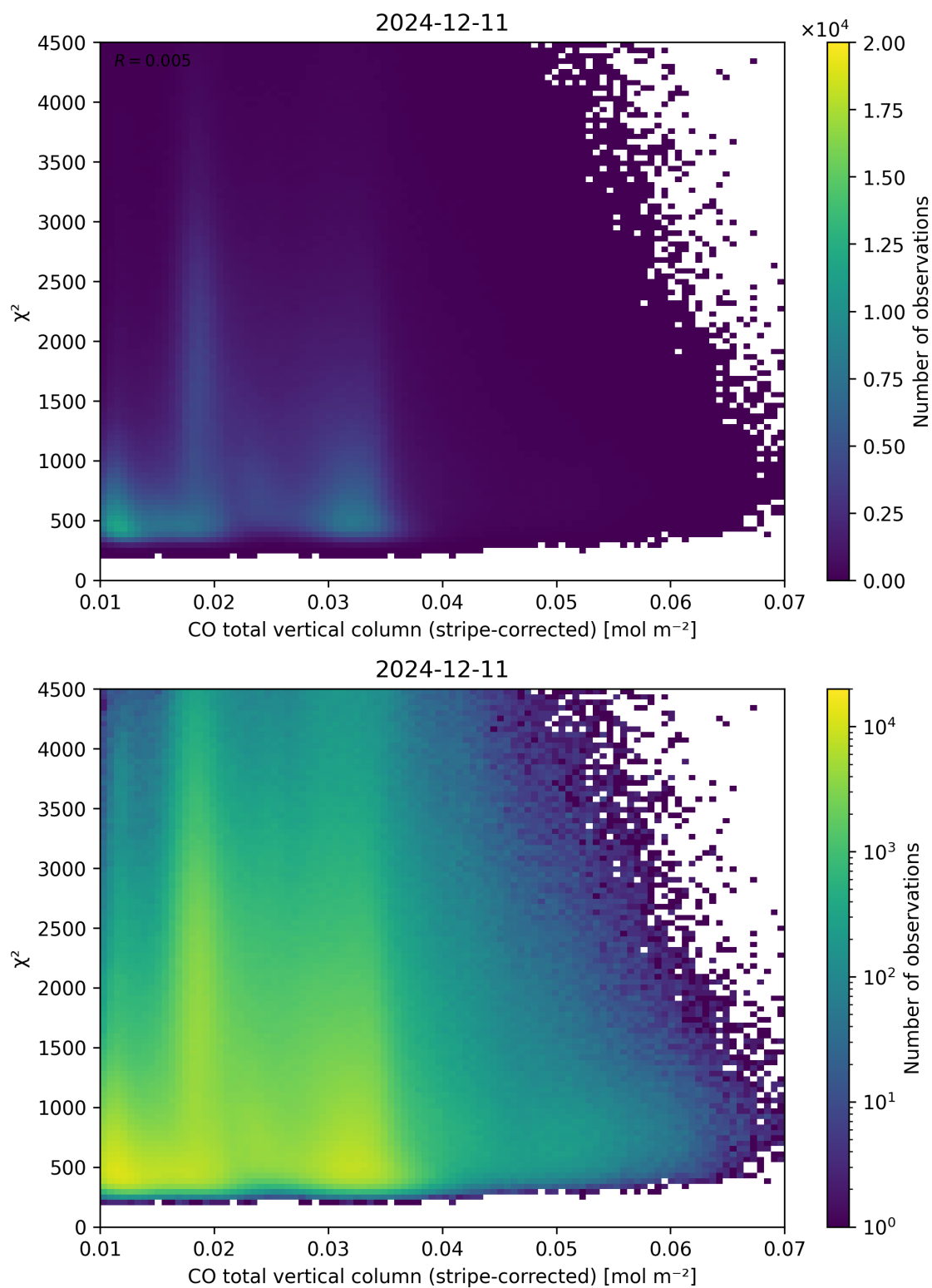
Figure 37: Scatter density plot of “CO total vertical column (stripe-corrected)” against “ \chi^2 ” for 2024-12-11 to 2024-12-12.
