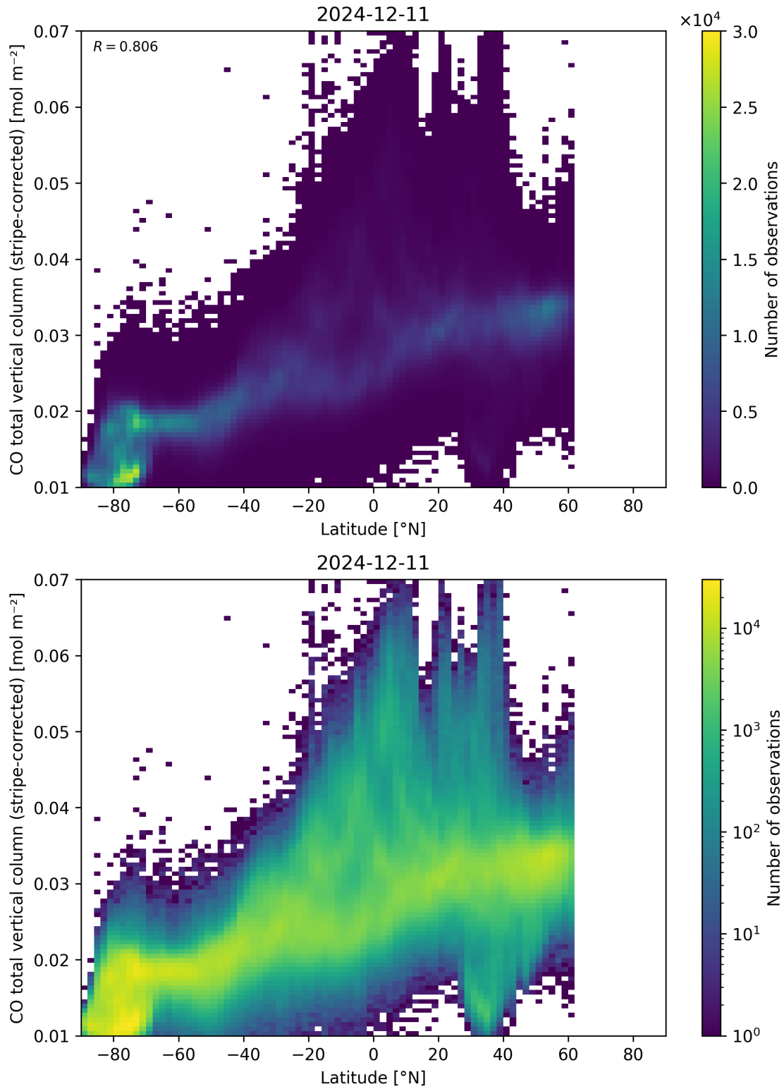
Figure 52: Scatter density plot of “Latitude” against “CO total vertical column (stripe-corrected)” for 2024-12-11 to 2024-12-12.
