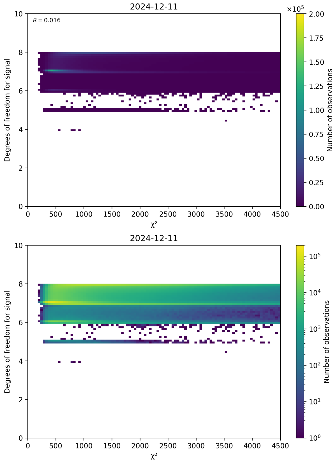
Figure 48: Scatter density plot of “ \chi^2 ” against “Degrees of freedom for signal” for 2024-12-11 to 2024-12-12.
