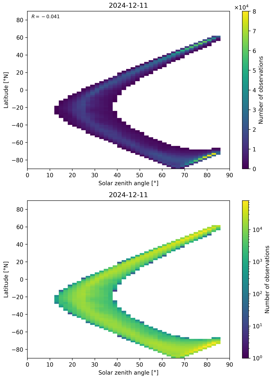
Figure 66: Scatter density plot of “Solar zenith angle” against “Latitude” for 2024-12-11 to 2024-12-12.
