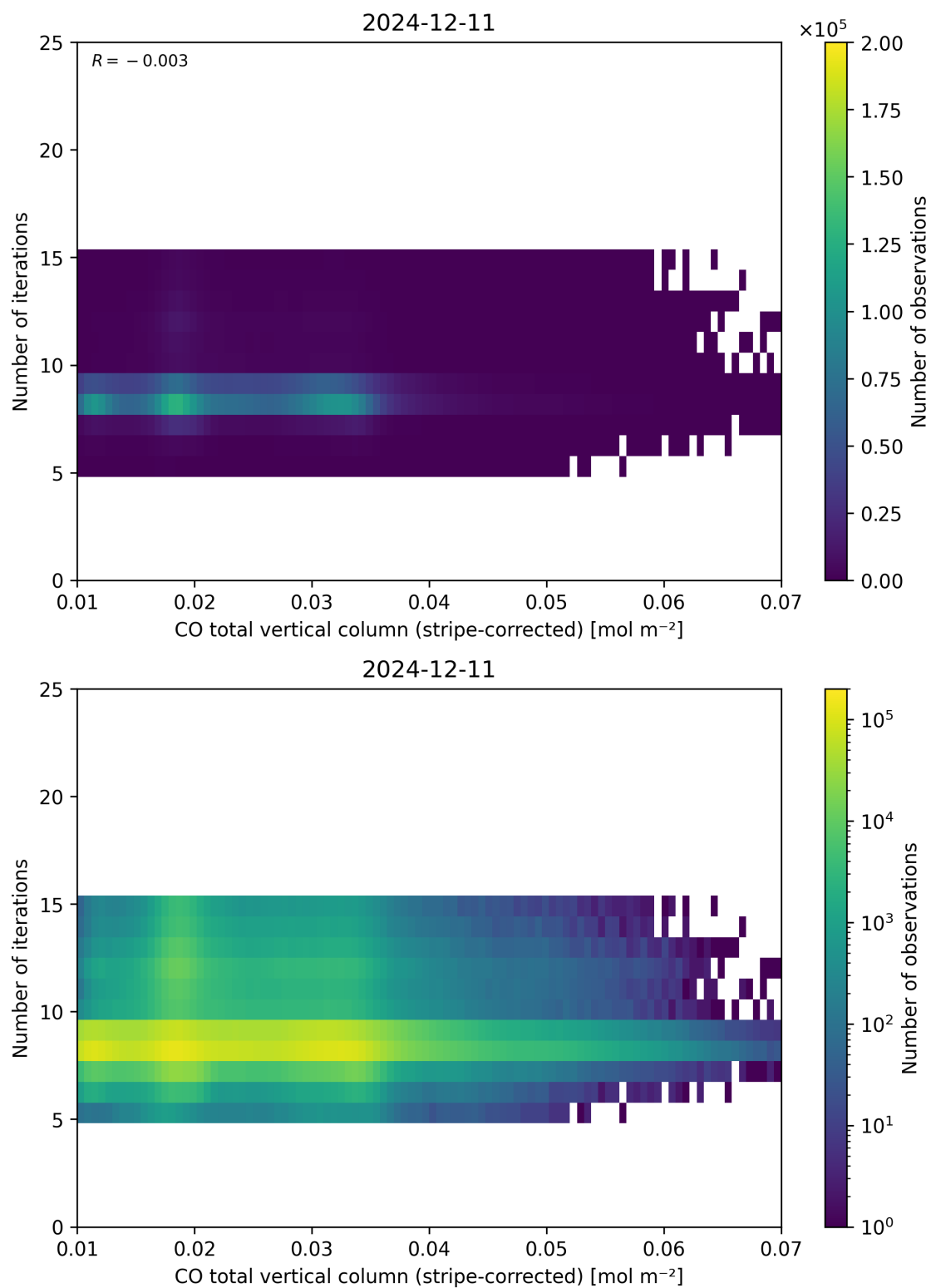
Figure 39: Scatter density plot of “CO total vertical column (stripe-corrected)” against “Number of iterations” for 2024-12-11 to 2024-12-12.
