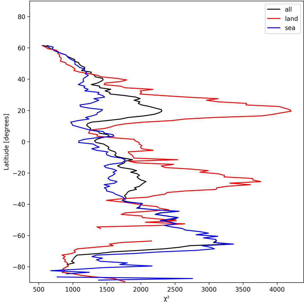
Figure 14: Zonal average of “ \chi^2 ” for 2024-12-11 to 2024-12-12.
