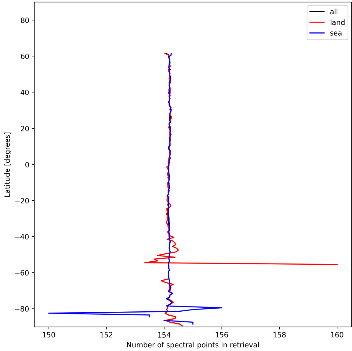
Figure 13: Zonal average of “Number of spectral points in retrieval” for 2024-12-11 to 2024-12-12.
