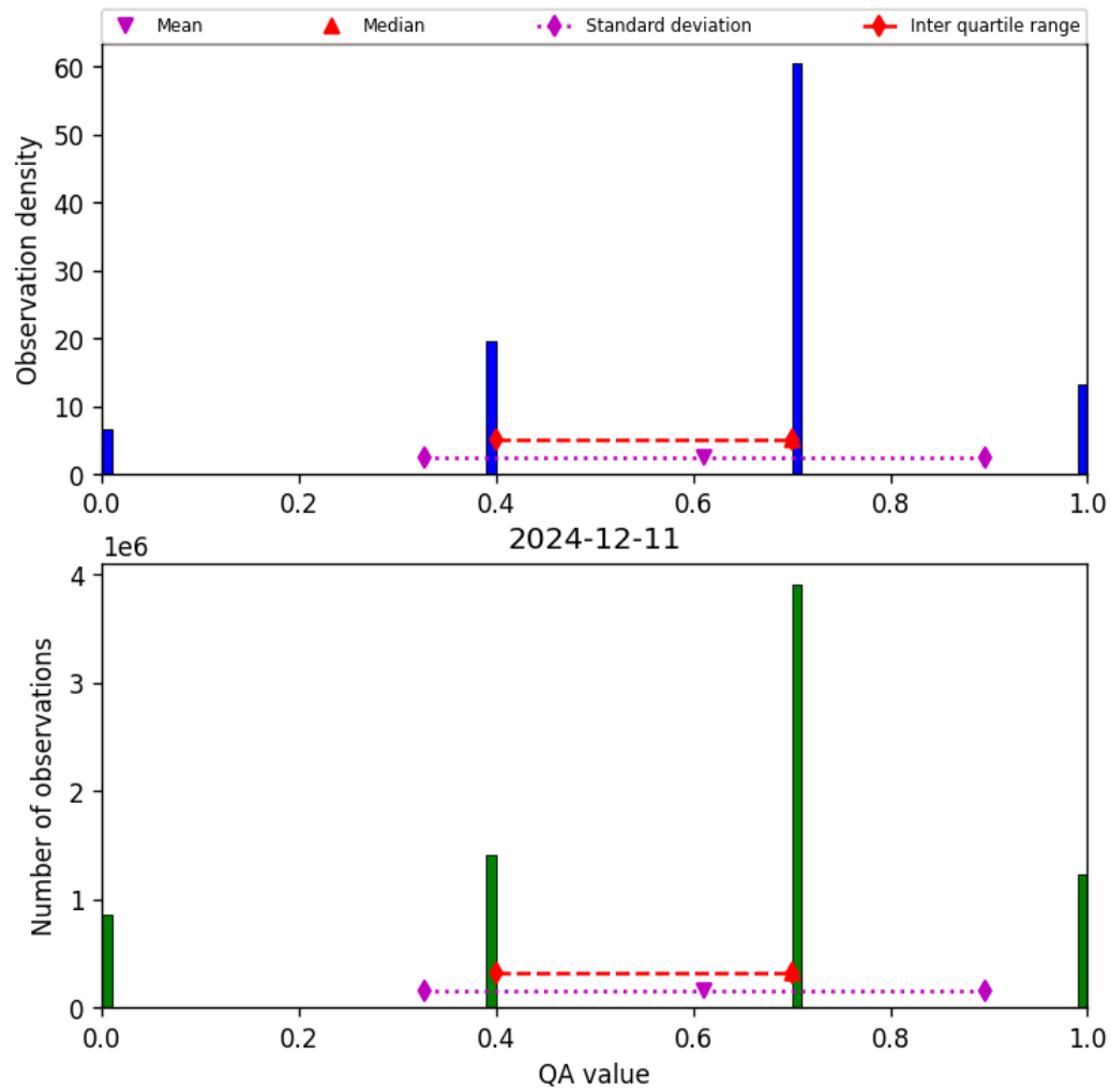
Figure 17: Histogram of “QA value” for 2024-12-11 to 2024-12-12
