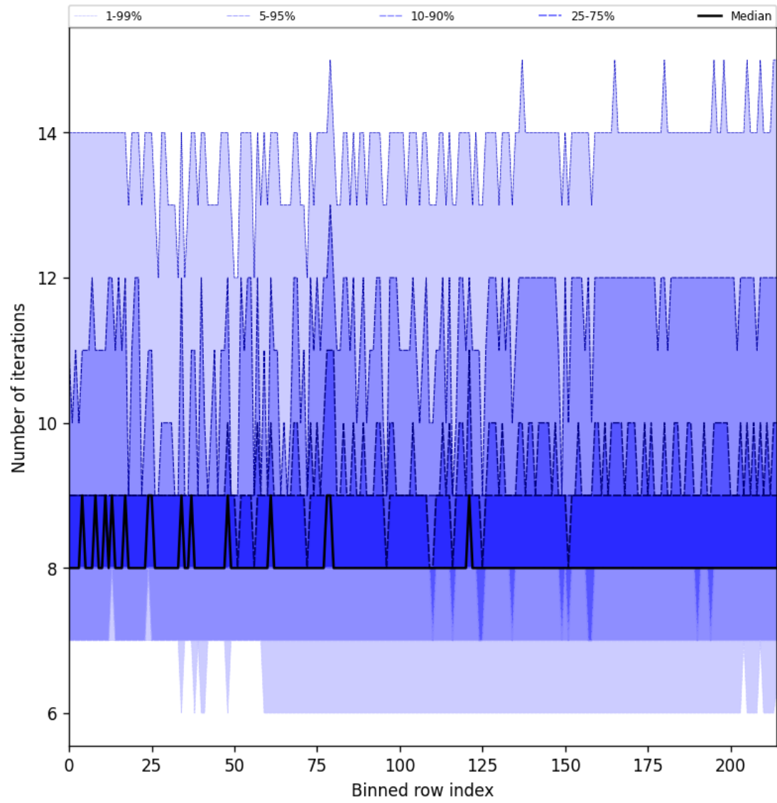
Figure 32: Along track statistics of “Number of iterations” for 2024-12-11 to 2024-12-12
