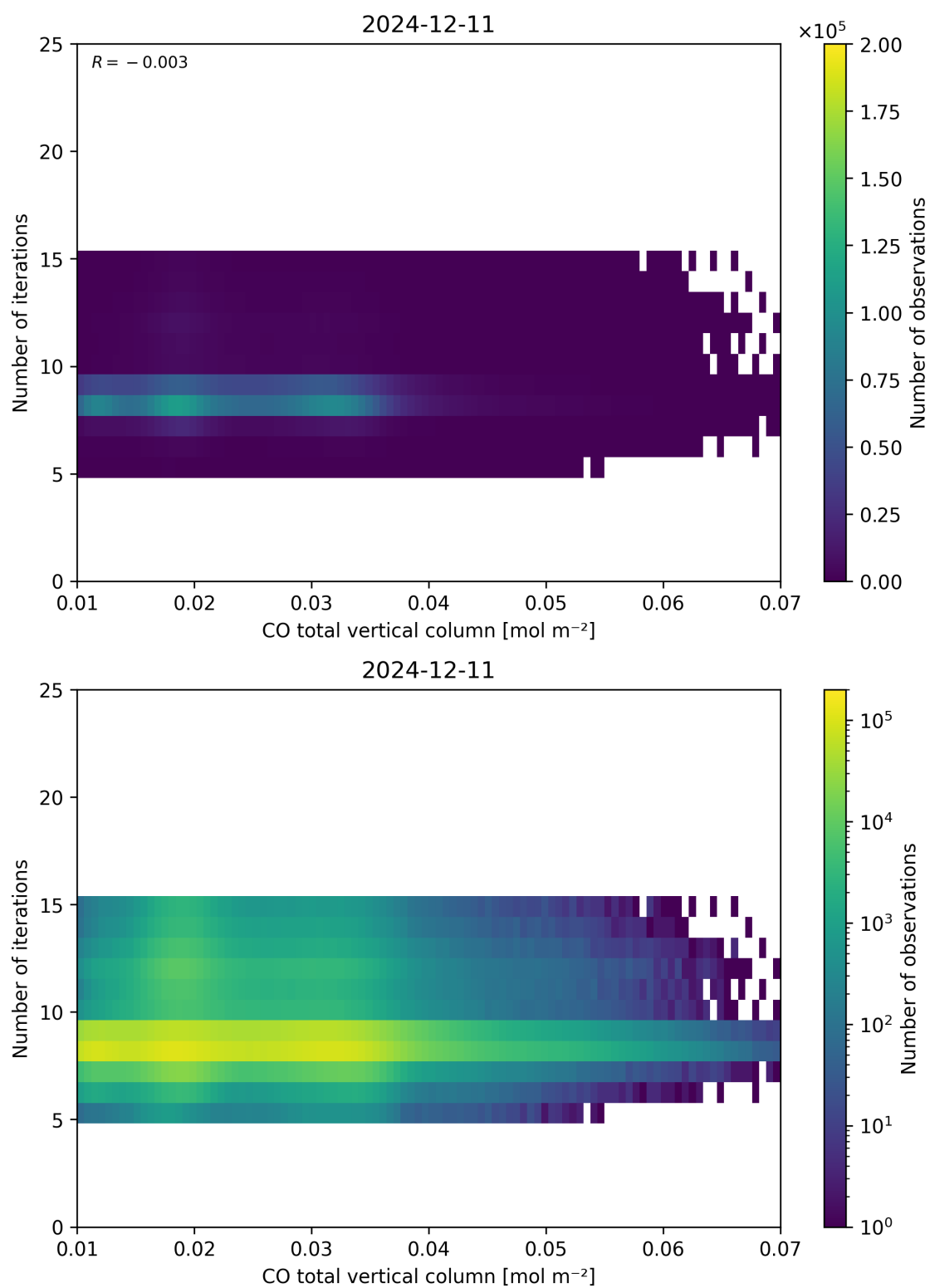
Figure 42: Scatter density plot of “CO total vertical column” against “Number of iterations” for 2024-12-11 to 2024-12-12.
