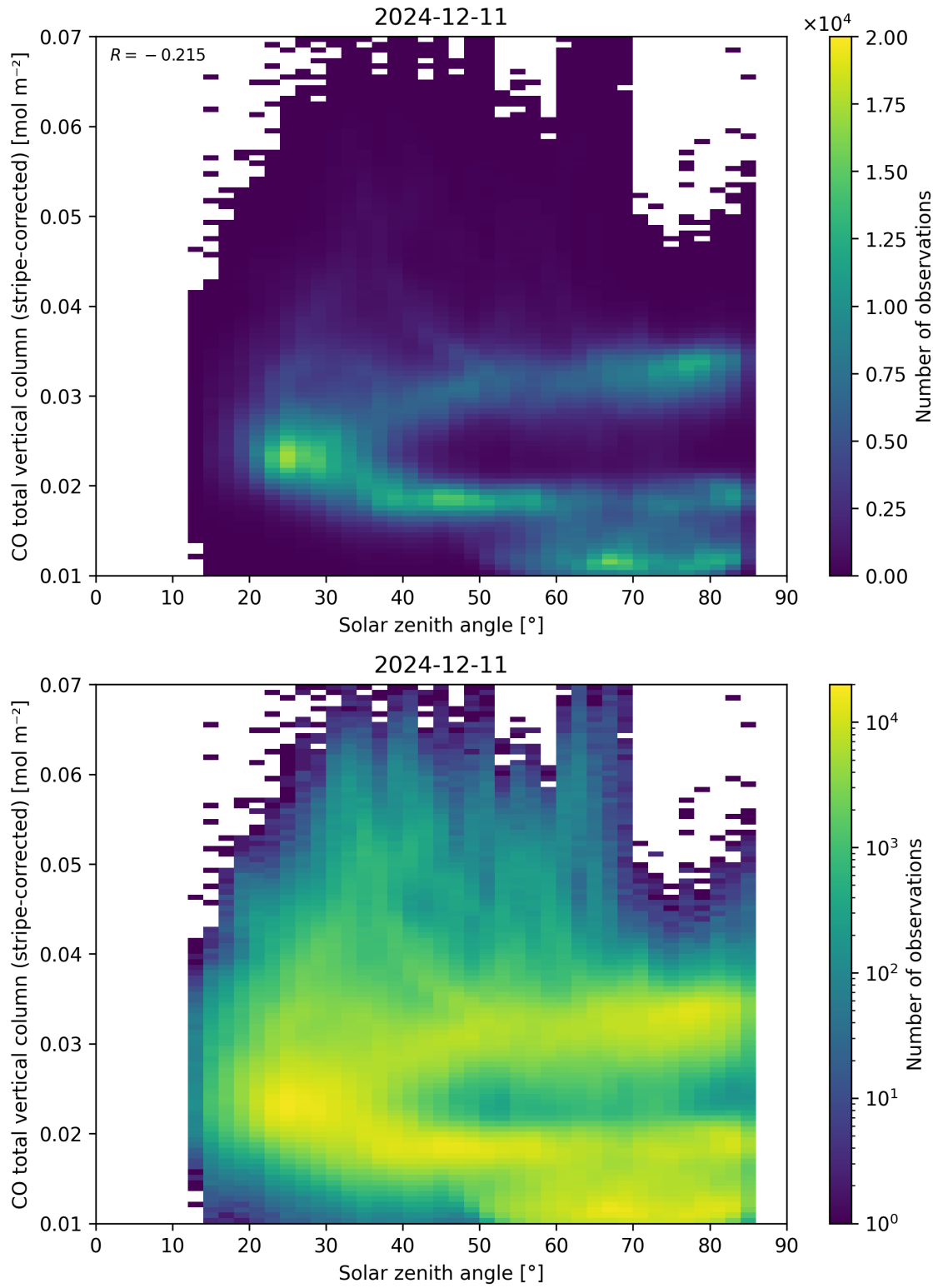
Figure 62: Scatter density plot of “Solar zenith angle” against “CO total vertical column (stripe-corrected)” for 2024-12-11 to 2024-12-12.
