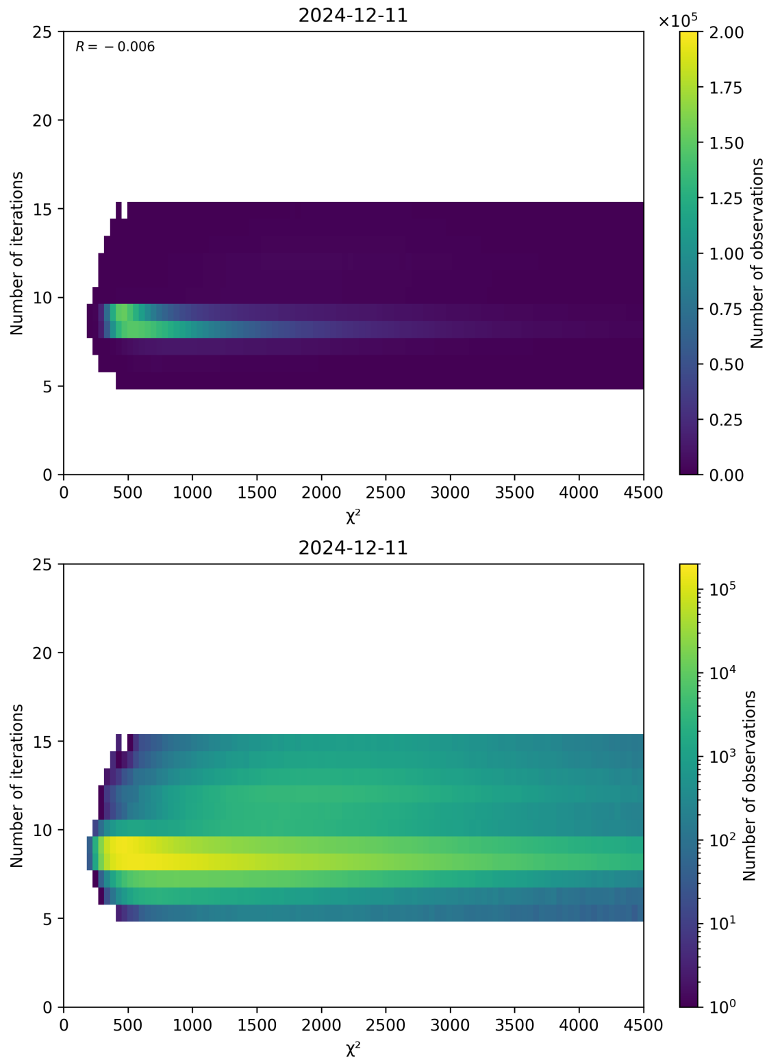
Figure 49: Scatter density plot of “ \chi^2 ” against “Number of iterations” for 2024-12-11 to 2024-12-12.
