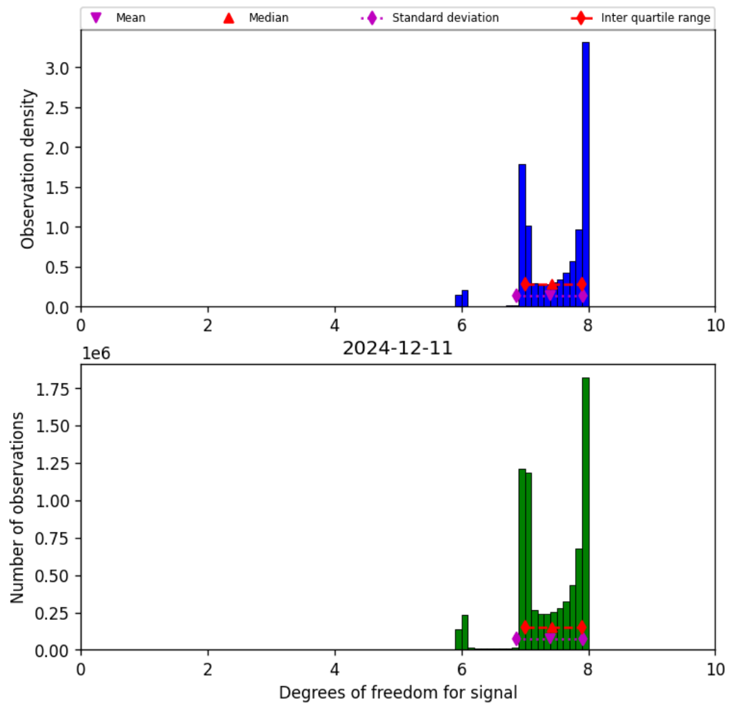
Figure 23: Histogram of “Degrees of freedom for signal” for 2024-12-11 to 2024-12-12
