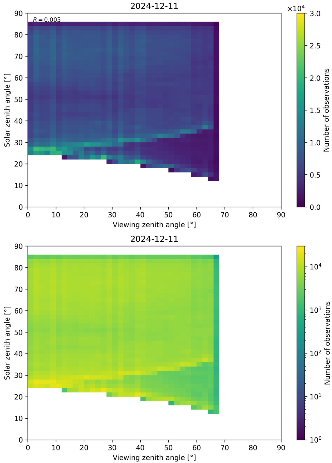
Figure 77: Scatter density plot of “Viewing zenith angle” against “Solar zenith angle” for 2024-12-11 to 2024-12-12.
