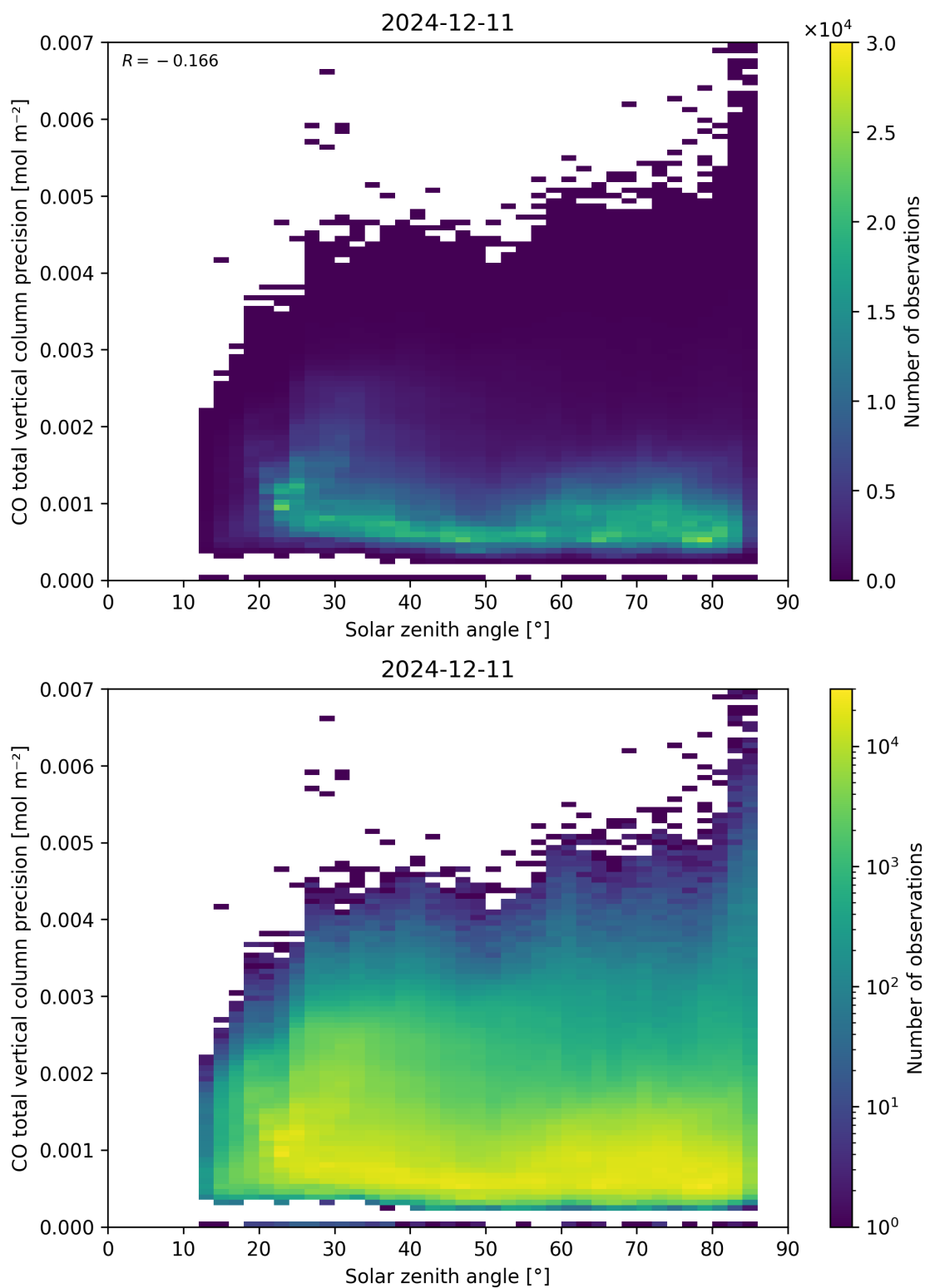
Figure 63: Scatter density plot of “Solar zenith angle” against “CO total vertical column precision” for 2024-12-11 to 2024-12-12.
