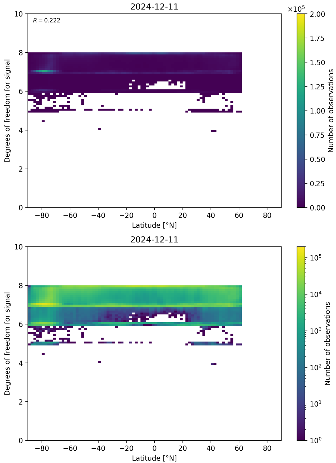
Figure 55: Scatter density plot of “Latitude” against “Degrees of freedom for signal” for 2024-12-11 to 2024-12-12.
