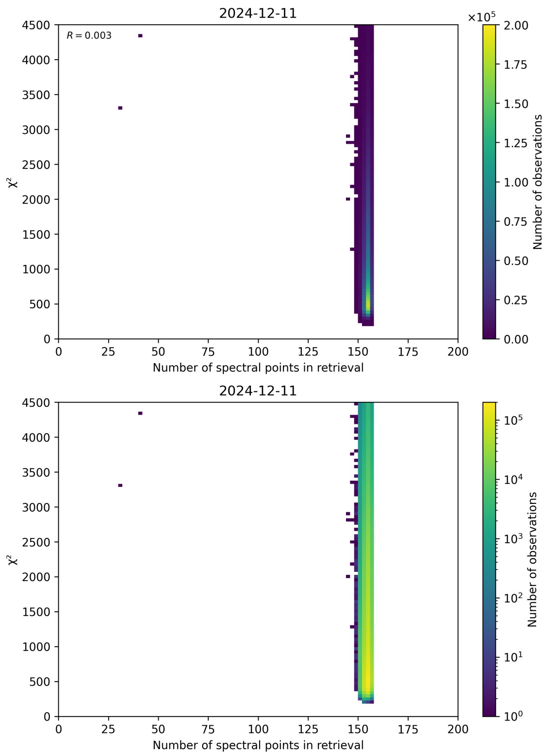
Figure 58: Scatter density plot of “Number of spectral points in retrieval” against “ \chi^2 ” for 2024-12-11 to 2024-12-12.
