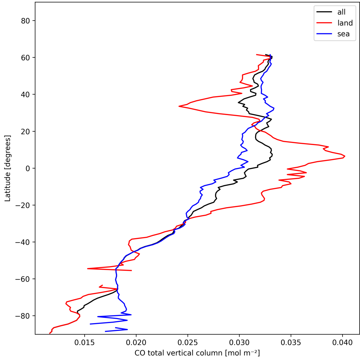
Figure 10: Zonal average of “CO total vertical column” for 2024-12-11 to 2024-12-12.
