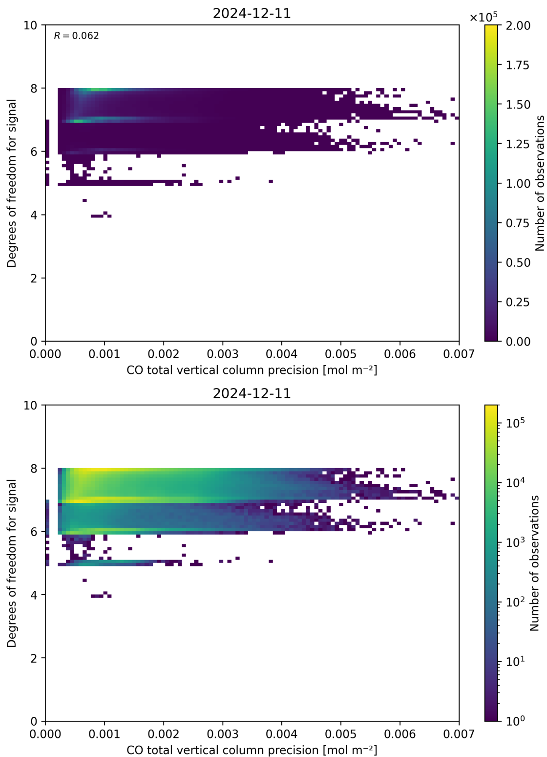
Figure 45: Scatter density plot of “CO total vertical column precision” against “Degrees of freedom for signal” for 2024-12-11 to 2024-12-12.
