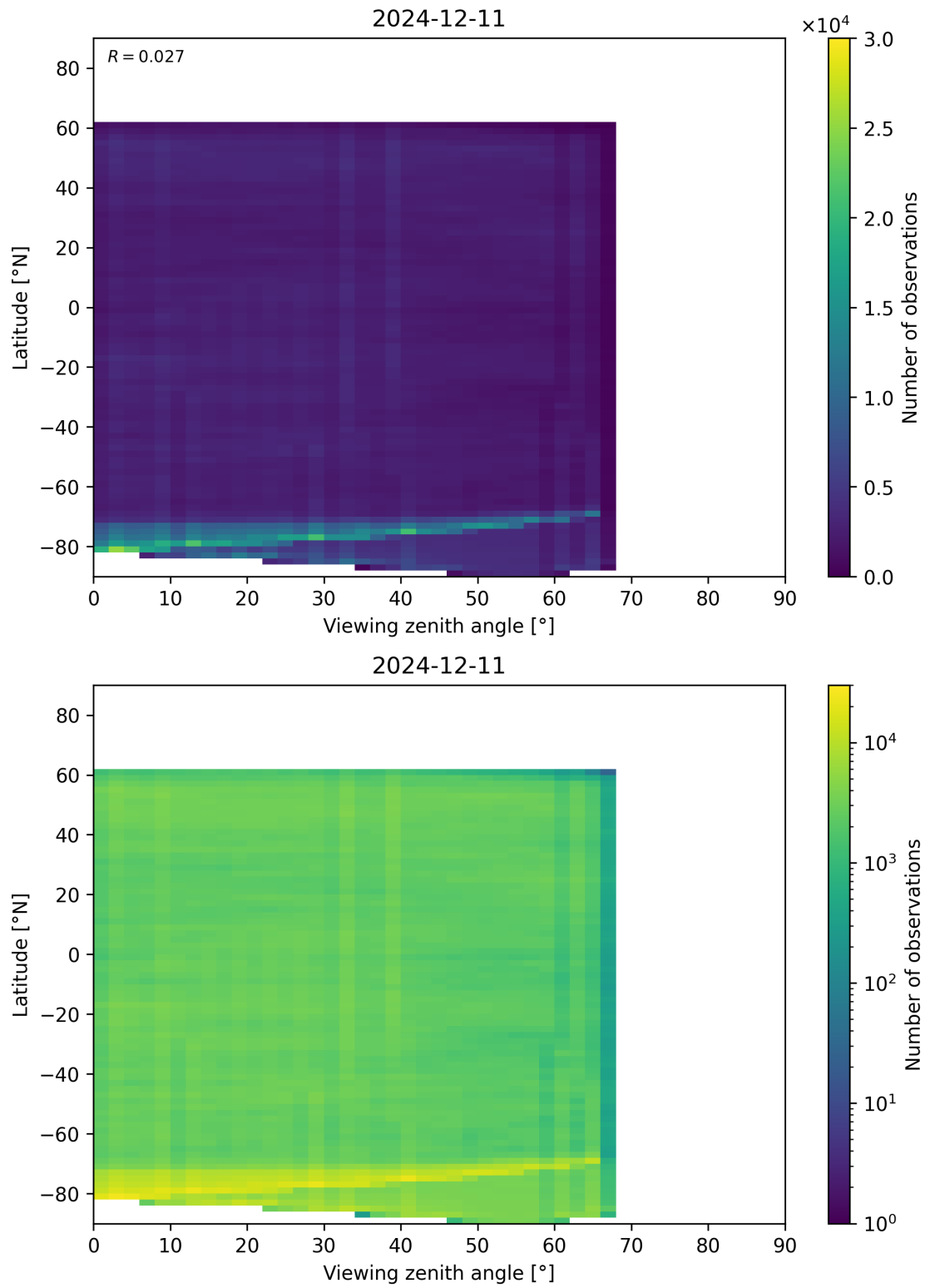
Figure 74: Scatter density plot of “Viewing zenith angle” against “Latitude” for 2024-12-11 to 2024-12-12.
