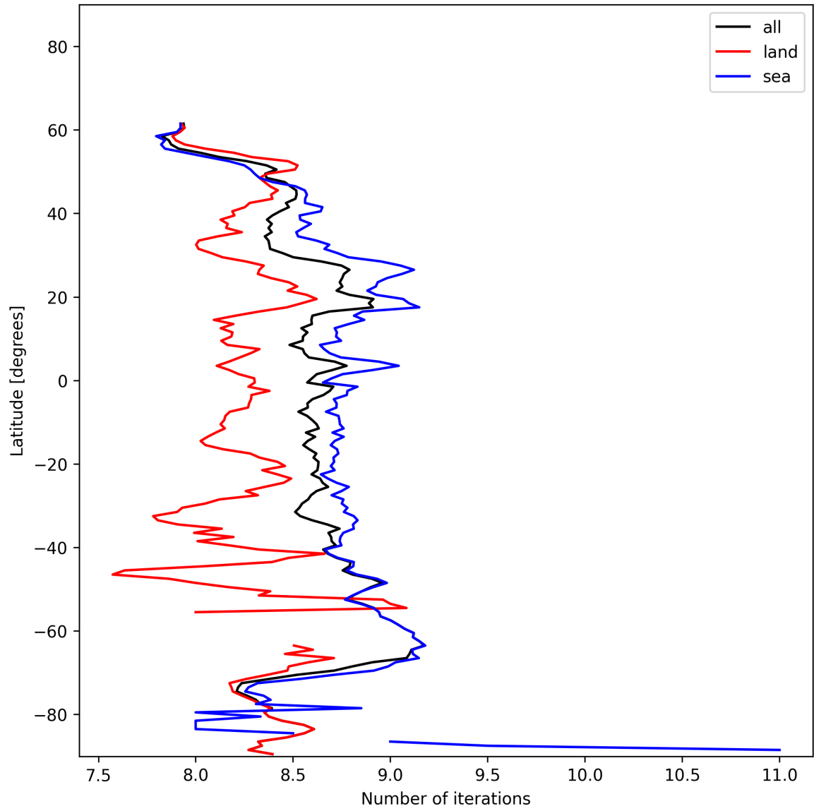
Figure 16: Zonal average of “Number of iterations” for 2024-12-11 to 2024-12-12.
