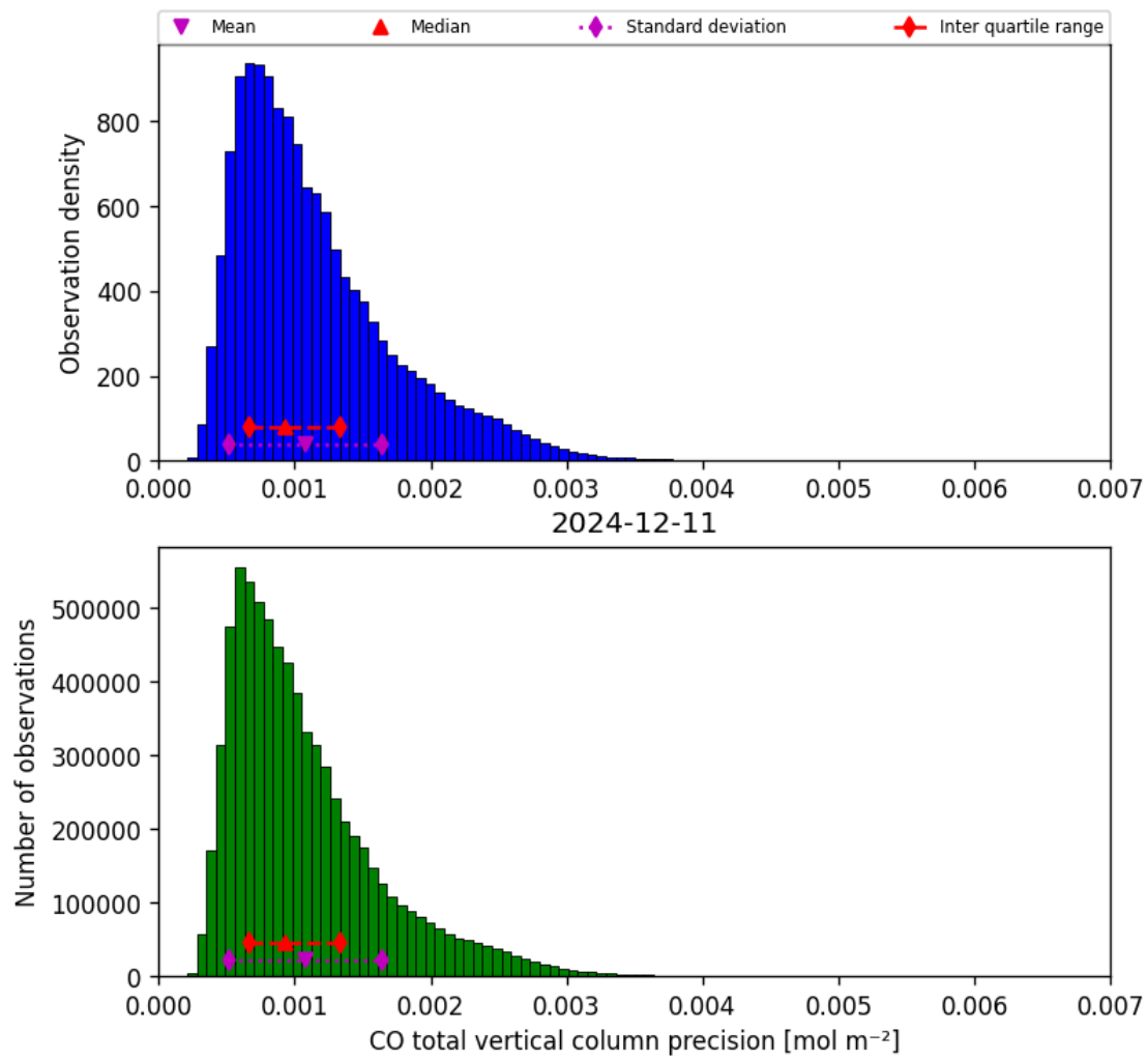
Figure 20: Histogram of “CO total vertical column precision” for 2024-12-11 to 2024-12-12
