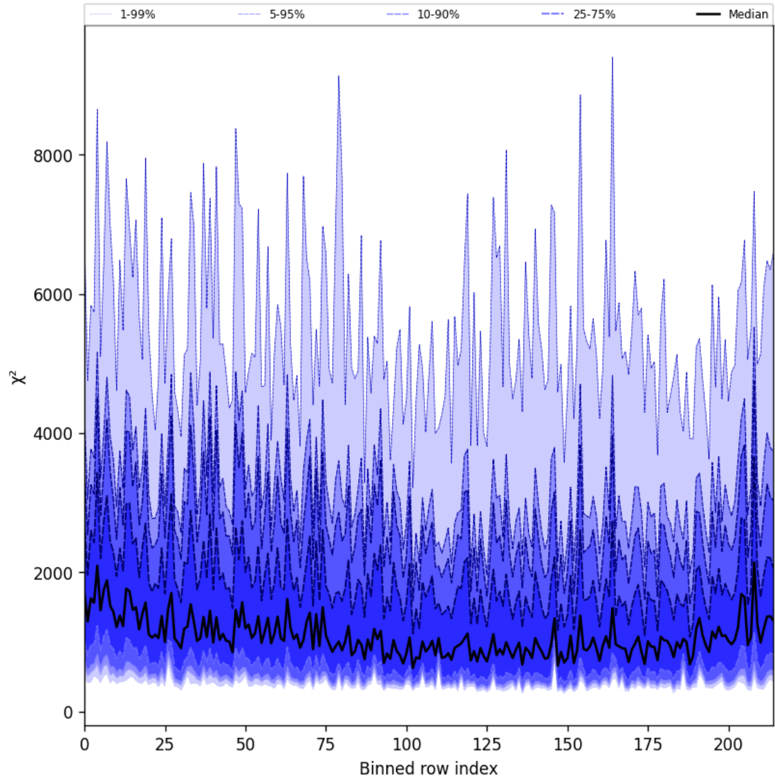
Figure 30: Along track statistics of “ \chi^2 ” for 2024-12-11 to 2024-12-12
