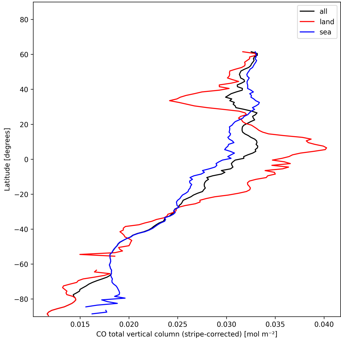
Figure 11: Zonal average of “CO total vertical column (stripe-corrected)” for 2024-12-11 to 2024-12-12.
