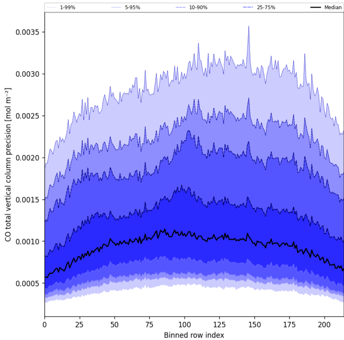
Figure 28: Along track statistics of “CO total vertical column precision” for 2024-12-11 to 2024-12-12
