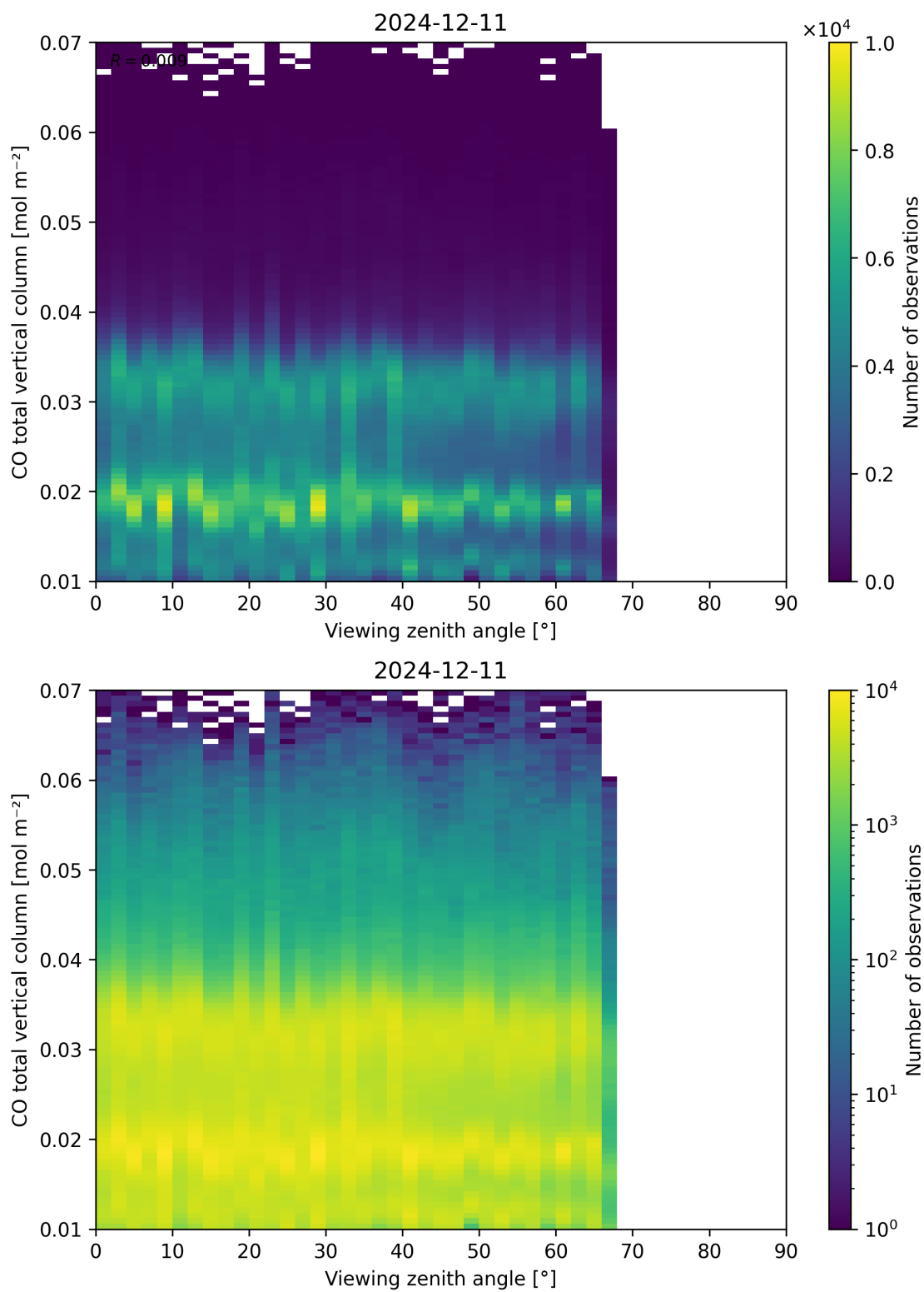
Figure 69: Scatter density plot of “Viewing zenith angle” against “CO total vertical column” for 2024-12-11 to 2024-12-12.
