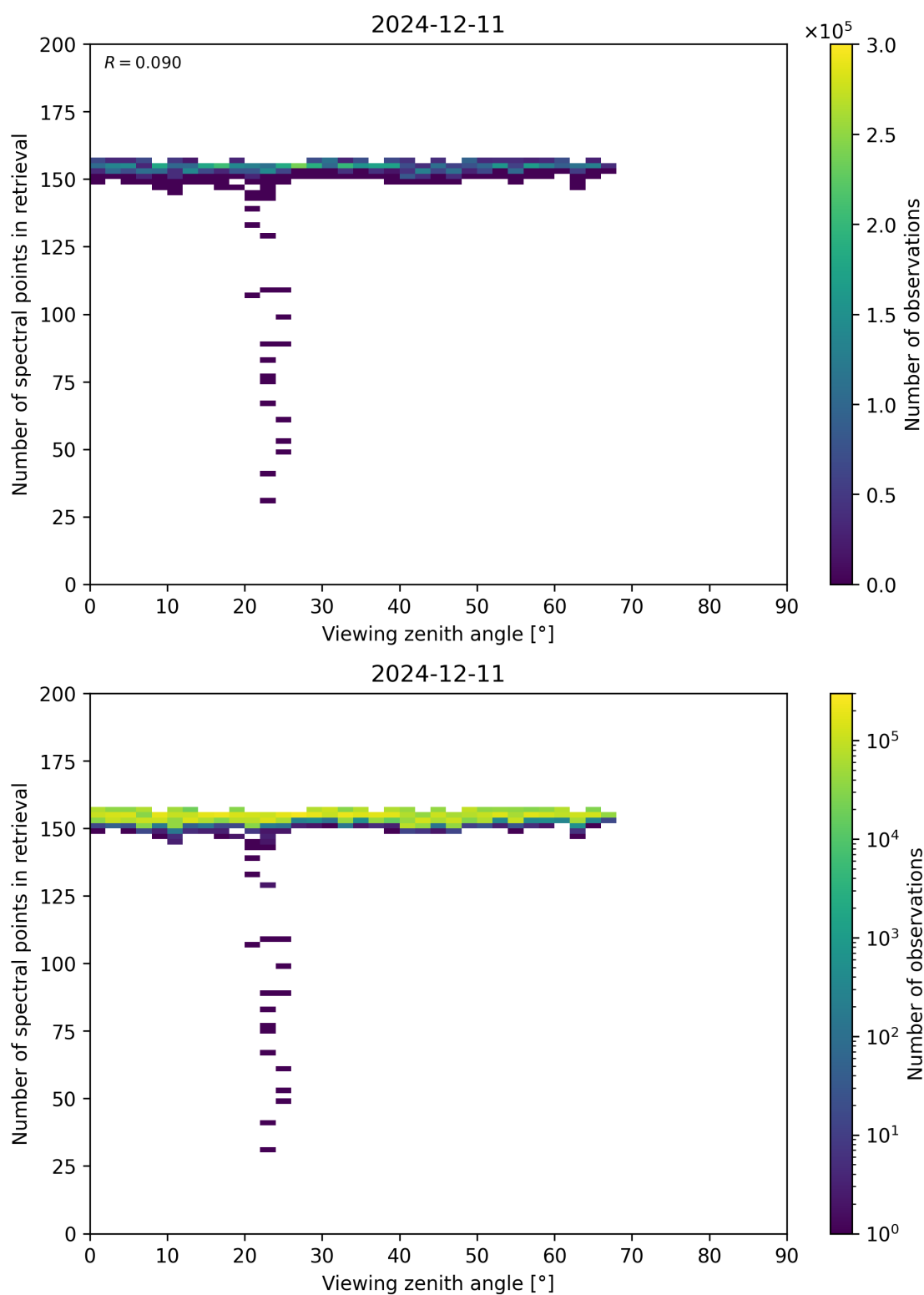
Figure 76: Scatter density plot of “Viewing zenith angle” against “Number of spectral points in retrieval” for 2024-12-11 to 2024-12-12.
