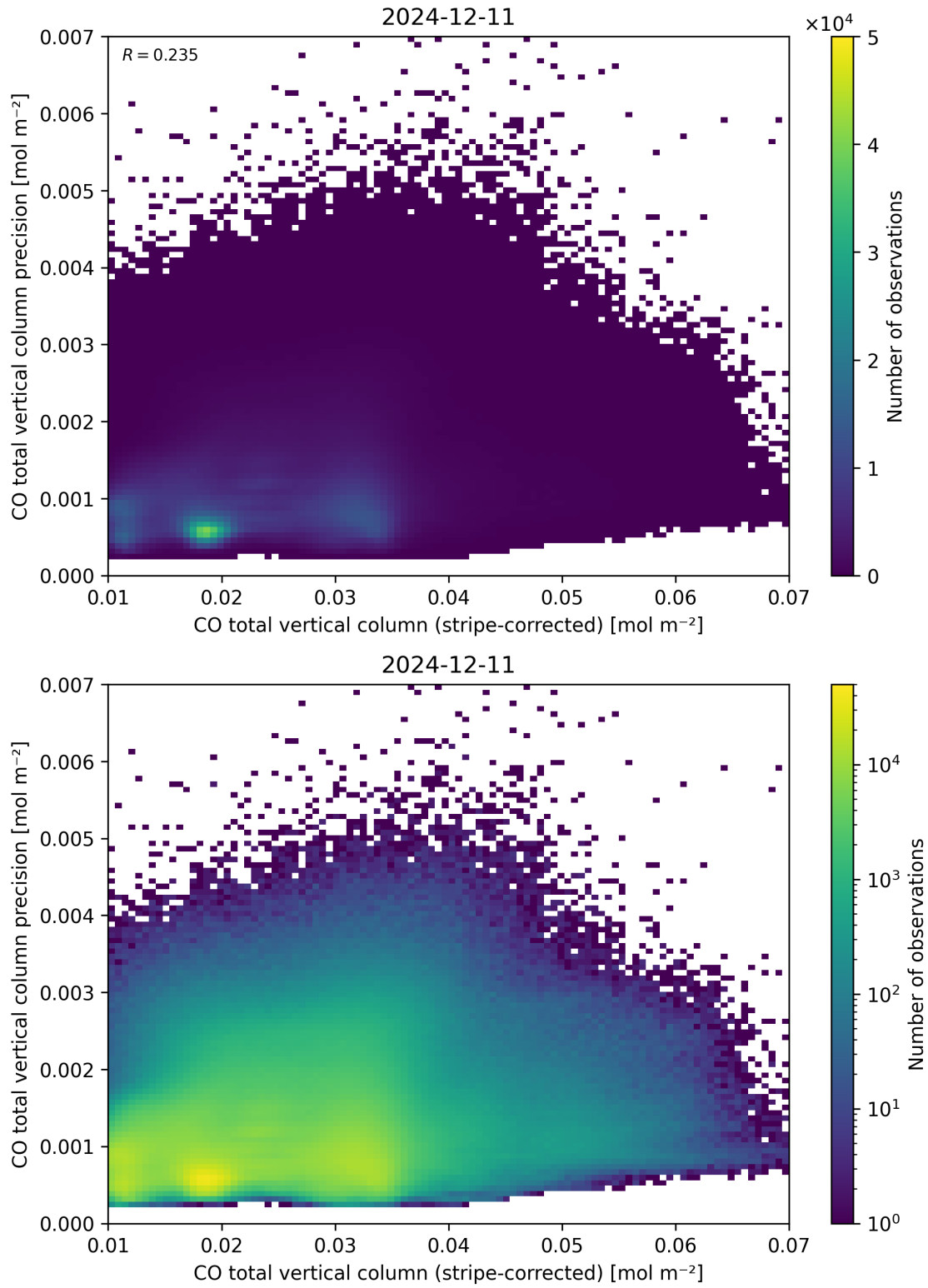
Figure 36: Scatter density plot of “CO total vertical column (stripe-corrected)” against “CO total vertical column precision” for 2024-12-11 to 2024-12-12.
