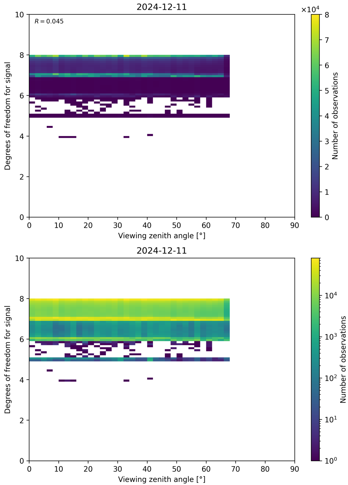
Figure 73: Scatter density plot of “Viewing zenith angle” against “Degrees of freedom for signal” for 2024-12-11 to 2024-12-12.
