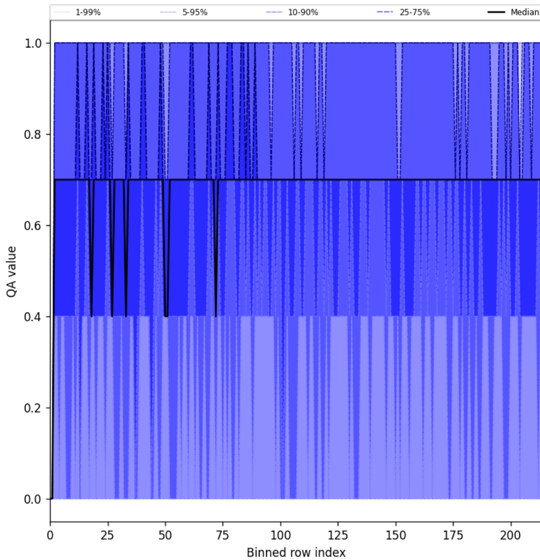
Figure 25: Along track statistics of “QA value” for 2024-12-11 to 2024-12-12
