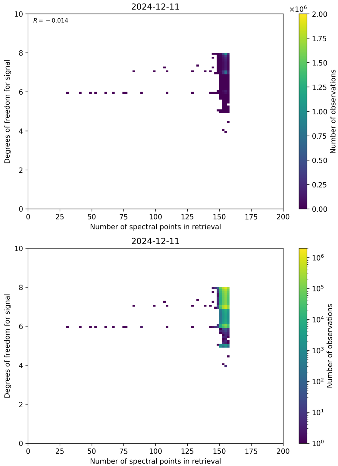
Figure 59: Scatter density plot of “Number of spectral points in retrieval” against “Degrees of freedom for signal” for 2024-12-11 to 2024-12-12.
