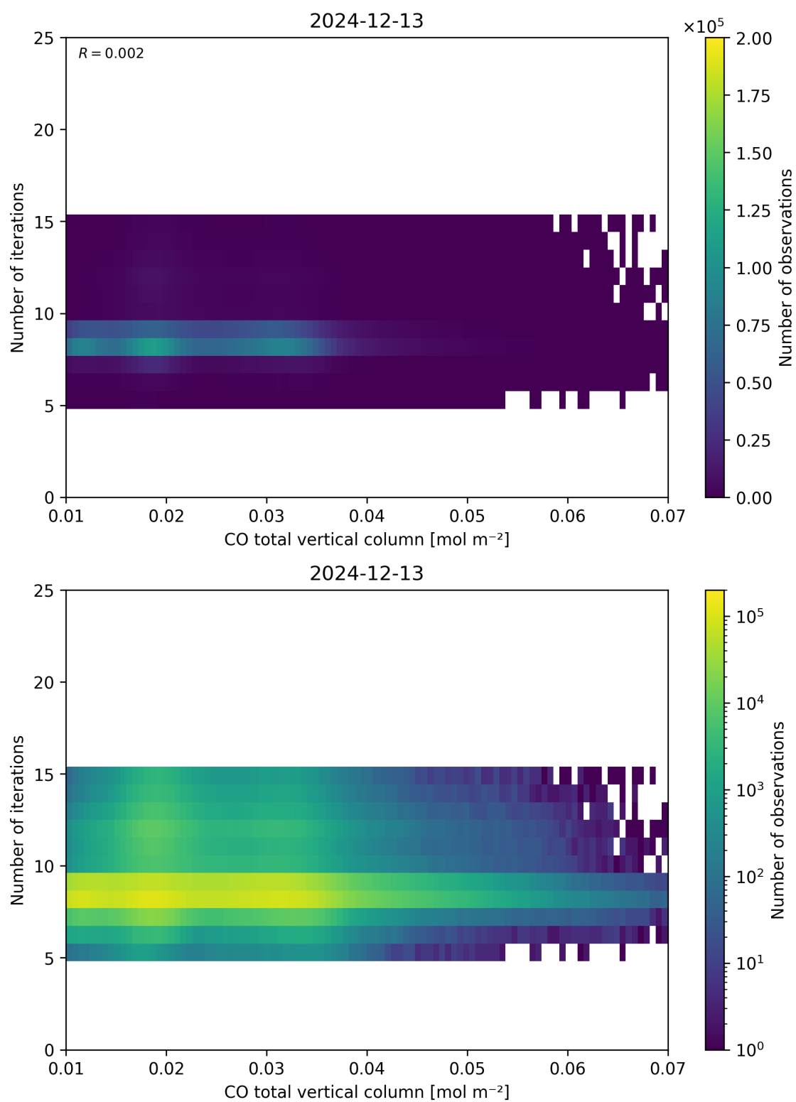
Figure 42: Scatter density plot of “CO total vertical column” against “Number of iterations” for 2024-12-12 to 2024-12-14.
