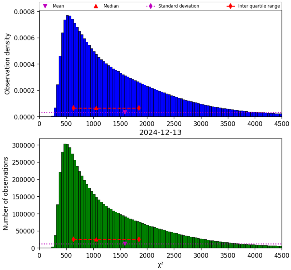
Figure 22: Histogram of “ \chi^2 ” for 2024-12-12 to 2024-12-14
