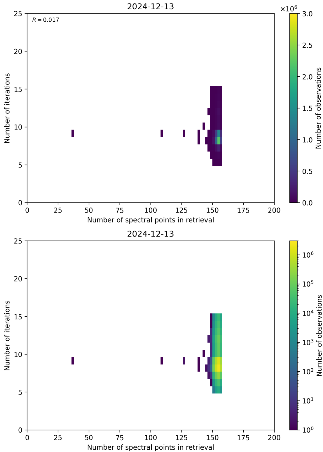
Figure 60: Scatter density plot of “Number of spectral points in retrieval” against “Number of iterations” for 2024-12-12 to 2024-12-14.
