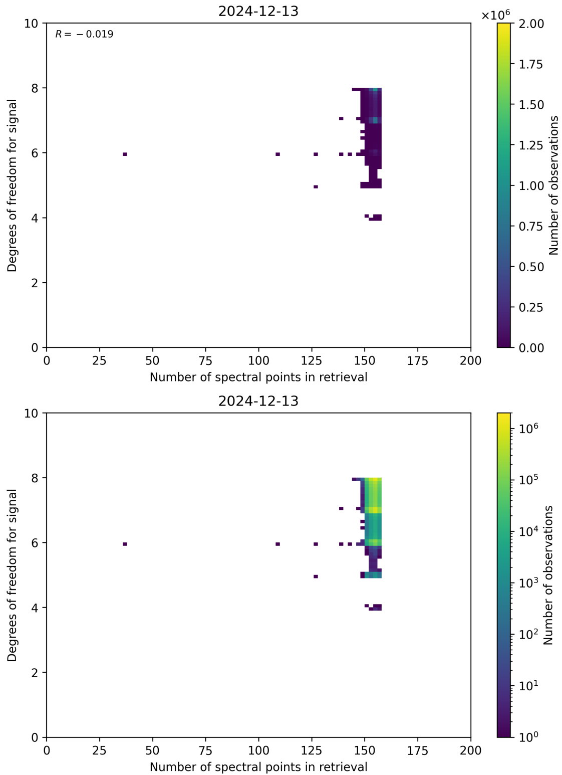
Figure 59: Scatter density plot of “Number of spectral points in retrieval” against “Degrees of freedom for signal” for 2024-12-12 to 2024-12-14.
