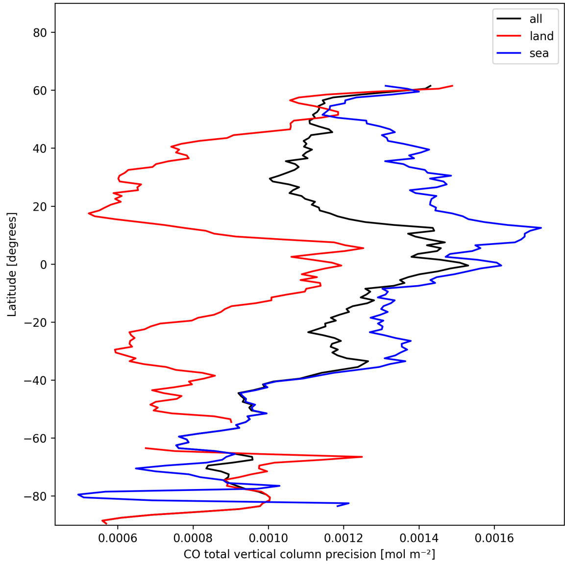
Figure 12: Zonal average of “CO total vertical column precision” for 2024-12-12 to 2024-12-14.
