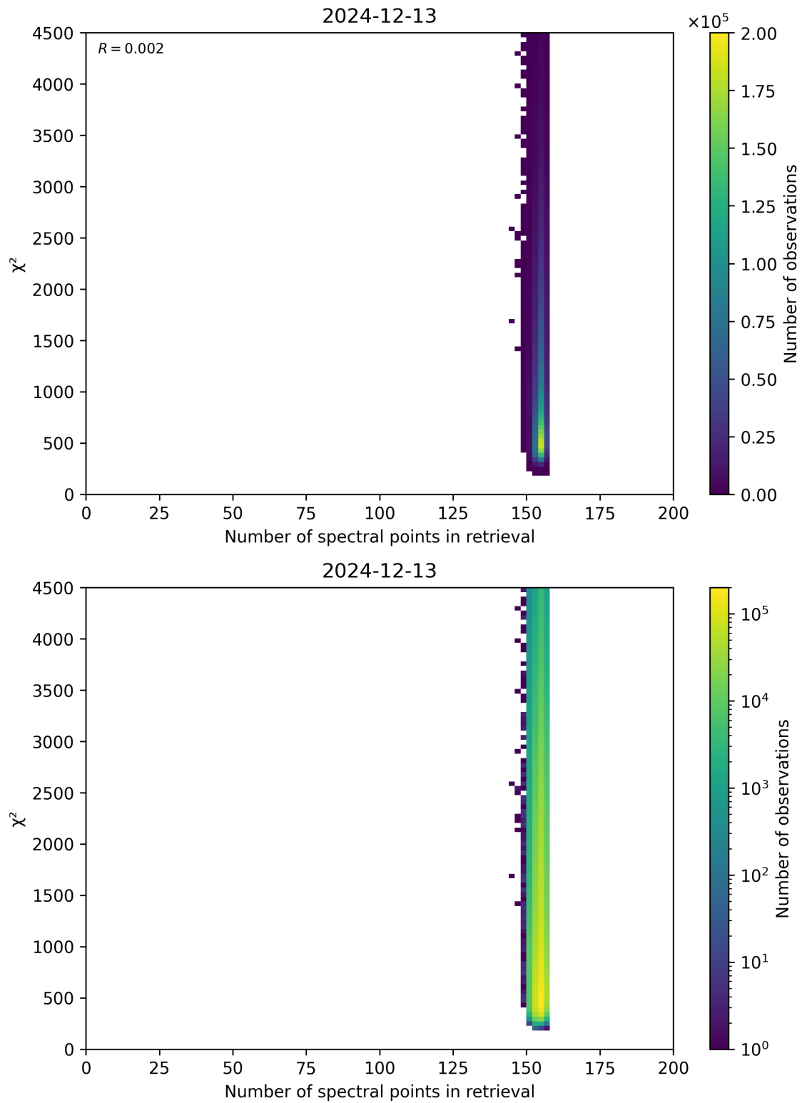
Figure 58: Scatter density plot of “Number of spectral points in retrieval” against “ \chi^2 ” for 2024-12-12 to 2024-12-14.
