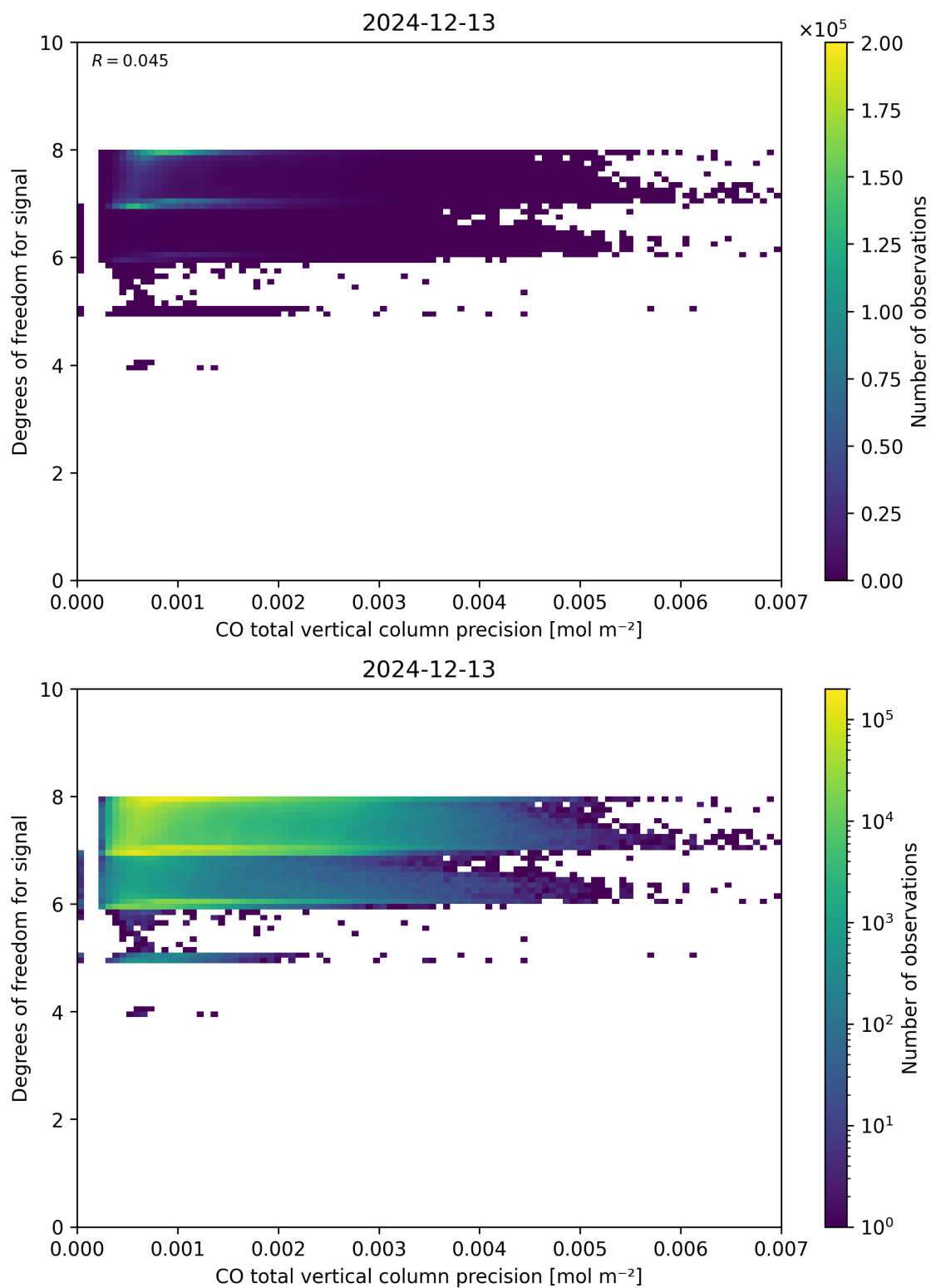
Figure 45: Scatter density plot of “CO total vertical column precision” against “Degrees of freedom for signal” for 2024-12-12 to 2024-12-14.
