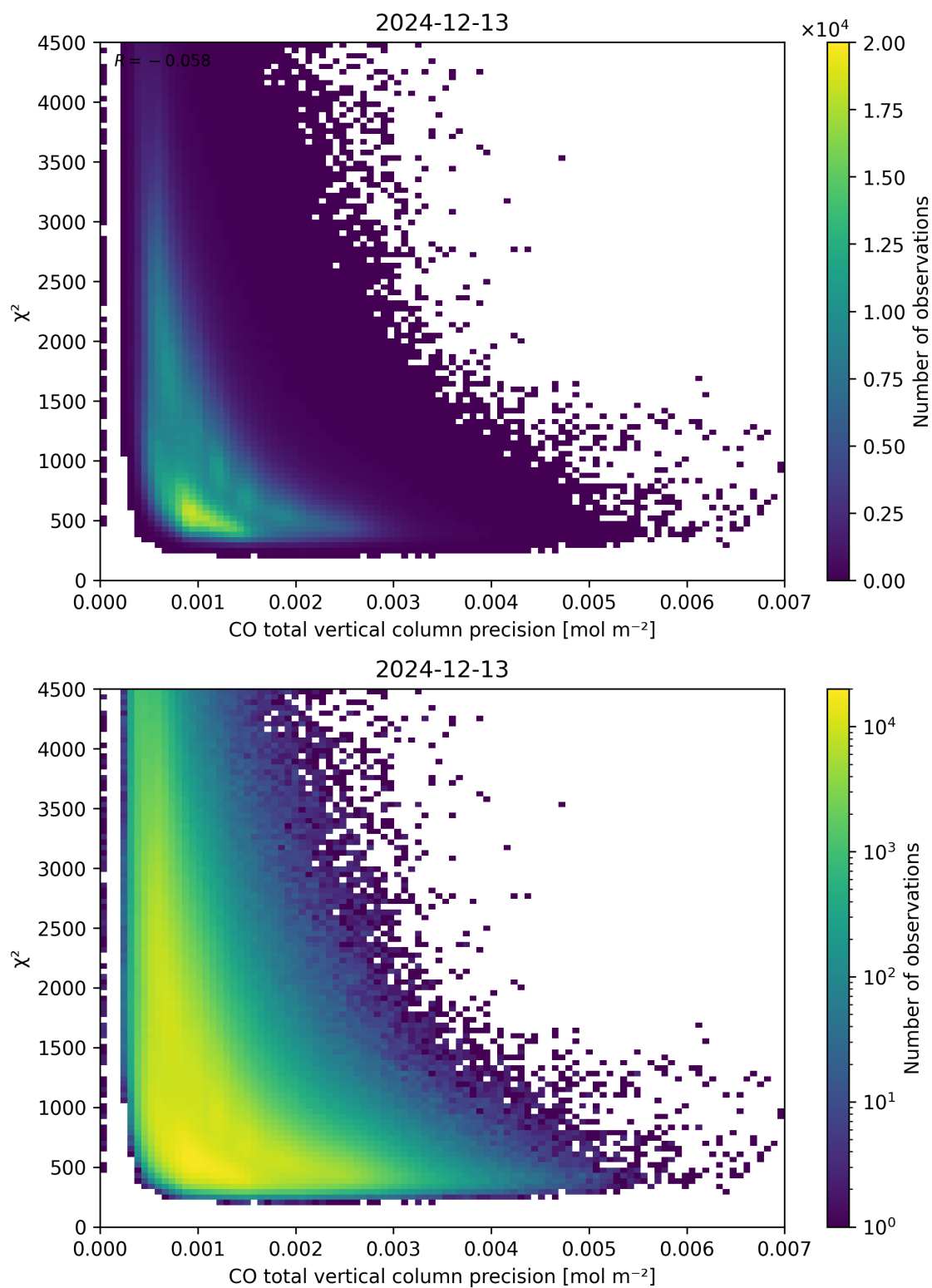
Figure 44: Scatter density plot of “CO total vertical column precision” against “ \chi^2 ” for 2024-12-12 to 2024-12-14.
