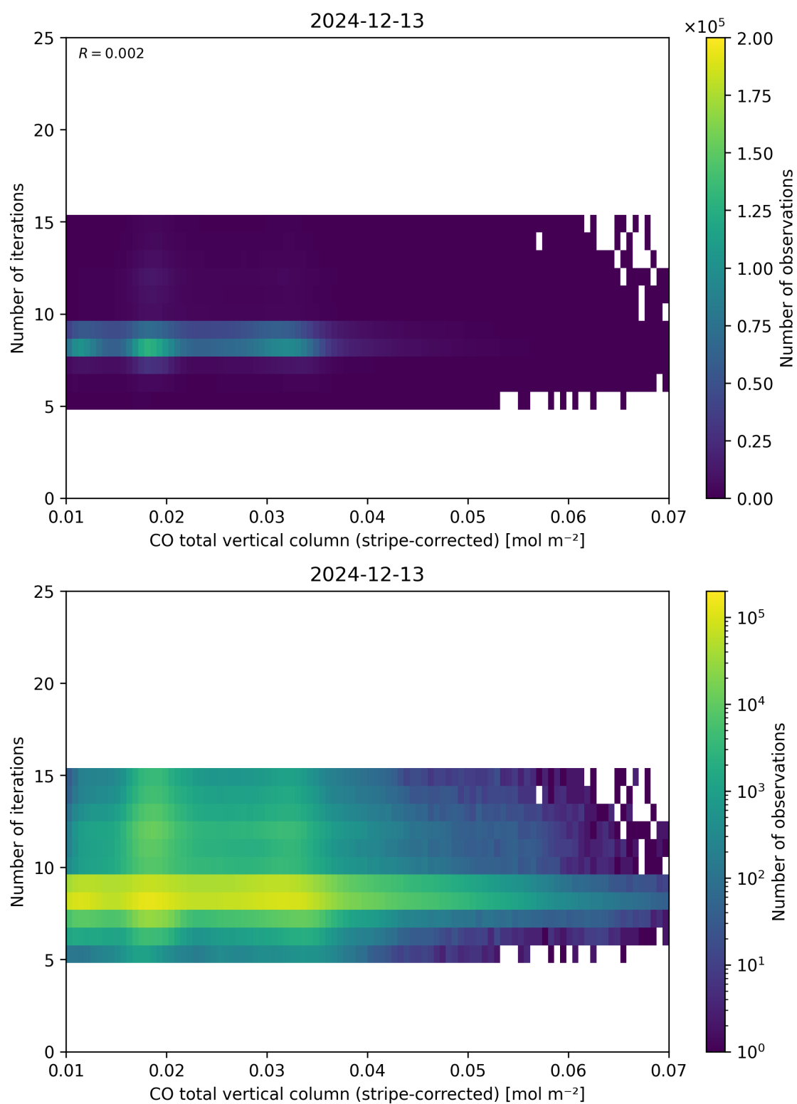
Figure 39: Scatter density plot of “CO total vertical column (stripe-corrected)” against “Number of iterations” for 2024-12-12 to 2024-12-14.
