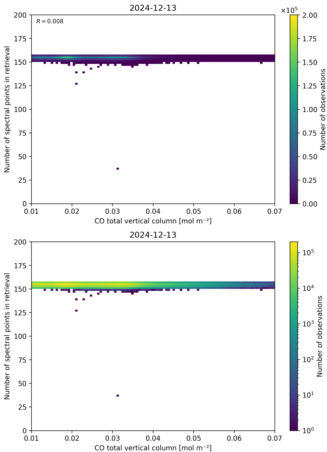
Figure 43: Scatter density plot of “CO total vertical column” against “Number of spectral points in retrieval” for 2024-12-12 to 2024-12-14.
