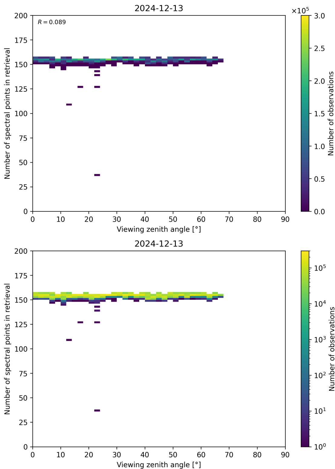
Figure 76: Scatter density plot of “Viewing zenith angle” against “Number of spectral points in retrieval” for 2024-12-12 to 2024-12-14.
