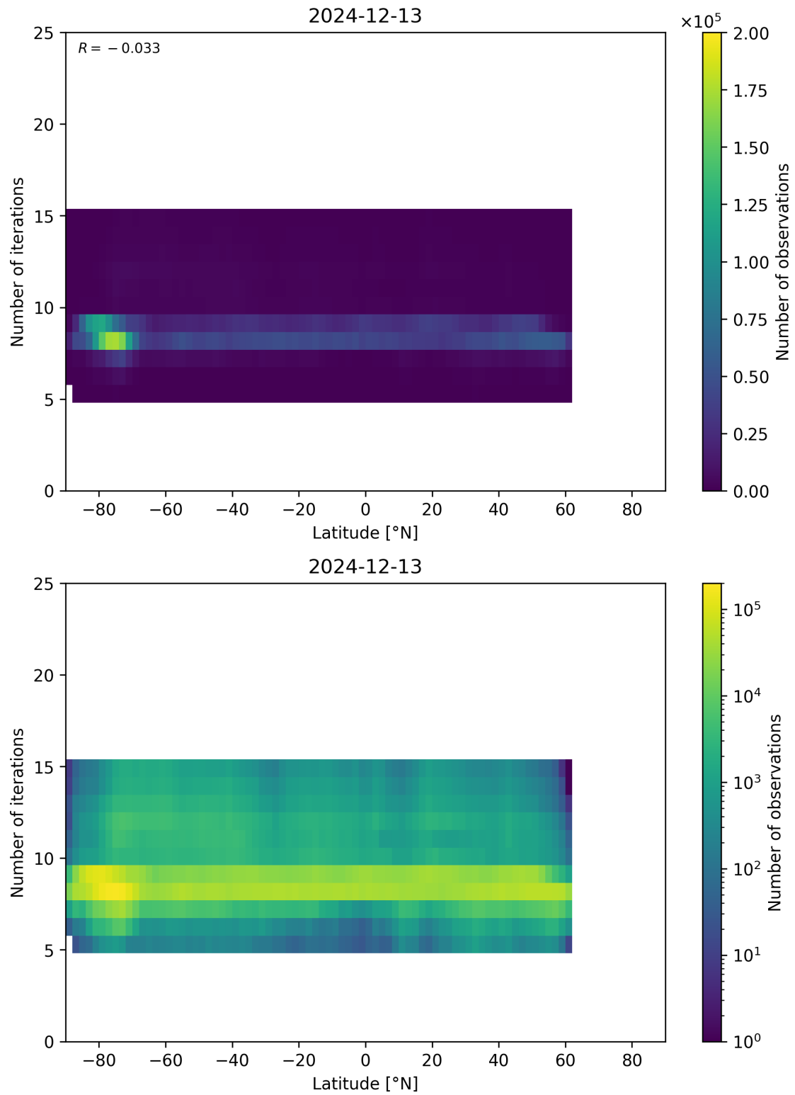
Figure 56: Scatter density plot of “Latitude” against “Number of iterations” for 2024-12-12 to 2024-12-14.
