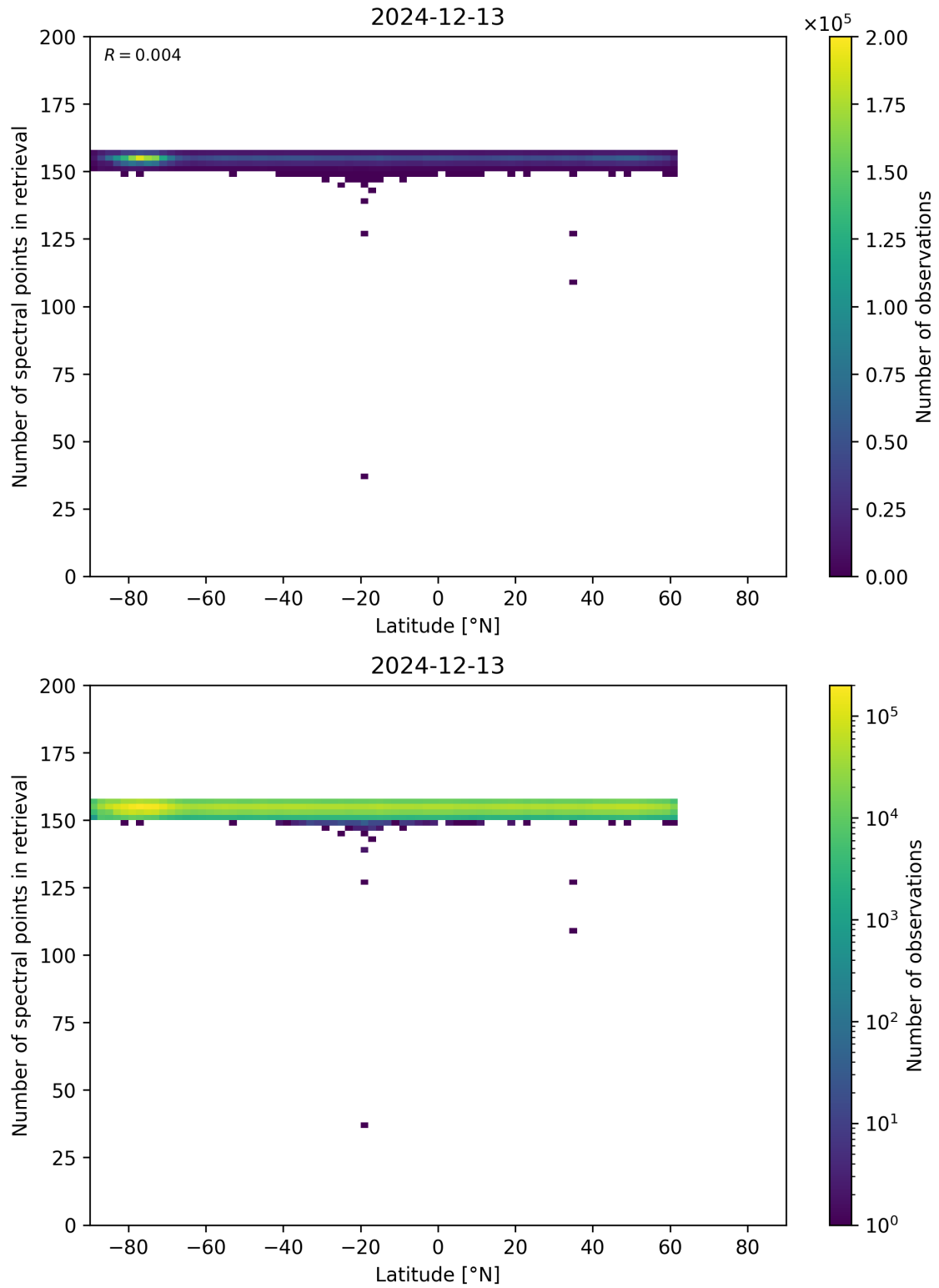
Figure 57: Scatter density plot of “Latitude” against “Number of spectral points in retrieval” for 2024-12-12 to 2024-12-14.
