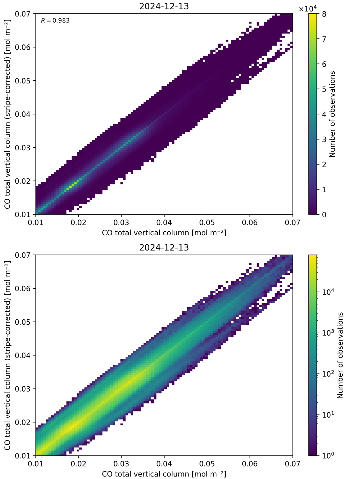
Figure 33: Scatter density plot of “CO total vertical column” against “CO total vertical column (stripe-corrected)” for 2024-12-12 to 2024-12-14.
