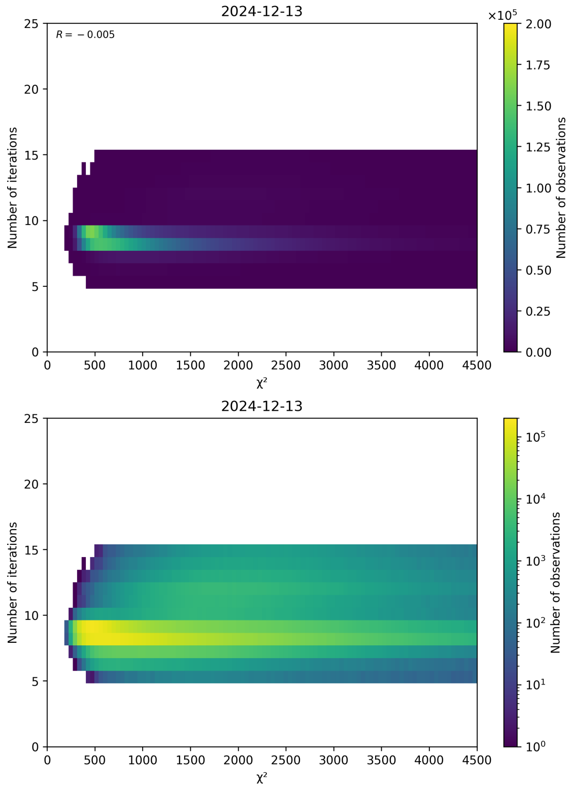
Figure 49: Scatter density plot of “ \chi^2 ” against “Number of iterations” for 2024-12-12 to 2024-12-14.
