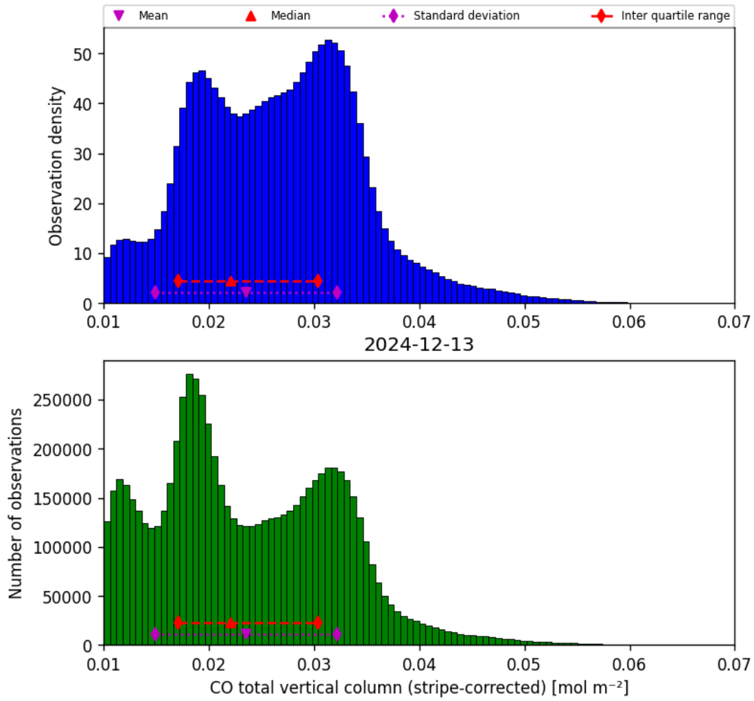
Figure 19: Histogram of “CO total vertical column (stripe-corrected)” for 2024-12-12 to 2024-12-14
