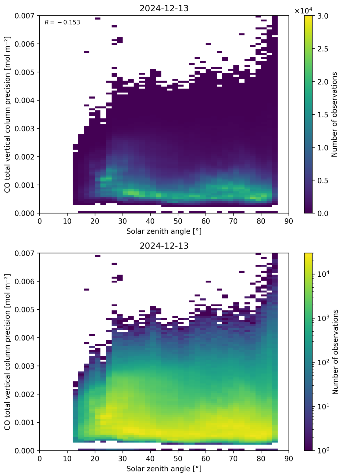
Figure 63: Scatter density plot of “Solar zenith angle” against “CO total vertical column precision” for 2024-12-12 to 2024-12-14.
