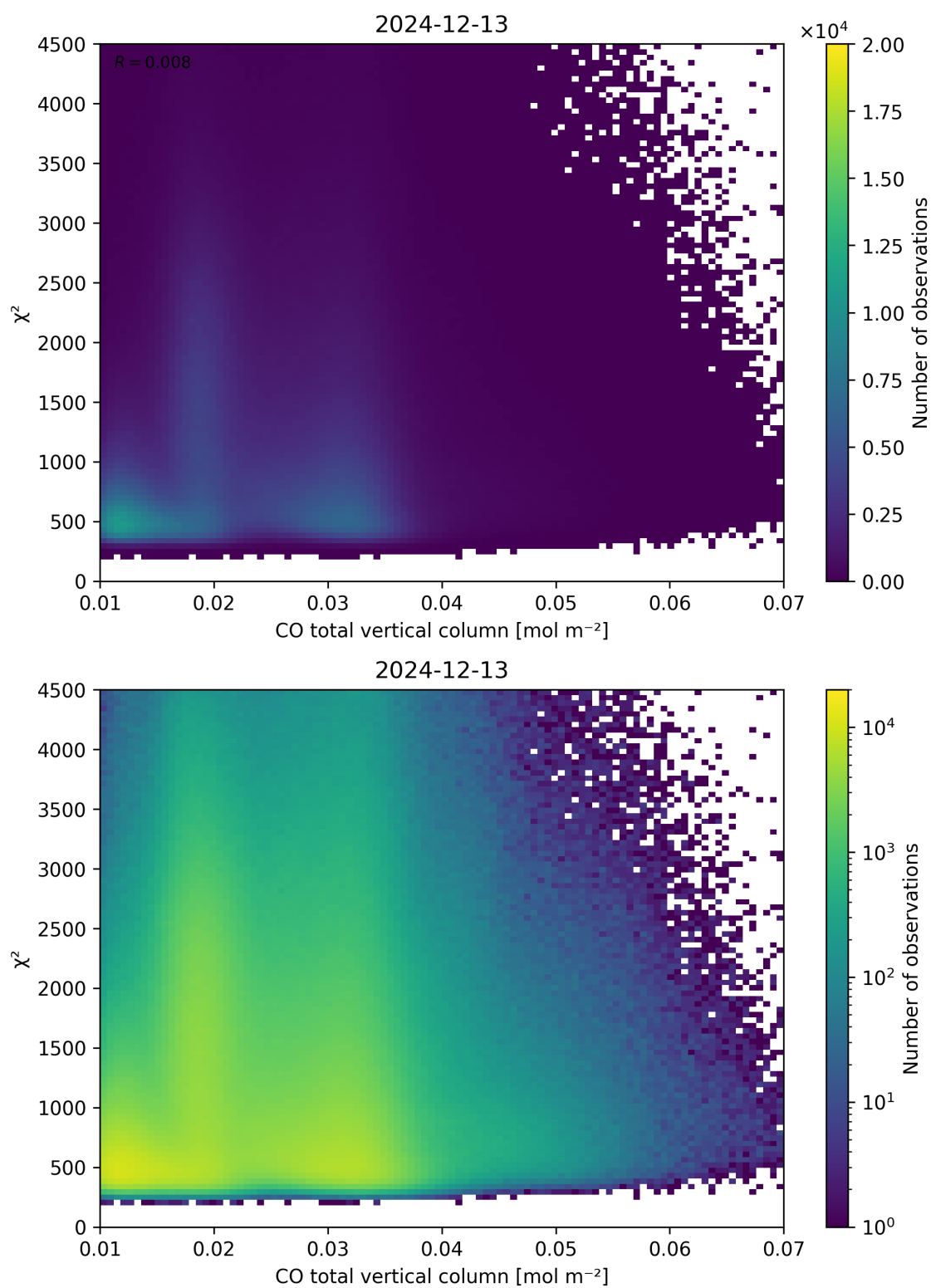
Figure 35: Scatter density plot of “CO total vertical column” against “ \chi^2 ” for 2024-12-12 to 2024-12-14.
