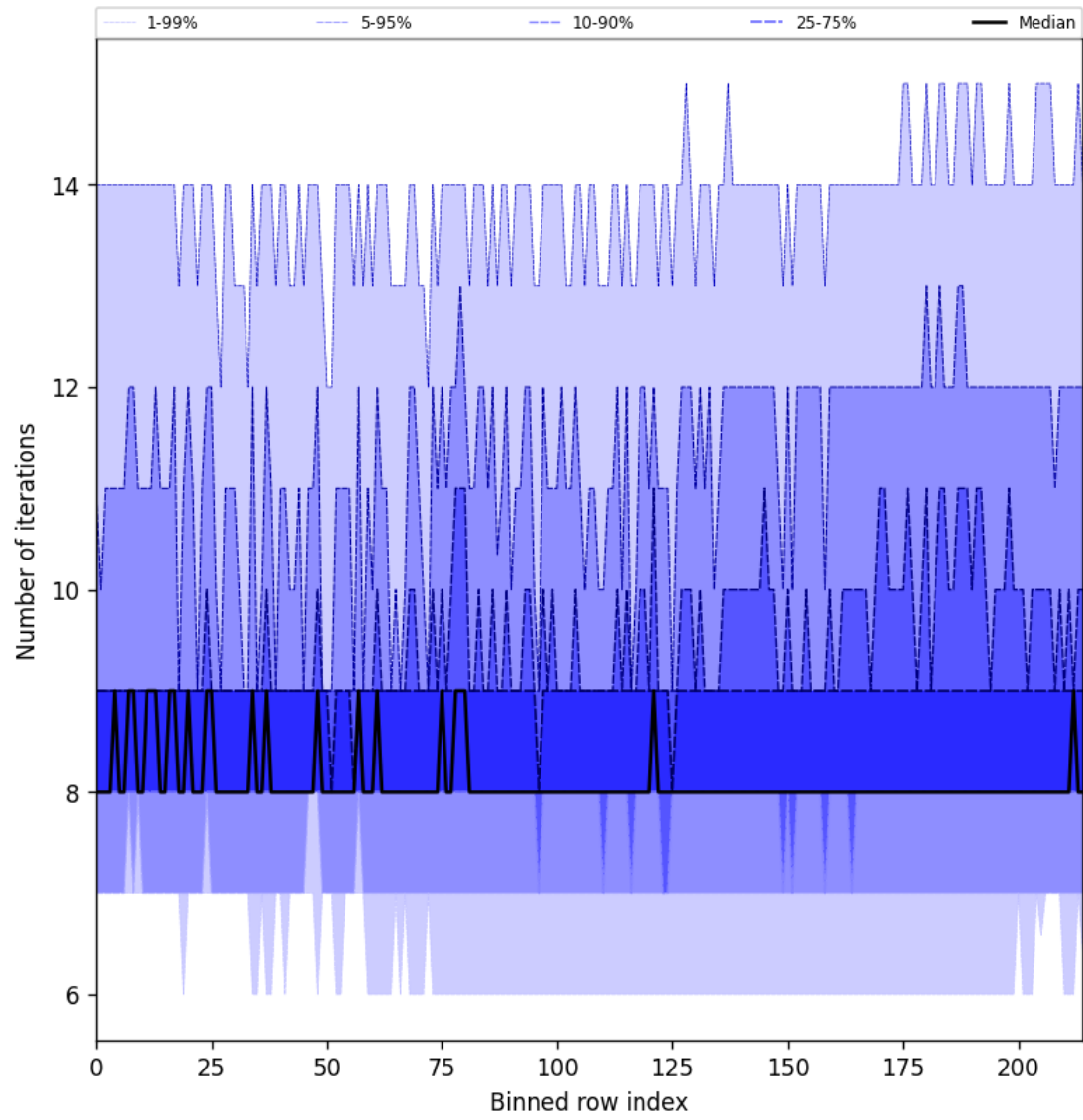
Figure 32: Along track statistics of “Number of iterations” for 2024-12-12 to 2024-12-14
