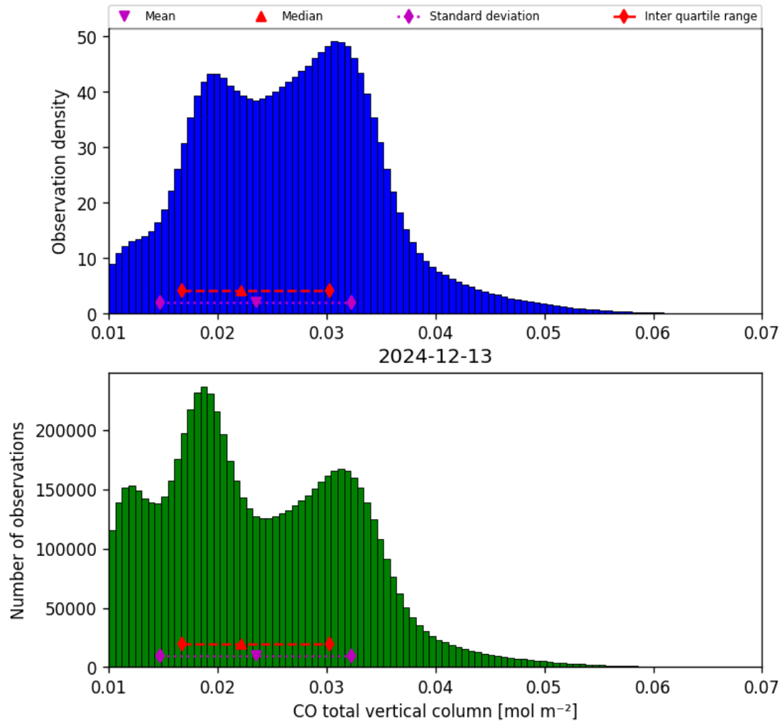
Figure 18: Histogram of “CO total vertical column” for 2024-12-12 to 2024-12-14
