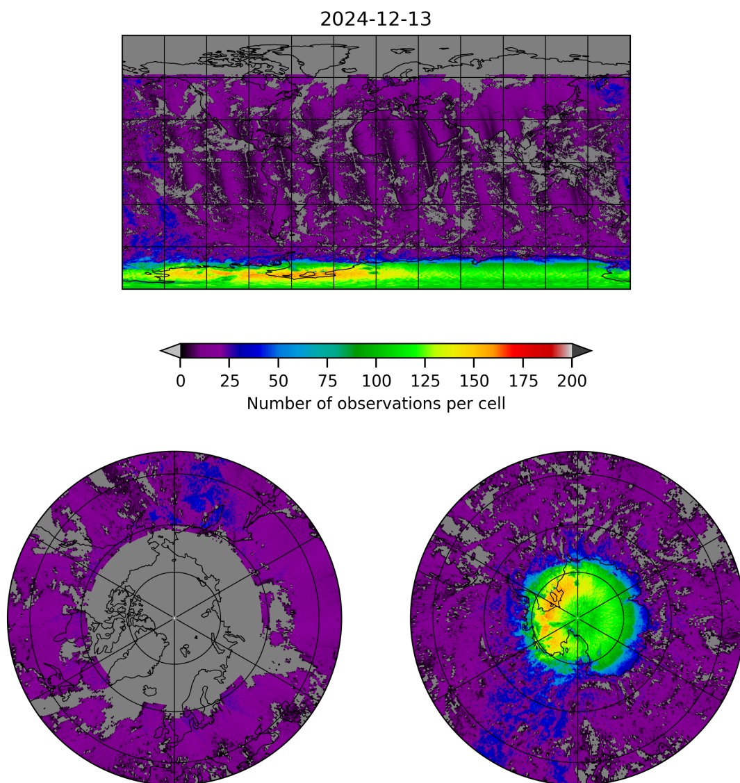
Figure 8: Map of the number of observations for 2024-12-12 to 2024-12-14
