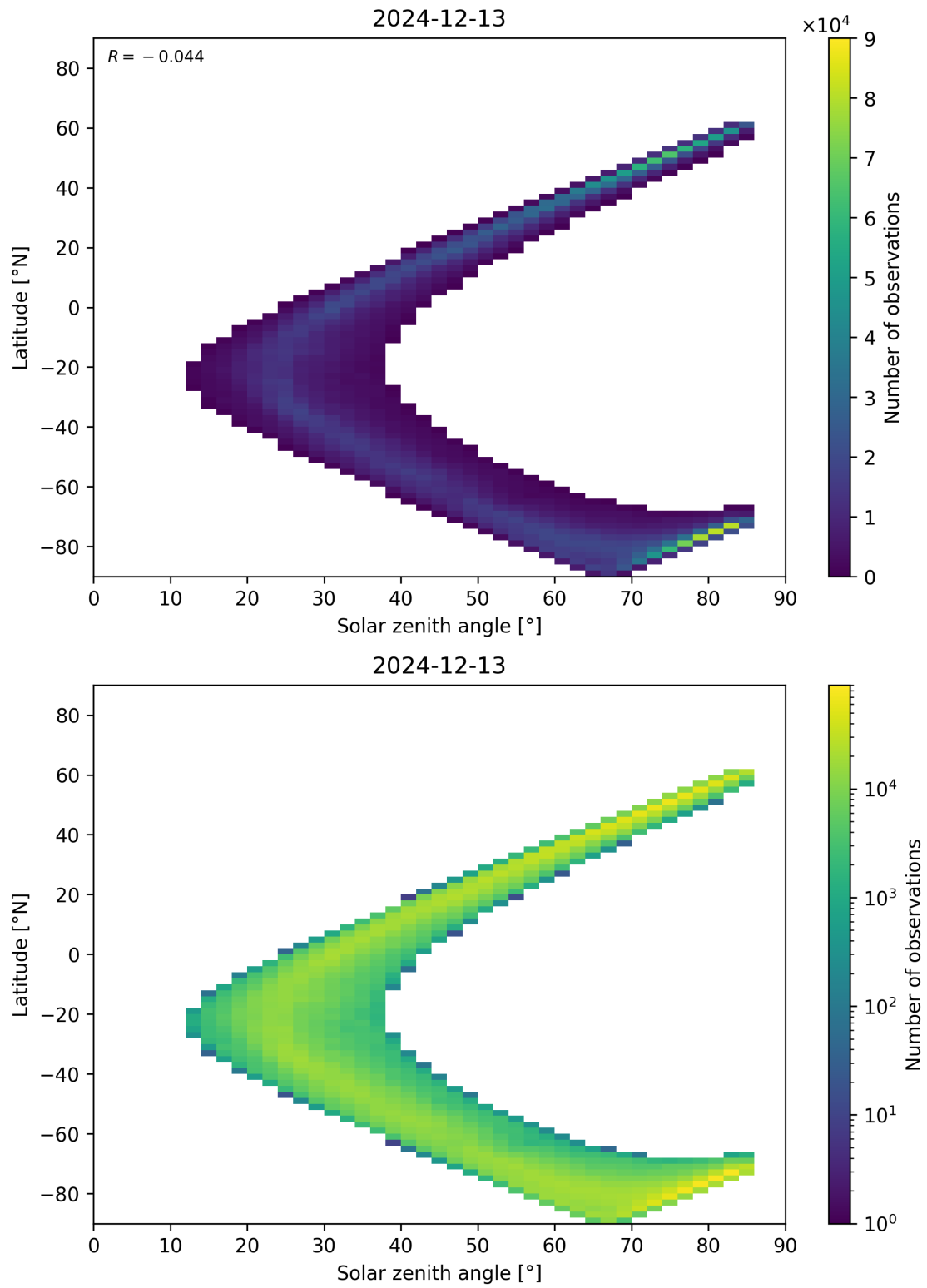
Figure 66: Scatter density plot of “Solar zenith angle” against “Latitude” for 2024-12-12 to 2024-12-14.
