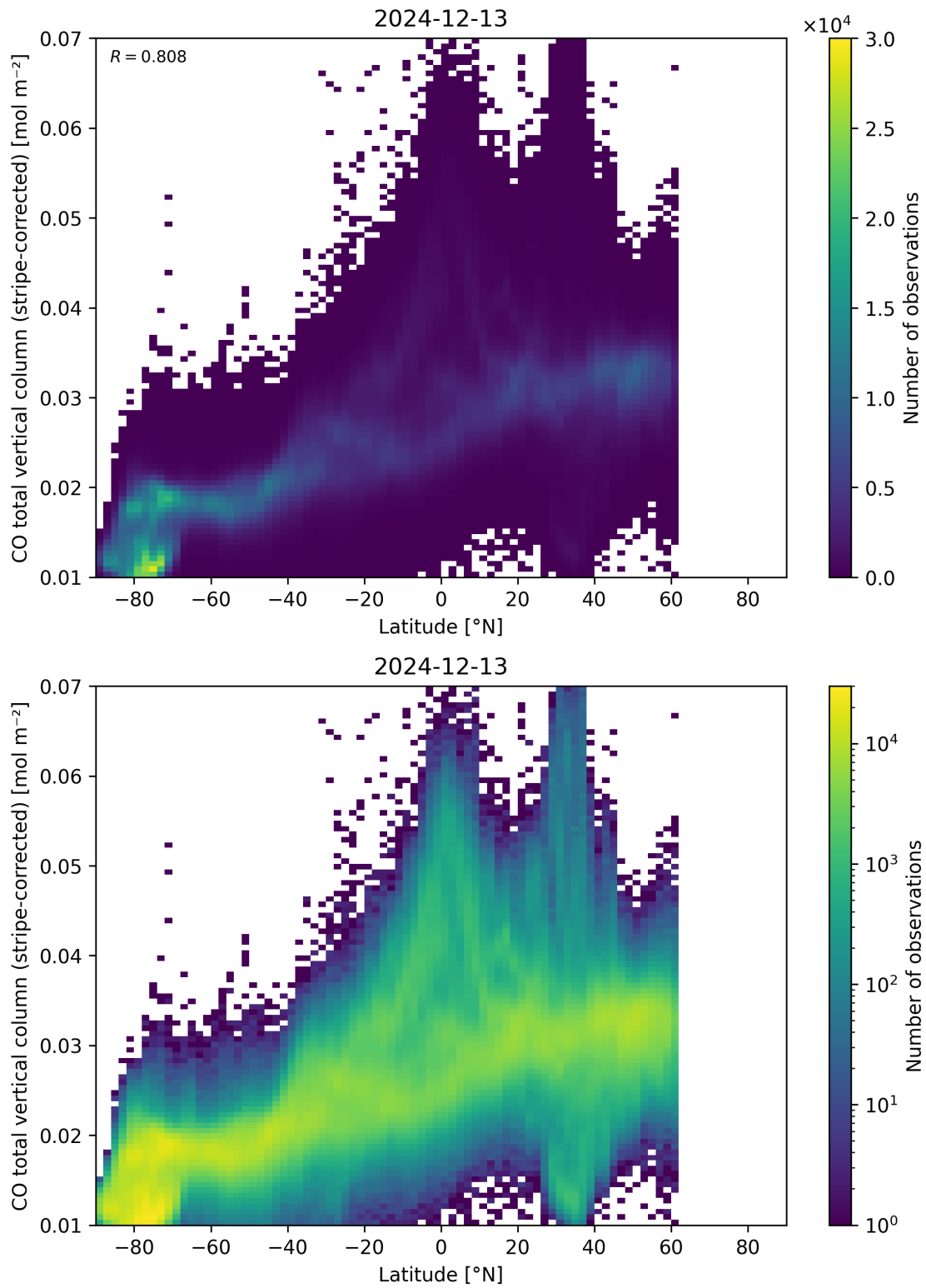
Figure 52: Scatter density plot of “Latitude” against “CO total vertical column (stripe-corrected)” for 2024-12-12 to 2024-12-14.
