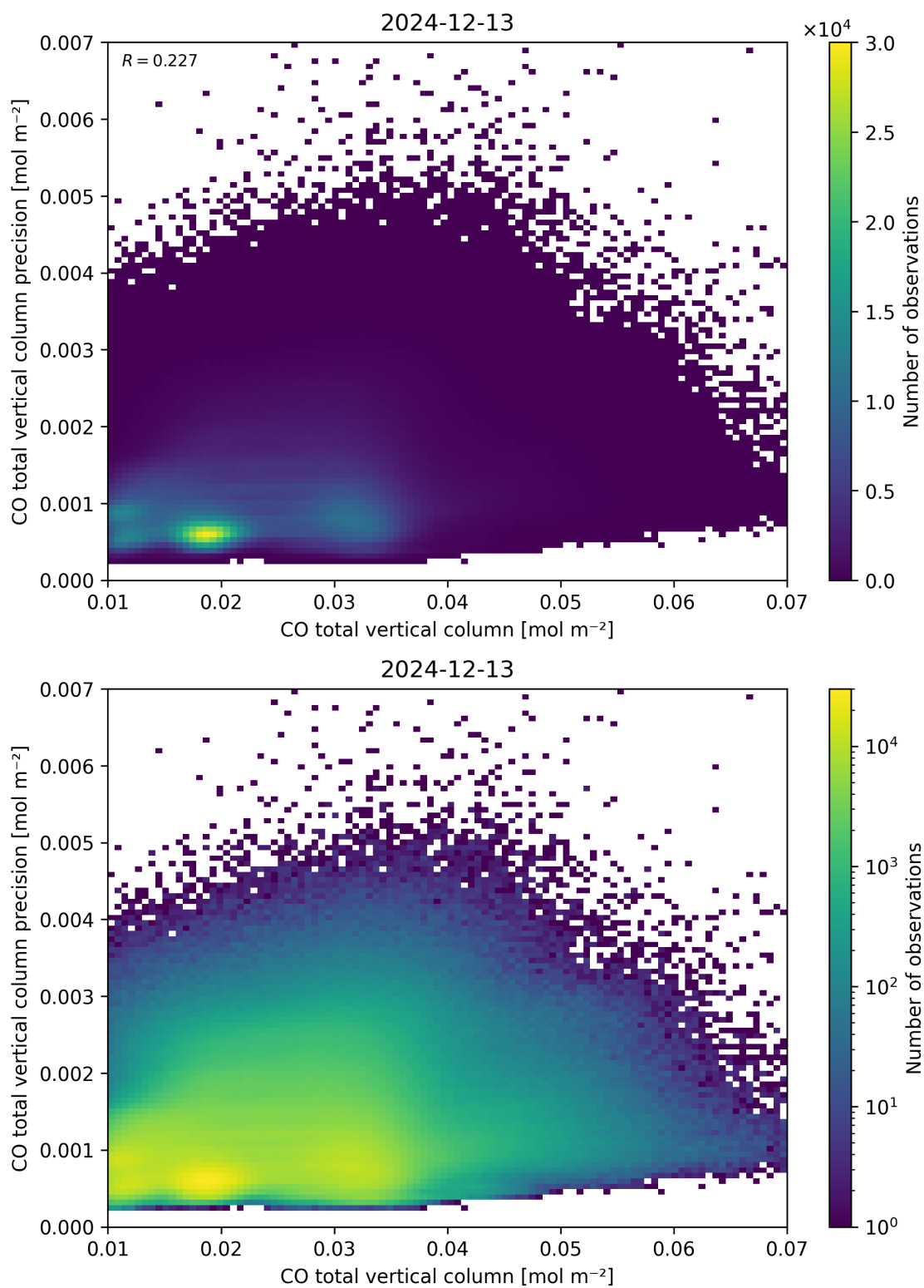
Figure 34: Scatter density plot of “CO total vertical column” against “CO total vertical column precision” for 2024-12-12 to 2024-12-14.
