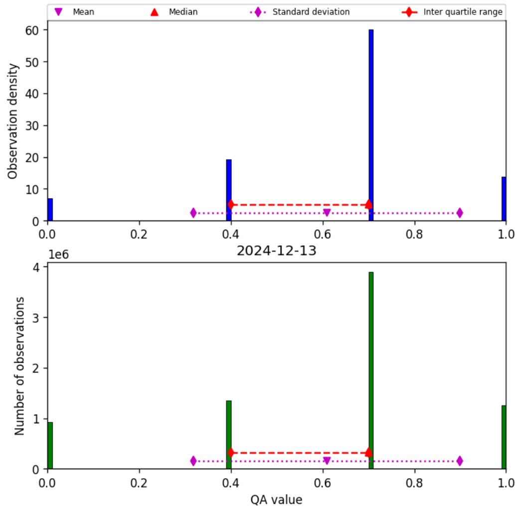
Figure 17: Histogram of “QA value” for 2024-12-12 to 2024-12-14
