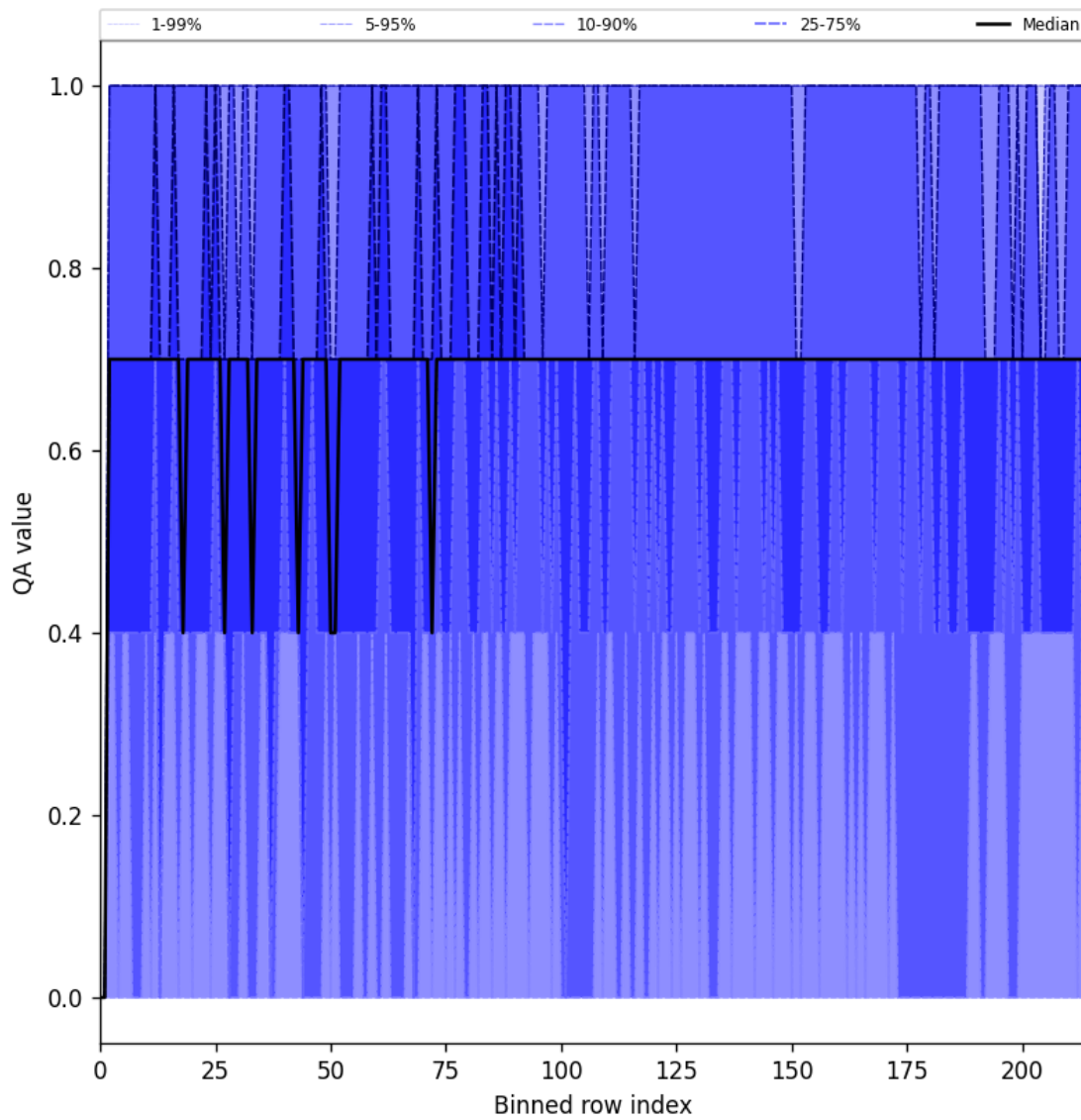
Figure 25: Along track statistics of “QA value” for 2024-12-12 to 2024-12-14
