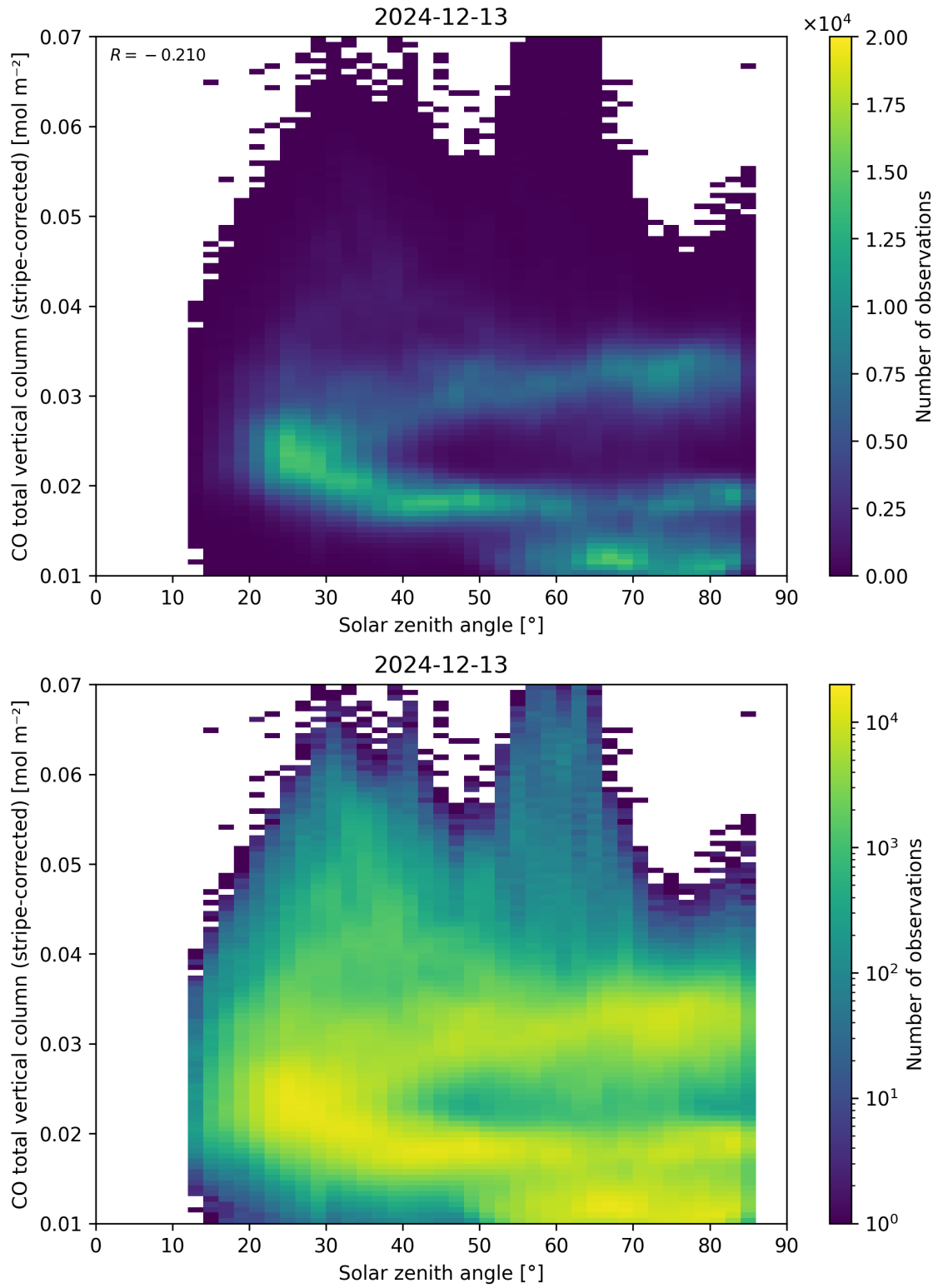
Figure 62: Scatter density plot of “Solar zenith angle” against “CO total vertical column (stripe-corrected)” for 2024-12-12 to 2024-12-14.
