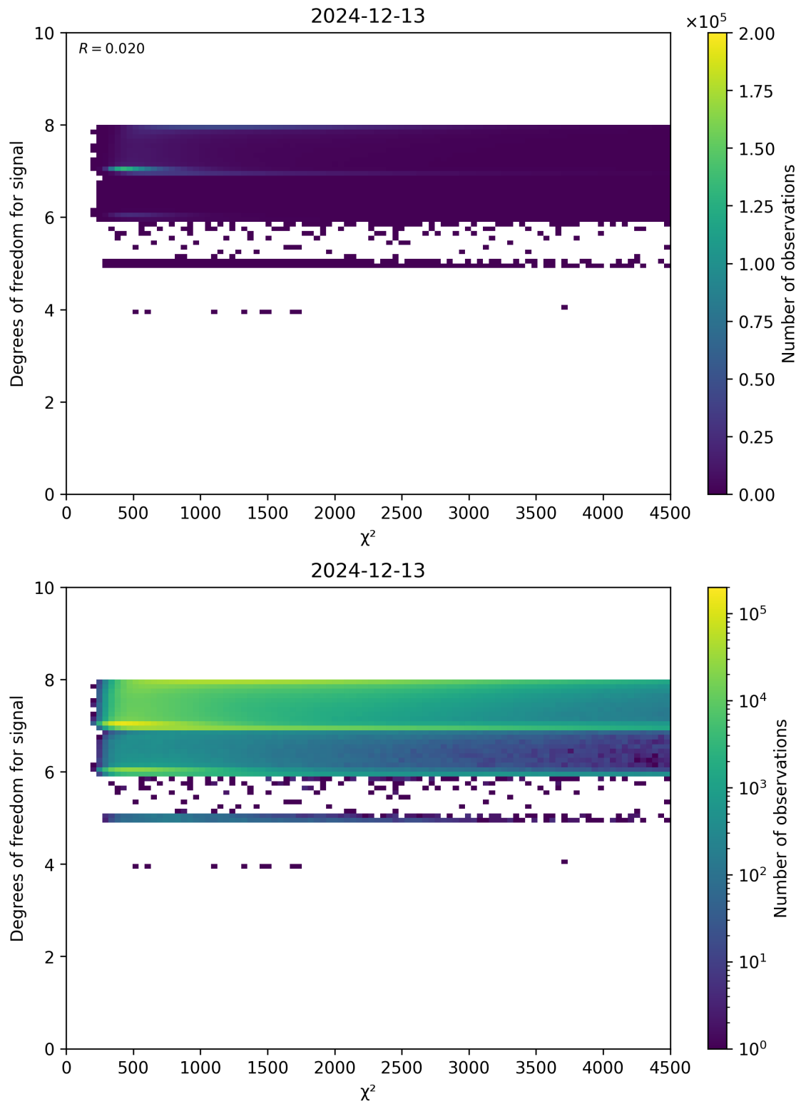
Figure 48: Scatter density plot of “ \chi^2 ” against “Degrees of freedom for signal” for 2024-12-12 to 2024-12-14.
