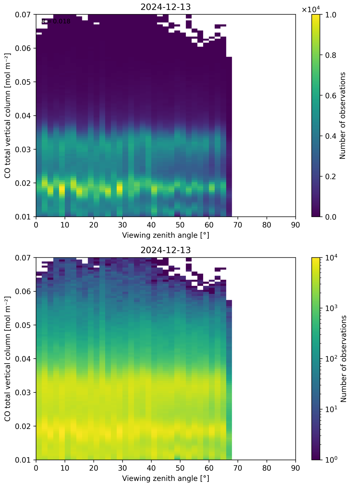
Figure 69: Scatter density plot of “Viewing zenith angle” against “CO total vertical column” for 2024-12-12 to 2024-12-14.
