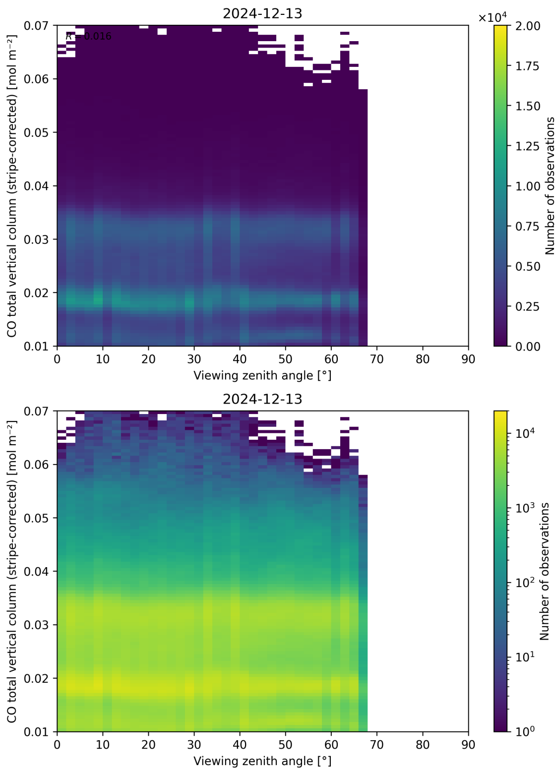
Figure 70: Scatter density plot of “Viewing zenith angle” against “CO total vertical column (stripe-corrected)” for 2024-12-12 to 2024-12-14.
