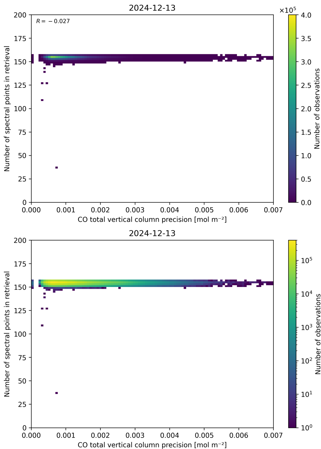
Figure 47: Scatter density plot of “CO total vertical column precision” against “Number of spectral points in retrieval” for 2024-12-12 to 2024-12-14.
