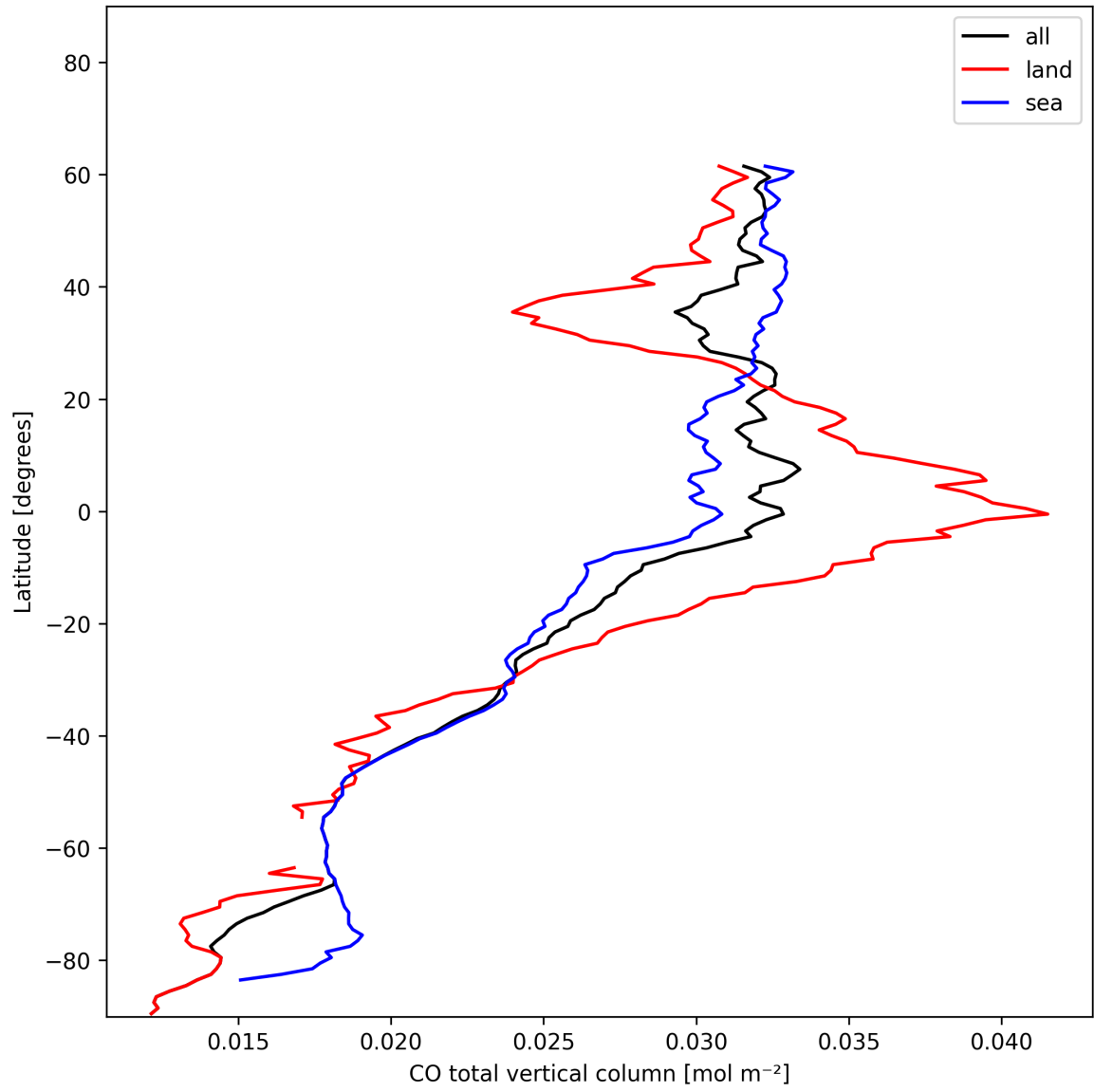
Figure 10: Zonal average of “CO total vertical column” for 2024-12-12 to 2024-12-14.
