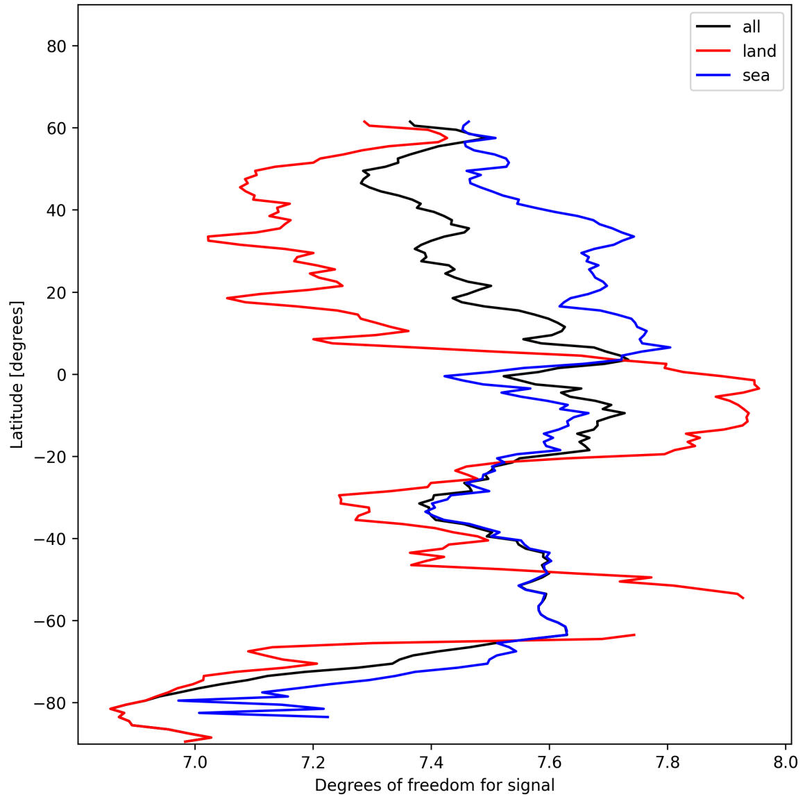
Figure 15: Zonal average of “Degrees of freedom for signal” for 2024-12-12 to 2024-12-14.
