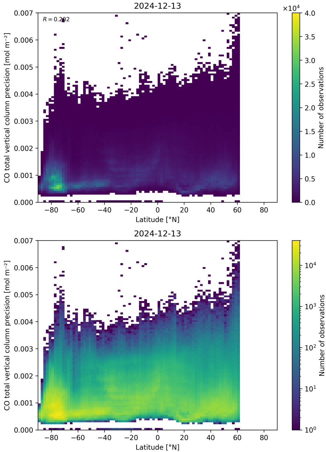
Figure 53: Scatter density plot of “Latitude” against “CO total vertical column precision” for 2024-12-12 to 2024-12-14.
