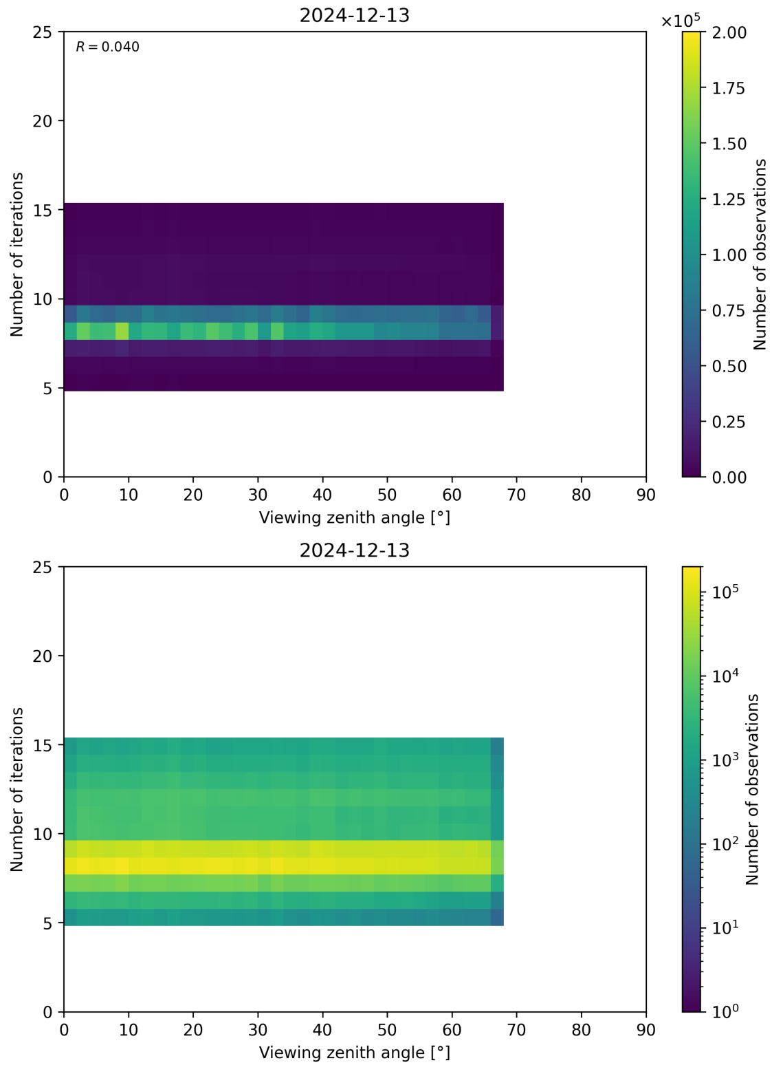
Figure 75: Scatter density plot of “Viewing zenith angle” against “Number of iterations” for 2024-12-12 to 2024-12-14.
