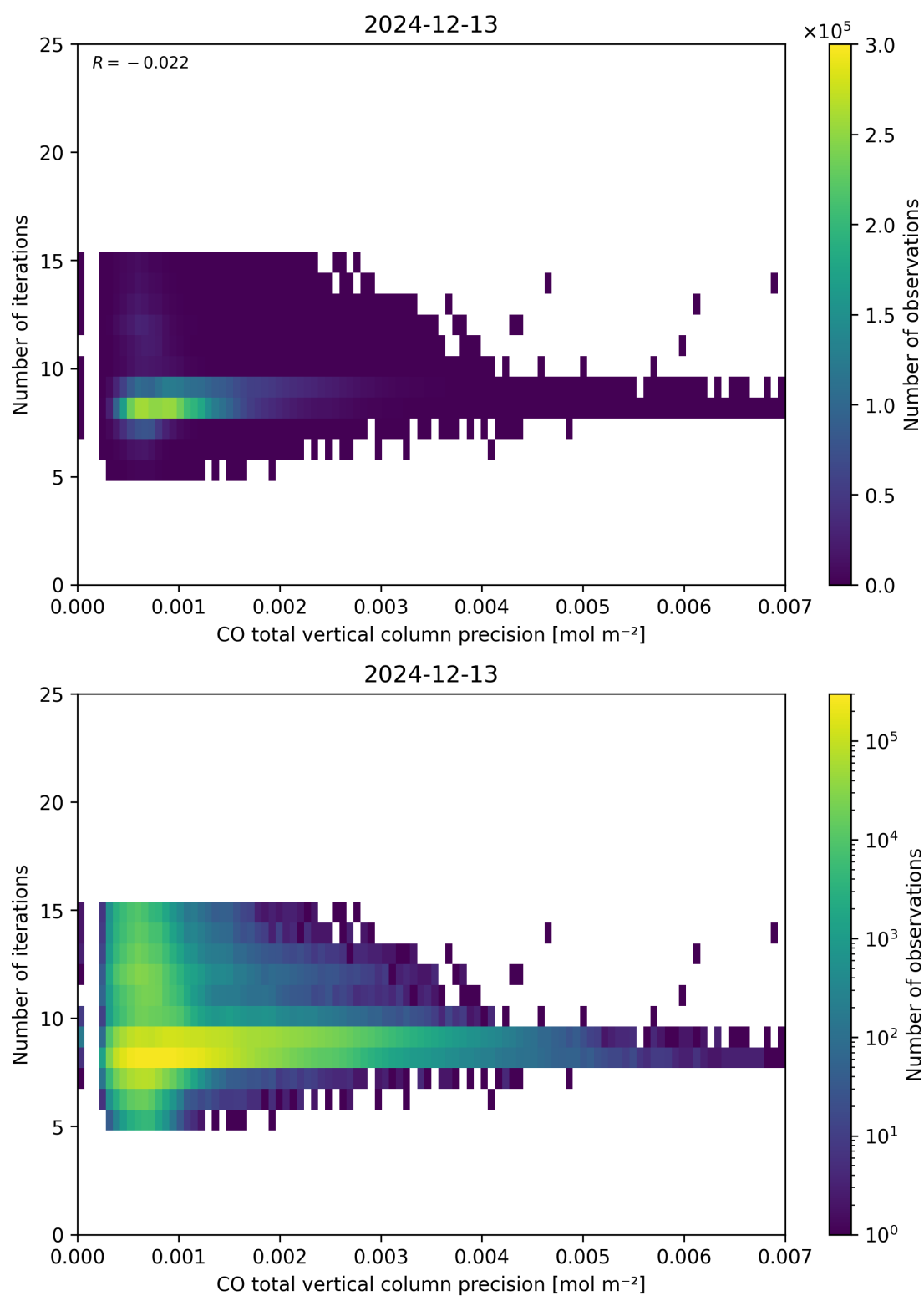
Figure 46: Scatter density plot of “CO total vertical column precision” against “Number of iterations” for 2024-12-12 to 2024-12-14.
