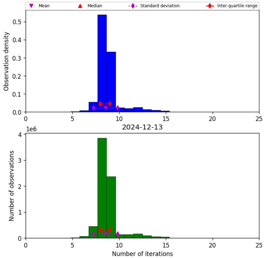
Figure 24: Histogram of “Number of iterations” for 2024-12-12 to 2024-12-14
