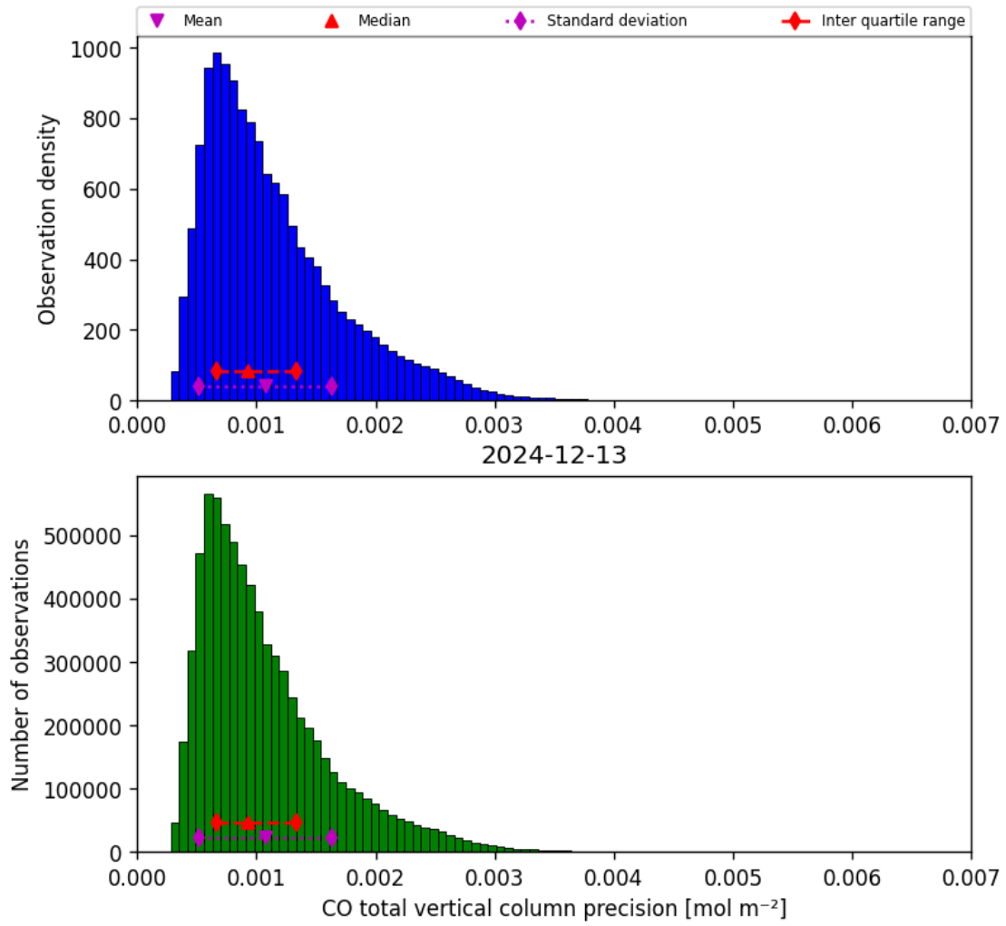
Figure 20: Histogram of “CO total vertical column precision” for 2024-12-12 to 2024-12-14
