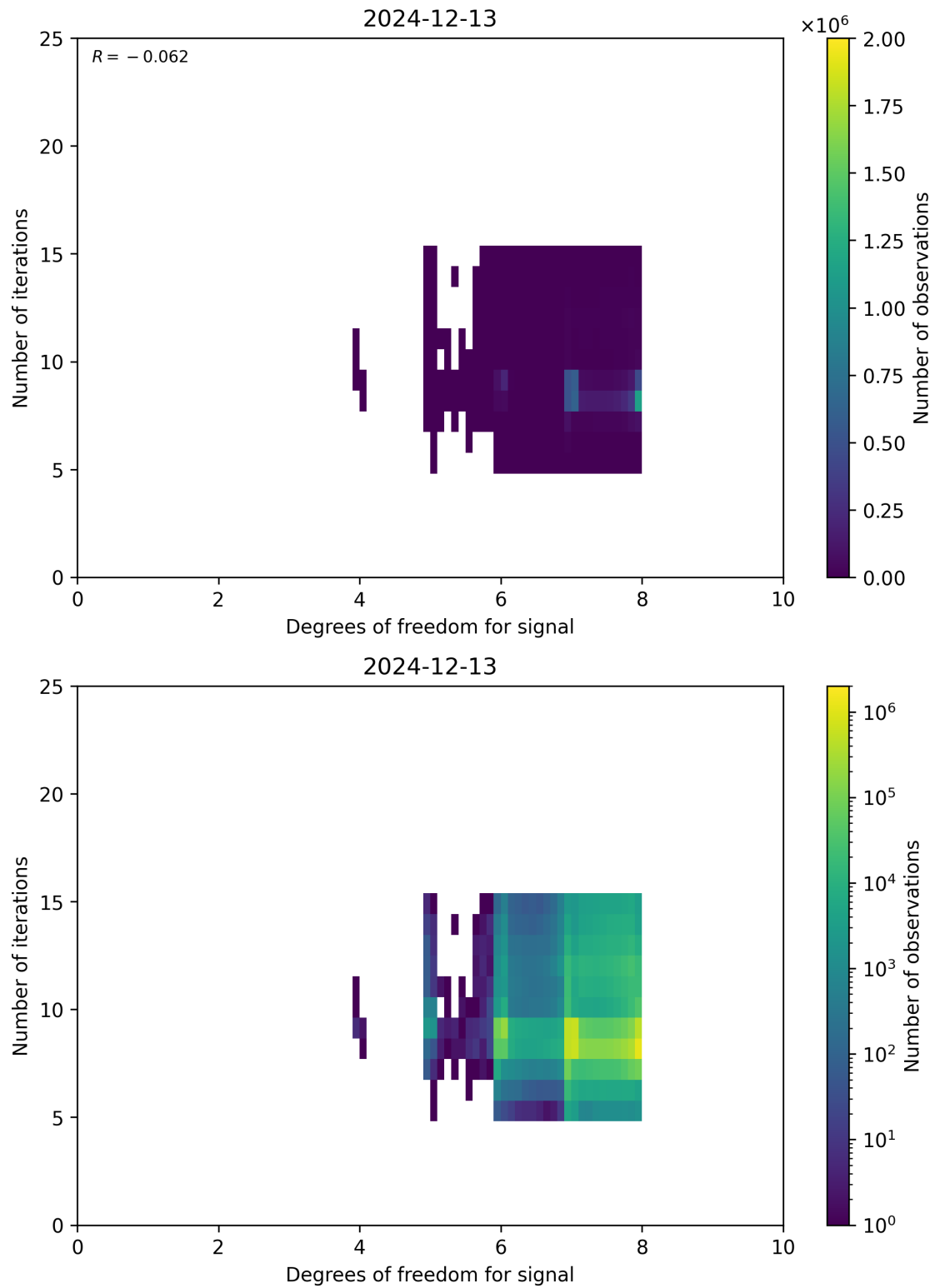
Figure 50: Scatter density plot of “Degrees of freedom for signal” against “Number of iterations” for 2024-12-12 to 2024-12-14.
