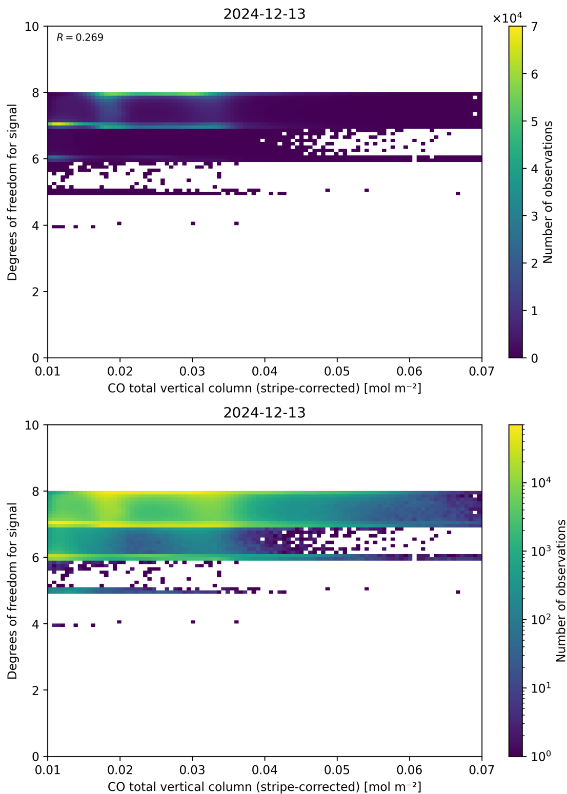
Figure 38: Scatter density plot of “CO total vertical column (stripe-corrected)” against “Degrees of freedom for signal” for 2024-12-12 to 2024-12-14.
