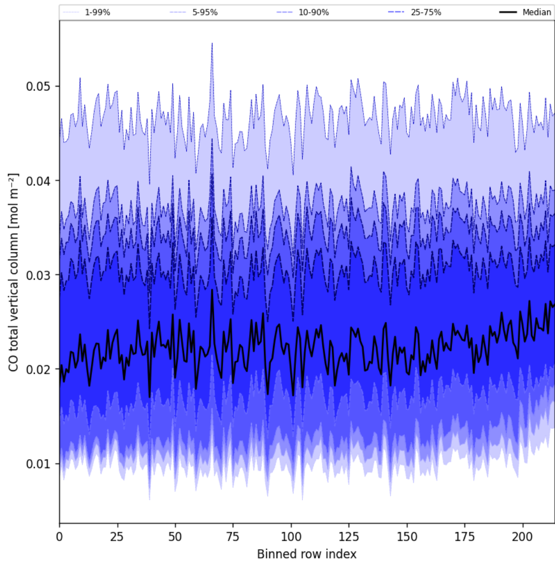
Figure 26: Along track statistics of “CO total vertical column” for 2024-12-12 to 2024-12-14
