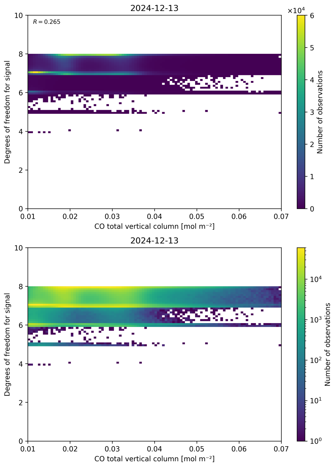
Figure 41: Scatter density plot of “CO total vertical column” against “Degrees of freedom for signal” for 2024-12-12 to 2024-12-14.
