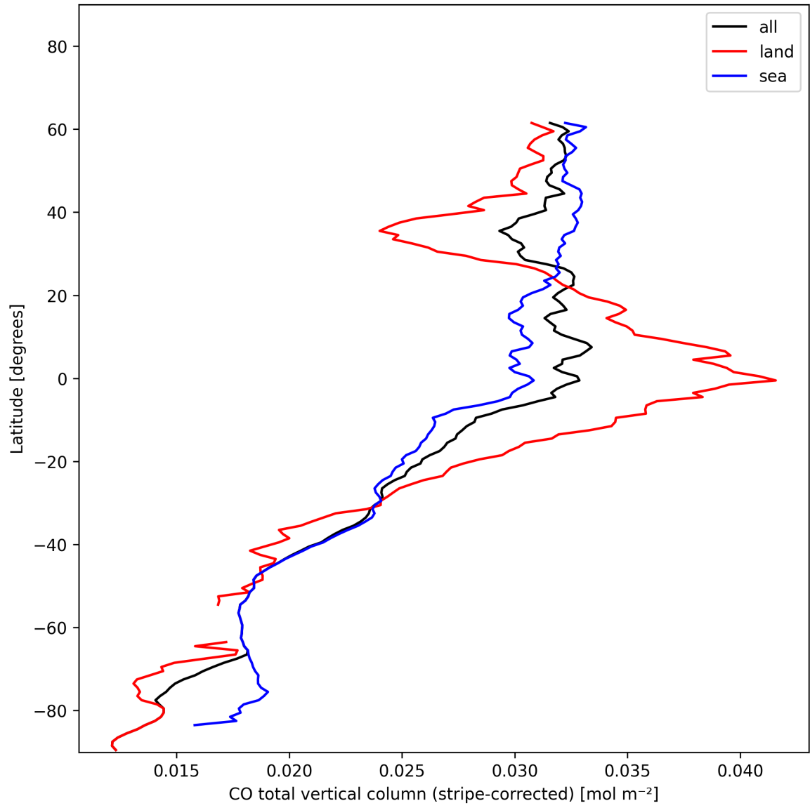
Figure 11: Zonal average of “CO total vertical column (stripe-corrected)” for 2024-12-12 to 2024-12-14.
