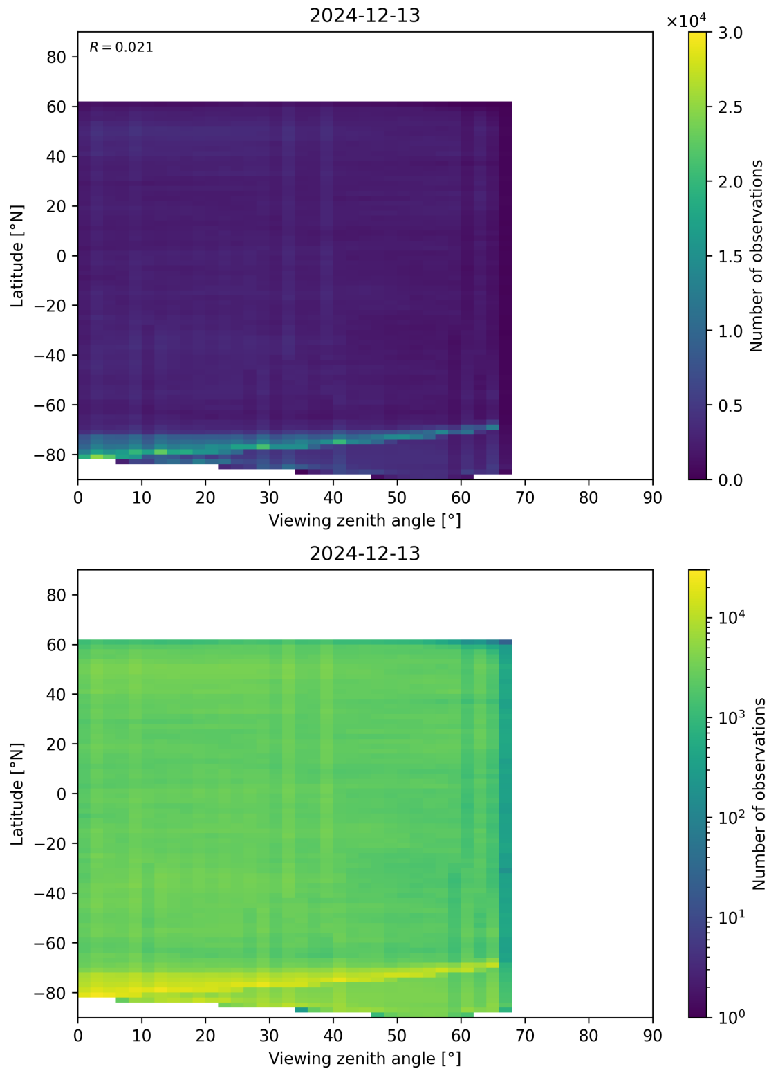
Figure 74: Scatter density plot of “Viewing zenith angle” against “Latitude” for 2024-12-12 to 2024-12-14.
