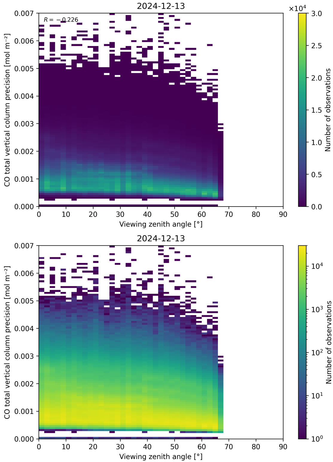
Figure 71: Scatter density plot of “Viewing zenith angle” against “CO total vertical column precision” for 2024-12-12 to 2024-12-14.
