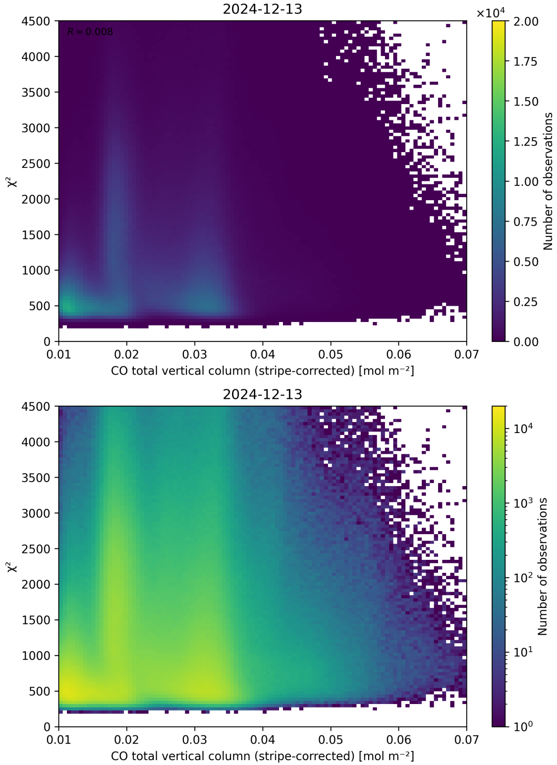
Figure 37: Scatter density plot of “CO total vertical column (stripe-corrected)” against “ \chi^2 ” for 2024-12-12 to 2024-12-14.
