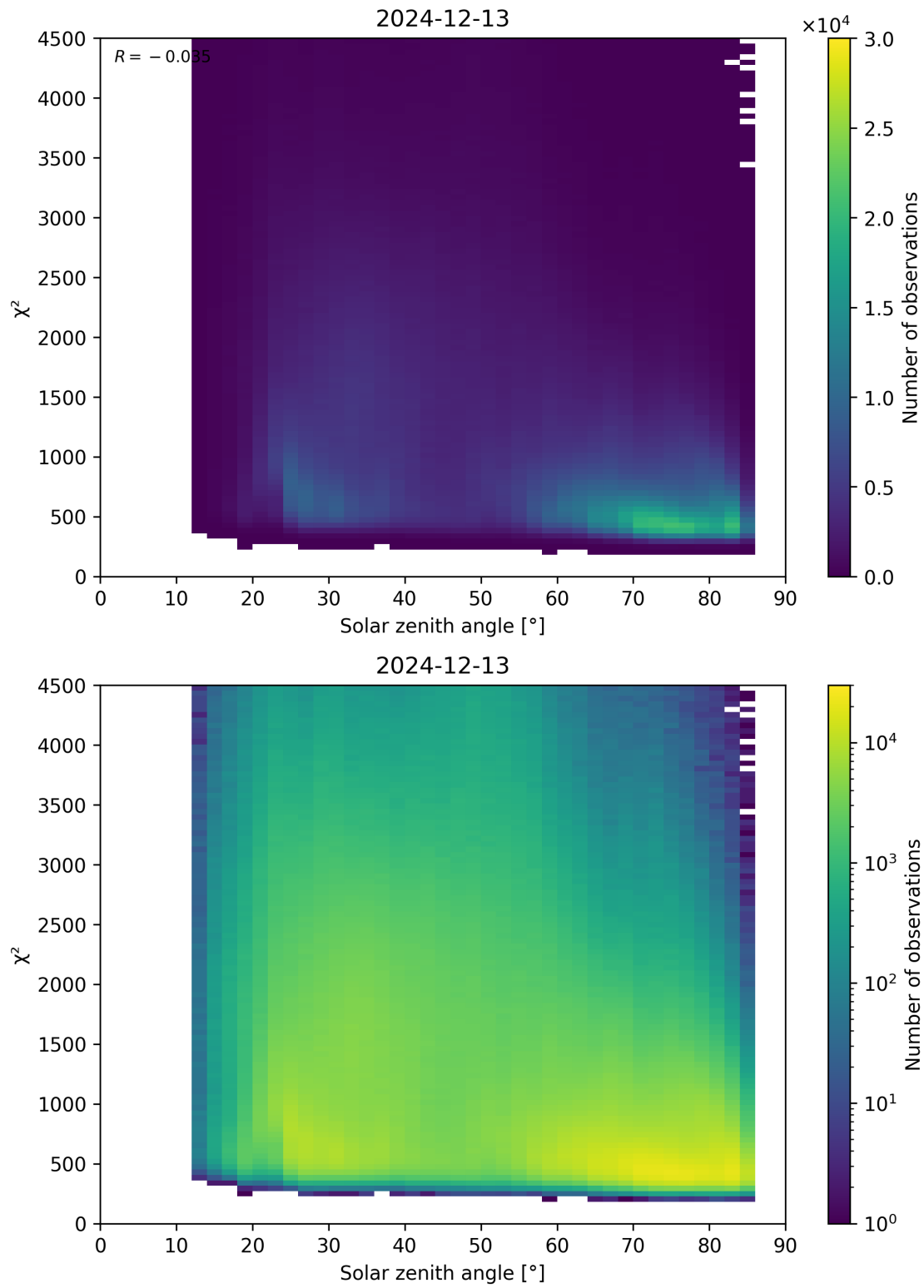
Figure 64: Scatter density plot of “Solar zenith angle” against “ \chi^2 ” for 2024-12-12 to 2024-12-14.
