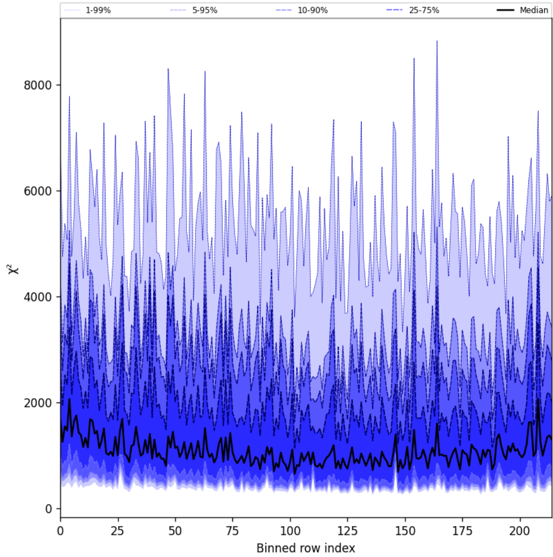
Figure 30: Along track statistics of “ \chi^2 ” for 2024-12-12 to 2024-12-14
