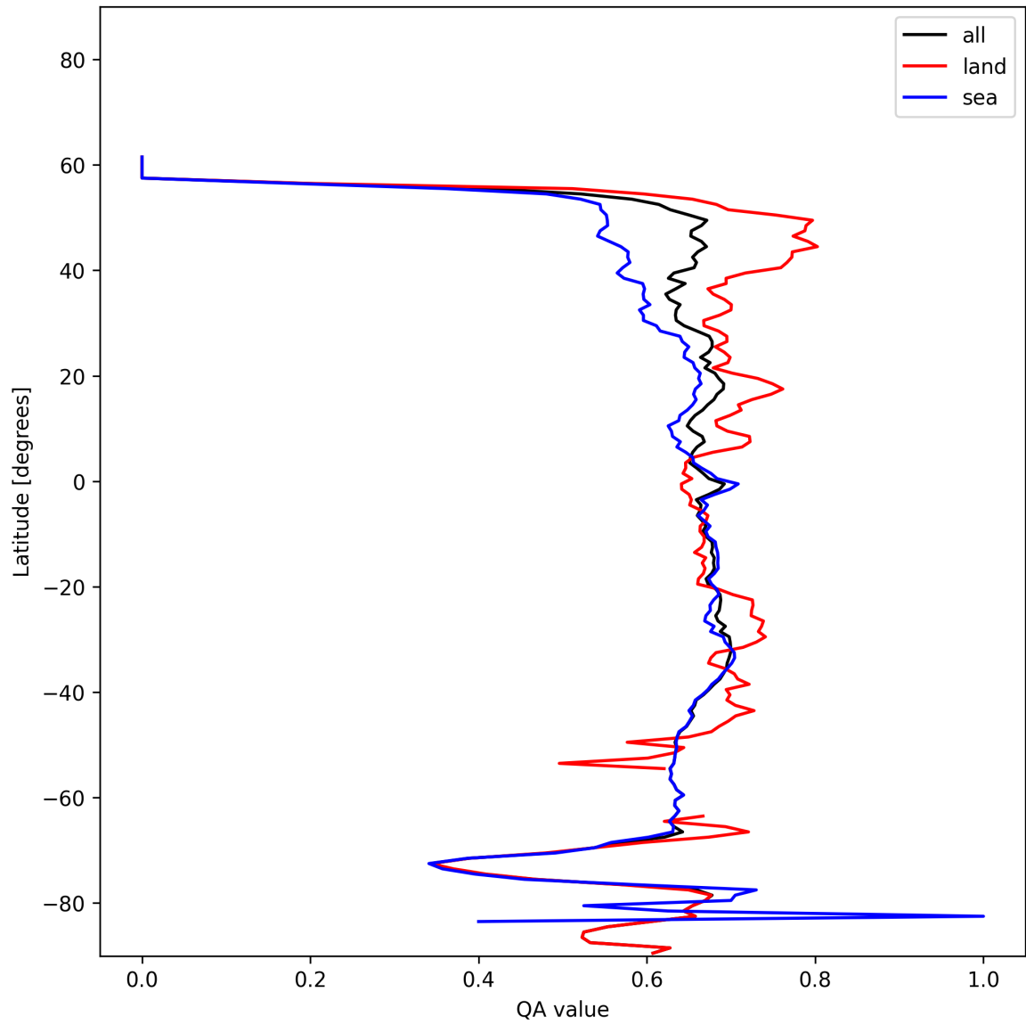
Figure 9: Zonal average of “QA value” for 2024-12-12 to 2024-12-14.
