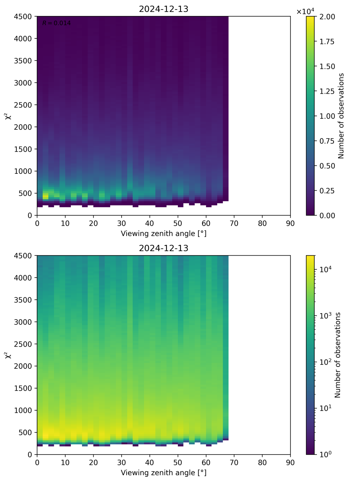
Figure 72: Scatter density plot of “Viewing zenith angle” against “ \chi^2 ” for 2024-12-12 to 2024-12-14.
