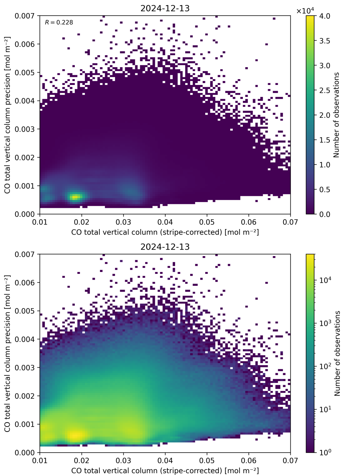
Figure 36: Scatter density plot of “CO total vertical column (stripe-corrected)” against “CO total vertical column precision” for 2024-12-12 to 2024-12-14.
