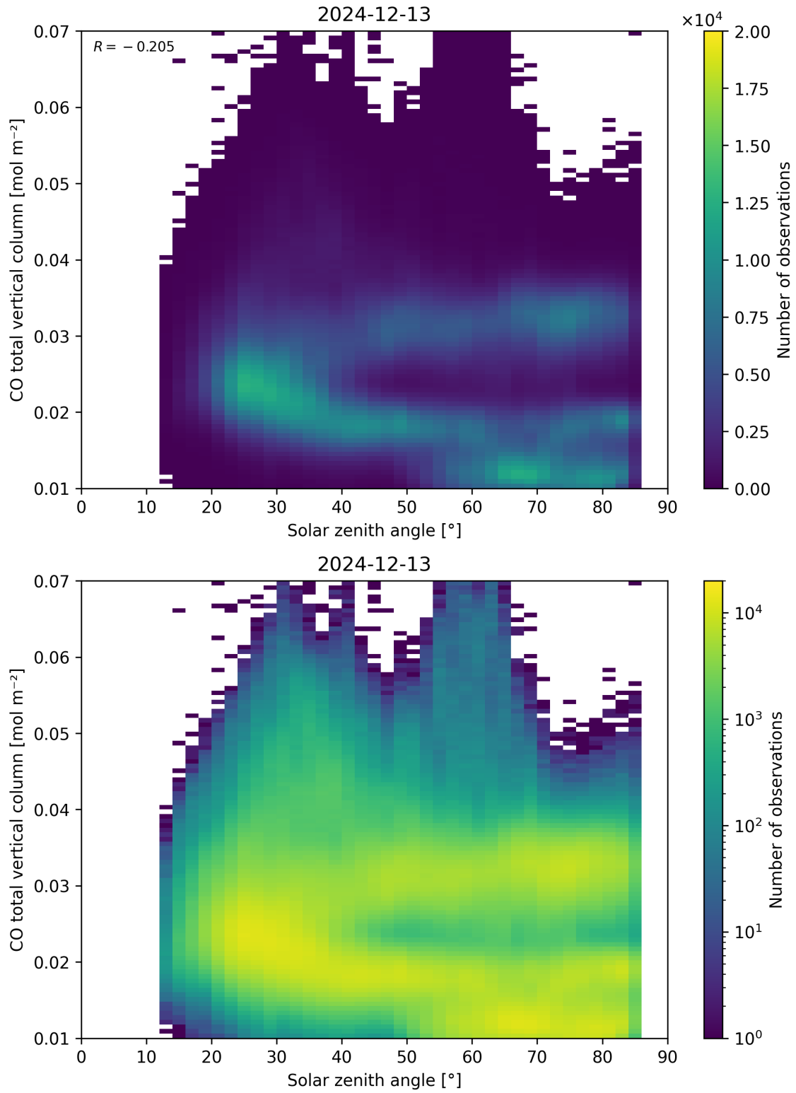
Figure 61: Scatter density plot of “Solar zenith angle” against “CO total vertical column” for 2024-12-12 to 2024-12-14.
