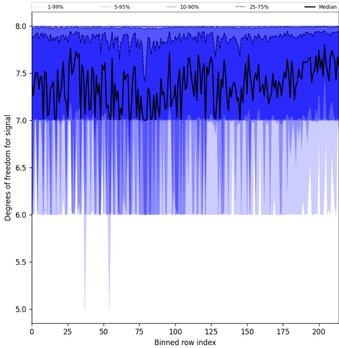
Figure 31: Along track statistics of “Degrees of freedom for signal” for 2024-12-12 to 2024-12-14
