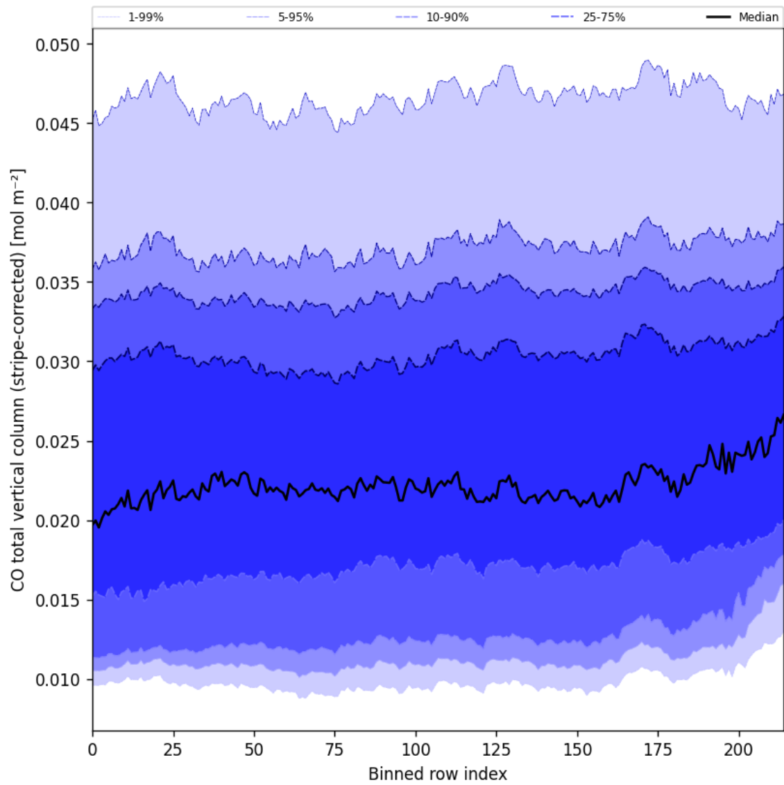
Figure 27: Along track statistics of “CO total vertical column (stripe-corrected)” for 2024-12-12 to 2024-12-14
