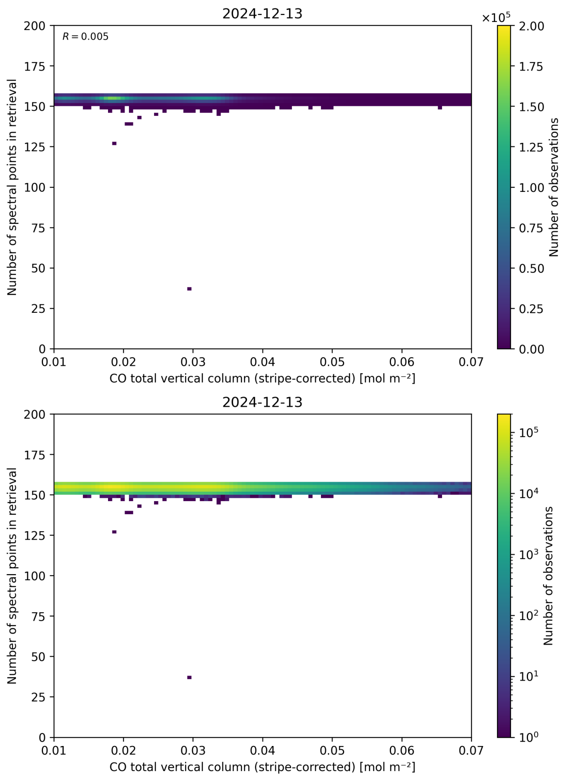
Figure 40: Scatter density plot of “CO total vertical column (stripe-corrected)” against “Number of spectral points in retrieval” for 2024-12-12 to 2024-12-14.
