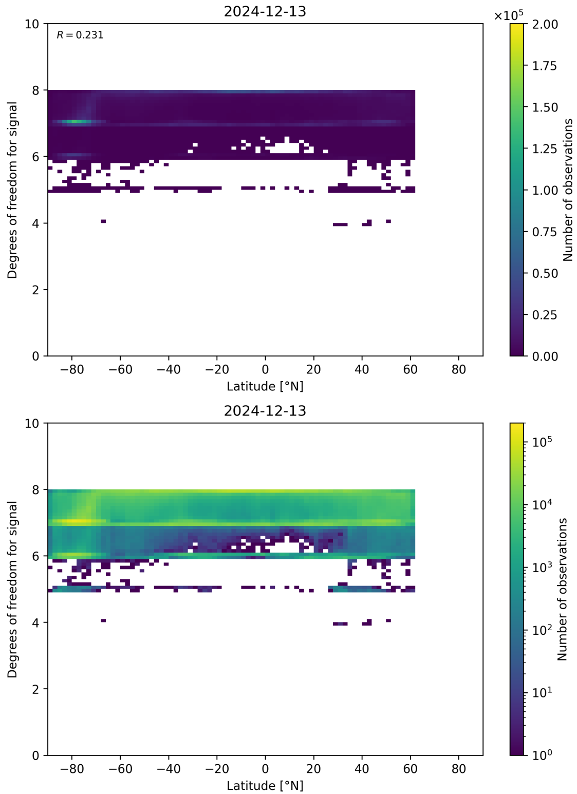
Figure 55: Scatter density plot of “Latitude” against “Degrees of freedom for signal” for 2024-12-12 to 2024-12-14.
