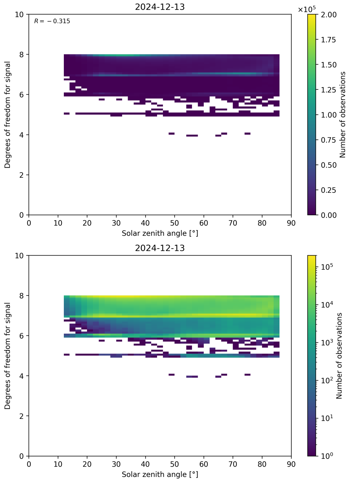
Figure 65: Scatter density plot of “Solar zenith angle” against “Degrees of freedom for signal” for 2024-12-12 to 2024-12-14.
