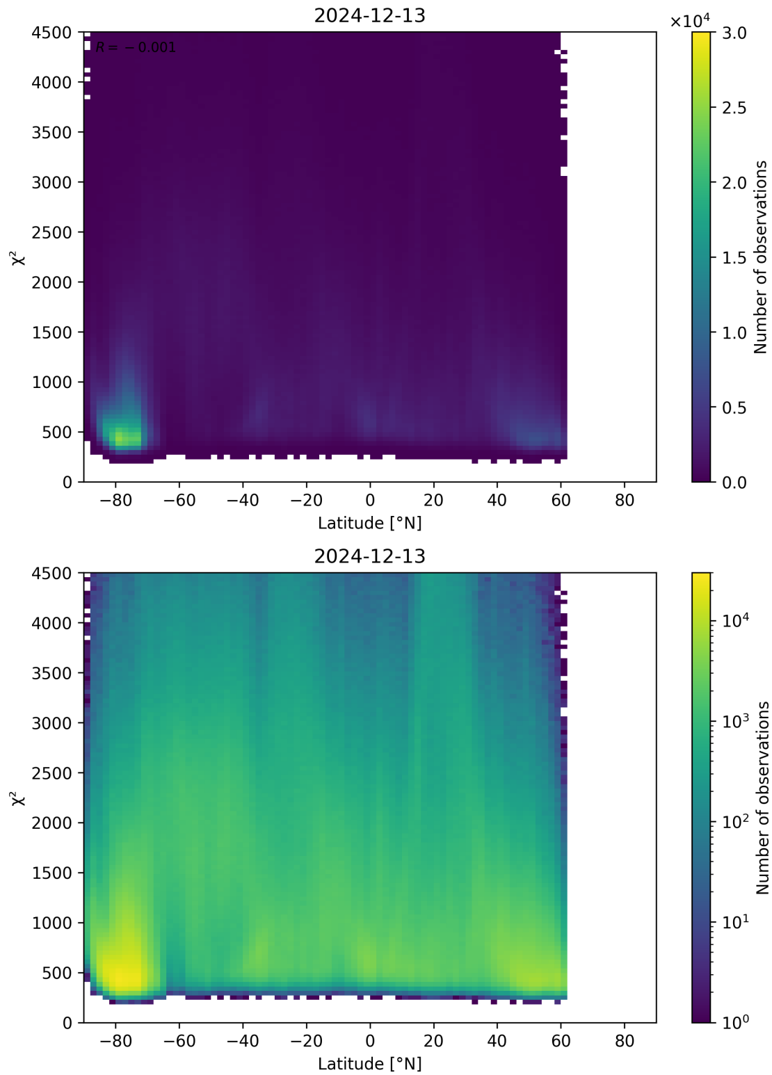
Figure 54: Scatter density plot of “Latitude” against “ \chi^2 ” for 2024-12-12 to 2024-12-14.
