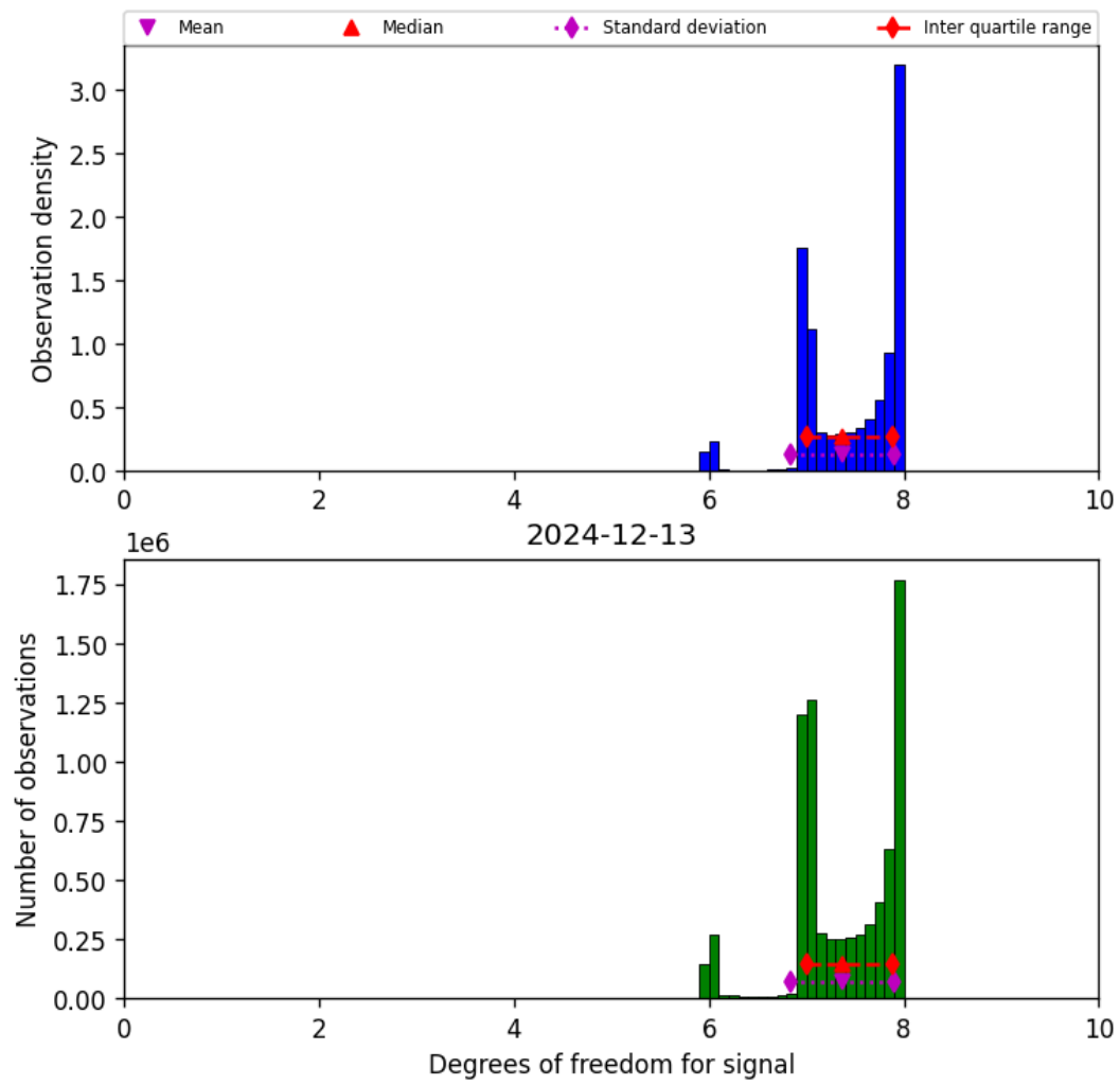
Figure 23: Histogram of “Degrees of freedom for signal” for 2024-12-12 to 2024-12-14
