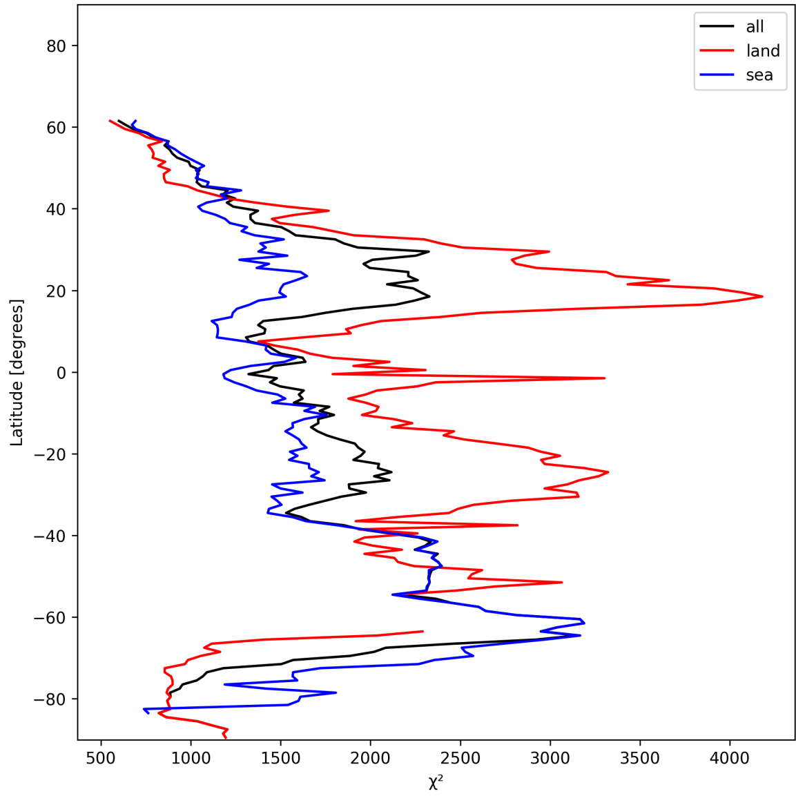
Figure 14: Zonal average of “ \chi^2 ” for 2024-12-12 to 2024-12-14.
