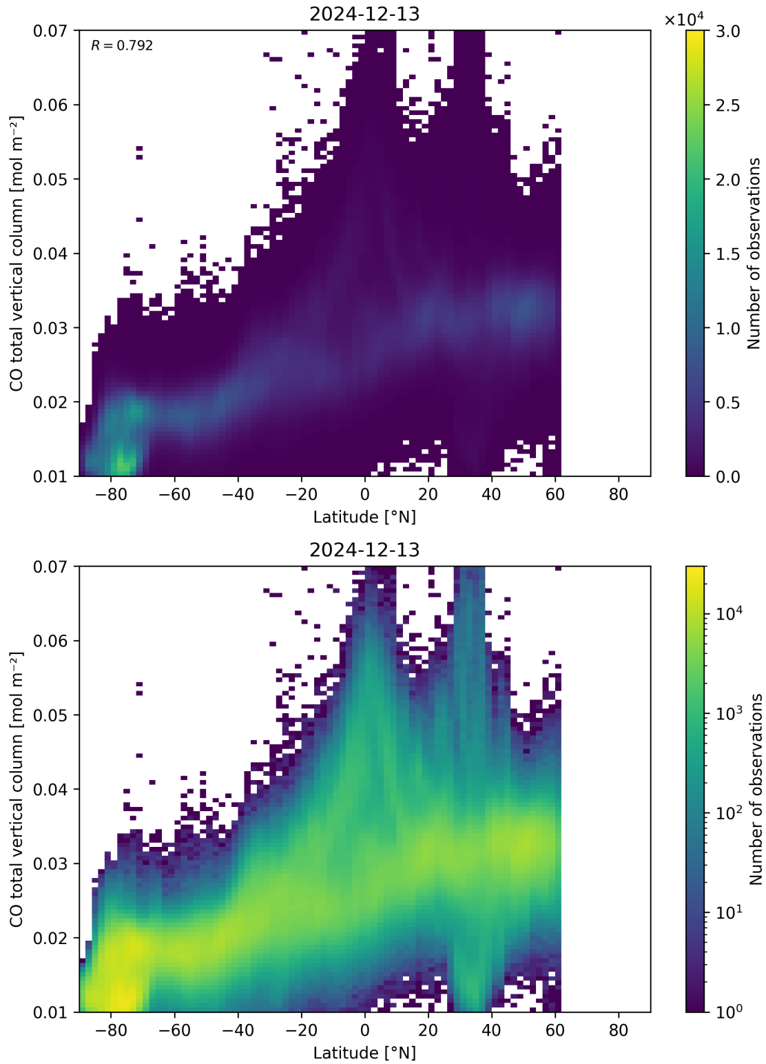
Figure 51: Scatter density plot of “Latitude” against “CO total vertical column” for 2024-12-12 to 2024-12-14.
