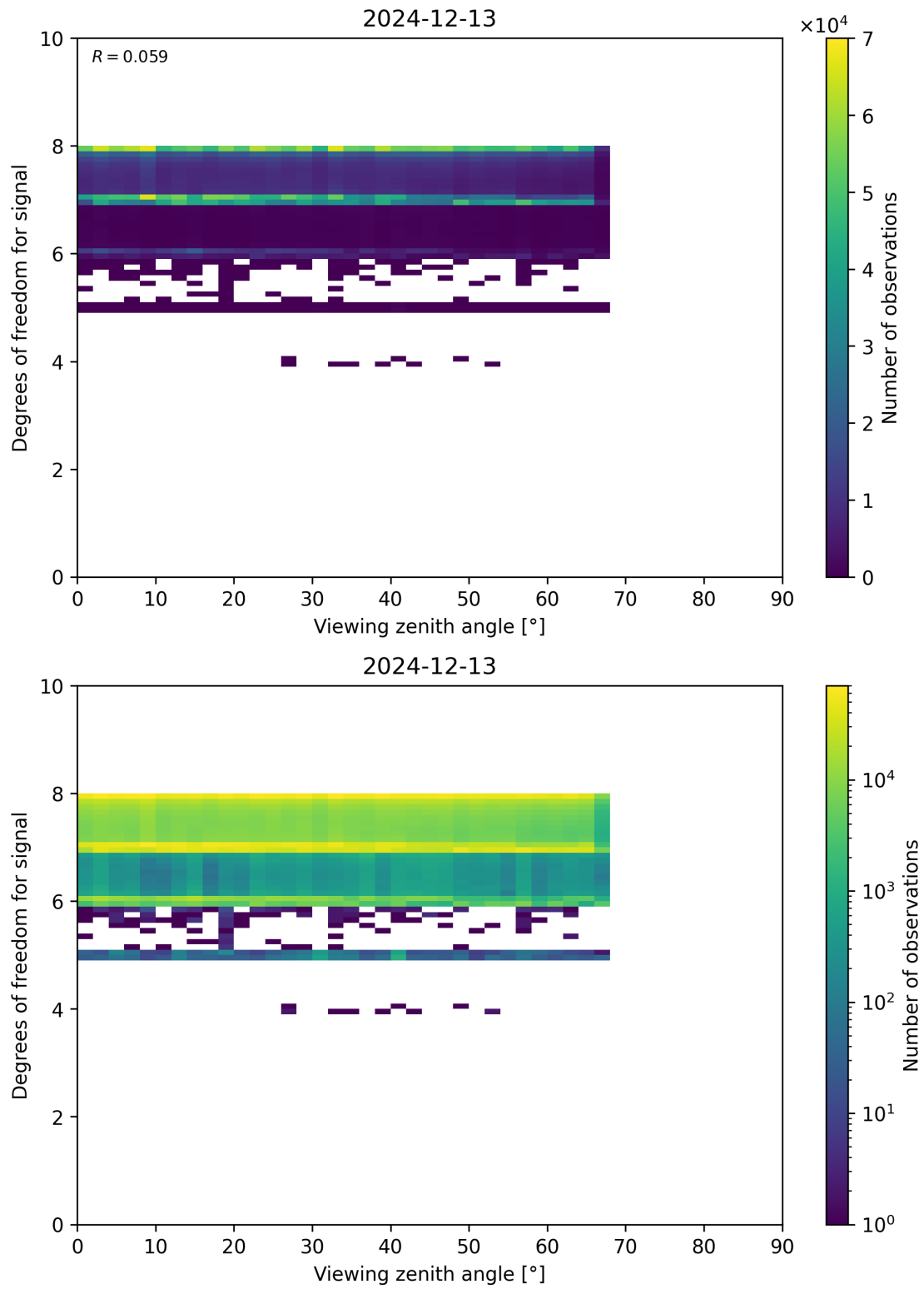
Figure 73: Scatter density plot of “Viewing zenith angle” against “Degrees of freedom for signal” for 2024-12-12 to 2024-12-14.
