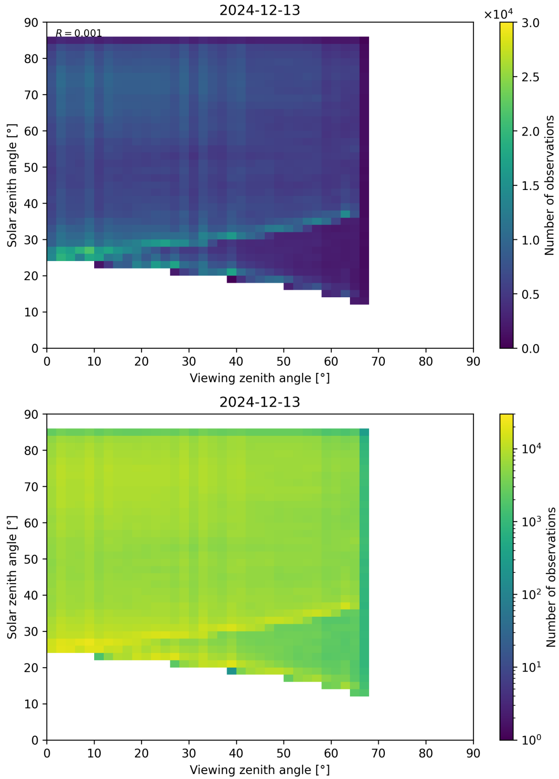
Figure 77: Scatter density plot of “Viewing zenith angle” against “Solar zenith angle” for 2024-12-12 to 2024-12-14.
