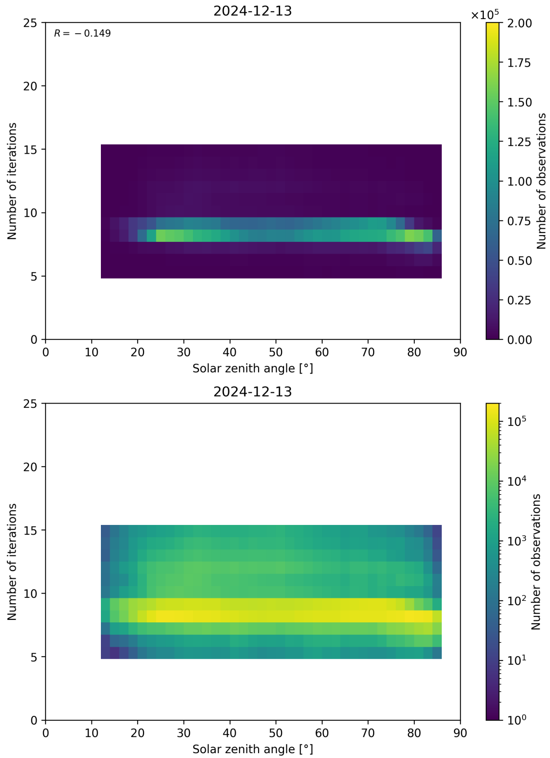
Figure 67: Scatter density plot of “Solar zenith angle” against “Number of iterations” for 2024-12-12 to 2024-12-14.
