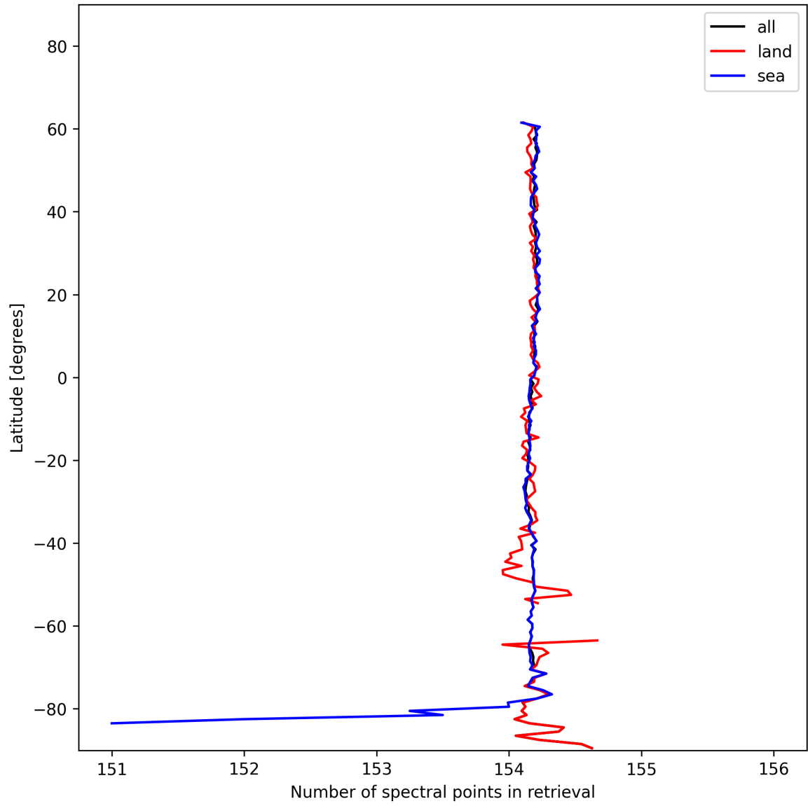
Figure 13: Zonal average of “Number of spectral points in retrieval” for 2024-12-12 to 2024-12-14.
