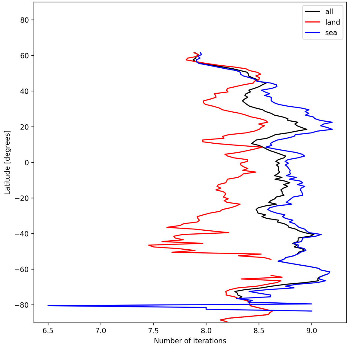
Figure 16: Zonal average of “Number of iterations” for 2024-12-12 to 2024-12-14.
