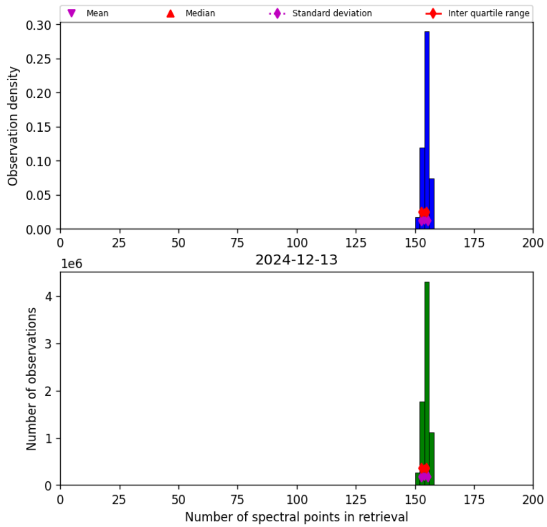
Figure 21: Histogram of “Number of spectral points in retrieval” for 2024-12-12 to 2024-12-14
