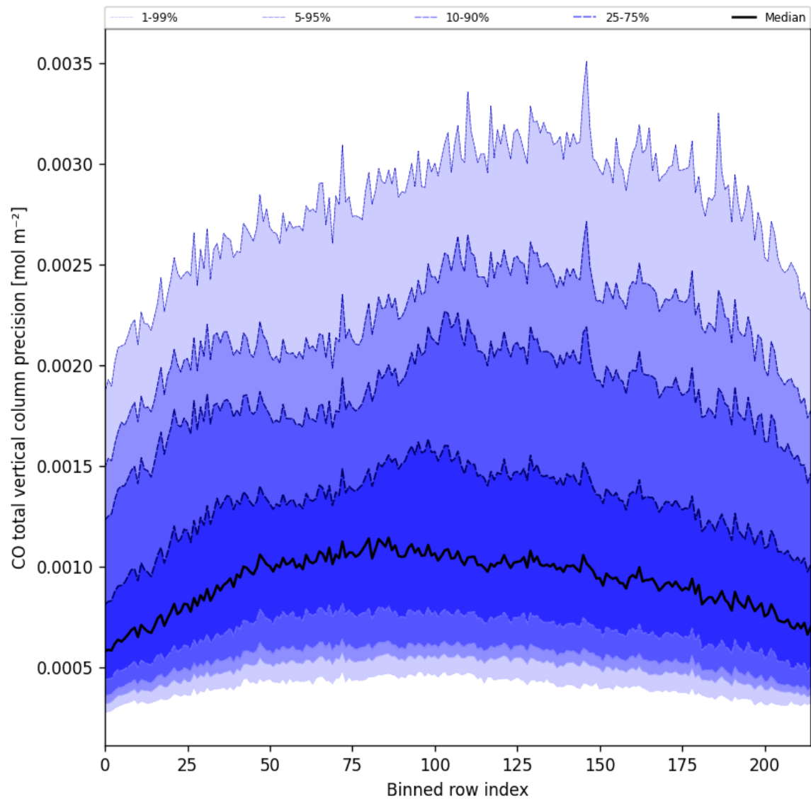
Figure 28: Along track statistics of “CO total vertical column precision” for 2024-12-12 to 2024-12-14
