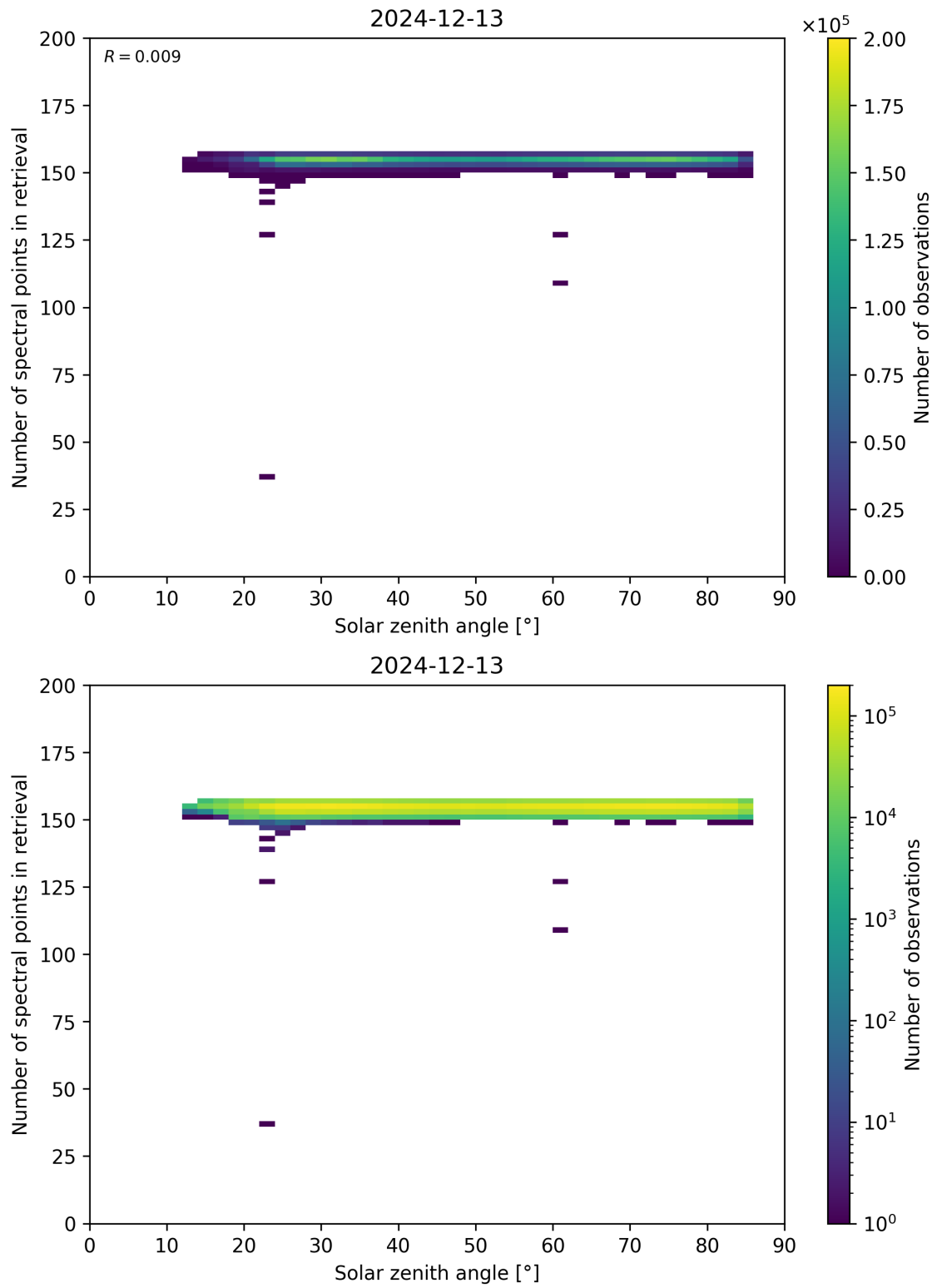
Figure 68: Scatter density plot of “Solar zenith angle” against “Number of spectral points in retrieval” for 2024-12-12 to 2024-12-14.
