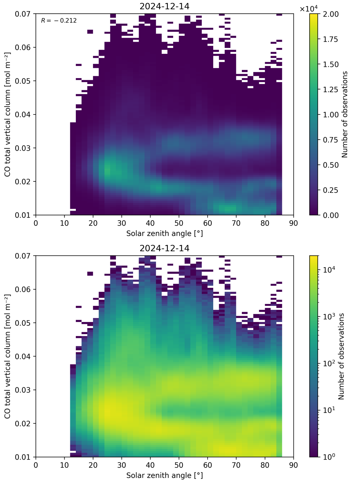
Figure 61: Scatter density plot of “Solar zenith angle” against “CO total vertical column” for 2024-12-13 to 2024-12-15.
