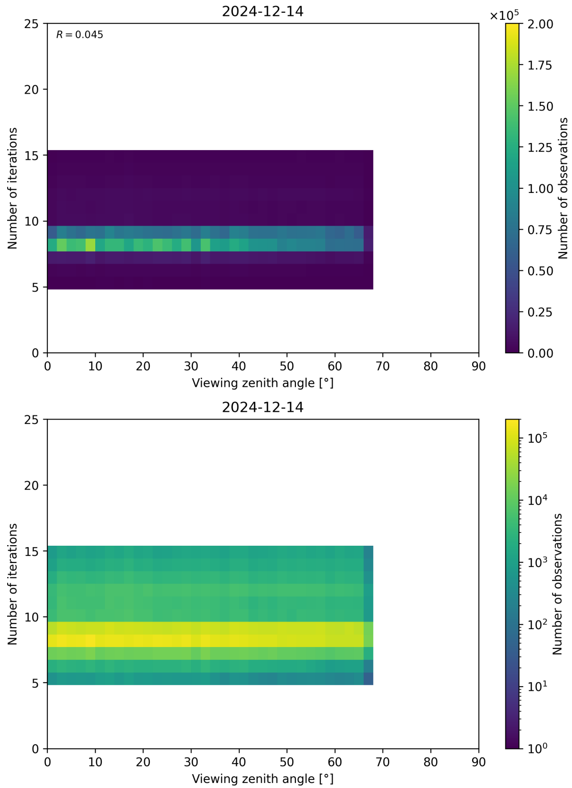
Figure 75: Scatter density plot of “Viewing zenith angle” against “Number of iterations” for 2024-12-13 to 2024-12-15.
