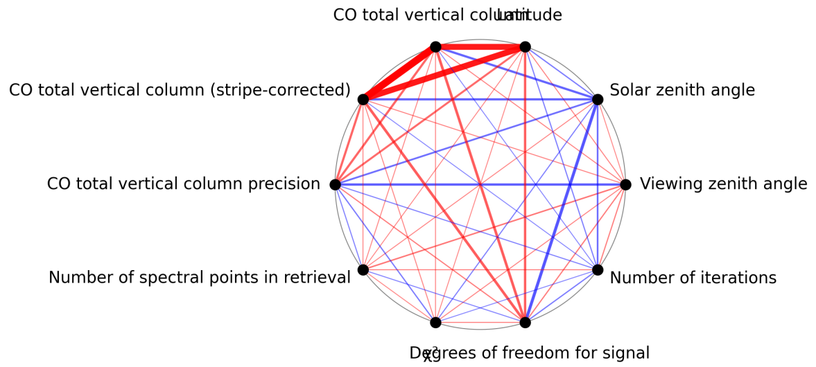
Figure 1: Map of correlation graph for 2024-12-13 to 2024-12-15.
