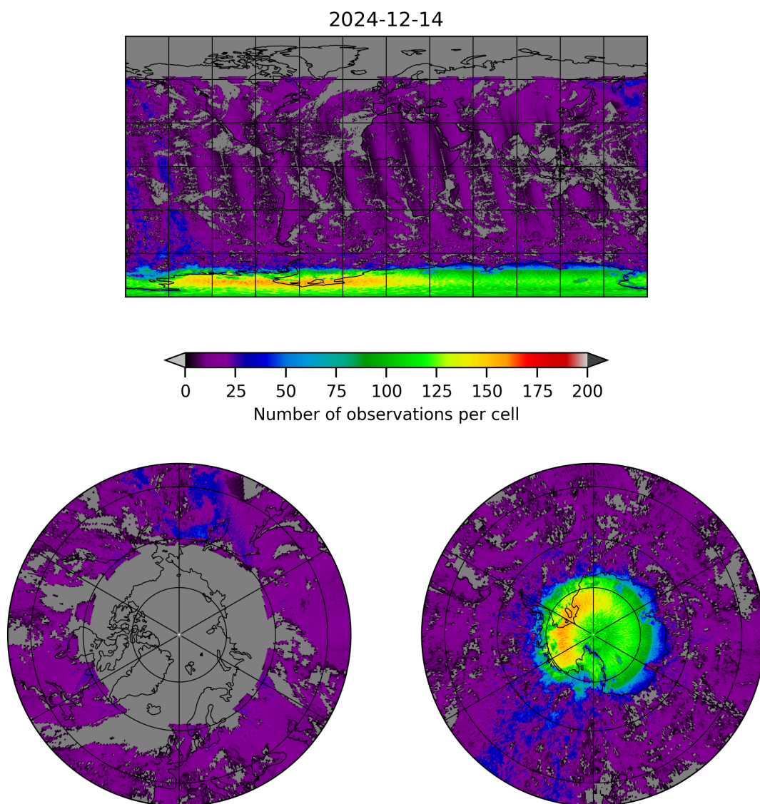
Figure 8: Map of the number of observations for 2024-12-13 to 2024-12-15
