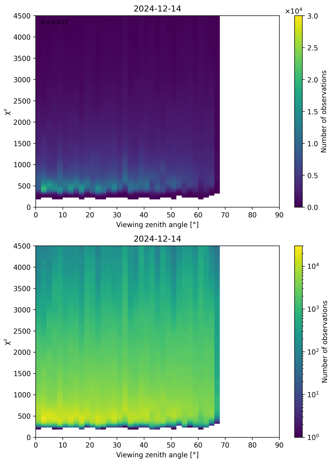
Figure 72: Scatter density plot of “Viewing zenith angle” against “ \chi^2 ” for 2024-12-13 to 2024-12-15.
