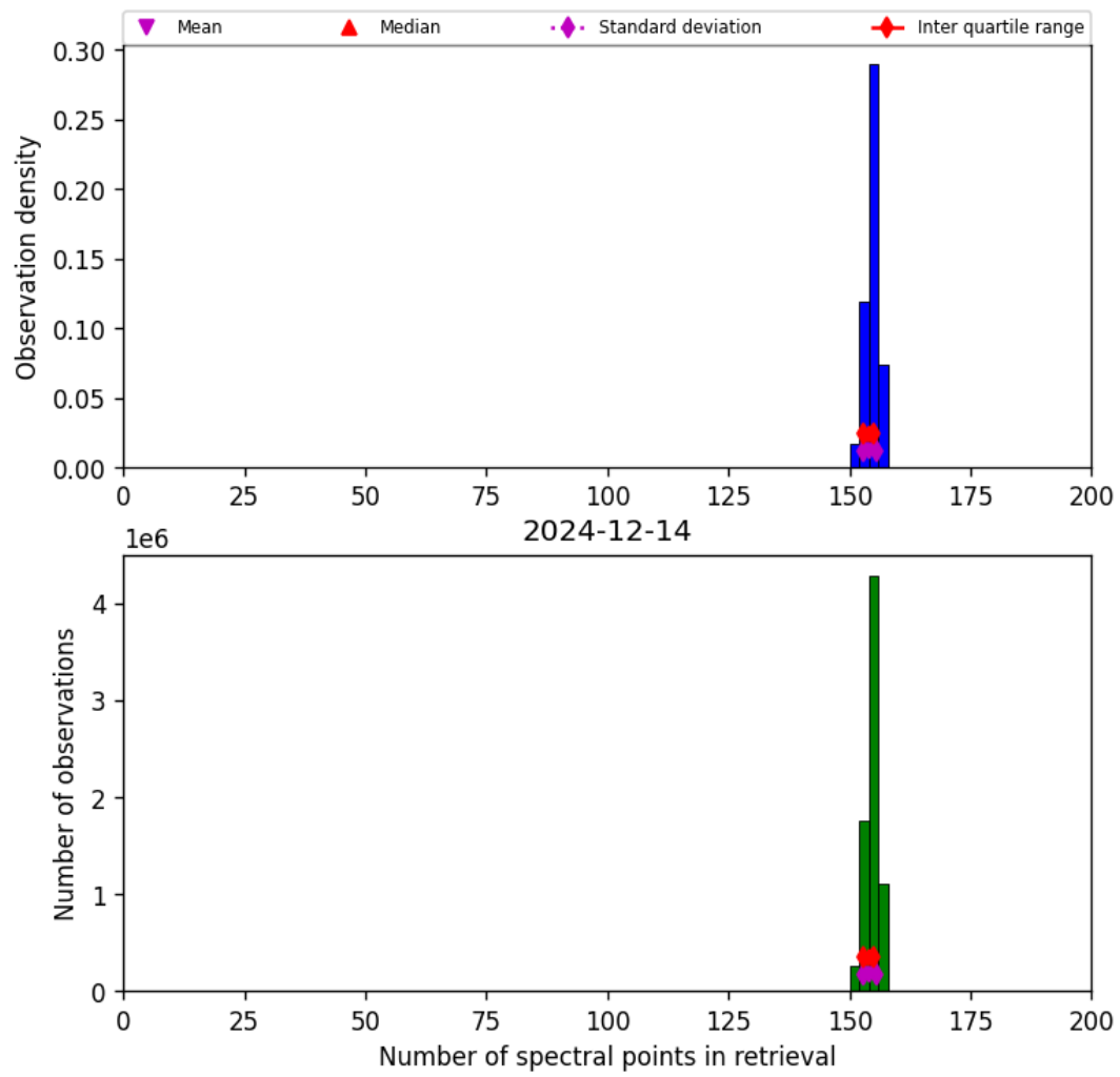
Figure 21: Histogram of “Number of spectral points in retrieval” for 2024-12-13 to 2024-12-15
