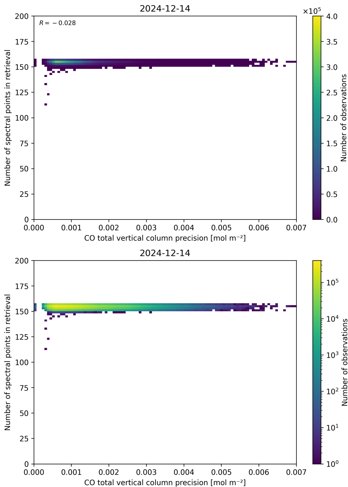
Figure 47: Scatter density plot of “CO total vertical column precision” against “Number of spectral points in retrieval” for 2024-12-13 to 2024-12-15.
