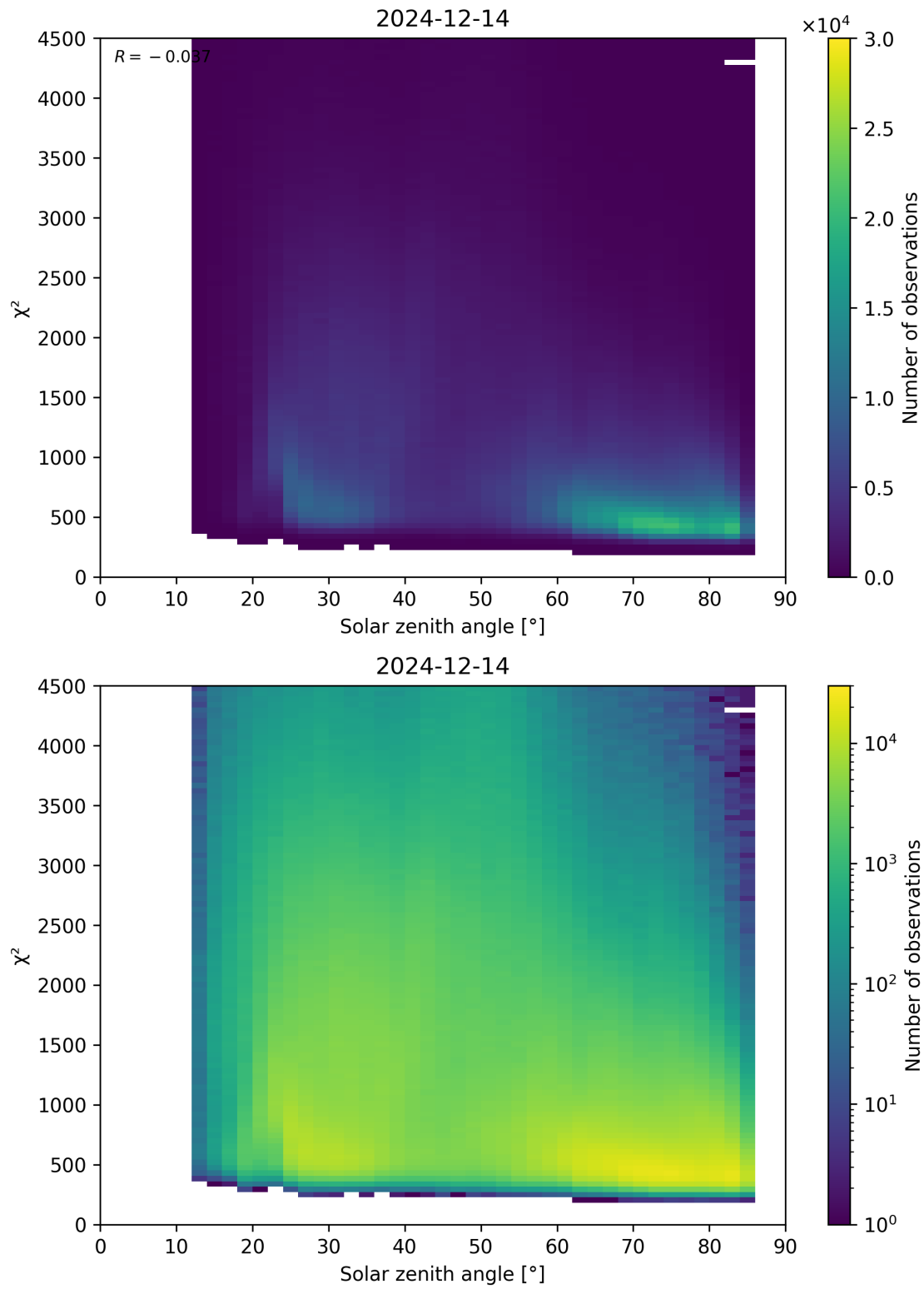
Figure 64: Scatter density plot of “Solar zenith angle” against “ \chi^2 ” for 2024-12-13 to 2024-12-15.
