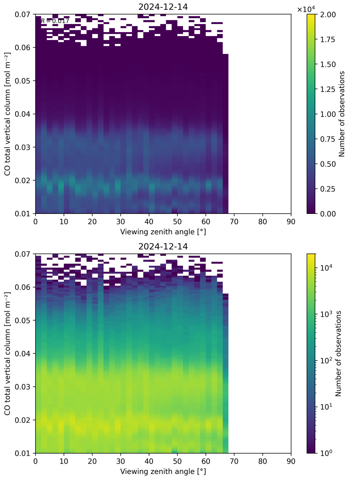
Figure 69: Scatter density plot of “Viewing zenith angle” against “CO total vertical column” for 2024-12-13 to 2024-12-15.
