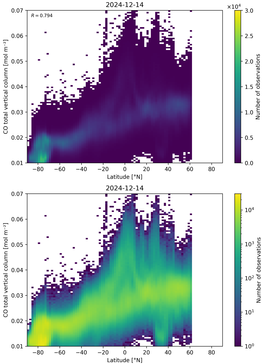
Figure 51: Scatter density plot of “Latitude” against “CO total vertical column” for 2024-12-13 to 2024-12-15.
