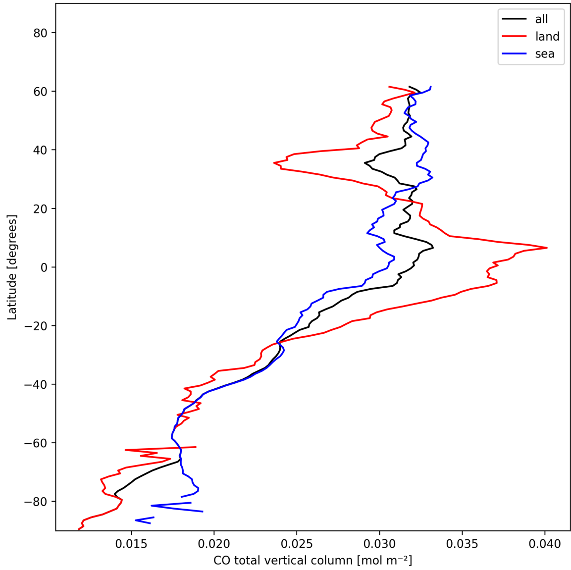
Figure 10: Zonal average of “CO total vertical column” for 2024-12-13 to 2024-12-15.
