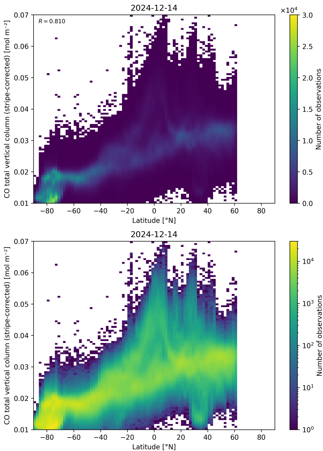
Figure 52: Scatter density plot of “Latitude” against “CO total vertical column (stripe-corrected)” for 2024-12-13 to 2024-12-15.
