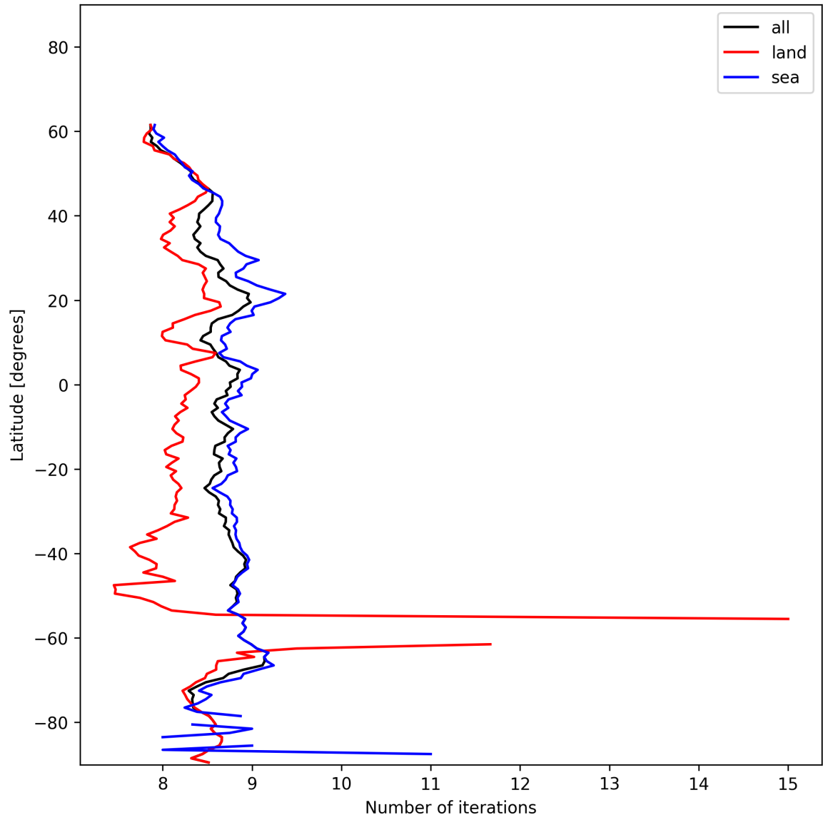
Figure 16: Zonal average of “Number of iterations” for 2024-12-13 to 2024-12-15.
