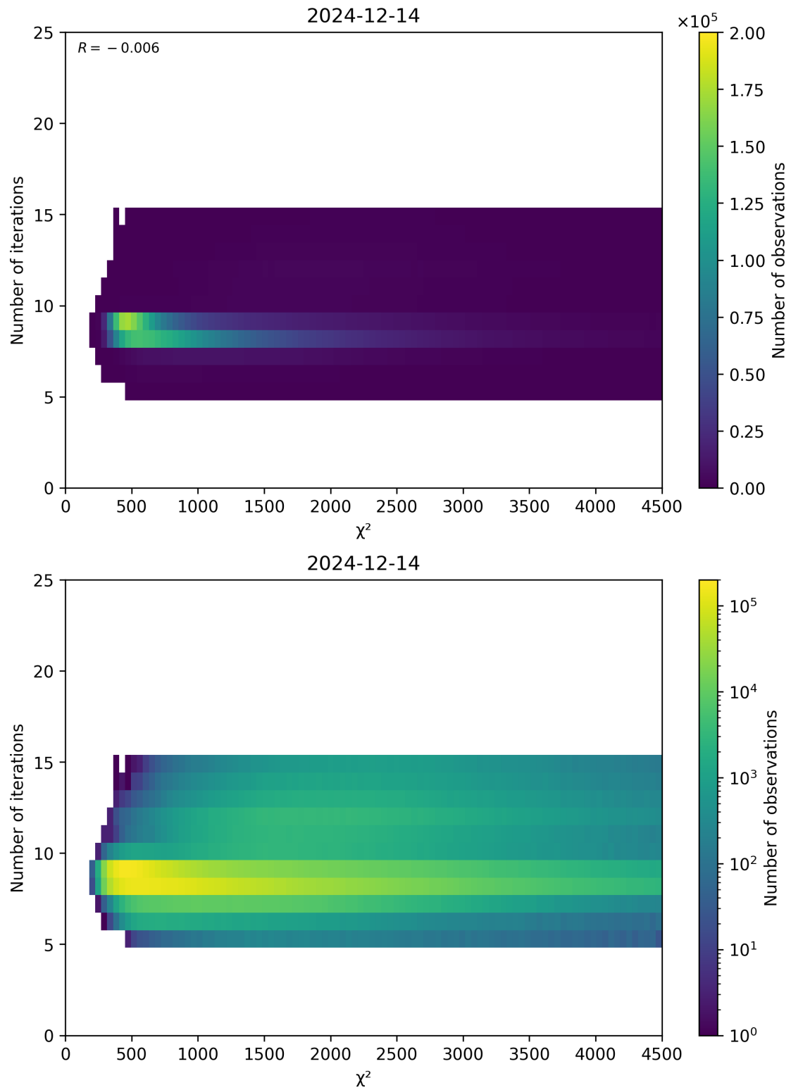
Figure 49: Scatter density plot of “ \chi^2 ” against “Number of iterations” for 2024-12-13 to 2024-12-15.
