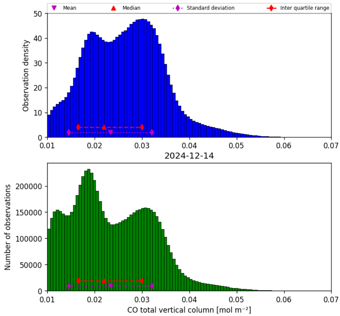
Figure 18: Histogram of “CO total vertical column” for 2024-12-13 to 2024-12-15
