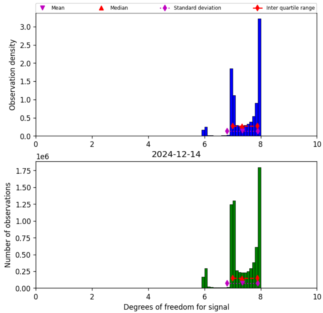
Figure 23: Histogram of “Degrees of freedom for signal” for 2024-12-13 to 2024-12-15
