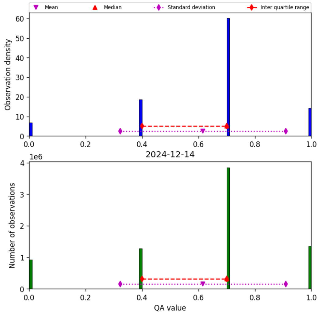
Figure 17: Histogram of “QA value” for 2024-12-13 to 2024-12-15
