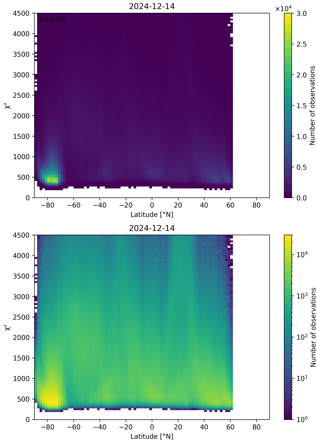
Figure 54: Scatter density plot of “Latitude” against “ \chi^2 ” for 2024-12-13 to 2024-12-15.
