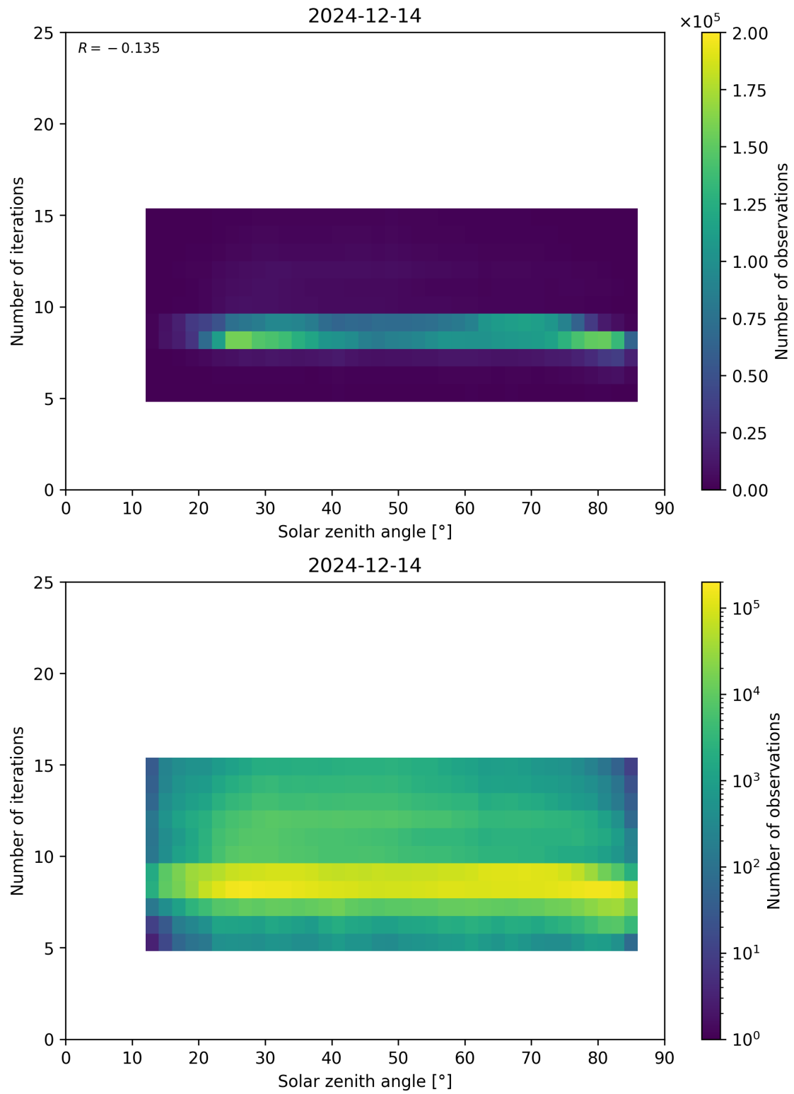
Figure 67: Scatter density plot of “Solar zenith angle” against “Number of iterations” for 2024-12-13 to 2024-12-15.
