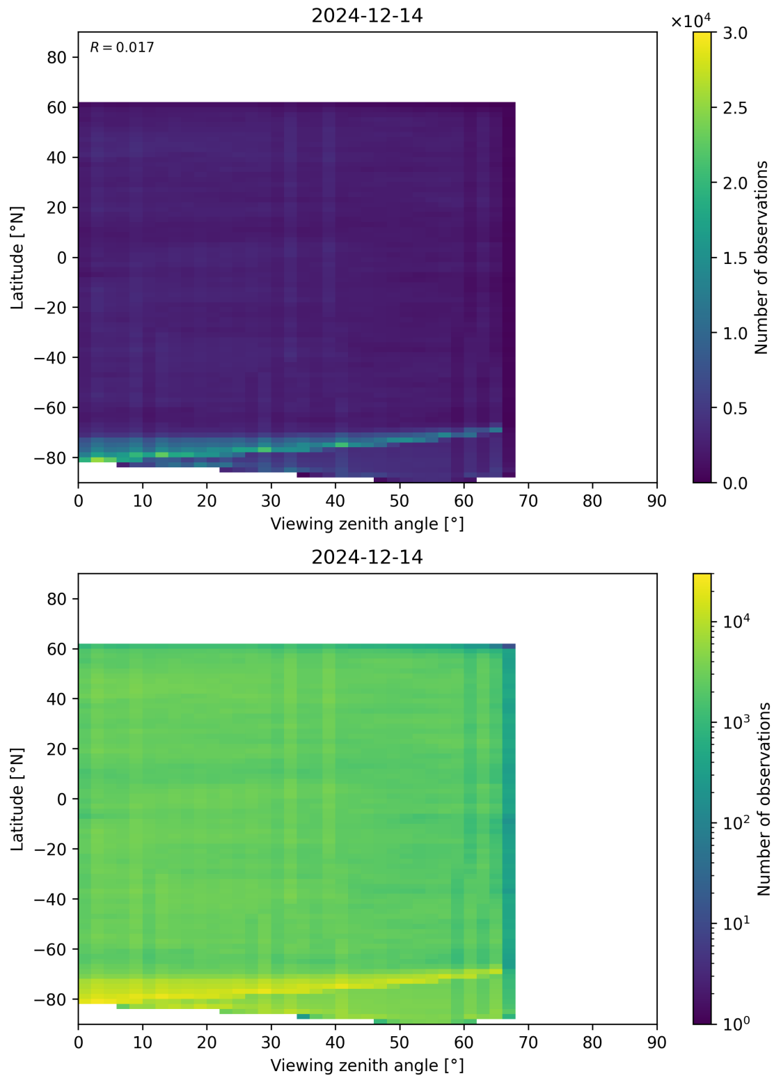
Figure 74: Scatter density plot of “Viewing zenith angle” against “Latitude” for 2024-12-13 to 2024-12-15.
