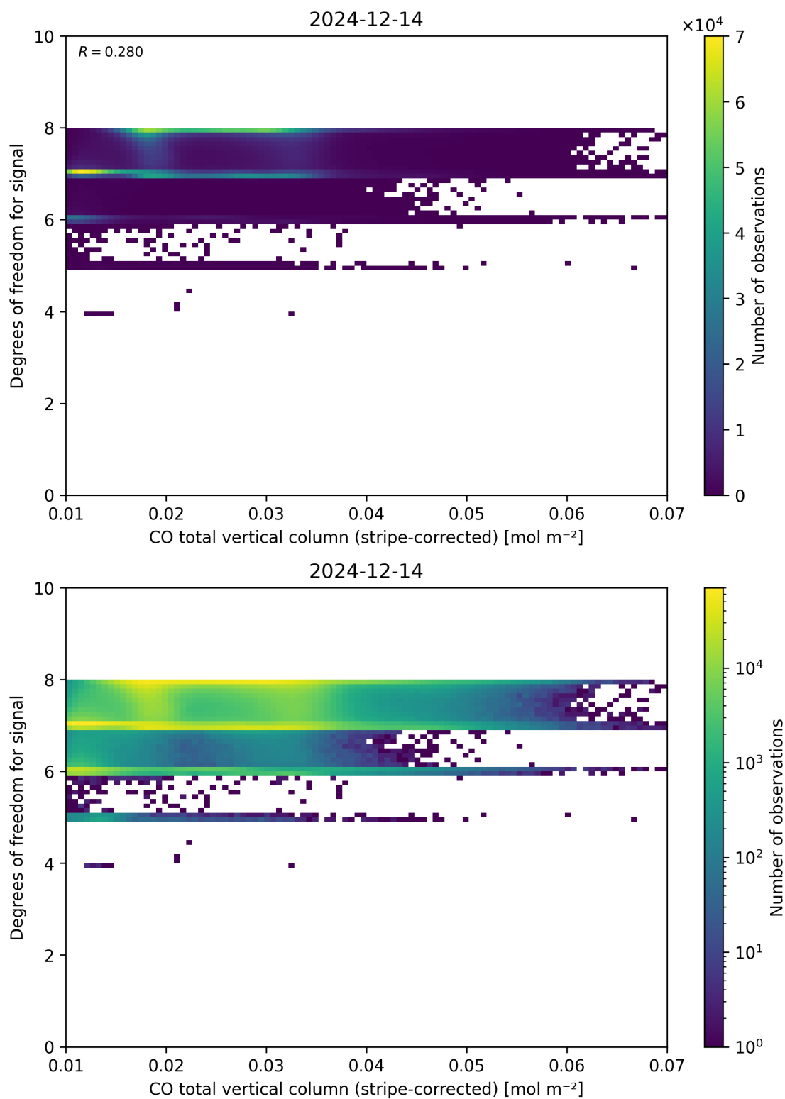
Figure 38: Scatter density plot of “CO total vertical column (stripe-corrected)” against “Degrees of freedom for signal” for 2024-12-13 to 2024-12-15.
