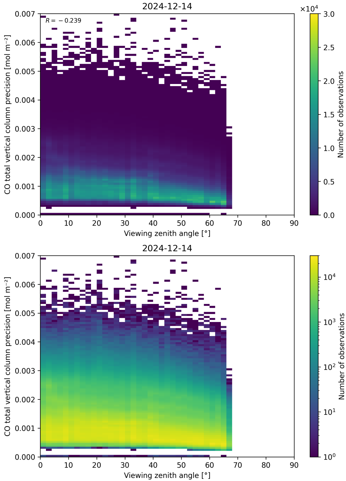
Figure 71: Scatter density plot of “Viewing zenith angle” against “CO total vertical column precision” for 2024-12-13 to 2024-12-15.
