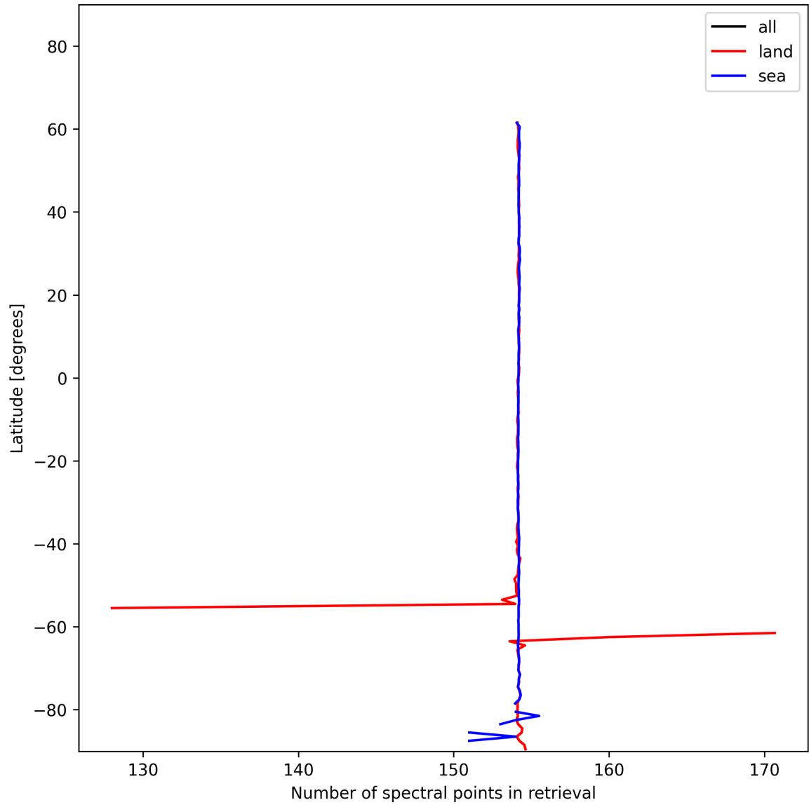
Figure 13: Zonal average of “Number of spectral points in retrieval” for 2024-12-13 to 2024-12-15.
