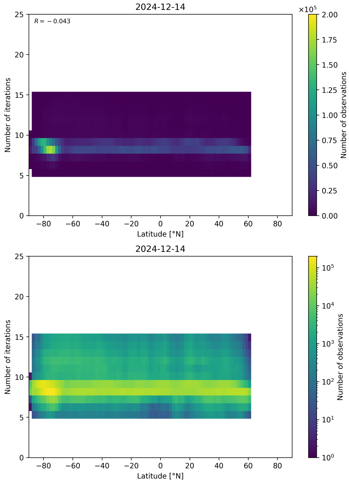
Figure 56: Scatter density plot of “Latitude” against “Number of iterations” for 2024-12-13 to 2024-12-15.
