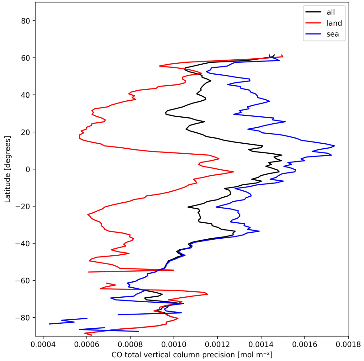
Figure 12: Zonal average of "CO total vertical column precision" for 2024-12-13 to 2024-12-15.
