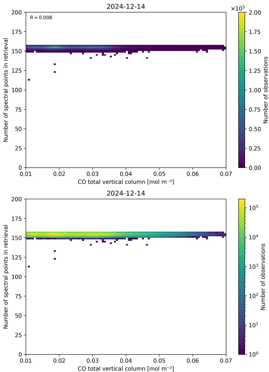
Figure 43: Scatter density plot of “CO total vertical column” against “Number of spectral points in retrieval” for 2024-12-13 to 2024-12-15.
