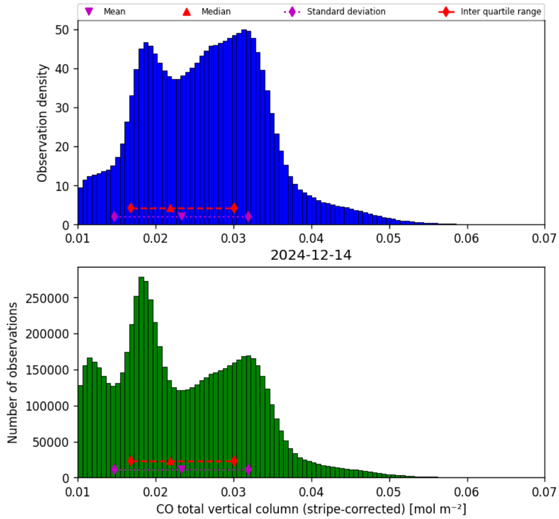
Figure 19: Histogram of “CO total vertical column (stripe-corrected)” for 2024-12-13 to 2024-12-15
