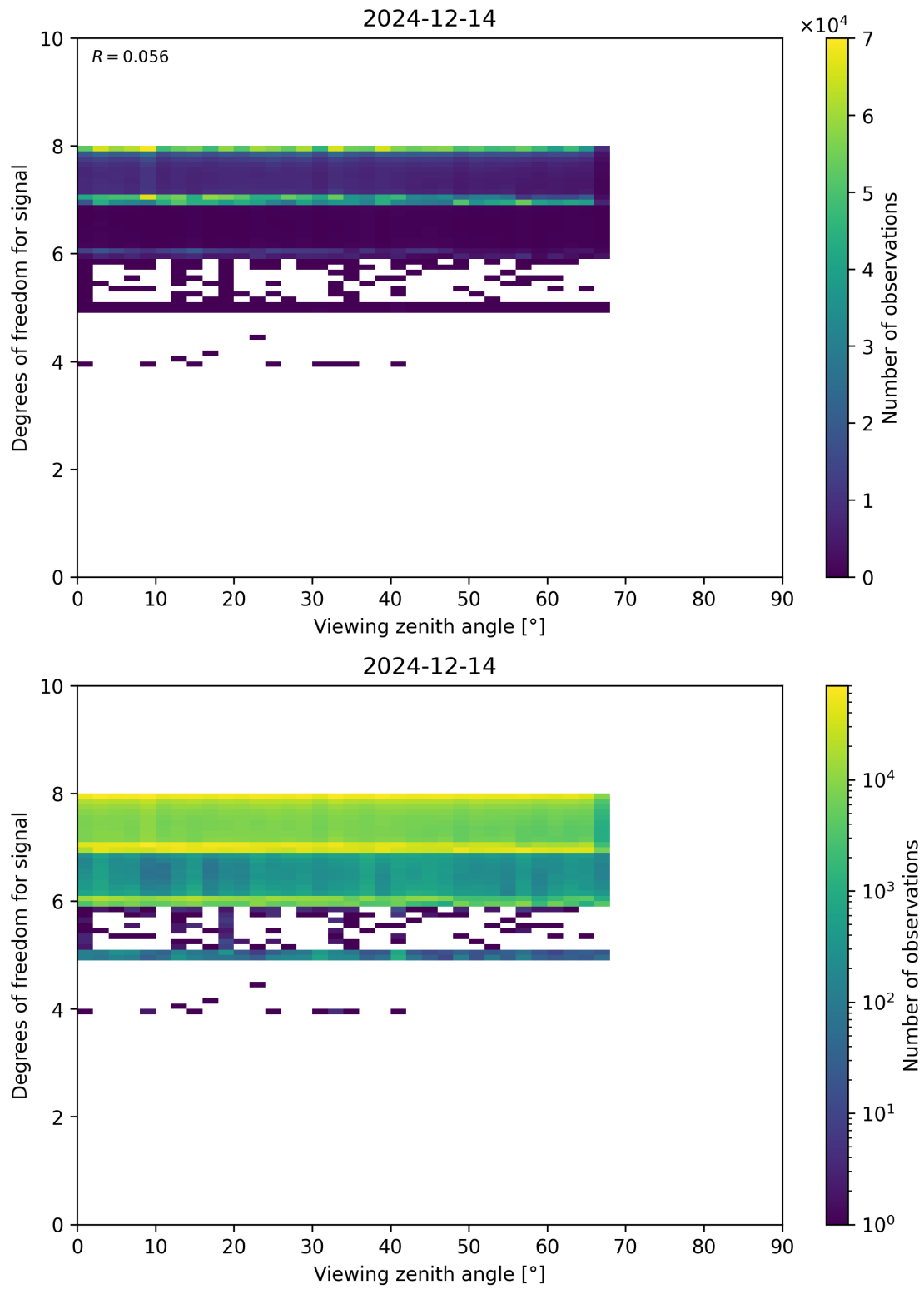
Figure 73: Scatter density plot of “Viewing zenith angle” against “Degrees of freedom for signal” for 2024-12-13 to 2024-12-15.
