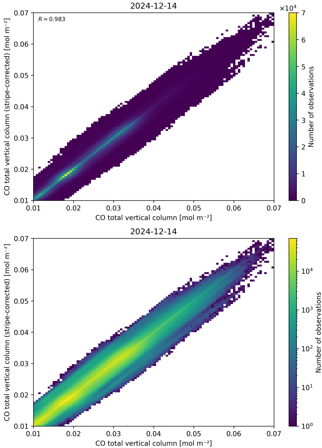
Figure 33: Scatter density plot of “CO total vertical column” against “CO total vertical column (stripe-corrected)” for 2024-12-13 to 2024-12-15.
