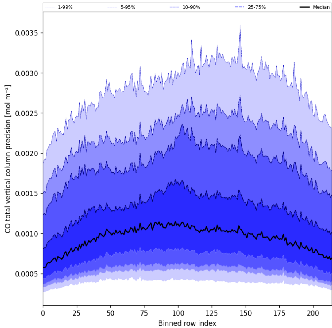
Figure 28: Along track statistics of “CO total vertical column precision” for 2024-12-13 to 2024-12-15
