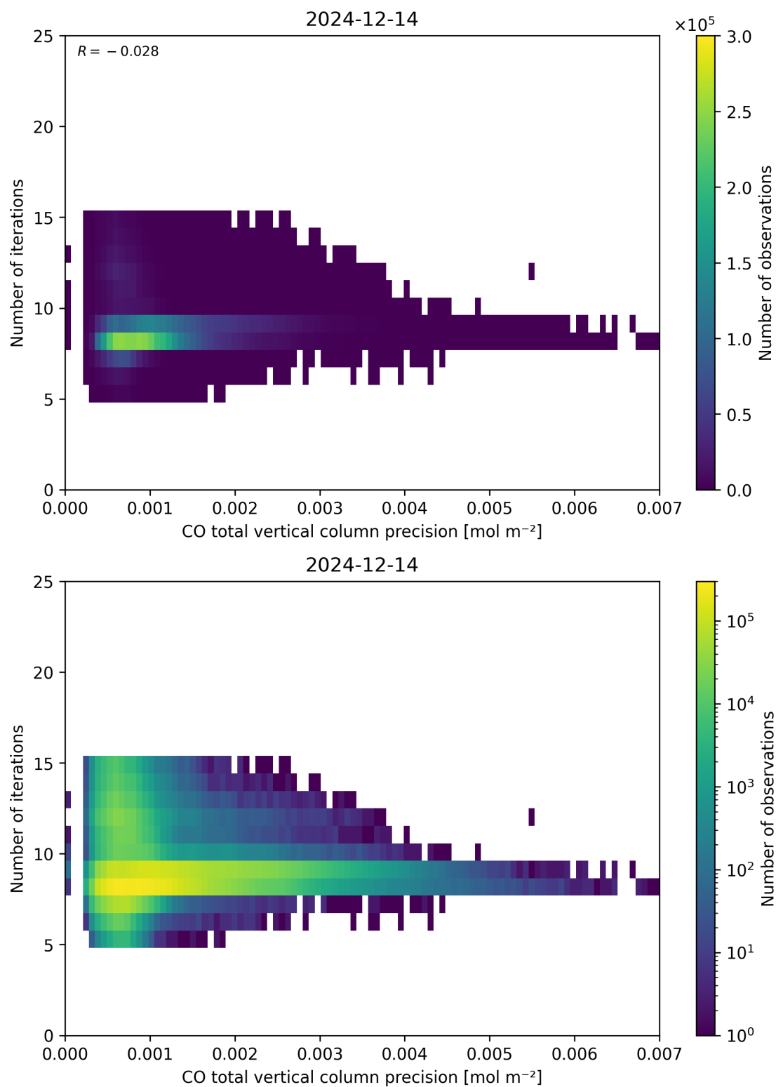
Figure 46: Scatter density plot of “CO total vertical column precision” against “Number of iterations” for 2024-12-13 to 2024-12-15.
