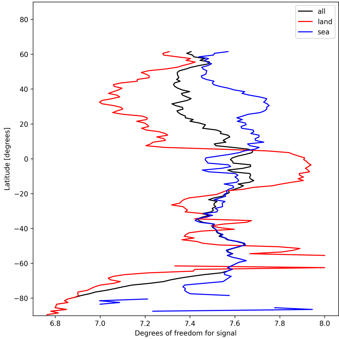
Figure 15: Zonal average of “Degrees of freedom for signal” for 2024-12-13 to 2024-12-15.
