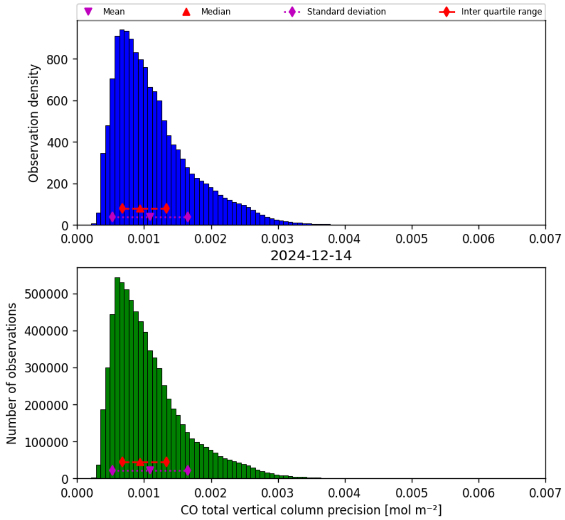
Figure 20: Histogram of “CO total vertical column precision” for 2024-12-13 to 2024-12-15
