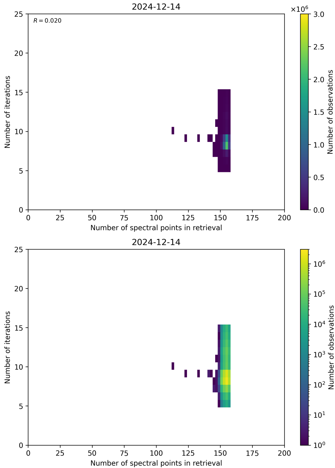
Figure 60: Scatter density plot of “Number of spectral points in retrieval” against “Number of iterations” for 2024-12-13 to 2024-12-15.
