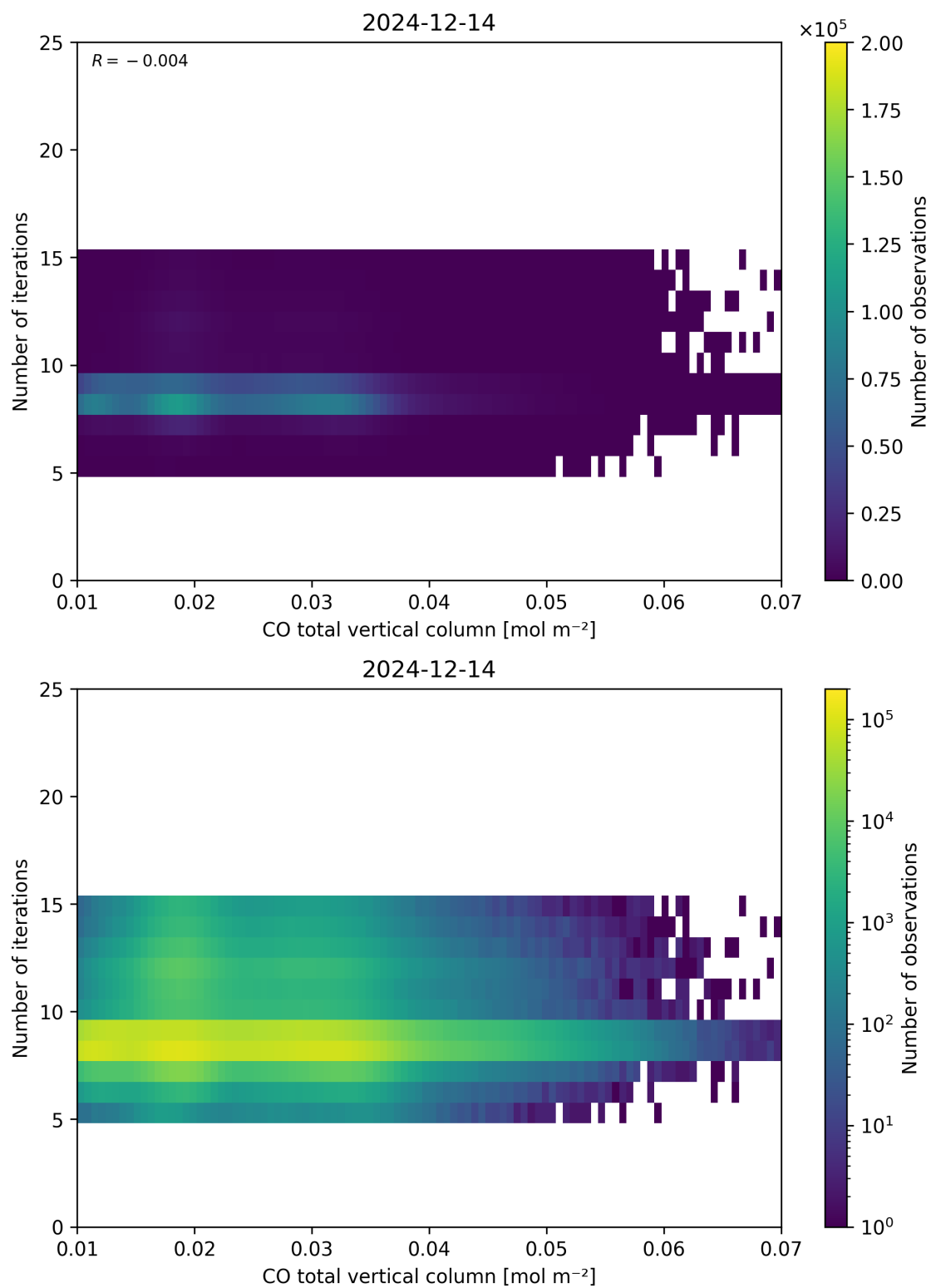
Figure 42: Scatter density plot of “CO total vertical column” against “Number of iterations” for 2024-12-13 to 2024-12-15.
