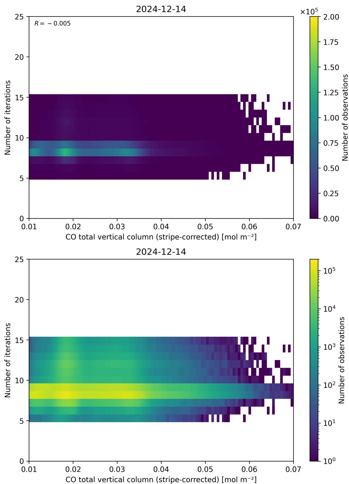
Figure 39: Scatter density plot of “CO total vertical column (stripe-corrected)” against “Number of iterations” for 2024-12-13 to 2024-12-15.
