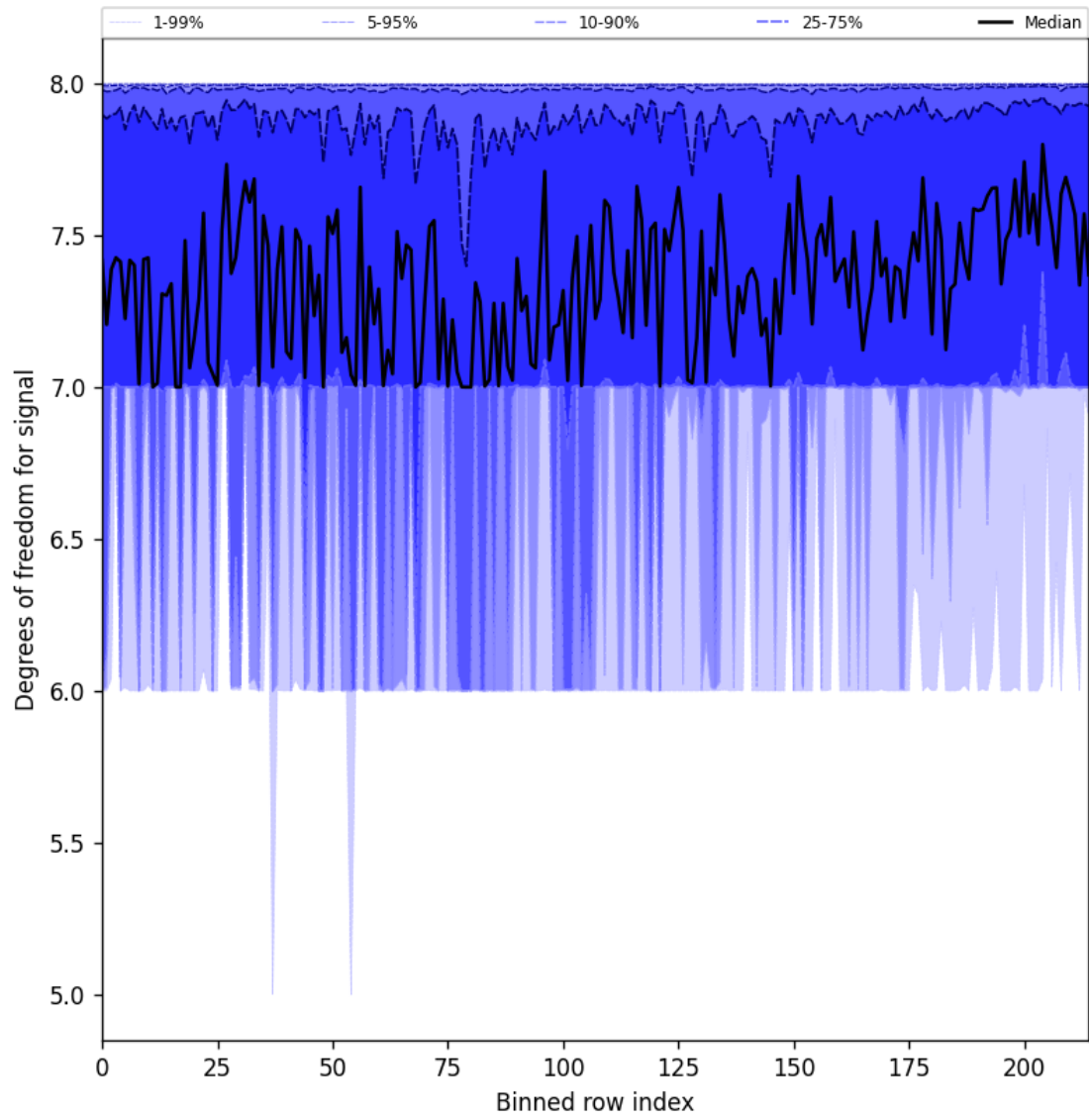
Figure 31: Along track statistics of “Degrees of freedom for signal” for 2024-12-13 to 2024-12-15
