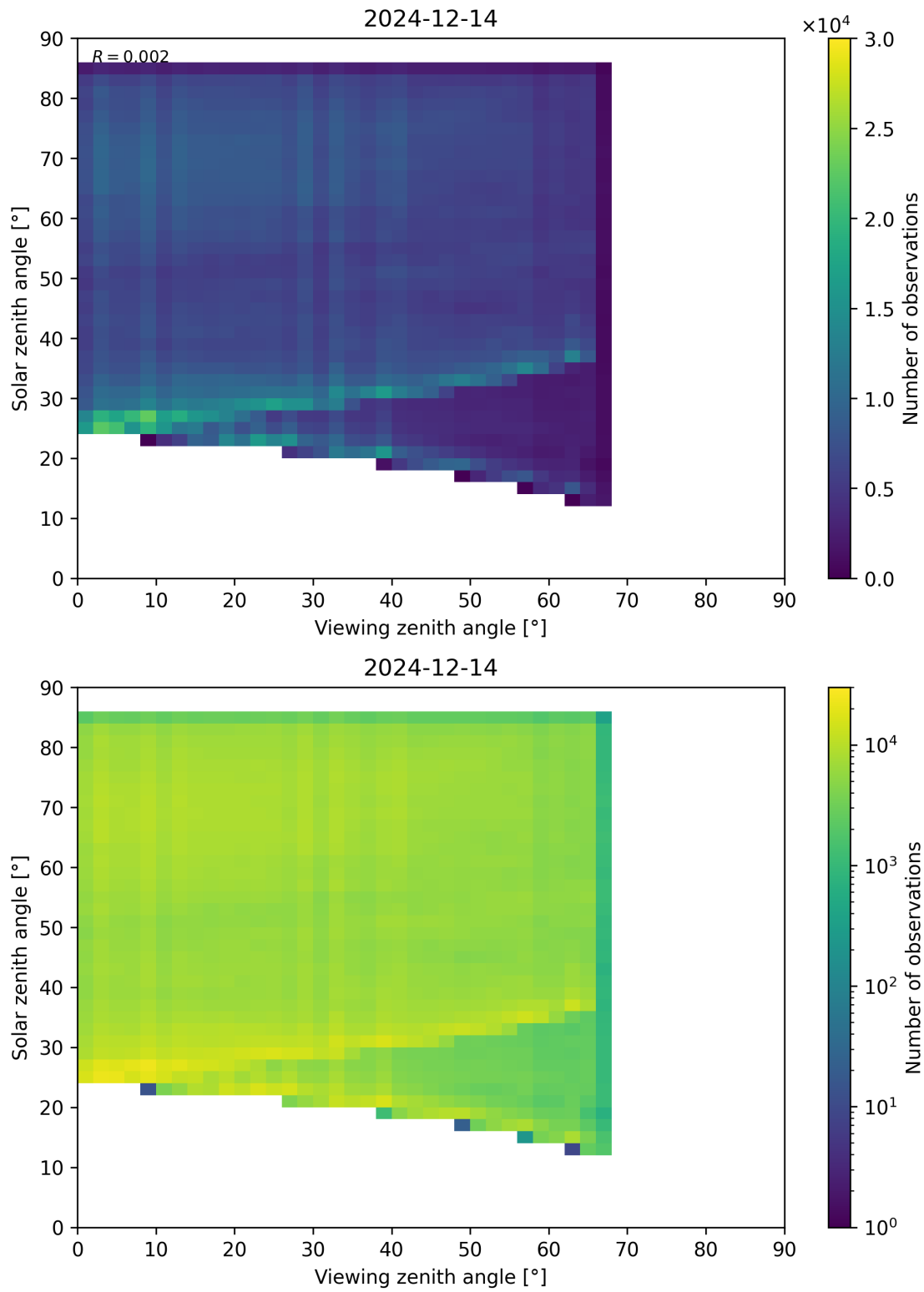
Figure 77: Scatter density plot of “Viewing zenith angle” against “Solar zenith angle” for 2024-12-13 to 2024-12-15.
