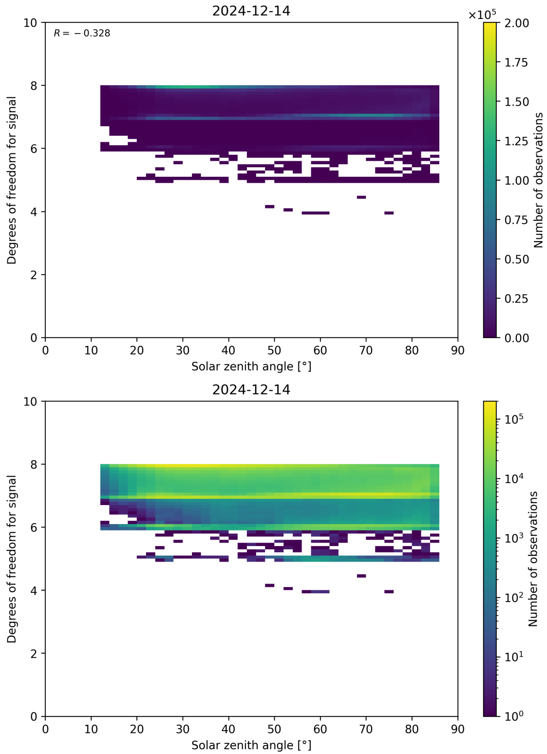
Figure 65: Scatter density plot of “Solar zenith angle” against “Degrees of freedom for signal” for 2024-12-13 to 2024-12-15.
