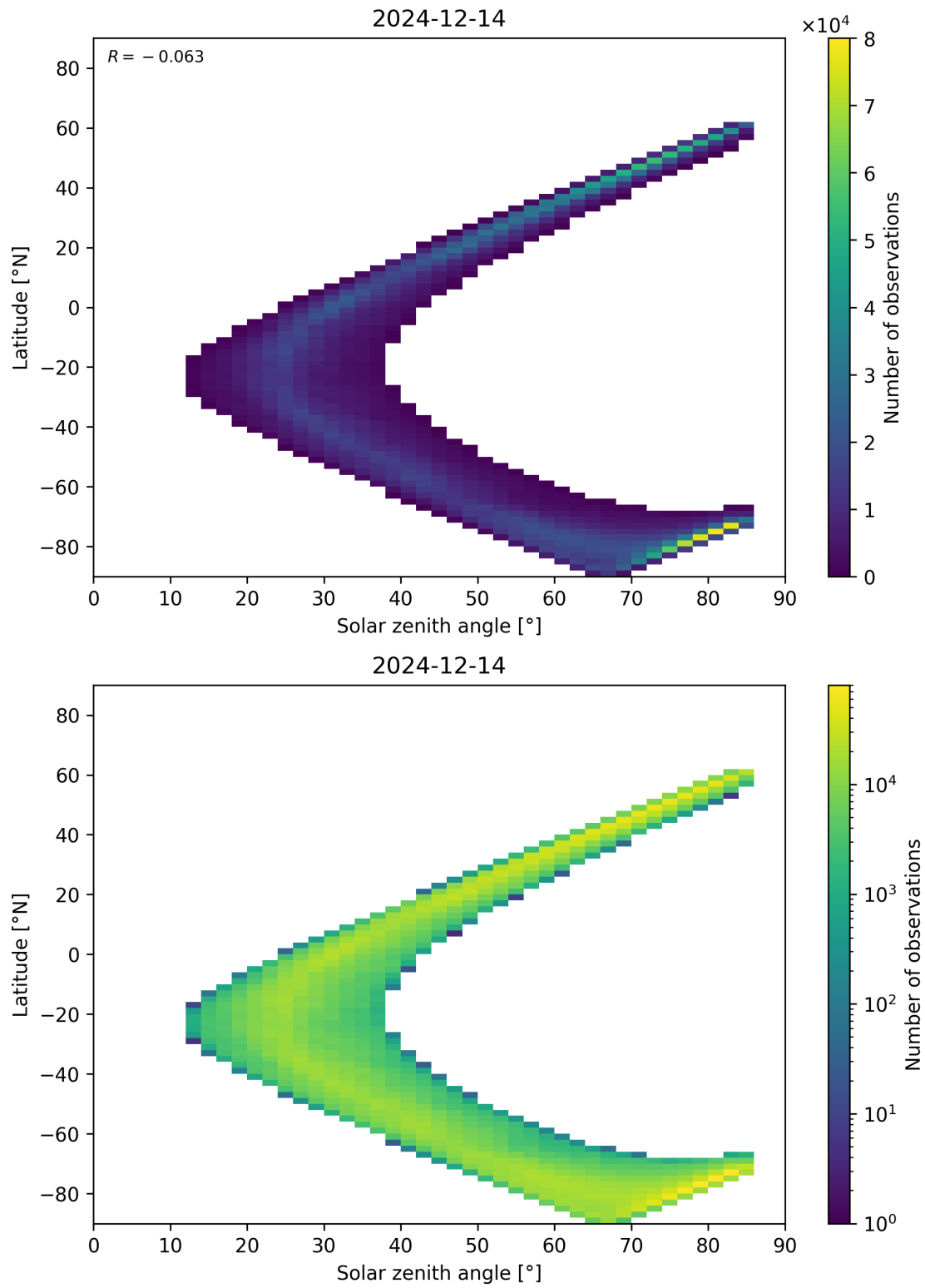
Figure 66: Scatter density plot of “Solar zenith angle” against “Latitude” for 2024-12-13 to 2024-12-15.
