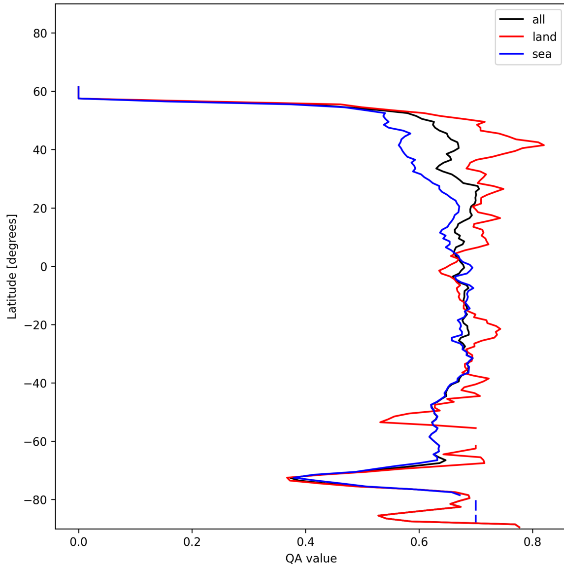
Figure 9: Zonal average of “QA value” for 2024-12-13 to 2024-12-15.
