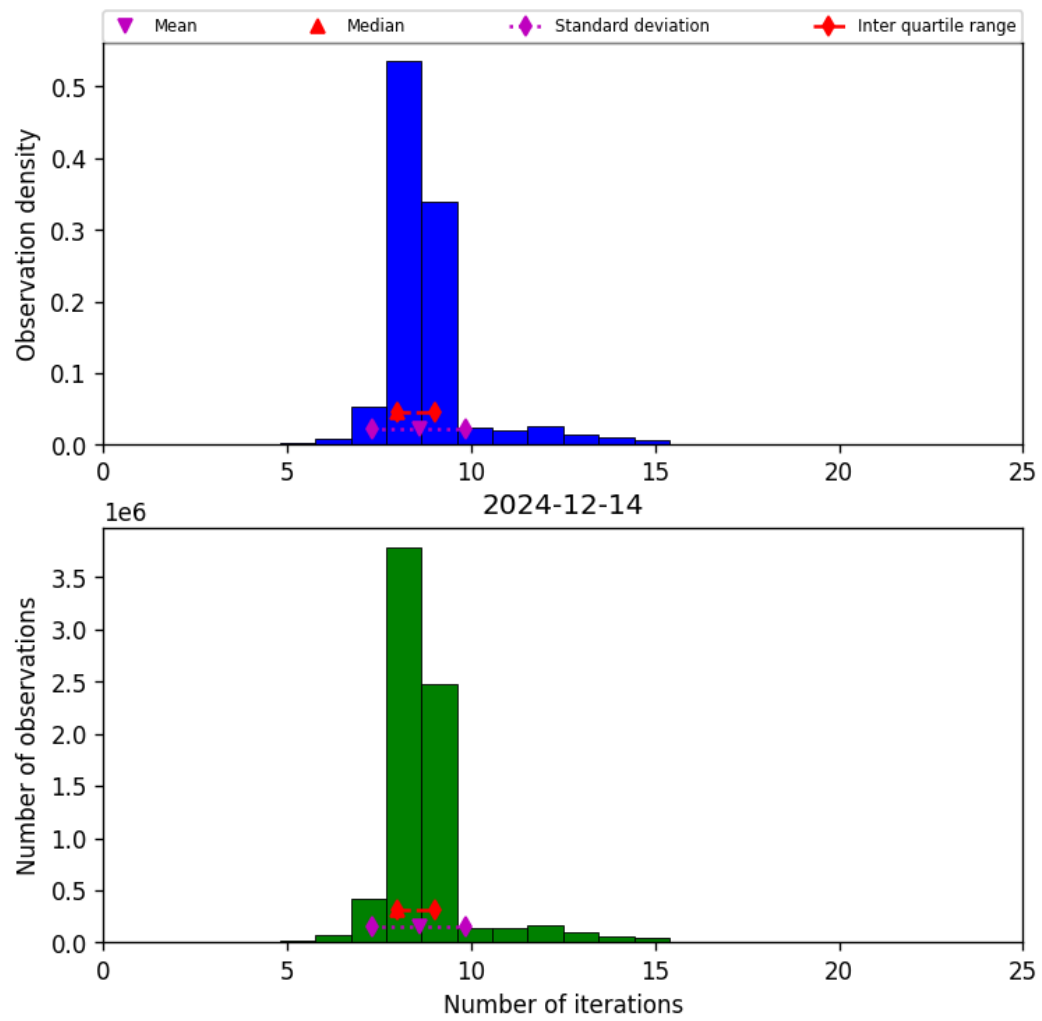
Figure 24: Histogram of “Number of iterations” for 2024-12-13 to 2024-12-15
