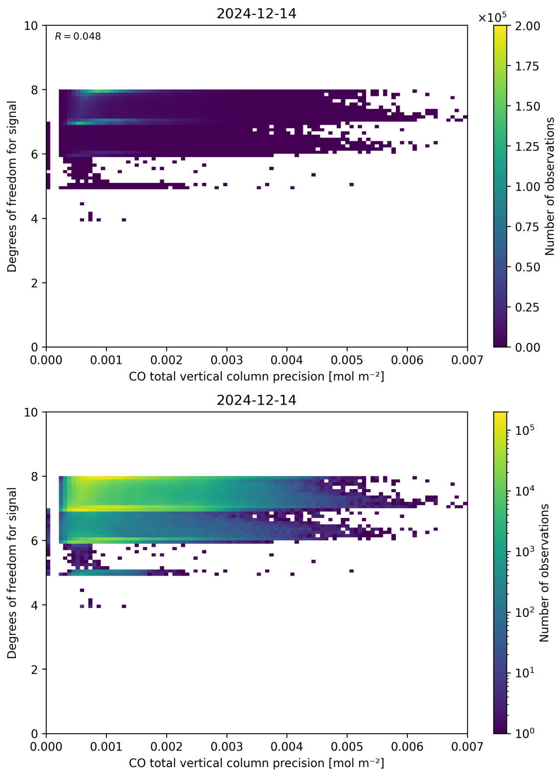
Figure 45: Scatter density plot of “CO total vertical column precision” against “Degrees of freedom for signal” for 2024-12-13 to 2024-12-15.
