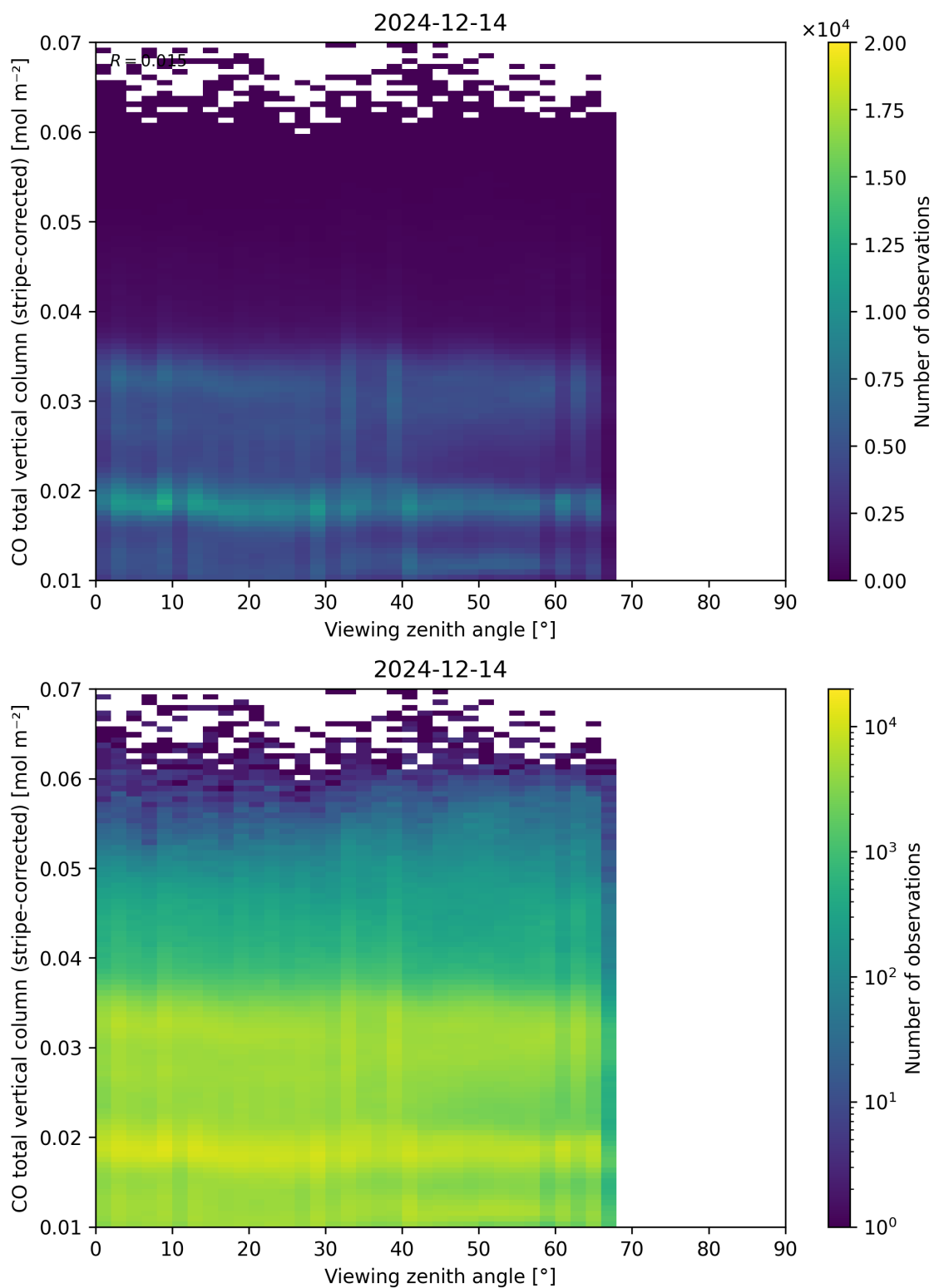
Figure 70: Scatter density plot of “Viewing zenith angle” against “CO total vertical column (stripe-corrected)” for 2024-12-13 to 2024-12-15.
