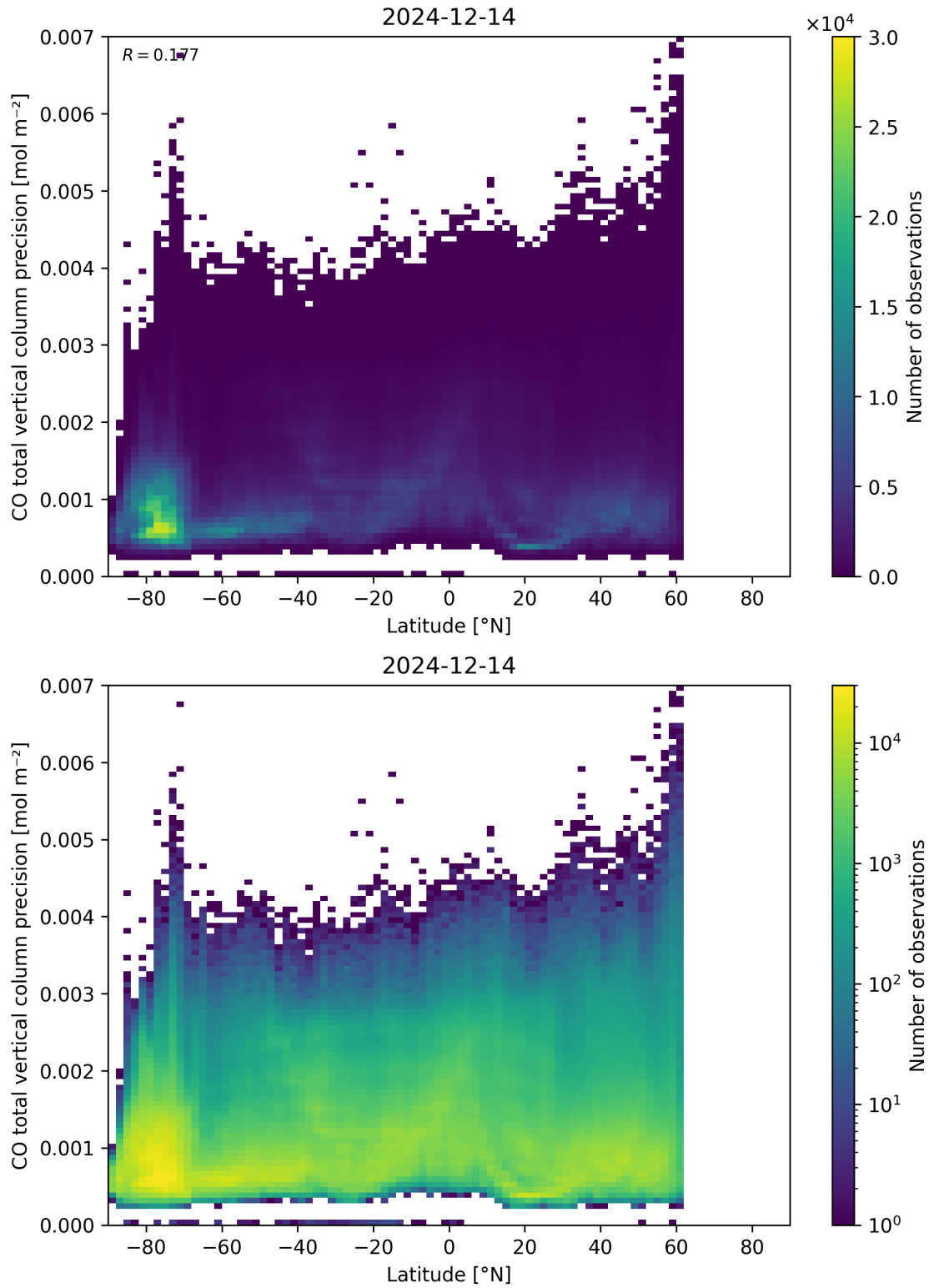
Figure 53: Scatter density plot of “Latitude” against “CO total vertical column precision” for 2024-12-13 to 2024-12-15.
