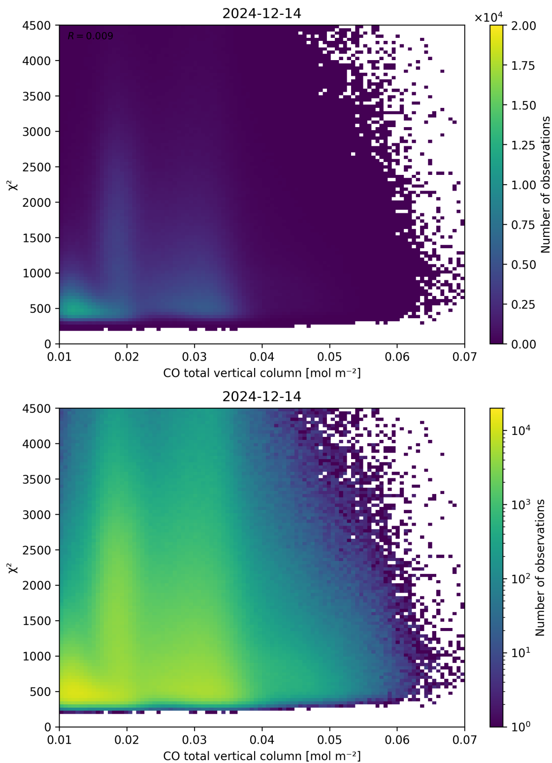
Figure 35: Scatter density plot of “CO total vertical column” against “ \chi^2 ” for 2024-12-13 to 2024-12-15.
