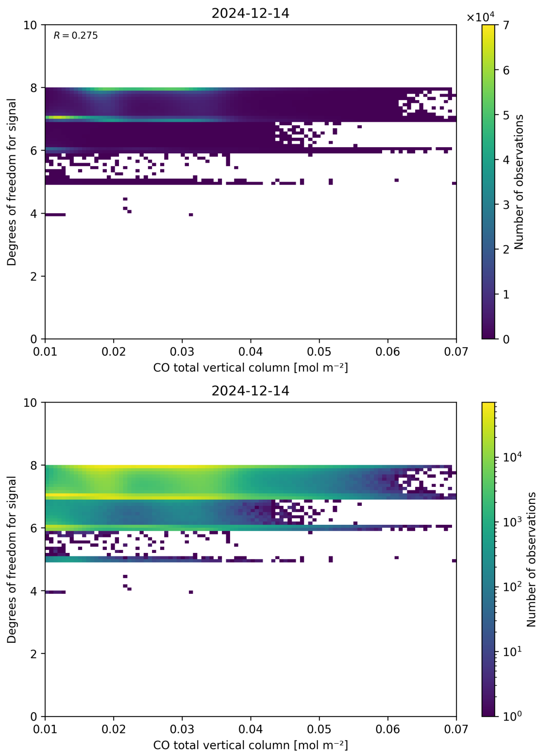
Figure 41: Scatter density plot of “CO total vertical column” against “Degrees of freedom for signal” for 2024-12-13 to 2024-12-15.
