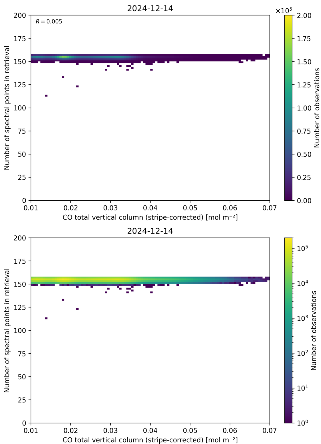
Figure 40: Scatter density plot of “CO total vertical column (stripe-corrected)” against “Number of spectral points in retrieval” for 2024-12-13 to 2024-12-15.
