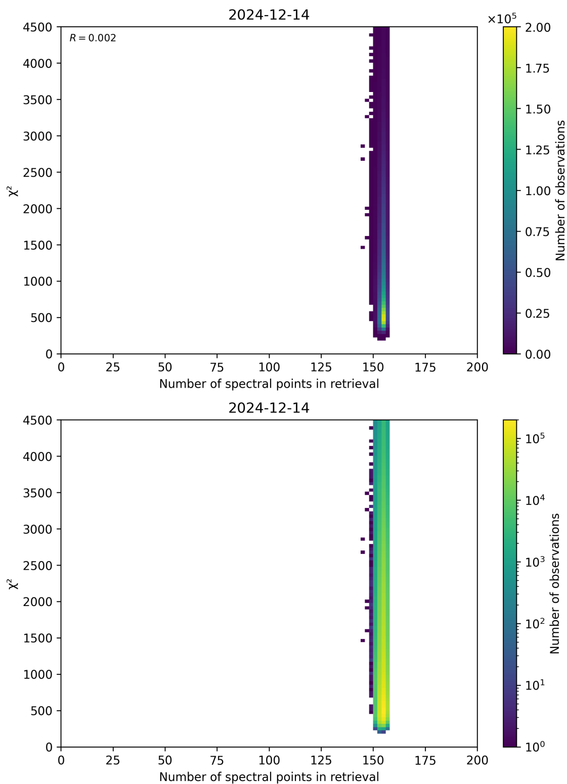
Figure 58: Scatter density plot of “Number of spectral points in retrieval” against “ \chi^2 ” for 2024-12-13 to 2024-12-15.
