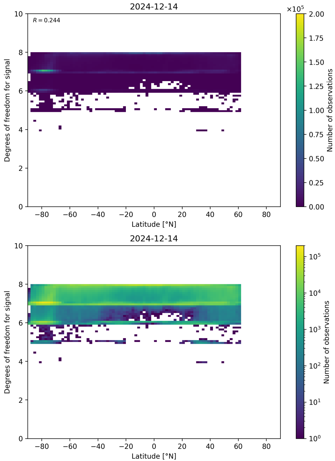
Figure 55: Scatter density plot of “Latitude” against “Degrees of freedom for signal” for 2024-12-13 to 2024-12-15.
