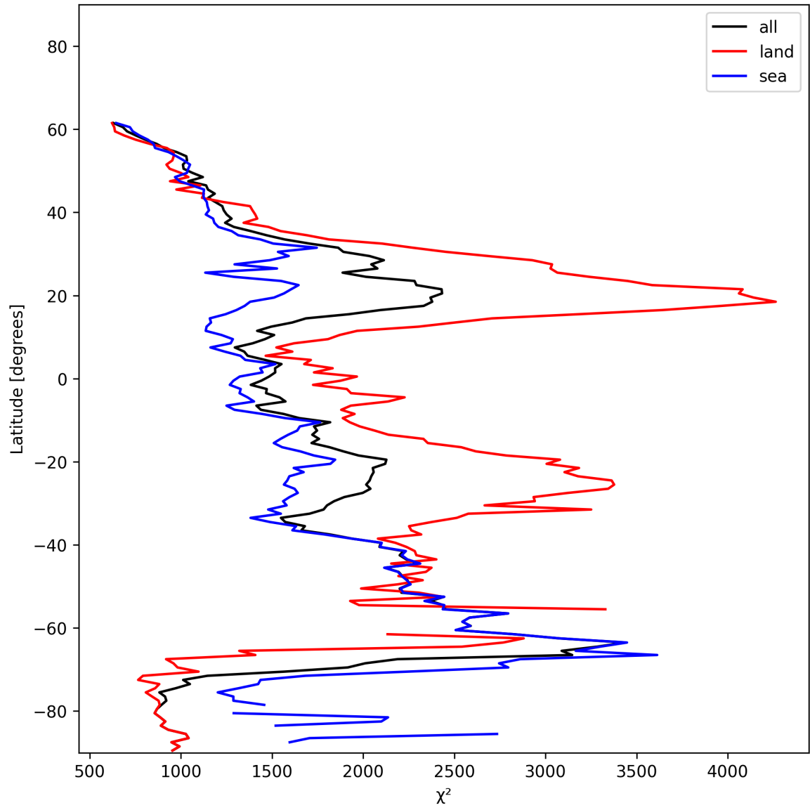
Figure 14: Zonal average of “ \chi^2 ” for 2024-12-13 to 2024-12-15.
