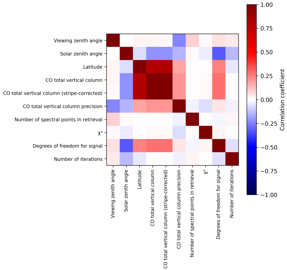
Figure 2: Map of correlation matrix for 2024-12-13 to 2024-12-15.
