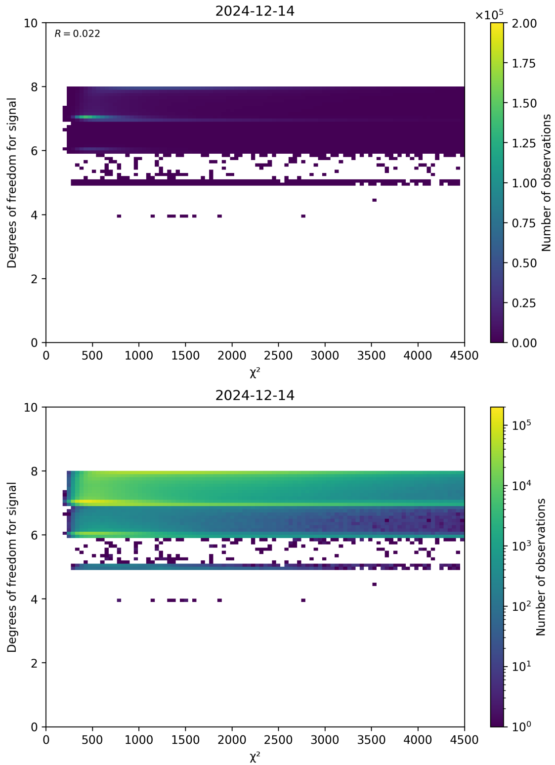
Figure 48: Scatter density plot of “ \chi^2 ” against “Degrees of freedom for signal” for 2024-12-13 to 2024-12-15.
