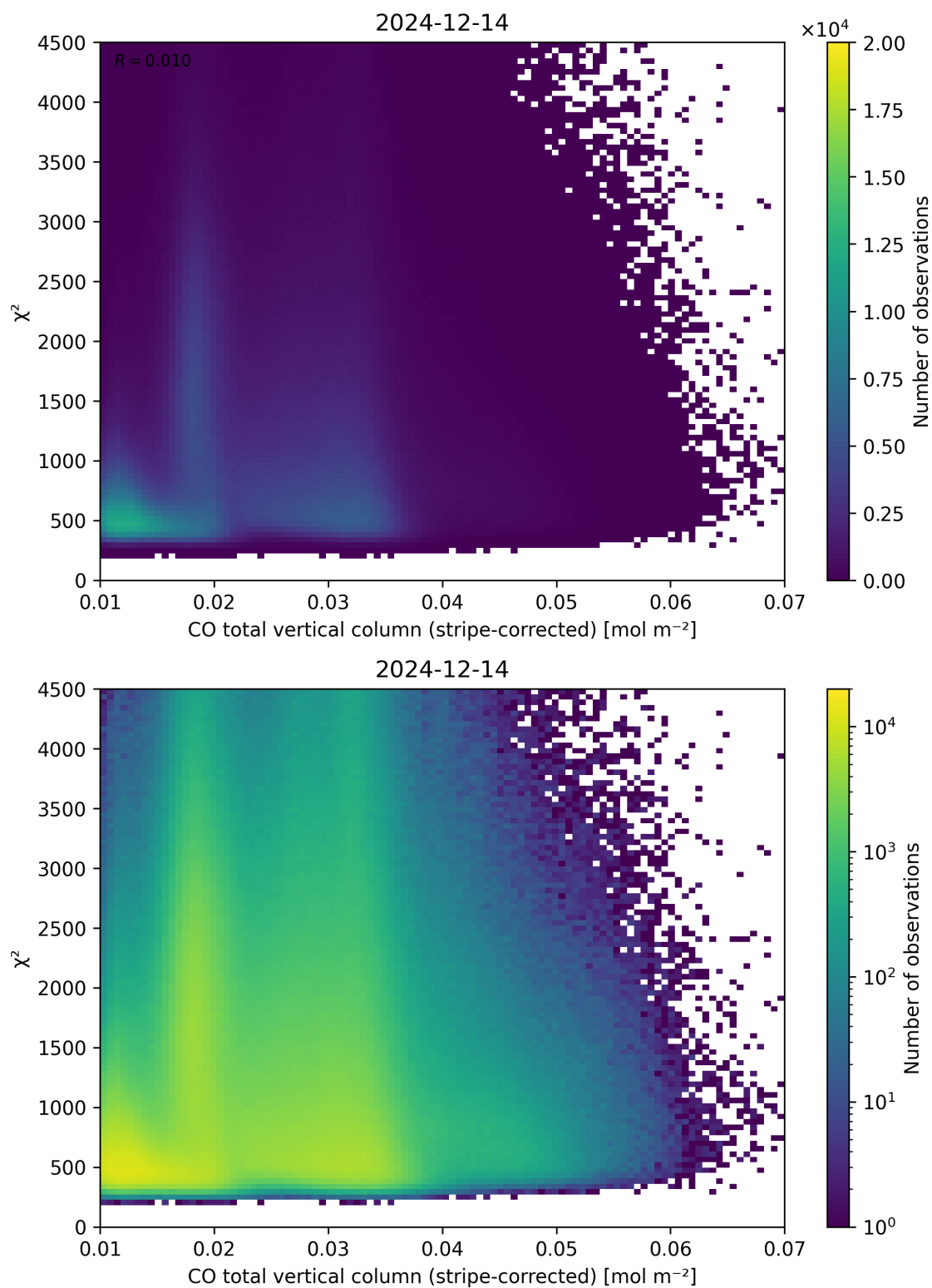
Figure 37: Scatter density plot of “CO total vertical column (stripe-corrected)” against “ \chi^2 ” for 2024-12-13 to 2024-12-15.
