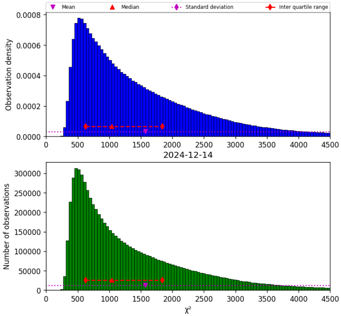
Figure 22: Histogram of “ \chi^2 ” for 2024-12-13 to 2024-12-15
