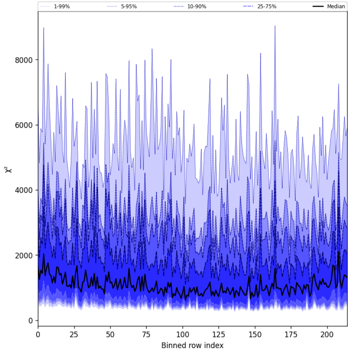
Figure 30: Along track statistics of “ \chi^2 ” for 2024-12-13 to 2024-12-15
