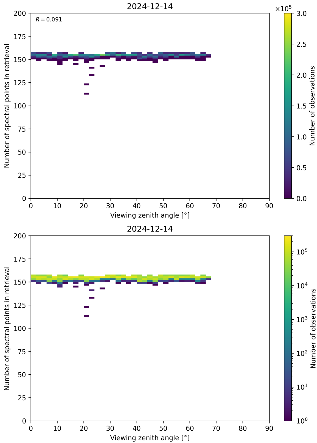
Figure 76: Scatter density plot of “Viewing zenith angle” against “Number of spectral points in retrieval” for 2024-12-13 to 2024-12-15.
