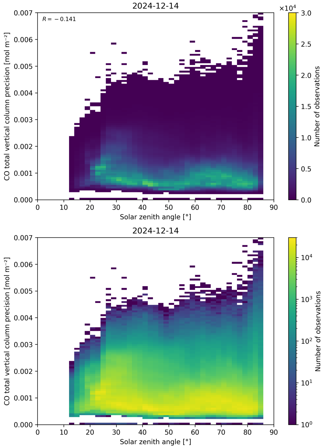
Figure 63: Scatter density plot of “Solar zenith angle” against “CO total vertical column precision” for 2024-12-13 to 2024-12-15.
