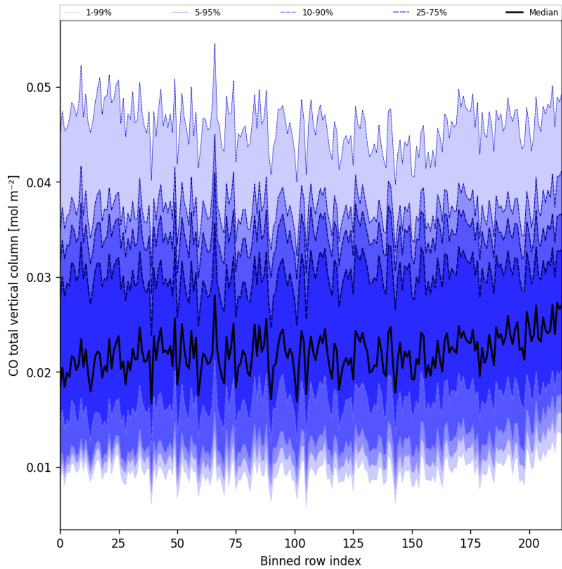
Figure 26: Along track statistics of “CO total vertical column” for 2024-12-13 to 2024-12-15
