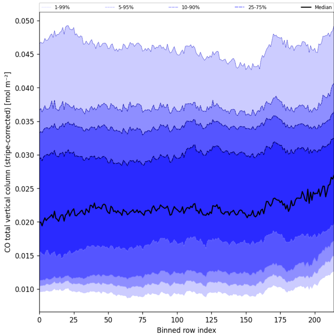
Figure 27: Along track statistics of “CO total vertical column (stripe-corrected)” for 2024-12-13 to 2024-12-15
