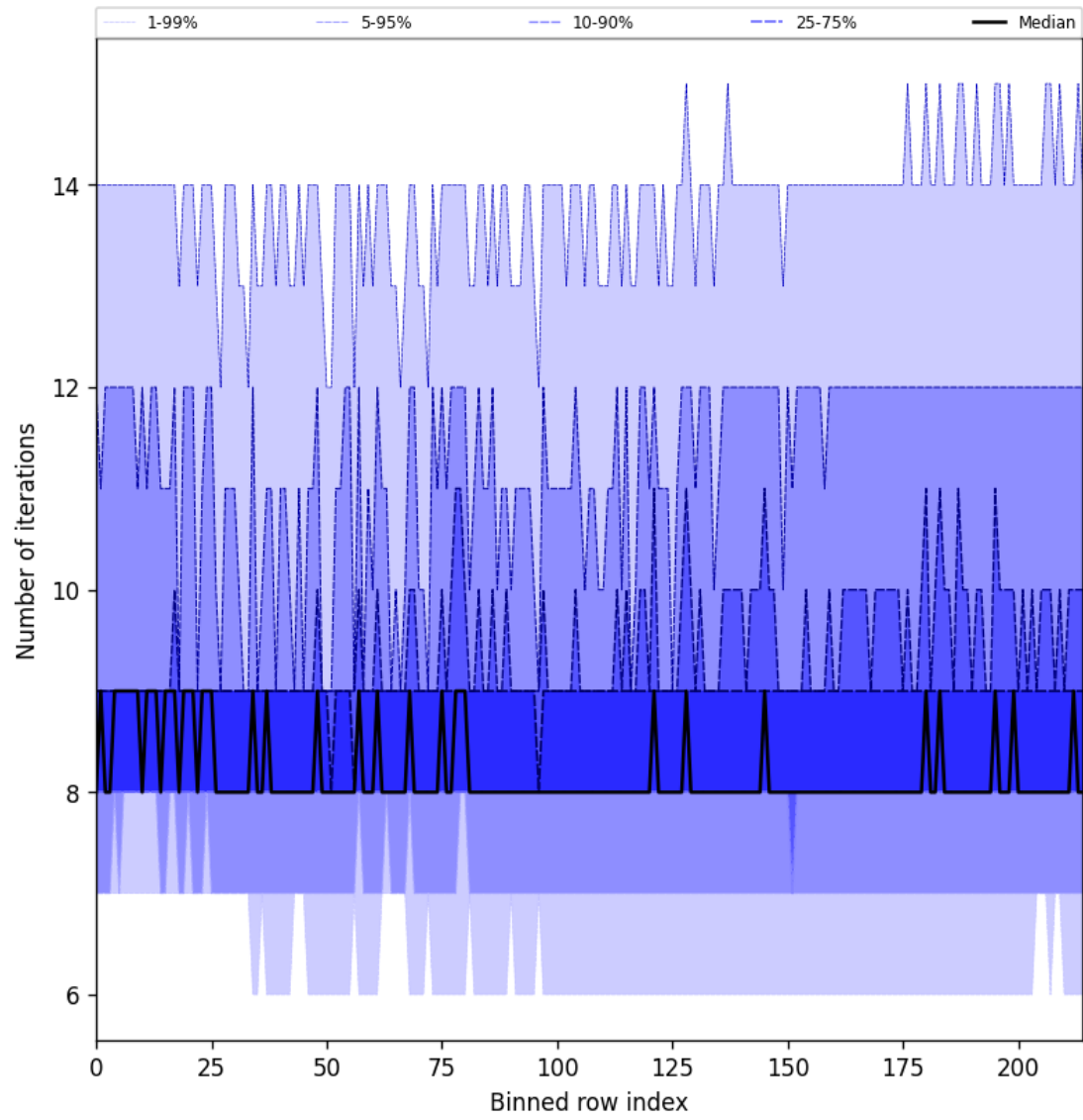
Figure 32: Along track statistics of “Number of iterations” for 2024-12-13 to 2024-12-15
