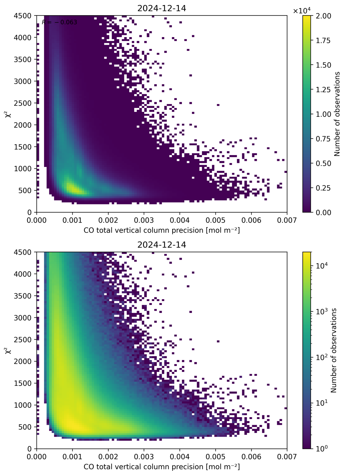
Figure 44: Scatter density plot of “CO total vertical column precision” against “ \chi^2 ” for 2024-12-13 to 2024-12-15.
