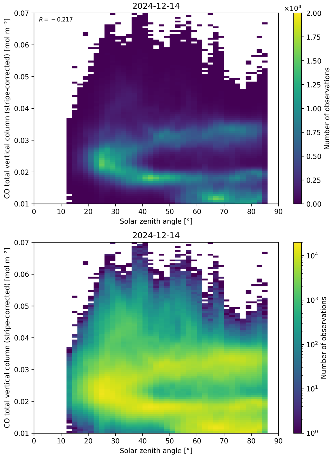
Figure 62: Scatter density plot of “Solar zenith angle” against “CO total vertical column (stripe-corrected)” for 2024-12-13 to 2024-12-15.
