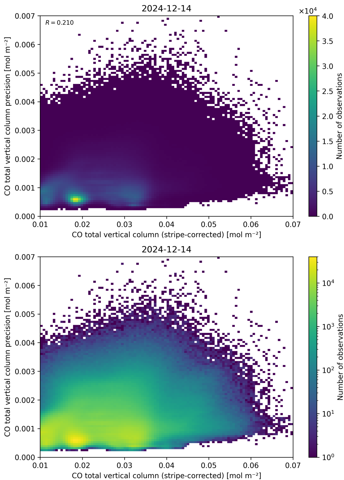
Figure 36: Scatter density plot of “CO total vertical column (stripe-corrected)” against “CO total vertical column precision” for 2024-12-13 to 2024-12-15.
