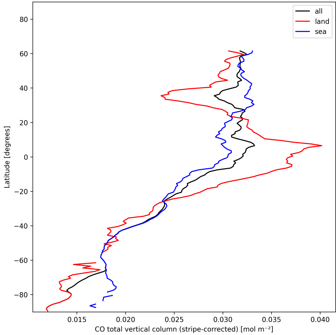
Figure 11: Zonal average of “CO total vertical column (stripe-corrected)” for 2024-12-13 to 2024-12-15.
