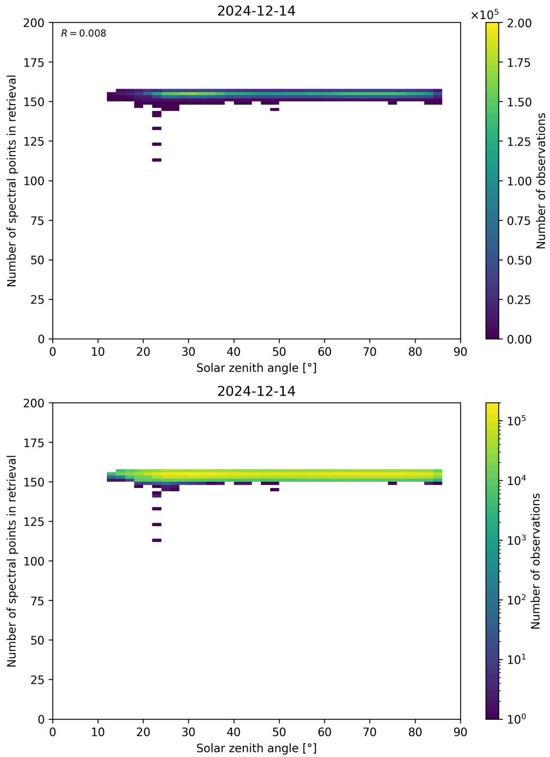
Figure 68: Scatter density plot of “Solar zenith angle” against “Number of spectral points in retrieval” for 2024-12-13 to 2024-12-15.
