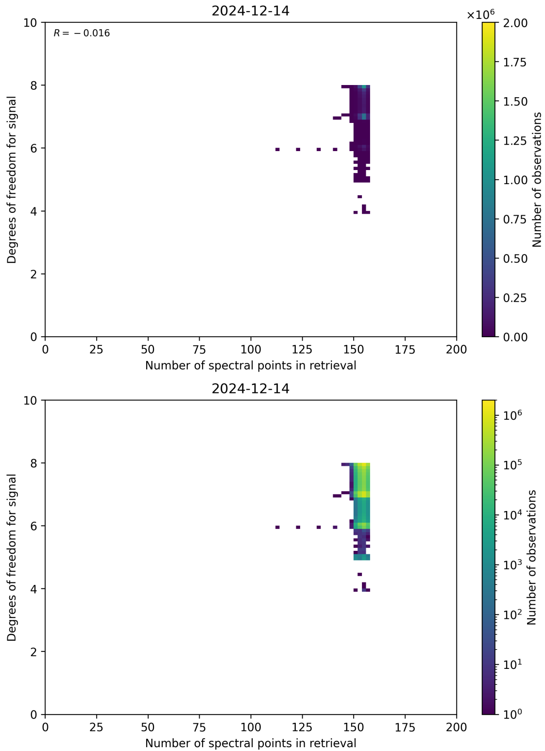
Figure 59: Scatter density plot of “Number of spectral points in retrieval” against “Degrees of freedom for signal” for 2024-12-13 to 2024-12-15.
