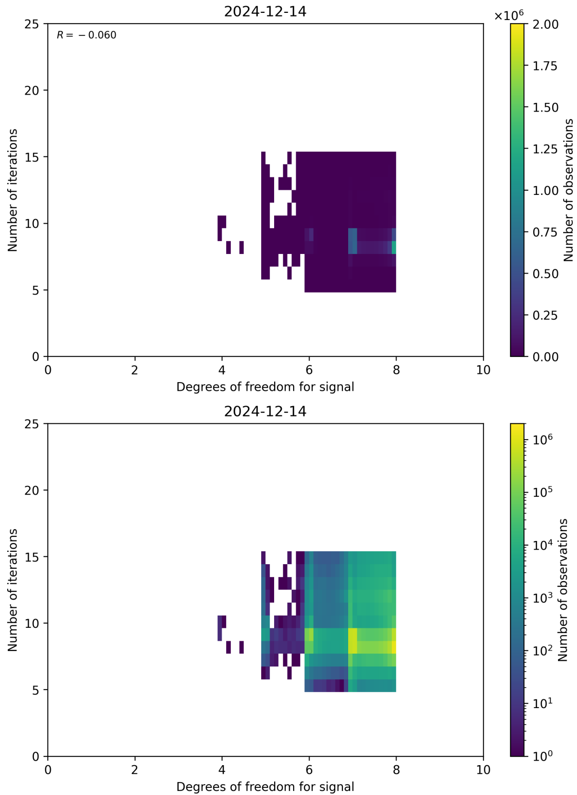
Figure 50: Scatter density plot of “Degrees of freedom for signal” against “Number of iterations” for 2024-12-13 to 2024-12-15.
