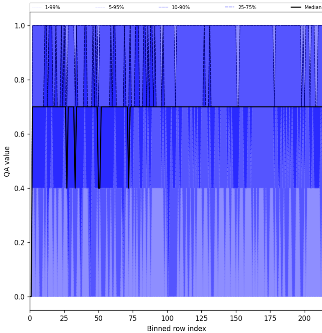
Figure 25: Along track statistics of “QA value” for 2024-12-13 to 2024-12-15
