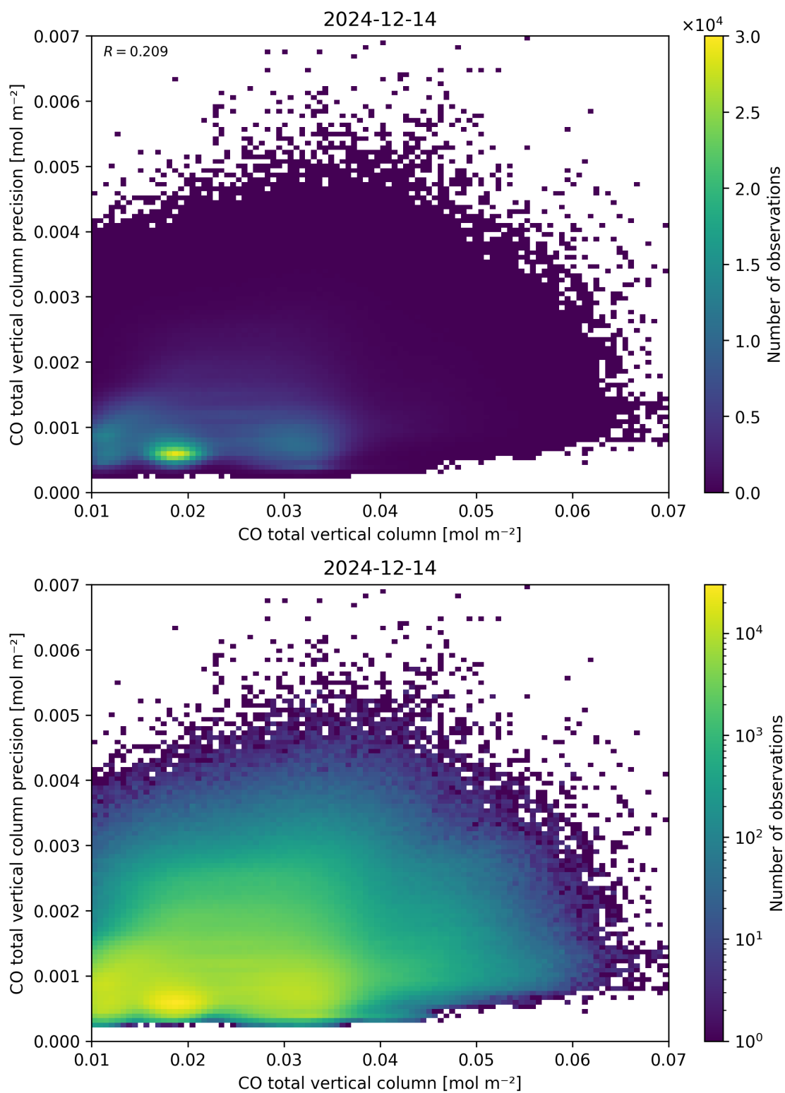
Figure 34: Scatter density plot of “CO total vertical column” against “CO total vertical column precision” for 2024-12-13 to 2024-12-15.
