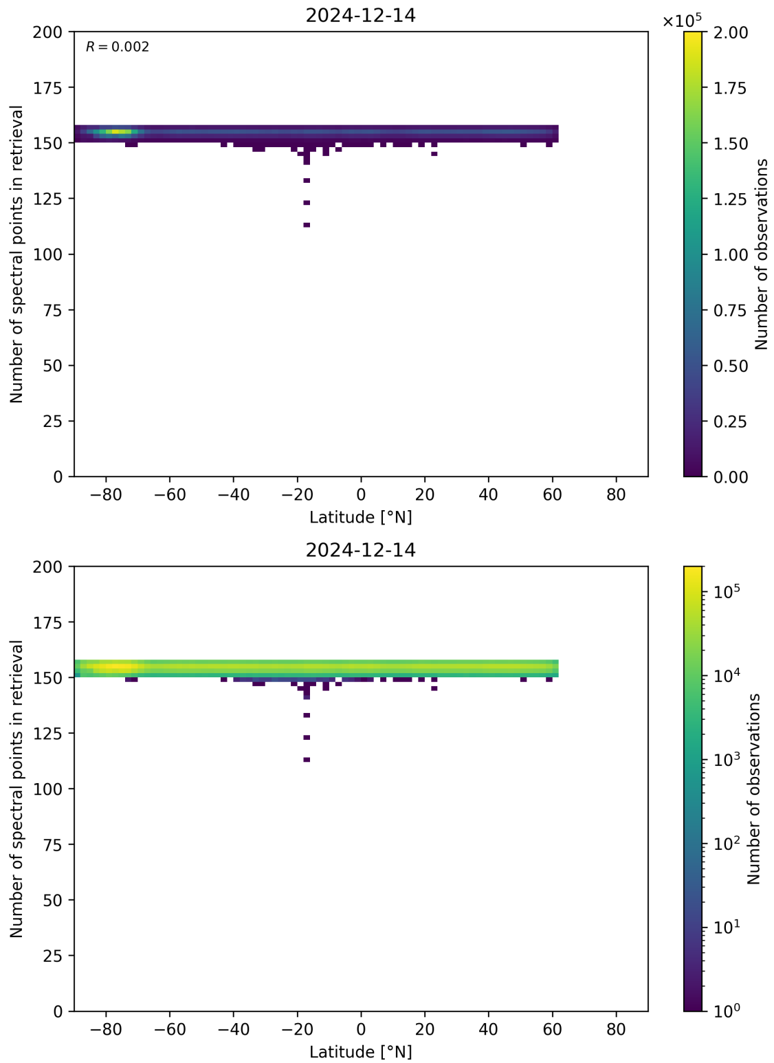
Figure 57: Scatter density plot of “Latitude” against “Number of spectral points in retrieval” for 2024-12-13 to 2024-12-15.
