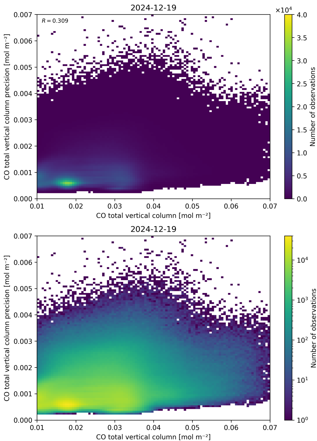
Figure 34: Scatter density plot of “CO total vertical column” against “CO total vertical column precision” for 2024-12-18 to 2024-12-20.
