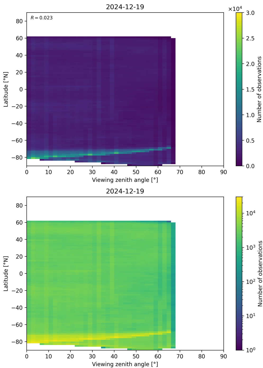
Figure 74: Scatter density plot of “Viewing zenith angle” against “Latitude” for 2024-12-18 to 2024-12-20.
