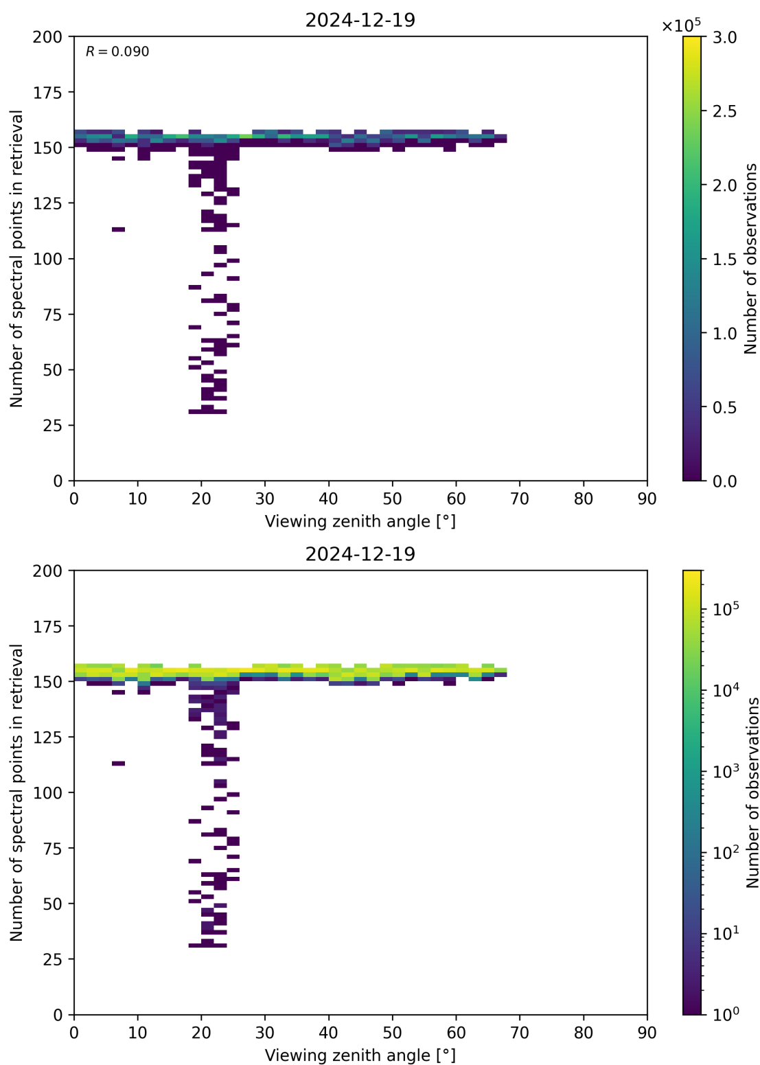
Figure 76: Scatter density plot of “Viewing zenith angle” against “Number of spectral points in retrieval” for 2024-12-18 to 2024-12-20.
