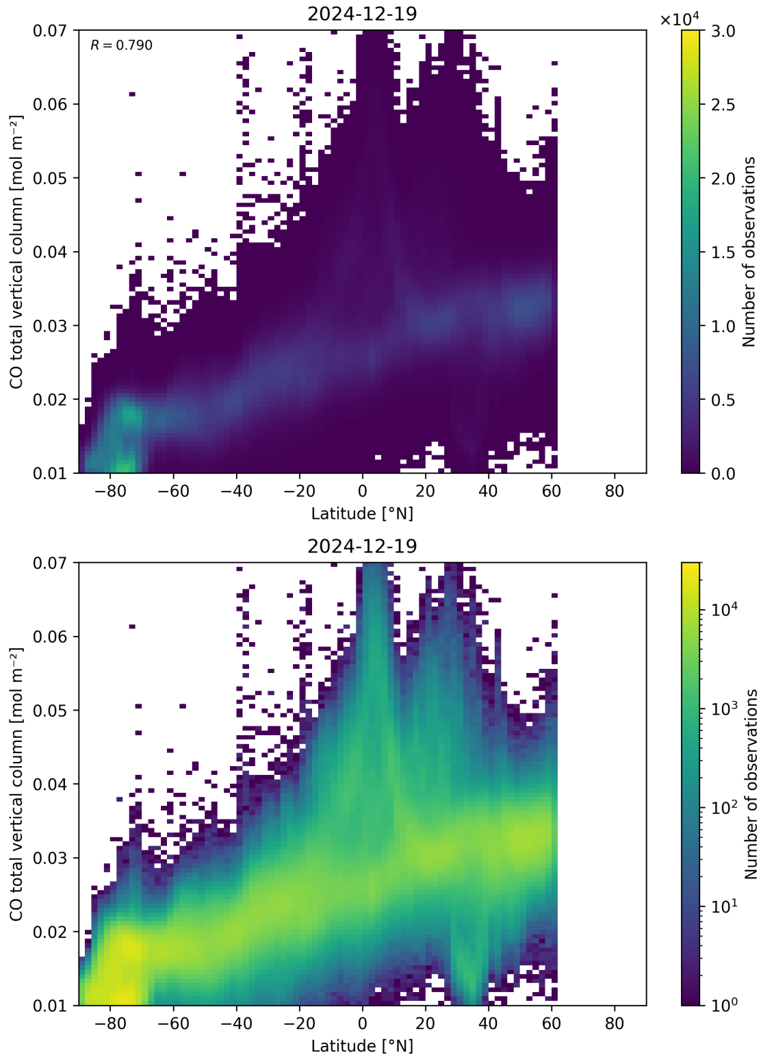
Figure 51: Scatter density plot of “Latitude” against “CO total vertical column” for 2024-12-18 to 2024-12-20.
