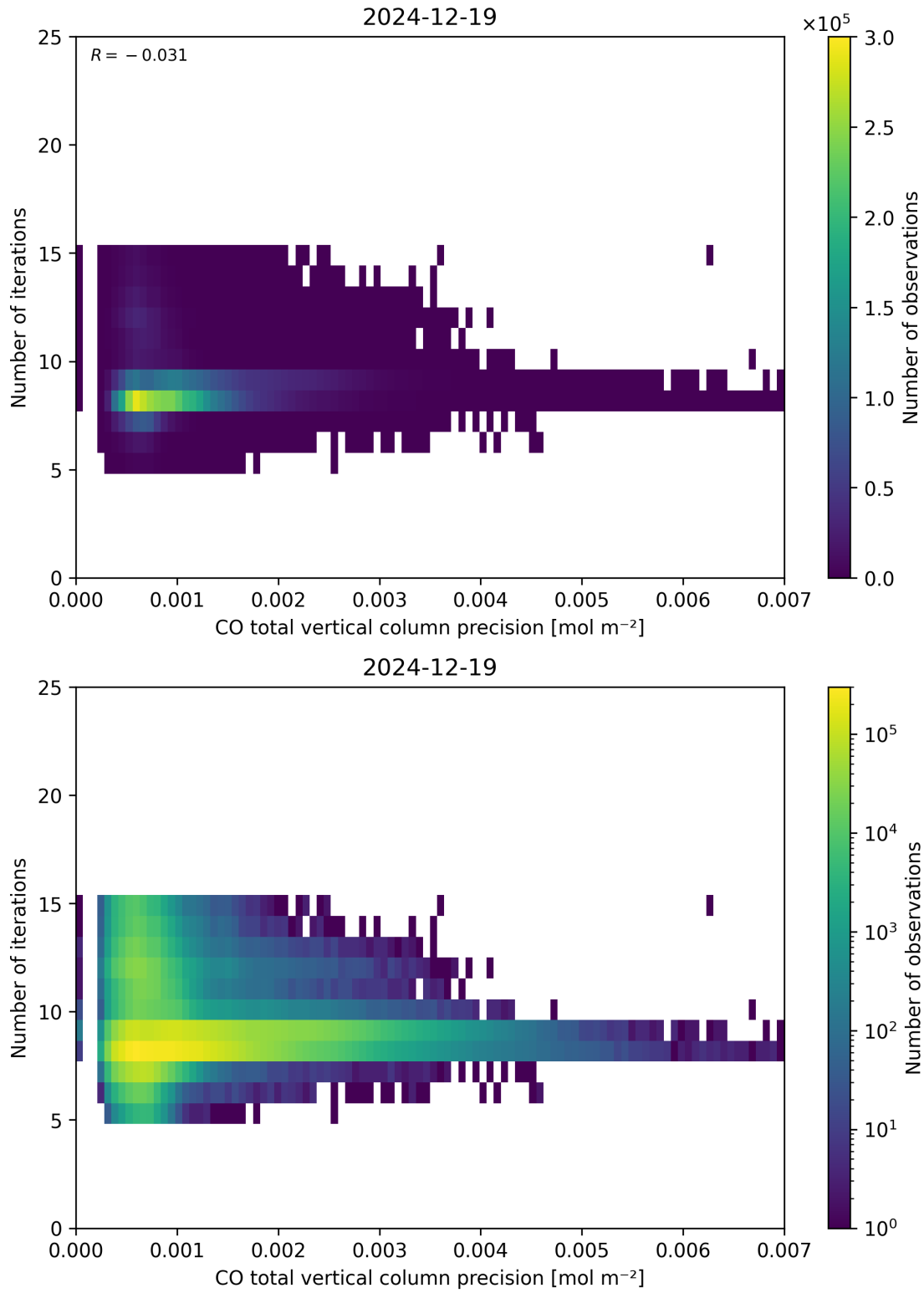
Figure 46: Scatter density plot of “CO total vertical column precision” against “Number of iterations” for 2024-12-18 to 2024-12-20.
