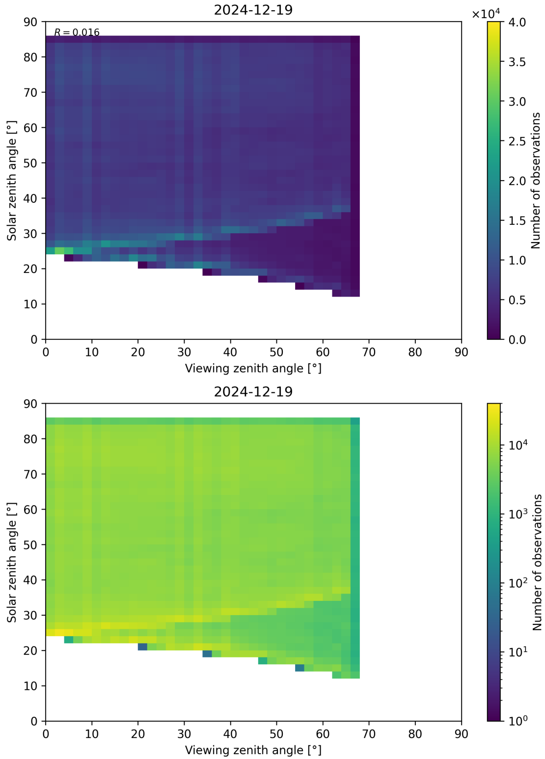
Figure 77: Scatter density plot of “Viewing zenith angle” against “Solar zenith angle” for 2024-12-18 to 2024-12-20.
