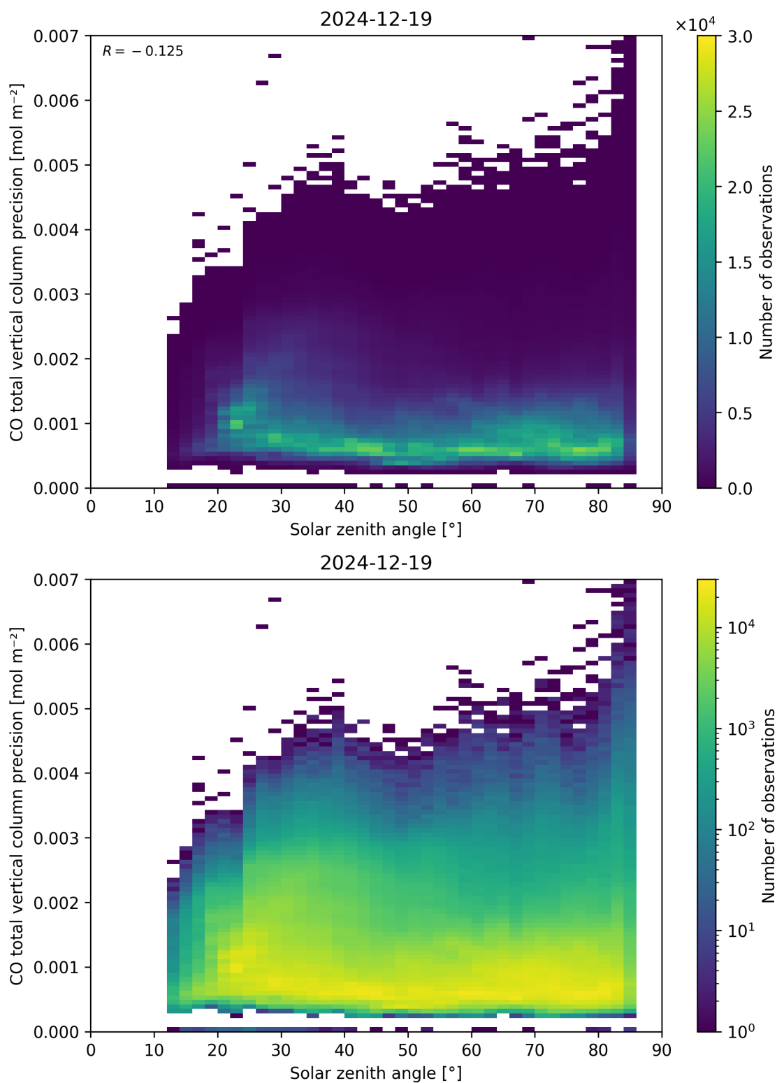
Figure 63: Scatter density plot of “Solar zenith angle” against “CO total vertical column precision” for 2024-12-18 to 2024-12-20.
