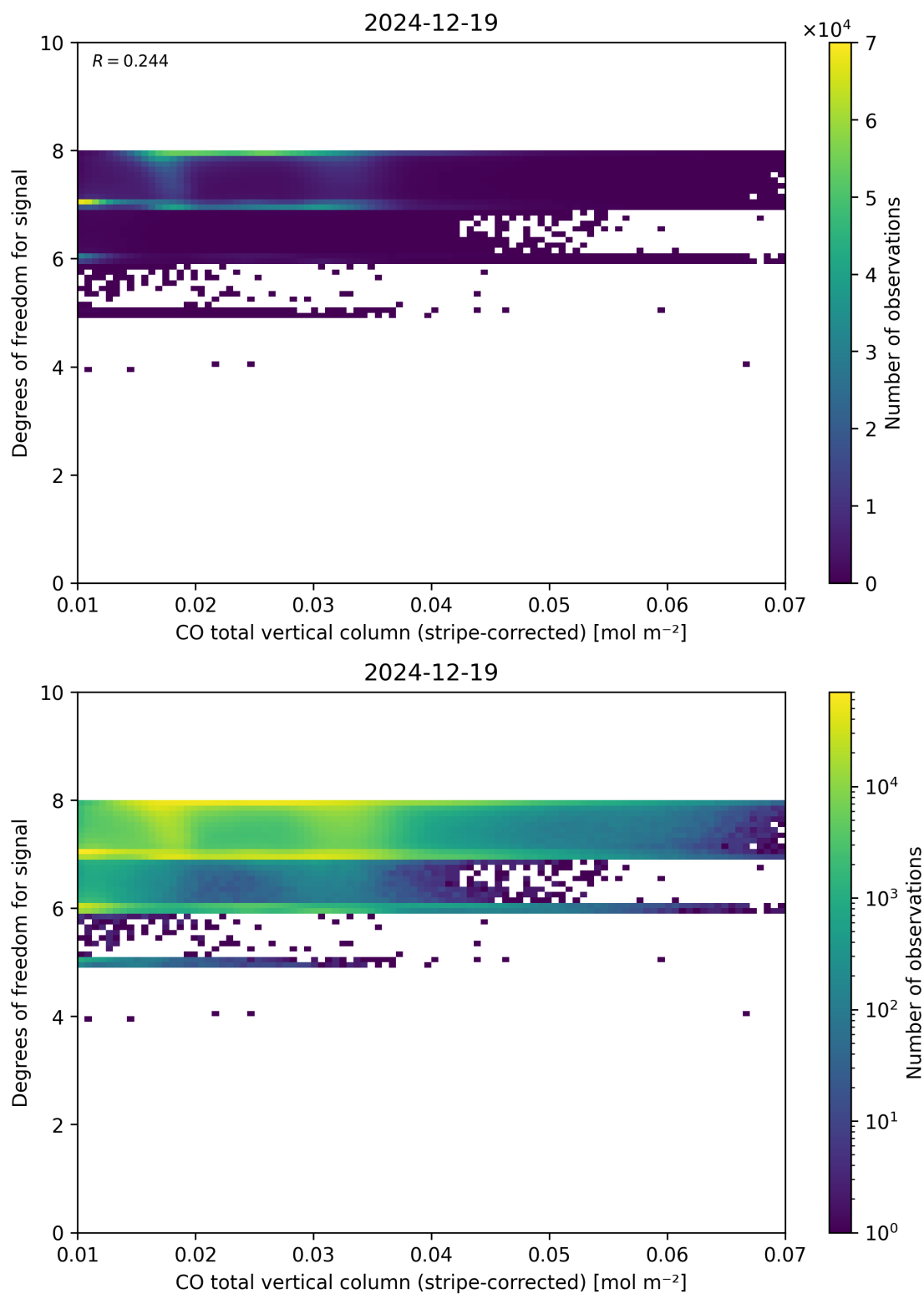
Figure 38: Scatter density plot of “CO total vertical column (stripe-corrected)” against “Degrees of freedom for signal” for 2024-12-18 to 2024-12-20.
