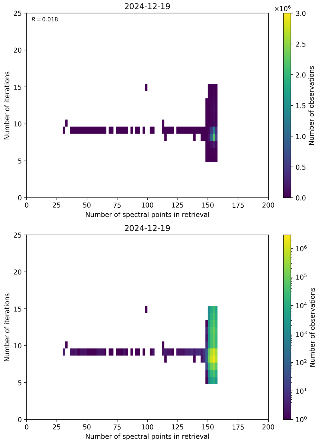
Figure 60: Scatter density plot of “Number of spectral points in retrieval” against “Number of iterations” for 2024-12-18 to 2024-12-20.
