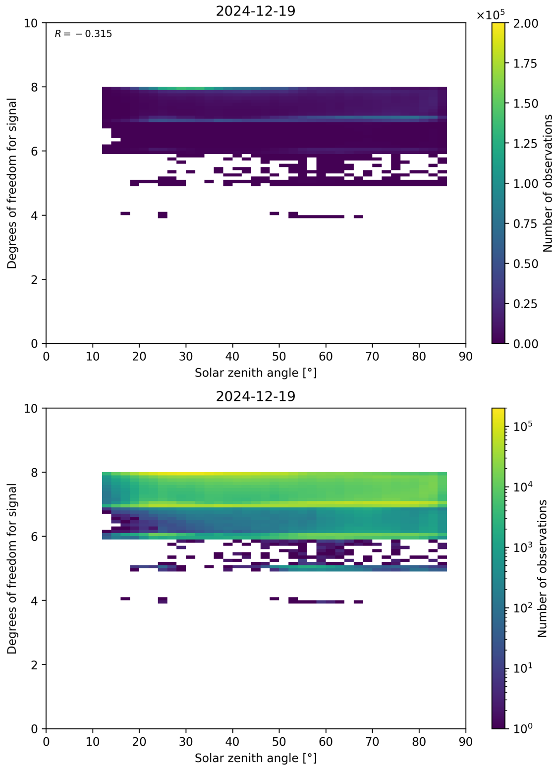
Figure 65: Scatter density plot of “Solar zenith angle” against “Degrees of freedom for signal” for 2024-12-18 to 2024-12-20.
