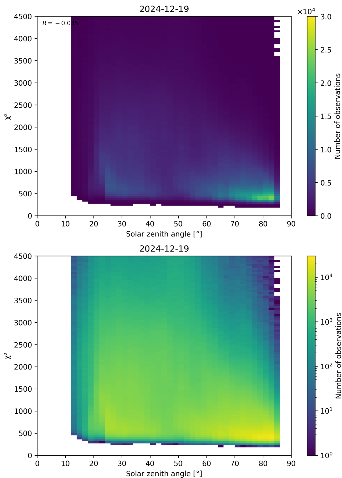
Figure 64: Scatter density plot of “Solar zenith angle” against “ \chi^2 ” for 2024-12-18 to 2024-12-20.
