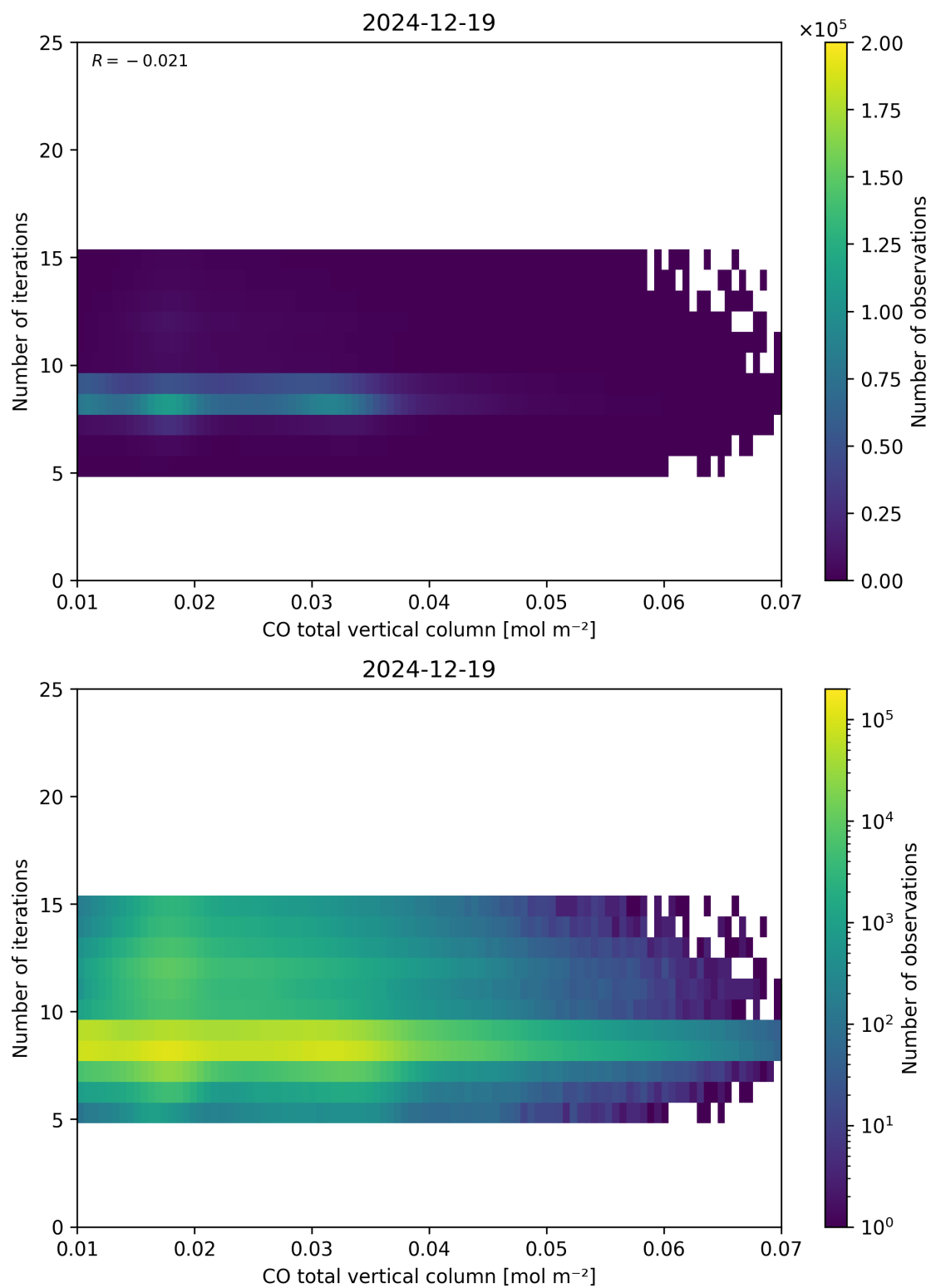
Figure 42: Scatter density plot of “CO total vertical column” against “Number of iterations” for 2024-12-18 to 2024-12-20.
