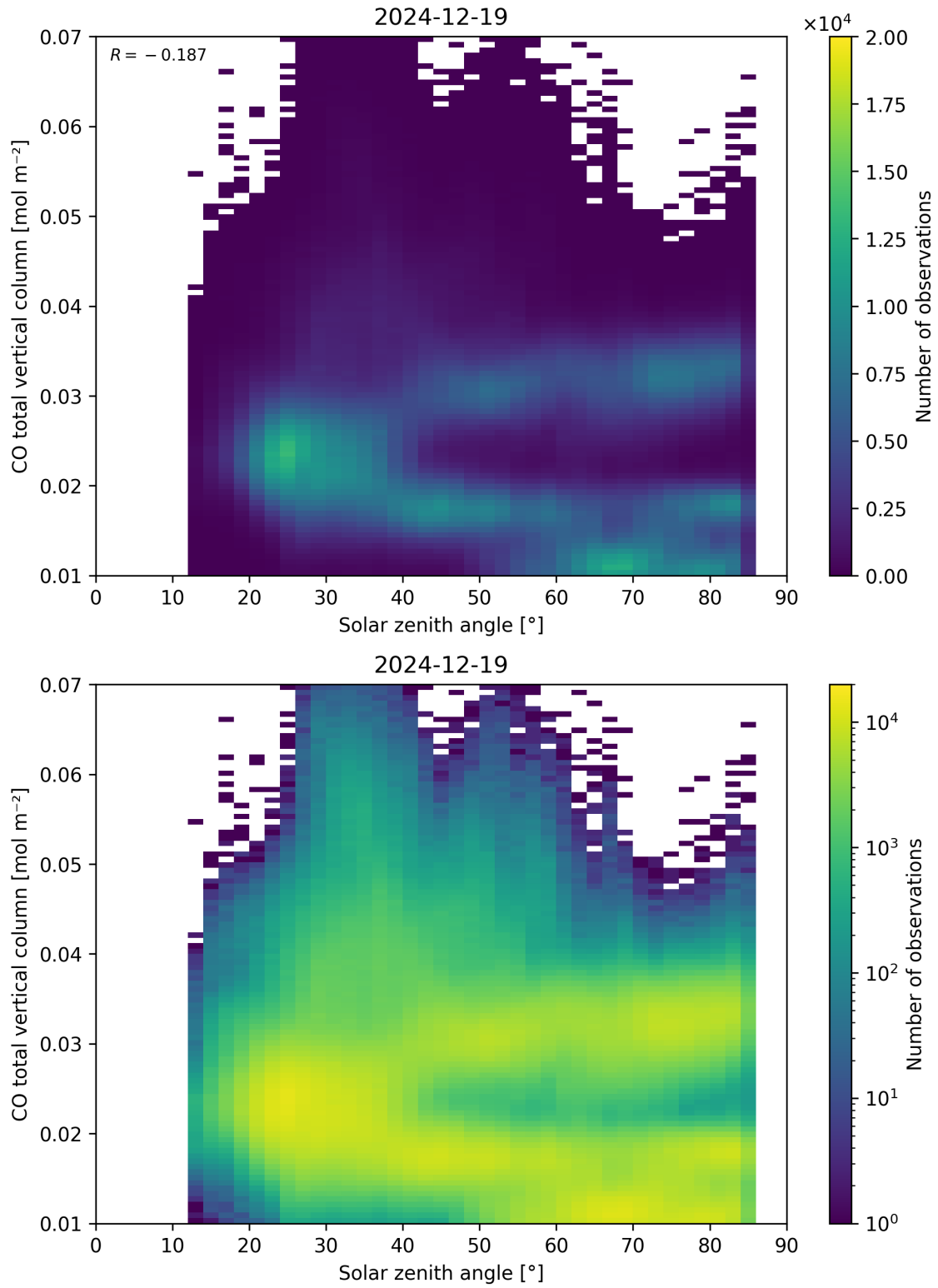
Figure 61: Scatter density plot of “Solar zenith angle” against “CO total vertical column” for 2024-12-18 to 2024-12-20.
