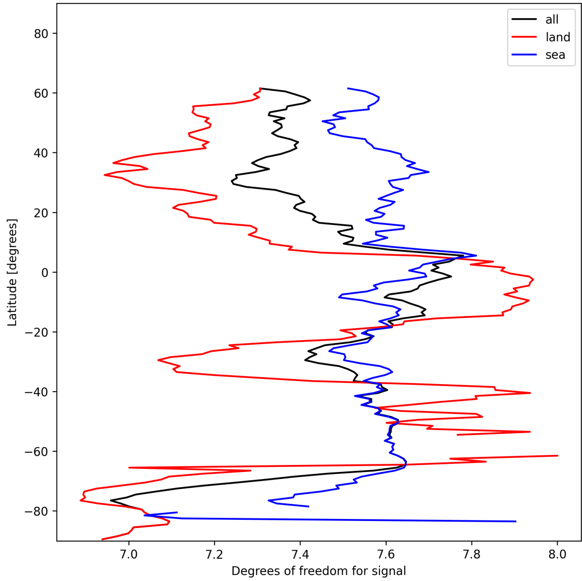
Figure 15: Zonal average of “Degrees of freedom for signal” for 2024-12-18 to 2024-12-20.
