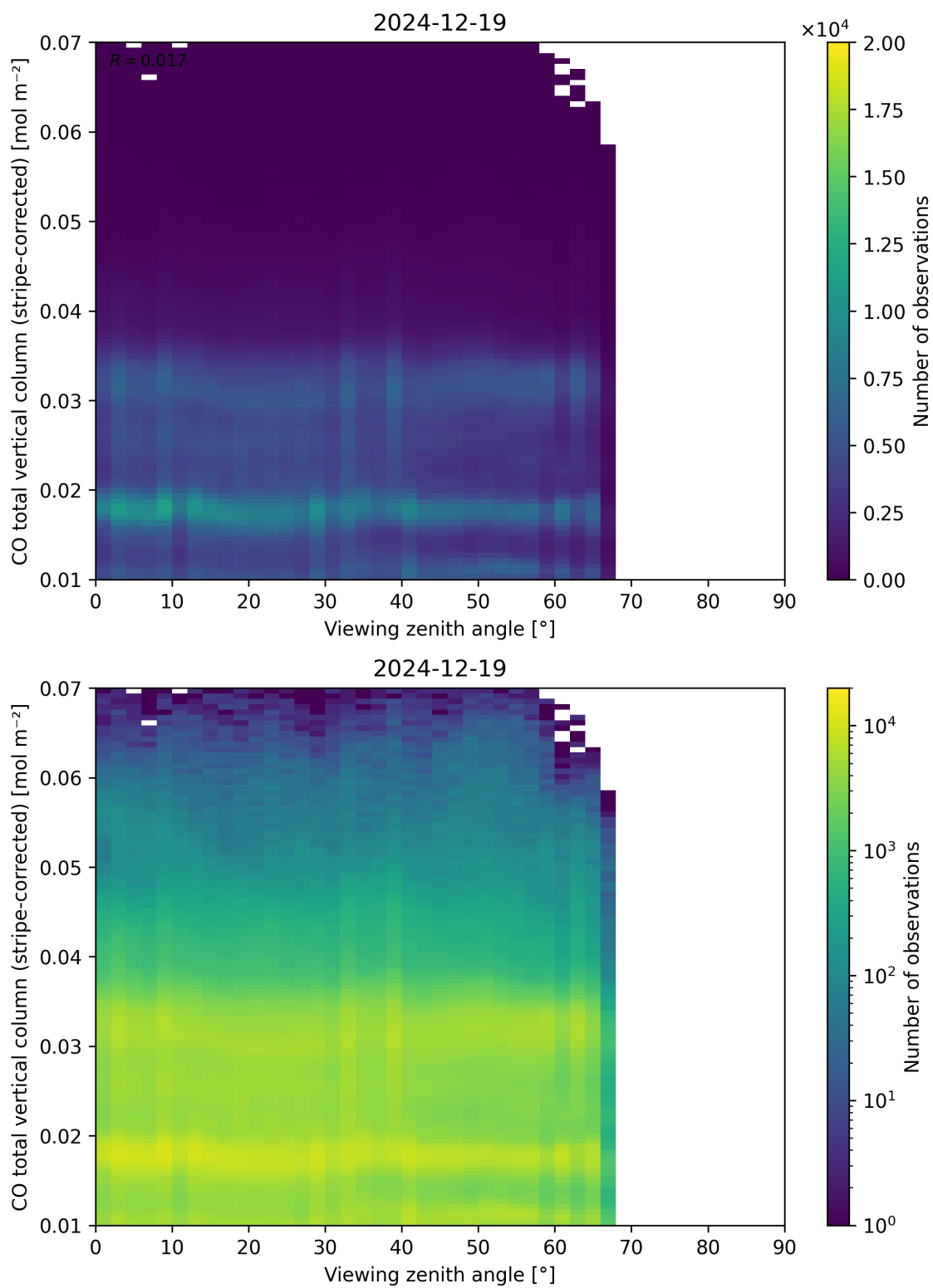
Figure 70: Scatter density plot of “Viewing zenith angle” against “CO total vertical column (stripe-corrected)” for 2024-12-18 to 2024-12-20.
