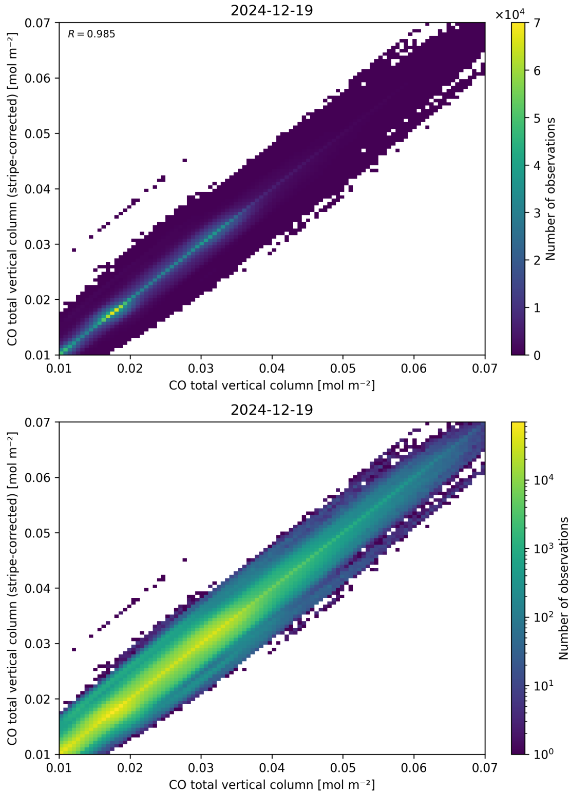
Figure 33: Scatter density plot of “CO total vertical column” against “CO total vertical column (stripe-corrected)” for 2024-12-18 to 2024-12-20.
