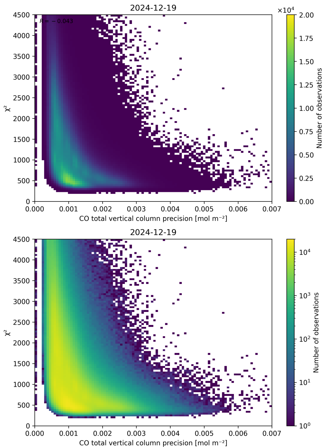
Figure 44: Scatter density plot of “CO total vertical column precision” against “ \chi^2 ” for 2024-12-18 to 2024-12-20.
