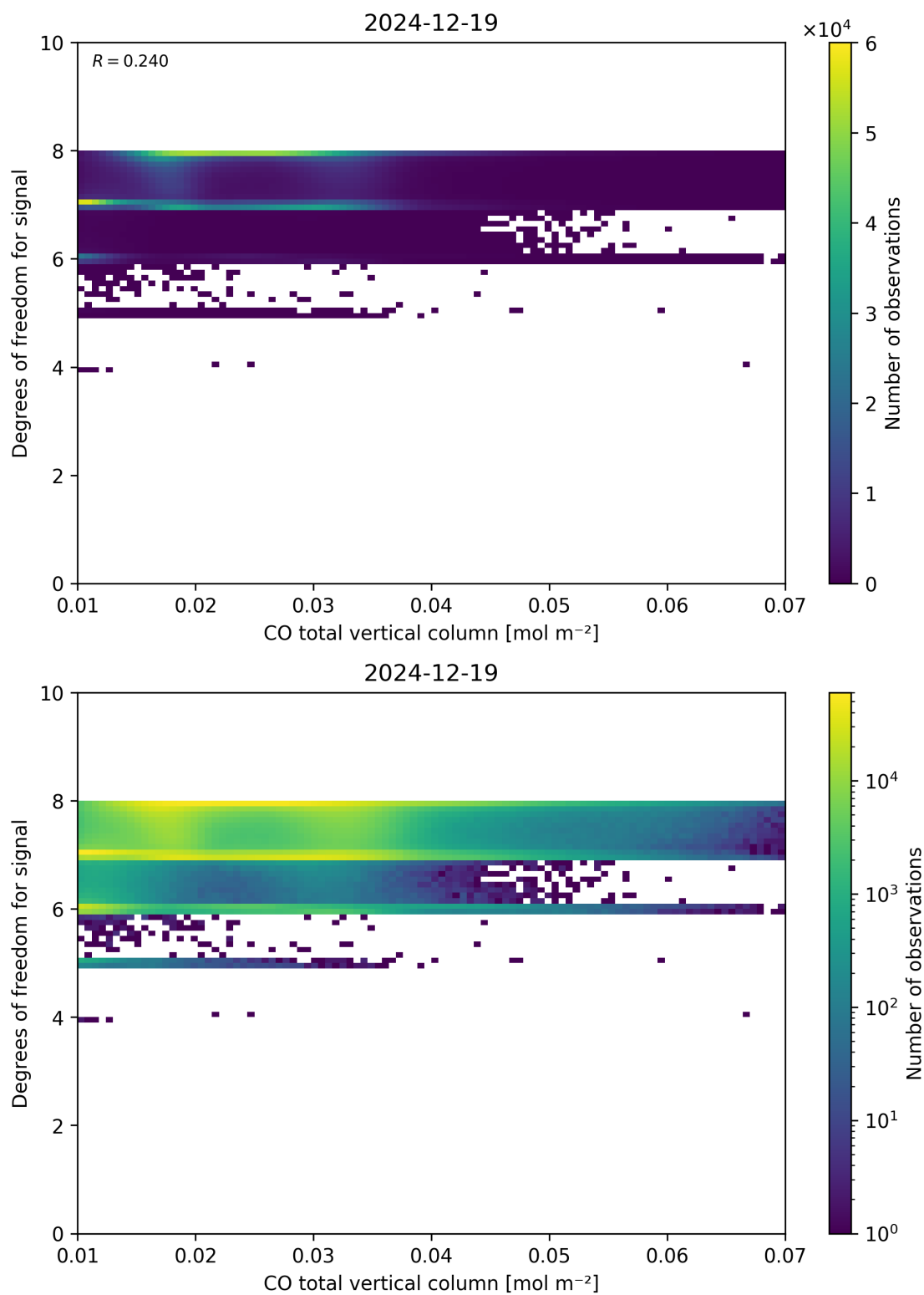
Figure 41: Scatter density plot of “CO total vertical column” against “Degrees of freedom for signal” for 2024-12-18 to 2024-12-20.
