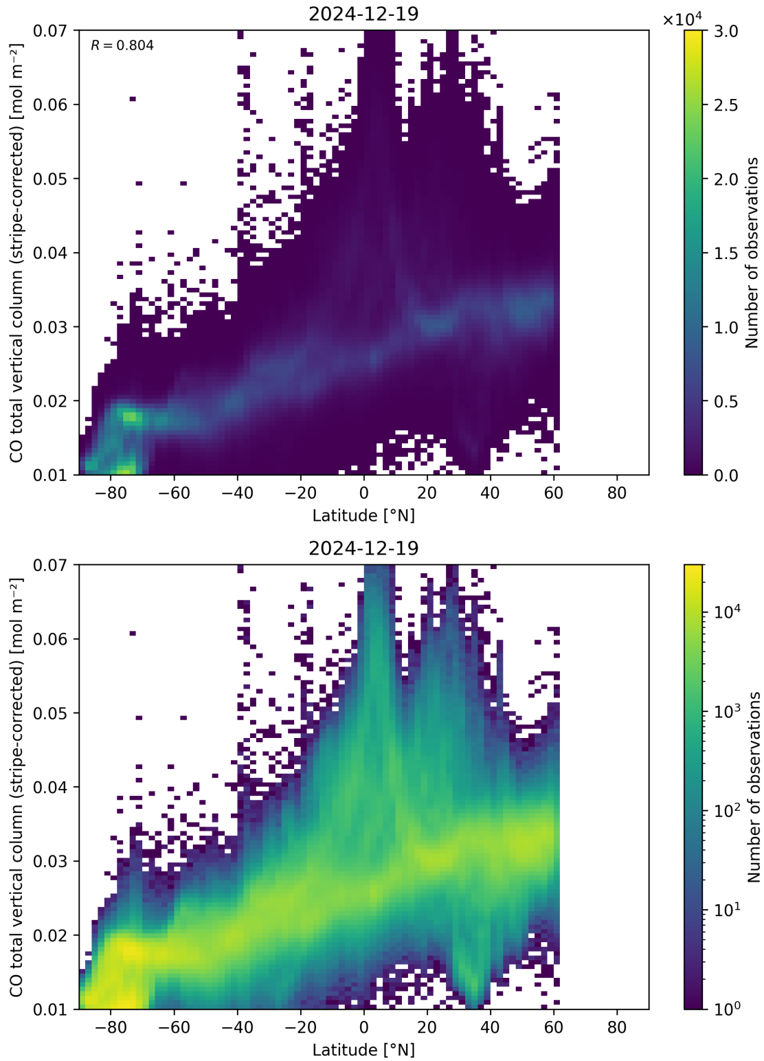
Figure 52: Scatter density plot of “Latitude” against “CO total vertical column (stripe-corrected)” for 2024-12-18 to 2024-12-20.
