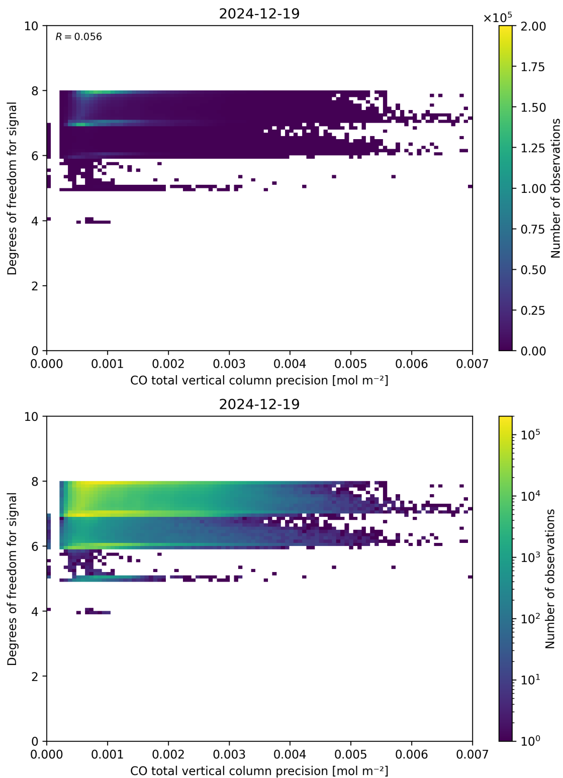
Figure 45: Scatter density plot of “CO total vertical column precision” against “Degrees of freedom for signal” for 2024-12-18 to 2024-12-20.
