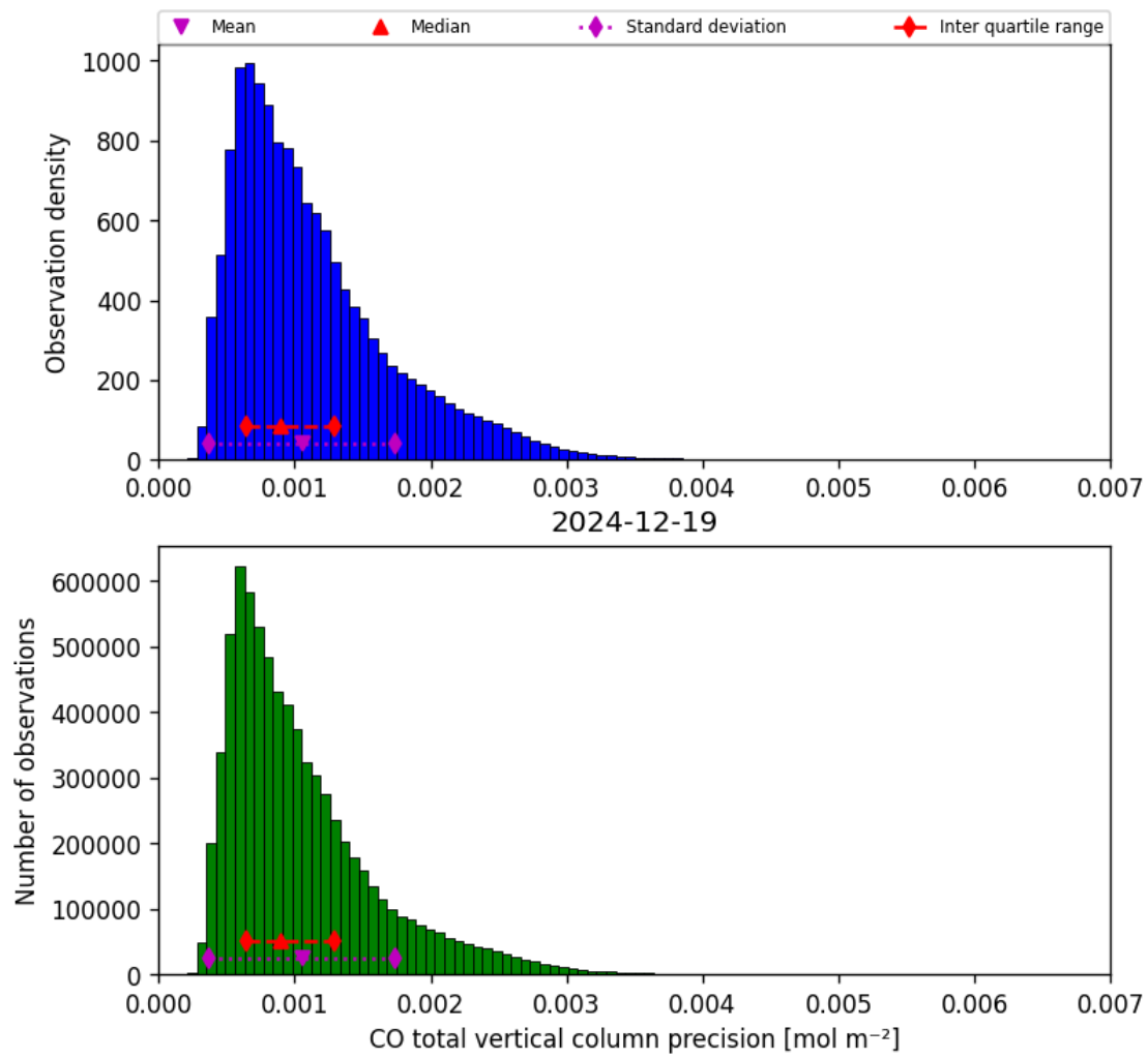
Figure 20: Histogram of “CO total vertical column precision” for 2024-12-18 to 2024-12-20
