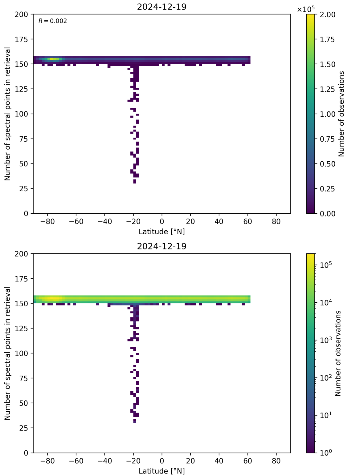
Figure 57: Scatter density plot of “Latitude” against “Number of spectral points in retrieval” for 2024-12-18 to 2024-12-20.
