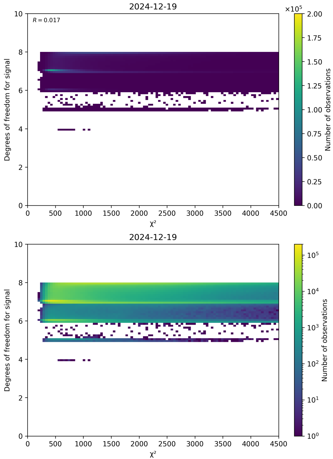
Figure 48: Scatter density plot of “ \chi^2 ” against “Degrees of freedom for signal” for 2024-12-18 to 2024-12-20.
