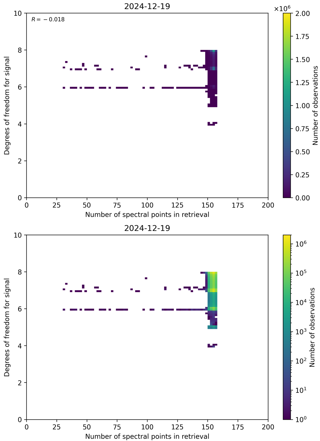
Figure 59: Scatter density plot of “Number of spectral points in retrieval” against “Degrees of freedom for signal” for 2024-12-18 to 2024-12-20.
