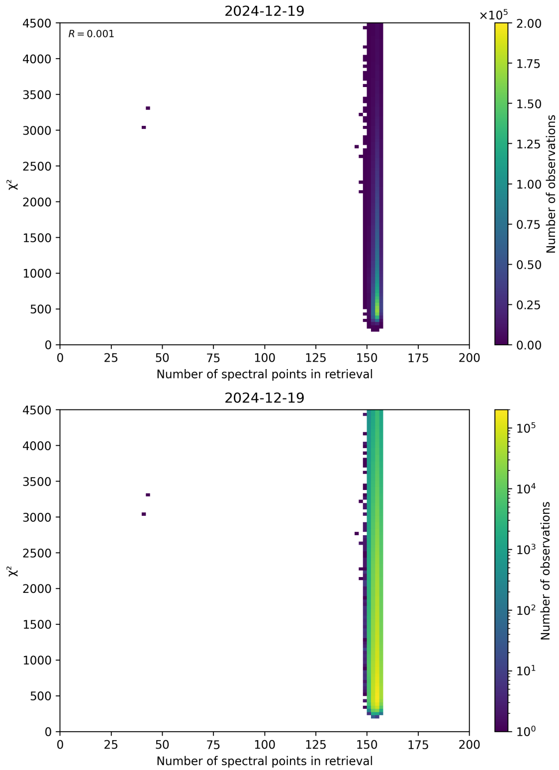
Figure 58: Scatter density plot of “Number of spectral points in retrieval” against “ \chi^2 ” for 2024-12-18 to 2024-12-20.
