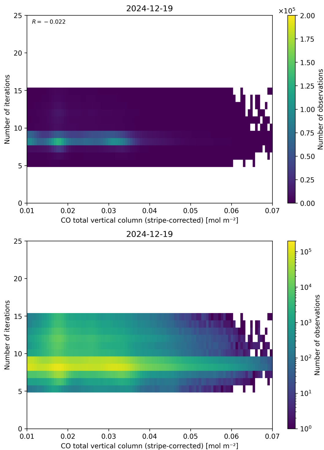
Figure 39: Scatter density plot of “CO total vertical column (stripe-corrected)” against “Number of iterations” for 2024-12-18 to 2024-12-20.
