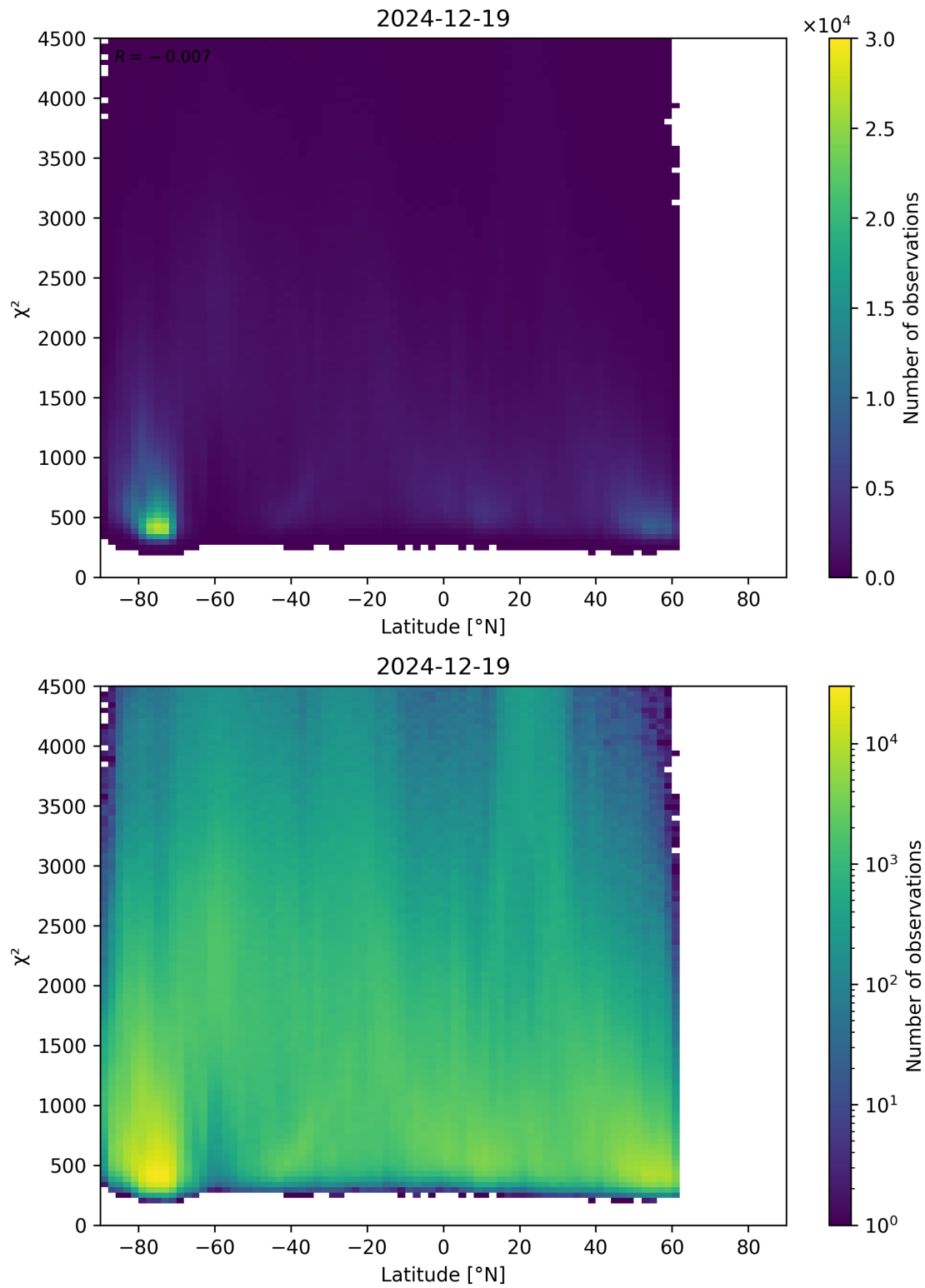
Figure 54: Scatter density plot of “Latitude” against “ \chi^2 ” for 2024-12-18 to 2024-12-20.
