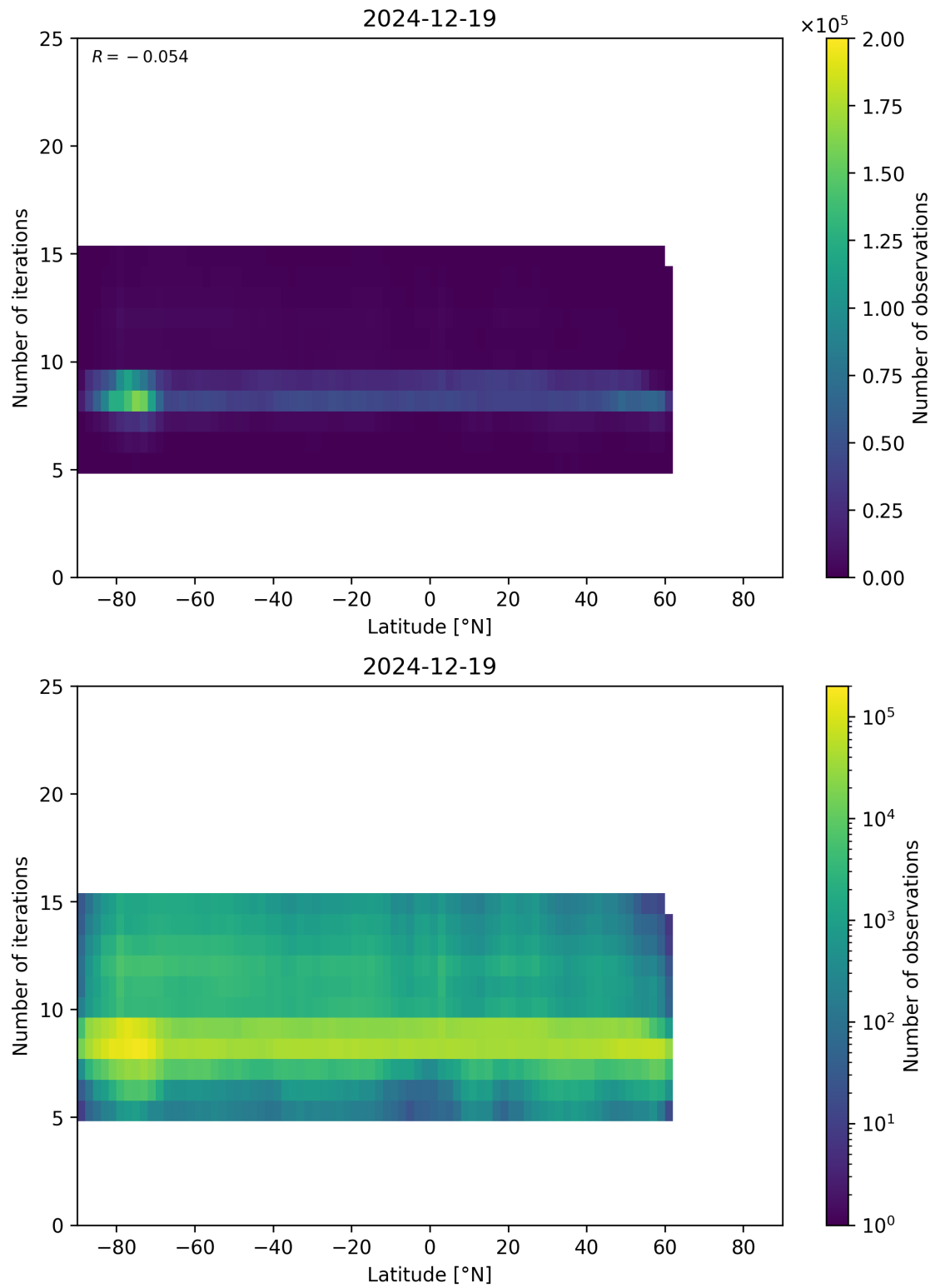
Figure 56: Scatter density plot of “Latitude” against “Number of iterations” for 2024-12-18 to 2024-12-20.
