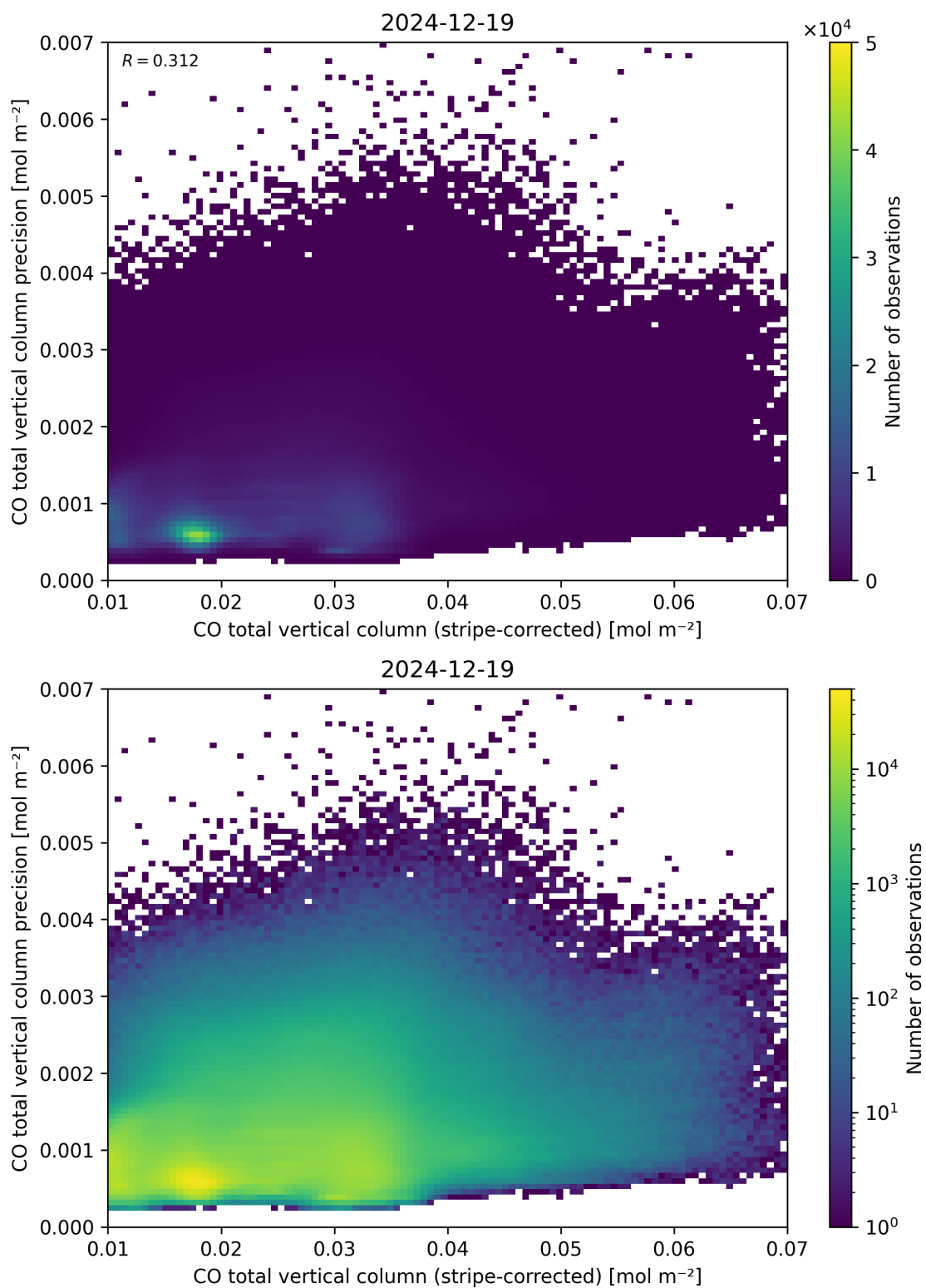
Figure 36: Scatter density plot of “CO total vertical column (stripe-corrected)” against “CO total vertical column precision” for 2024-12-18 to 2024-12-20.
