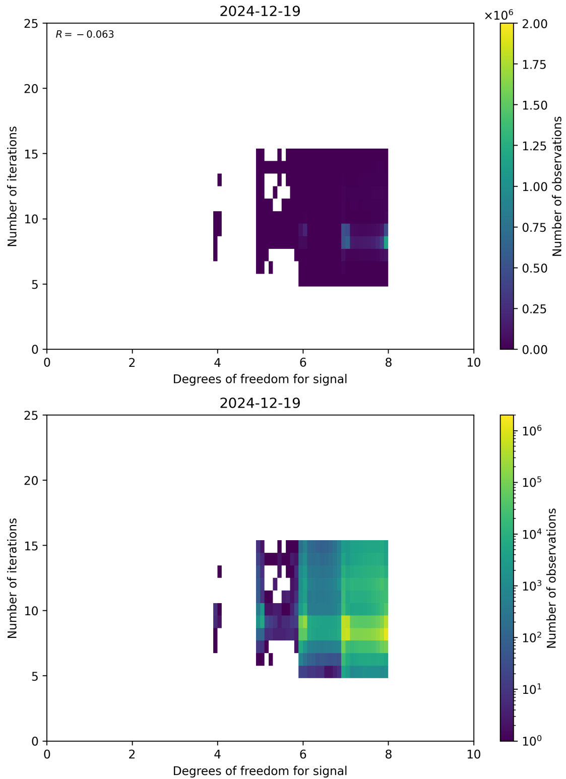
Figure 50: Scatter density plot of “Degrees of freedom for signal” against “Number of iterations” for 2024-12-18 to 2024-12-20.
