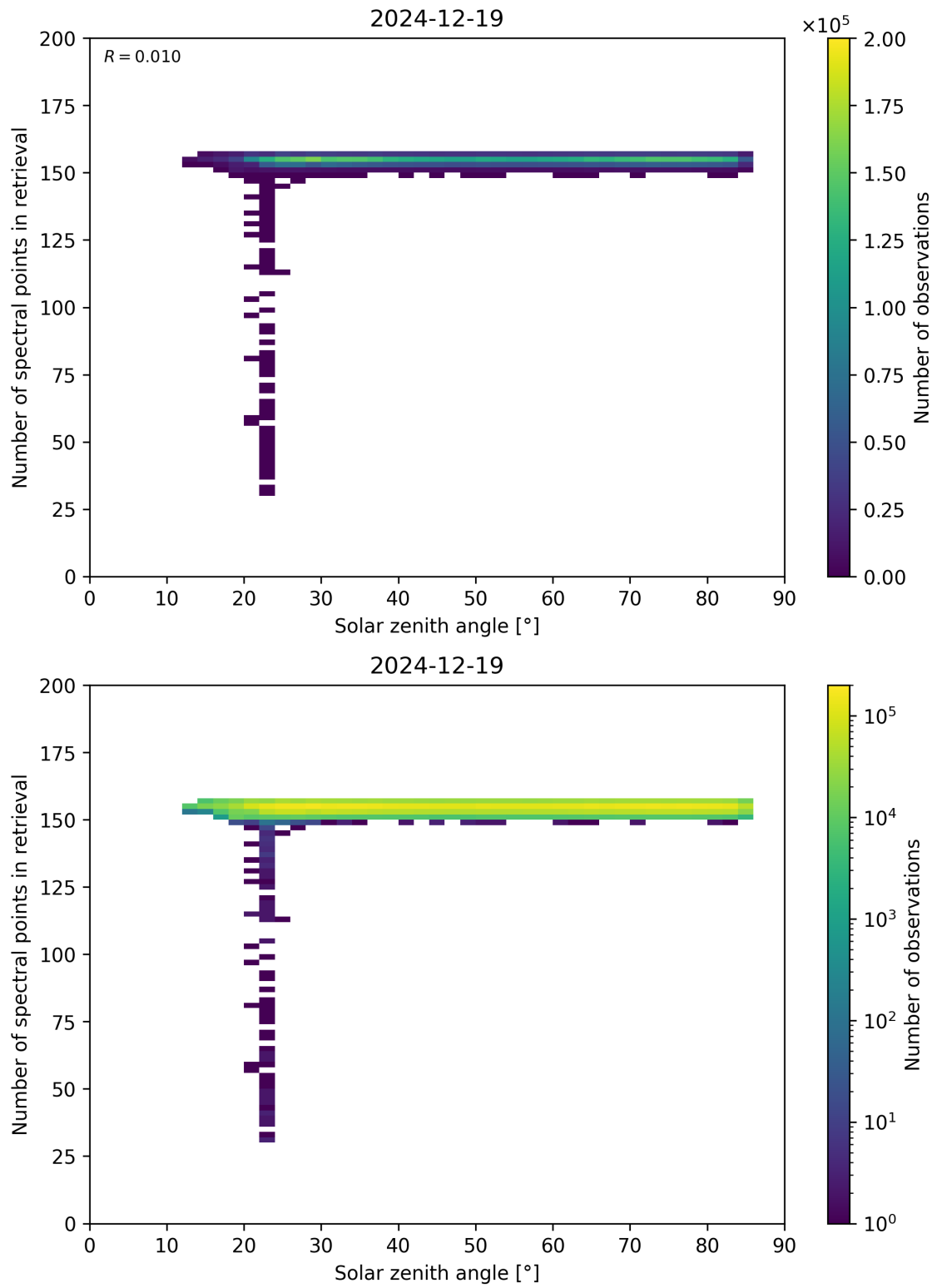
Figure 68: Scatter density plot of “Solar zenith angle” against “Number of spectral points in retrieval” for 2024-12-18 to 2024-12-20.
