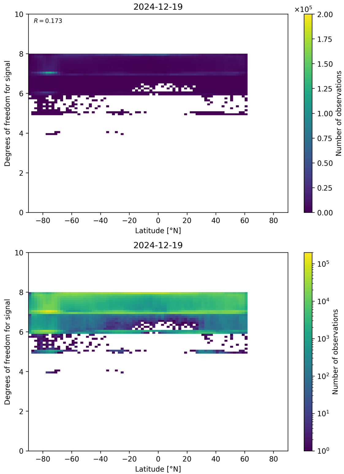
Figure 55: Scatter density plot of “Latitude” against “Degrees of freedom for signal” for 2024-12-18 to 2024-12-20.
