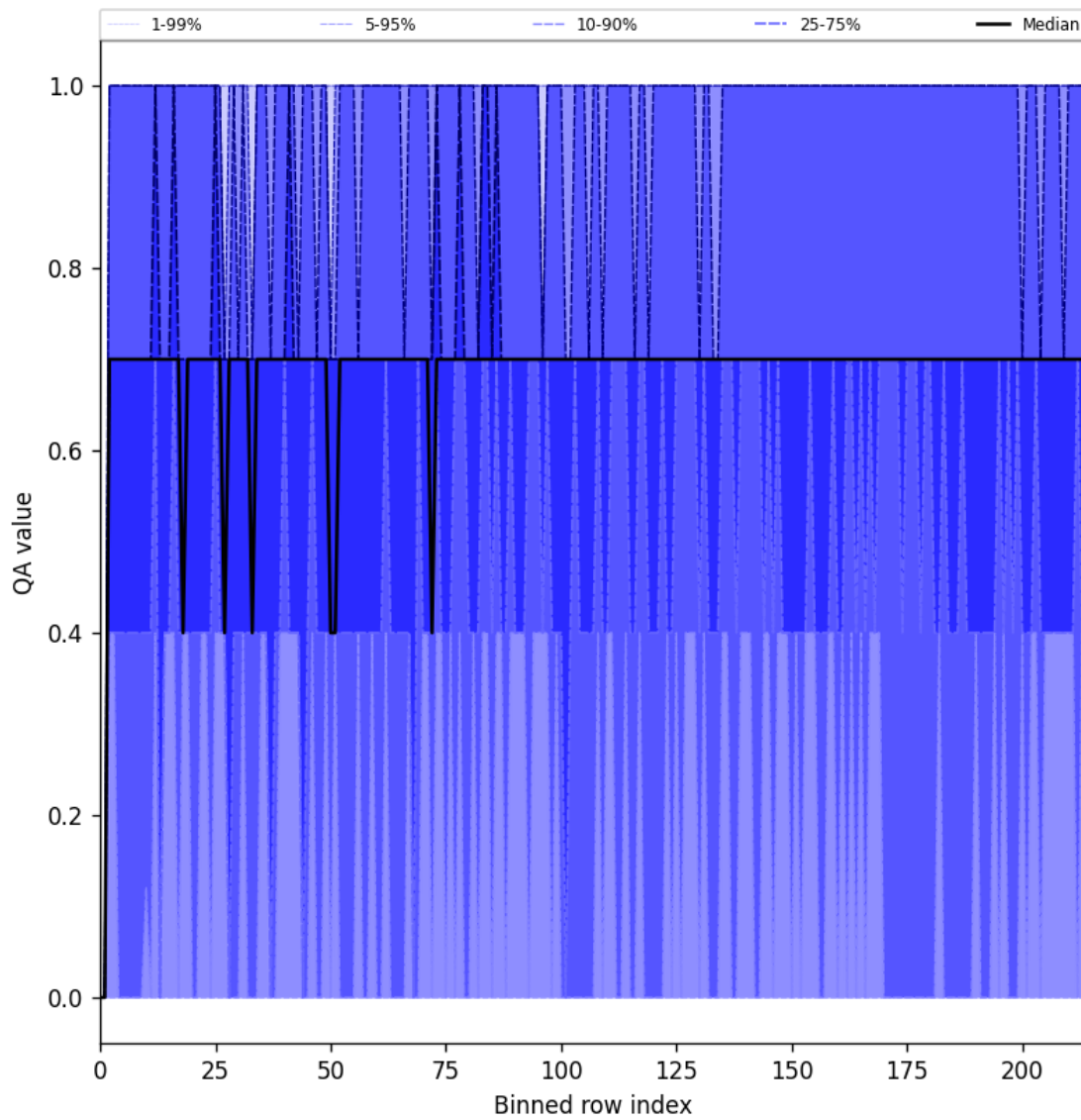
Figure 25: Along track statistics of “QA value” for 2024-12-18 to 2024-12-20
