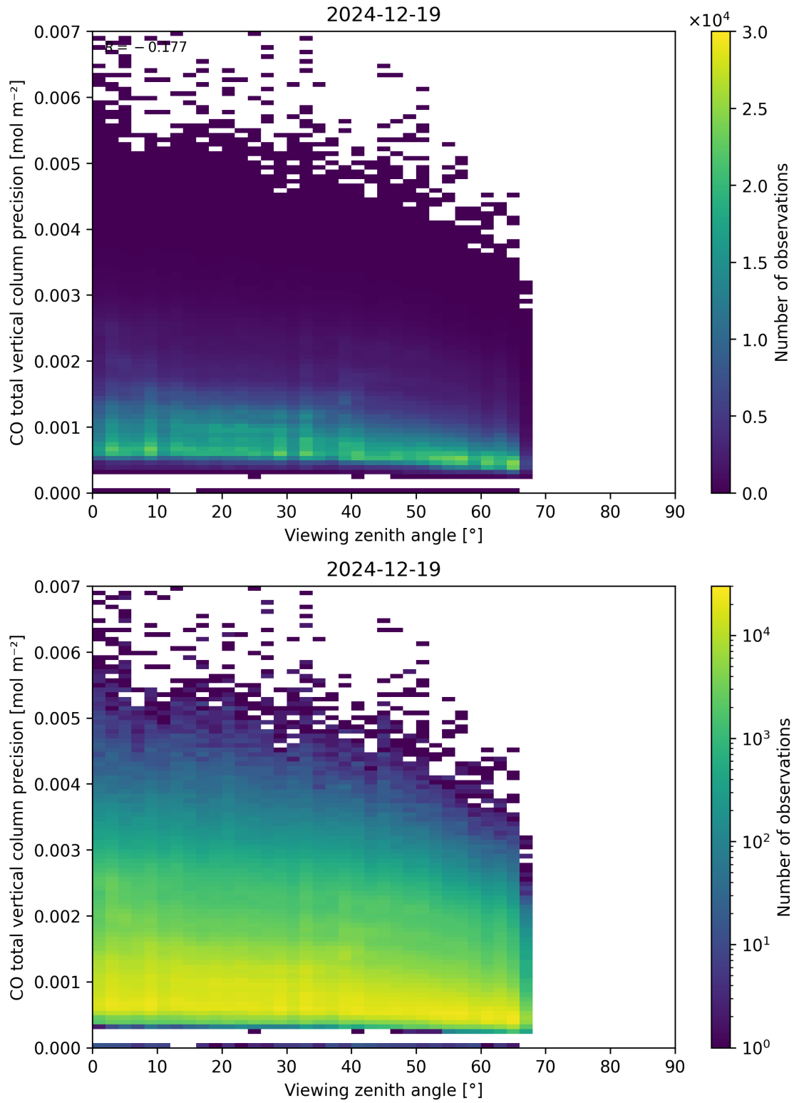
Figure 71: Scatter density plot of “Viewing zenith angle” against “CO total vertical column precision” for 2024-12-18 to 2024-12-20.
