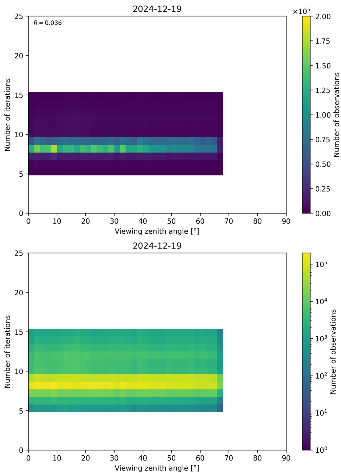
Figure 75: Scatter density plot of “Viewing zenith angle” against “Number of iterations” for 2024-12-18 to 2024-12-20.
