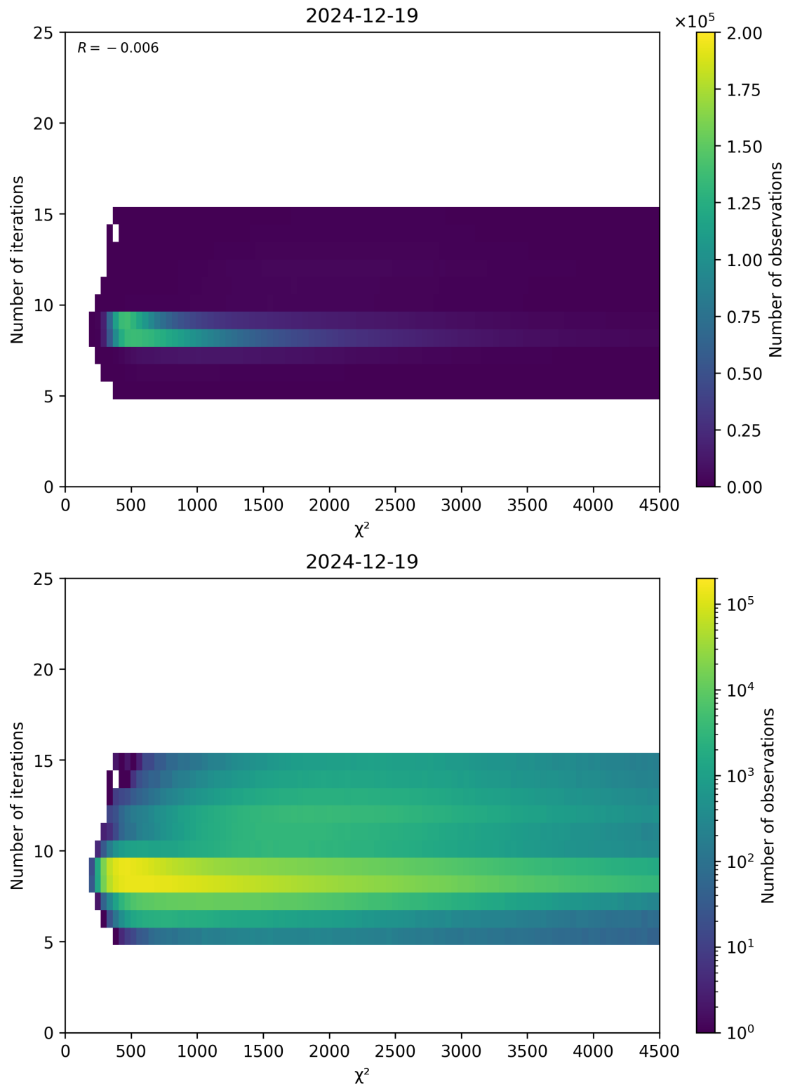
Figure 49: Scatter density plot of “ \chi^2 ” against “Number of iterations” for 2024-12-18 to 2024-12-20.
