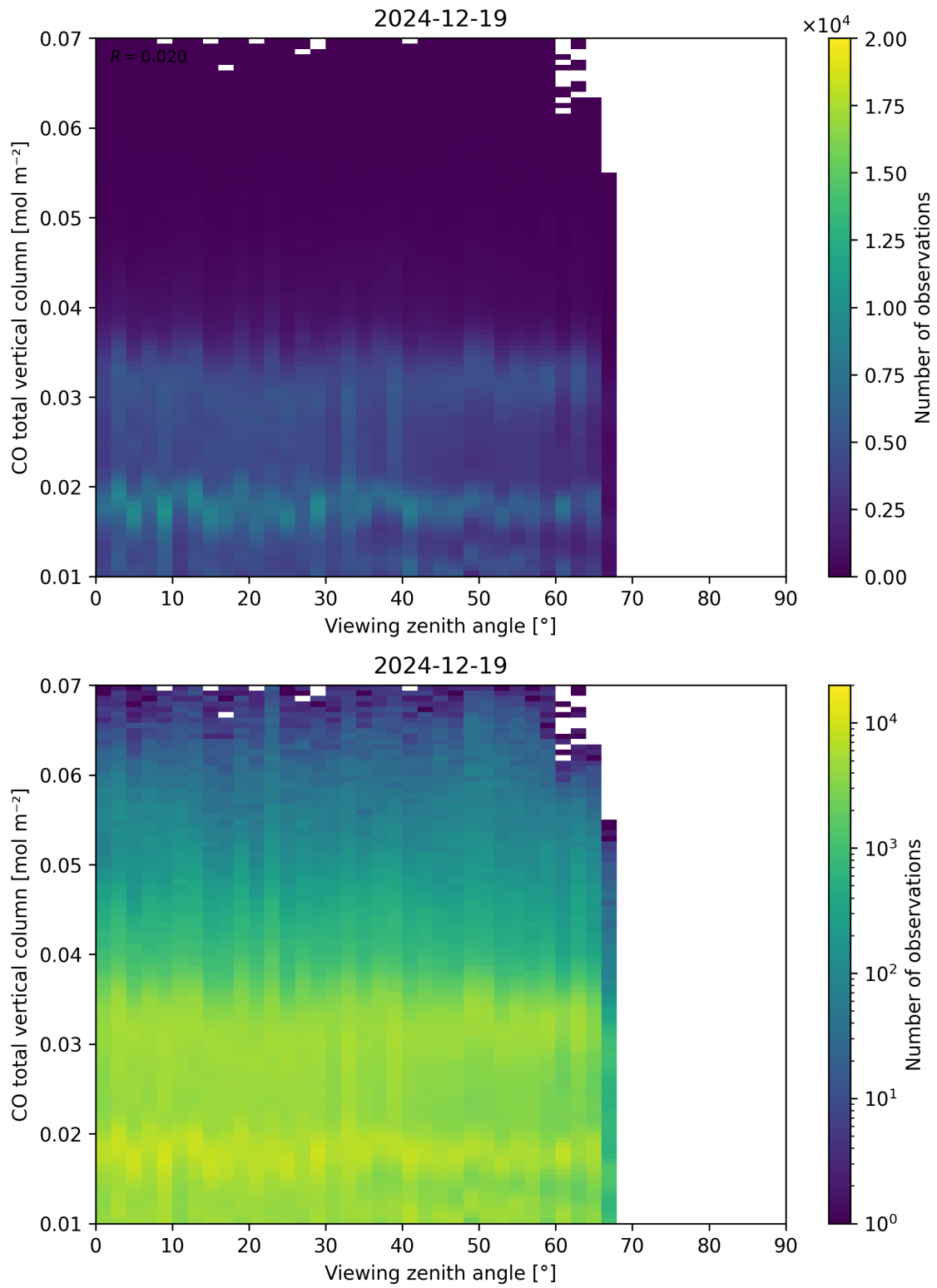
Figure 69: Scatter density plot of “Viewing zenith angle” against “CO total vertical column” for 2024-12-18 to 2024-12-20.
