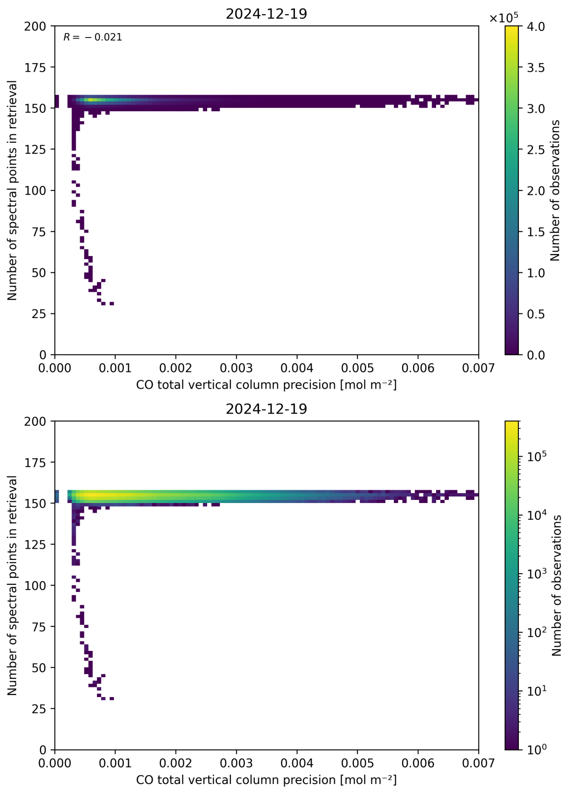
Figure 47: Scatter density plot of “CO total vertical column precision” against “Number of spectral points in retrieval” for 2024-12-18 to 2024-12-20.
