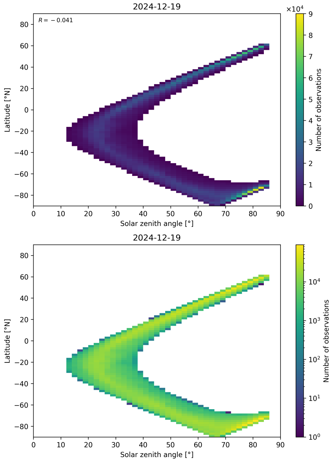
Figure 66: Scatter density plot of “Solar zenith angle” against “Latitude” for 2024-12-18 to 2024-12-20.
