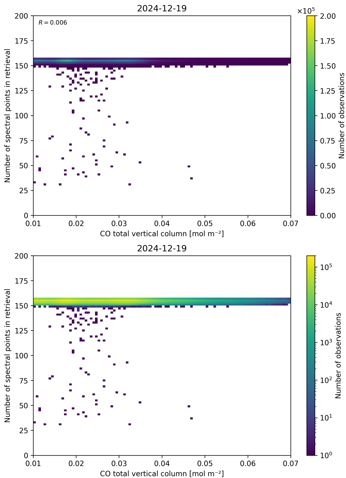
Figure 43: Scatter density plot of “CO total vertical column” against “Number of spectral points in retrieval” for 2024-12-18 to 2024-12-20.
