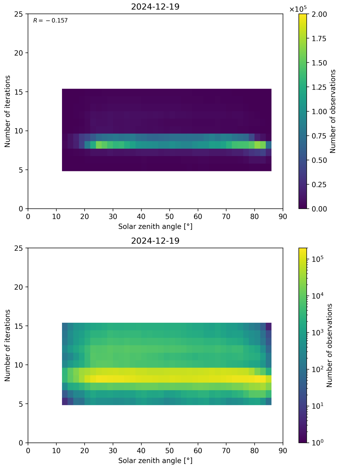
Figure 67: Scatter density plot of “Solar zenith angle” against “Number of iterations” for 2024-12-18 to 2024-12-20.
