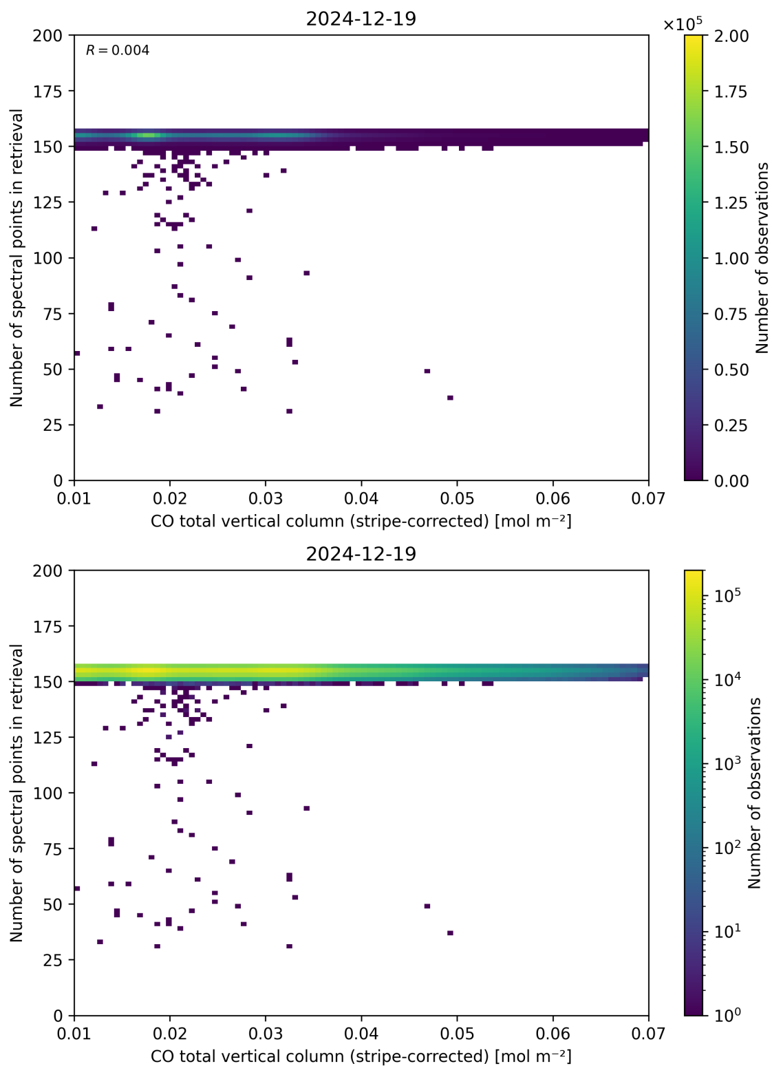
Figure 40: Scatter density plot of “CO total vertical column (stripe-corrected)” against “Number of spectral points in retrieval” for 2024-12-18 to 2024-12-20.
