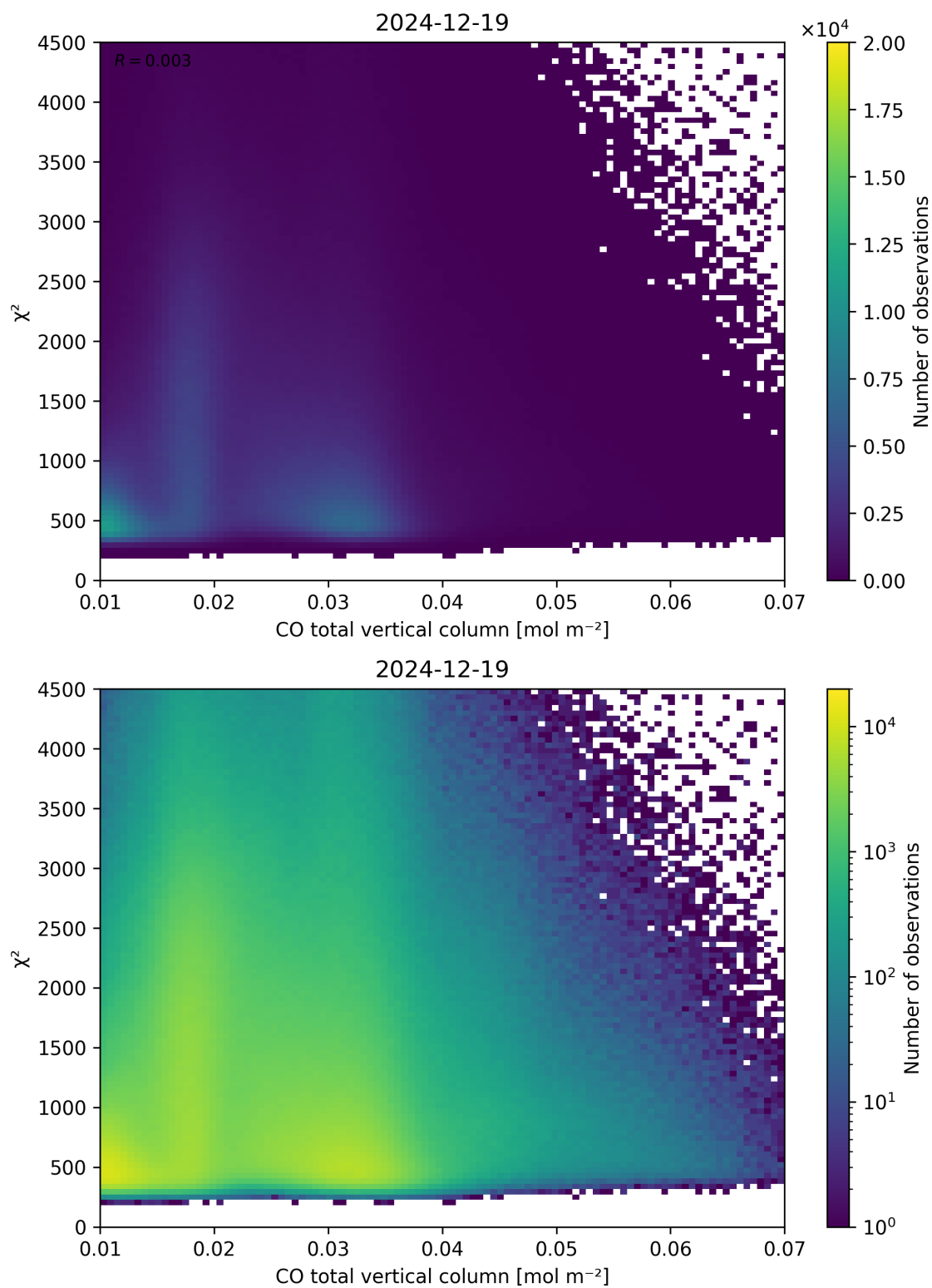
Figure 35: Scatter density plot of “CO total vertical column” against “ \chi^2 ” for 2024-12-18 to 2024-12-20.
