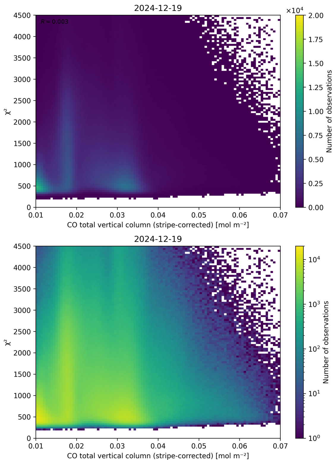
Figure 37: Scatter density plot of “CO total vertical column (stripe-corrected)” against “ \chi^2 ” for 2024-12-18 to 2024-12-20.
