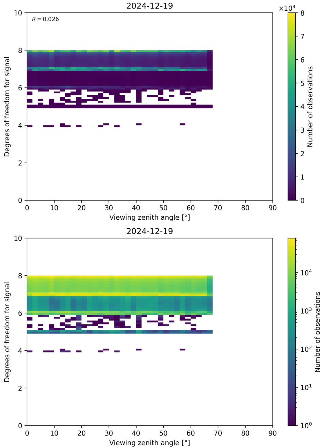
Figure 73: Scatter density plot of “Viewing zenith angle” against “Degrees of freedom for signal” for 2024-12-18 to 2024-12-20.
