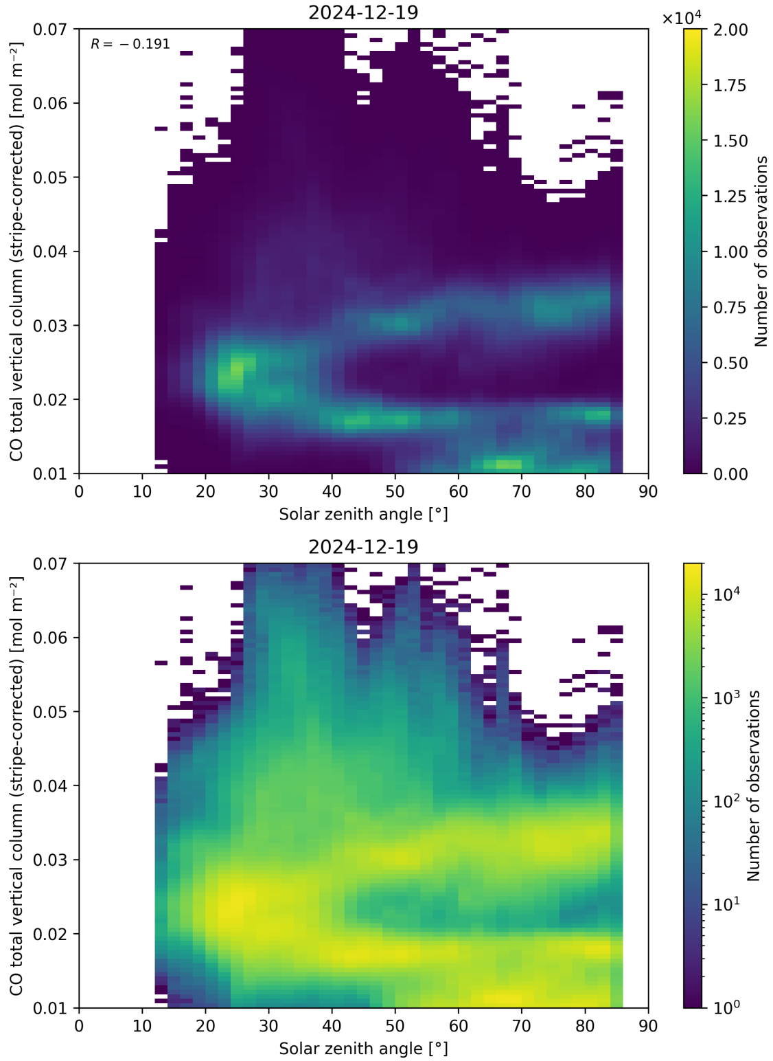
Figure 62: Scatter density plot of “Solar zenith angle” against “CO total vertical column (stripe-corrected)” for 2024-12-18 to 2024-12-20.
