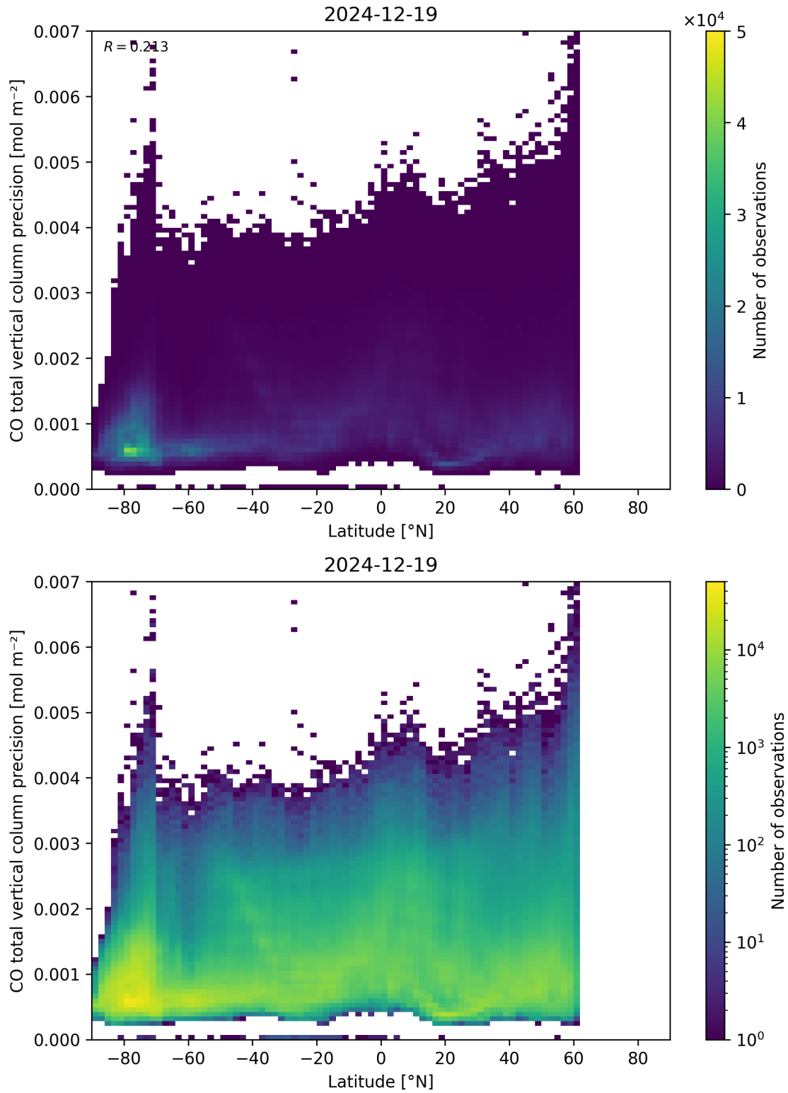
Figure 53: Scatter density plot of “Latitude” against “CO total vertical column precision” for 2024-12-18 to 2024-12-20.
