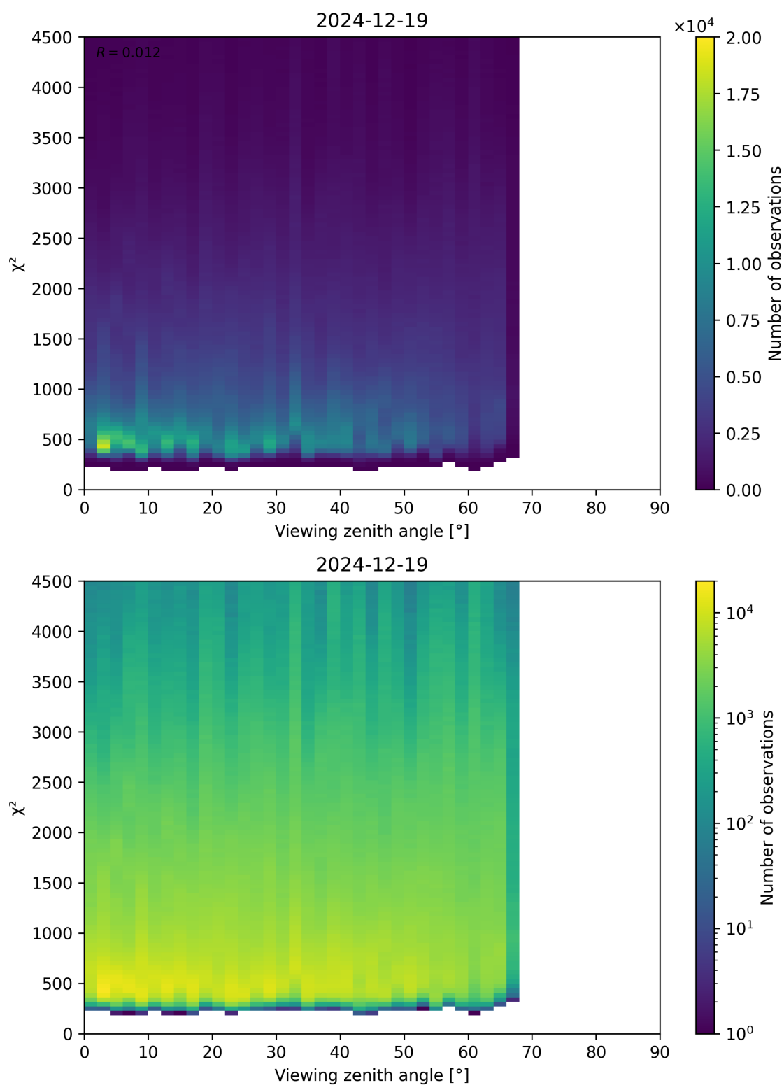
Figure 72: Scatter density plot of “Viewing zenith angle” against “ \chi^2 ” for 2024-12-18 to 2024-12-20.
