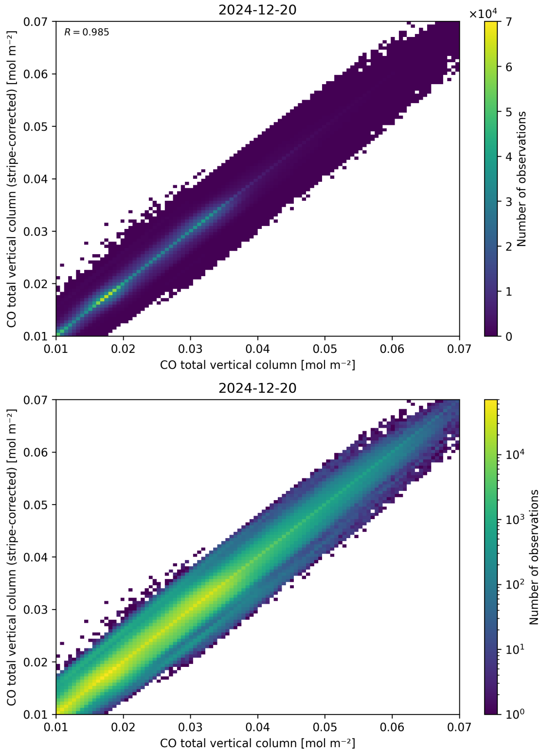
Figure 33: Scatter density plot of “CO total vertical column” against “CO total vertical column (stripe-corrected)” for 2024-12-19 to 2024-12-21.
