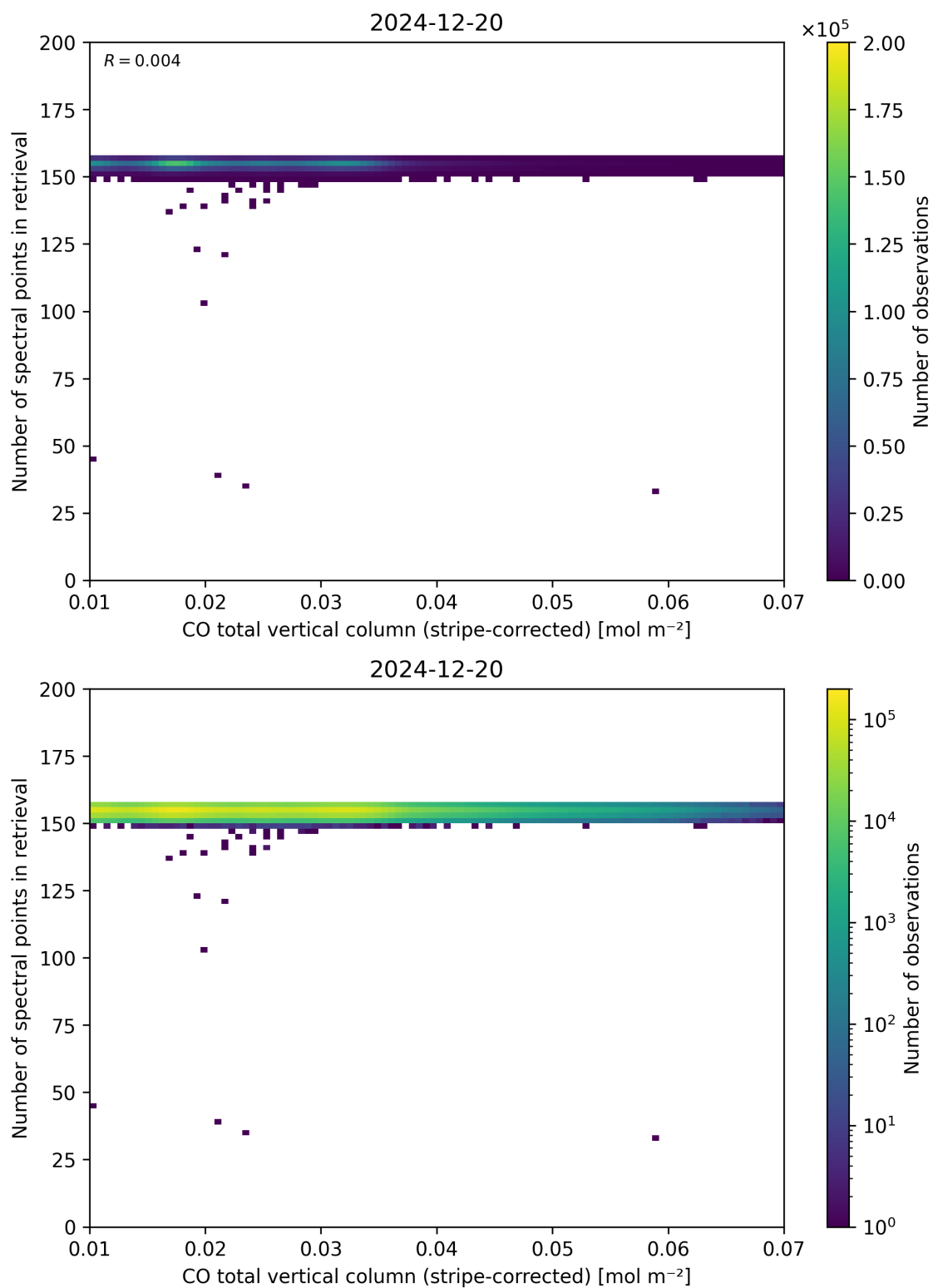
Figure 40: Scatter density plot of “CO total vertical column (stripe-corrected)” against “Number of spectral points in retrieval” for 2024-12-19 to 2024-12-21.
