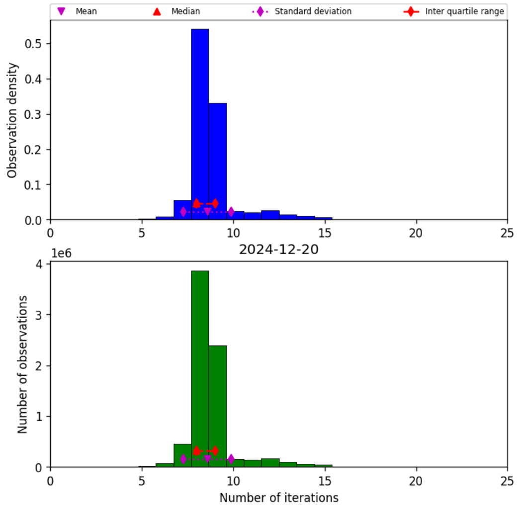
Figure 24: Histogram of “Number of iterations” for 2024-12-19 to 2024-12-21
