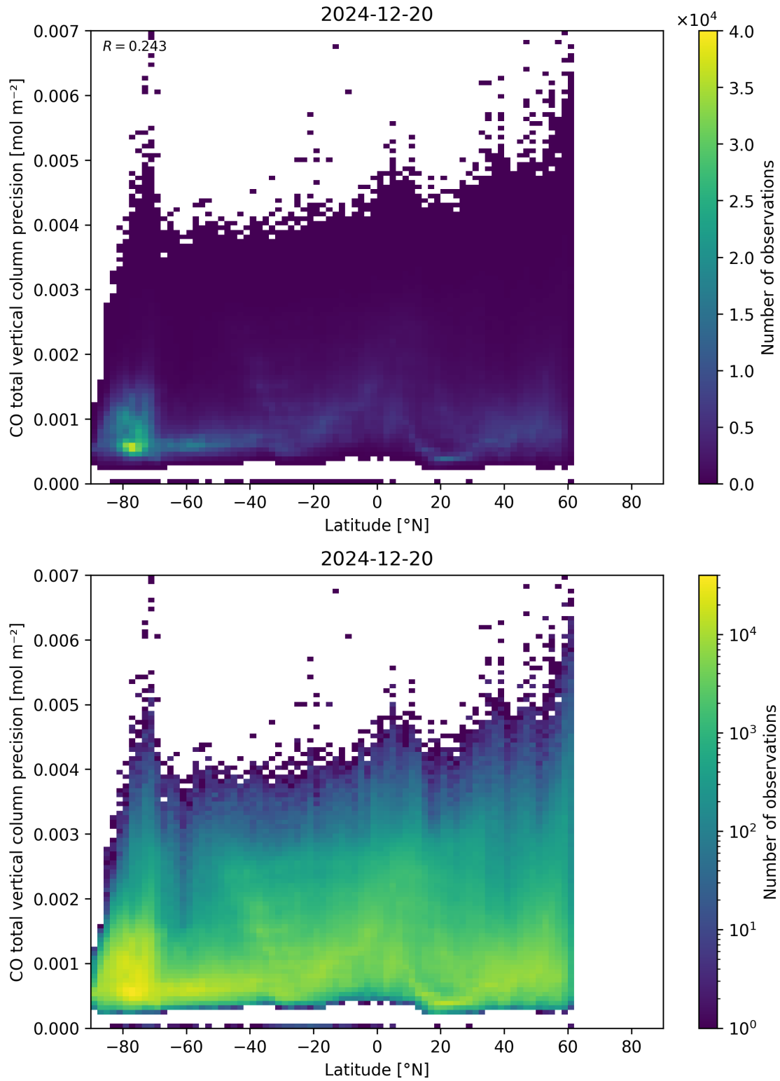
Figure 53: Scatter density plot of “Latitude” against “CO total vertical column precision” for 2024-12-19 to 2024-12-21.
