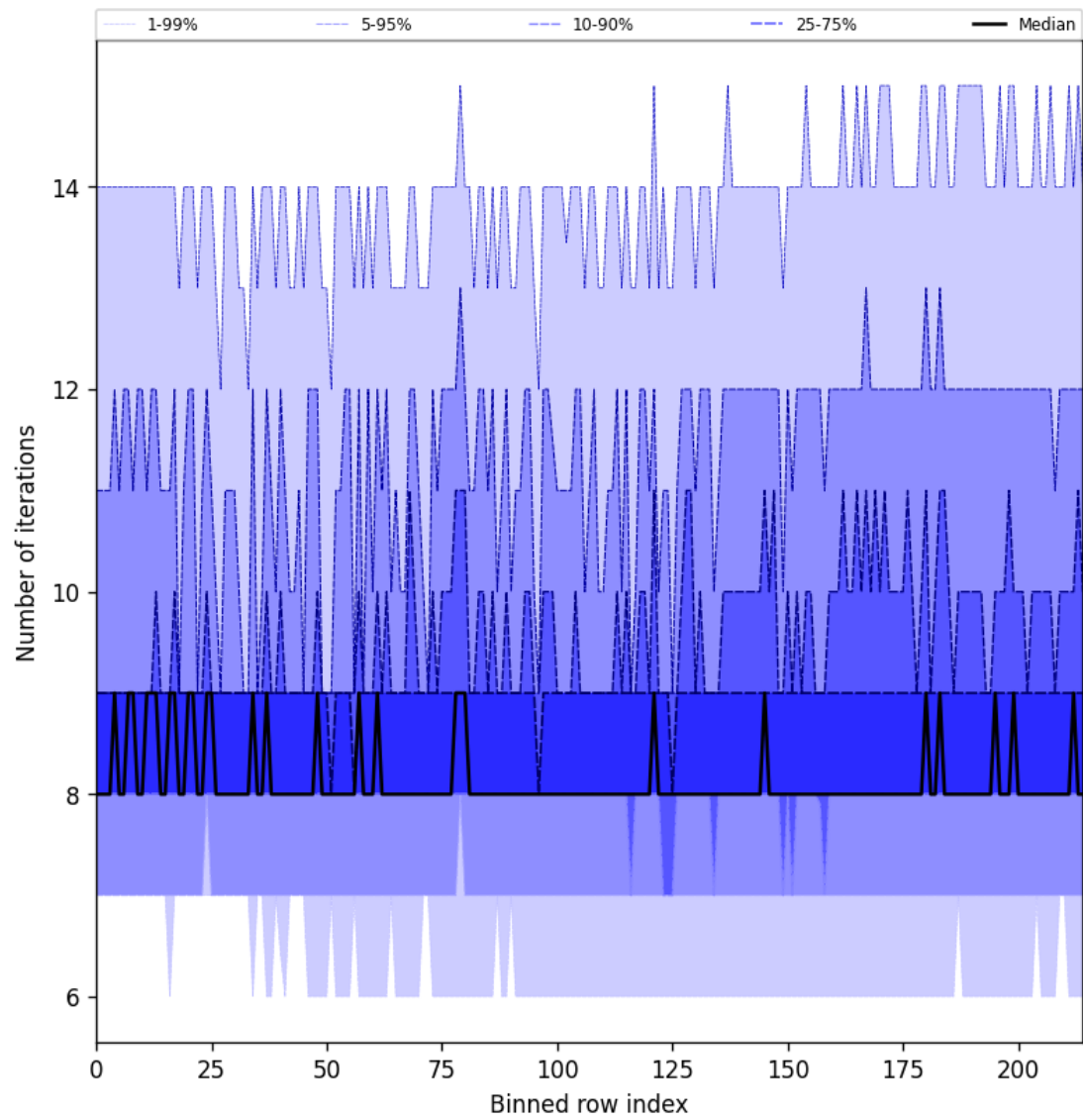
Figure 32: Along track statistics of “Number of iterations” for 2024-12-19 to 2024-12-21
