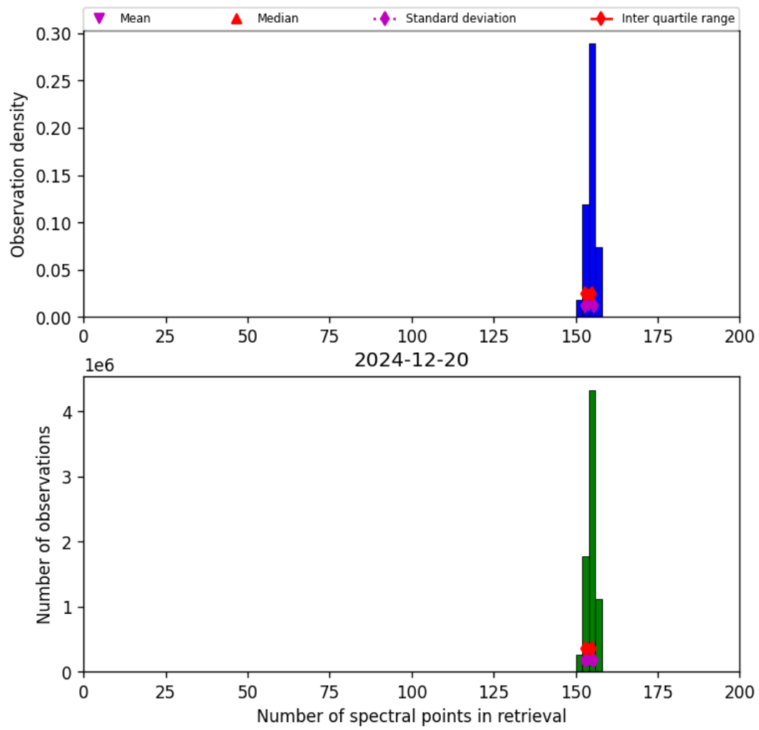
Figure 21: Histogram of “Number of spectral points in retrieval” for 2024-12-19 to 2024-12-21
