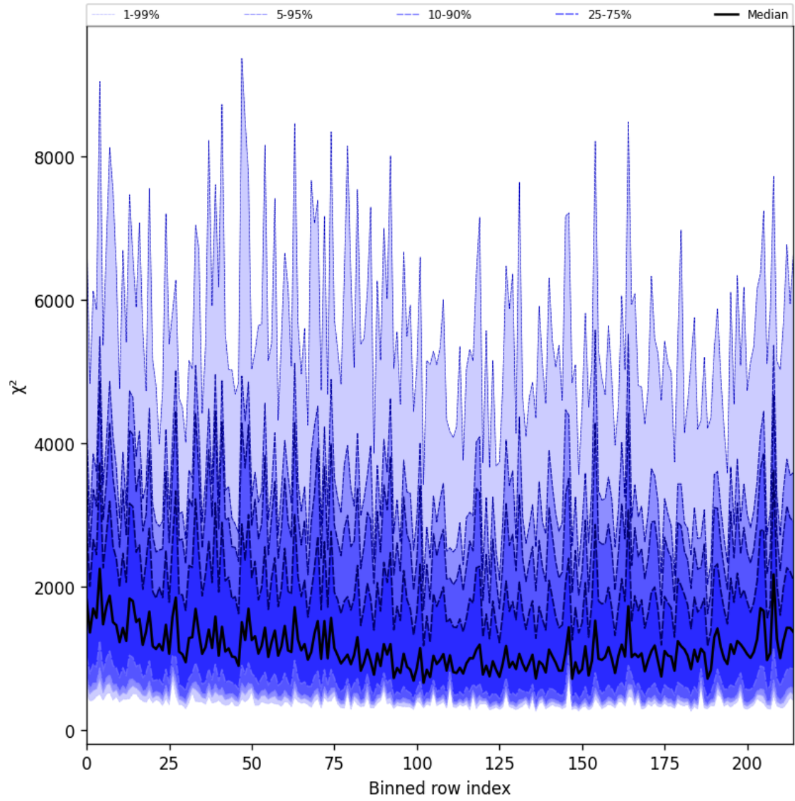
Figure 30: Along track statistics of “ \chi^2 ” for 2024-12-19 to 2024-12-21
