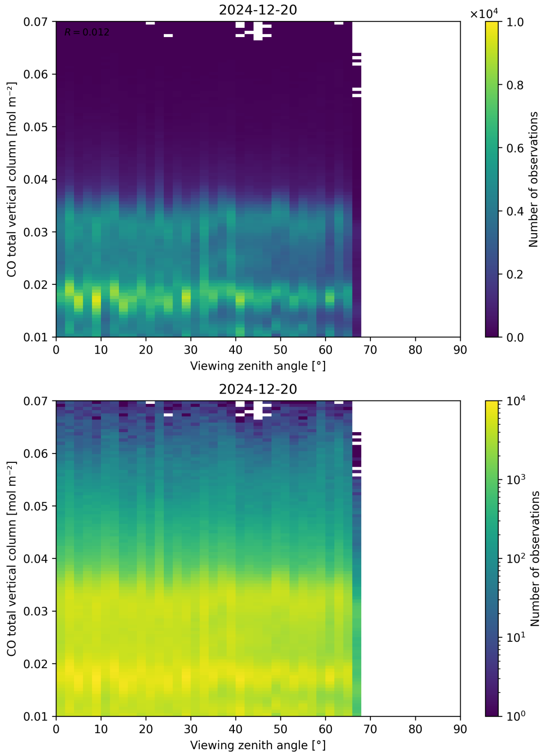
Figure 69: Scatter density plot of “Viewing zenith angle” against “CO total vertical column” for 2024-12-19 to 2024-12-21.
