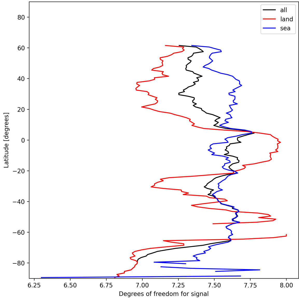
Figure 15: Zonal average of “Degrees of freedom for signal” for 2024-12-19 to 2024-12-21.
