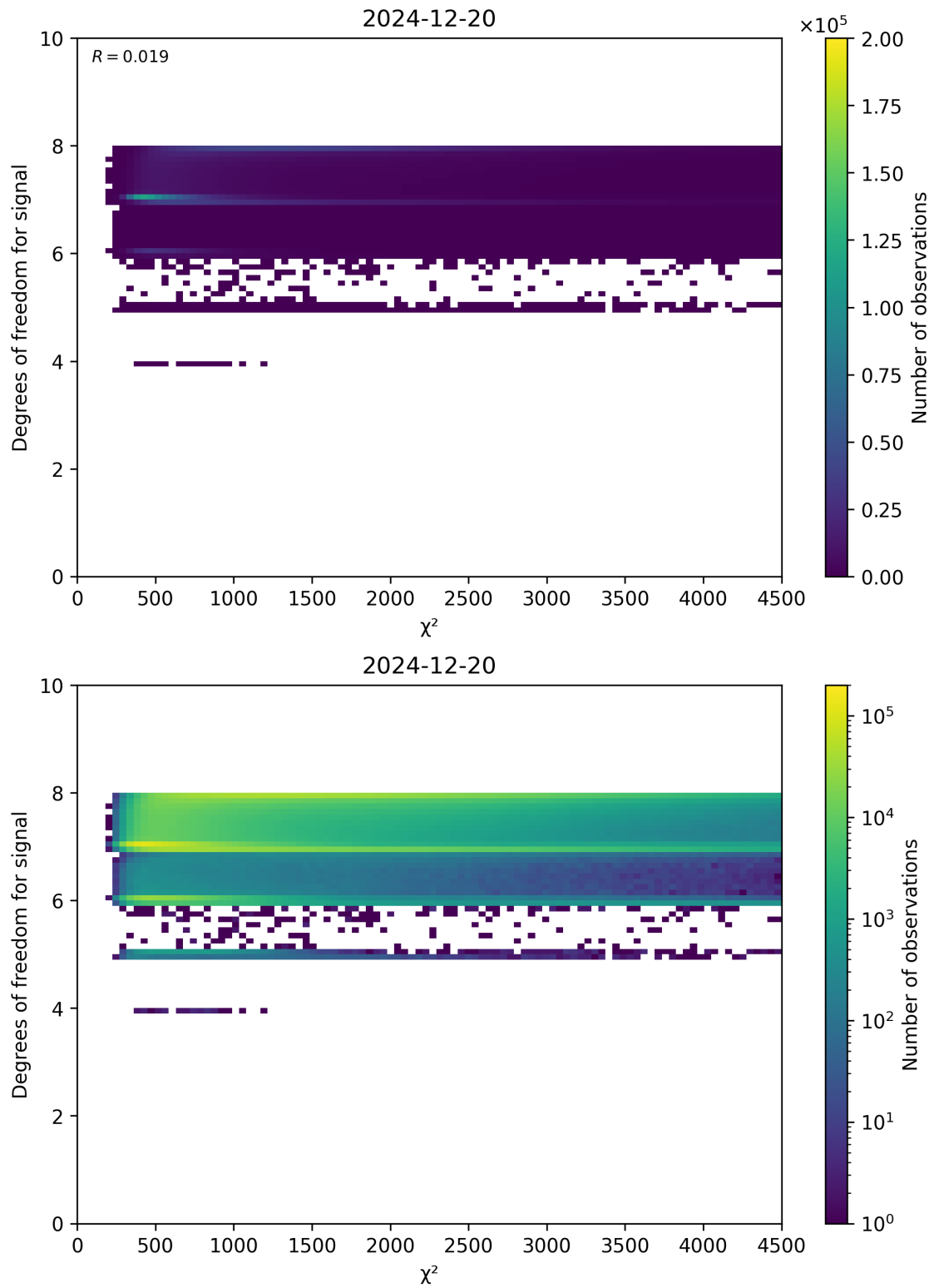
Figure 48: Scatter density plot of “ \chi^2 ” against “Degrees of freedom for signal” for 2024-12-19 to 2024-12-21.
