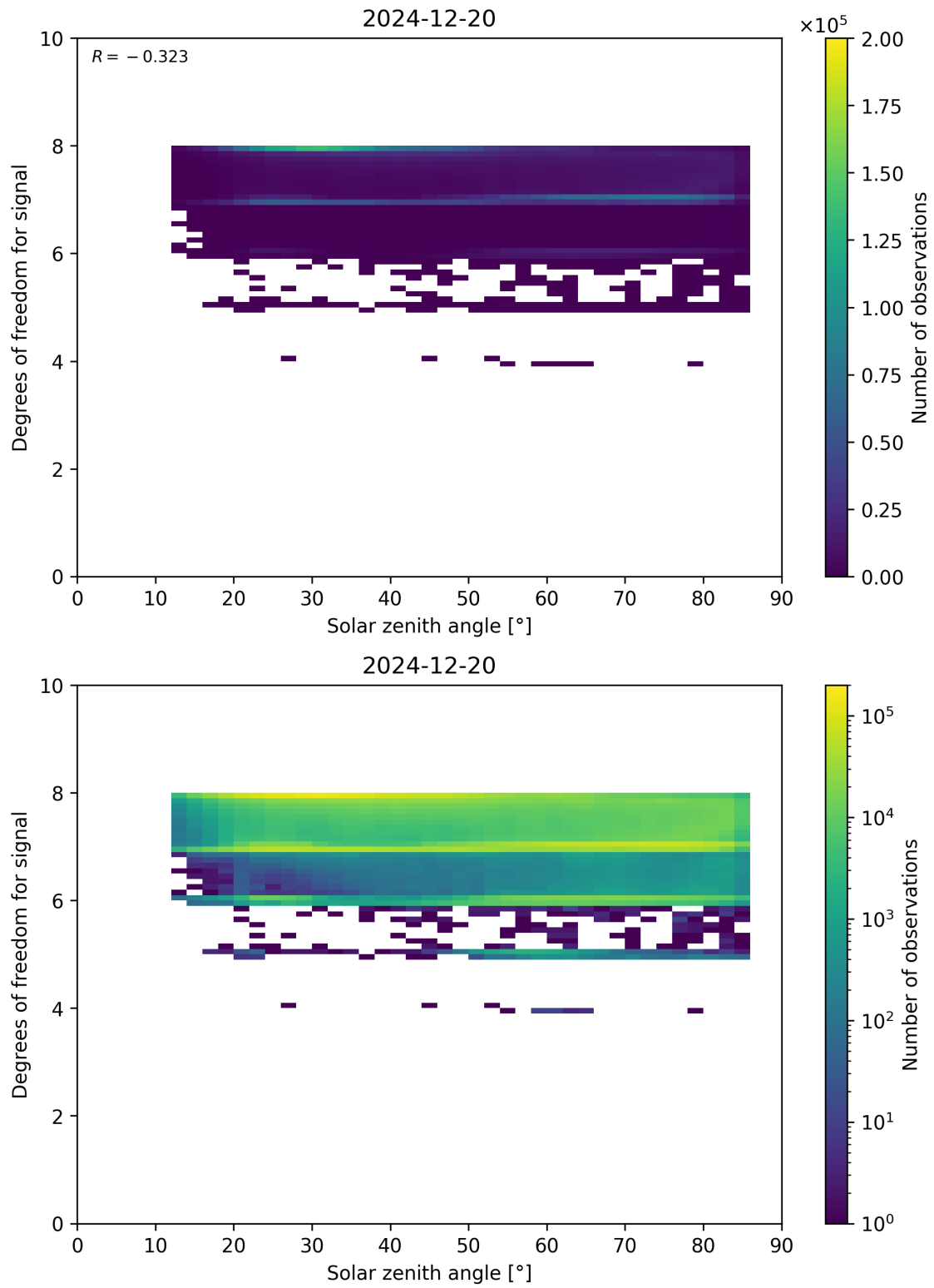
Figure 65: Scatter density plot of “Solar zenith angle” against “Degrees of freedom for signal” for 2024-12-19 to 2024-12-21.
