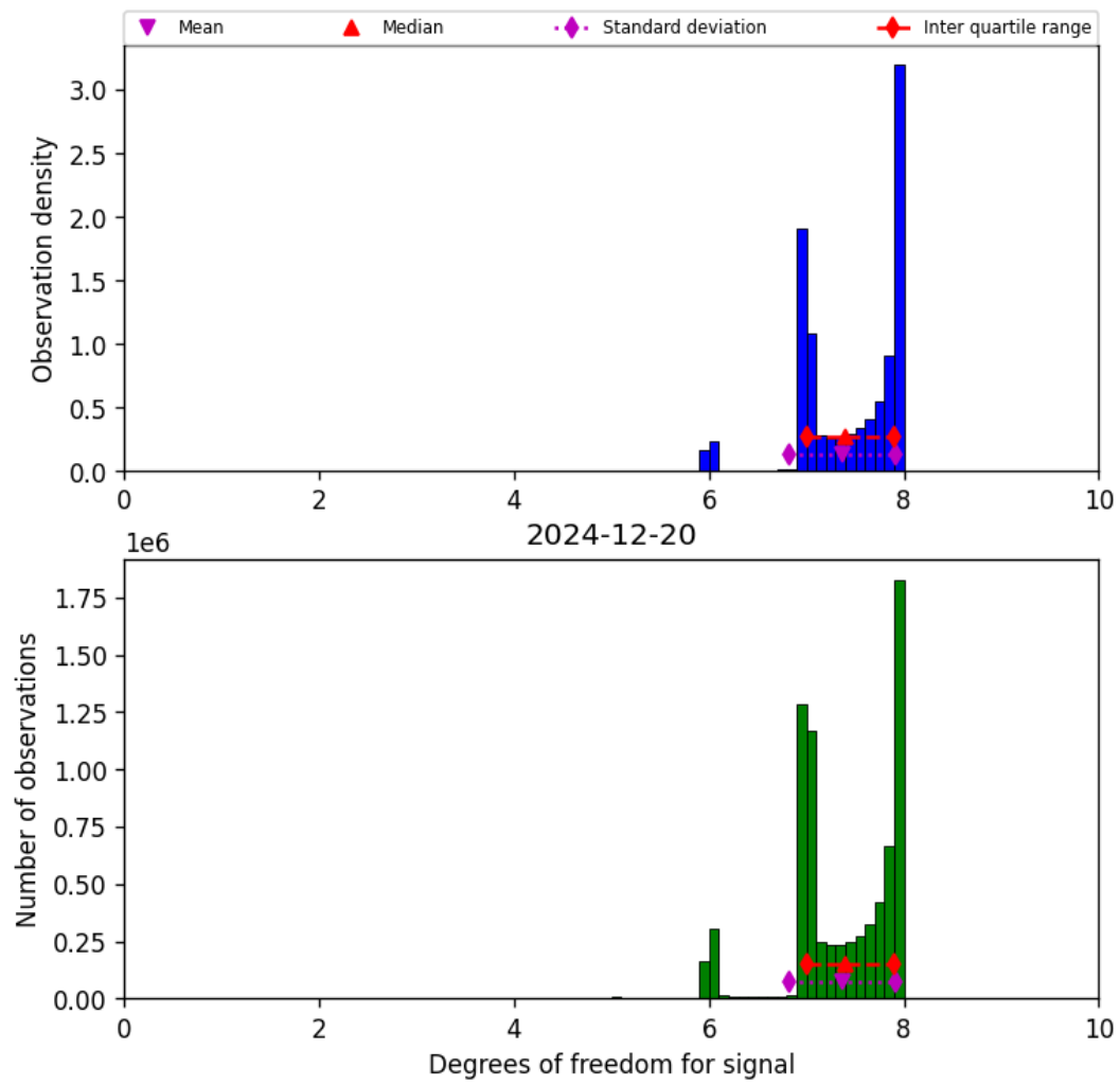
Figure 23: Histogram of “Degrees of freedom for signal” for 2024-12-19 to 2024-12-21
