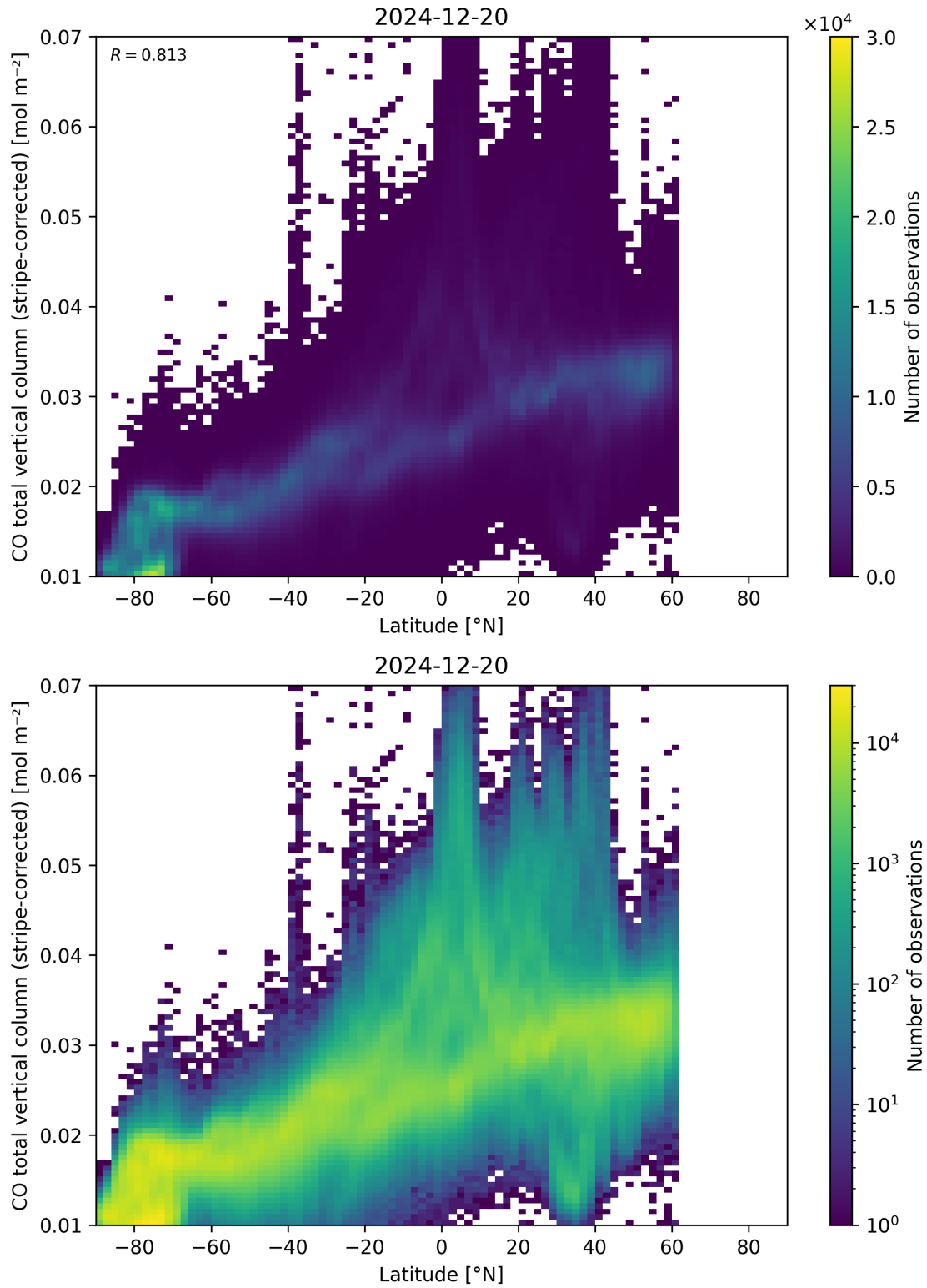
Figure 52: Scatter density plot of “Latitude” against “CO total vertical column (stripe-corrected)” for 2024-12-19 to 2024-12-21.
