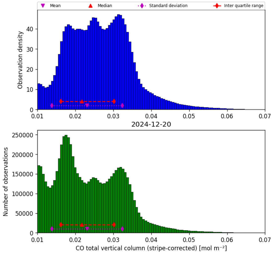
Figure 19: Histogram of “CO total vertical column (stripe-corrected)” for 2024-12-19 to 2024-12-21
