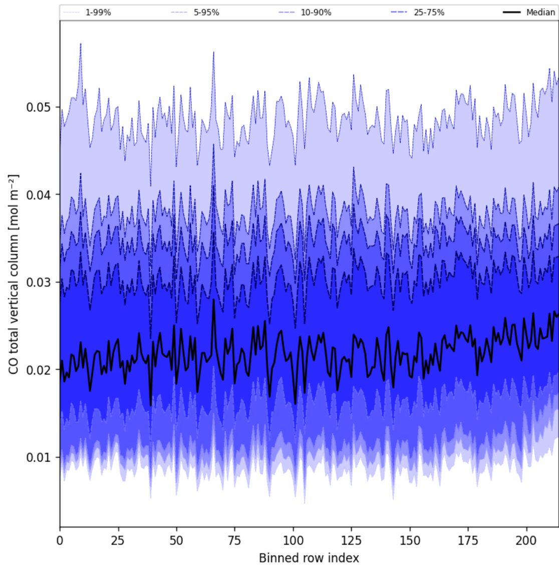
Figure 26: Along track statistics of “CO total vertical column” for 2024-12-19 to 2024-12-21
