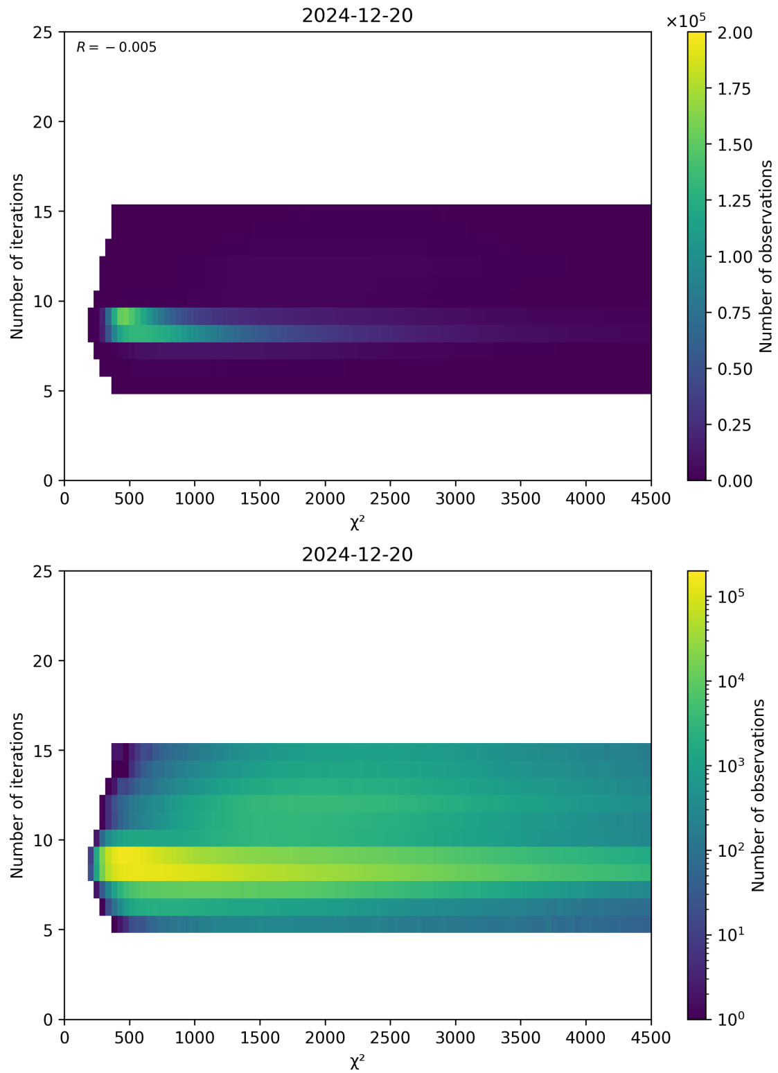
Figure 49: Scatter density plot of “ \chi^2 ” against “Number of iterations” for 2024-12-19 to 2024-12-21.
