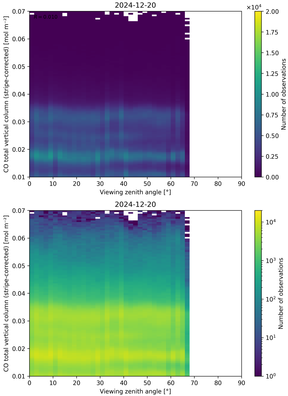
Figure 70: Scatter density plot of “Viewing zenith angle” against “CO total vertical column (stripe-corrected)” for 2024-12-19 to 2024-12-21.
