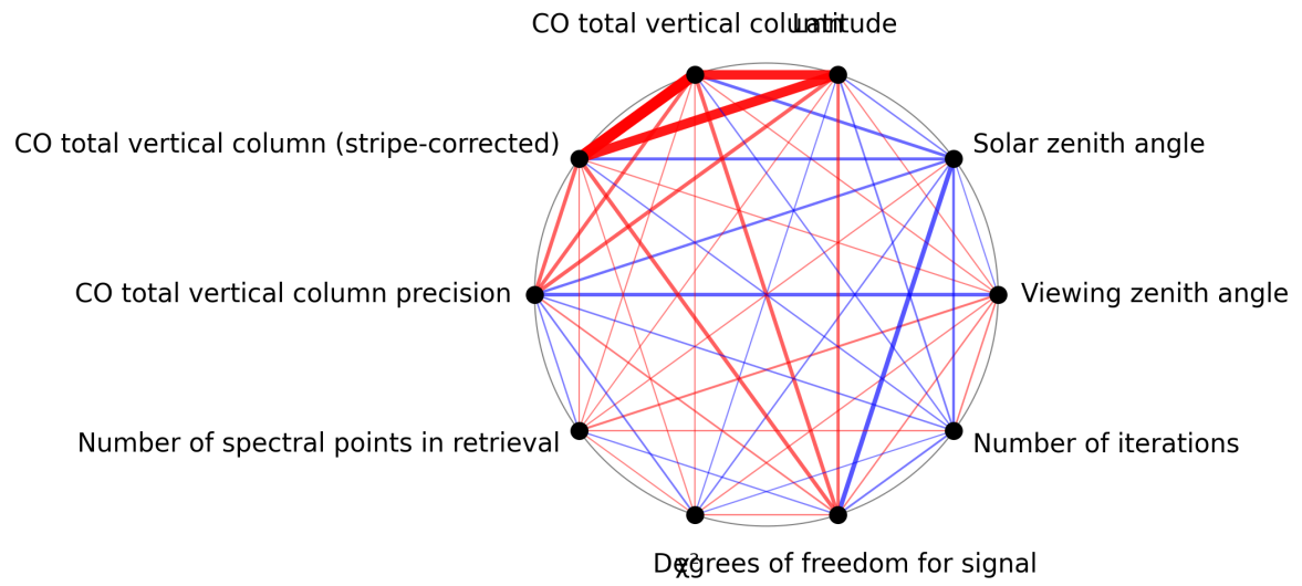
Figure 1: Map of correlation graph for 2024-12-19 to 2024-12-21.
