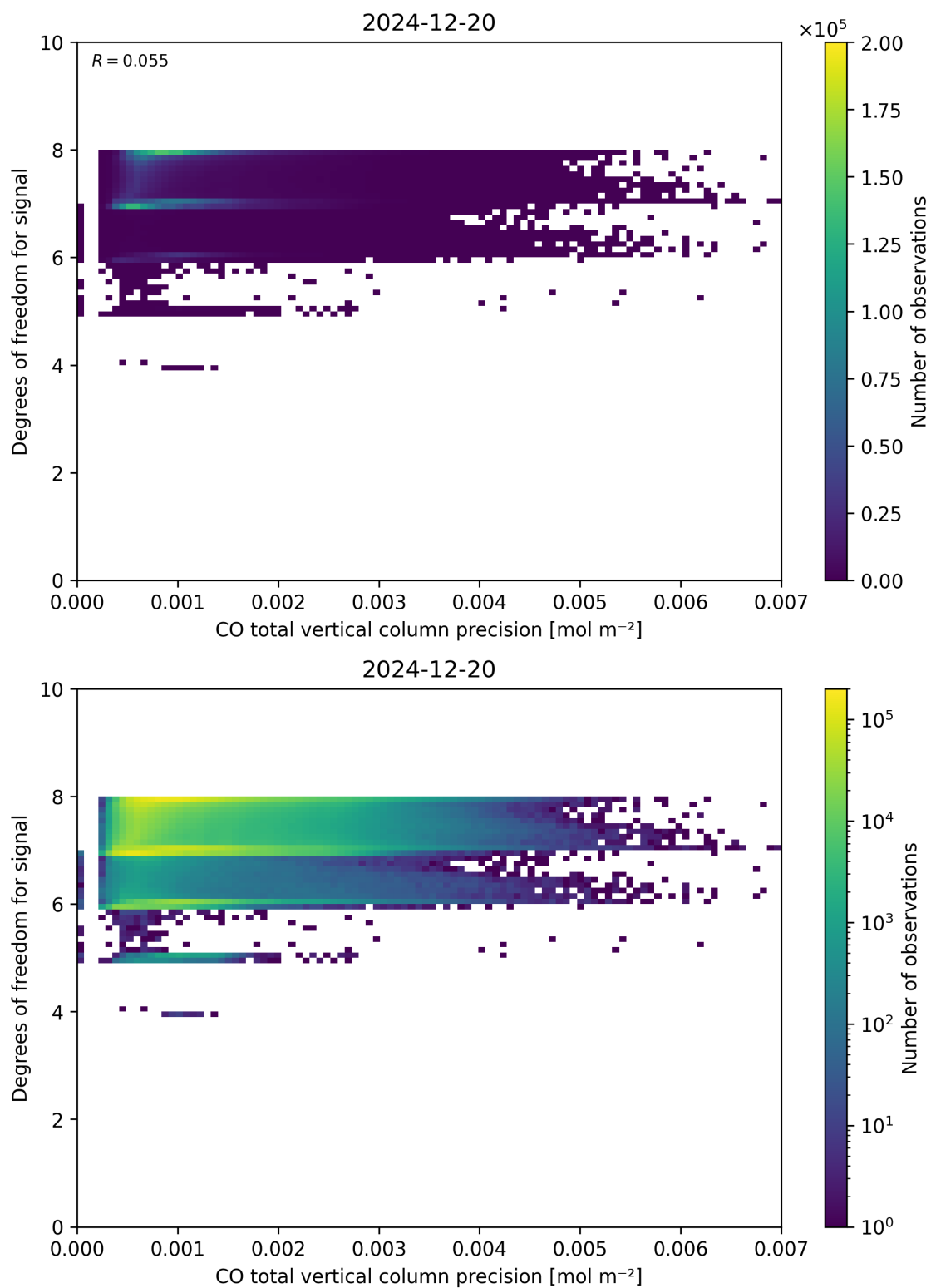
Figure 45: Scatter density plot of “CO total vertical column precision” against “Degrees of freedom for signal” for 2024-12-19 to 2024-12-21.
