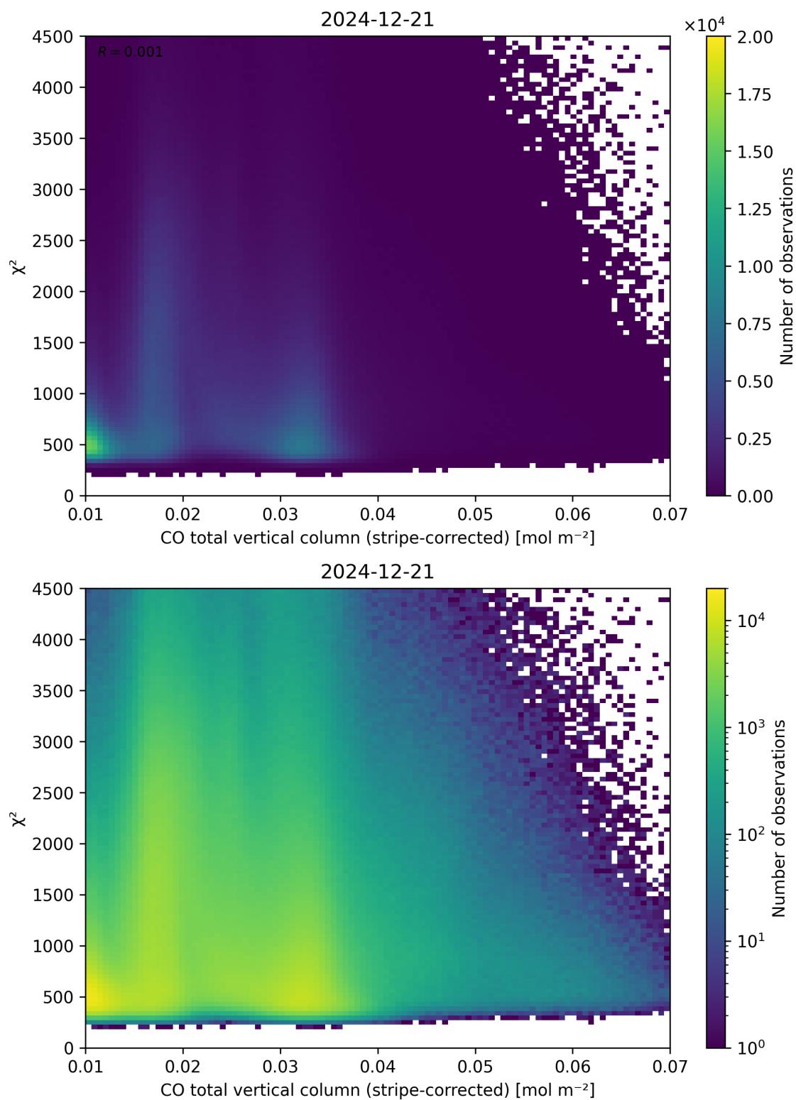
Figure 37: Scatter density plot of “CO total vertical column (stripe-corrected)” against “ \chi^2 ” for 2024-12-20 to 2024-12-22.
