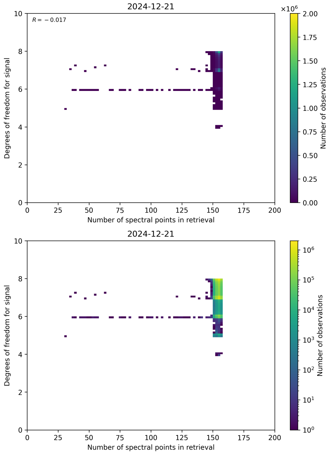
Figure 59: Scatter density plot of “Number of spectral points in retrieval” against “Degrees of freedom for signal” for 2024-12-20 to 2024-12-22.
