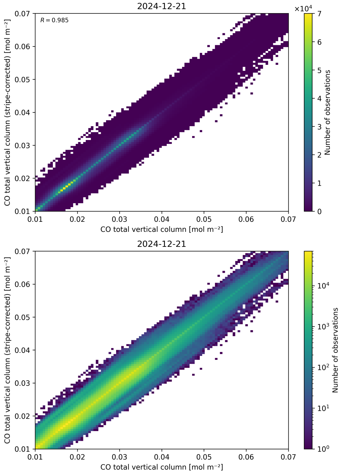
Figure 33: Scatter density plot of “CO total vertical column” against “CO total vertical column (stripe-corrected)” for 2024-12-20 to 2024-12-22.
