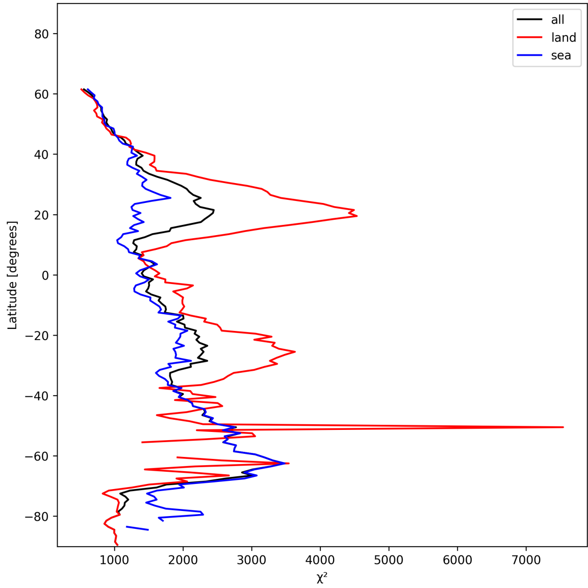
Figure 14: Zonal average of “ \chi^2 ” for 2024-12-20 to 2024-12-22.
