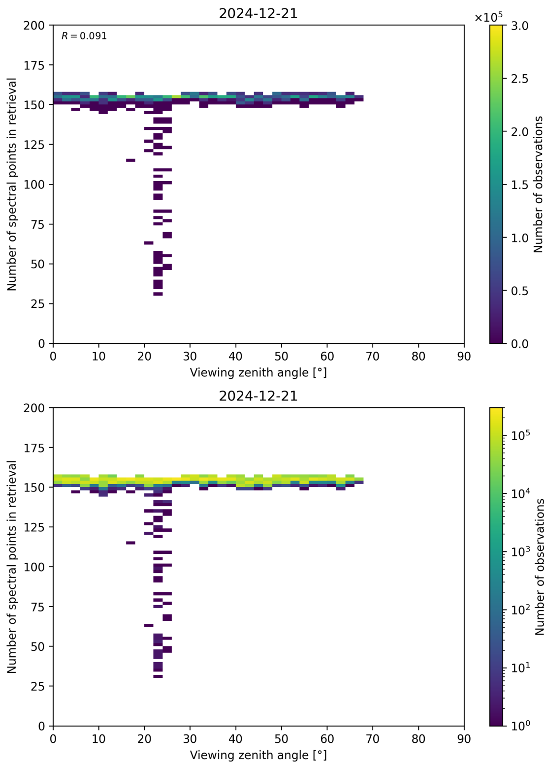
Figure 76: Scatter density plot of “Viewing zenith angle” against “Number of spectral points in retrieval” for 2024-12-20 to 2024-12-22.
