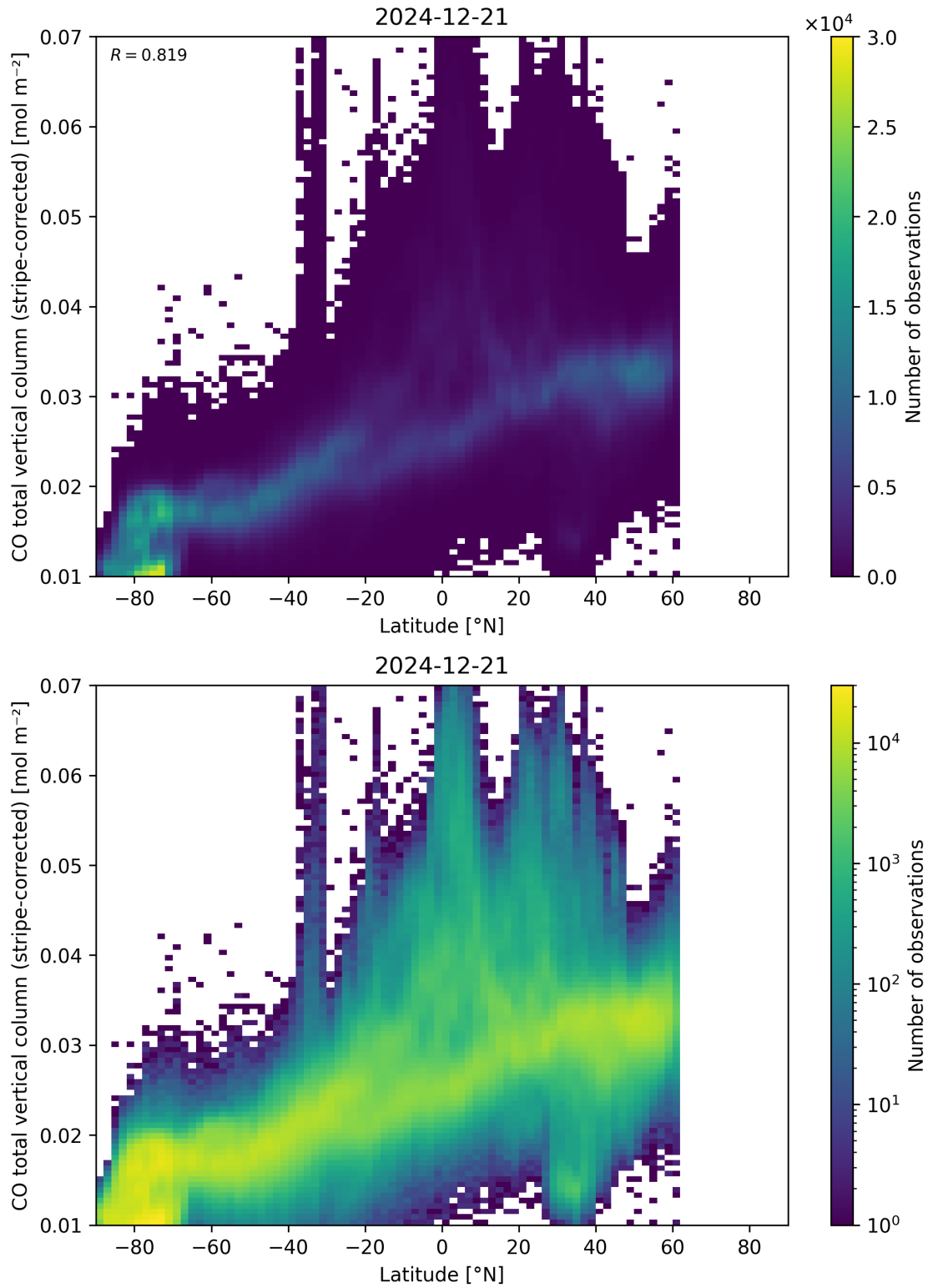
Figure 52: Scatter density plot of “Latitude” against “CO total vertical column (stripe-corrected)” for 2024-12-20 to 2024-12-22.
