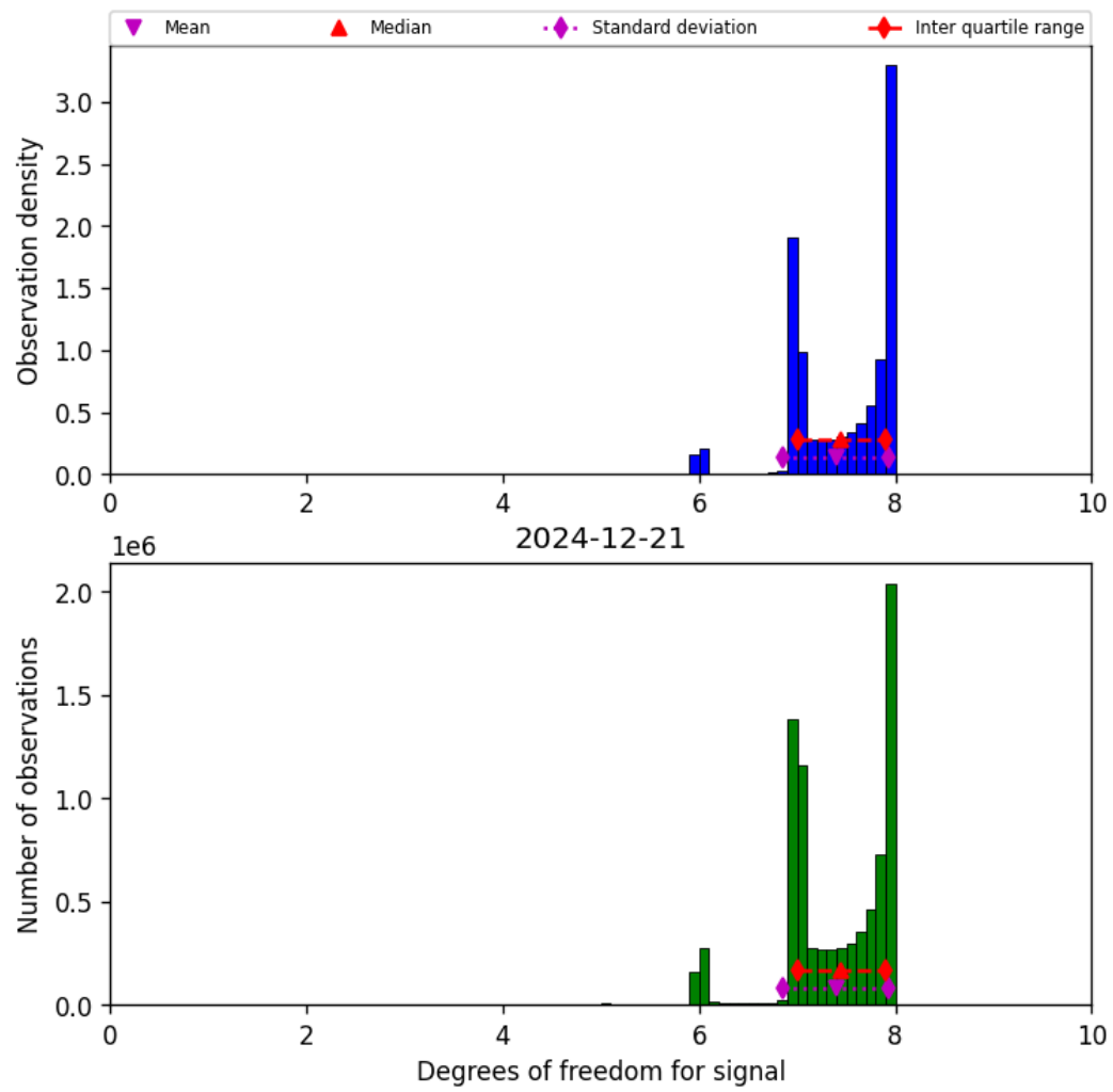
Figure 23: Histogram of “Degrees of freedom for signal” for 2024-12-20 to 2024-12-22
