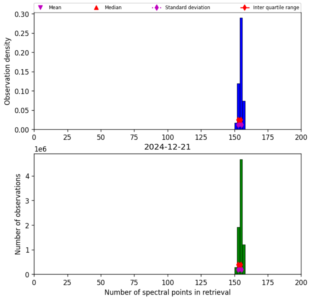
Figure 21: Histogram of “Number of spectral points in retrieval” for 2024-12-20 to 2024-12-22
