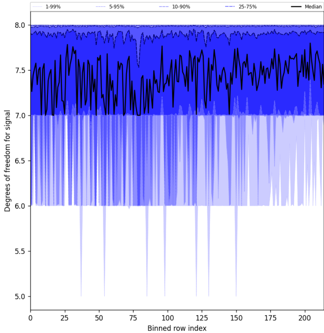
Figure 31: Along track statistics of “Degrees of freedom for signal” for 2024-12-20 to 2024-12-22
