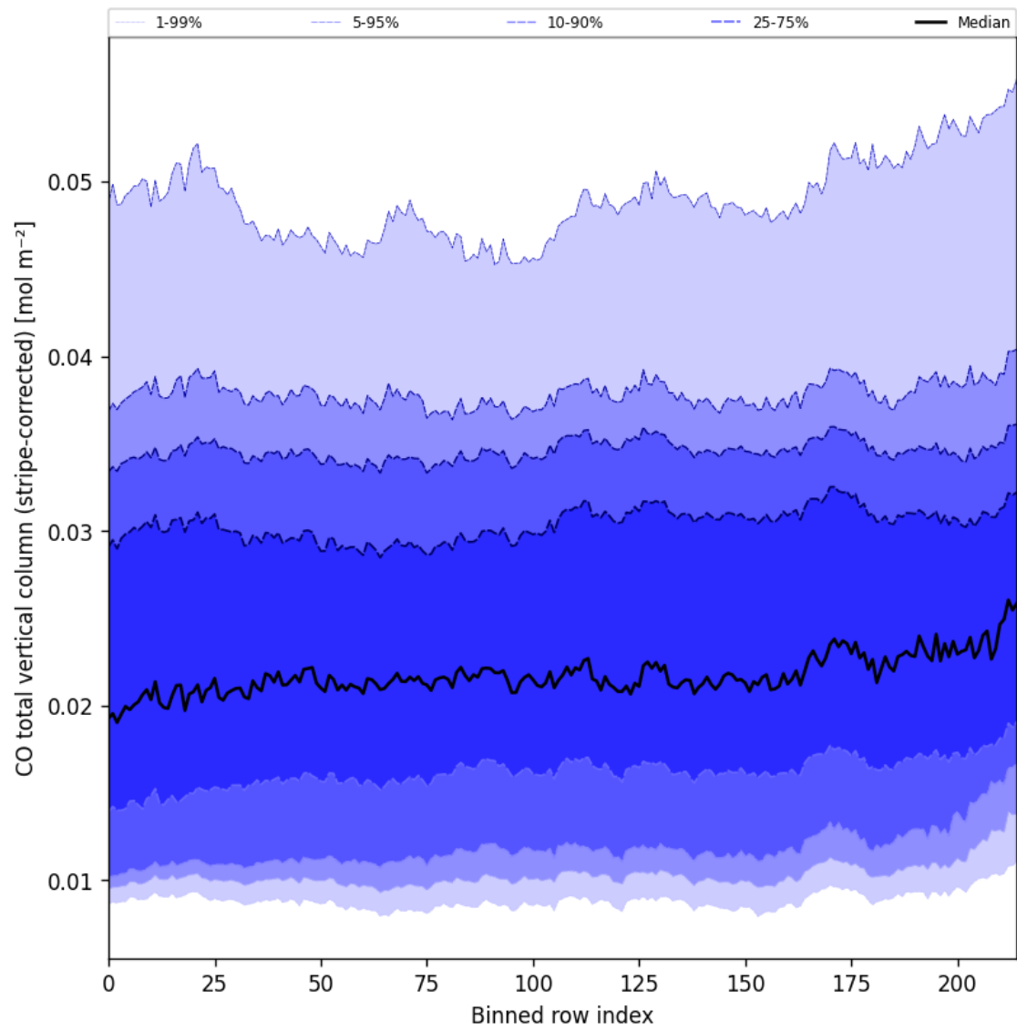
Figure 27: Along track statistics of “CO total vertical column (stripe-corrected)” for 2024-12-20 to 2024-12-22
