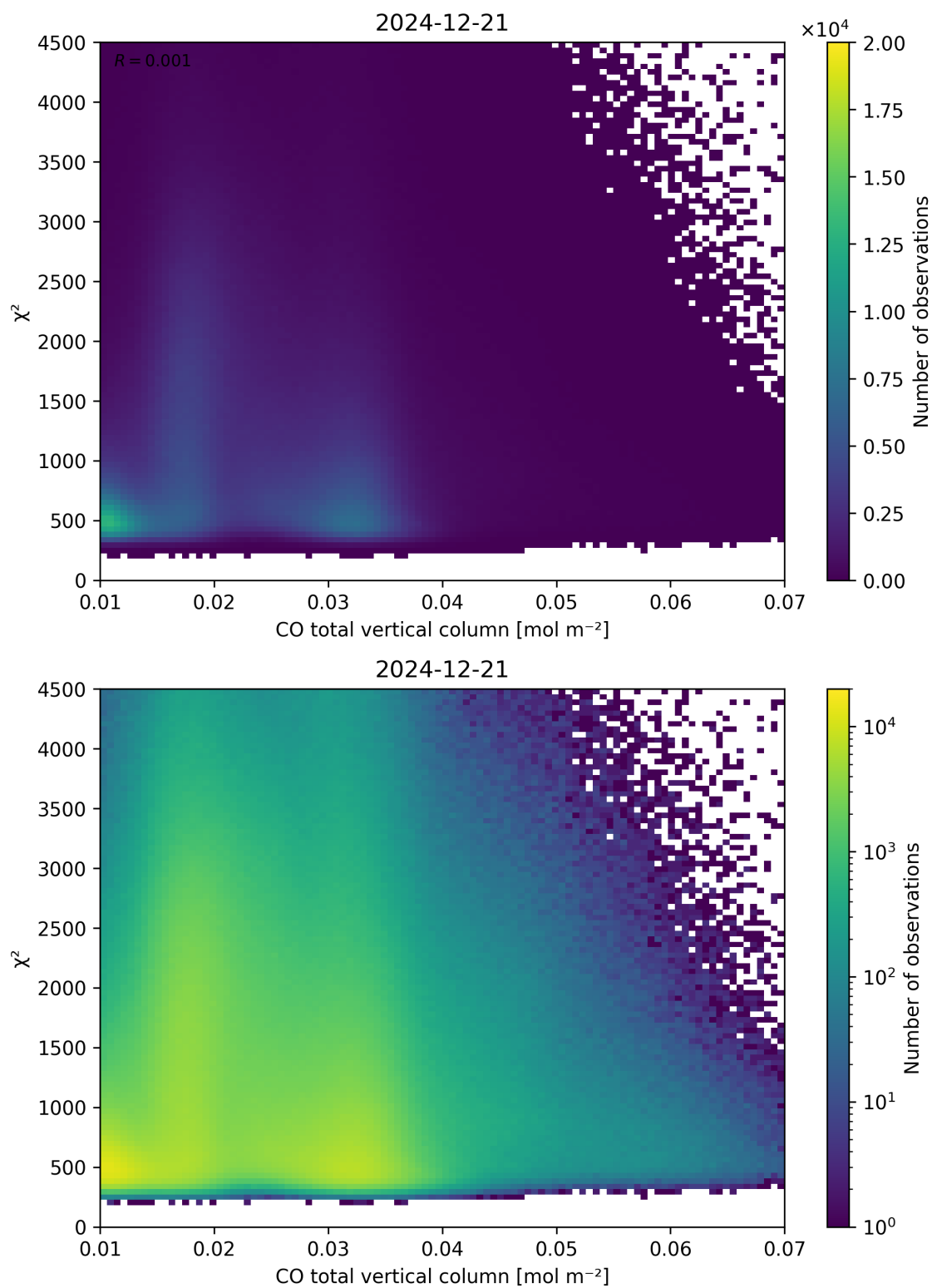
Figure 35: Scatter density plot of “CO total vertical column” against “ \chi^2 ” for 2024-12-20 to 2024-12-22.
