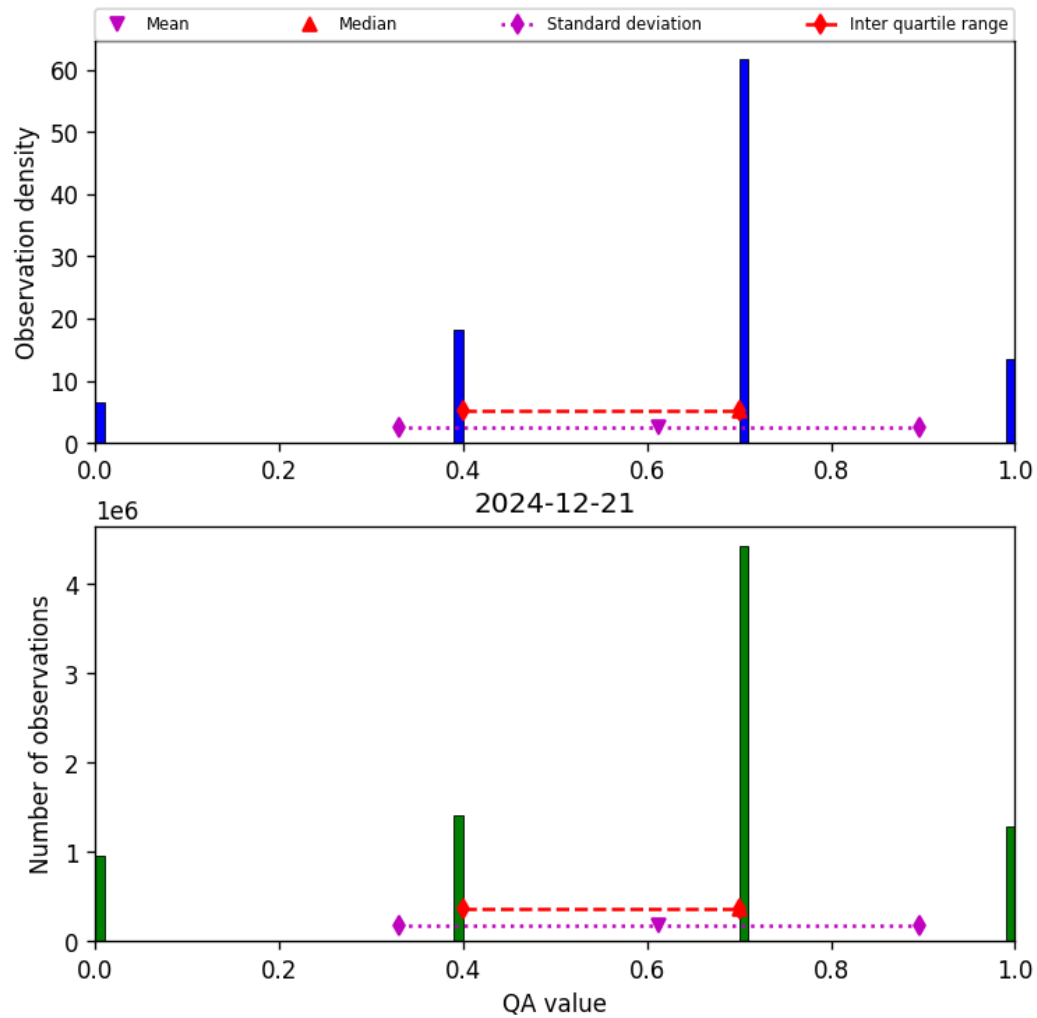
Figure 17: Histogram of “QA value” for 2024-12-20 to 2024-12-22
