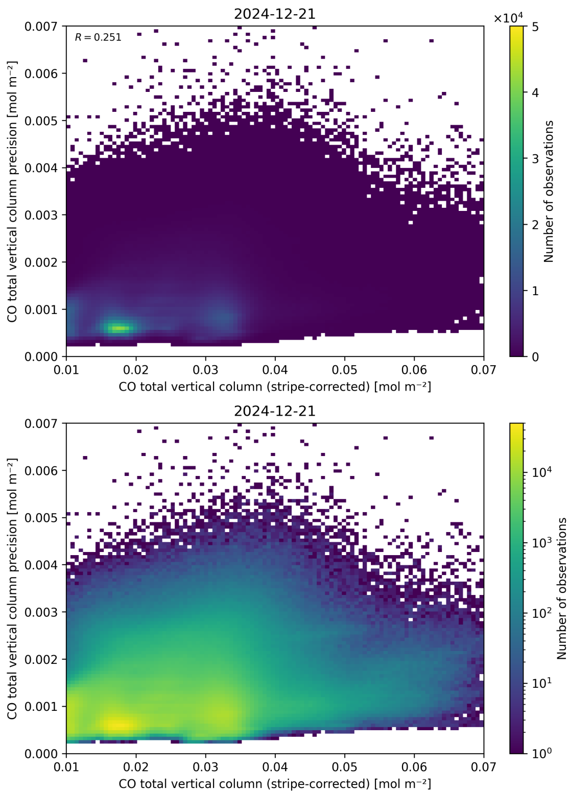
Figure 36: Scatter density plot of “CO total vertical column (stripe-corrected)” against “CO total vertical column precision” for 2024-12-20 to 2024-12-22.
