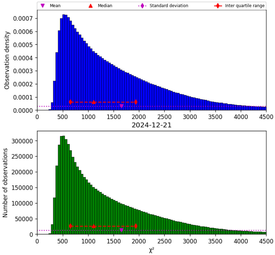
Figure 22: Histogram of “ \chi^2 ” for 2024-12-20 to 2024-12-22
