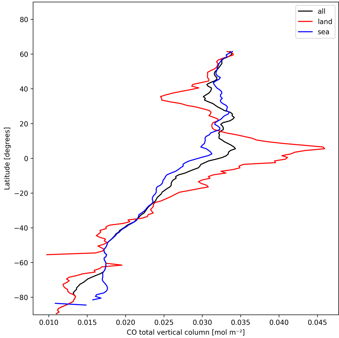
Figure 10: Zonal average of “CO total vertical column” for 2024-12-20 to 2024-12-22.
