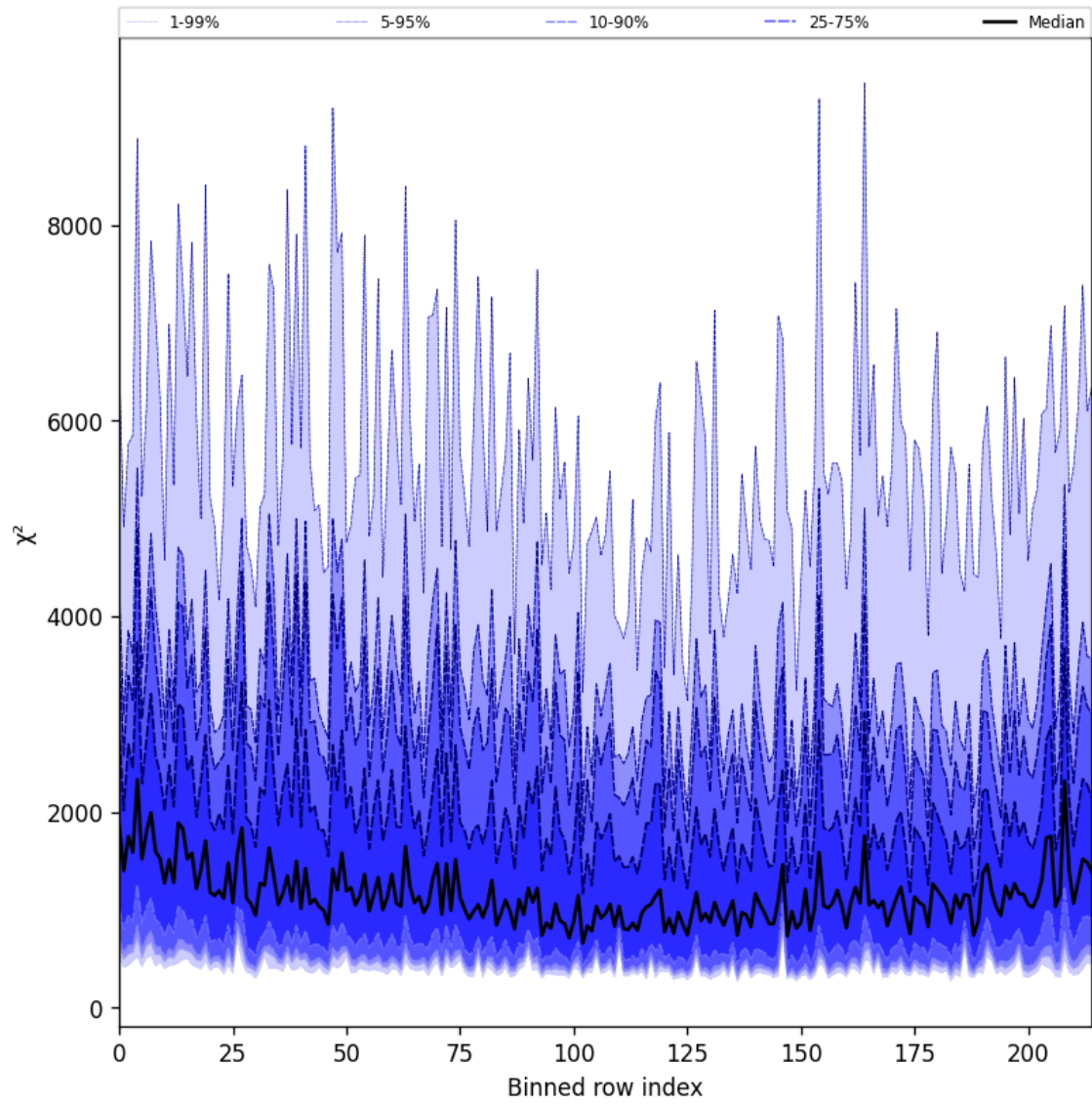
Figure 30: Along track statistics of “ \chi^2 ” for 2024-12-20 to 2024-12-22
