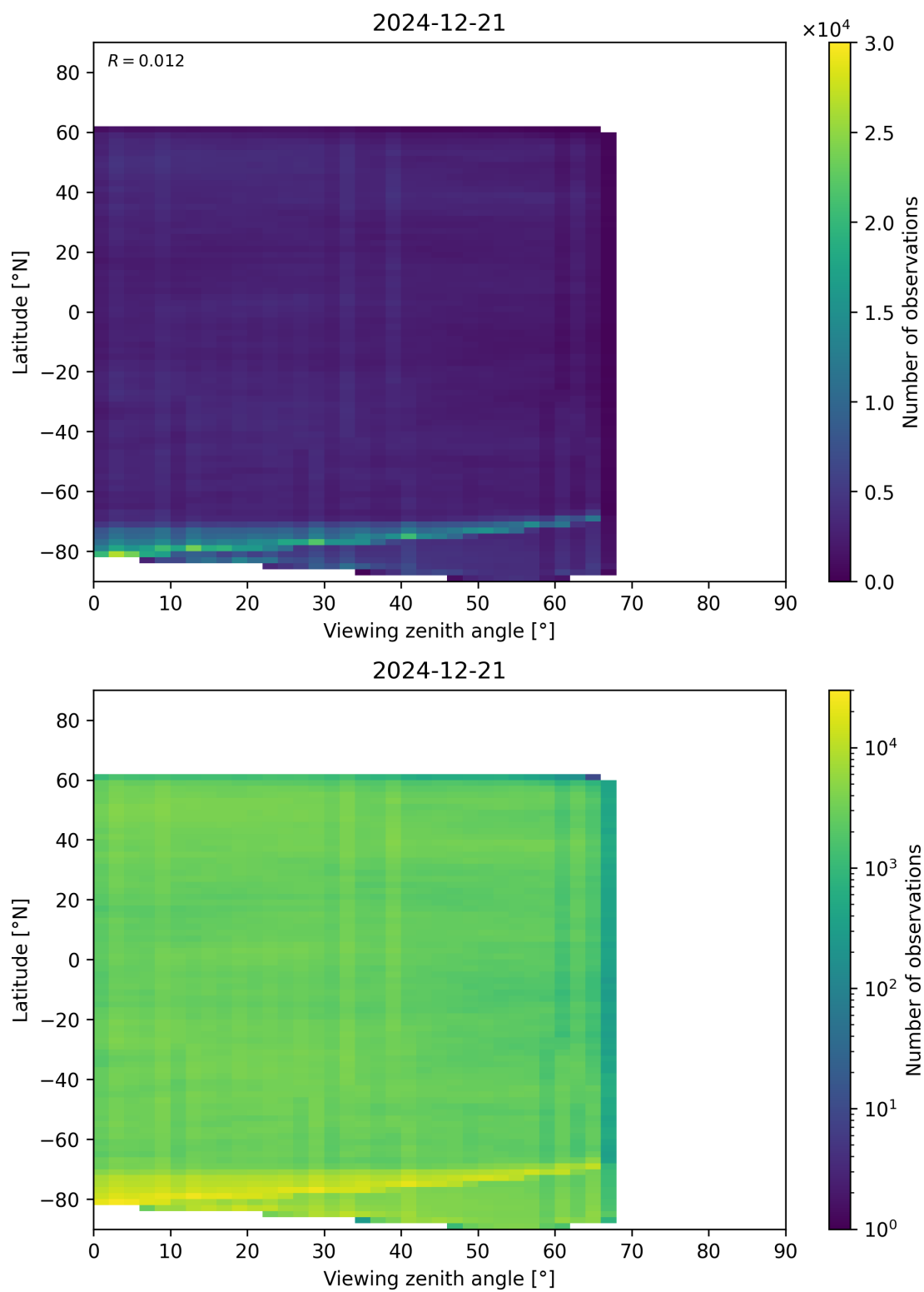
Figure 74: Scatter density plot of “Viewing zenith angle” against “Latitude” for 2024-12-20 to 2024-12-22.
