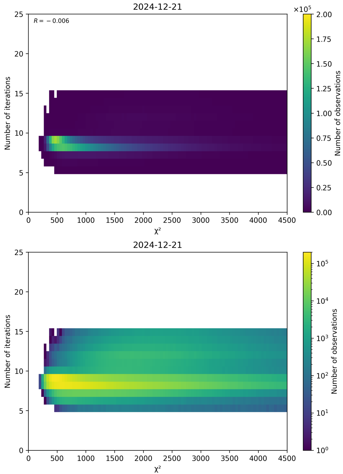
Figure 49: Scatter density plot of “ \chi^2 ” against “Number of iterations” for 2024-12-20 to 2024-12-22.
