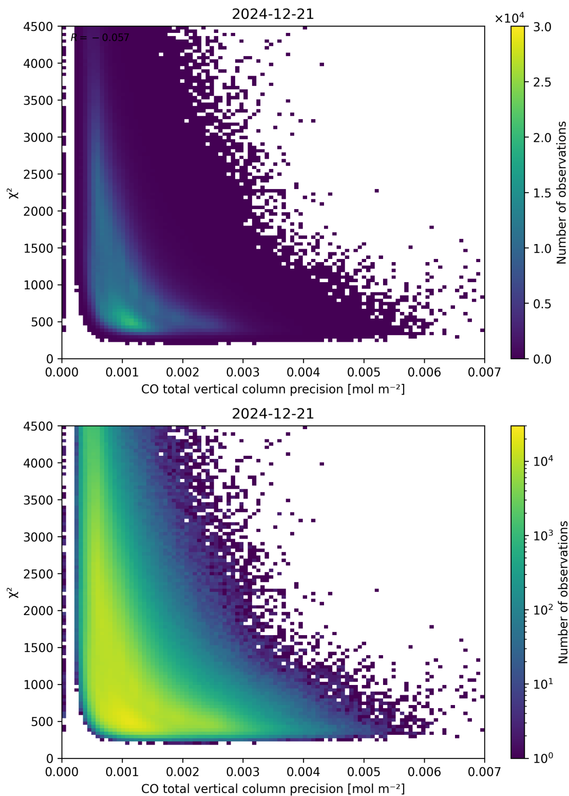
Figure 44: Scatter density plot of “CO total vertical column precision” against “ \chi^2 ” for 2024-12-20 to 2024-12-22.
