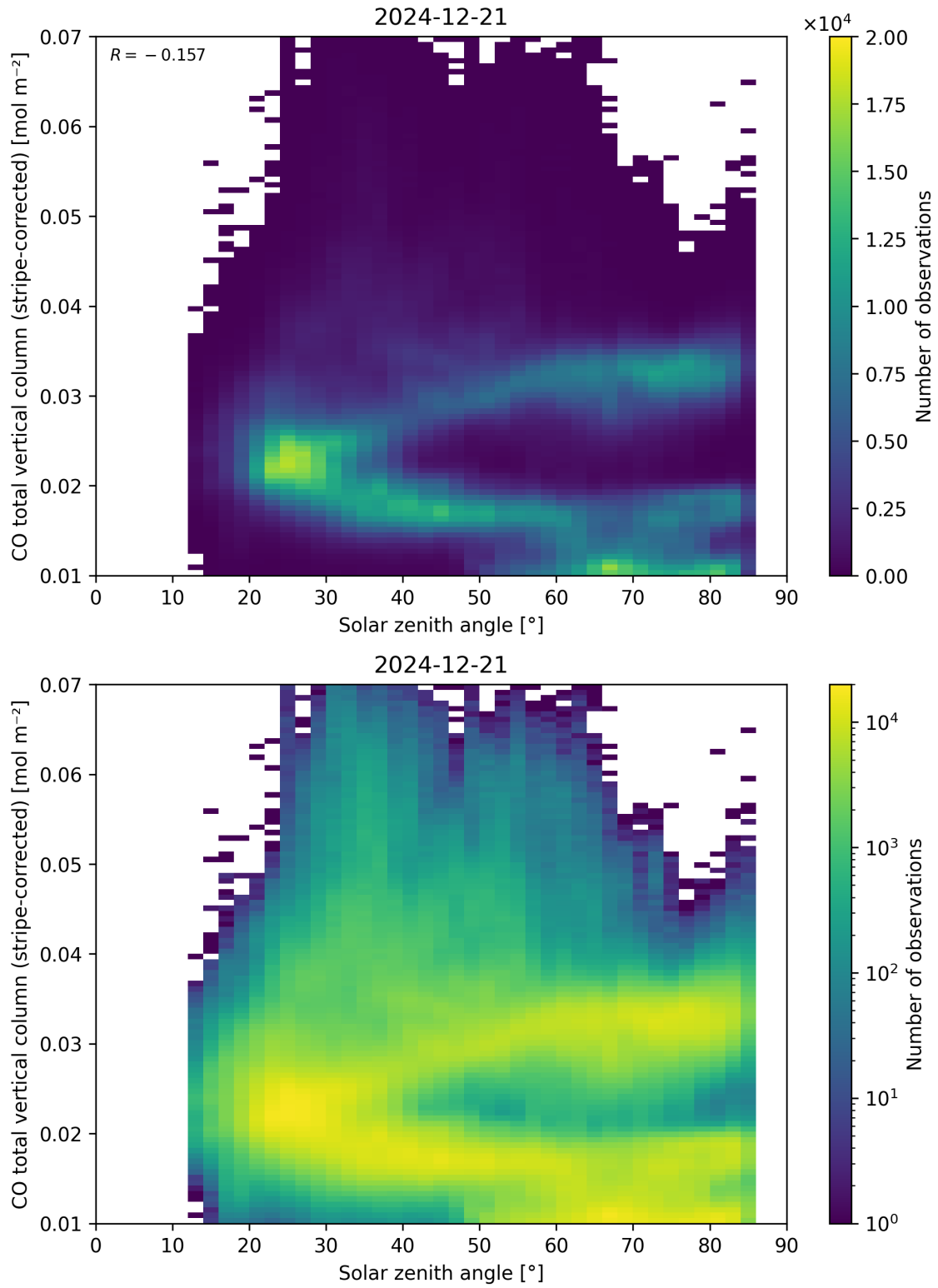
Figure 62: Scatter density plot of “Solar zenith angle” against “CO total vertical column (stripe-corrected)” for 2024-12-20 to 2024-12-22.
