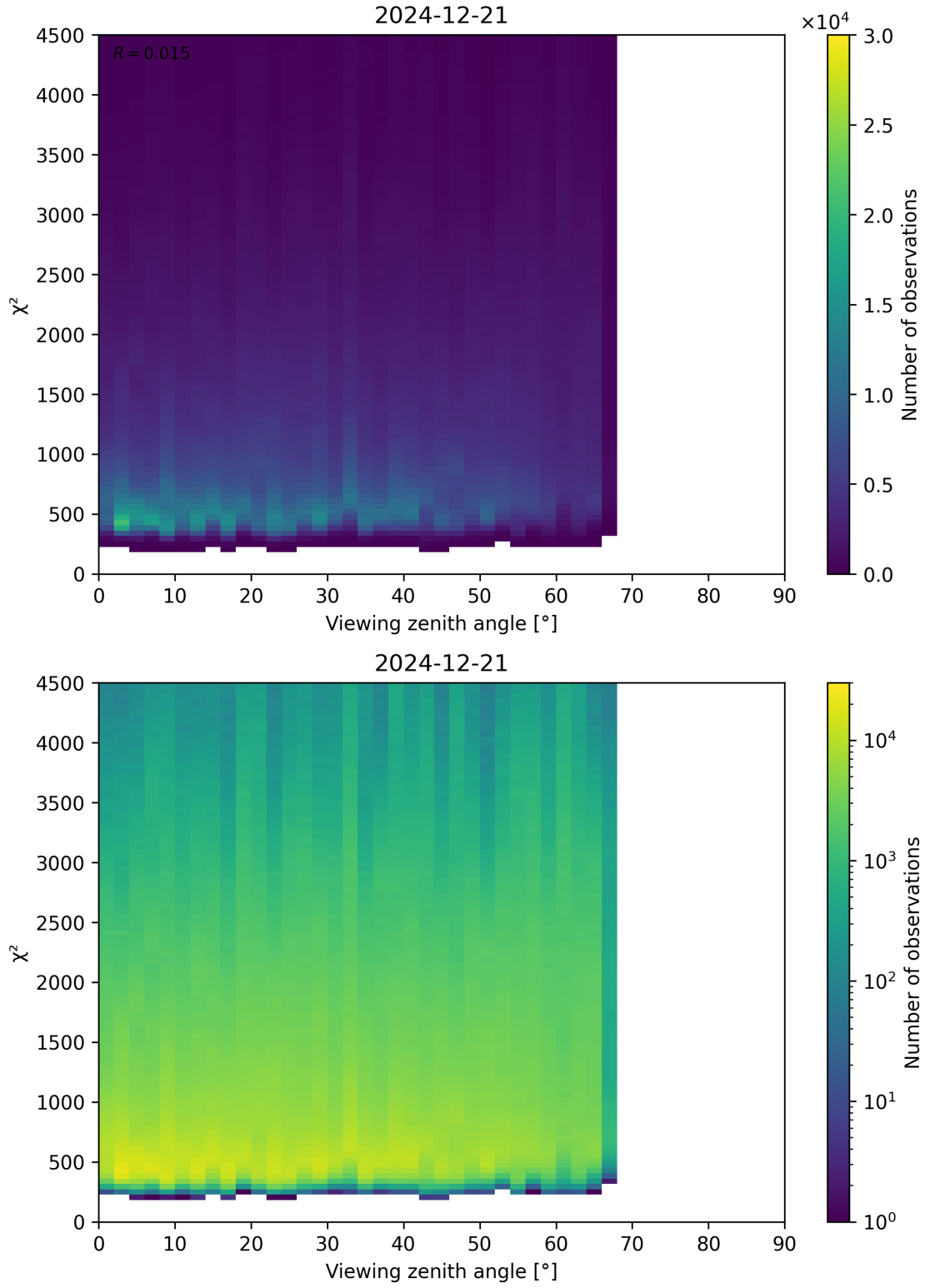
Figure 72: Scatter density plot of “Viewing zenith angle” against “ \chi^2 ” for 2024-12-20 to 2024-12-22.
