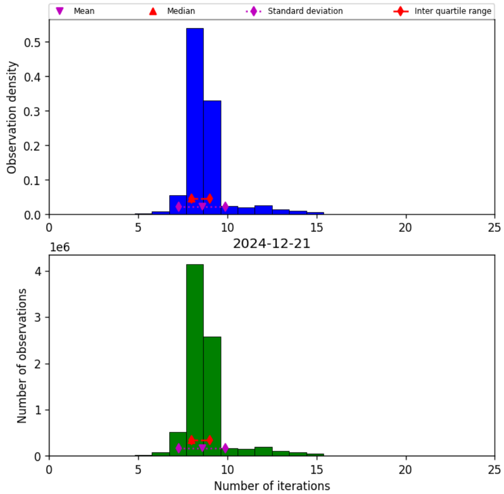
Figure 24: Histogram of “Number of iterations” for 2024-12-20 to 2024-12-22
