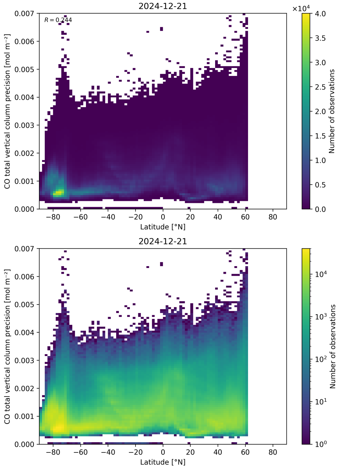
Figure 53: Scatter density plot of “Latitude” against “CO total vertical column precision” for 2024-12-20 to 2024-12-22.
