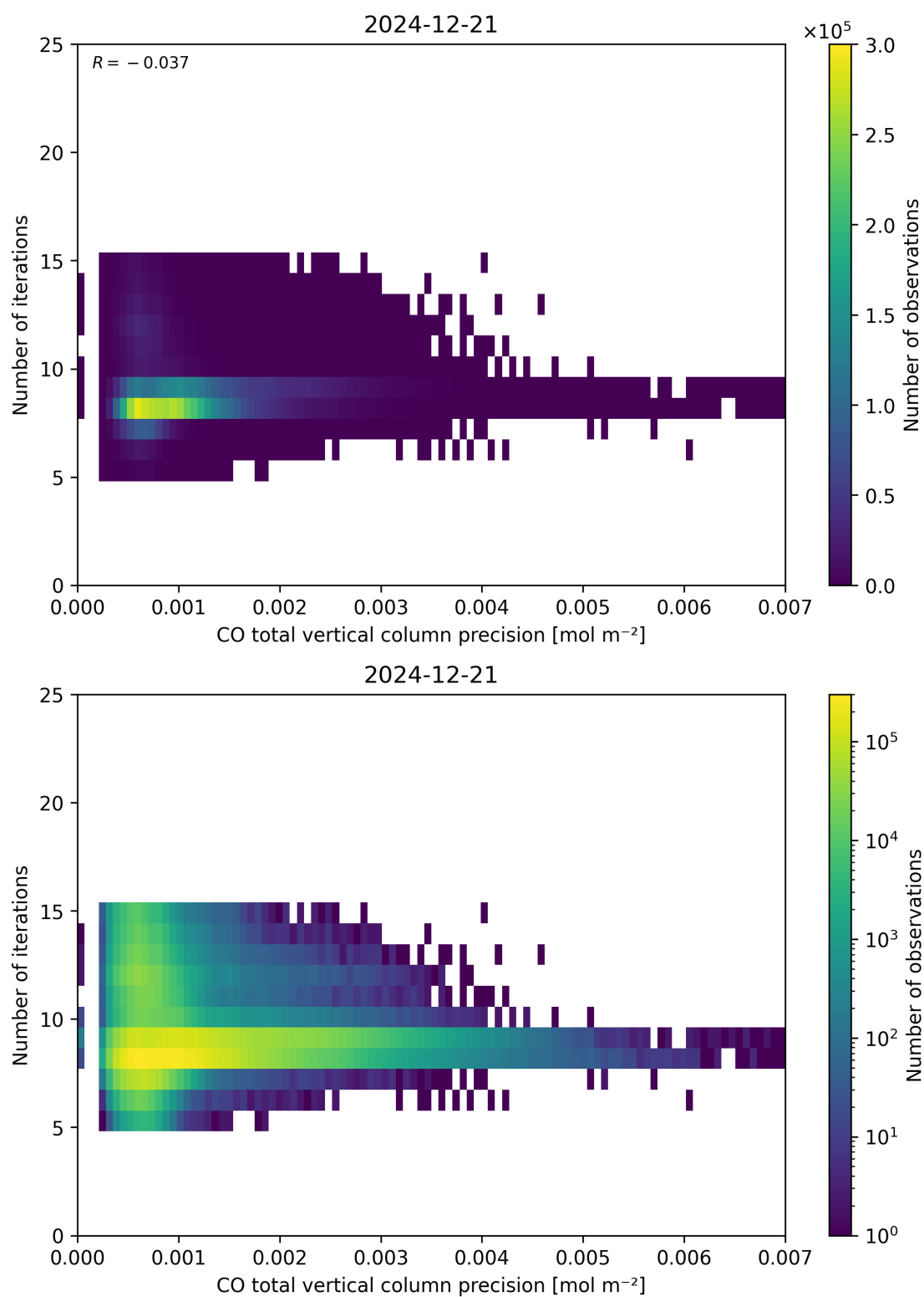
Figure 46: Scatter density plot of “CO total vertical column precision” against “Number of iterations” for 2024-12-20 to 2024-12-22.
