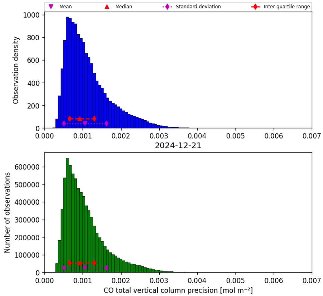
Figure 20: Histogram of “CO total vertical column precision” for 2024-12-20 to 2024-12-22
