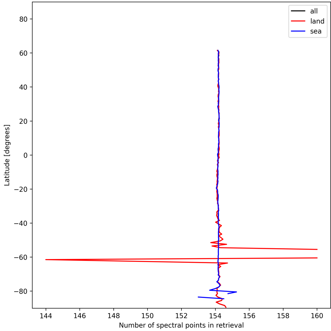
Figure 13: Zonal average of “Number of spectral points in retrieval” for 2024-12-20 to 2024-12-22.
