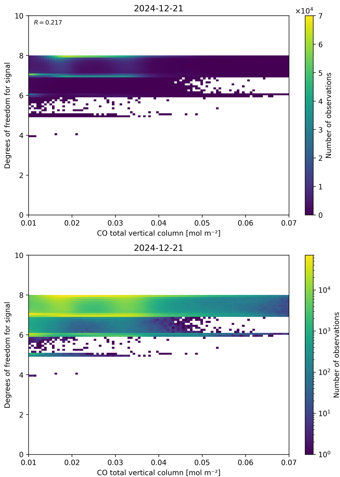
Figure 41: Scatter density plot of “CO total vertical column” against “Degrees of freedom for signal” for 2024-12-20 to 2024-12-22.
