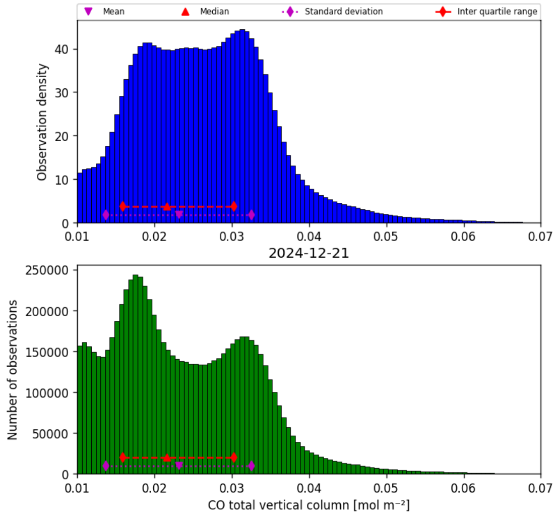
Figure 18: Histogram of “CO total vertical column” for 2024-12-20 to 2024-12-22
