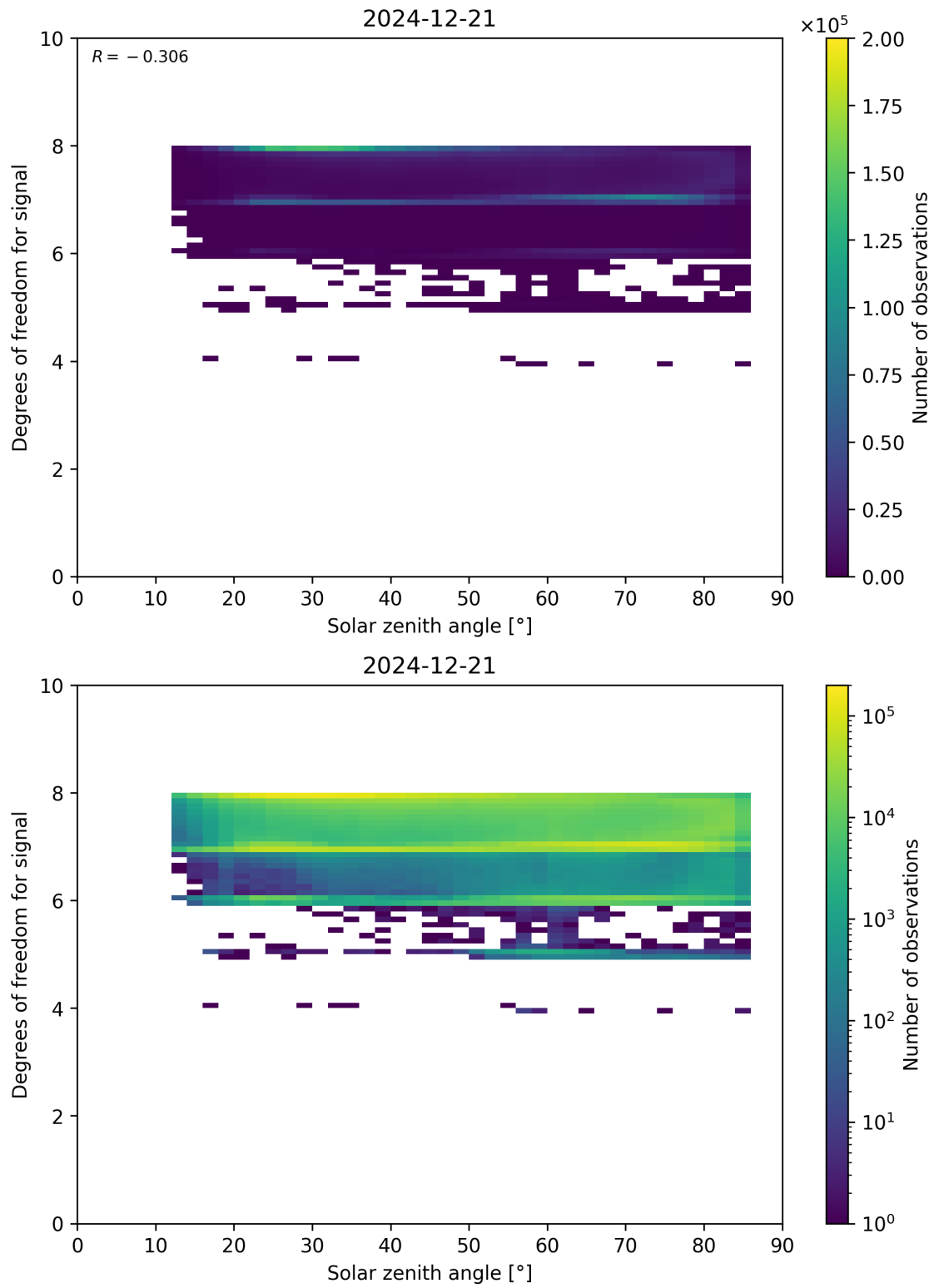
Figure 65: Scatter density plot of “Solar zenith angle” against “Degrees of freedom for signal” for 2024-12-20 to 2024-12-22.
