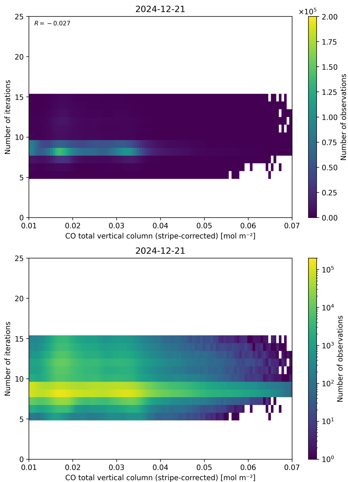
Figure 39: Scatter density plot of “CO total vertical column (stripe-corrected)” against “Number of iterations” for 2024-12-20 to 2024-12-22.
