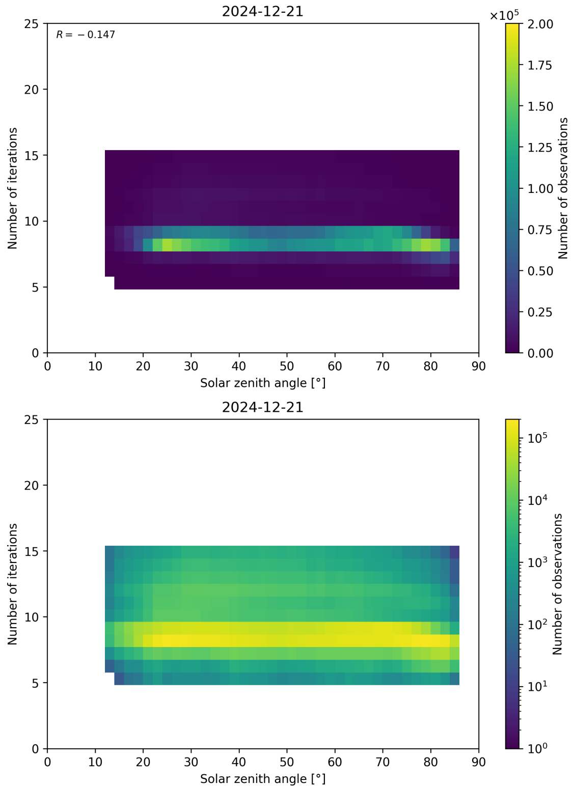
Figure 67: Scatter density plot of “Solar zenith angle” against “Number of iterations” for 2024-12-20 to 2024-12-22.
