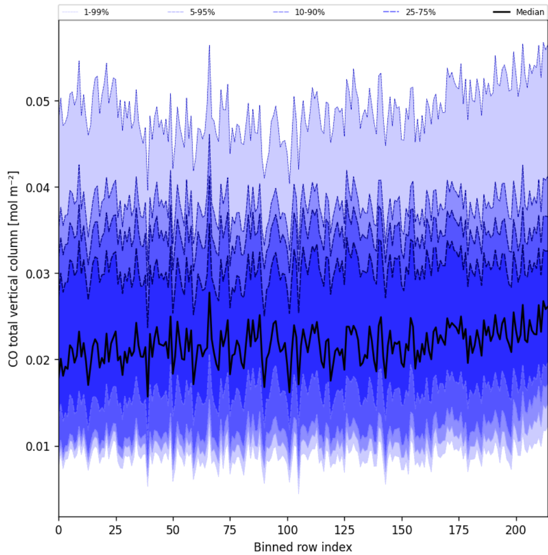
Figure 26: Along track statistics of “CO total vertical column” for 2024-12-20 to 2024-12-22
