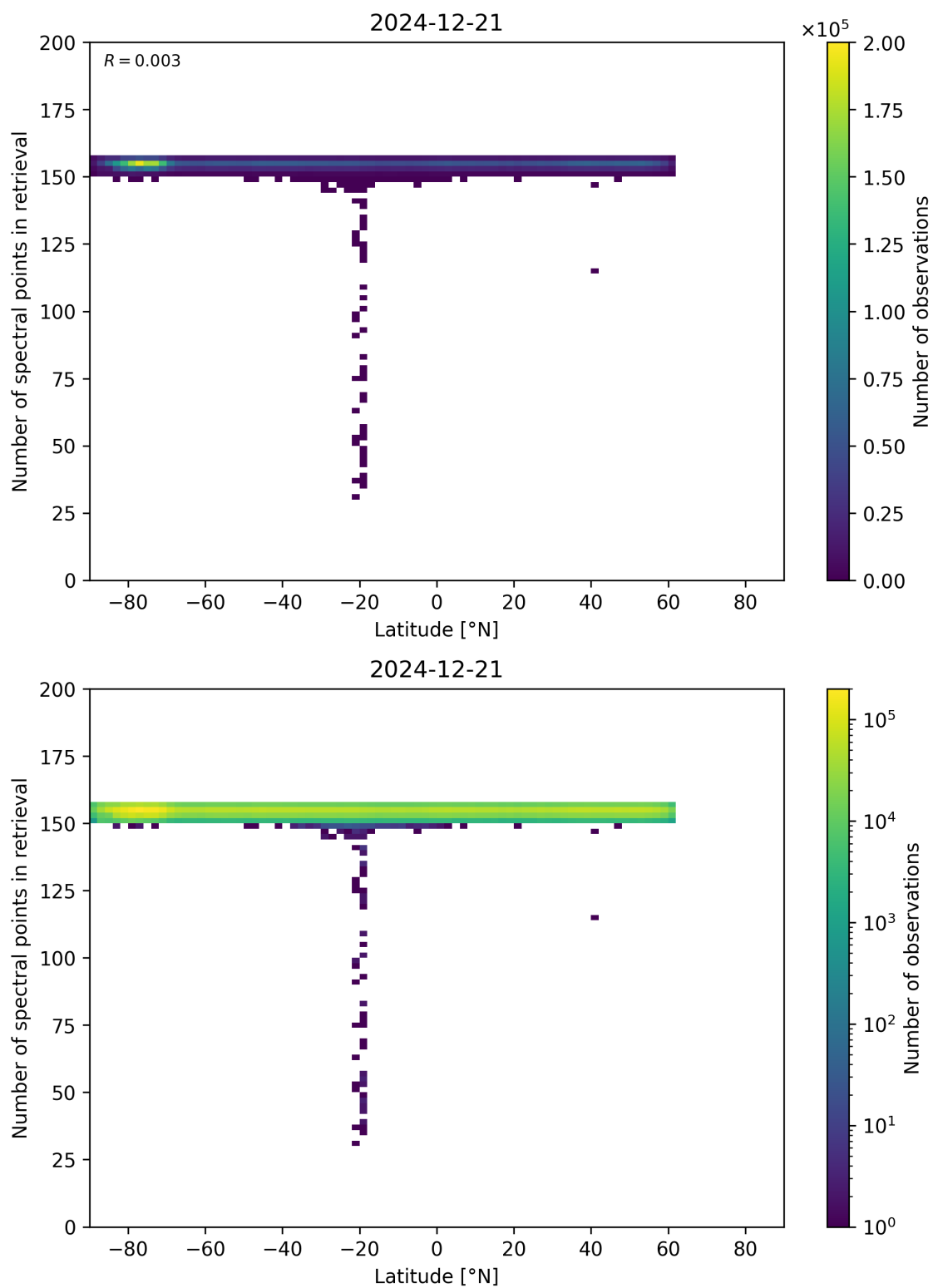
Figure 57: Scatter density plot of “Latitude” against “Number of spectral points in retrieval” for 2024-12-20 to 2024-12-22.
