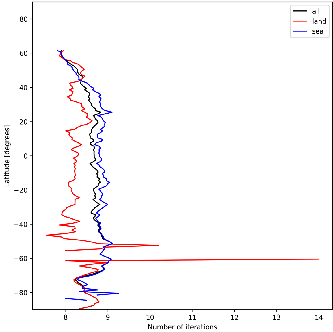
Figure 16: Zonal average of “Number of iterations” for 2024-12-20 to 2024-12-22.
