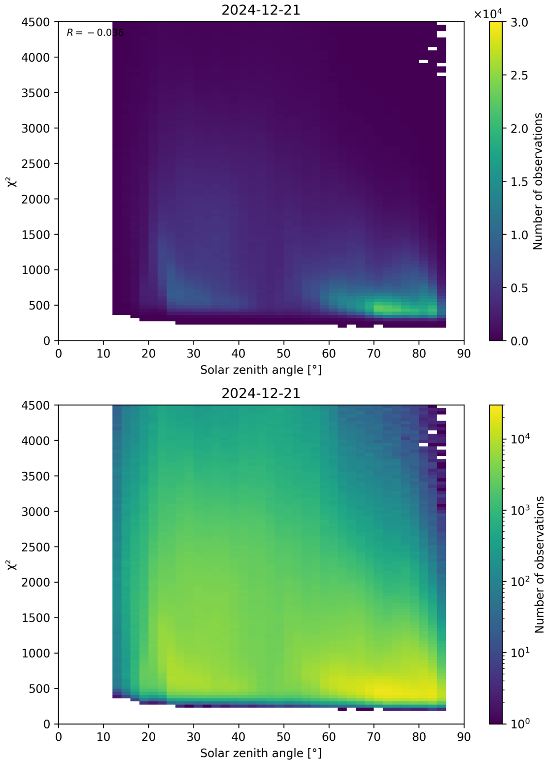
Figure 64: Scatter density plot of “Solar zenith angle” against “ \chi^2 ” for 2024-12-20 to 2024-12-22.
