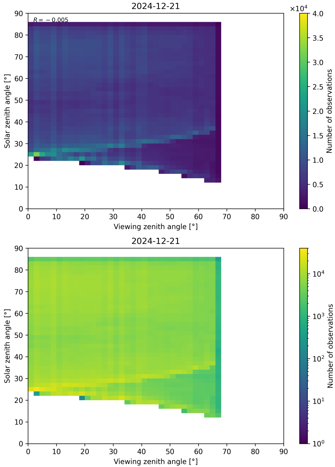
Figure 77: Scatter density plot of “Viewing zenith angle” against “Solar zenith angle” for 2024-12-20 to 2024-12-22.
