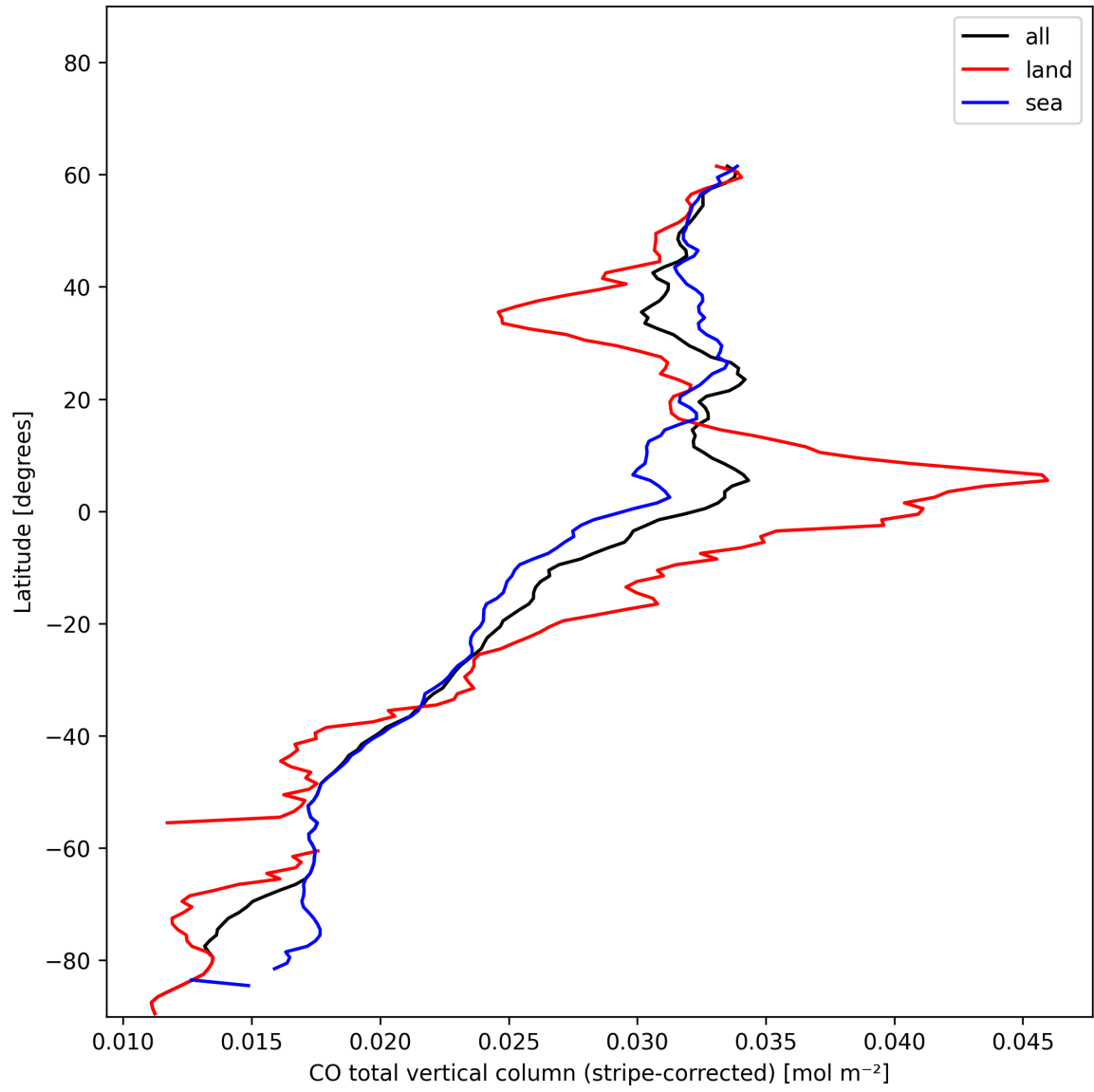
Figure 11: Zonal average of “CO total vertical column (stripe-corrected)” for 2024-12-20 to 2024-12-22.
