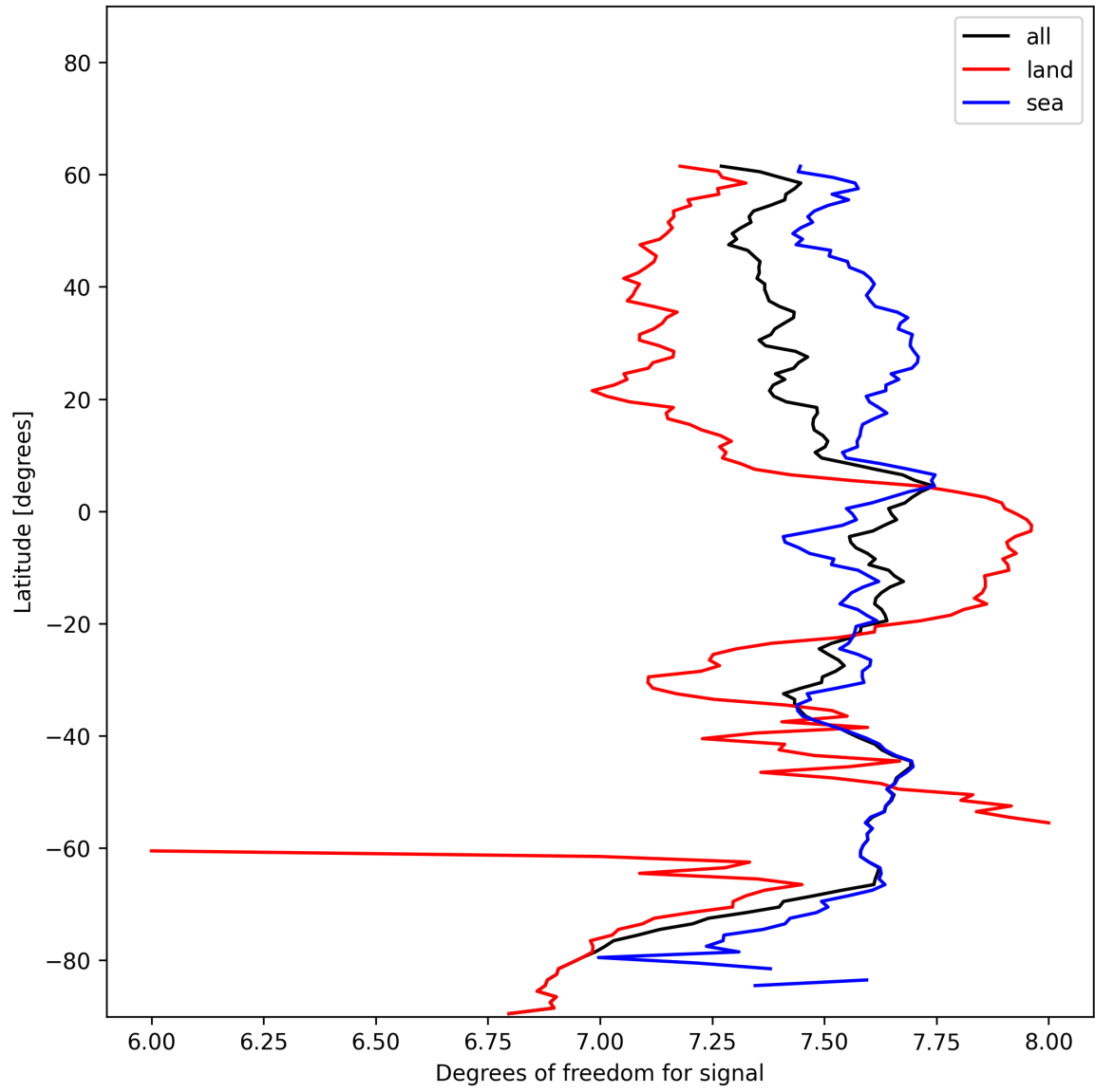
Figure 15: Zonal average of “Degrees of freedom for signal” for 2024-12-20 to 2024-12-22.
