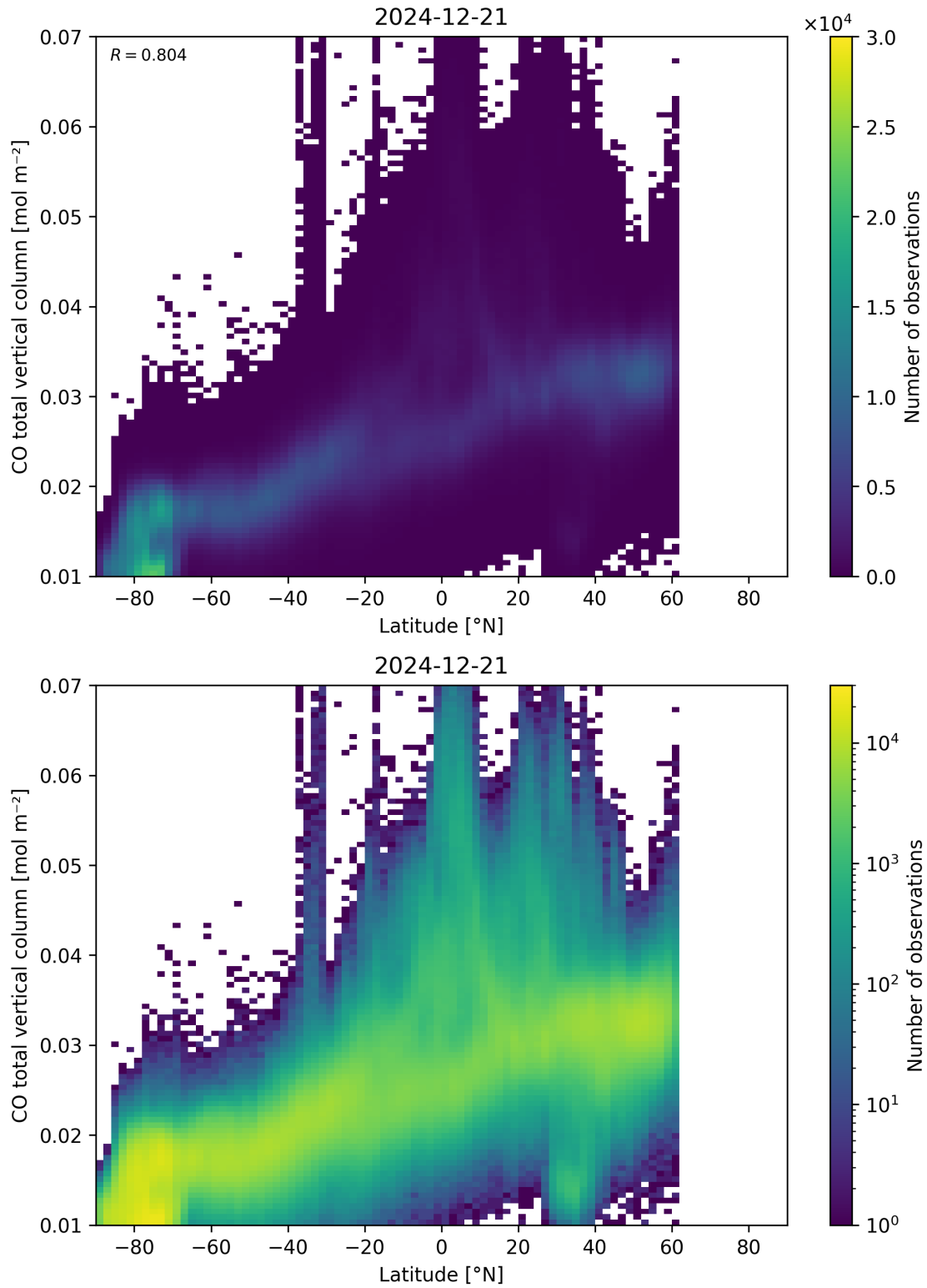
Figure 51: Scatter density plot of “Latitude” against “CO total vertical column” for 2024-12-20 to 2024-12-22.
