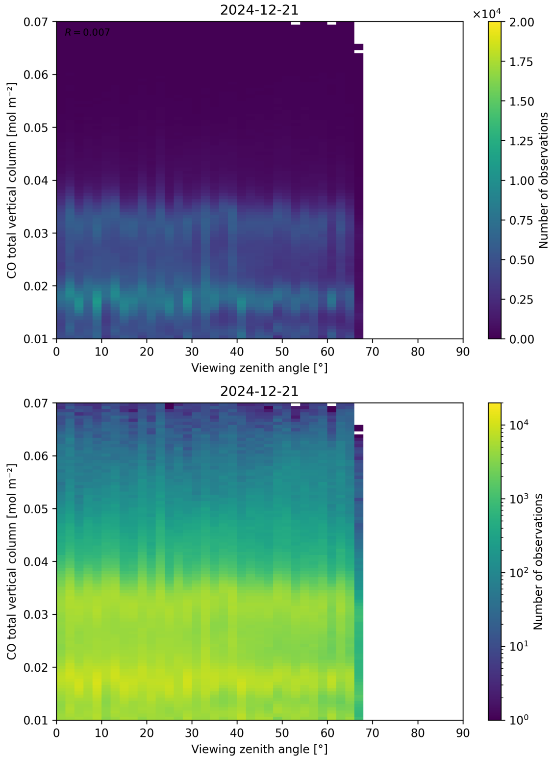
Figure 69: Scatter density plot of “Viewing zenith angle” against “CO total vertical column” for 2024-12-20 to 2024-12-22.
