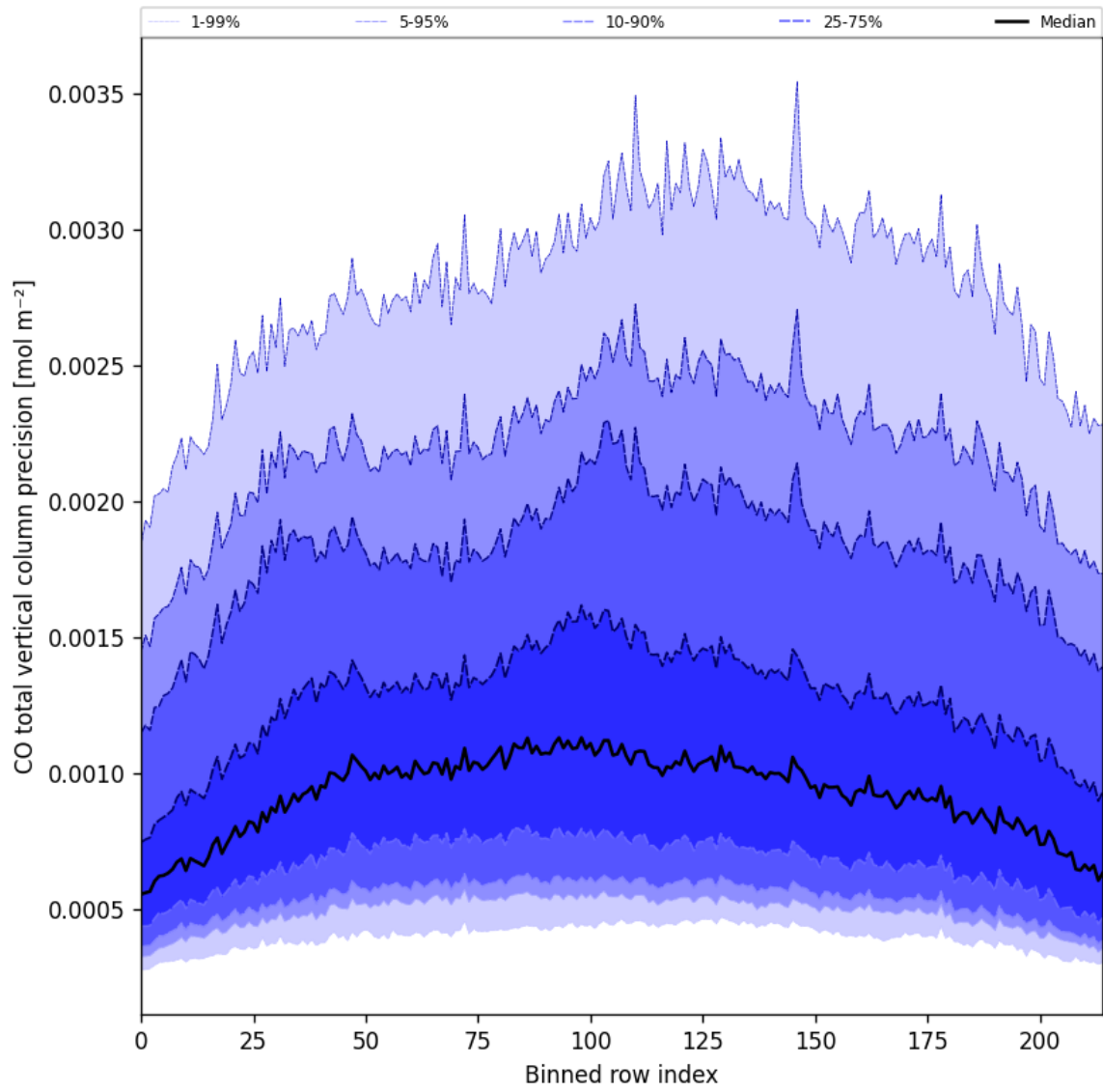
Figure 28: Along track statistics of “CO total vertical column precision” for 2024-12-20 to 2024-12-22
