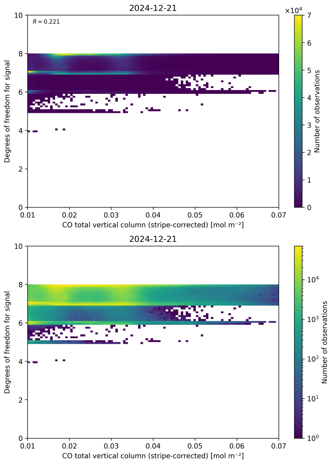
Figure 38: Scatter density plot of “CO total vertical column (stripe-corrected)” against “Degrees of freedom for signal” for 2024-12-20 to 2024-12-22.
