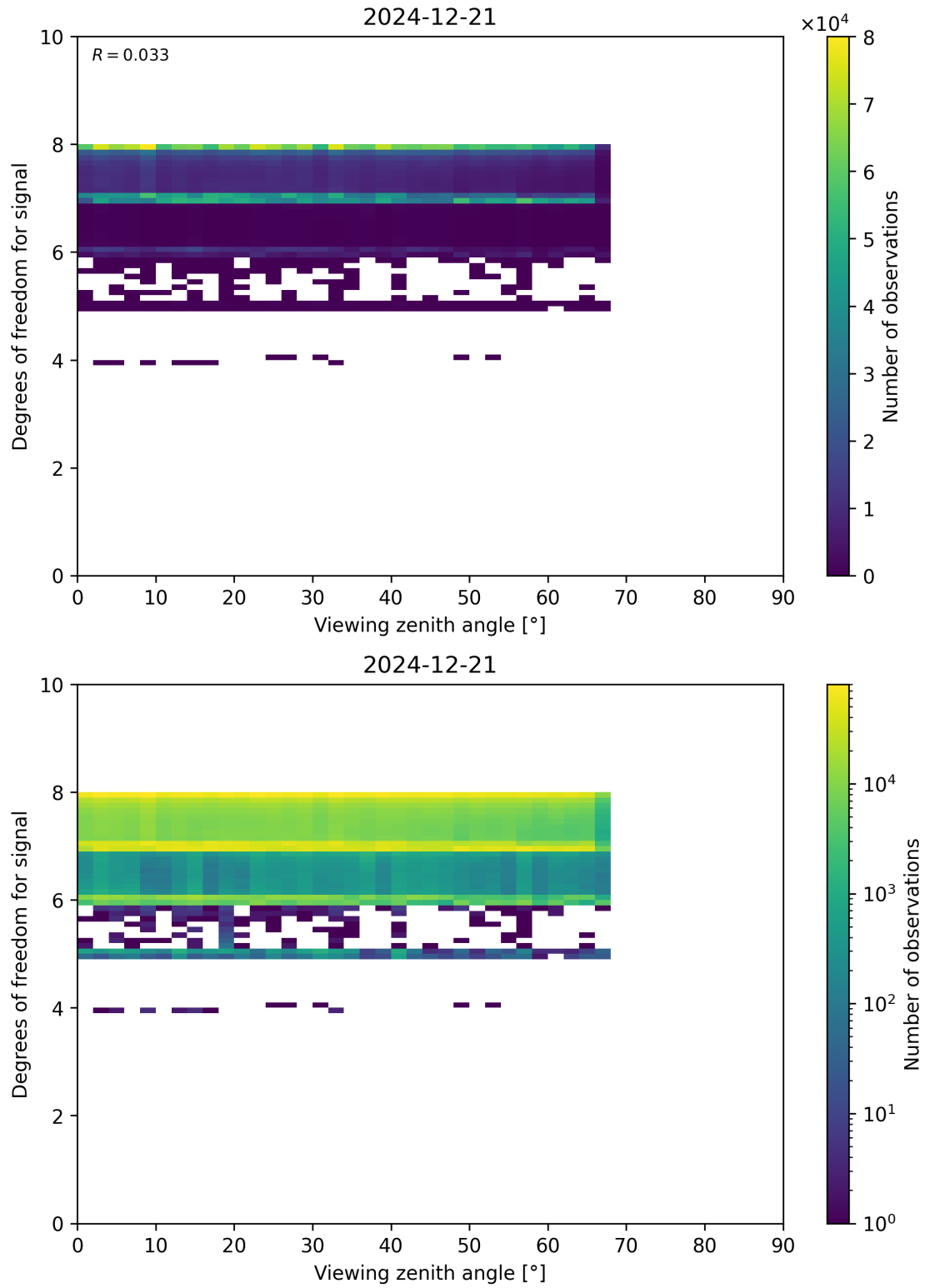
Figure 73: Scatter density plot of “Viewing zenith angle” against “Degrees of freedom for signal” for 2024-12-20 to 2024-12-22.
