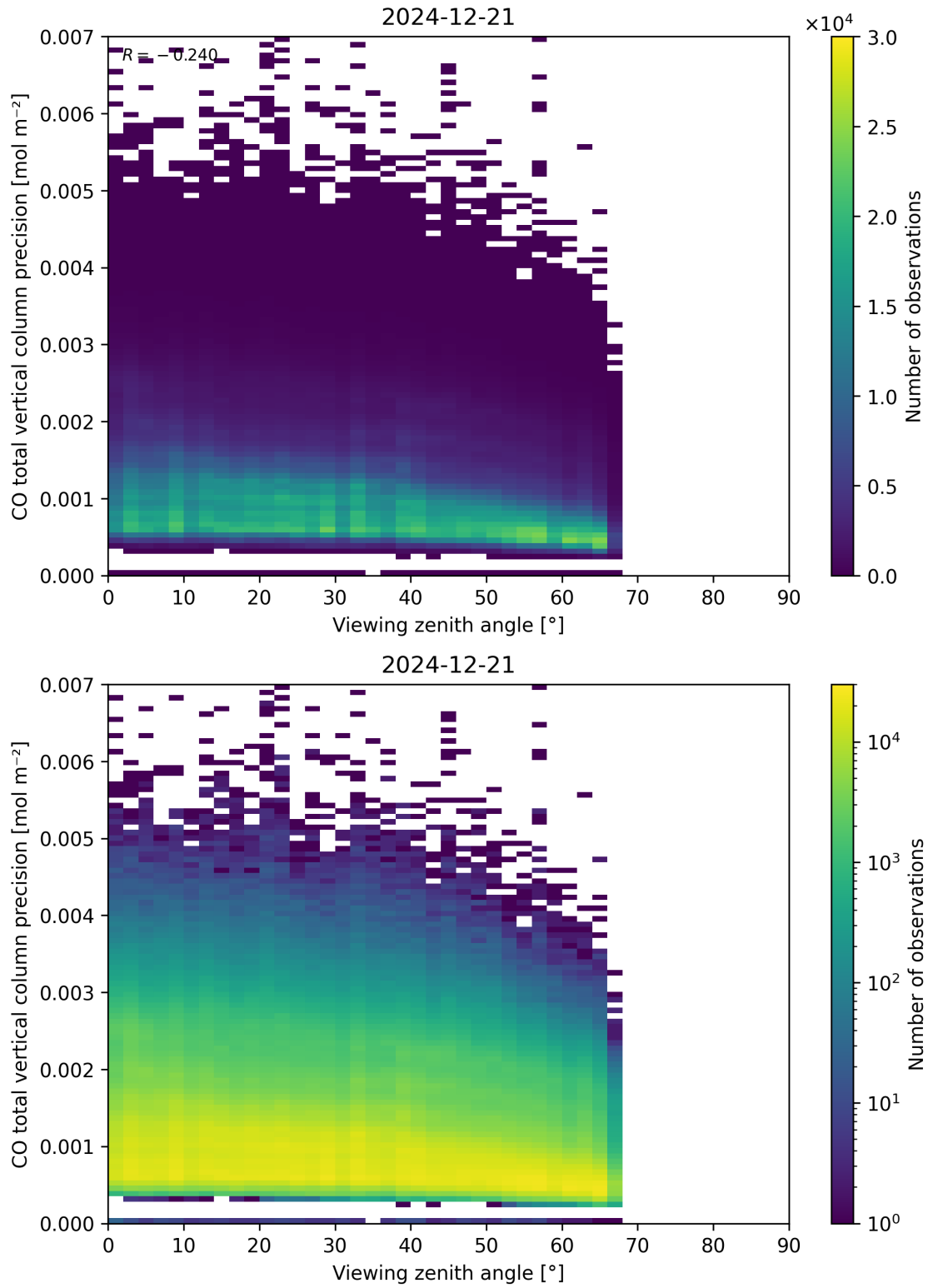
Figure 71: Scatter density plot of “Viewing zenith angle” against “CO total vertical column precision” for 2024-12-20 to 2024-12-22.
