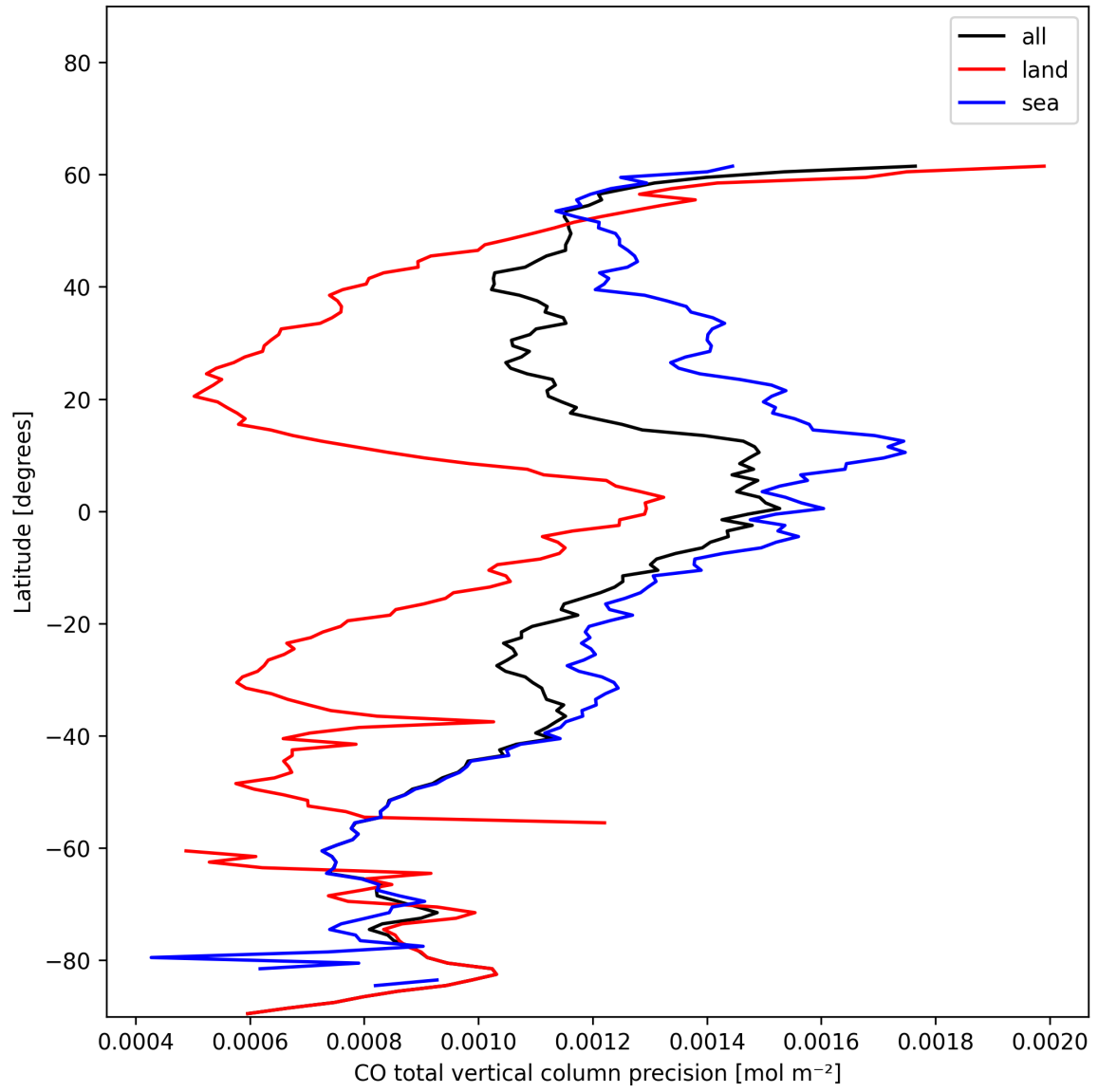
Figure 12: Zonal average of “CO total vertical column precision” for 2024-12-20 to 2024-12-22.
