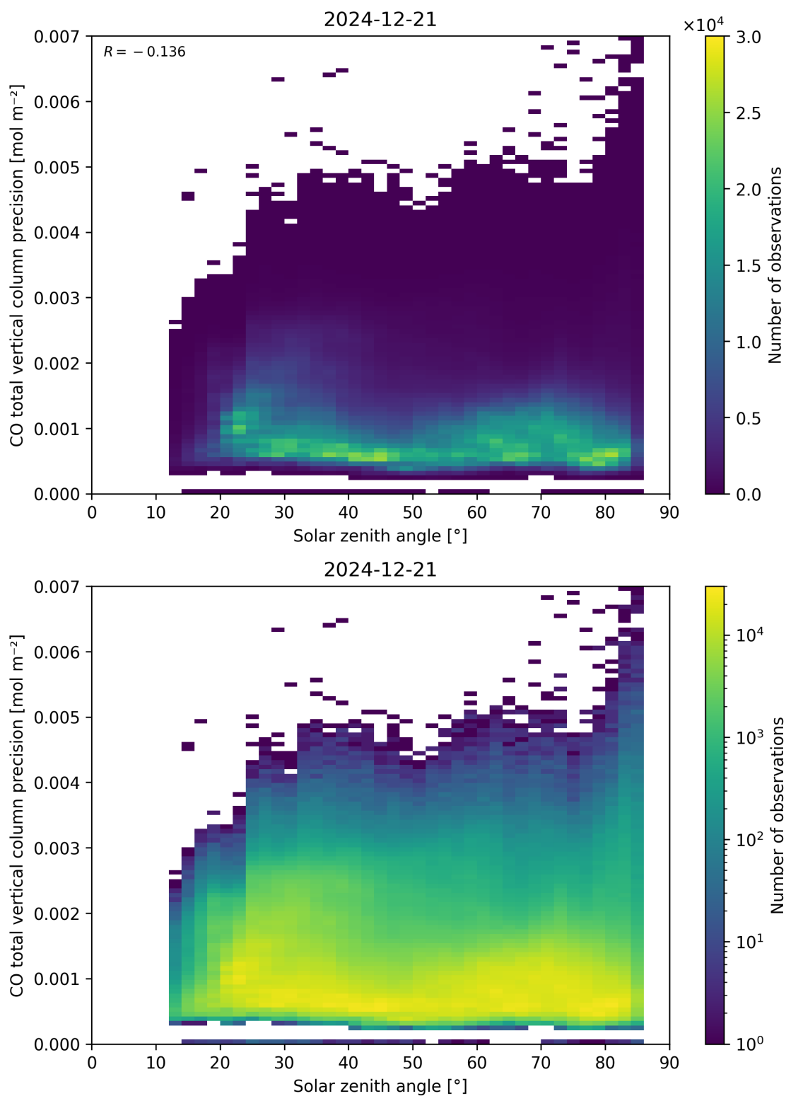
Figure 63: Scatter density plot of “Solar zenith angle” against “CO total vertical column precision” for 2024-12-20 to 2024-12-22.
