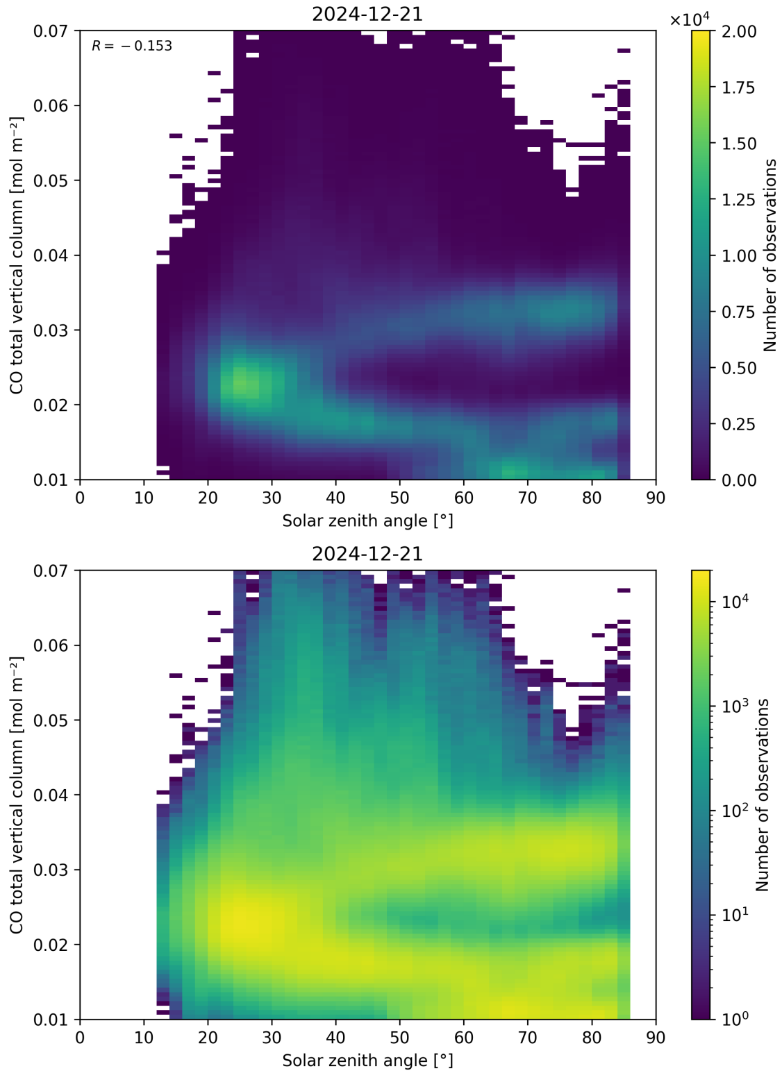
Figure 61: Scatter density plot of “Solar zenith angle” against “CO total vertical column” for 2024-12-20 to 2024-12-22.
