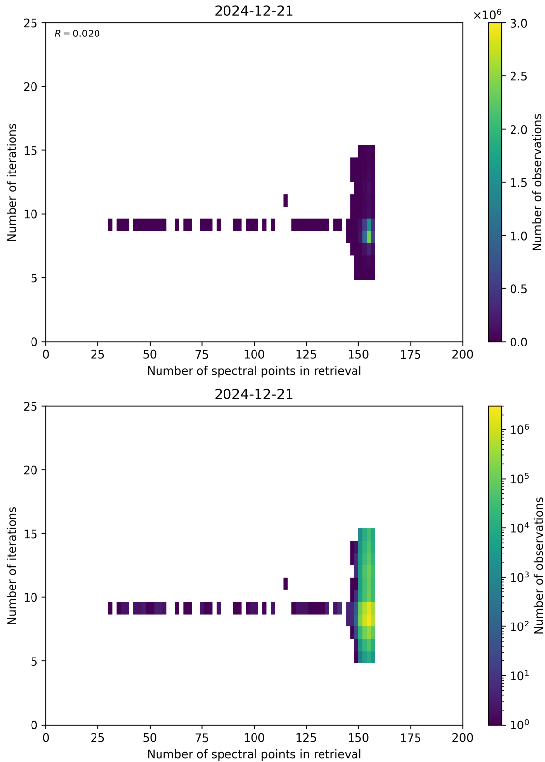
Figure 60: Scatter density plot of “Number of spectral points in retrieval” against “Number of iterations” for 2024-12-20 to 2024-12-22.
