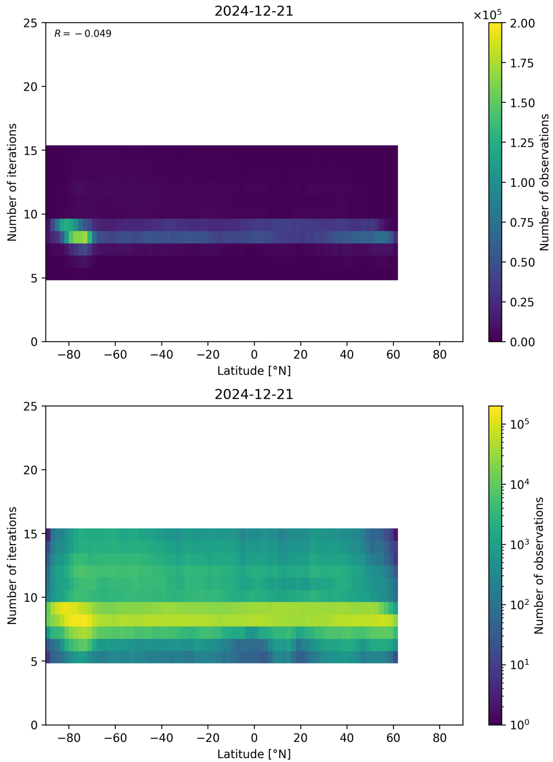
Figure 56: Scatter density plot of “Latitude” against “Number of iterations” for 2024-12-20 to 2024-12-22.
