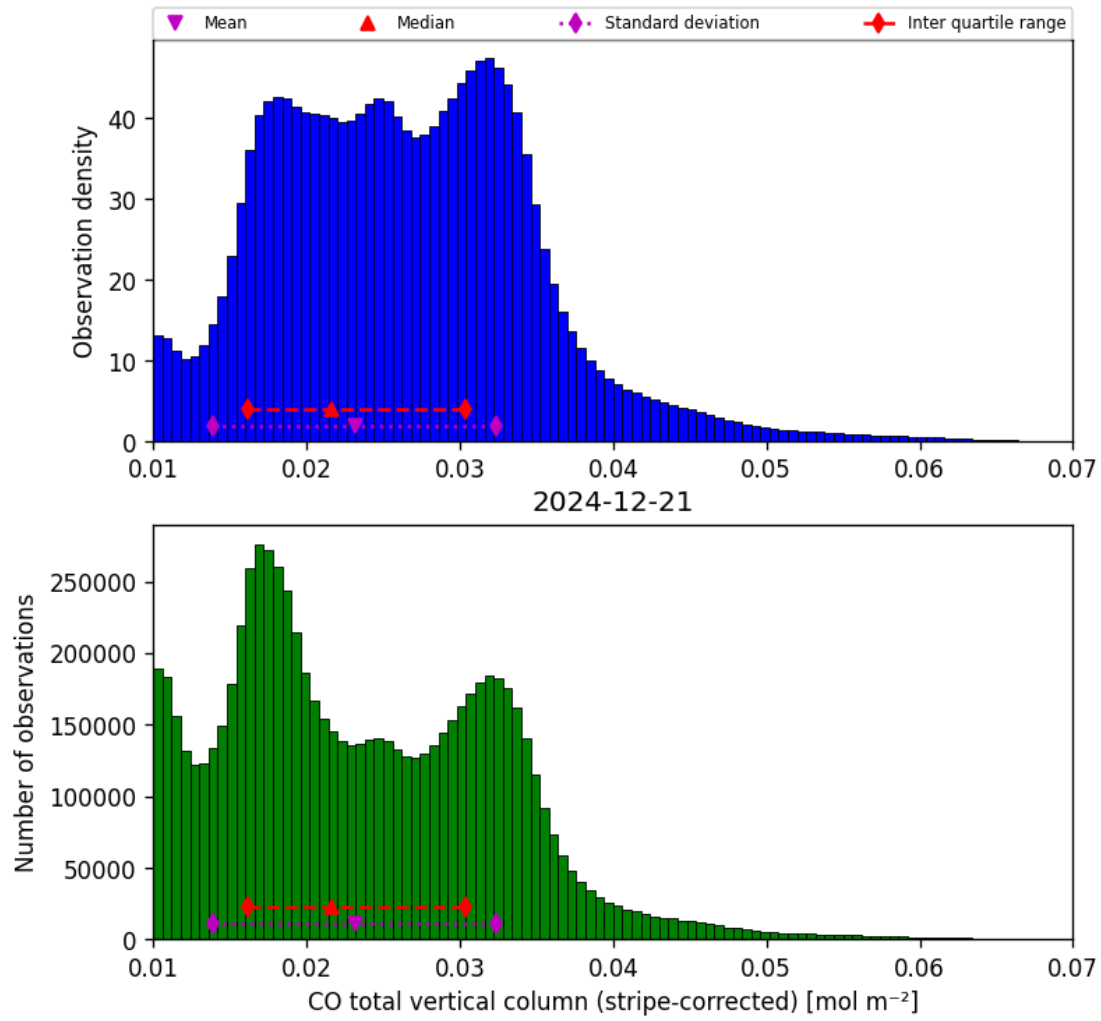
Figure 19: Histogram of “CO total vertical column (stripe-corrected)” for 2024-12-20 to 2024-12-22
