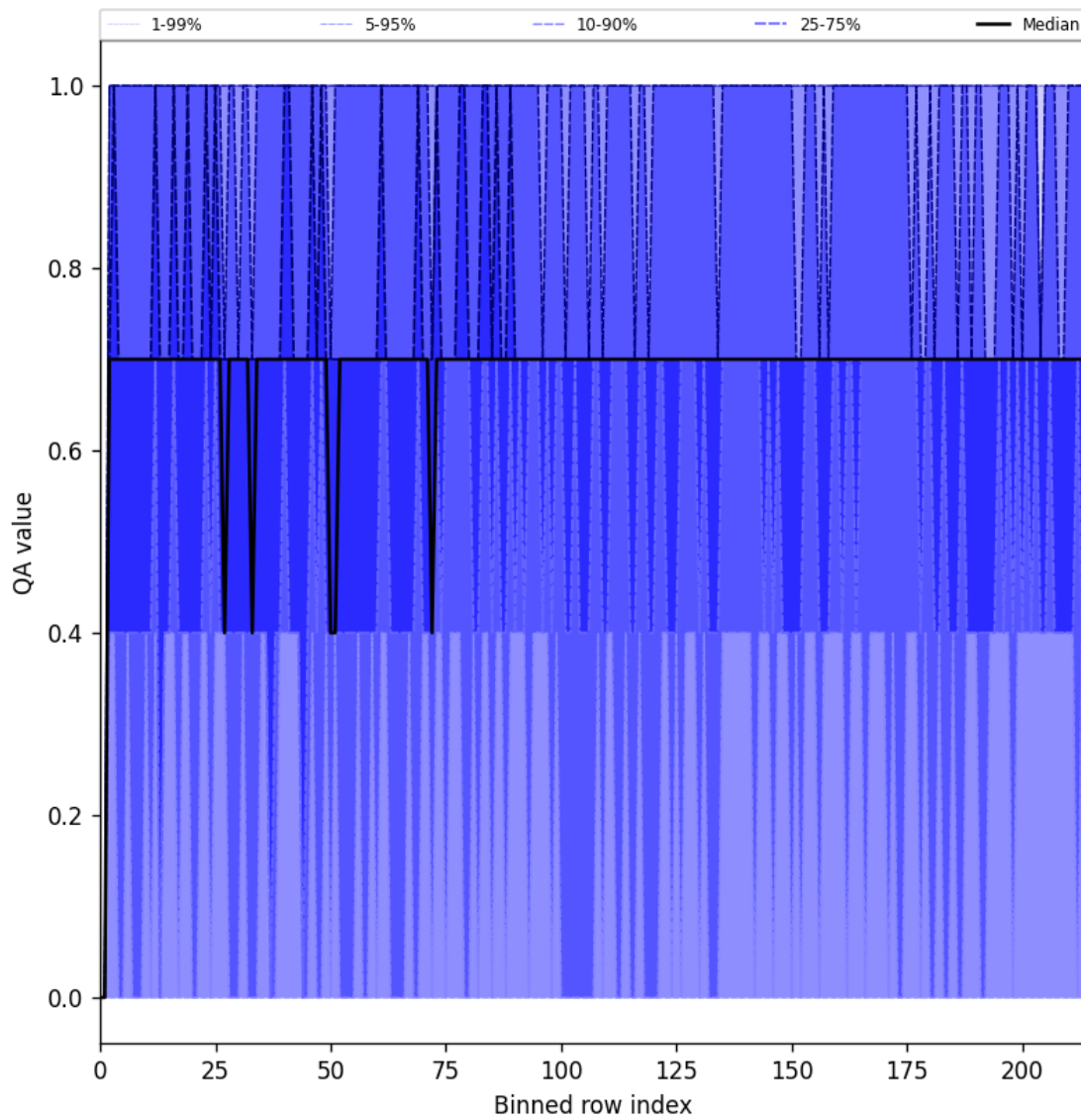
Figure 25: Along track statistics of “QA value” for 2024-12-20 to 2024-12-22
