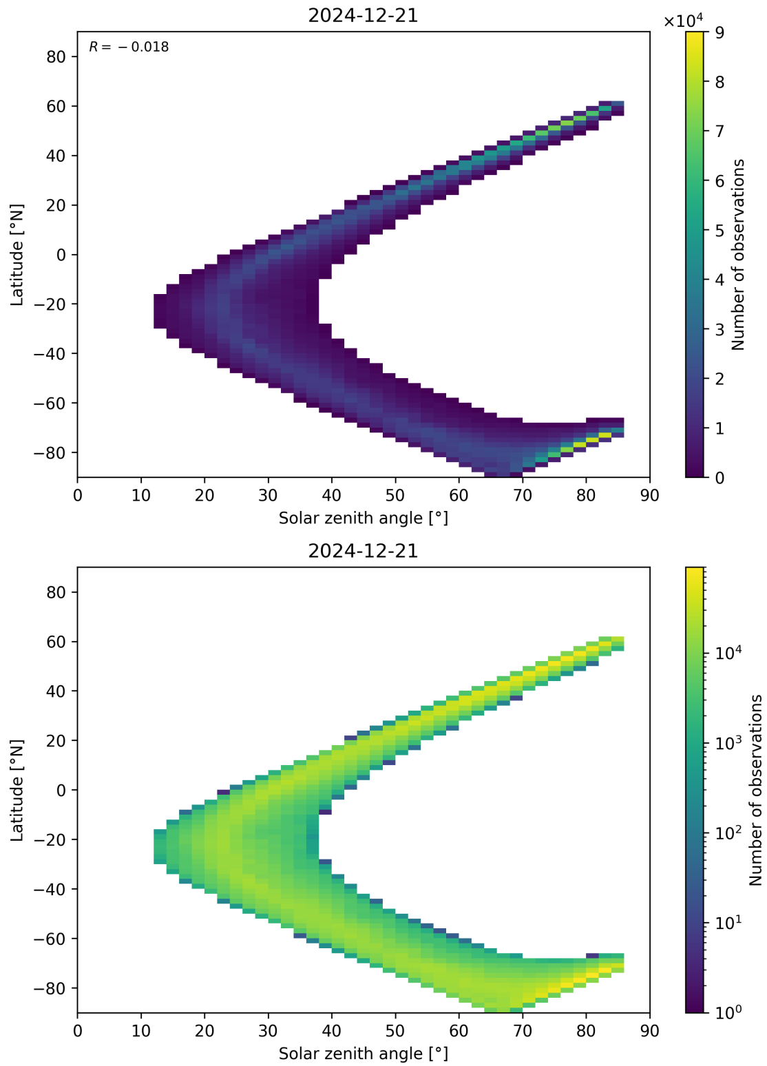
Figure 66: Scatter density plot of “Solar zenith angle” against “Latitude” for 2024-12-20 to 2024-12-22.
