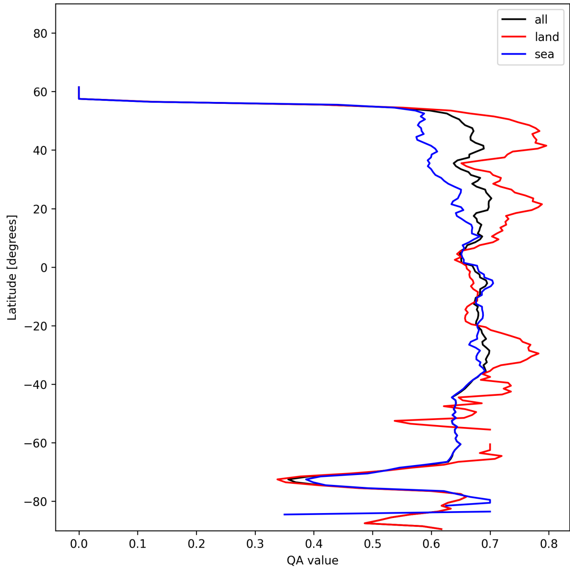
Figure 9: Zonal average of “QA value” for 2024-12-20 to 2024-12-22.
