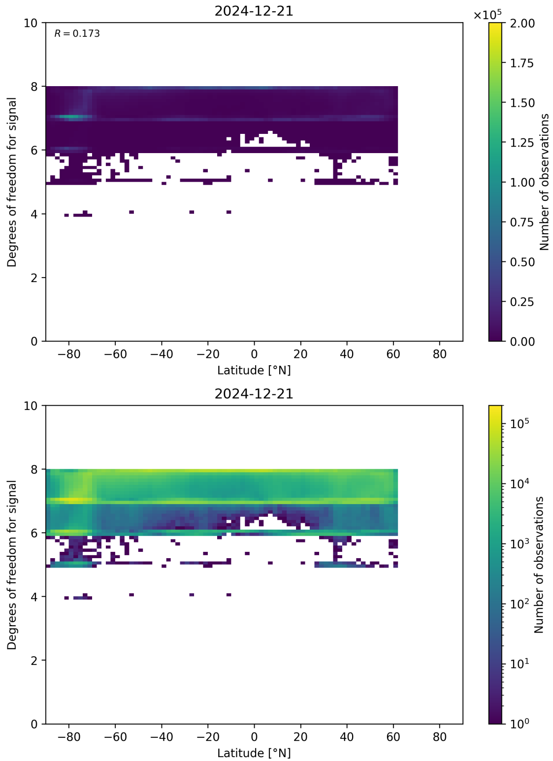
Figure 55: Scatter density plot of “Latitude” against “Degrees of freedom for signal” for 2024-12-20 to 2024-12-22.
