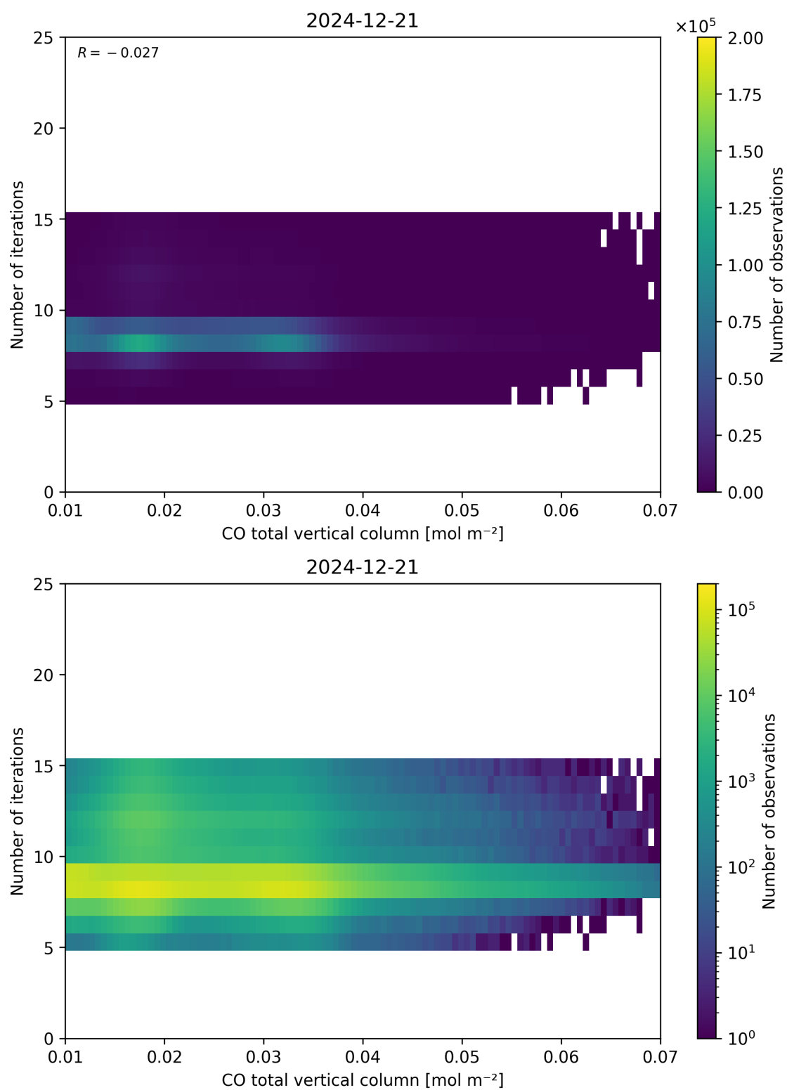
Figure 42: Scatter density plot of “CO total vertical column” against “Number of iterations” for 2024-12-20 to 2024-12-22.
