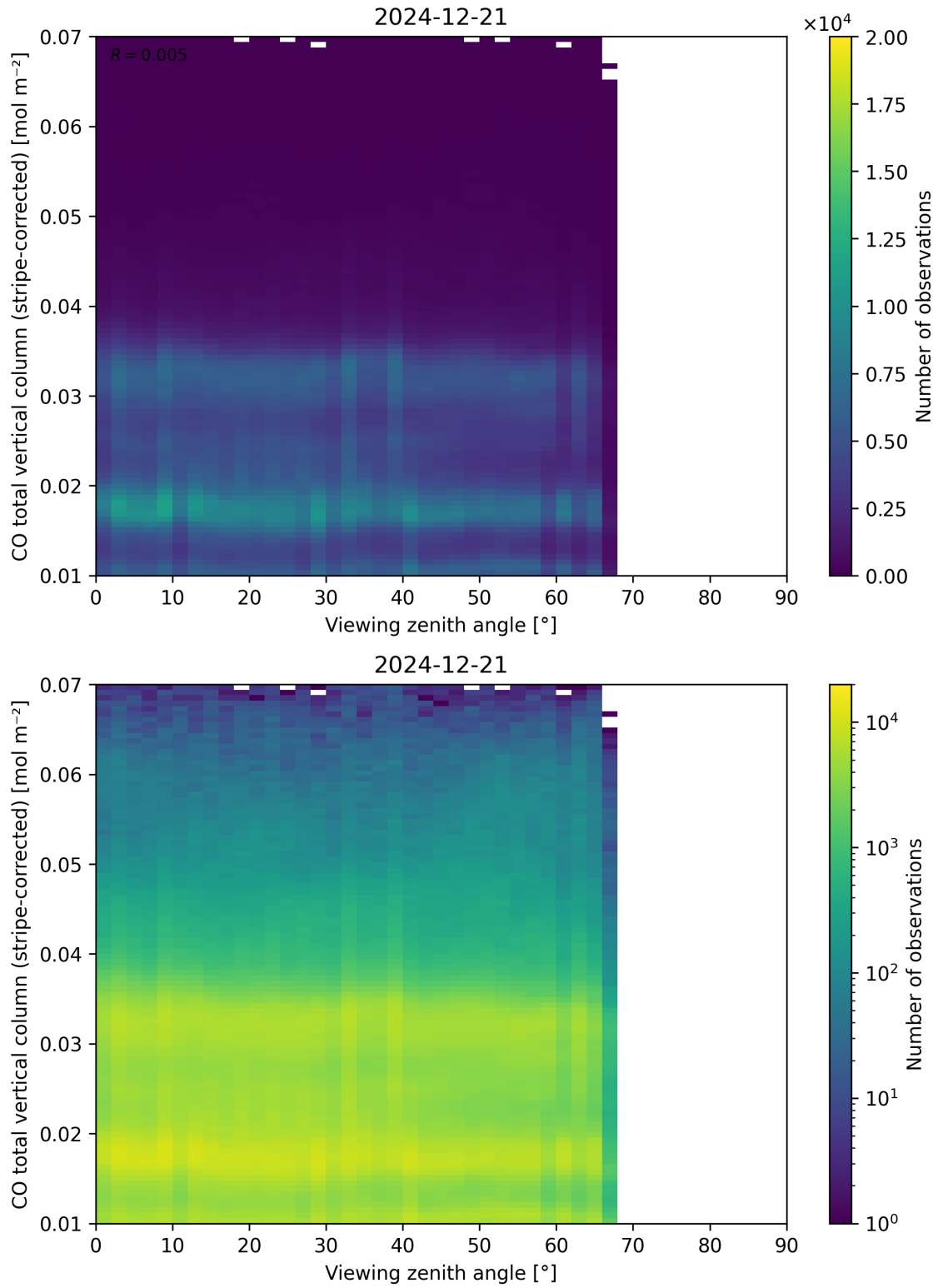
Figure 70: Scatter density plot of “Viewing zenith angle” against “CO total vertical column (stripe-corrected)” for 2024-12-20 to 2024-12-22.
