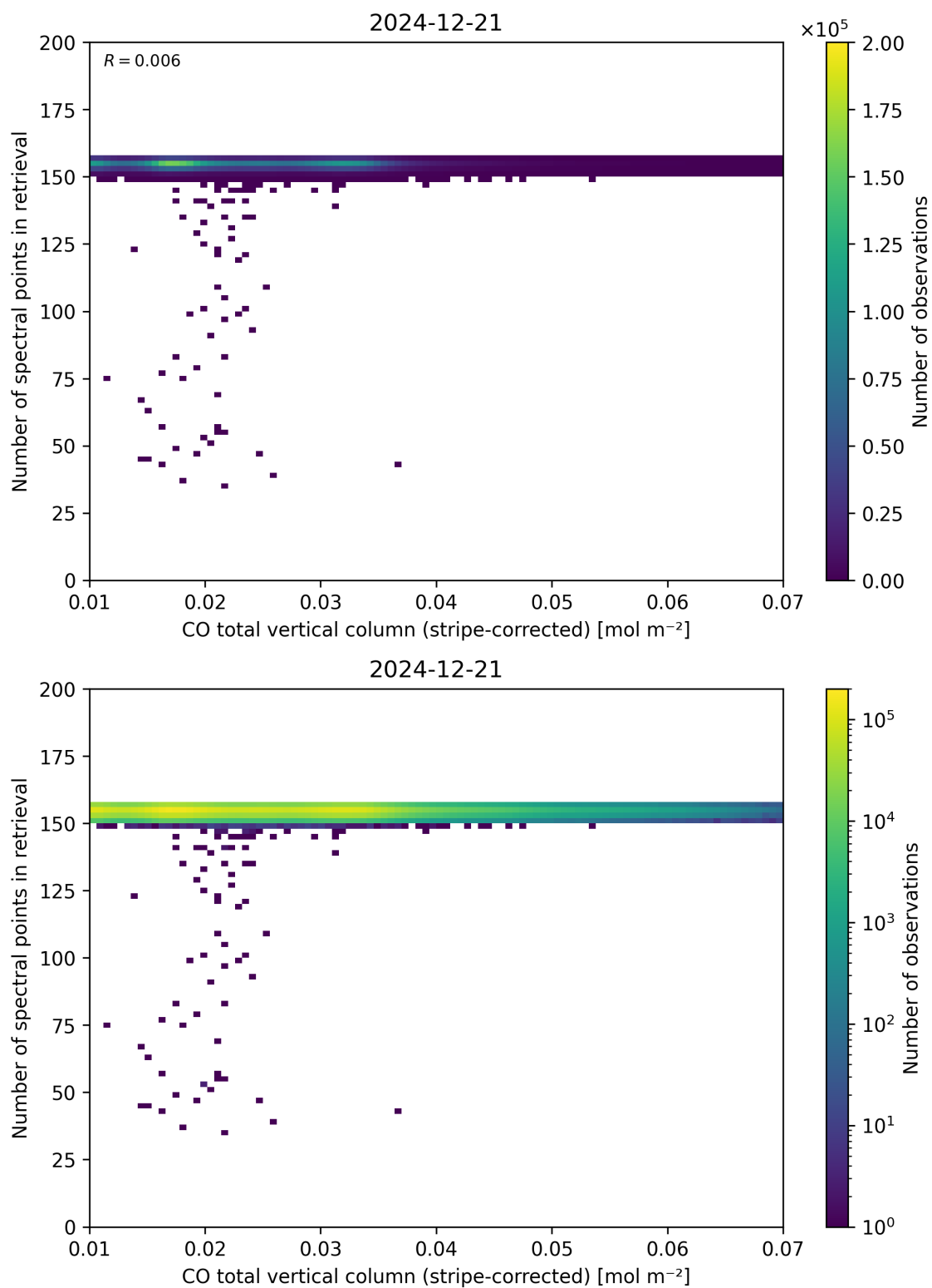
Figure 40: Scatter density plot of “CO total vertical column (stripe-corrected)” against “Number of spectral points in retrieval” for 2024-12-20 to 2024-12-22.
