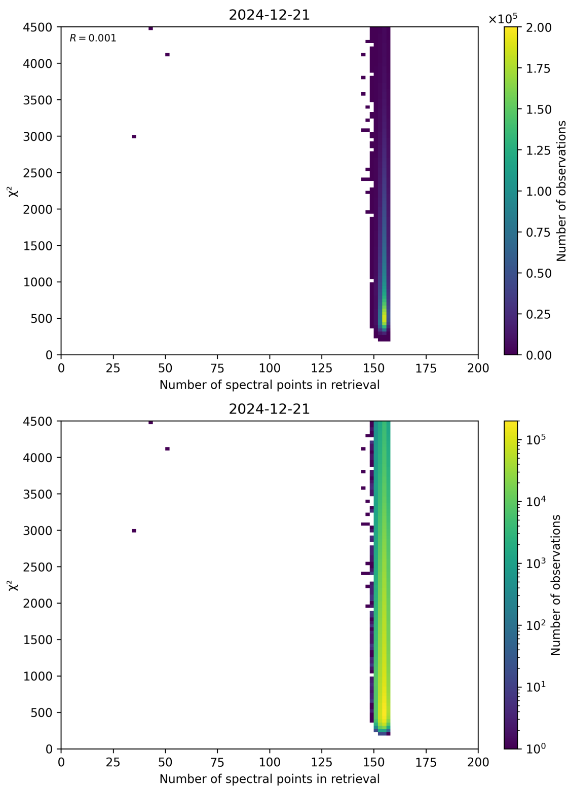
Figure 58: Scatter density plot of “Number of spectral points in retrieval” against “ \chi^2 ” for 2024-12-20 to 2024-12-22.
