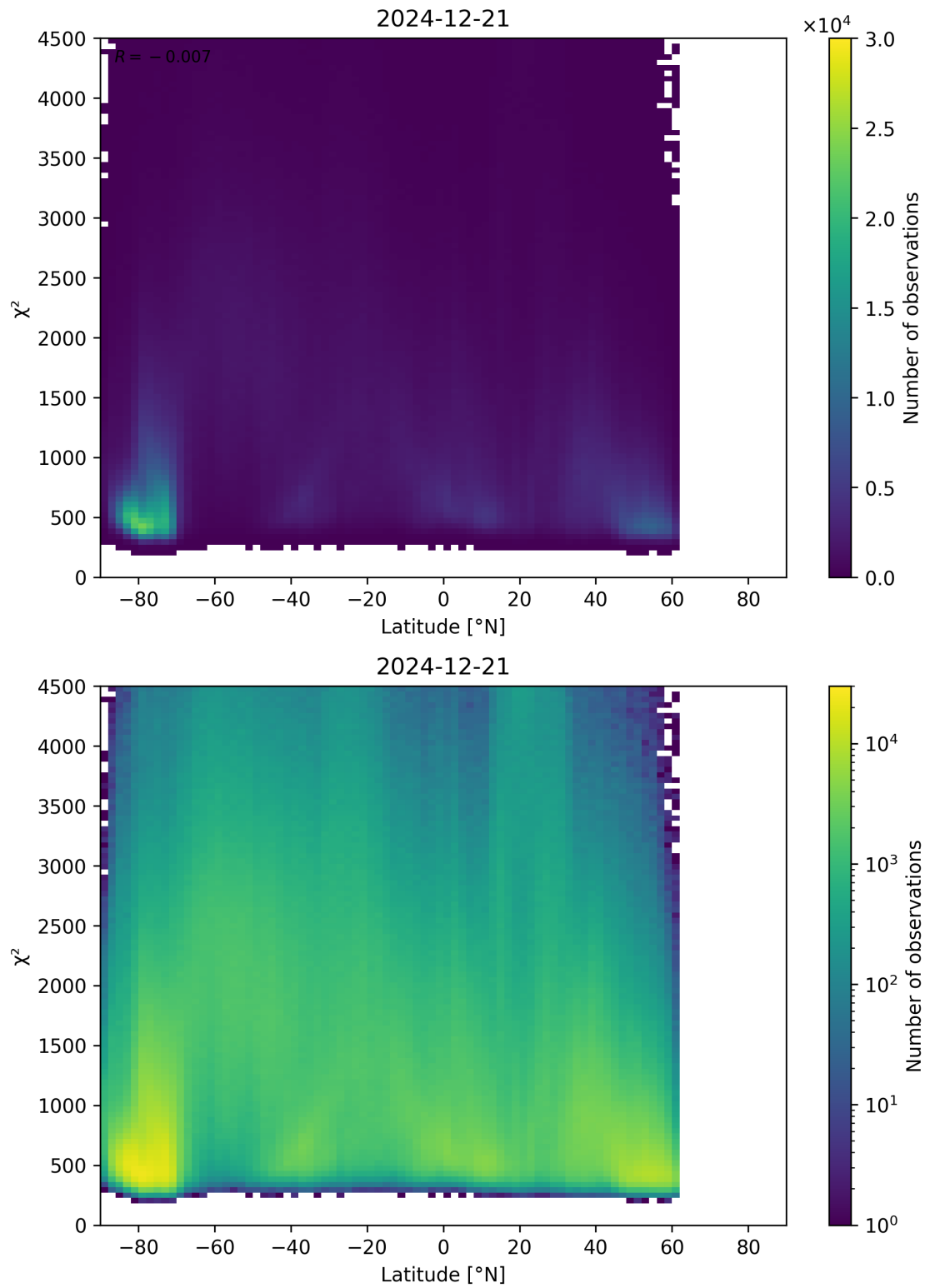
Figure 54: Scatter density plot of “Latitude” against “ \chi^2 ” for 2024-12-20 to 2024-12-22.
