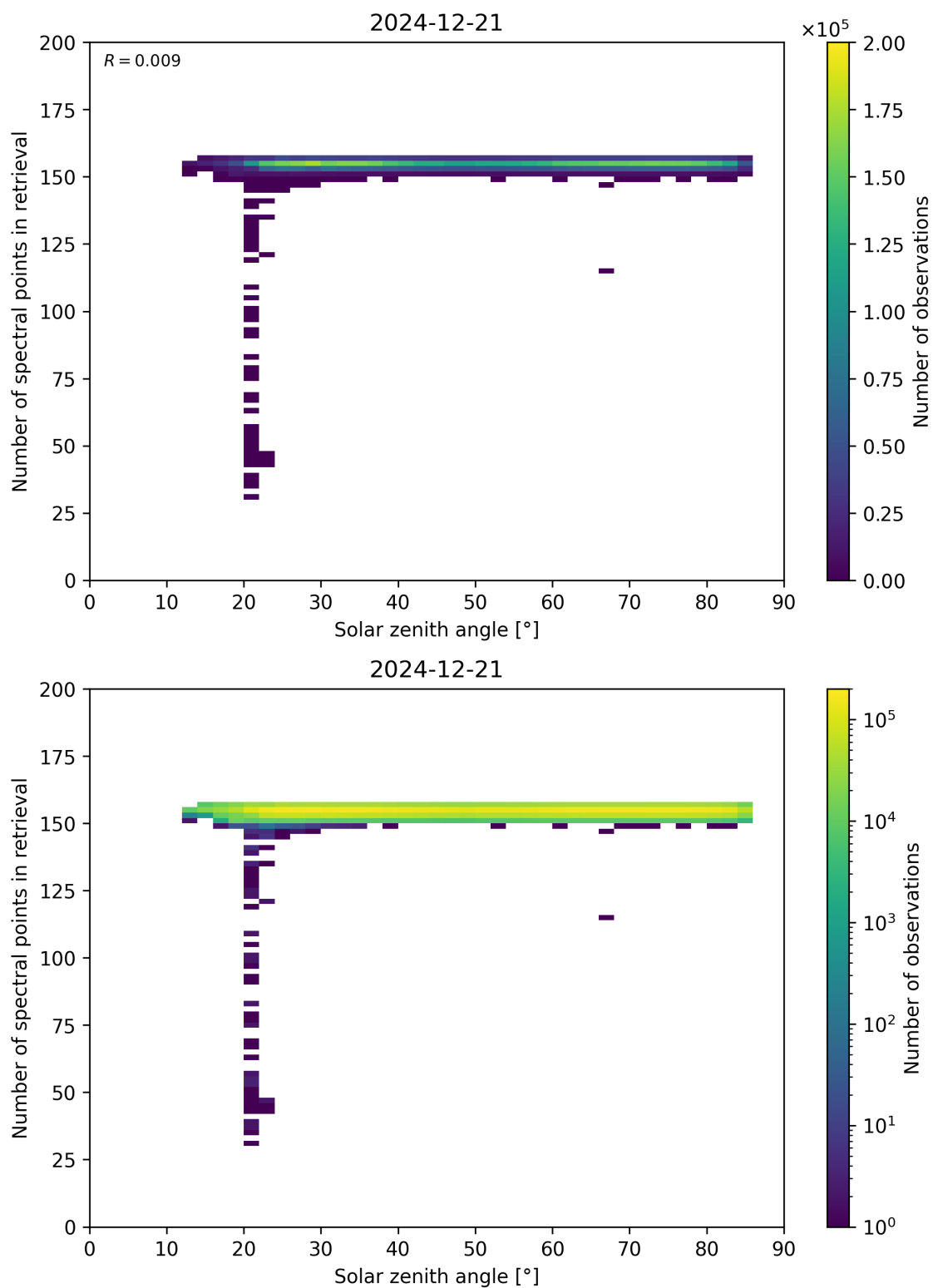
Figure 68: Scatter density plot of “Solar zenith angle” against “Number of spectral points in retrieval” for 2024-12-20 to 2024-12-22.
