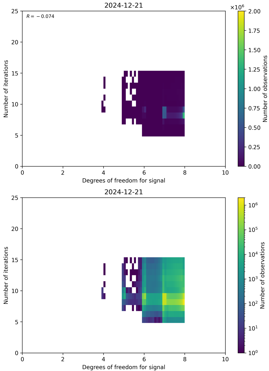
Figure 50: Scatter density plot of “Degrees of freedom for signal” against “Number of iterations” for 2024-12-20 to 2024-12-22.
