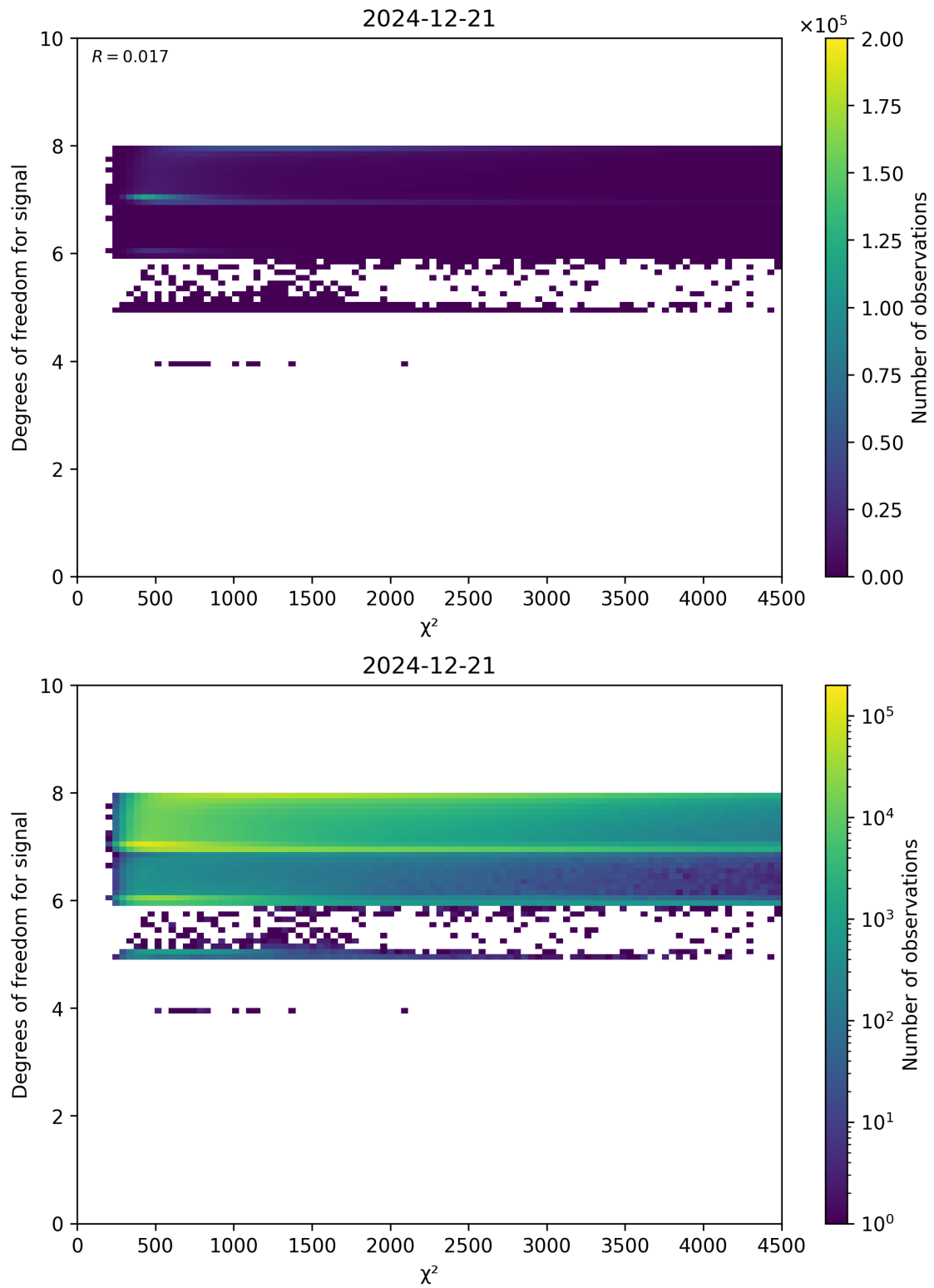
Figure 48: Scatter density plot of “ \chi^2 ” against “Degrees of freedom for signal” for 2024-12-20 to 2024-12-22.
