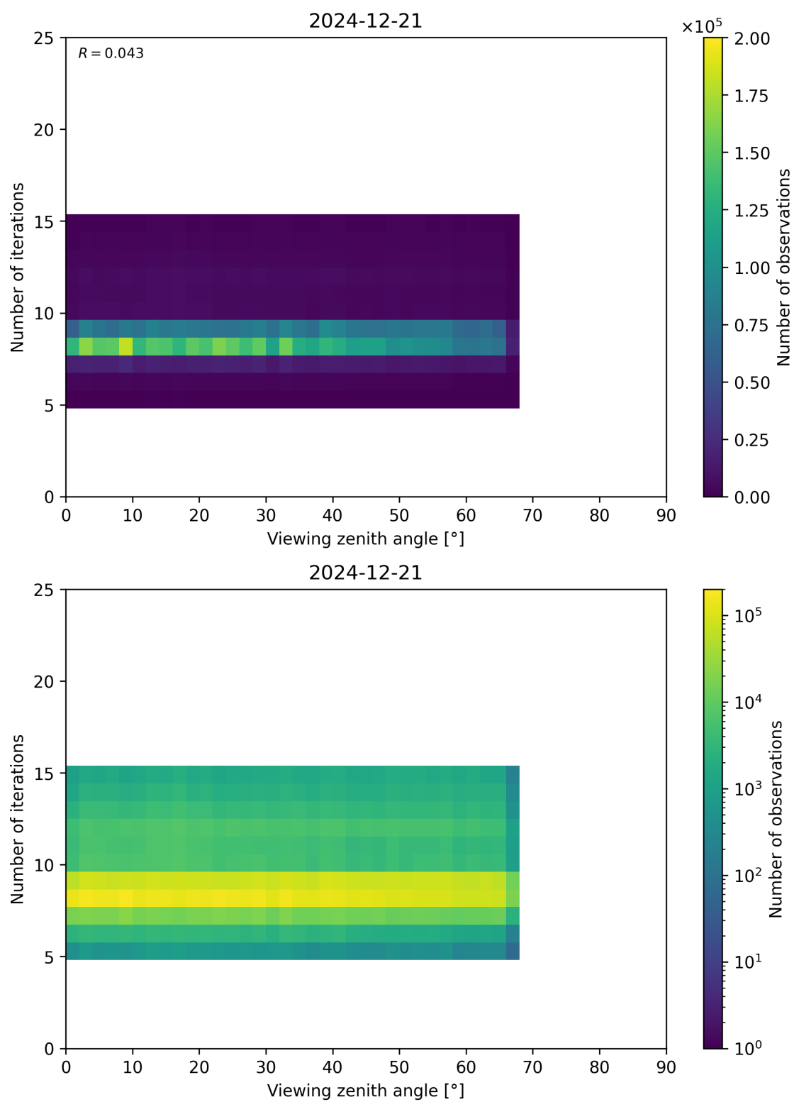
Figure 75: Scatter density plot of “Viewing zenith angle” against “Number of iterations” for 2024-12-20 to 2024-12-22.
