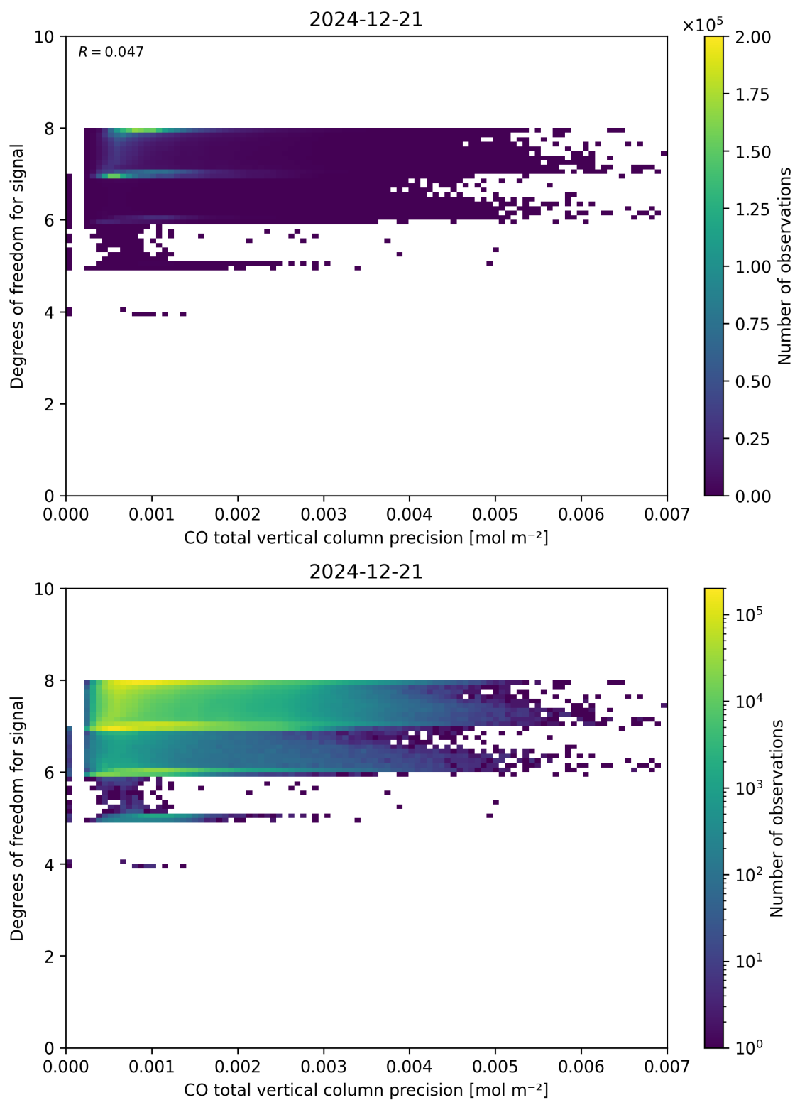
Figure 45: Scatter density plot of “CO total vertical column precision” against “Degrees of freedom for signal” for 2024-12-20 to 2024-12-22.
