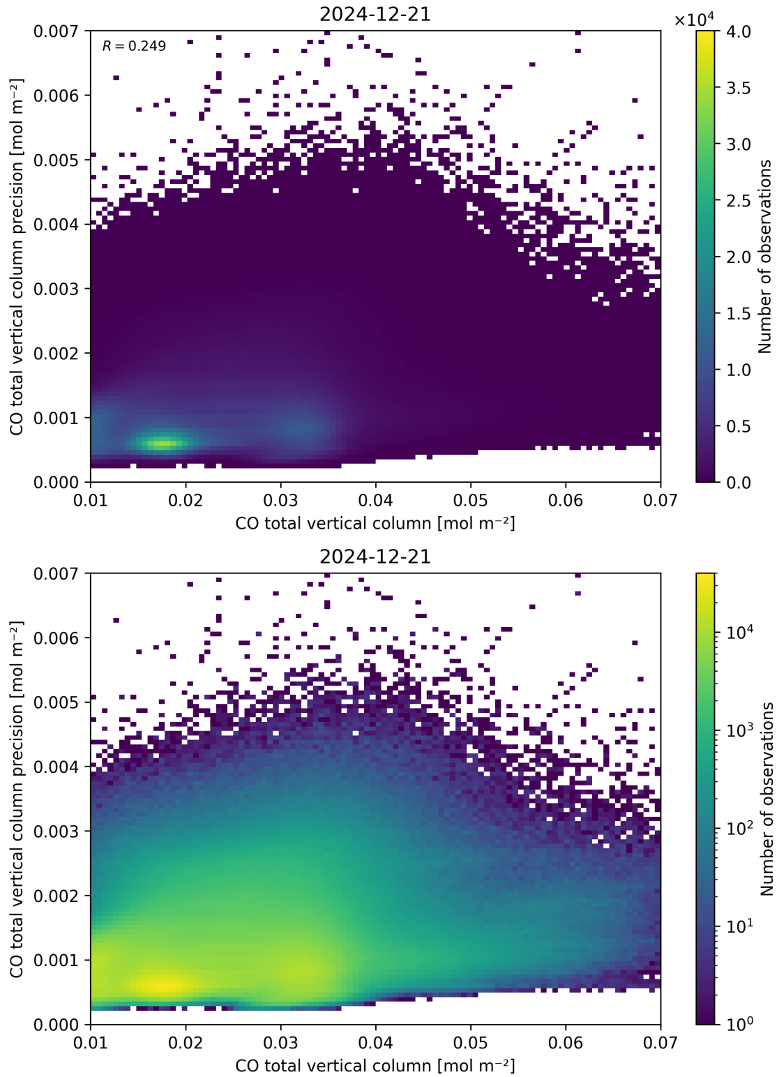
Figure 34: Scatter density plot of “CO total vertical column” against “CO total vertical column precision” for 2024-12-20 to 2024-12-22.
