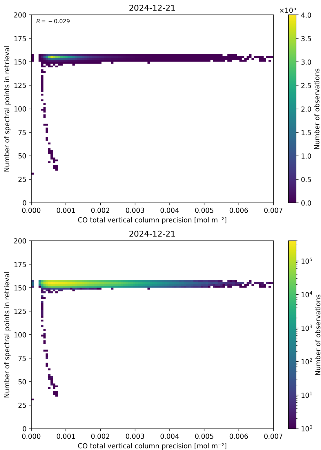
Figure 47: Scatter density plot of “CO total vertical column precision” against “Number of spectral points in retrieval” for 2024-12-20 to 2024-12-22.
