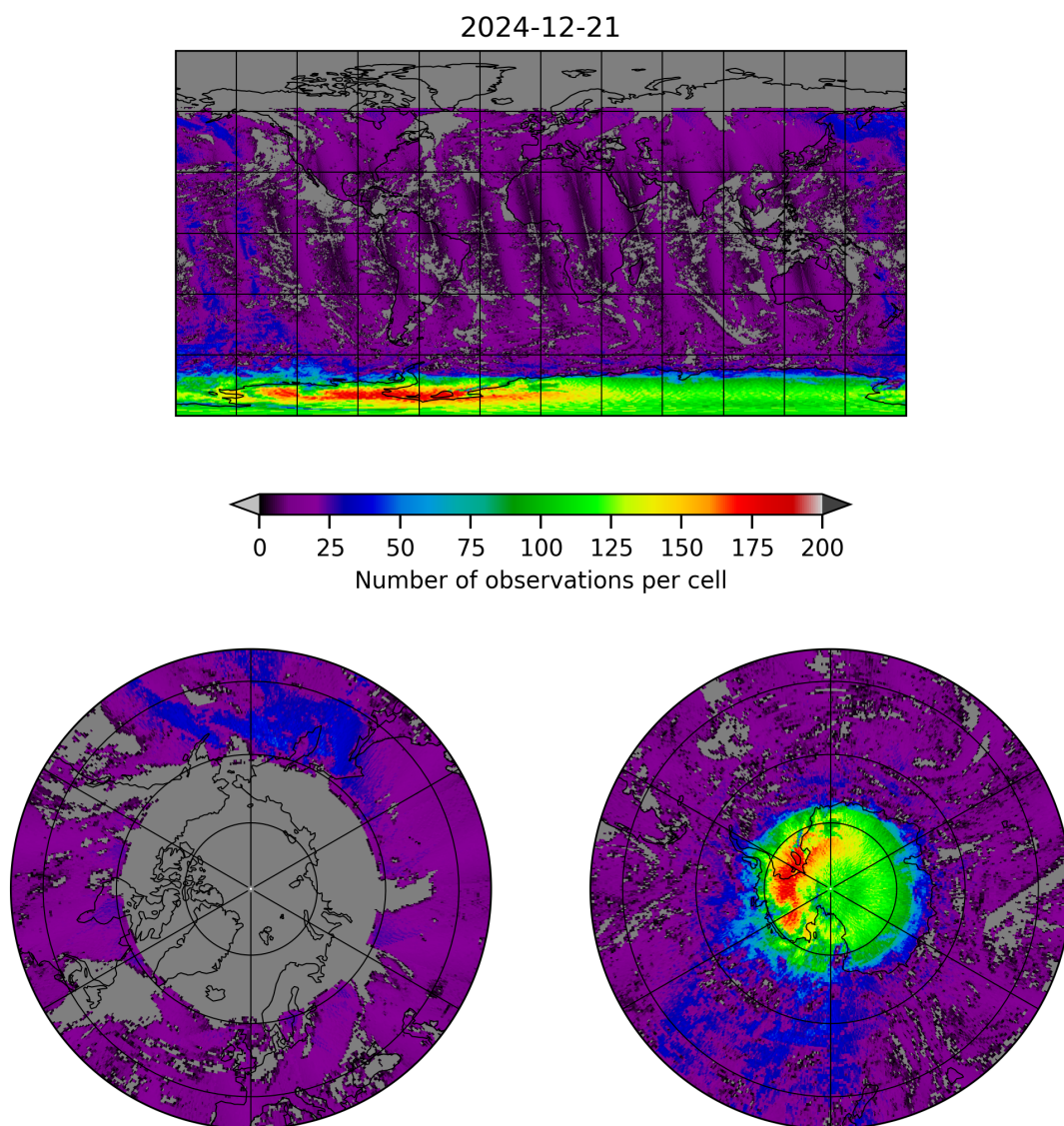
Figure 8: Map of the number of observations for 2024-12-20 to 2024-12-22
