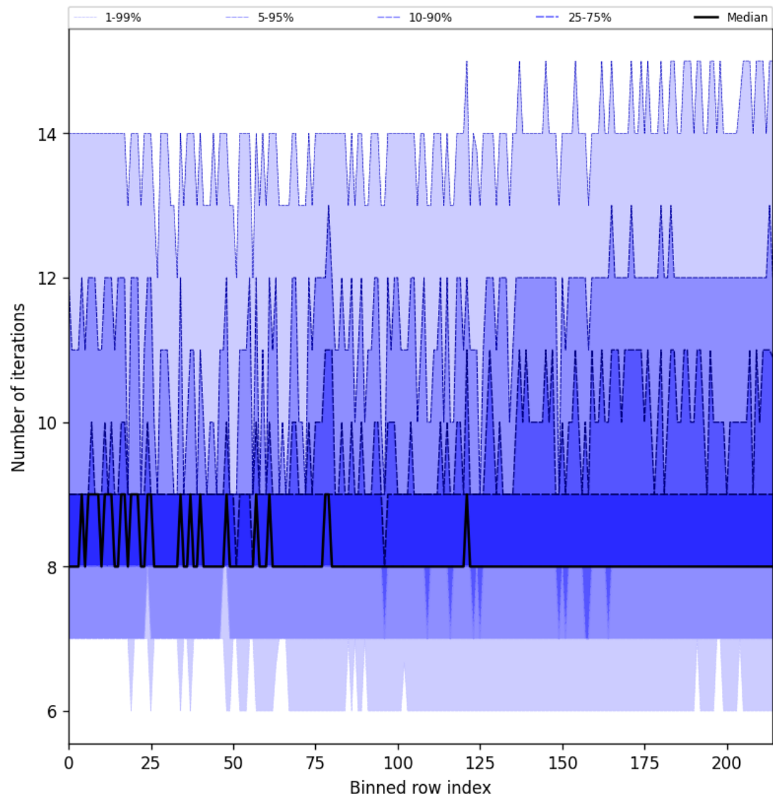
Figure 32: Along track statistics of “Number of iterations” for 2024-12-20 to 2024-12-22
