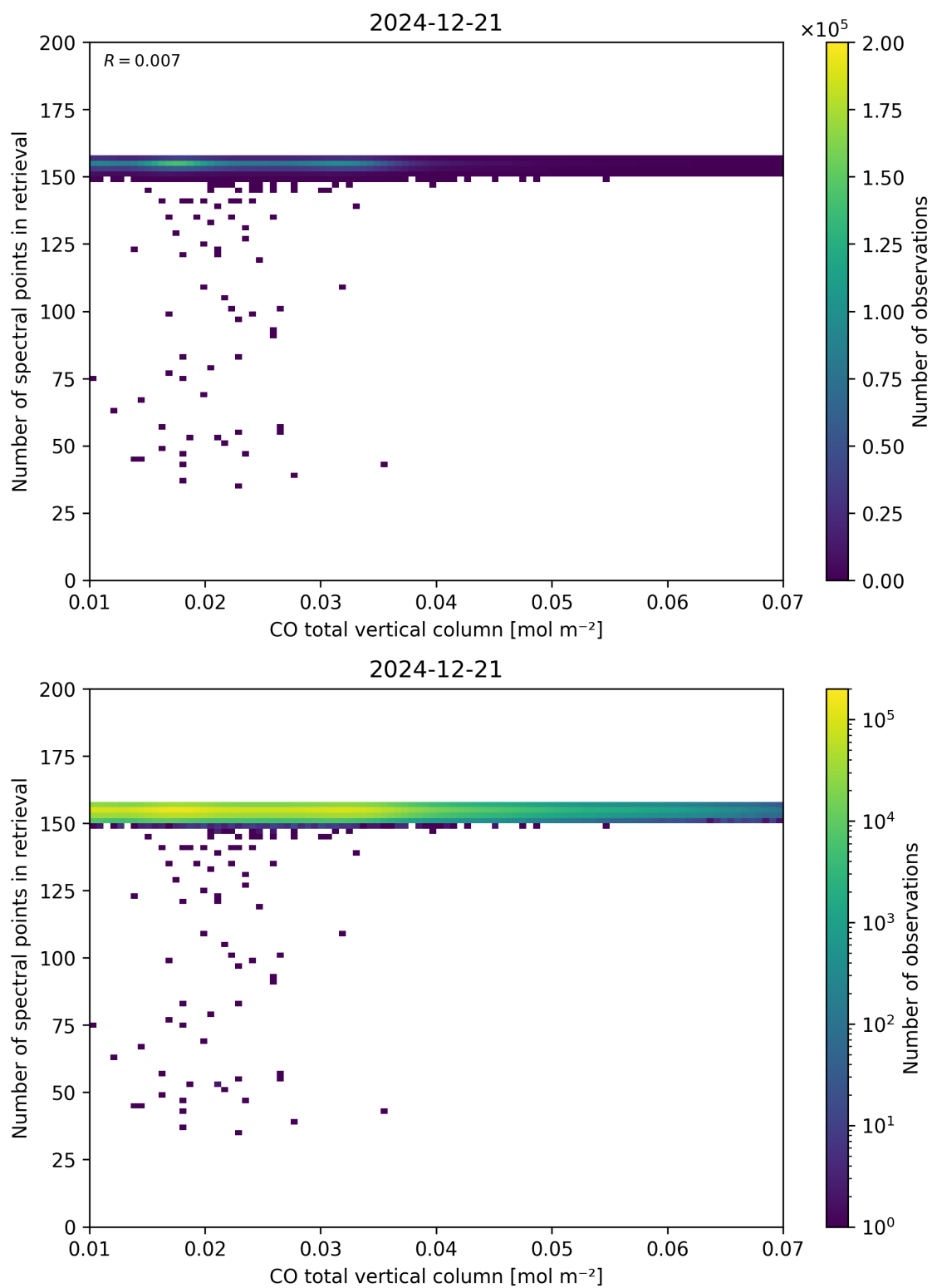
Figure 43: Scatter density plot of “CO total vertical column” against “Number of spectral points in retrieval” for 2024-12-20 to 2024-12-22.
