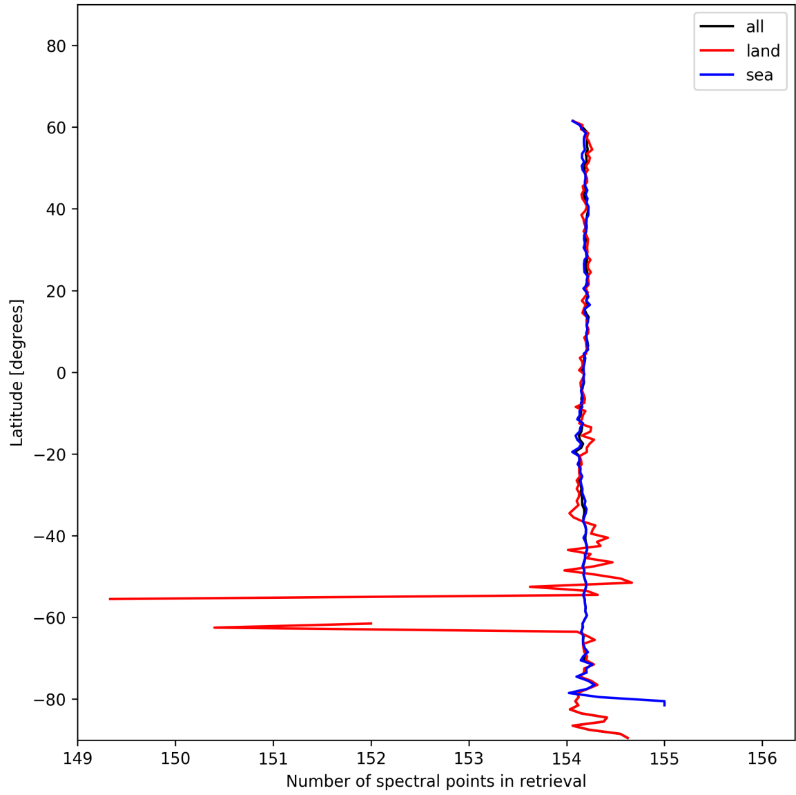
Figure 13: Zonal average of “Number of spectral points in retrieval” for 2024-12-22 to 2024-12-23.
