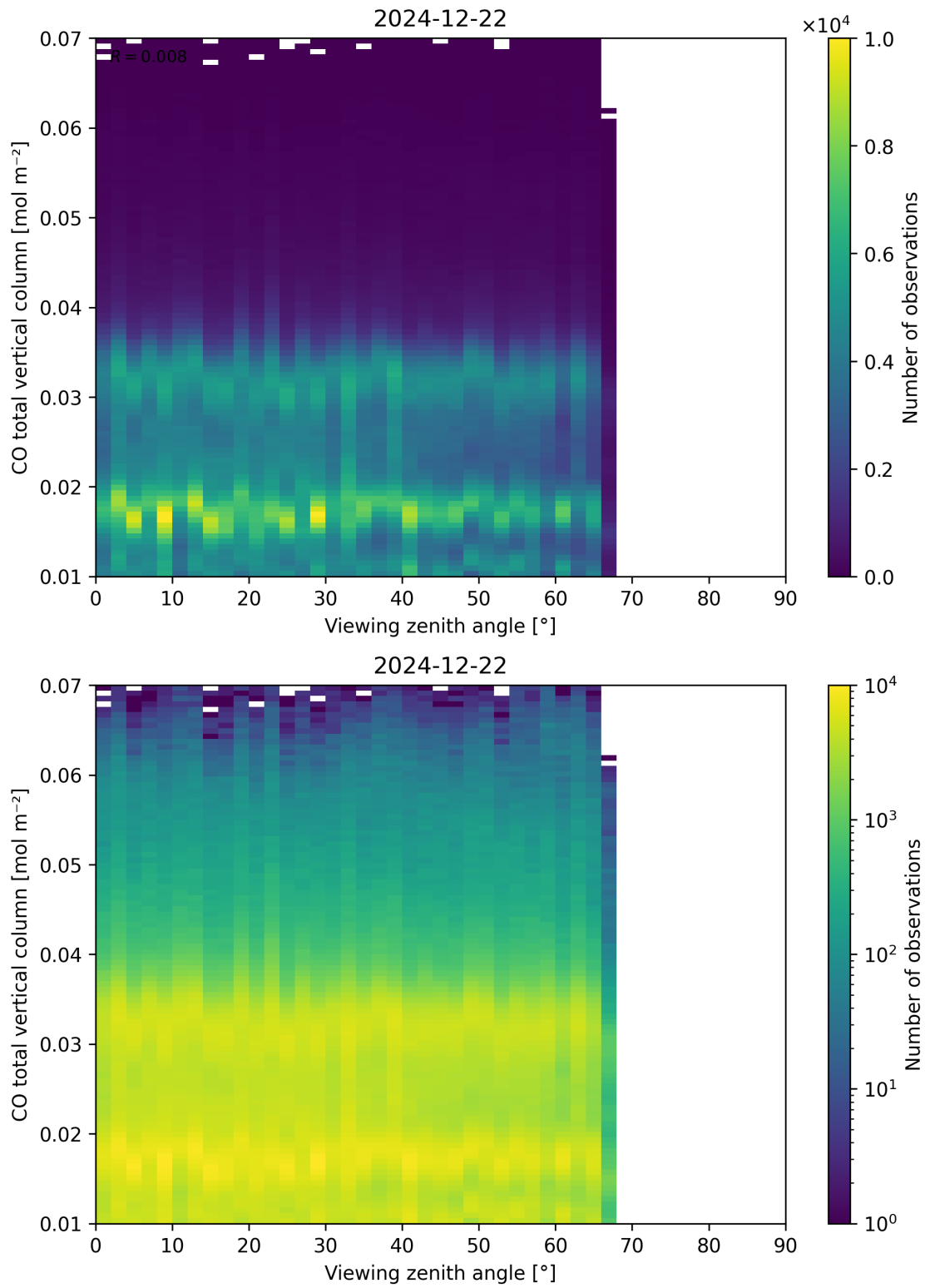
Figure 69: Scatter density plot of “Viewing zenith angle” against “CO total vertical column” for 2024-12-22 to 2024-12-23.
