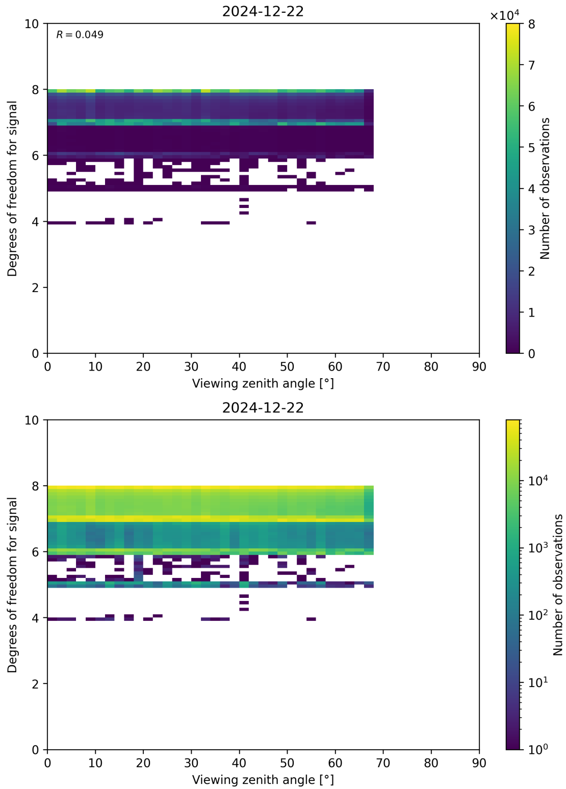
Figure 73: Scatter density plot of “Viewing zenith angle” against “Degrees of freedom for signal” for 2024-12-22 to 2024-12-23.
