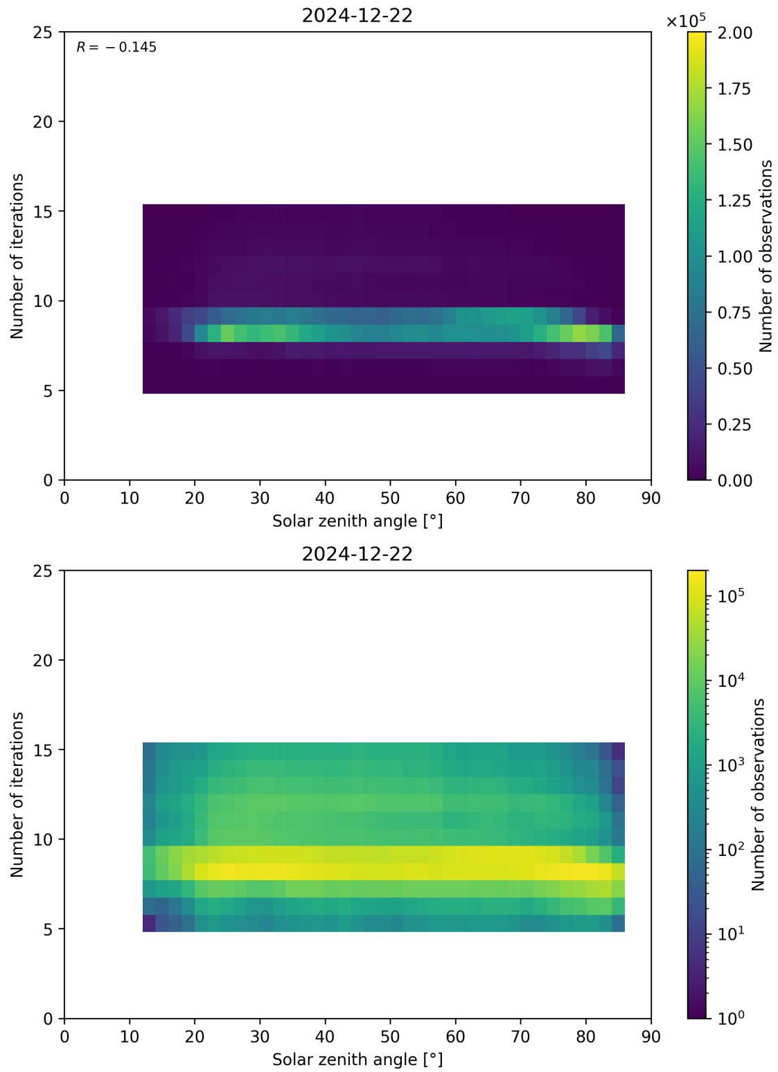
Figure 67: Scatter density plot of “Solar zenith angle” against “Number of iterations” for 2024-12-22 to 2024-12-23.
