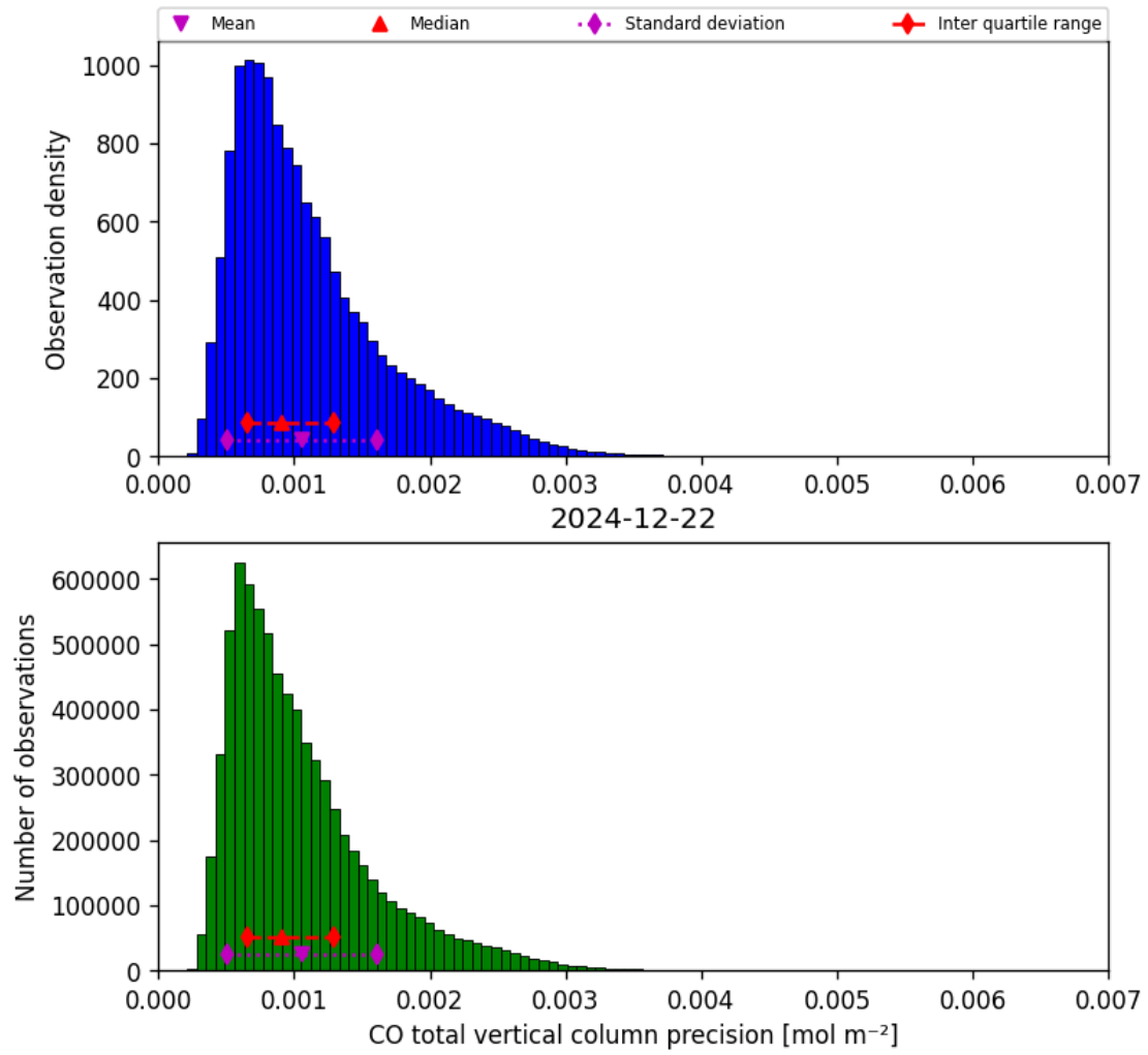
Figure 20: Histogram of “CO total vertical column precision” for 2024-12-22 to 2024-12-23
