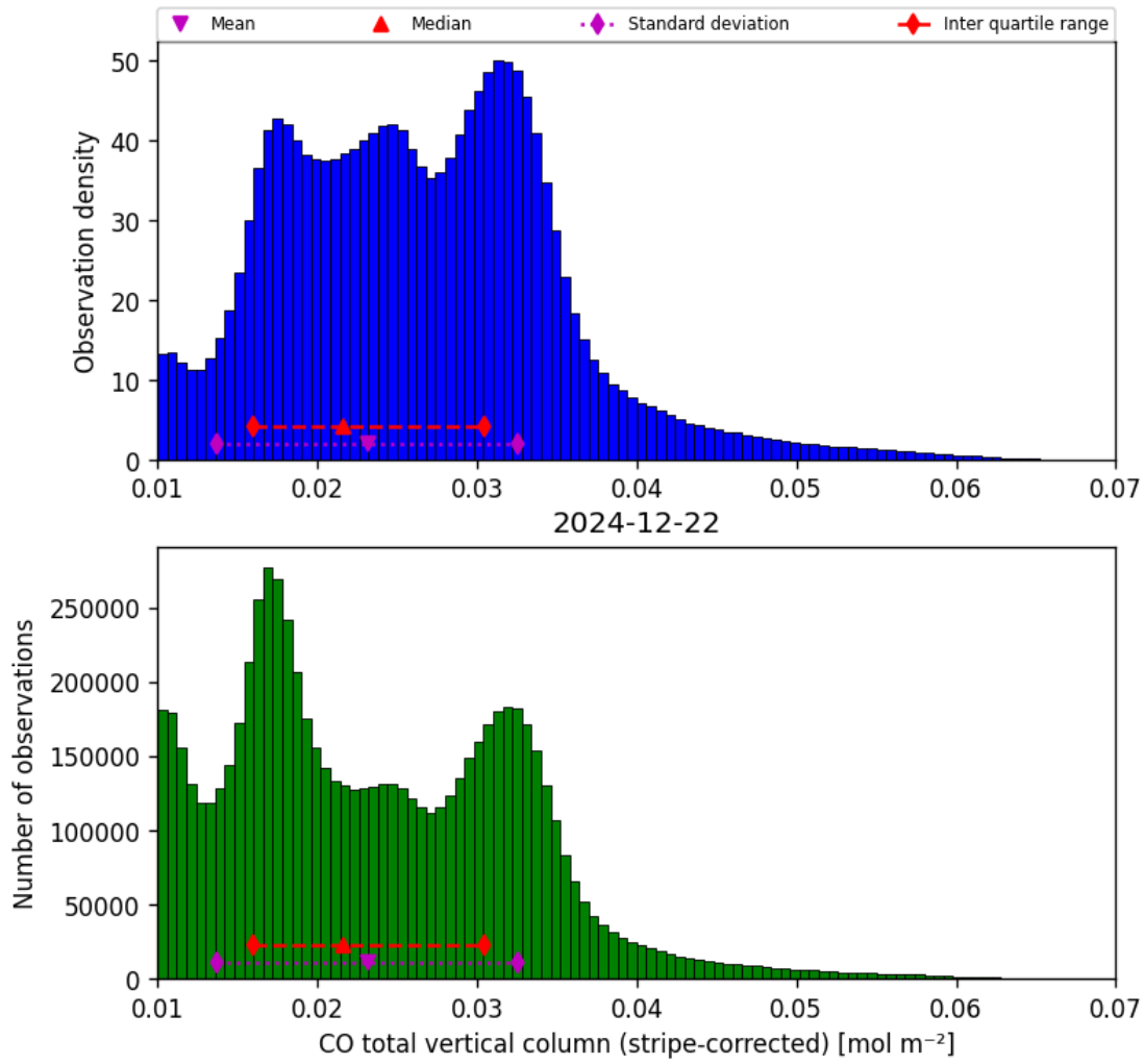
Figure 19: Histogram of “CO total vertical column (stripe-corrected)” for 2024-12-22 to 2024-12-23
