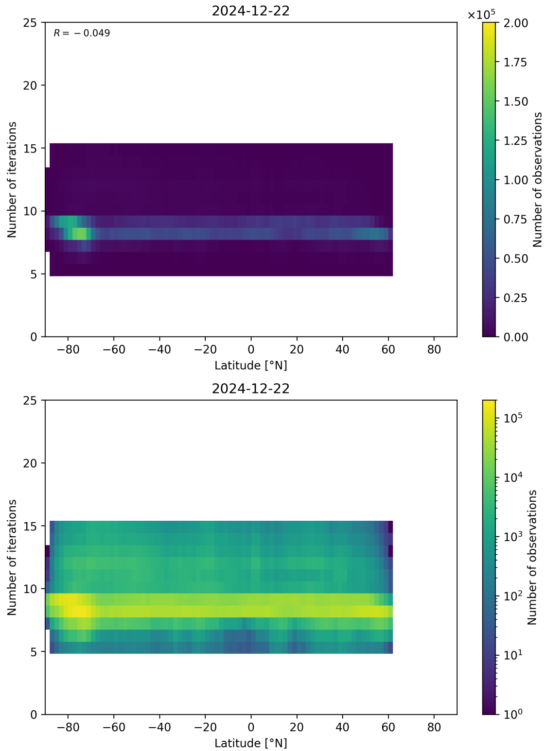
Figure 56: Scatter density plot of “Latitude” against “Number of iterations” for 2024-12-22 to 2024-12-23.
