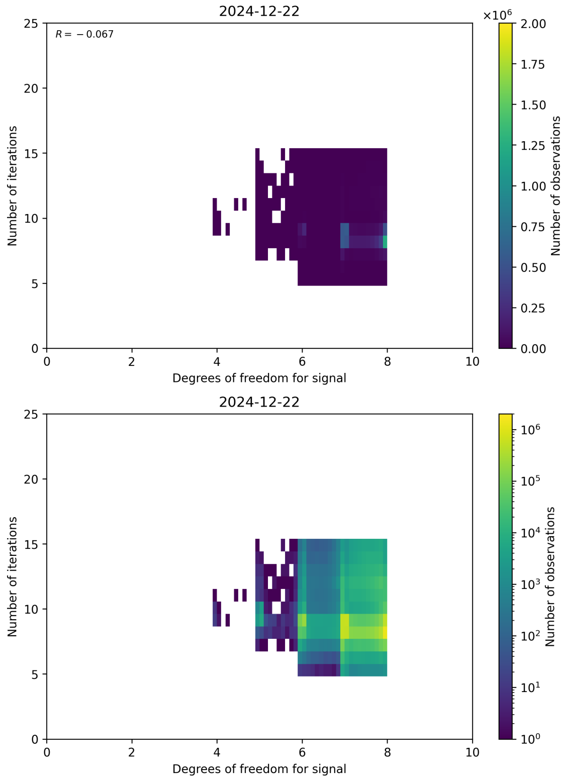
Figure 50: Scatter density plot of “Degrees of freedom for signal” against “Number of iterations” for 2024-12-22 to 2024-12-23.
