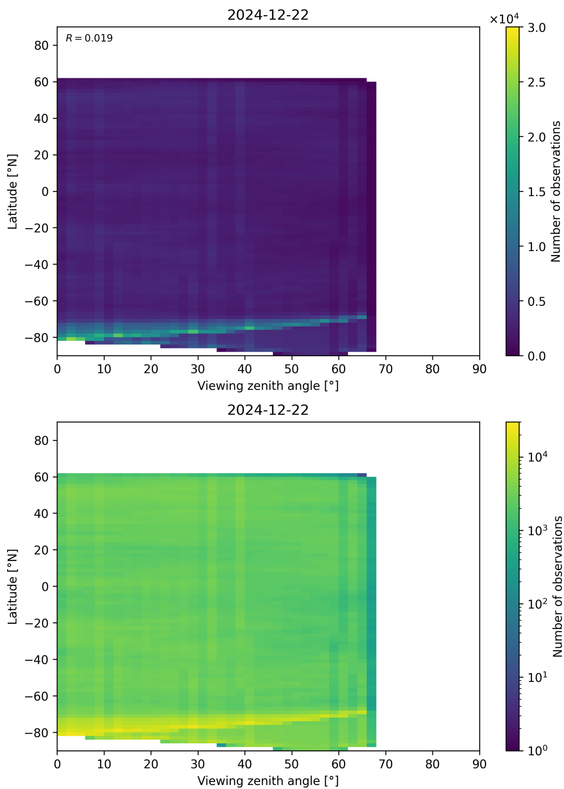
Figure 74: Scatter density plot of “Viewing zenith angle” against “Latitude” for 2024-12-22 to 2024-12-23.
