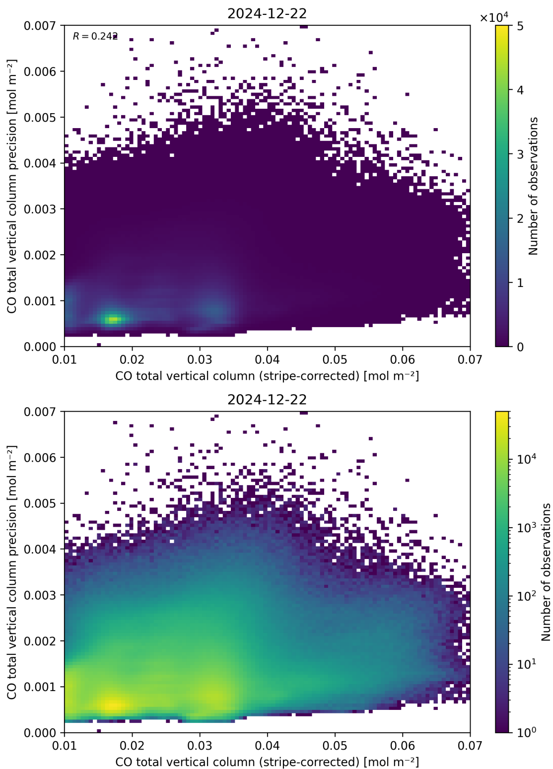
Figure 36: Scatter density plot of “CO total vertical column (stripe-corrected)” against “CO total vertical column precision” for 2024-12-22 to 2024-12-23.
