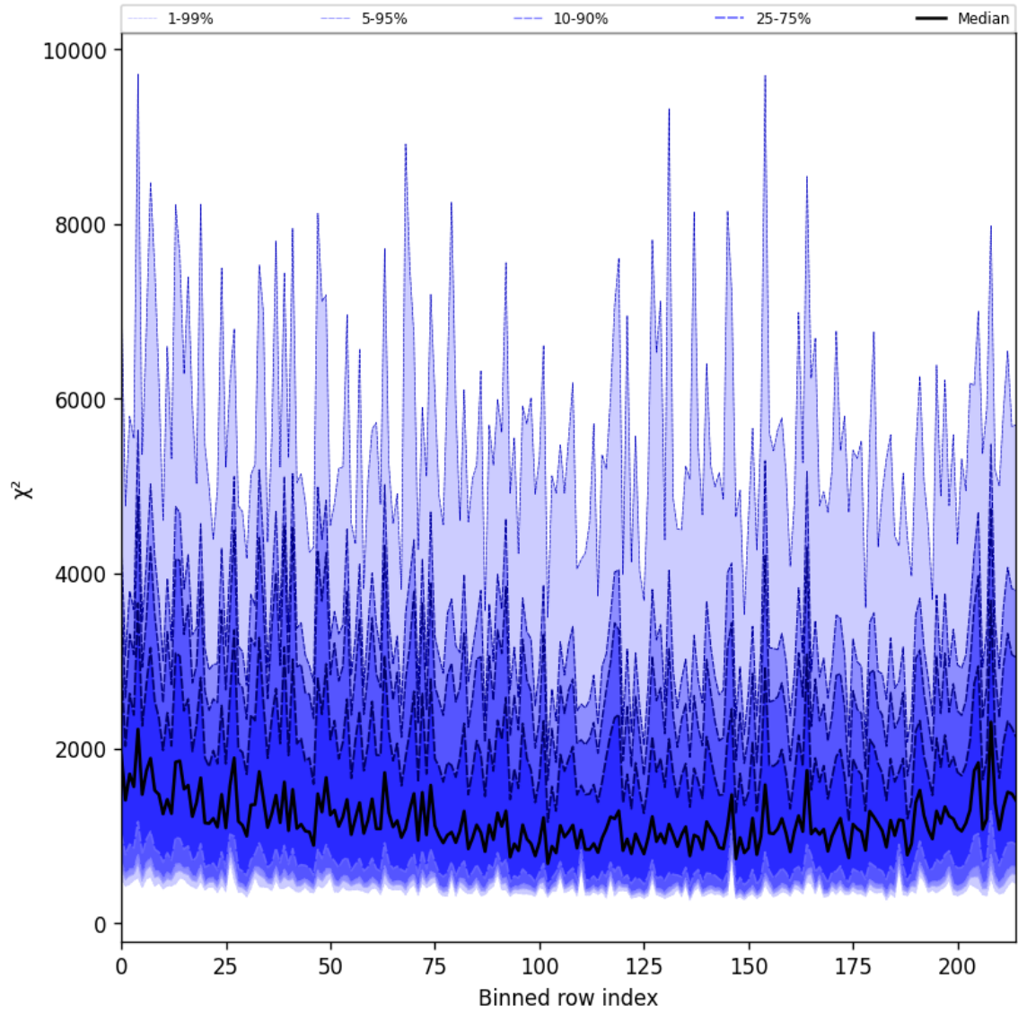
Figure 30: Along track statistics of “ \chi^2 ” for 2024-12-22 to 2024-12-23
