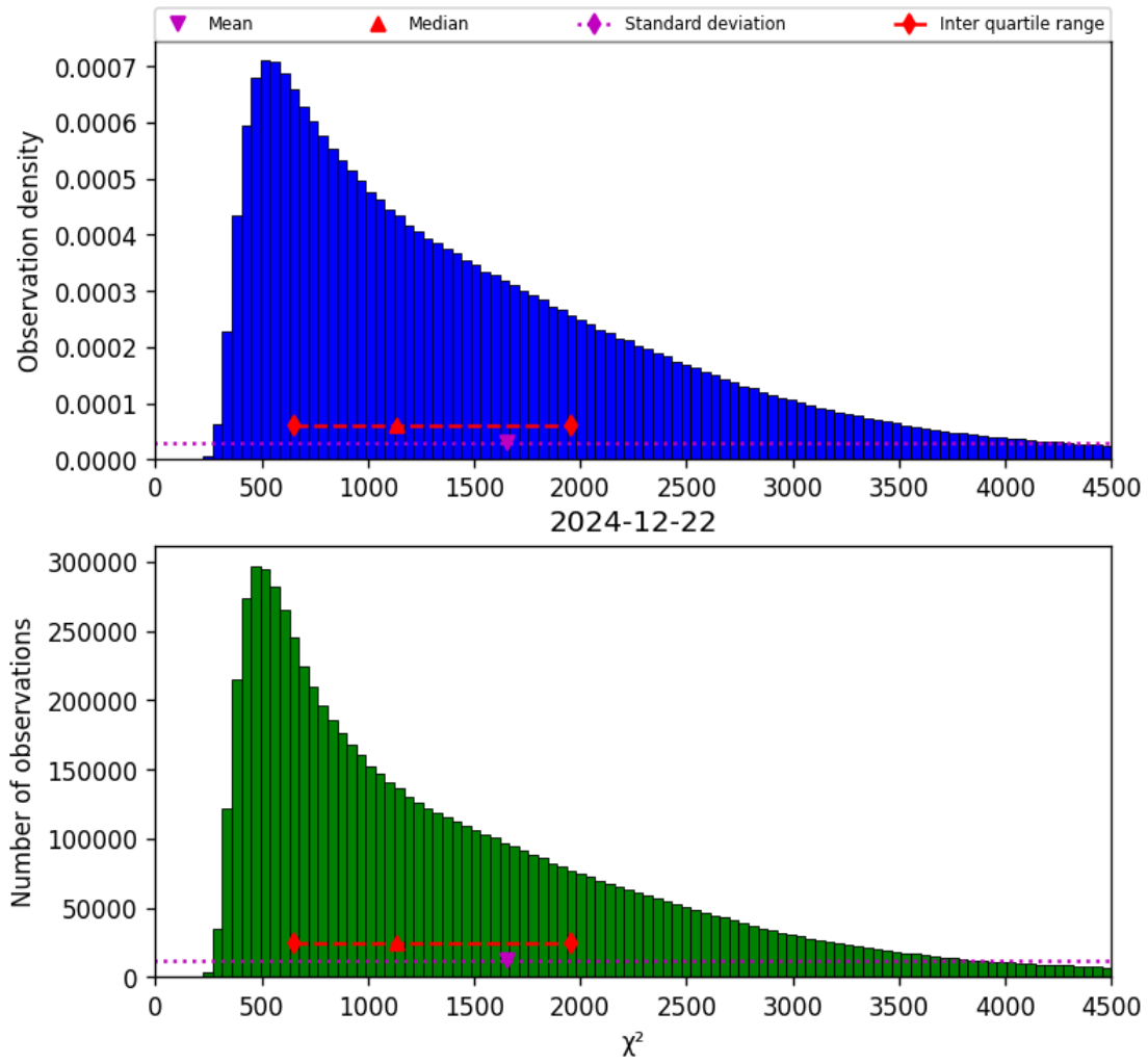
Figure 22: Histogram of “ \chi^2 ” for 2024-12-22 to 2024-12-23
