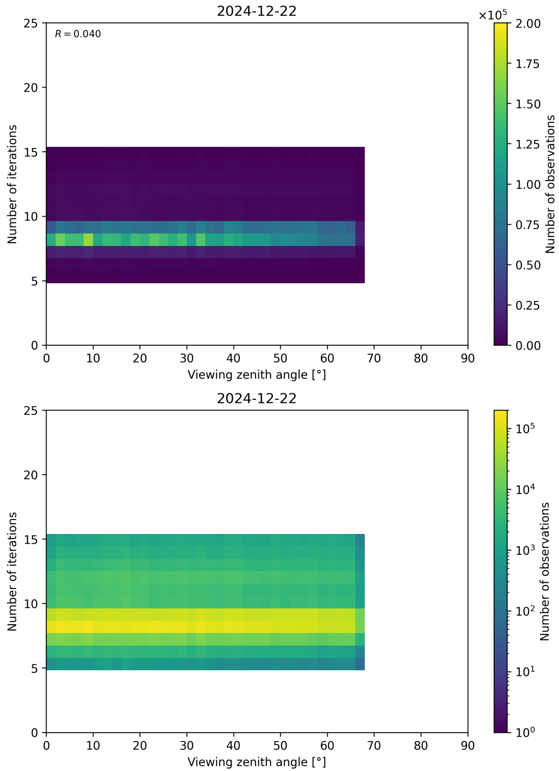
Figure 75: Scatter density plot of “Viewing zenith angle” against “Number of iterations” for 2024-12-22 to 2024-12-23.
