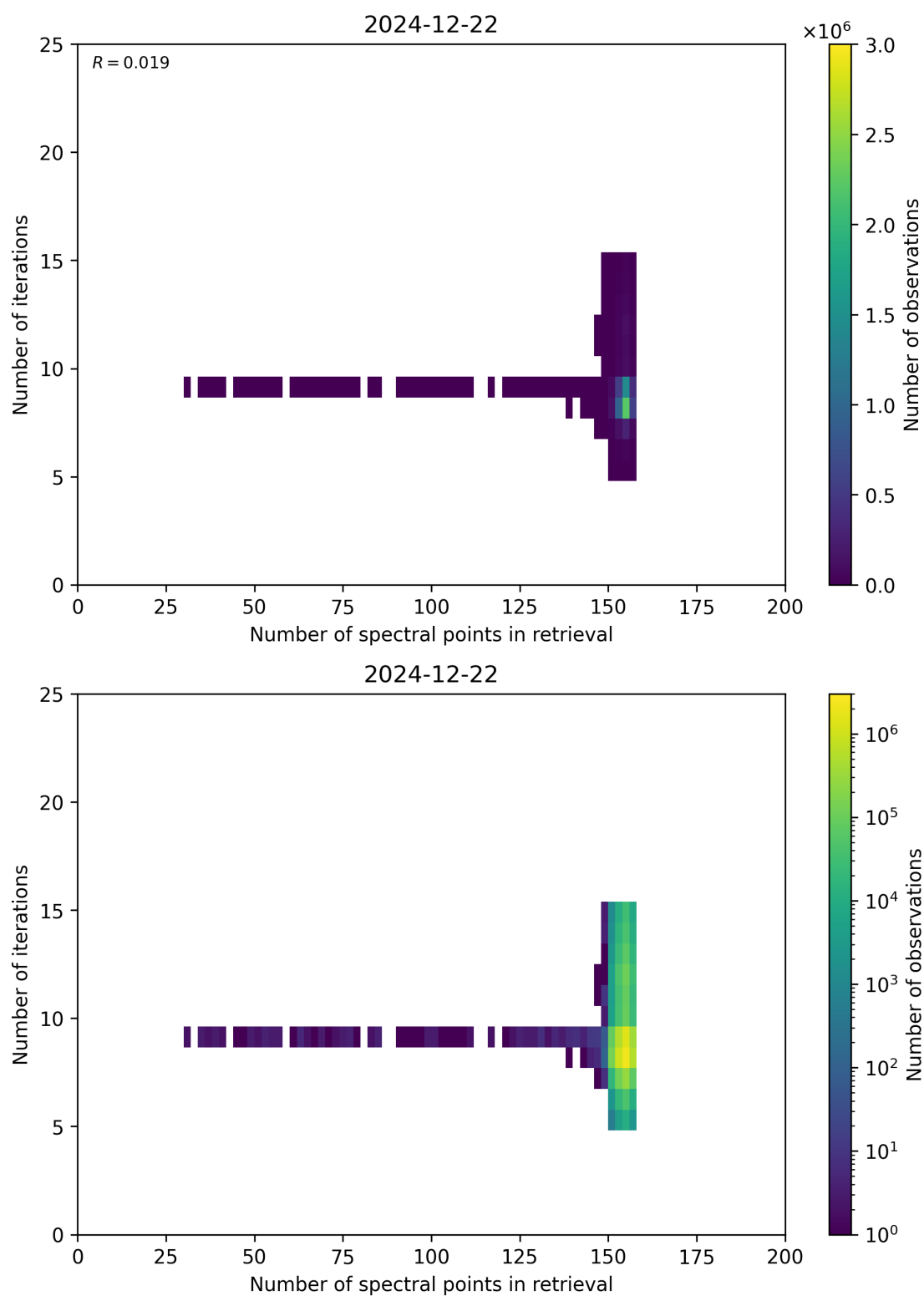
Figure 60: Scatter density plot of “Number of spectral points in retrieval” against “Number of iterations” for 2024-12-22 to 2024-12-23.
