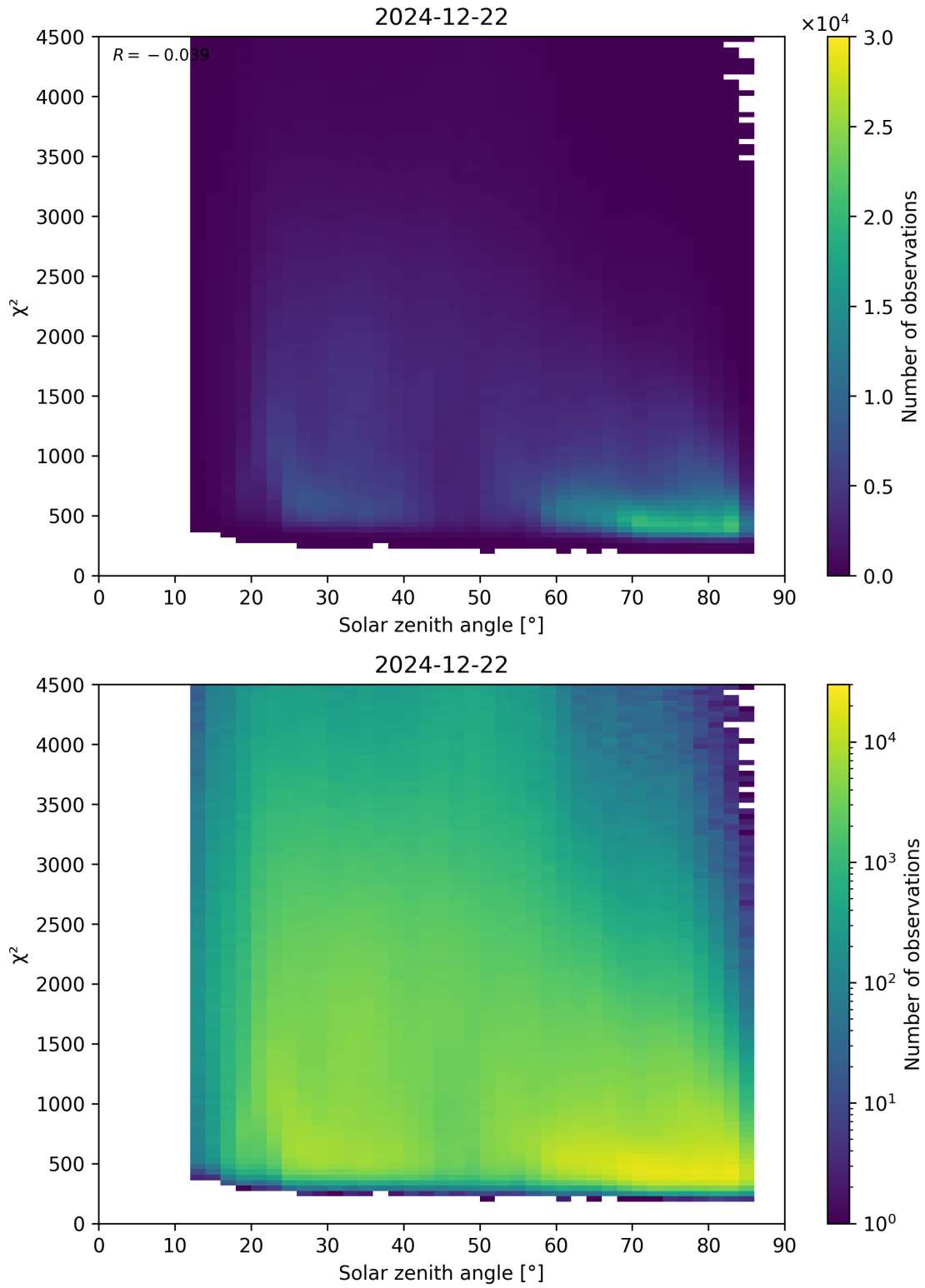
Figure 64: Scatter density plot of “Solar zenith angle” against “ \chi^2 ” for 2024-12-22 to 2024-12-23.
