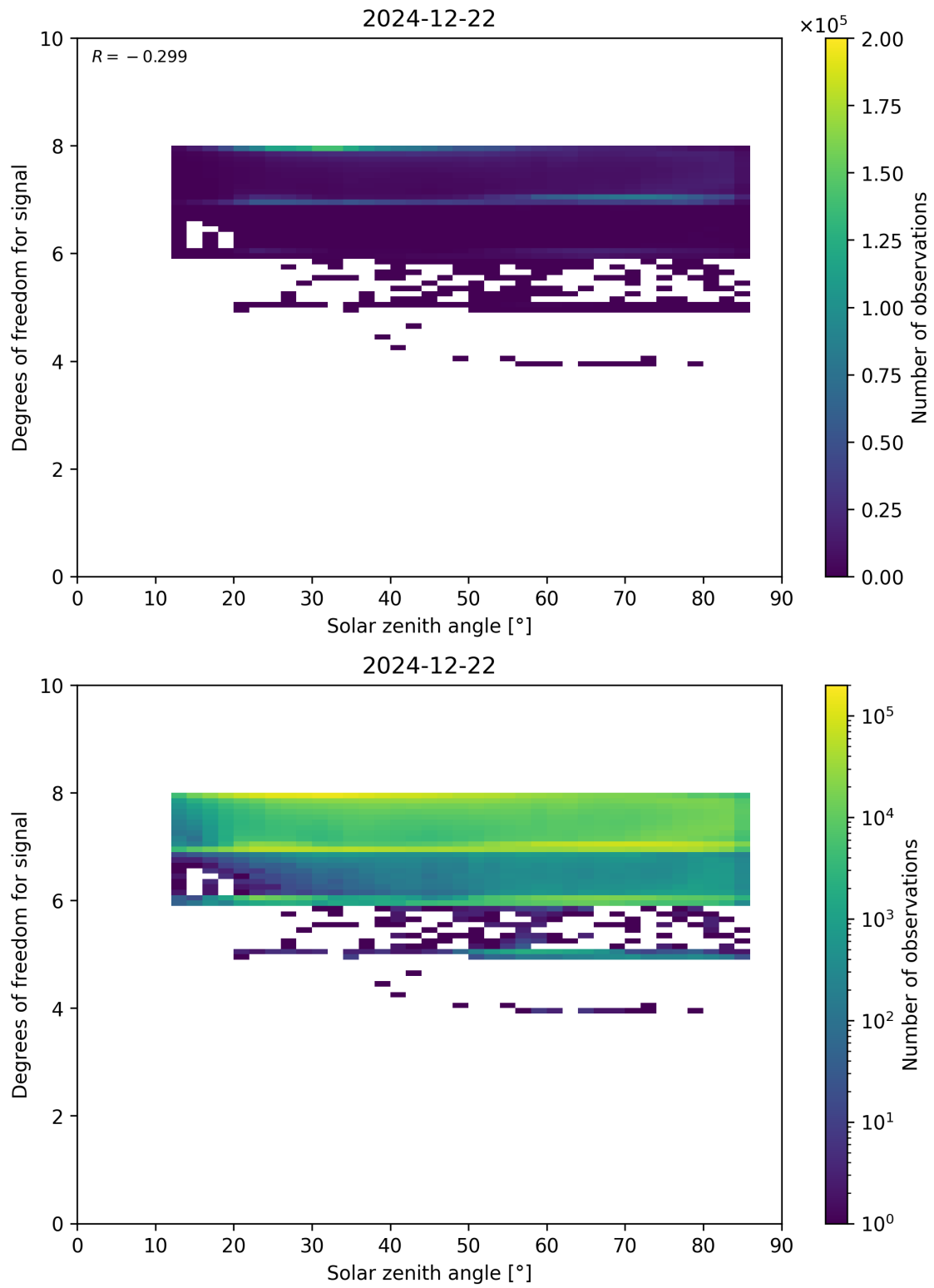
Figure 65: Scatter density plot of “Solar zenith angle” against “Degrees of freedom for signal” for 2024-12-22 to 2024-12-23.
