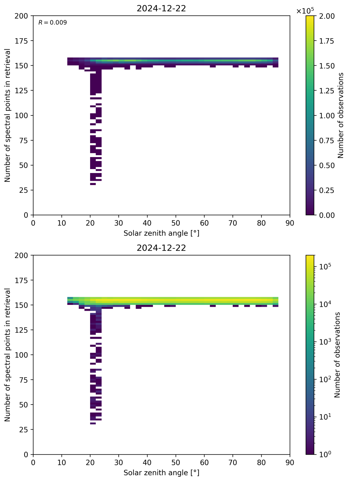
Figure 68: Scatter density plot of “Solar zenith angle” against “Number of spectral points in retrieval” for 2024-12-22 to 2024-12-23.
