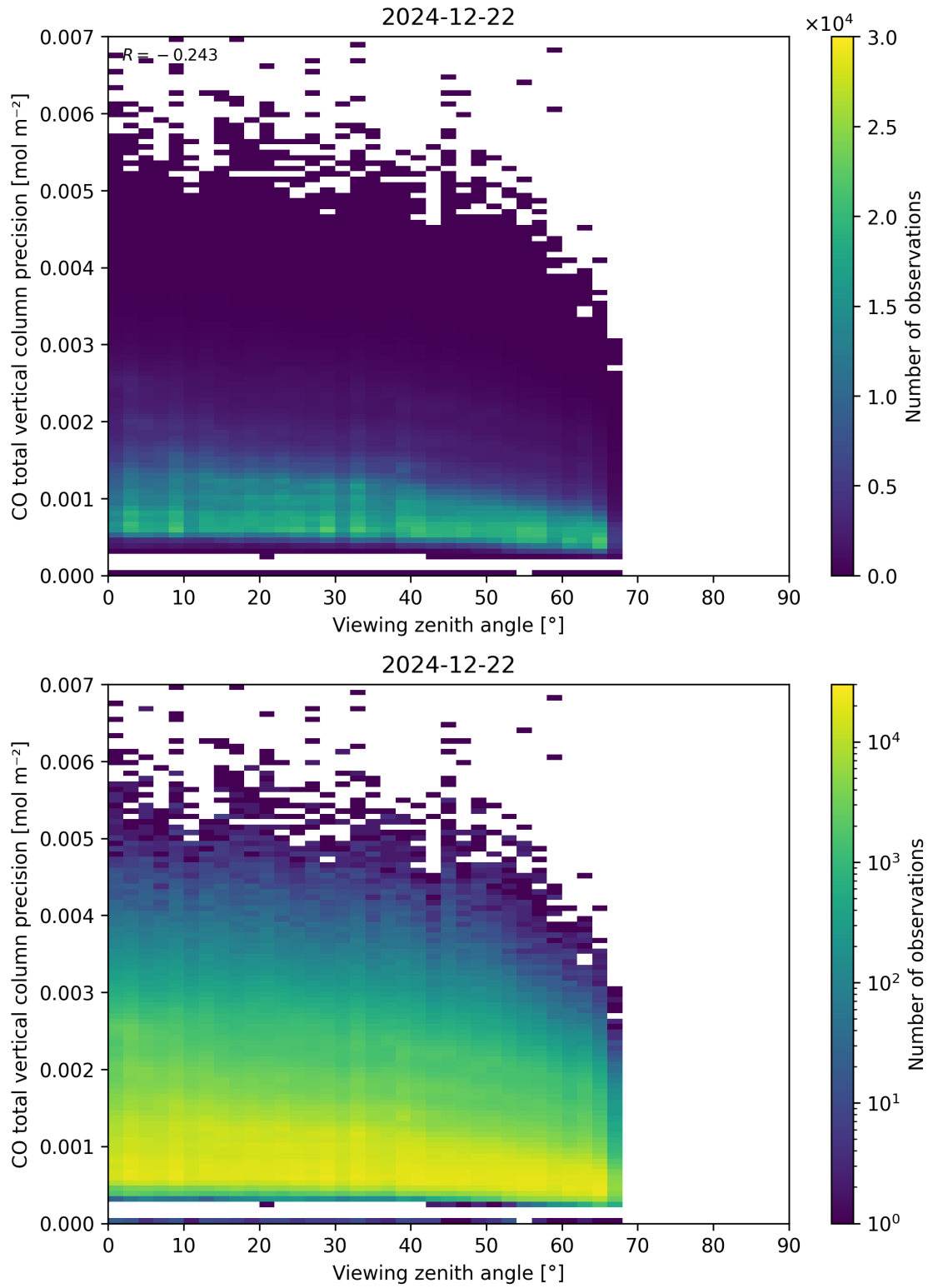
Figure 71: Scatter density plot of “Viewing zenith angle” against “CO total vertical column precision” for 2024-12-22 to 2024-12-23.
