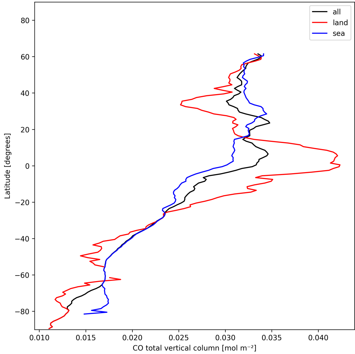
Figure 10: Zonal average of “CO total vertical column” for 2024-12-22 to 2024-12-23.
