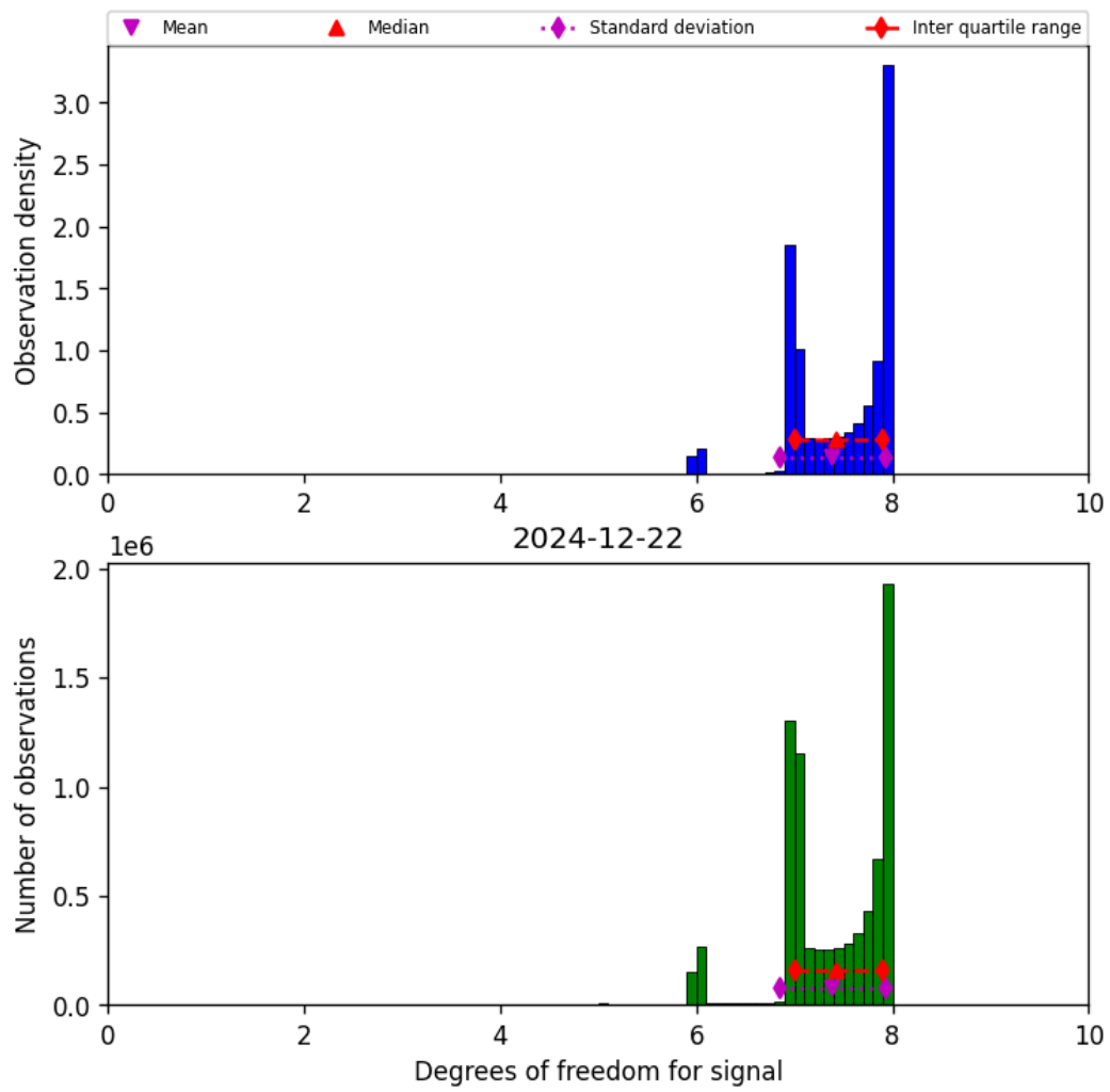
Figure 23: Histogram of “Degrees of freedom for signal” for 2024-12-22 to 2024-12-23
