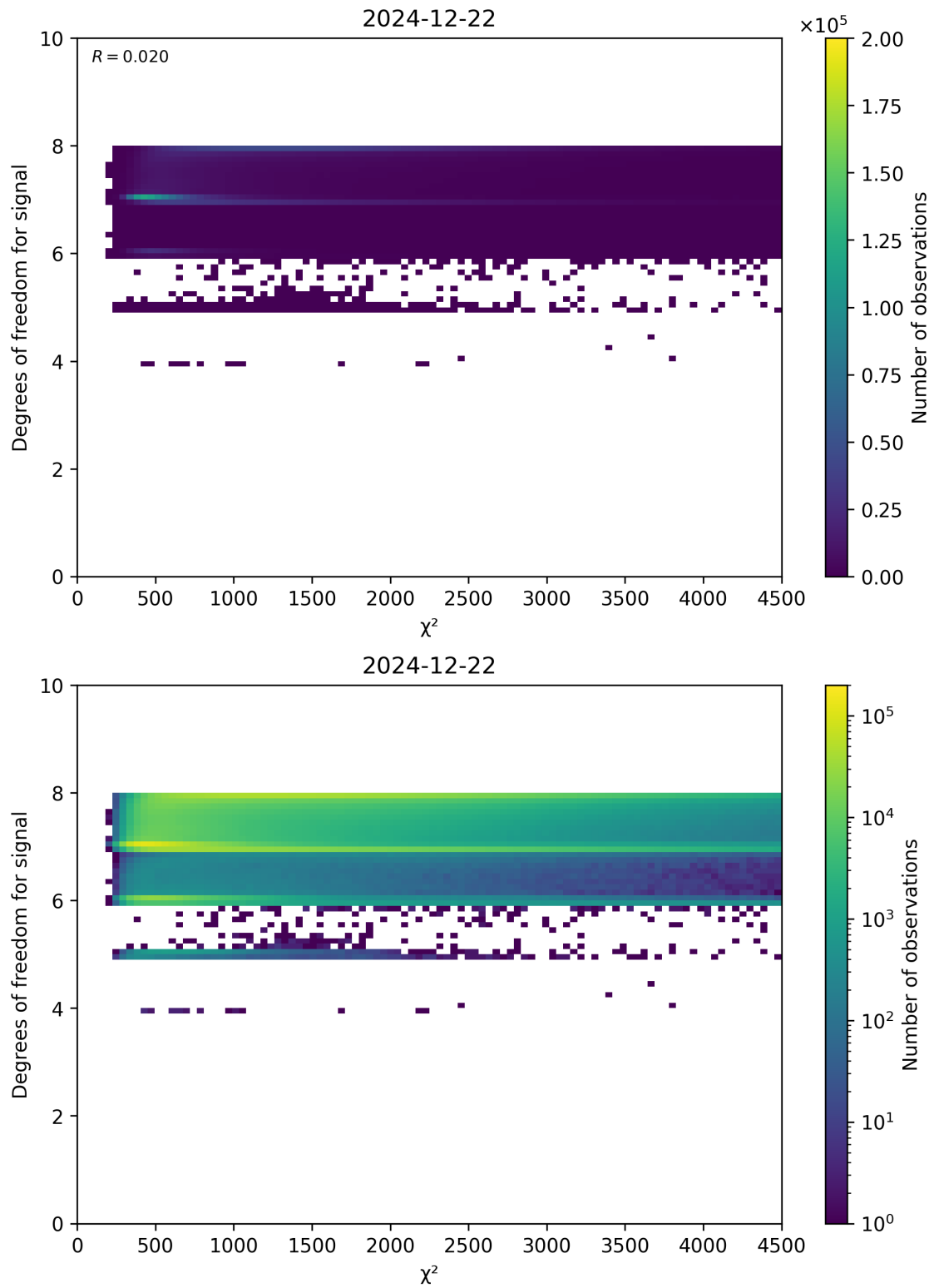
Figure 48: Scatter density plot of “ \chi^2 ” against “Degrees of freedom for signal” for 2024-12-22 to 2024-12-23.
