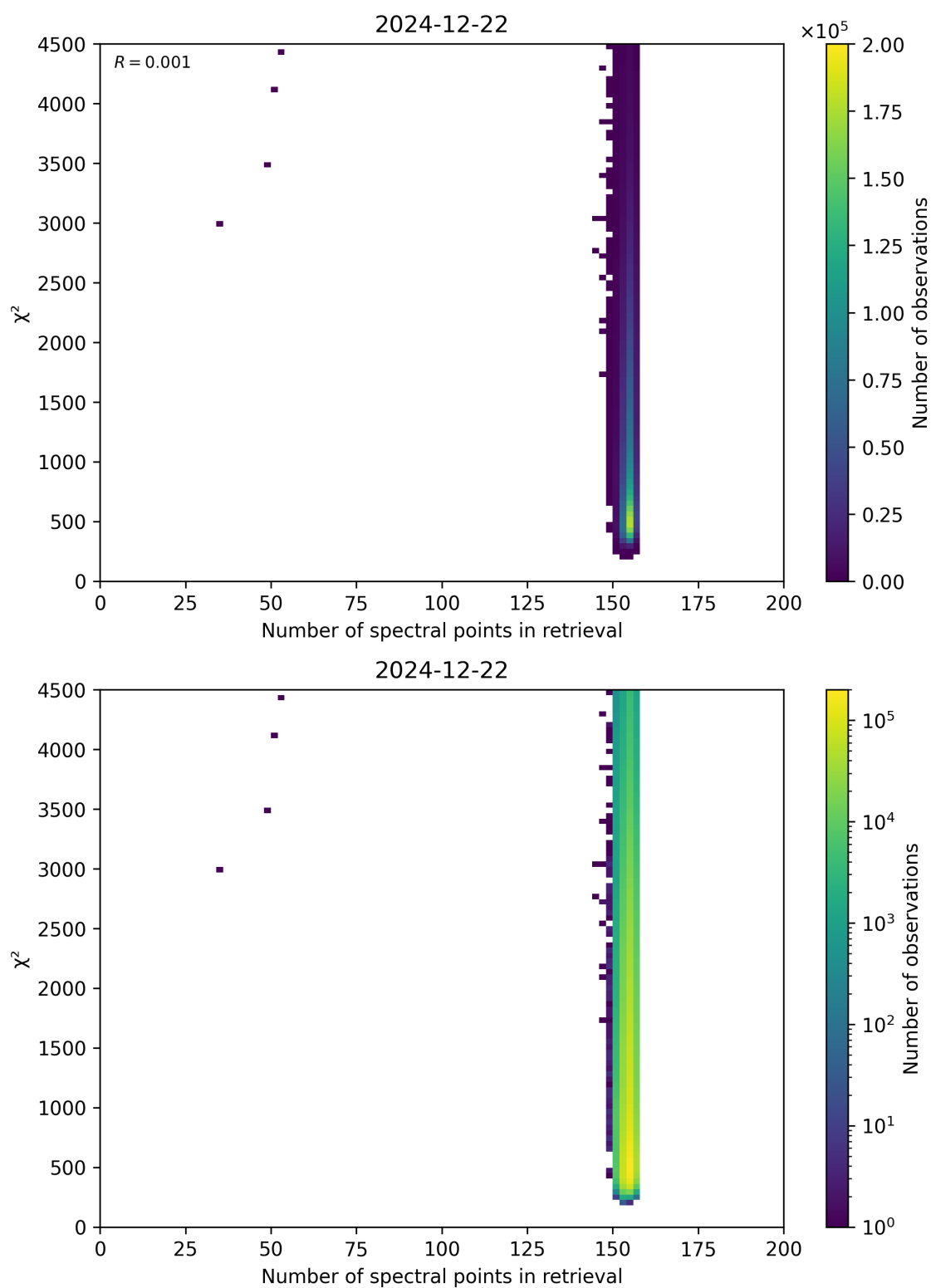
Figure 58: Scatter density plot of “Number of spectral points in retrieval” against “ \chi^2 ” for 2024-12-22 to 2024-12-23.
