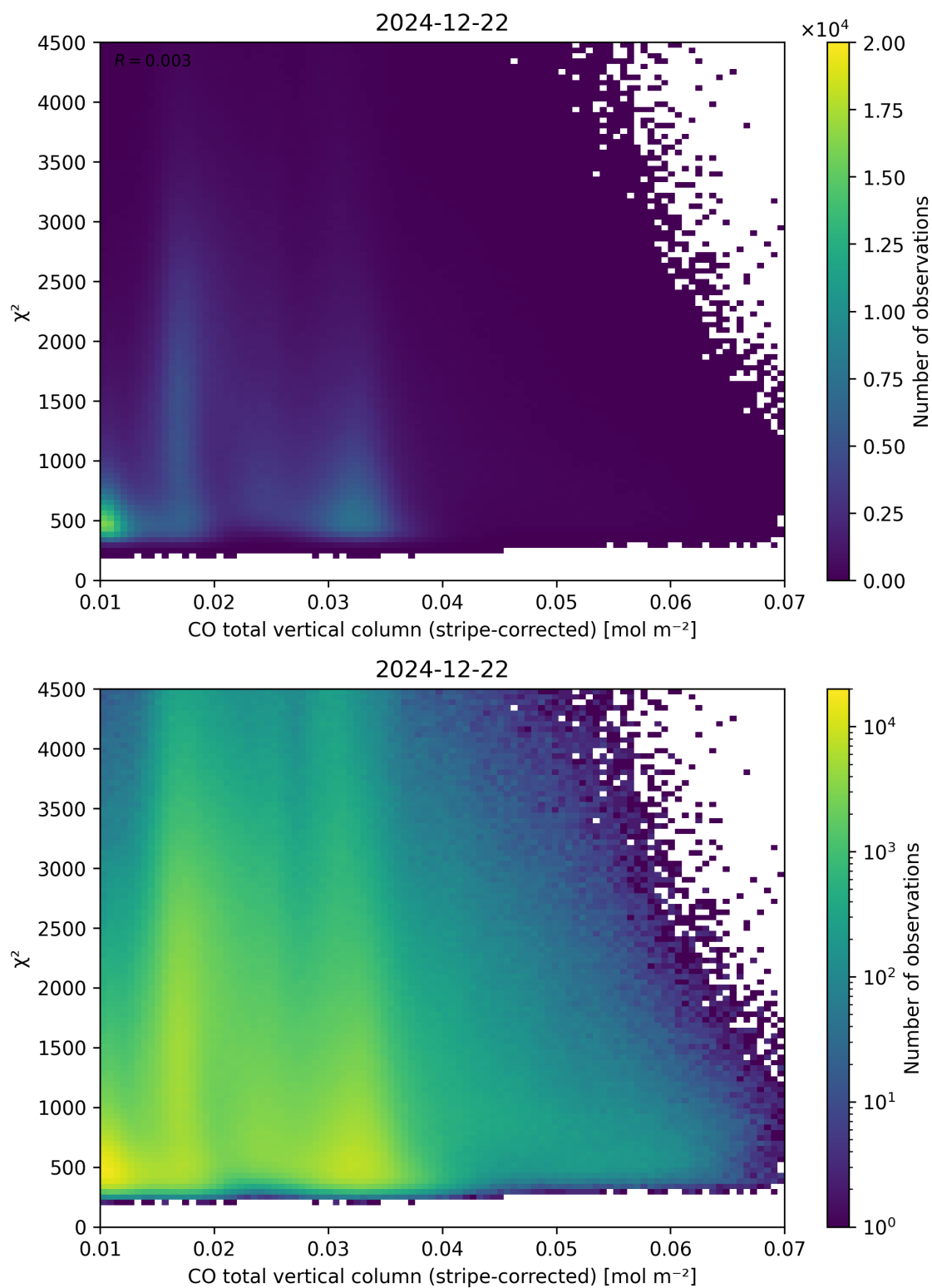
Figure 37: Scatter density plot of “CO total vertical column (stripe-corrected)” against “ \chi^2 ” for 2024-12-22 to 2024-12-23.
