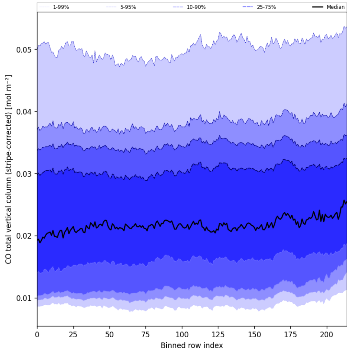
Figure 27: Along track statistics of “CO total vertical column (stripe-corrected)” for 2024-12-22 to 2024-12-23
