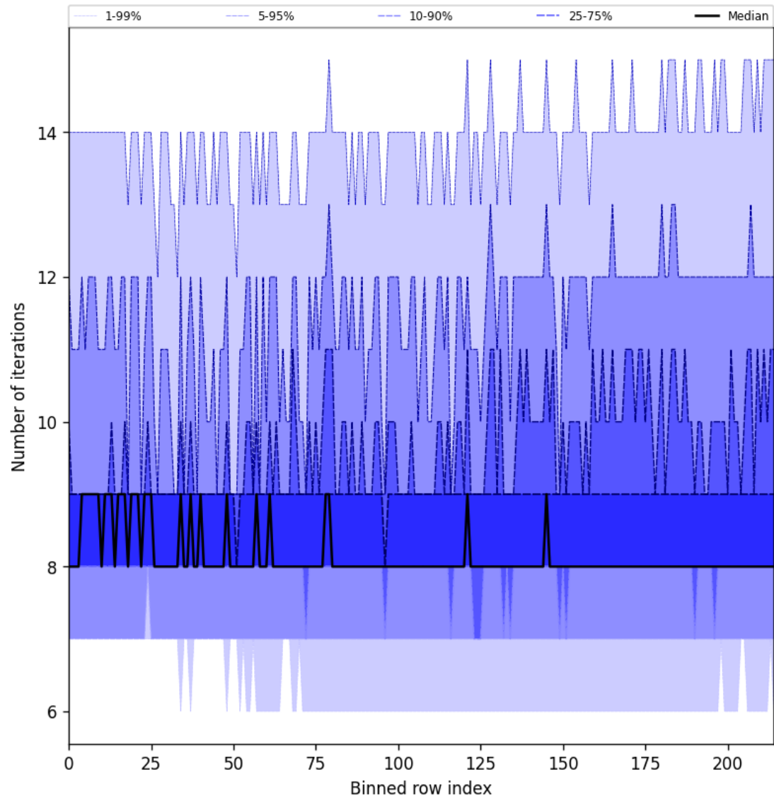
Figure 32: Along track statistics of “Number of iterations” for 2024-12-22 to 2024-12-23
