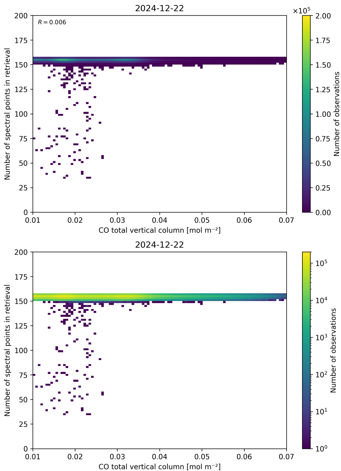
Figure 43: Scatter density plot of “CO total vertical column” against “Number of spectral points in retrieval” for 2024-12-22 to 2024-12-23.
