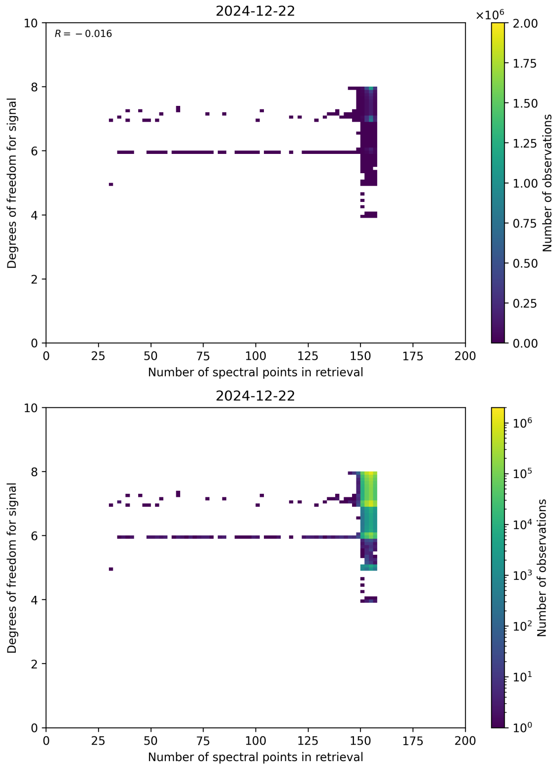
Figure 59: Scatter density plot of “Number of spectral points in retrieval” against “Degrees of freedom for signal” for 2024-12-22 to 2024-12-23.
