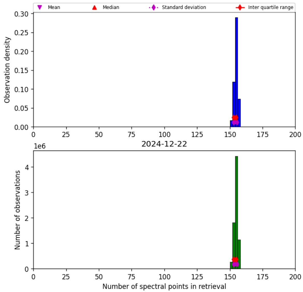
Figure 21: Histogram of “Number of spectral points in retrieval” for 2024-12-22 to 2024-12-23
