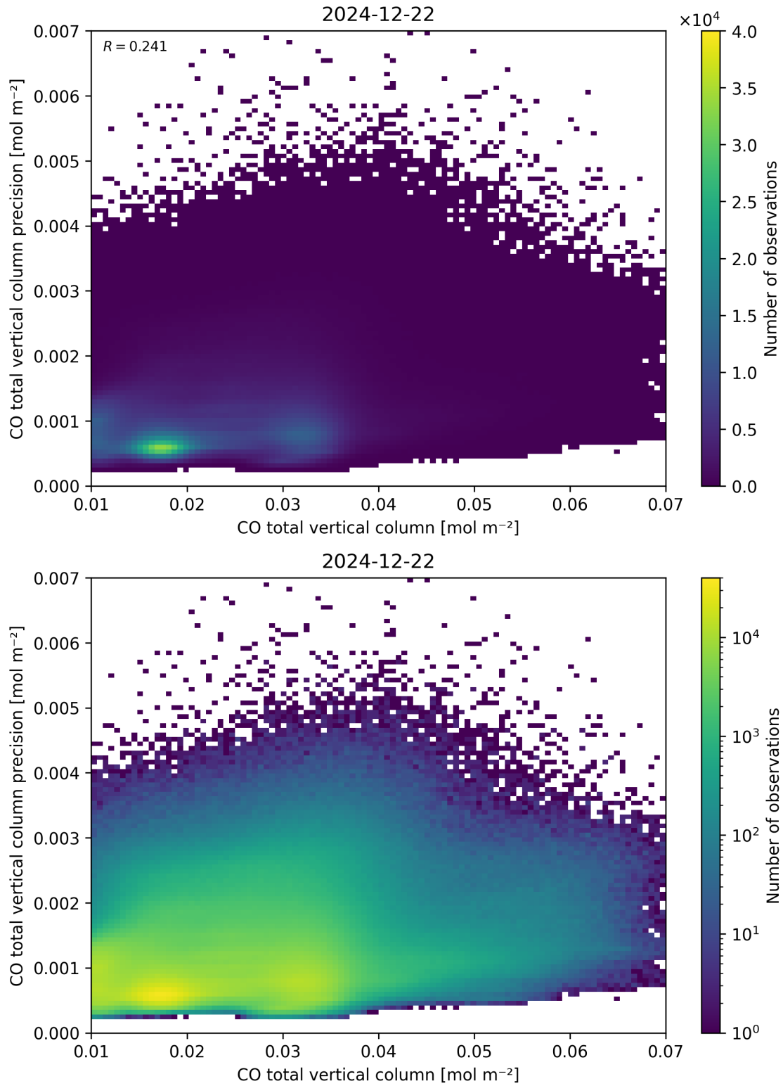
Figure 34: Scatter density plot of “CO total vertical column” against “CO total vertical column precision” for 2024-12-22 to 2024-12-23.
