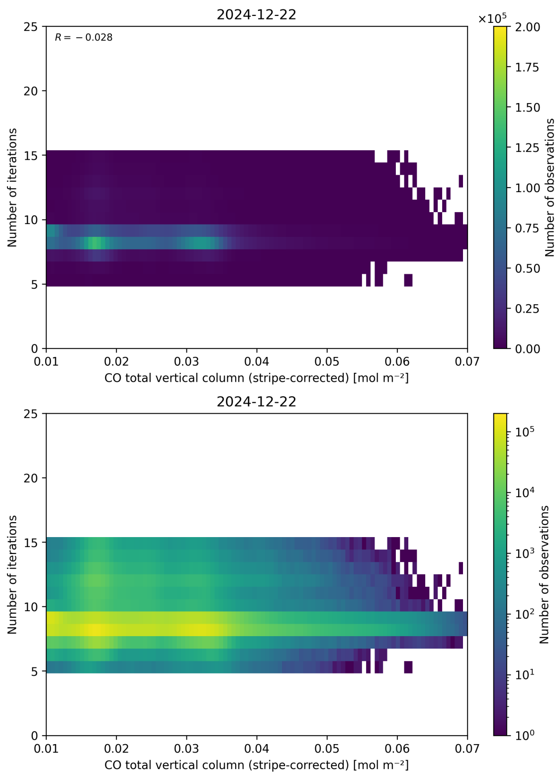
Figure 39: Scatter density plot of “CO total vertical column (stripe-corrected)” against “Number of iterations” for 2024-12-22 to 2024-12-23.
