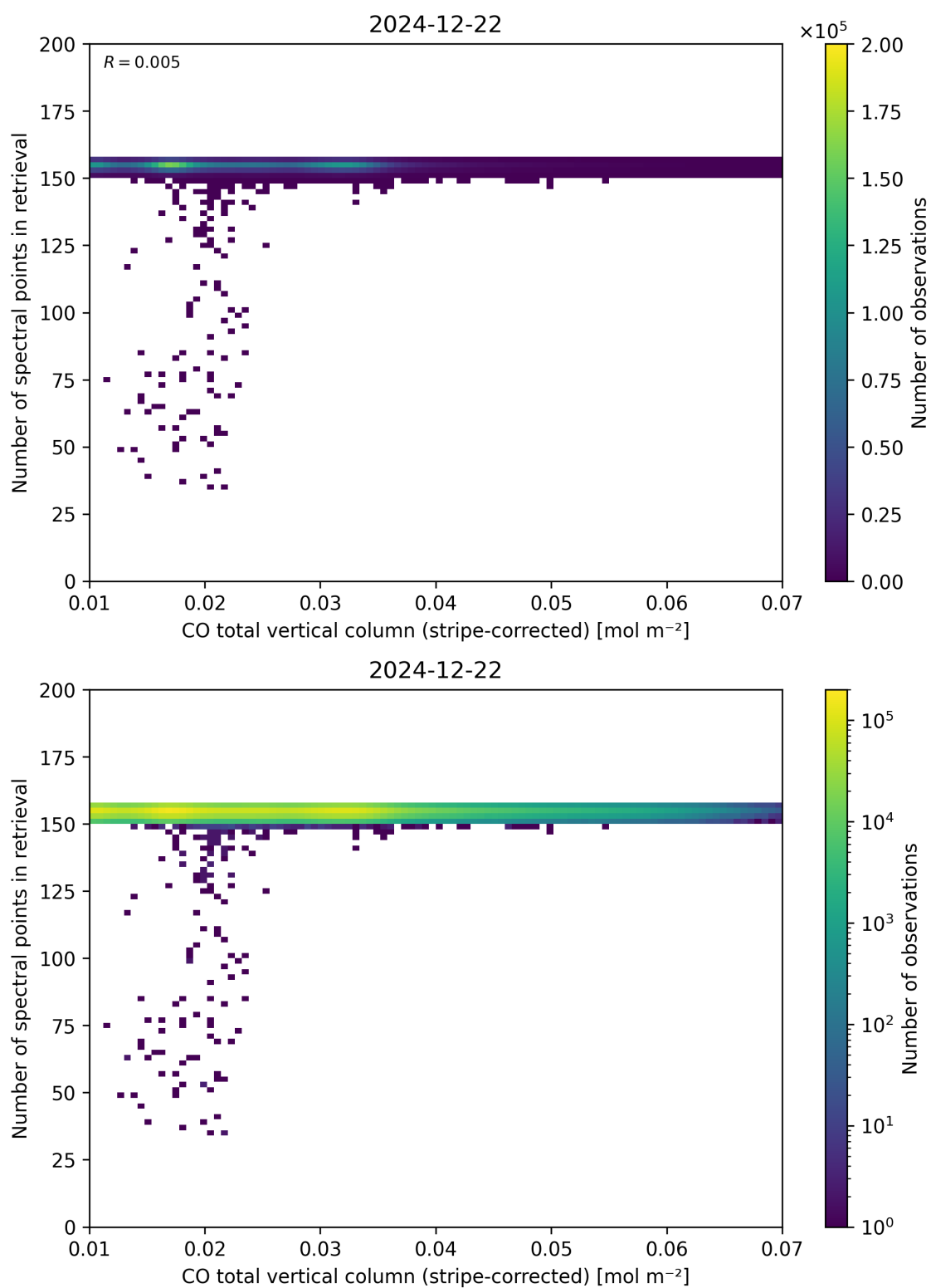
Figure 40: Scatter density plot of “CO total vertical column (stripe-corrected)” against “Number of spectral points in retrieval” for 2024-12-22 to 2024-12-23.
