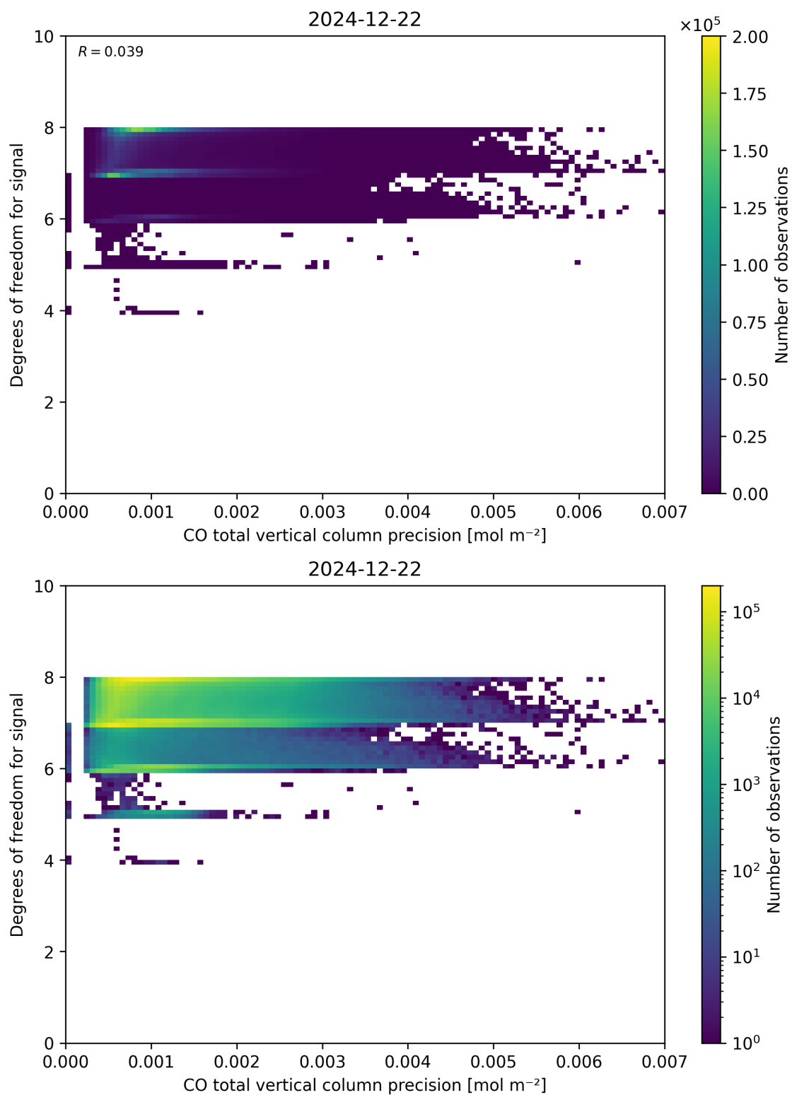
Figure 45: Scatter density plot of “CO total vertical column precision” against “Degrees of freedom for signal” for 2024-12-22 to 2024-12-23.
