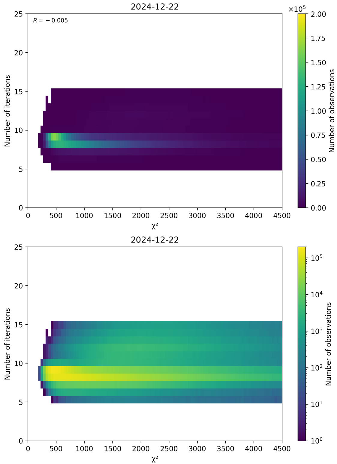
Figure 49: Scatter density plot of “ \chi^2 ” against “Number of iterations” for 2024-12-22 to 2024-12-23.
