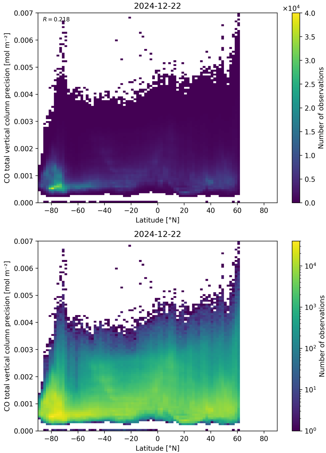
Figure 53: Scatter density plot of “Latitude” against “CO total vertical column precision” for 2024-12-22 to 2024-12-23.
