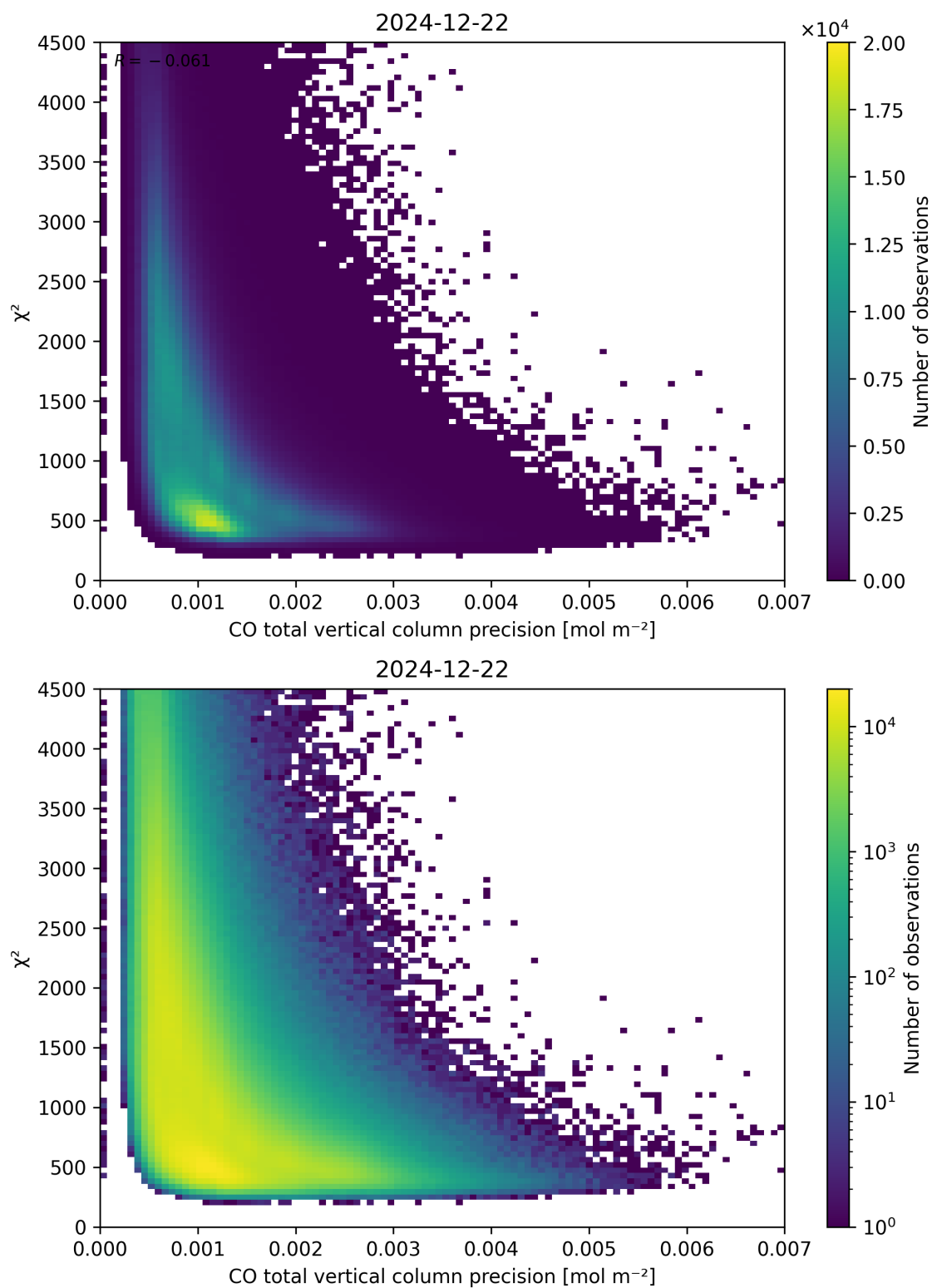
Figure 44: Scatter density plot of “CO total vertical column precision” against “ \chi^2 ” for 2024-12-22 to 2024-12-23.
