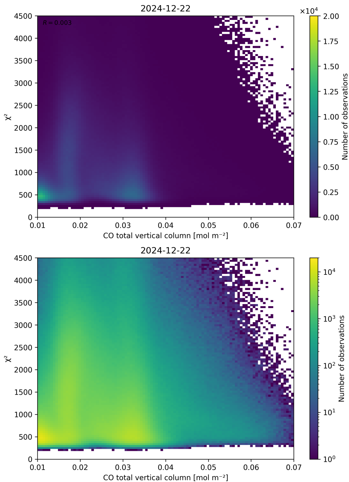
Figure 35: Scatter density plot of “CO total vertical column” against “ \chi^2 ” for 2024-12-22 to 2024-12-23.
