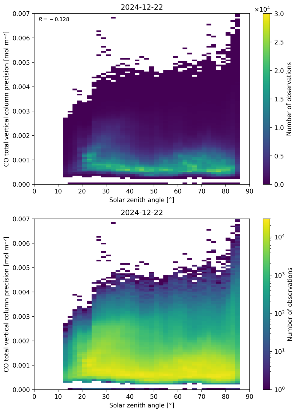
Figure 63: Scatter density plot of “Solar zenith angle” against “CO total vertical column precision” for 2024-12-22 to 2024-12-23.
