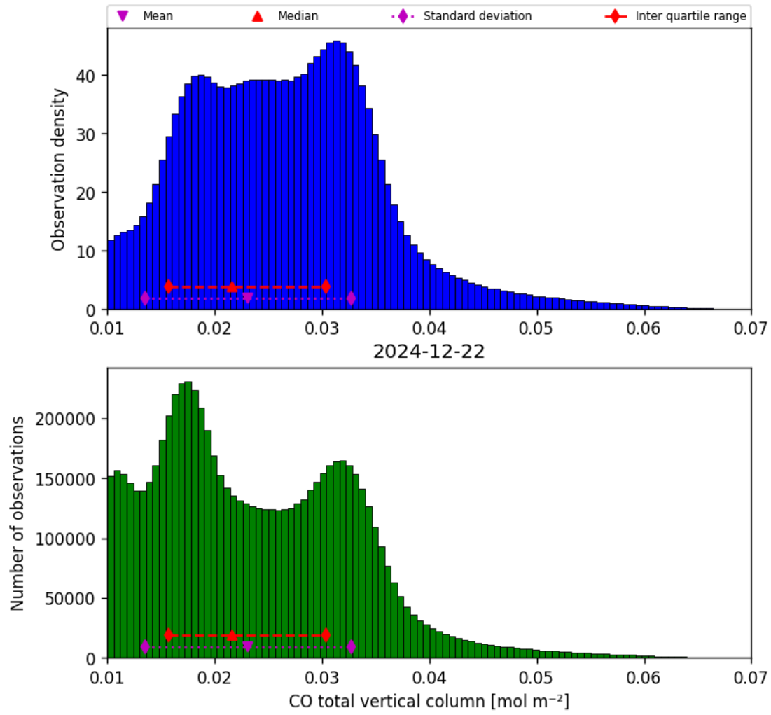
Figure 18: Histogram of “CO total vertical column” for 2024-12-22 to 2024-12-23
