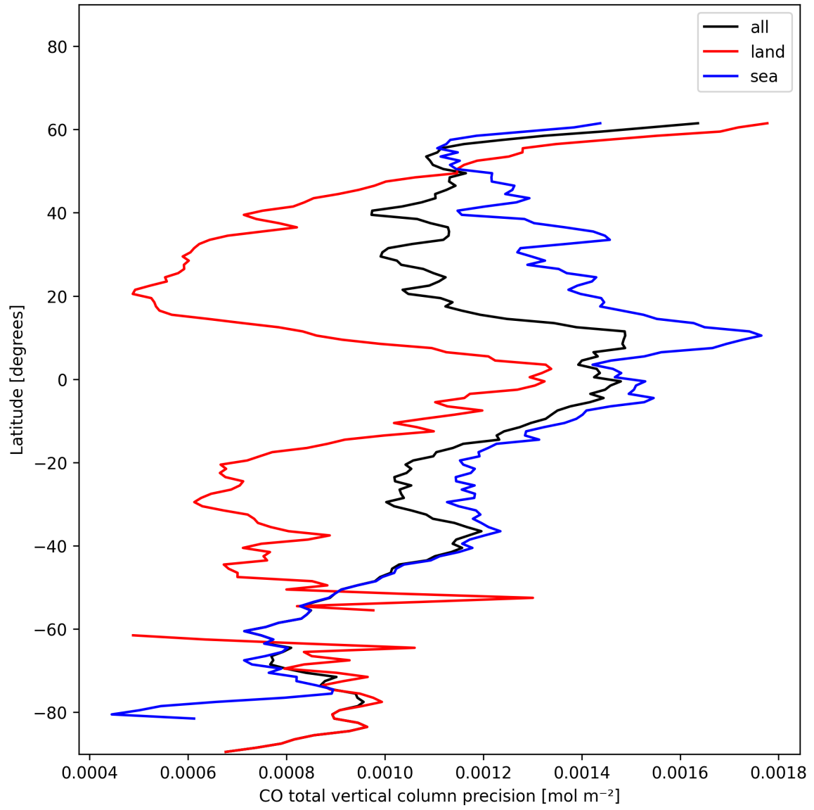
Figure 12: Zonal average of “CO total vertical column precision” for 2024-12-22 to 2024-12-23.
