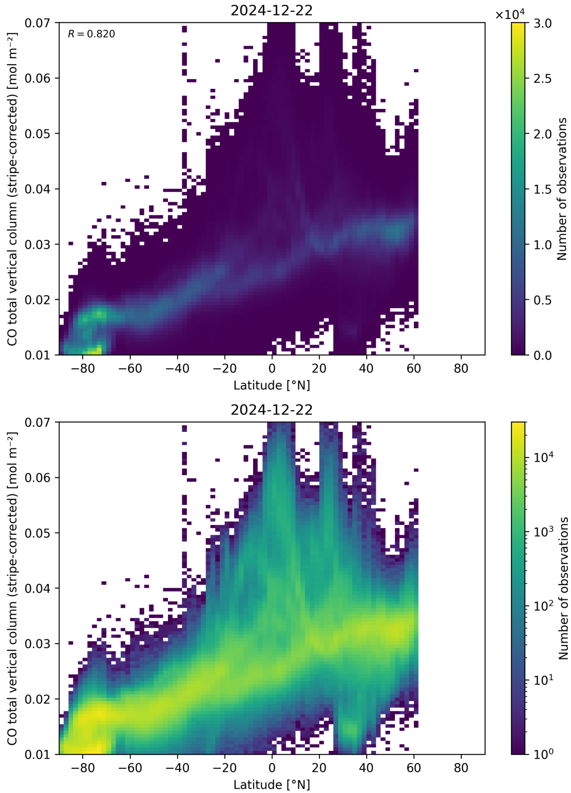
Figure 52: Scatter density plot of “Latitude” against “CO total vertical column (stripe-corrected)” for 2024-12-22 to 2024-12-23.
