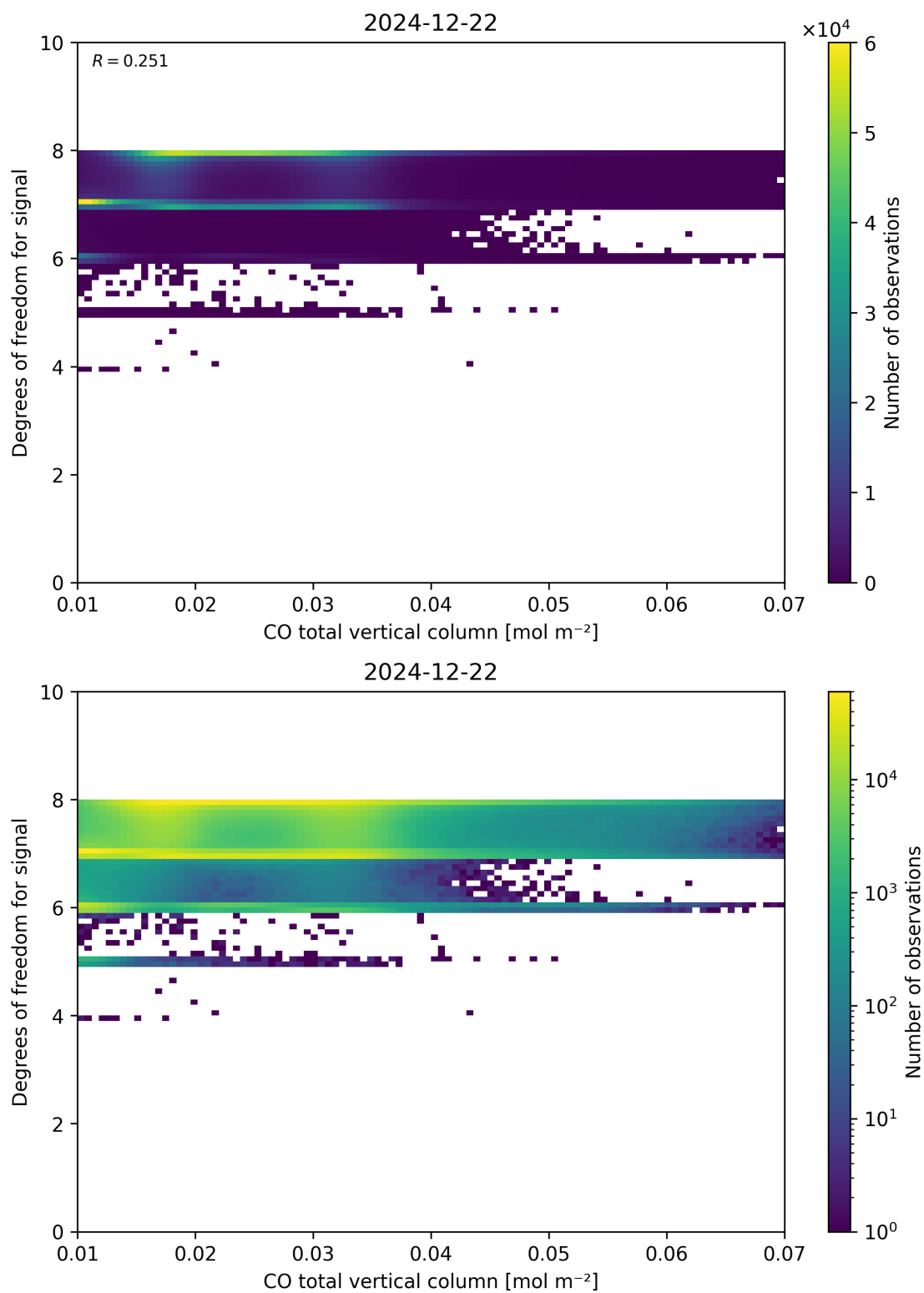
Figure 41: Scatter density plot of “CO total vertical column” against “Degrees of freedom for signal” for 2024-12-22 to 2024-12-23.
