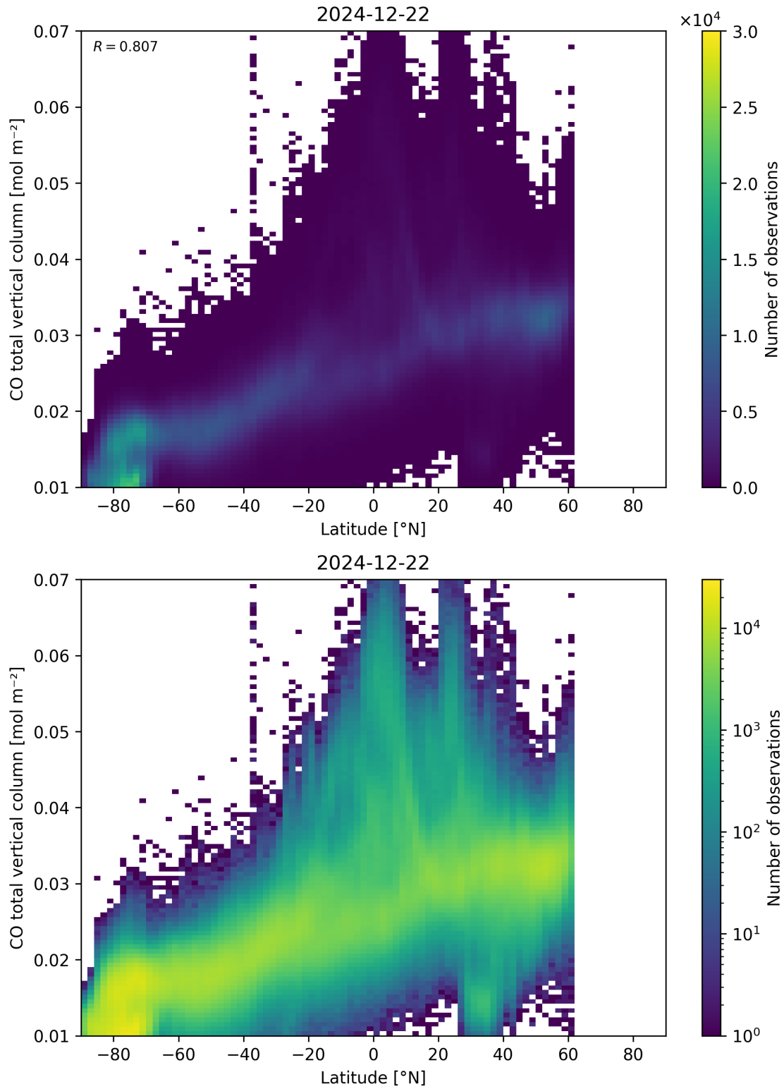
Figure 51: Scatter density plot of “Latitude” against “CO total vertical column” for 2024-12-22 to 2024-12-23.
