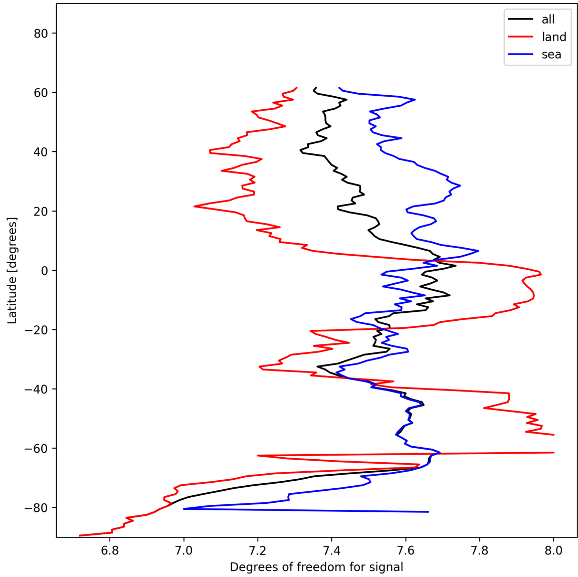
Figure 15: Zonal average of “Degrees of freedom for signal” for 2024-12-22 to 2024-12-23.
