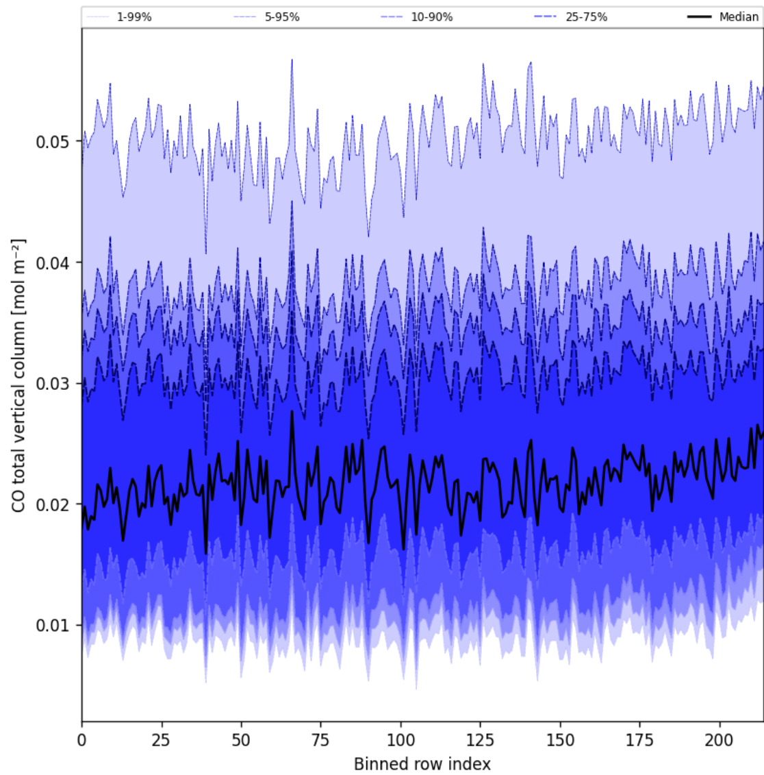
Figure 26: Along track statistics of “CO total vertical column” for 2024-12-22 to 2024-12-23
