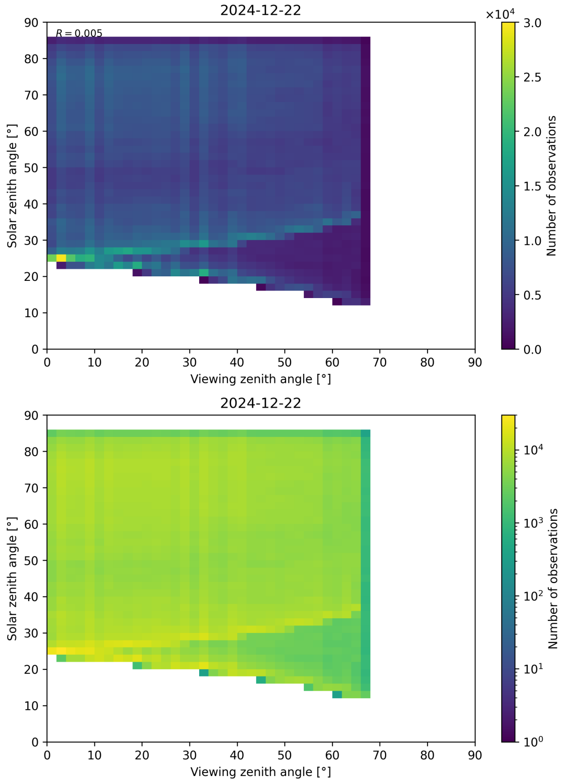
Figure 77: Scatter density plot of “Viewing zenith angle” against “Solar zenith angle” for 2024-12-22 to 2024-12-23.
