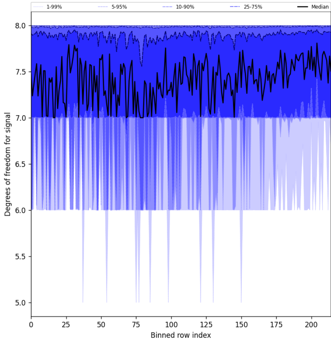
Figure 31: Along track statistics of “Degrees of freedom for signal” for 2024-12-22 to 2024-12-23
