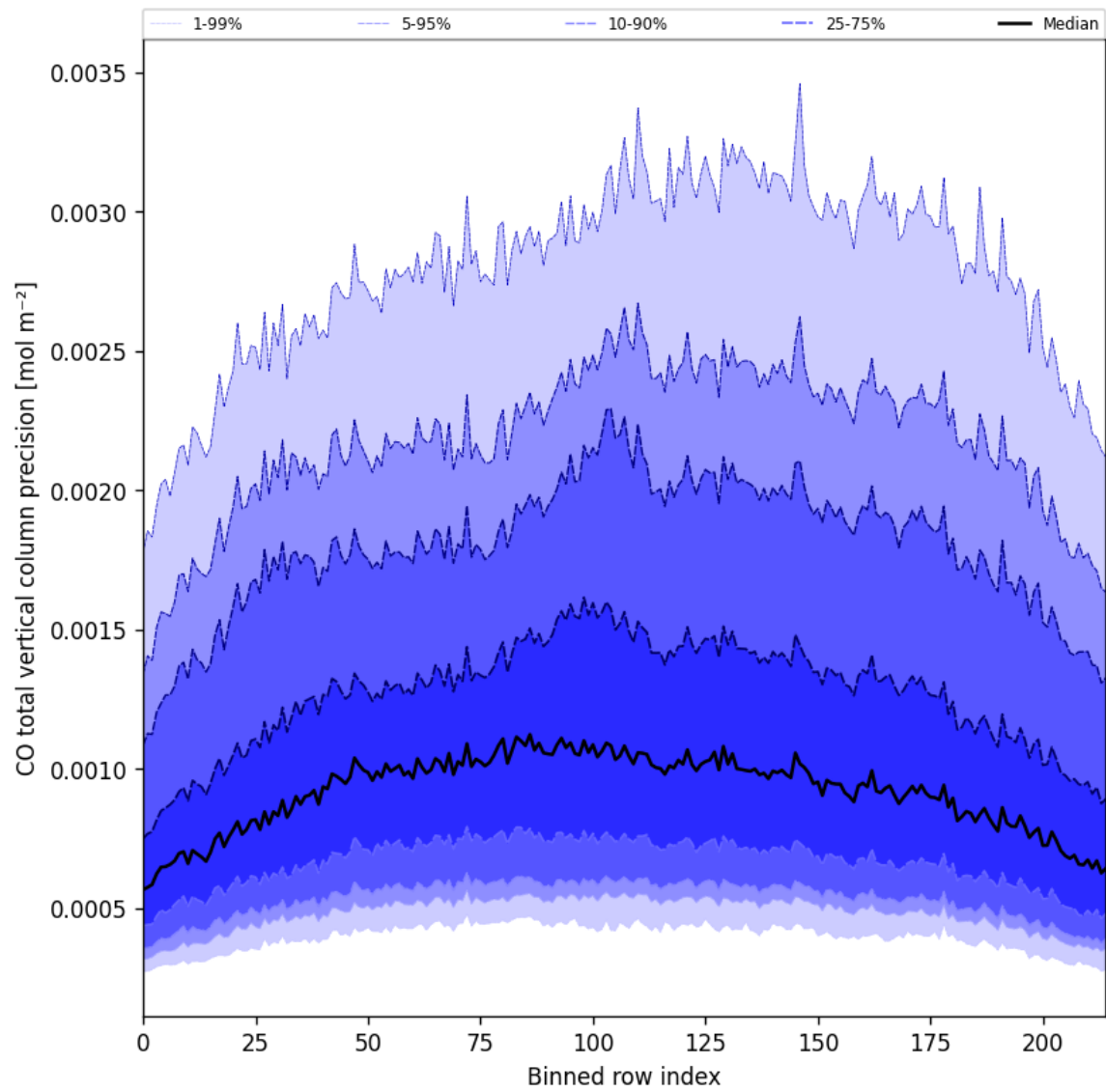
Figure 28: Along track statistics of “CO total vertical column precision” for 2024-12-22 to 2024-12-23
