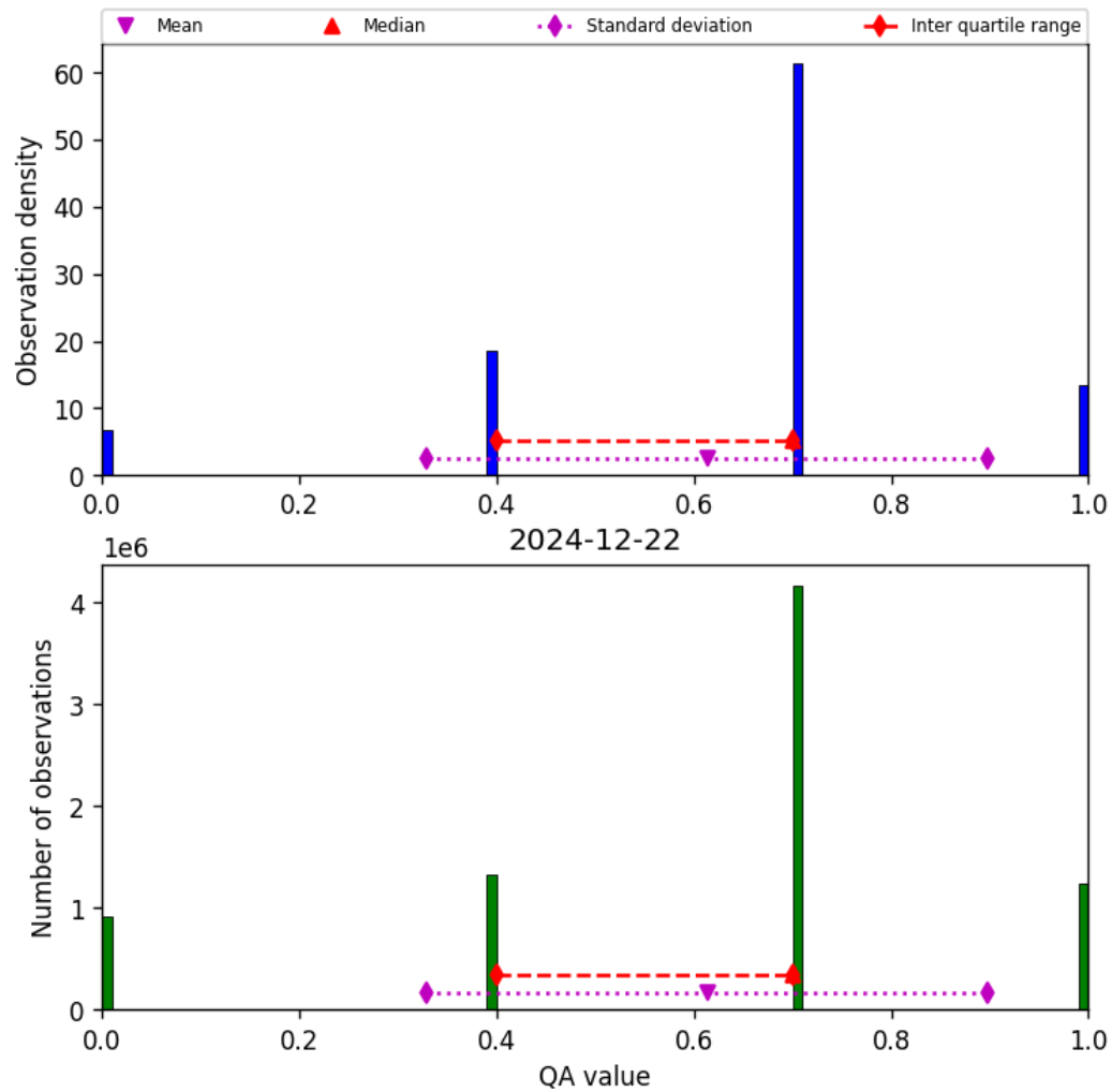
Figure 17: Histogram of “QA value” for 2024-12-22 to 2024-12-23
