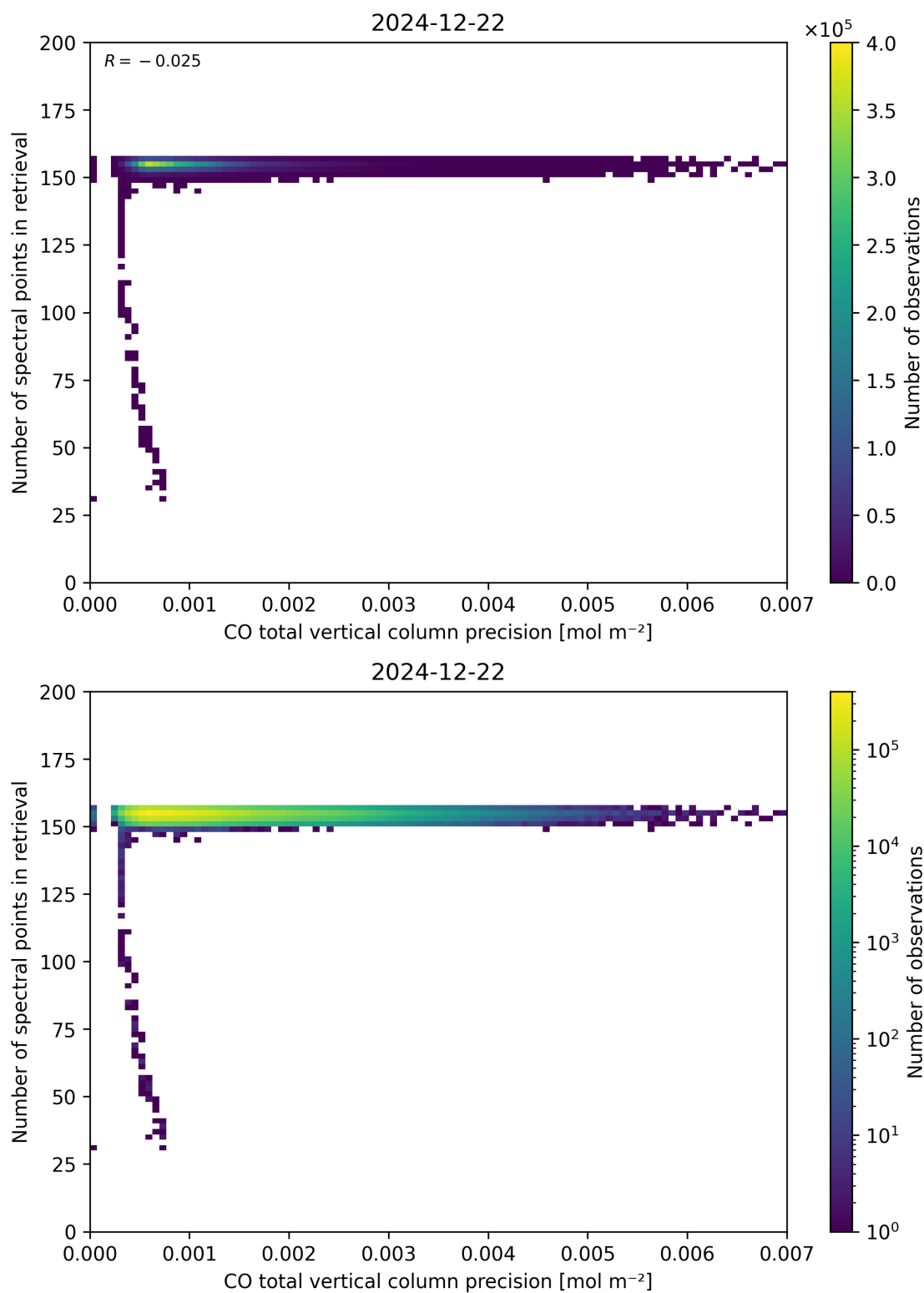
Figure 47: Scatter density plot of “CO total vertical column precision” against “Number of spectral points in retrieval” for 2024-12-22 to 2024-12-23.
