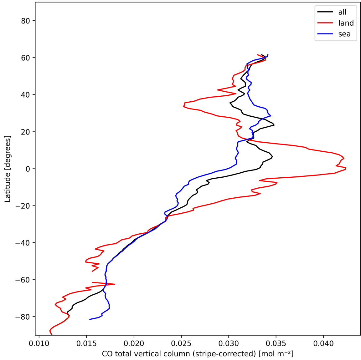
Figure 11: Zonal average of “CO total vertical column (stripe-corrected)” for 2024-12-22 to 2024-12-23.
