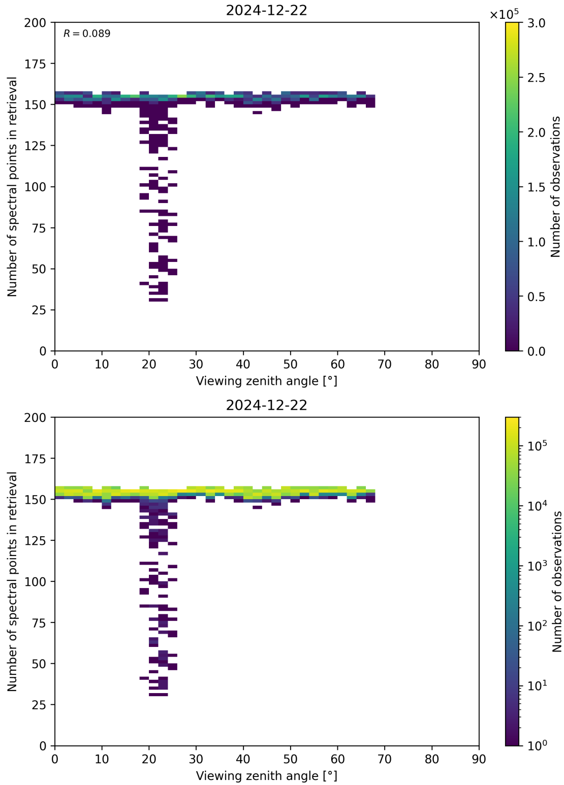
Figure 76: Scatter density plot of “Viewing zenith angle” against “Number of spectral points in retrieval” for 2024-12-22 to 2024-12-23.
