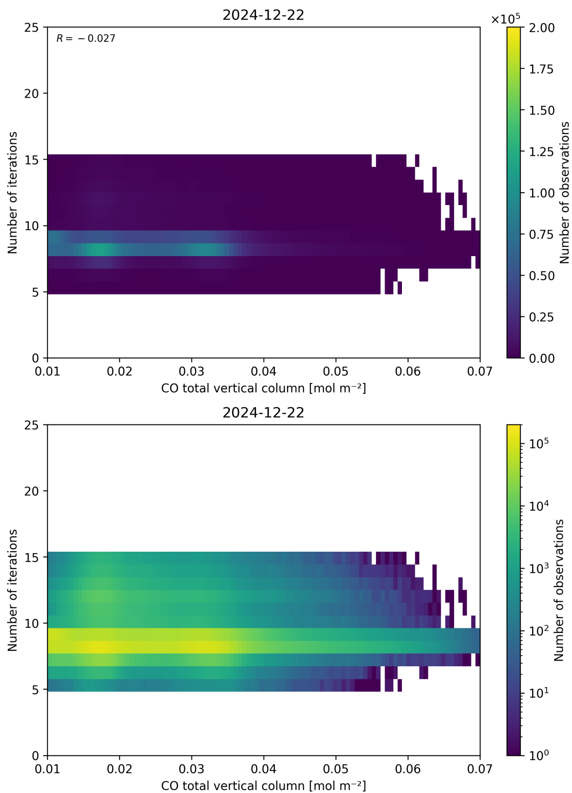
Figure 42: Scatter density plot of “CO total vertical column” against “Number of iterations” for 2024-12-22 to 2024-12-23.
