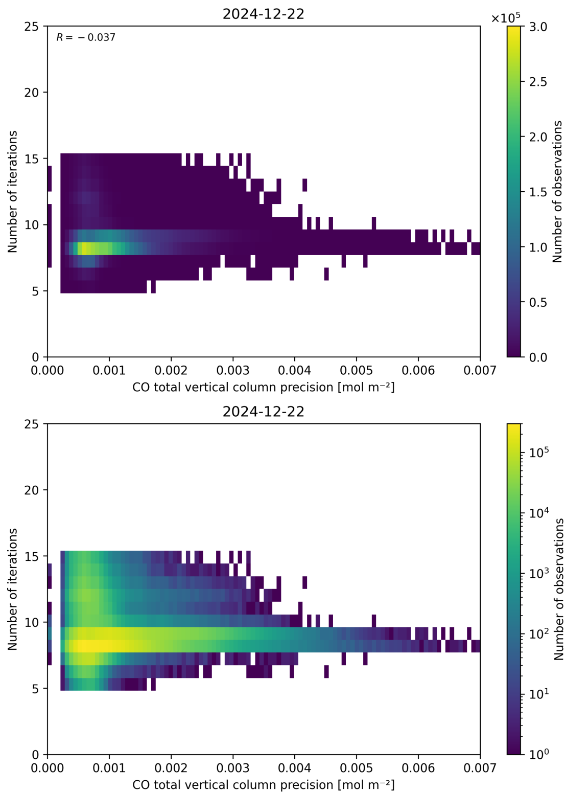
Figure 46: Scatter density plot of “CO total vertical column precision” against “Number of iterations” for 2024-12-22 to 2024-12-23.
