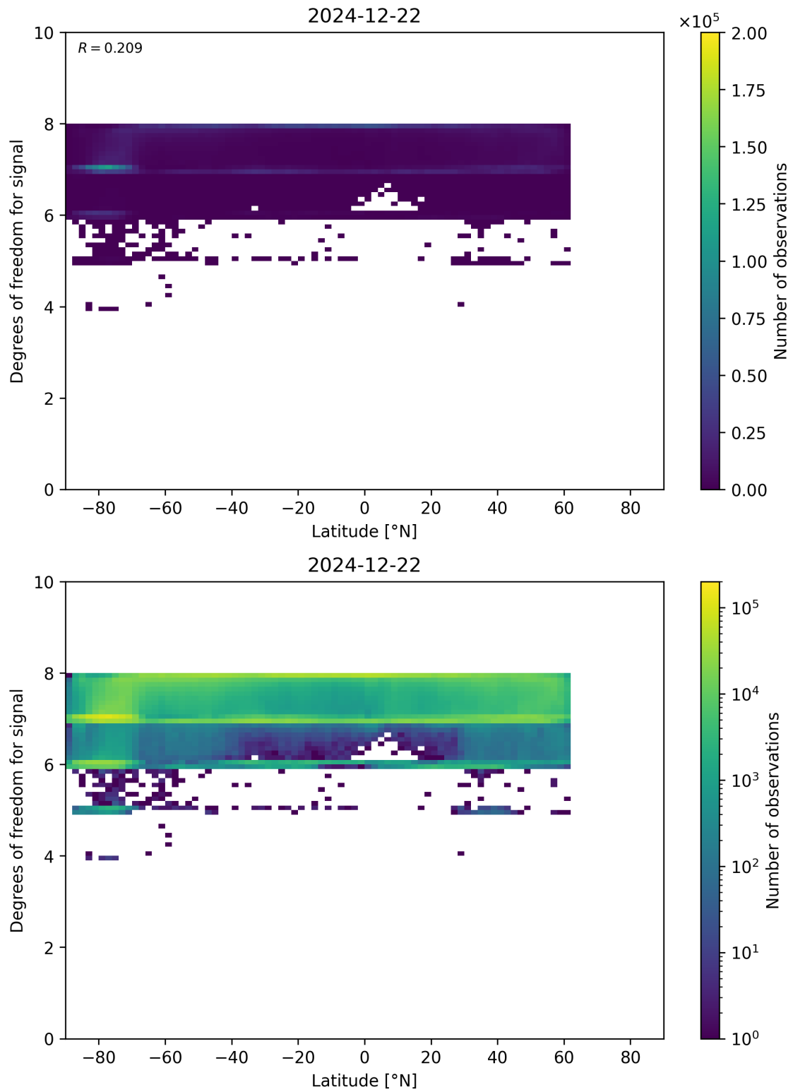
Figure 55: Scatter density plot of “Latitude” against “Degrees of freedom for signal” for 2024-12-22 to 2024-12-23.
