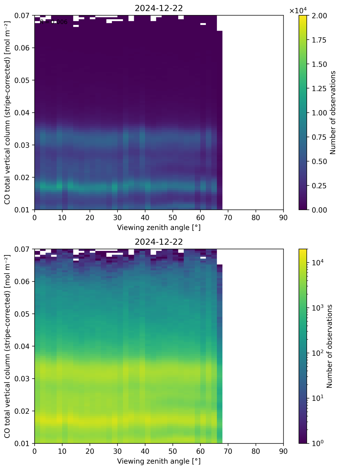
Figure 70: Scatter density plot of “Viewing zenith angle” against “CO total vertical column (stripe-corrected)” for 2024-12-22 to 2024-12-23.
