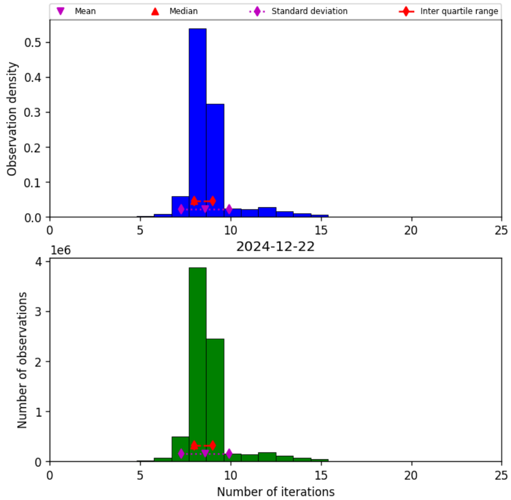
Figure 24: Histogram of “Number of iterations” for 2024-12-22 to 2024-12-23
