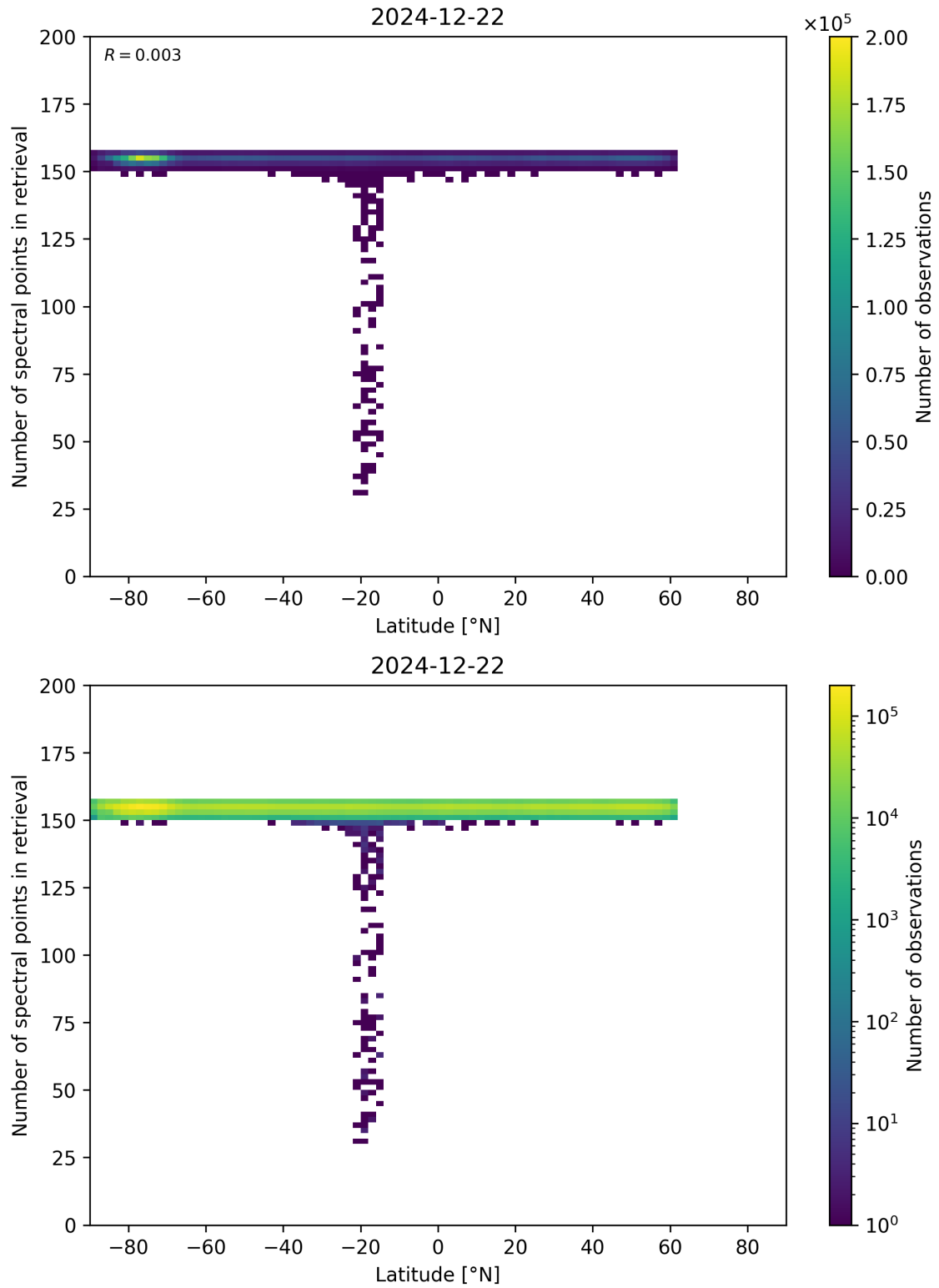
Figure 57: Scatter density plot of “Latitude” against “Number of spectral points in retrieval” for 2024-12-22 to 2024-12-23.
