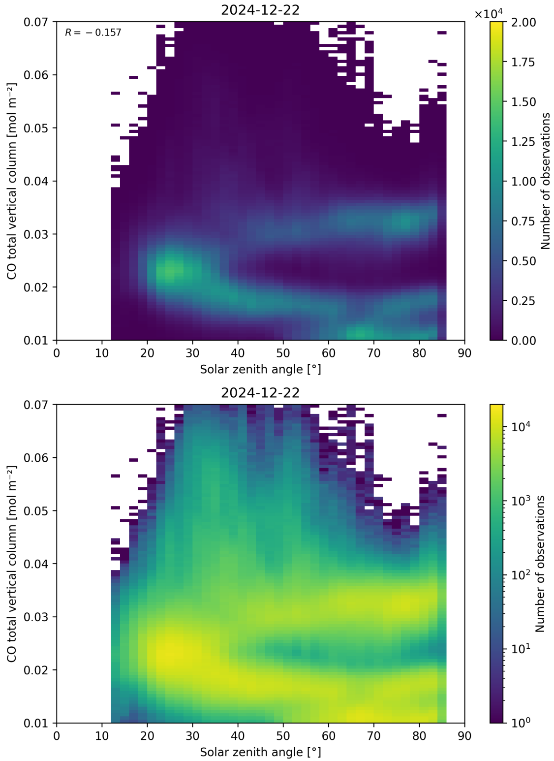
Figure 61: Scatter density plot of “Solar zenith angle” against “CO total vertical column” for 2024-12-22 to 2024-12-23.
