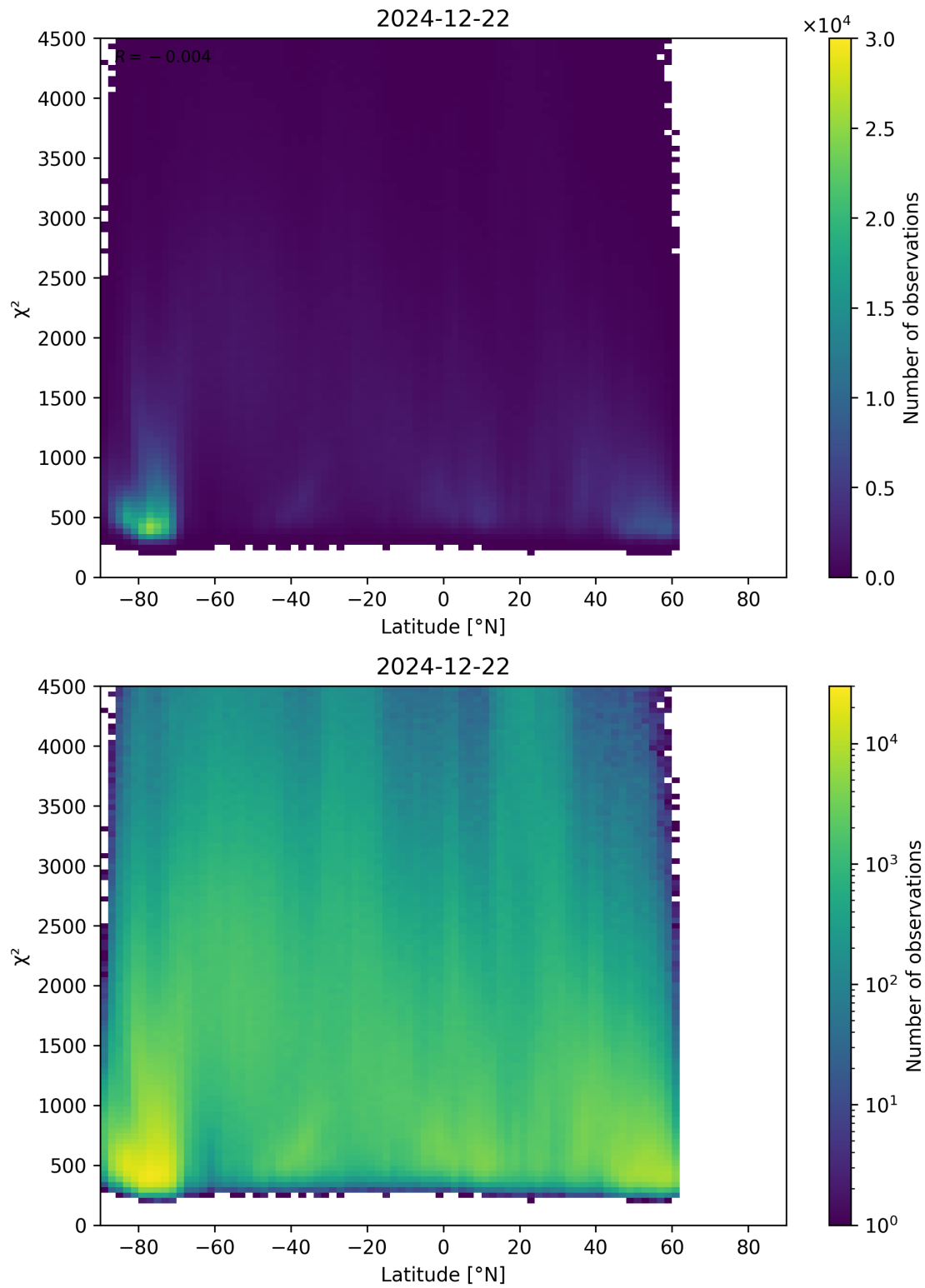
Figure 54: Scatter density plot of “Latitude” against “ \chi^2 ” for 2024-12-22 to 2024-12-23.
