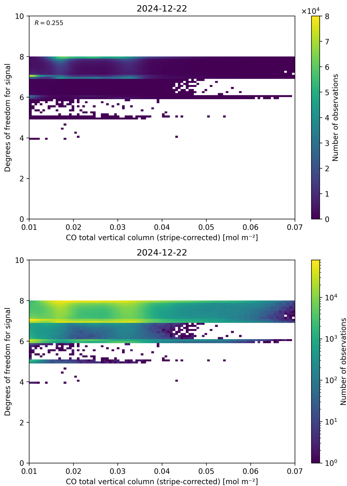
Figure 38: Scatter density plot of “CO total vertical column (stripe-corrected)” against “Degrees of freedom for signal” for 2024-12-22 to 2024-12-23.
