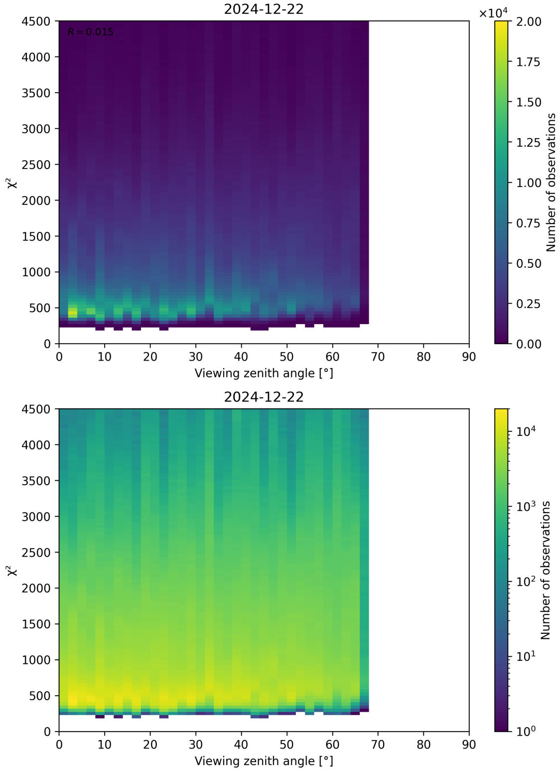
Figure 72: Scatter density plot of “Viewing zenith angle” against “ \chi^2 ” for 2024-12-22 to 2024-12-23.
