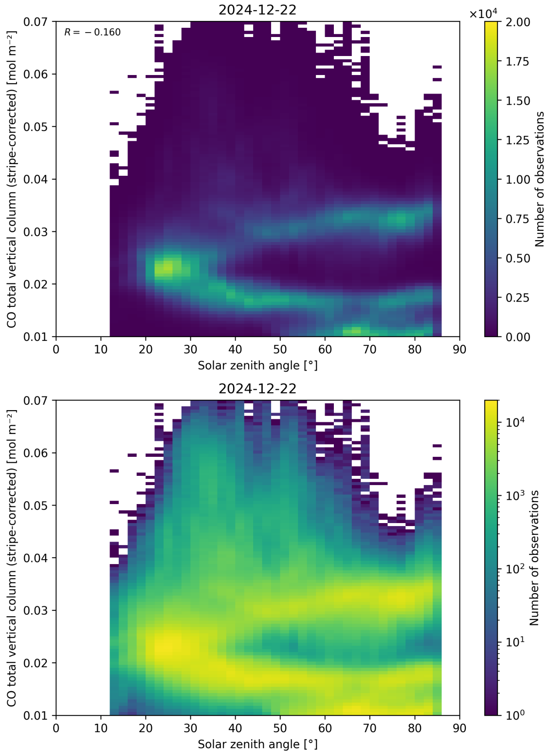
Figure 62: Scatter density plot of “Solar zenith angle” against “CO total vertical column (stripe-corrected)” for 2024-12-22 to 2024-12-23.
