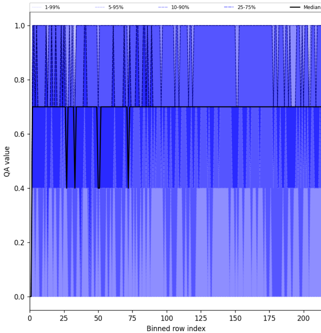
Figure 25: Along track statistics of “QA value” for 2024-12-22 to 2024-12-23
