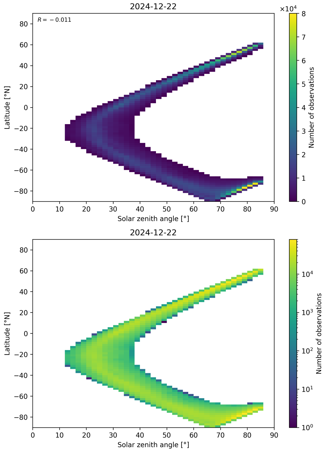
Figure 66: Scatter density plot of “Solar zenith angle” against “Latitude” for 2024-12-22 to 2024-12-23.
