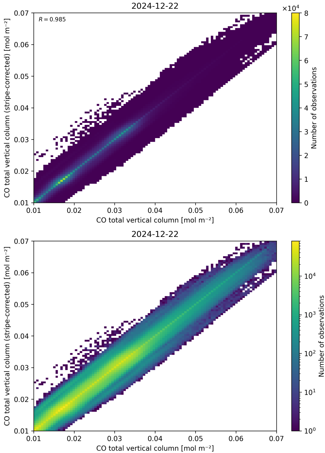
Figure 33: Scatter density plot of “CO total vertical column” against “CO total vertical column (stripe-corrected)” for 2024-12-22 to 2024-12-23.
