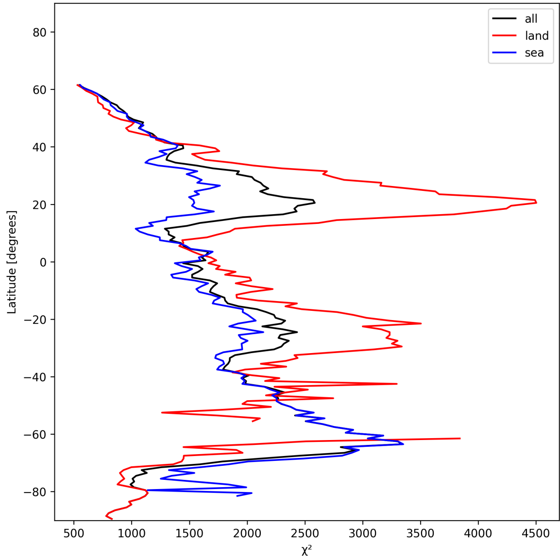
Figure 14: Zonal average of “ \chi^2 ” for 2024-12-22 to 2024-12-23.
