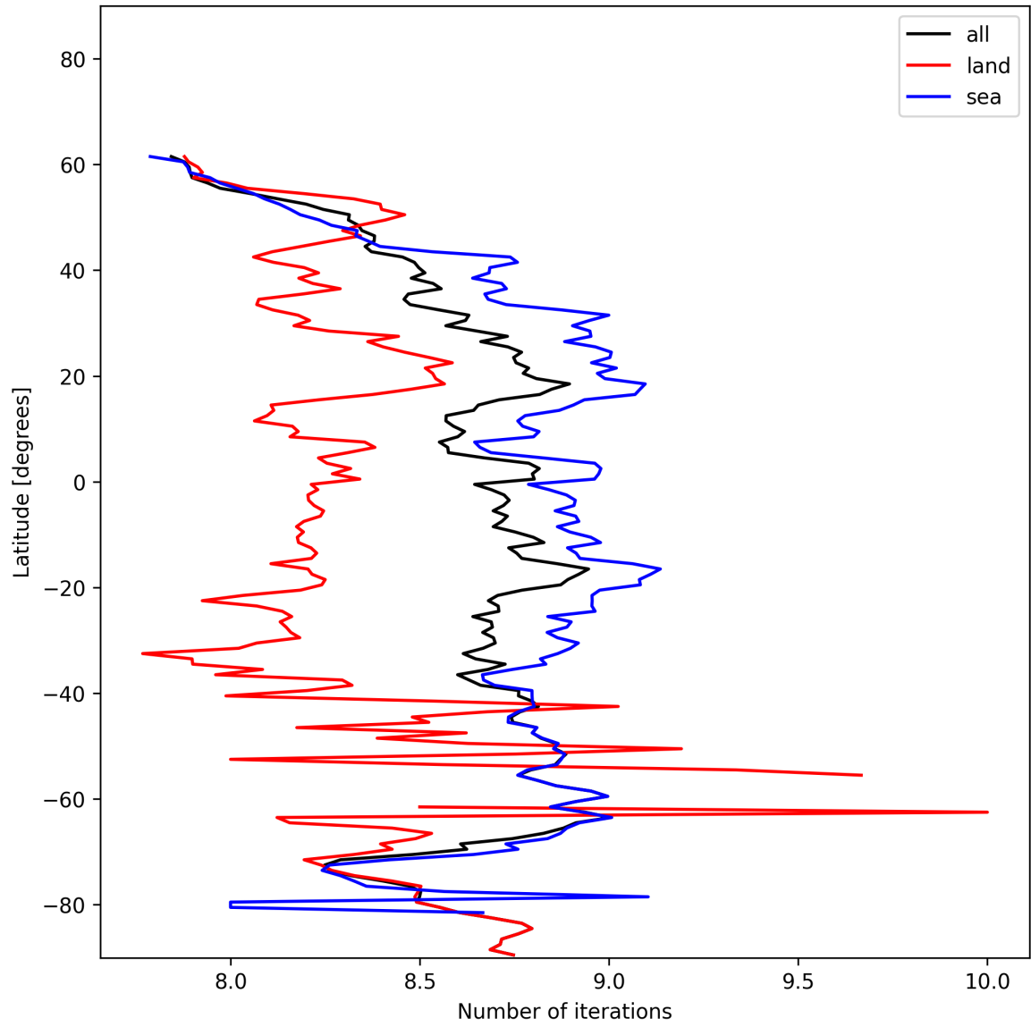
Figure 16: Zonal average of “Number of iterations” for 2024-12-22 to 2024-12-23.
