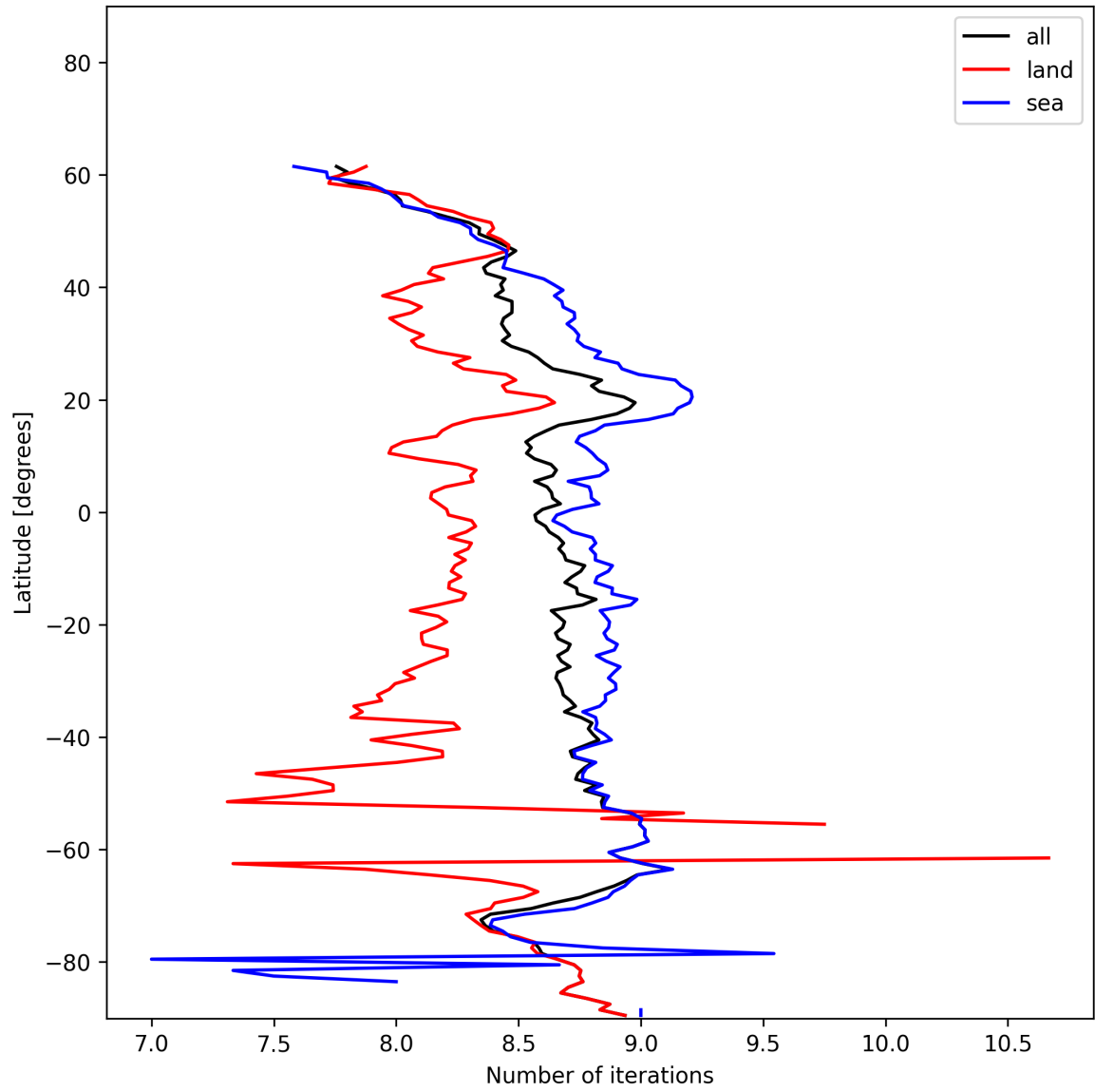
Figure 16: Zonal average of “Number of iterations” for 2024-12-22 to 2024-12-24.
