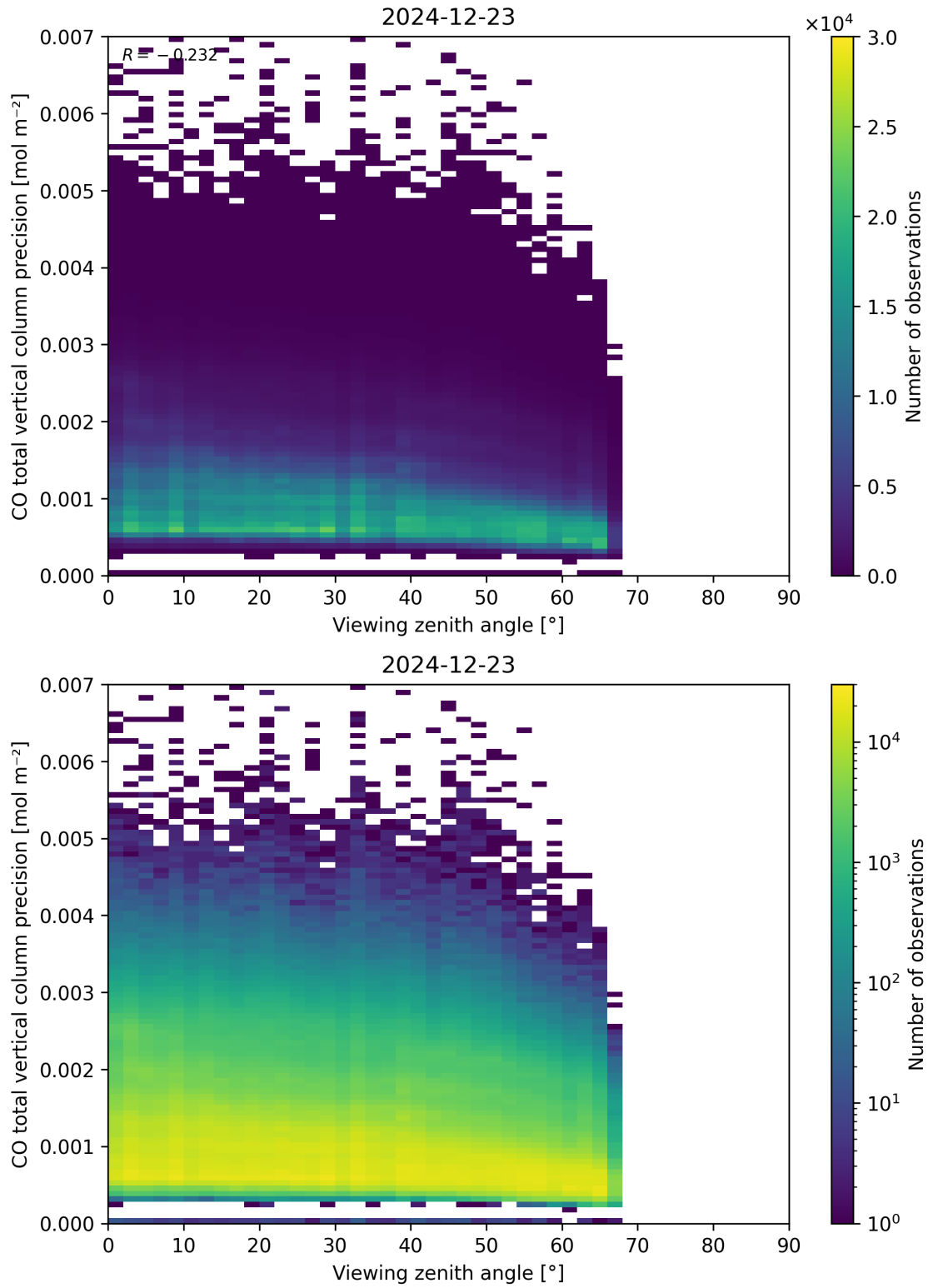
Figure 71: Scatter density plot of “Viewing zenith angle” against “CO total vertical column precision” for 2024-12-22 to 2024-12-24.
