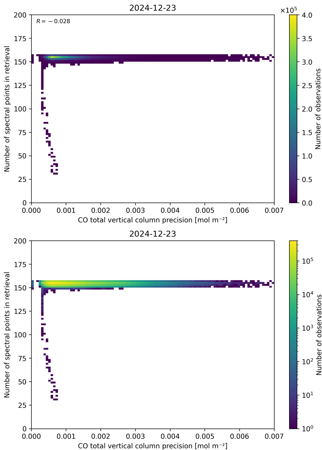
Figure 47: Scatter density plot of “CO total vertical column precision” against “Number of spectral points in retrieval” for 2024-12-22 to 2024-12-24.
