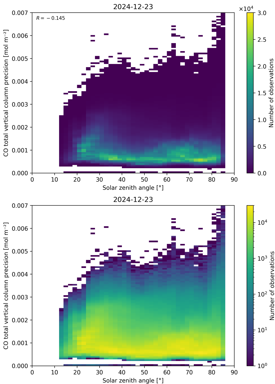
Figure 63: Scatter density plot of “Solar zenith angle” against “CO total vertical column precision” for 2024-12-22 to 2024-12-24.
