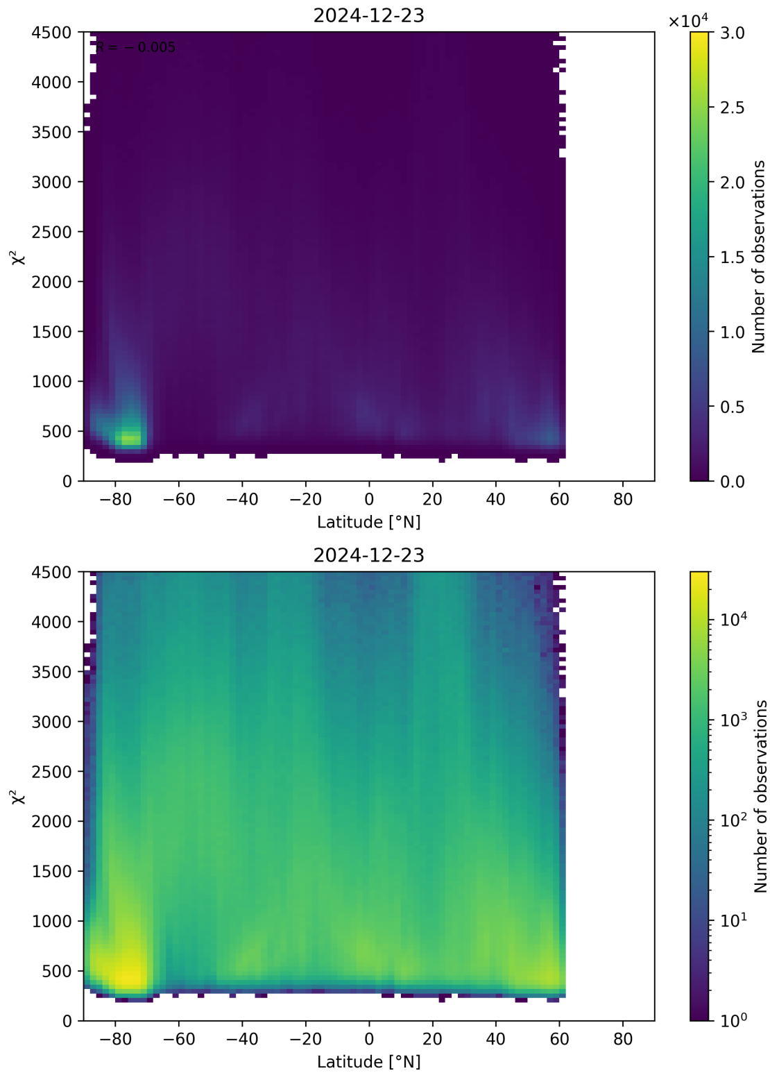
Figure 54: Scatter density plot of “Latitude” against “ \chi^2 ” for 2024-12-22 to 2024-12-24.
