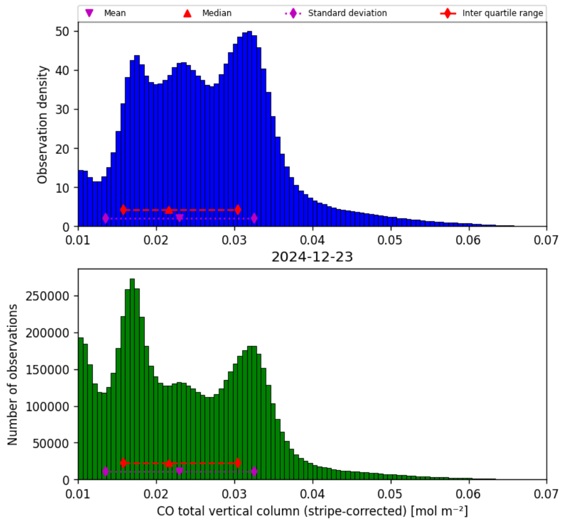
Figure 19: Histogram of “CO total vertical column (stripe-corrected)” for 2024-12-22 to 2024-12-24
