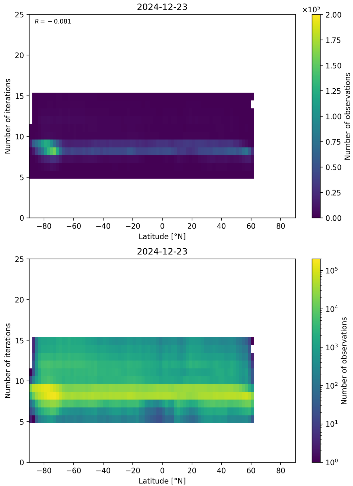
Figure 56: Scatter density plot of “Latitude” against “Number of iterations” for 2024-12-22 to 2024-12-24.
