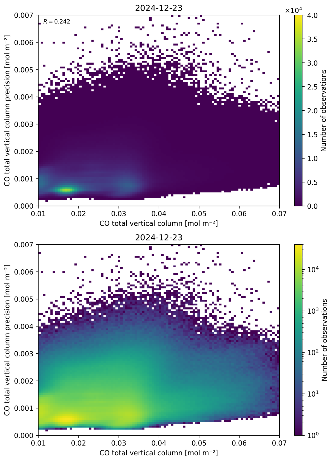
Figure 34: Scatter density plot of “CO total vertical column” against “CO total vertical column precision” for 2024-12-22 to 2024-12-24.
