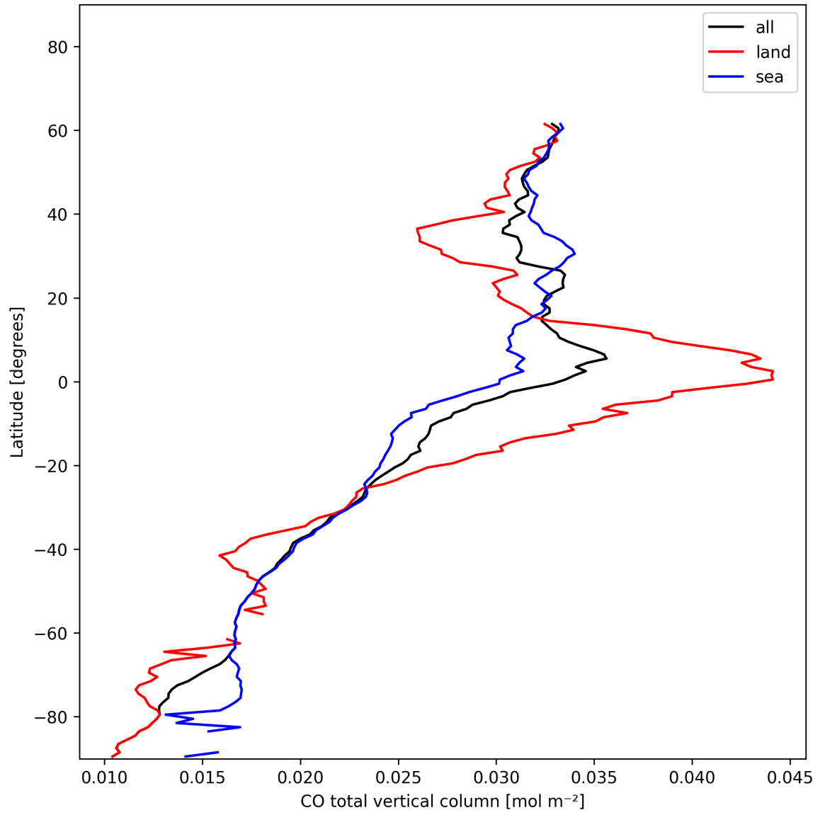
Figure 10: Zonal average of “CO total vertical column” for 2024-12-22 to 2024-12-24.
