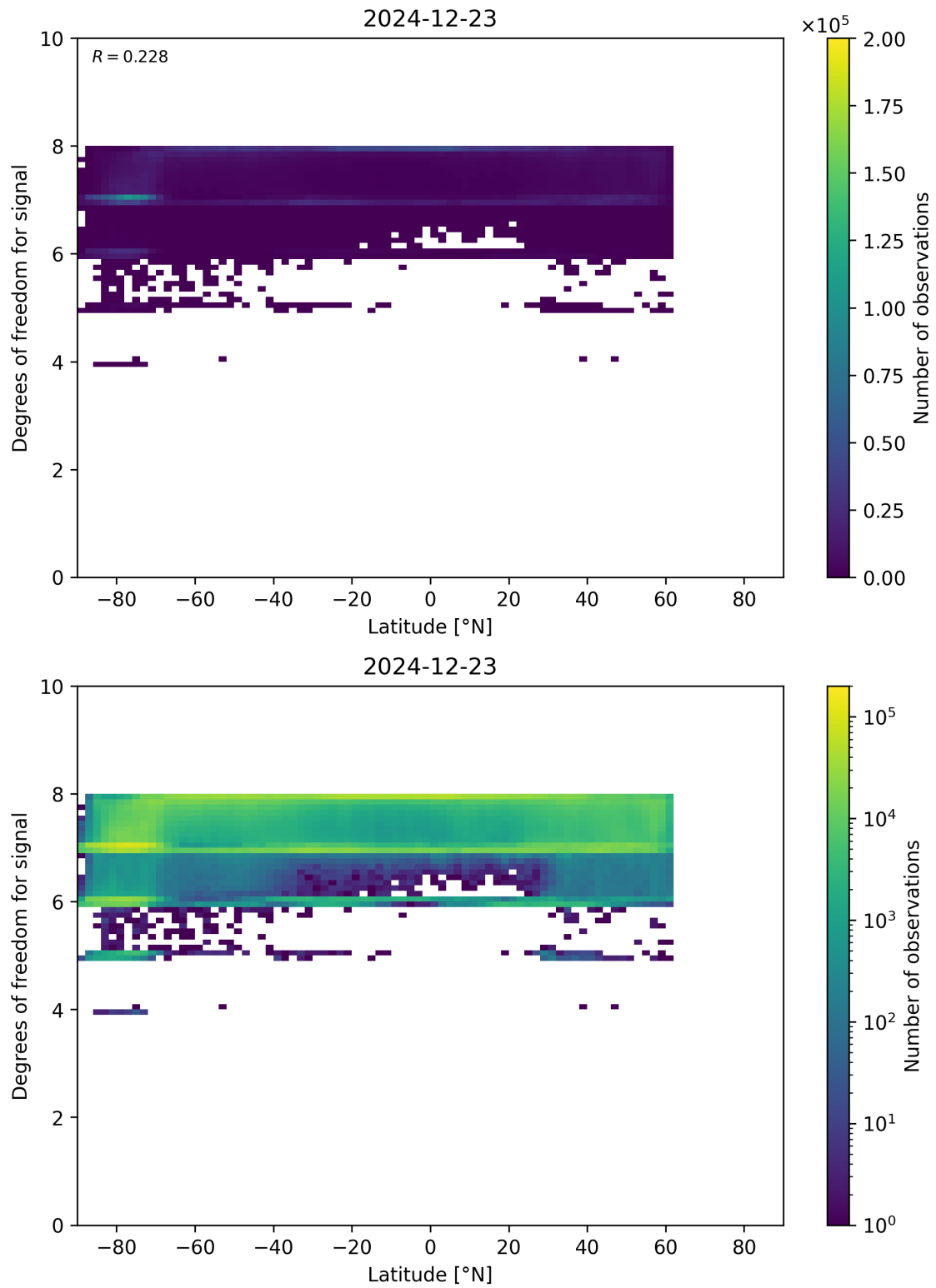
Figure 55: Scatter density plot of “Latitude” against “Degrees of freedom for signal” for 2024-12-22 to 2024-12-24.
