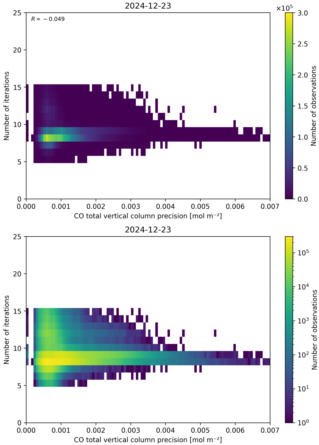
Figure 46: Scatter density plot of “CO total vertical column precision” against “Number of iterations” for 2024-12-22 to 2024-12-24.
