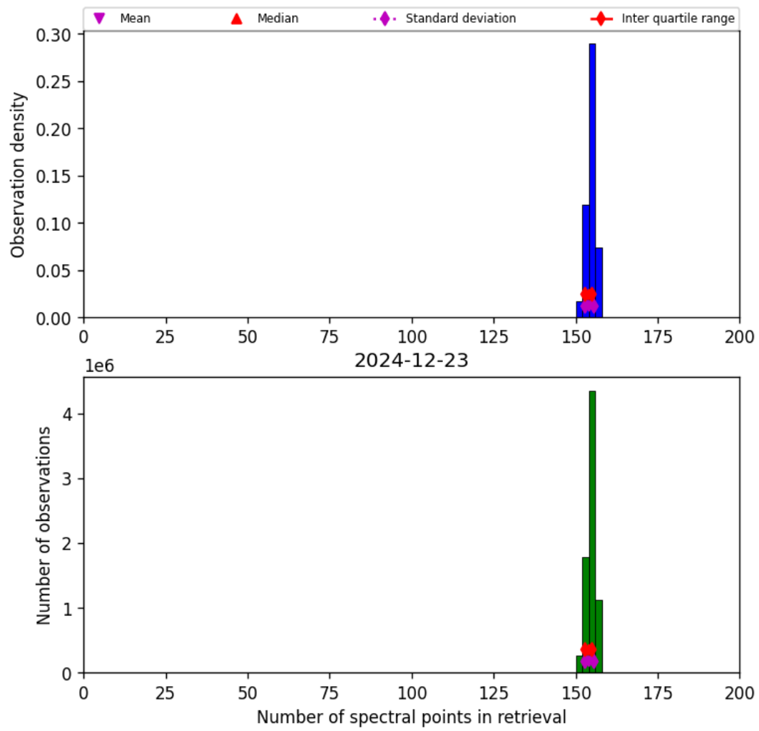
Figure 21: Histogram of “Number of spectral points in retrieval” for 2024-12-22 to 2024-12-24
