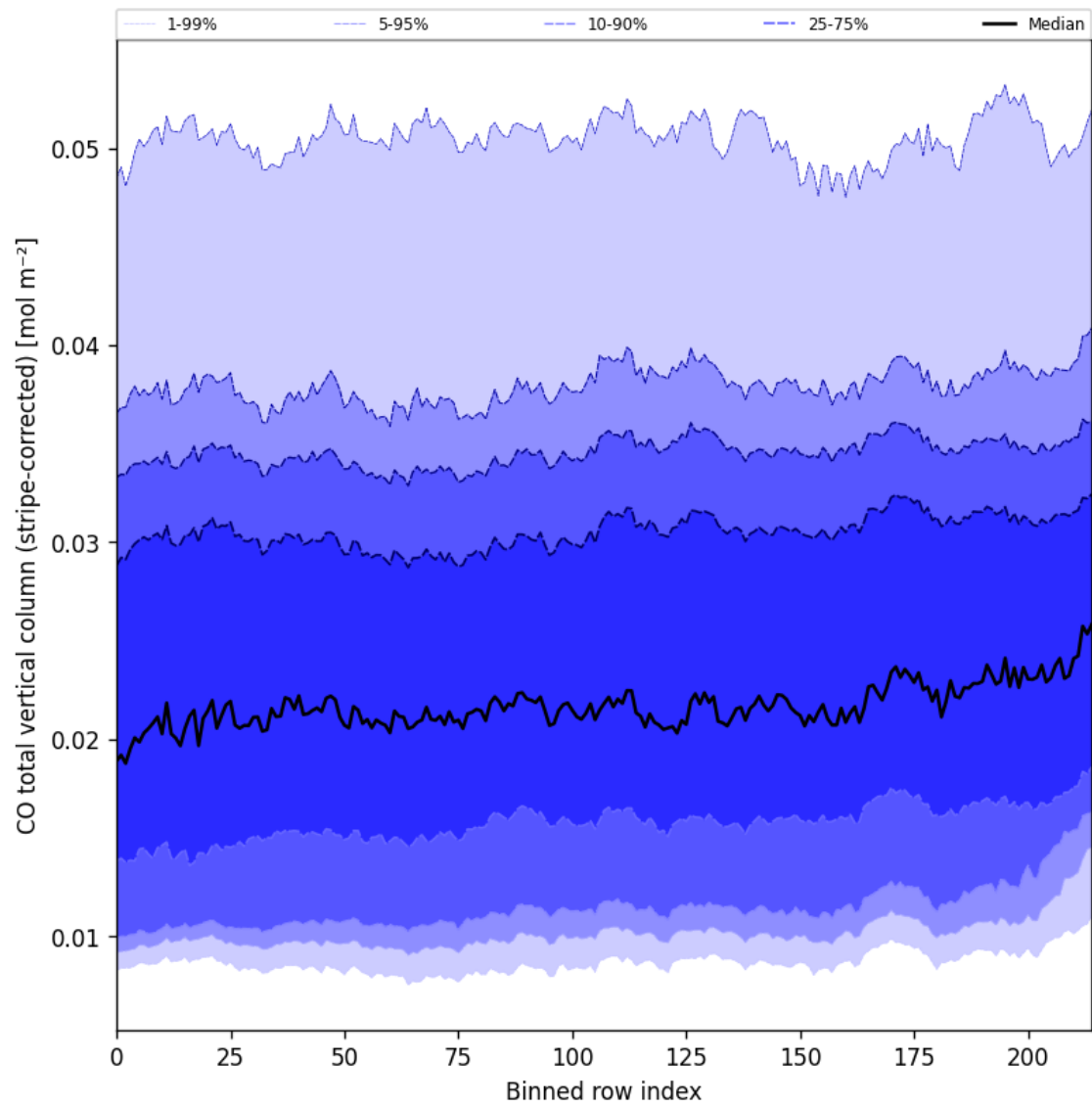
Figure 27: Along track statistics of “CO total vertical column (stripe-corrected)” for 2024-12-22 to 2024-12-24
