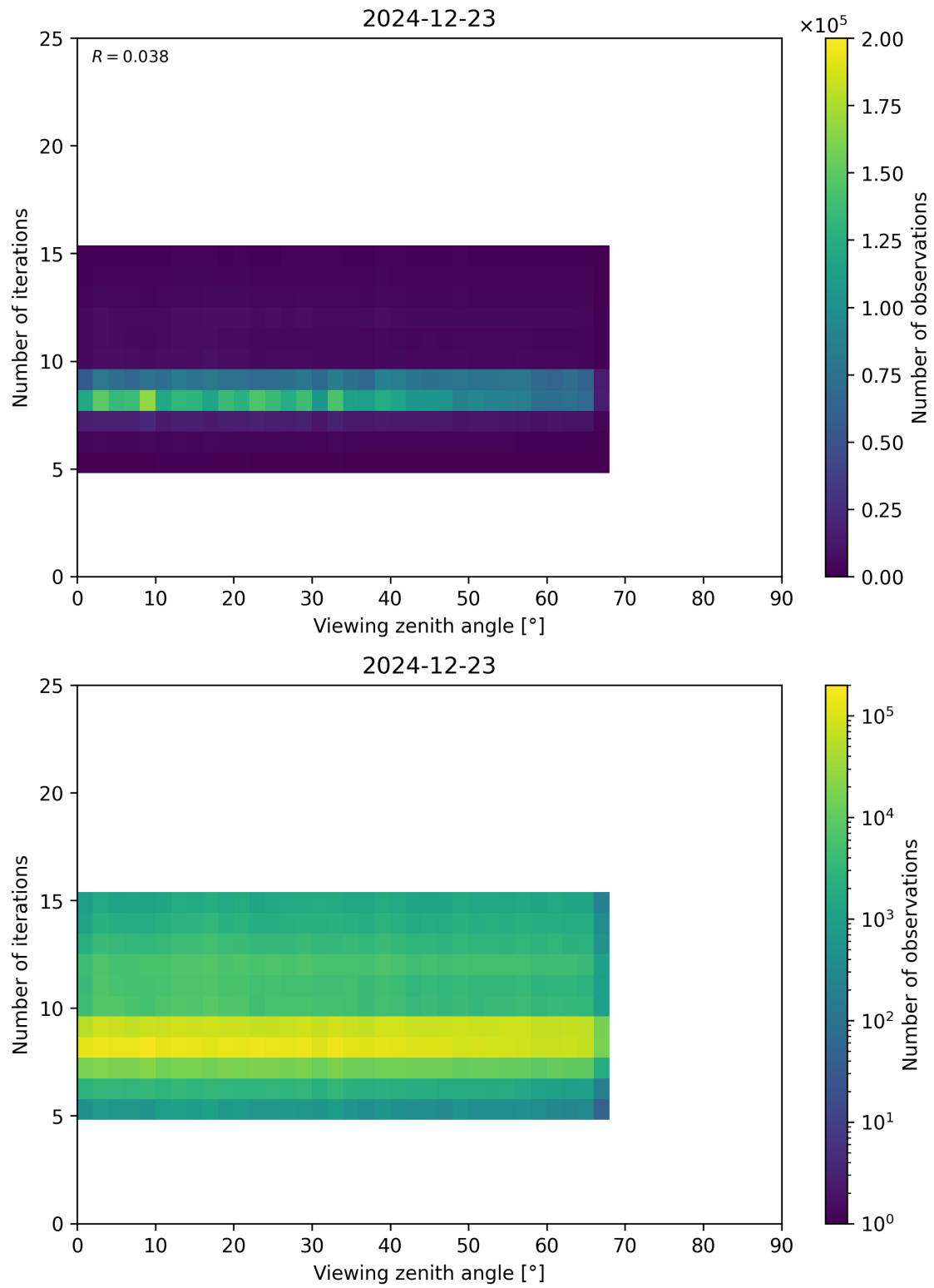
Figure 75: Scatter density plot of “Viewing zenith angle” against “Number of iterations” for 2024-12-22 to 2024-12-24.
