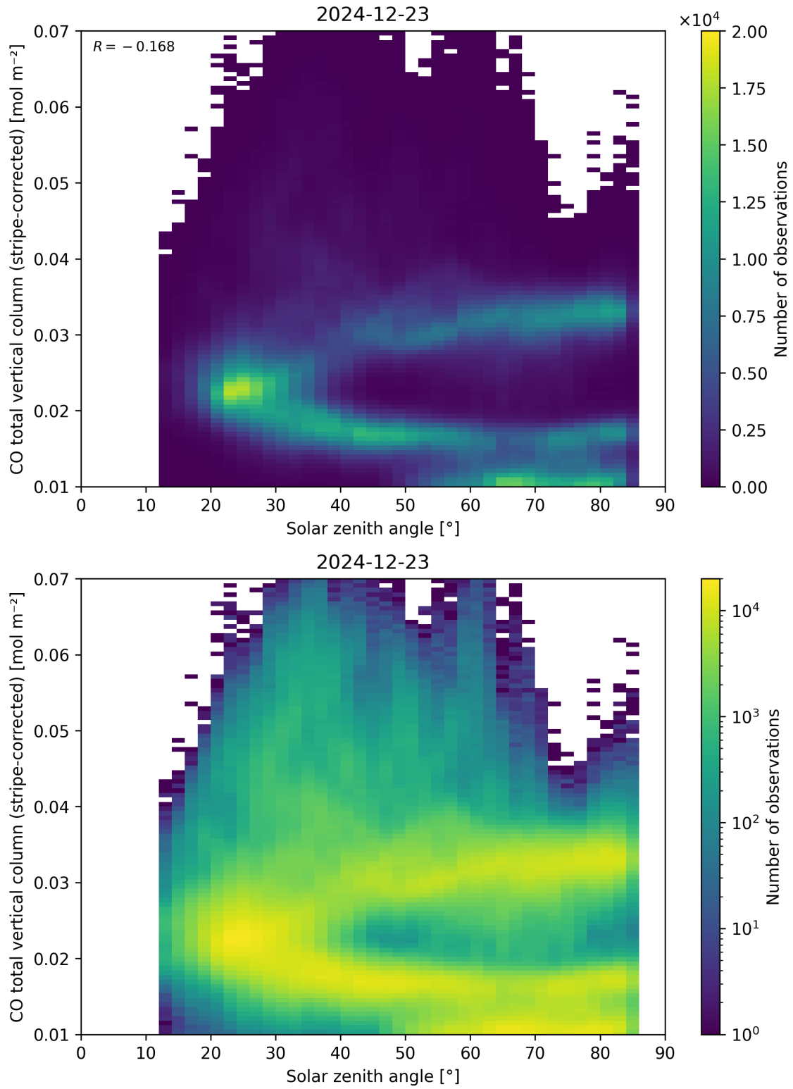
Figure 62: Scatter density plot of “Solar zenith angle” against “CO total vertical column (stripe-corrected)” for 2024-12-22 to 2024-12-24.
