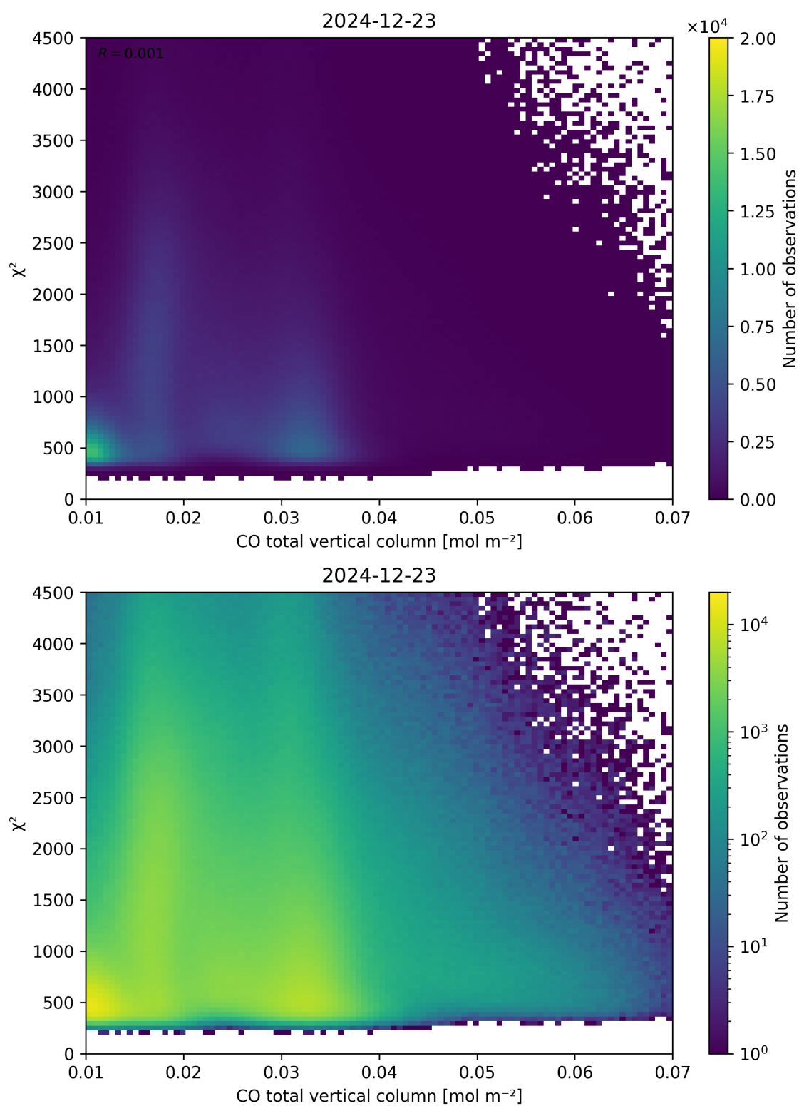
Figure 35: Scatter density plot of “CO total vertical column” against “ \chi^2 ” for 2024-12-22 to 2024-12-24.
