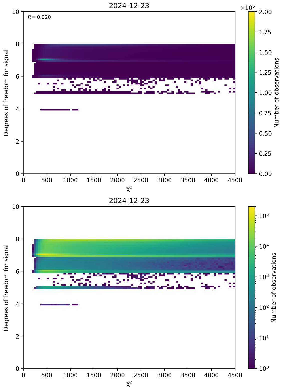
Figure 48: Scatter density plot of “ \chi^2 ” against “Degrees of freedom for signal” for 2024-12-22 to 2024-12-24.
