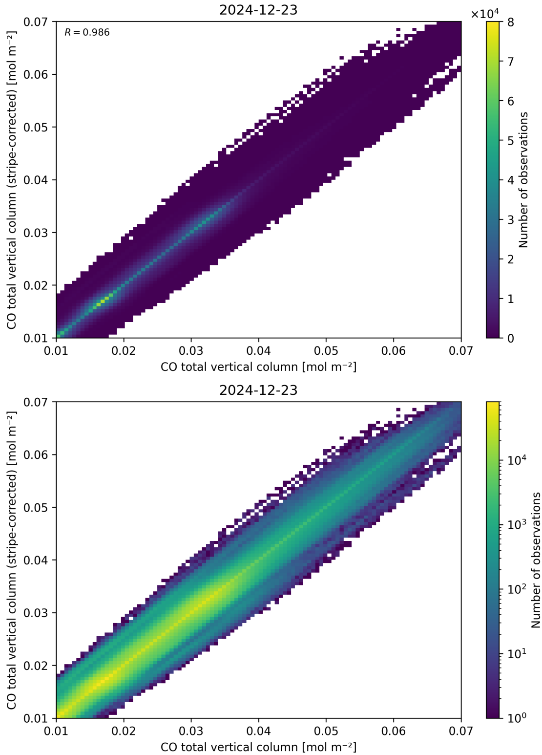
Figure 33: Scatter density plot of “CO total vertical column” against “CO total vertical column (stripe-corrected)” for 2024-12-22 to 2024-12-24.
