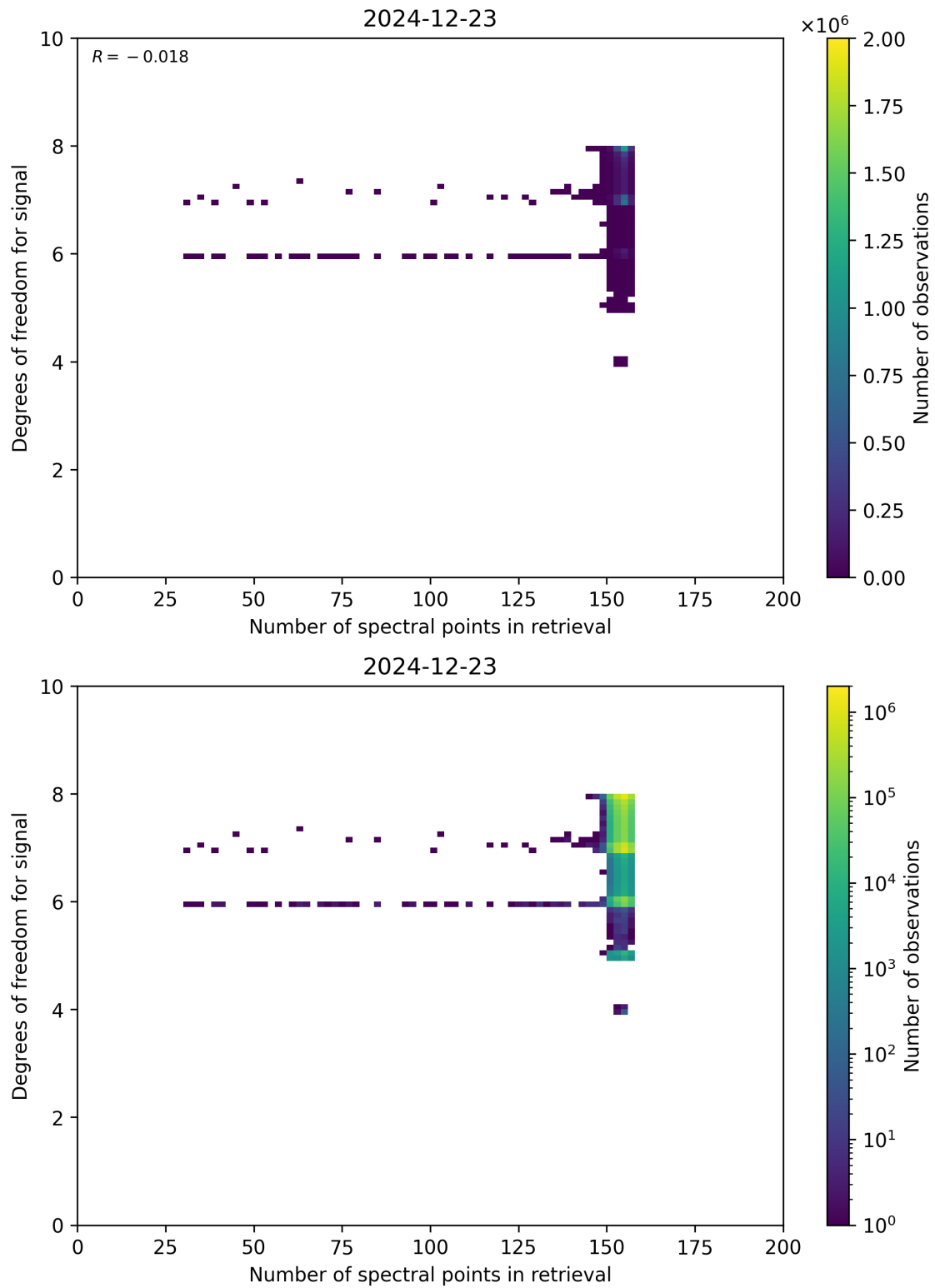
Figure 59: Scatter density plot of “Number of spectral points in retrieval” against “Degrees of freedom for signal” for 2024-12-22 to 2024-12-24.
