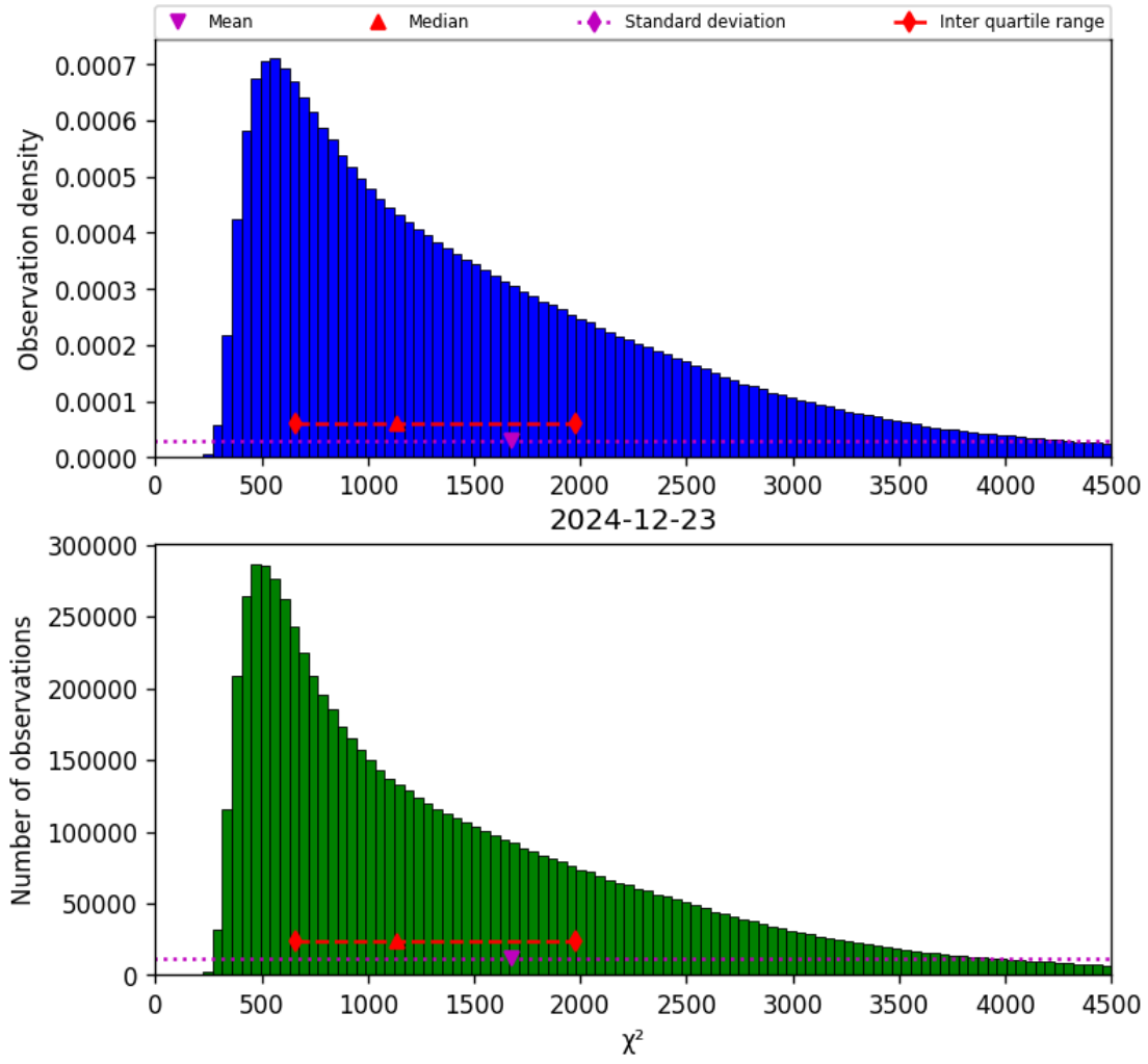
Figure 22: Histogram of “ \chi^2 ” for 2024-12-22 to 2024-12-24
