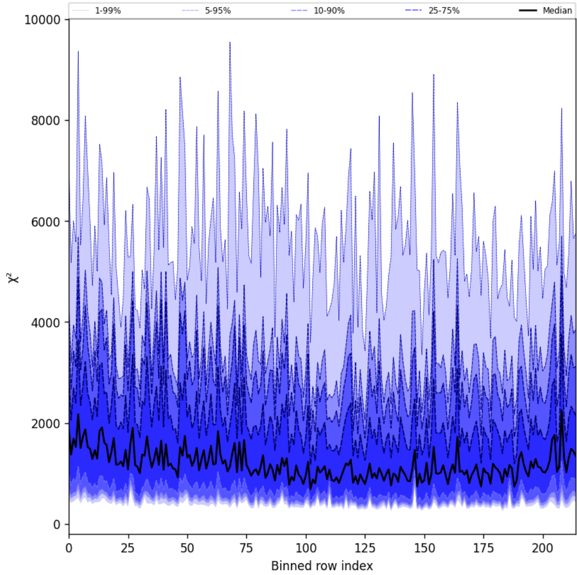
Figure 30: Along track statistics of “ \chi^2 ” for 2024-12-22 to 2024-12-24
