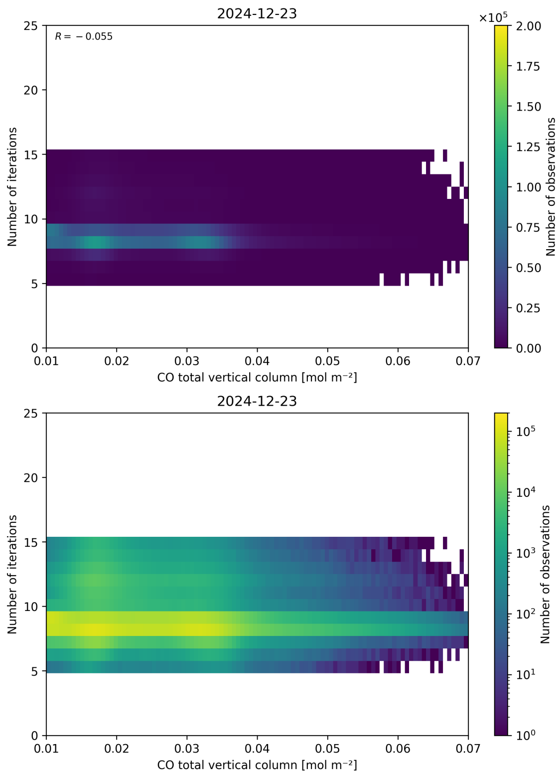
Figure 42: Scatter density plot of “CO total vertical column” against “Number of iterations” for 2024-12-22 to 2024-12-24.
