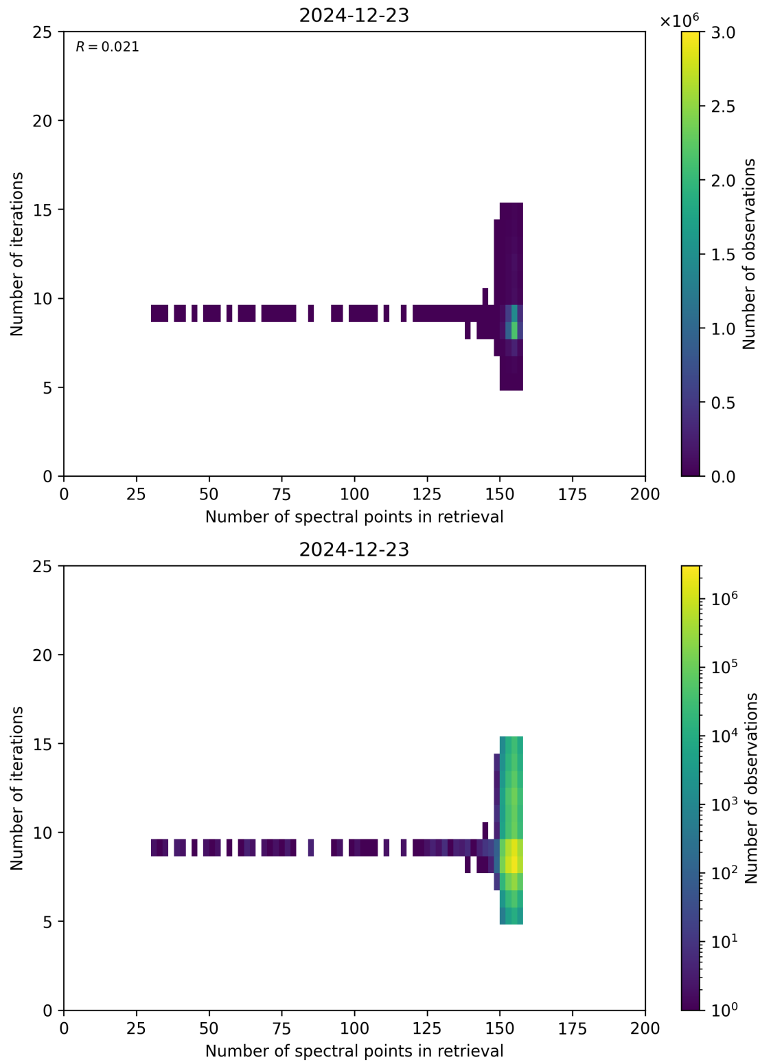
Figure 60: Scatter density plot of “Number of spectral points in retrieval” against “Number of iterations” for 2024-12-22 to 2024-12-24.
