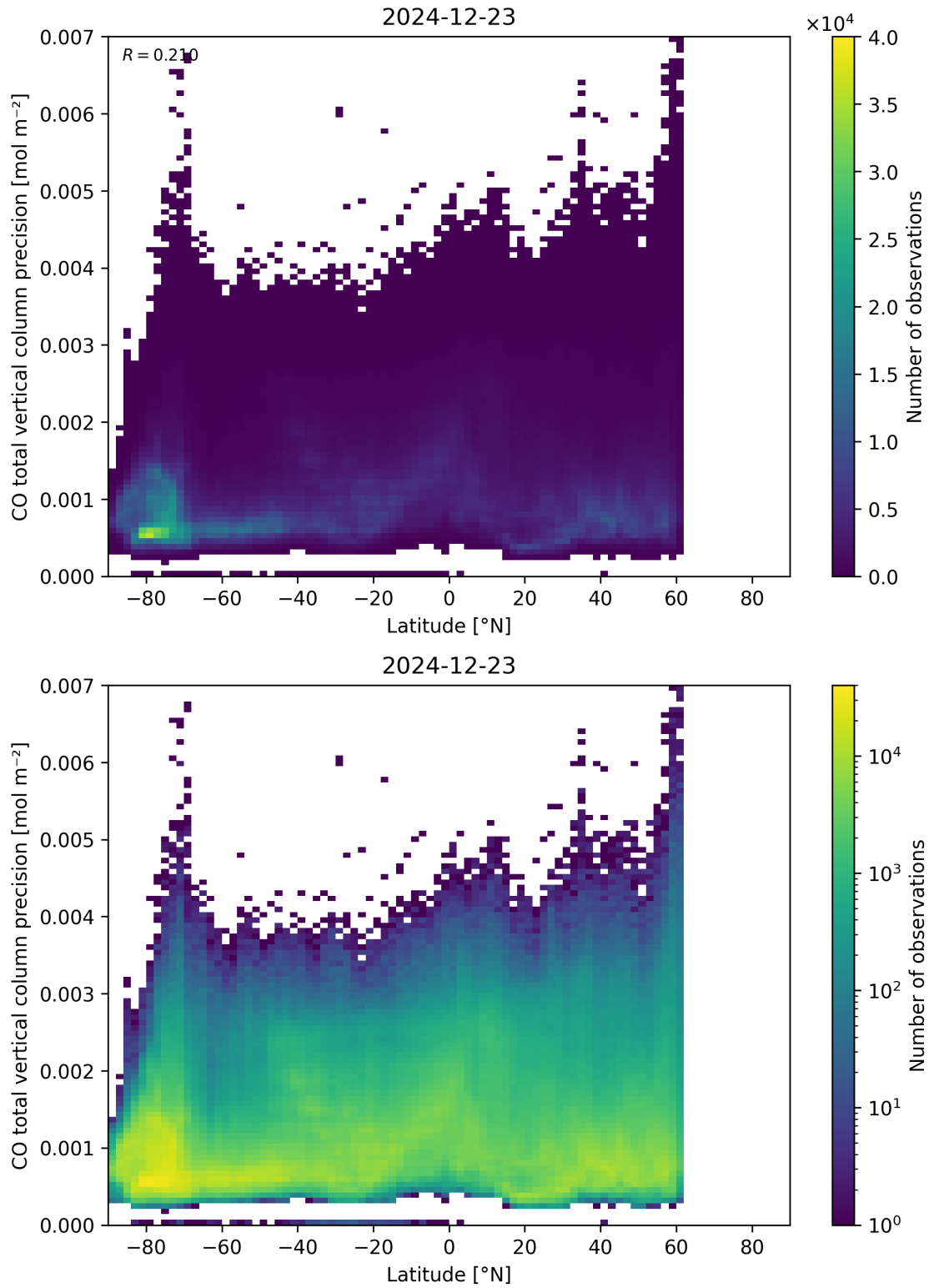
Figure 53: Scatter density plot of “Latitude” against “CO total vertical column precision” for 2024-12-22 to 2024-12-24.
