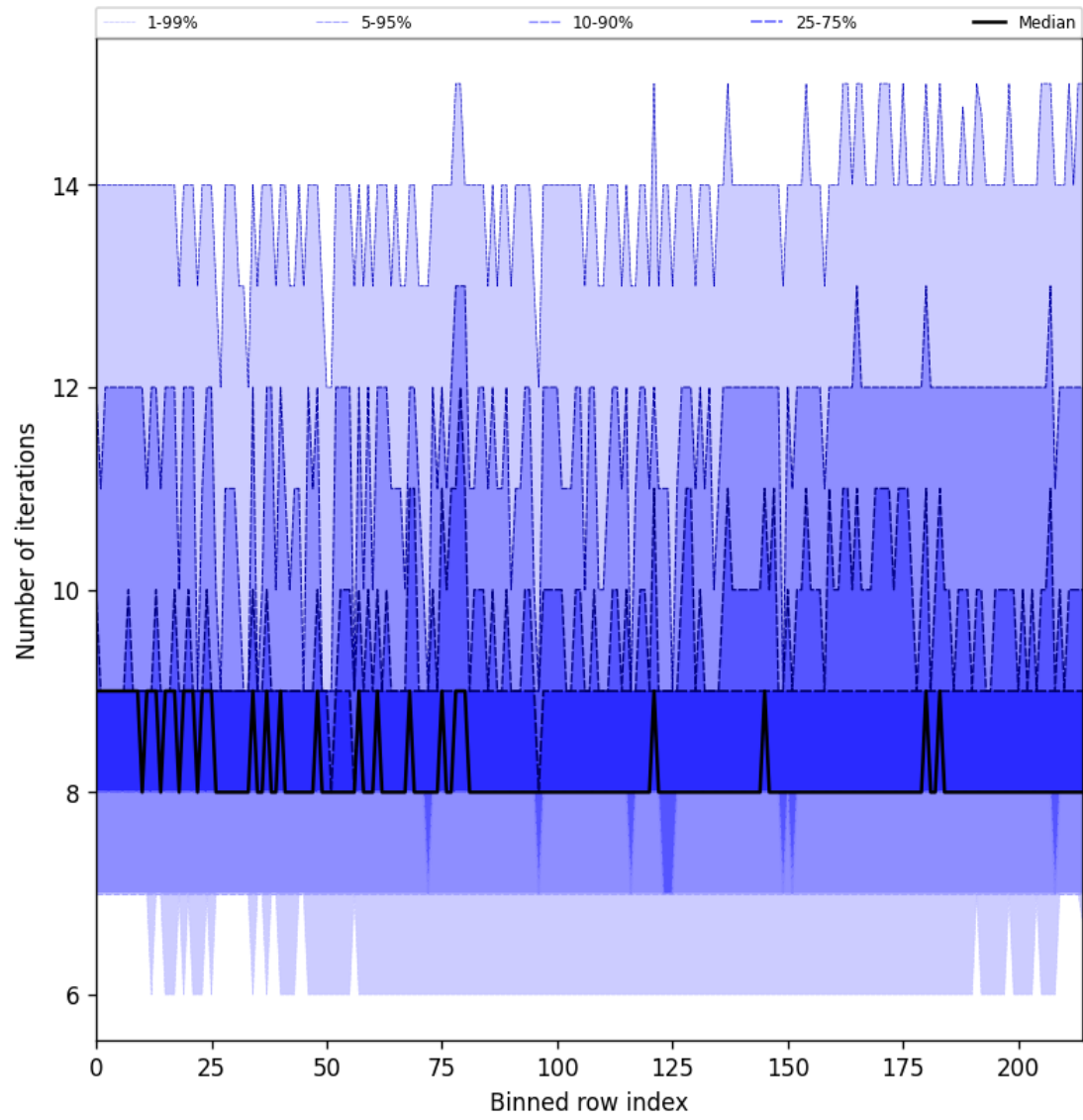
Figure 32: Along track statistics of “Number of iterations” for 2024-12-22 to 2024-12-24
