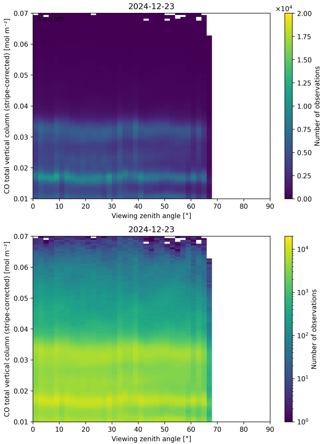
Figure 70: Scatter density plot of “Viewing zenith angle” against “CO total vertical column (stripe-corrected)” for 2024-12-22 to 2024-12-24.
