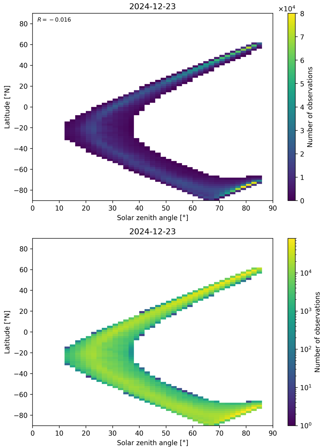
Figure 66: Scatter density plot of “Solar zenith angle” against “Latitude” for 2024-12-22 to 2024-12-24.
