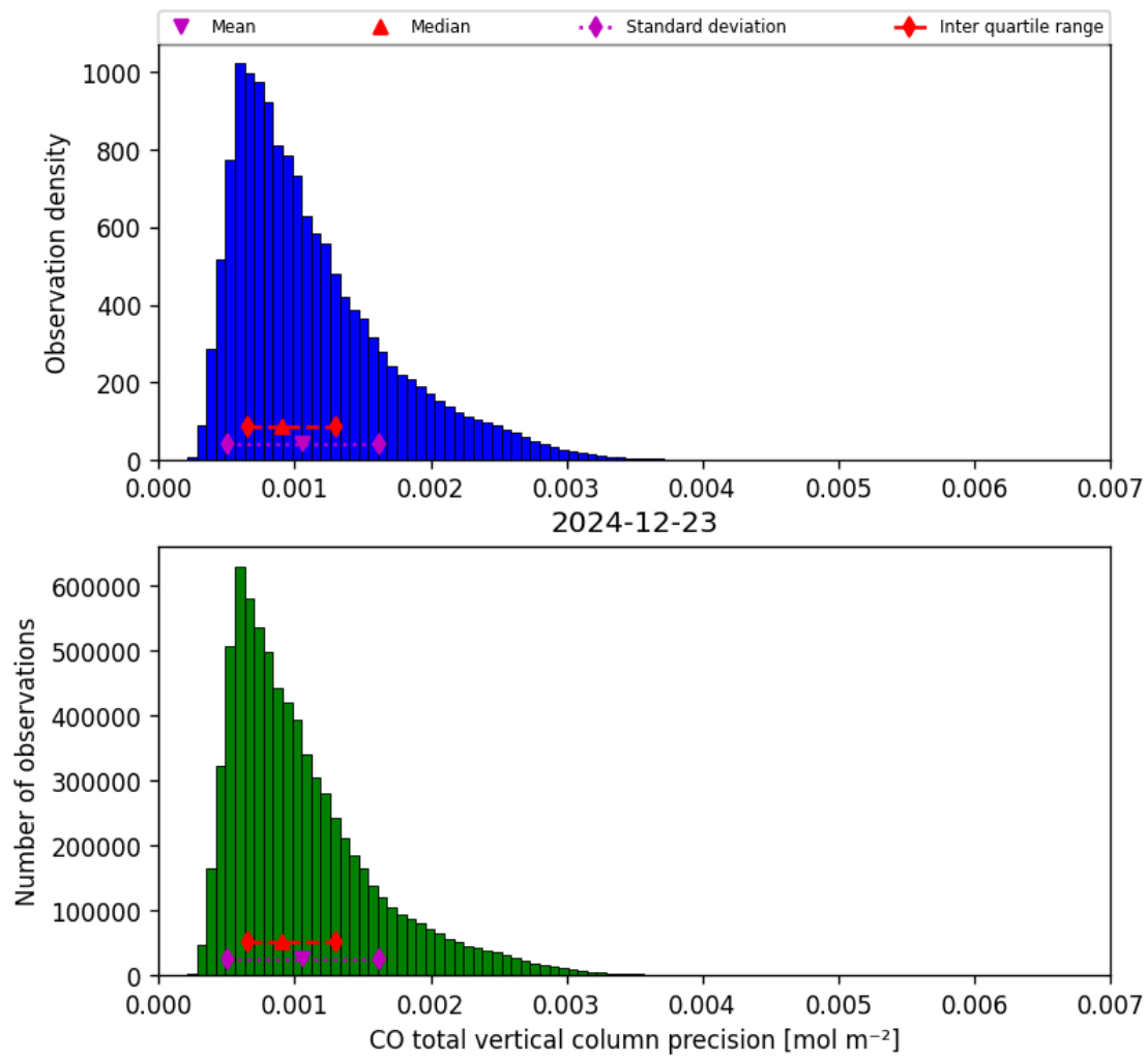
Figure 20: Histogram of “CO total vertical column precision” for 2024-12-22 to 2024-12-24
