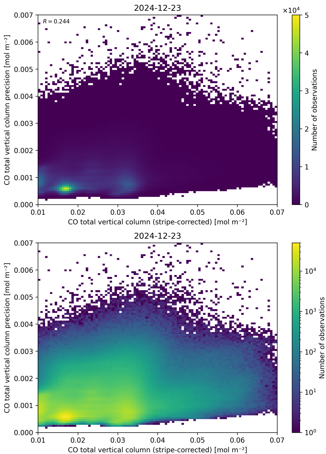
Figure 36: Scatter density plot of “CO total vertical column (stripe-corrected)” against “CO total vertical column precision” for 2024-12-22 to 2024-12-24.
