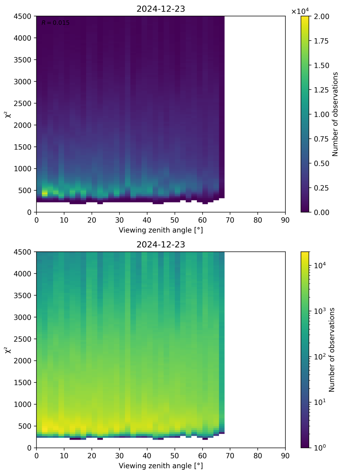
Figure 72: Scatter density plot of “Viewing zenith angle” against “ \chi^2 ” for 2024-12-22 to 2024-12-24.
