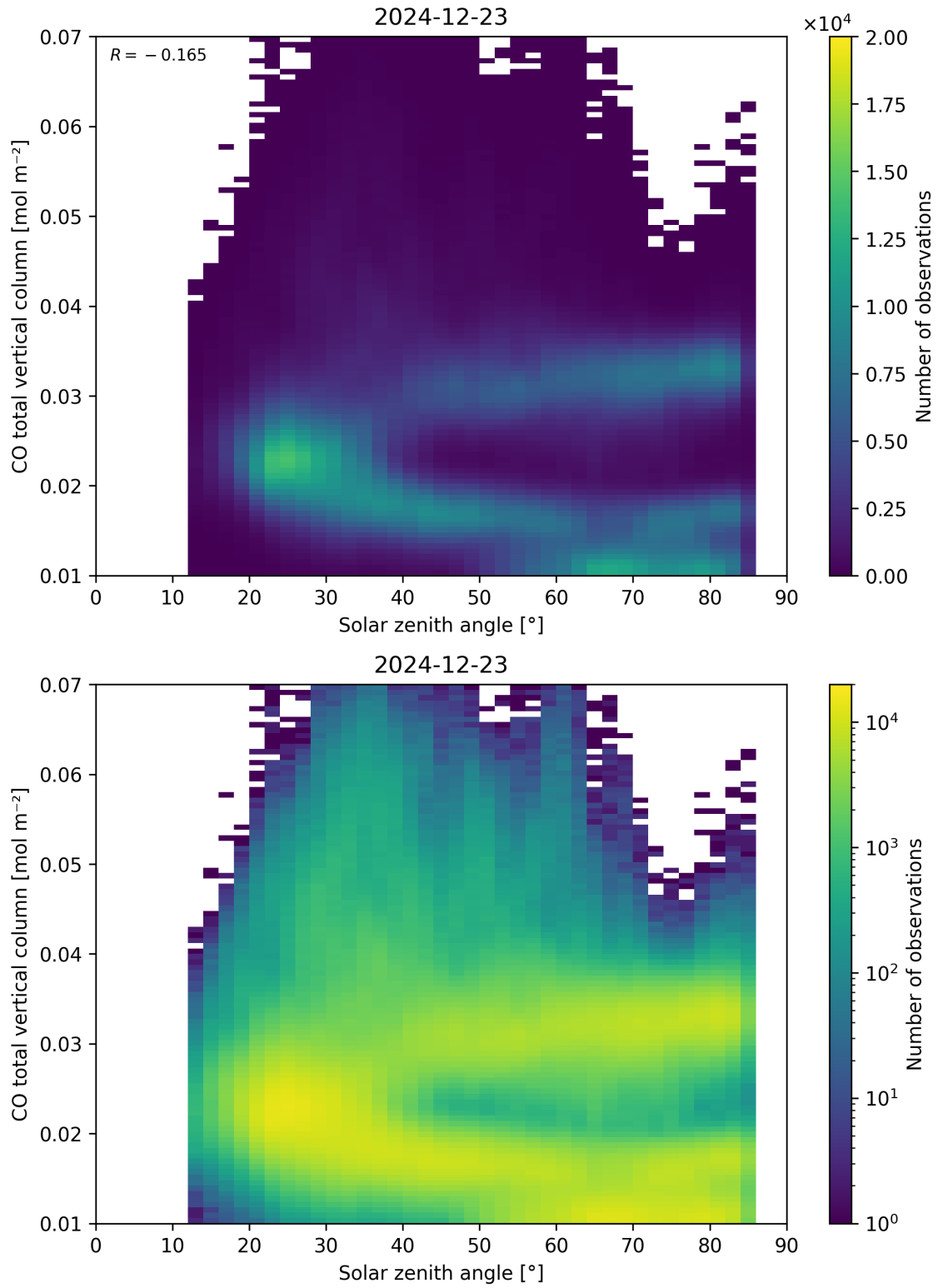
Figure 61: Scatter density plot of “Solar zenith angle” against “CO total vertical column” for 2024-12-22 to 2024-12-24.
