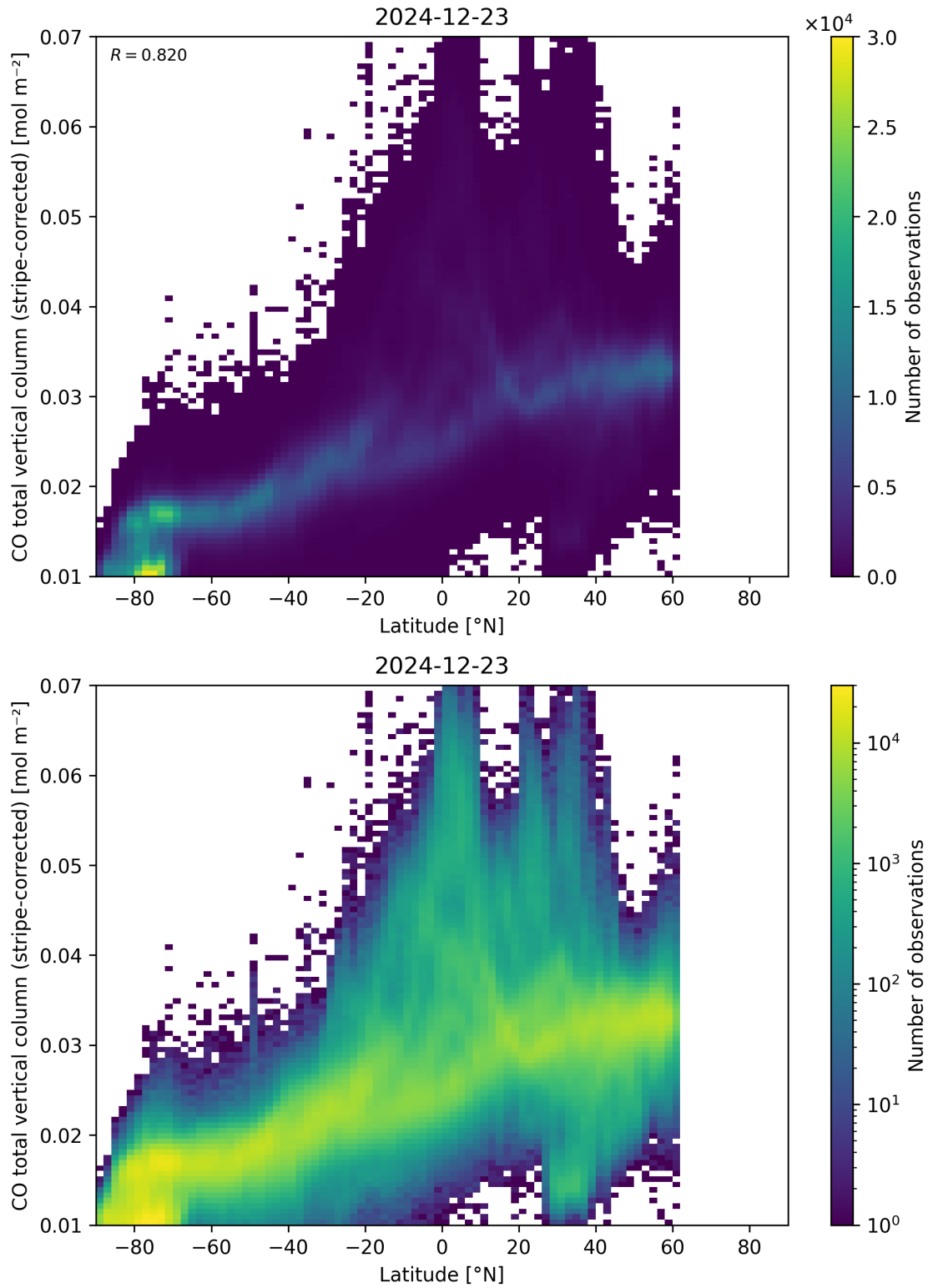
Figure 52: Scatter density plot of “Latitude” against “CO total vertical column (stripe-corrected)” for 2024-12-22 to 2024-12-24.
