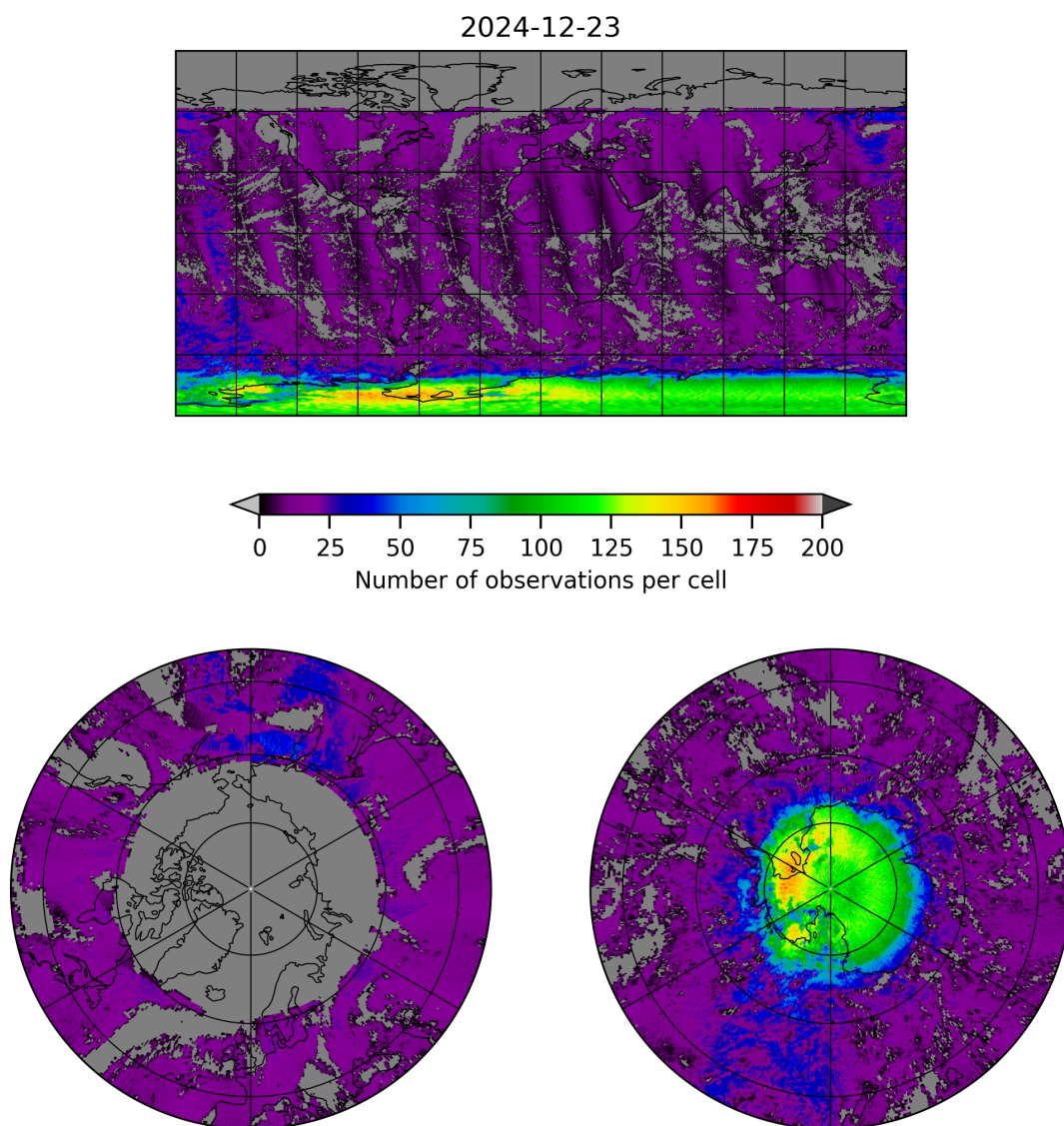
Figure 8: Map of the number of observations for 2024-12-22 to 2024-12-24
