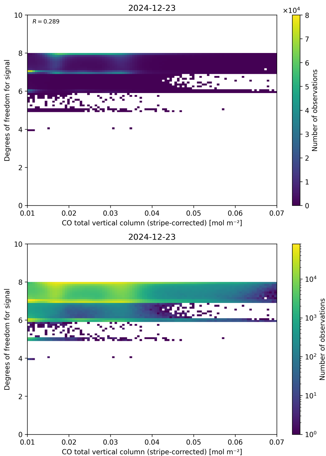
Figure 38: Scatter density plot of “CO total vertical column (stripe-corrected)” against “Degrees of freedom for signal” for 2024-12-22 to 2024-12-24.
