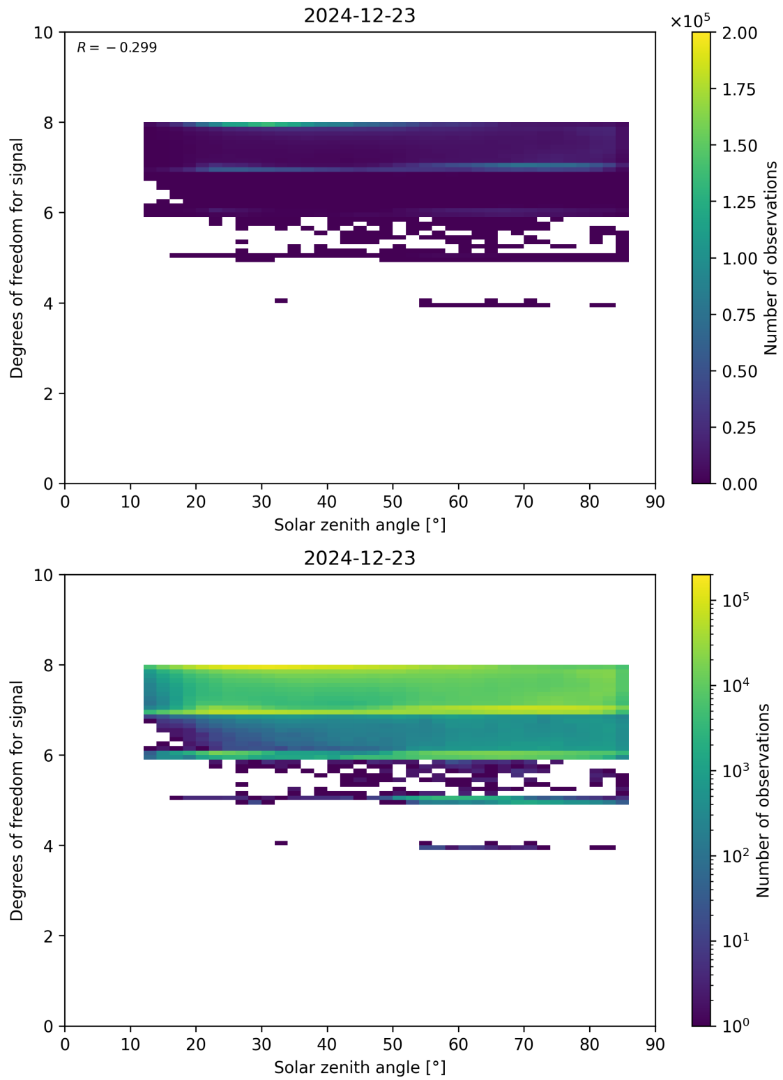
Figure 65: Scatter density plot of “Solar zenith angle” against “Degrees of freedom for signal” for 2024-12-22 to 2024-12-24.
