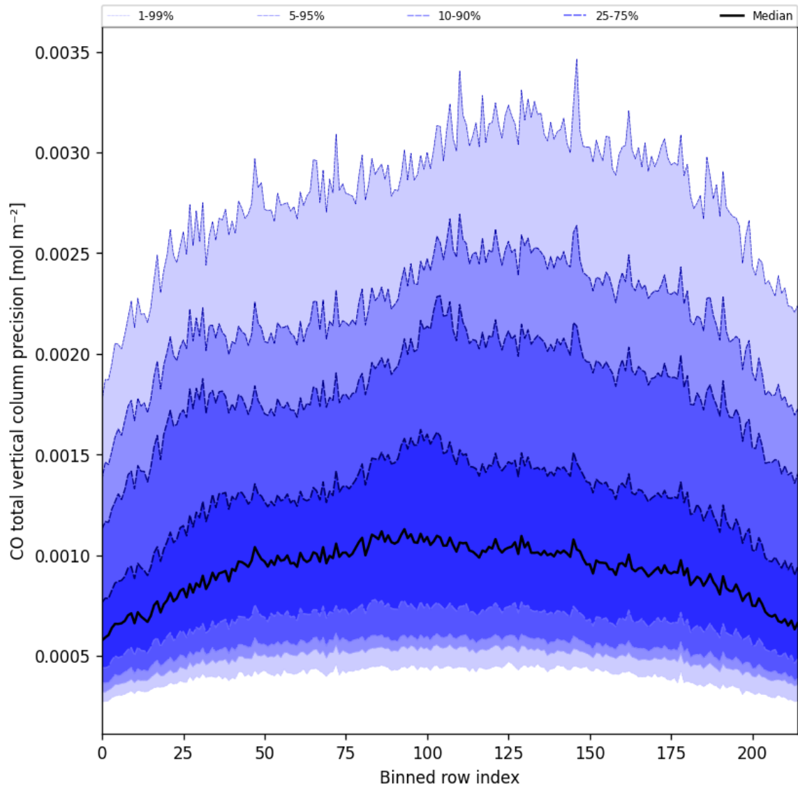
Figure 28: Along track statistics of “CO total vertical column precision” for 2024-12-22 to 2024-12-24
