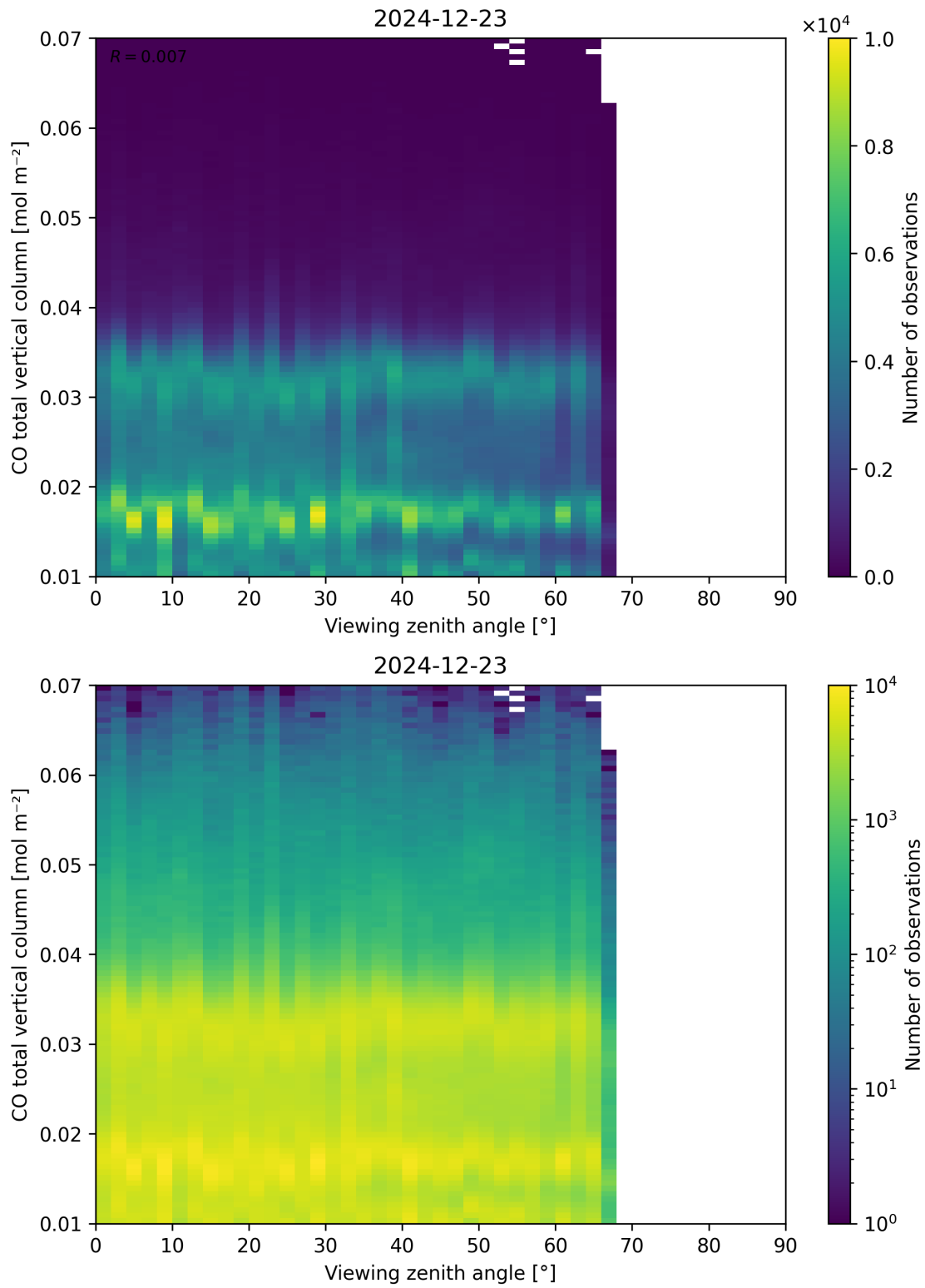
Figure 69: Scatter density plot of “Viewing zenith angle” against “CO total vertical column” for 2024-12-22 to 2024-12-24.
