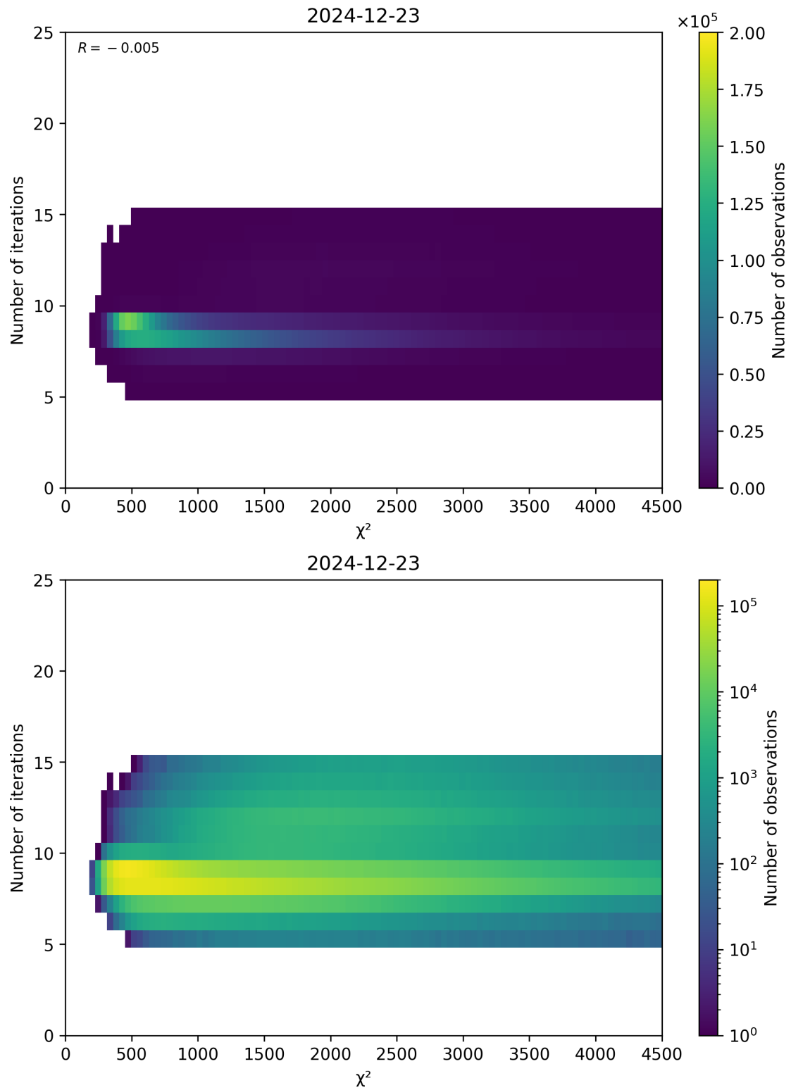
Figure 49: Scatter density plot of “ \chi^2 ” against “Number of iterations” for 2024-12-22 to 2024-12-24.
