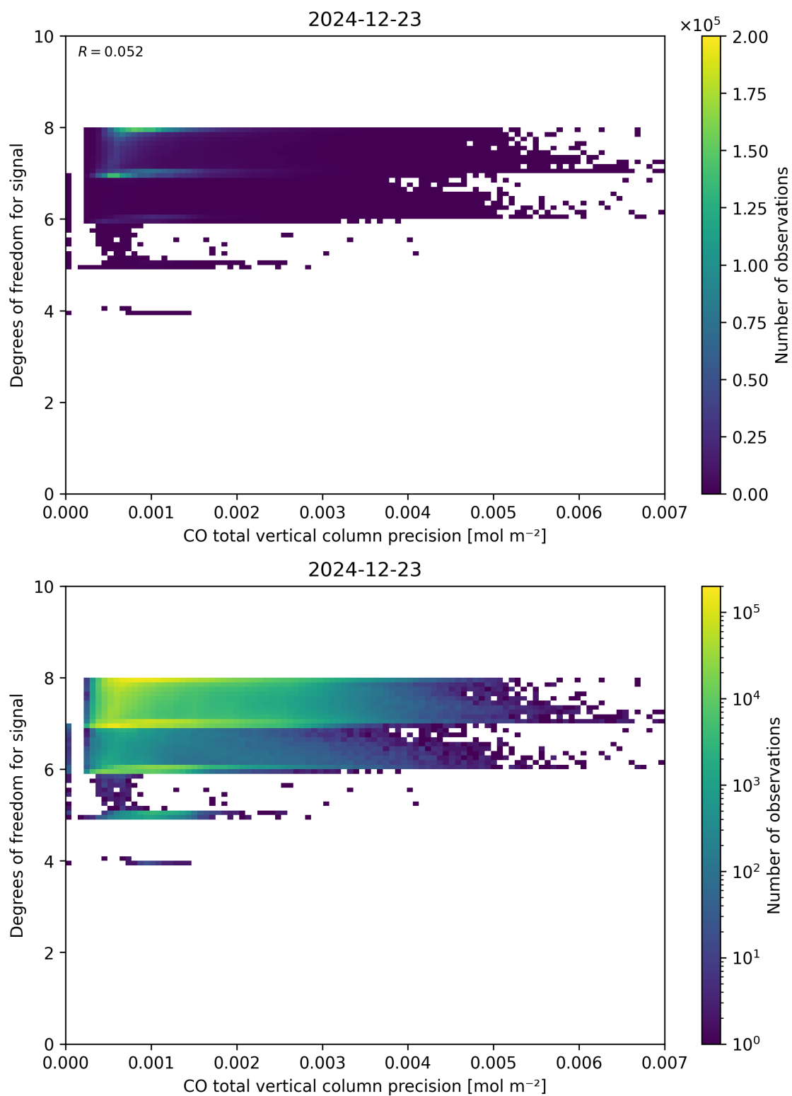
Figure 45: Scatter density plot of “CO total vertical column precision” against “Degrees of freedom for signal” for 2024-12-22 to 2024-12-24.
