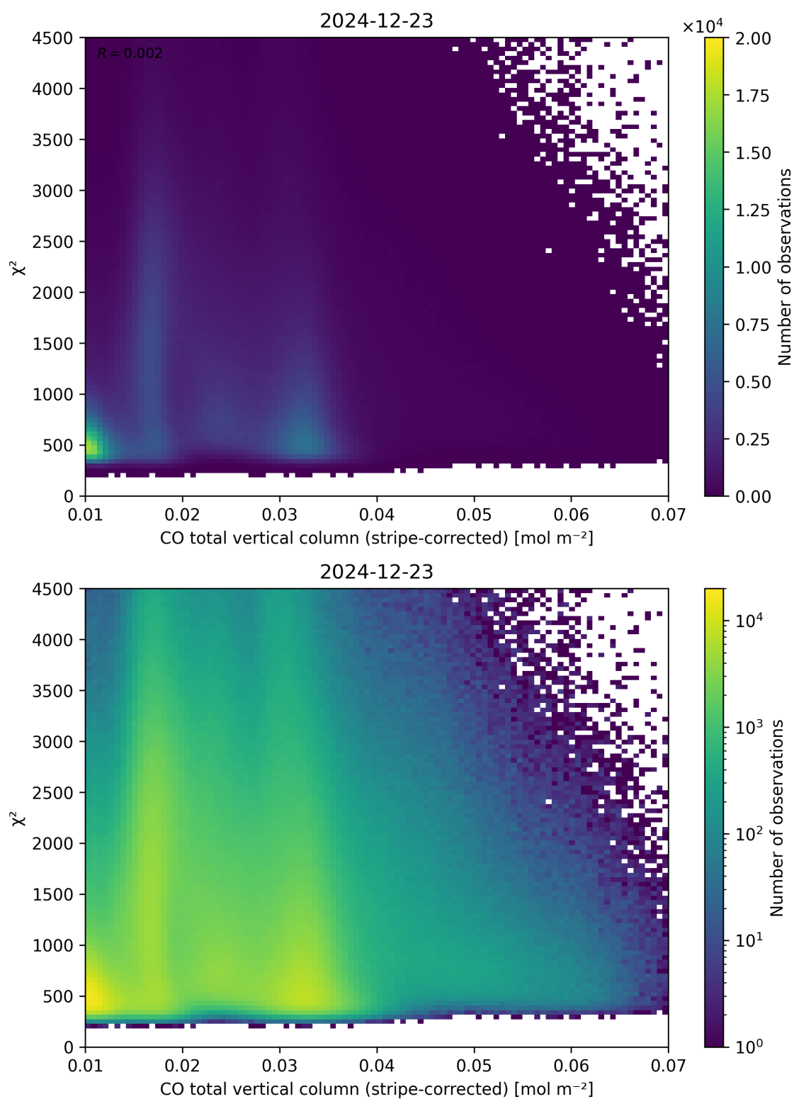
Figure 37: Scatter density plot of “CO total vertical column (stripe-corrected)” against “ \chi^2 ” for 2024-12-22 to 2024-12-24.
