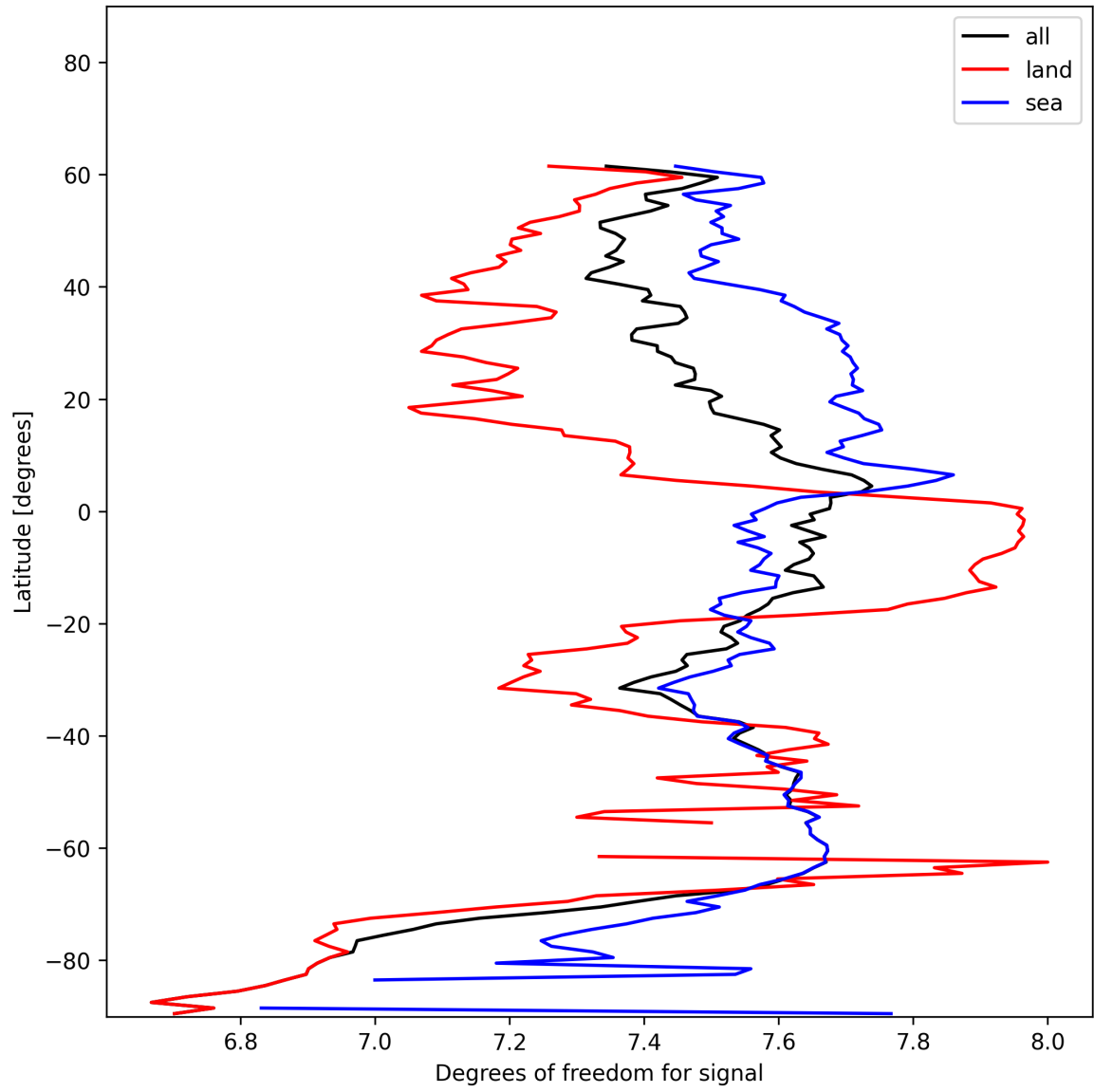
Figure 15: Zonal average of “Degrees of freedom for signal” for 2024-12-22 to 2024-12-24.
