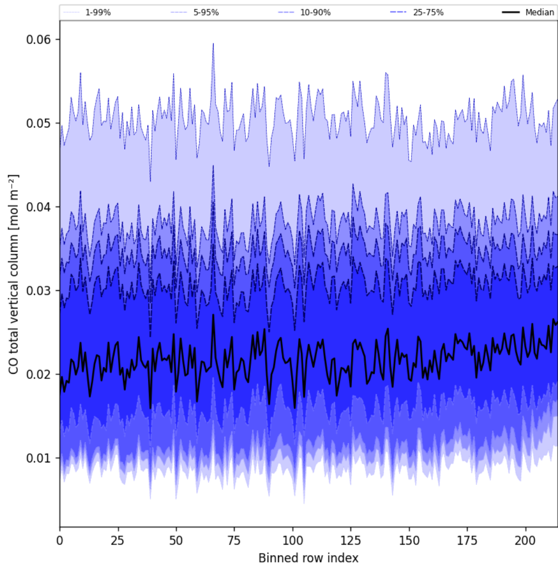
Figure 26: Along track statistics of “CO total vertical column” for 2024-12-22 to 2024-12-24
