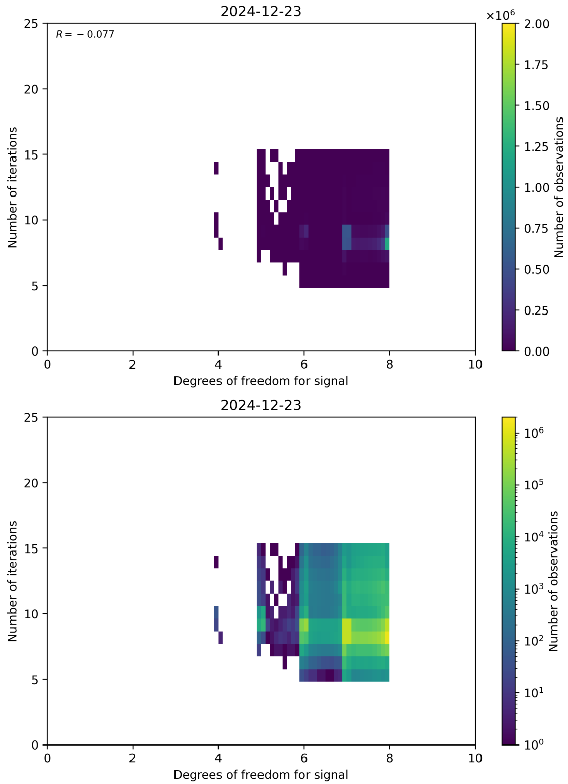
Figure 50: Scatter density plot of “Degrees of freedom for signal” against “Number of iterations” for 2024-12-22 to 2024-12-24.
