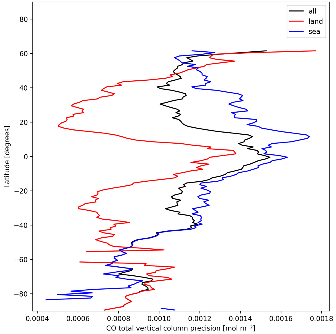
Figure 12: Zonal average of "CO total vertical column precision" for 2024-12-22 to 2024-12-24.
