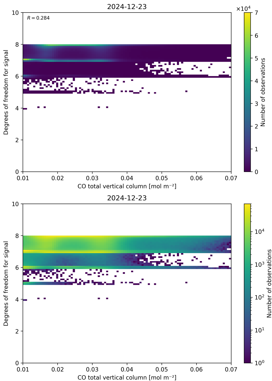
Figure 41: Scatter density plot of “CO total vertical column” against “Degrees of freedom for signal” for 2024-12-22 to 2024-12-24.
