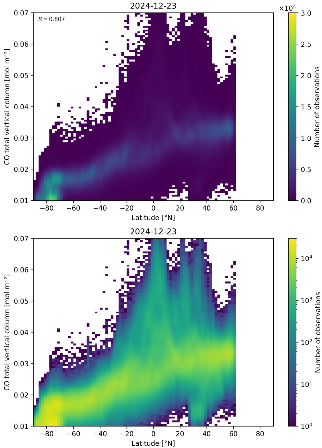
Figure 51: Scatter density plot of “Latitude” against “CO total vertical column” for 2024-12-22 to 2024-12-24.
