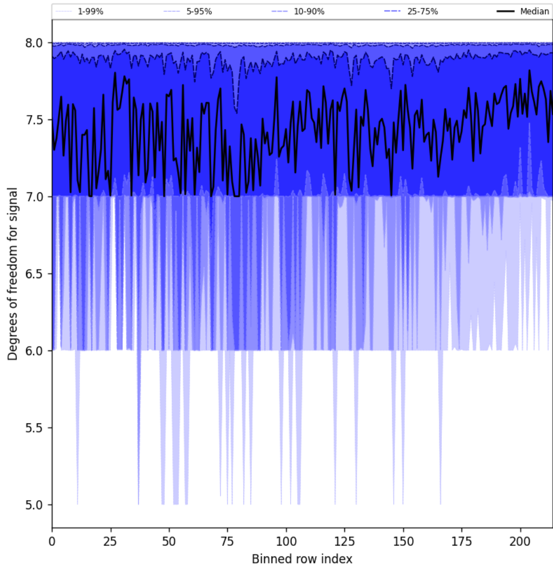
Figure 31: Along track statistics of “Degrees of freedom for signal” for 2024-12-22 to 2024-12-24
