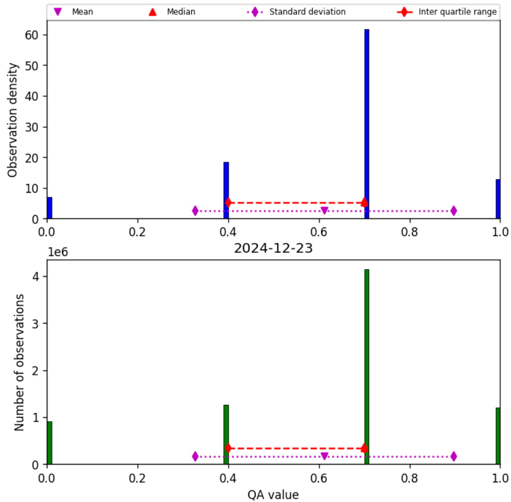
Figure 17: Histogram of “QA value” for 2024-12-22 to 2024-12-24
