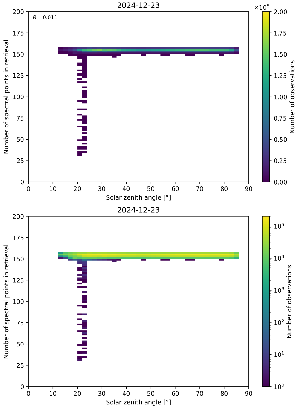
Figure 68: Scatter density plot of “Solar zenith angle” against “Number of spectral points in retrieval” for 2024-12-22 to 2024-12-24.
