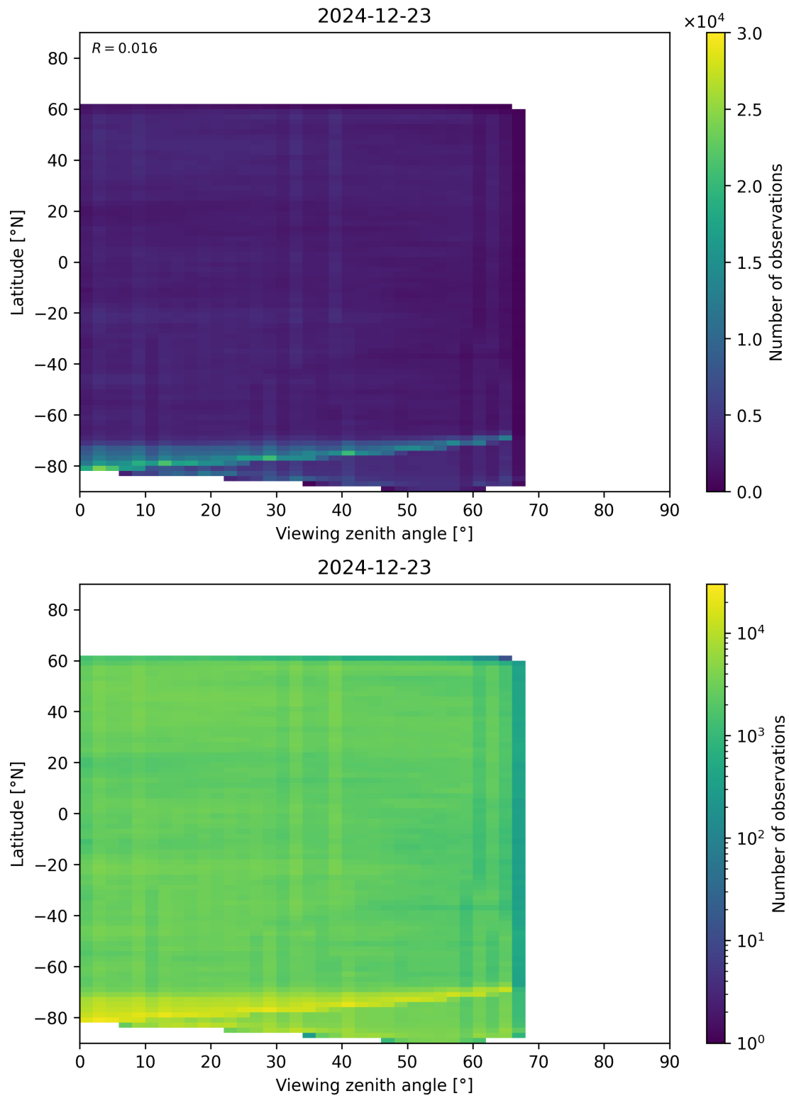
Figure 74: Scatter density plot of “Viewing zenith angle” against “Latitude” for 2024-12-22 to 2024-12-24.
