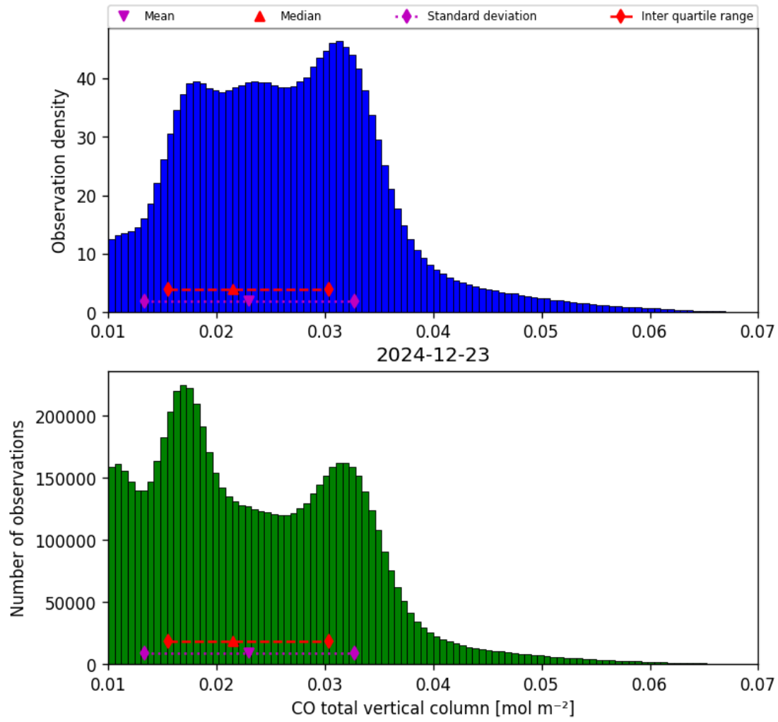
Figure 18: Histogram of “CO total vertical column” for 2024-12-22 to 2024-12-24
