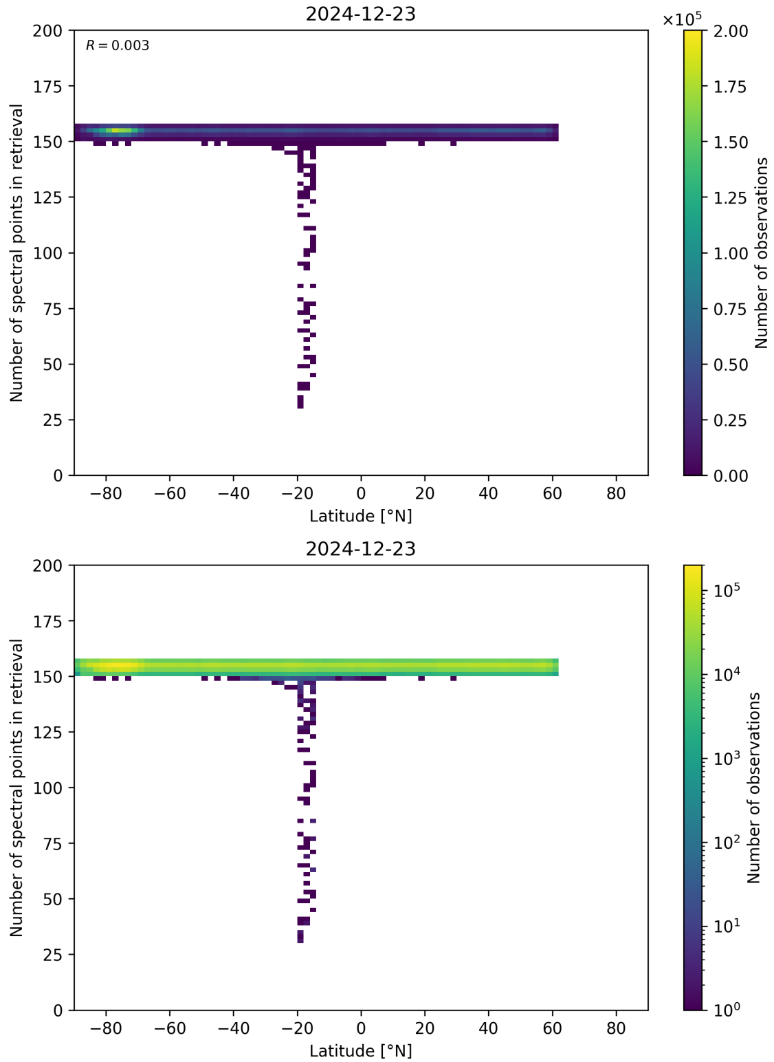
Figure 57: Scatter density plot of “Latitude” against “Number of spectral points in retrieval” for 2024-12-22 to 2024-12-24.
