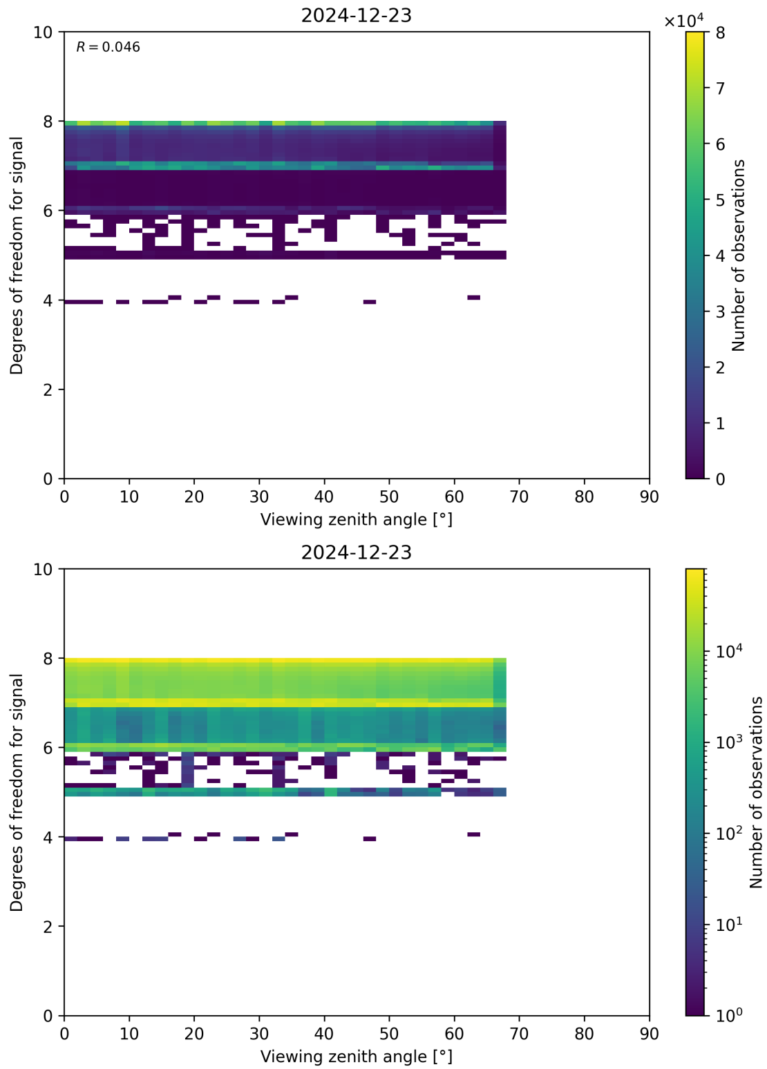
Figure 73: Scatter density plot of “Viewing zenith angle” against “Degrees of freedom for signal” for 2024-12-22 to 2024-12-24.
