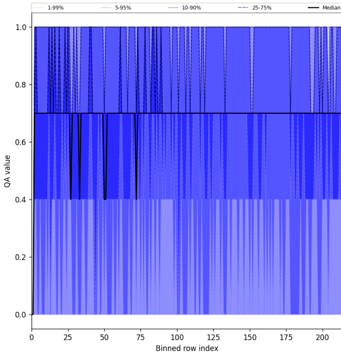
Figure 25: Along track statistics of “QA value” for 2024-12-22 to 2024-12-24
