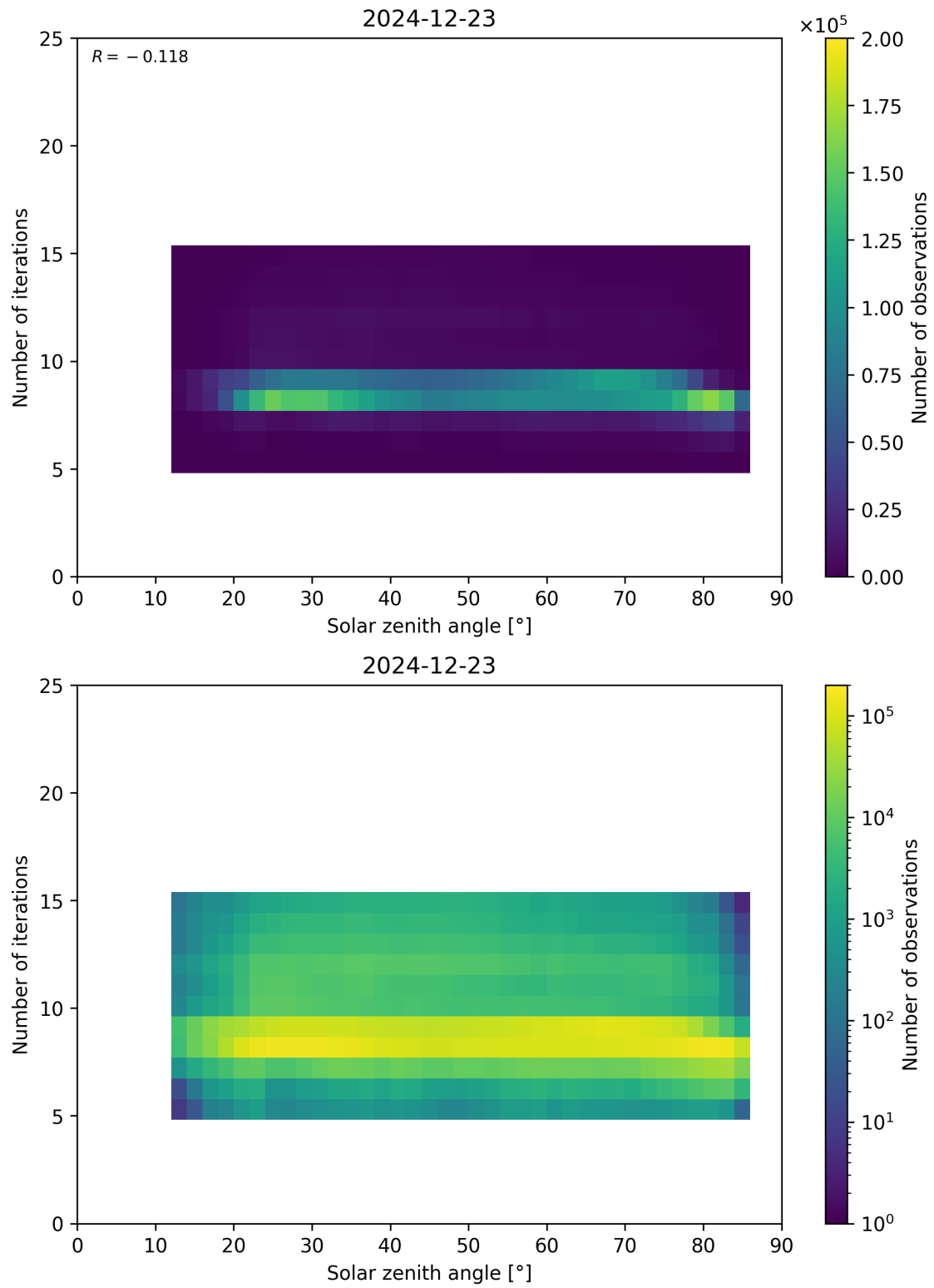
Figure 67: Scatter density plot of “Solar zenith angle” against “Number of iterations” for 2024-12-22 to 2024-12-24.
