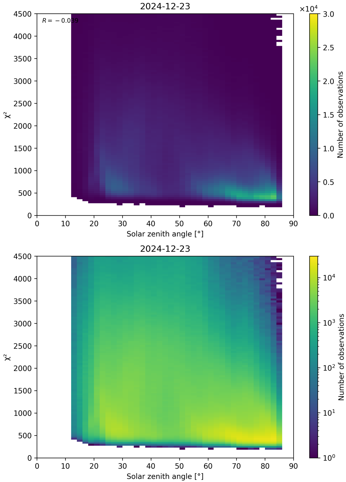
Figure 64: Scatter density plot of “Solar zenith angle” against “ \chi^2 ” for 2024-12-22 to 2024-12-24.
