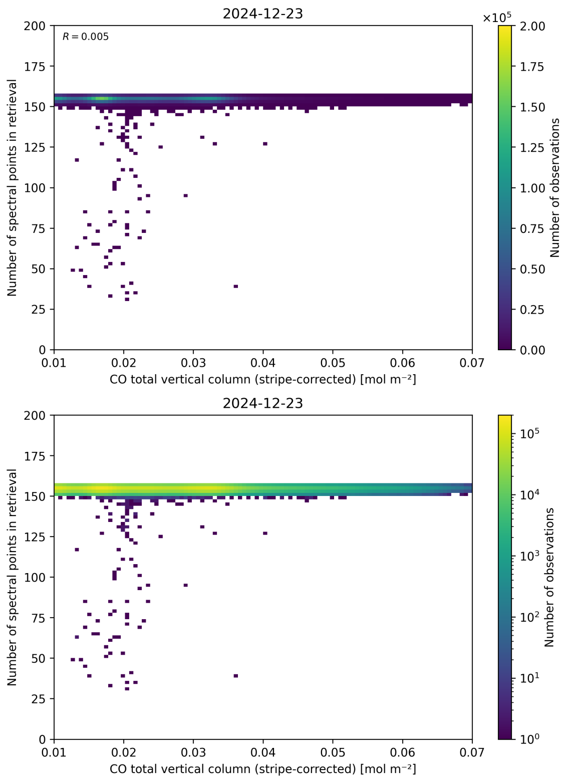
Figure 40: Scatter density plot of “CO total vertical column (stripe-corrected)” against “Number of spectral points in retrieval” for 2024-12-22 to 2024-12-24.
