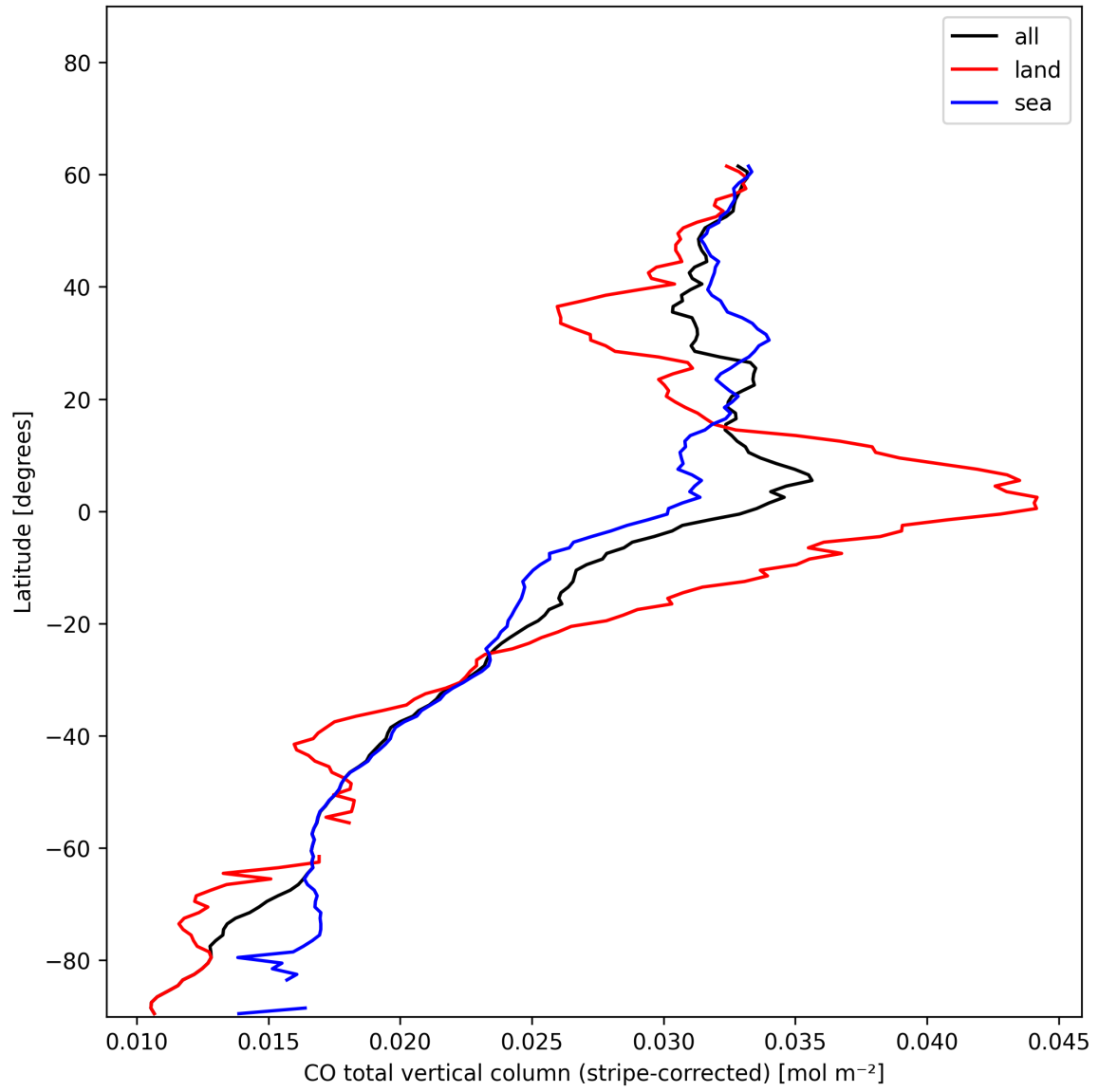
Figure 11: Zonal average of “CO total vertical column (stripe-corrected)” for 2024-12-22 to 2024-12-24.
