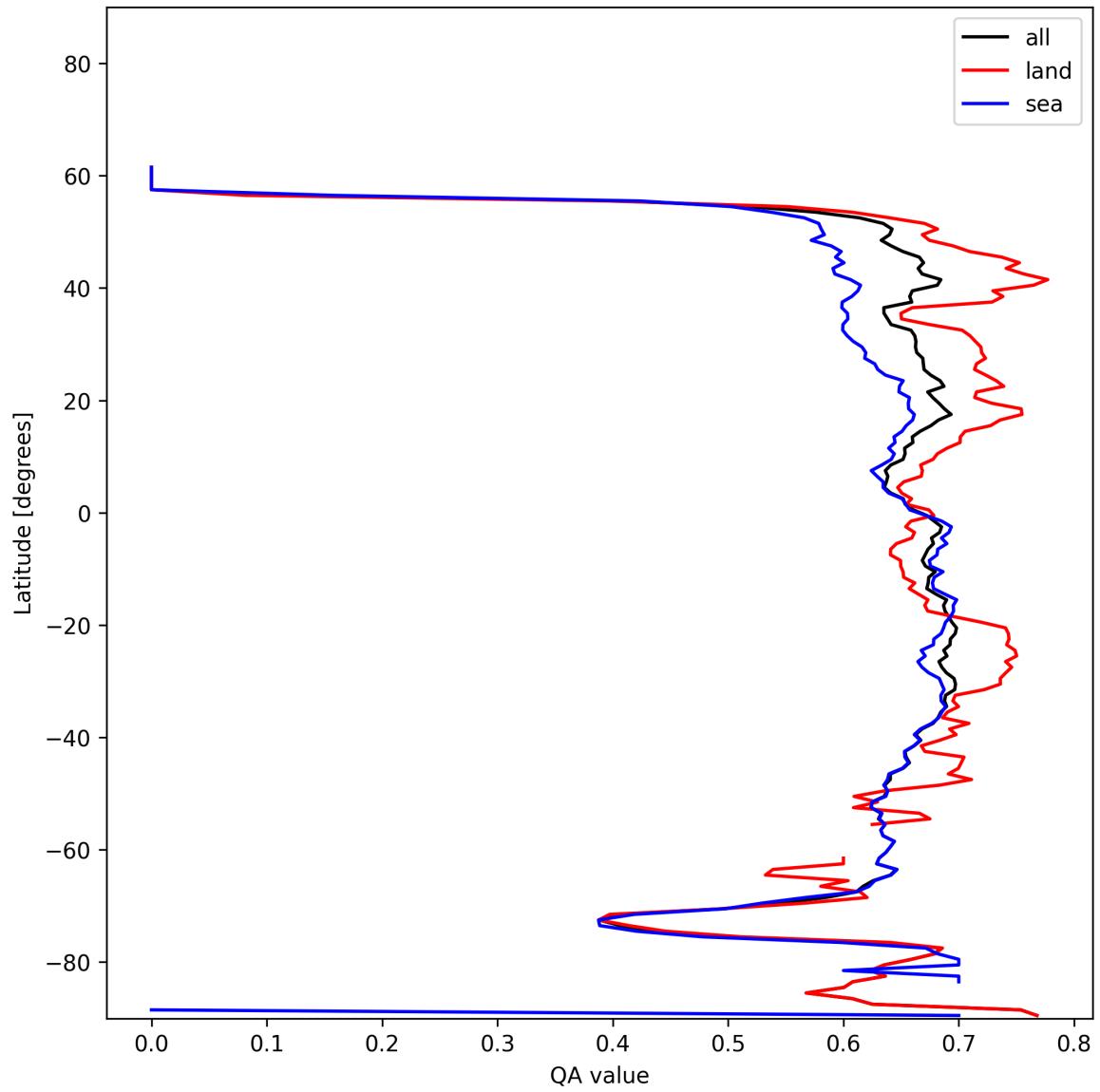
Figure 9: Zonal average of “QA value” for 2024-12-22 to 2024-12-24.
