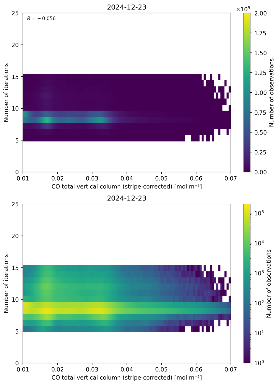
Figure 39: Scatter density plot of “CO total vertical column (stripe-corrected)” against “Number of iterations” for 2024-12-22 to 2024-12-24.
