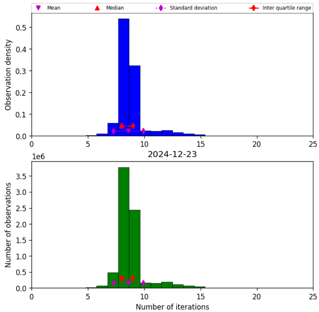
Figure 24: Histogram of “Number of iterations” for 2024-12-22 to 2024-12-24
