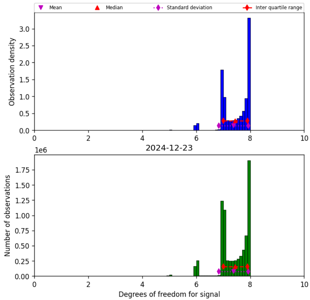
Figure 23: Histogram of “Degrees of freedom for signal” for 2024-12-22 to 2024-12-24
