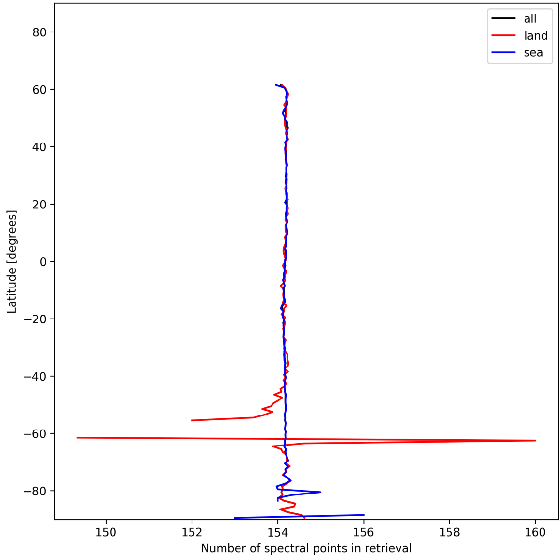
Figure 13: Zonal average of “Number of spectral points in retrieval” for 2024-12-22 to 2024-12-24.
