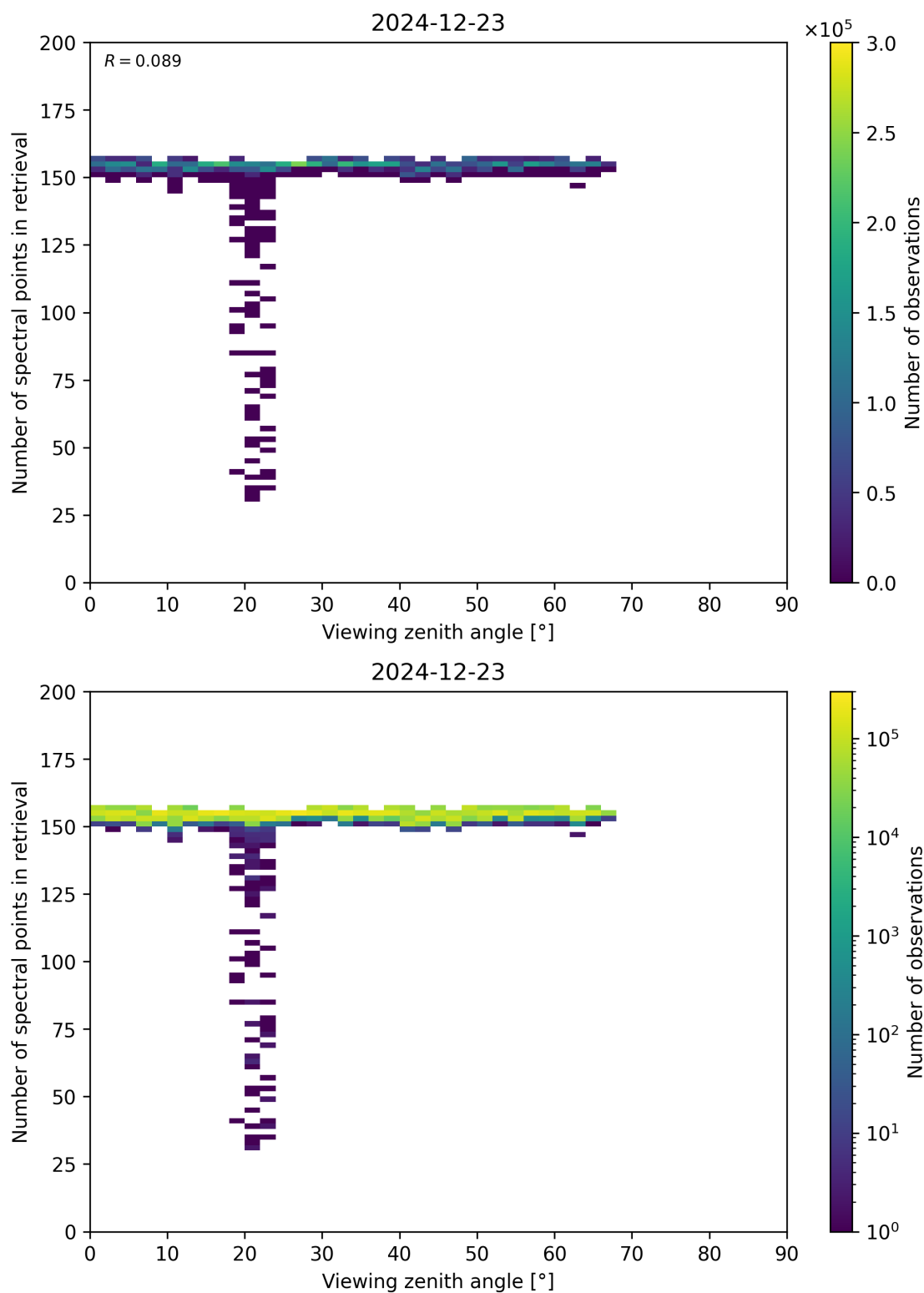
Figure 76: Scatter density plot of “Viewing zenith angle” against “Number of spectral points in retrieval” for 2024-12-22 to 2024-12-24.
