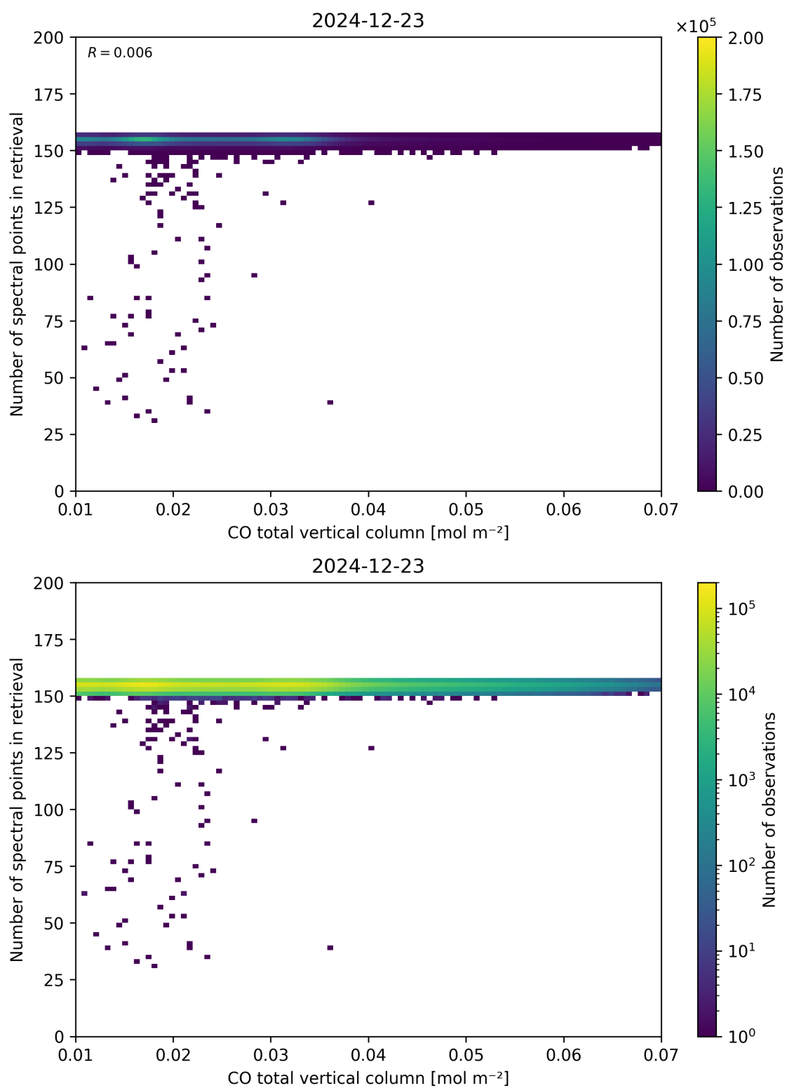
Figure 43: Scatter density plot of “CO total vertical column” against “Number of spectral points in retrieval” for 2024-12-22 to 2024-12-24.
