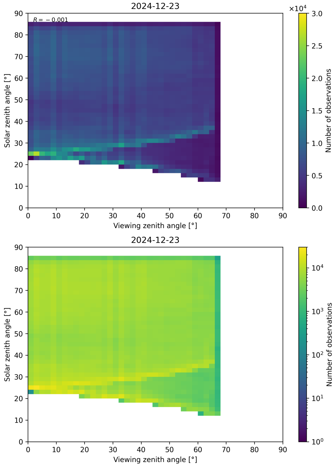
Figure 77: Scatter density plot of “Viewing zenith angle” against “Solar zenith angle” for 2024-12-22 to 2024-12-24.
