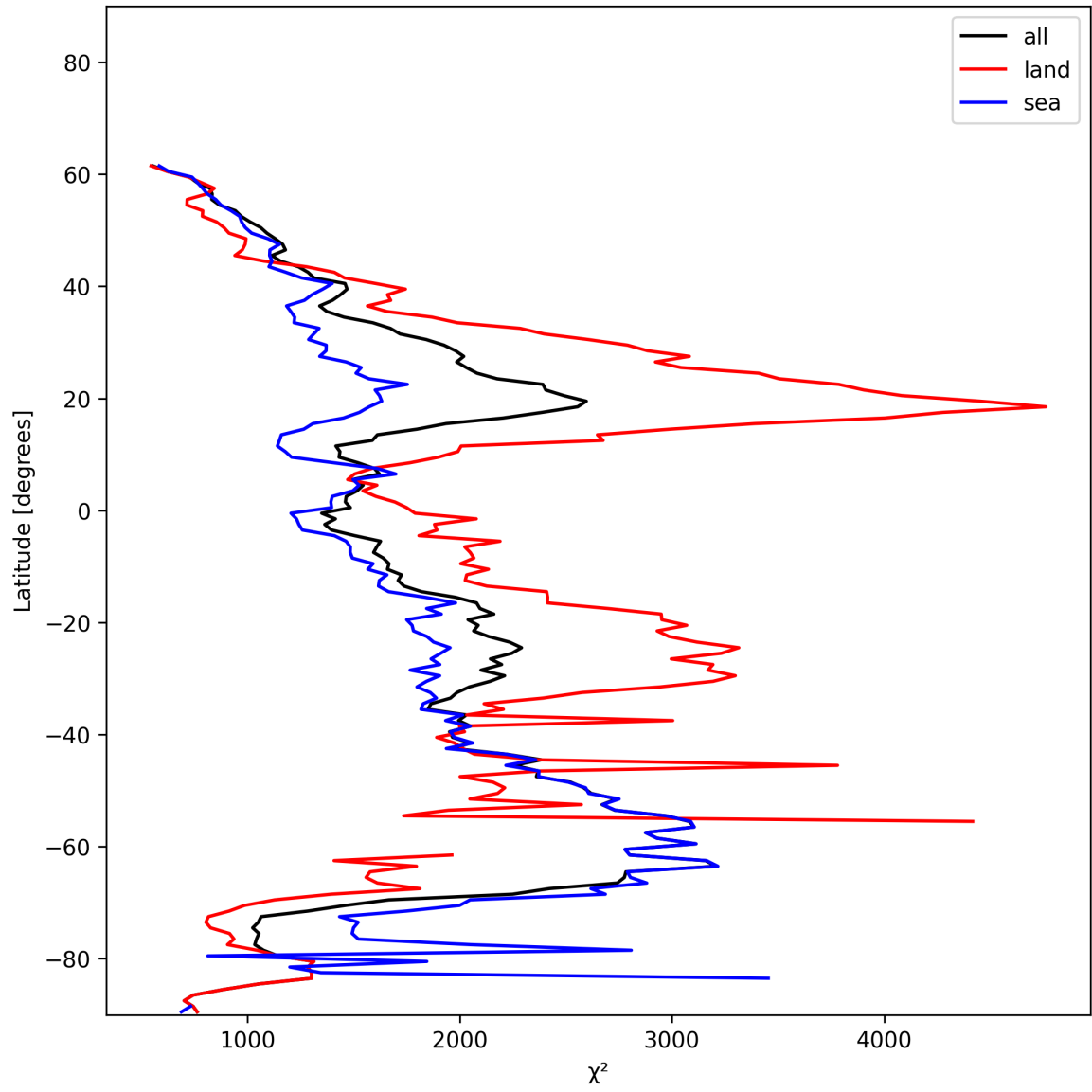
Figure 14: Zonal average of “ \chi^2 ” for 2024-12-22 to 2024-12-24.
