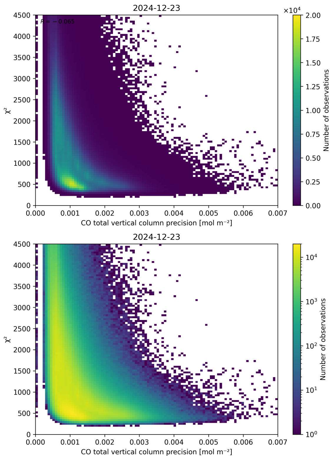
Figure 44: Scatter density plot of “CO total vertical column precision” against “ \chi^2 ” for 2024-12-22 to 2024-12-24.
