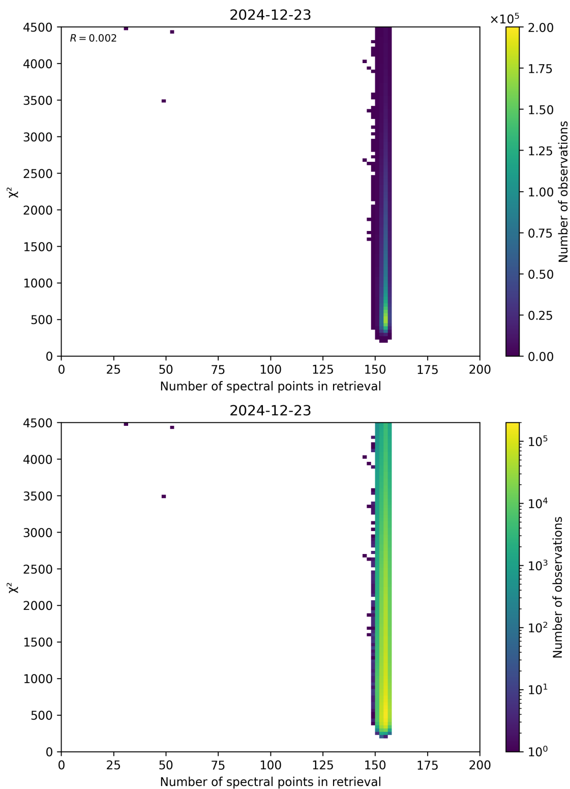
Figure 58: Scatter density plot of “Number of spectral points in retrieval” against “ \chi^2 ” for 2024-12-22 to 2024-12-24.
