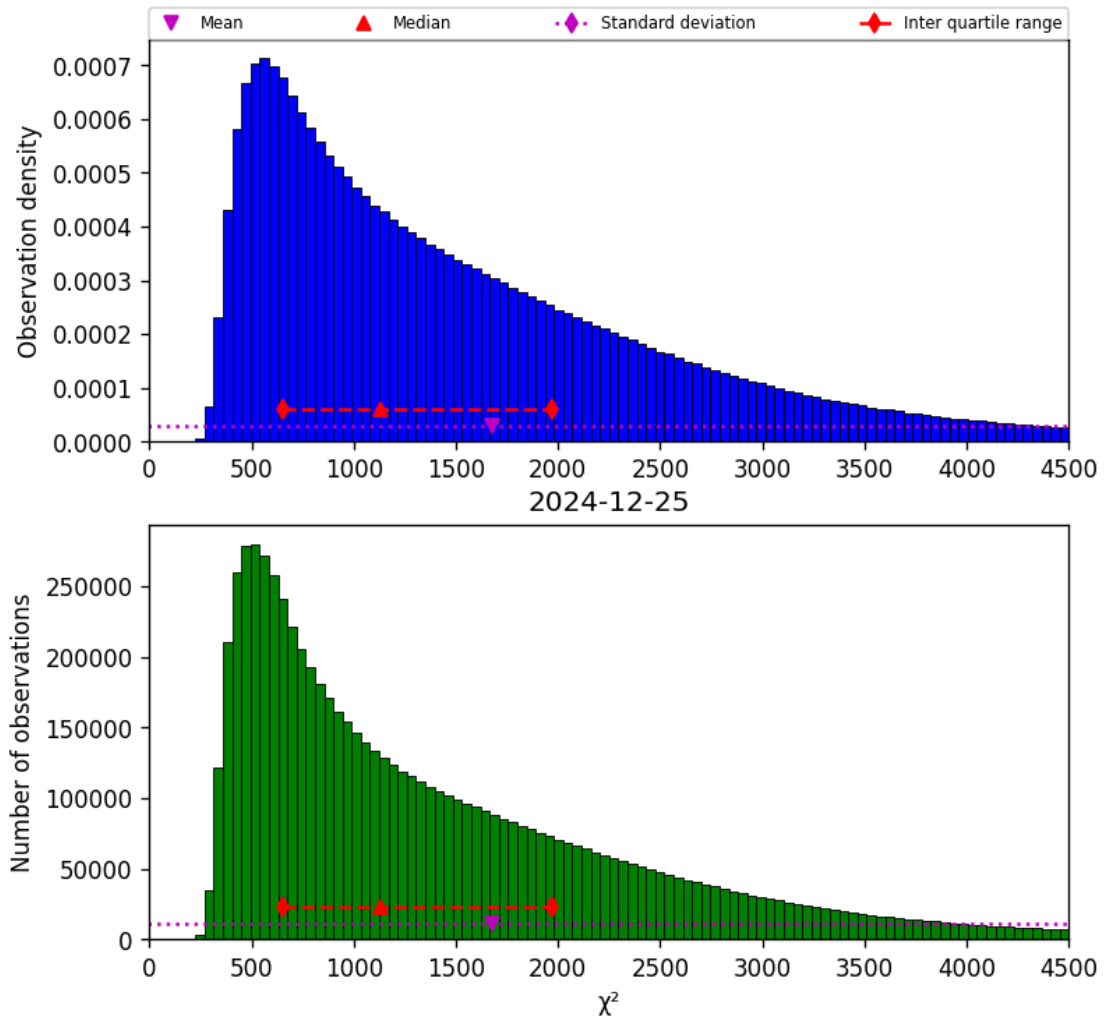
Figure 22: Histogram of “ \chi^2 ” for 2024-12-24 to 2024-12-26
