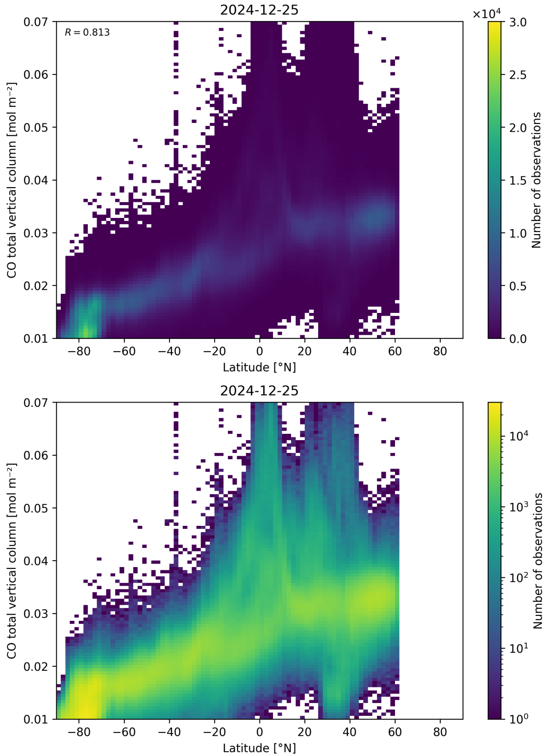
Figure 51: Scatter density plot of “Latitude” against “CO total vertical column” for 2024-12-24 to 2024-12-26.
