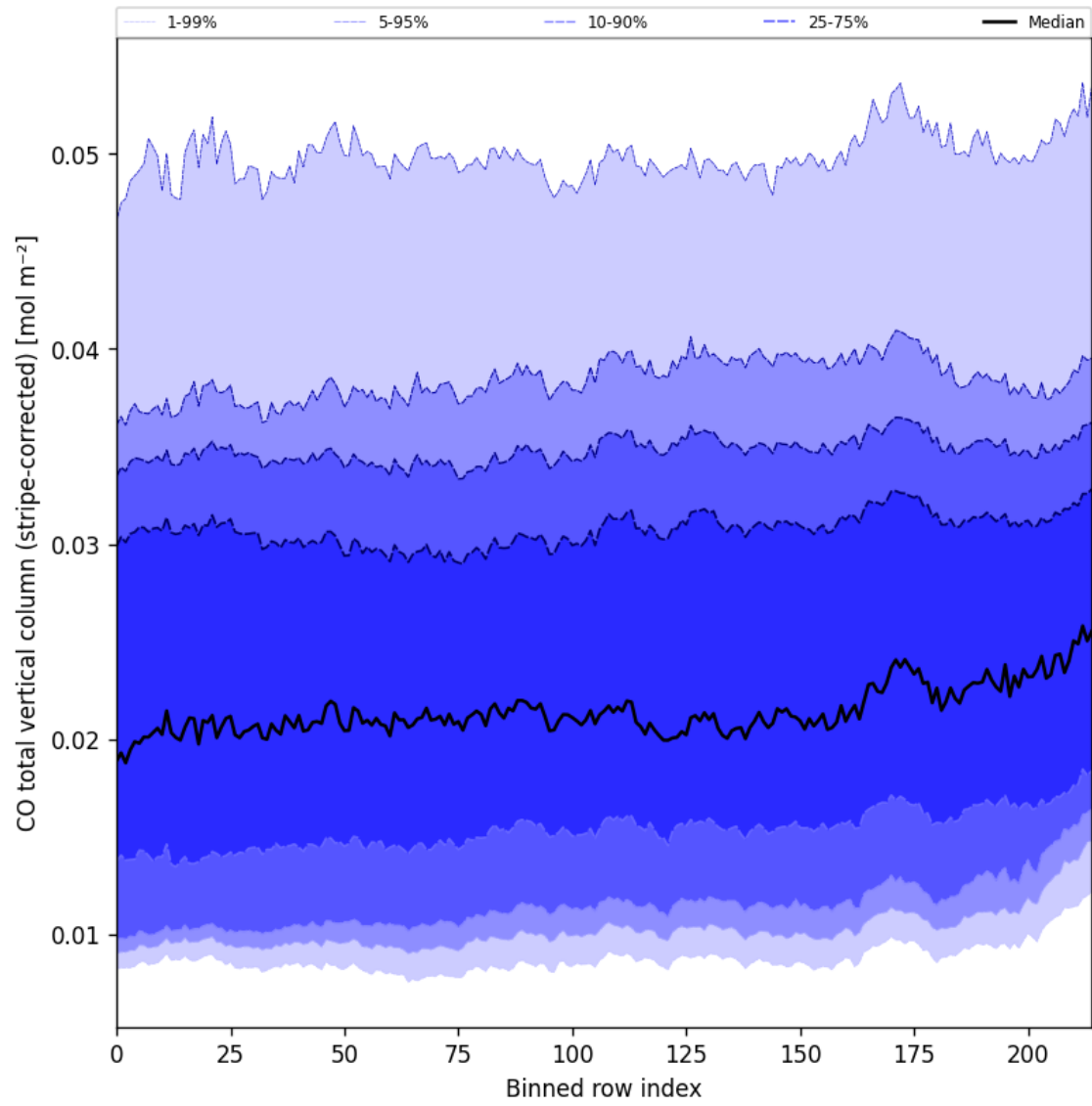
Figure 27: Along track statistics of “CO total vertical column (stripe-corrected)” for 2024-12-24 to 2024-12-26
