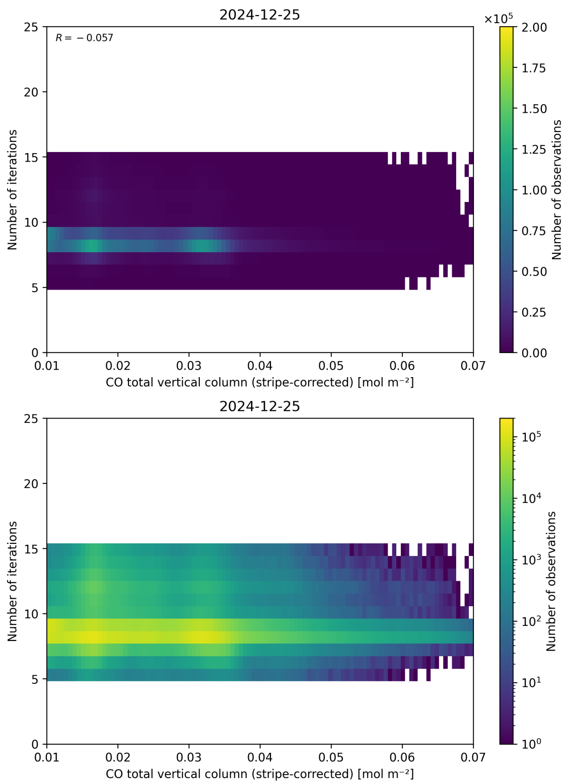
Figure 39: Scatter density plot of “CO total vertical column (stripe-corrected)” against “Number of iterations” for 2024-12-24 to 2024-12-26.
