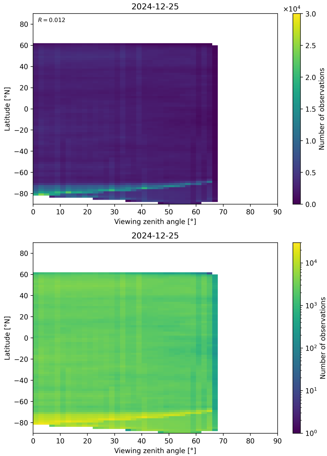
Figure 74: Scatter density plot of “Viewing zenith angle” against “Latitude” for 2024-12-24 to 2024-12-26.
