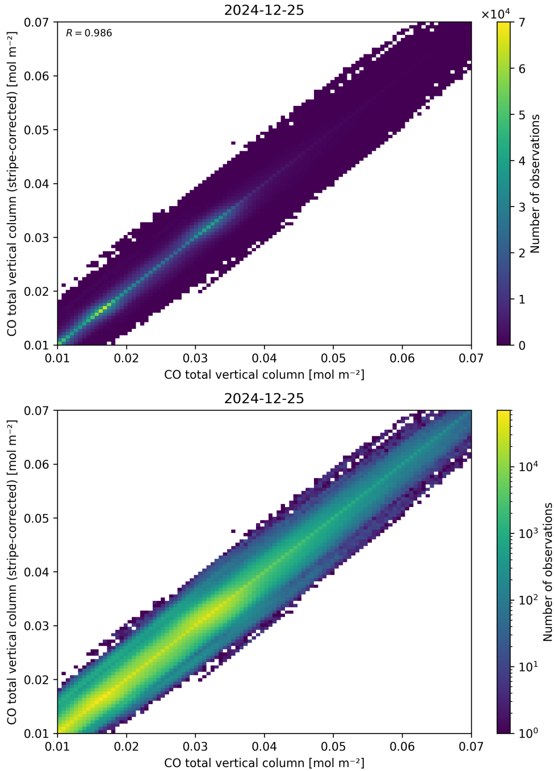
Figure 33: Scatter density plot of “CO total vertical column” against “CO total vertical column (stripe-corrected)” for 2024-12-24 to 2024-12-26.
