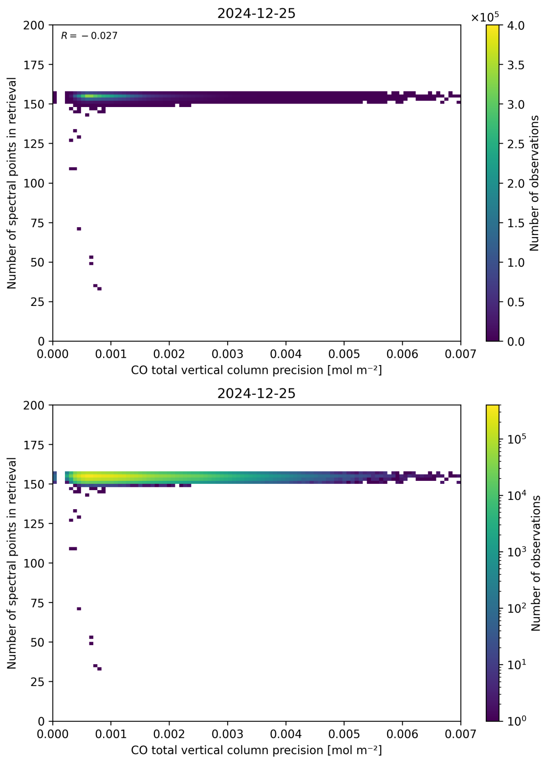
Figure 47: Scatter density plot of “CO total vertical column precision” against “Number of spectral points in retrieval” for 2024-12-24 to 2024-12-26.
