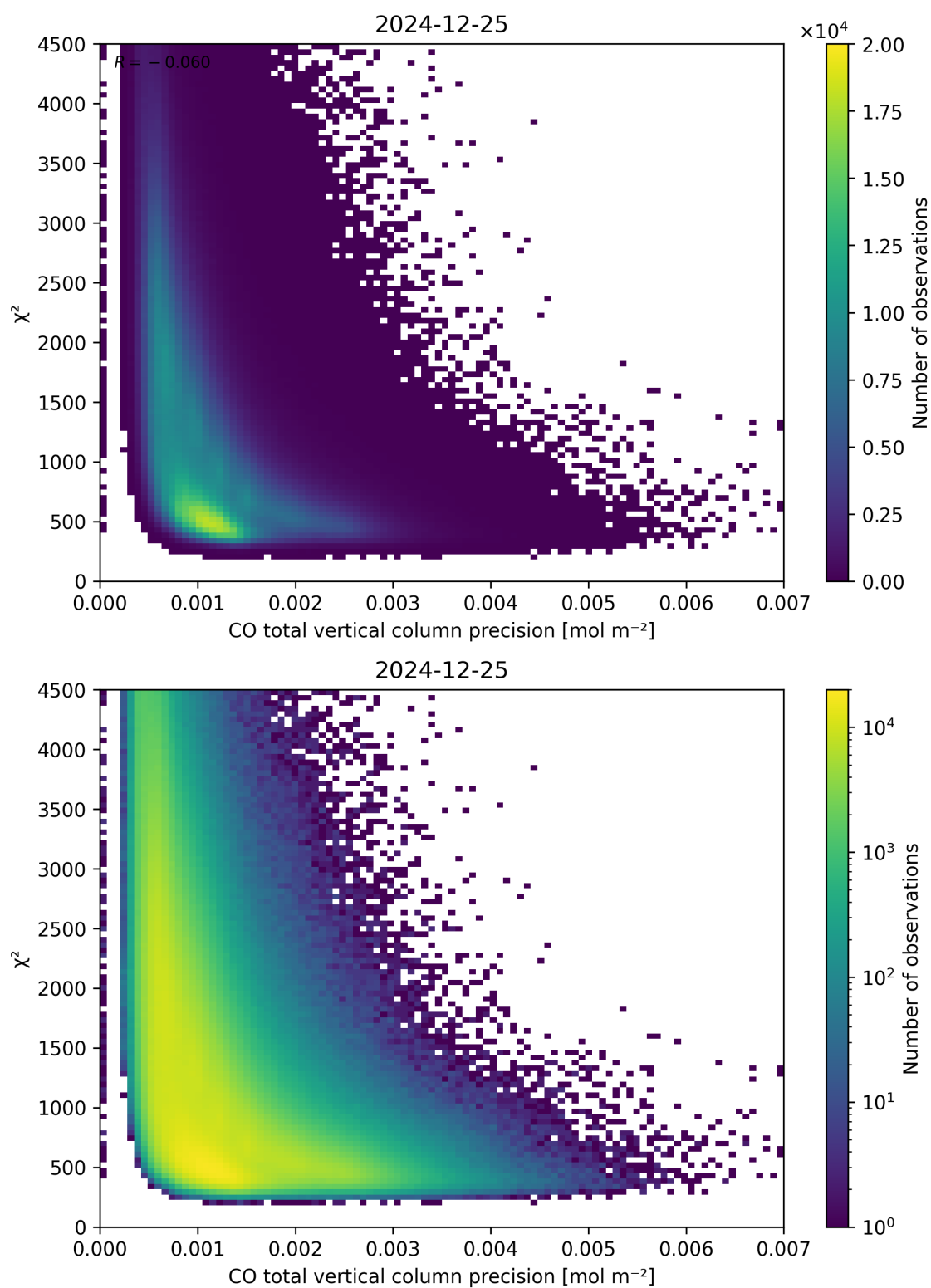
Figure 44: Scatter density plot of “CO total vertical column precision” against “ \chi^2 ” for 2024-12-24 to 2024-12-26.
