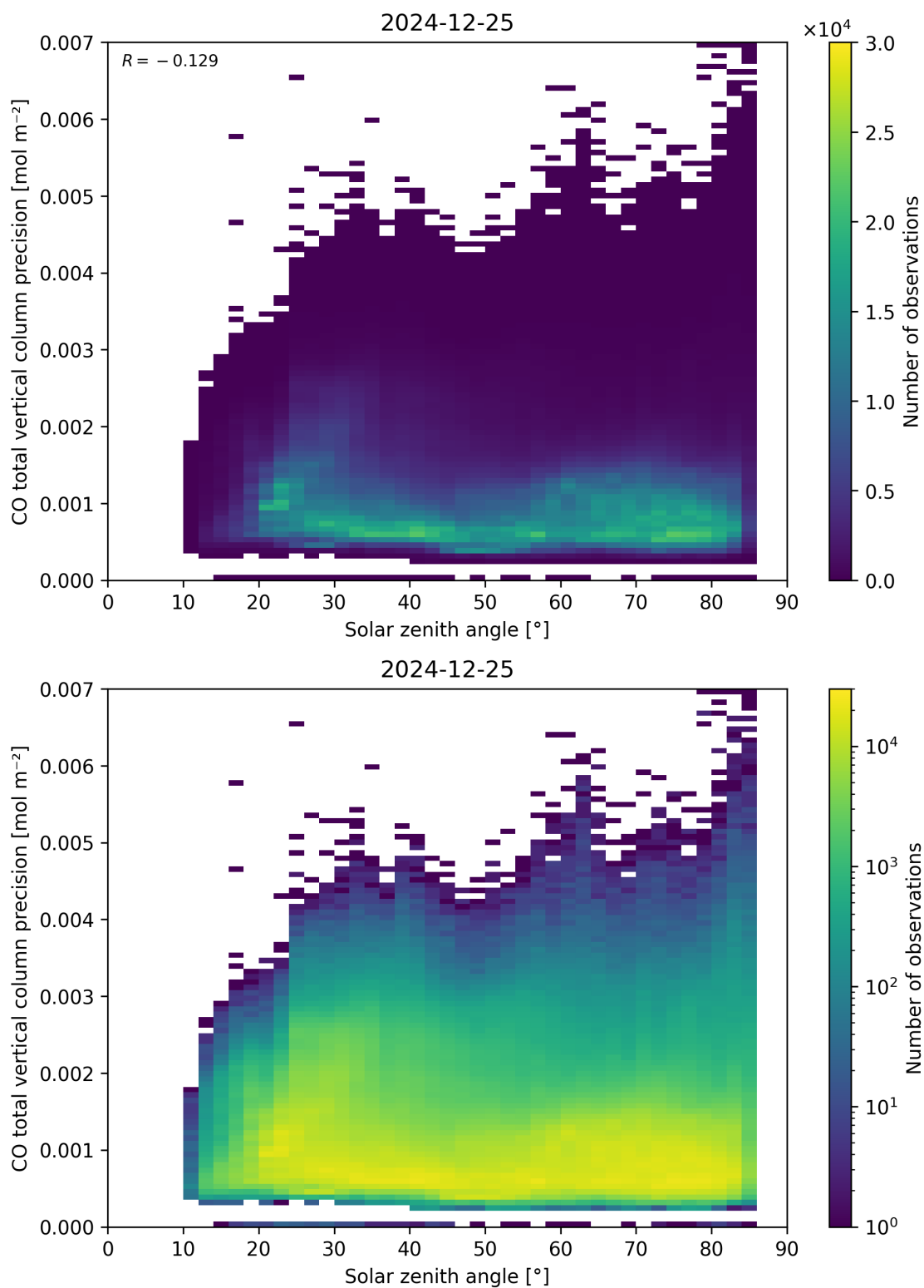
Figure 63: Scatter density plot of “Solar zenith angle” against “CO total vertical column precision” for 2024-12-24 to 2024-12-26.
