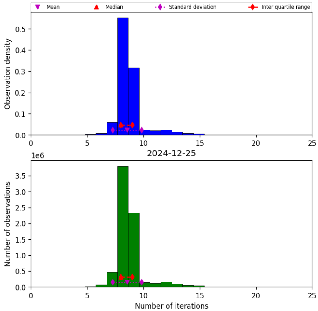
Figure 24: Histogram of “Number of iterations” for 2024-12-24 to 2024-12-26
