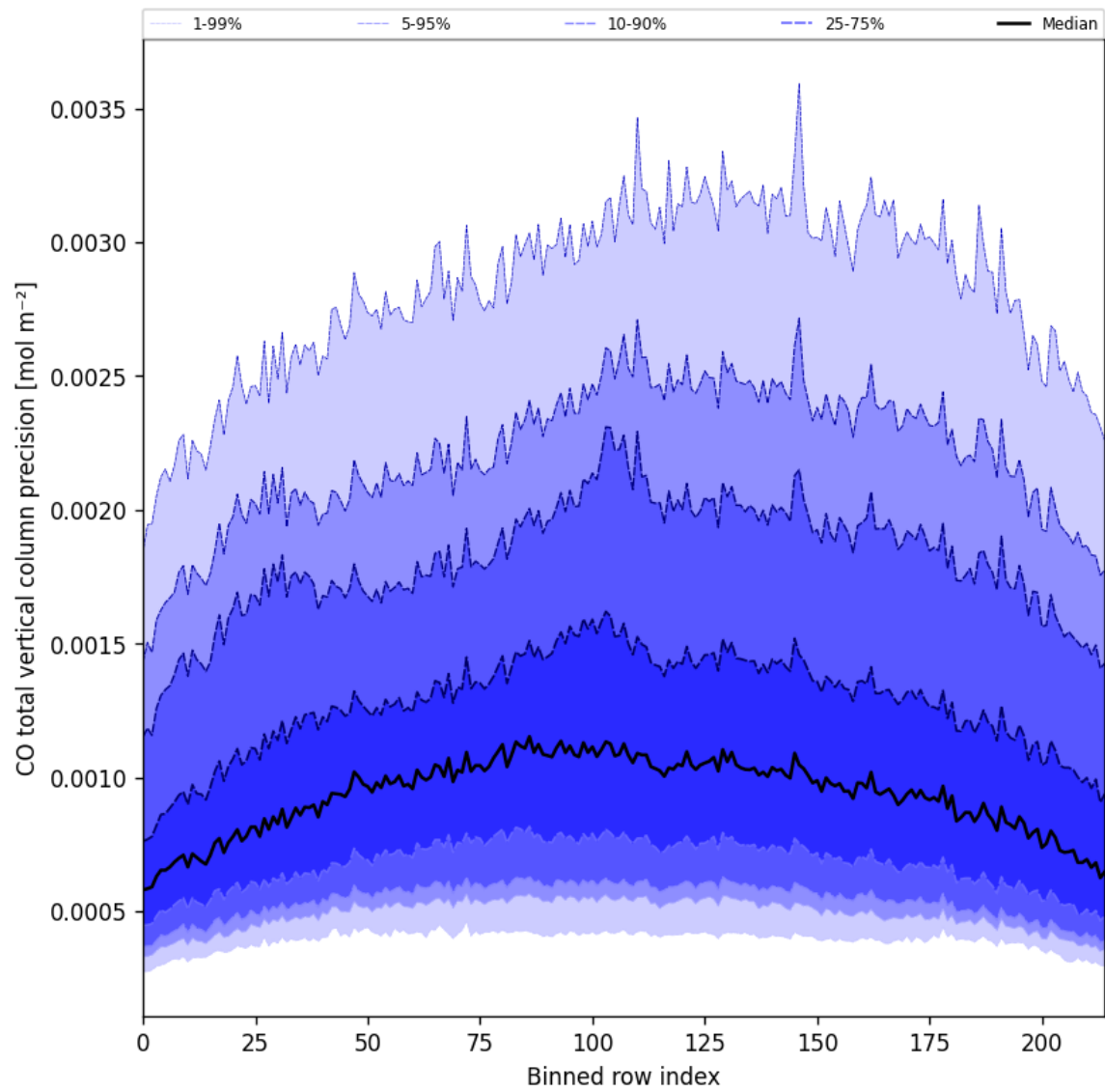
Figure 28: Along track statistics of “CO total vertical column precision” for 2024-12-24 to 2024-12-26
