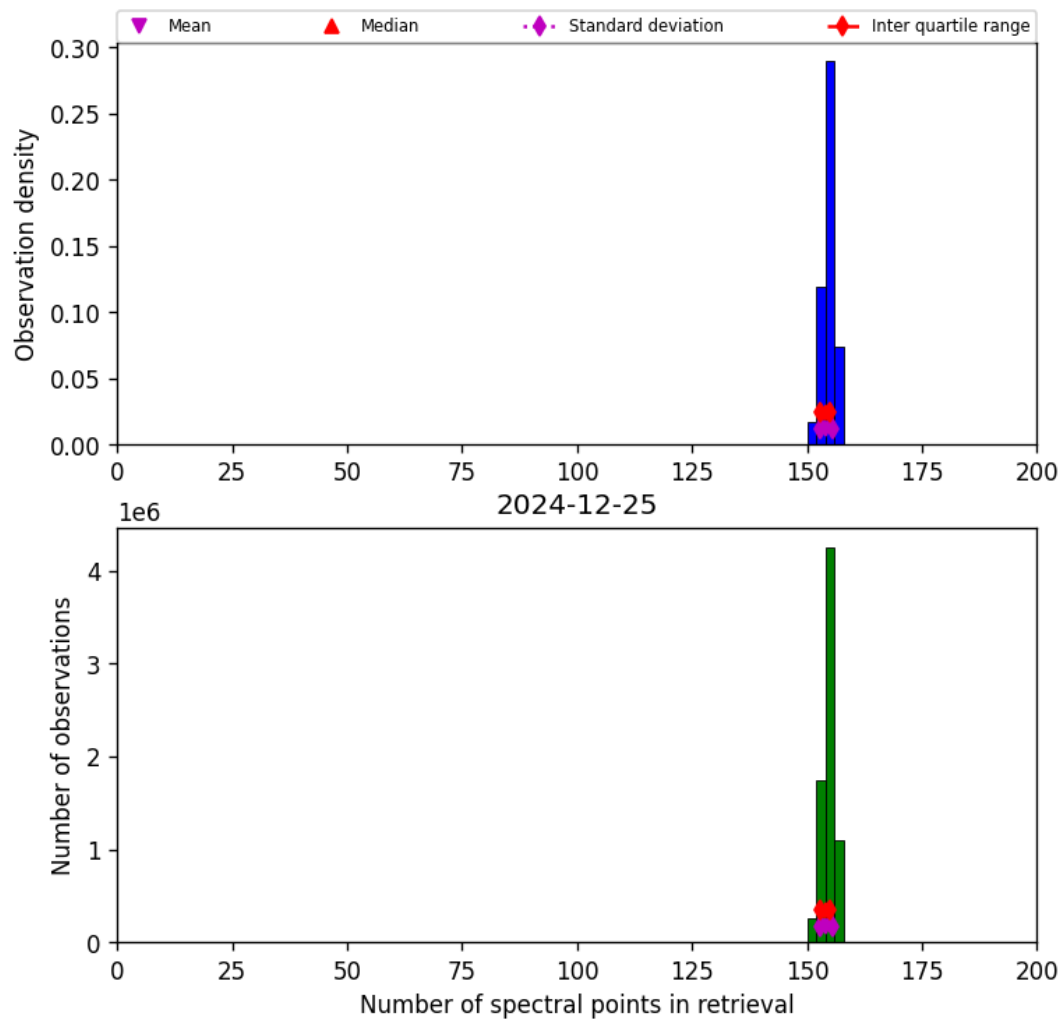
Figure 21: Histogram of “Number of spectral points in retrieval” for 2024-12-24 to 2024-12-26
