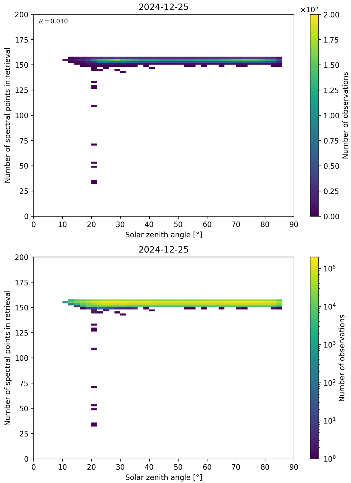
Figure 68: Scatter density plot of “Solar zenith angle” against “Number of spectral points in retrieval” for 2024-12-24 to 2024-12-26.
