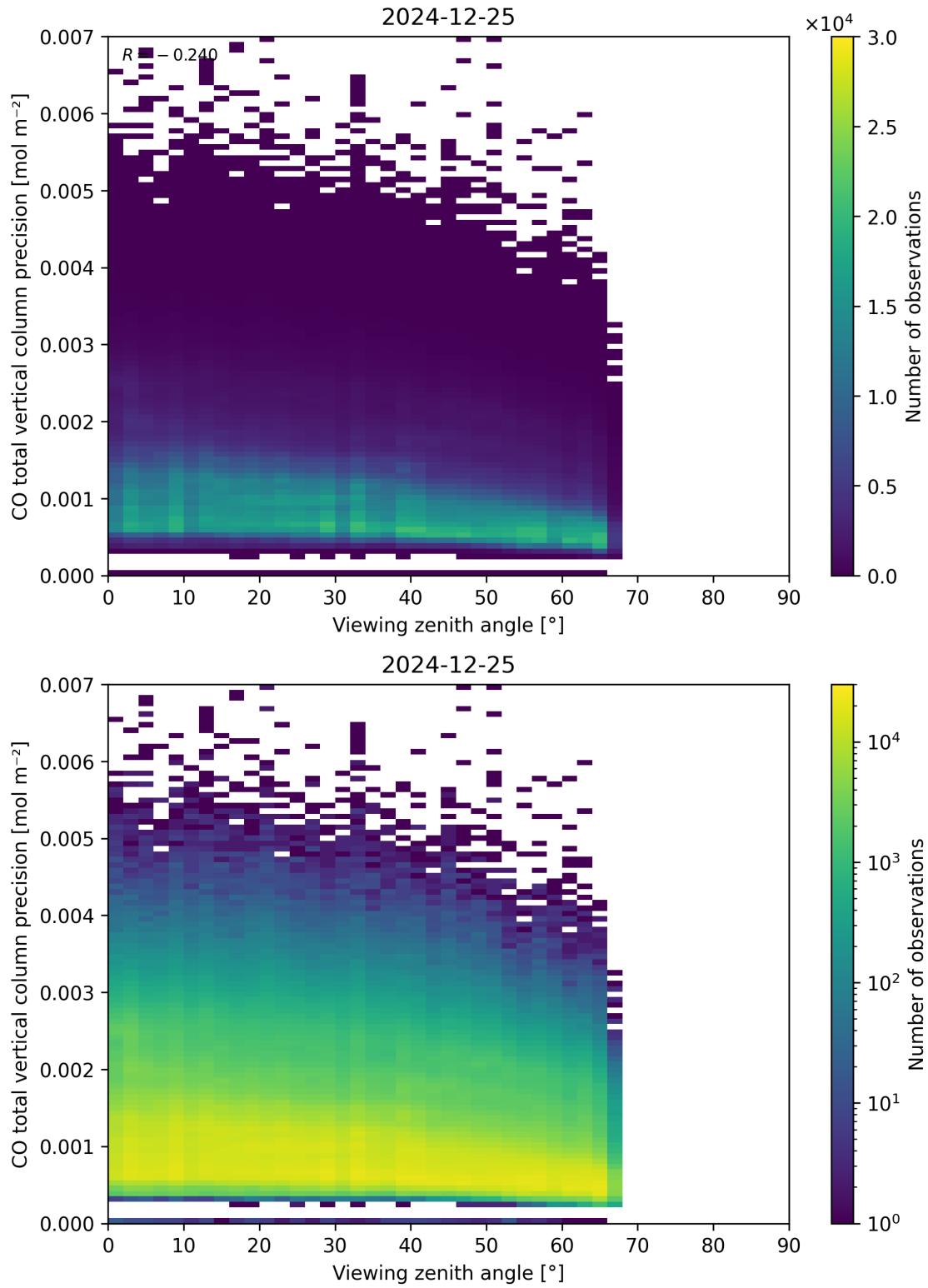
Figure 71: Scatter density plot of “Viewing zenith angle” against “CO total vertical column precision” for 2024-12-24 to 2024-12-26.
