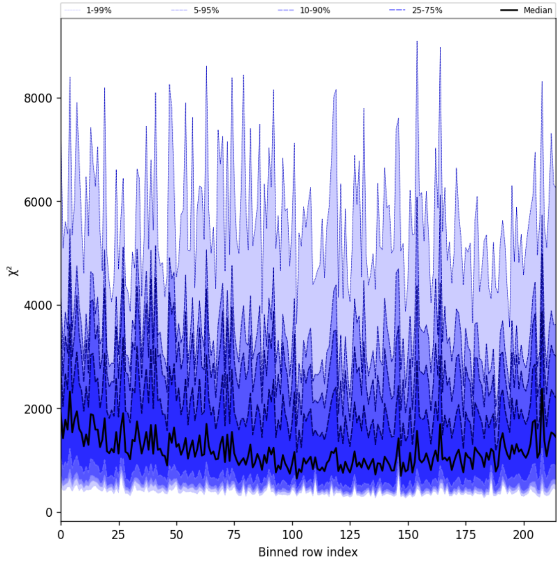
Figure 30: Along track statistics of “ \chi^2 ” for 2024-12-24 to 2024-12-26
