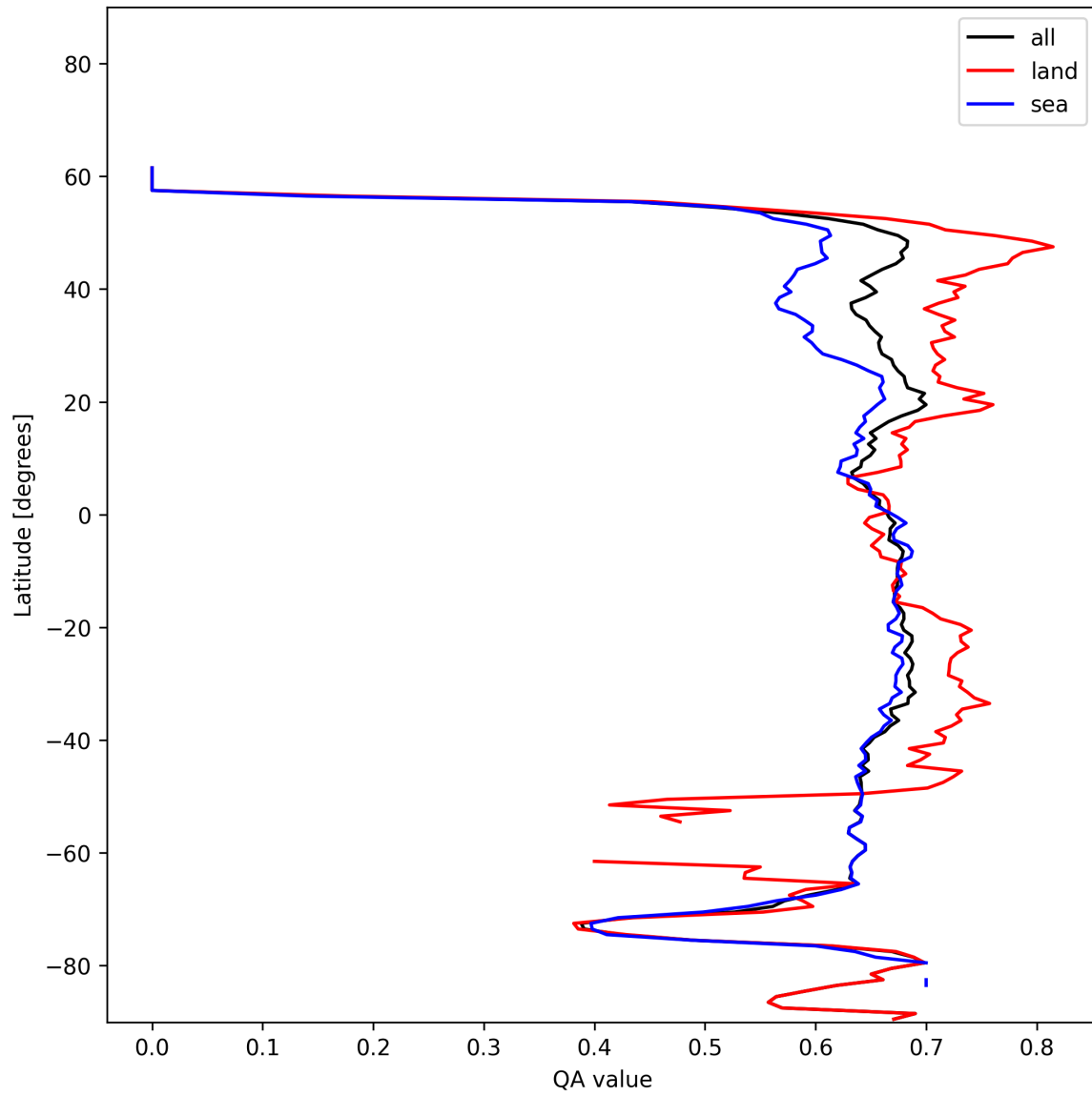
Figure 9: Zonal average of “QA value” for 2024-12-24 to 2024-12-26.
