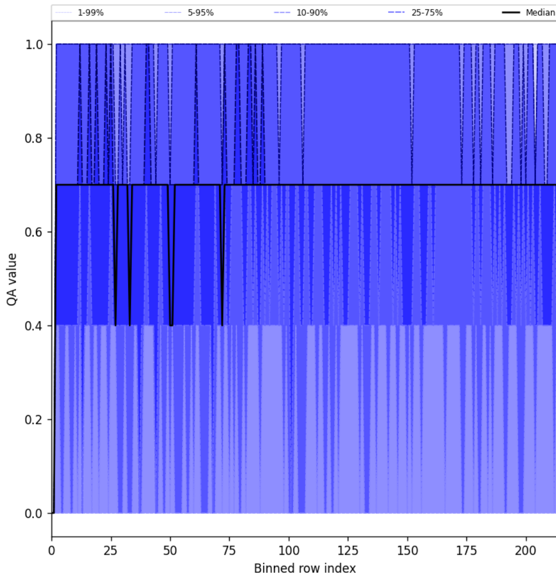
Figure 25: Along track statistics of “QA value” for 2024-12-24 to 2024-12-26
