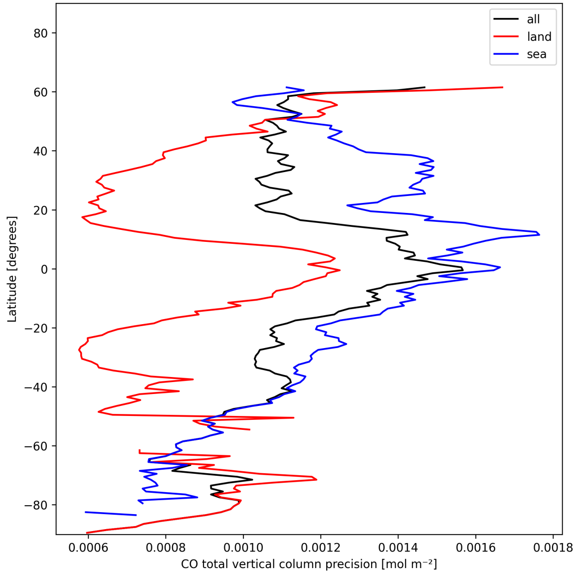
Figure 12: Zonal average of “CO total vertical column precision” for 2024-12-24 to 2024-12-26.
