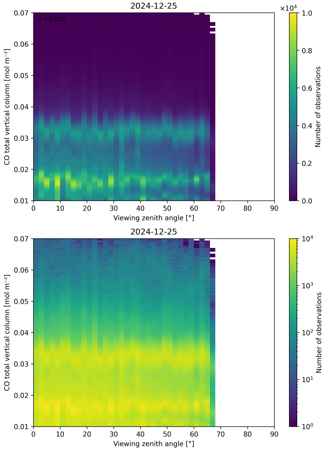
Figure 69: Scatter density plot of “Viewing zenith angle” against “CO total vertical column” for 2024-12-24 to 2024-12-26.
