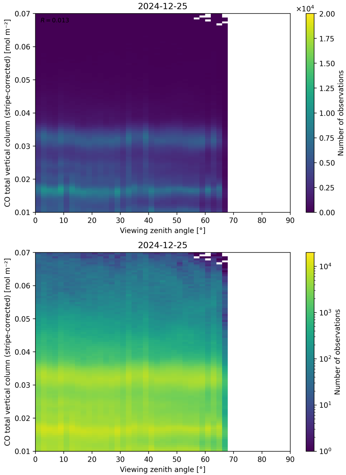
Figure 70: Scatter density plot of “Viewing zenith angle” against “CO total vertical column (stripe-corrected)” for 2024-12-24 to 2024-12-26.
