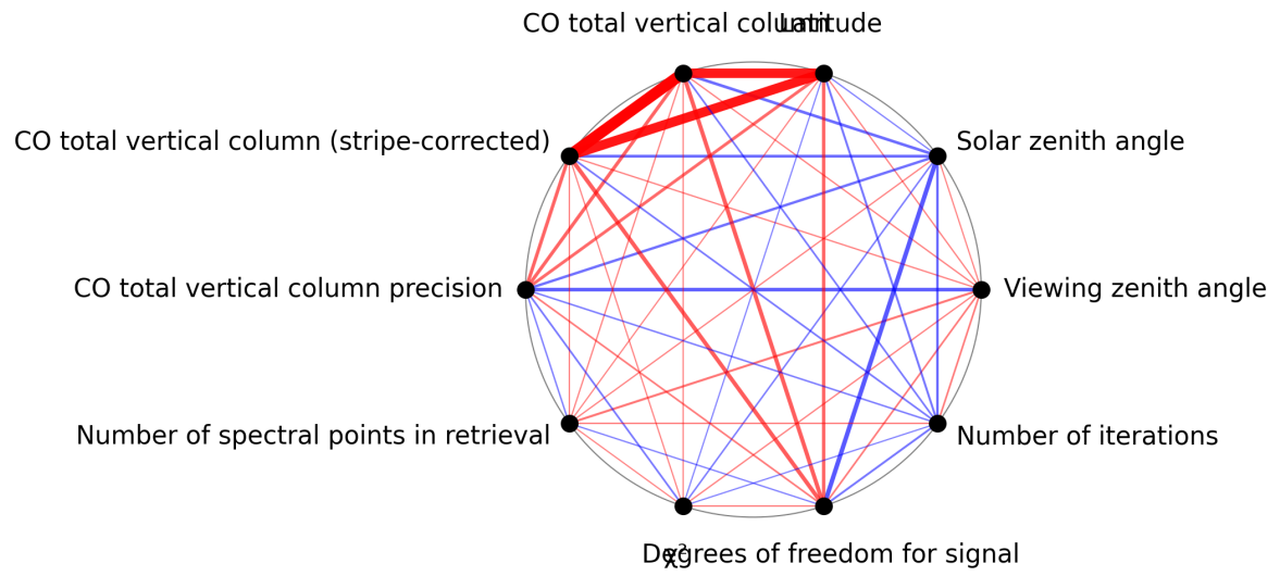
Figure 1: Map of correlation graph for 2024-12-24 to 2024-12-26.
