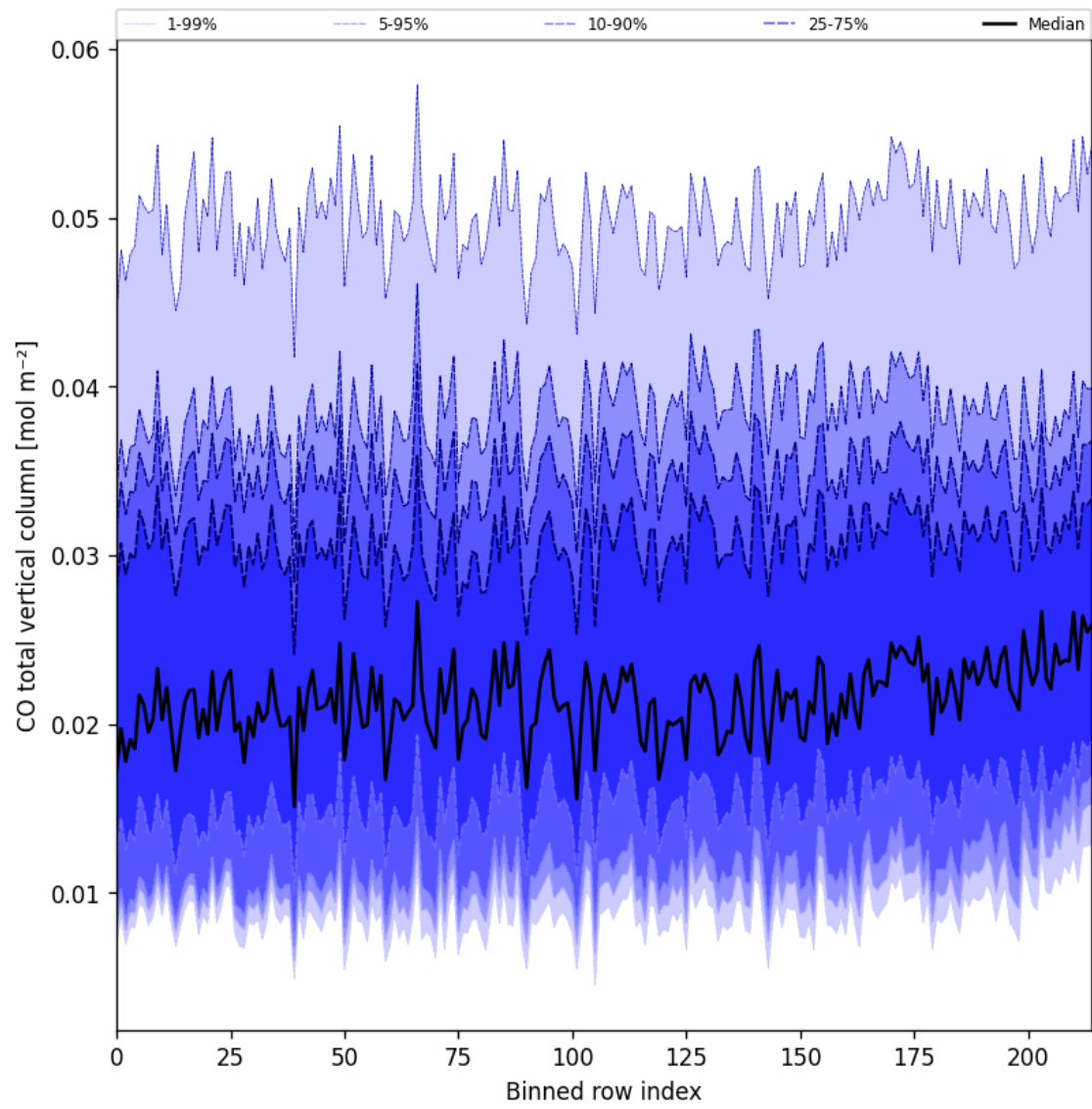
Figure 26: Along track statistics of “CO total vertical column” for 2024-12-24 to 2024-12-26
