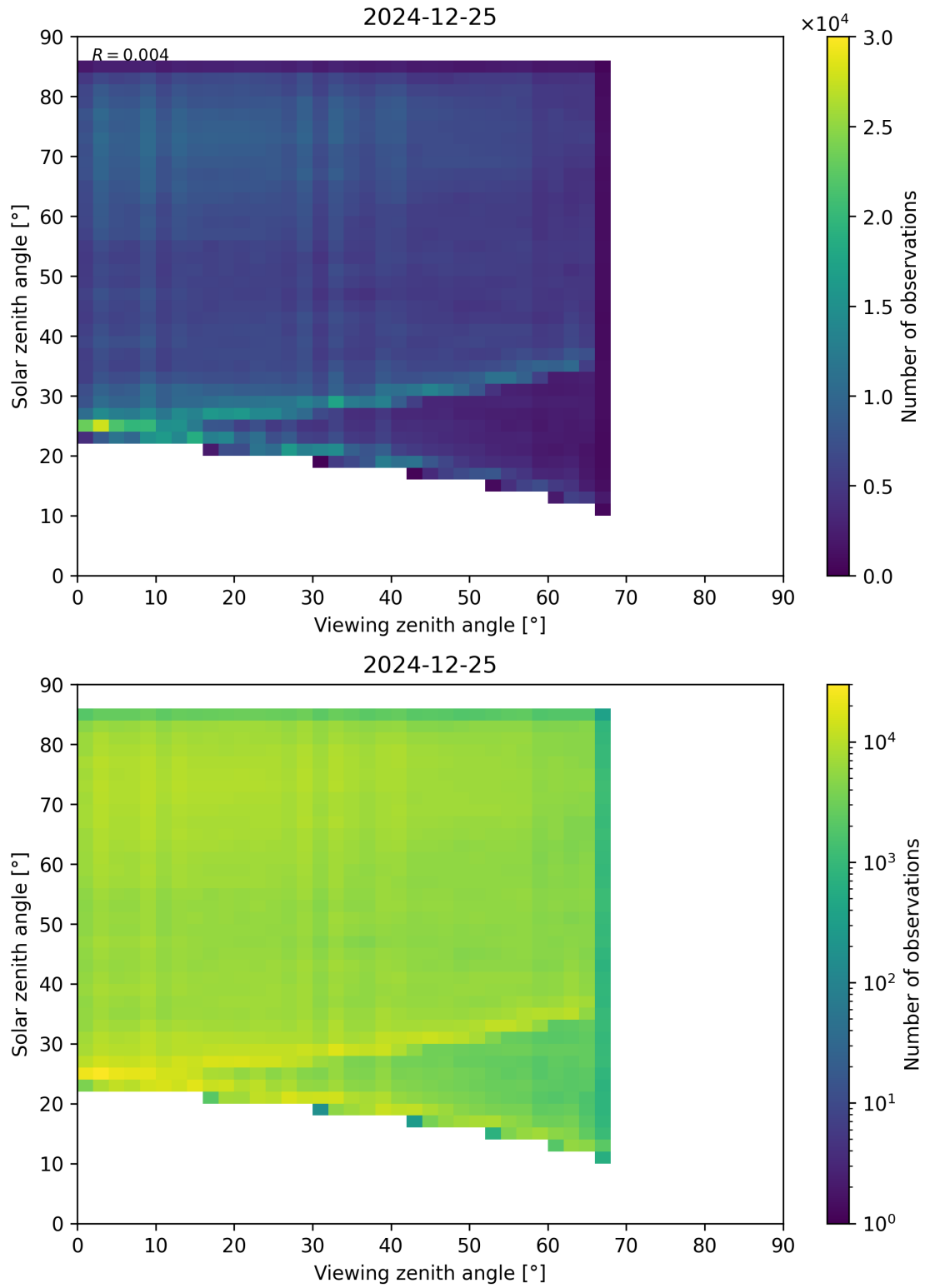
Figure 77: Scatter density plot of “Viewing zenith angle” against “Solar zenith angle” for 2024-12-24 to 2024-12-26.
