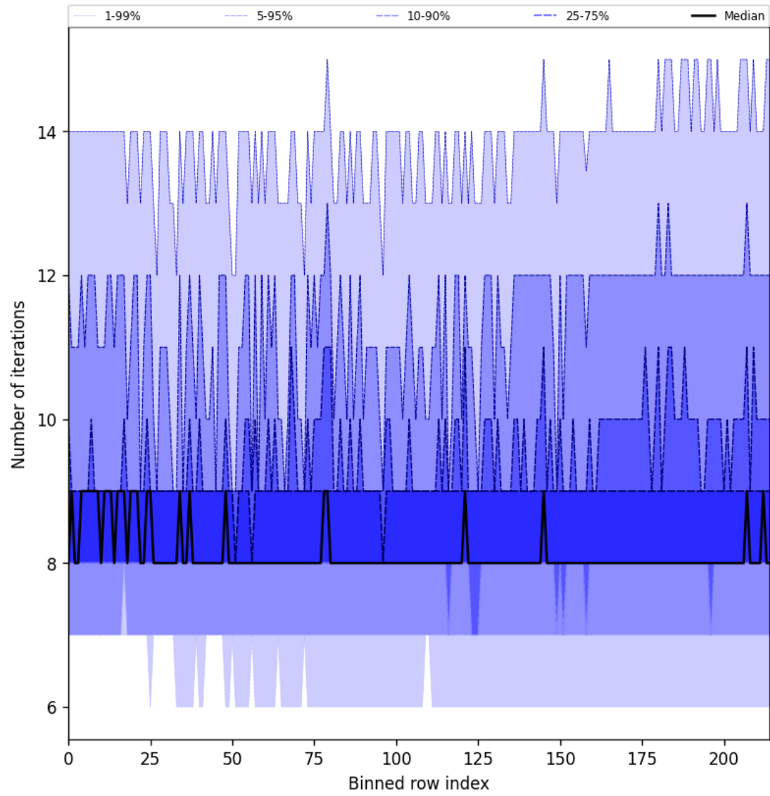
Figure 32: Along track statistics of “Number of iterations” for 2024-12-24 to 2024-12-26
