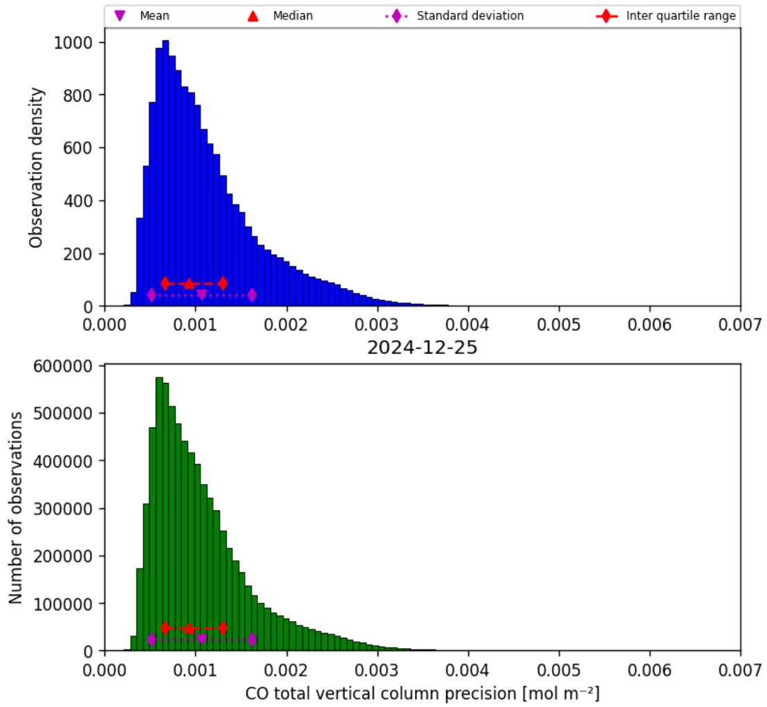
Figure 20: Histogram of “CO total vertical column precision” for 2024-12-24 to 2024-12-26
