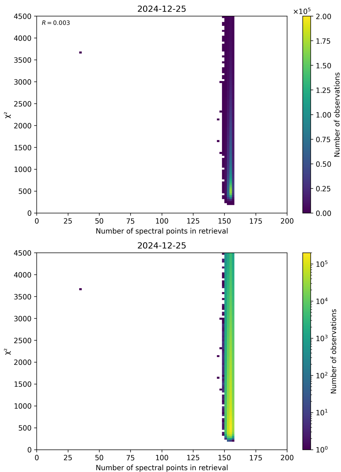
Figure 58: Scatter density plot of “Number of spectral points in retrieval” against “ \chi^2 ” for 2024-12-24 to 2024-12-26.
