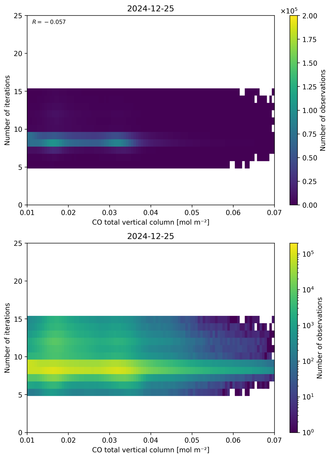
Figure 42: Scatter density plot of “CO total vertical column” against “Number of iterations” for 2024-12-24 to 2024-12-26.
