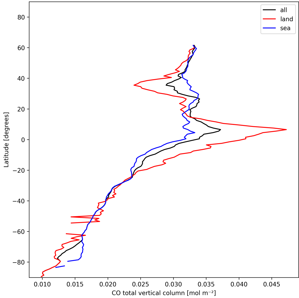
Figure 10: Zonal average of “CO total vertical column” for 2024-12-24 to 2024-12-26.
