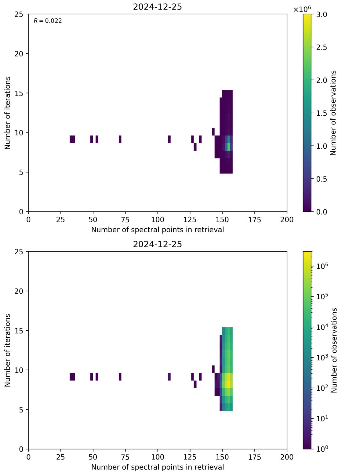
Figure 60: Scatter density plot of “Number of spectral points in retrieval” against “Number of iterations” for 2024-12-24 to 2024-12-26.
