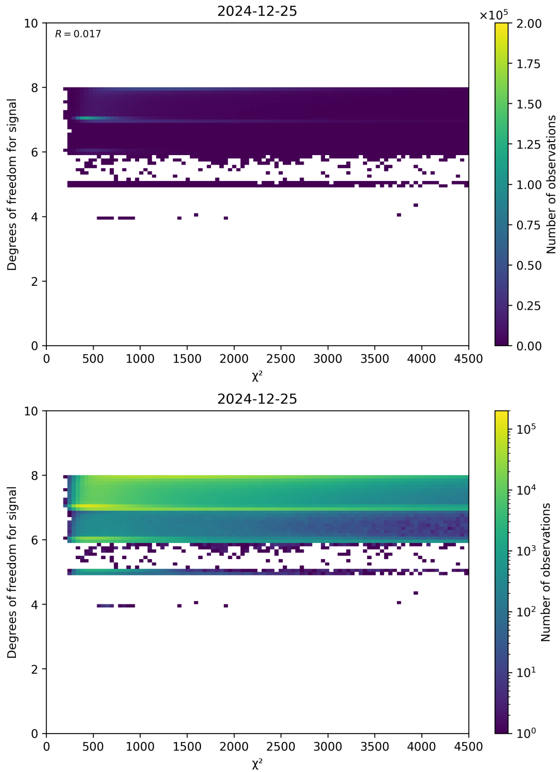
Figure 48: Scatter density plot of “ \chi^2 ” against “Degrees of freedom for signal” for 2024-12-24 to 2024-12-26.
