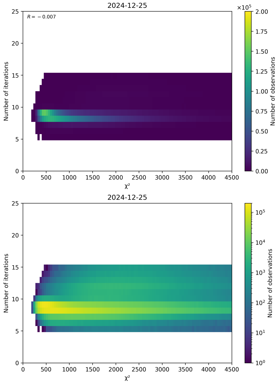
Figure 49: Scatter density plot of “ \chi^2 ” against “Number of iterations” for 2024-12-24 to 2024-12-26.
