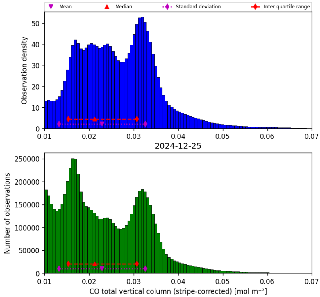
Figure 19: Histogram of “CO total vertical column (stripe-corrected)” for 2024-12-24 to 2024-12-26
