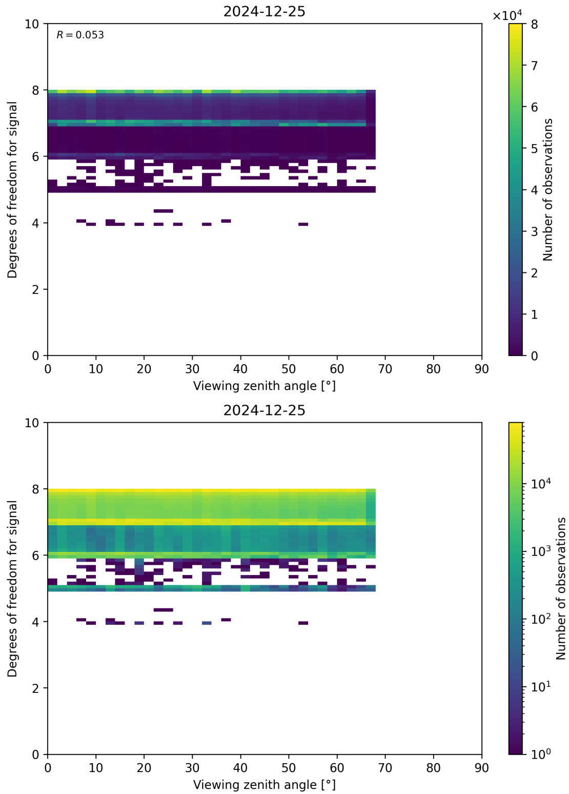
Figure 73: Scatter density plot of “Viewing zenith angle” against “Degrees of freedom for signal” for 2024-12-24 to 2024-12-26.
