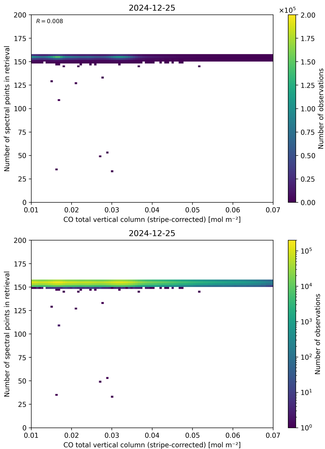
Figure 40: Scatter density plot of “CO total vertical column (stripe-corrected)” against “Number of spectral points in retrieval” for 2024-12-24 to 2024-12-26.
