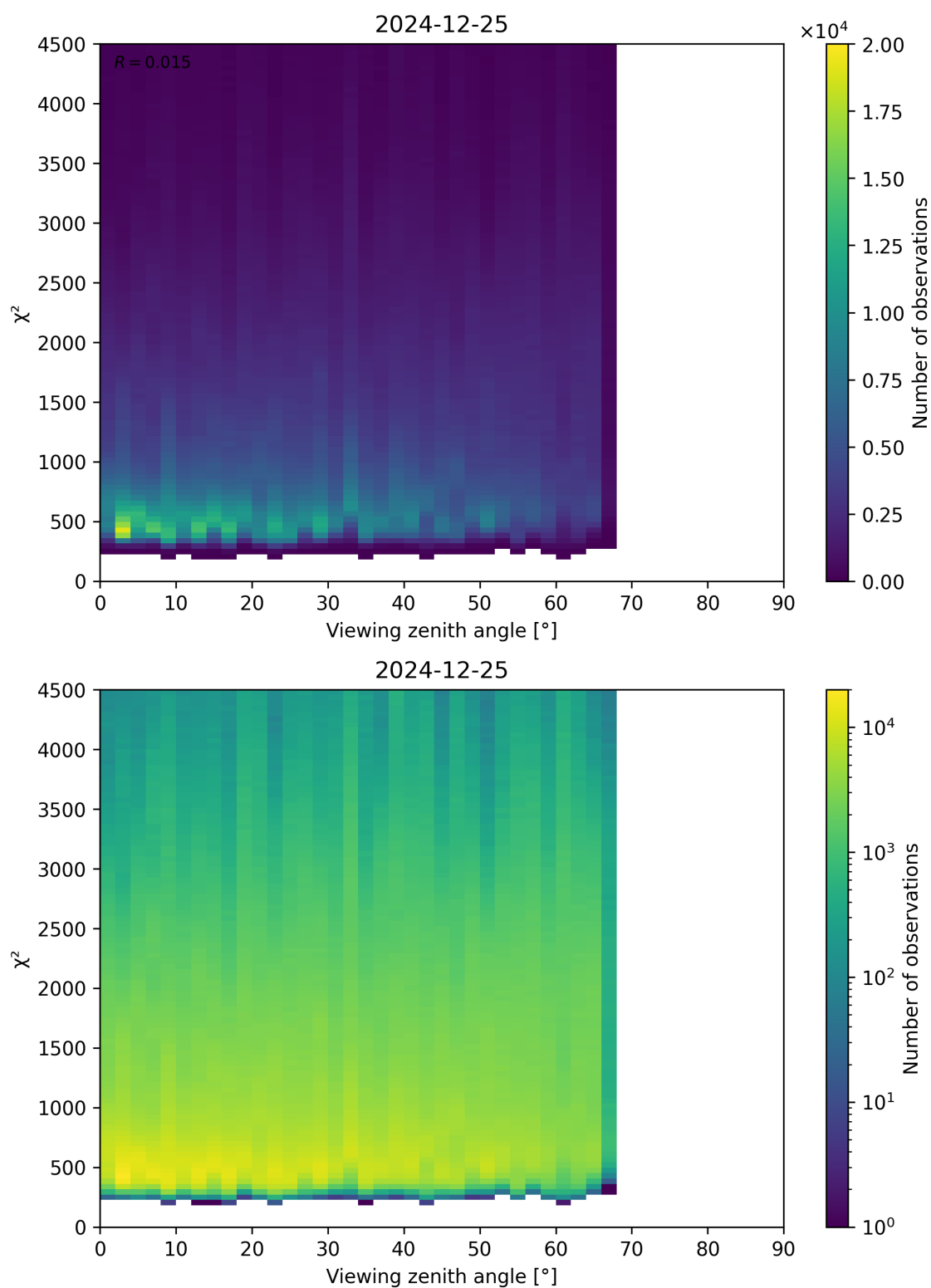
Figure 72: Scatter density plot of “Viewing zenith angle” against “ \chi^2 ” for 2024-12-24 to 2024-12-26.
