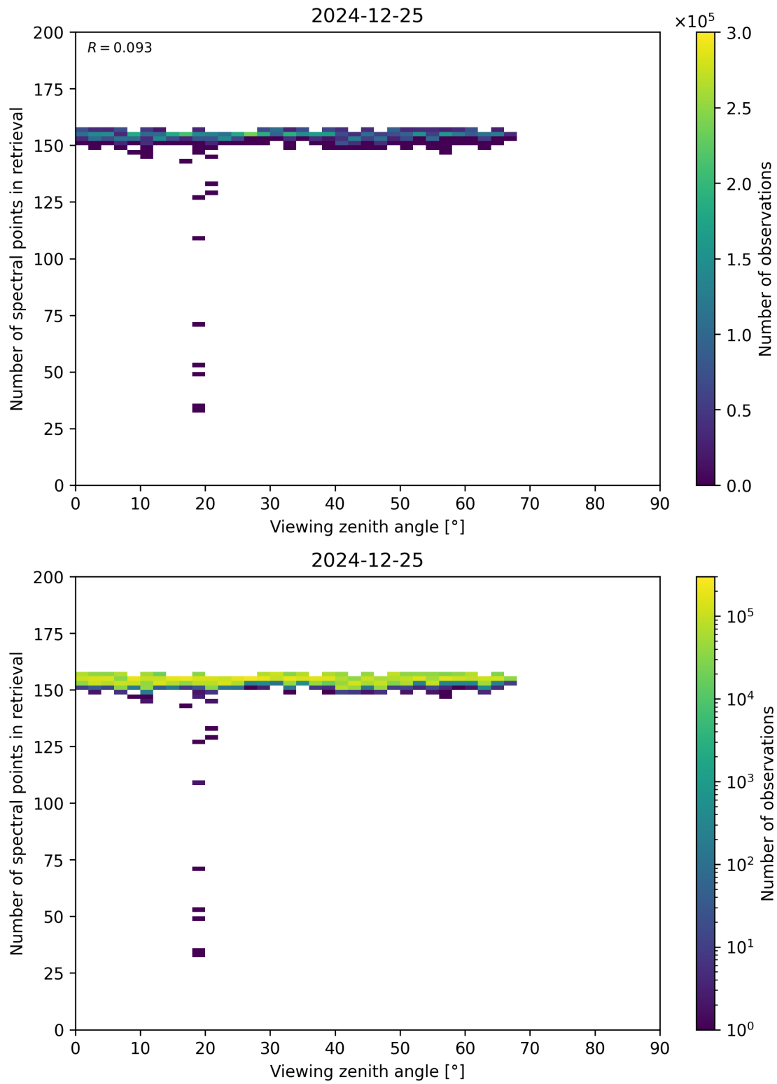
Figure 76: Scatter density plot of “Viewing zenith angle” against “Number of spectral points in retrieval” for 2024-12-24 to 2024-12-26.
