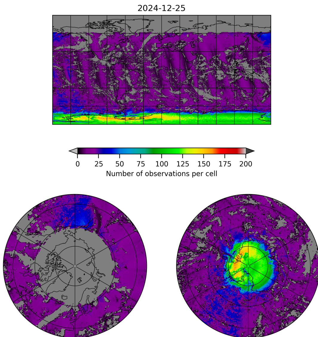
Figure 8: Map of the number of observations for 2024-12-24 to 2024-12-26
