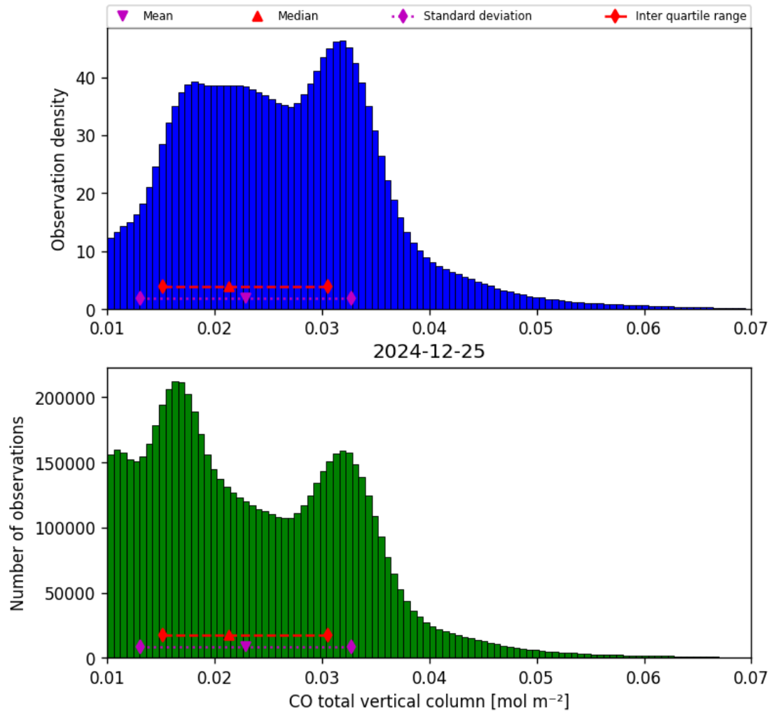
Figure 18: Histogram of “CO total vertical column” for 2024-12-24 to 2024-12-26
