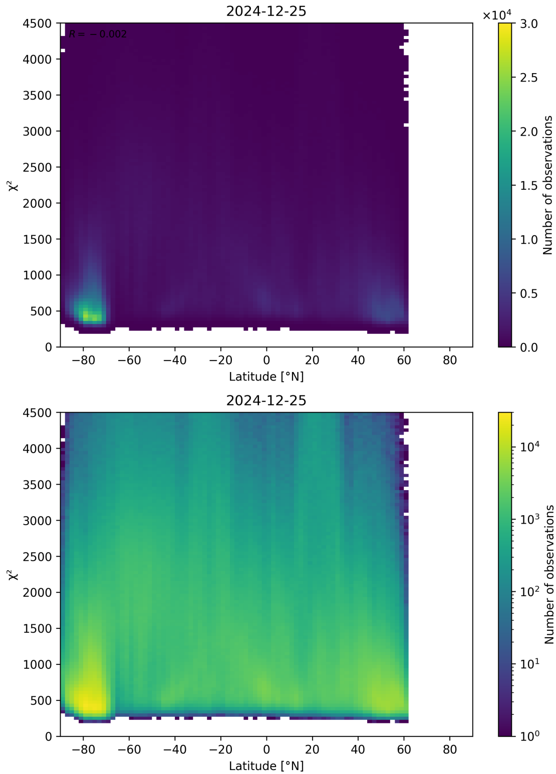
Figure 54: Scatter density plot of “Latitude” against “ \chi^2 ” for 2024-12-24 to 2024-12-26.
