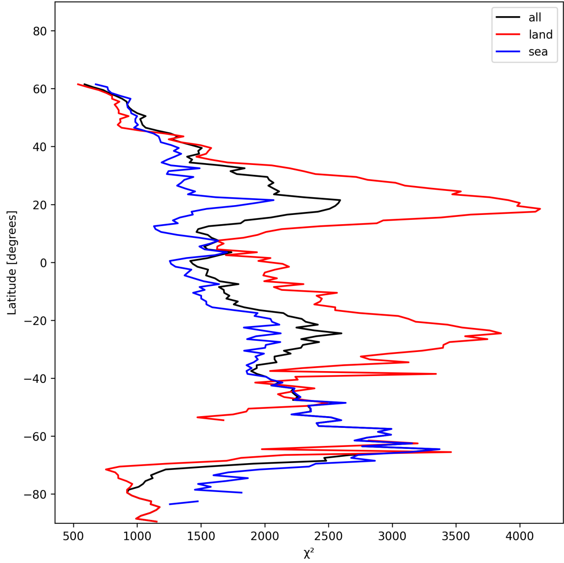
Figure 14: Zonal average of “ \chi^2 ” for 2024-12-24 to 2024-12-26.
