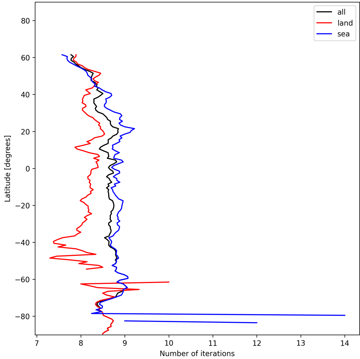
Figure 16: Zonal average of “Number of iterations” for 2024-12-24 to 2024-12-26.
