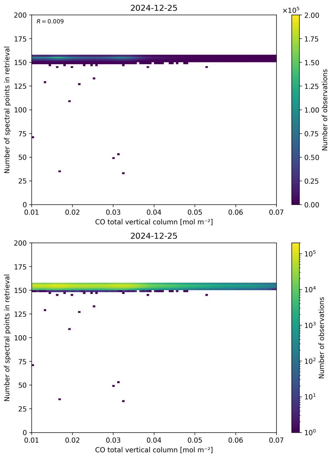
Figure 43: Scatter density plot of “CO total vertical column” against “Number of spectral points in retrieval” for 2024-12-24 to 2024-12-26.
