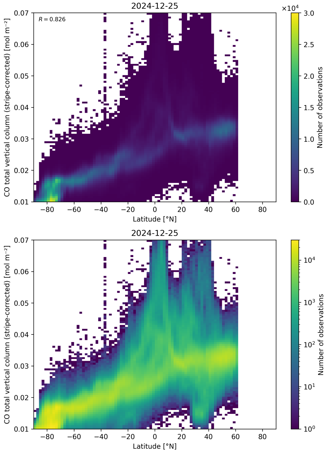
Figure 52: Scatter density plot of “Latitude” against “CO total vertical column (stripe-corrected)” for 2024-12-24 to 2024-12-26.
