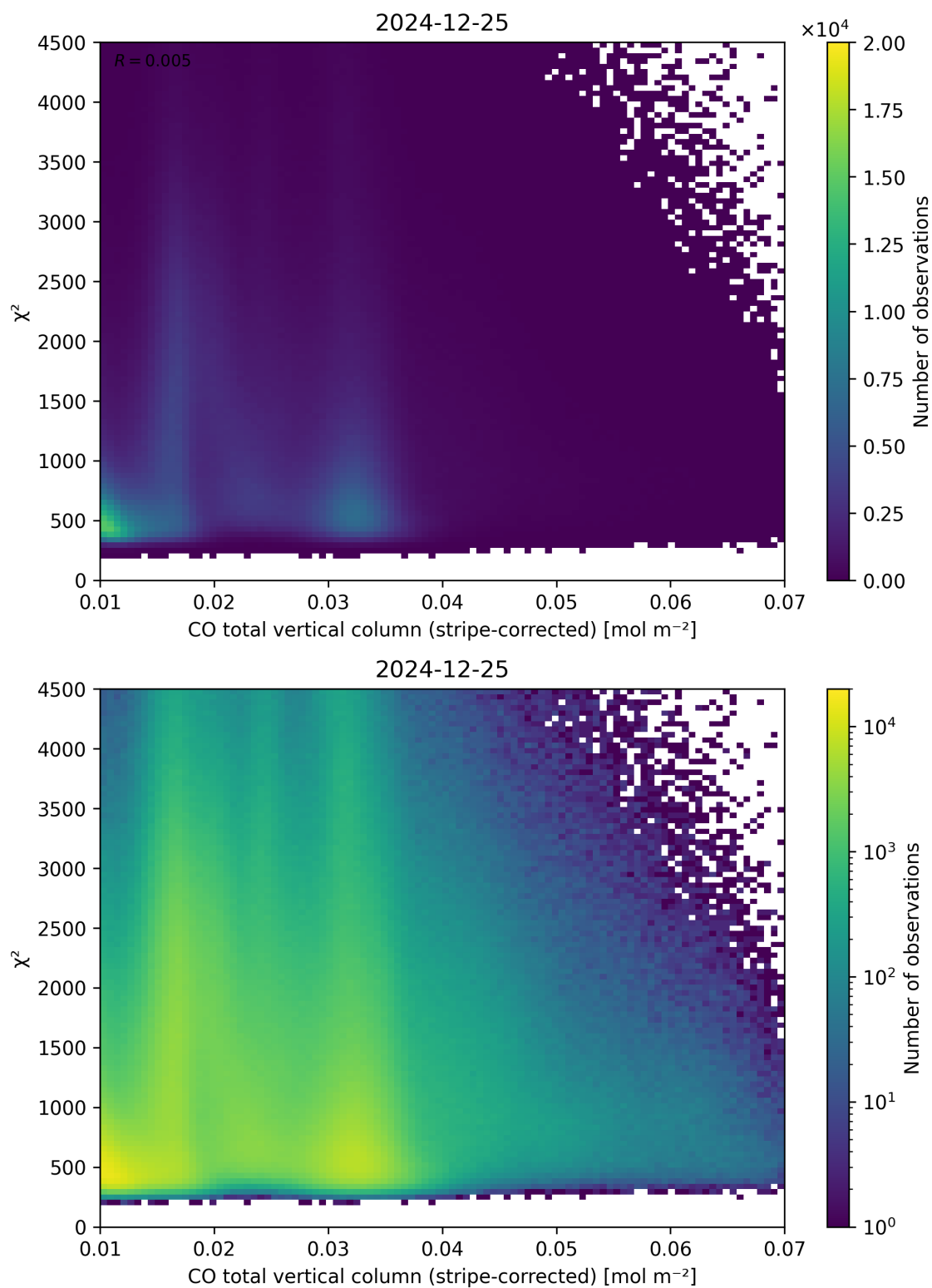
Figure 37: Scatter density plot of “CO total vertical column (stripe-corrected)” against “ \chi^2 ” for 2024-12-24 to 2024-12-26.
