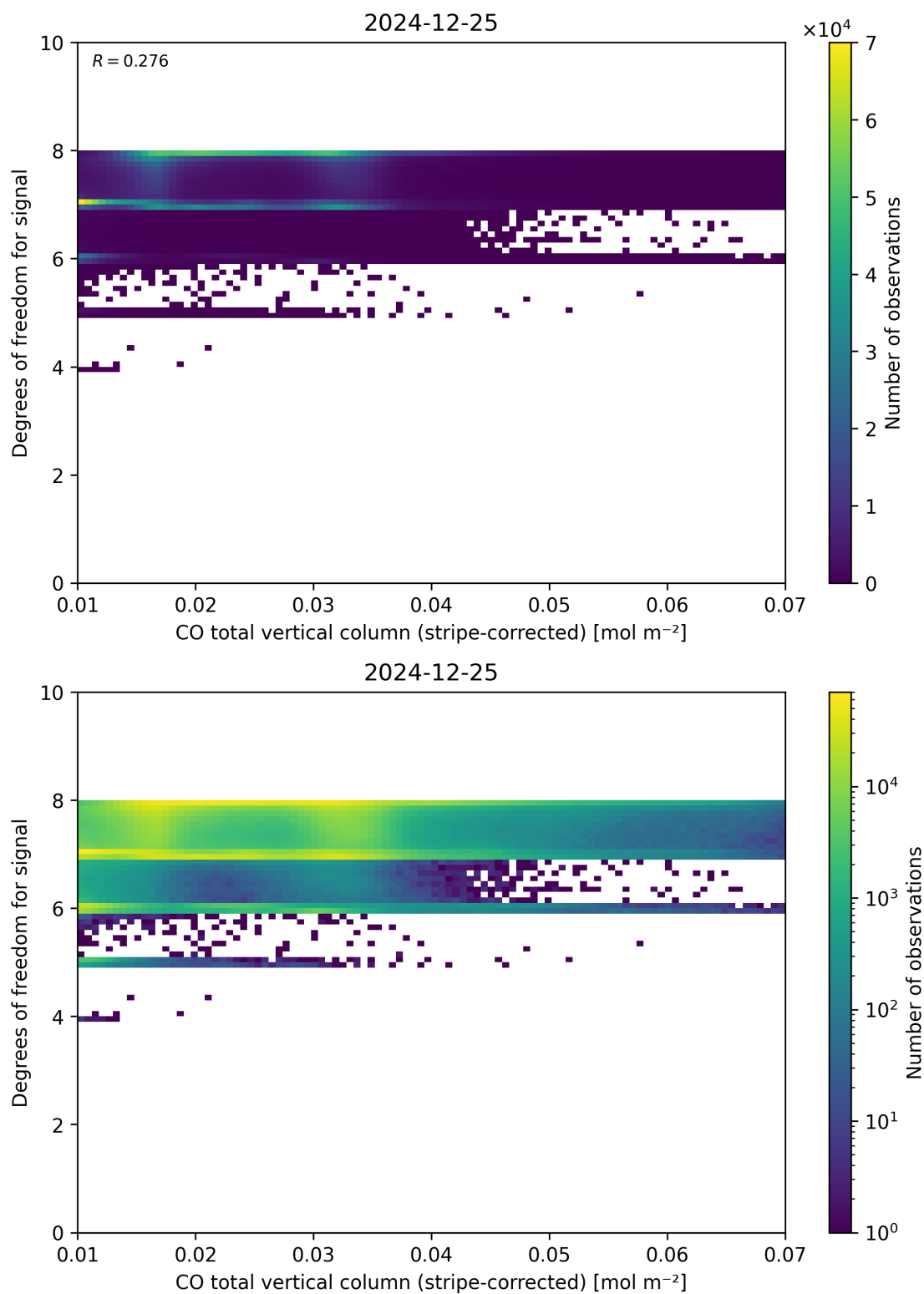
Figure 38: Scatter density plot of “CO total vertical column (stripe-corrected)” against “Degrees of freedom for signal” for 2024-12-24 to 2024-12-26.
