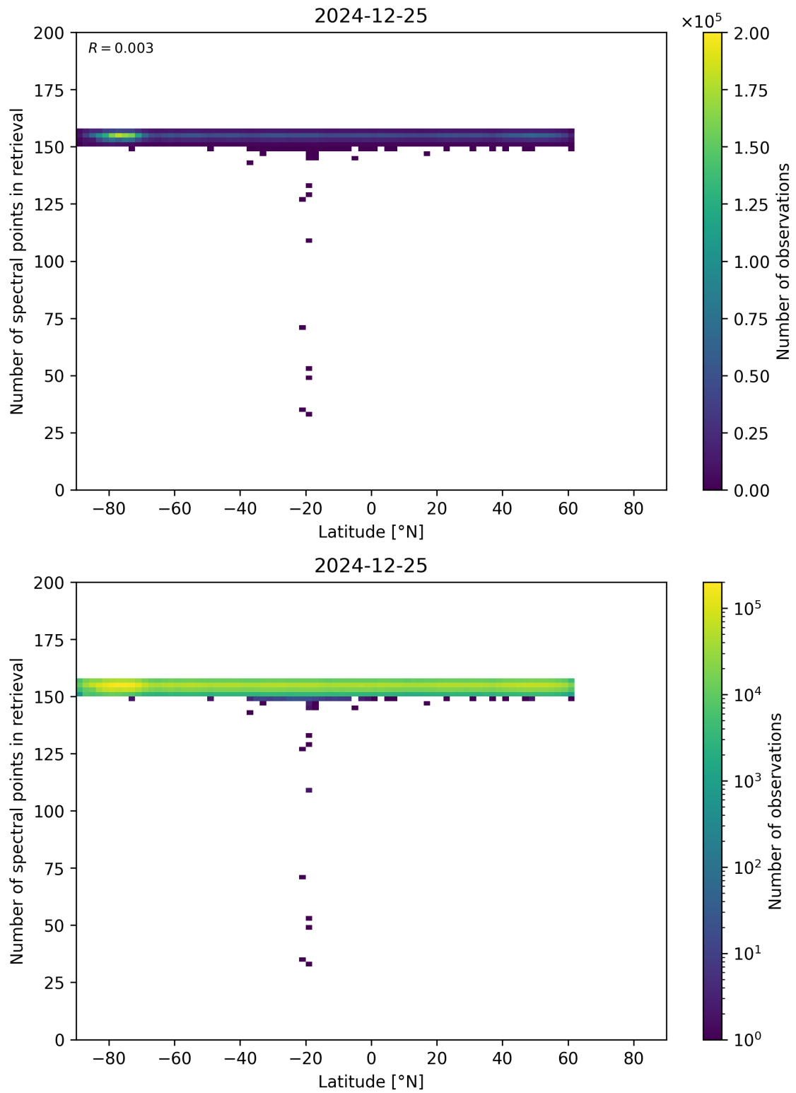
Figure 57: Scatter density plot of “Latitude” against “Number of spectral points in retrieval” for 2024-12-24 to 2024-12-26.
