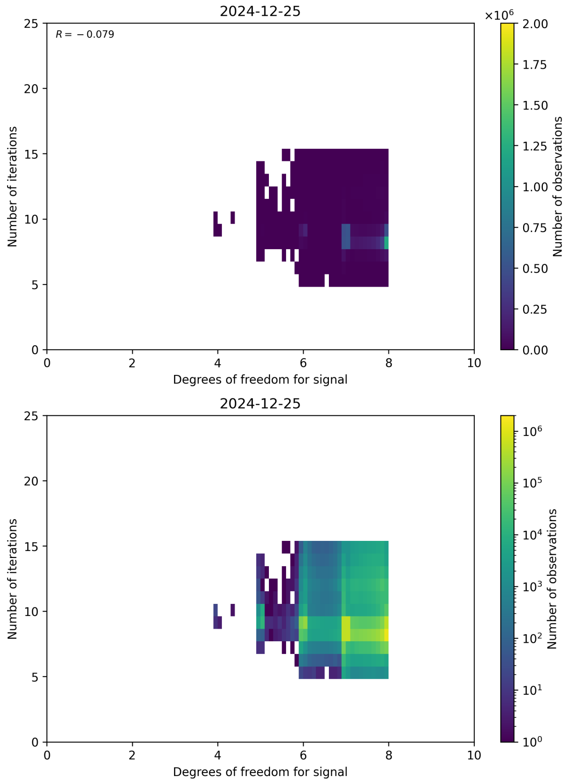
Figure 50: Scatter density plot of “Degrees of freedom for signal” against “Number of iterations” for 2024-12-24 to 2024-12-26.
