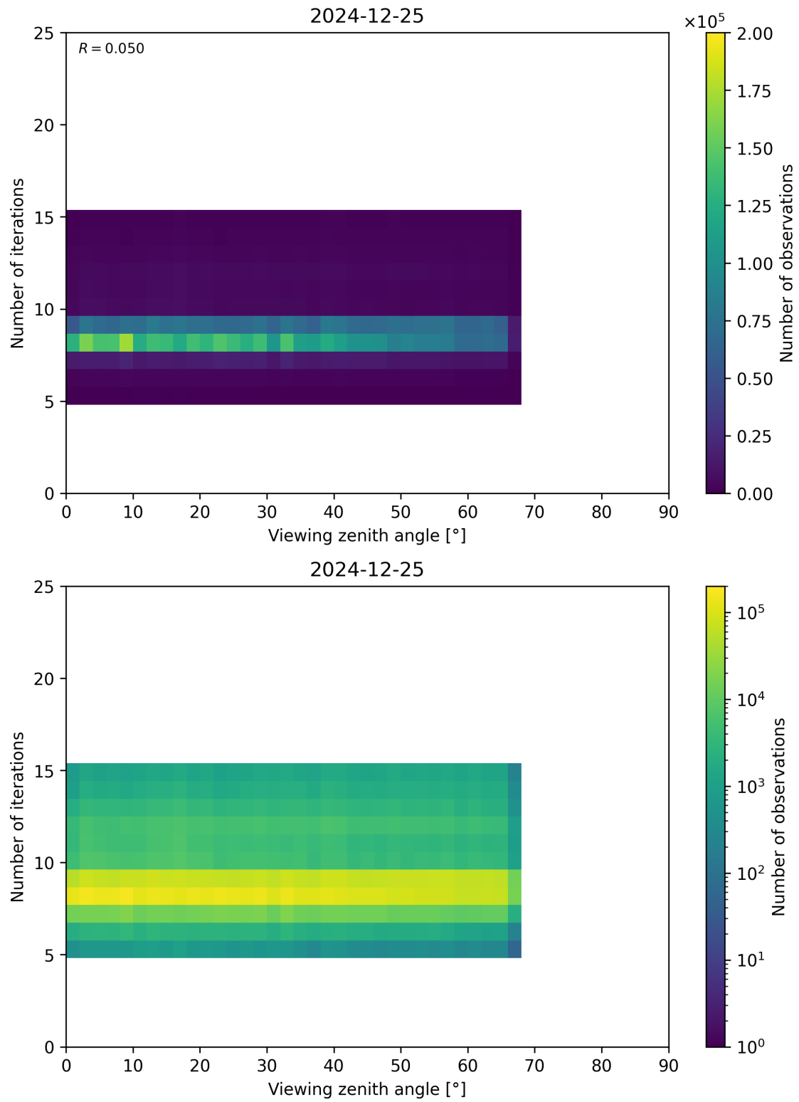
Figure 75: Scatter density plot of “Viewing zenith angle” against “Number of iterations” for 2024-12-24 to 2024-12-26.
