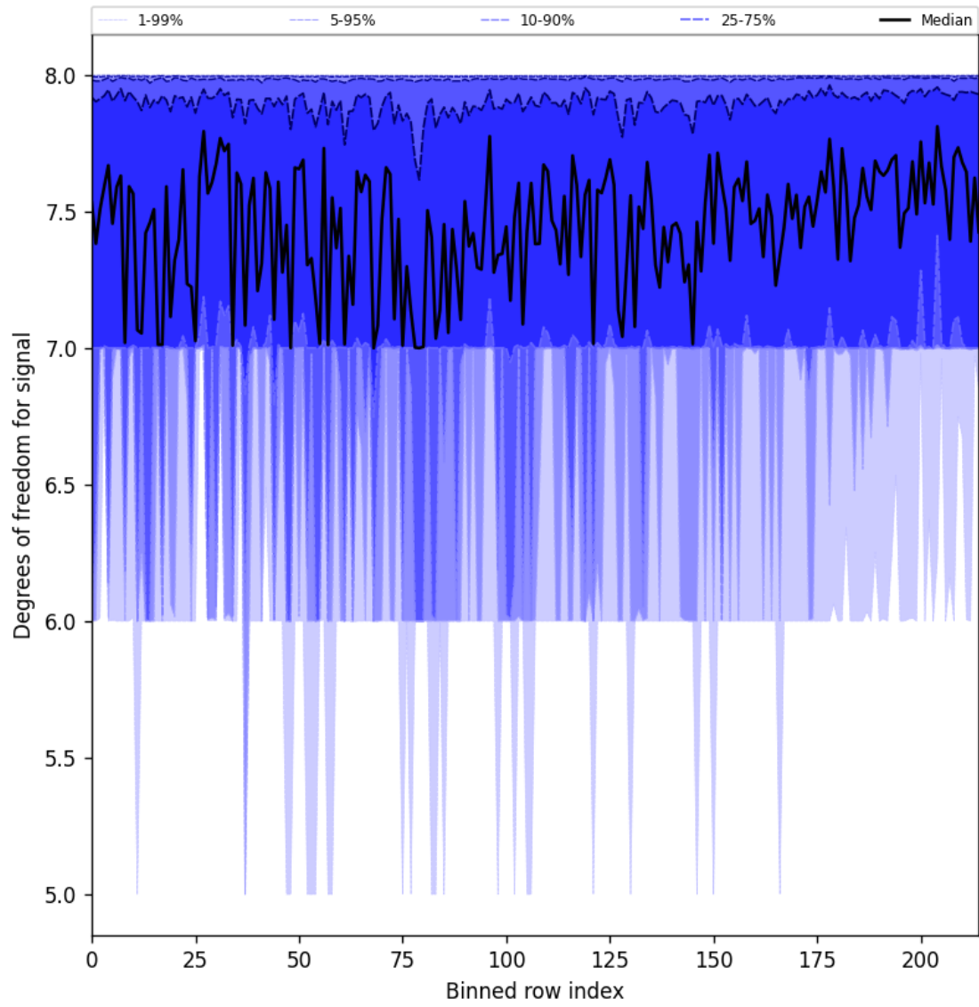
Figure 31: Along track statistics of “Degrees of freedom for signal” for 2024-12-24 to 2024-12-26
