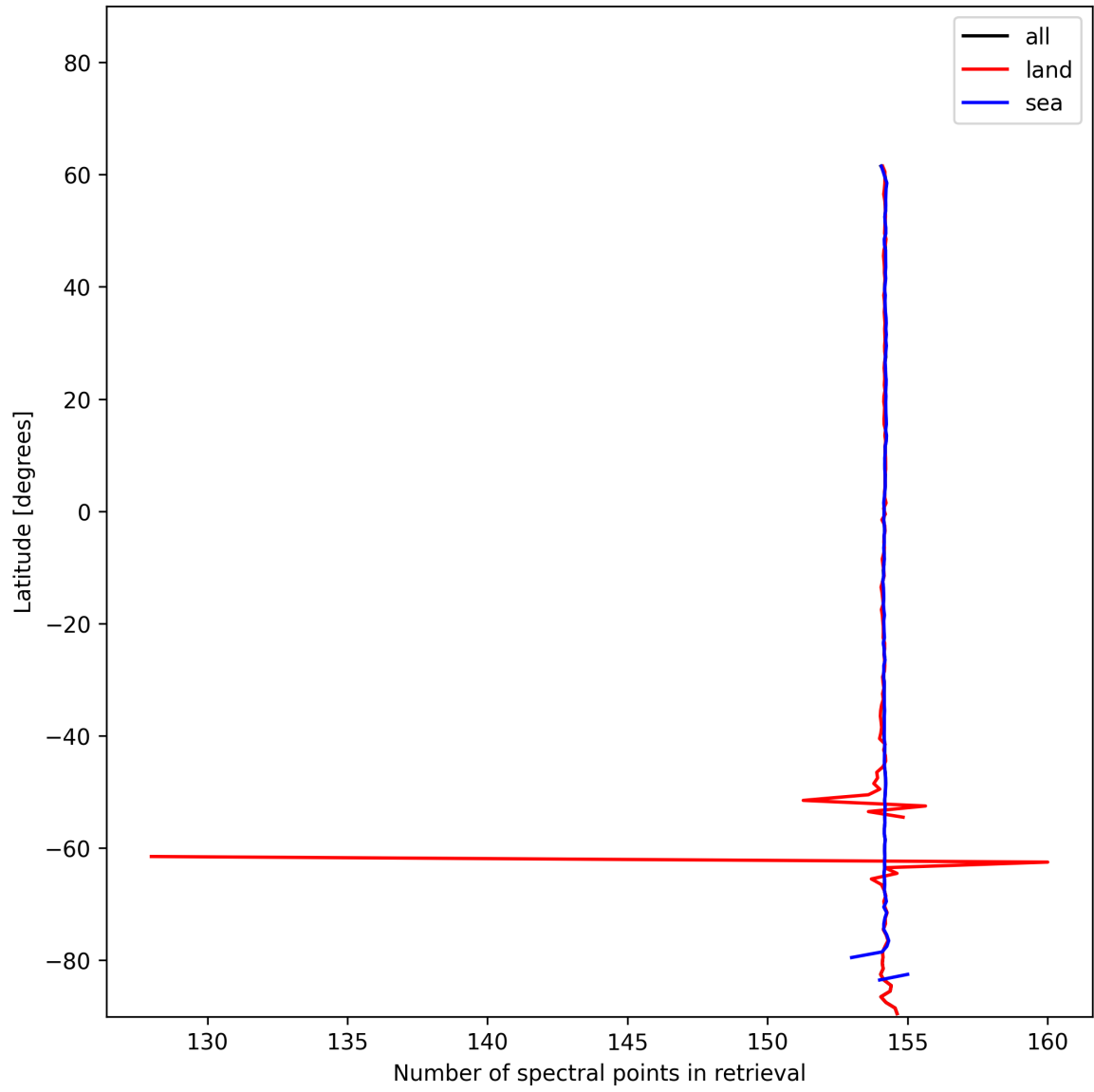
Figure 13: Zonal average of “Number of spectral points in retrieval” for 2024-12-24 to 2024-12-26.
