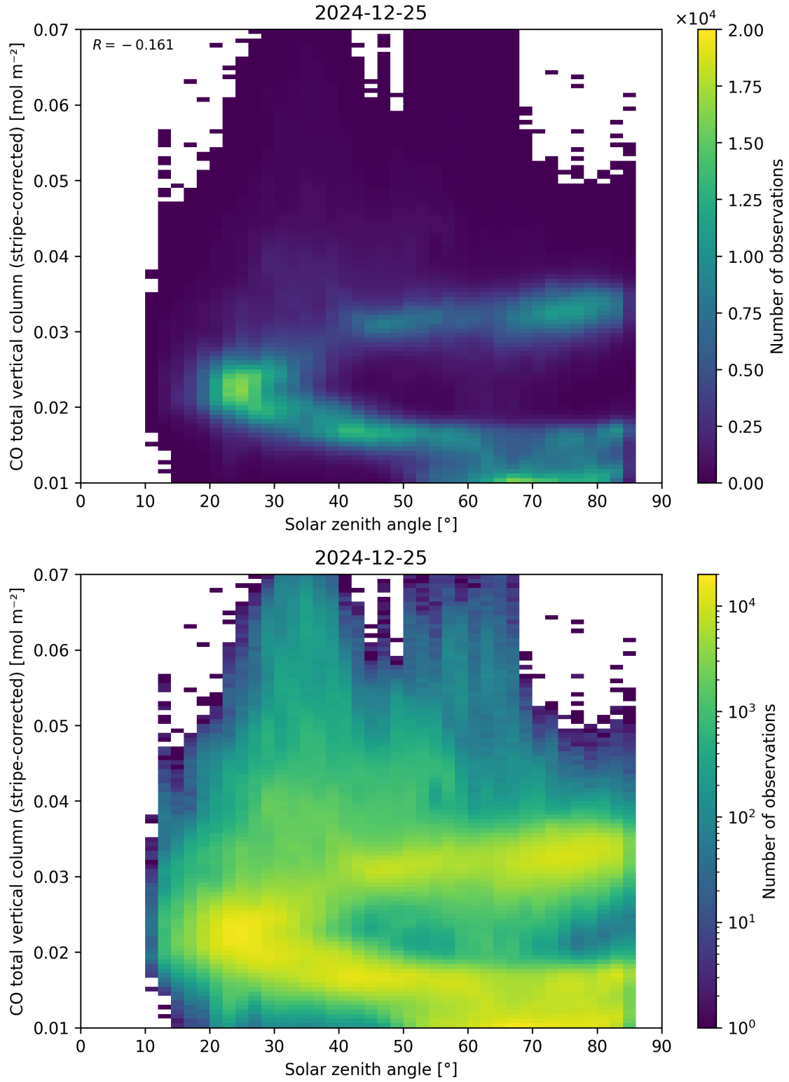
Figure 62: Scatter density plot of “Solar zenith angle” against “CO total vertical column (stripe-corrected)” for 2024-12-24 to 2024-12-26.
