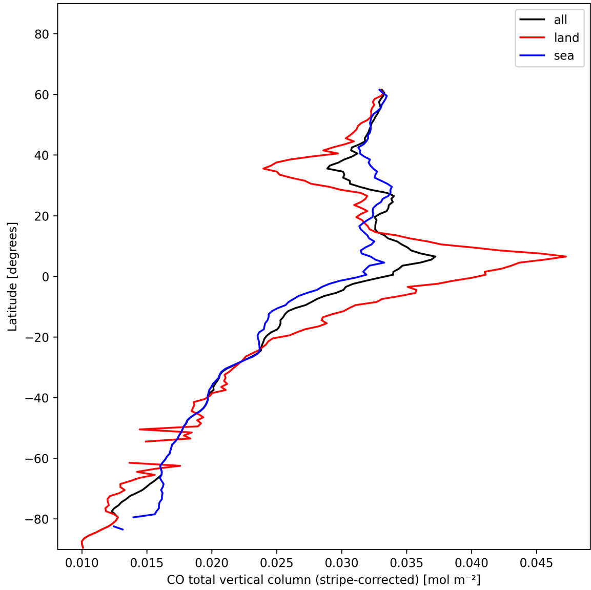
Figure 11: Zonal average of “CO total vertical column (stripe-corrected)” for 2024-12-24 to 2024-12-26.
