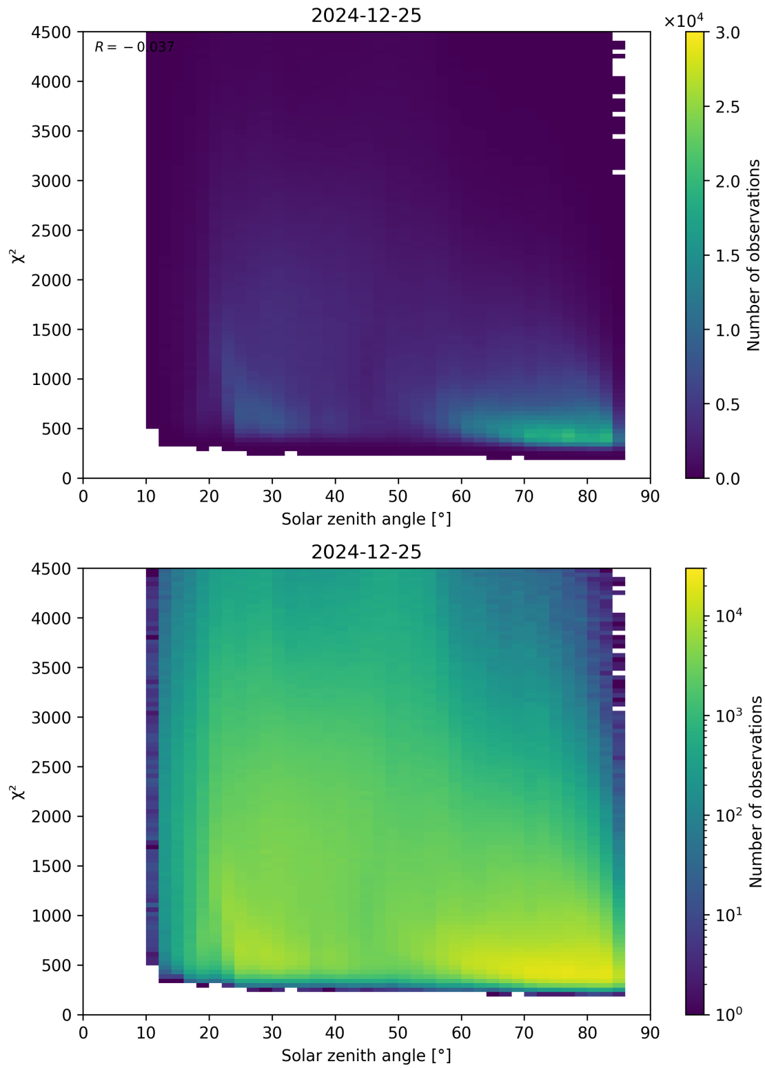
Figure 64: Scatter density plot of “Solar zenith angle” against “ \chi^2 ” for 2024-12-24 to 2024-12-26.
