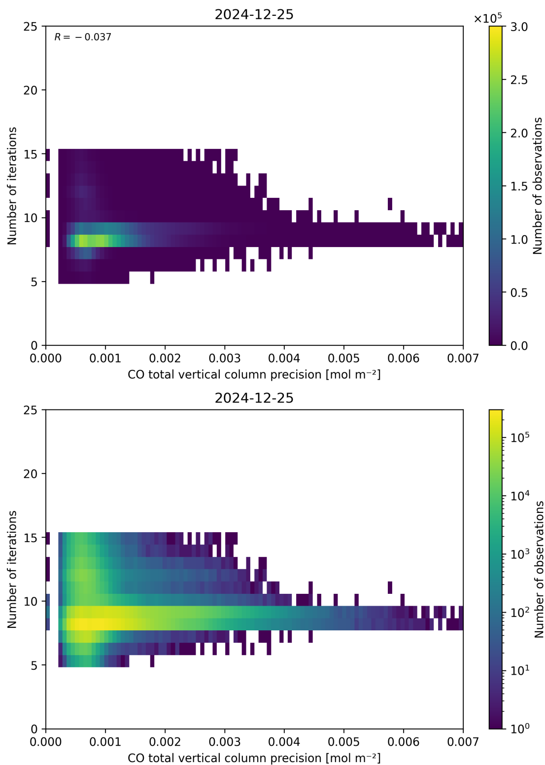
Figure 46: Scatter density plot of “CO total vertical column precision” against “Number of iterations” for 2024-12-24 to 2024-12-26.
