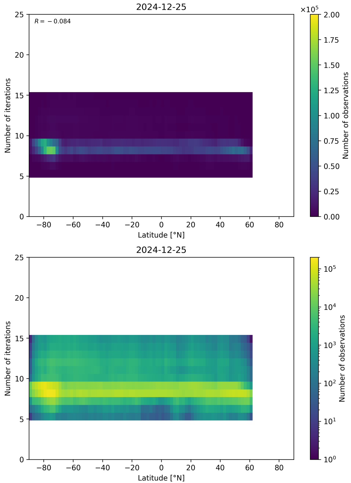
Figure 56: Scatter density plot of “Latitude” against “Number of iterations” for 2024-12-24 to 2024-12-26.
