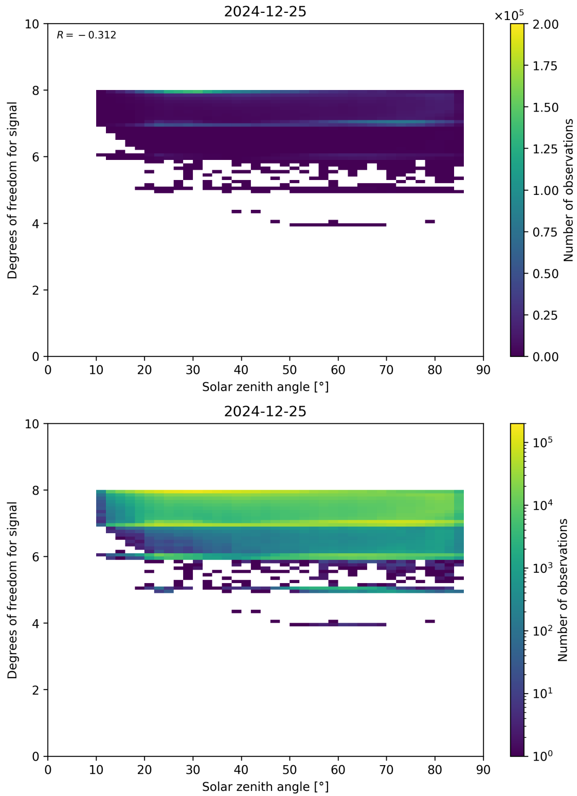
Figure 65: Scatter density plot of “Solar zenith angle” against “Degrees of freedom for signal” for 2024-12-24 to 2024-12-26.
