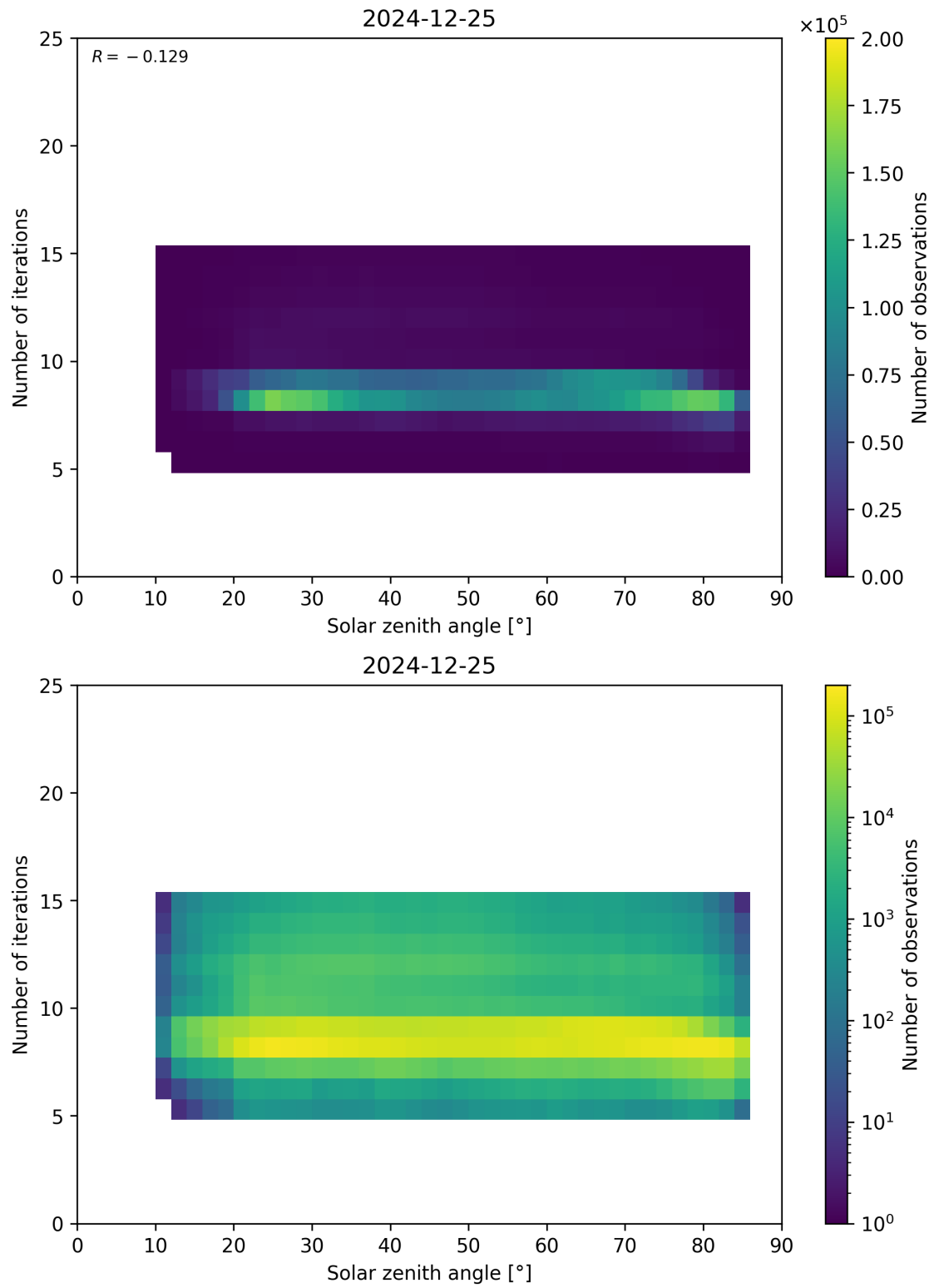
Figure 67: Scatter density plot of “Solar zenith angle” against “Number of iterations” for 2024-12-24 to 2024-12-26.
