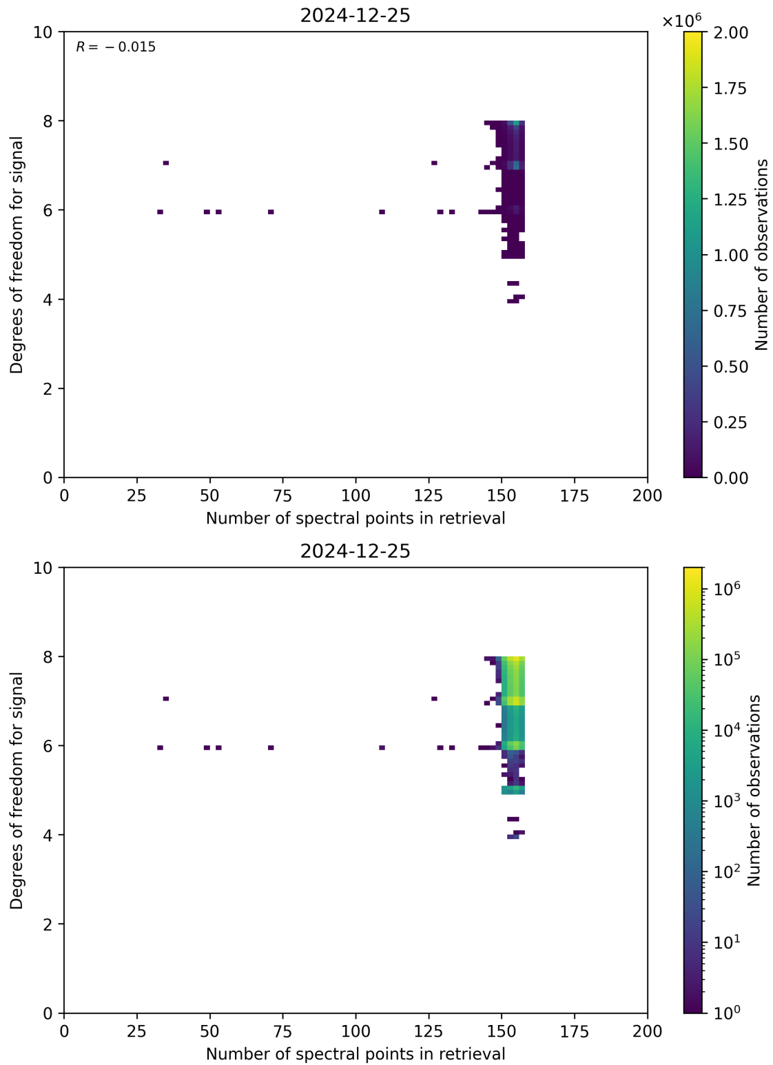
Figure 59: Scatter density plot of “Number of spectral points in retrieval” against “Degrees of freedom for signal” for 2024-12-24 to 2024-12-26.
