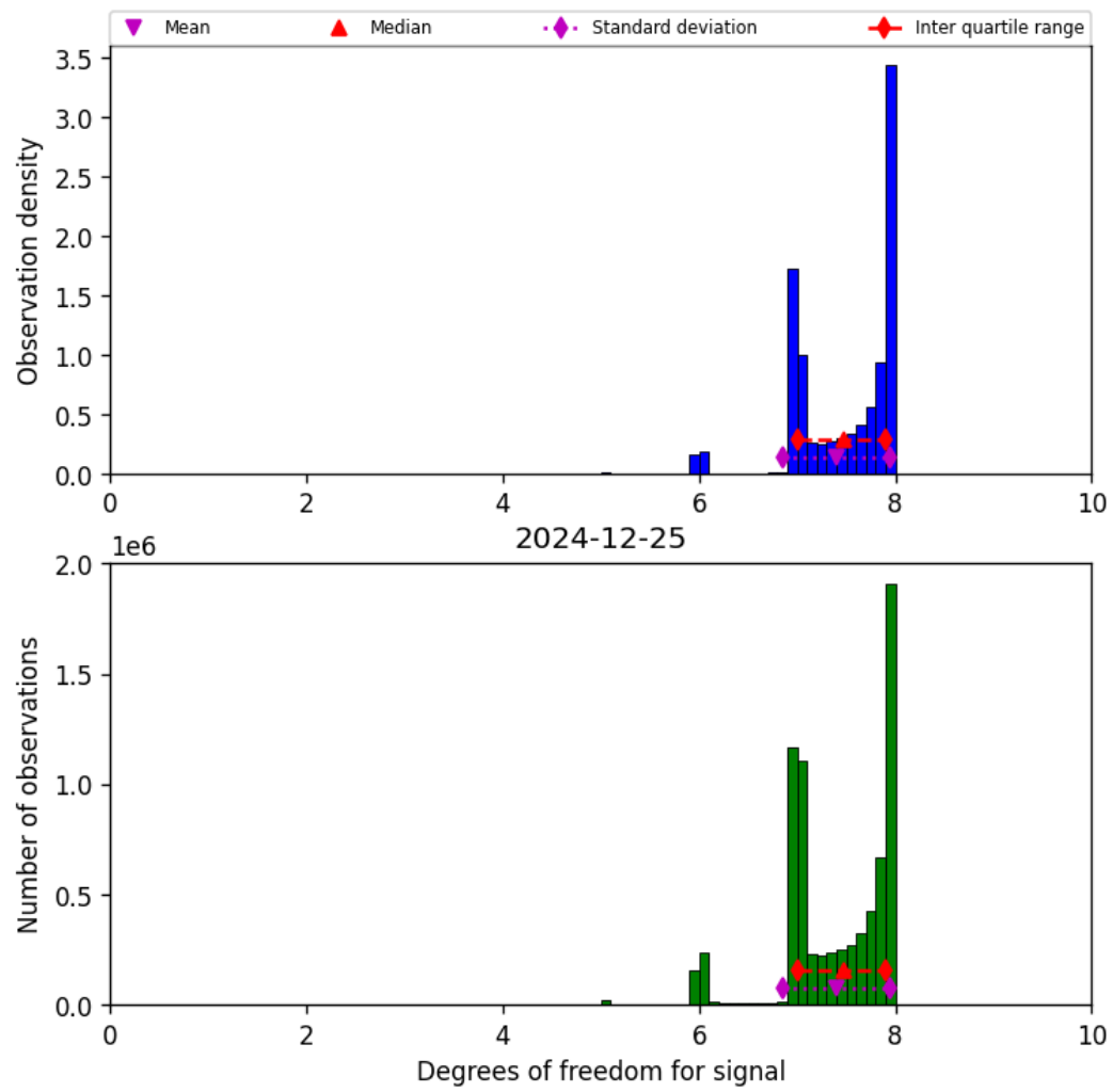
Figure 23: Histogram of “Degrees of freedom for signal” for 2024-12-24 to 2024-12-26
