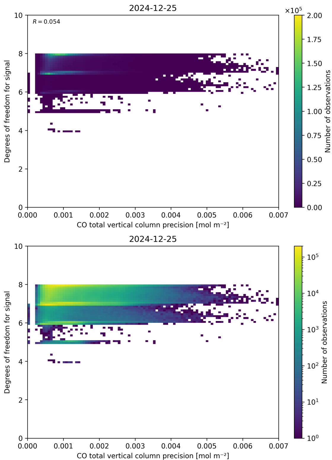
Figure 45: Scatter density plot of “CO total vertical column precision” against “Degrees of freedom for signal” for 2024-12-24 to 2024-12-26.
