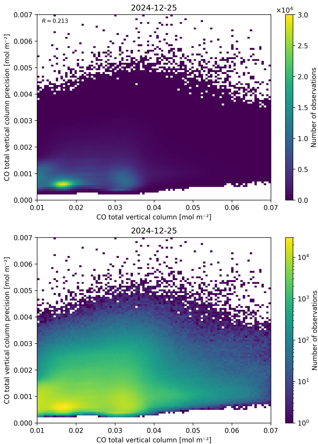
Figure 34: Scatter density plot of “CO total vertical column” against “CO total vertical column precision” for 2024-12-24 to 2024-12-26.
