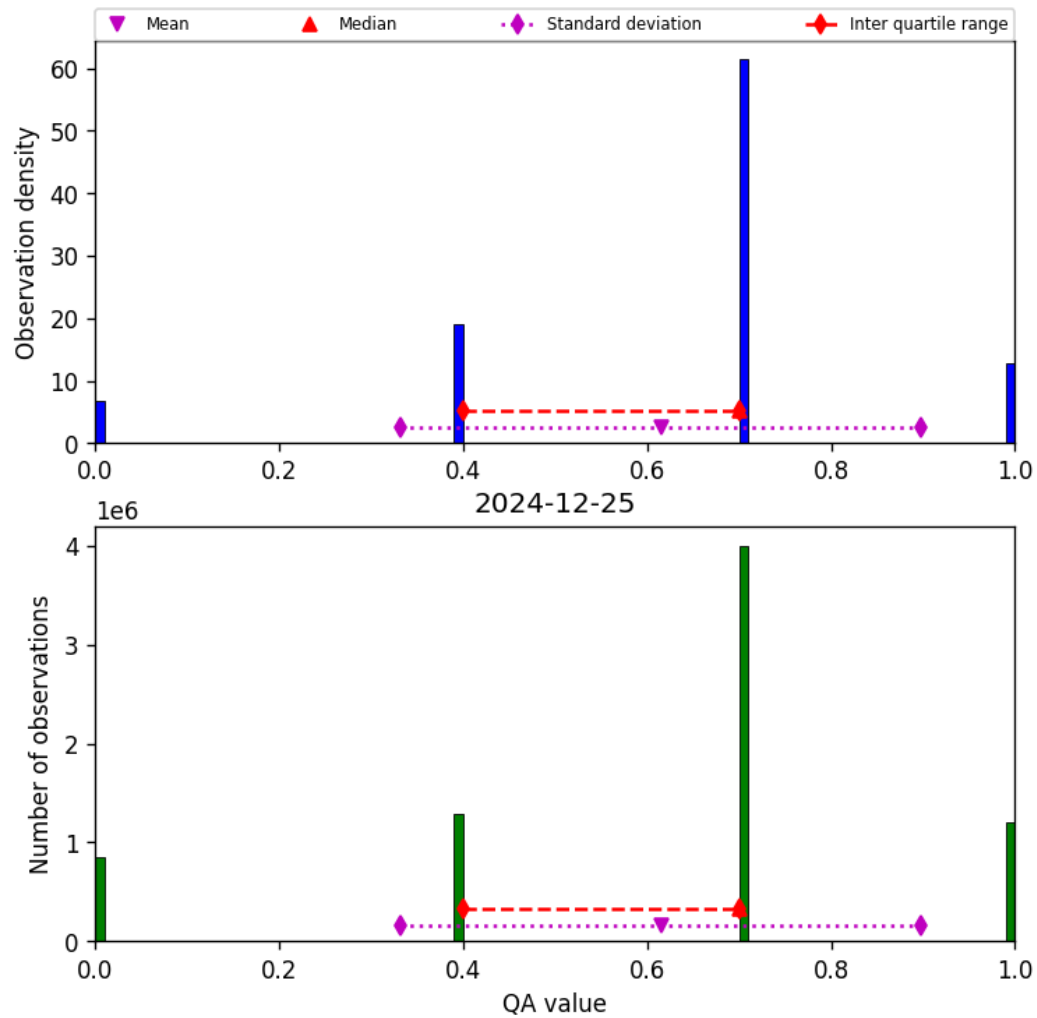
Figure 17: Histogram of “QA value” for 2024-12-24 to 2024-12-26
