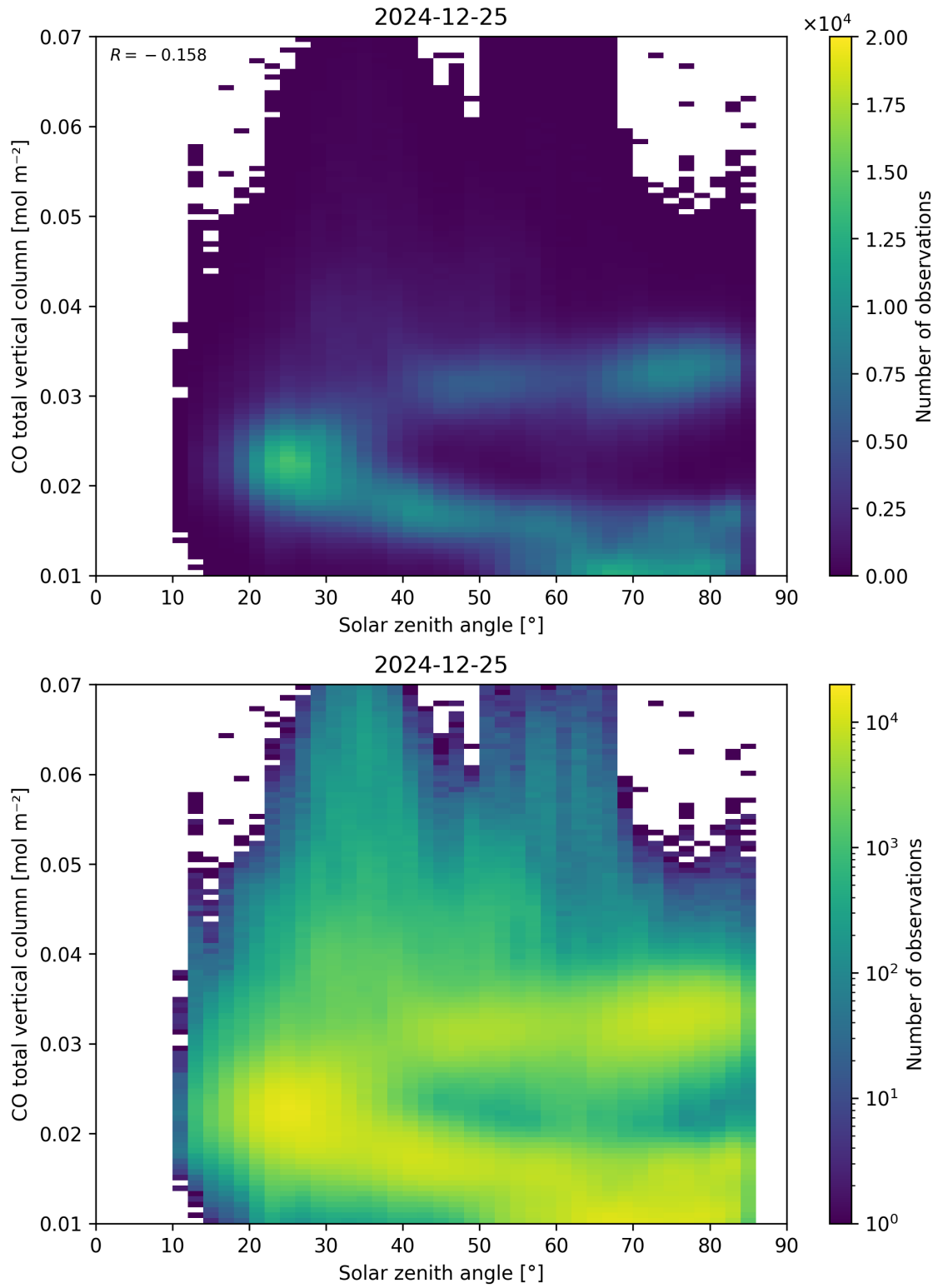
Figure 61: Scatter density plot of “Solar zenith angle” against “CO total vertical column” for 2024-12-24 to 2024-12-26.
