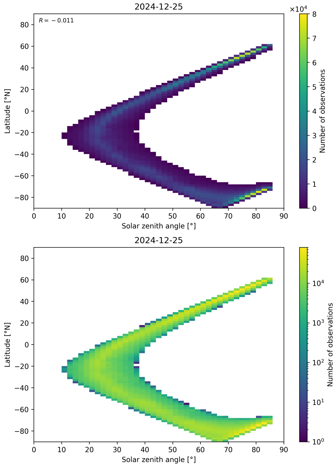
Figure 66: Scatter density plot of “Solar zenith angle” against “Latitude” for 2024-12-24 to 2024-12-26.
