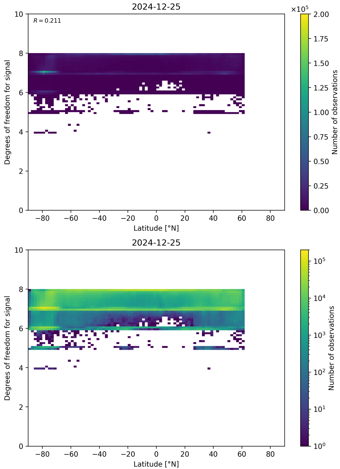
Figure 55: Scatter density plot of “Latitude” against “Degrees of freedom for signal” for 2024-12-24 to 2024-12-26.
