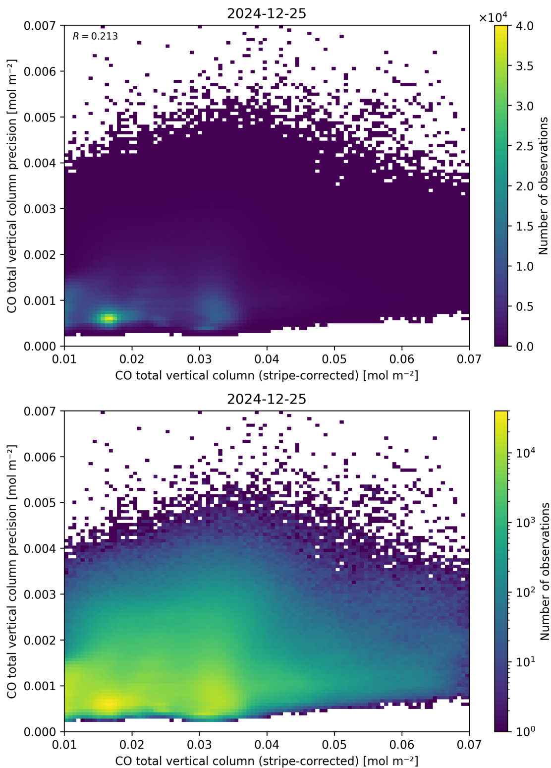
Figure 36: Scatter density plot of “CO total vertical column (stripe-corrected)” against “CO total vertical column precision” for 2024-12-24 to 2024-12-26.
