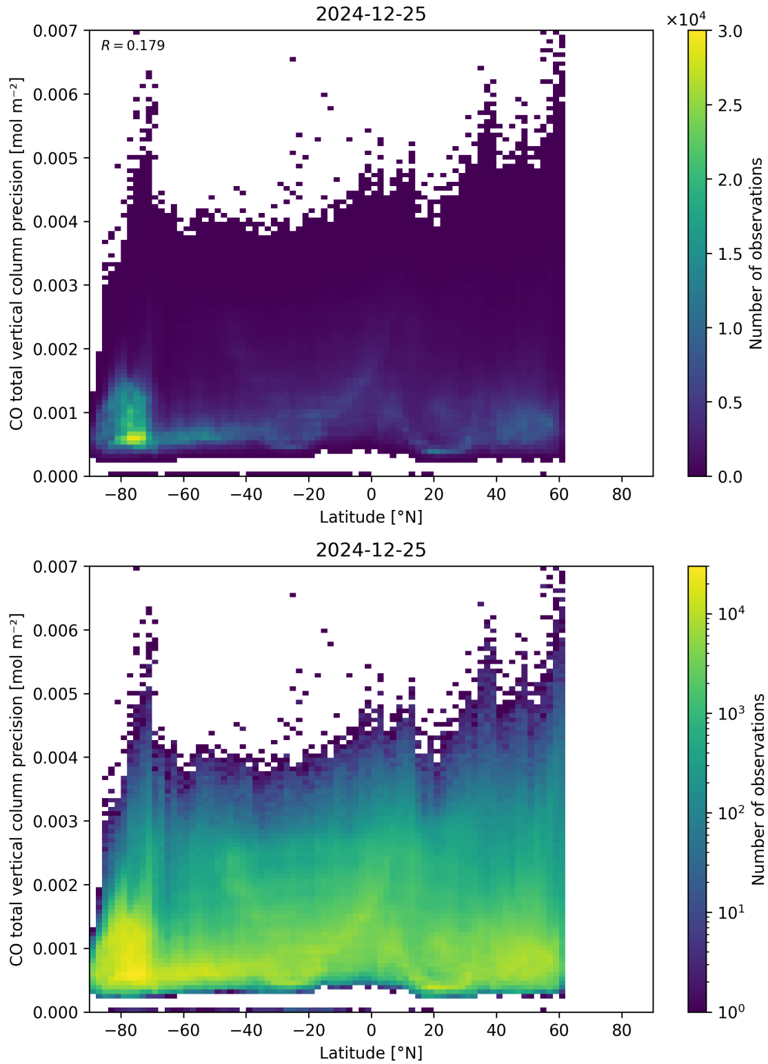
Figure 53: Scatter density plot of “Latitude” against “CO total vertical column precision” for 2024-12-24 to 2024-12-26.
