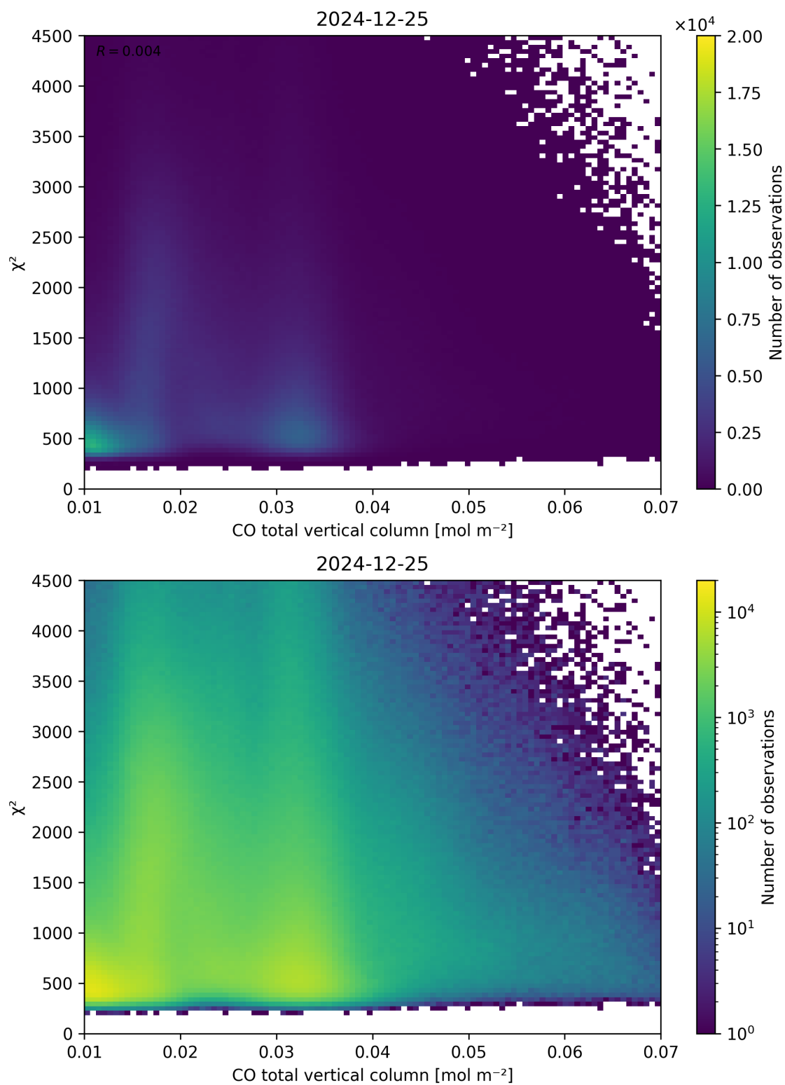
Figure 35: Scatter density plot of “CO total vertical column” against “ \chi^2 ” for 2024-12-24 to 2024-12-26.
