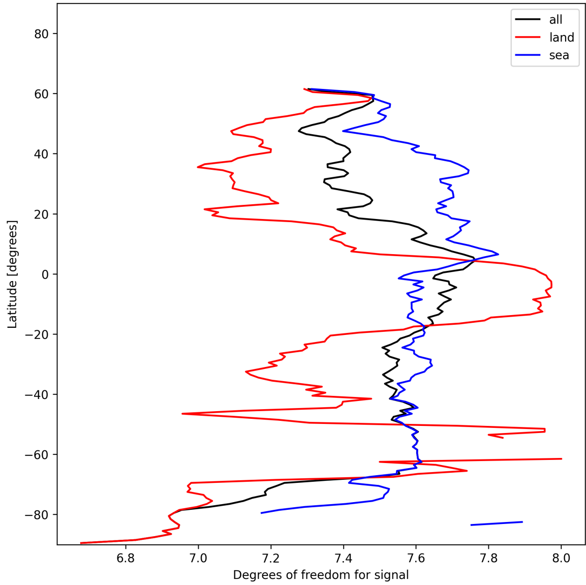
Figure 15: Zonal average of “Degrees of freedom for signal” for 2024-12-24 to 2024-12-26.
