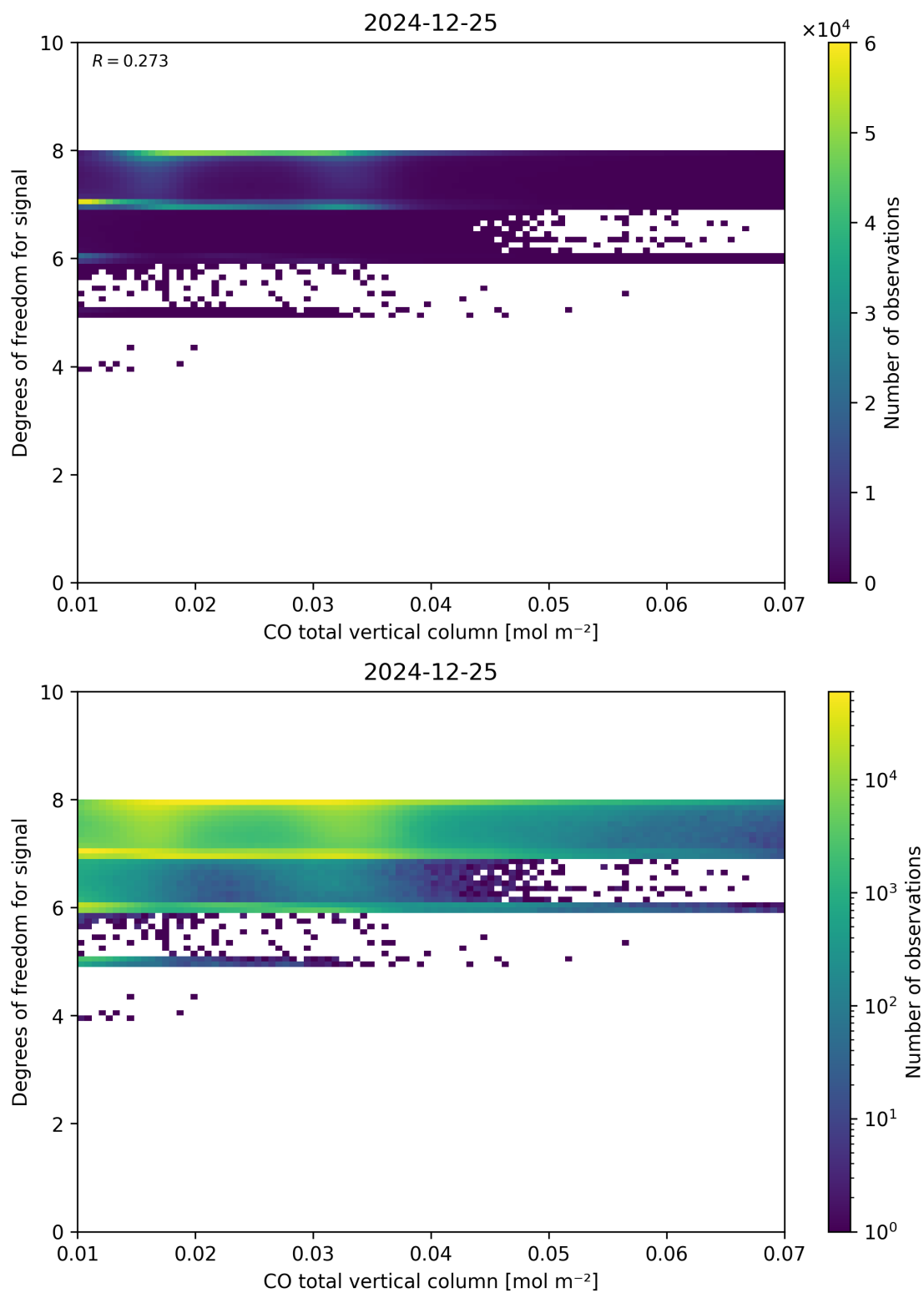
Figure 41: Scatter density plot of “CO total vertical column” against “Degrees of freedom for signal” for 2024-12-24 to 2024-12-26.
