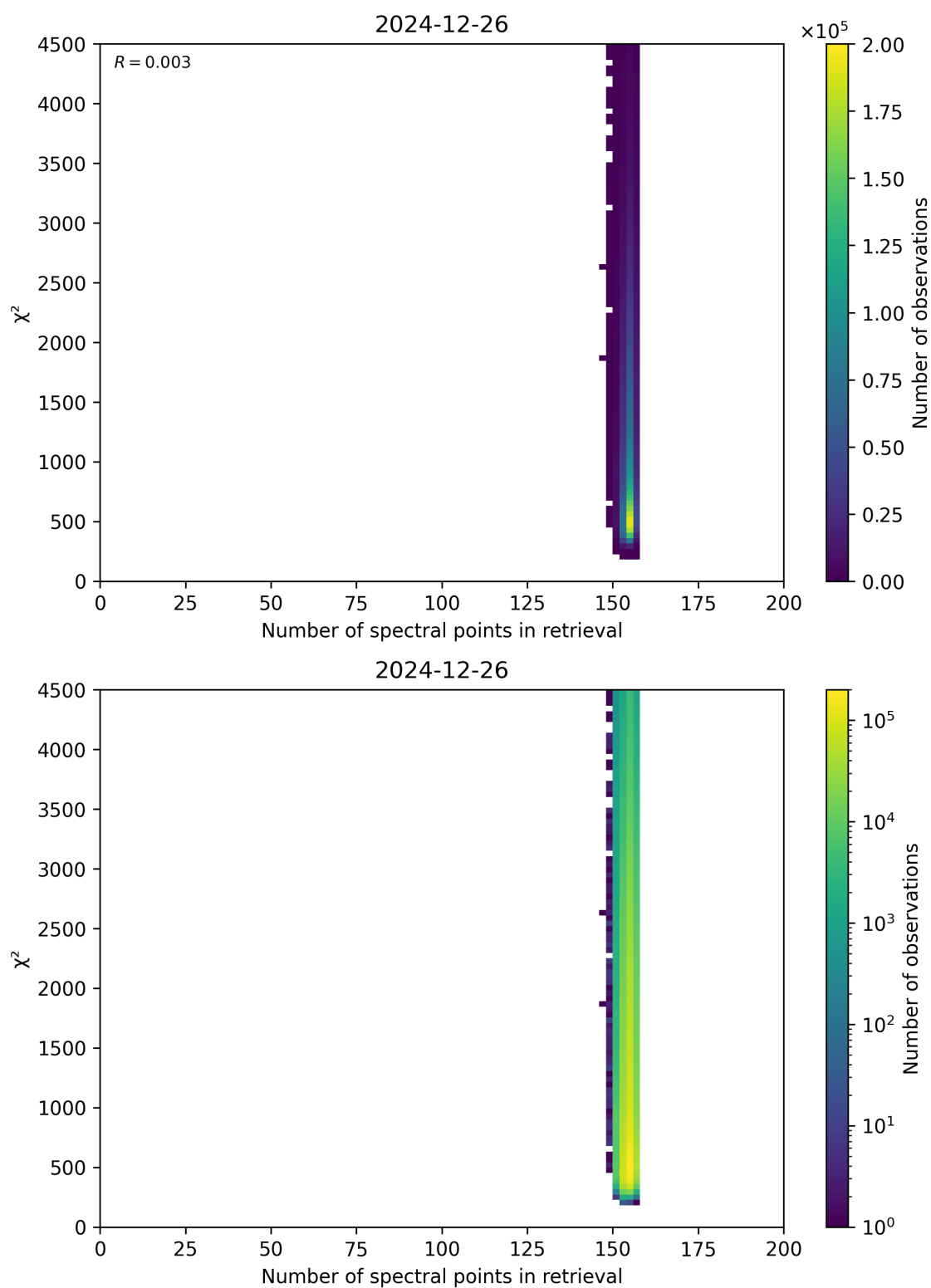
Figure 58: Scatter density plot of “Number of spectral points in retrieval” against “ \chi^2 ” for 2024-12-25 to 2024-12-27.
