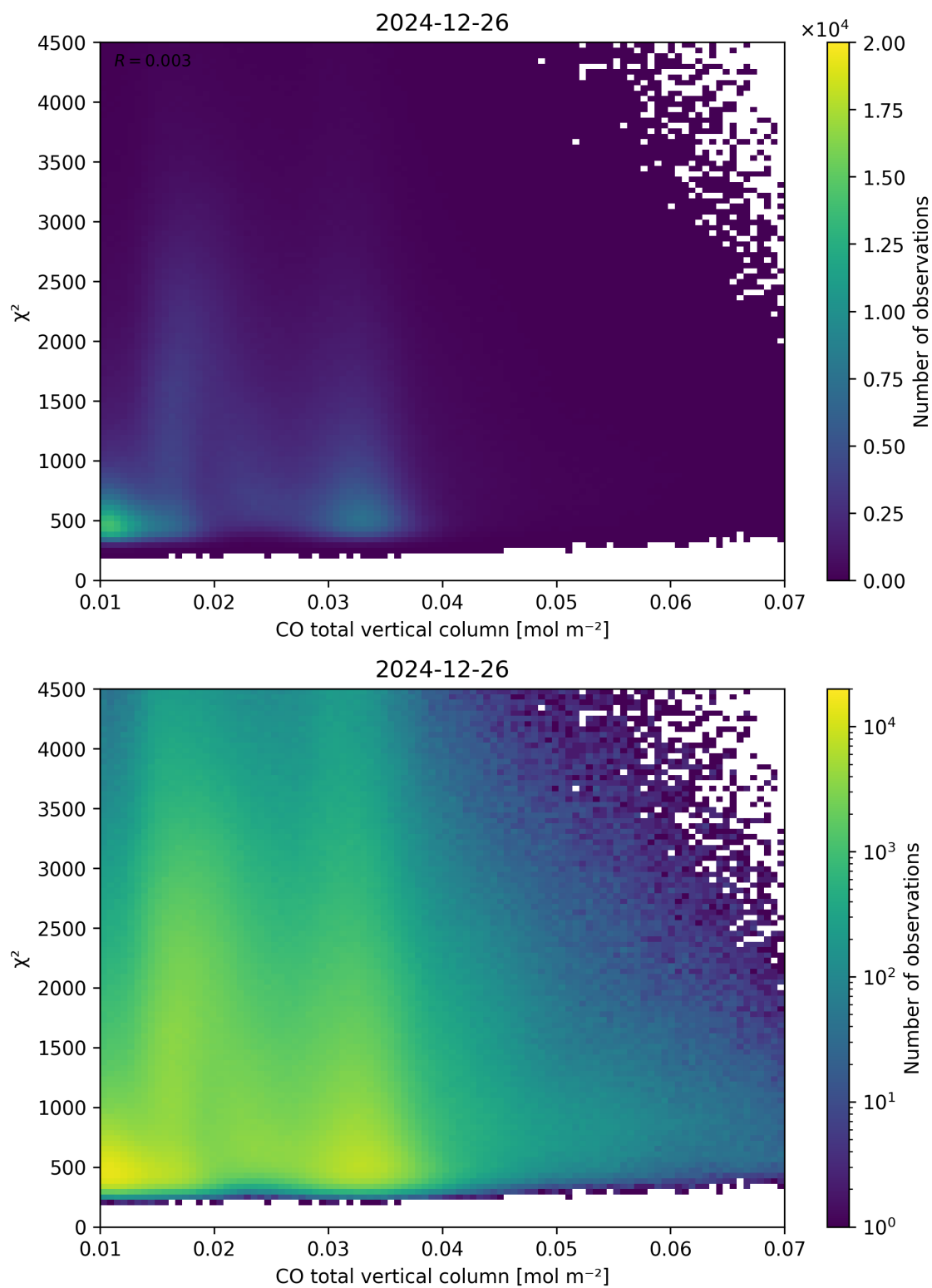
Figure 35: Scatter density plot of “CO total vertical column” against “ \chi^2 ” for 2024-12-25 to 2024-12-27.
