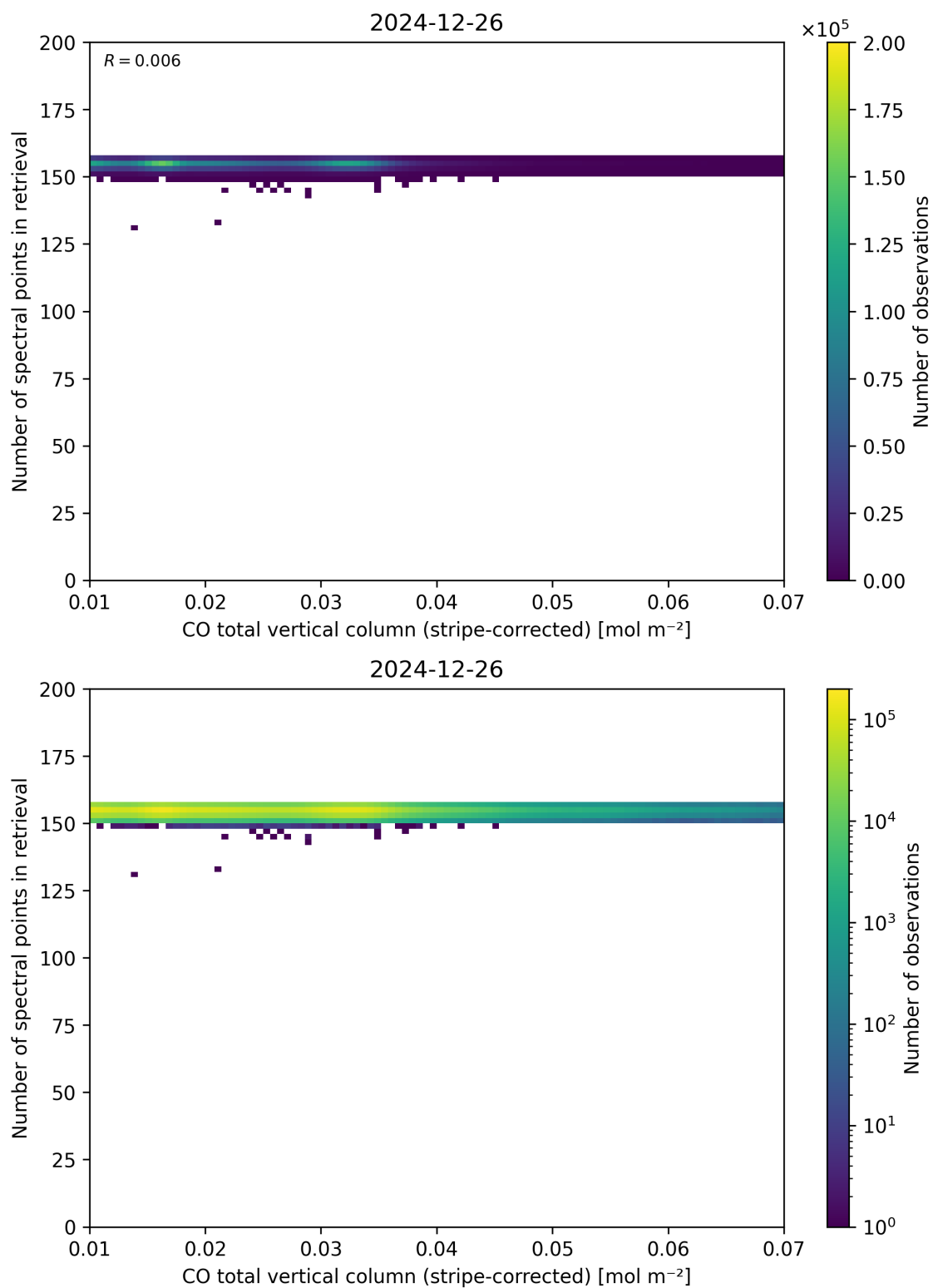
Figure 40: Scatter density plot of “CO total vertical column (stripe-corrected)” against “Number of spectral points in retrieval” for 2024-12-25 to 2024-12-27.
