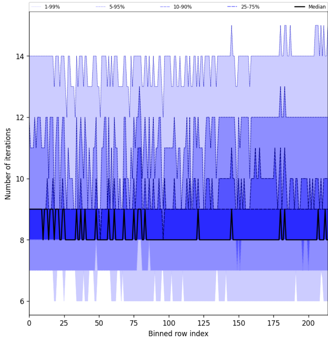
Figure 32: Along track statistics of “Number of iterations” for 2024-12-25 to 2024-12-27
