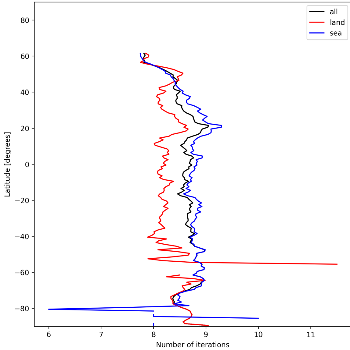
Figure 16: Zonal average of “Number of iterations” for 2024-12-25 to 2024-12-27.
