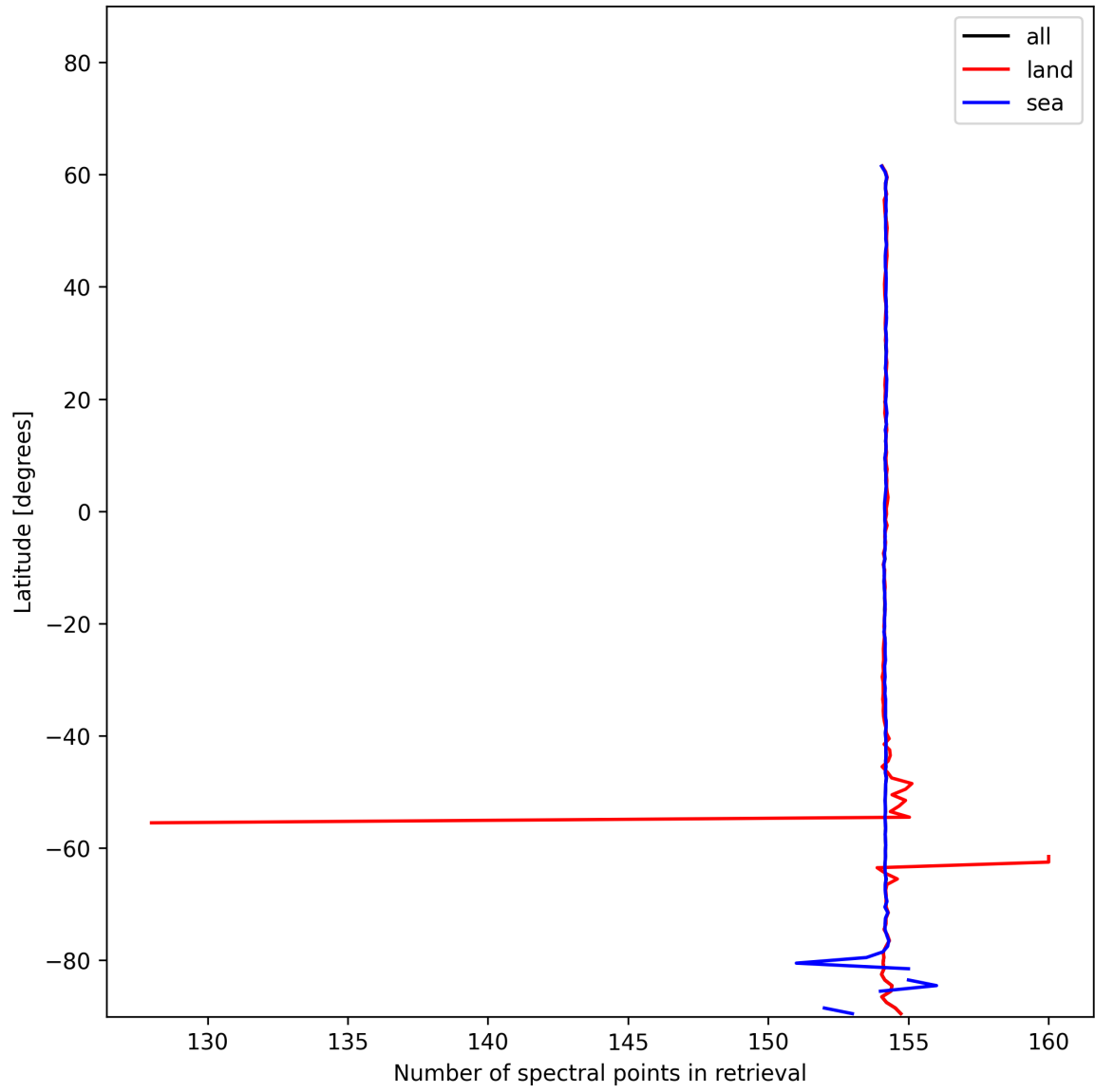
Figure 13: Zonal average of “Number of spectral points in retrieval” for 2024-12-25 to 2024-12-27.
