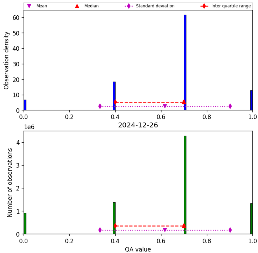
Figure 17: Histogram of “QA value” for 2024-12-25 to 2024-12-27
