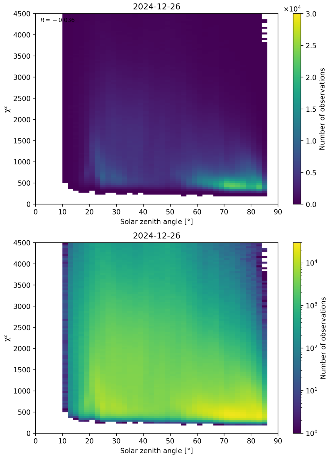
Figure 64: Scatter density plot of “Solar zenith angle” against “ \chi^2 ” for 2024-12-25 to 2024-12-27.
