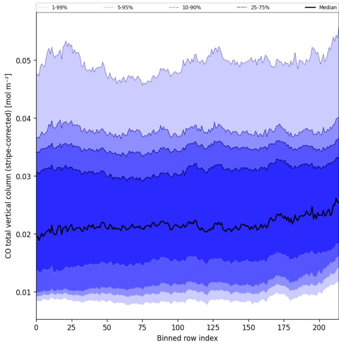
Figure 27: Along track statistics of “CO total vertical column (stripe-corrected)” for 2024-12-25 to 2024-12-27
