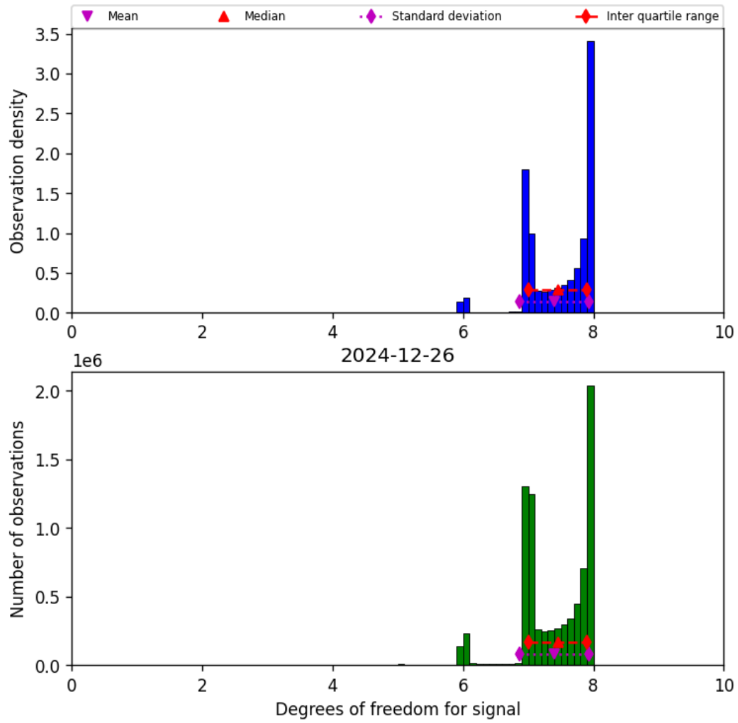
Figure 23: Histogram of “Degrees of freedom for signal” for 2024-12-25 to 2024-12-27
