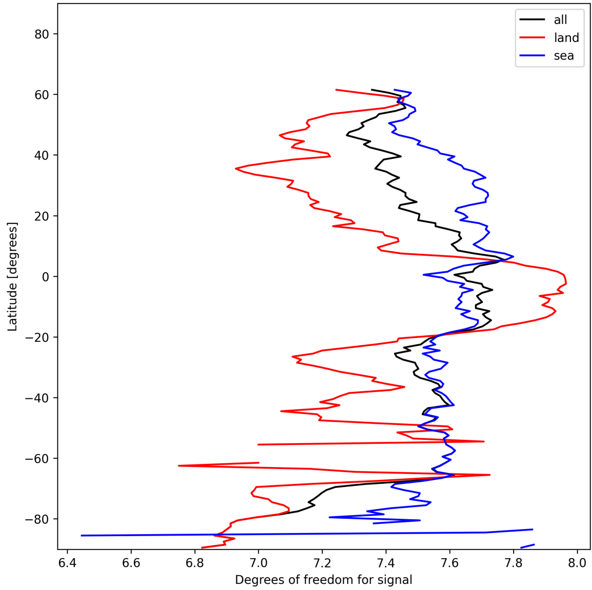
Figure 15: Zonal average of “Degrees of freedom for signal” for 2024-12-25 to 2024-12-27.
