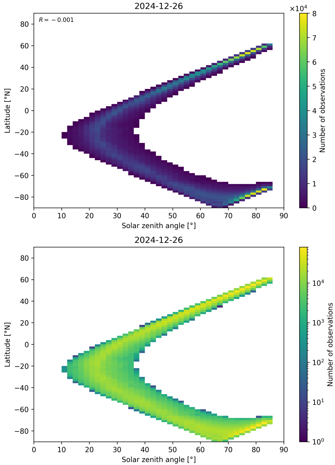
Figure 66: Scatter density plot of “Solar zenith angle” against “Latitude” for 2024-12-25 to 2024-12-27.
