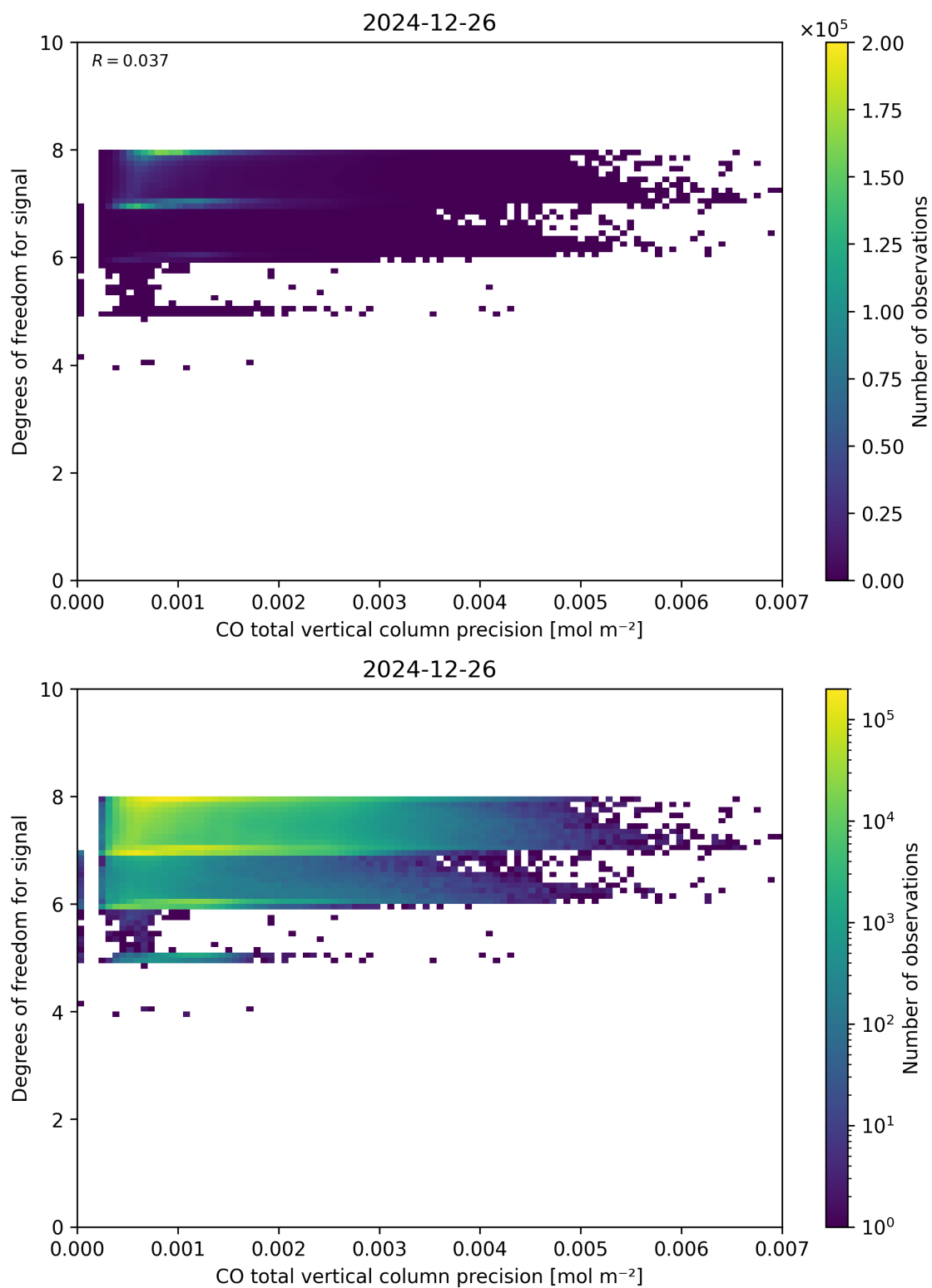
Figure 45: Scatter density plot of “CO total vertical column precision” against “Degrees of freedom for signal” for 2024-12-25 to 2024-12-27.
