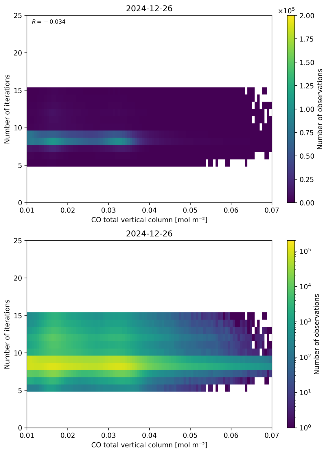
Figure 42: Scatter density plot of “CO total vertical column” against “Number of iterations” for 2024-12-25 to 2024-12-27.
