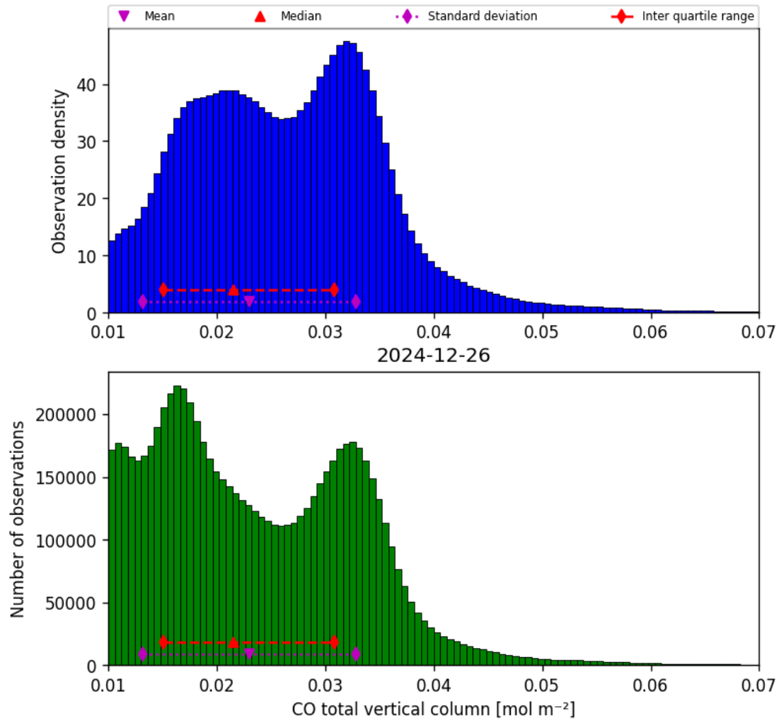
Figure 18: Histogram of “CO total vertical column” for 2024-12-25 to 2024-12-27
