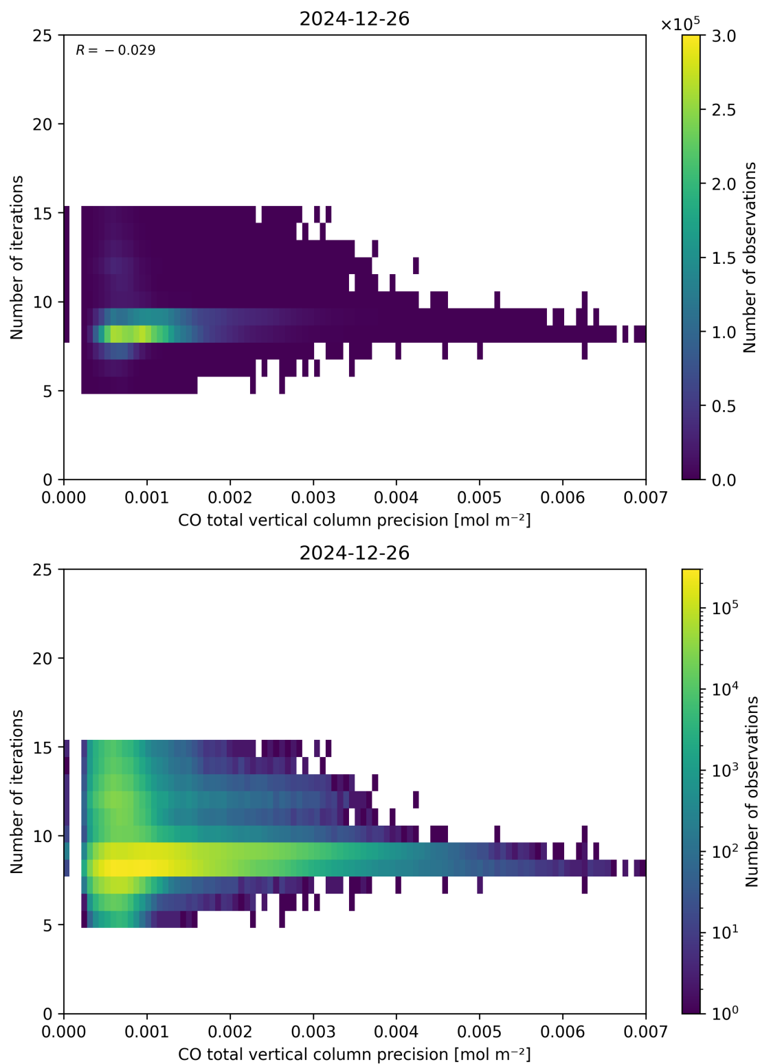
Figure 46: Scatter density plot of “CO total vertical column precision” against “Number of iterations” for 2024-12-25 to 2024-12-27.
