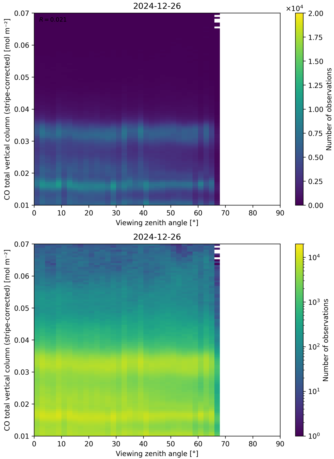
Figure 70: Scatter density plot of “Viewing zenith angle” against “CO total vertical column (stripe-corrected)” for 2024-12-25 to 2024-12-27.
