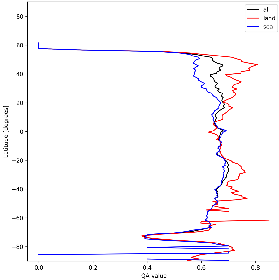
Figure 9: Zonal average of “QA value” for 2024-12-25 to 2024-12-27.
