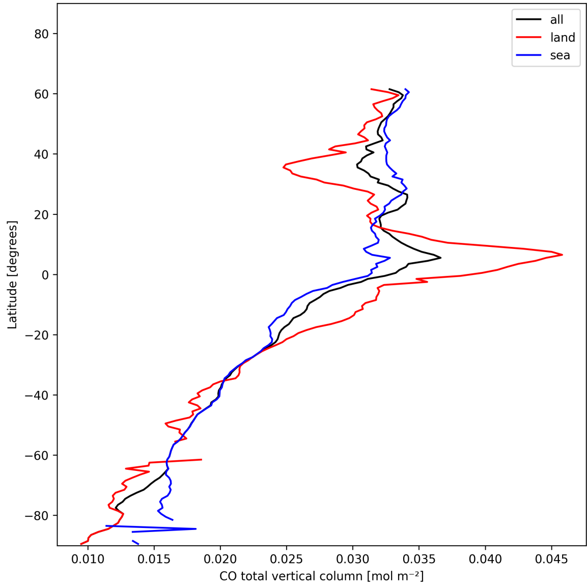
Figure 10: Zonal average of “CO total vertical column” for 2024-12-25 to 2024-12-27.
