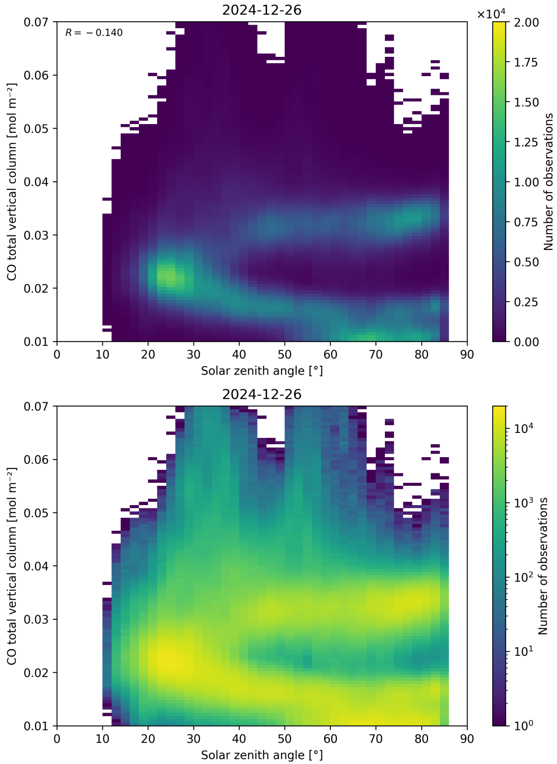
Figure 61: Scatter density plot of “Solar zenith angle” against “CO total vertical column” for 2024-12-25 to 2024-12-27.
