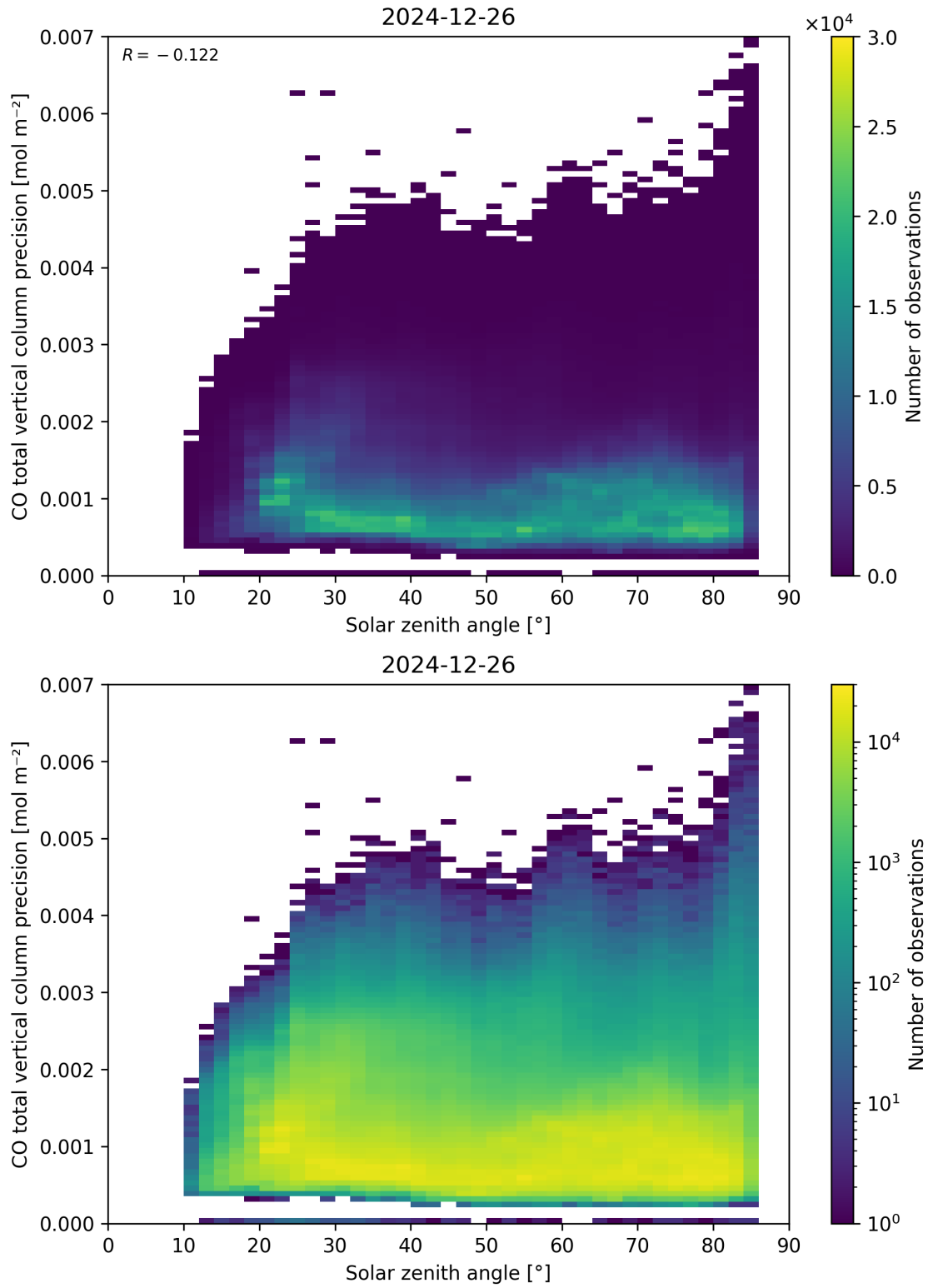
Figure 63: Scatter density plot of “Solar zenith angle” against “CO total vertical column precision” for 2024-12-25 to 2024-12-27.
