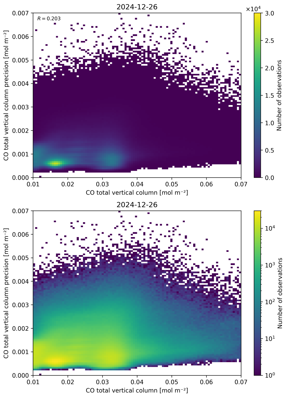
Figure 34: Scatter density plot of “CO total vertical column” against “CO total vertical column precision” for 2024-12-25 to 2024-12-27.
