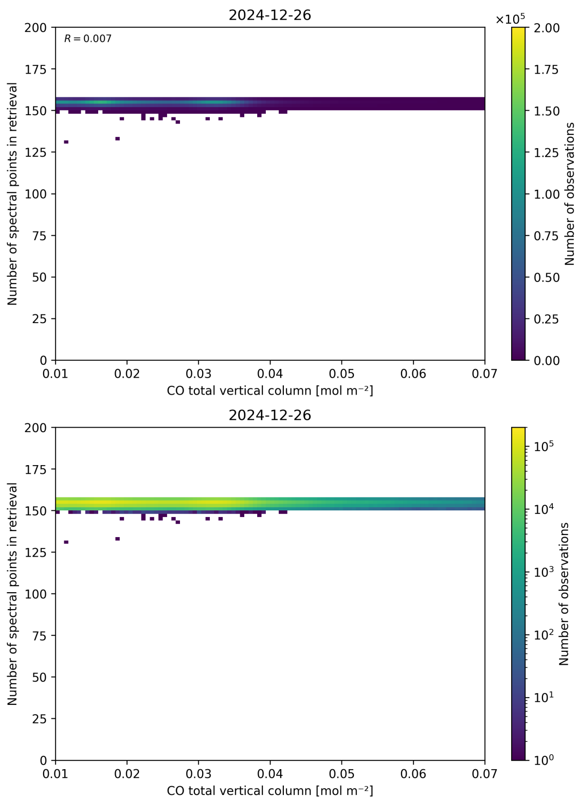
Figure 43: Scatter density plot of “CO total vertical column” against “Number of spectral points in retrieval” for 2024-12-25 to 2024-12-27.
