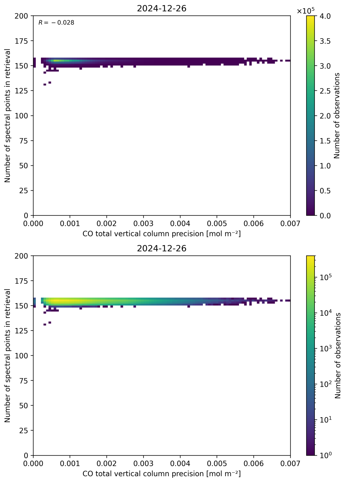
Figure 47: Scatter density plot of “CO total vertical column precision” against “Number of spectral points in retrieval” for 2024-12-25 to 2024-12-27.
