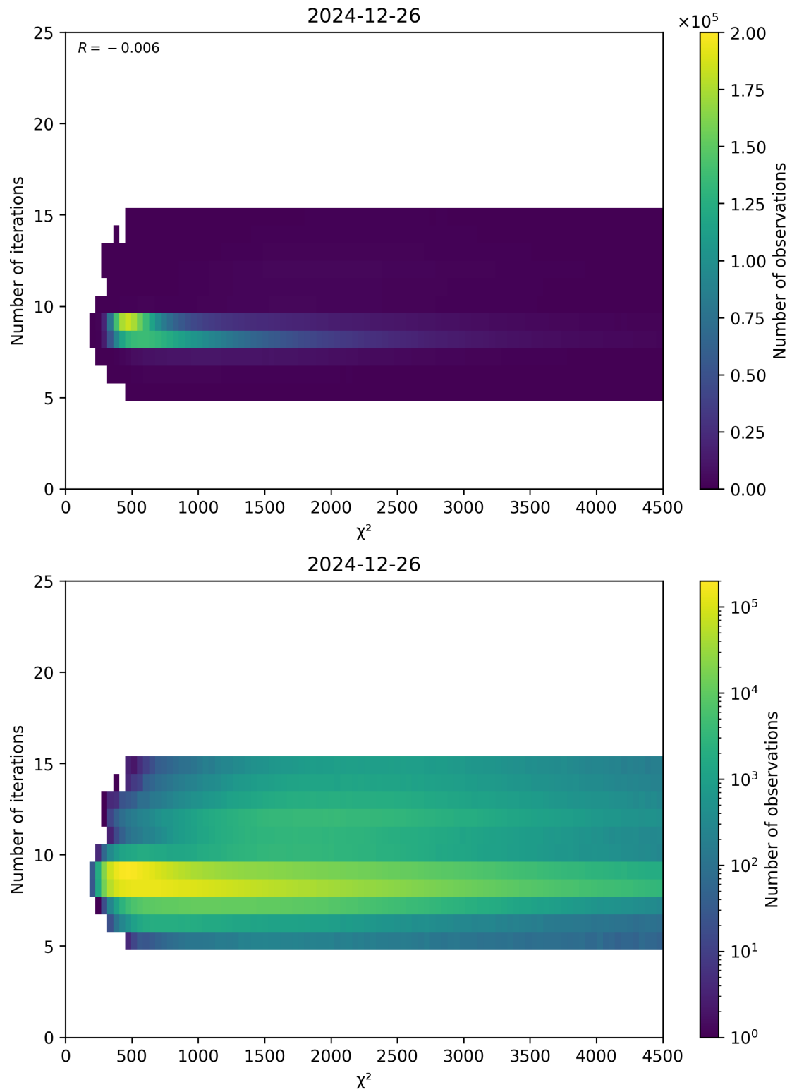
Figure 49: Scatter density plot of “ \chi^2 ” against “Number of iterations” for 2024-12-25 to 2024-12-27.
