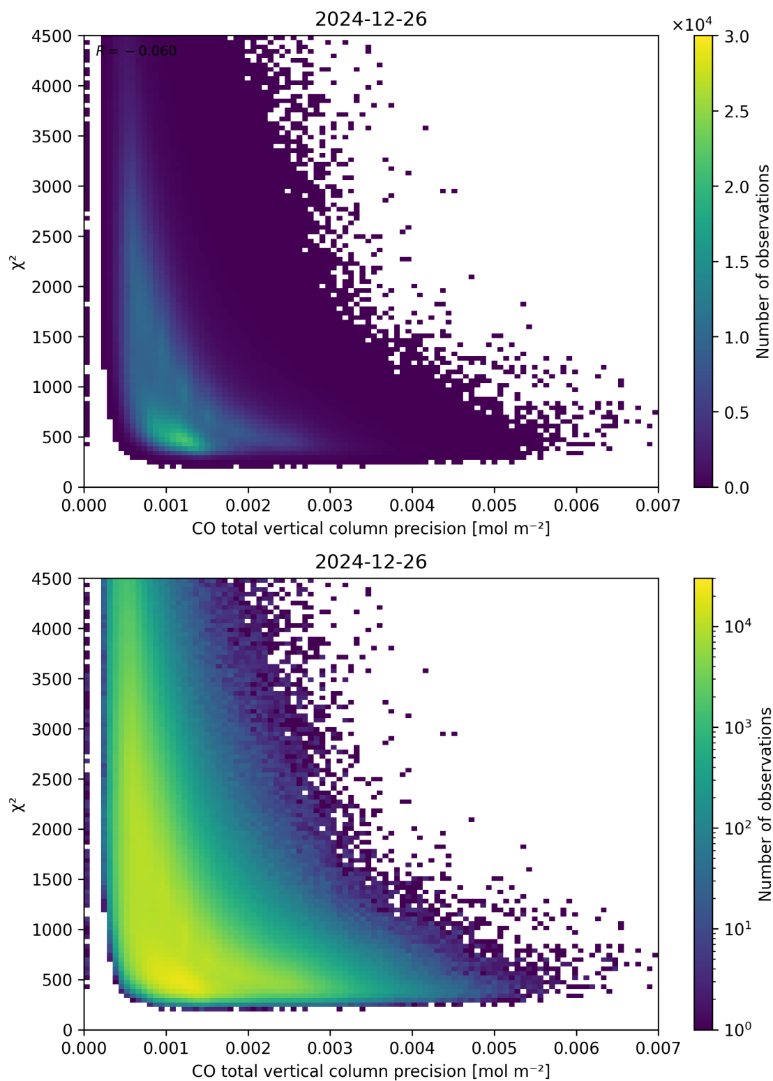
Figure 44: Scatter density plot of “CO total vertical column precision” against “ \chi^2 ” for 2024-12-25 to 2024-12-27.
