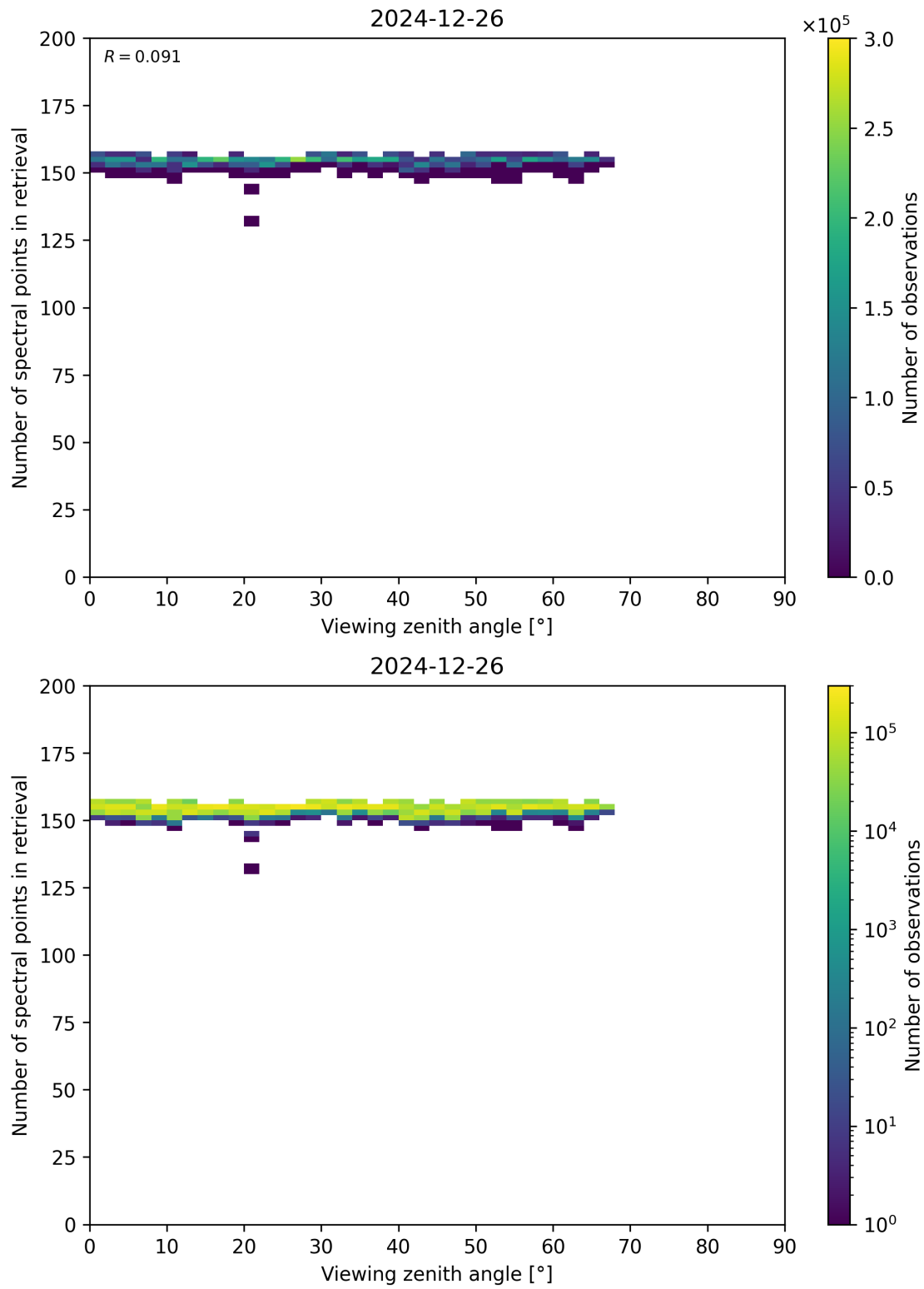
Figure 76: Scatter density plot of “Viewing zenith angle” against “Number of spectral points in retrieval” for 2024-12-25 to 2024-12-27.
