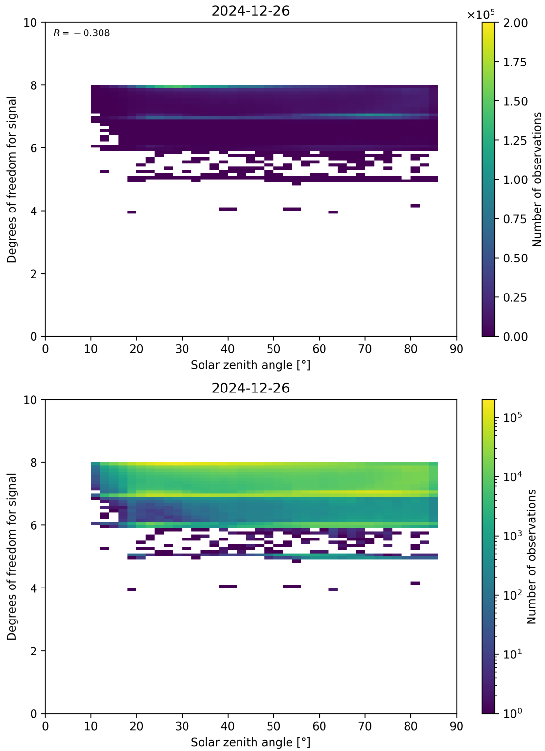
Figure 65: Scatter density plot of “Solar zenith angle” against “Degrees of freedom for signal” for 2024-12-25 to 2024-12-27.
