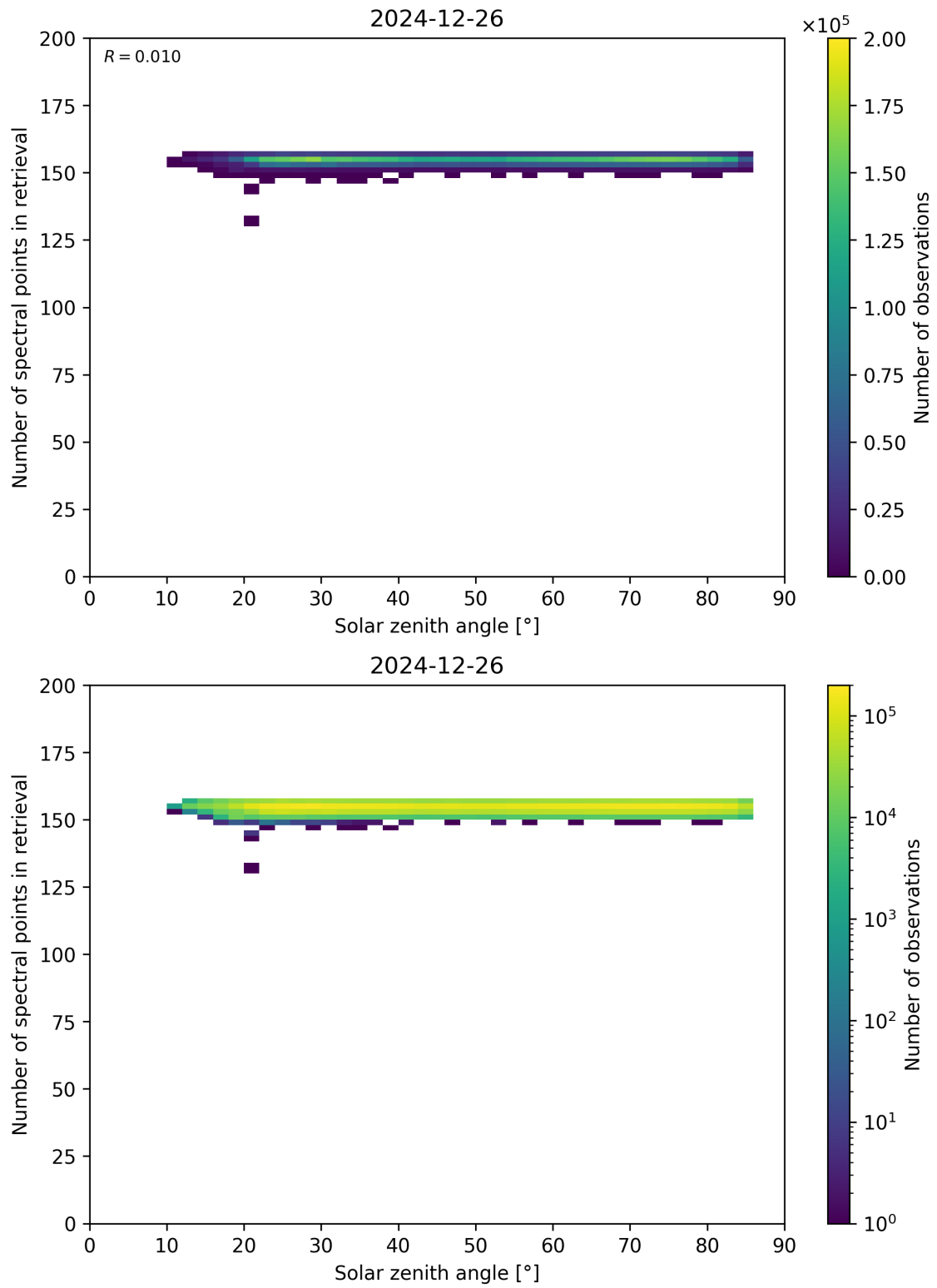
Figure 68: Scatter density plot of “Solar zenith angle” against “Number of spectral points in retrieval” for 2024-12-25 to 2024-12-27.
