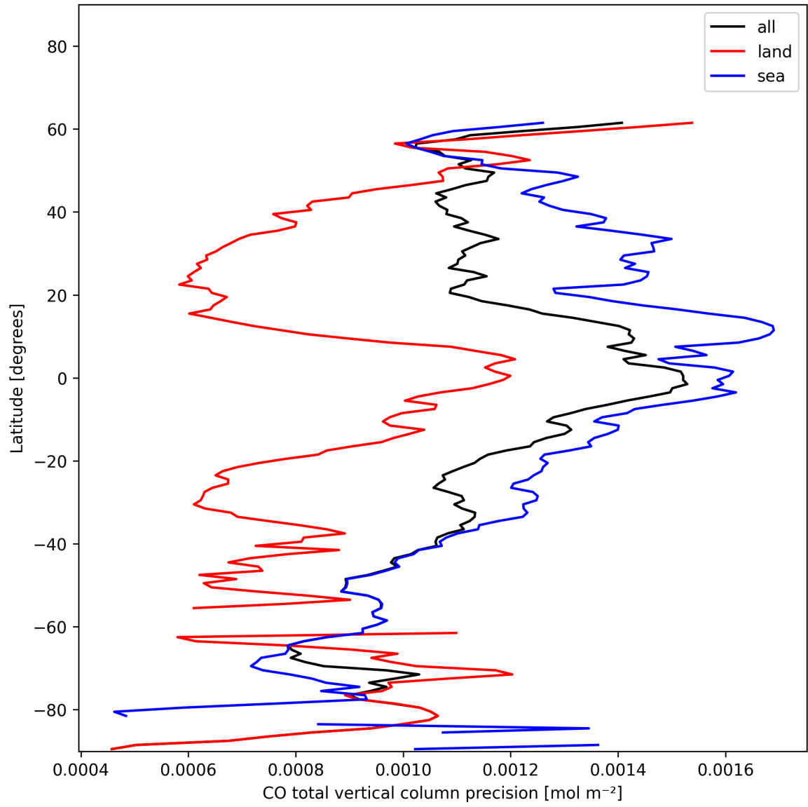
Figure 12: Zonal average of “CO total vertical column precision” for 2024-12-25 to 2024-12-27.
