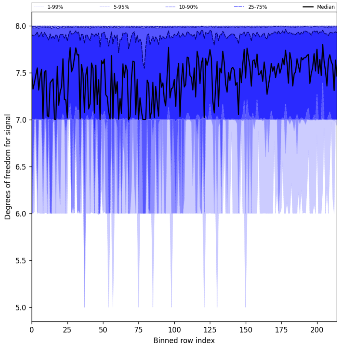
Figure 31: Along track statistics of “Degrees of freedom for signal” for 2024-12-25 to 2024-12-27
