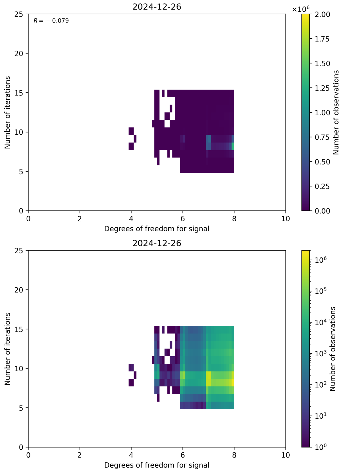
Figure 50: Scatter density plot of “Degrees of freedom for signal” against “Number of iterations” for 2024-12-25 to 2024-12-27.
