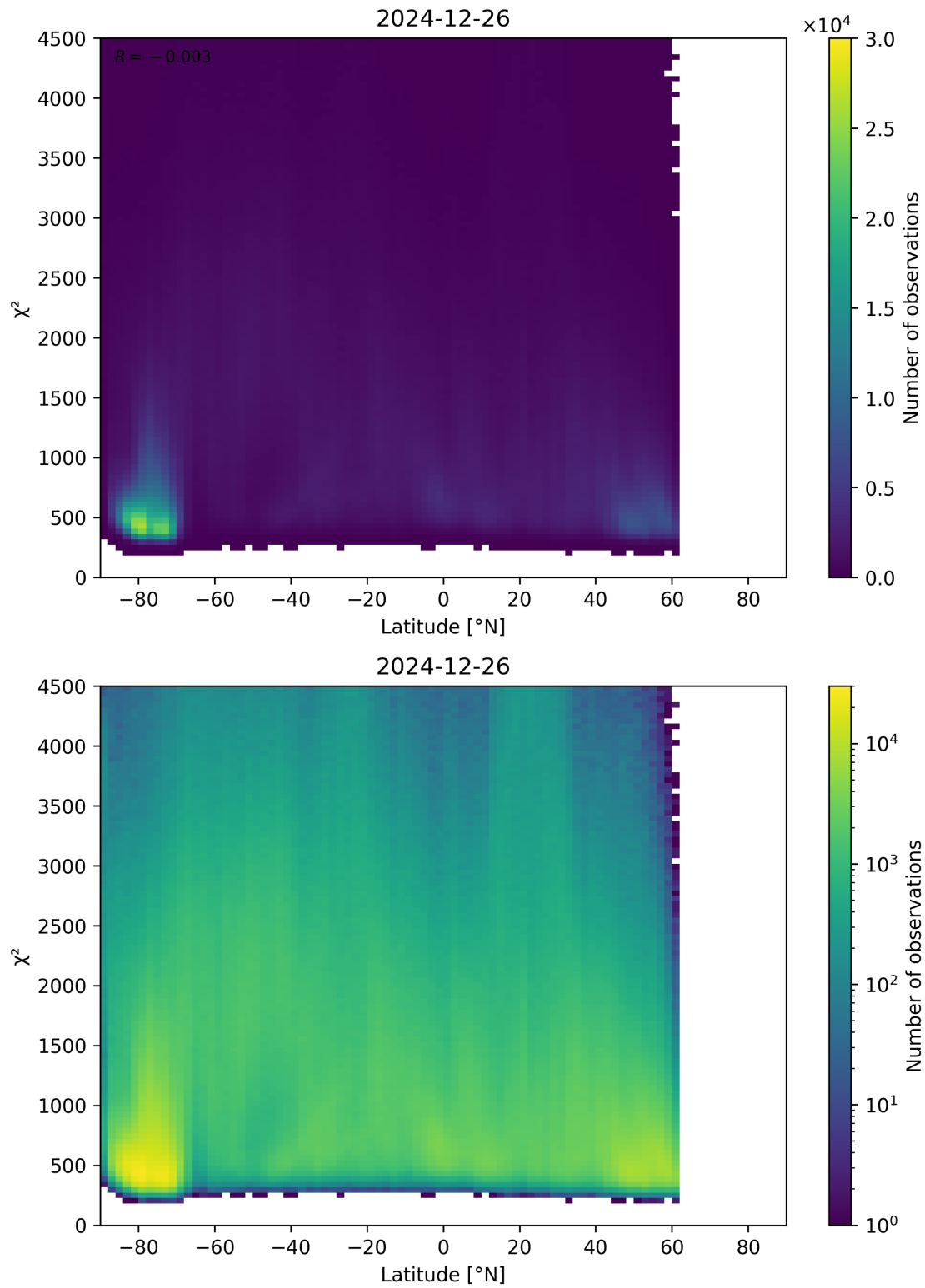
Figure 54: Scatter density plot of “Latitude” against “ \chi^2 ” for 2024-12-25 to 2024-12-27.
