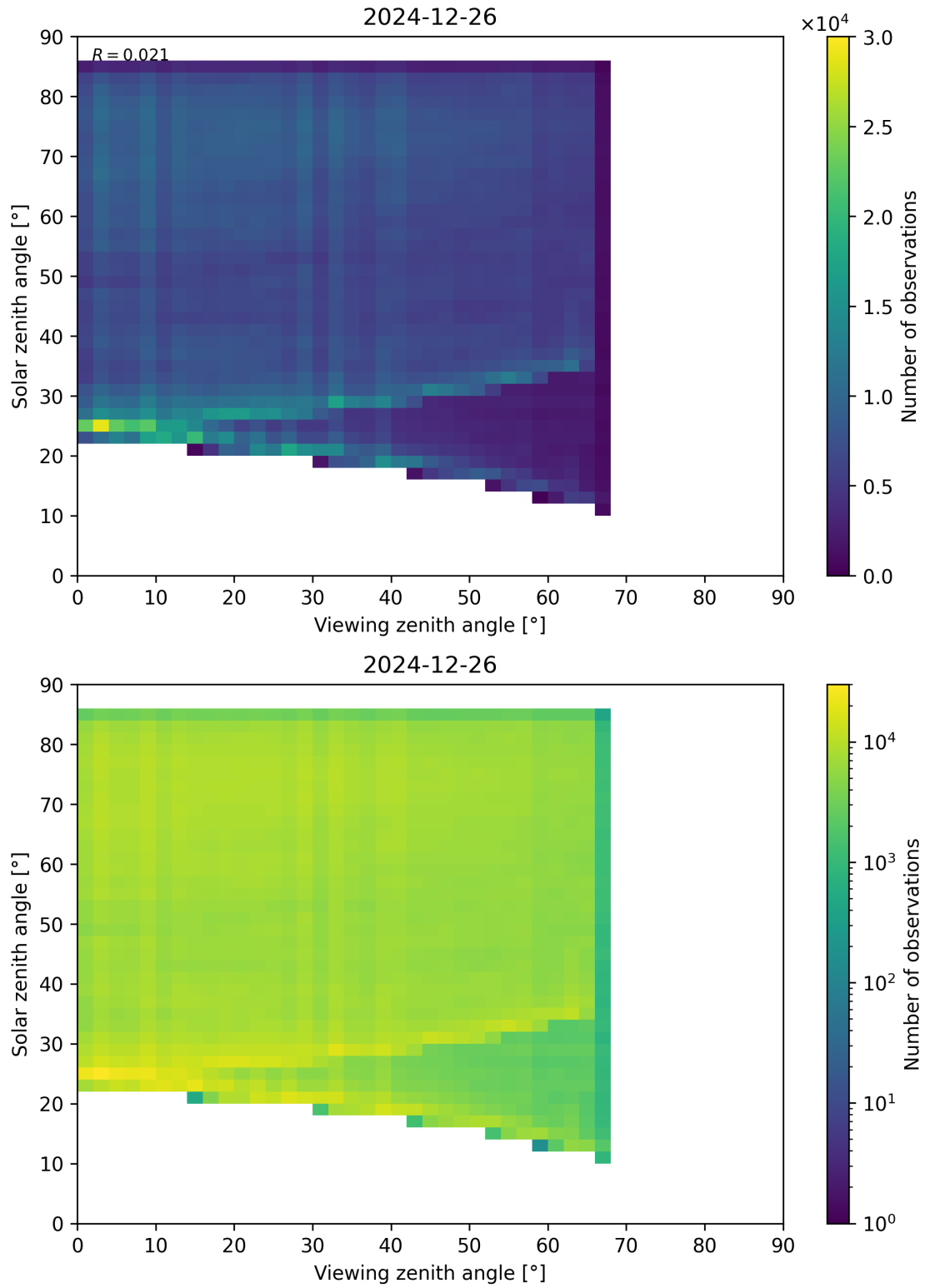
Figure 77: Scatter density plot of “Viewing zenith angle” against “Solar zenith angle” for 2024-12-25 to 2024-12-27.
