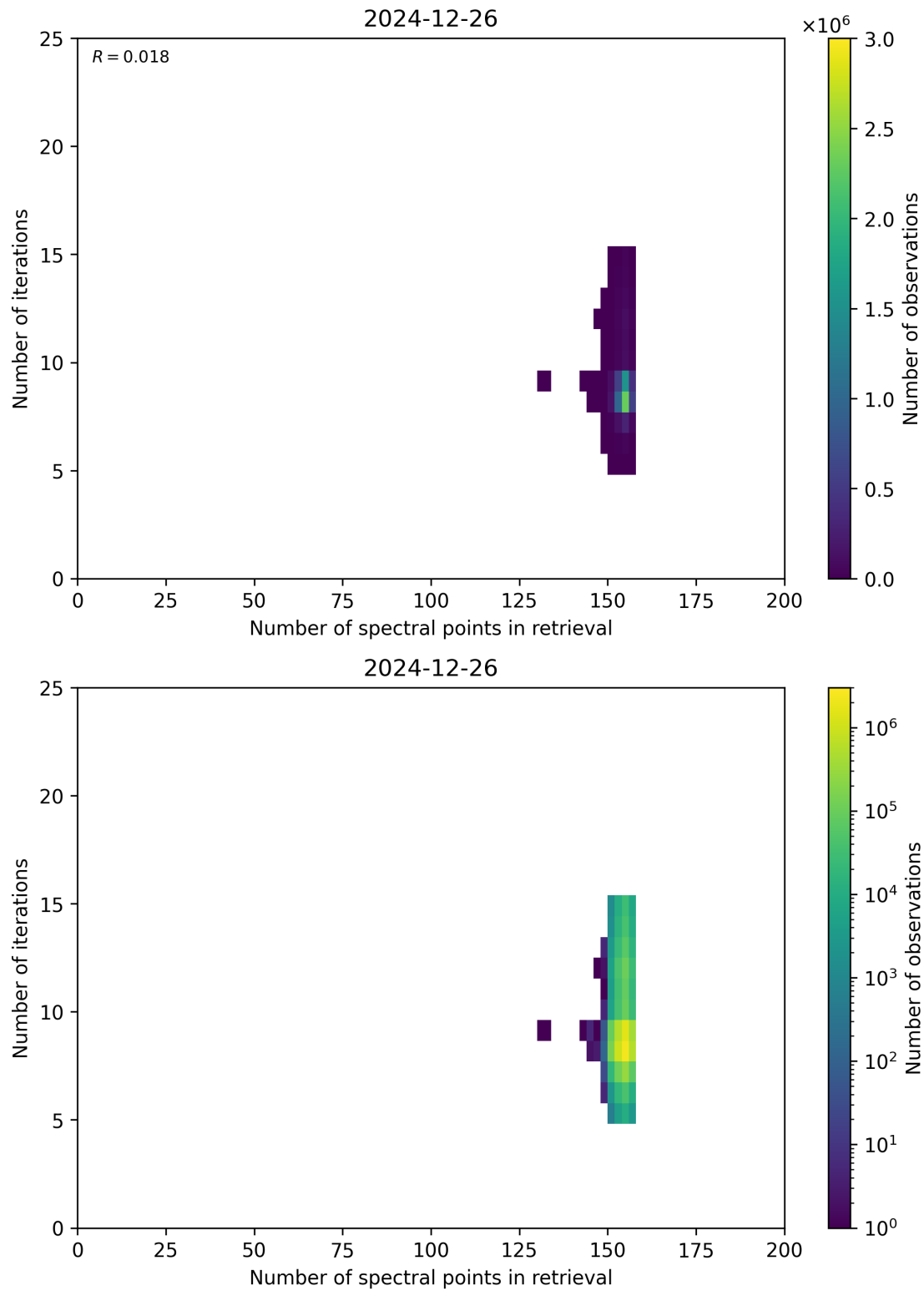
Figure 60: Scatter density plot of “Number of spectral points in retrieval” against “Number of iterations” for 2024-12-25 to 2024-12-27.
