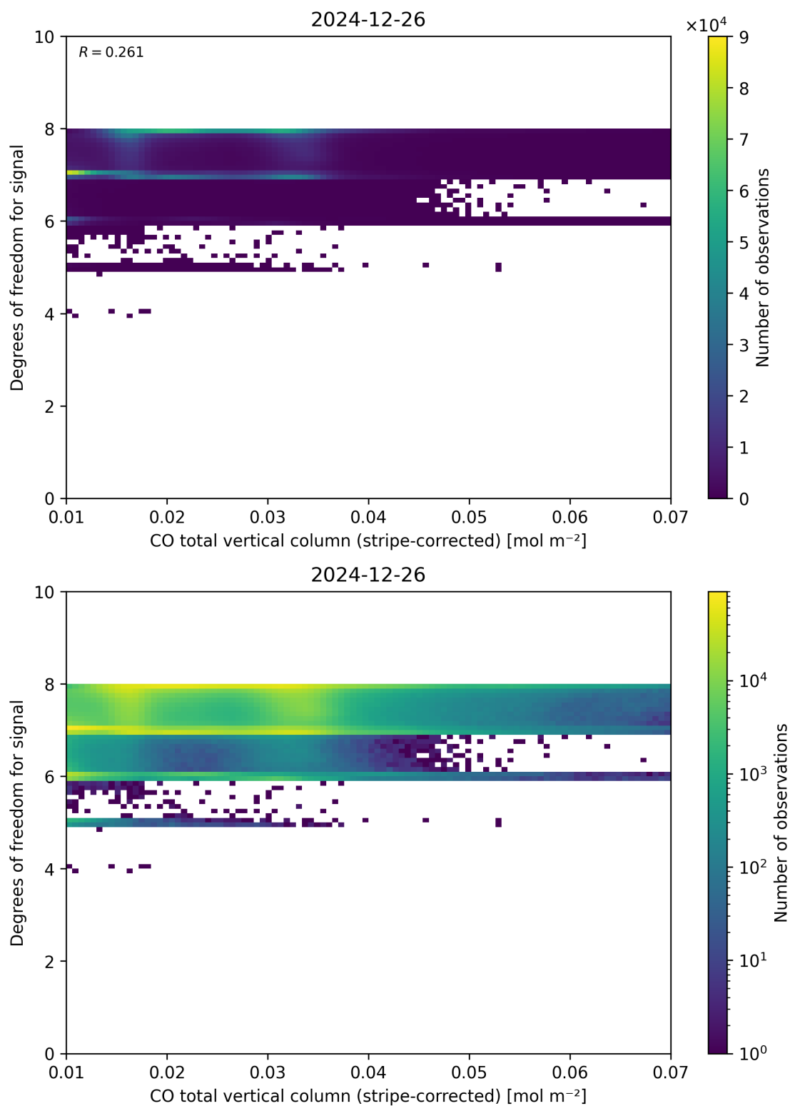
Figure 38: Scatter density plot of “CO total vertical column (stripe-corrected)” against “Degrees of freedom for signal” for 2024-12-25 to 2024-12-27.
