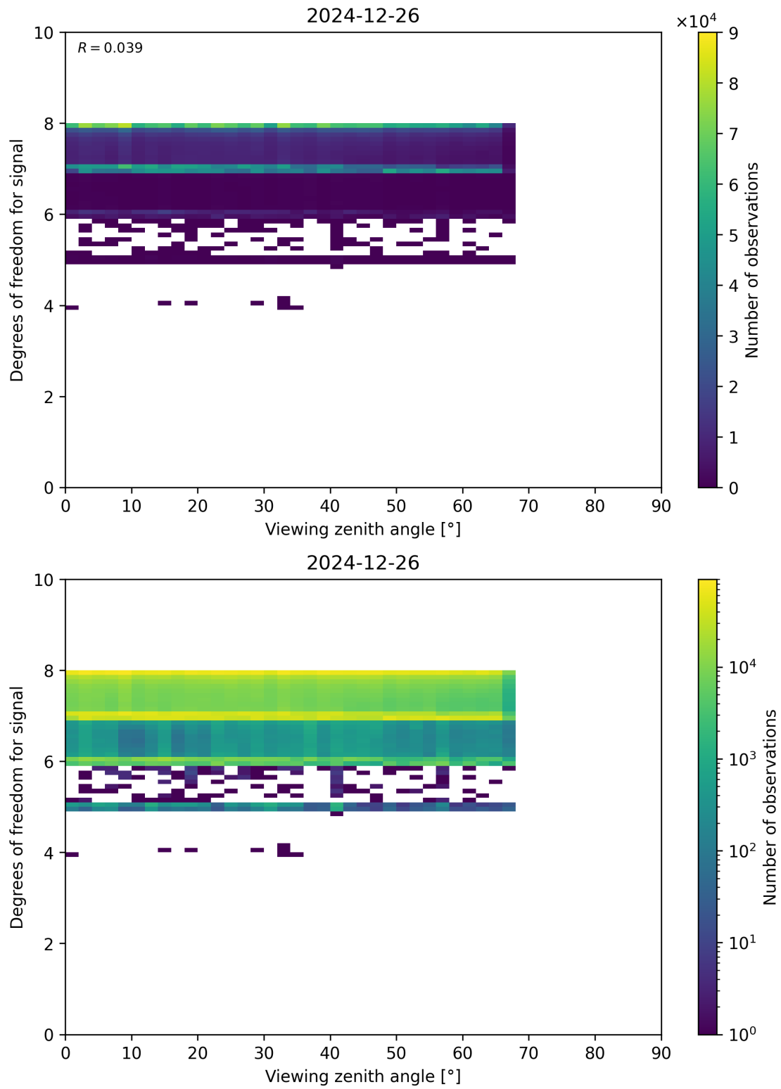
Figure 73: Scatter density plot of “Viewing zenith angle” against “Degrees of freedom for signal” for 2024-12-25 to 2024-12-27.
