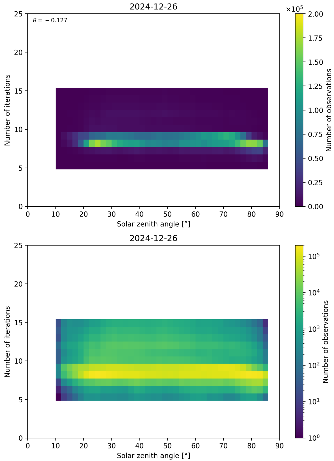
Figure 67: Scatter density plot of “Solar zenith angle” against “Number of iterations” for 2024-12-25 to 2024-12-27.
