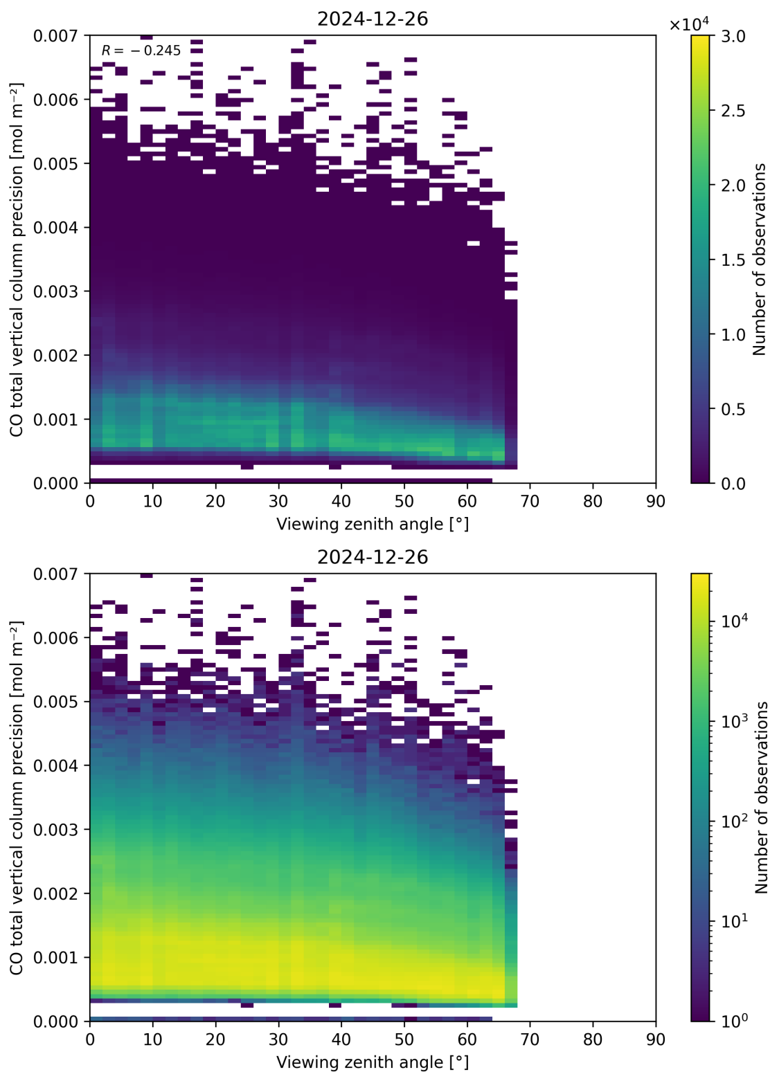
Figure 71: Scatter density plot of “Viewing zenith angle” against “CO total vertical column precision” for 2024-12-25 to 2024-12-27.
