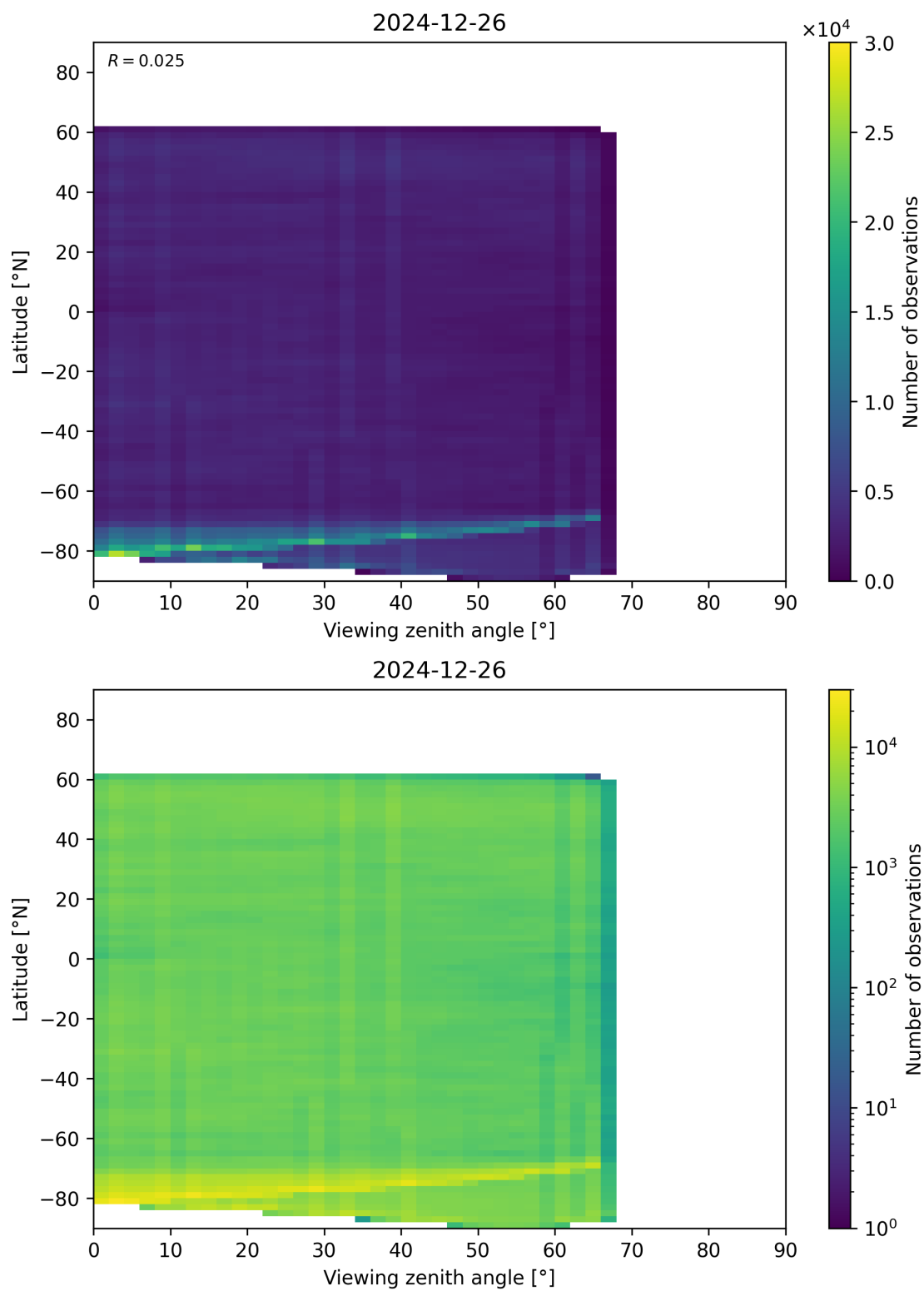
Figure 74: Scatter density plot of “Viewing zenith angle” against “Latitude” for 2024-12-25 to 2024-12-27.
