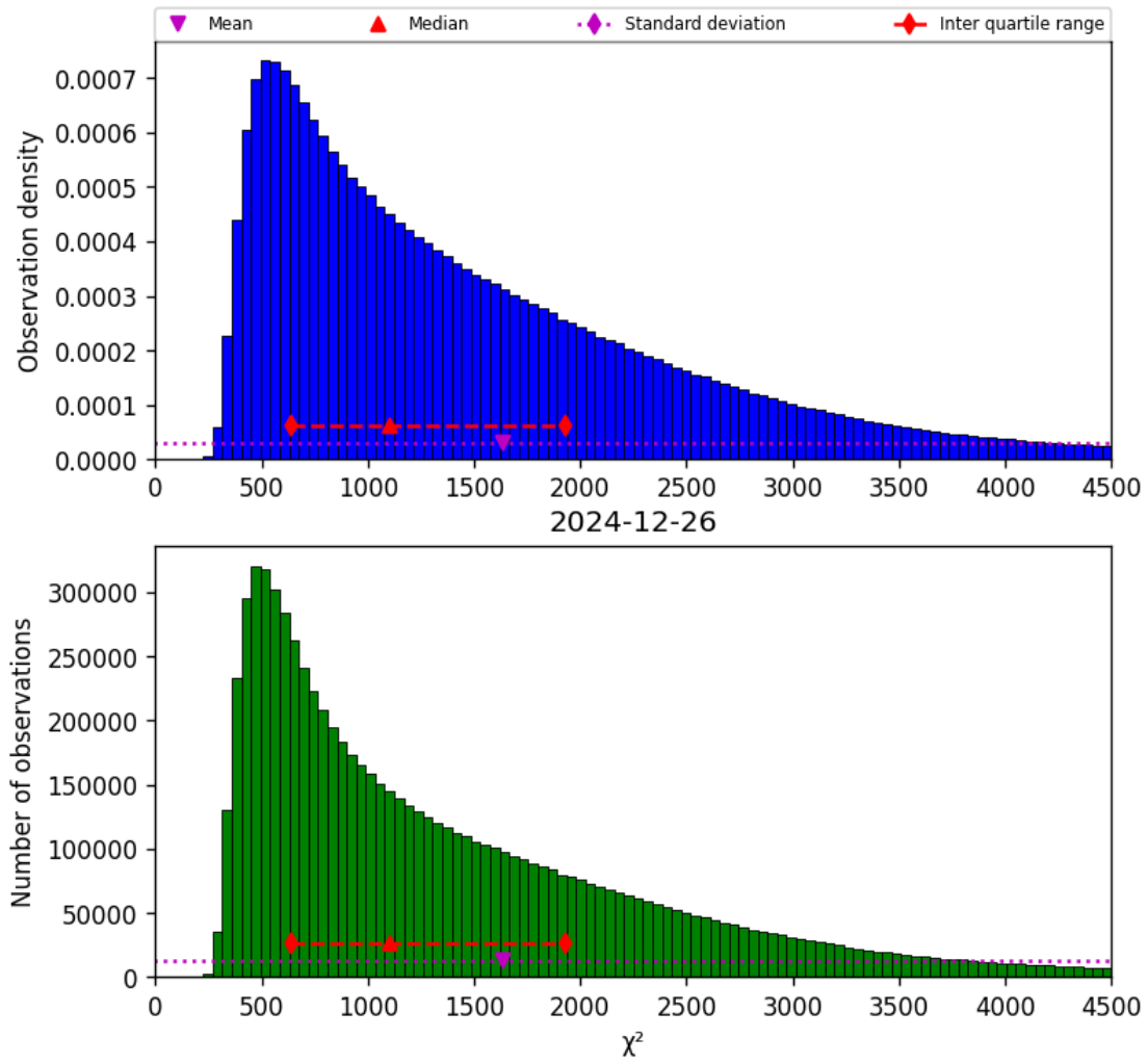
Figure 22: Histogram of “ \chi^2 ” for 2024-12-25 to 2024-12-27
