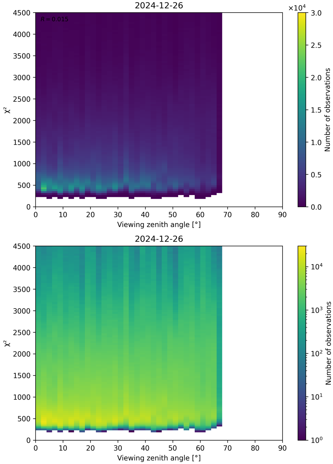
Figure 72: Scatter density plot of “Viewing zenith angle” against “ \chi^2 ” for 2024-12-25 to 2024-12-27.
