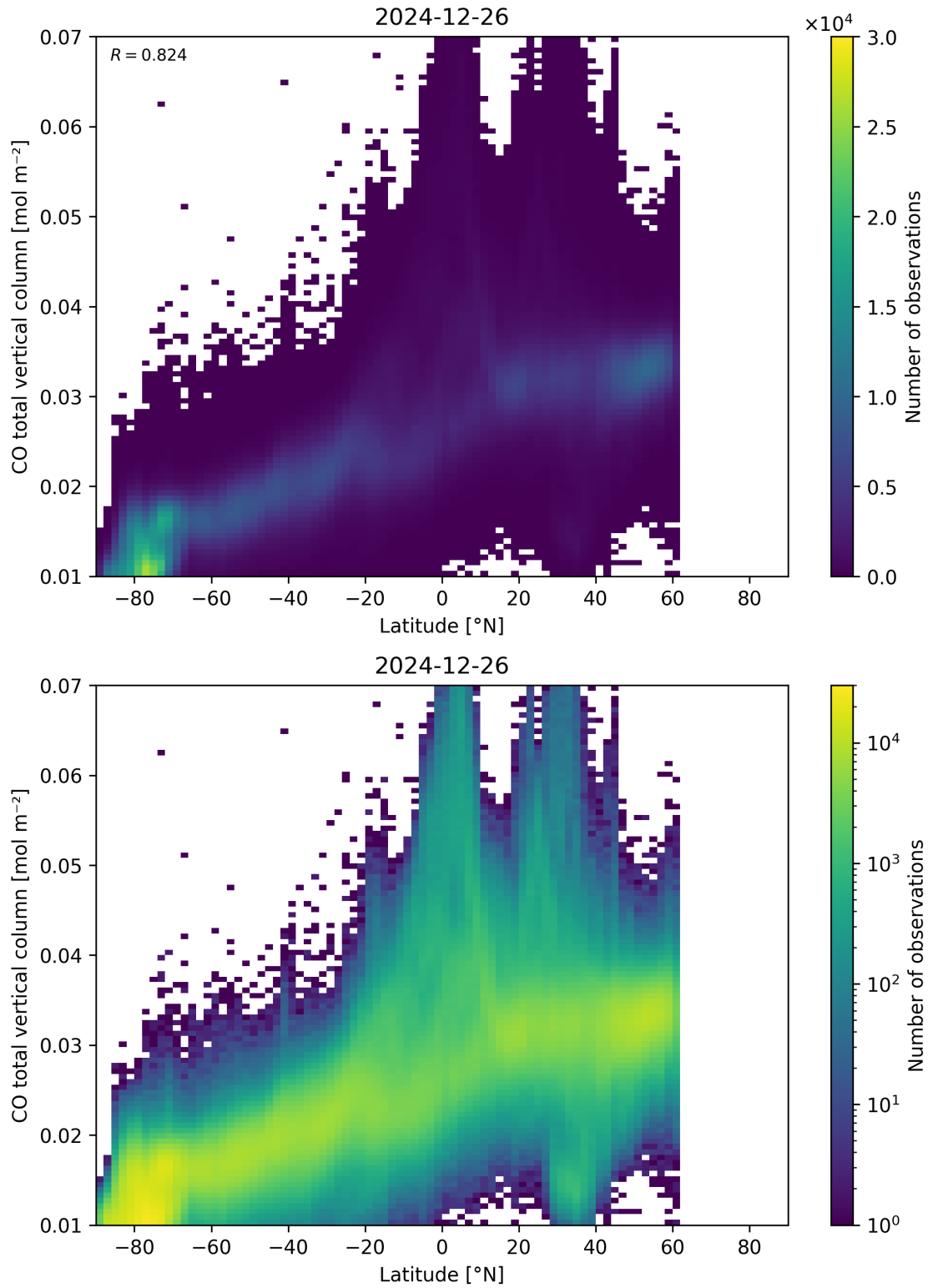
Figure 51: Scatter density plot of “Latitude” against “CO total vertical column” for 2024-12-25 to 2024-12-27.
