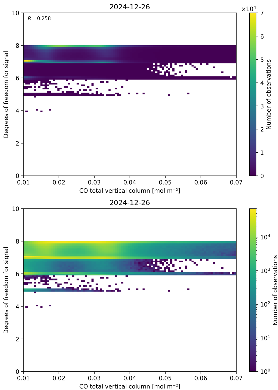
Figure 41: Scatter density plot of “CO total vertical column” against “Degrees of freedom for signal” for 2024-12-25 to 2024-12-27.
