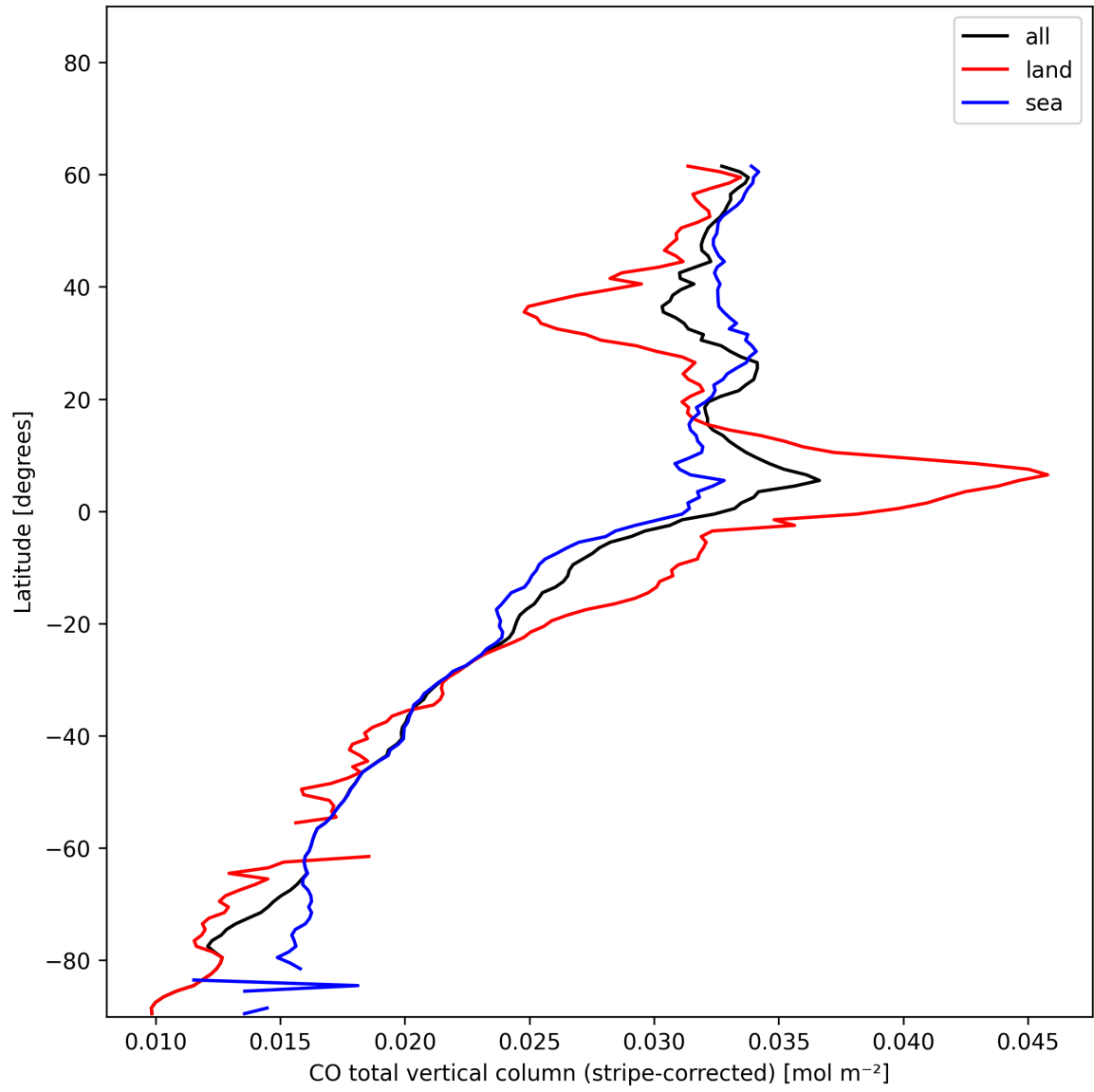
Figure 11: Zonal average of “CO total vertical column (stripe-corrected)” for 2024-12-25 to 2024-12-27.
