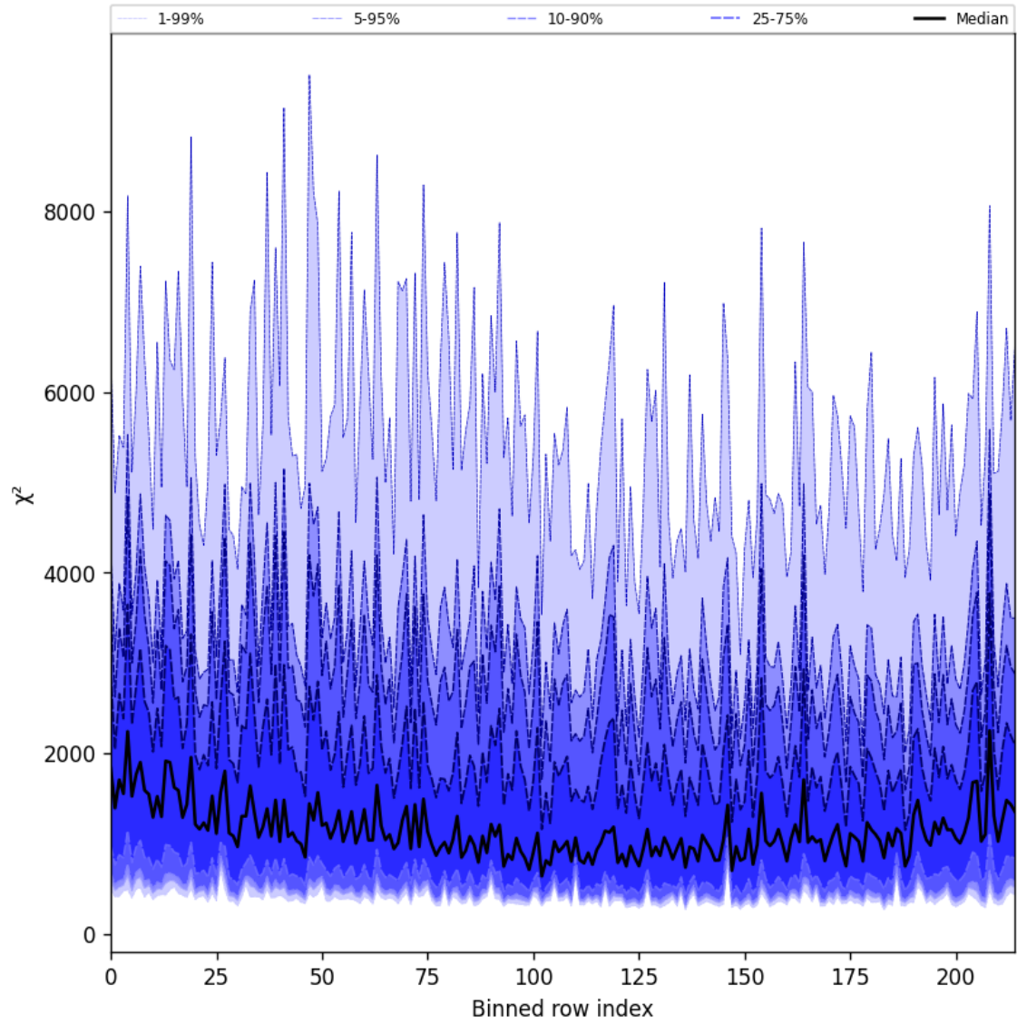
Figure 30: Along track statistics of “ \chi^2 ” for 2024-12-25 to 2024-12-27
