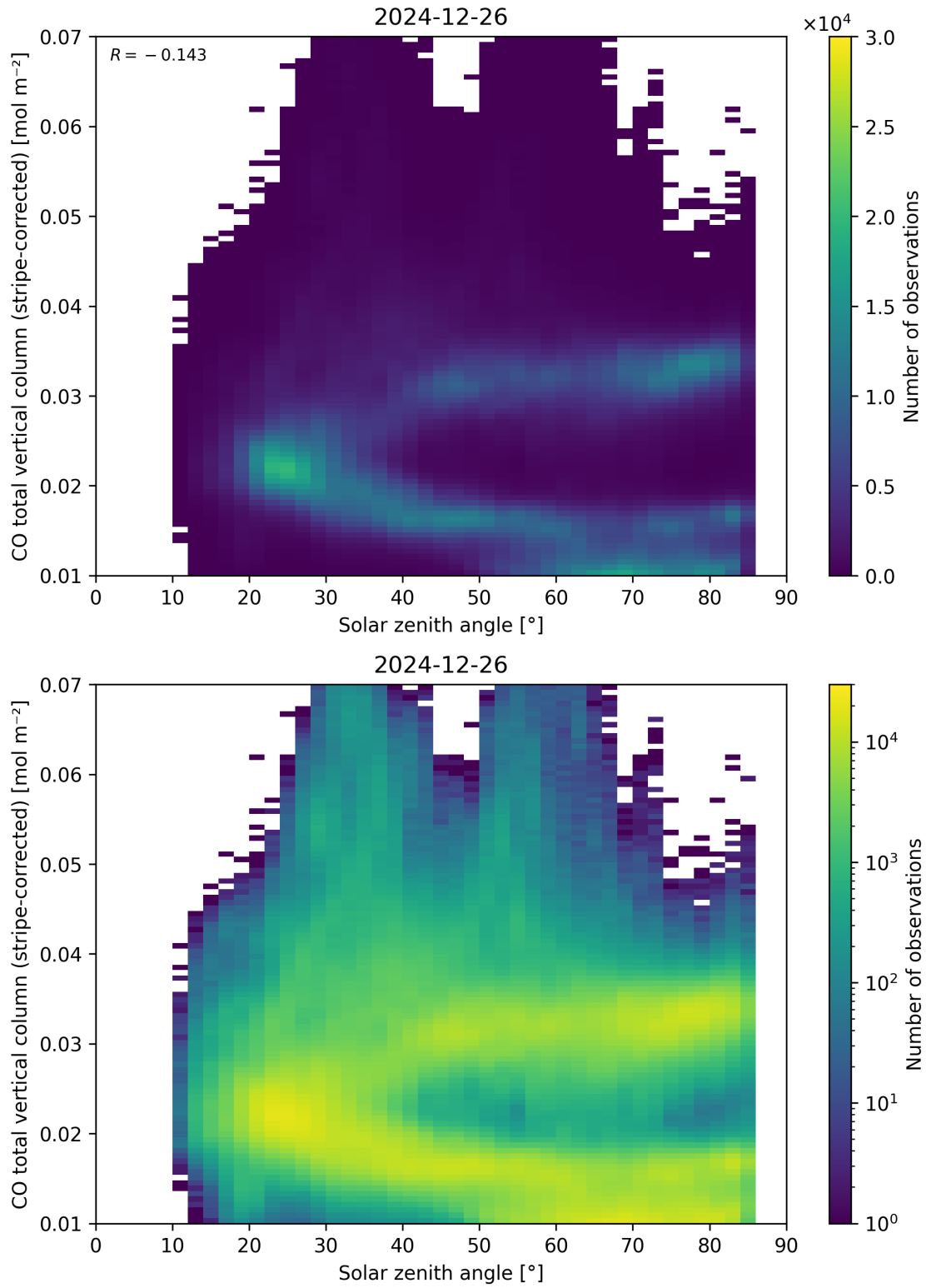
Figure 62: Scatter density plot of “Solar zenith angle” against “CO total vertical column (stripe-corrected)” for 2024-12-25 to 2024-12-27.
