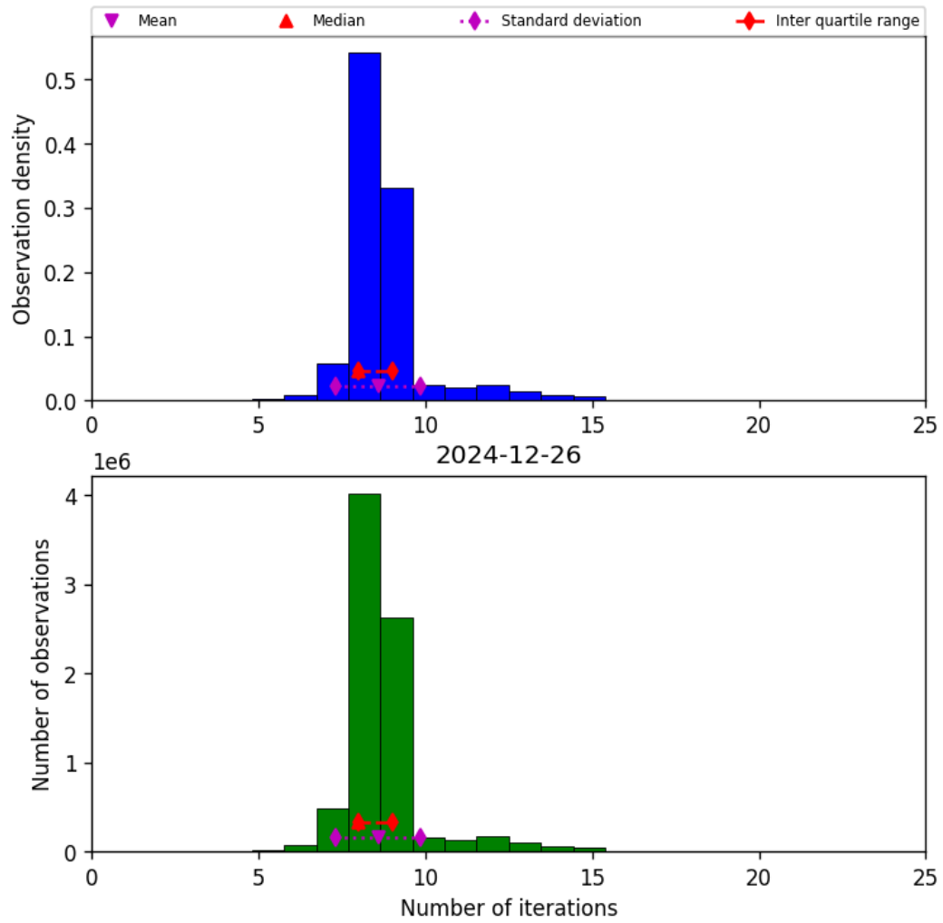
Figure 24: Histogram of “Number of iterations” for 2024-12-25 to 2024-12-27
