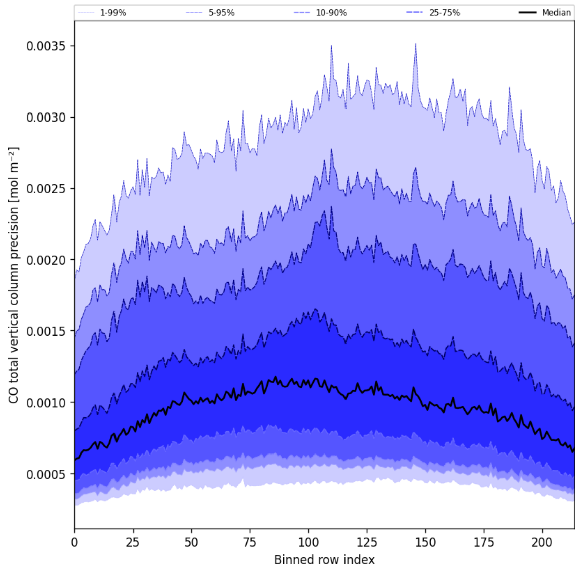
Figure 28: Along track statistics of “CO total vertical column precision” for 2024-12-25 to 2024-12-27
