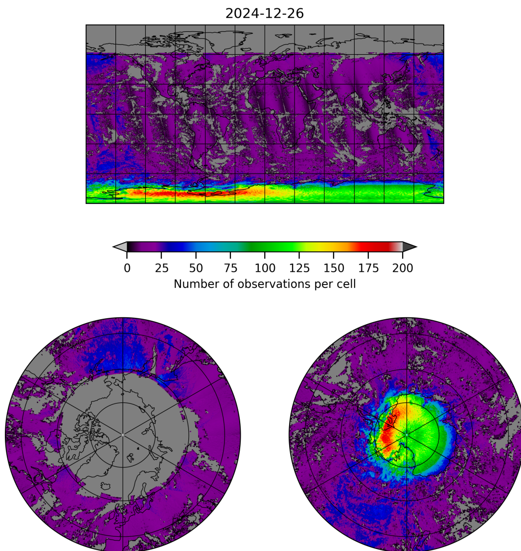
Figure 8: Map of the number of observations for 2024-12-25 to 2024-12-27
