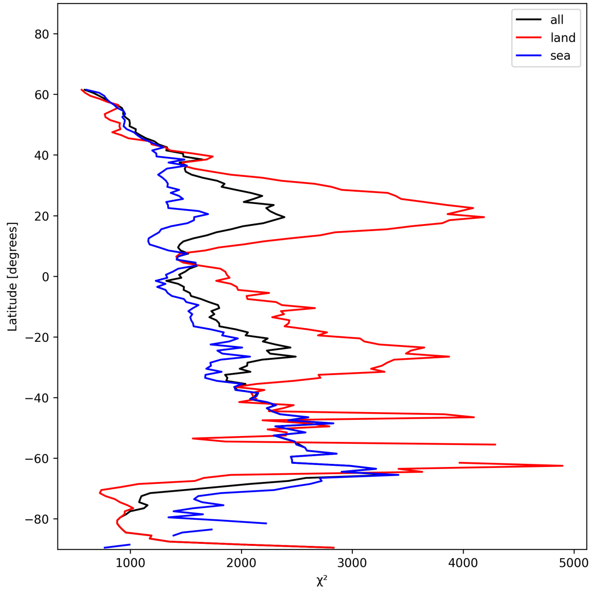
Figure 14: Zonal average of “ \chi^2 ” for 2024-12-25 to 2024-12-27.
