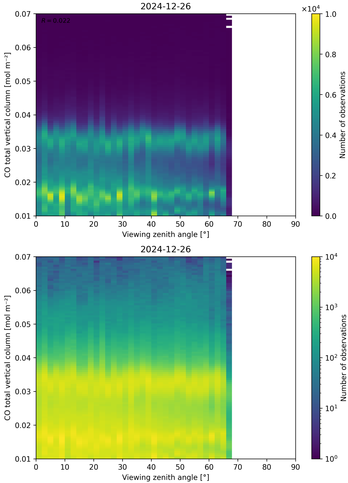
Figure 69: Scatter density plot of “Viewing zenith angle” against “CO total vertical column” for 2024-12-25 to 2024-12-27.
