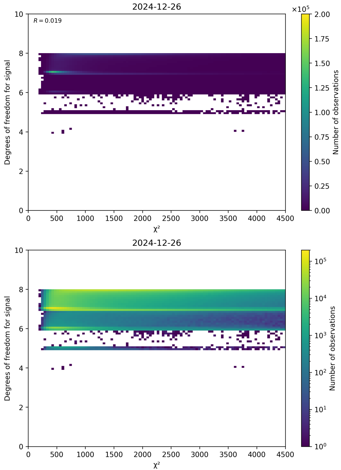
Figure 48: Scatter density plot of “ \chi^2 ” against “Degrees of freedom for signal” for 2024-12-25 to 2024-12-27.
