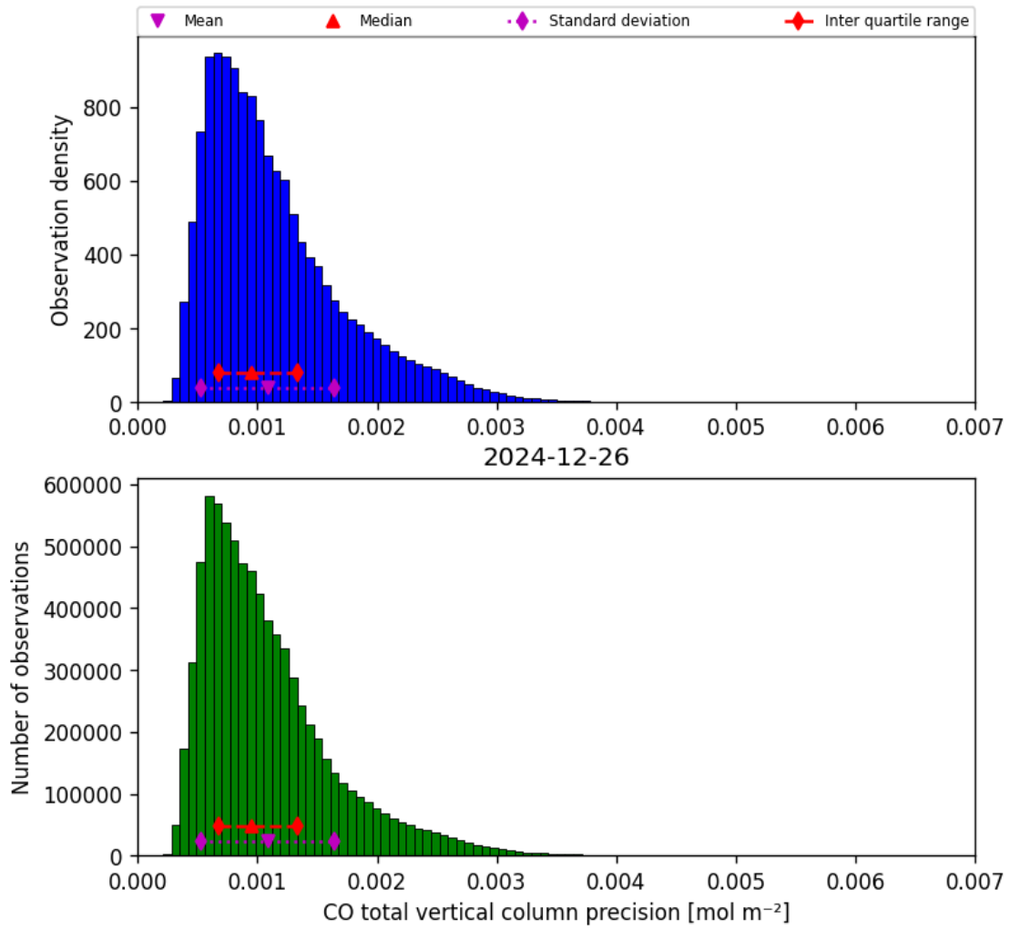
Figure 20: Histogram of “CO total vertical column precision” for 2024-12-25 to 2024-12-27
