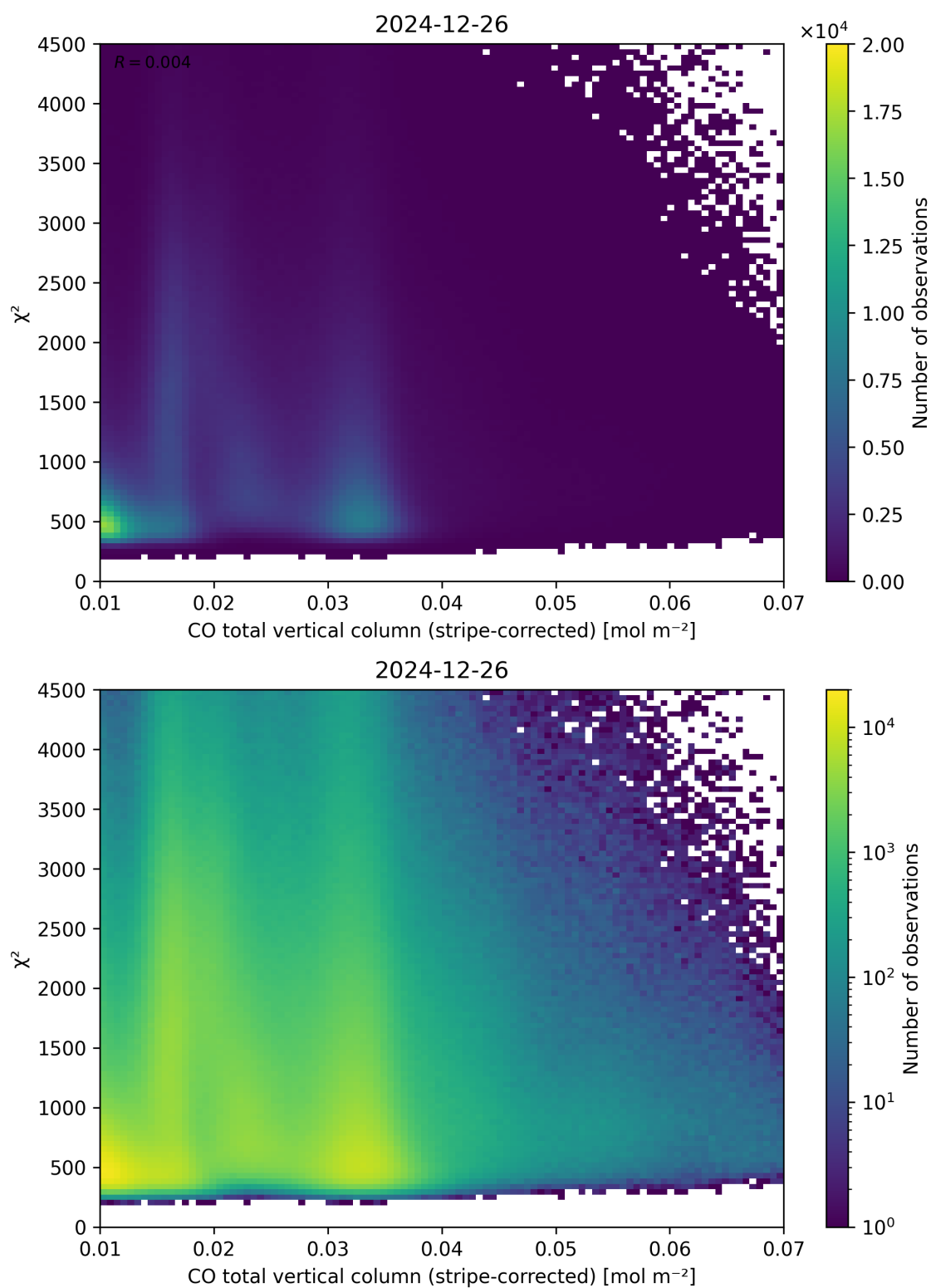
Figure 37: Scatter density plot of “CO total vertical column (stripe-corrected)” against “ \chi^2 ” for 2024-12-25 to 2024-12-27.
