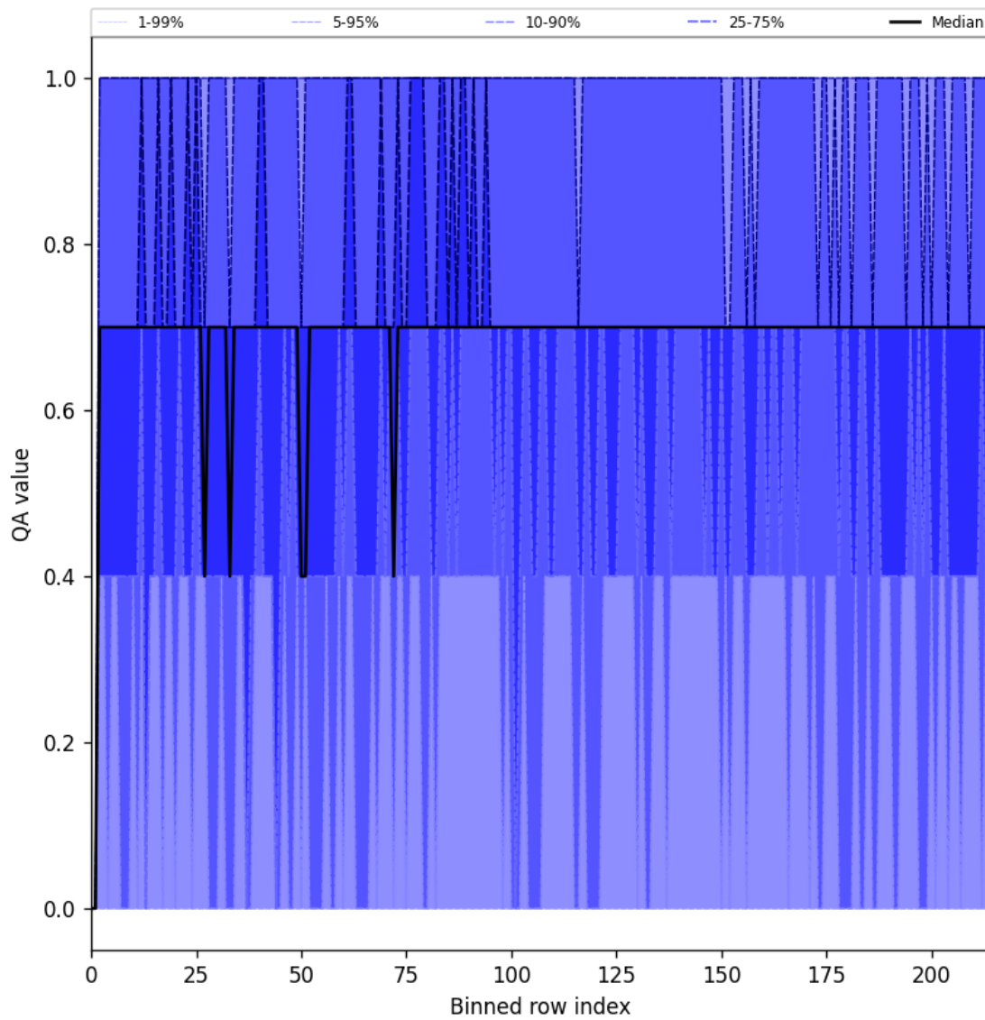
Figure 25: Along track statistics of “QA value” for 2024-12-25 to 2024-12-27
