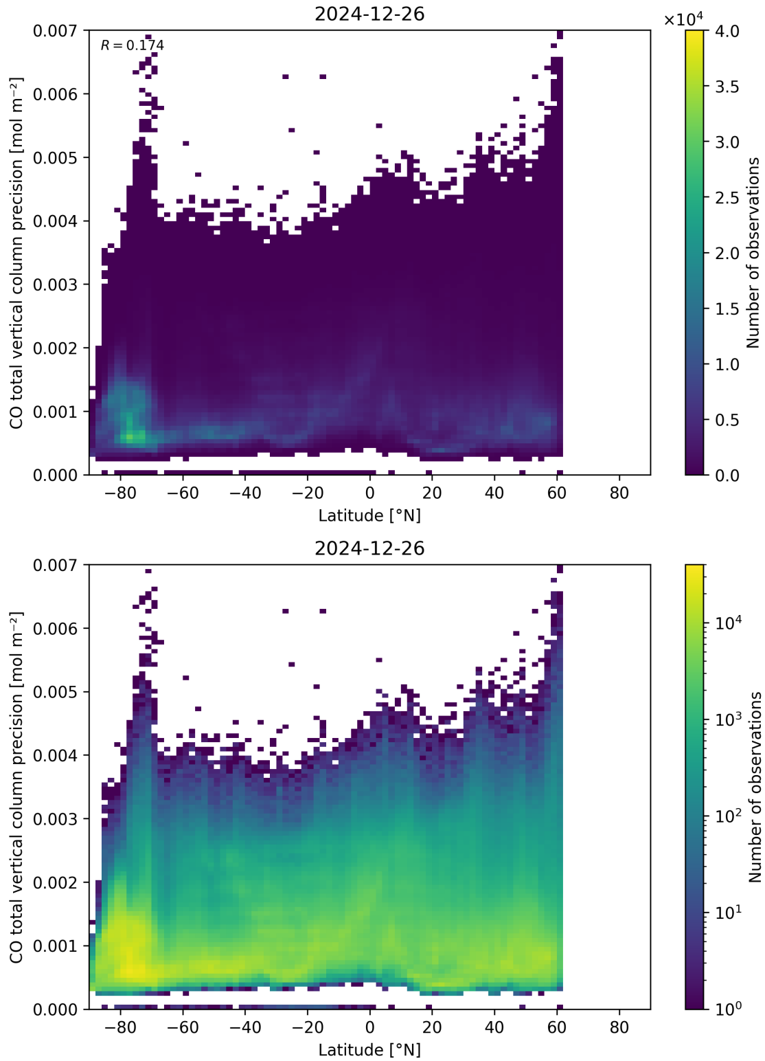
Figure 53: Scatter density plot of “Latitude” against “CO total vertical column precision” for 2024-12-25 to 2024-12-27.
