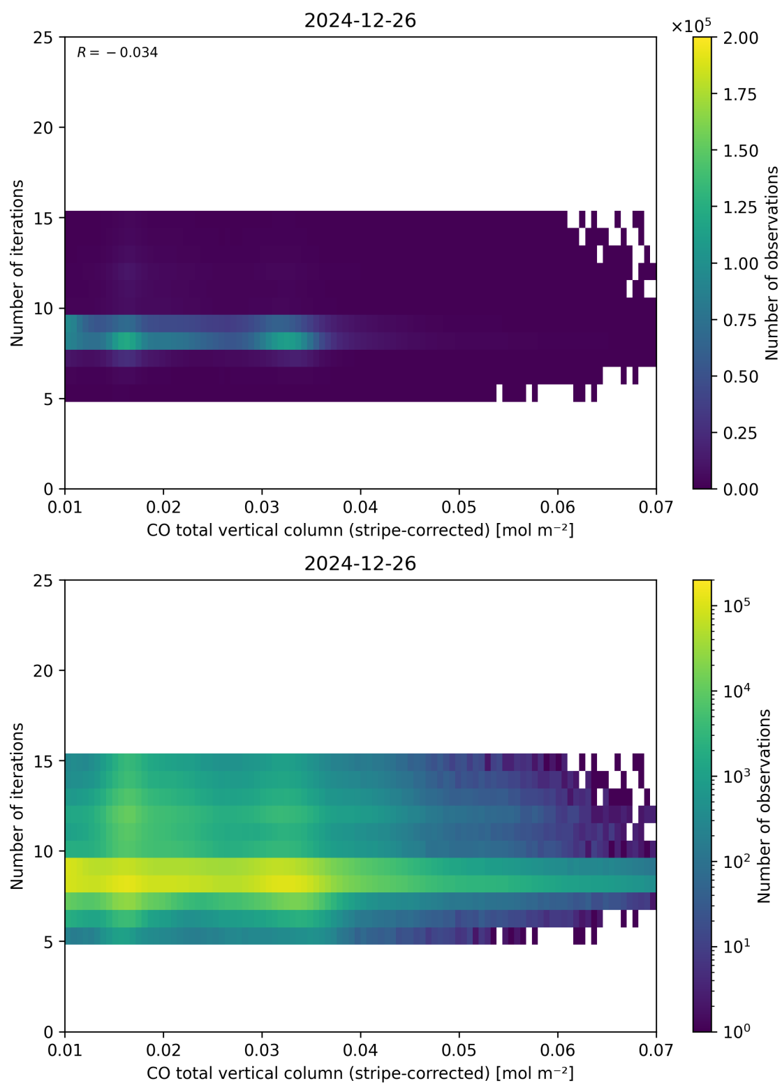
Figure 39: Scatter density plot of “CO total vertical column (stripe-corrected)” against “Number of iterations” for 2024-12-25 to 2024-12-27.
