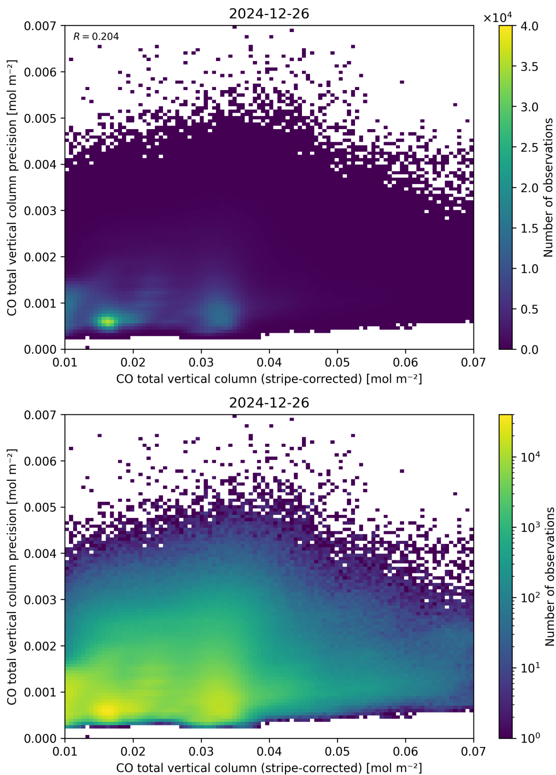
Figure 36: Scatter density plot of “CO total vertical column (stripe-corrected)” against “CO total vertical column precision” for 2024-12-25 to 2024-12-27.
