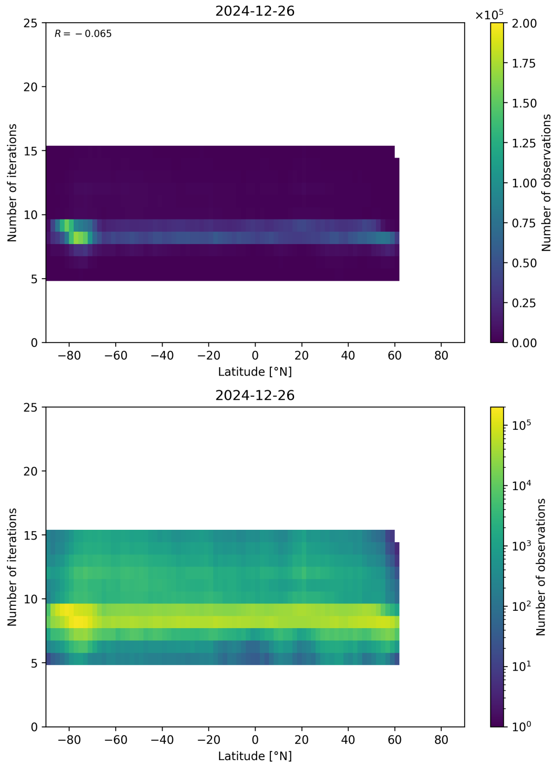
Figure 56: Scatter density plot of “Latitude” against “Number of iterations” for 2024-12-25 to 2024-12-27.
