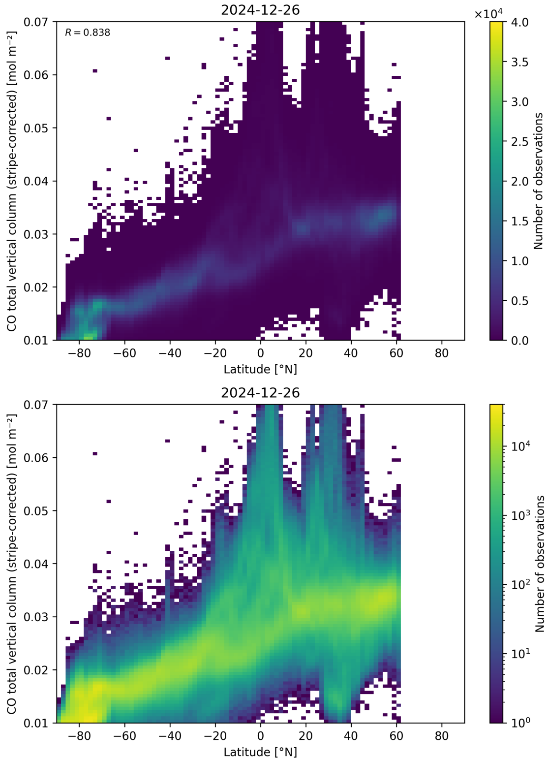
Figure 52: Scatter density plot of “Latitude” against “CO total vertical column (stripe-corrected)” for 2024-12-25 to 2024-12-27.
