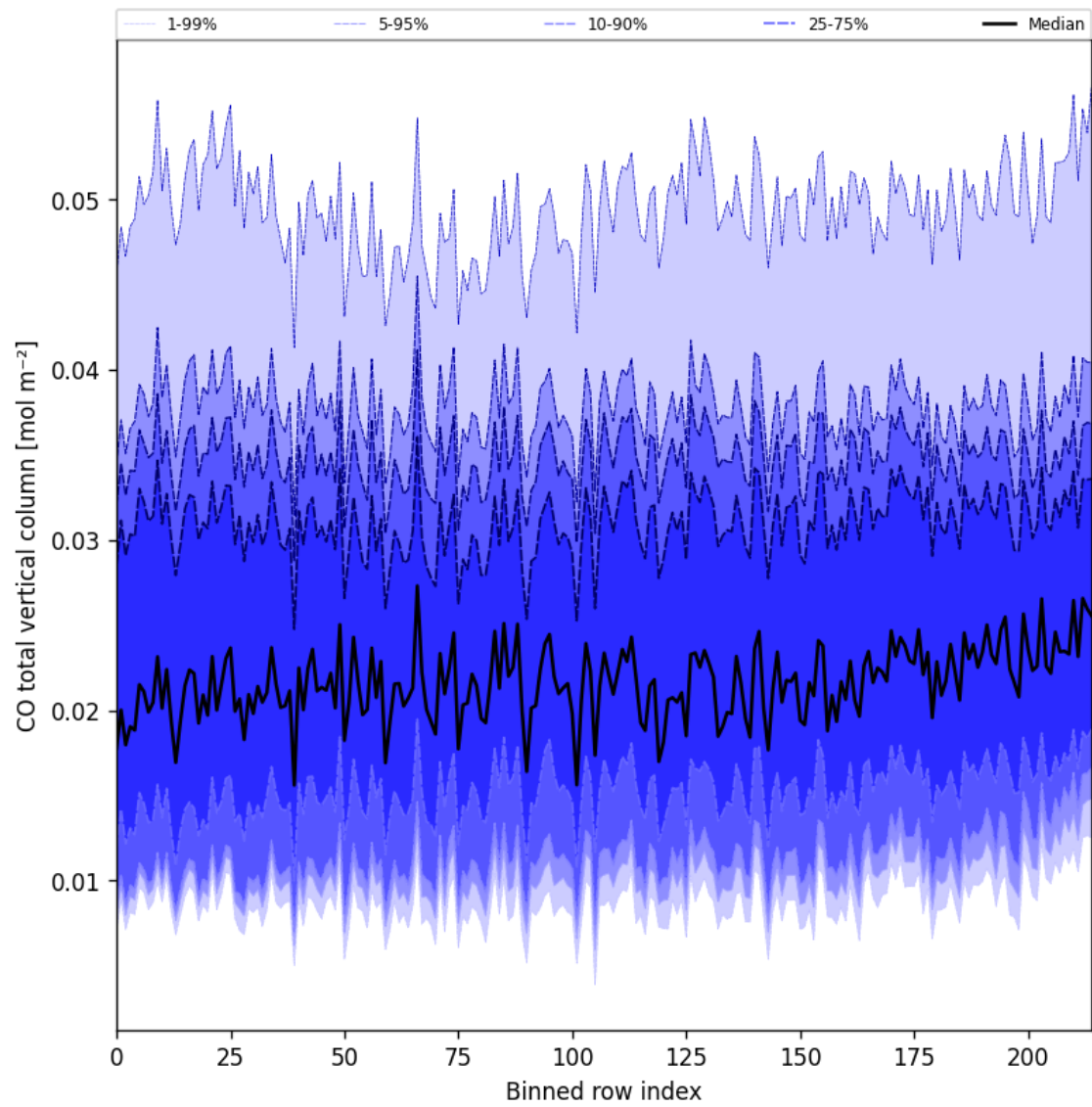
Figure 26: Along track statistics of “CO total vertical column” for 2024-12-25 to 2024-12-27
