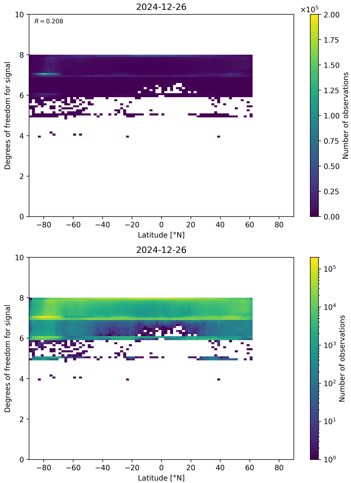
Figure 55: Scatter density plot of “Latitude” against “Degrees of freedom for signal” for 2024-12-25 to 2024-12-27.
