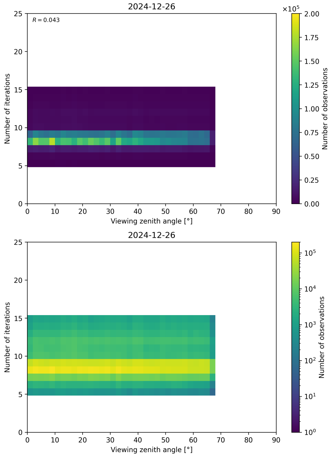
Figure 75: Scatter density plot of “Viewing zenith angle” against “Number of iterations” for 2024-12-25 to 2024-12-27.
