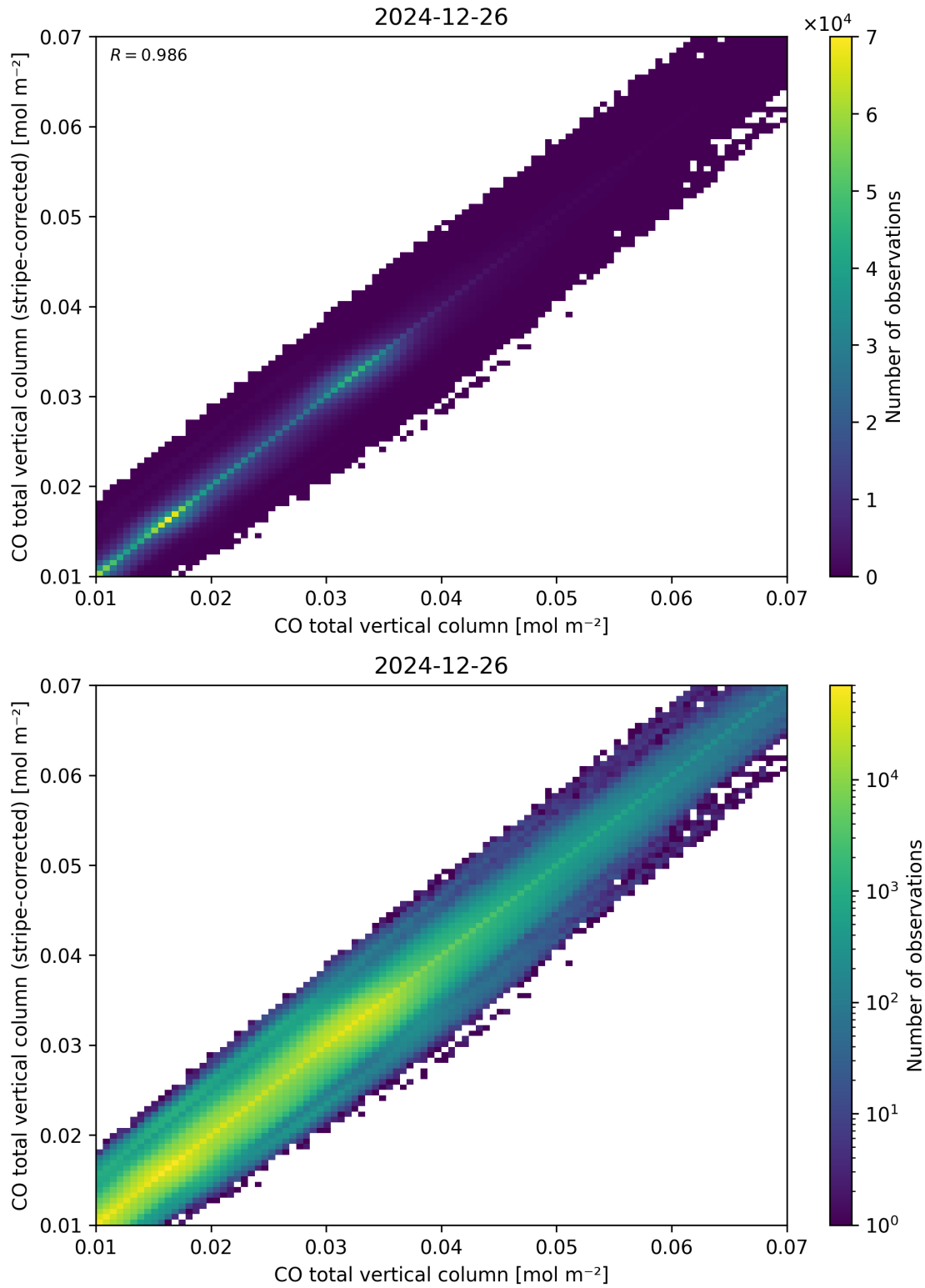
Figure 33: Scatter density plot of “CO total vertical column” against “CO total vertical column (stripe-corrected)” for 2024-12-25 to 2024-12-27.
