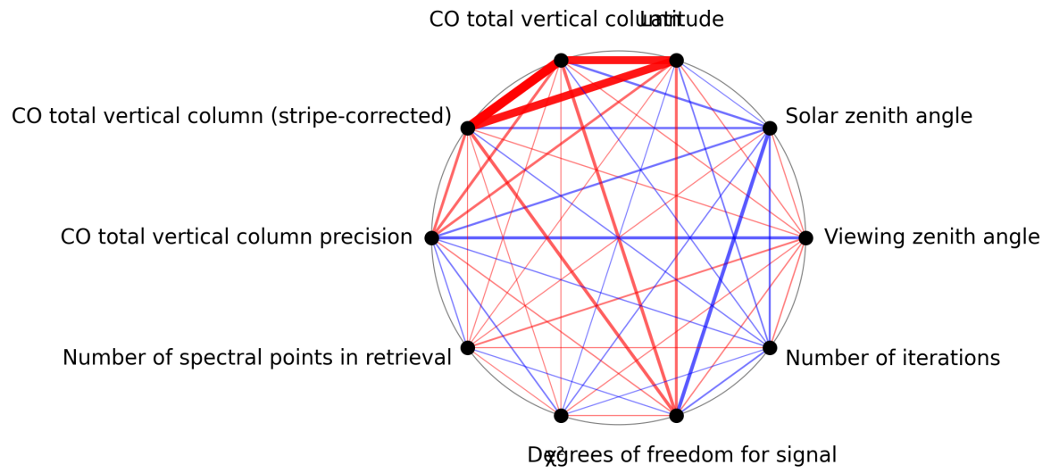
Figure 1: Map of correlation graph for 2024-12-25 to 2024-12-27.
