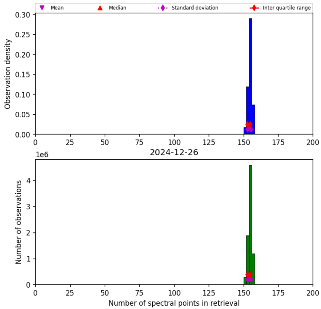
Figure 21: Histogram of “Number of spectral points in retrieval” for 2024-12-25 to 2024-12-27
