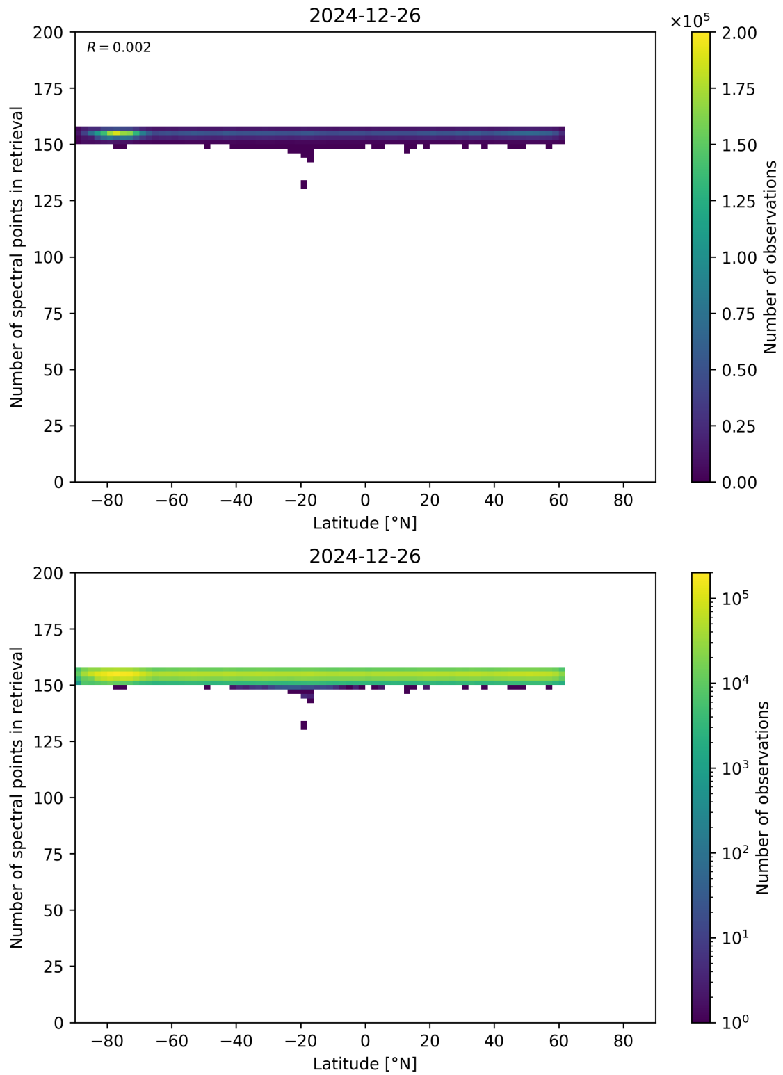
Figure 57: Scatter density plot of “Latitude” against “Number of spectral points in retrieval” for 2024-12-25 to 2024-12-27.
