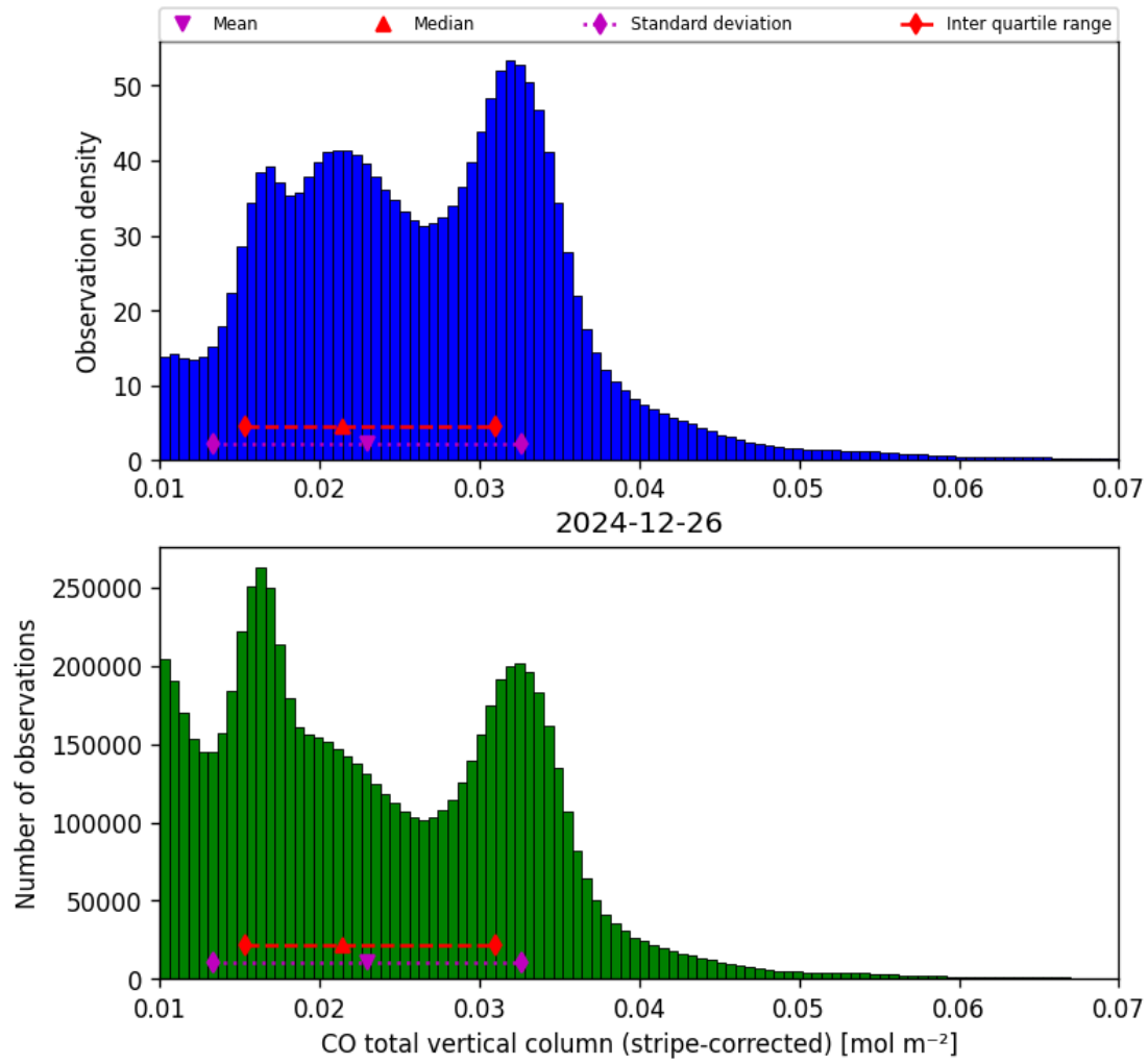
Figure 19: Histogram of “CO total vertical column (stripe-corrected)” for 2024-12-25 to 2024-12-27
