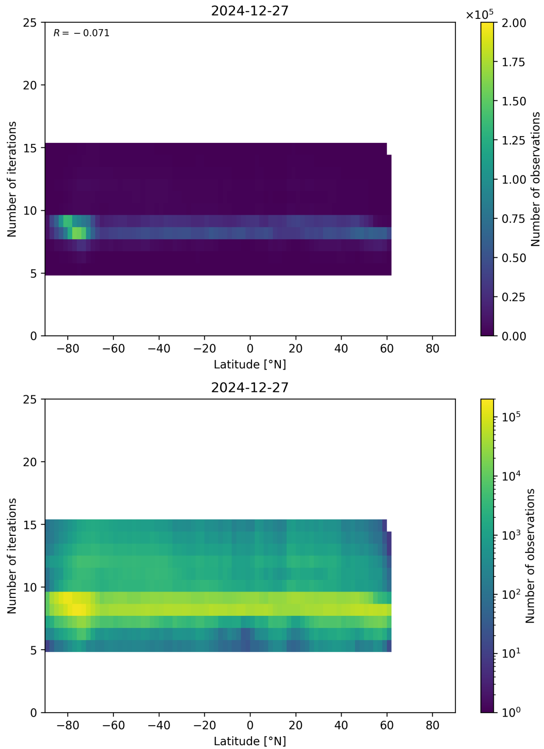
Figure 56: Scatter density plot of “Latitude” against “Number of iterations” for 2024-12-27 to 2024-12-28.
