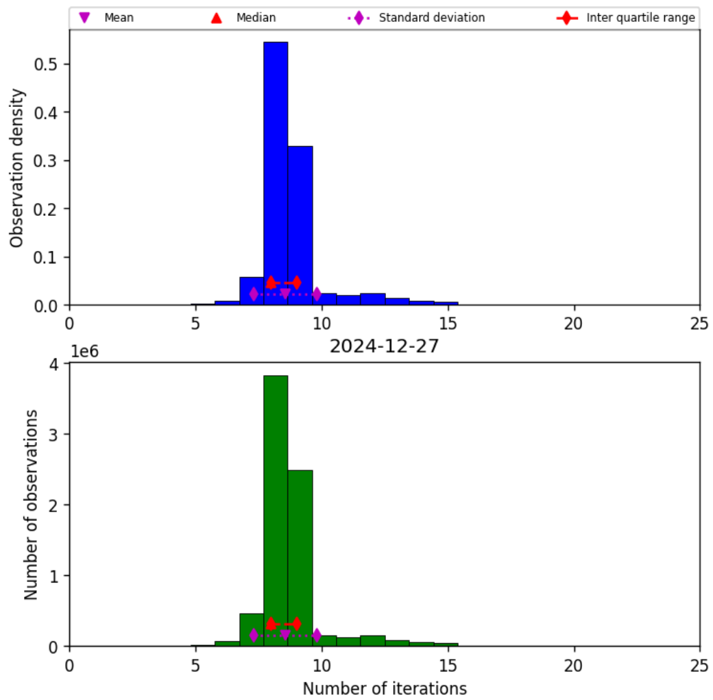
Figure 24: Histogram of “Number of iterations” for 2024-12-27 to 2024-12-28
