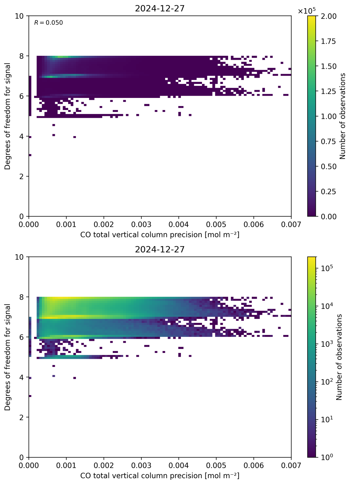
Figure 45: Scatter density plot of “CO total vertical column precision” against “Degrees of freedom for signal” for 2024-12-27 to 2024-12-28.
