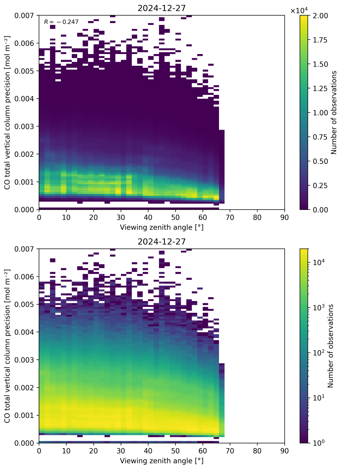
Figure 71: Scatter density plot of “Viewing zenith angle” against “CO total vertical column precision” for 2024-12-27 to 2024-12-28.
