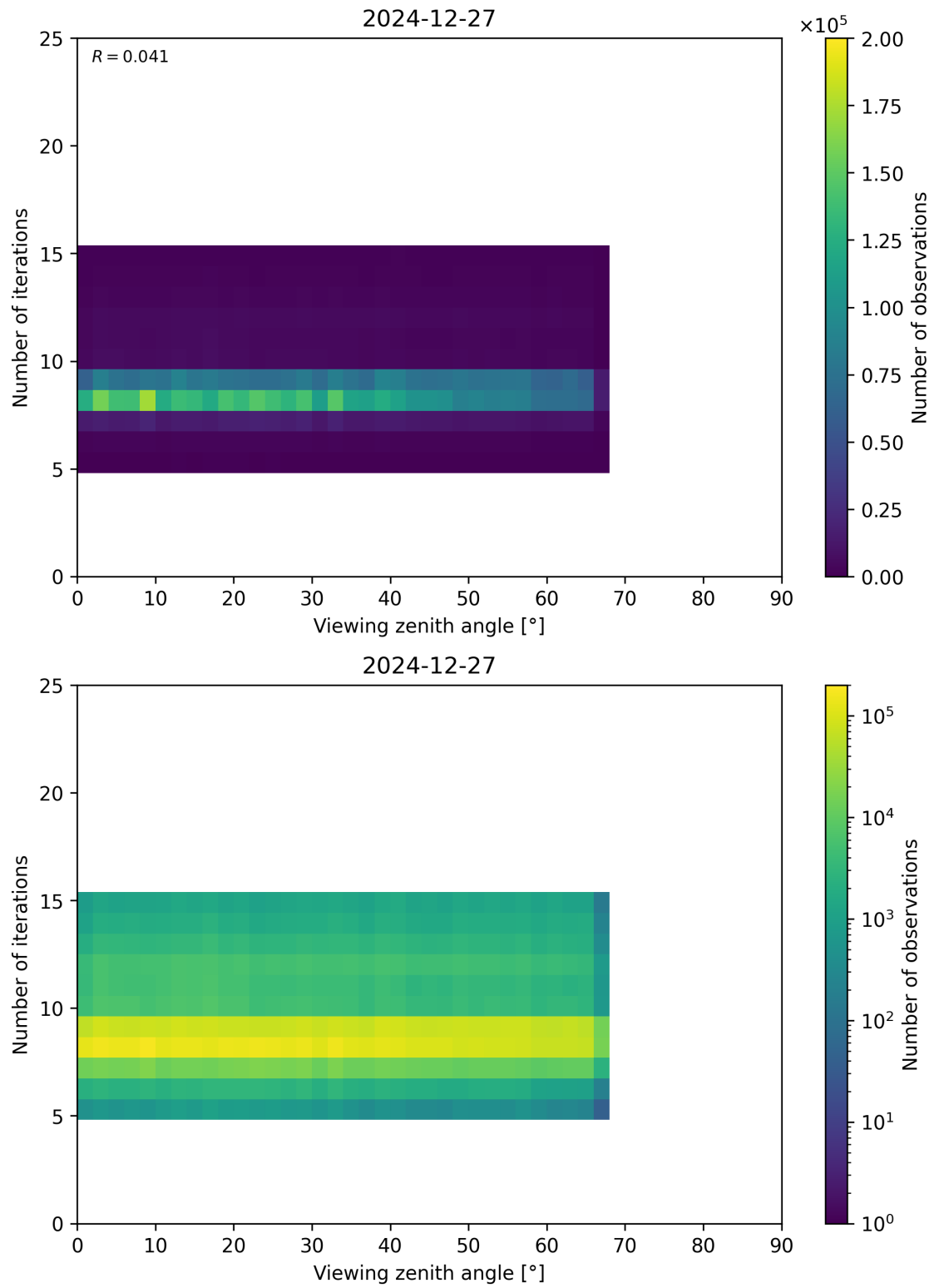
Figure 75: Scatter density plot of “Viewing zenith angle” against “Number of iterations” for 2024-12-27 to 2024-12-28.
