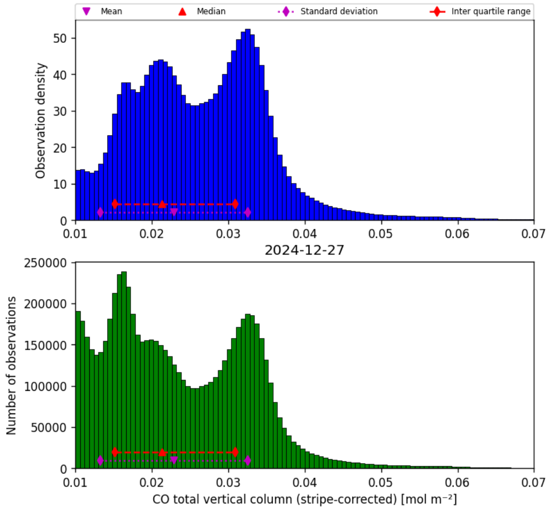
Figure 19: Histogram of “CO total vertical column (stripe-corrected)” for 2024-12-27 to 2024-12-28
