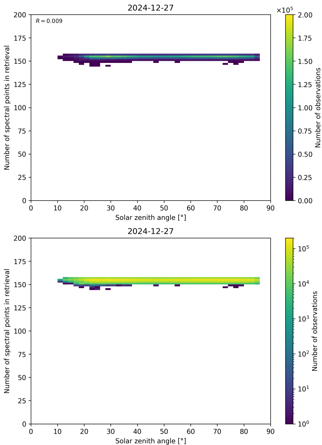
Figure 68: Scatter density plot of “Solar zenith angle” against “Number of spectral points in retrieval” for 2024-12-27 to 2024-12-28.
