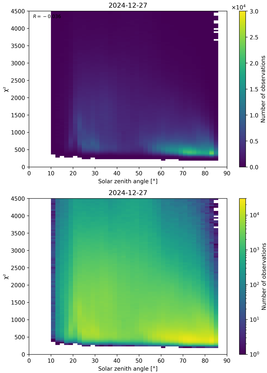
Figure 64: Scatter density plot of “Solar zenith angle” against “ \chi^2 ” for 2024-12-27 to 2024-12-28.
