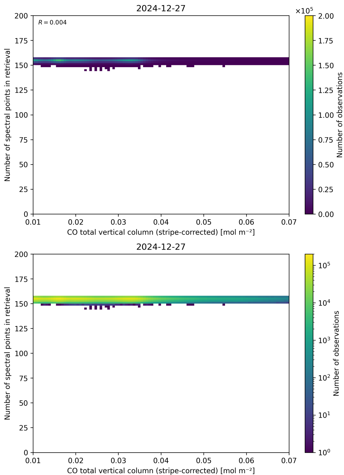
Figure 40: Scatter density plot of “CO total vertical column (stripe-corrected)” against “Number of spectral points in retrieval” for 2024-12-27 to 2024-12-28.
