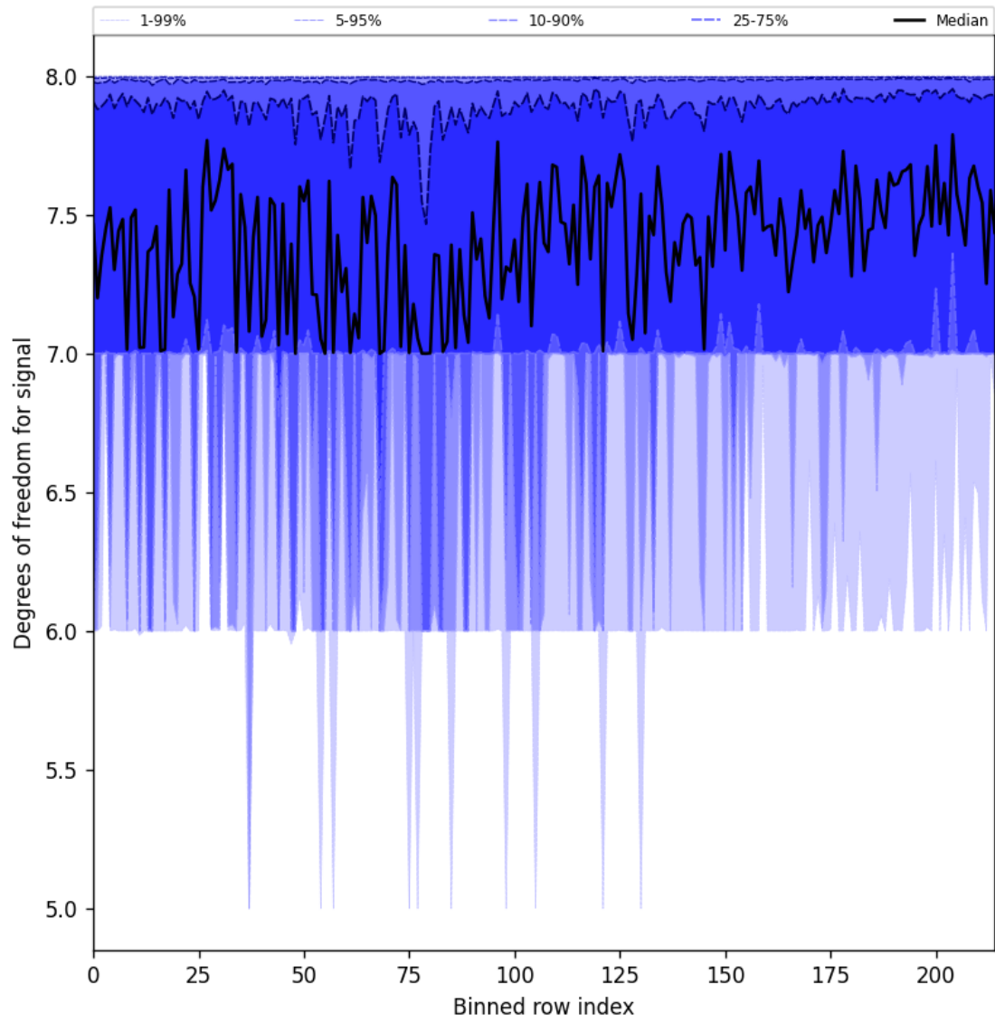
Figure 31: Along track statistics of “Degrees of freedom for signal” for 2024-12-27 to 2024-12-28
