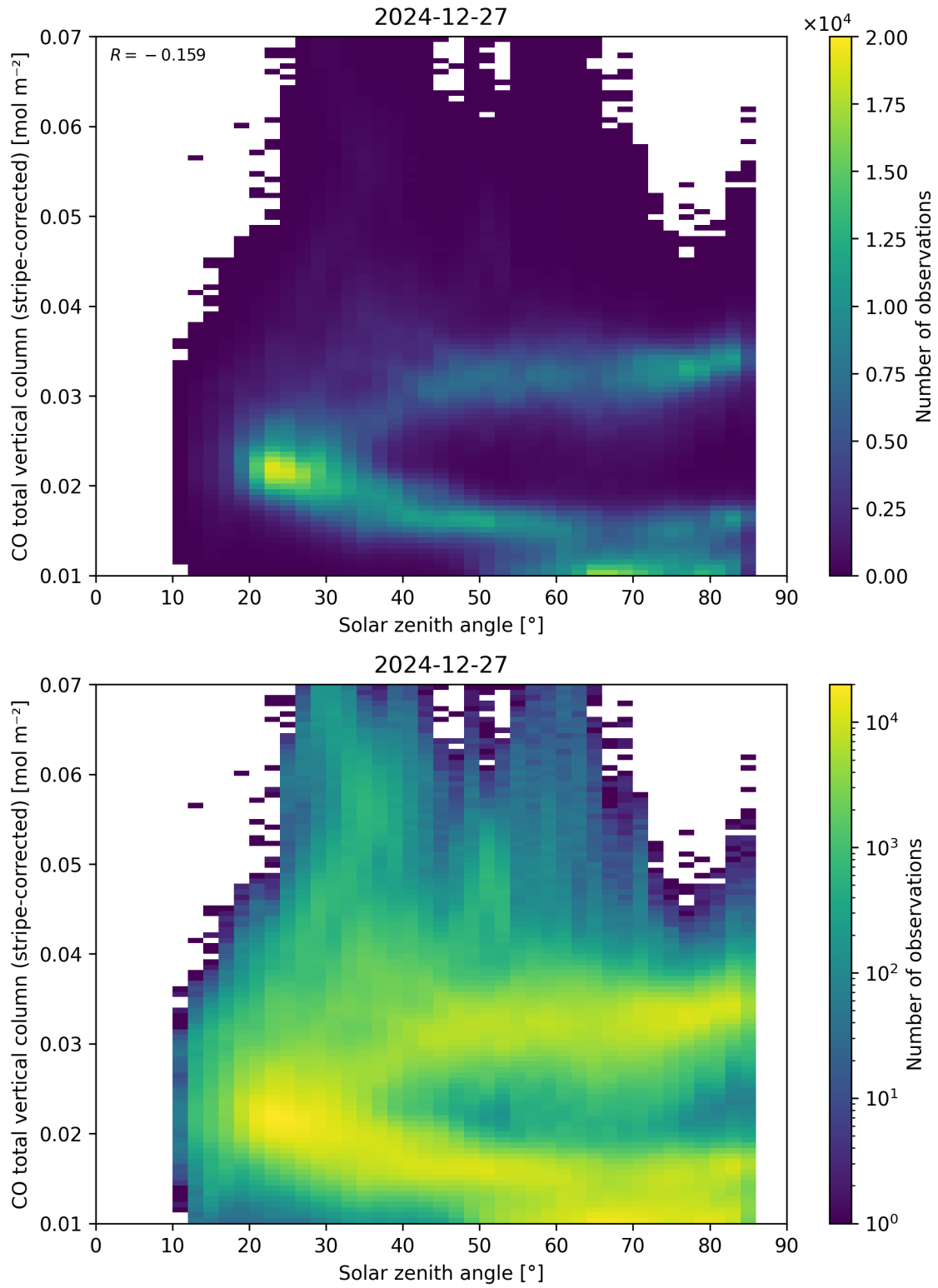
Figure 62: Scatter density plot of “Solar zenith angle” against “CO total vertical column (stripe-corrected)” for 2024-12-27 to 2024-12-28.
