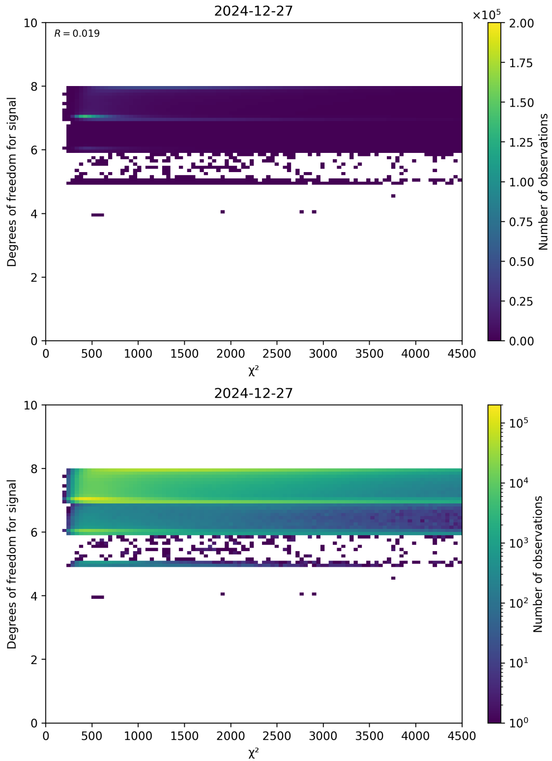
Figure 48: Scatter density plot of “ \chi^2 ” against “Degrees of freedom for signal” for 2024-12-27 to 2024-12-28.
