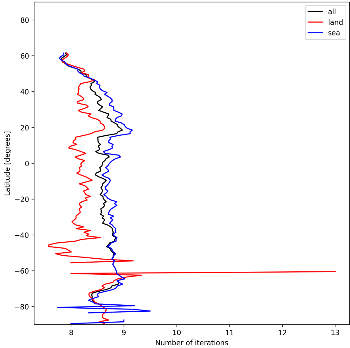
Figure 16: Zonal average of “Number of iterations” for 2024-12-27 to 2024-12-28.
