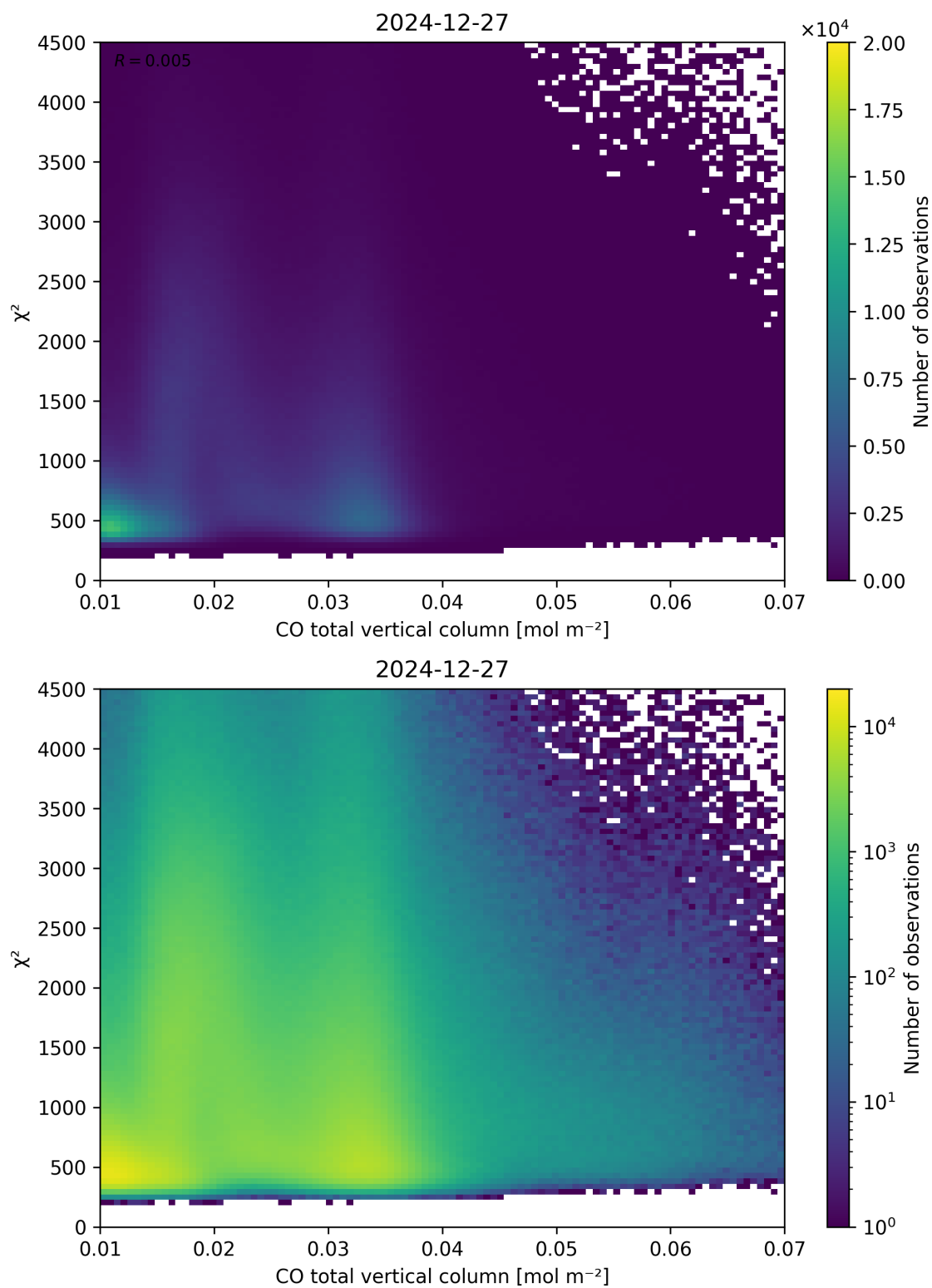
Figure 35: Scatter density plot of “CO total vertical column” against “ \chi^2 ” for 2024-12-27 to 2024-12-28.
