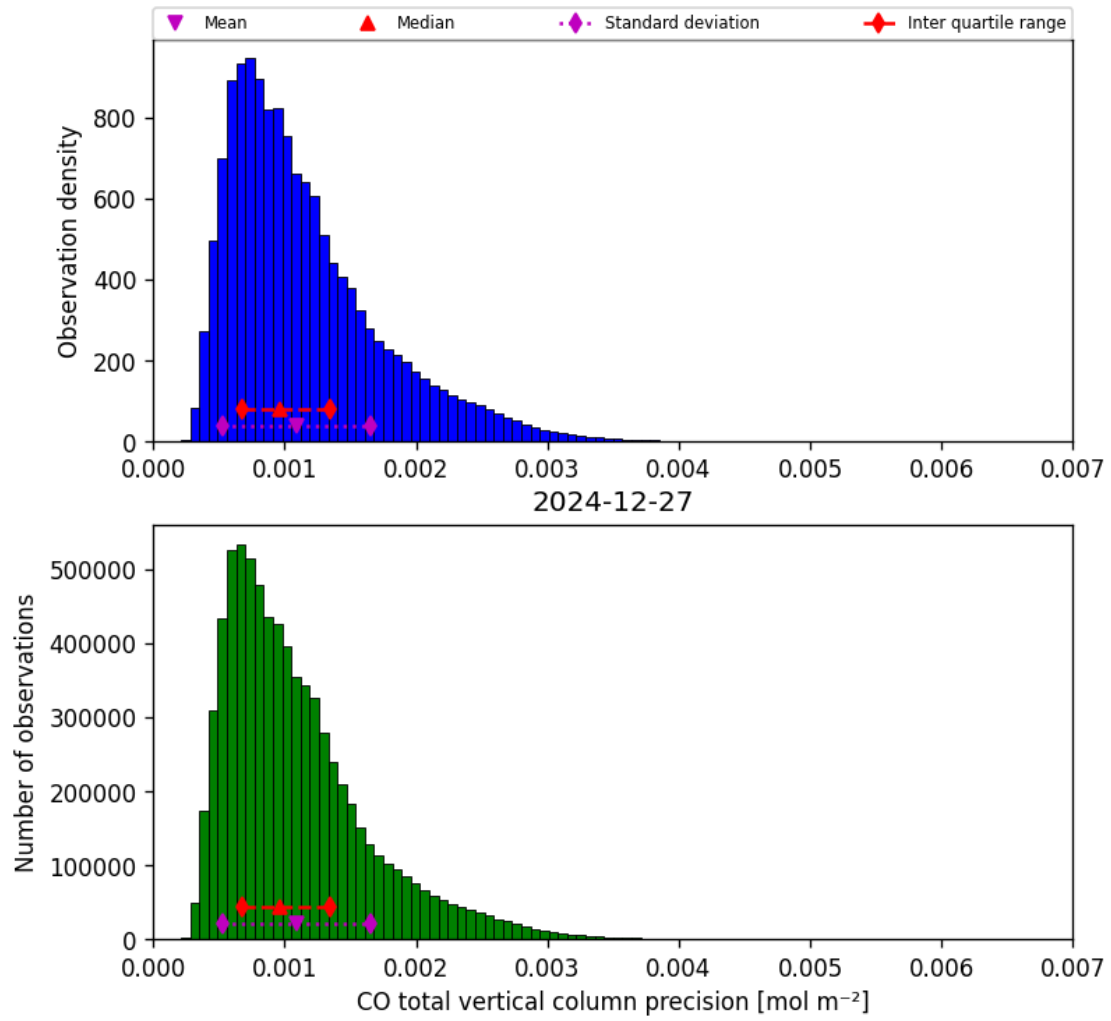
Figure 20: Histogram of “CO total vertical column precision” for 2024-12-27 to 2024-12-28
