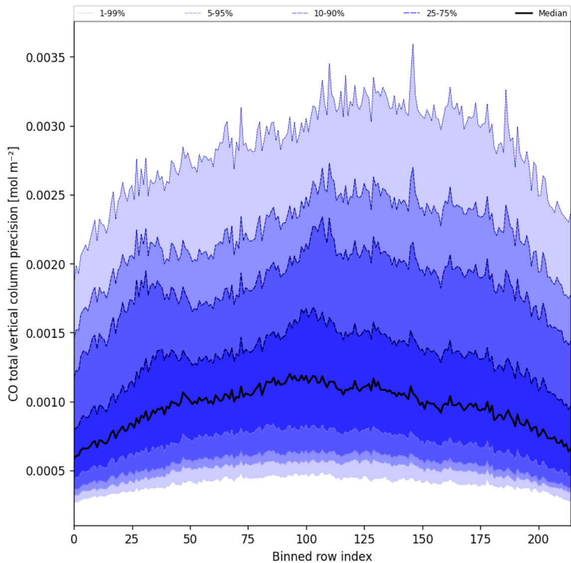
Figure 28: Along track statistics of “CO total vertical column precision” for 2024-12-27 to 2024-12-28
