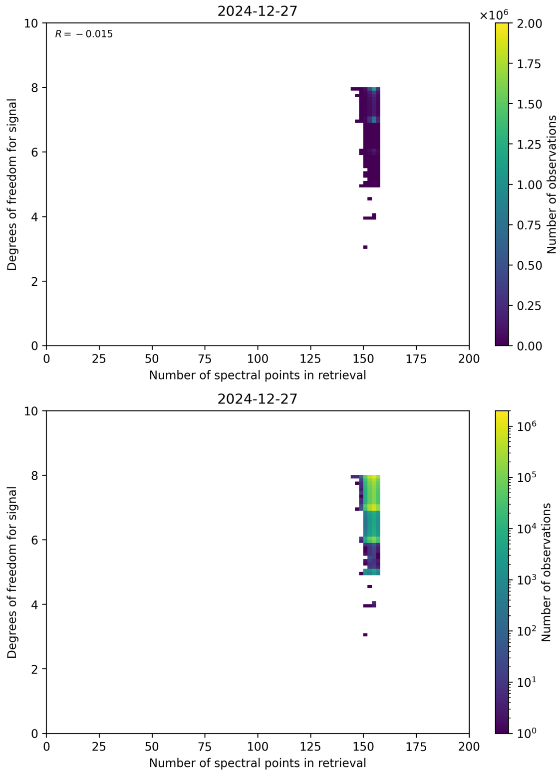
Figure 59: Scatter density plot of “Number of spectral points in retrieval” against “Degrees of freedom for signal” for 2024-12-27 to 2024-12-28.
