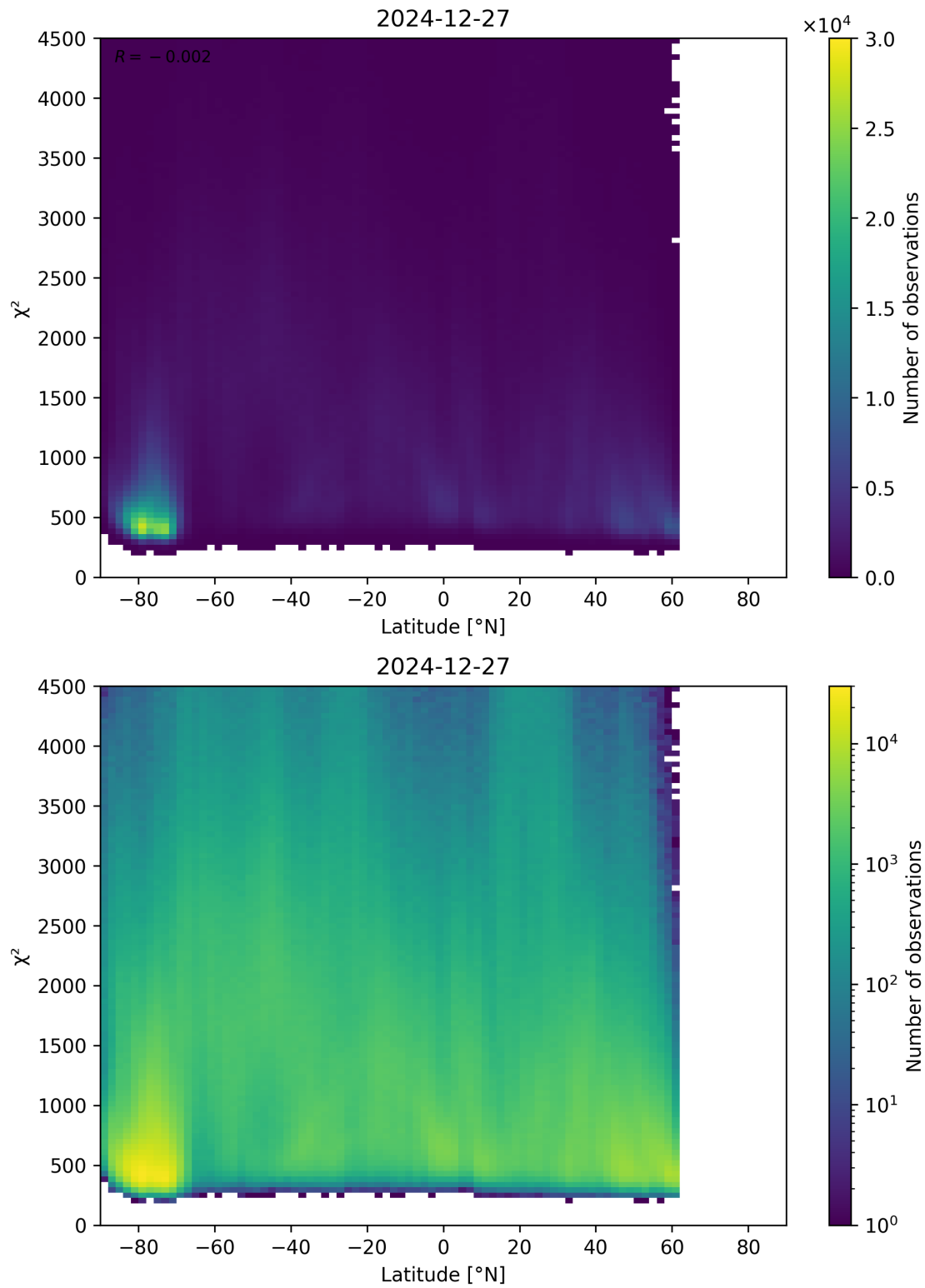
Figure 54: Scatter density plot of “Latitude” against “ \chi^2 ” for 2024-12-27 to 2024-12-28.
