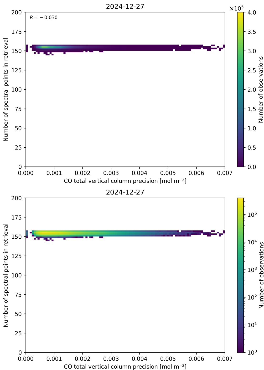
Figure 47: Scatter density plot of “CO total vertical column precision” against “Number of spectral points in retrieval” for 2024-12-27 to 2024-12-28.
