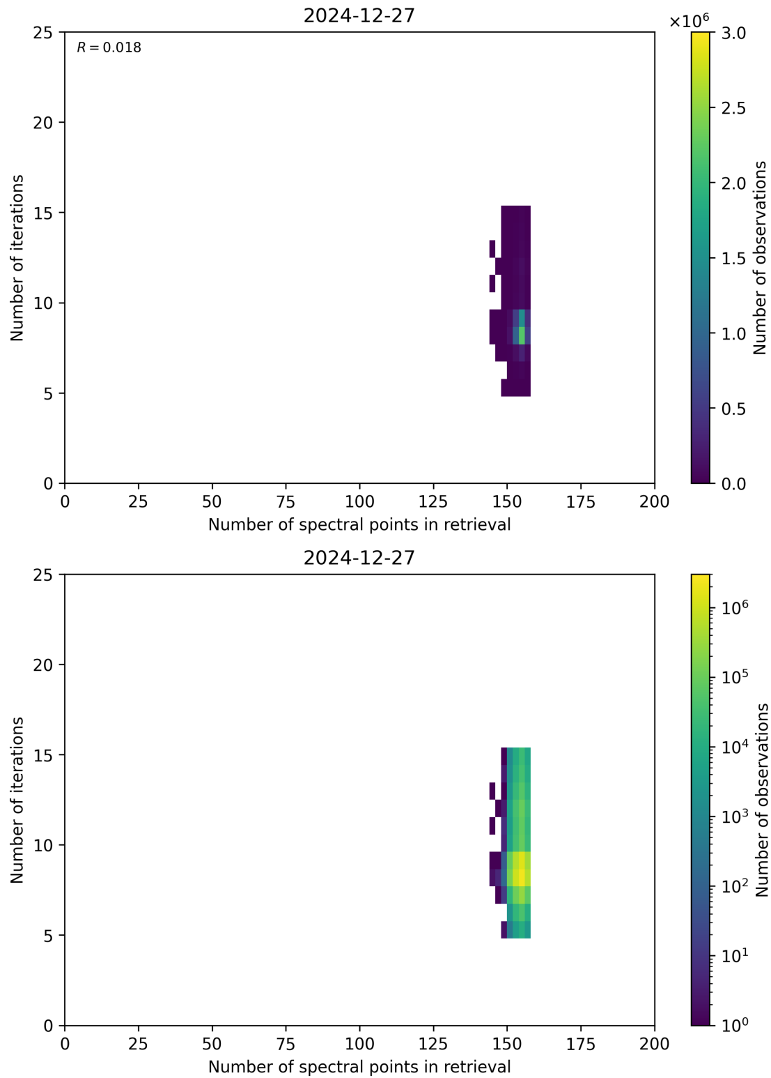
Figure 60: Scatter density plot of “Number of spectral points in retrieval” against “Number of iterations” for 2024-12-27 to 2024-12-28.
