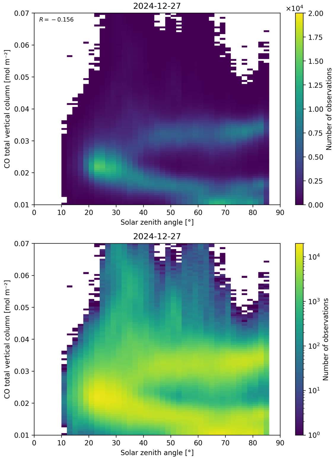
Figure 61: Scatter density plot of “Solar zenith angle” against “CO total vertical column” for 2024-12-27 to 2024-12-28.
