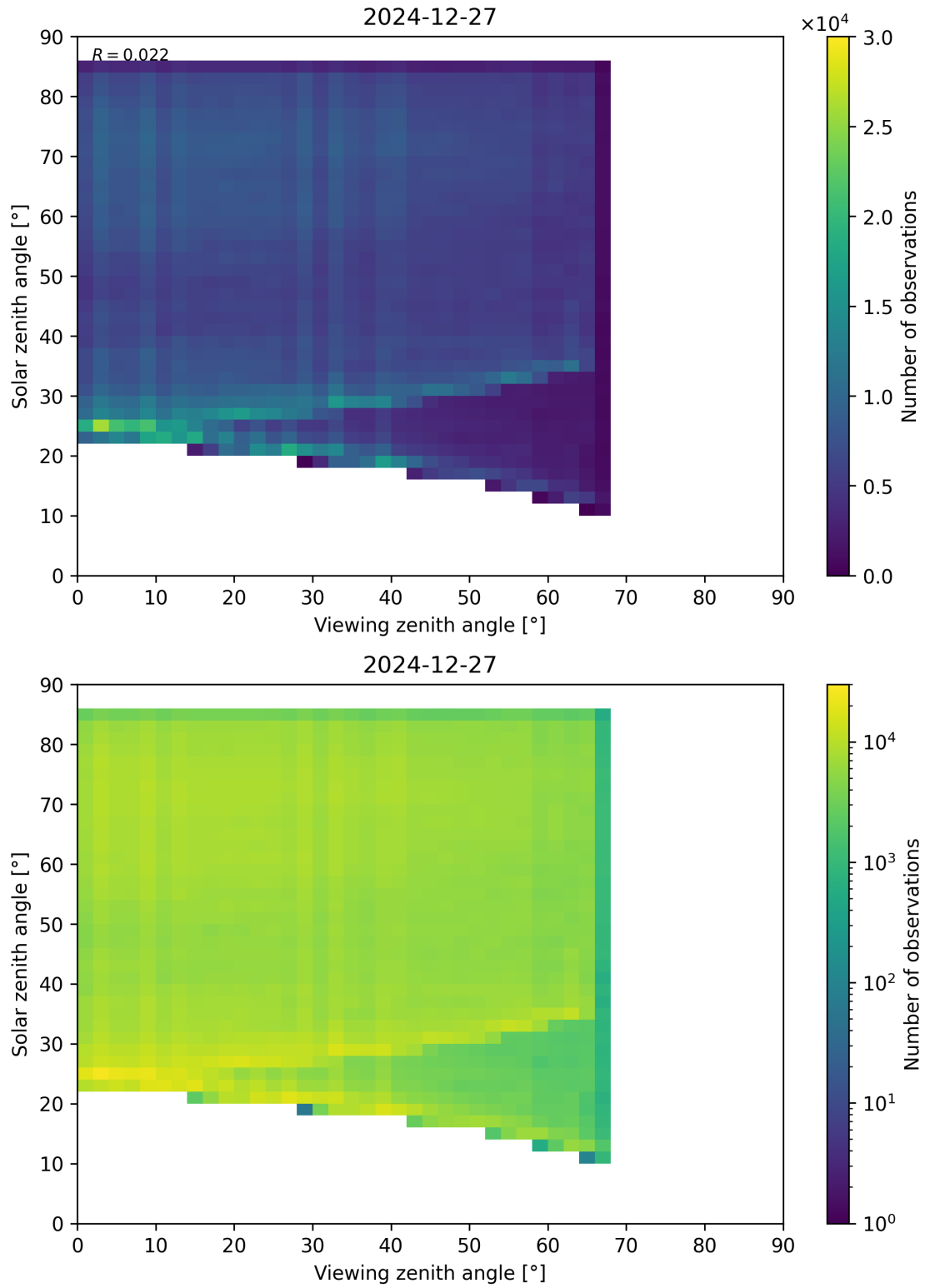
Figure 77: Scatter density plot of “Viewing zenith angle” against “Solar zenith angle” for 2024-12-27 to 2024-12-28.
