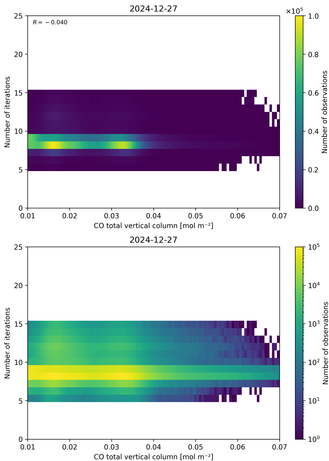
Figure 42: Scatter density plot of “CO total vertical column” against “Number of iterations” for 2024-12-27 to 2024-12-28.
