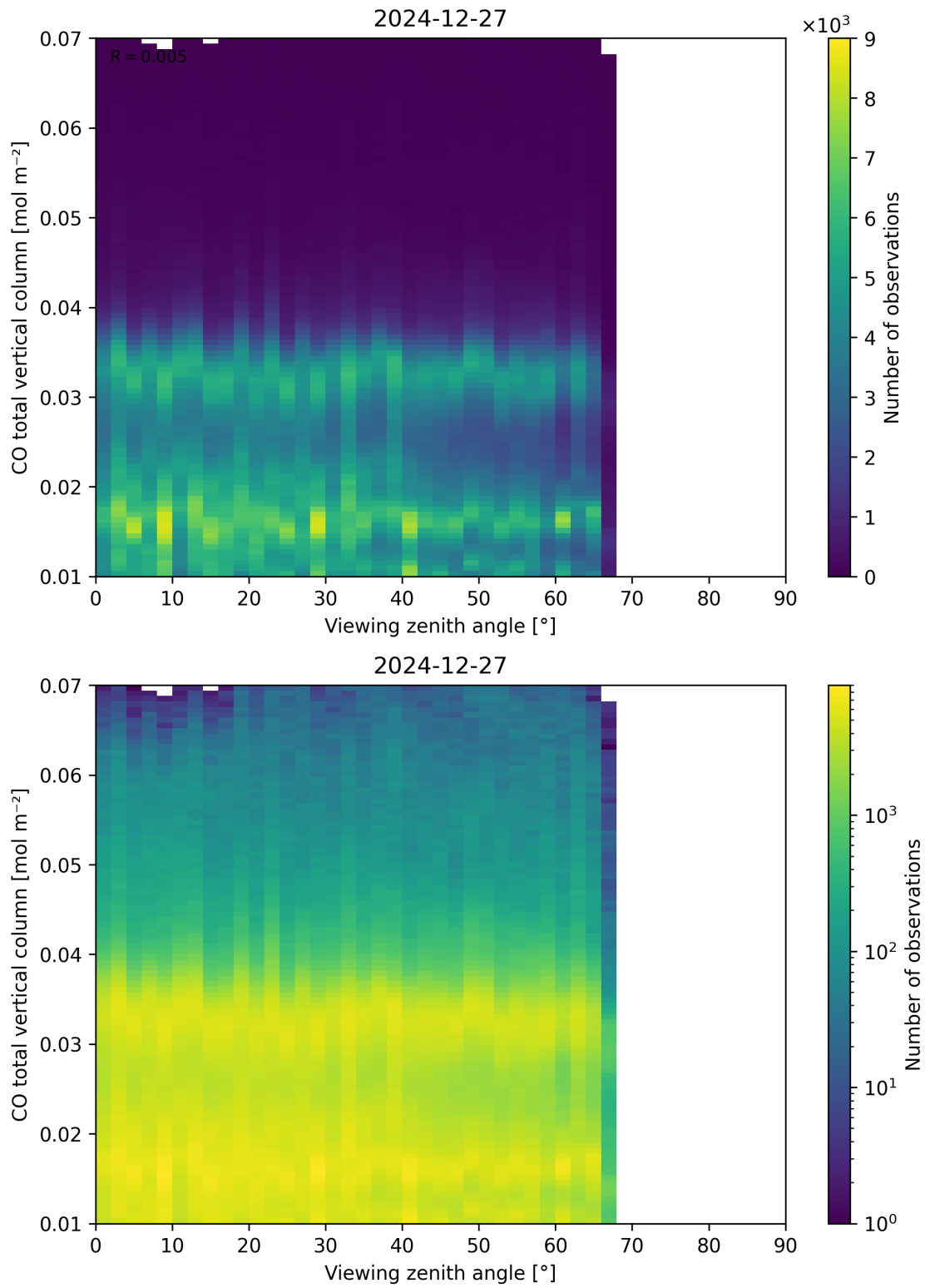
Figure 69: Scatter density plot of “Viewing zenith angle” against “CO total vertical column” for 2024-12-27 to 2024-12-28.
