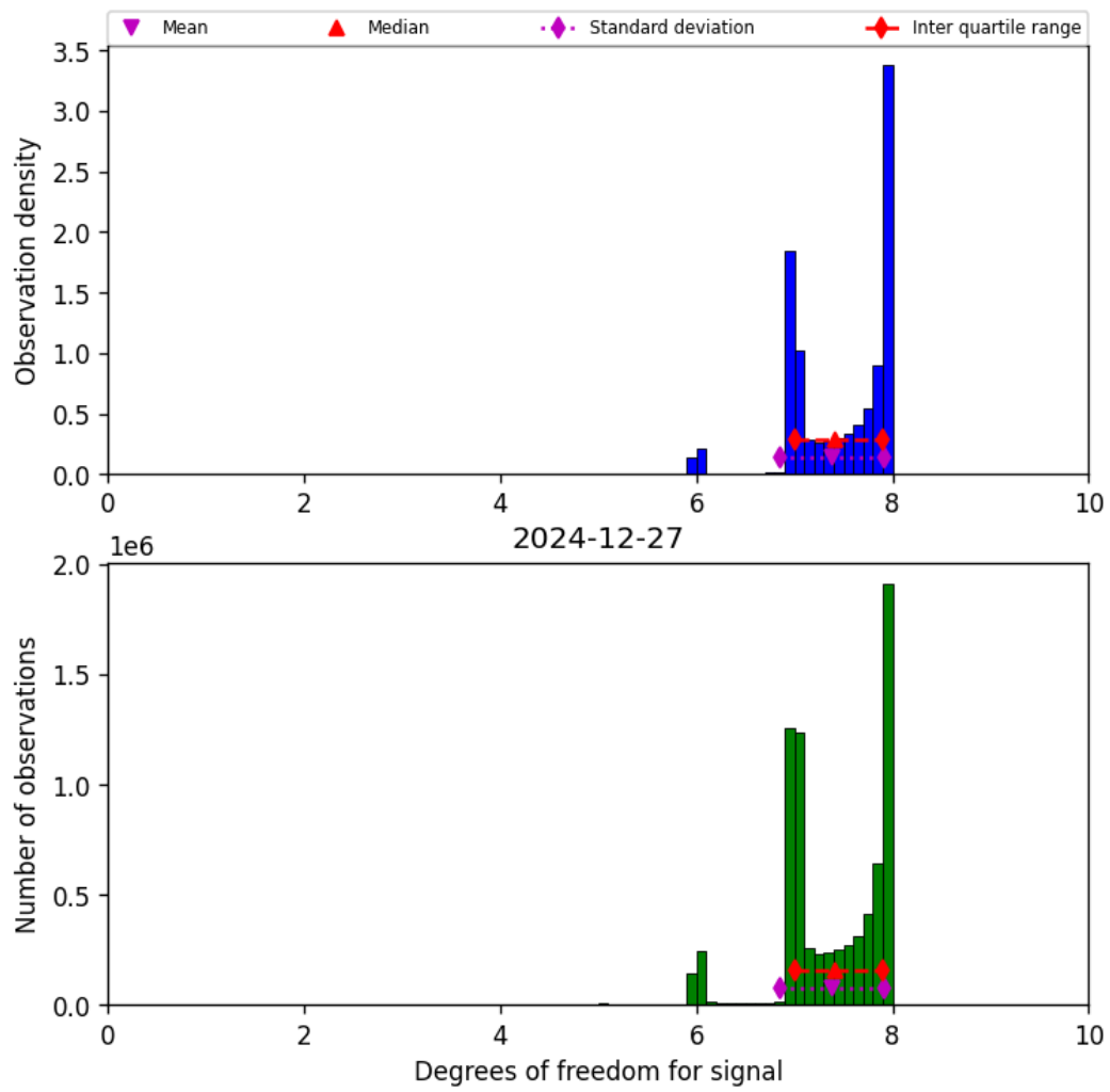
Figure 23: Histogram of “Degrees of freedom for signal” for 2024-12-27 to 2024-12-28
