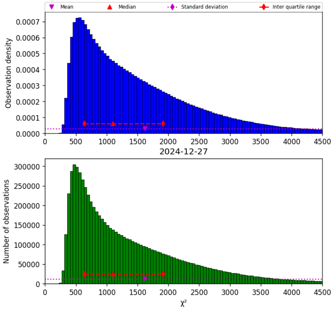
Figure 22: Histogram of “ \chi^2 ” for 2024-12-27 to 2024-12-28
