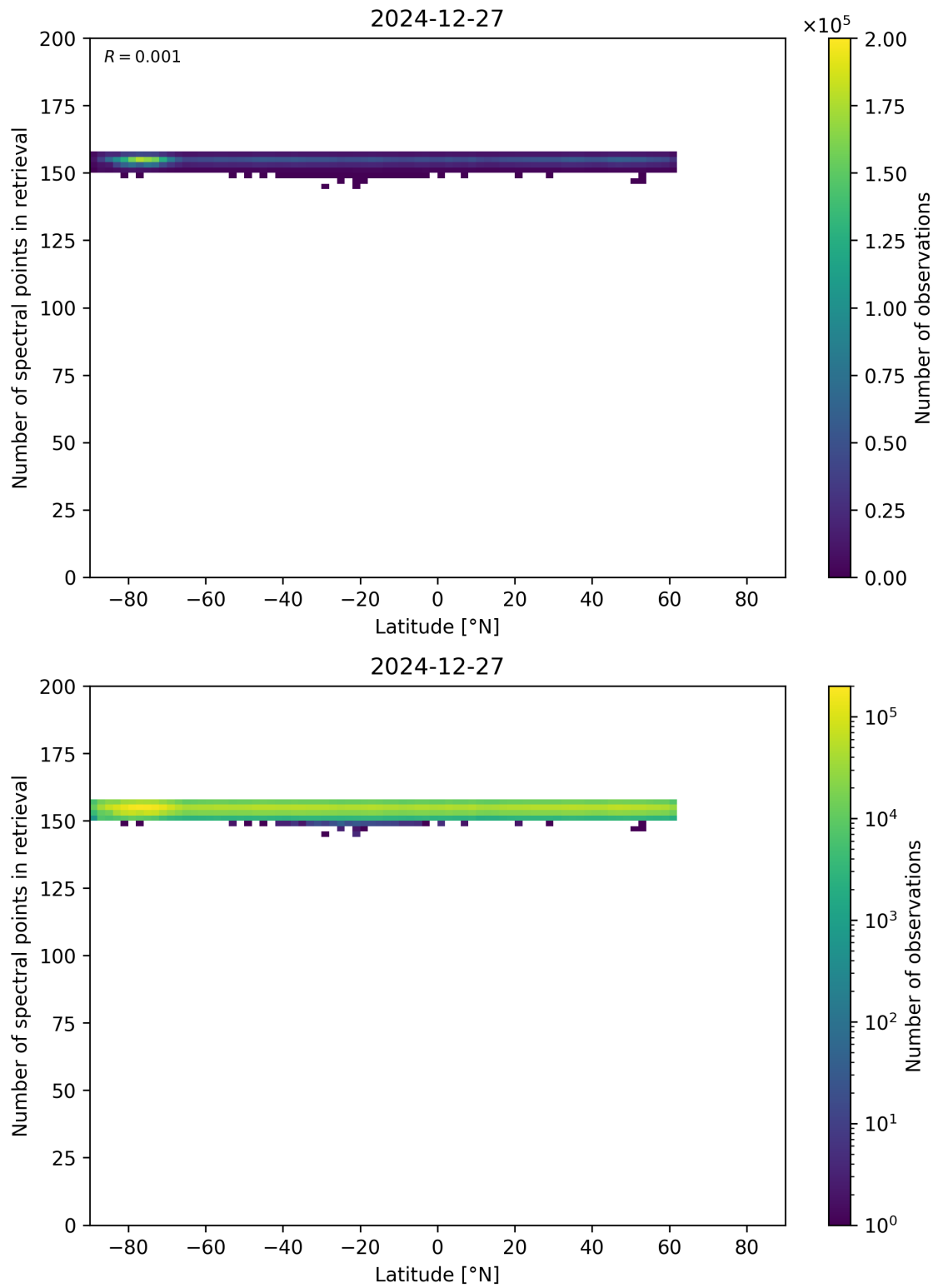
Figure 57: Scatter density plot of “Latitude” against “Number of spectral points in retrieval” for 2024-12-27 to 2024-12-28.
