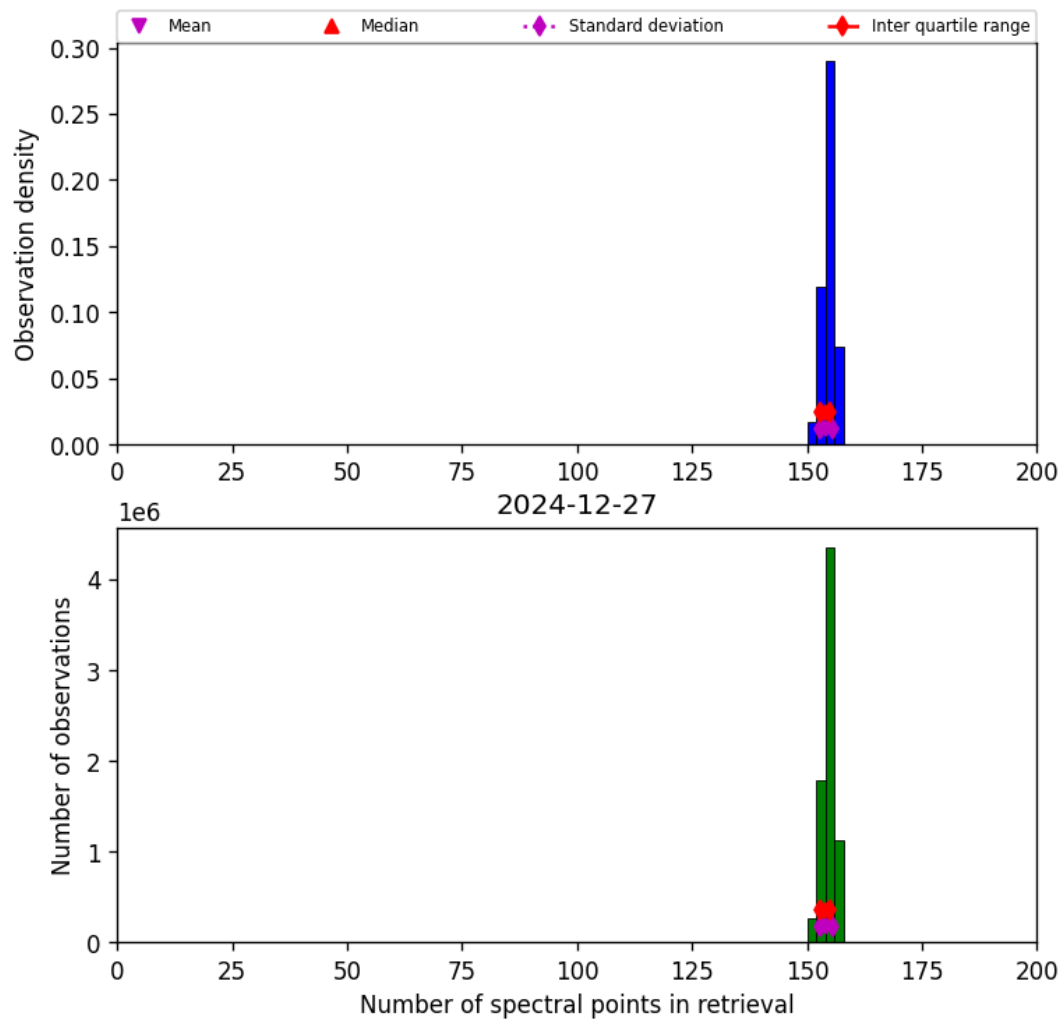
Figure 21: Histogram of “Number of spectral points in retrieval” for 2024-12-27 to 2024-12-28
