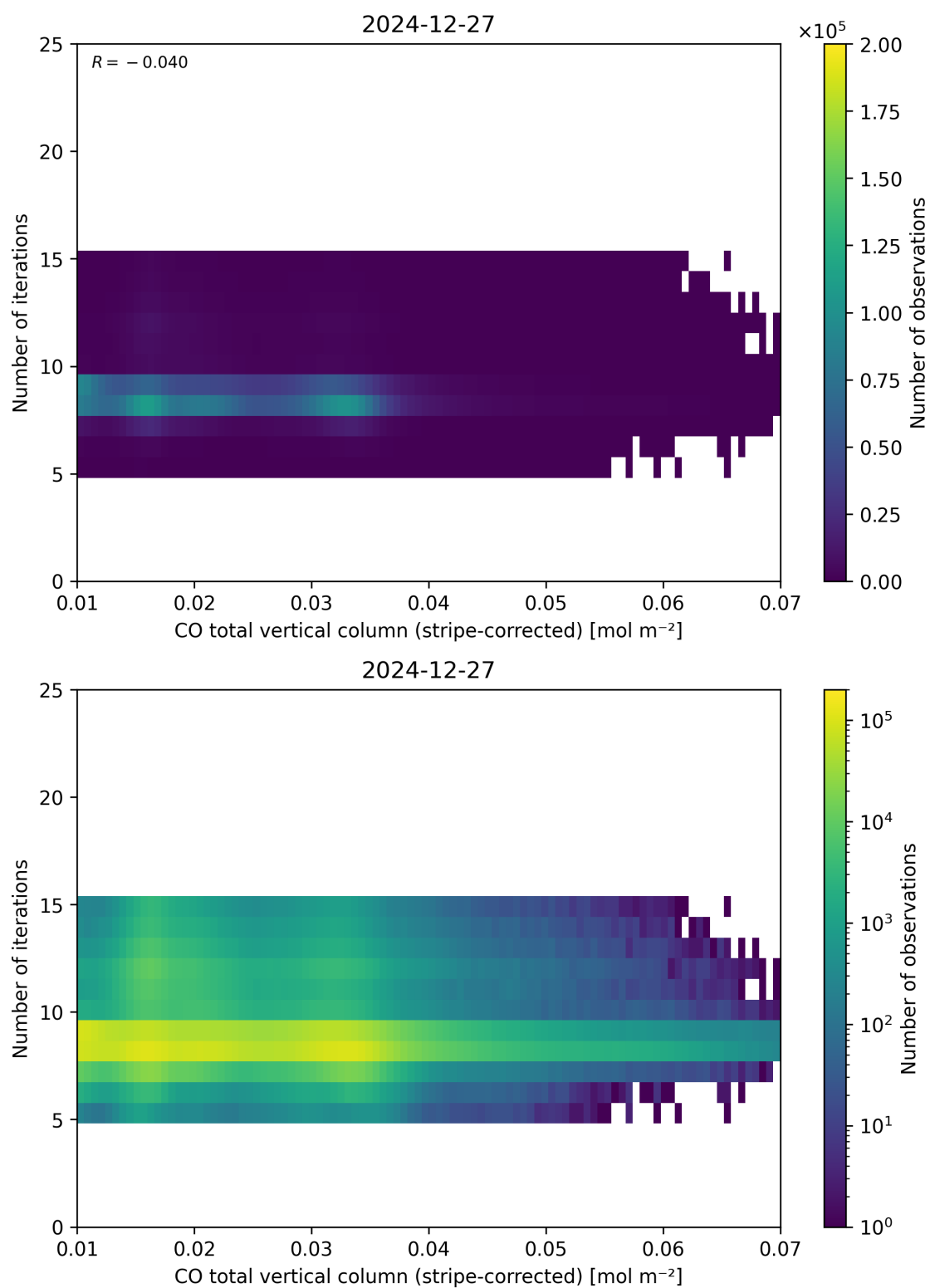
Figure 39: Scatter density plot of “CO total vertical column (stripe-corrected)” against “Number of iterations” for 2024-12-27 to 2024-12-28.
