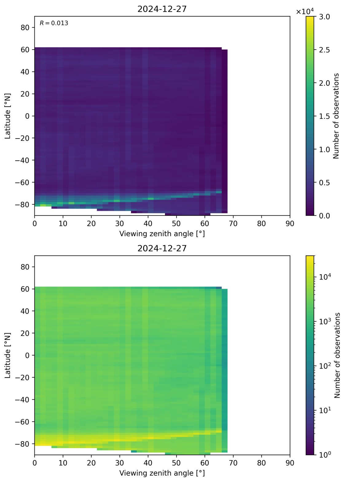
Figure 74: Scatter density plot of “Viewing zenith angle” against “Latitude” for 2024-12-27 to 2024-12-28.
