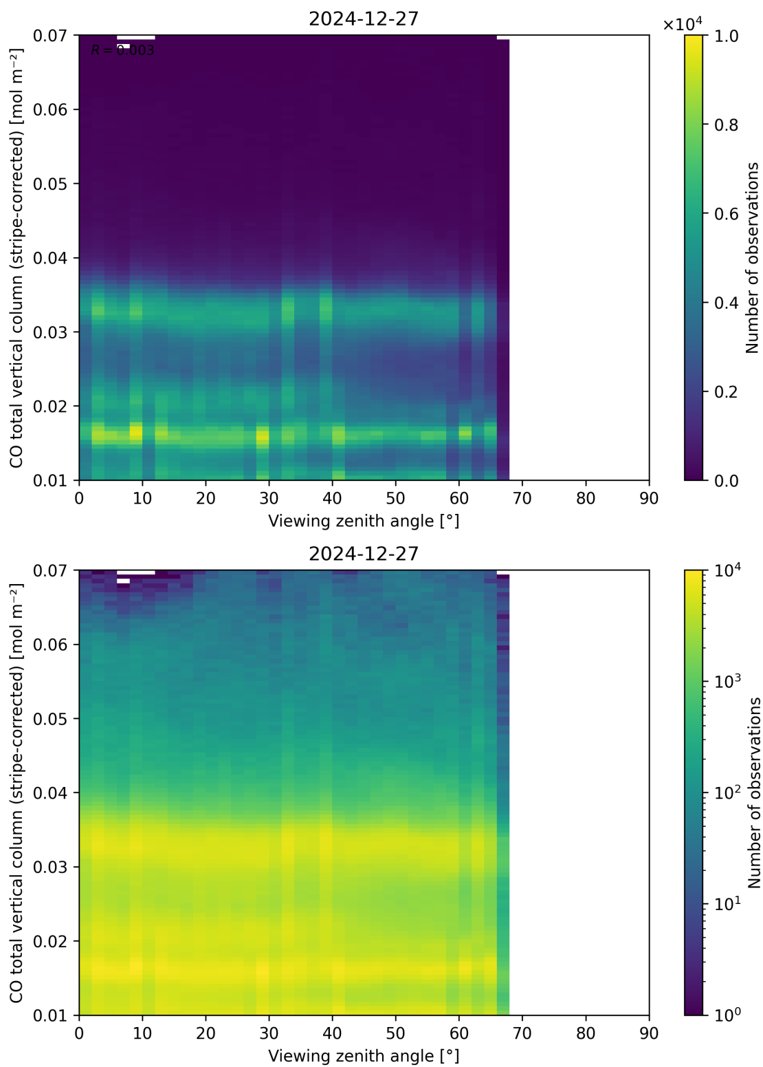
Figure 70: Scatter density plot of “Viewing zenith angle” against “CO total vertical column (stripe-corrected)” for 2024-12-27 to 2024-12-28.
