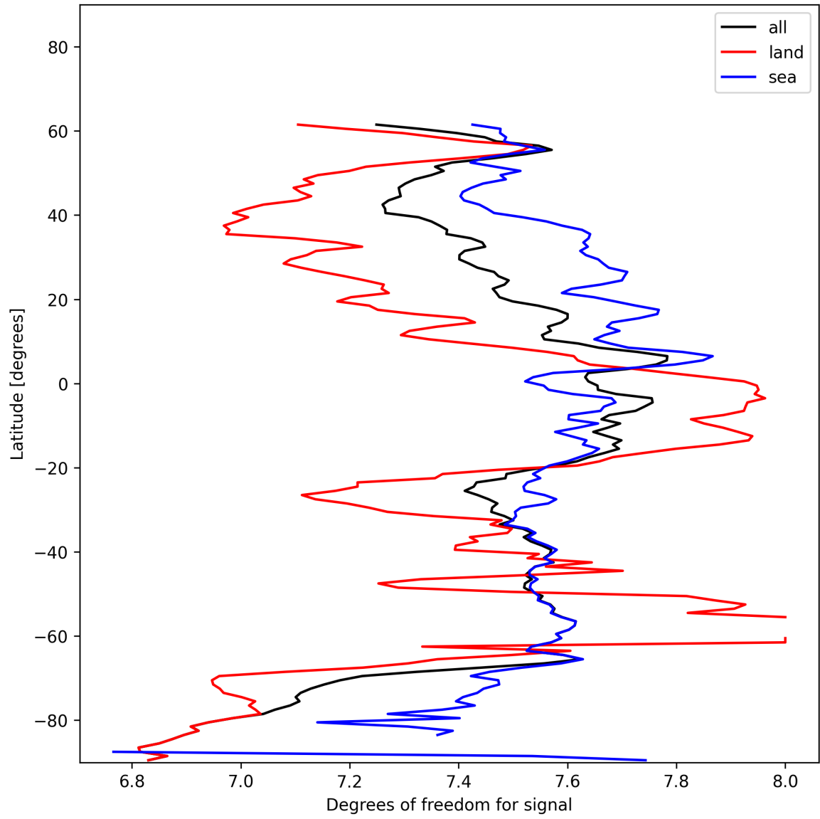
Figure 15: Zonal average of “Degrees of freedom for signal” for 2024-12-27 to 2024-12-28.
