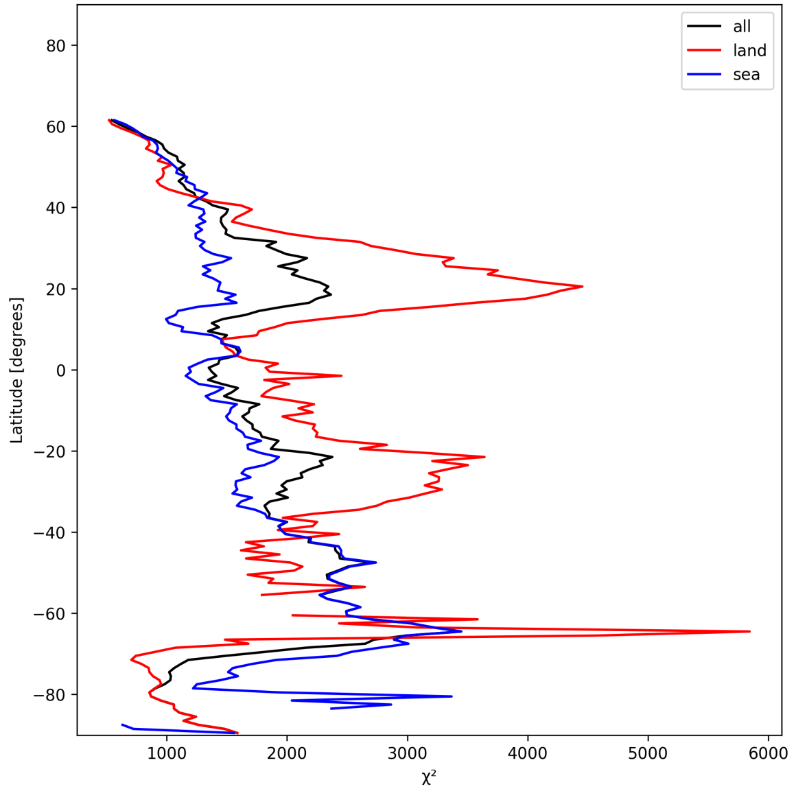
Figure 14: Zonal average of “ \chi^2 ” for 2024-12-27 to 2024-12-28.
