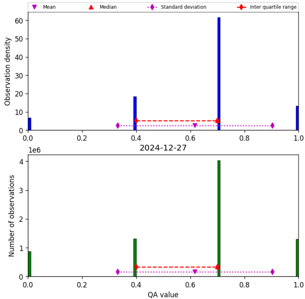
Figure 17: Histogram of “QA value” for 2024-12-27 to 2024-12-28
