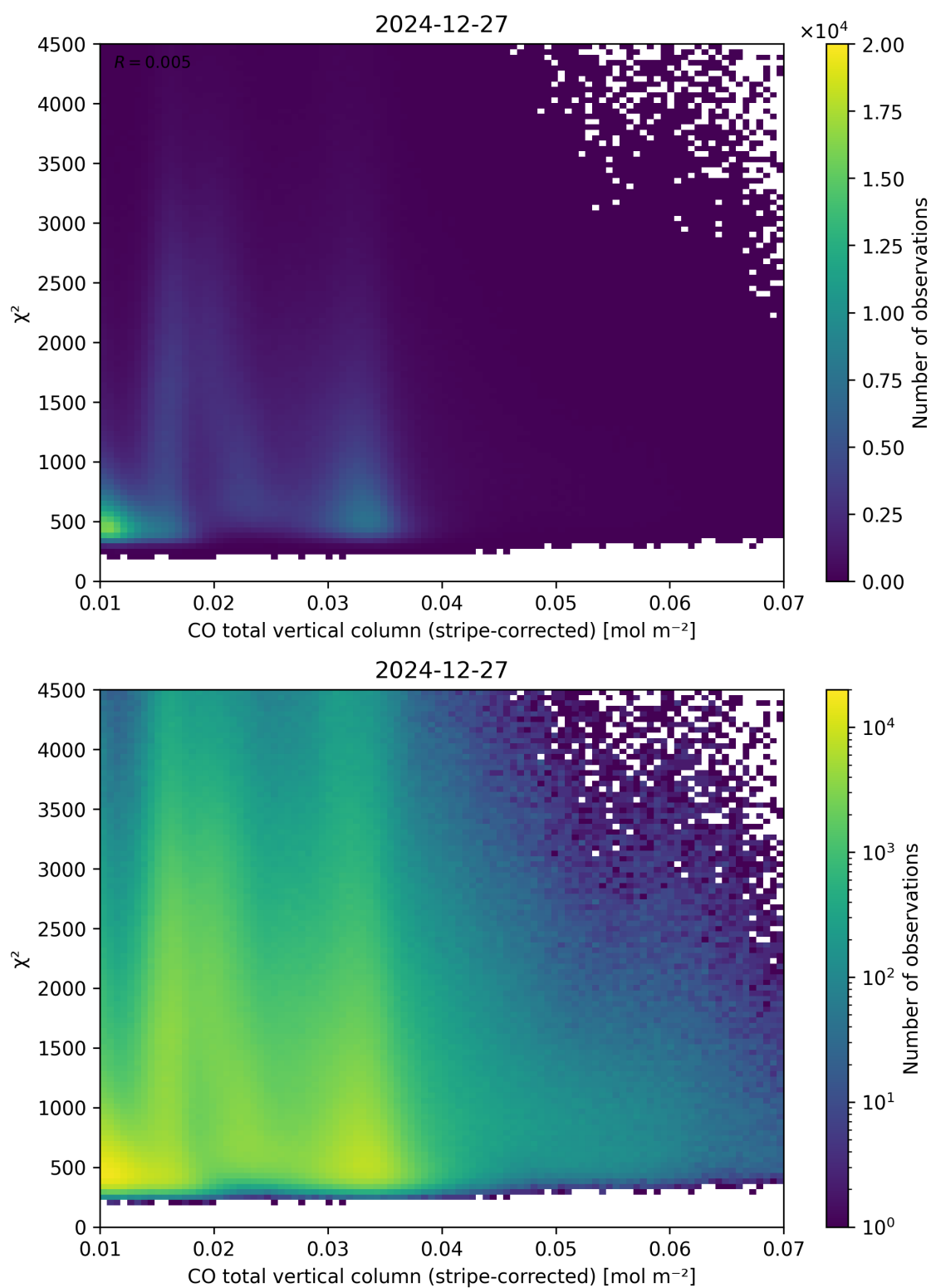
Figure 37: Scatter density plot of “CO total vertical column (stripe-corrected)” against “ \chi^2 ” for 2024-12-27 to 2024-12-28.
