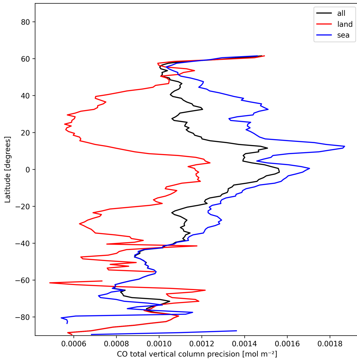
Figure 12: Zonal average of “CO total vertical column precision” for 2024-12-27 to 2024-12-28.
