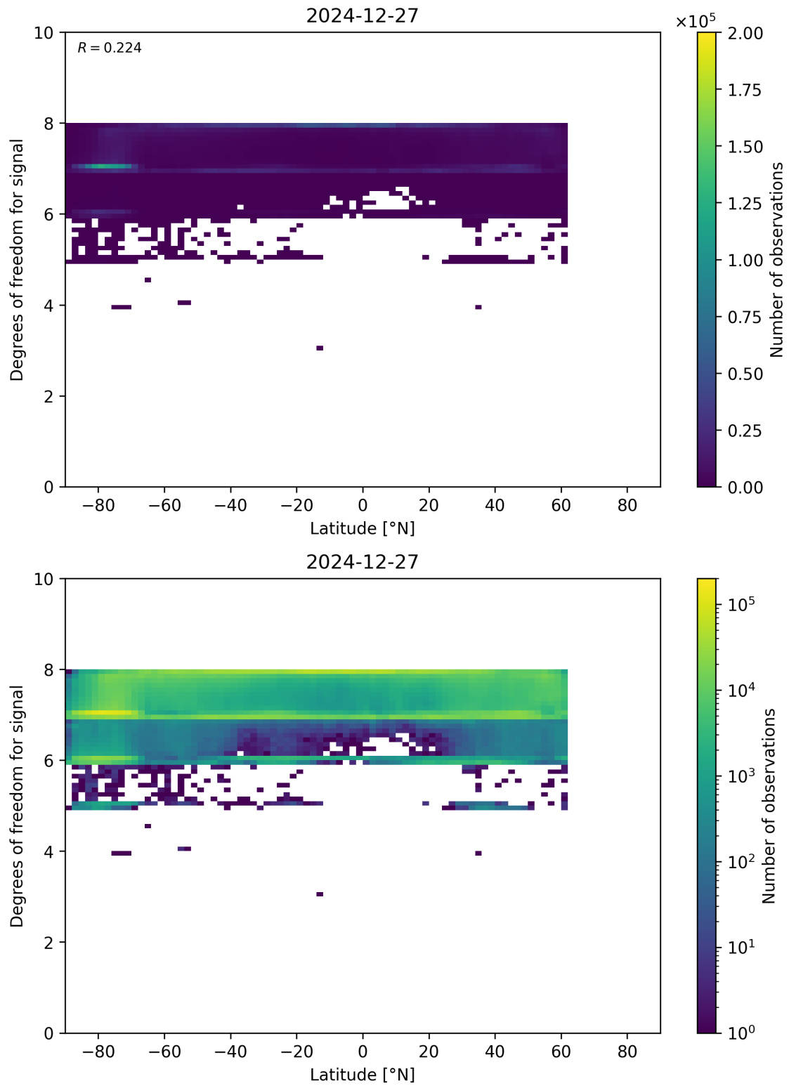
Figure 55: Scatter density plot of “Latitude” against “Degrees of freedom for signal” for 2024-12-27 to 2024-12-28.
