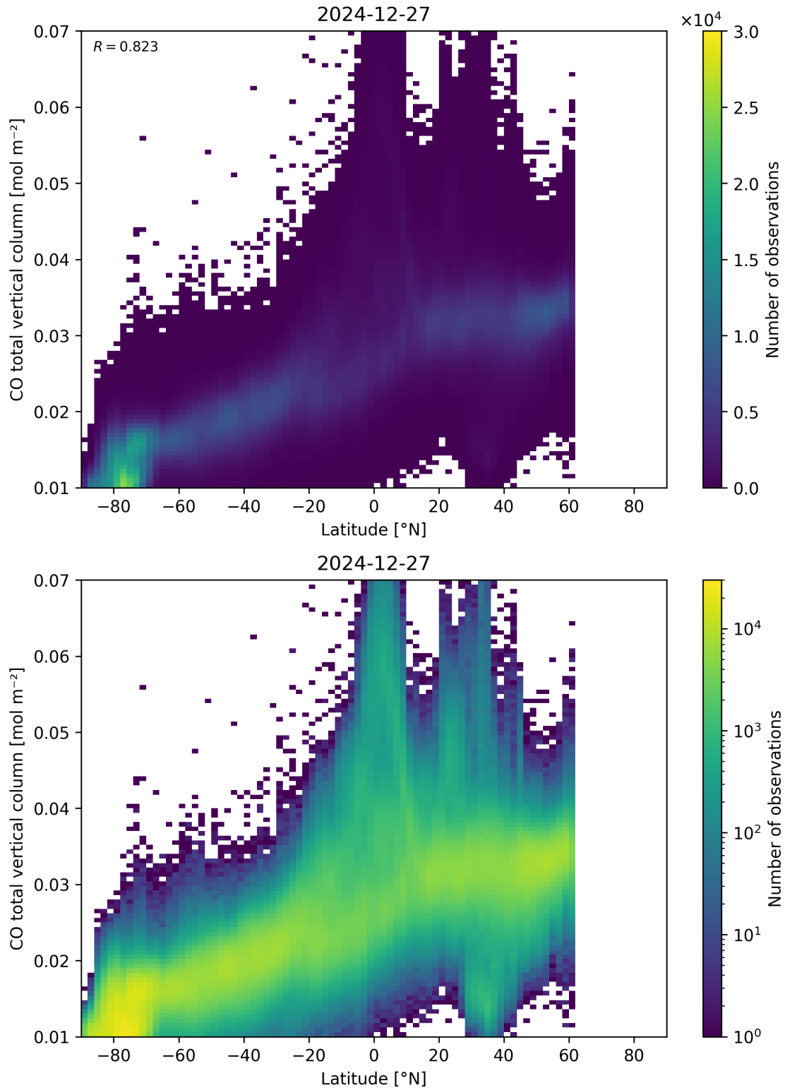
Figure 51: Scatter density plot of “Latitude” against “CO total vertical column” for 2024-12-27 to 2024-12-28.
