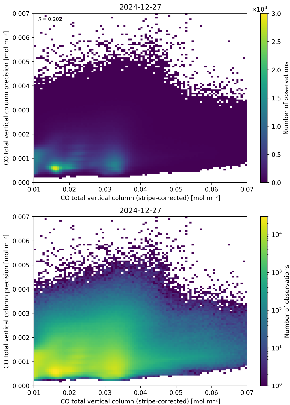
Figure 36: Scatter density plot of “CO total vertical column (stripe-corrected)” against “CO total vertical column precision” for 2024-12-27 to 2024-12-28.
