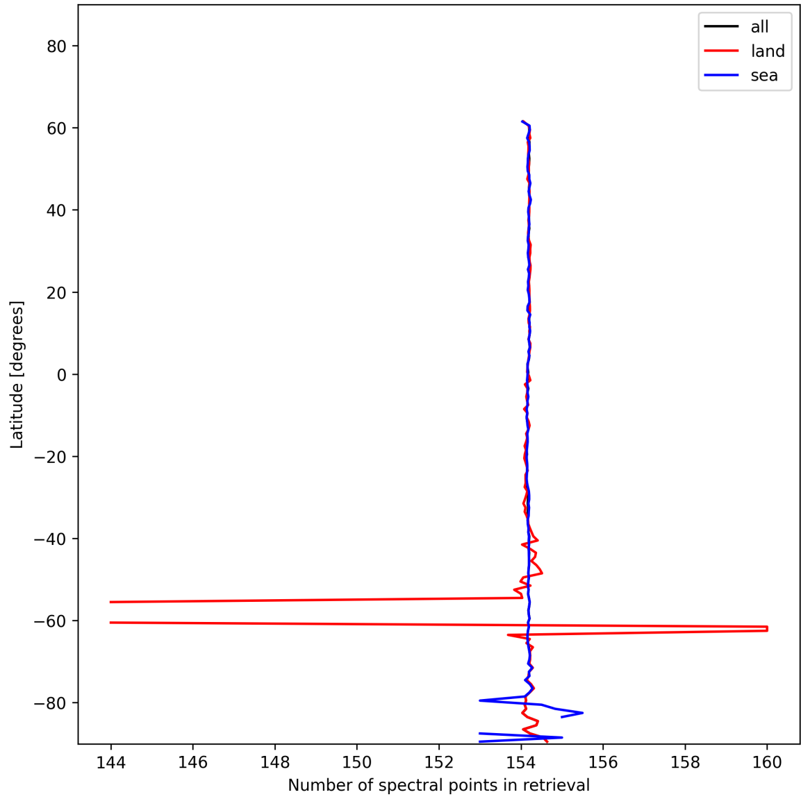
Figure 13: Zonal average of “Number of spectral points in retrieval” for 2024-12-27 to 2024-12-28.
