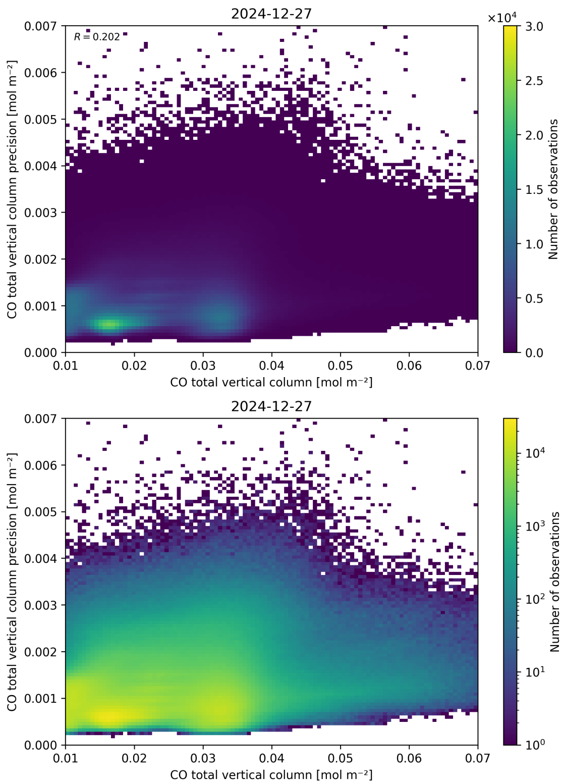
Figure 34: Scatter density plot of “CO total vertical column” against “CO total vertical column precision” for 2024-12-27 to 2024-12-28.
