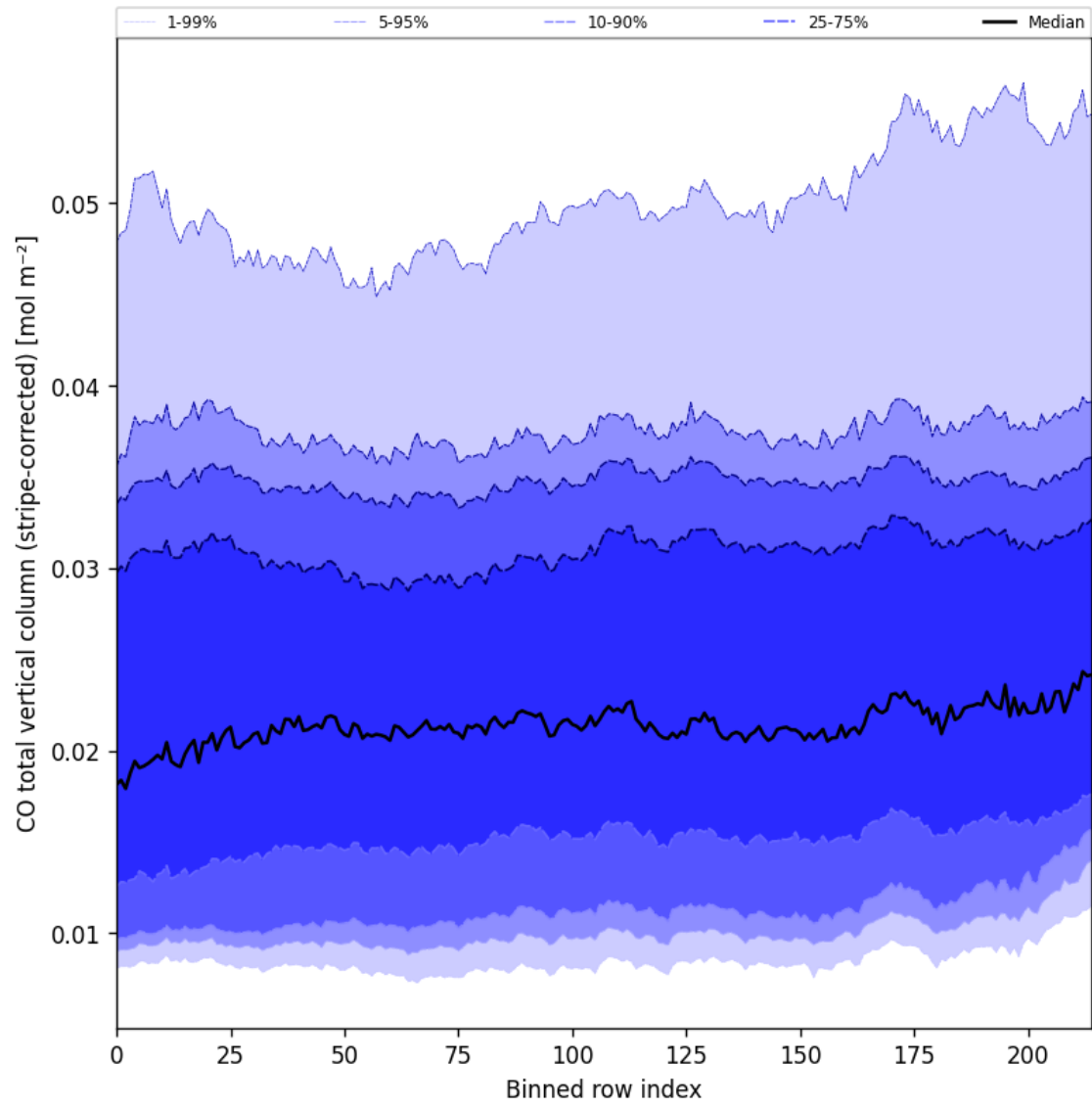
Figure 27: Along track statistics of “CO total vertical column (stripe-corrected)” for 2024-12-27 to 2024-12-28
