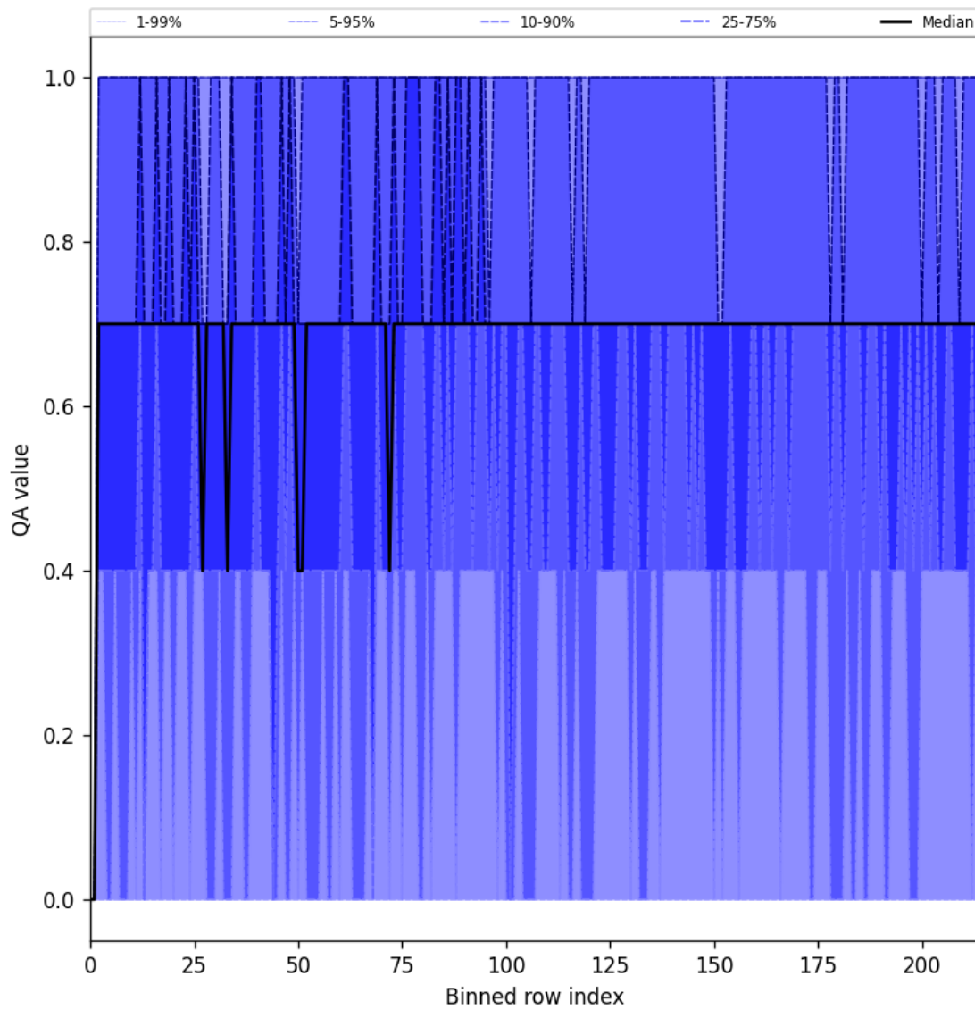
Figure 25: Along track statistics of “QA value” for 2024-12-27 to 2024-12-28
