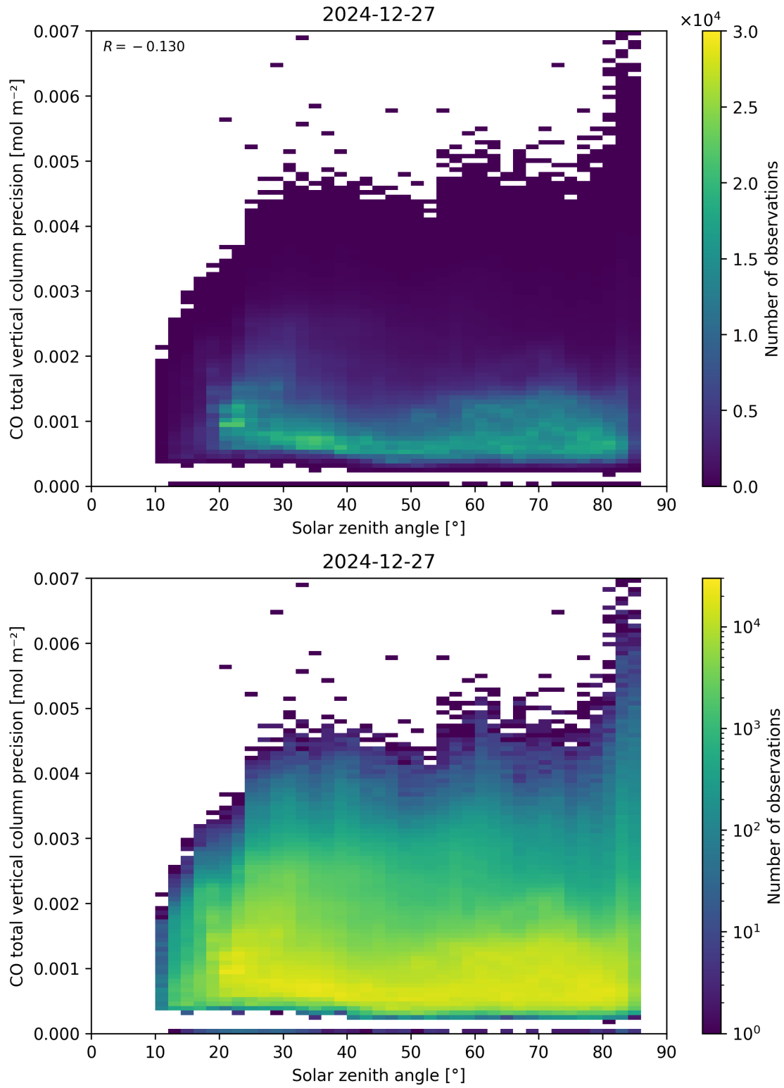
Figure 63: Scatter density plot of “Solar zenith angle” against “CO total vertical column precision” for 2024-12-27 to 2024-12-28.
