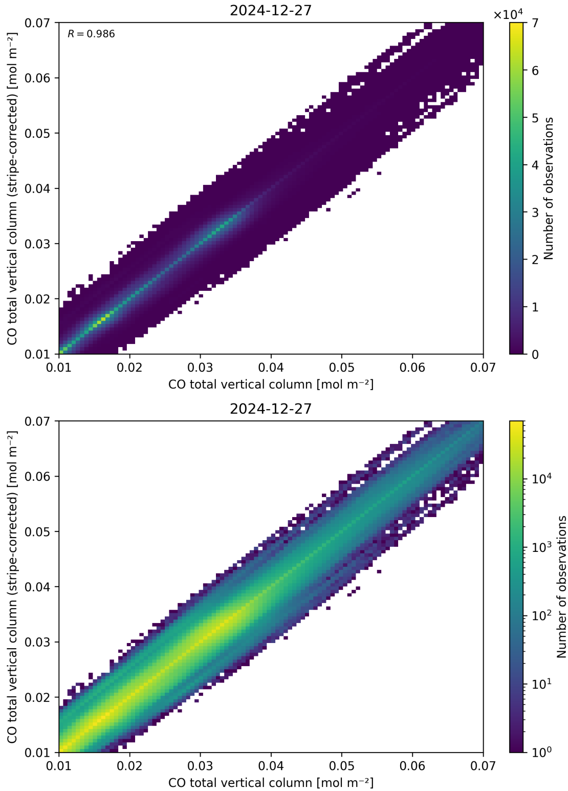
Figure 33: Scatter density plot of “CO total vertical column” against “CO total vertical column (stripe-corrected)” for 2024-12-27 to 2024-12-28.
