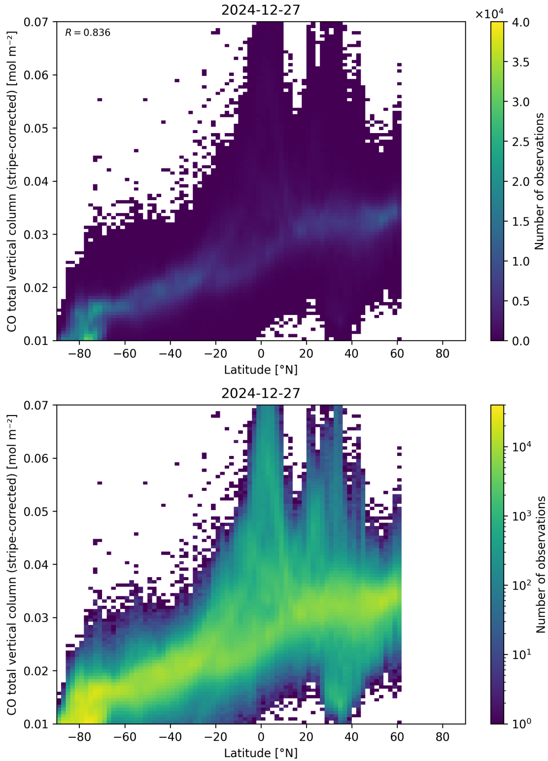
Figure 52: Scatter density plot of “Latitude” against “CO total vertical column (stripe-corrected)” for 2024-12-27 to 2024-12-28.
