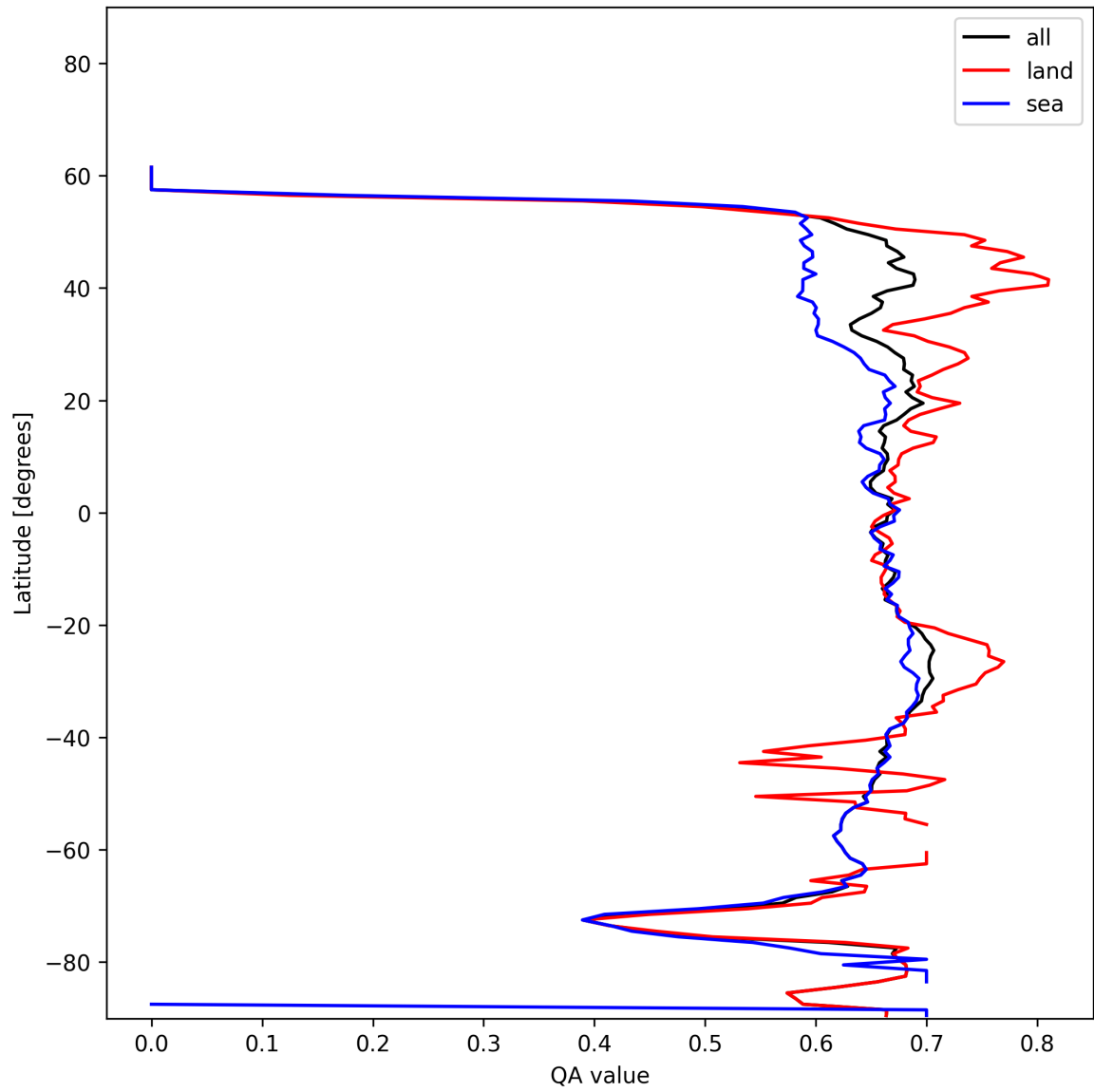
Figure 9: Zonal average of “QA value” for 2024-12-27 to 2024-12-28.
