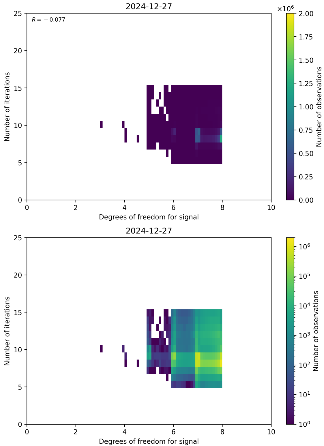
Figure 50: Scatter density plot of “Degrees of freedom for signal” against “Number of iterations” for 2024-12-27 to 2024-12-28.
