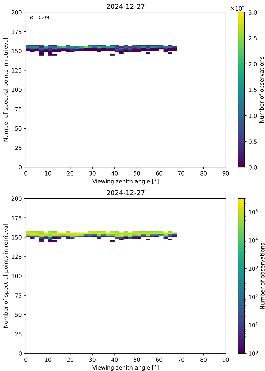
Figure 76: Scatter density plot of “Viewing zenith angle” against “Number of spectral points in retrieval” for 2024-12-27 to 2024-12-28.
