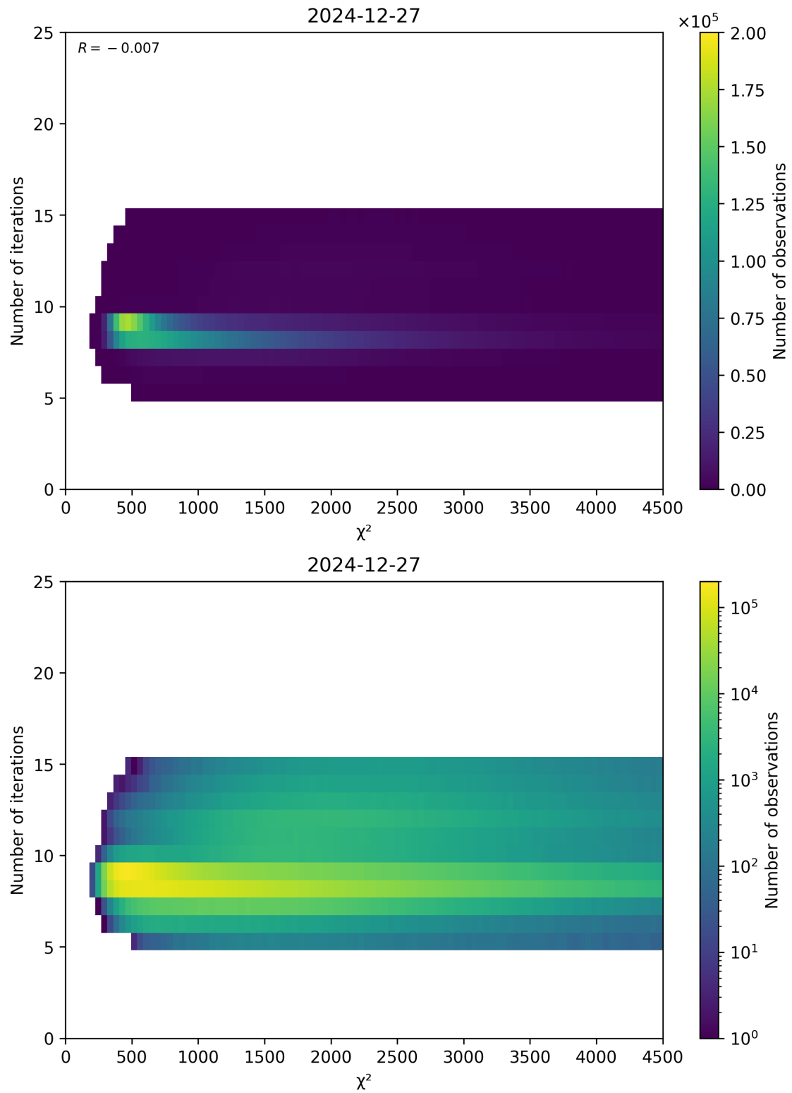
Figure 49: Scatter density plot of “ \chi^2 ” against “Number of iterations” for 2024-12-27 to 2024-12-28.
