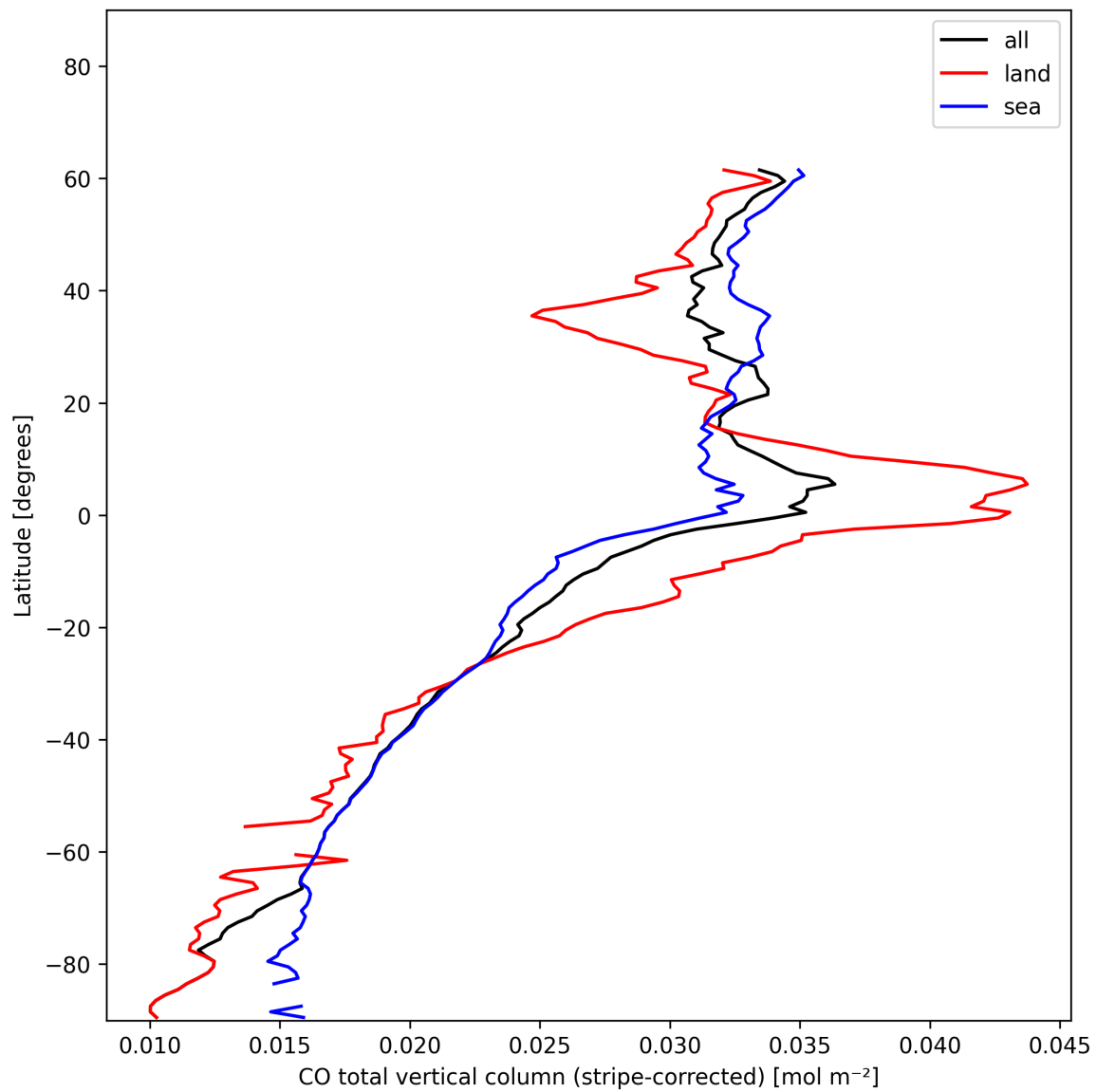
Figure 11: Zonal average of “CO total vertical column (stripe-corrected)” for 2024-12-27 to 2024-12-28.
