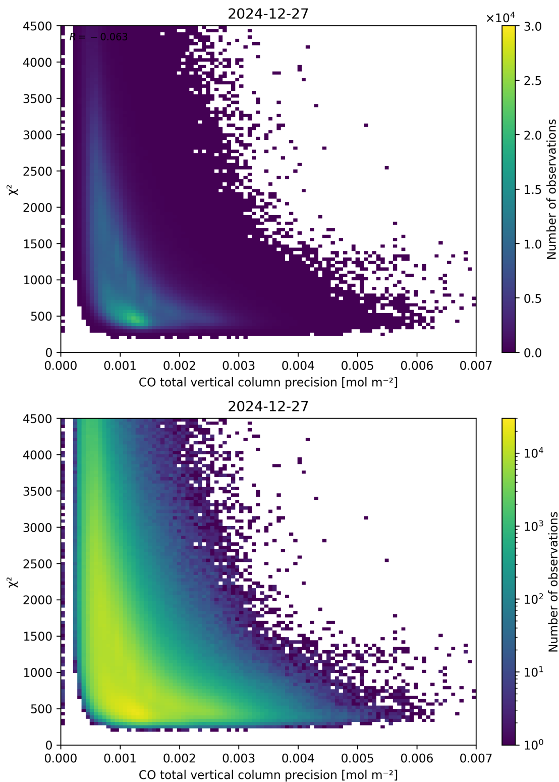
Figure 44: Scatter density plot of “CO total vertical column precision” against “ \chi^2 ” for 2024-12-27 to 2024-12-28.
