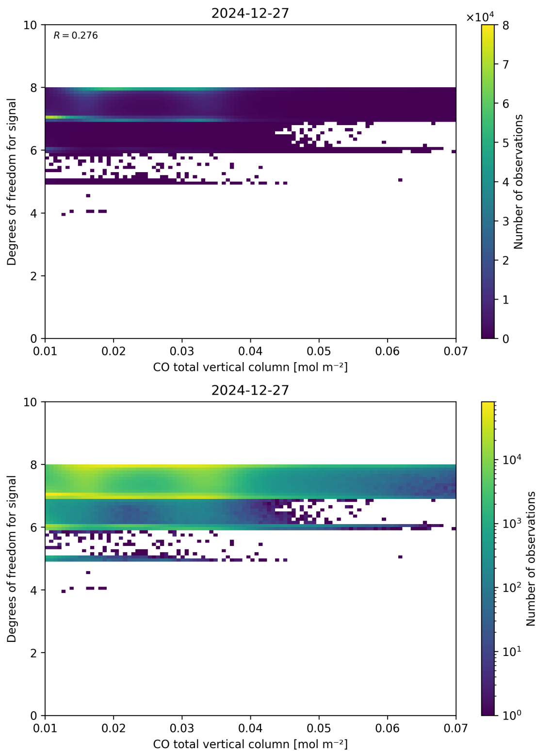
Figure 41: Scatter density plot of “CO total vertical column” against “Degrees of freedom for signal” for 2024-12-27 to 2024-12-28.
