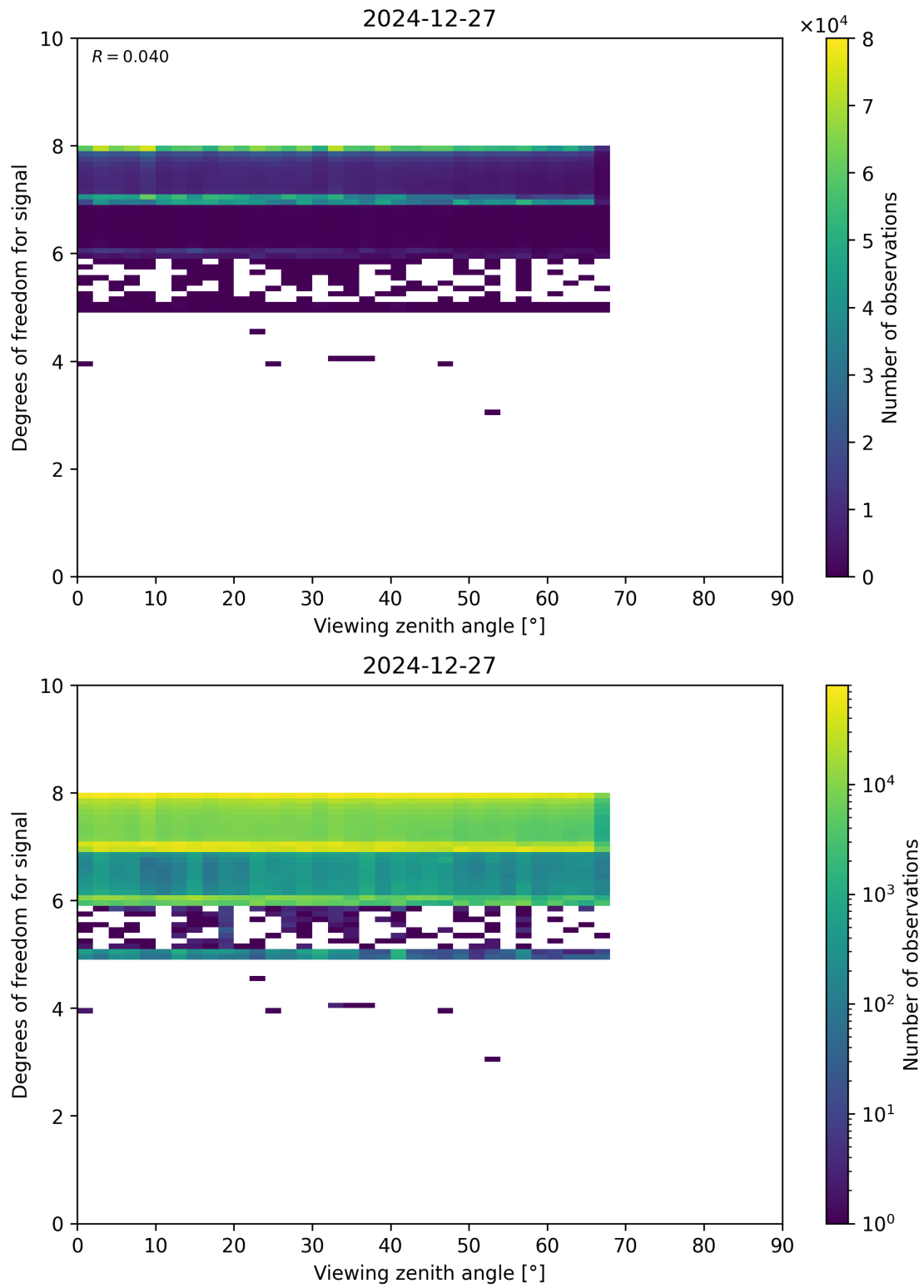
Figure 73: Scatter density plot of “Viewing zenith angle” against “Degrees of freedom for signal” for 2024-12-27 to 2024-12-28.
