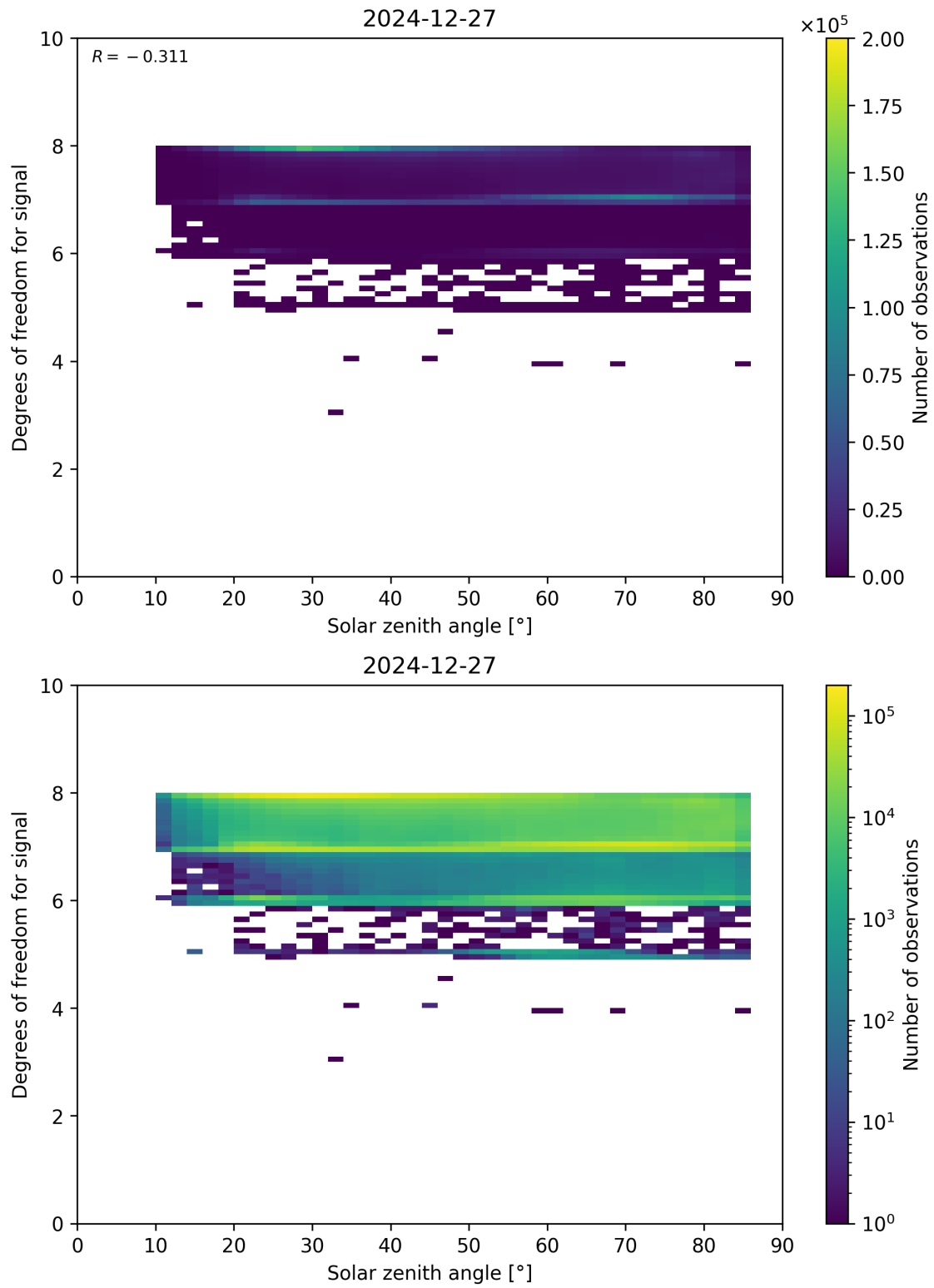
Figure 65: Scatter density plot of “Solar zenith angle” against “Degrees of freedom for signal” for 2024-12-27 to 2024-12-28.
