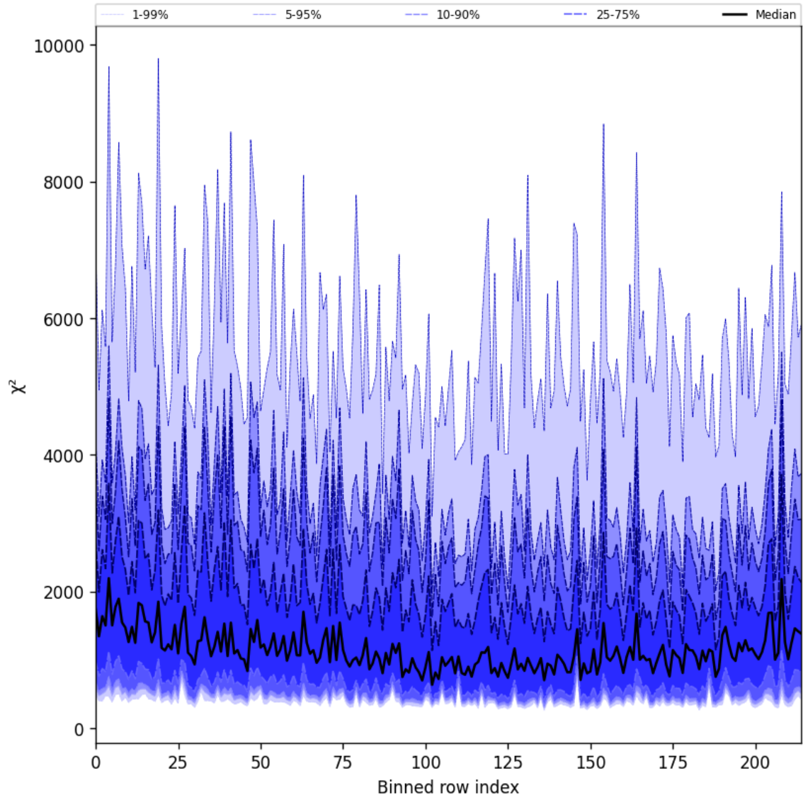
Figure 30: Along track statistics of “ \chi^2 ” for 2024-12-27 to 2024-12-28
