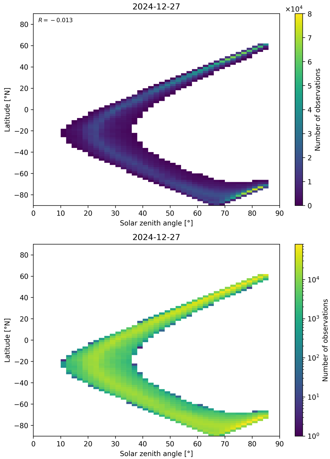
Figure 66: Scatter density plot of “Solar zenith angle” against “Latitude” for 2024-12-27 to 2024-12-28.
