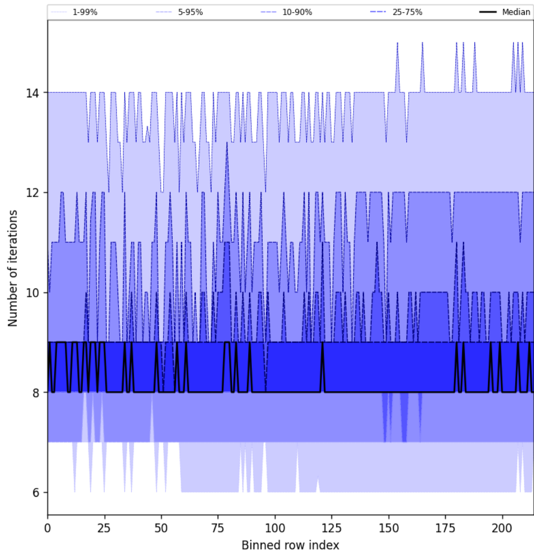
Figure 32: Along track statistics of “Number of iterations” for 2024-12-27 to 2024-12-28
