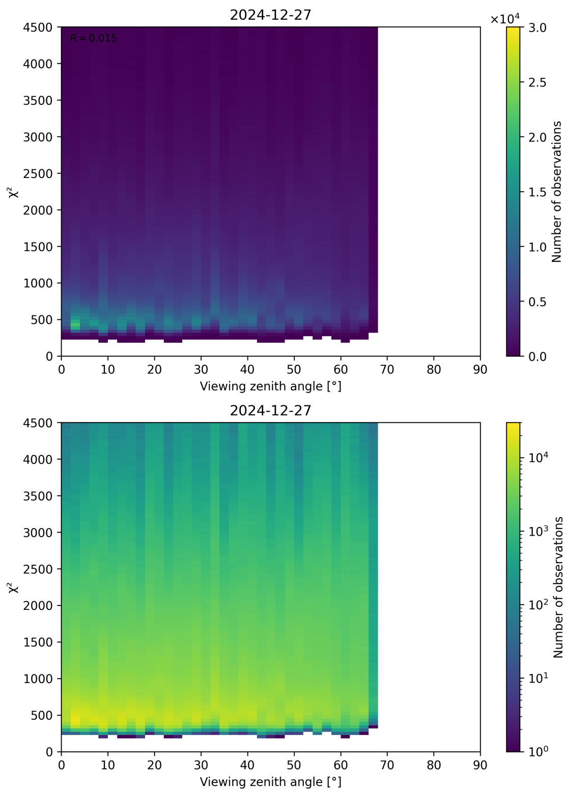
Figure 72: Scatter density plot of “Viewing zenith angle” against “ \chi^2 ” for 2024-12-27 to 2024-12-28.
