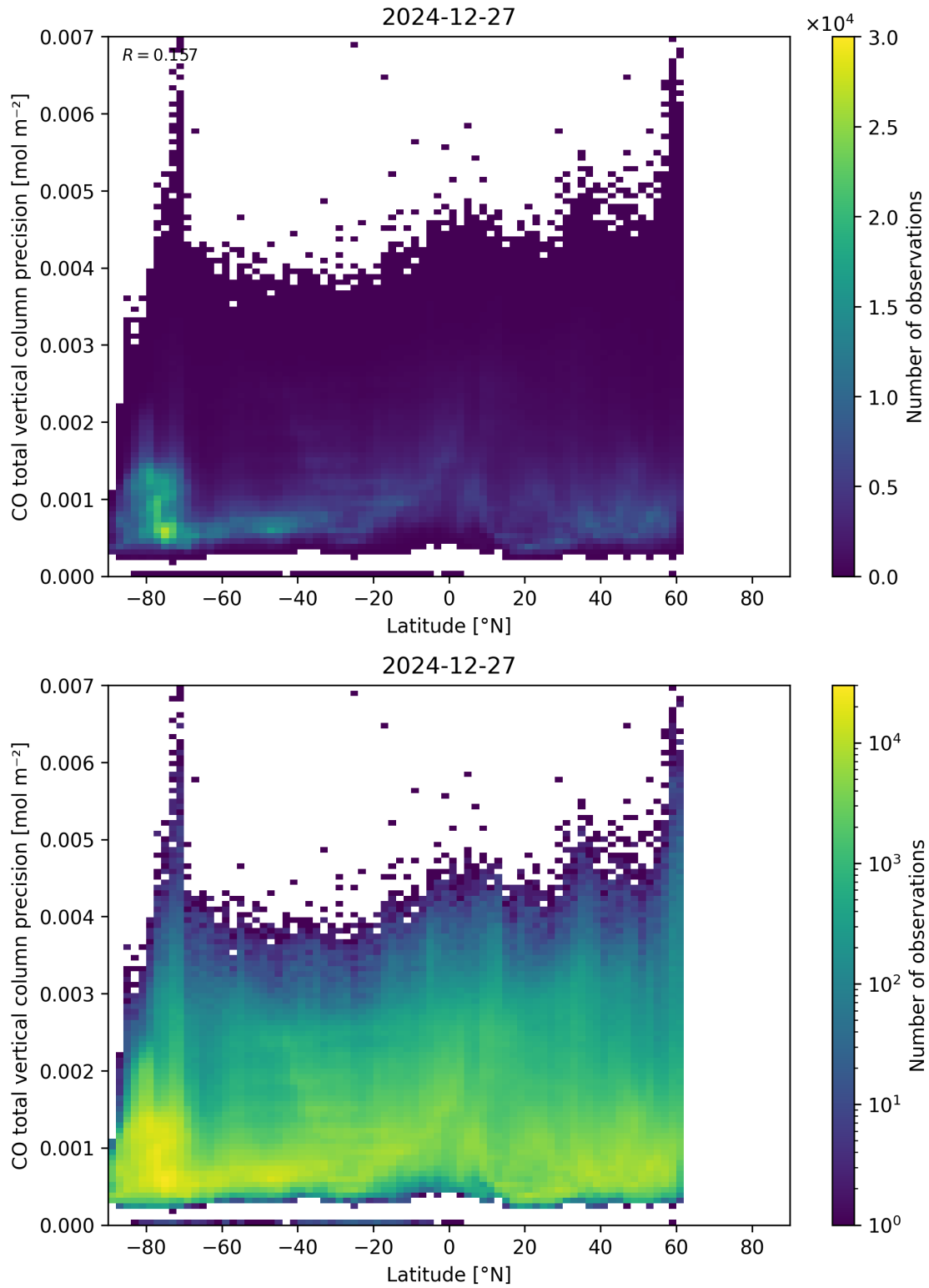
Figure 53: Scatter density plot of “Latitude” against “CO total vertical column precision” for 2024-12-27 to 2024-12-28.
