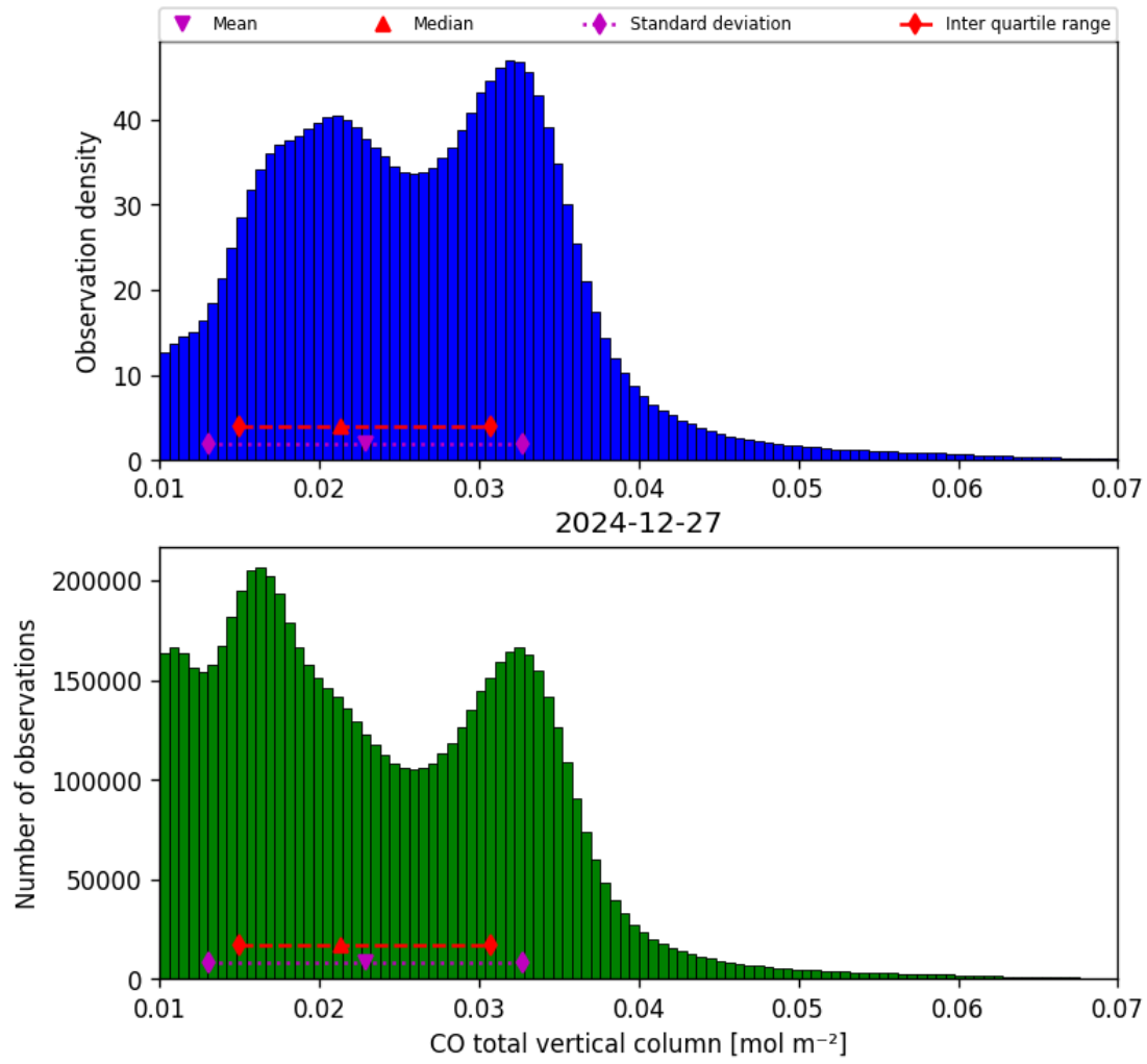
Figure 18: Histogram of “CO total vertical column” for 2024-12-27 to 2024-12-28
