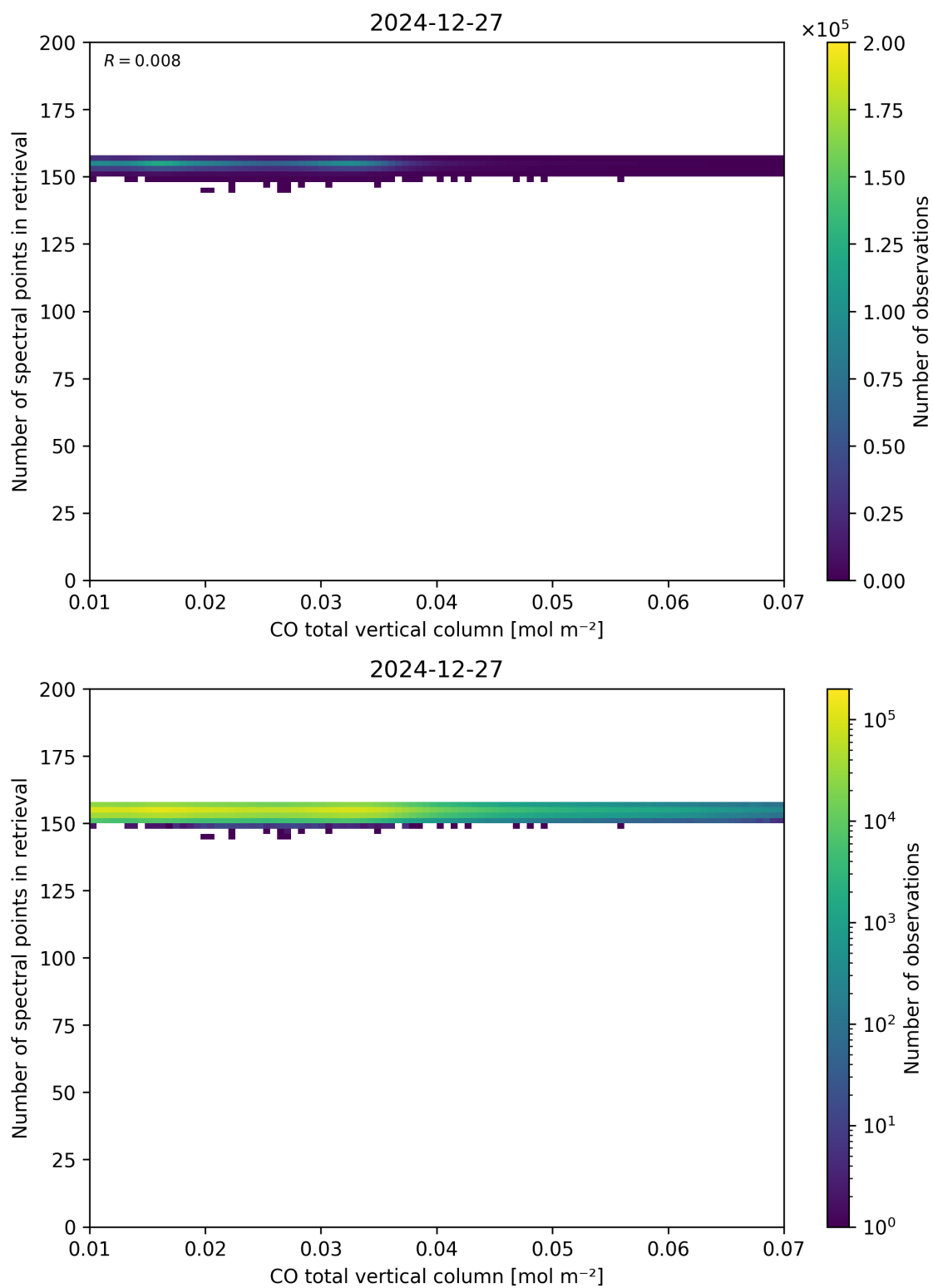
Figure 43: Scatter density plot of “CO total vertical column” against “Number of spectral points in retrieval” for 2024-12-27 to 2024-12-28.
