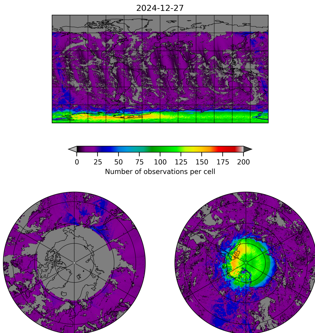
Figure 8: Map of the number of observations for 2024-12-27 to 2024-12-28
