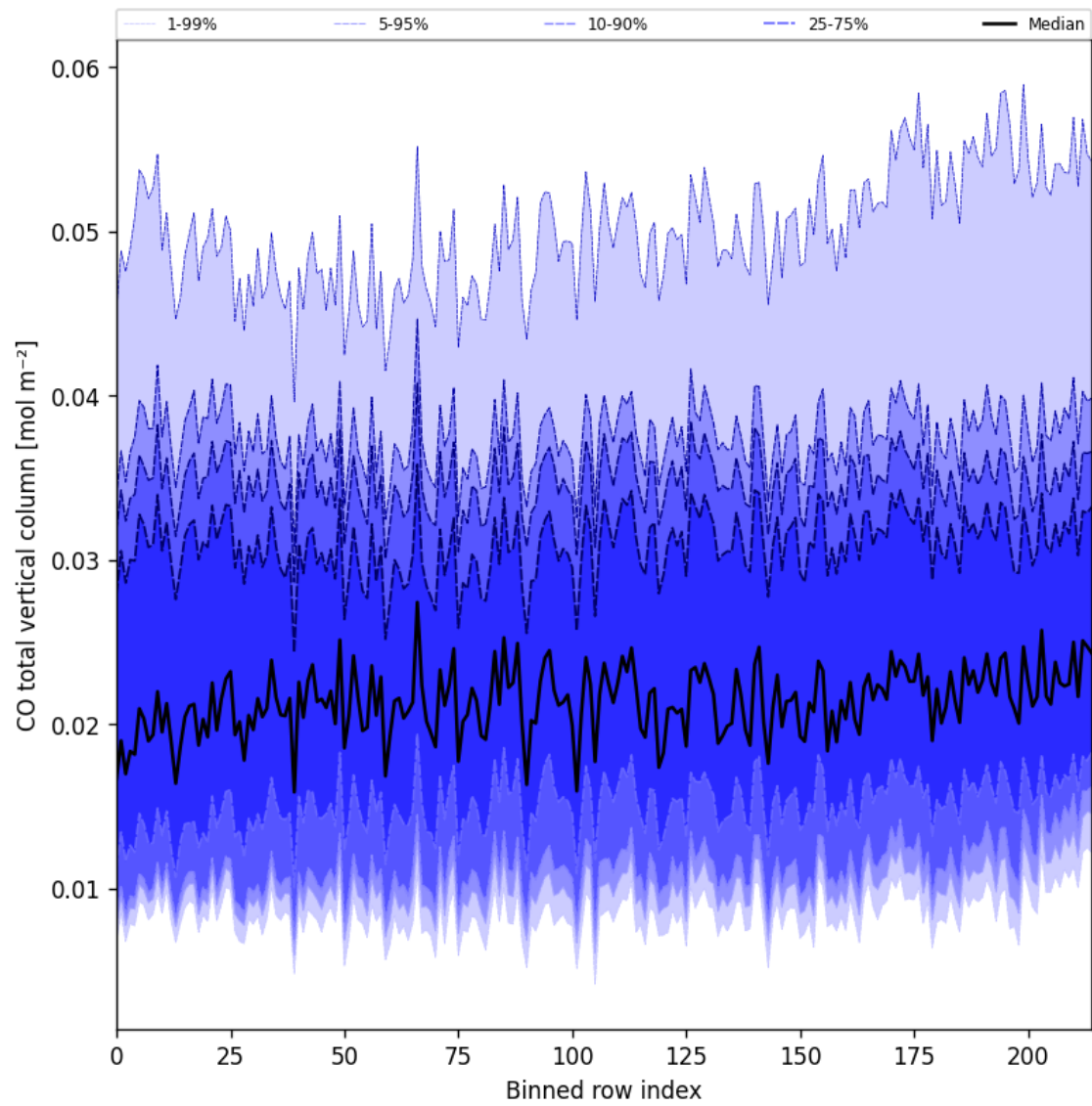
Figure 26: Along track statistics of “CO total vertical column” for 2024-12-27 to 2024-12-28
