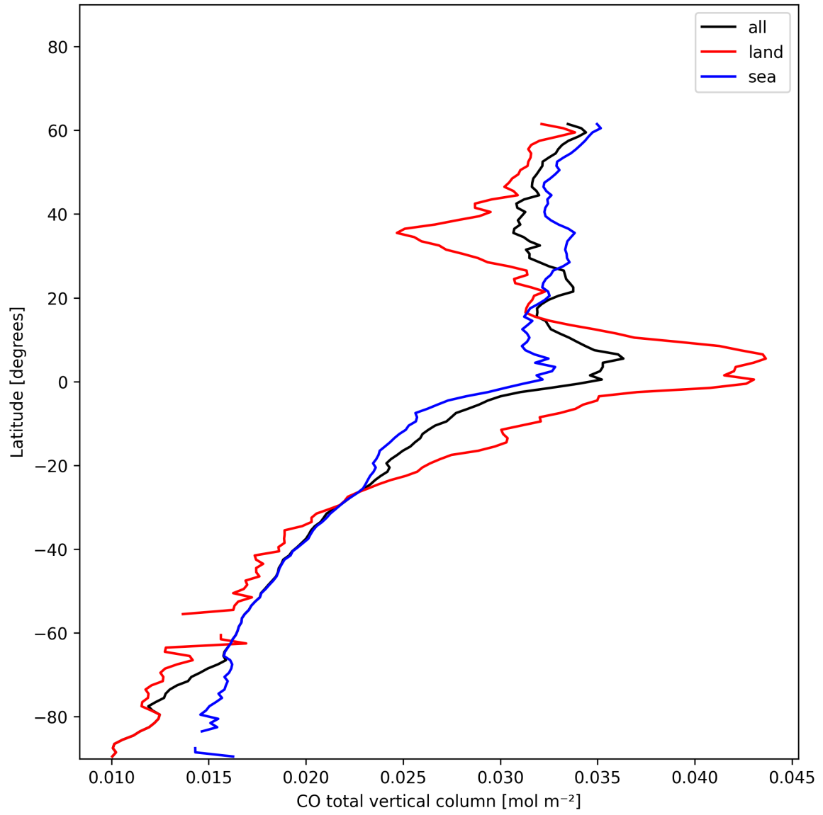
Figure 10: Zonal average of “CO total vertical column” for 2024-12-27 to 2024-12-28.
