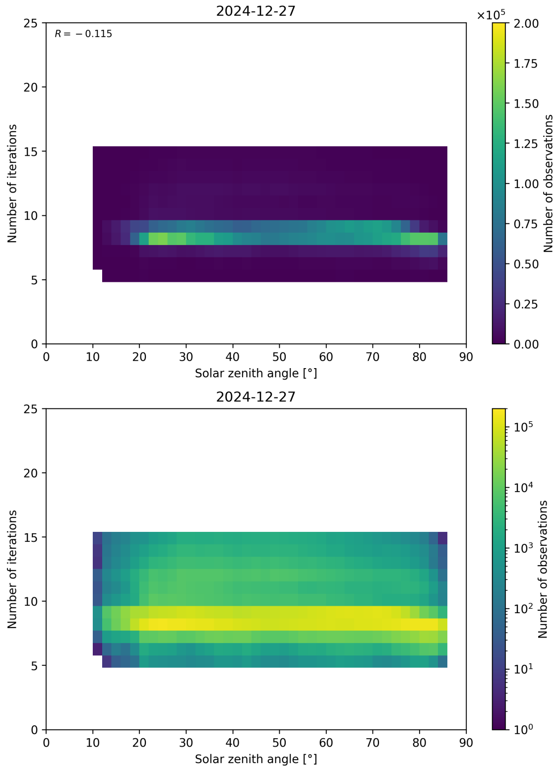
Figure 67: Scatter density plot of “Solar zenith angle” against “Number of iterations” for 2024-12-27 to 2024-12-28.
