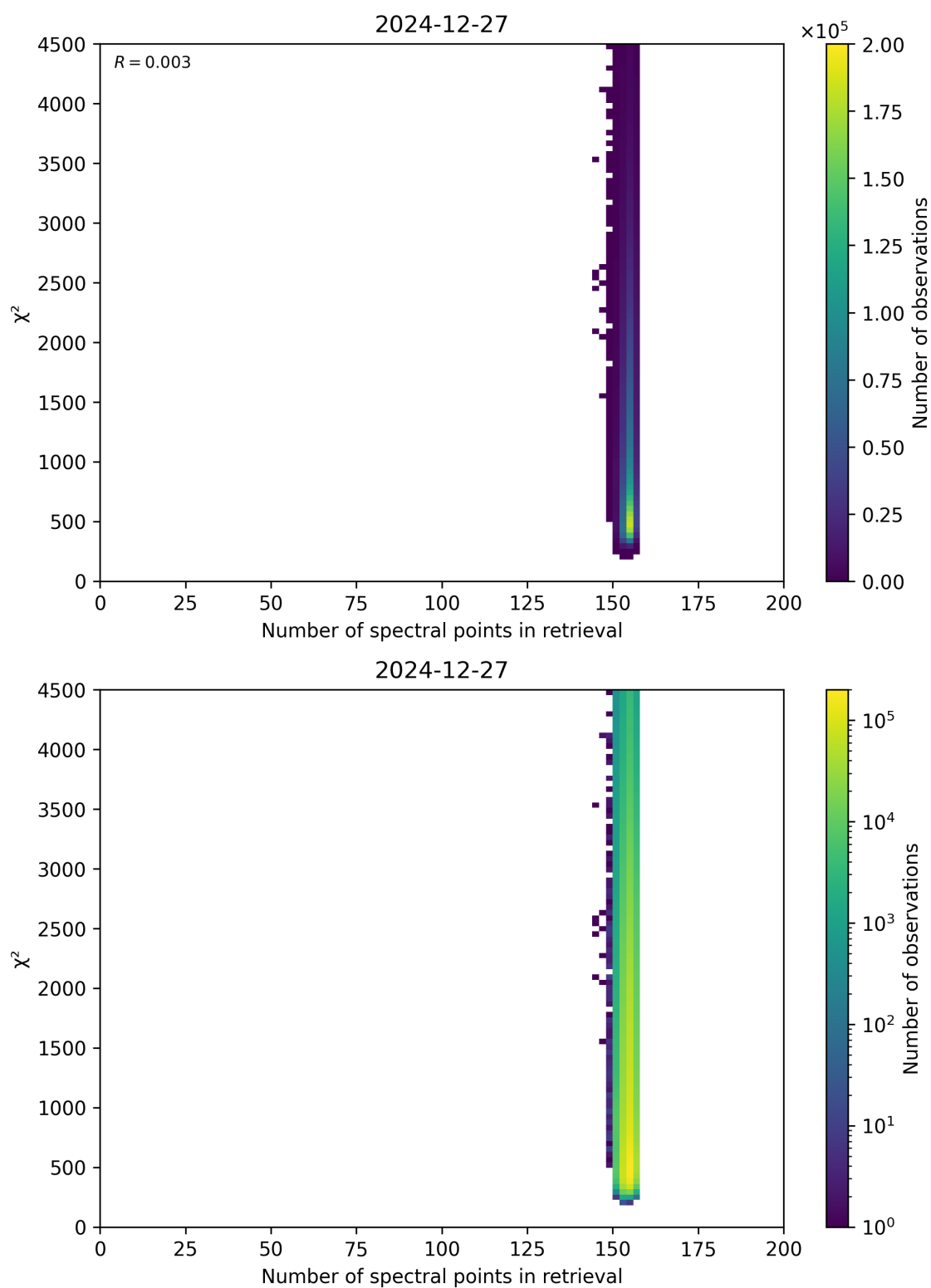
Figure 58: Scatter density plot of “Number of spectral points in retrieval” against “ \chi^2 ” for 2024-12-27 to 2024-12-28.
