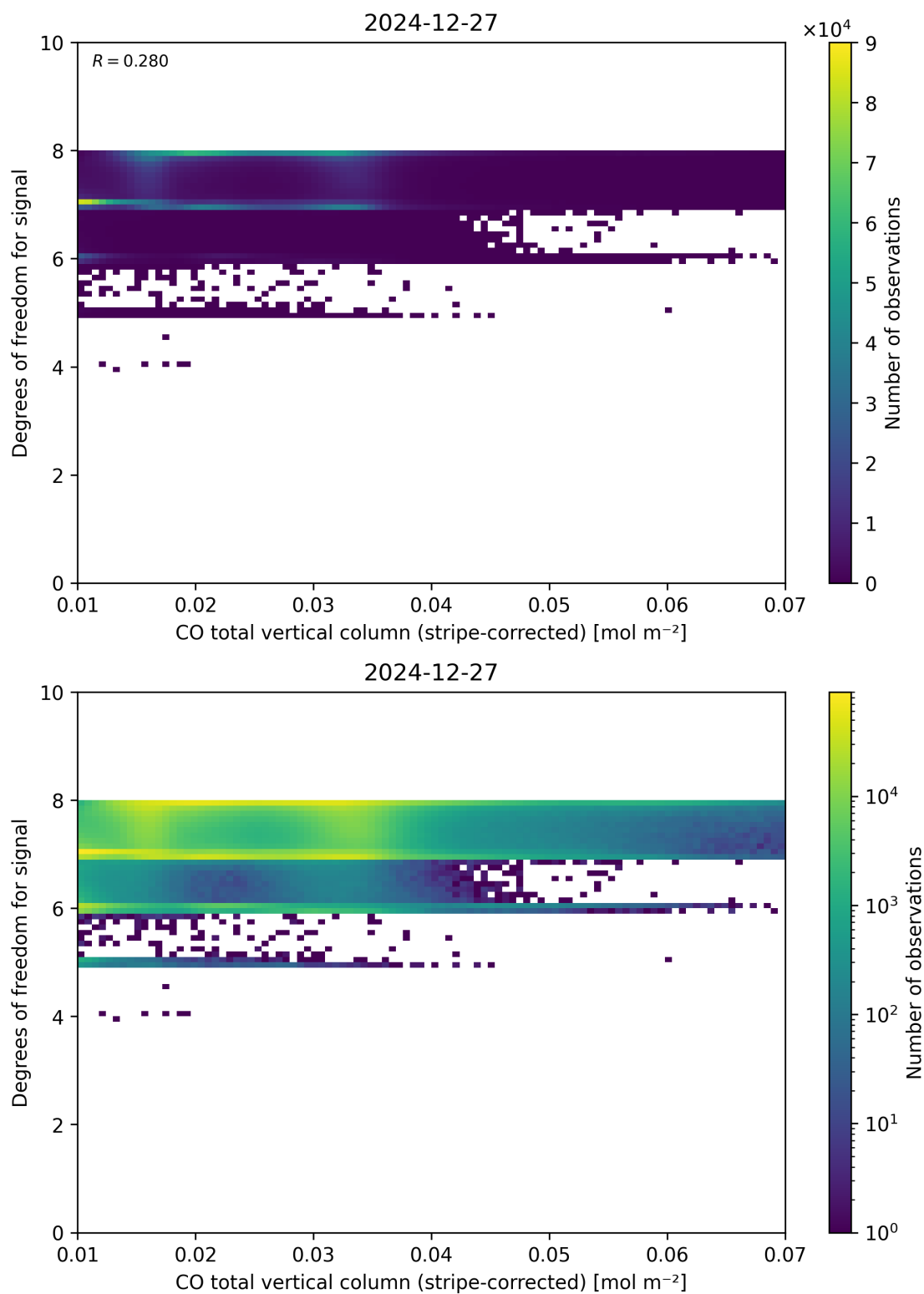
Figure 38: Scatter density plot of “CO total vertical column (stripe-corrected)” against “Degrees of freedom for signal” for 2024-12-27 to 2024-12-28.
