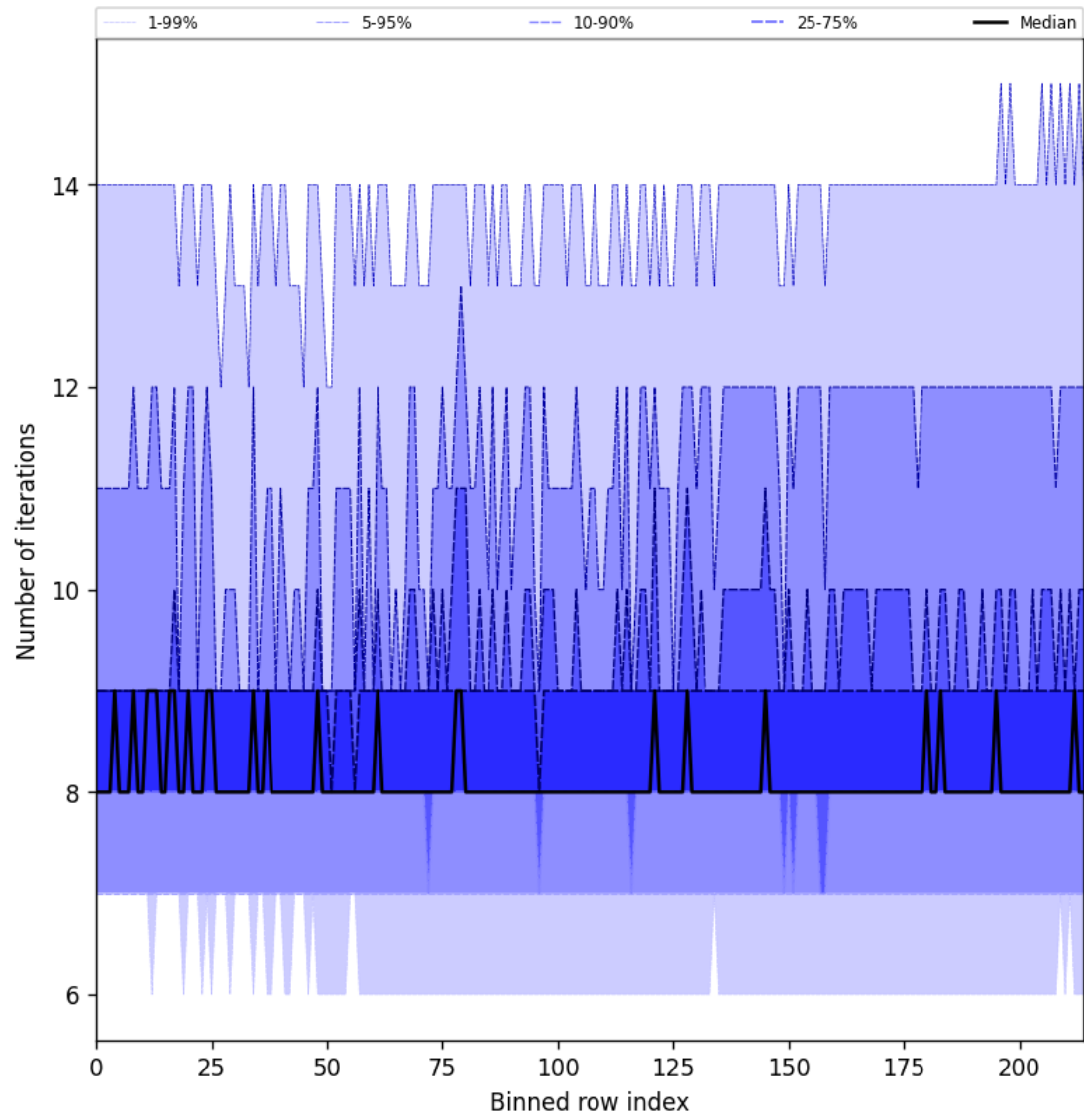
Figure 32: Along track statistics of “Number of iterations” for 2024-12-27 to 2024-12-29
