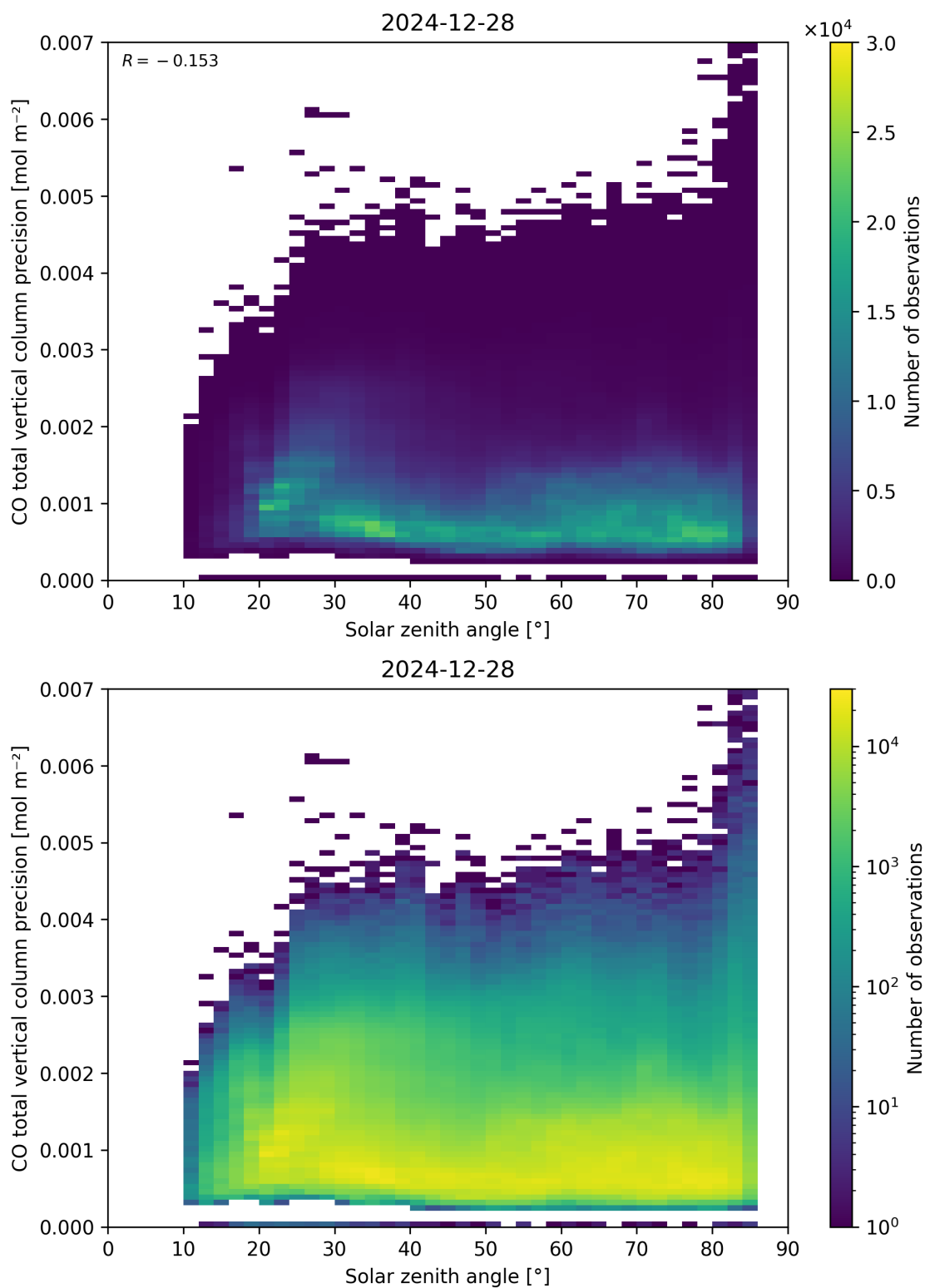
Figure 63: Scatter density plot of “Solar zenith angle” against “CO total vertical column precision” for 2024-12-27 to 2024-12-29.
