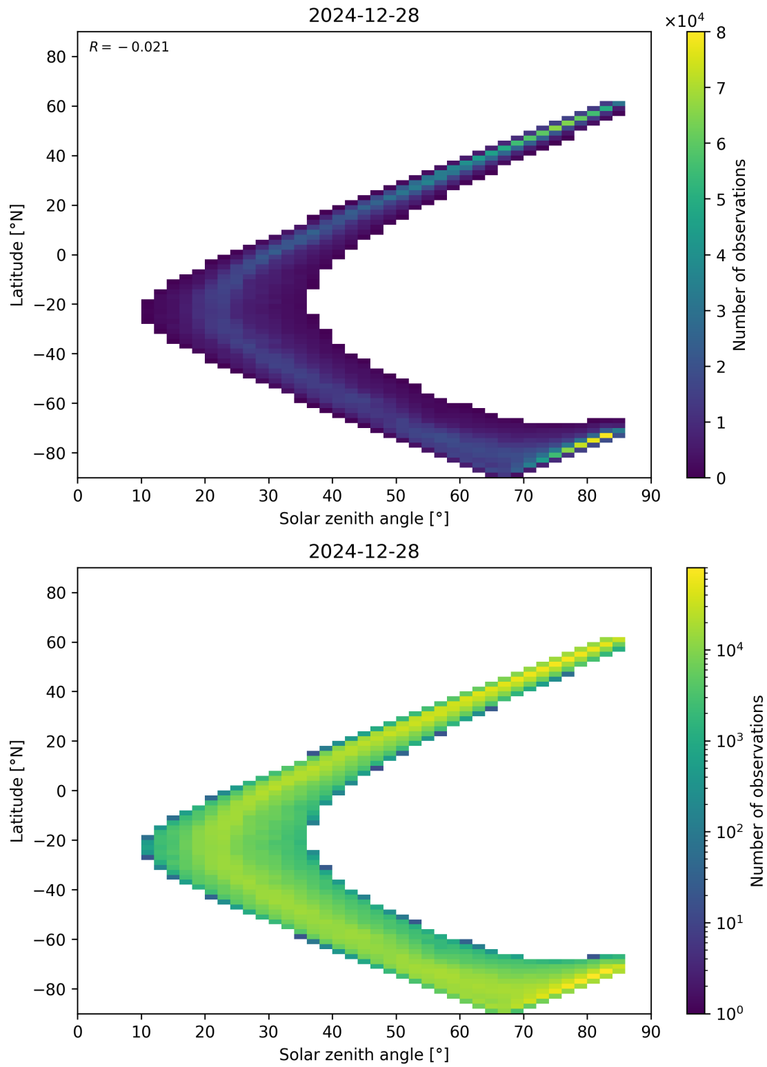
Figure 66: Scatter density plot of “Solar zenith angle” against “Latitude” for 2024-12-27 to 2024-12-29.
