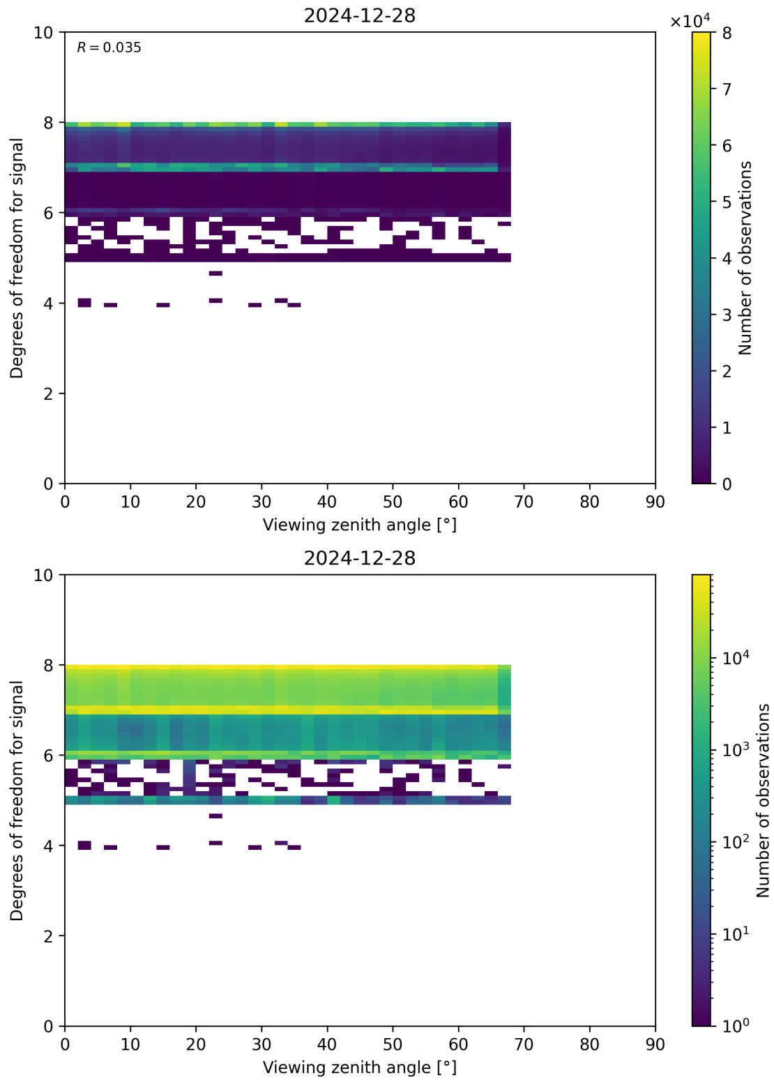
Figure 73: Scatter density plot of “Viewing zenith angle” against “Degrees of freedom for signal” for 2024-12-27 to 2024-12-29.
