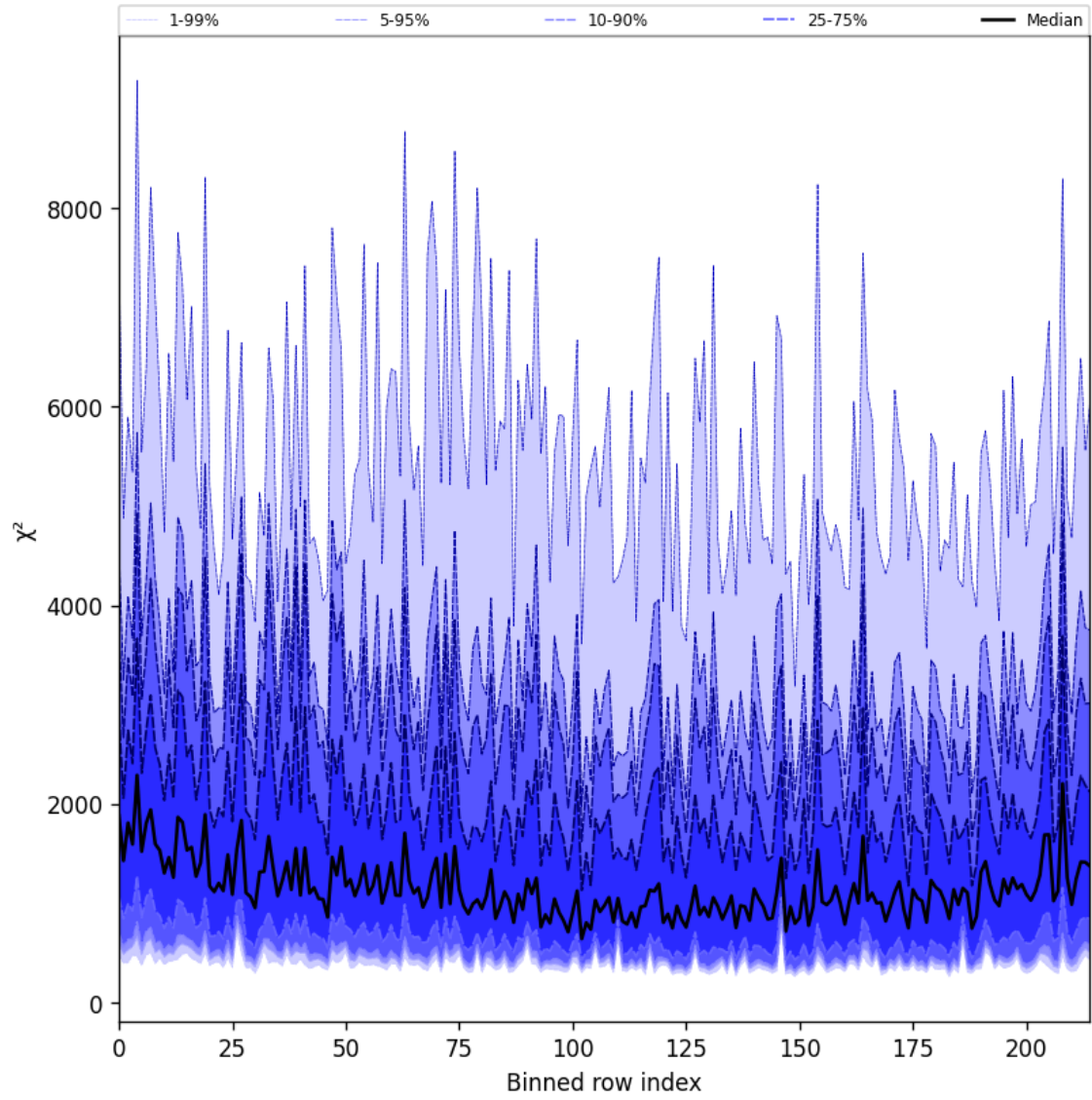
Figure 30: Along track statistics of “ \chi^2 ” for 2024-12-27 to 2024-12-29
