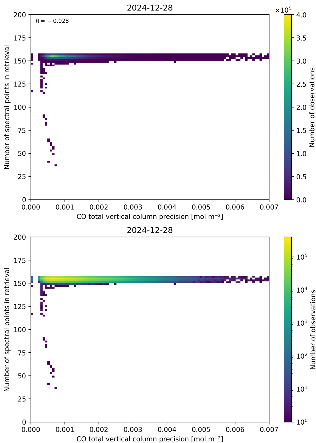
Figure 47: Scatter density plot of “CO total vertical column precision” against “Number of spectral points in retrieval” for 2024-12-27 to 2024-12-29.
