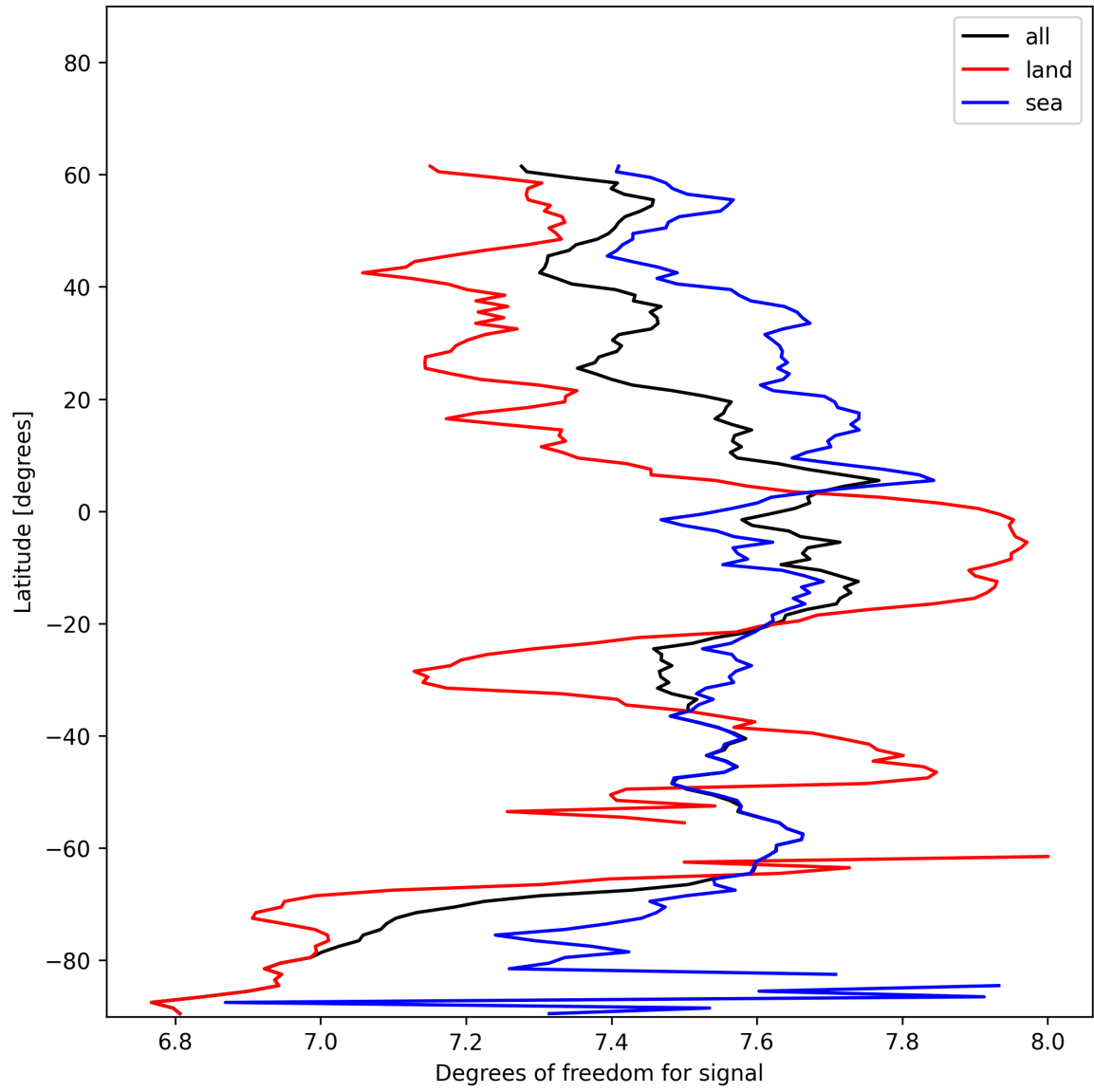
Figure 15: Zonal average of “Degrees of freedom for signal” for 2024-12-27 to 2024-12-29.
