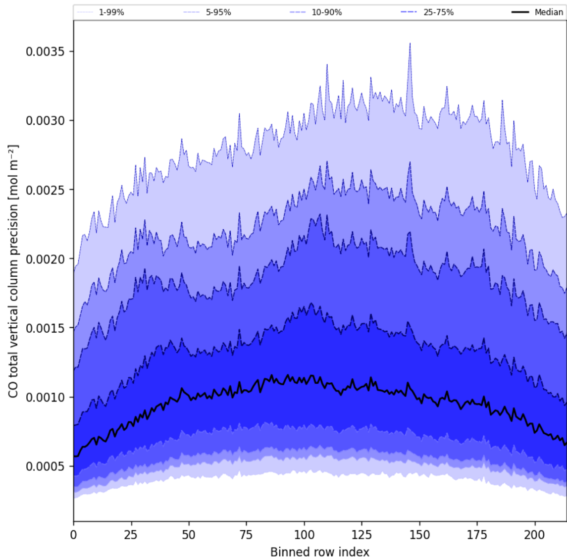
Figure 28: Along track statistics of “CO total vertical column precision” for 2024-12-27 to 2024-12-29
