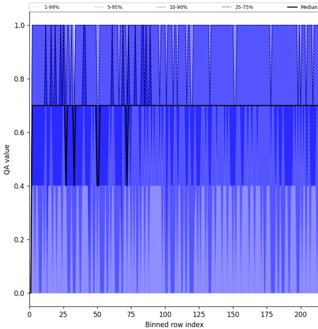
Figure 25: Along track statistics of “QA value” for 2024-12-27 to 2024-12-29
