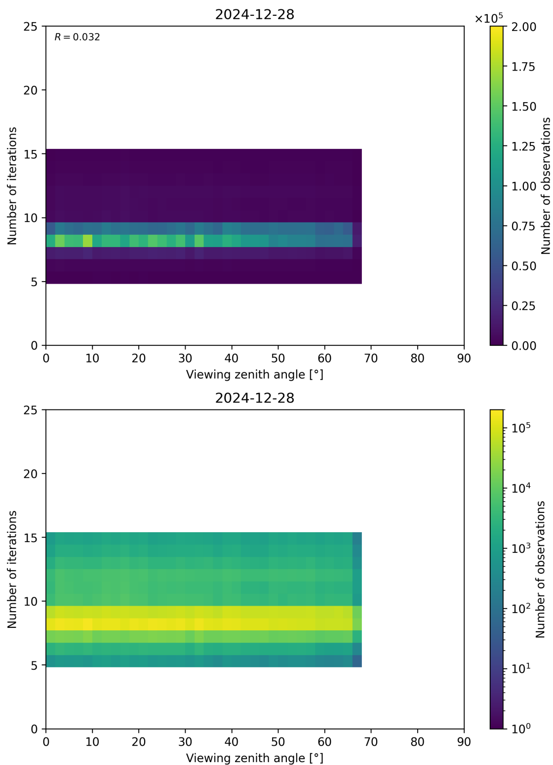
Figure 75: Scatter density plot of “Viewing zenith angle” against “Number of iterations” for 2024-12-27 to 2024-12-29.
