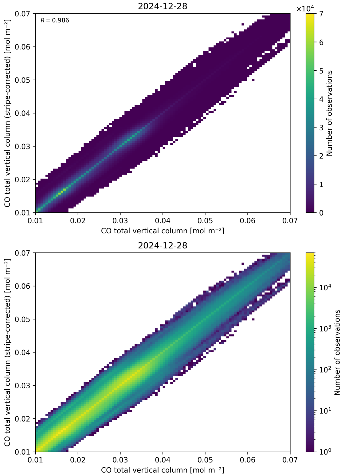
Figure 33: Scatter density plot of “CO total vertical column” against “CO total vertical column (stripe-corrected)” for 2024-12-27 to 2024-12-29.
