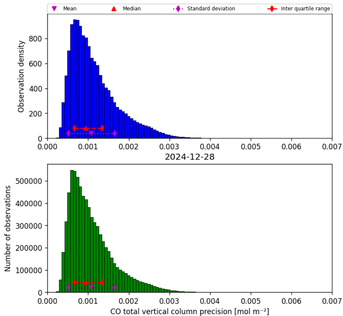
Figure 20: Histogram of “CO total vertical column precision” for 2024-12-27 to 2024-12-29
