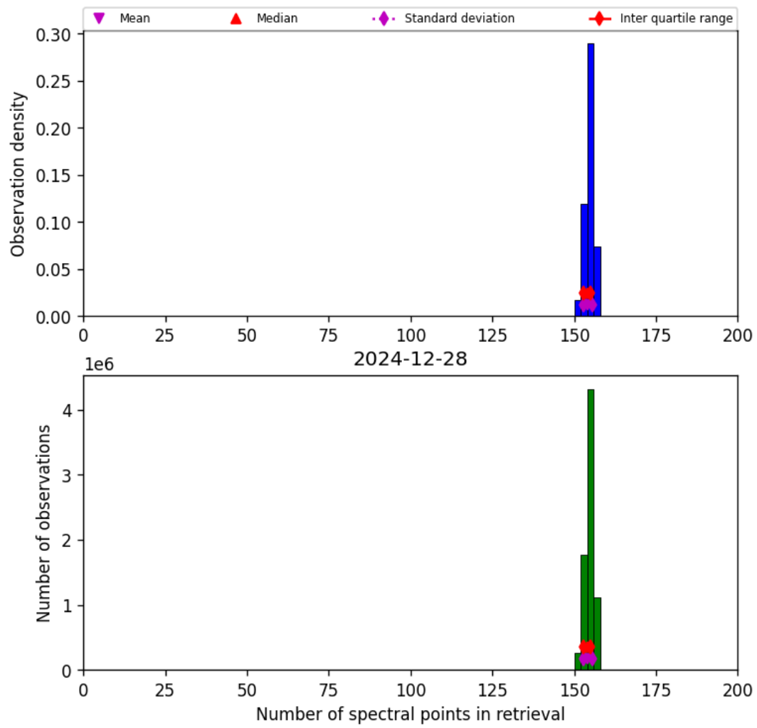
Figure 21: Histogram of “Number of spectral points in retrieval” for 2024-12-27 to 2024-12-29
