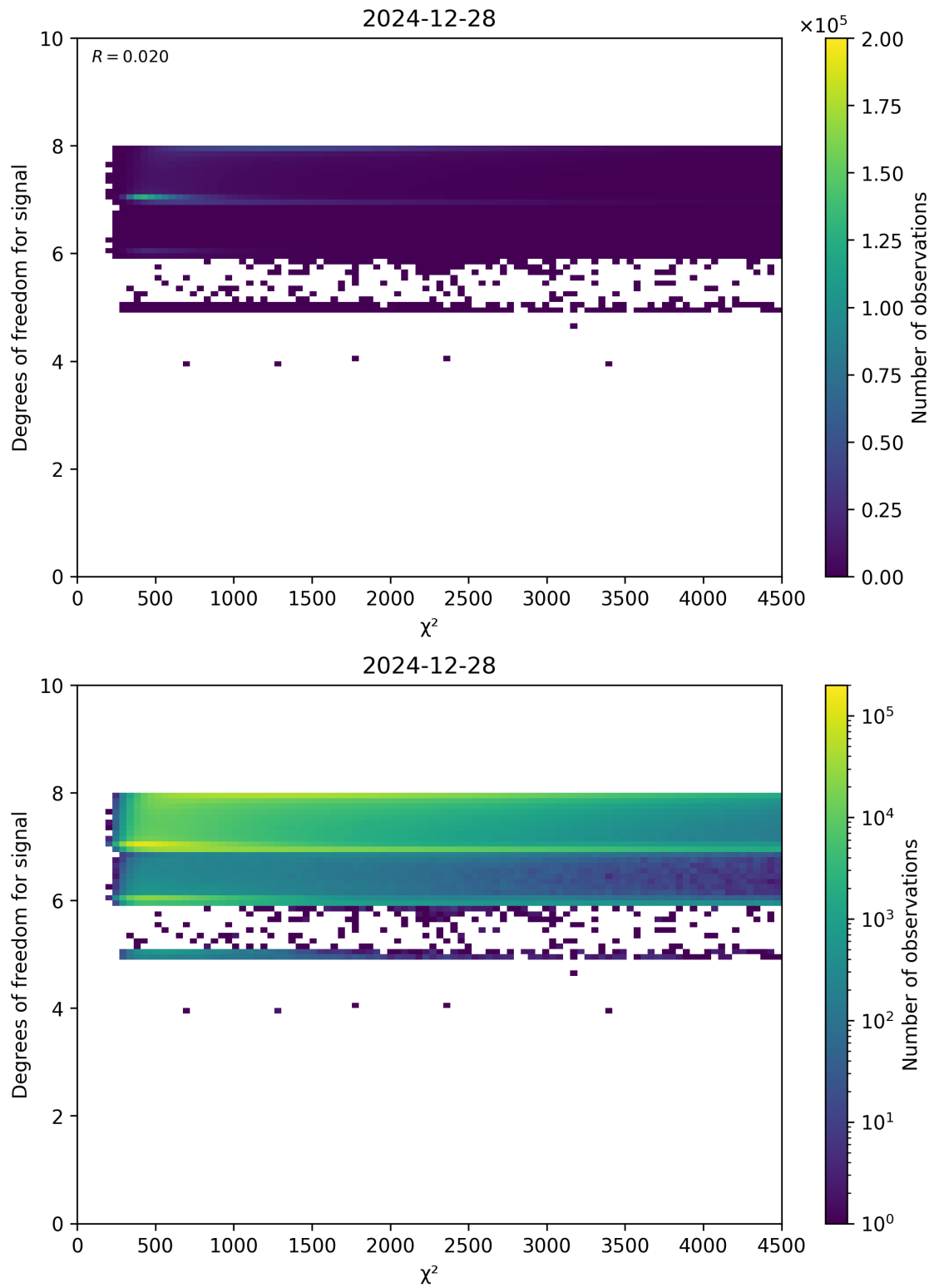
Figure 48: Scatter density plot of “ \chi^2 ” against “Degrees of freedom for signal” for 2024-12-27 to 2024-12-29.
