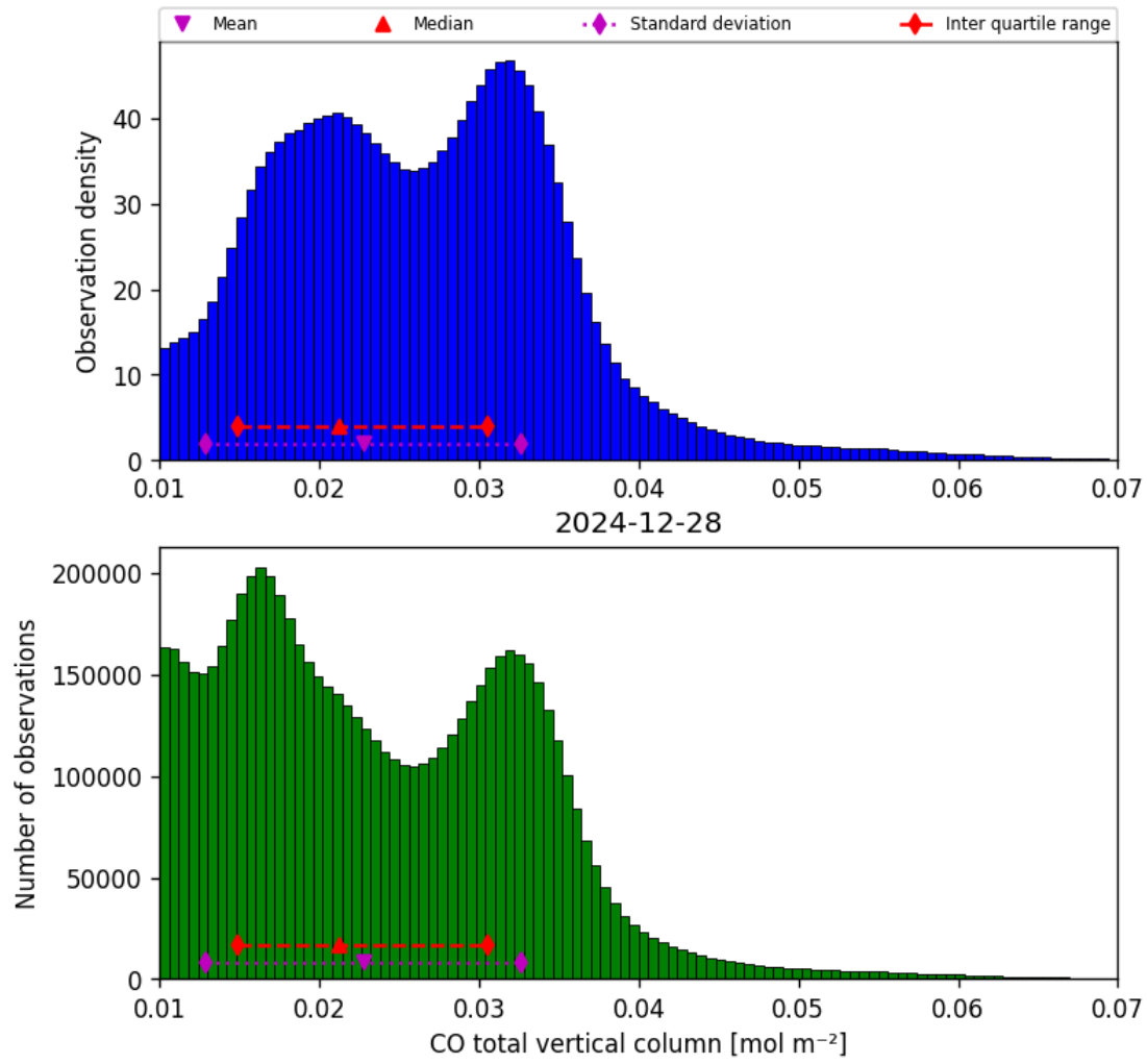
Figure 18: Histogram of “CO total vertical column” for 2024-12-27 to 2024-12-29
