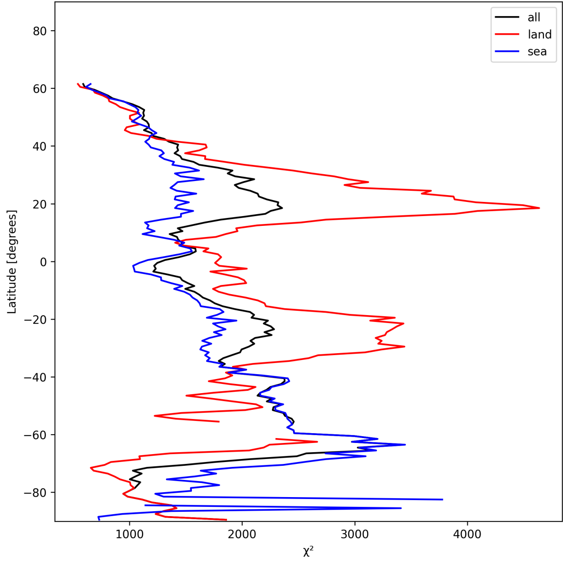
Figure 14: Zonal average of “ \chi^2 ” for 2024-12-27 to 2024-12-29.
