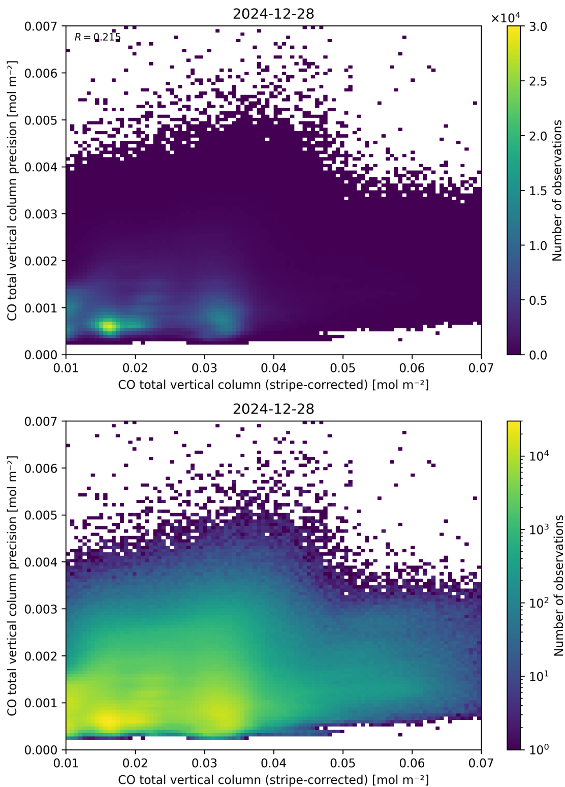
Figure 36: Scatter density plot of “CO total vertical column (stripe-corrected)” against “CO total vertical column precision” for 2024-12-27 to 2024-12-29.
