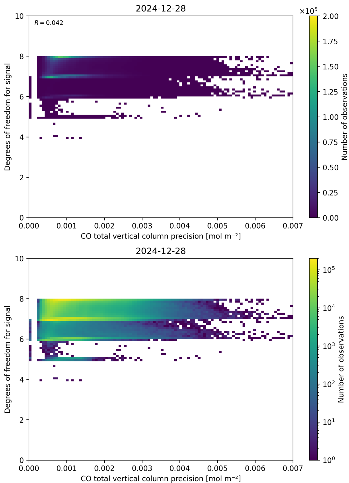
Figure 45: Scatter density plot of “CO total vertical column precision” against “Degrees of freedom for signal” for 2024-12-27 to 2024-12-29.
