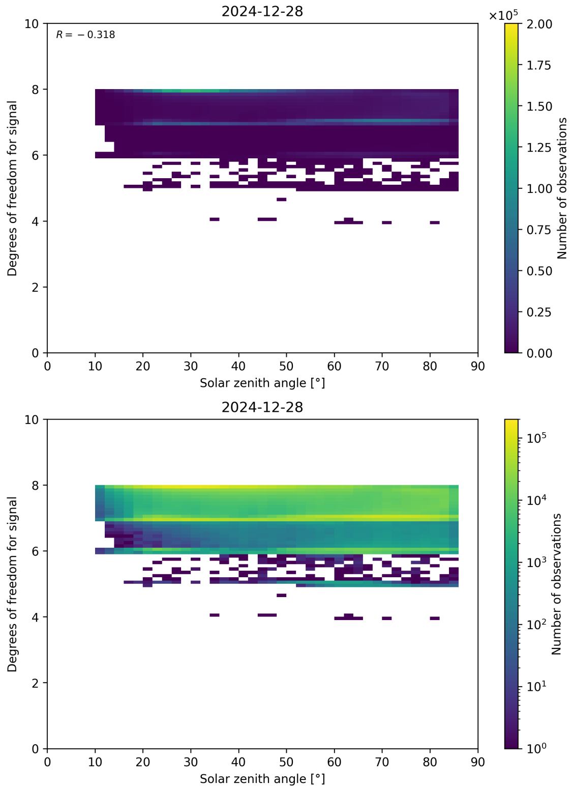
Figure 65: Scatter density plot of “Solar zenith angle” against “Degrees of freedom for signal” for 2024-12-27 to 2024-12-29.
