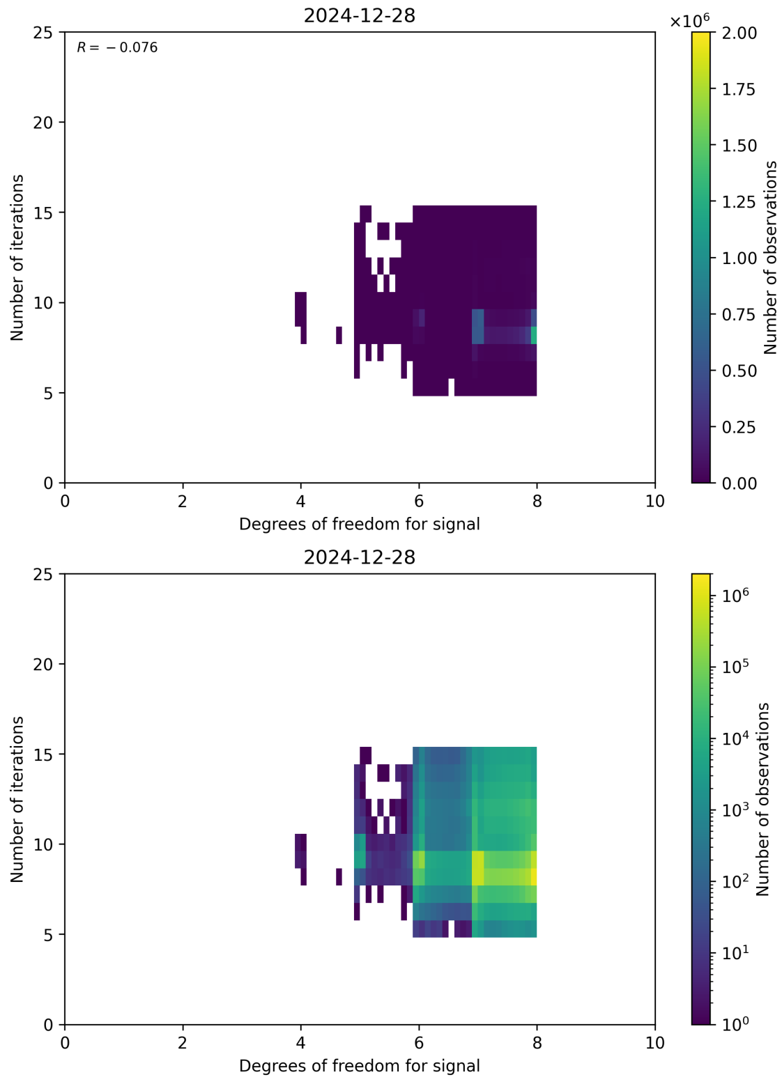
Figure 50: Scatter density plot of “Degrees of freedom for signal” against “Number of iterations” for 2024-12-27 to 2024-12-29.
