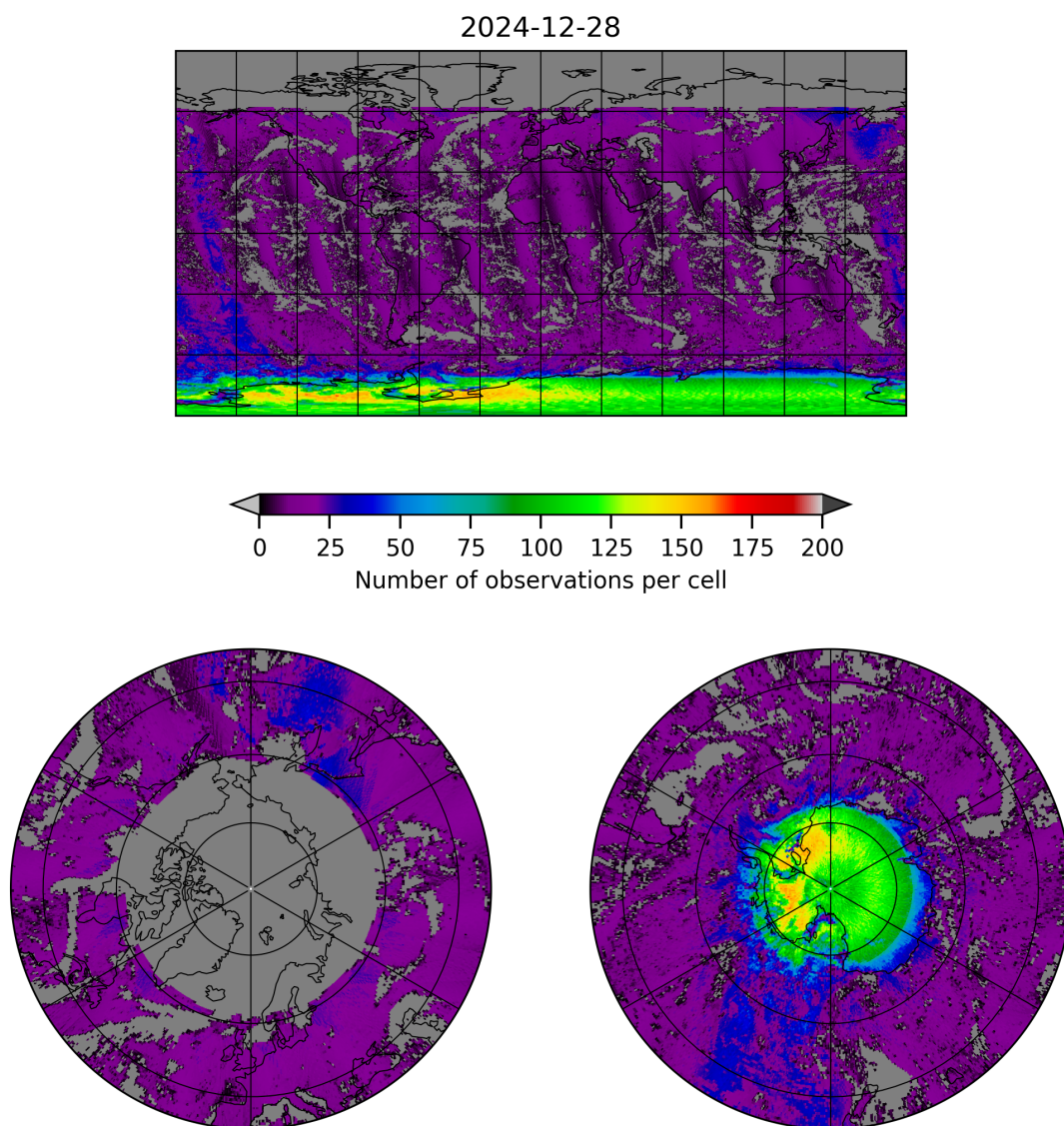
Figure 8: Map of the number of observations for 2024-12-27 to 2024-12-29
