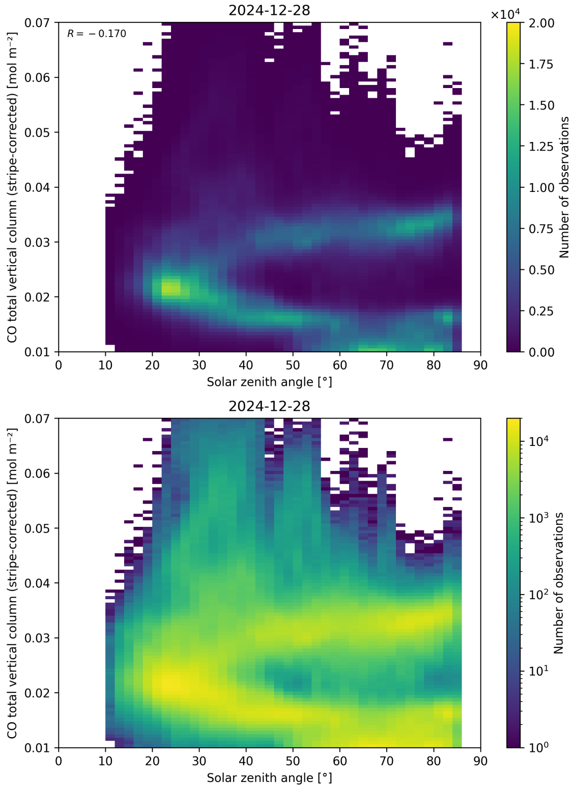
Figure 62: Scatter density plot of “Solar zenith angle” against “CO total vertical column (stripe-corrected)” for 2024-12-27 to 2024-12-29.
