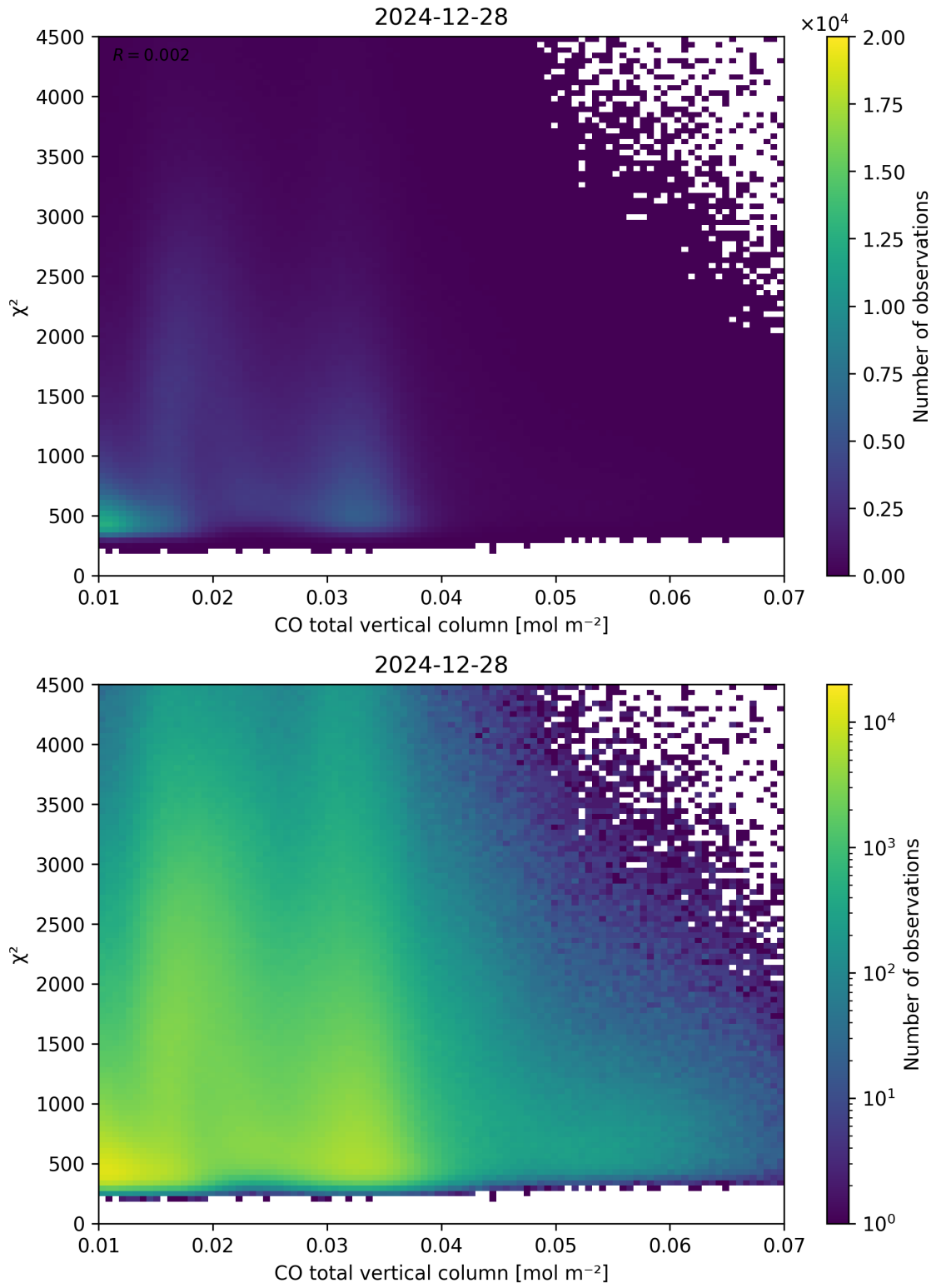
Figure 35: Scatter density plot of “CO total vertical column” against “ \chi^2 ” for 2024-12-27 to 2024-12-29.
