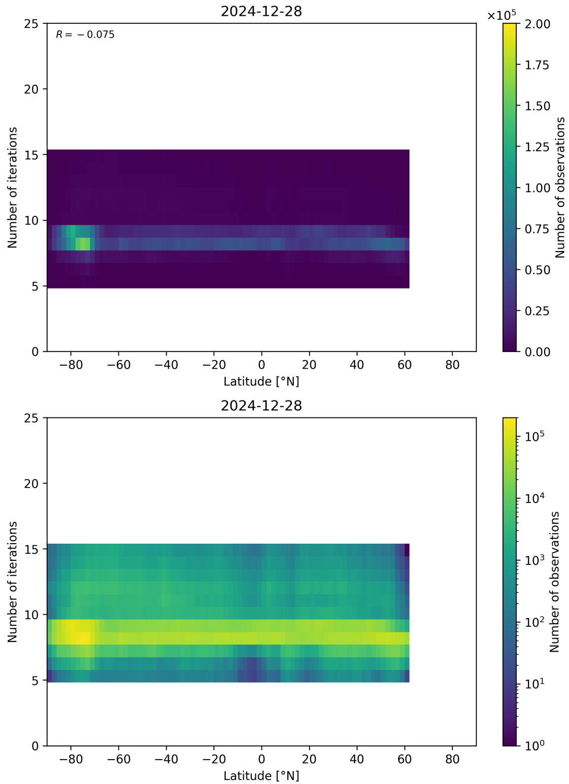
Figure 56: Scatter density plot of “Latitude” against “Number of iterations” for 2024-12-27 to 2024-12-29.
