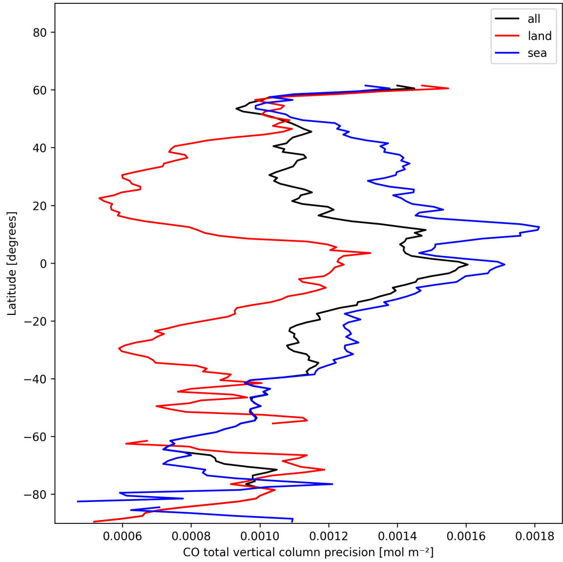
Figure 12: Zonal average of "CO total vertical column precision" for 2024-12-27 to 2024-12-29.
