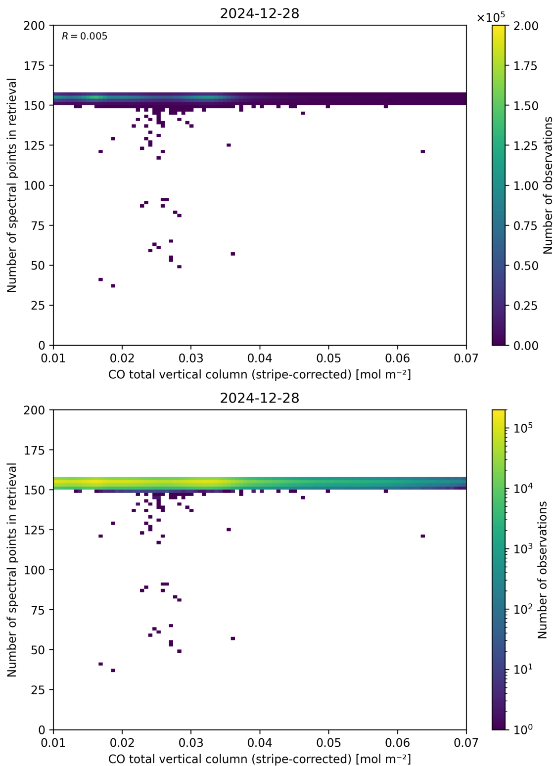
Figure 40: Scatter density plot of “CO total vertical column (stripe-corrected)” against “Number of spectral points in retrieval” for 2024-12-27 to 2024-12-29.
