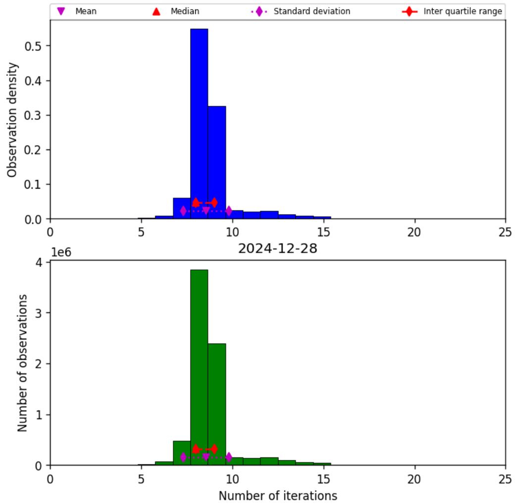
Figure 24: Histogram of “Number of iterations” for 2024-12-27 to 2024-12-29
