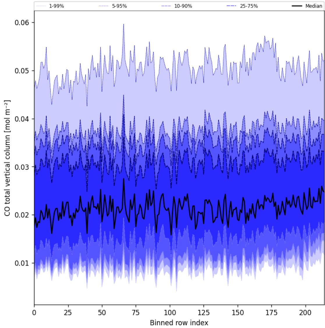
Figure 26: Along track statistics of “CO total vertical column” for 2024-12-27 to 2024-12-29
