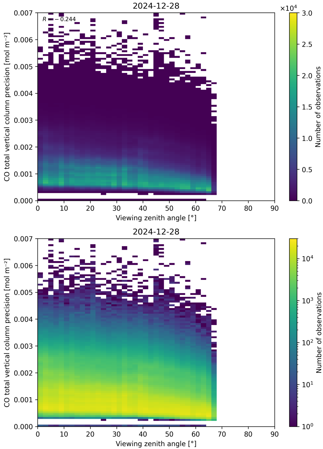
Figure 71: Scatter density plot of “Viewing zenith angle” against “CO total vertical column precision” for 2024-12-27 to 2024-12-29.
