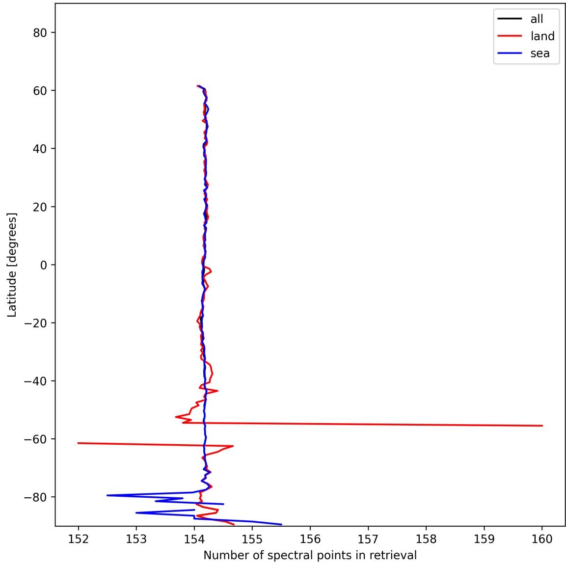
Figure 13: Zonal average of “Number of spectral points in retrieval” for 2024-12-27 to 2024-12-29.
