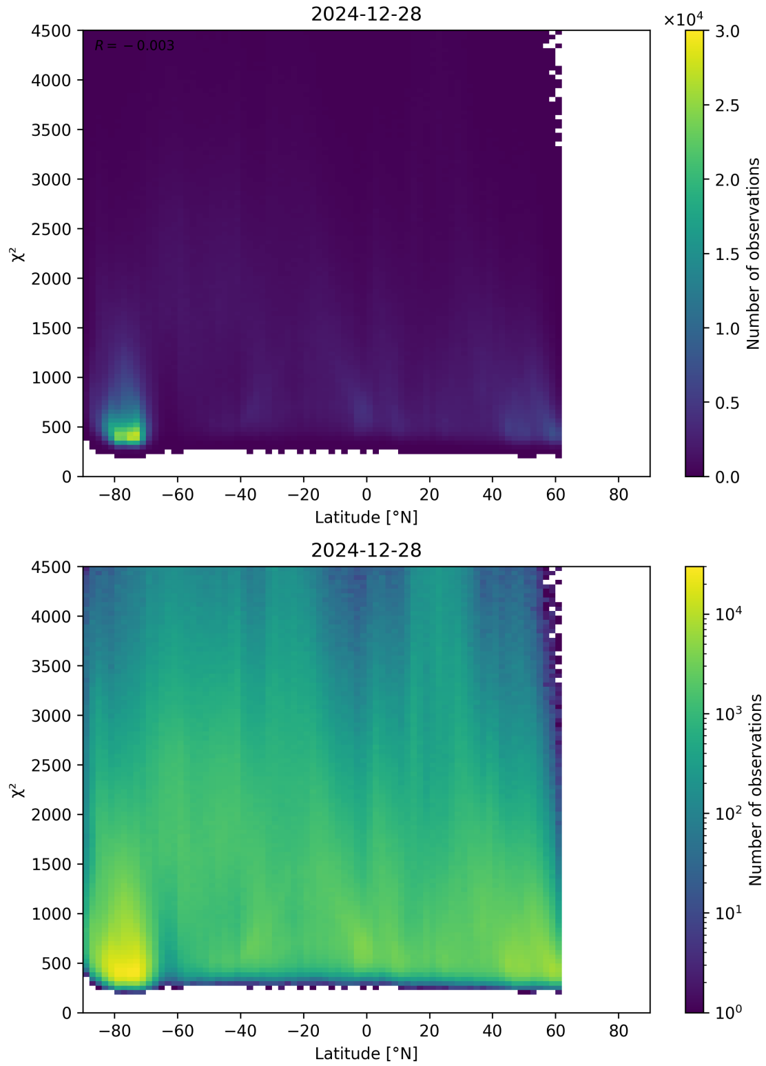
Figure 54: Scatter density plot of “Latitude” against “ \chi^2 ” for 2024-12-27 to 2024-12-29.
