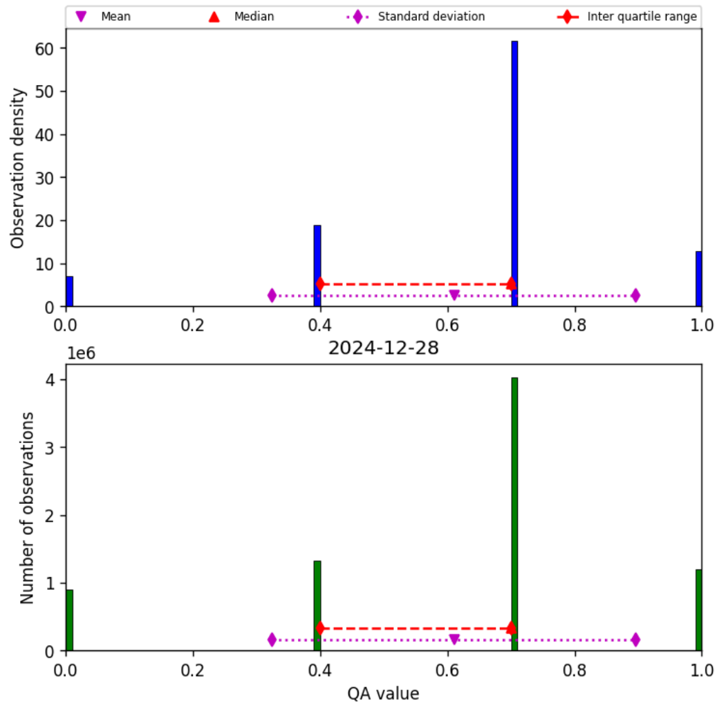
Figure 17: Histogram of “QA value” for 2024-12-27 to 2024-12-29
