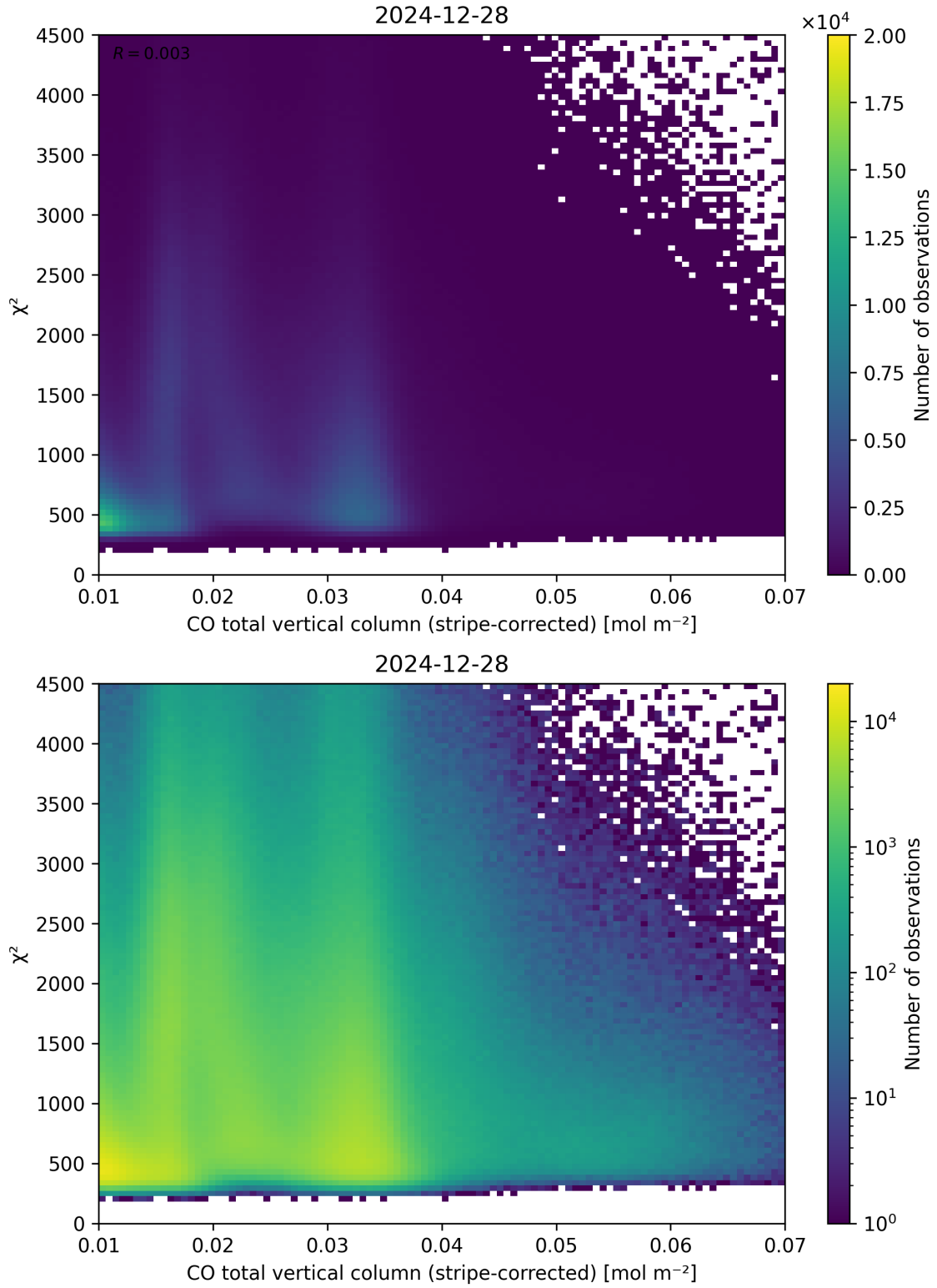
Figure 37: Scatter density plot of “CO total vertical column (stripe-corrected)” against “ \chi^2 ” for 2024-12-27 to 2024-12-29.
