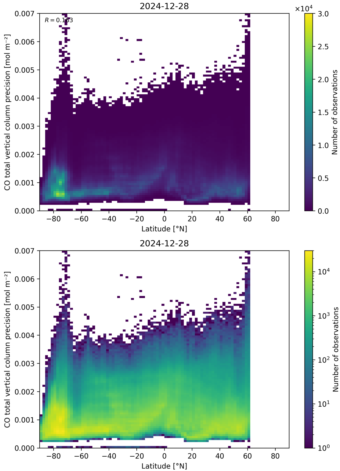
Figure 53: Scatter density plot of “Latitude” against “CO total vertical column precision” for 2024-12-27 to 2024-12-29.
