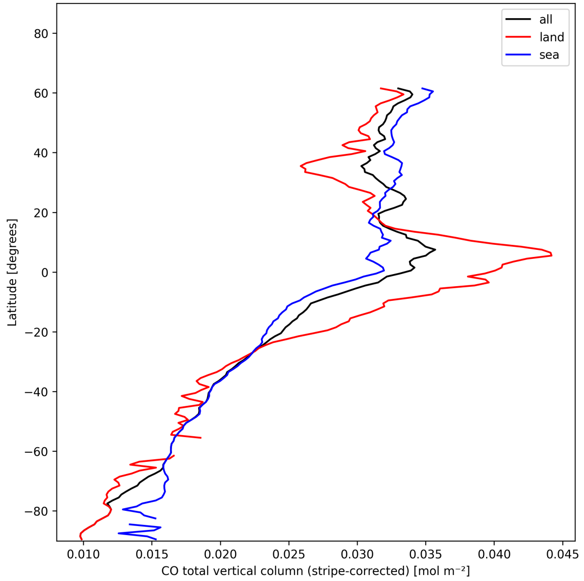
Figure 11: Zonal average of “CO total vertical column (stripe-corrected)” for 2024-12-27 to 2024-12-29.
