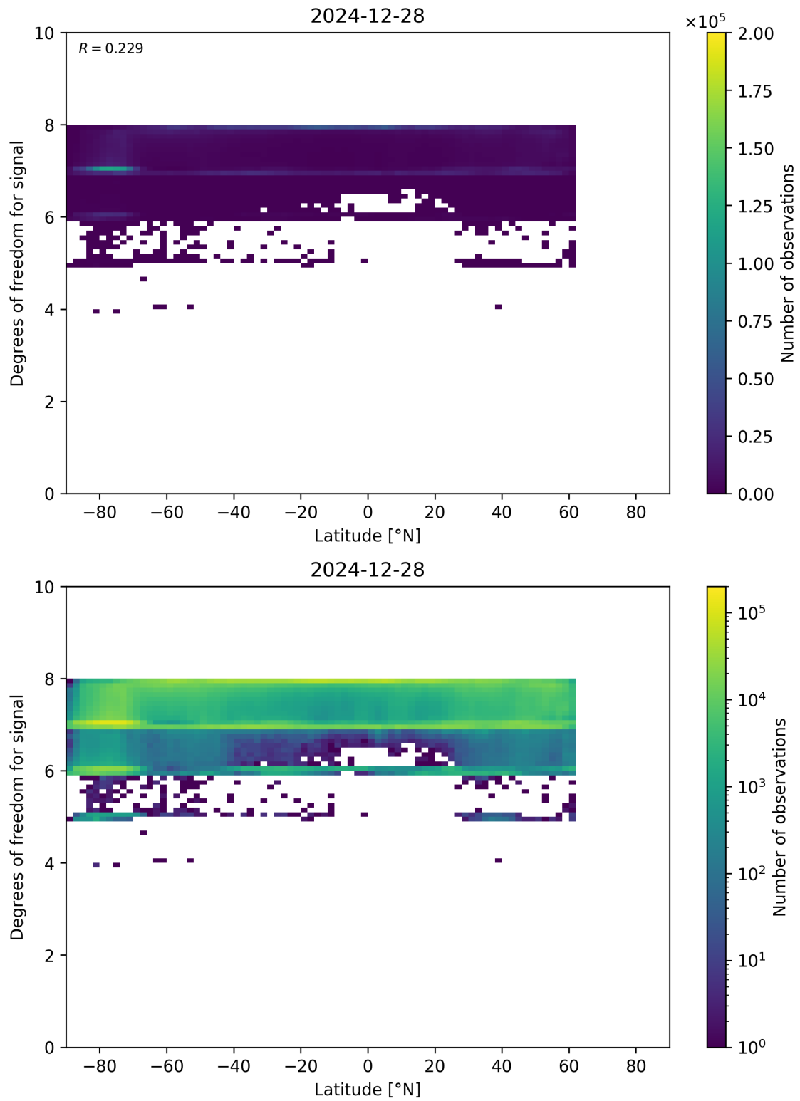
Figure 55: Scatter density plot of “Latitude” against “Degrees of freedom for signal” for 2024-12-27 to 2024-12-29.
