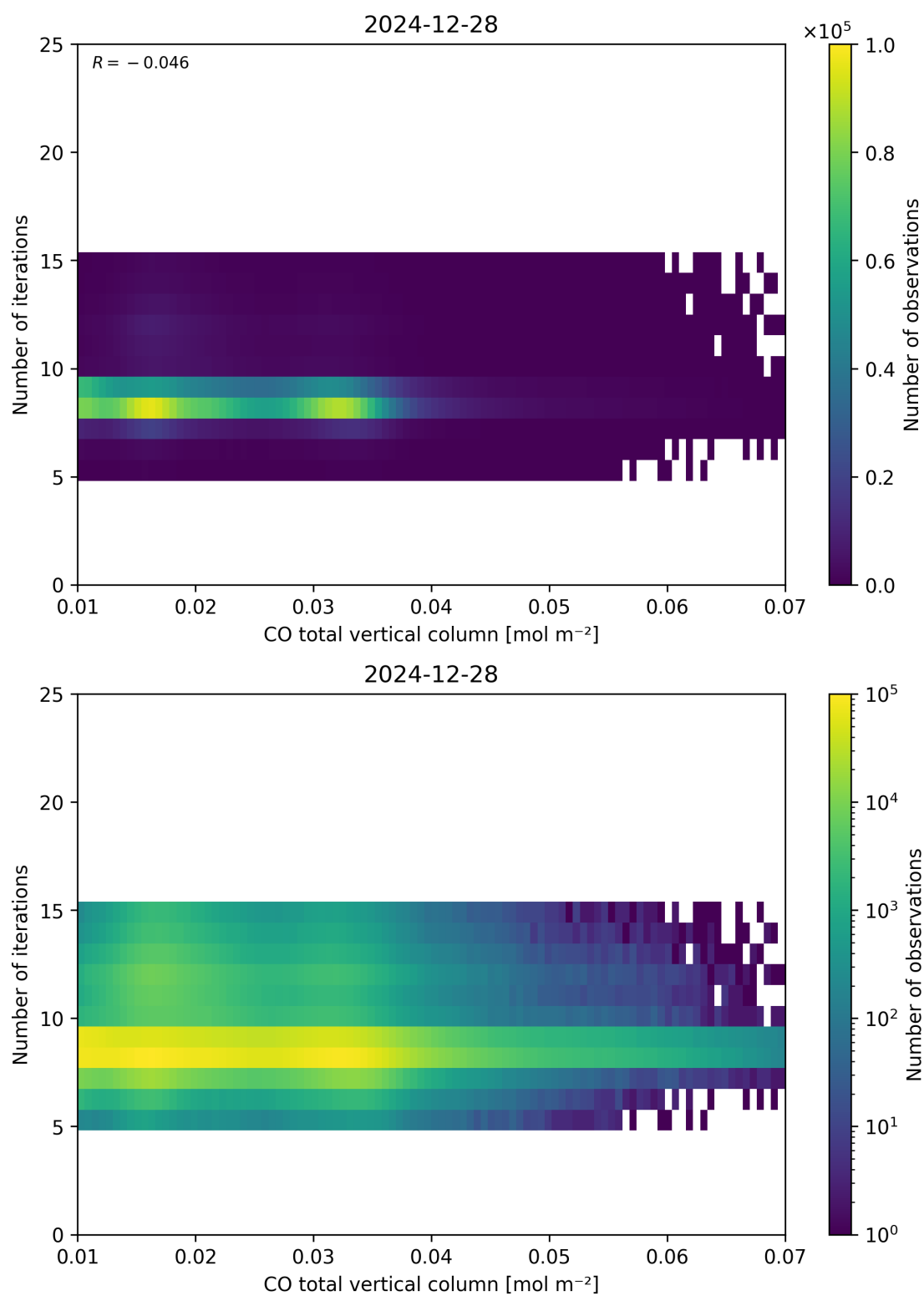
Figure 42: Scatter density plot of “CO total vertical column” against “Number of iterations” for 2024-12-27 to 2024-12-29.
