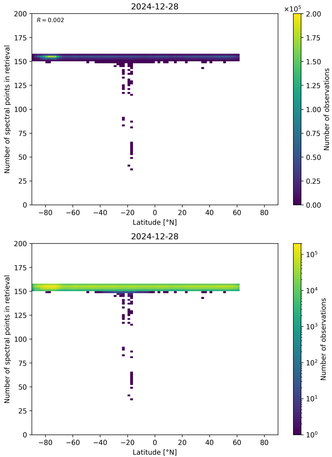
Figure 57: Scatter density plot of “Latitude” against “Number of spectral points in retrieval” for 2024-12-27 to 2024-12-29.
