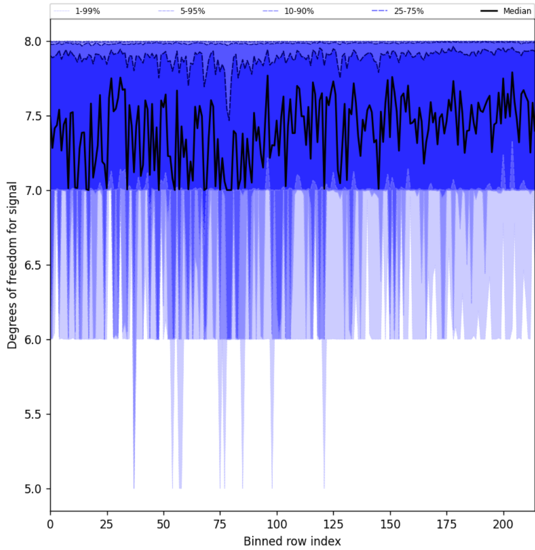
Figure 31: Along track statistics of “Degrees of freedom for signal” for 2024-12-27 to 2024-12-29
