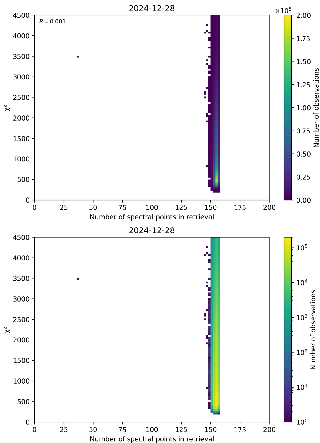
Figure 58: Scatter density plot of “Number of spectral points in retrieval” against “ \chi^2 ” for 2024-12-27 to 2024-12-29.
