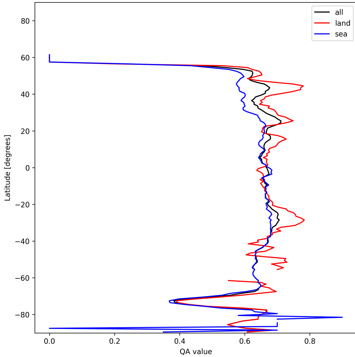
Figure 9: Zonal average of “QA value” for 2024-12-27 to 2024-12-29.
