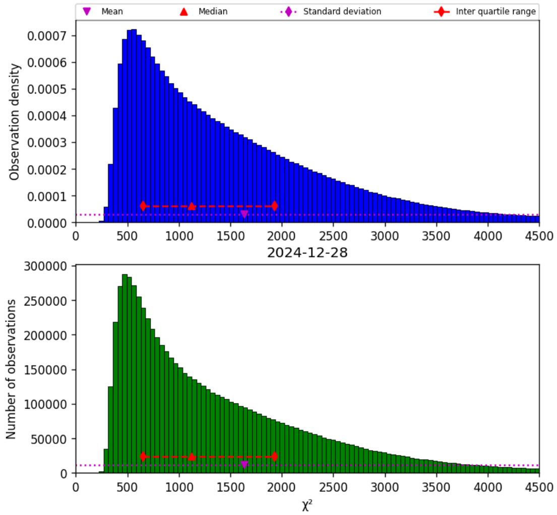
Figure 22: Histogram of “ \chi^2 ” for 2024-12-27 to 2024-12-29
