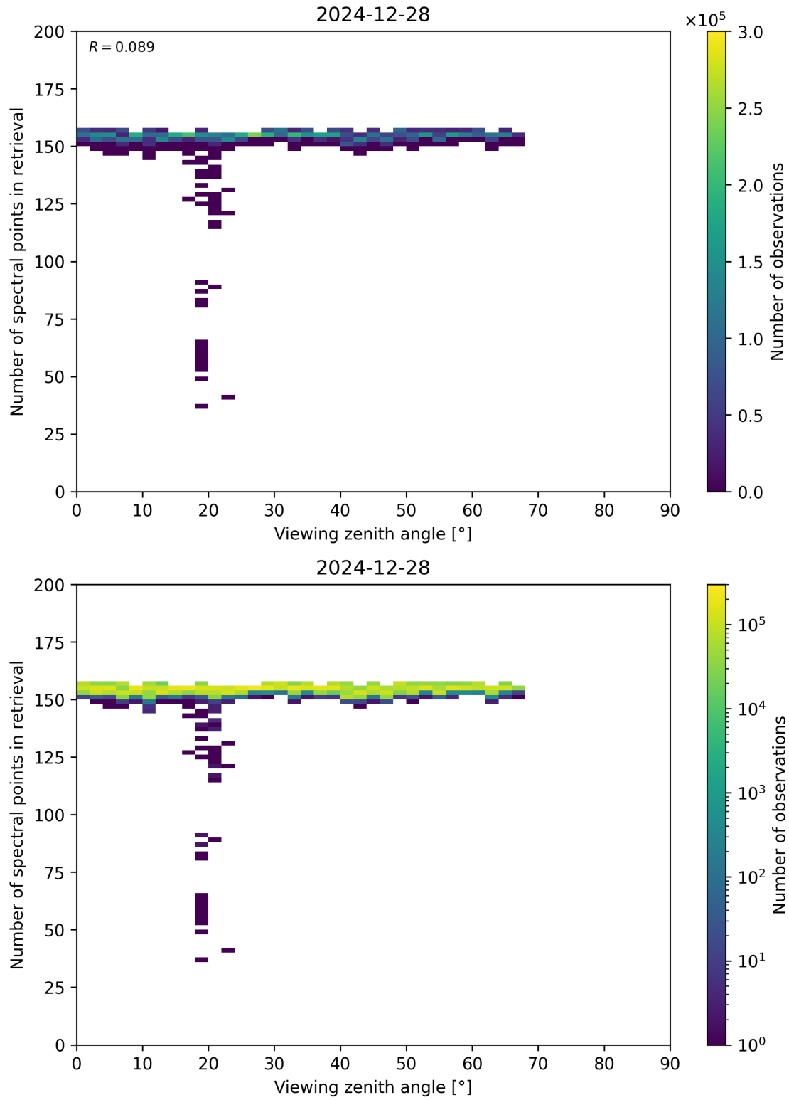
Figure 76: Scatter density plot of “Viewing zenith angle” against “Number of spectral points in retrieval” for 2024-12-27 to 2024-12-29.
