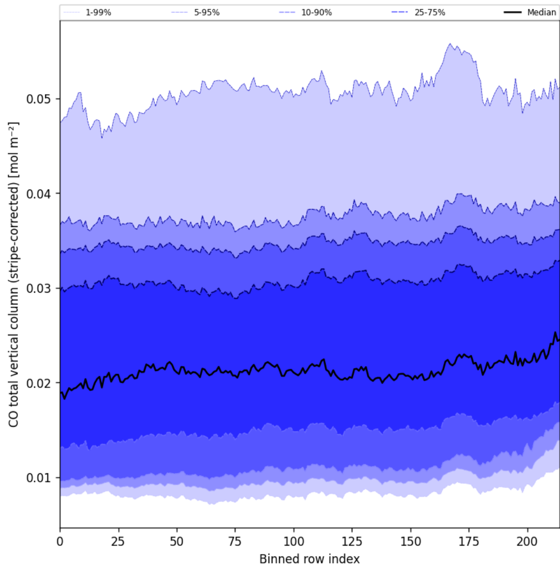
Figure 27: Along track statistics of “CO total vertical column (stripe-corrected)” for 2024-12-27 to 2024-12-29
