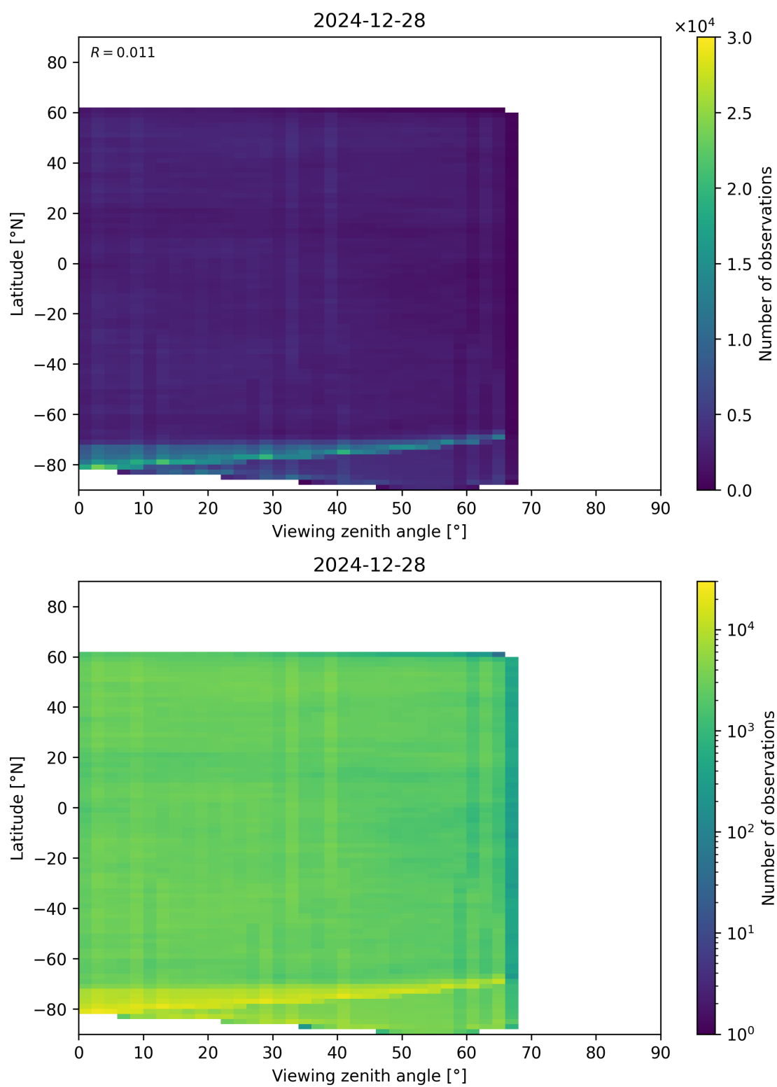
Figure 74: Scatter density plot of “Viewing zenith angle” against “Latitude” for 2024-12-27 to 2024-12-29.
