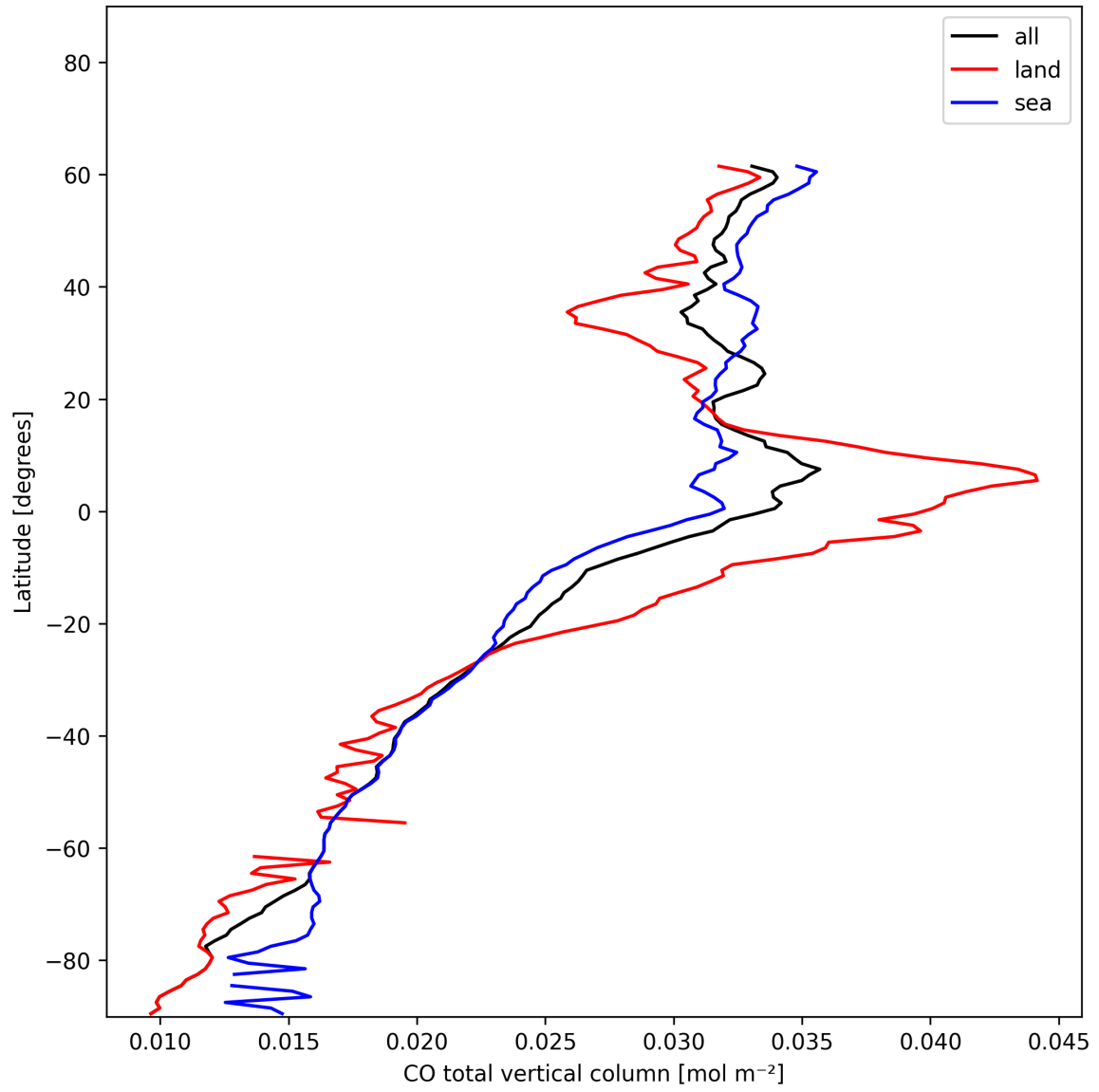
Figure 10: Zonal average of “CO total vertical column” for 2024-12-27 to 2024-12-29.
