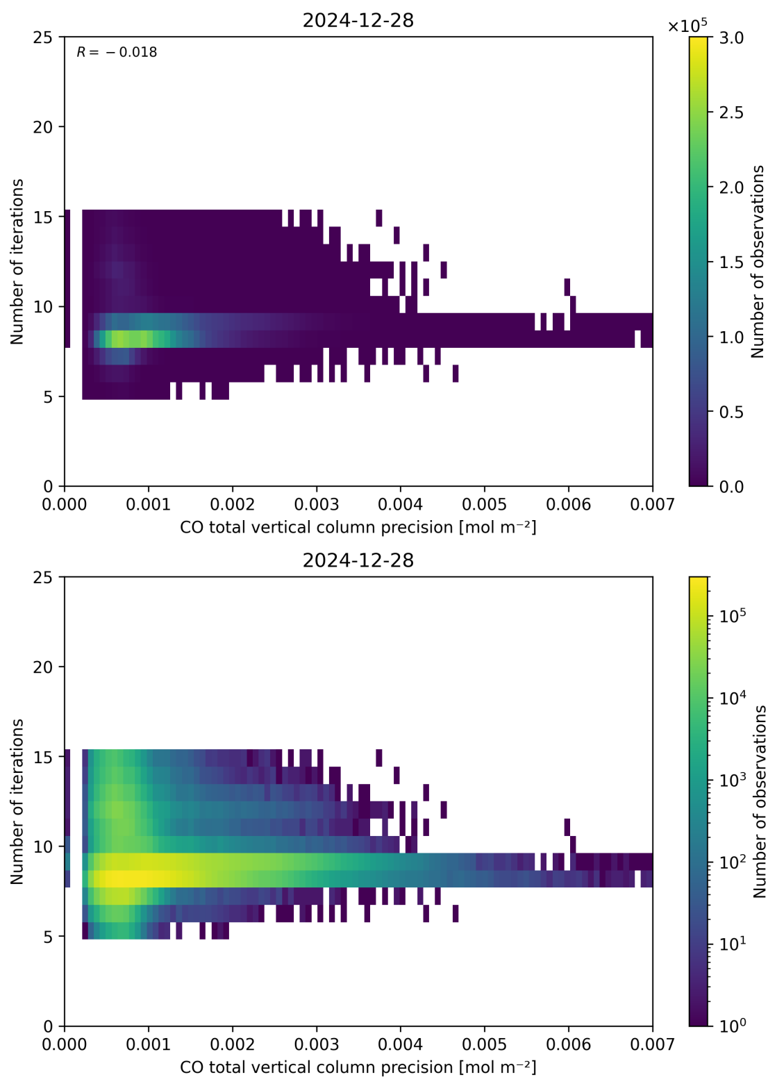
Figure 46: Scatter density plot of “CO total vertical column precision” against “Number of iterations” for 2024-12-27 to 2024-12-29.
