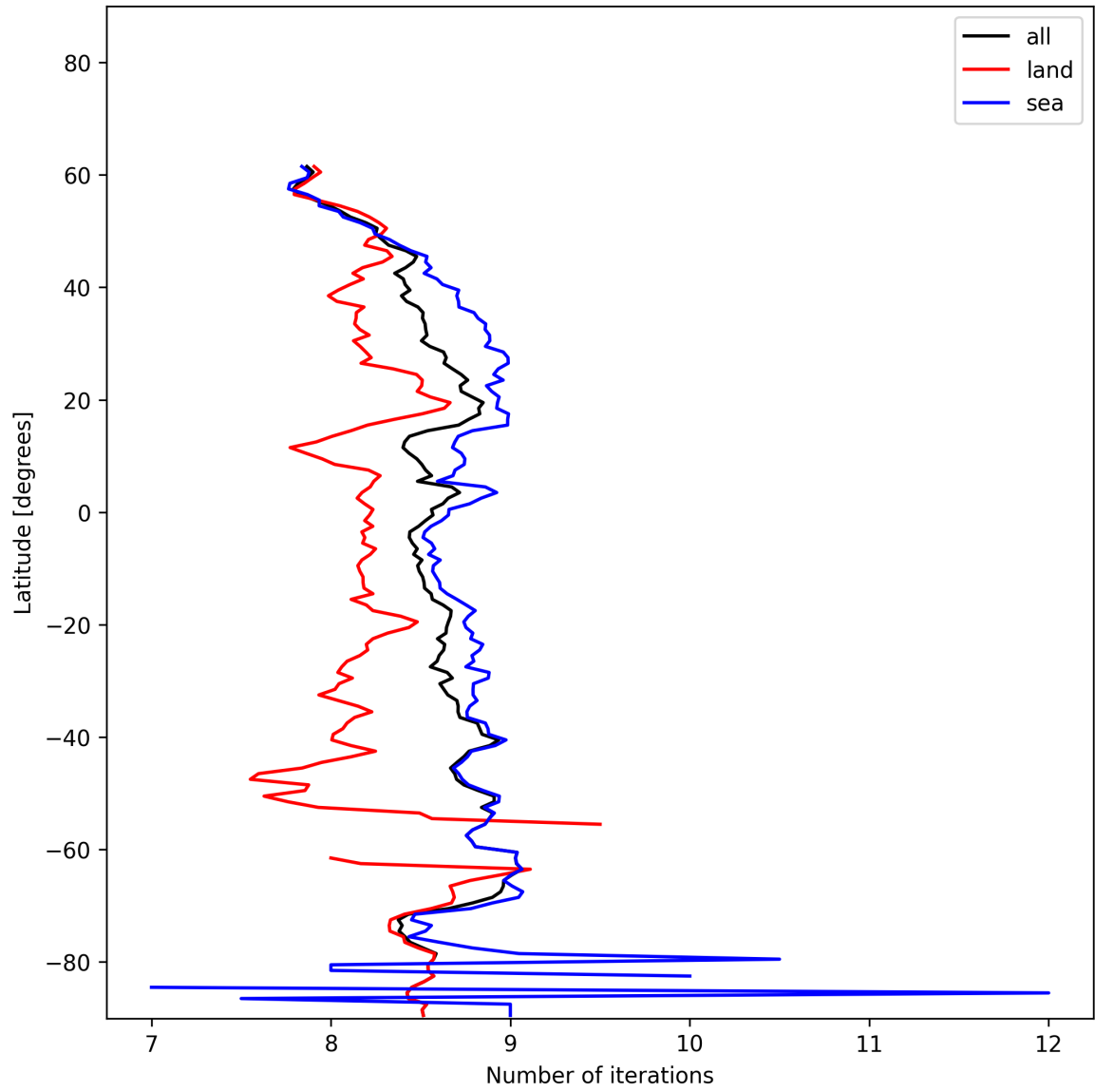
Figure 16: Zonal average of “Number of iterations” for 2024-12-27 to 2024-12-29.
