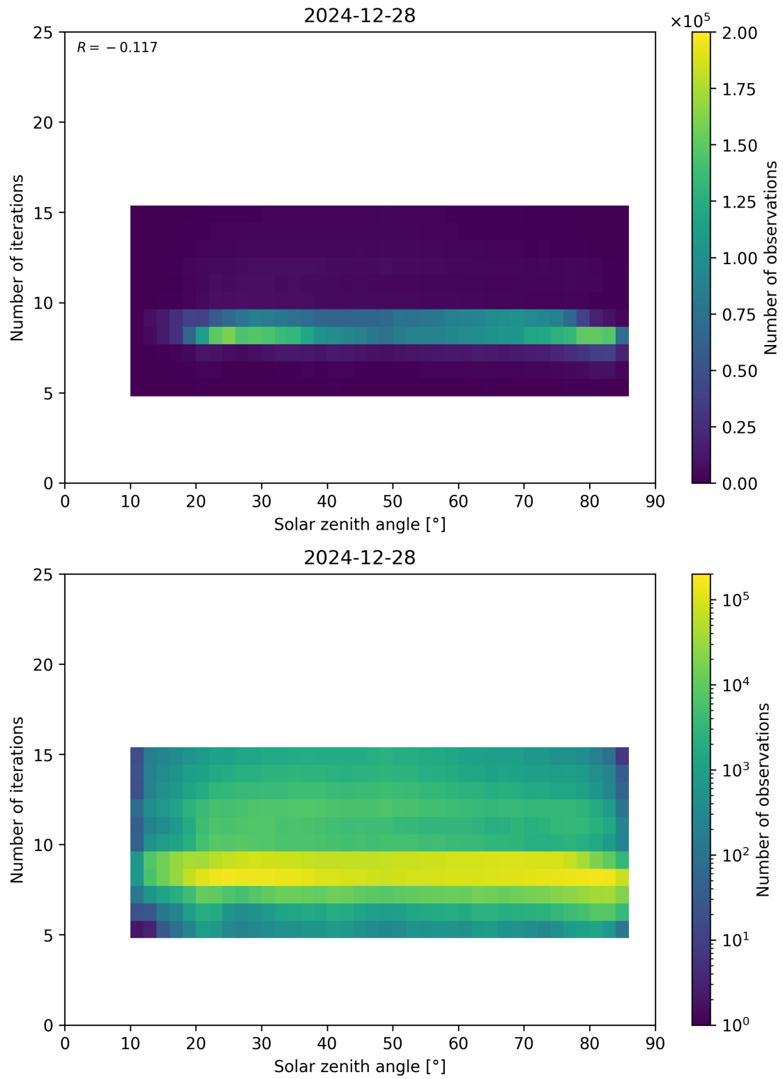
Figure 67: Scatter density plot of “Solar zenith angle” against “Number of iterations” for 2024-12-27 to 2024-12-29.
