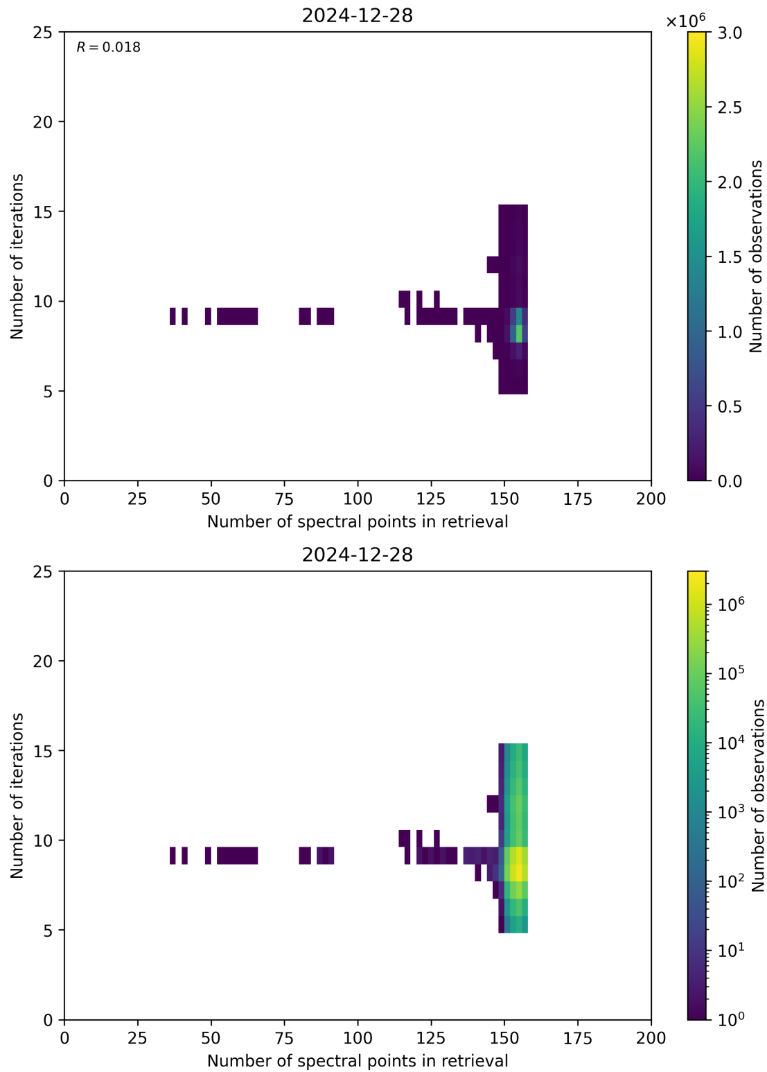
Figure 60: Scatter density plot of “Number of spectral points in retrieval” against “Number of iterations” for 2024-12-27 to 2024-12-29.
