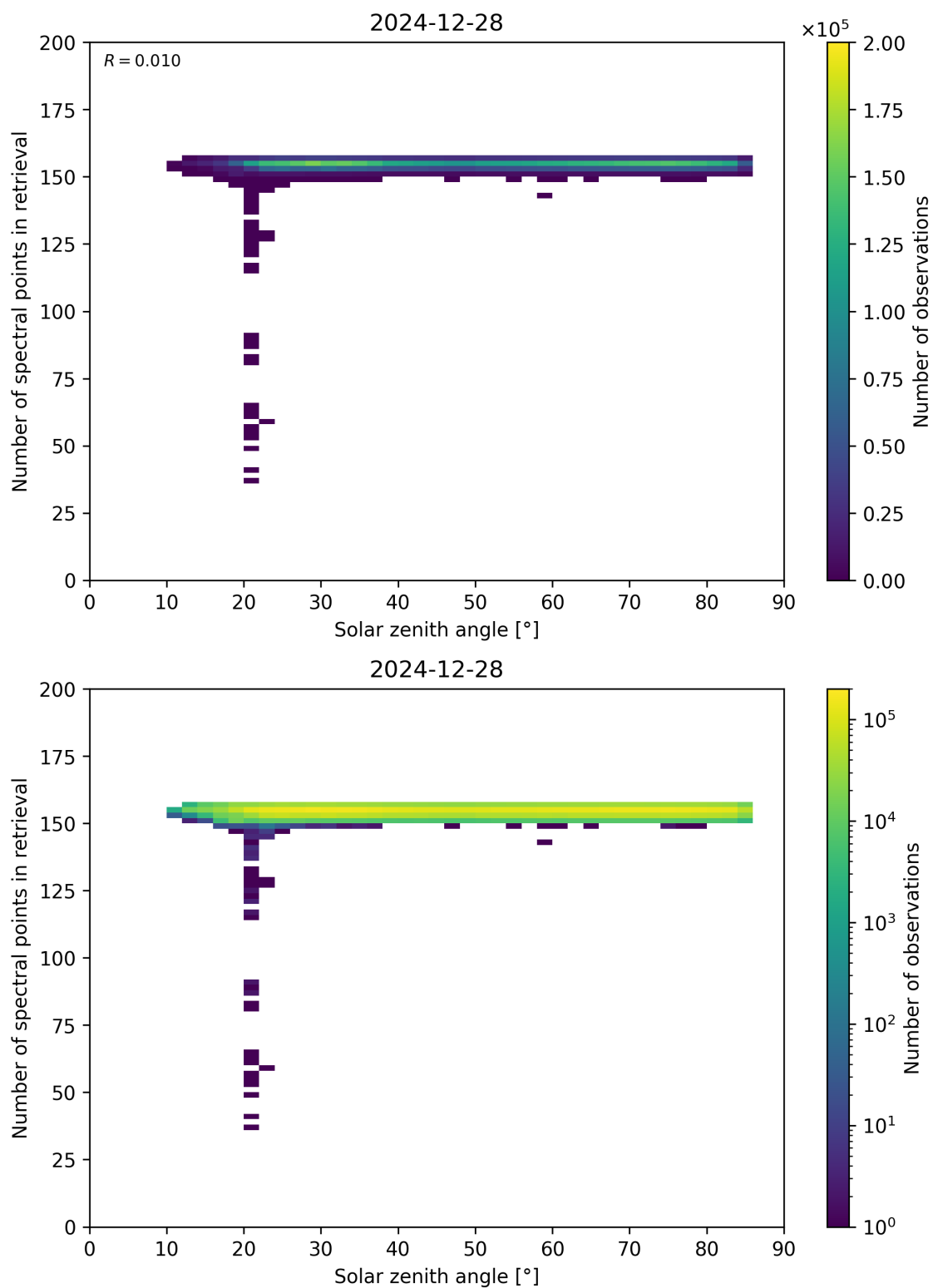
Figure 68: Scatter density plot of “Solar zenith angle” against “Number of spectral points in retrieval” for 2024-12-27 to 2024-12-29.
