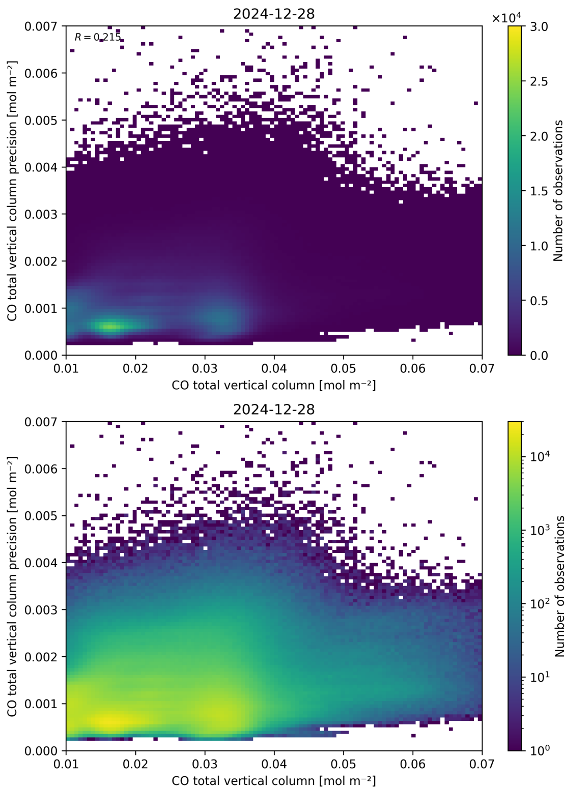
Figure 34: Scatter density plot of “CO total vertical column” against “CO total vertical column precision” for 2024-12-27 to 2024-12-29.
