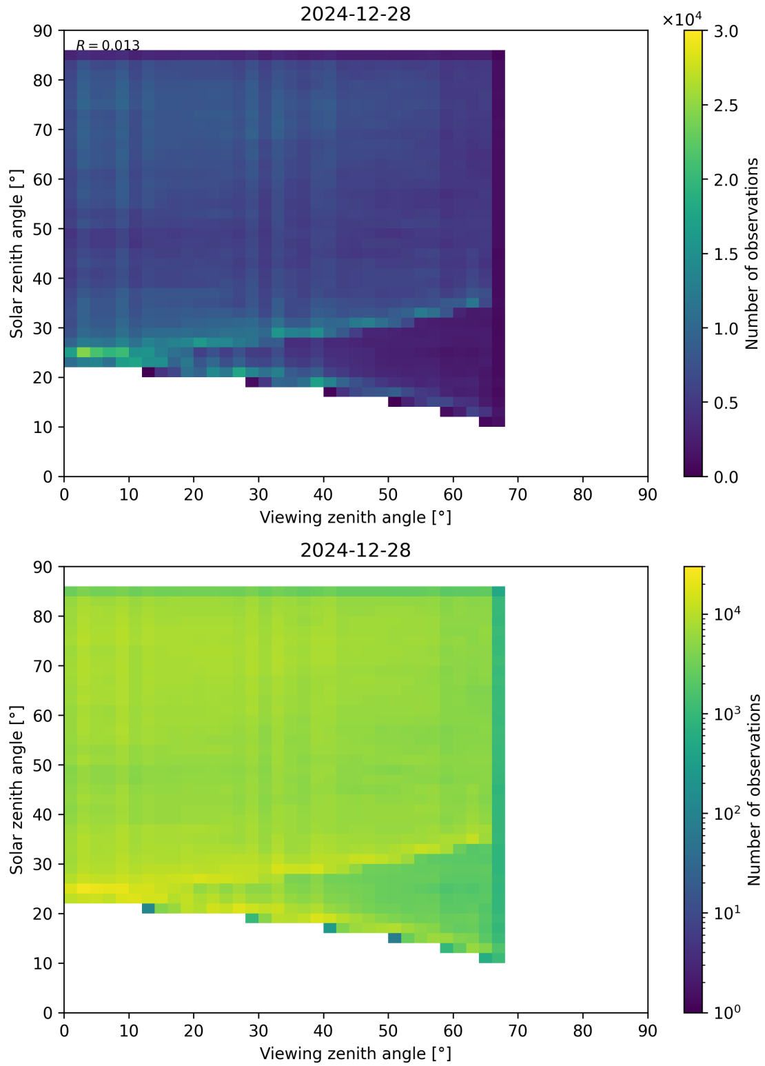
Figure 77: Scatter density plot of “Viewing zenith angle” against “Solar zenith angle” for 2024-12-27 to 2024-12-29.
