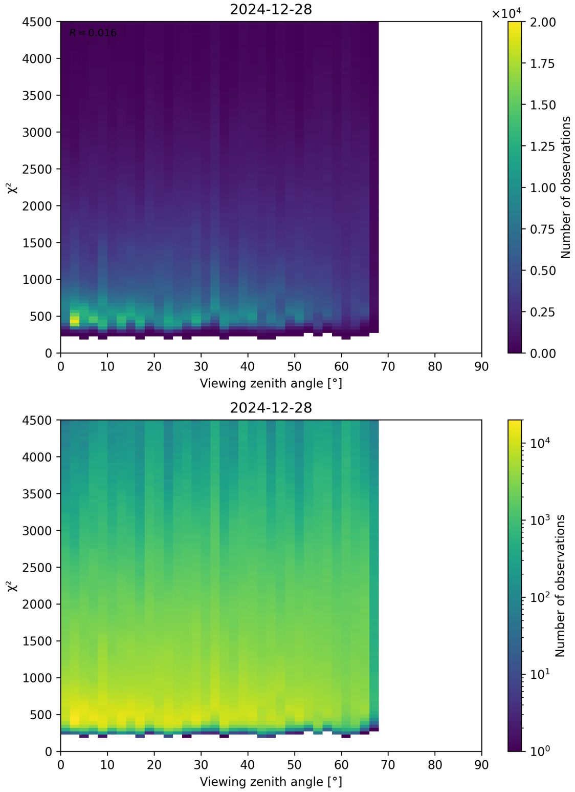
Figure 72: Scatter density plot of “Viewing zenith angle” against “ \chi^2 ” for 2024-12-27 to 2024-12-29.
