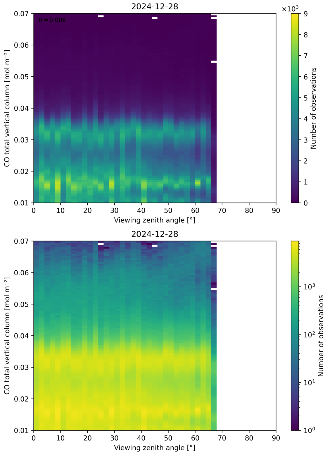
Figure 69: Scatter density plot of “Viewing zenith angle” against “CO total vertical column” for 2024-12-27 to 2024-12-29.
