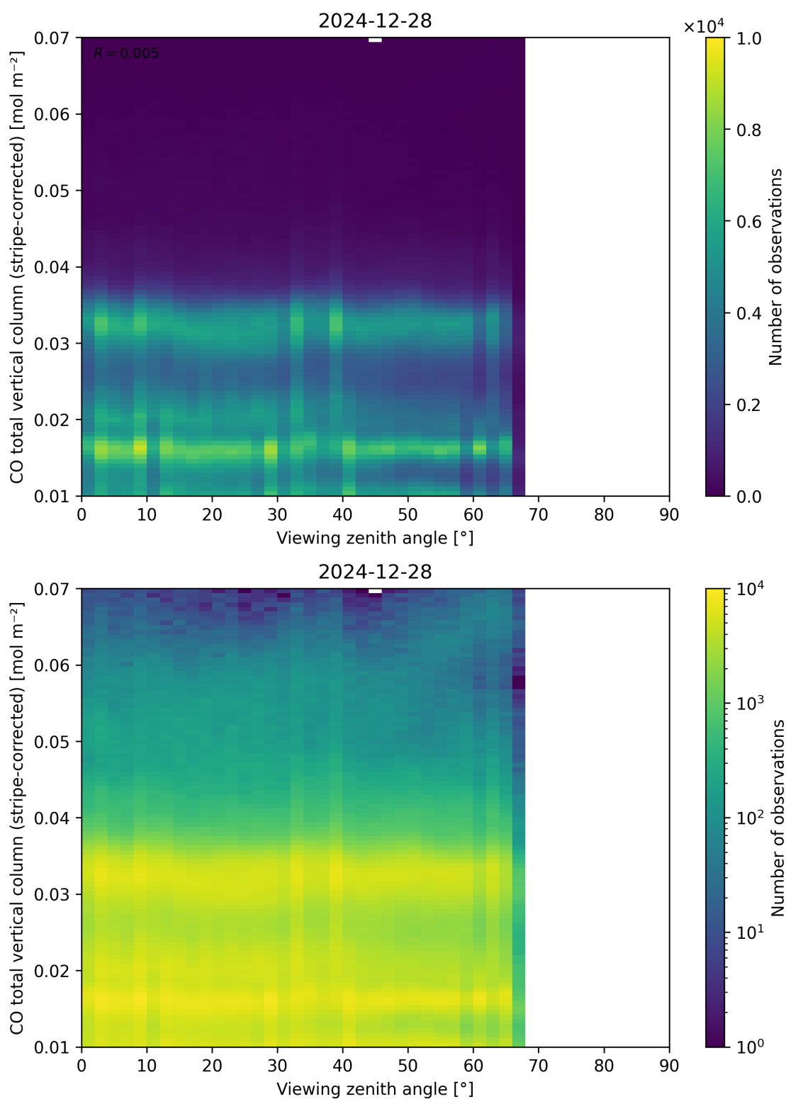
Figure 70: Scatter density plot of “Viewing zenith angle” against “CO total vertical column (stripe-corrected)” for 2024-12-27 to 2024-12-29.
