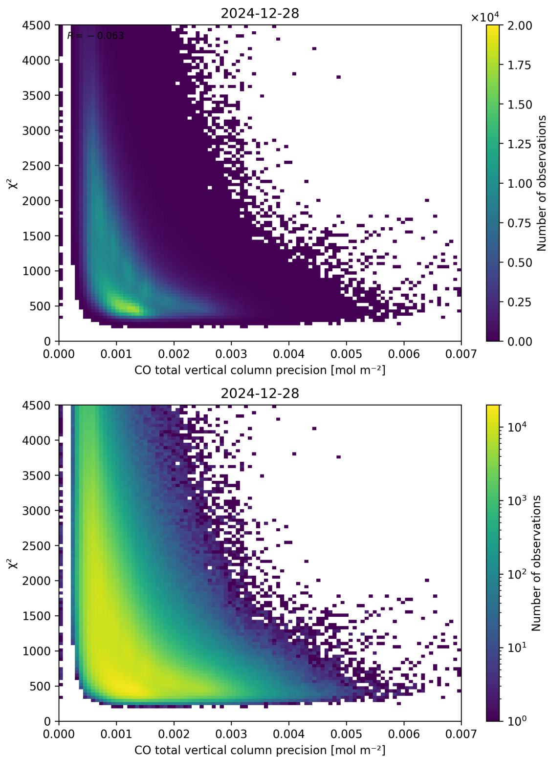
Figure 44: Scatter density plot of “CO total vertical column precision” against “ \chi^2 ” for 2024-12-27 to 2024-12-29.
