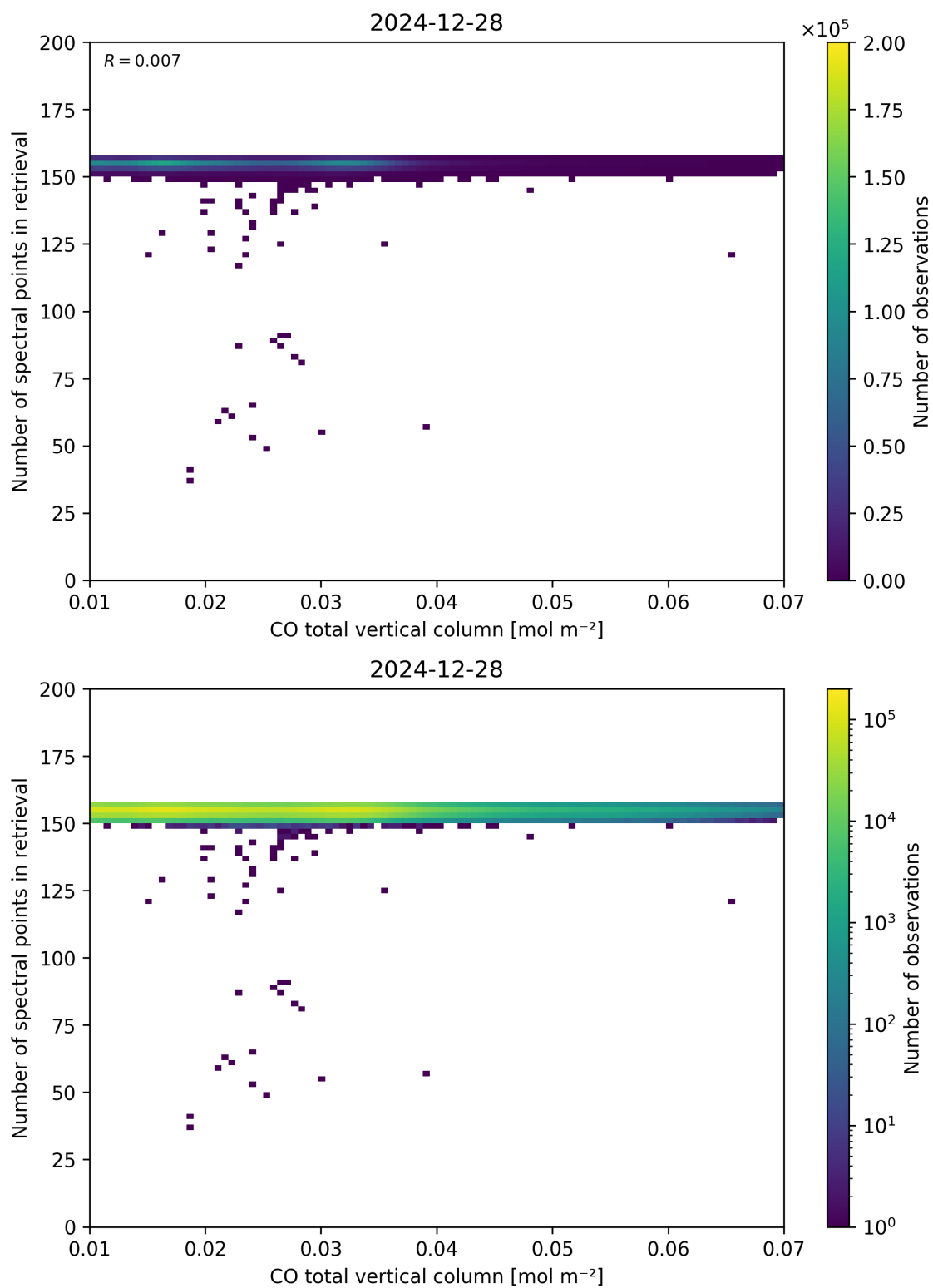
Figure 43: Scatter density plot of “CO total vertical column” against “Number of spectral points in retrieval” for 2024-12-27 to 2024-12-29.
