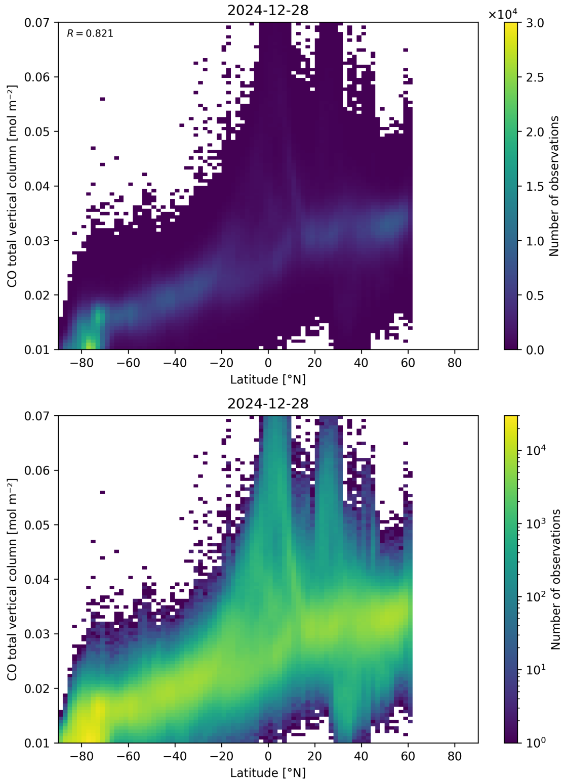
Figure 51: Scatter density plot of “Latitude” against “CO total vertical column” for 2024-12-27 to 2024-12-29.
