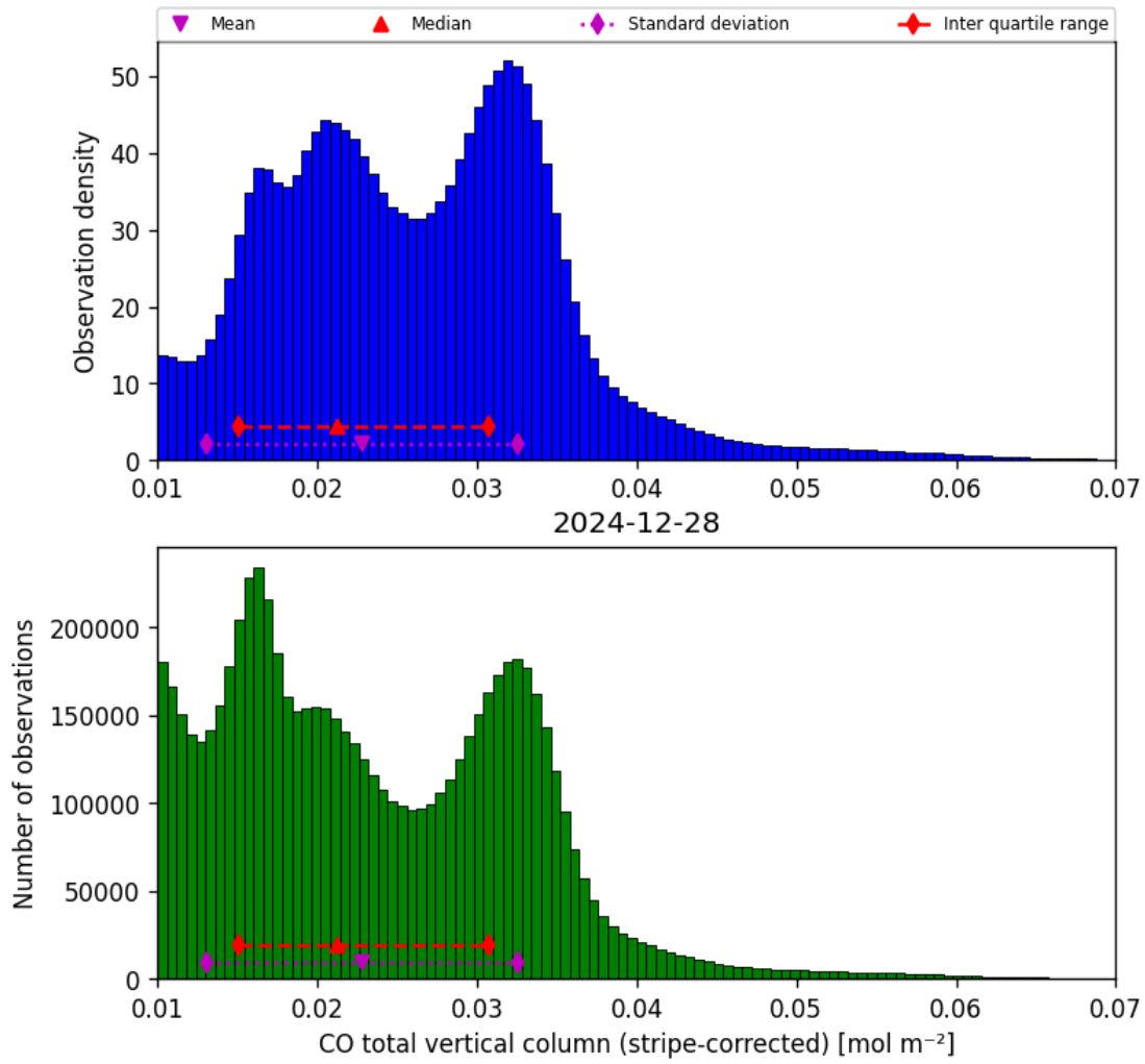
Figure 19: Histogram of “CO total vertical column (stripe-corrected)” for 2024-12-27 to 2024-12-29
