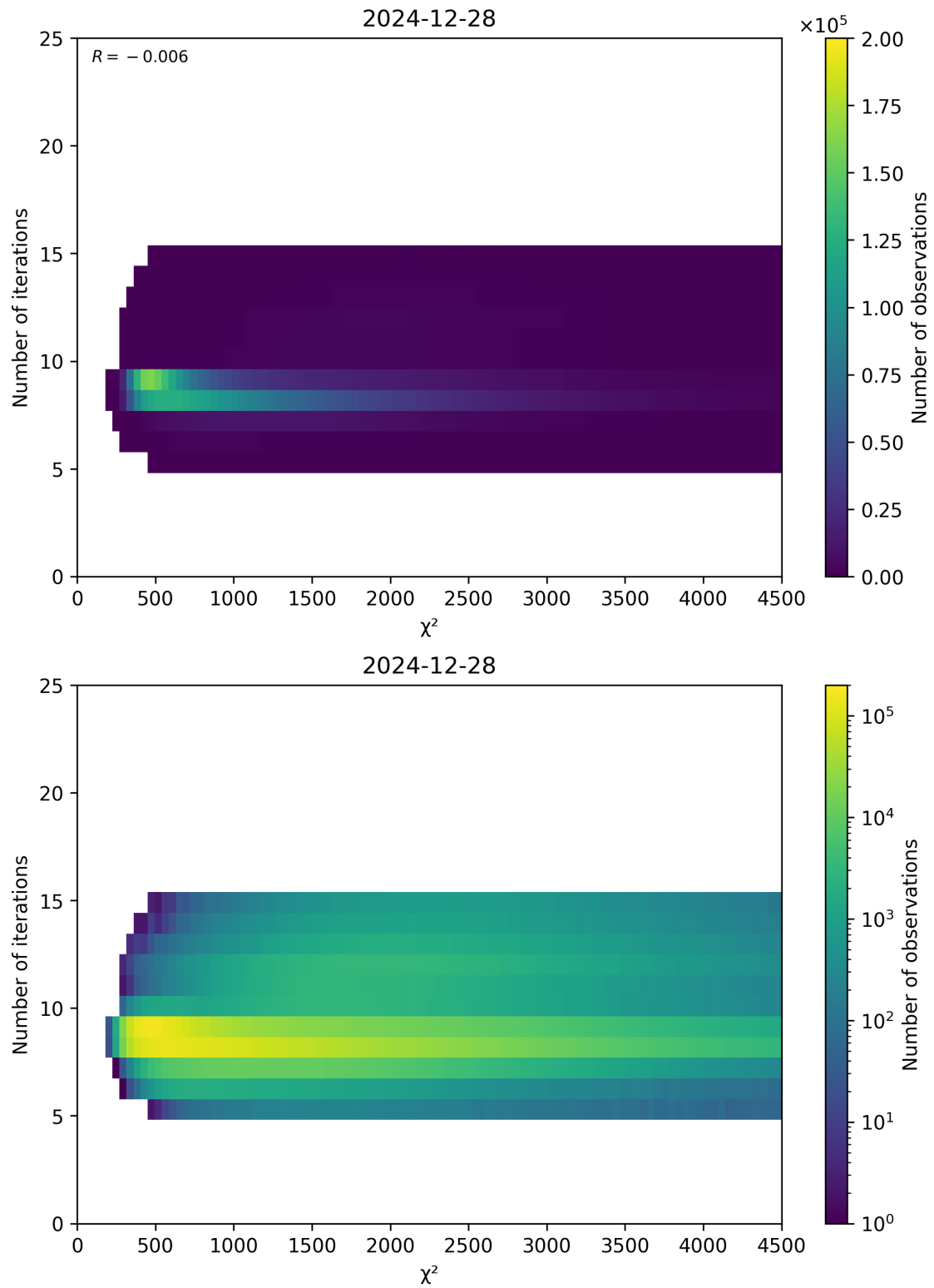
Figure 49: Scatter density plot of “ \chi^2 ” against “Number of iterations” for 2024-12-27 to 2024-12-29.
