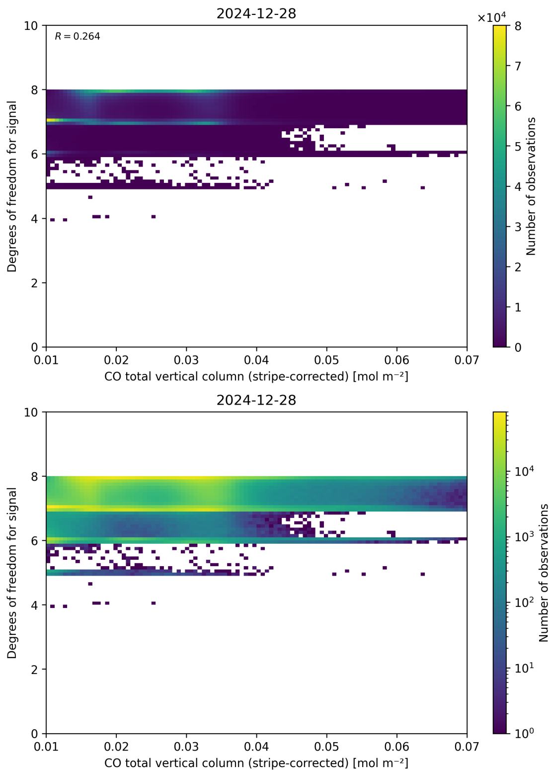
Figure 38: Scatter density plot of “CO total vertical column (stripe-corrected)” against “Degrees of freedom for signal” for 2024-12-27 to 2024-12-29.
