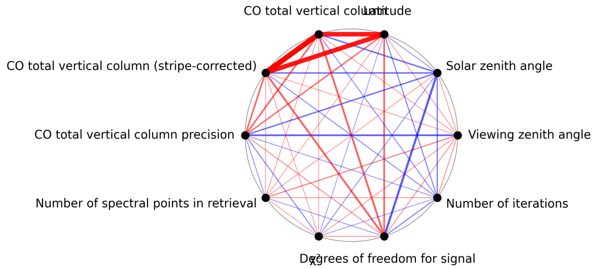
Figure 1: Map of correlation graph for 2024-12-27 to 2024-12-29.
