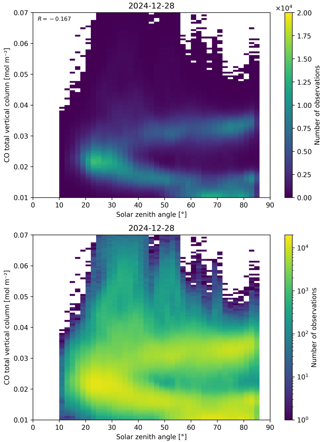
Figure 61: Scatter density plot of “Solar zenith angle” against “CO total vertical column” for 2024-12-27 to 2024-12-29.
