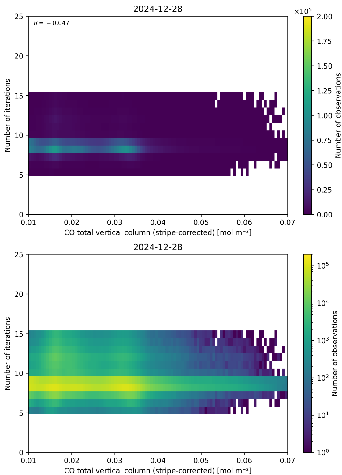
Figure 39: Scatter density plot of “CO total vertical column (stripe-corrected)” against “Number of iterations” for 2024-12-27 to 2024-12-29.
