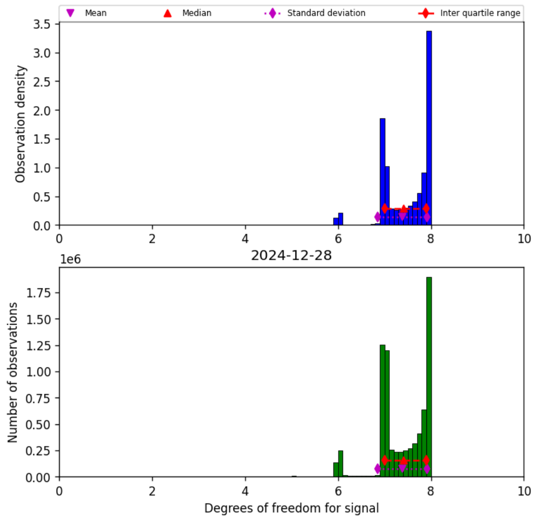
Figure 23: Histogram of “Degrees of freedom for signal” for 2024-12-27 to 2024-12-29
