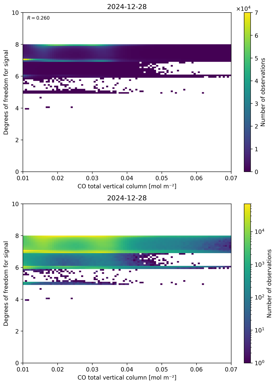
Figure 41: Scatter density plot of “CO total vertical column” against “Degrees of freedom for signal” for 2024-12-27 to 2024-12-29.
