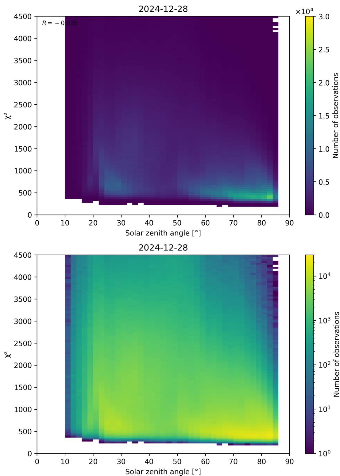
Figure 64: Scatter density plot of “Solar zenith angle” against “ \chi^2 ” for 2024-12-27 to 2024-12-29.
