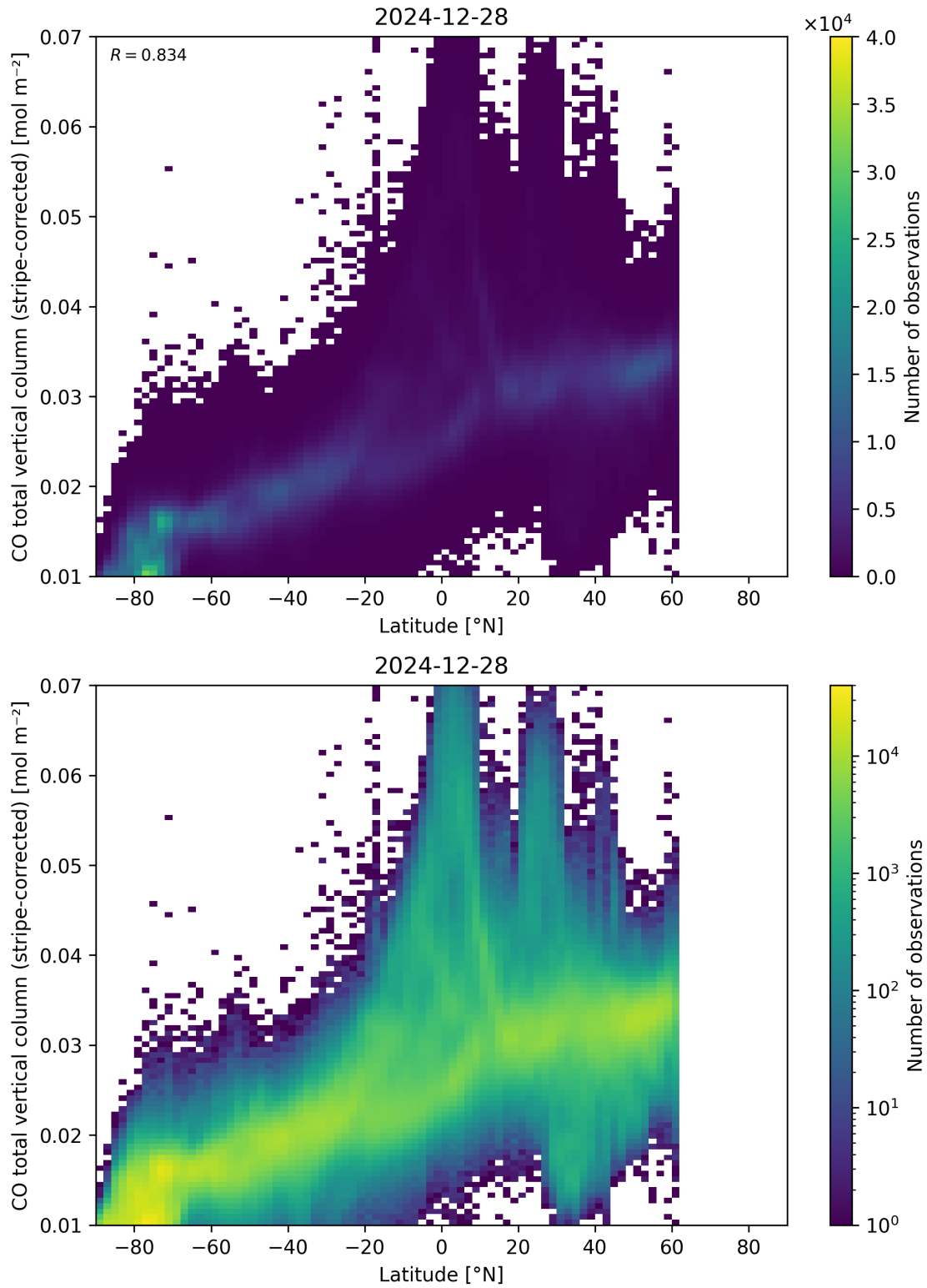
Figure 52: Scatter density plot of “Latitude” against “CO total vertical column (stripe-corrected)” for 2024-12-27 to 2024-12-29.
