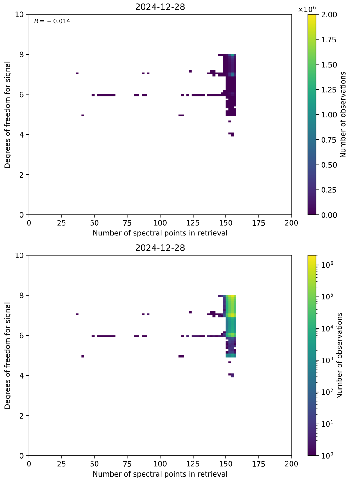
Figure 59: Scatter density plot of “Number of spectral points in retrieval” against “Degrees of freedom for signal” for 2024-12-27 to 2024-12-29.
