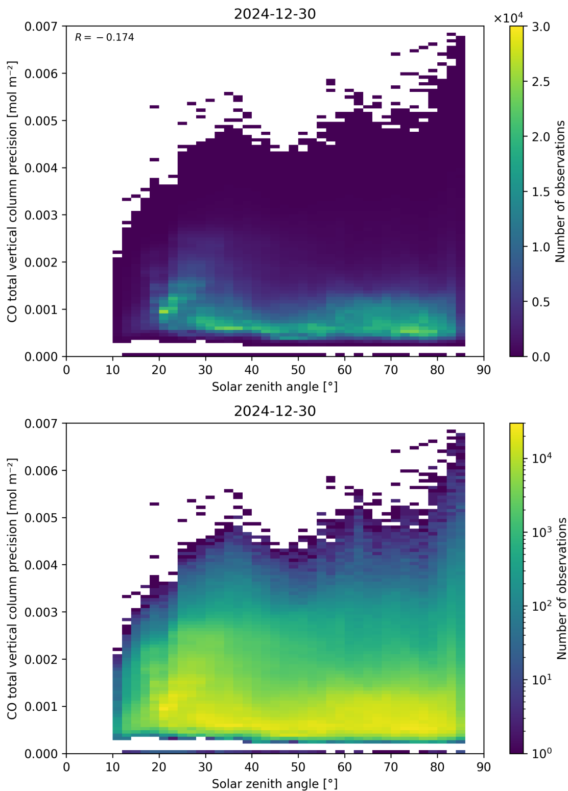
Figure 63: Scatter density plot of “Solar zenith angle” against “CO total vertical column precision” for 2024-12-29 to 2024-12-31.
