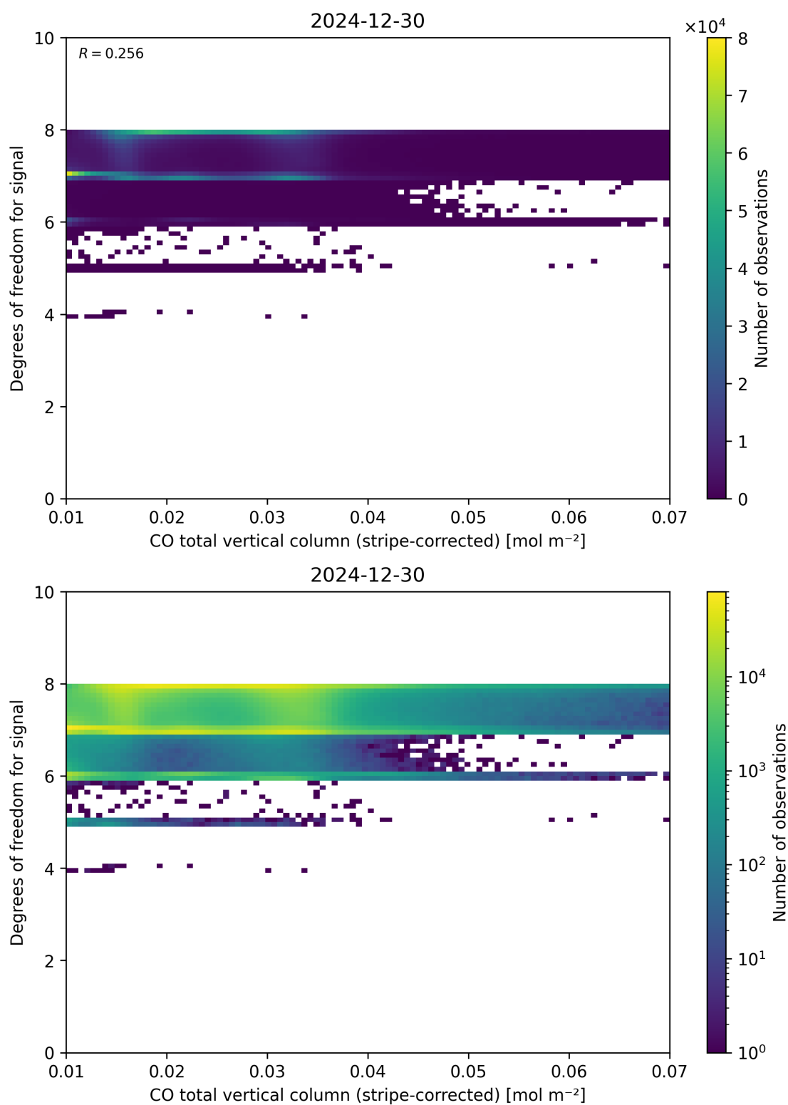
Figure 38: Scatter density plot of “CO total vertical column (stripe-corrected)” against “Degrees of freedom for signal” for 2024-12-29 to 2024-12-31.
