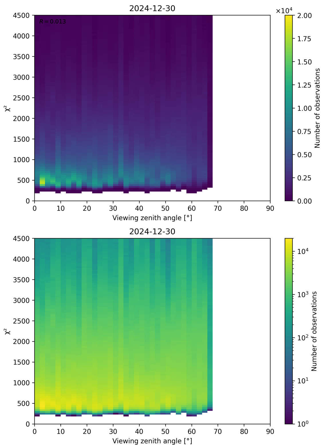
Figure 72: Scatter density plot of “Viewing zenith angle” against “ \chi^2 ” for 2024-12-29 to 2024-12-31.
