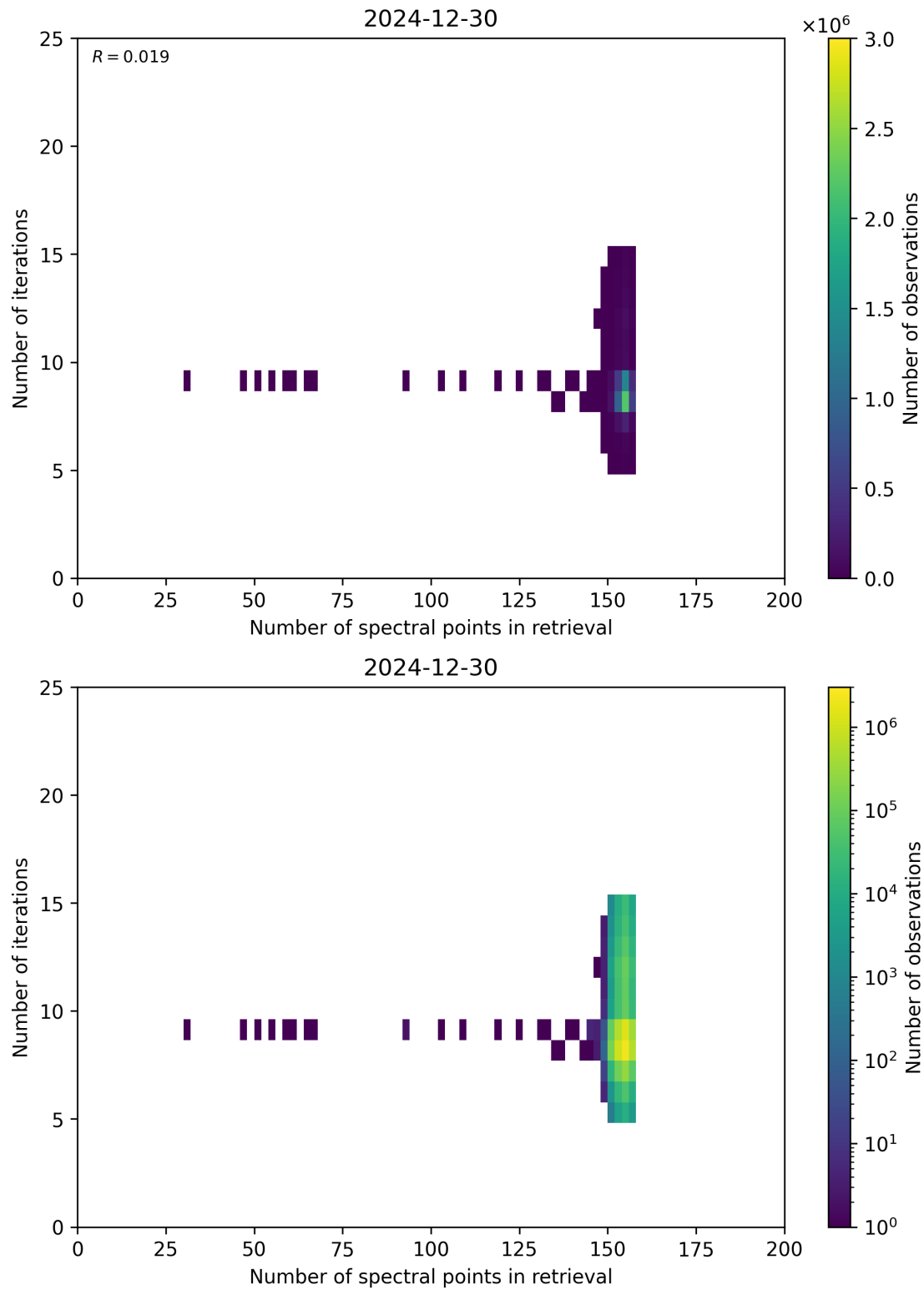
Figure 60: Scatter density plot of “Number of spectral points in retrieval” against “Number of iterations” for 2024-12-29 to 2024-12-31.
