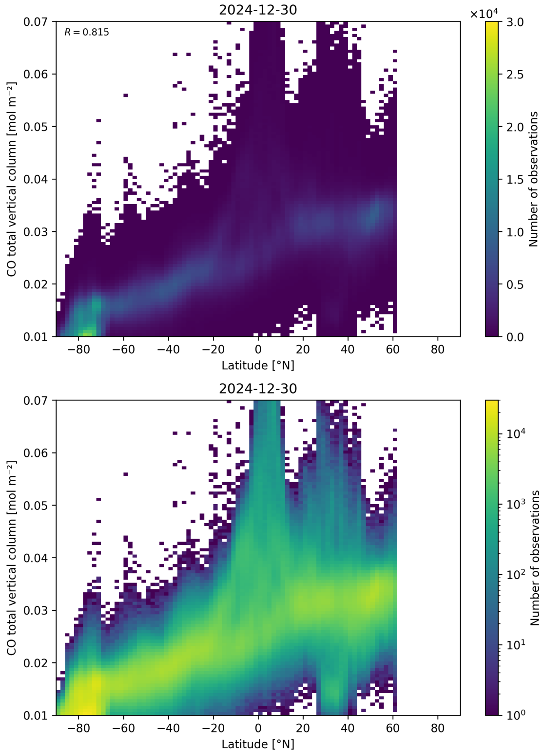
Figure 51: Scatter density plot of “Latitude” against “CO total vertical column” for 2024-12-29 to 2024-12-31.
