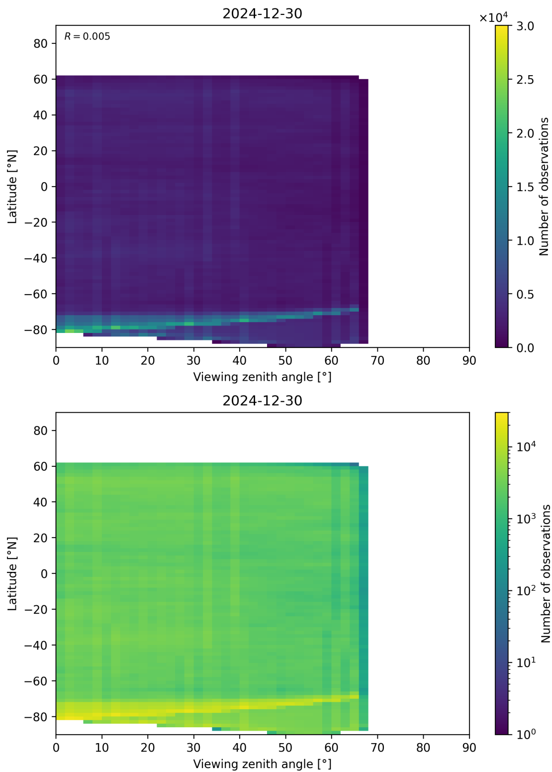
Figure 74: Scatter density plot of “Viewing zenith angle” against “Latitude” for 2024-12-29 to 2024-12-31.
