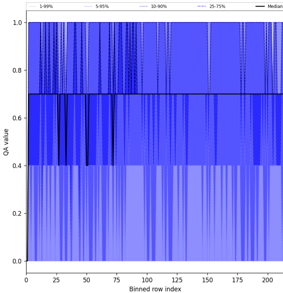
Figure 25: Along track statistics of “QA value” for 2024-12-29 to 2024-12-31
