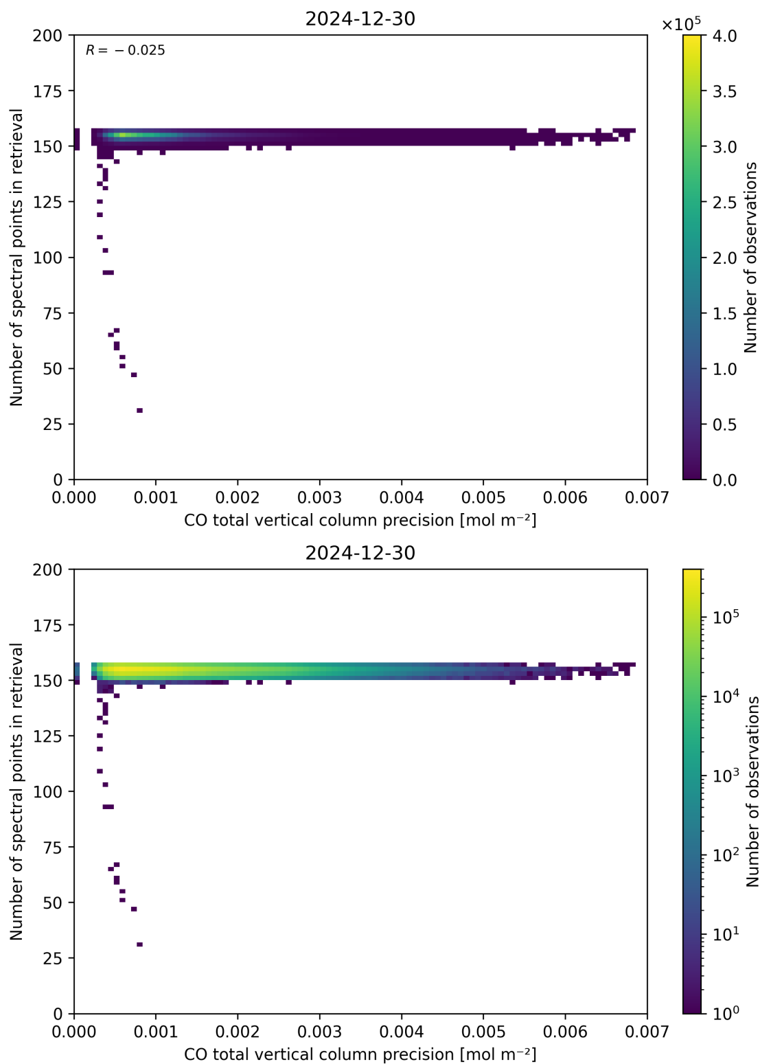
Figure 47: Scatter density plot of “CO total vertical column precision” against “Number of spectral points in retrieval” for 2024-12-29 to 2024-12-31.
