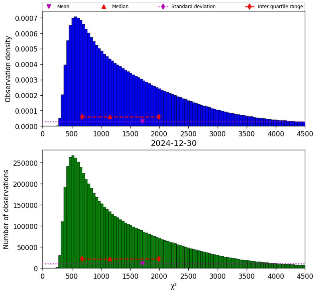
Figure 22: Histogram of “ \chi^2 ” for 2024-12-29 to 2024-12-31
