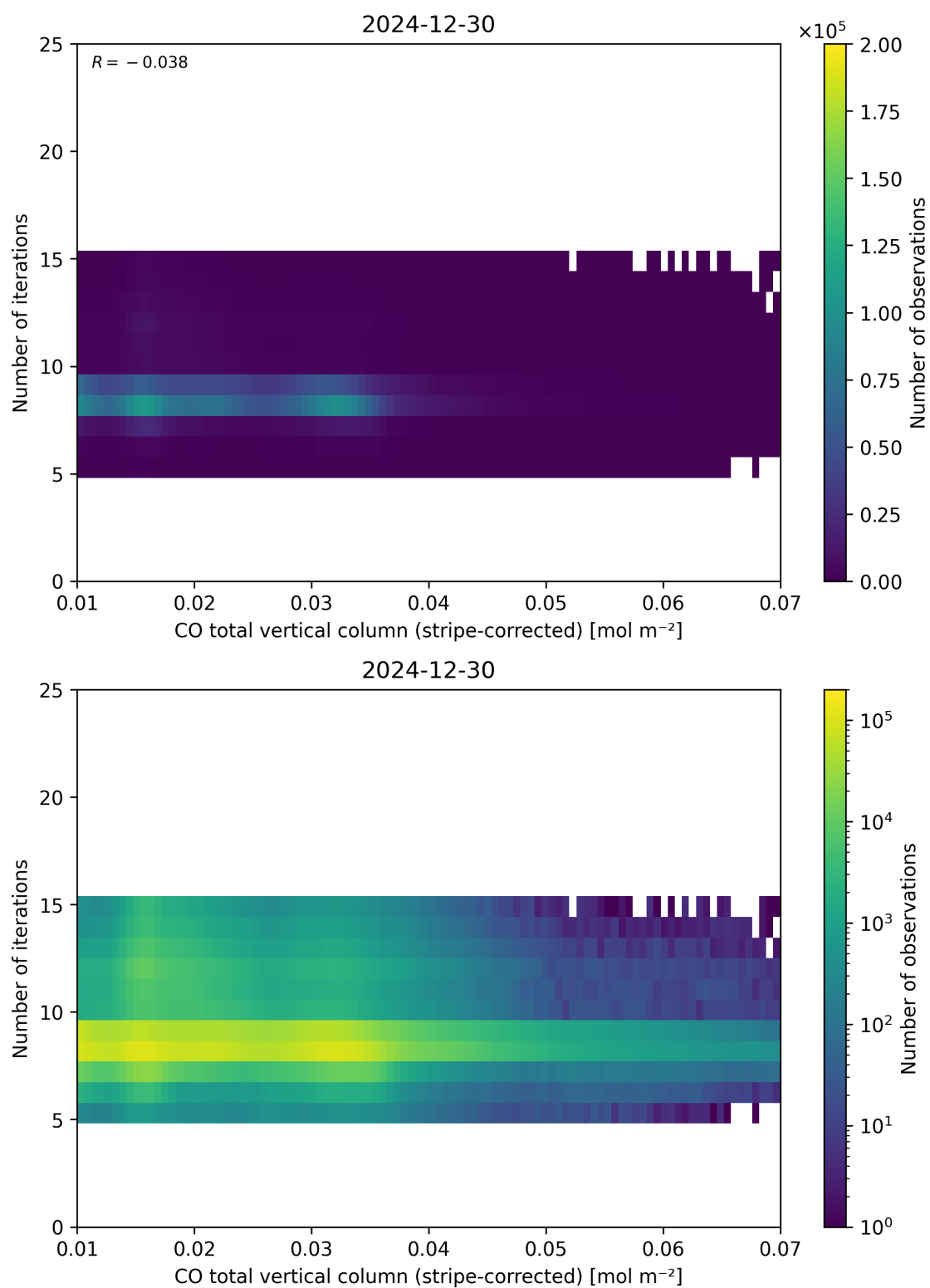
Figure 39: Scatter density plot of “CO total vertical column (stripe-corrected)” against “Number of iterations” for 2024-12-29 to 2024-12-31.
