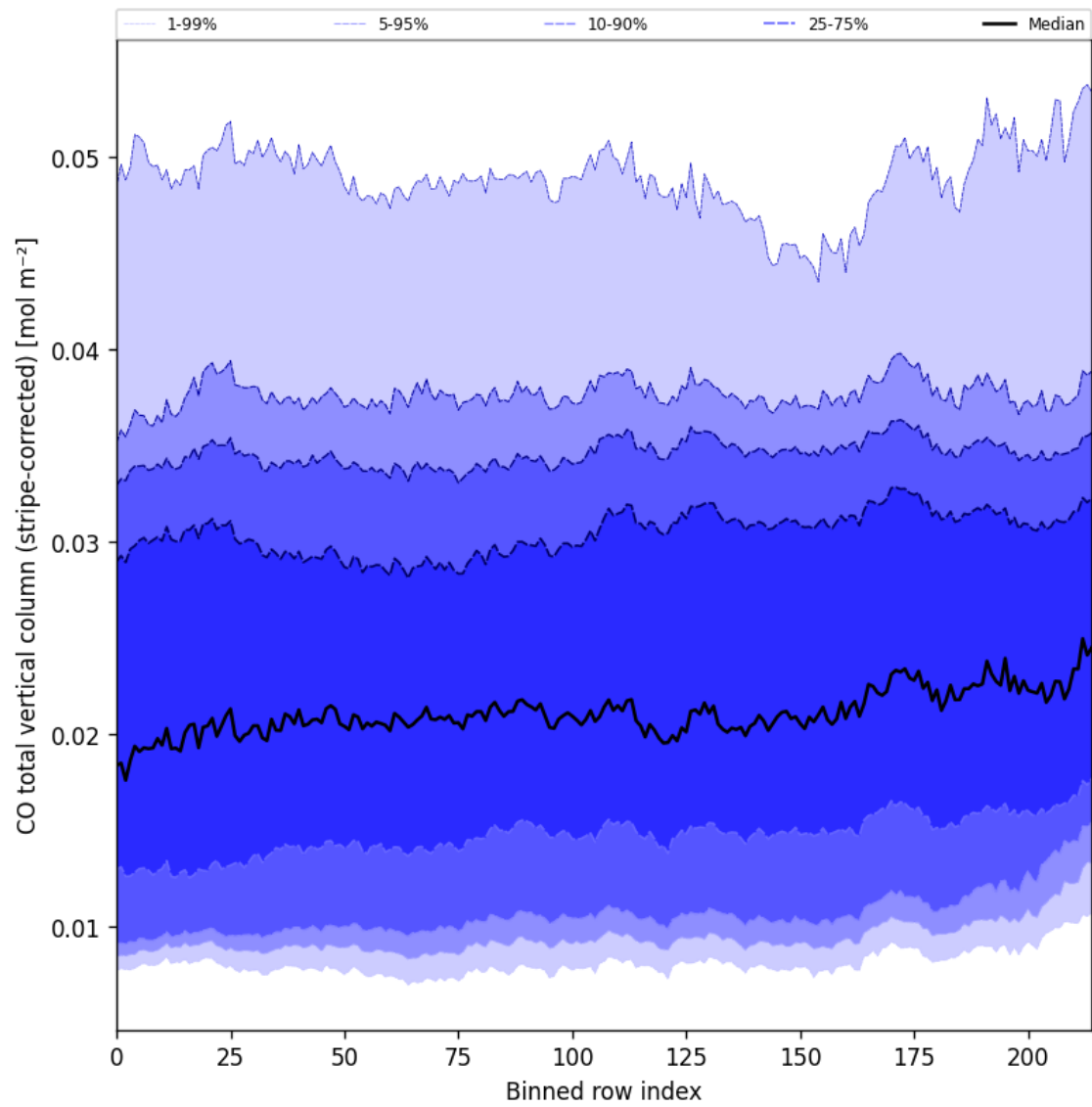
Figure 27: Along track statistics of “CO total vertical column (stripe-corrected)” for 2024-12-29 to 2024-12-31
