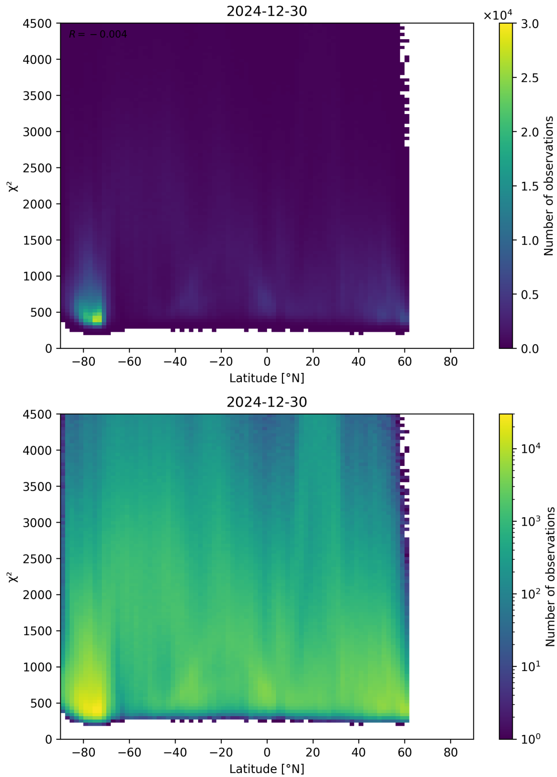
Figure 54: Scatter density plot of “Latitude” against “ \chi^2 ” for 2024-12-29 to 2024-12-31.
