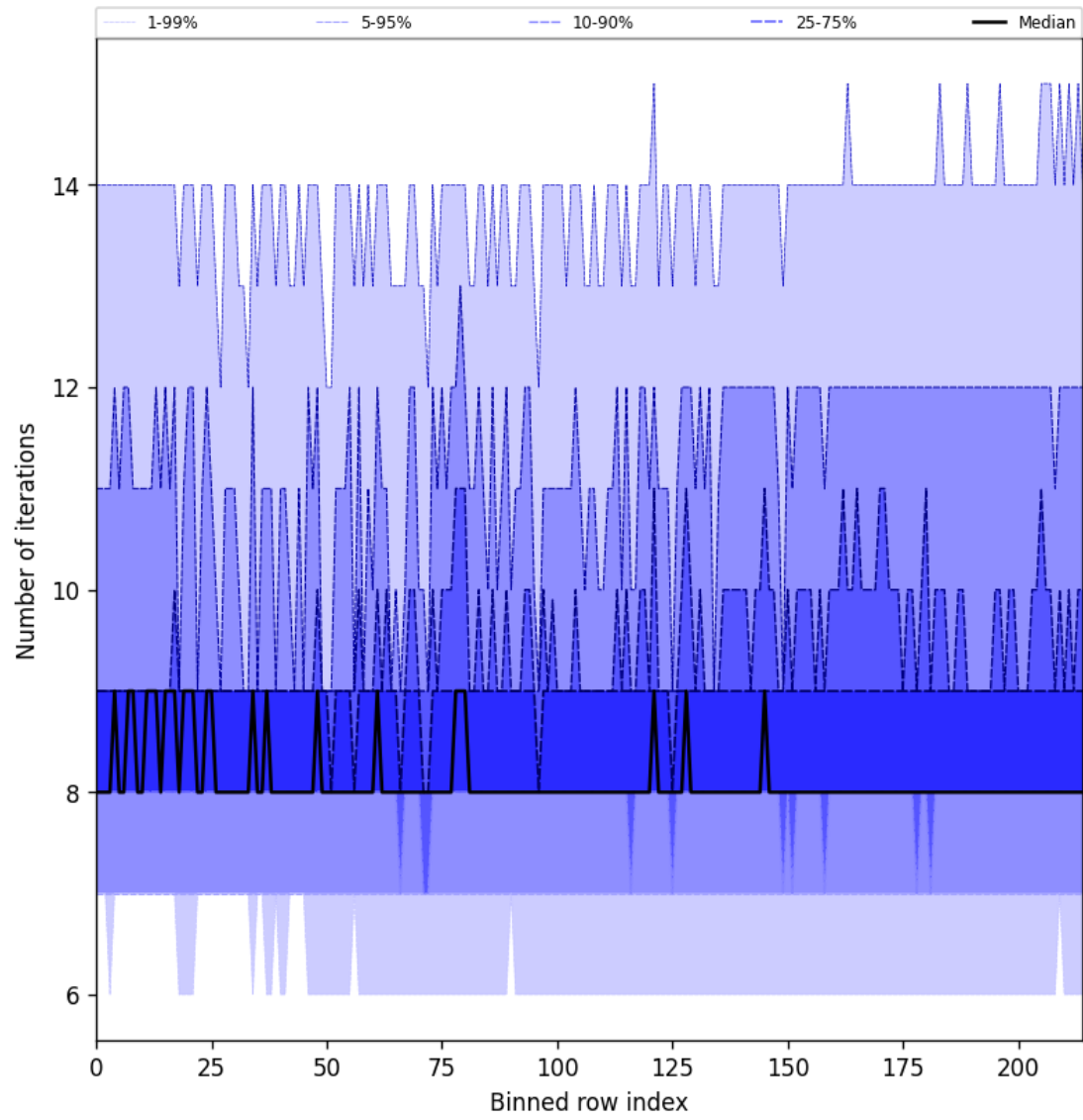
Figure 32: Along track statistics of “Number of iterations” for 2024-12-29 to 2024-12-31
