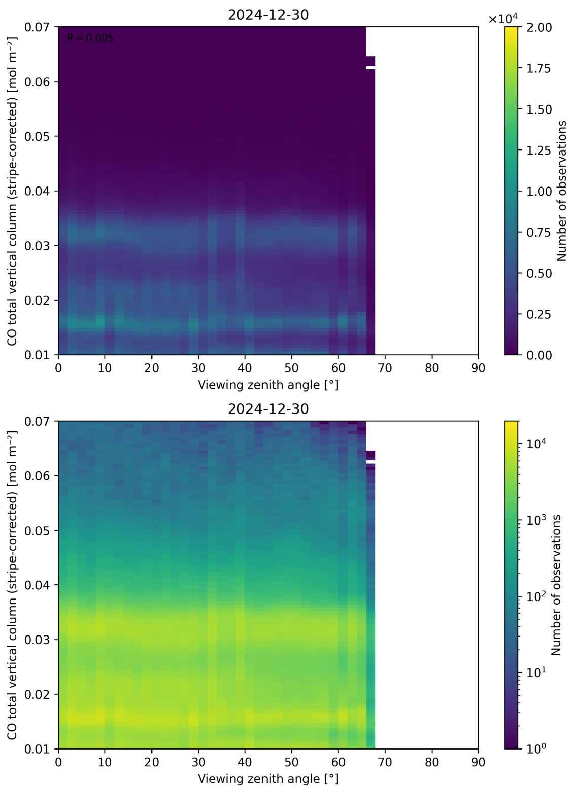
Figure 70: Scatter density plot of “Viewing zenith angle” against “CO total vertical column (stripe-corrected)” for 2024-12-29 to 2024-12-31.
