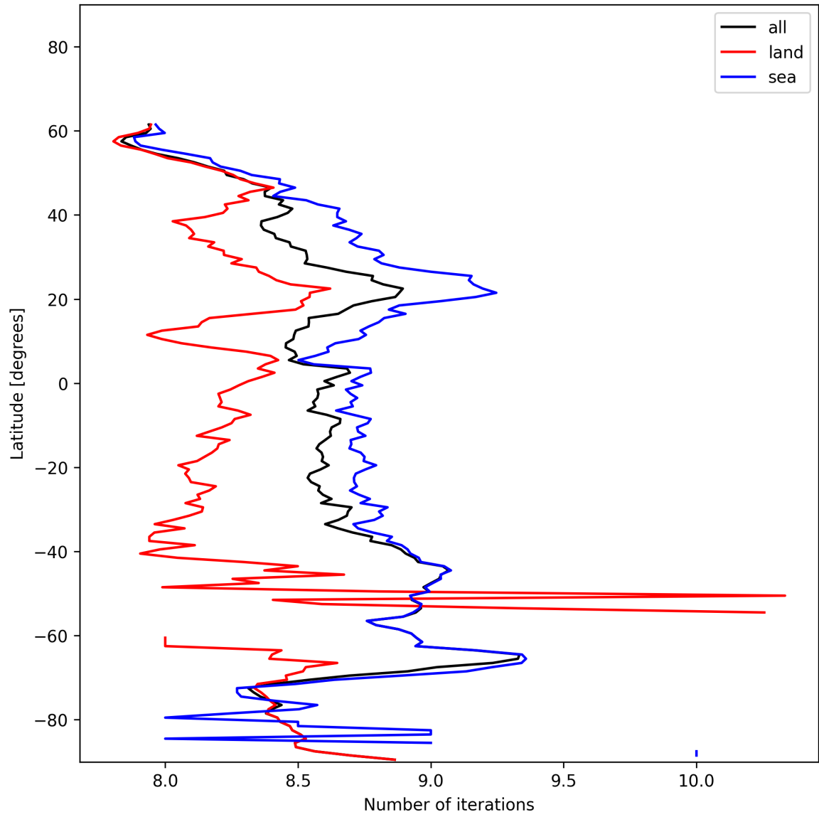
Figure 16: Zonal average of “Number of iterations” for 2024-12-29 to 2024-12-31.
