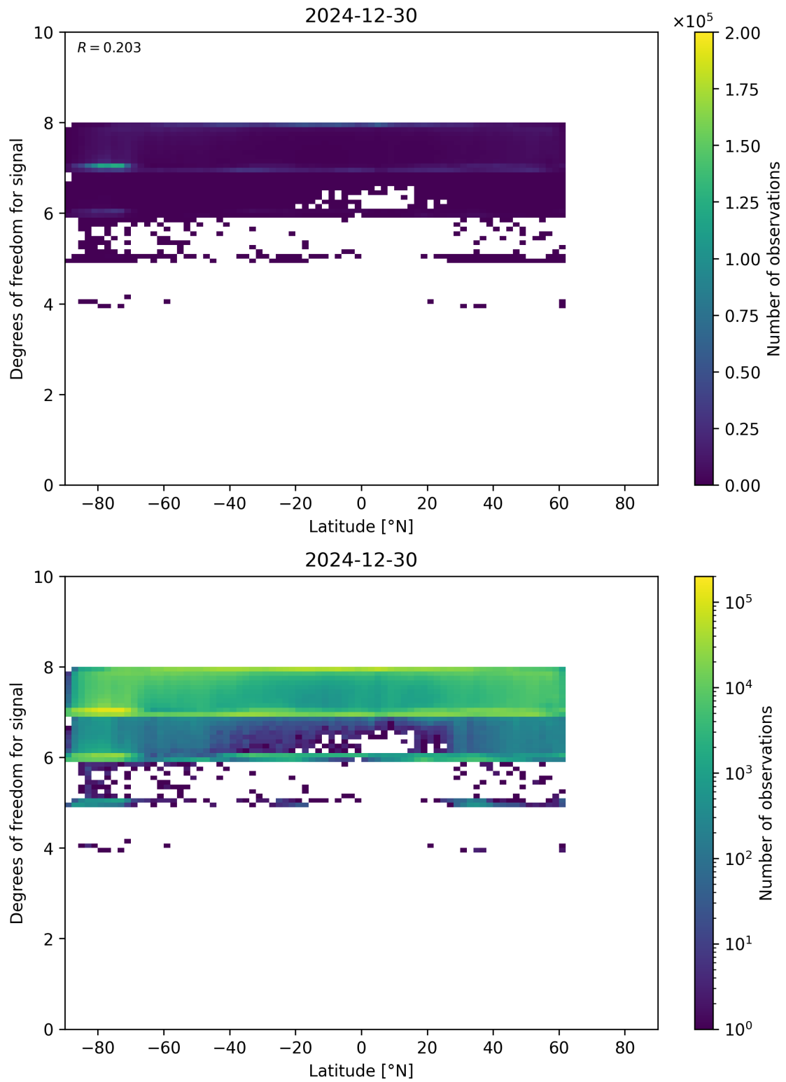
Figure 55: Scatter density plot of “Latitude” against “Degrees of freedom for signal” for 2024-12-29 to 2024-12-31.
