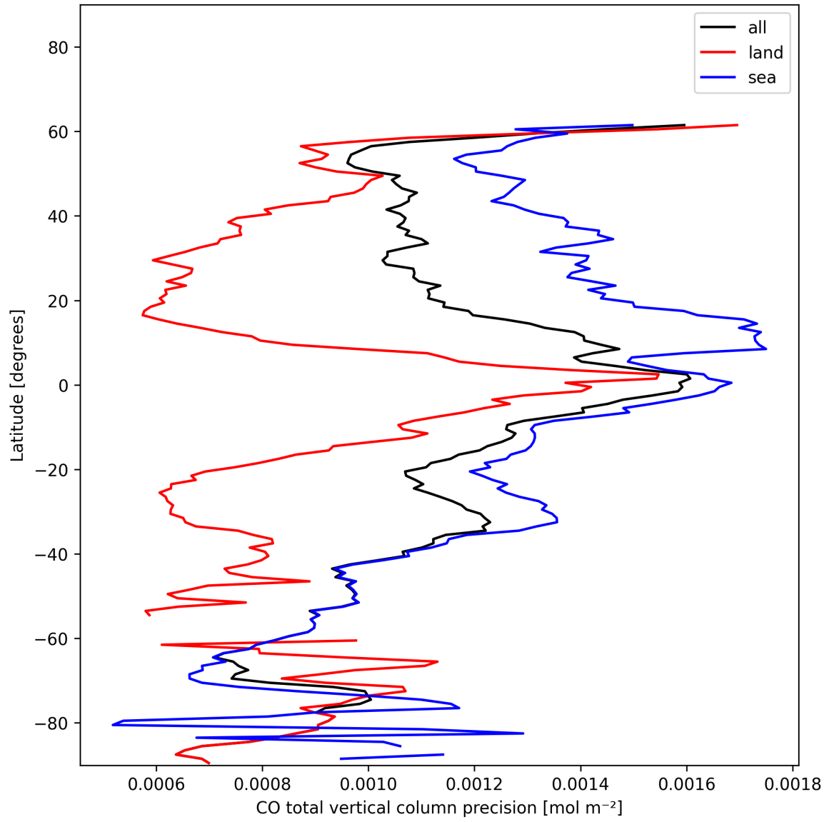
Figure 12: Zonal average of “CO total vertical column precision” for 2024-12-29 to 2024-12-31.
