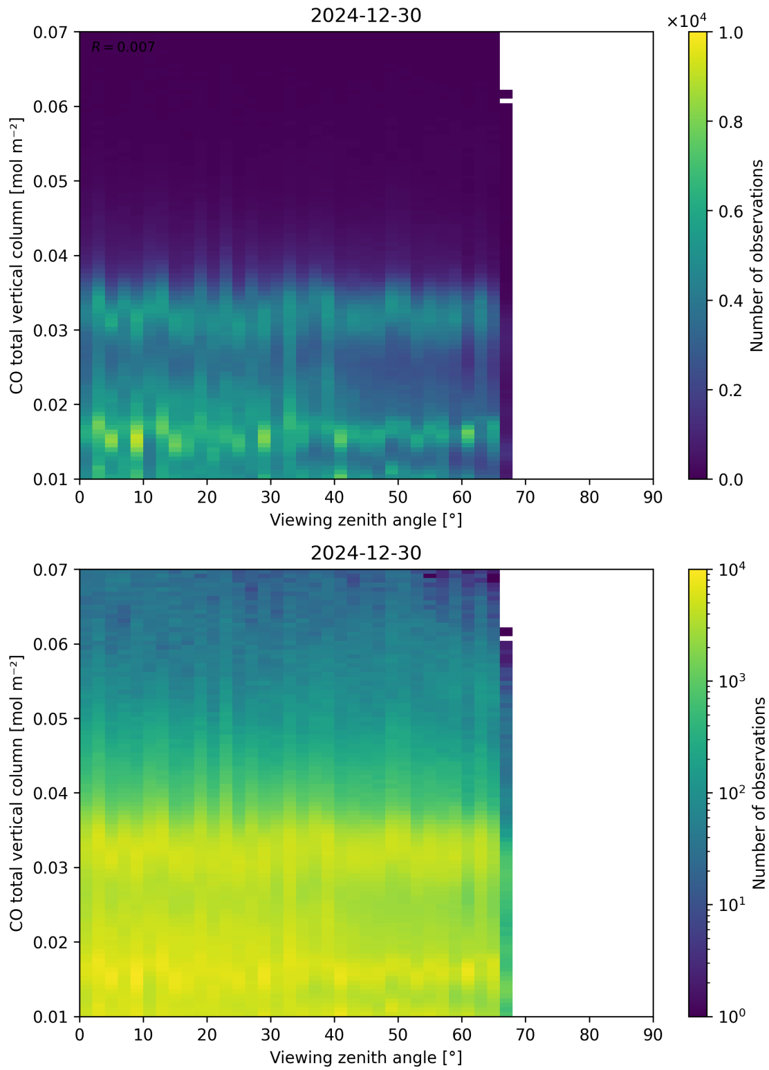
Figure 69: Scatter density plot of “Viewing zenith angle” against “CO total vertical column” for 2024-12-29 to 2024-12-31.
