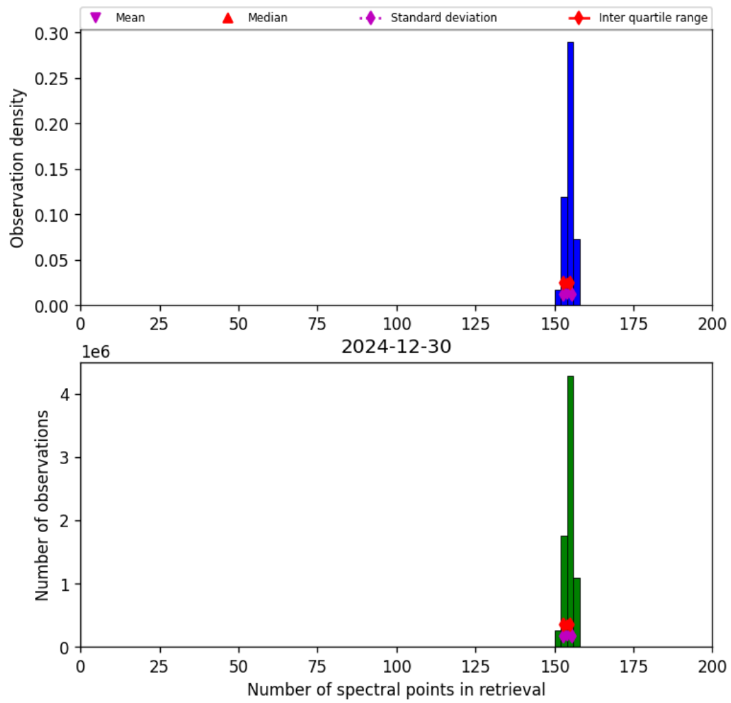
Figure 21: Histogram of “Number of spectral points in retrieval” for 2024-12-29 to 2024-12-31
