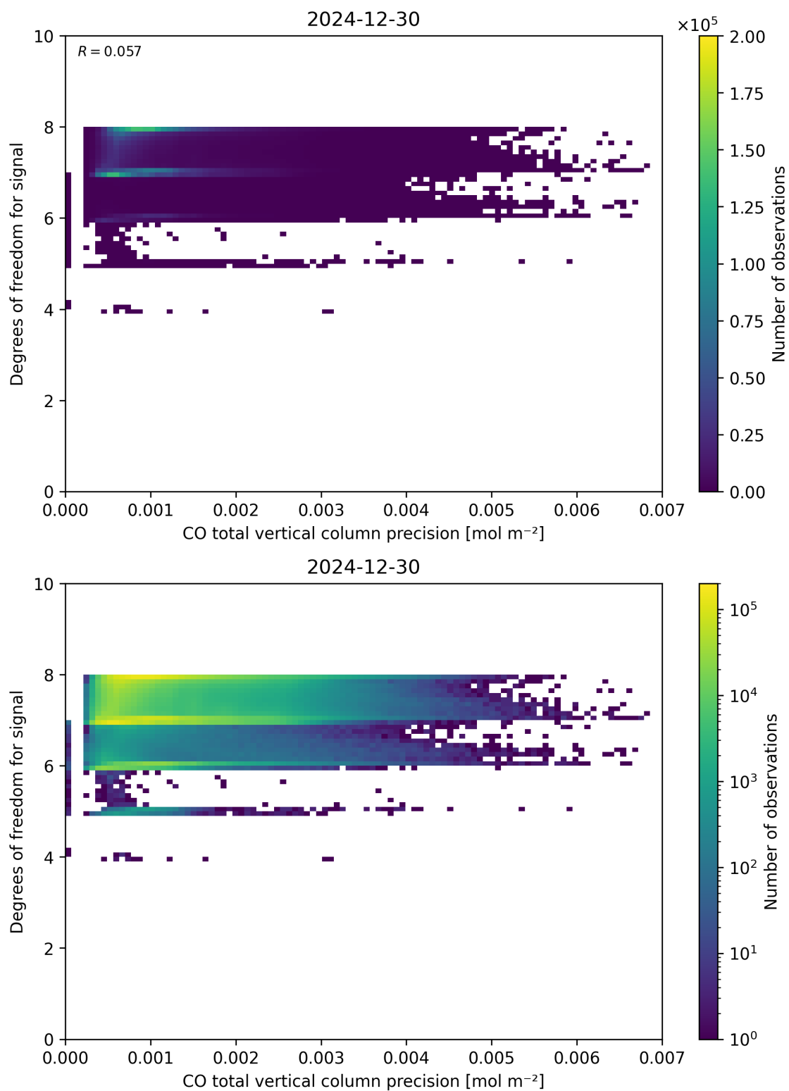
Figure 45: Scatter density plot of “CO total vertical column precision” against “Degrees of freedom for signal” for 2024-12-29 to 2024-12-31.
