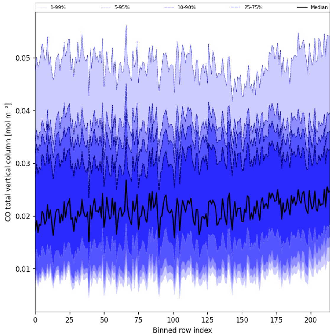
Figure 26: Along track statistics of “CO total vertical column” for 2024-12-29 to 2024-12-31
