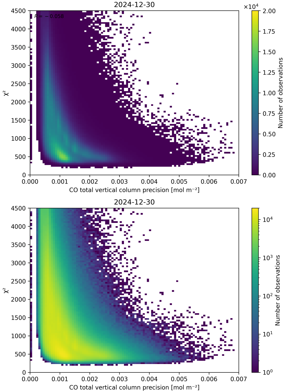
Figure 44: Scatter density plot of “CO total vertical column precision” against “ \chi^2 ” for 2024-12-29 to 2024-12-31.
