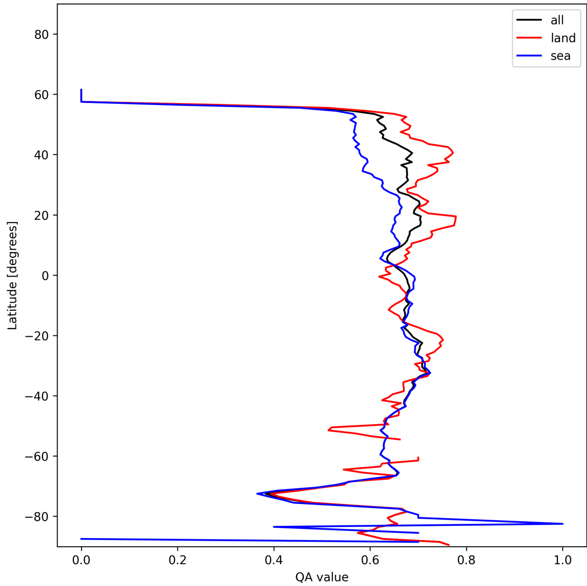
Figure 9: Zonal average of “QA value” for 2024-12-29 to 2024-12-31.
