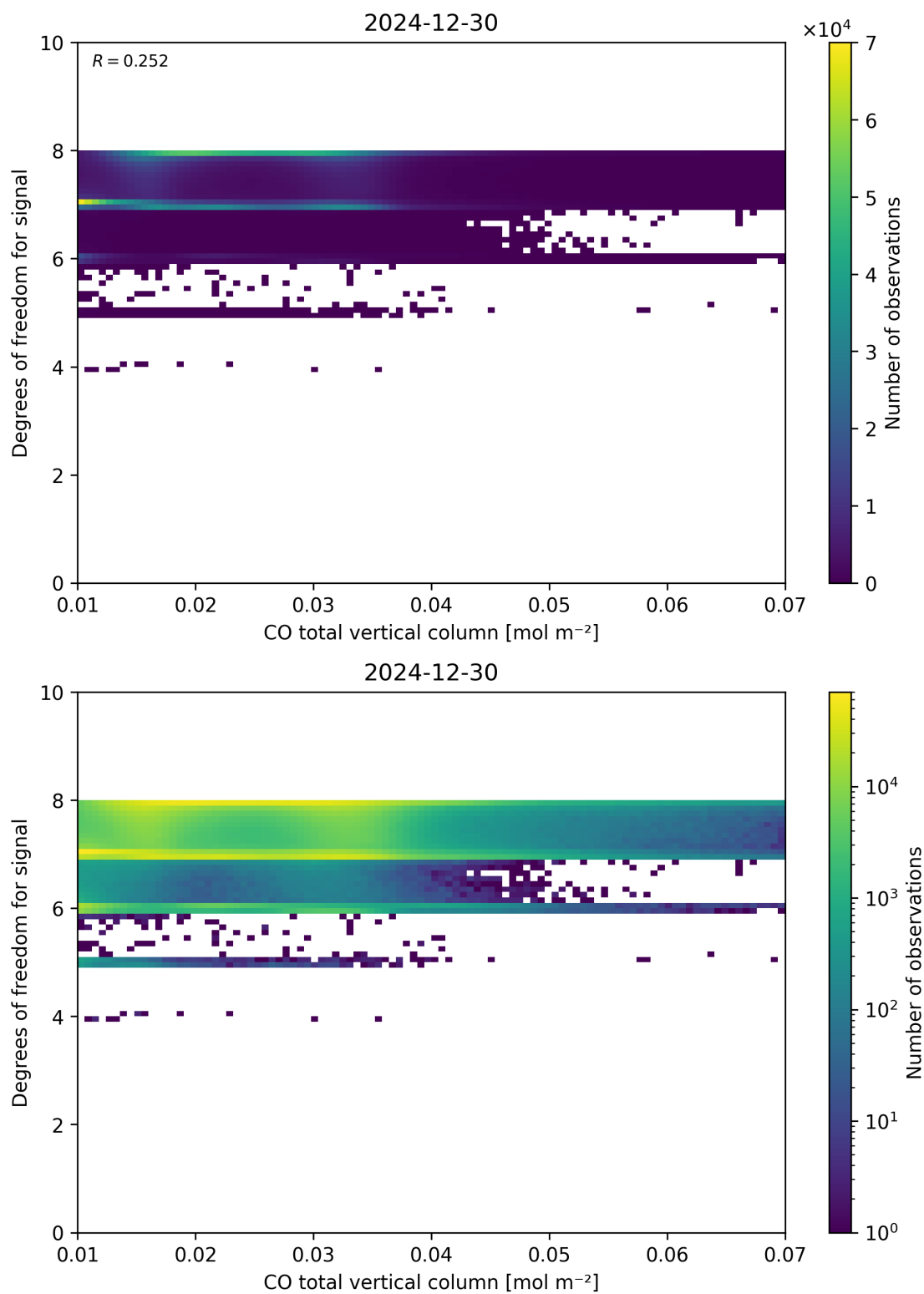
Figure 41: Scatter density plot of “CO total vertical column” against “Degrees of freedom for signal” for 2024-12-29 to 2024-12-31.
