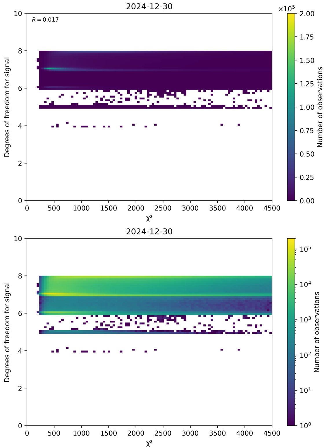
Figure 48: Scatter density plot of “ \chi^2 ” against “Degrees of freedom for signal” for 2024-12-29 to 2024-12-31.
