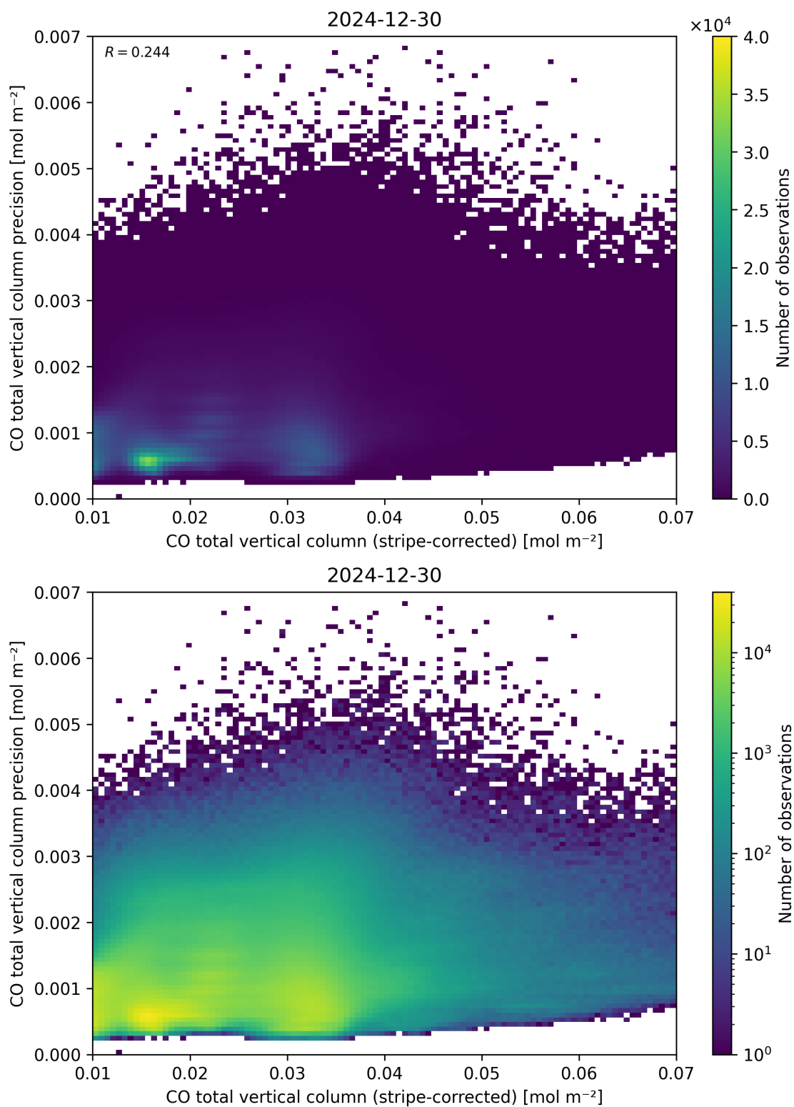
Figure 36: Scatter density plot of “CO total vertical column (stripe-corrected)” against “CO total vertical column precision” for 2024-12-29 to 2024-12-31.
