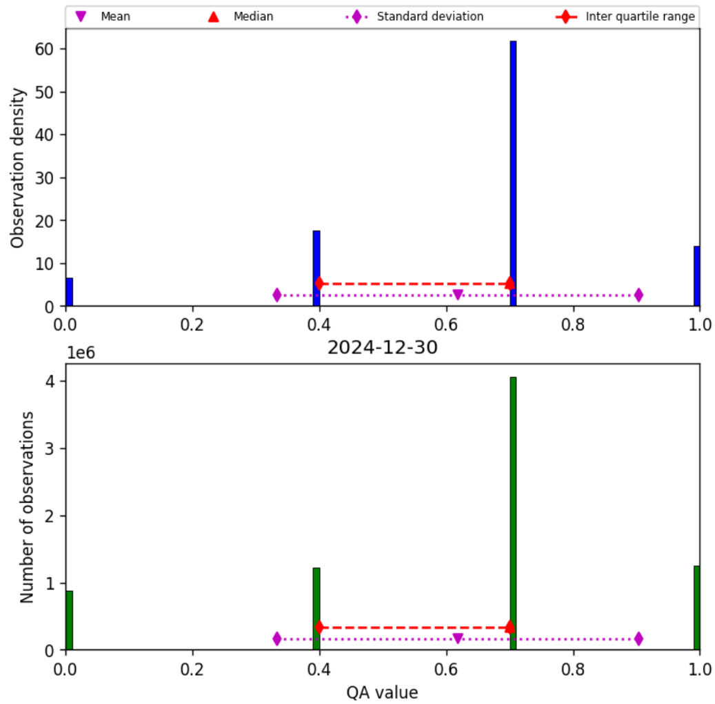
Figure 17: Histogram of “QA value” for 2024-12-29 to 2024-12-31
