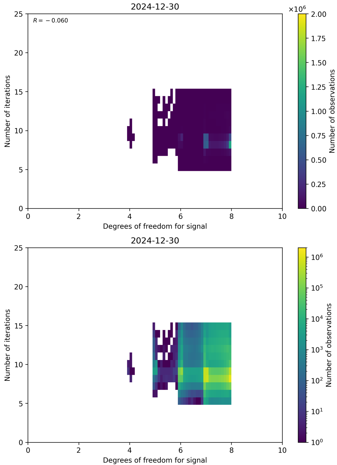
Figure 50: Scatter density plot of “Degrees of freedom for signal” against “Number of iterations” for 2024-12-29 to 2024-12-31.
