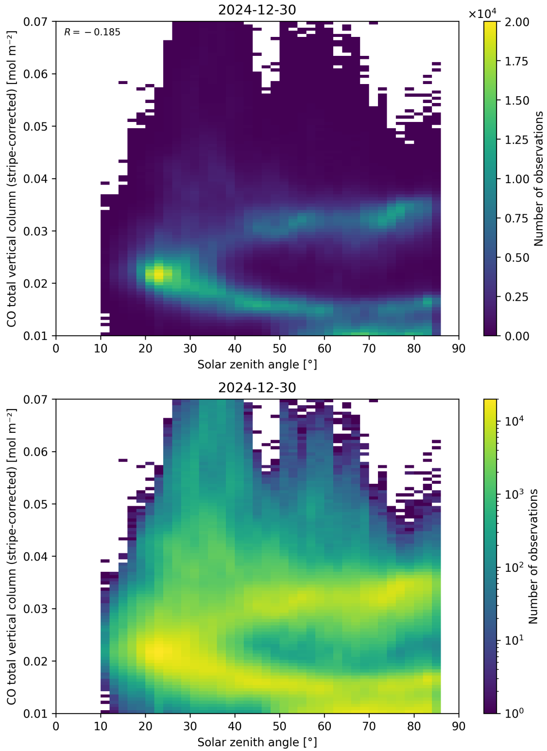
Figure 62: Scatter density plot of “Solar zenith angle” against “CO total vertical column (stripe-corrected)” for 2024-12-29 to 2024-12-31.
