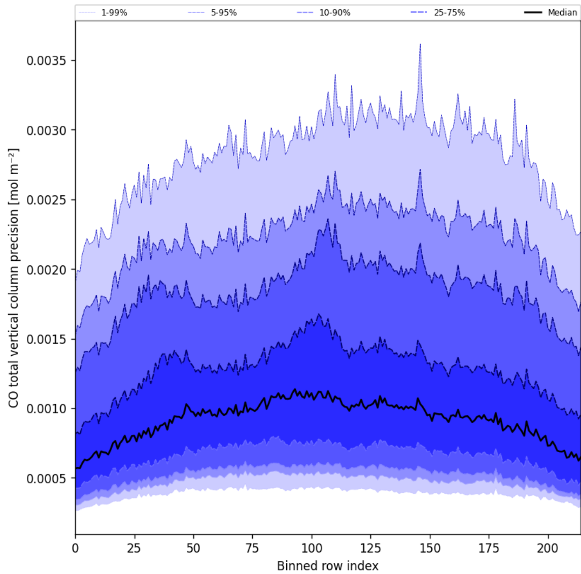
Figure 28: Along track statistics of “CO total vertical column precision” for 2024-12-29 to 2024-12-31
