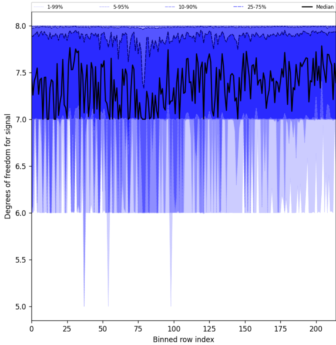
Figure 31: Along track statistics of “Degrees of freedom for signal” for 2024-12-29 to 2024-12-31
