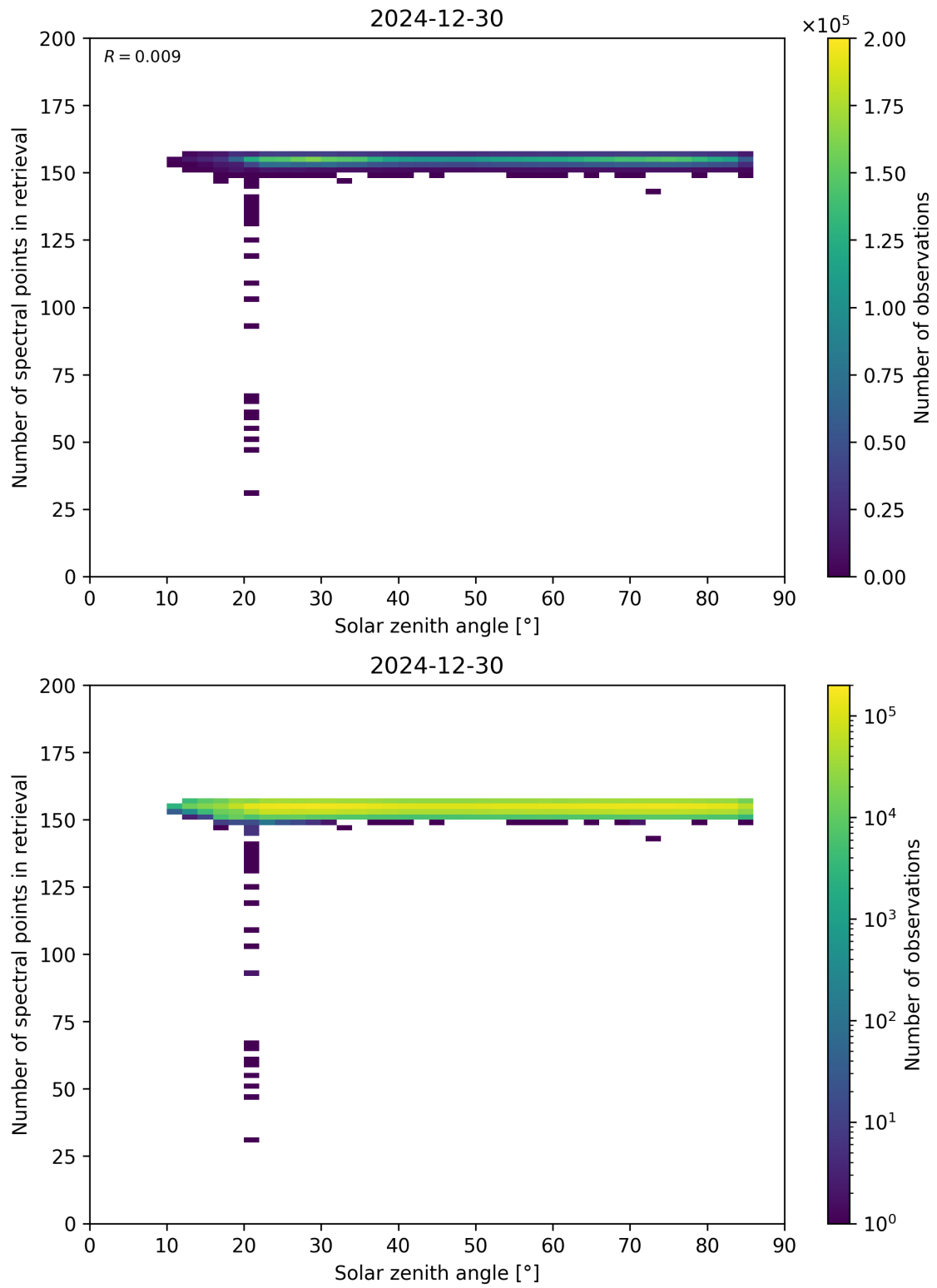
Figure 68: Scatter density plot of “Solar zenith angle” against “Number of spectral points in retrieval” for 2024-12-29 to 2024-12-31.
