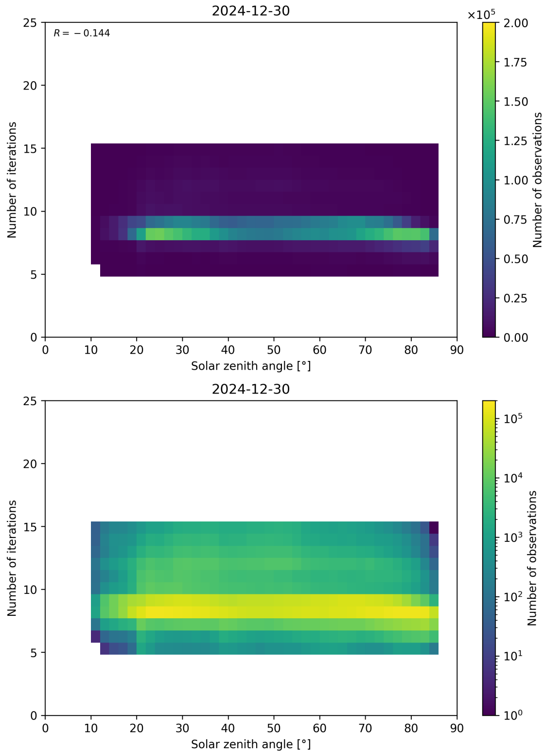
Figure 67: Scatter density plot of “Solar zenith angle” against “Number of iterations” for 2024-12-29 to 2024-12-31.
