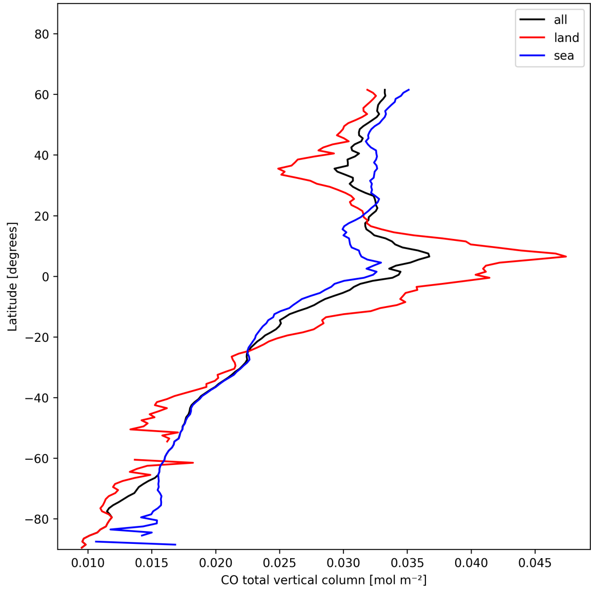
Figure 10: Zonal average of “CO total vertical column” for 2024-12-29 to 2024-12-31.
