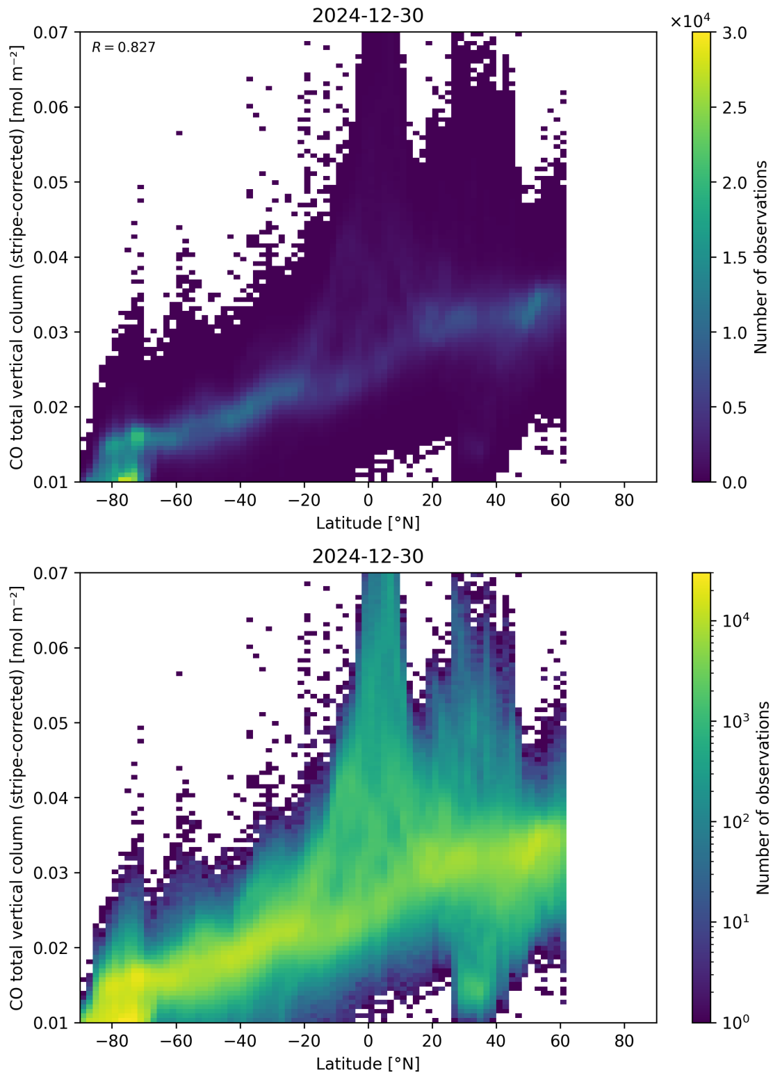
Figure 52: Scatter density plot of “Latitude” against “CO total vertical column (stripe-corrected)” for 2024-12-29 to 2024-12-31.
