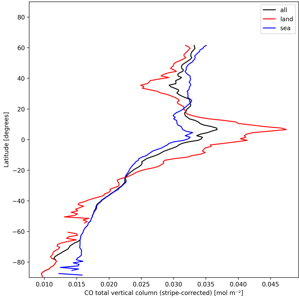
Figure 11: Zonal average of “CO total vertical column (stripe-corrected)” for 2024-12-29 to 2024-12-31.
