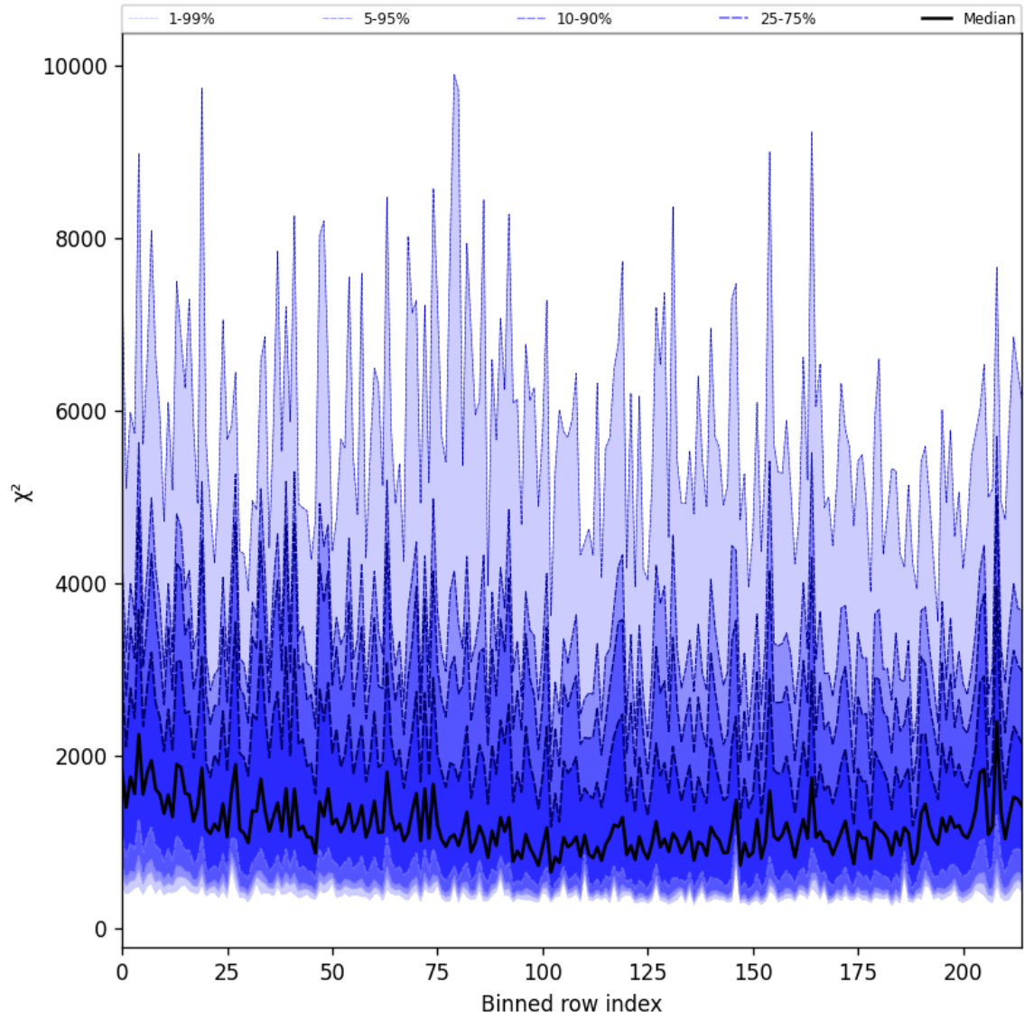
Figure 30: Along track statistics of “ \chi^2 ” for 2024-12-29 to 2024-12-31
