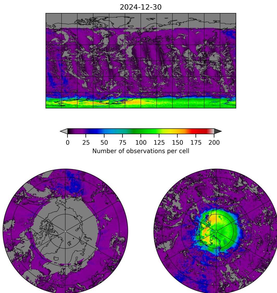
Figure 8: Map of the number of observations for 2024-12-29 to 2024-12-31
