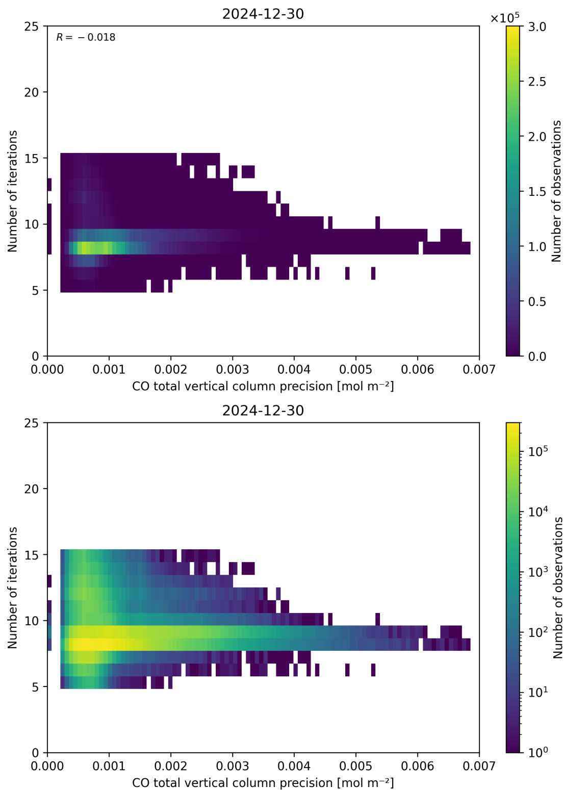
Figure 46: Scatter density plot of “CO total vertical column precision” against “Number of iterations” for 2024-12-29 to 2024-12-31.
