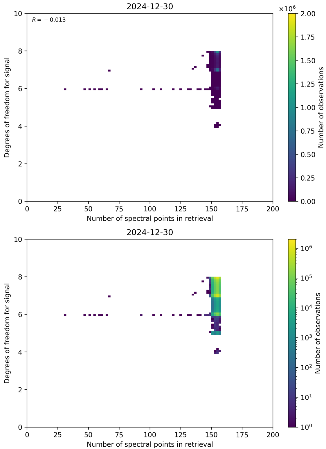
Figure 59: Scatter density plot of “Number of spectral points in retrieval” against “Degrees of freedom for signal” for 2024-12-29 to 2024-12-31.
