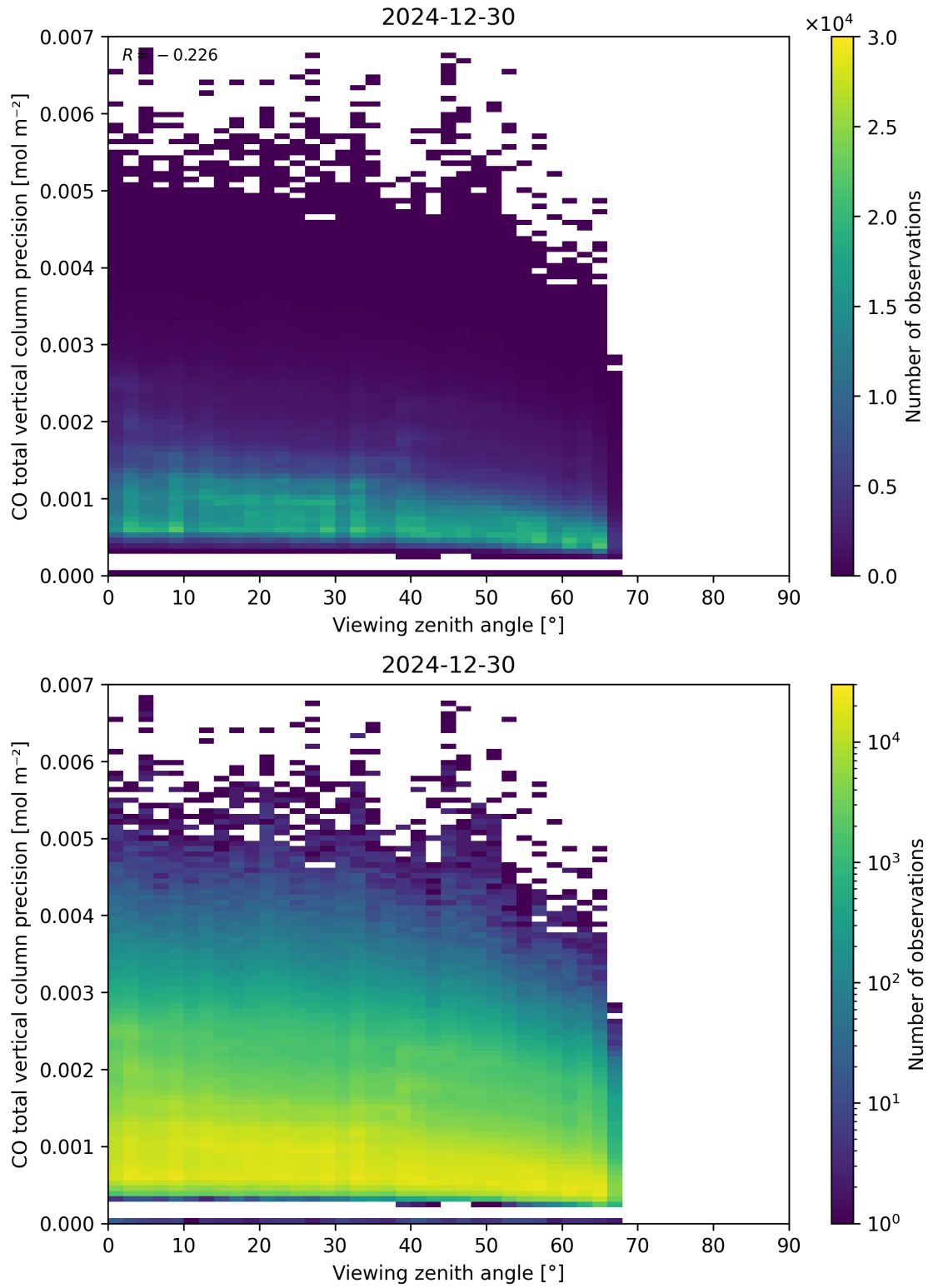
Figure 71: Scatter density plot of “Viewing zenith angle” against “CO total vertical column precision” for 2024-12-29 to 2024-12-31.
