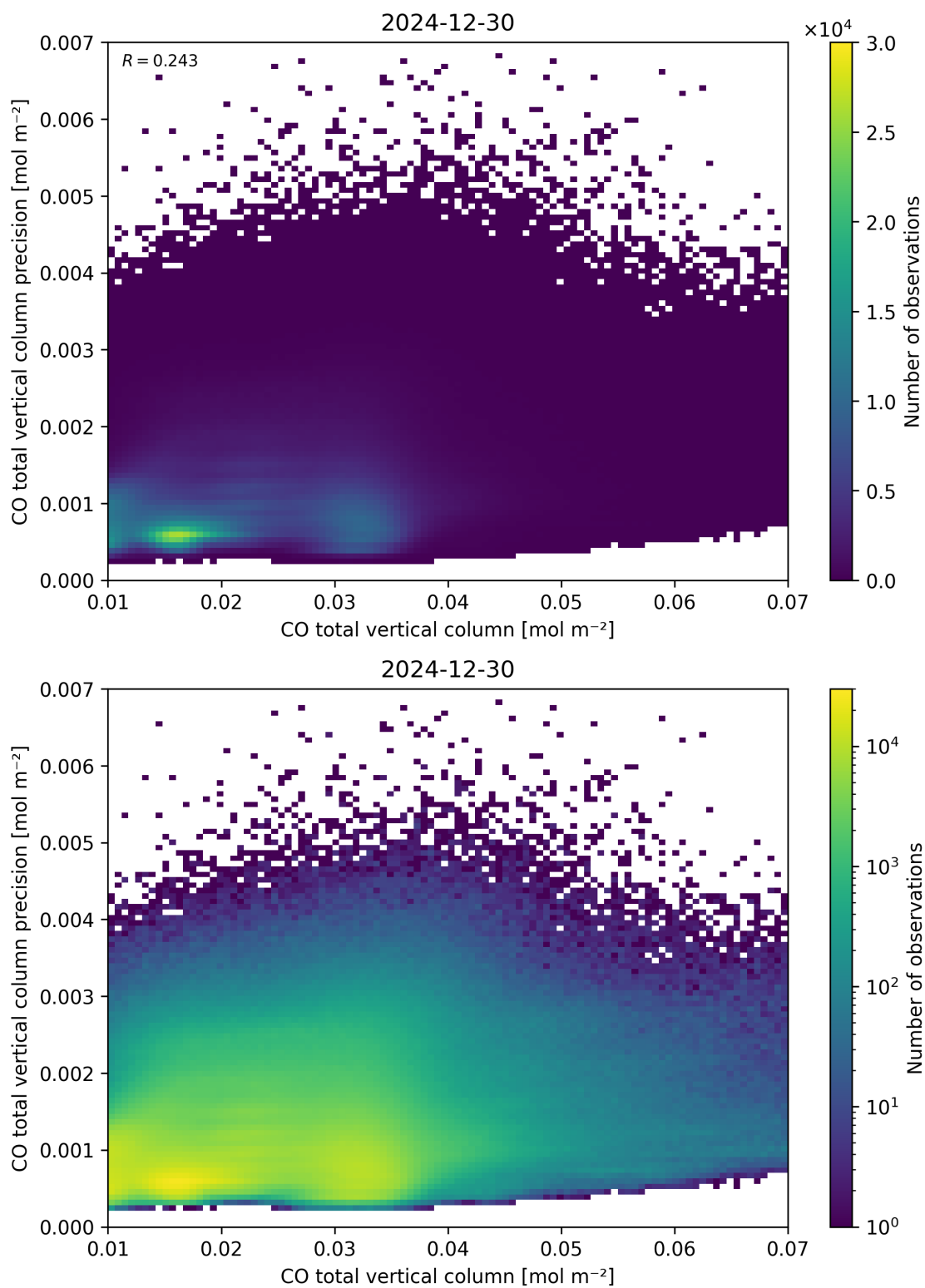
Figure 34: Scatter density plot of “CO total vertical column” against “CO total vertical column precision” for 2024-12-29 to 2024-12-31.
