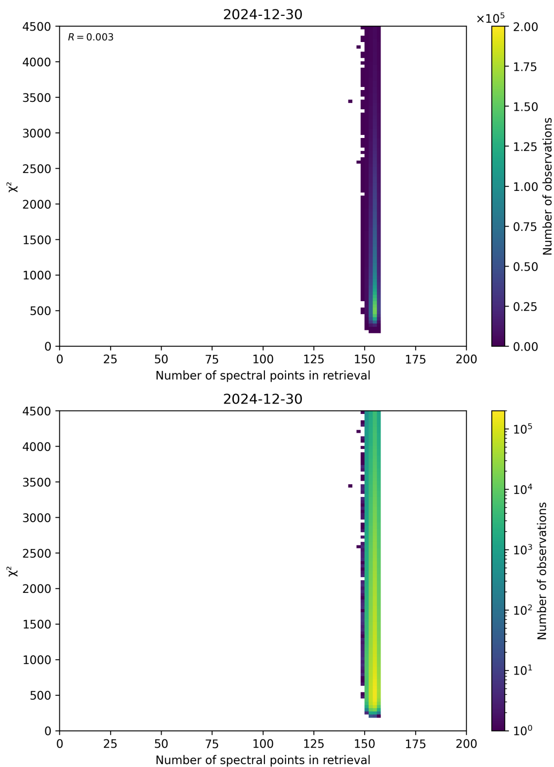
Figure 58: Scatter density plot of “Number of spectral points in retrieval” against “ \chi^2 ” for 2024-12-29 to 2024-12-31.
