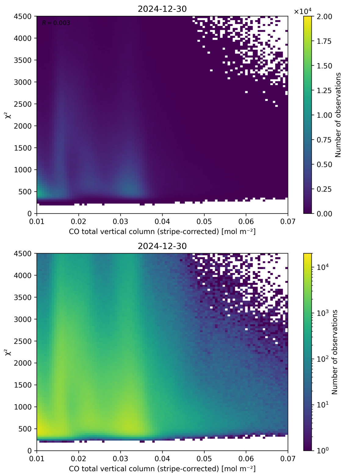
Figure 37: Scatter density plot of “CO total vertical column (stripe-corrected)” against “ \chi^2 ” for 2024-12-29 to 2024-12-31.
