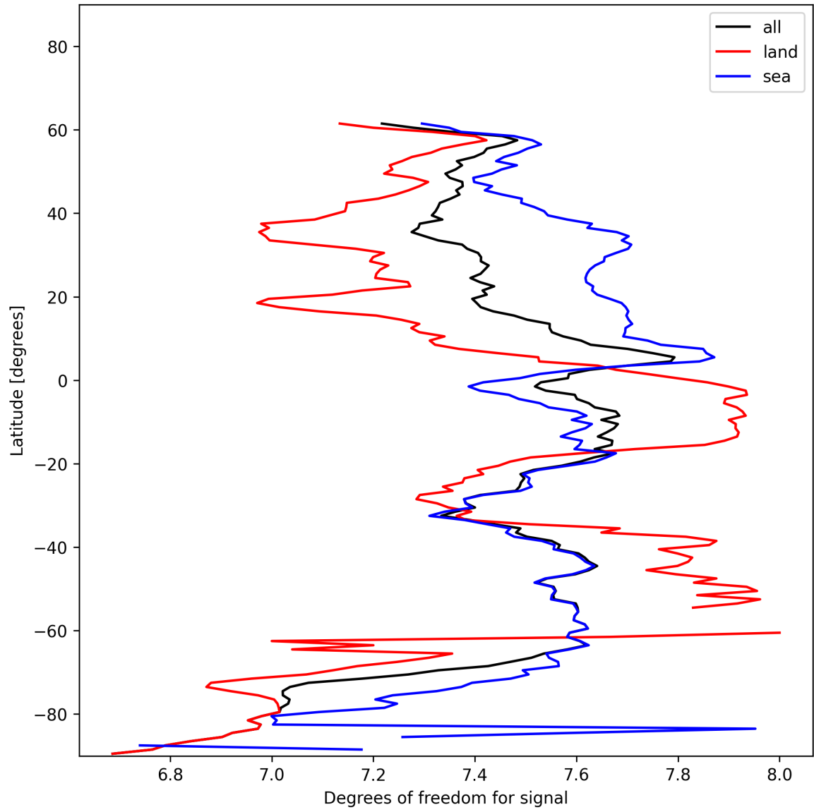
Figure 15: Zonal average of “Degrees of freedom for signal” for 2024-12-29 to 2024-12-31.
