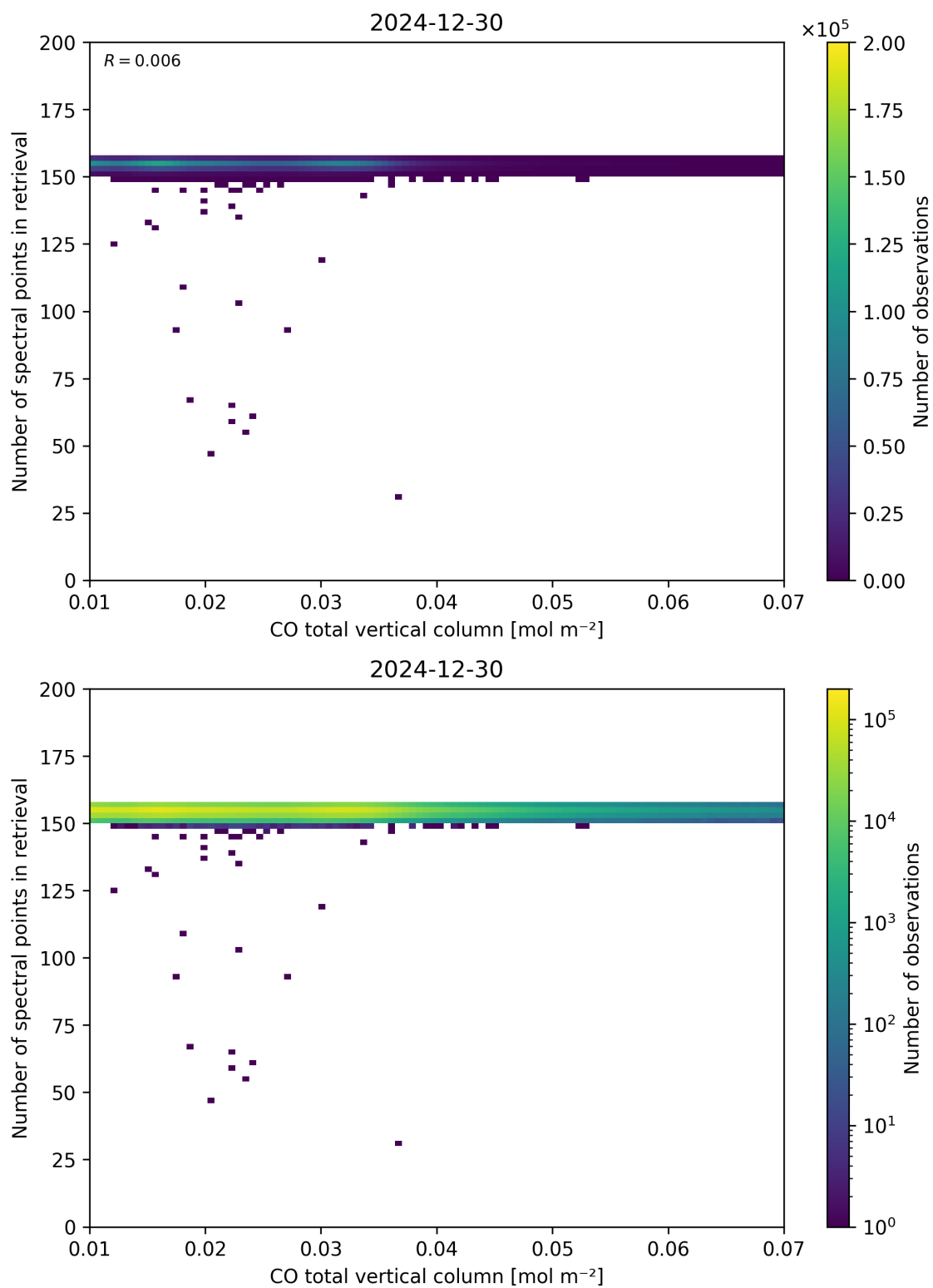
Figure 43: Scatter density plot of “CO total vertical column” against “Number of spectral points in retrieval” for 2024-12-29 to 2024-12-31.
