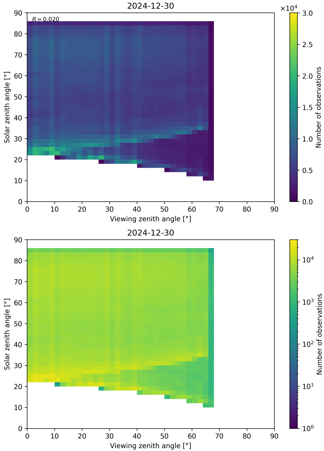
Figure 77: Scatter density plot of “Viewing zenith angle” against “Solar zenith angle” for 2024-12-29 to 2024-12-31.
