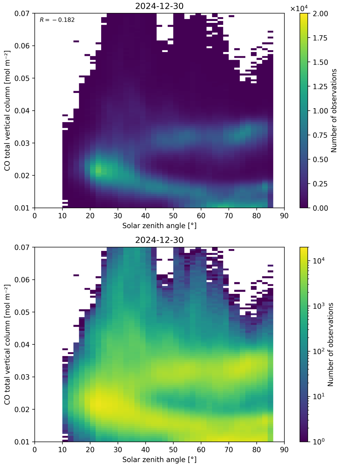
Figure 61: Scatter density plot of “Solar zenith angle” against “CO total vertical column” for 2024-12-29 to 2024-12-31.
