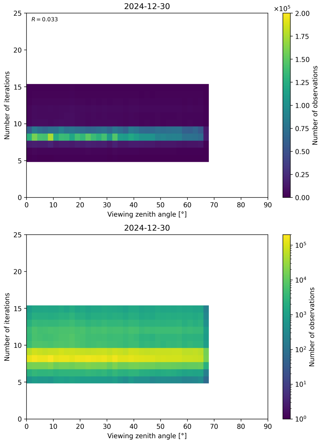
Figure 75: Scatter density plot of “Viewing zenith angle” against “Number of iterations” for 2024-12-29 to 2024-12-31.
