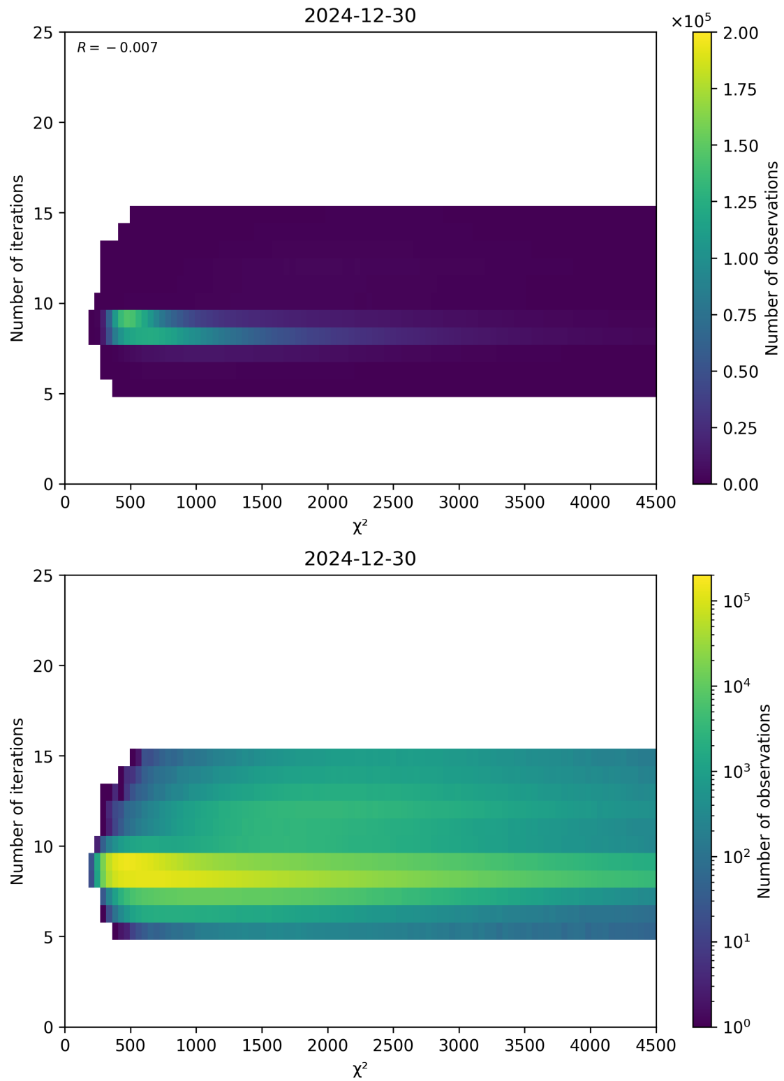
Figure 49: Scatter density plot of “ \chi^2 ” against “Number of iterations” for 2024-12-29 to 2024-12-31.
