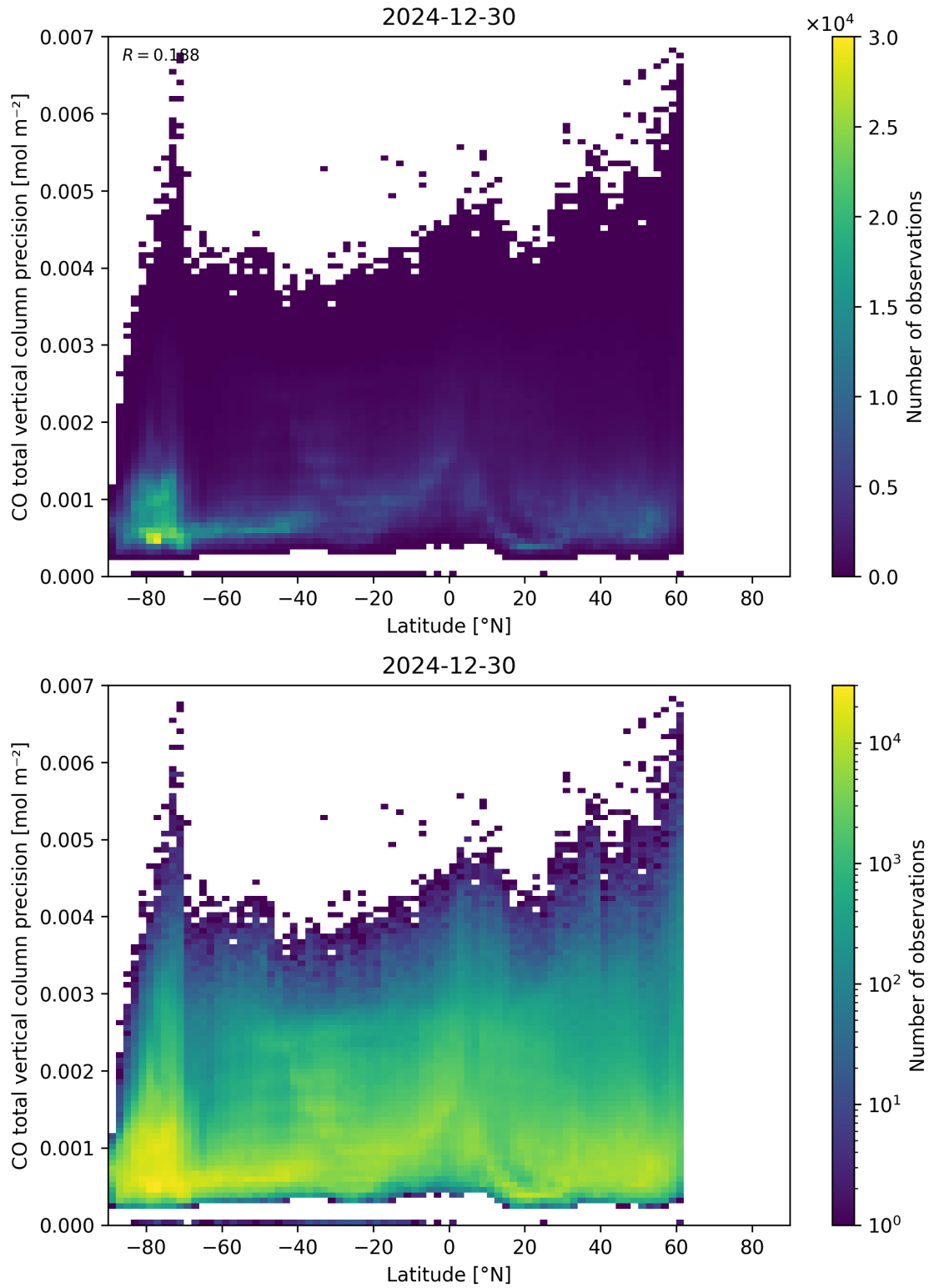
Figure 53: Scatter density plot of “Latitude” against “CO total vertical column precision” for 2024-12-29 to 2024-12-31.
