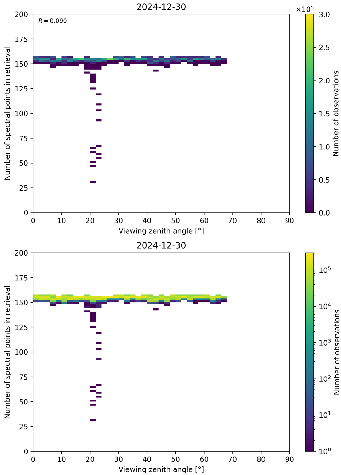
Figure 76: Scatter density plot of “Viewing zenith angle” against “Number of spectral points in retrieval” for 2024-12-29 to 2024-12-31.
