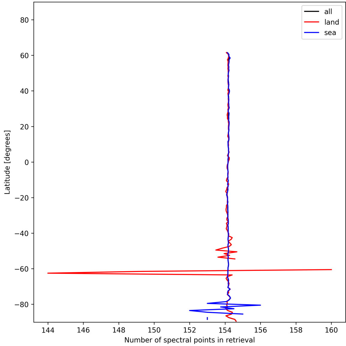
Figure 13: Zonal average of “Number of spectral points in retrieval” for 2024-12-29 to 2024-12-31.
