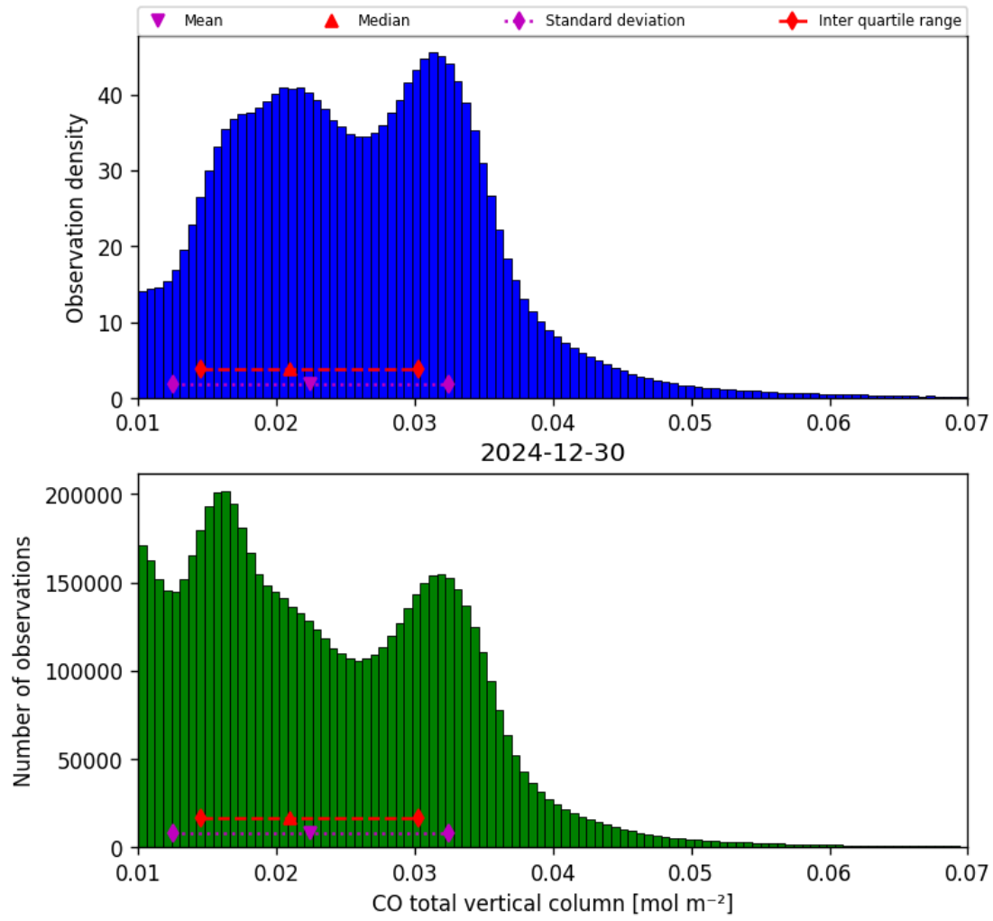
Figure 18: Histogram of “CO total vertical column” for 2024-12-29 to 2024-12-31
