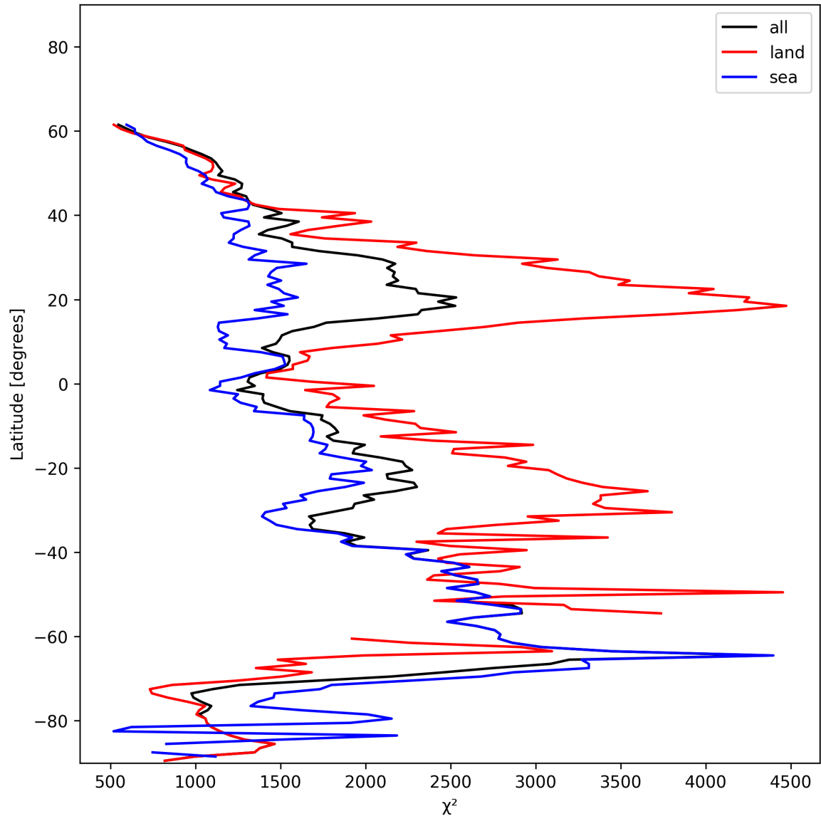
Figure 14: Zonal average of “ \chi^2 ” for 2024-12-29 to 2024-12-31.
