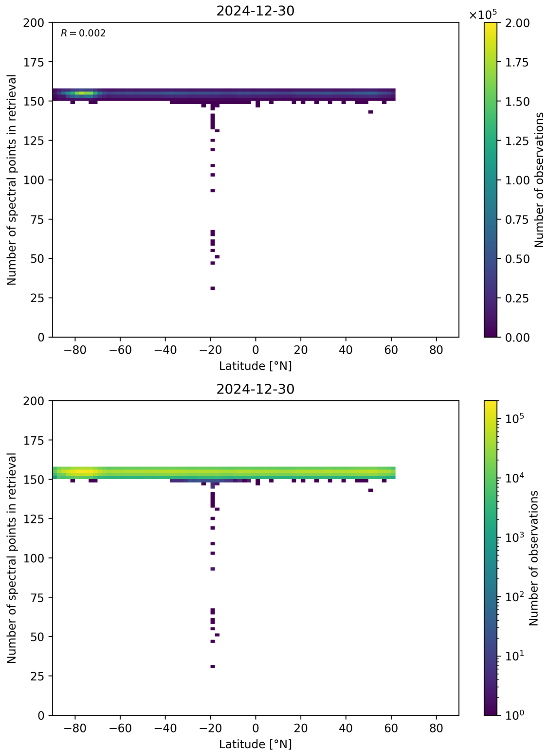
Figure 57: Scatter density plot of “Latitude” against “Number of spectral points in retrieval” for 2024-12-29 to 2024-12-31.
