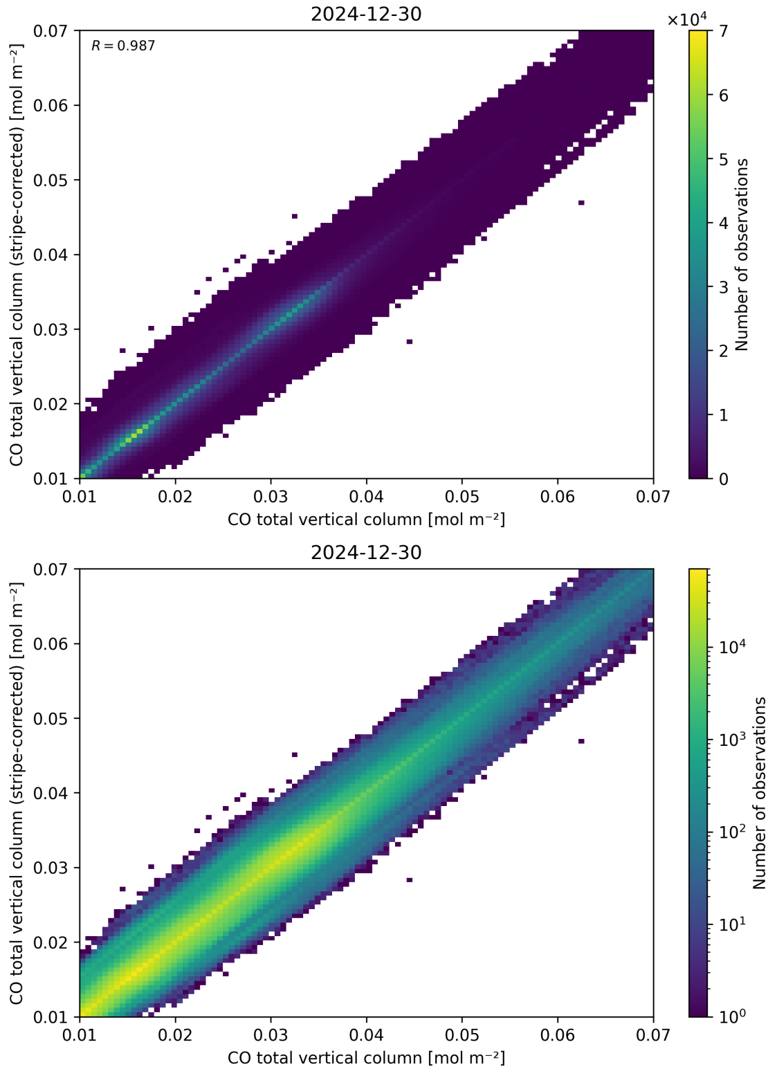
Figure 33: Scatter density plot of “CO total vertical column” against “CO total vertical column (stripe-corrected)” for 2024-12-29 to 2024-12-31.
