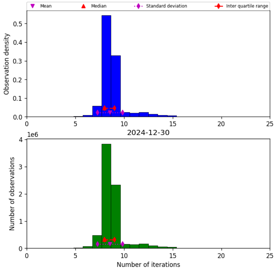
Figure 24: Histogram of “Number of iterations” for 2024-12-29 to 2024-12-31
