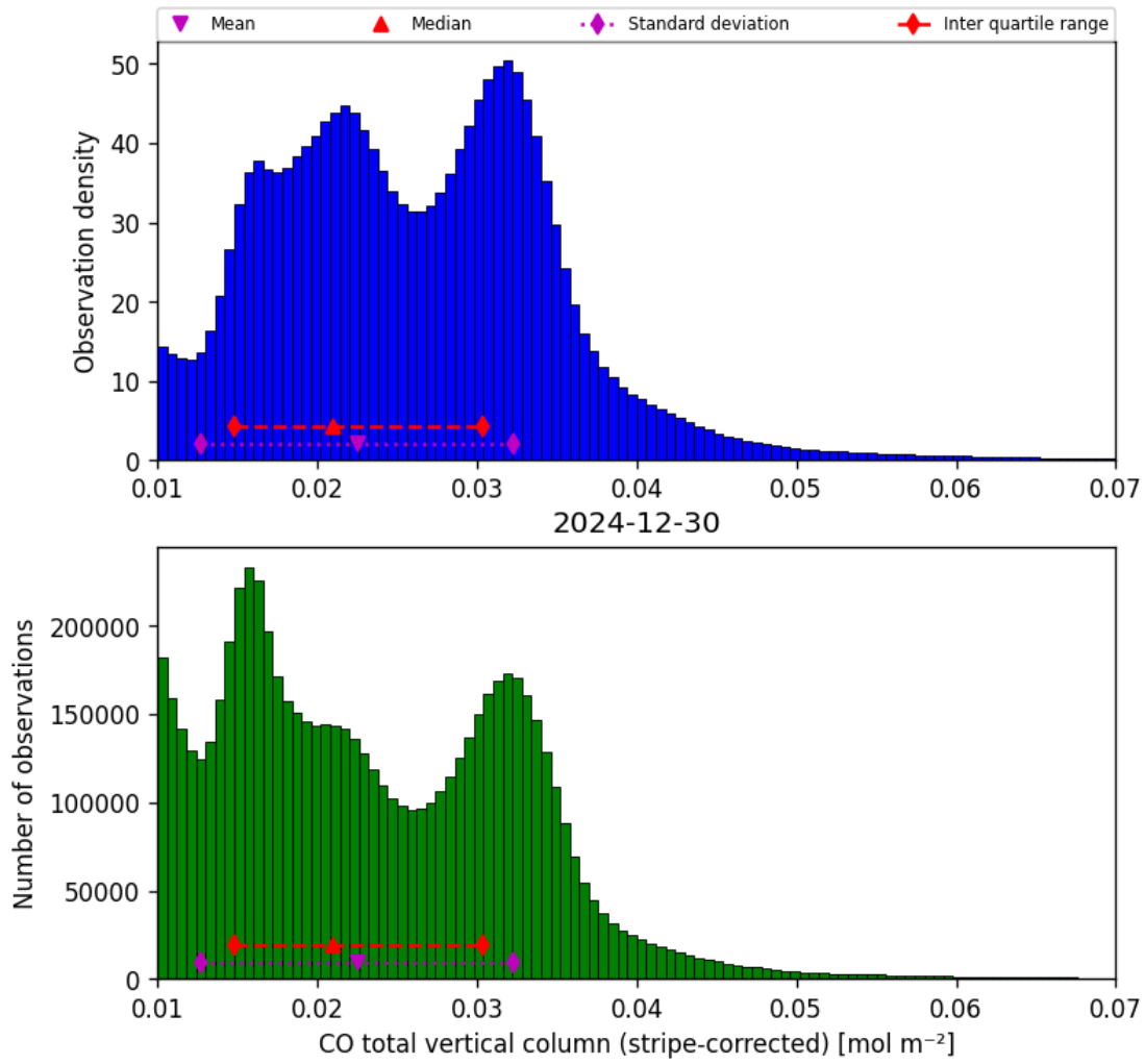
Figure 19: Histogram of “CO total vertical column (stripe-corrected)” for 2024-12-29 to 2024-12-31
