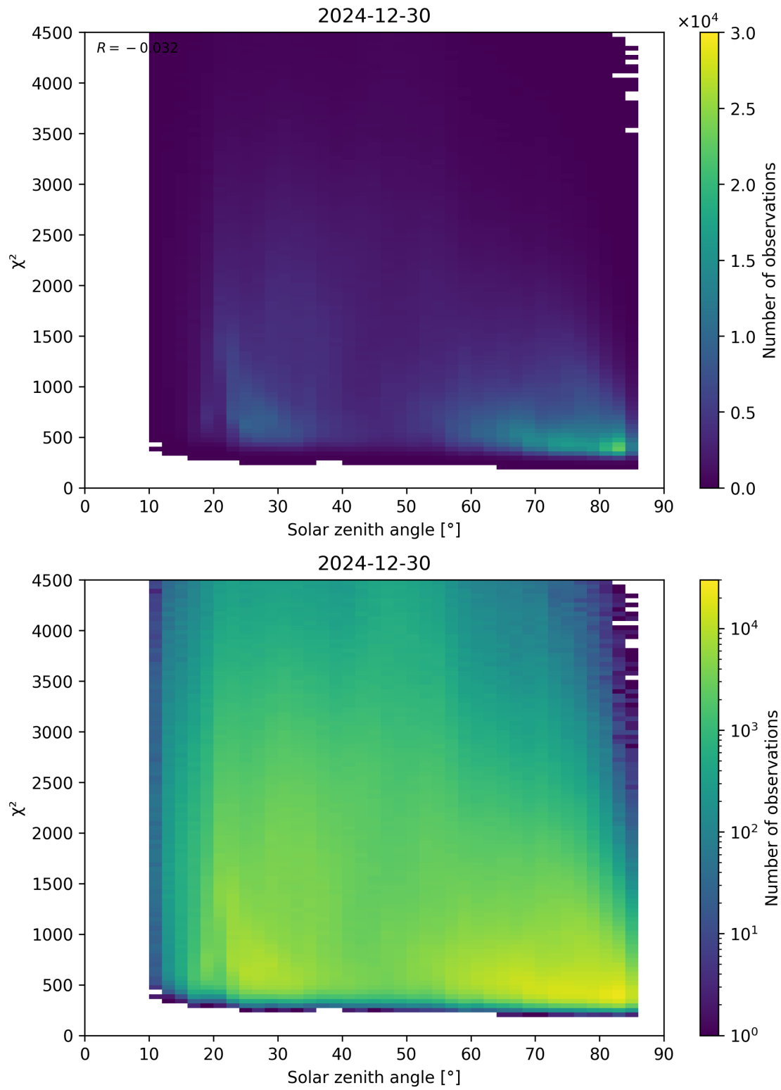
Figure 64: Scatter density plot of “Solar zenith angle” against “ \chi^2 ” for 2024-12-29 to 2024-12-31.
