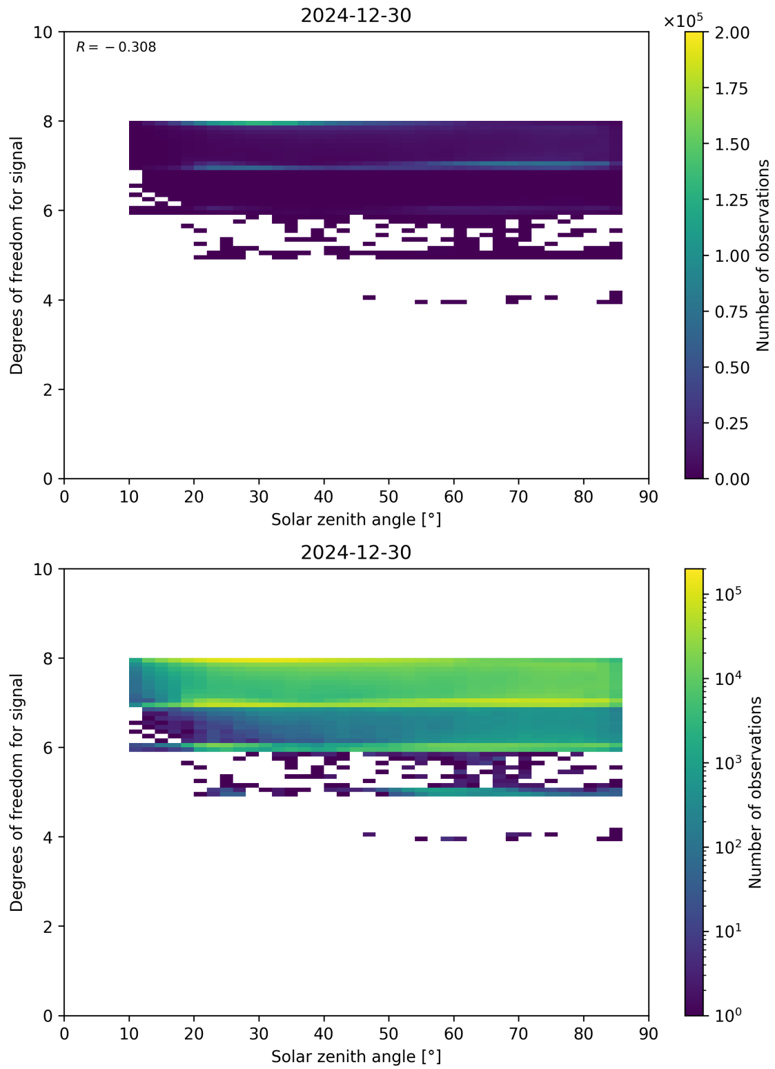
Figure 65: Scatter density plot of “Solar zenith angle” against “Degrees of freedom for signal” for 2024-12-29 to 2024-12-31.
