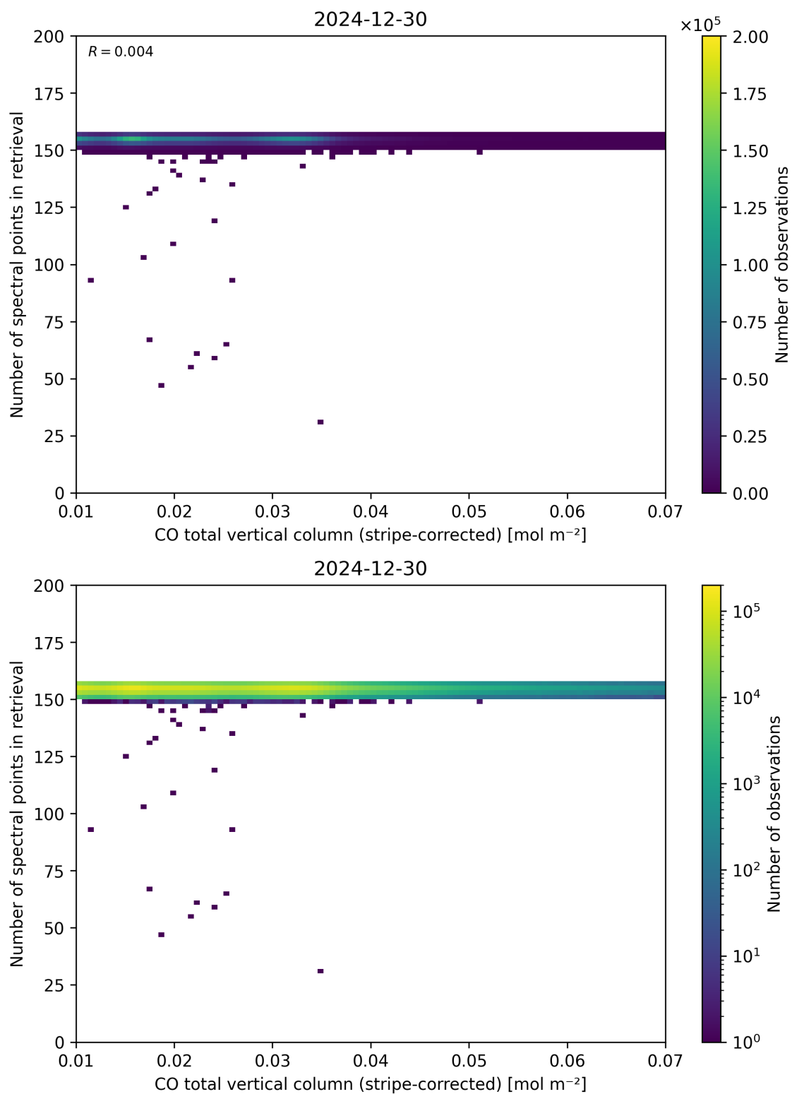
Figure 40: Scatter density plot of “CO total vertical column (stripe-corrected)” against “Number of spectral points in retrieval” for 2024-12-29 to 2024-12-31.
