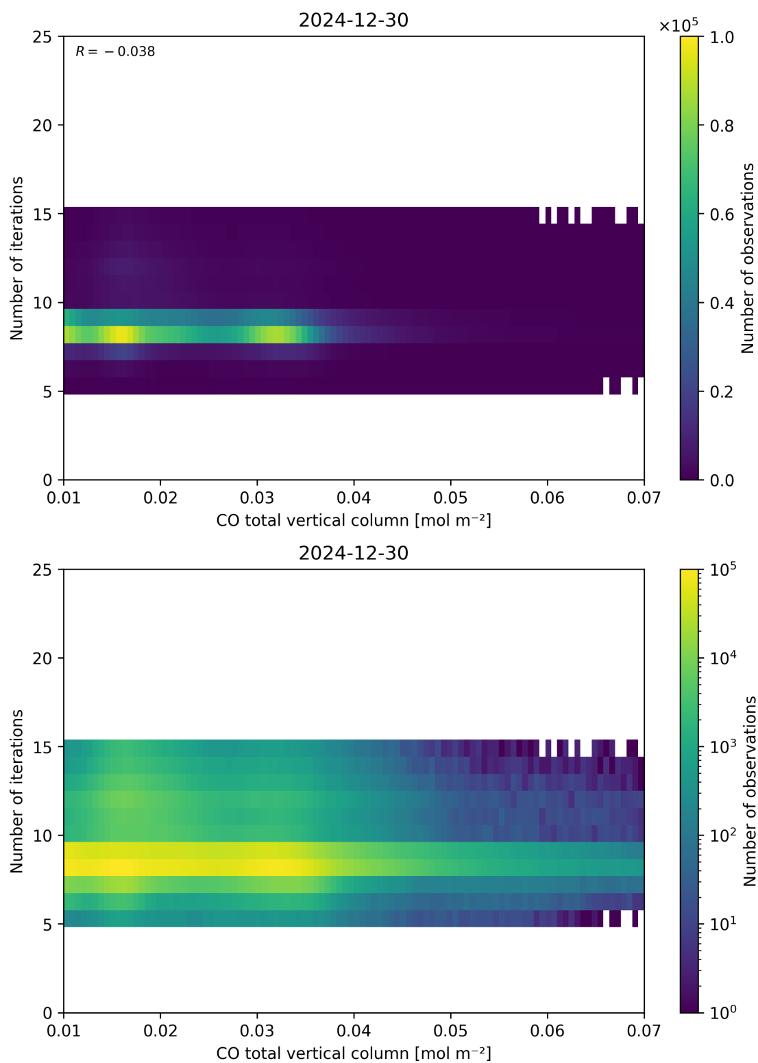
Figure 42: Scatter density plot of “CO total vertical column” against “Number of iterations” for 2024-12-29 to 2024-12-31.
