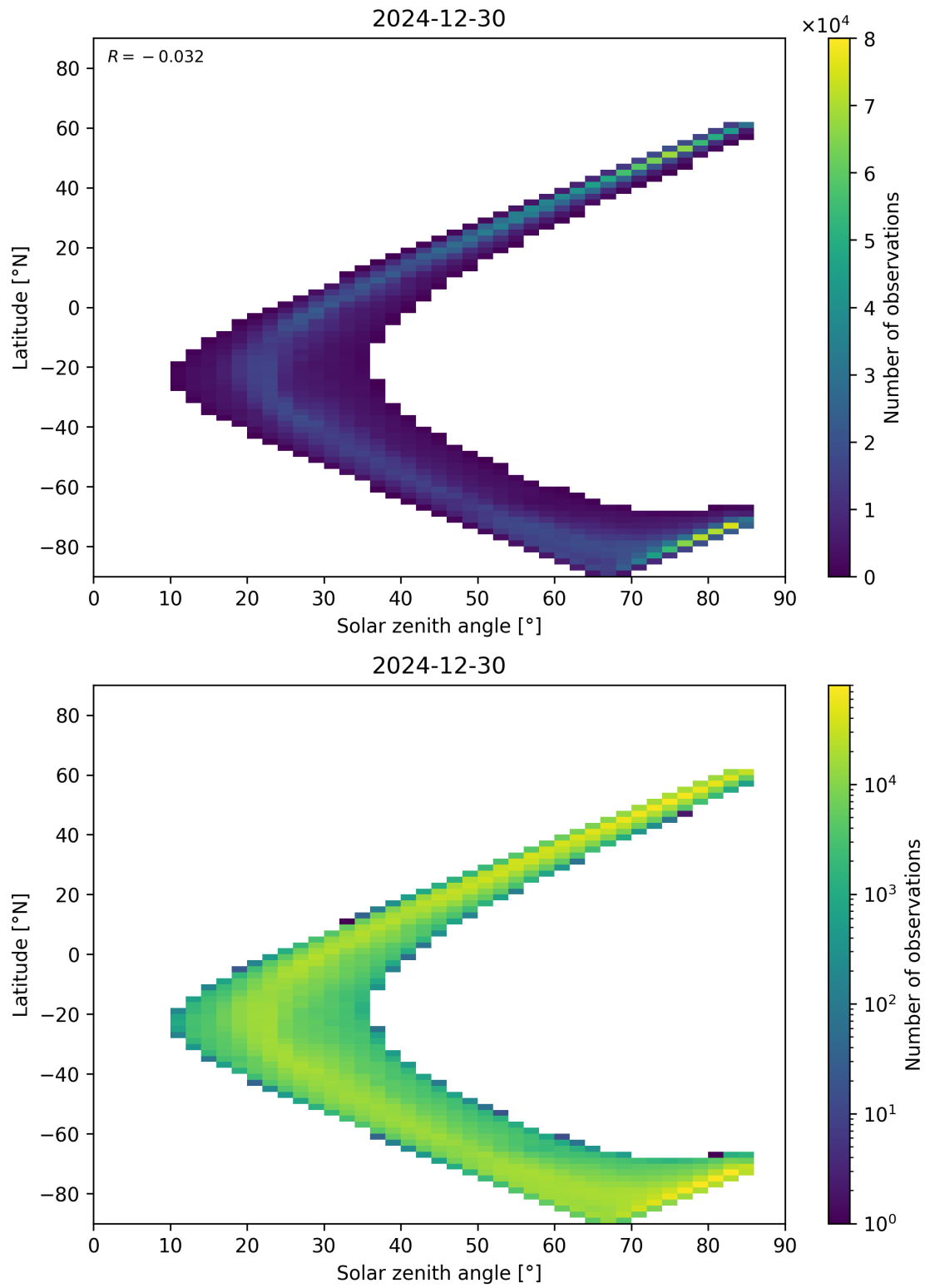
Figure 66: Scatter density plot of “Solar zenith angle” against “Latitude” for 2024-12-29 to 2024-12-31.
