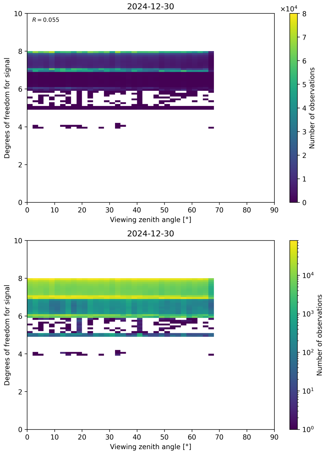
Figure 73: Scatter density plot of “Viewing zenith angle” against “Degrees of freedom for signal” for 2024-12-29 to 2024-12-31.
