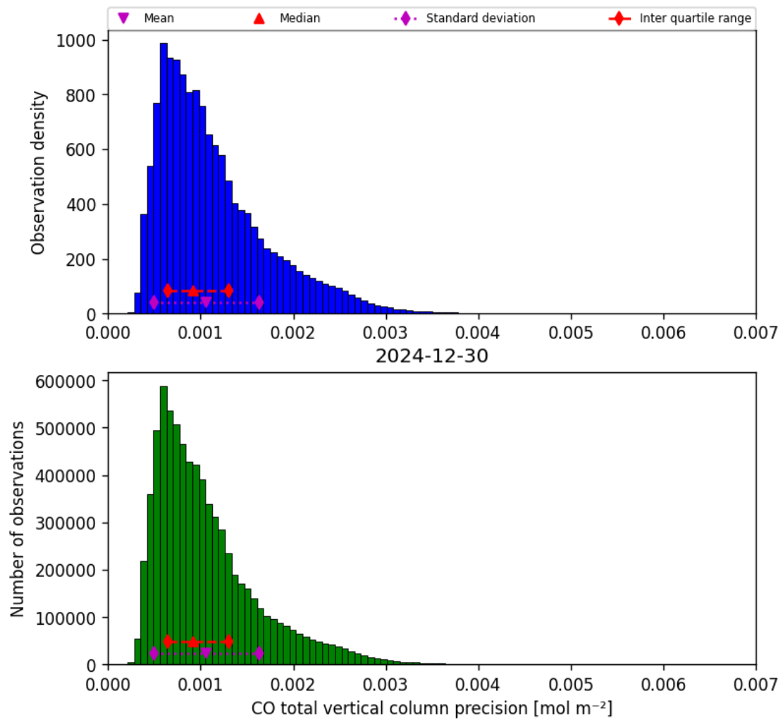
Figure 20: Histogram of “CO total vertical column precision” for 2024-12-29 to 2024-12-31
