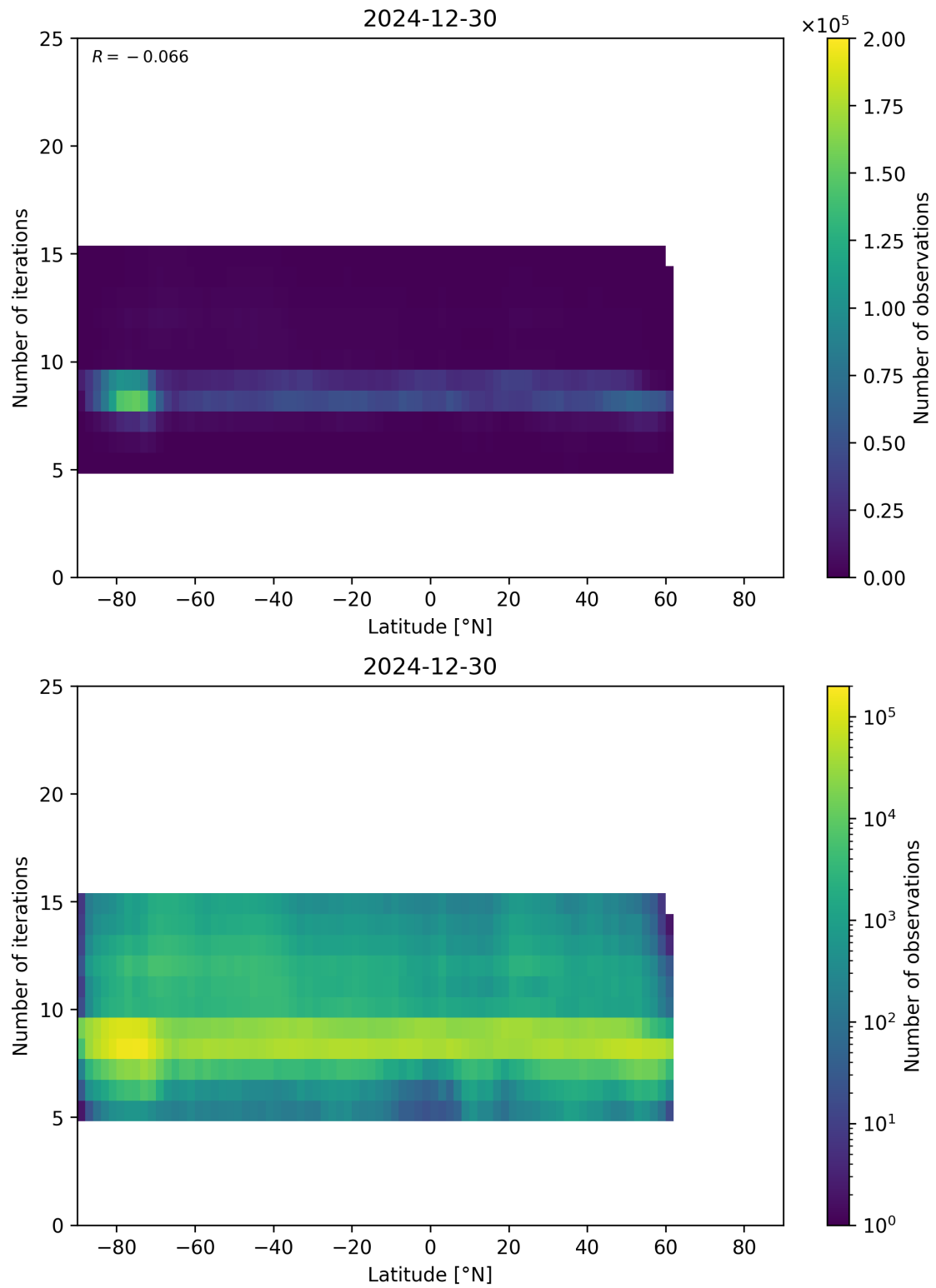
Figure 56: Scatter density plot of “Latitude” against “Number of iterations” for 2024-12-29 to 2024-12-31.
