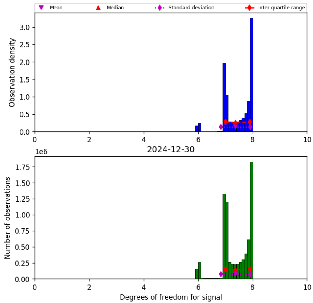
Figure 23: Histogram of “Degrees of freedom for signal” for 2024-12-29 to 2024-12-31
