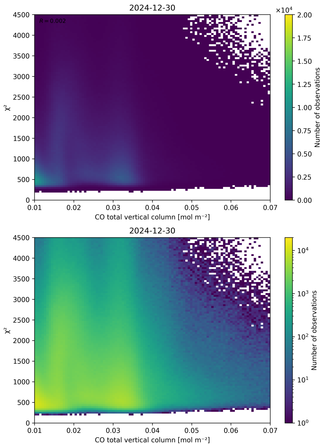
Figure 35: Scatter density plot of “CO total vertical column” against “ \chi^2 ” for 2024-12-29 to 2024-12-31.
