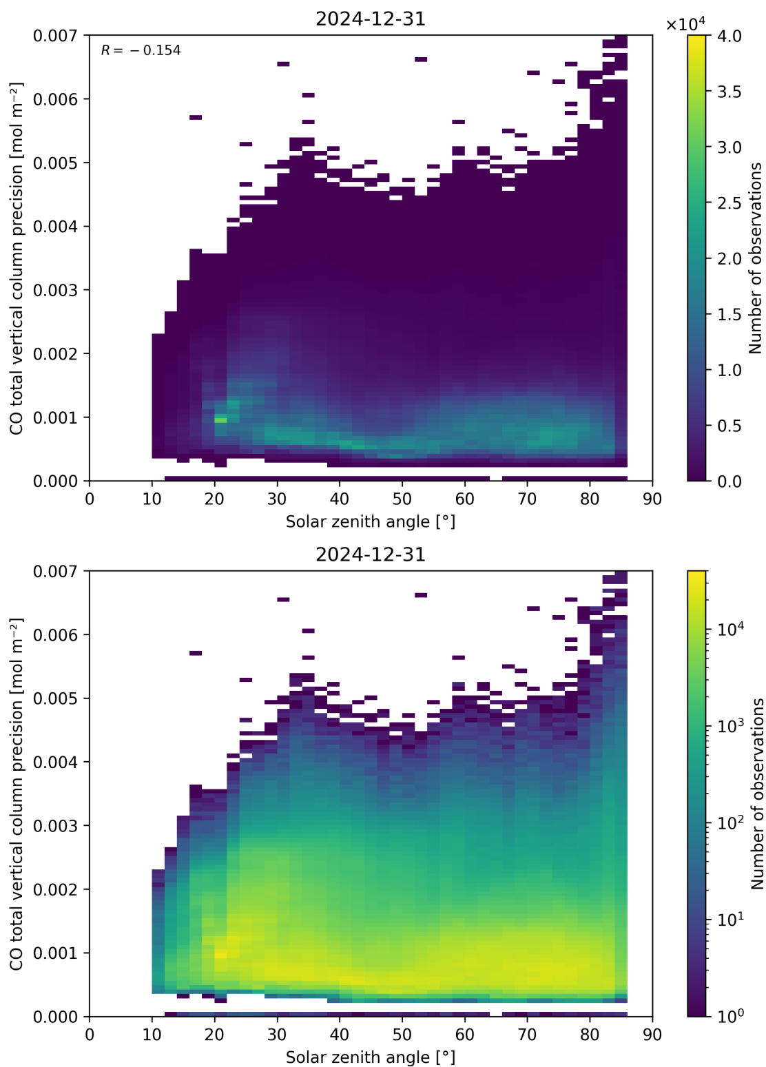
Figure 63: Scatter density plot of “Solar zenith angle” against “CO total vertical column precision” for 2024-12-30 to 2025-01-01.
