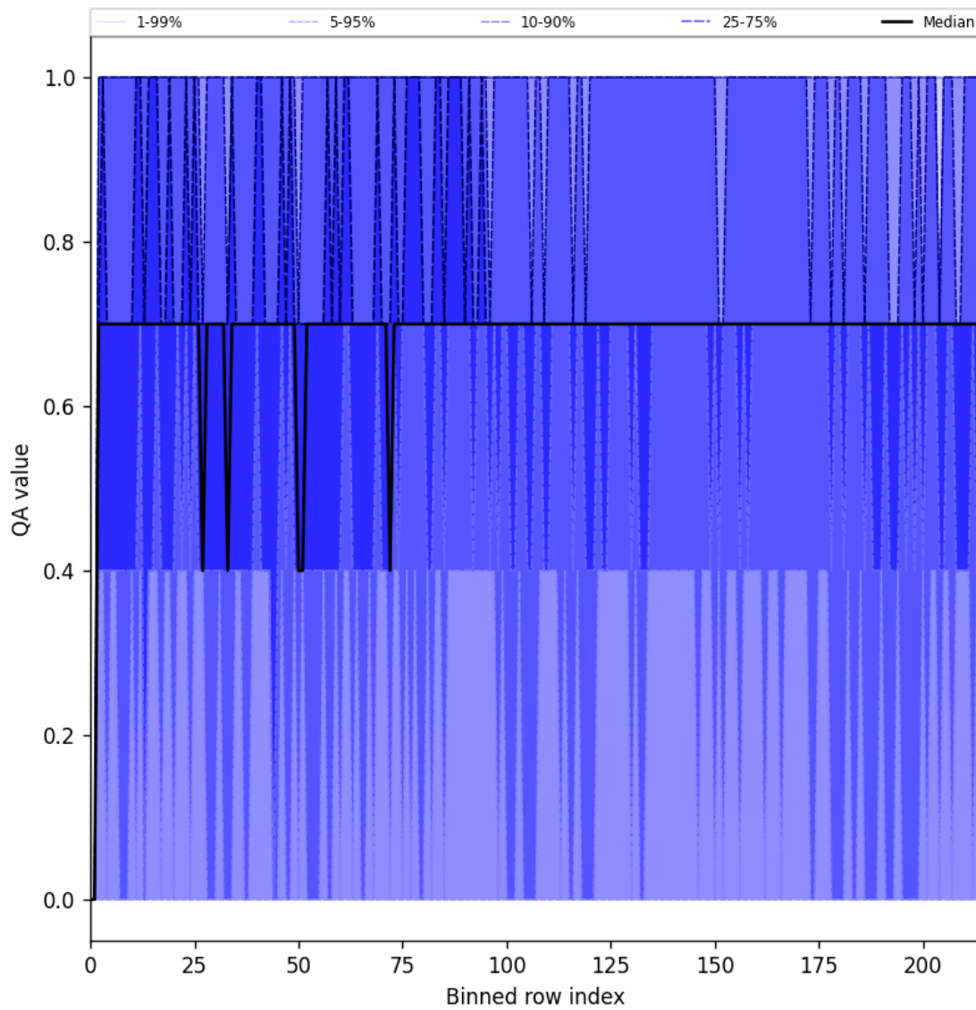
Figure 25: Along track statistics of “QA value” for 2024-12-30 to 2025-01-01
