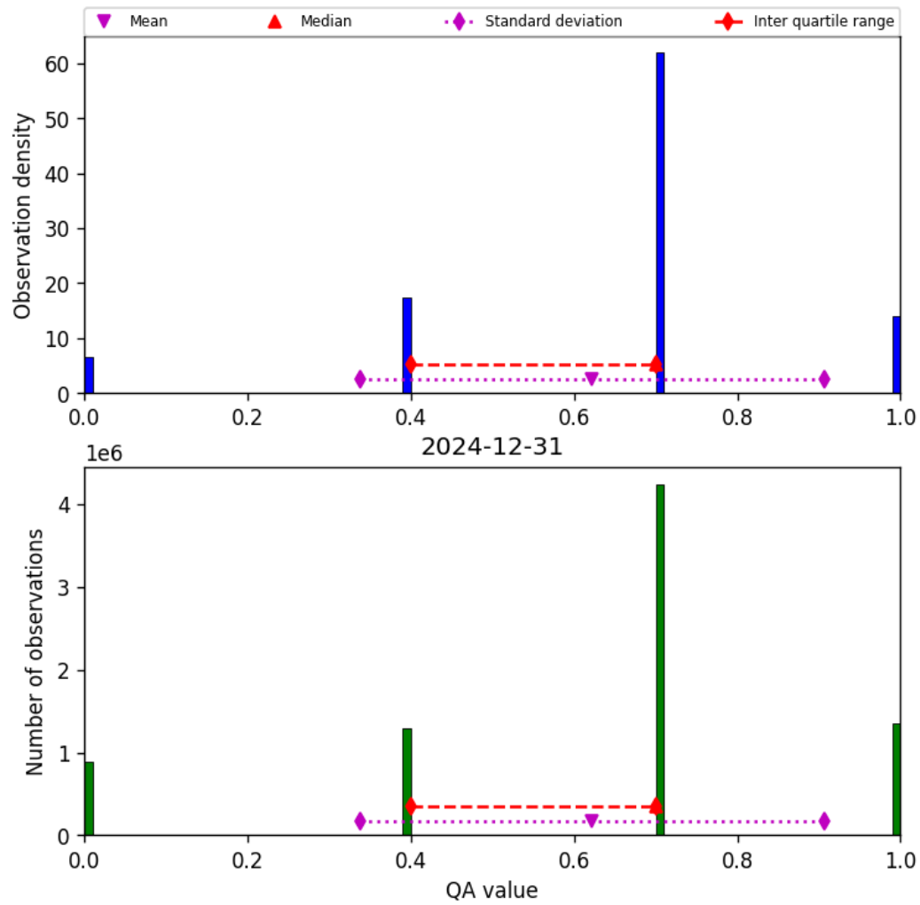
Figure 17: Histogram of “QA value” for 2024-12-30 to 2025-01-01
