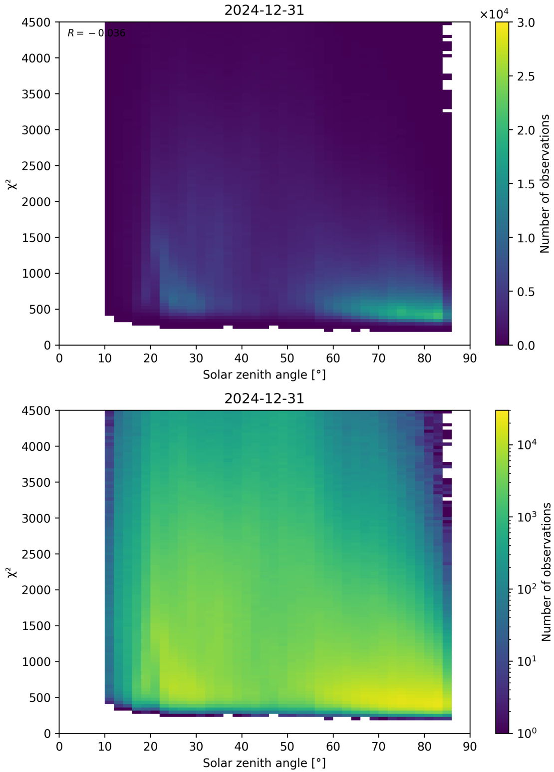
Figure 64: Scatter density plot of “Solar zenith angle” against “ \chi^2 ” for 2024-12-30 to 2025-01-01.
