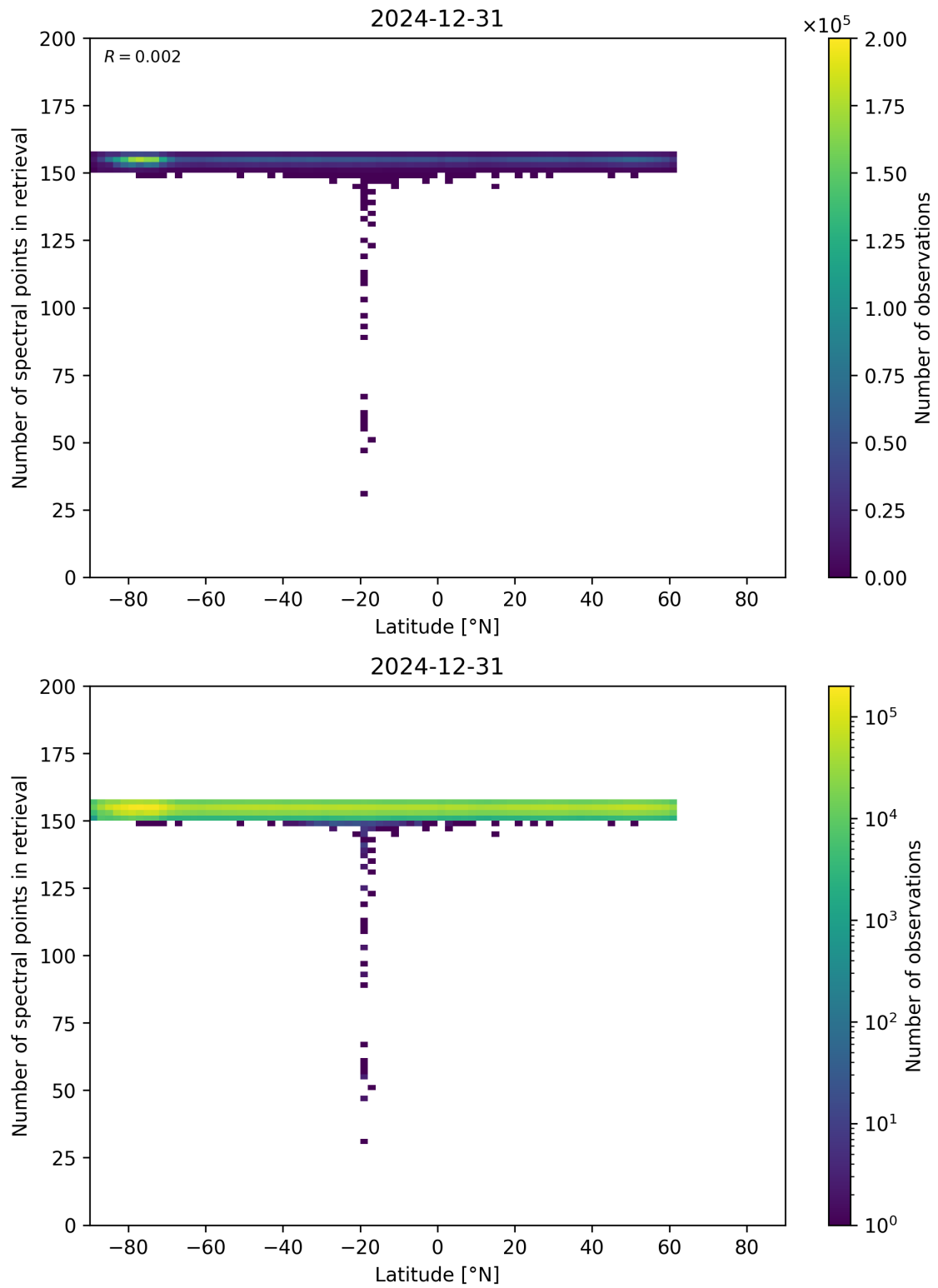
Figure 57: Scatter density plot of “Latitude” against “Number of spectral points in retrieval” for 2024-12-30 to 2025-01-01.
