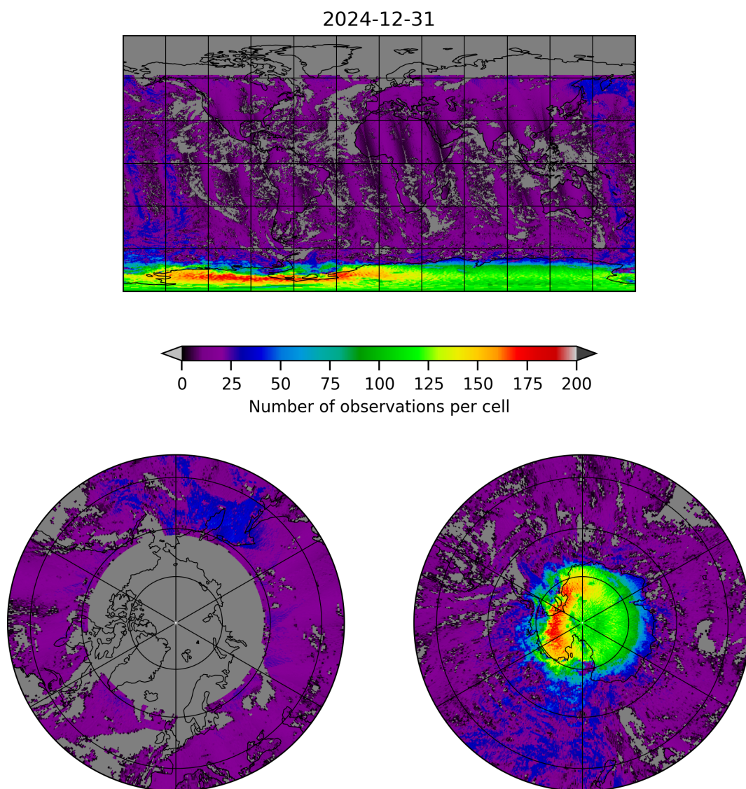
Figure 8: Map of the number of observations for 2024-12-30 to 2025-01-01
