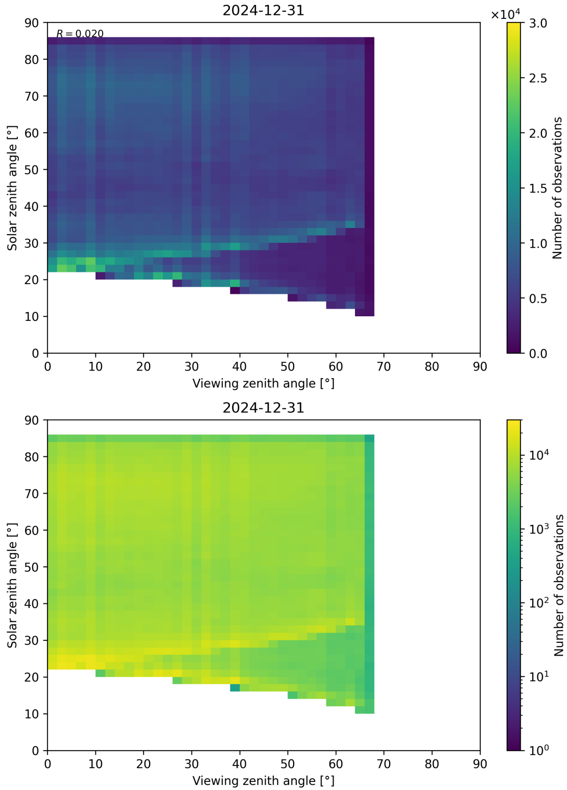
Figure 77: Scatter density plot of “Viewing zenith angle” against “Solar zenith angle” for 2024-12-30 to 2025-01-01.
