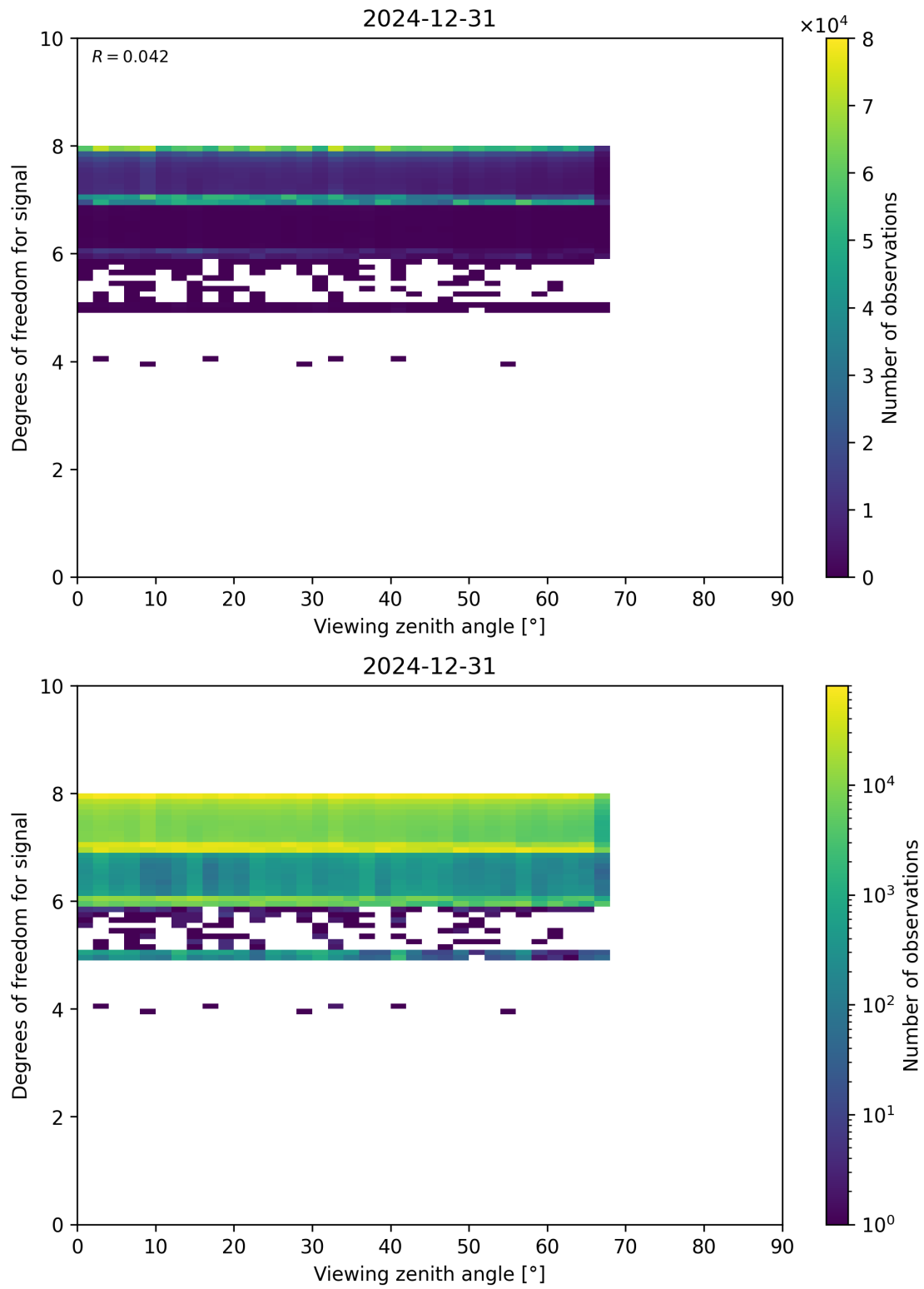
Figure 73: Scatter density plot of “Viewing zenith angle” against “Degrees of freedom for signal” for 2024-12-30 to 2025-01-01.
