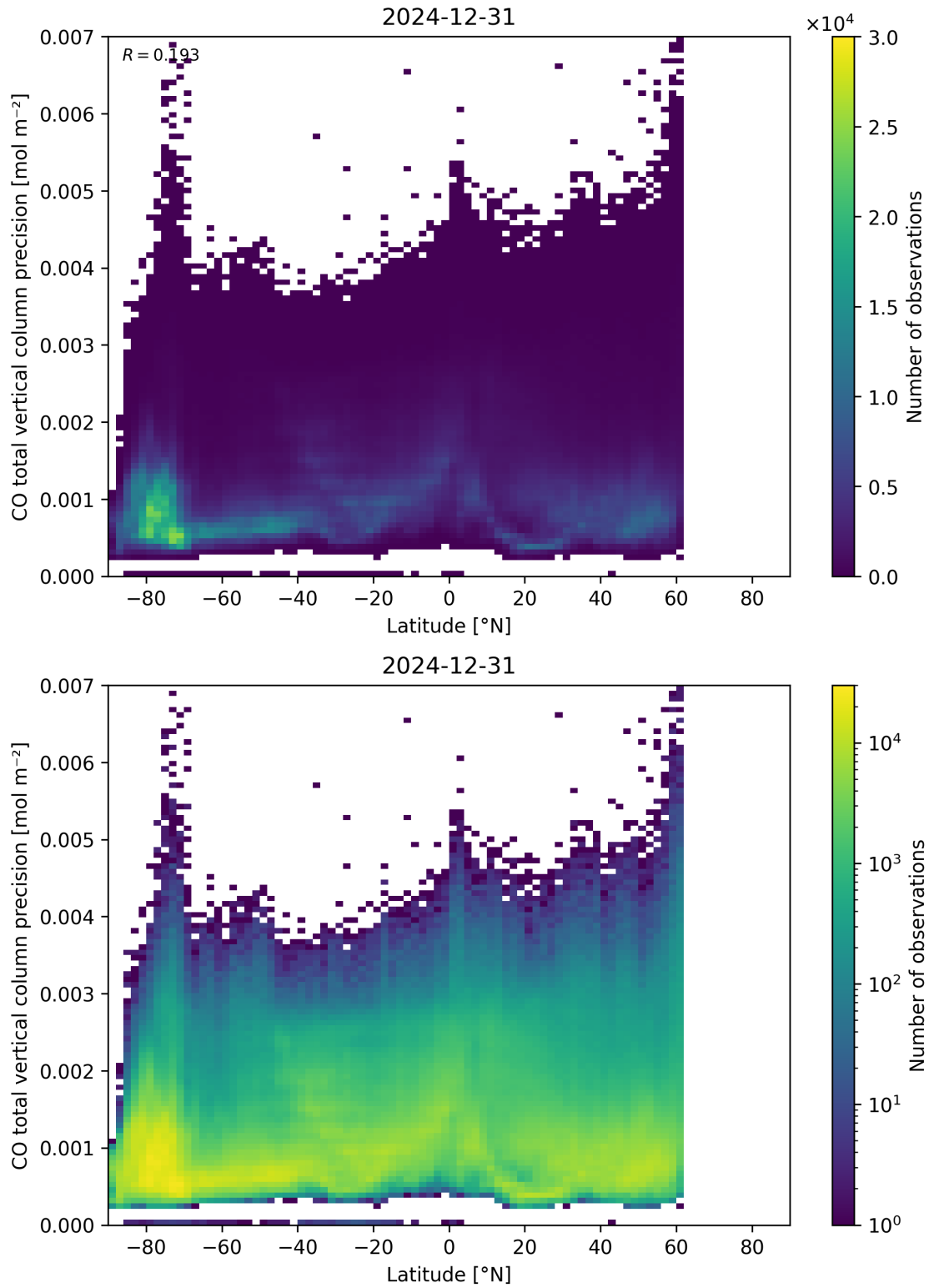
Figure 53: Scatter density plot of “Latitude” against “CO total vertical column precision” for 2024-12-30 to 2025-01-01.
