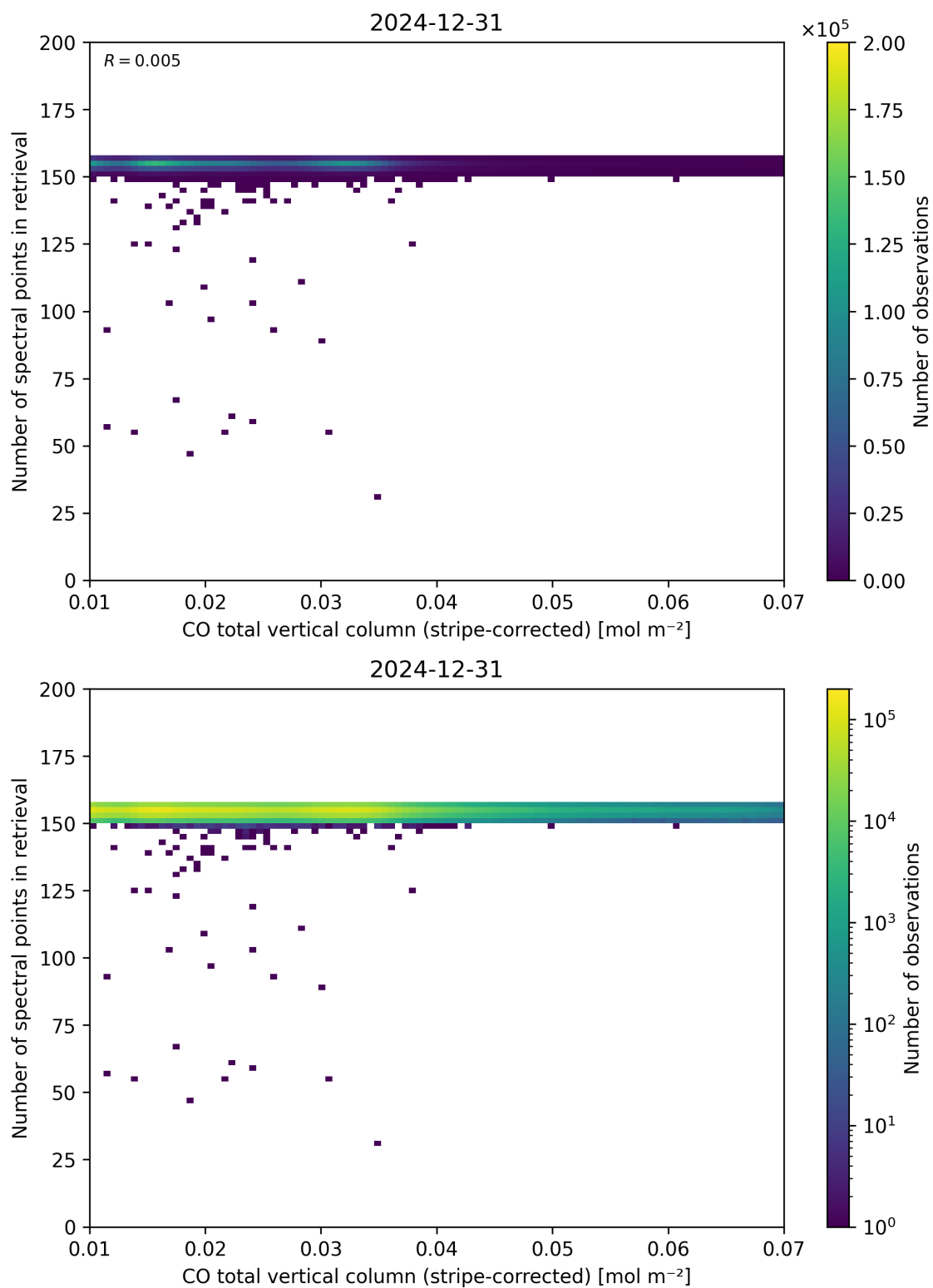
Figure 40: Scatter density plot of “CO total vertical column (stripe-corrected)” against “Number of spectral points in retrieval” for 2024-12-30 to 2025-01-01.
