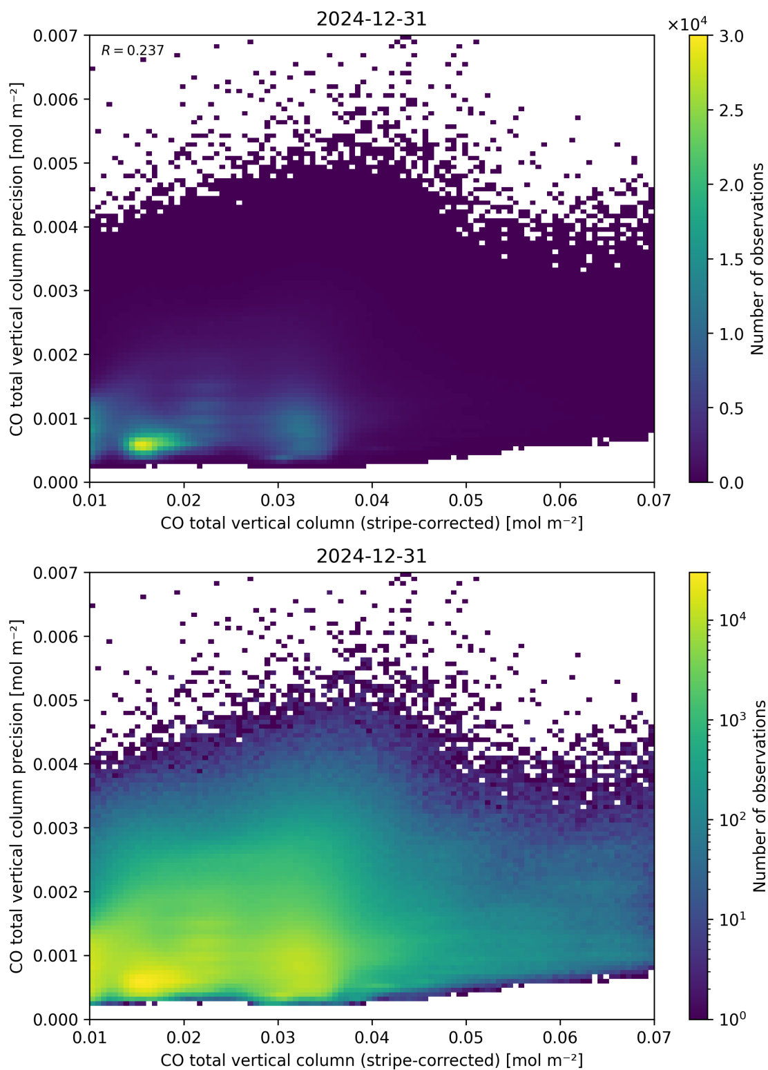
Figure 36: Scatter density plot of “CO total vertical column (stripe-corrected)” against “CO total vertical column precision” for 2024-12-30 to 2025-01-01.
