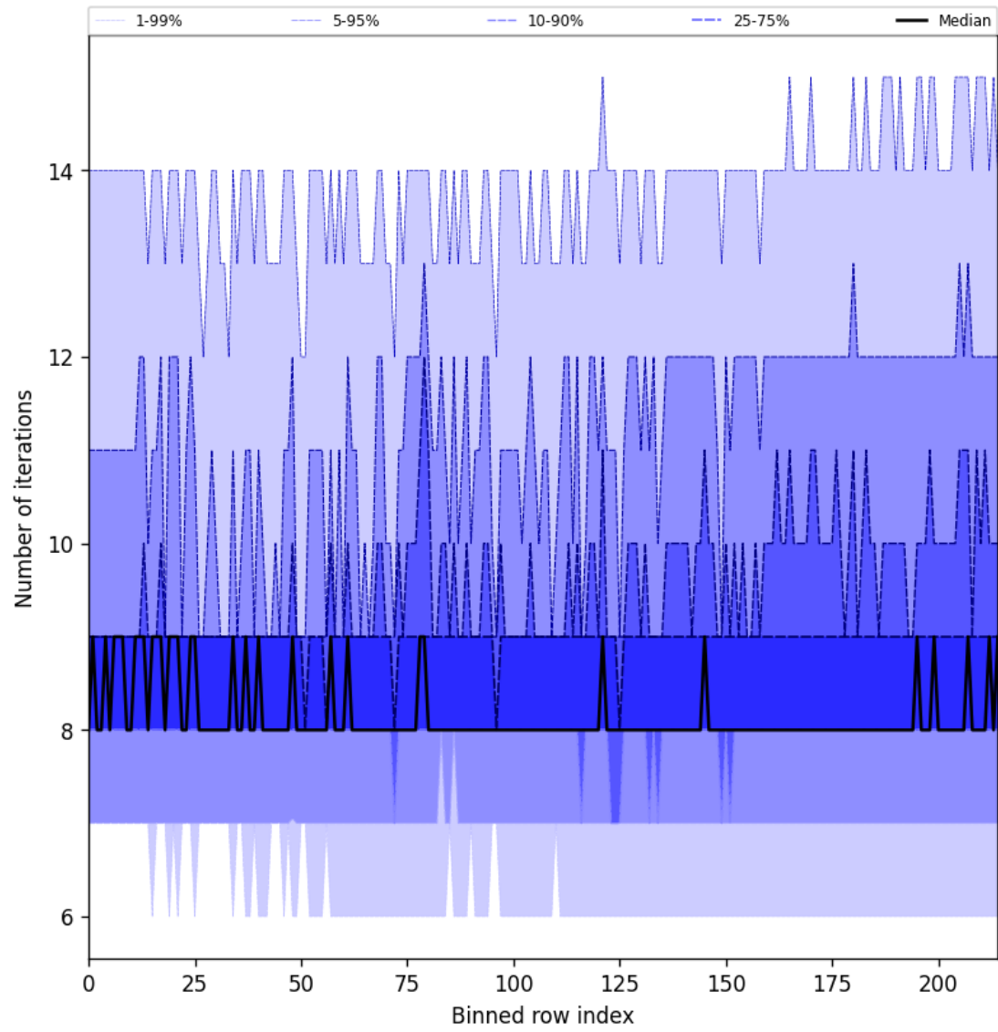
Figure 32: Along track statistics of “Number of iterations” for 2024-12-30 to 2025-01-01
