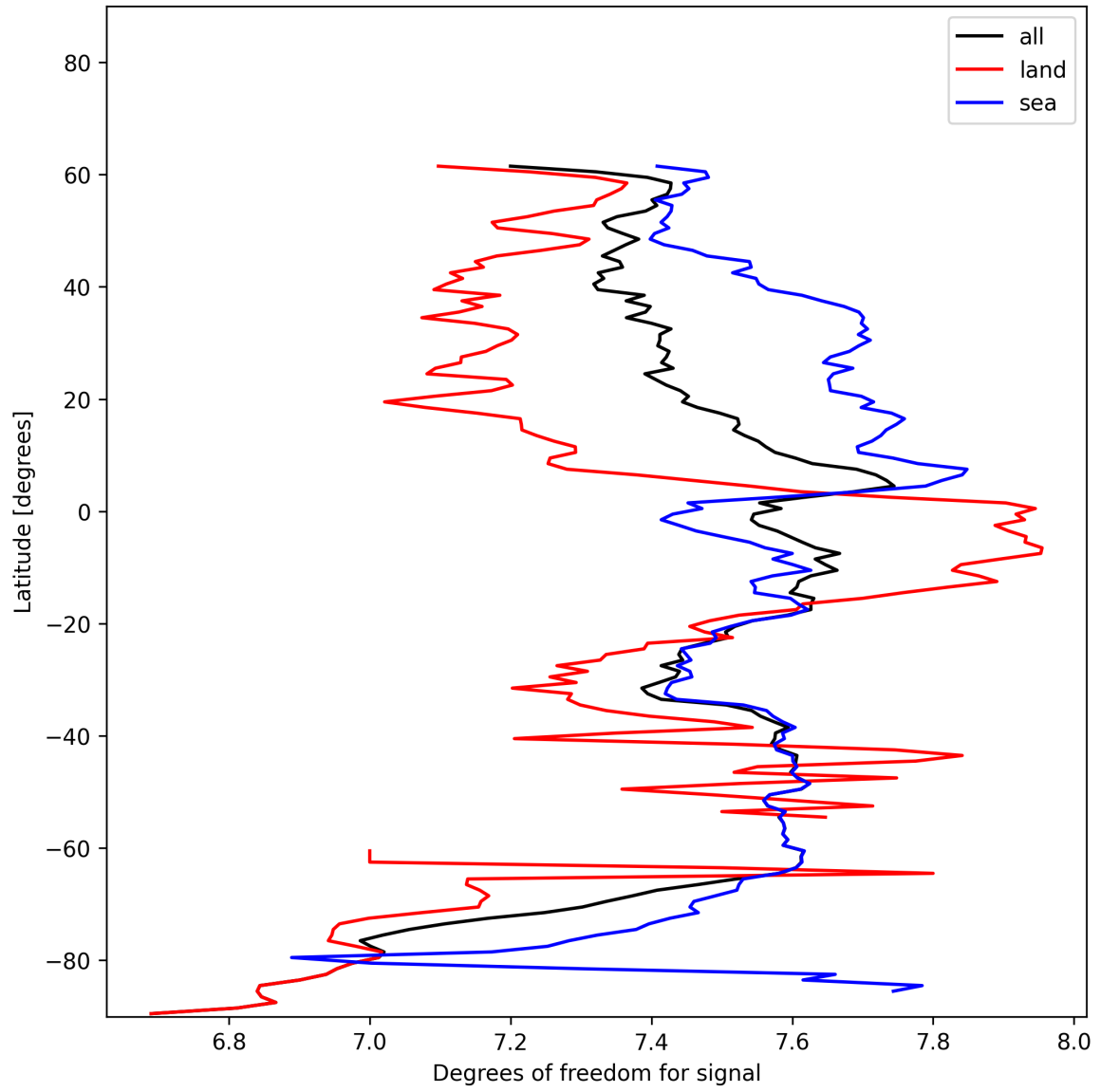
Figure 15: Zonal average of “Degrees of freedom for signal” for 2024-12-30 to 2025-01-01.
