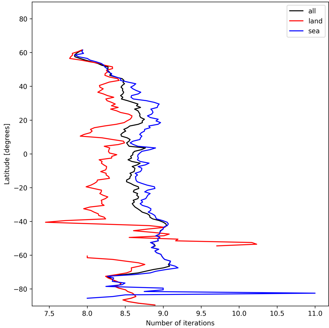
Figure 16: Zonal average of “Number of iterations” for 2024-12-30 to 2025-01-01.
