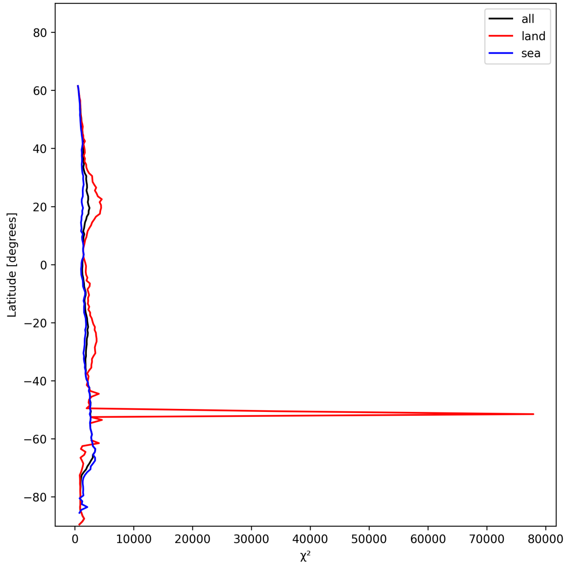
Figure 14: Zonal average of “ \chi^2 ” for 2024-12-30 to 2025-01-01.
