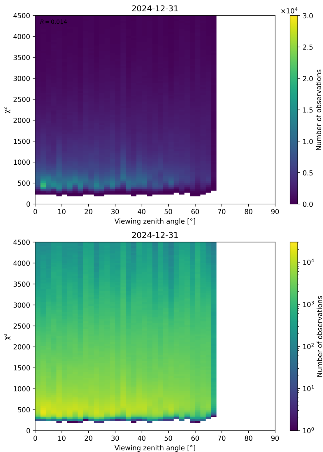
Figure 72: Scatter density plot of “Viewing zenith angle” against “ \chi^2 ” for 2024-12-30 to 2025-01-01.
