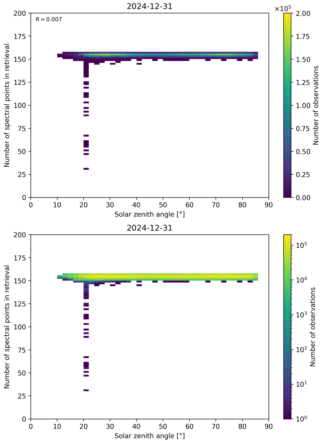
Figure 68: Scatter density plot of “Solar zenith angle” against “Number of spectral points in retrieval” for 2024-12-30 to 2025-01-01.
