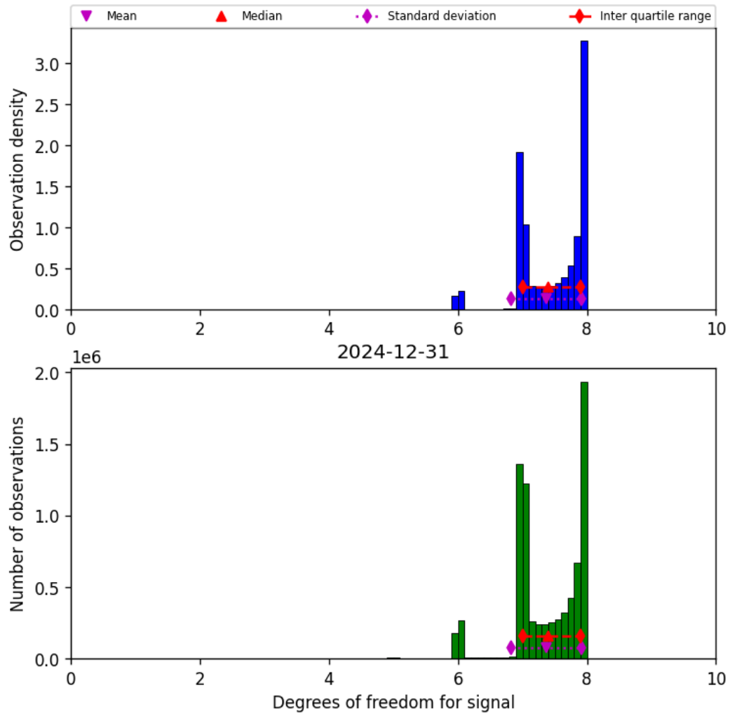
Figure 23: Histogram of “Degrees of freedom for signal” for 2024-12-30 to 2025-01-01
