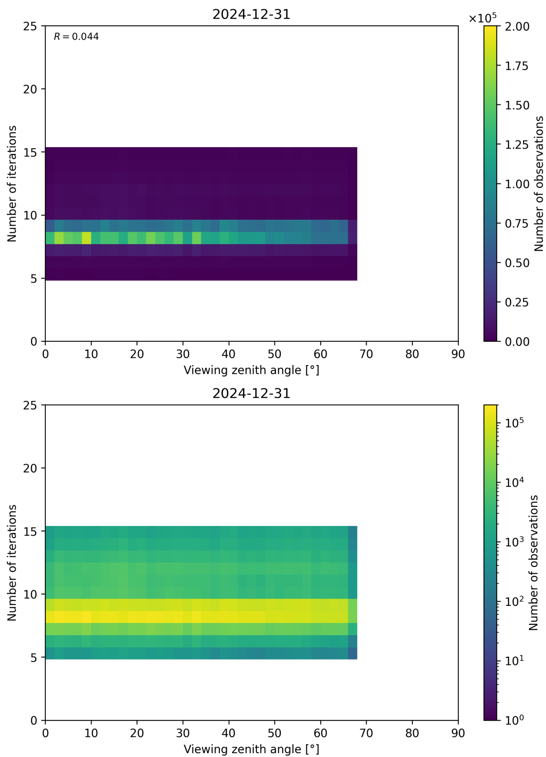
Figure 75: Scatter density plot of “Viewing zenith angle” against “Number of iterations” for 2024-12-30 to 2025-01-01.
