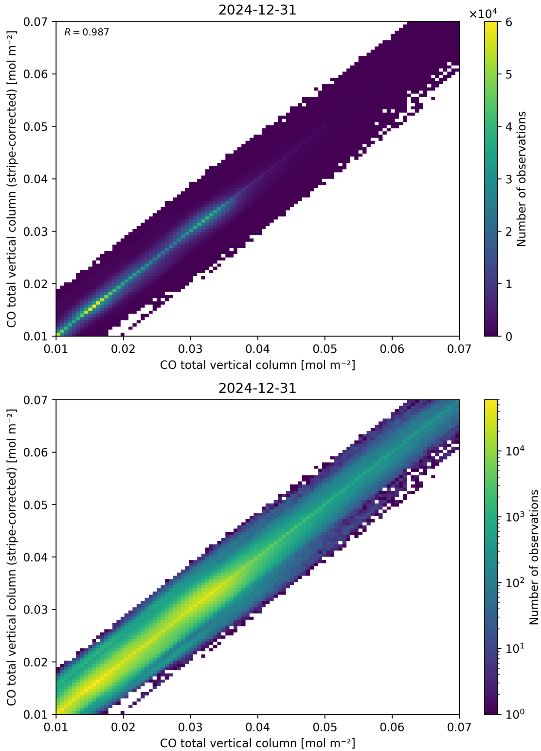
Figure 33: Scatter density plot of “CO total vertical column” against “CO total vertical column (stripe-corrected)” for 2024-12-30 to 2025-01-01.
