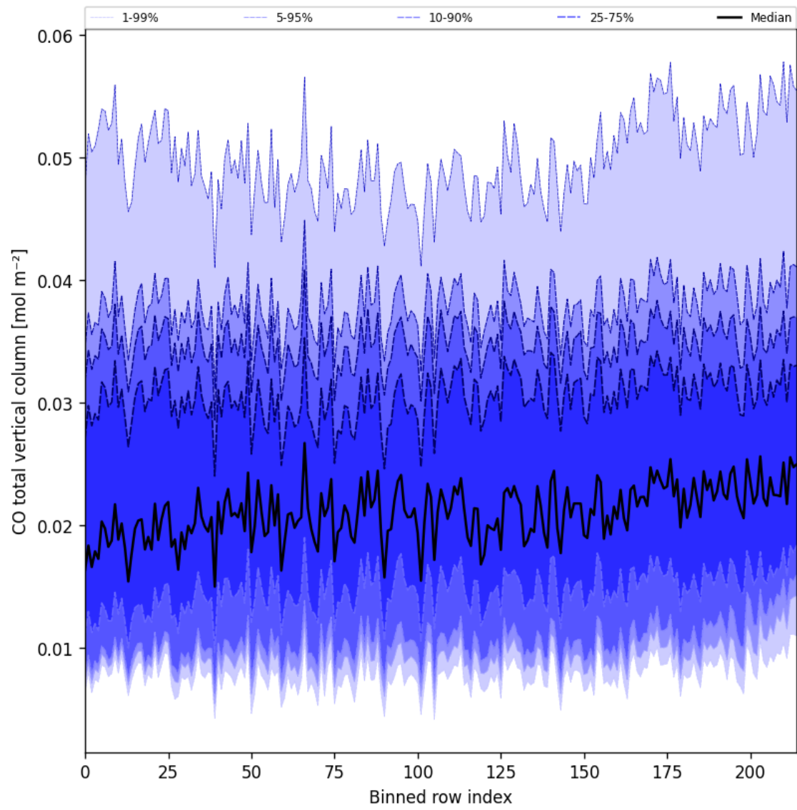
Figure 26: Along track statistics of “CO total vertical column” for 2024-12-30 to 2025-01-01
