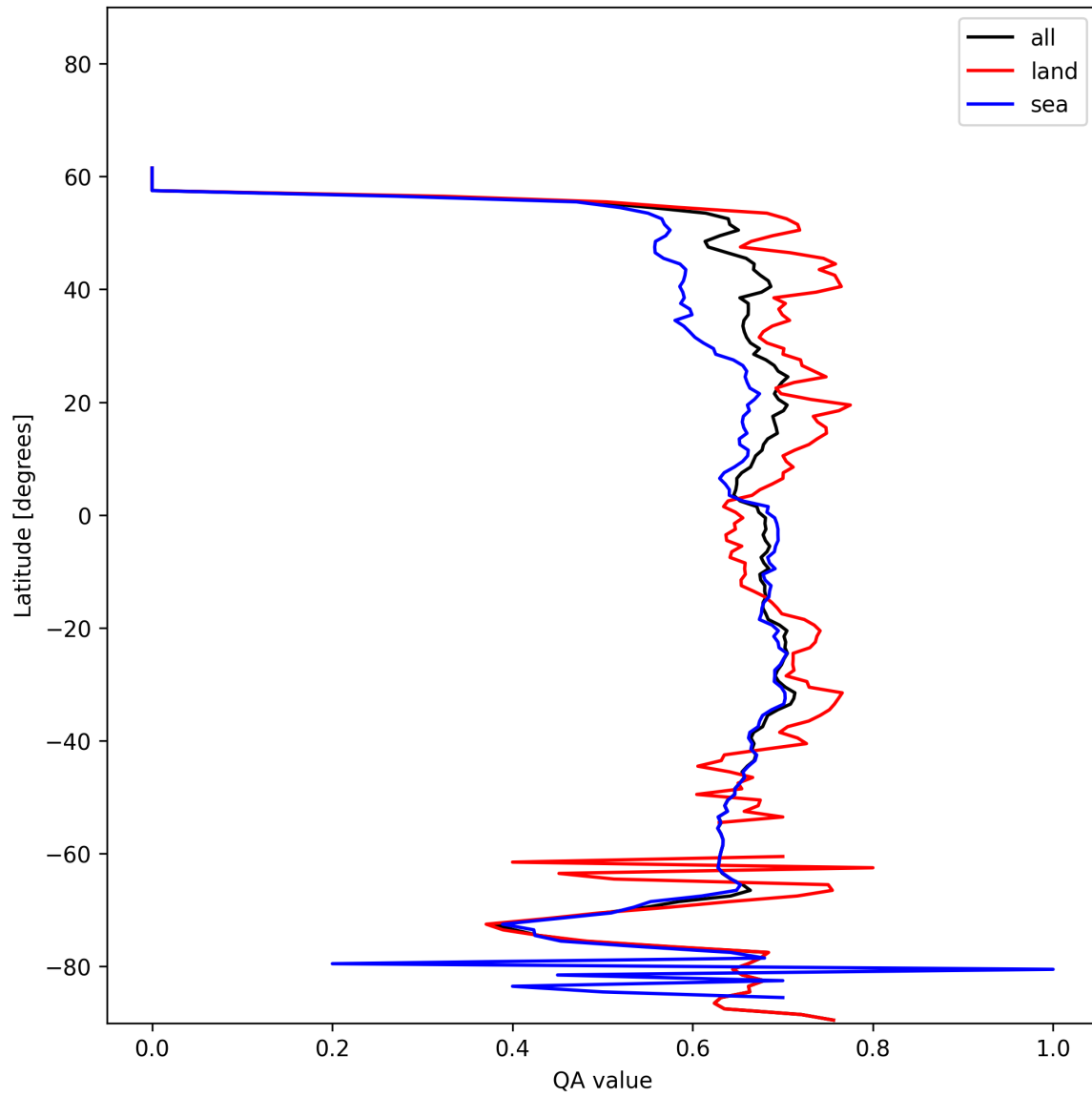
Figure 9: Zonal average of “QA value” for 2024-12-30 to 2025-01-01.
