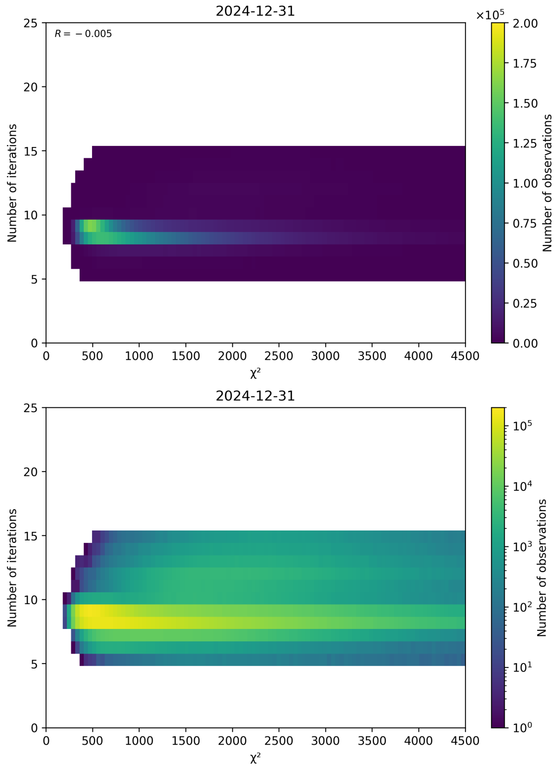
Figure 49: Scatter density plot of “ \chi^2 ” against “Number of iterations” for 2024-12-30 to 2025-01-01.
