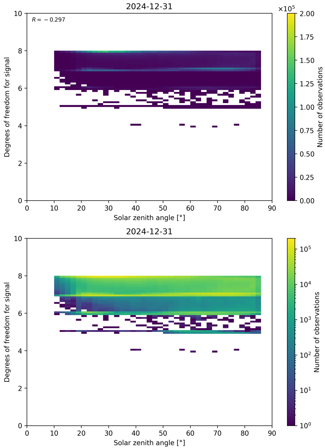
Figure 65: Scatter density plot of “Solar zenith angle” against “Degrees of freedom for signal” for 2024-12-30 to 2025-01-01.
