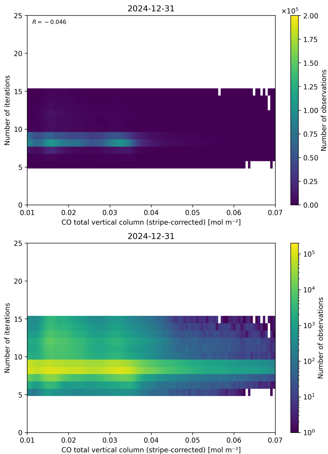
Figure 39: Scatter density plot of “CO total vertical column (stripe-corrected)” against “Number of iterations” for 2024-12-30 to 2025-01-01.
