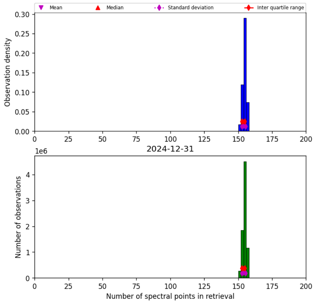
Figure 21: Histogram of “Number of spectral points in retrieval” for 2024-12-30 to 2025-01-01
