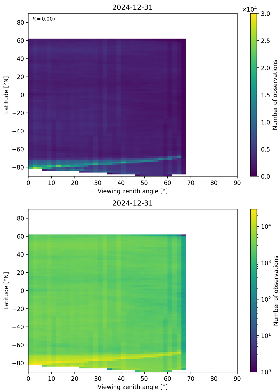
Figure 74: Scatter density plot of “Viewing zenith angle” against “Latitude” for 2024-12-30 to 2025-01-01.
