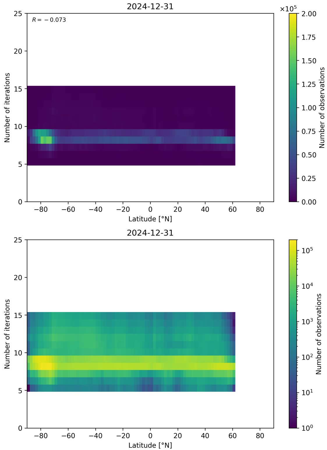
Figure 56: Scatter density plot of “Latitude” against “Number of iterations” for 2024-12-30 to 2025-01-01.
