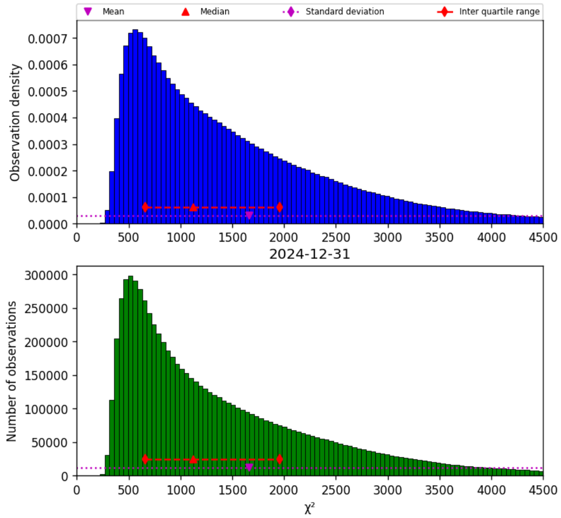
Figure 22: Histogram of " \chi^2 " for 2024-12-30 to 2025-01-01
