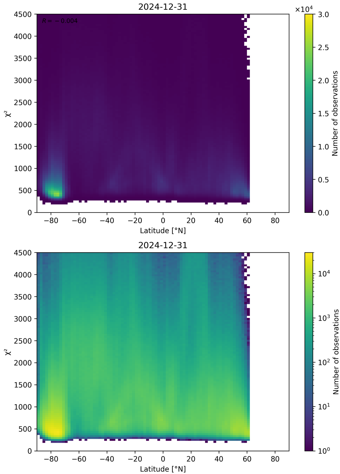
Figure 54: Scatter density plot of “Latitude” against “ \chi^2 ” for 2024-12-30 to 2025-01-01.
