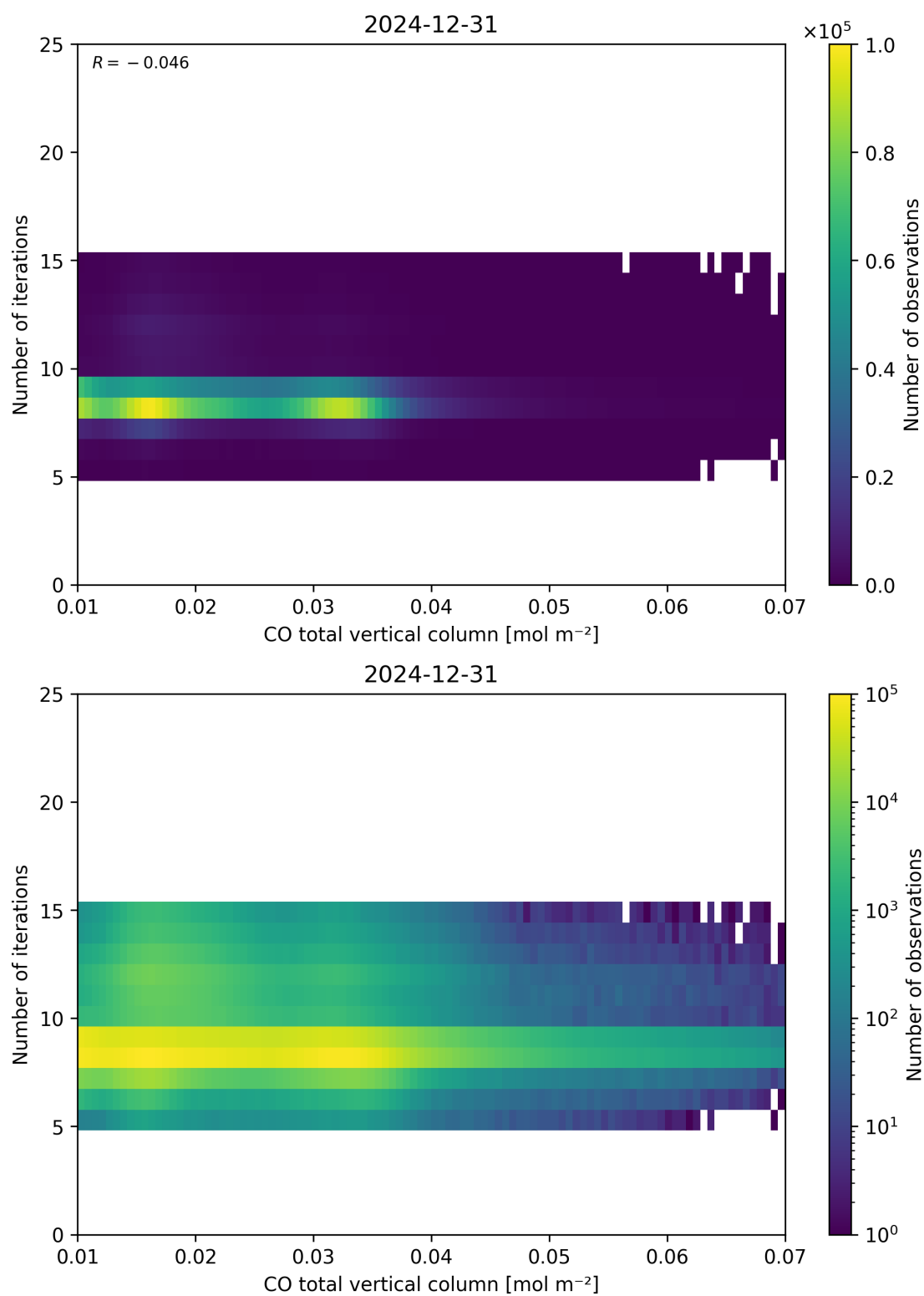
Figure 42: Scatter density plot of “CO total vertical column” against “Number of iterations” for 2024-12-30 to 2025-01-01.
