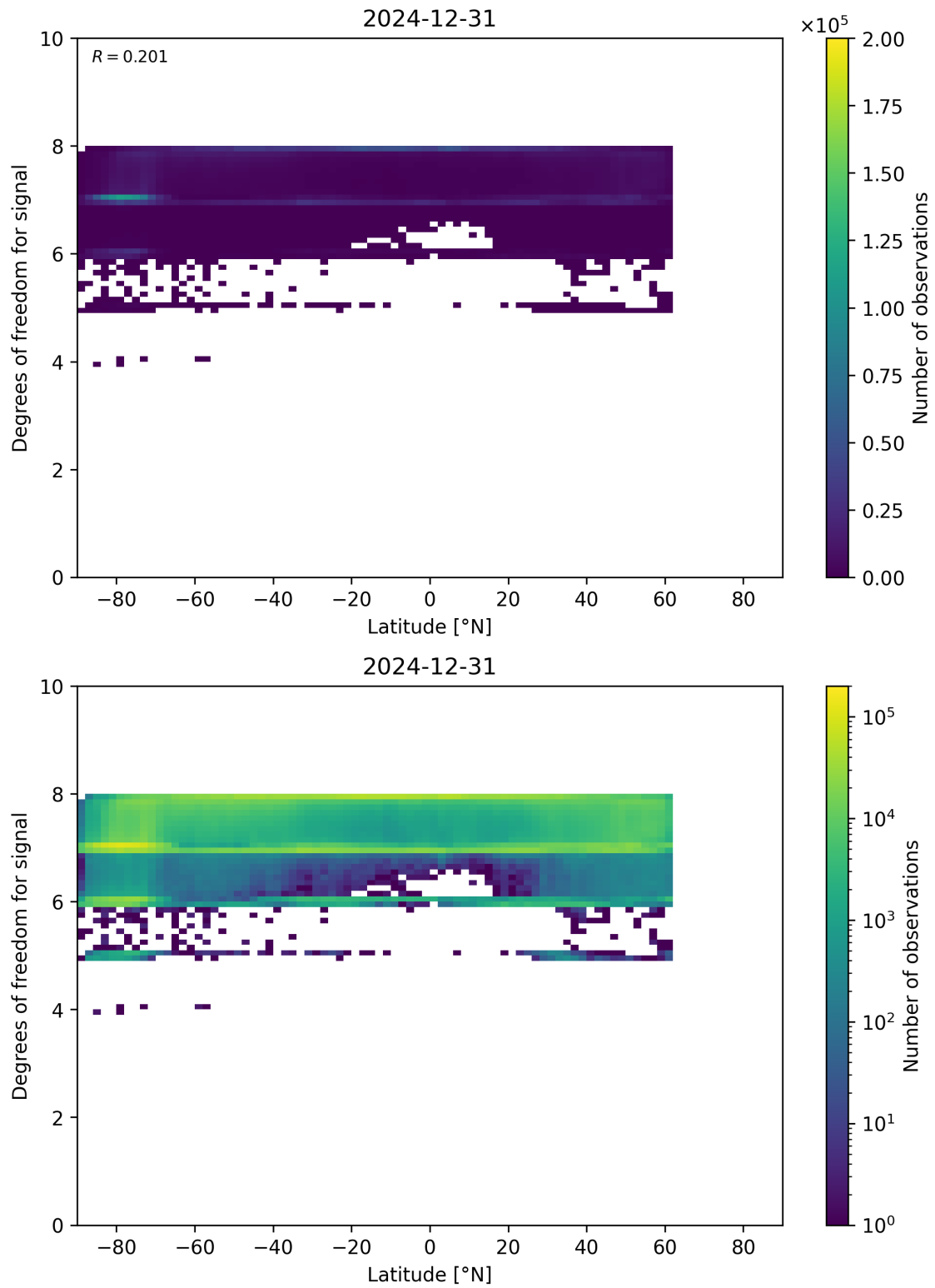
Figure 55: Scatter density plot of “Latitude” against “Degrees of freedom for signal” for 2024-12-30 to 2025-01-01.
