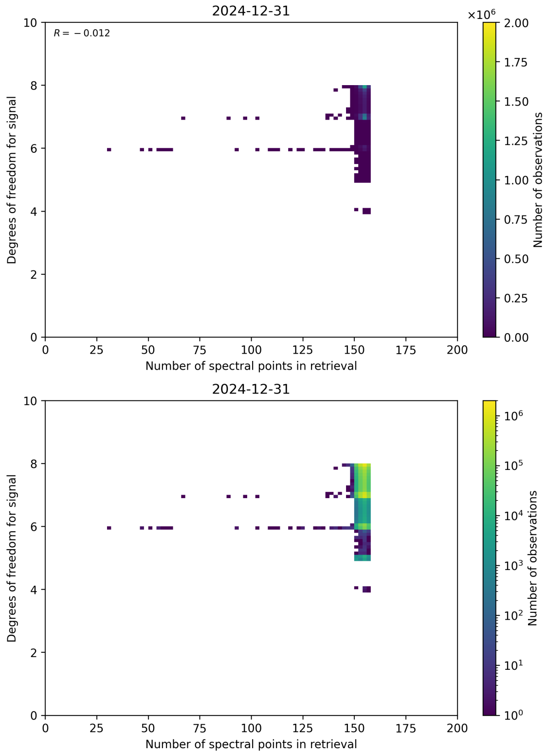
Figure 59: Scatter density plot of “Number of spectral points in retrieval” against “Degrees of freedom for signal” for 2024-12-30 to 2025-01-01.
