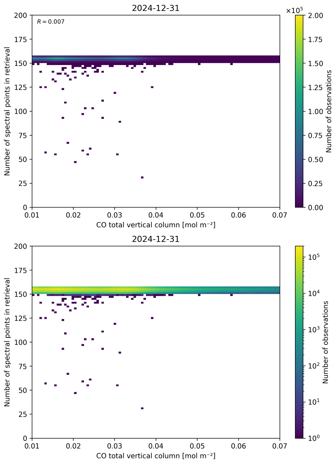
Figure 43: Scatter density plot of “CO total vertical column” against “Number of spectral points in retrieval” for 2024-12-30 to 2025-01-01.
