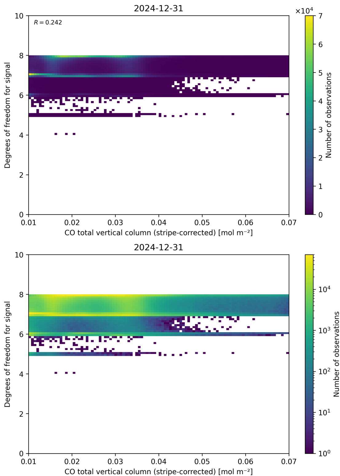
Figure 38: Scatter density plot of “CO total vertical column (stripe-corrected)” against “Degrees of freedom for signal” for 2024-12-30 to 2025-01-01.
