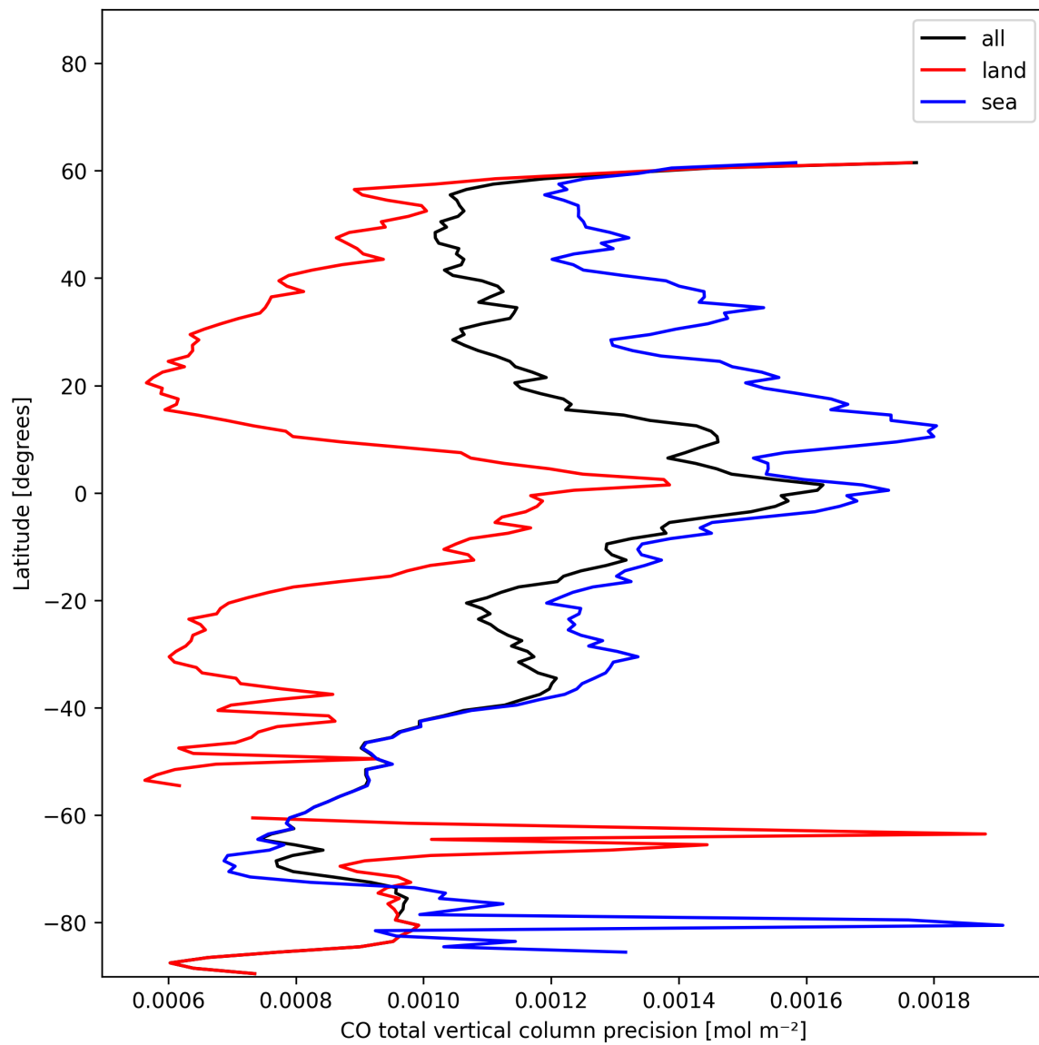
Figure 12: Zonal average of “CO total vertical column precision” for 2024-12-30 to 2025-01-01.
