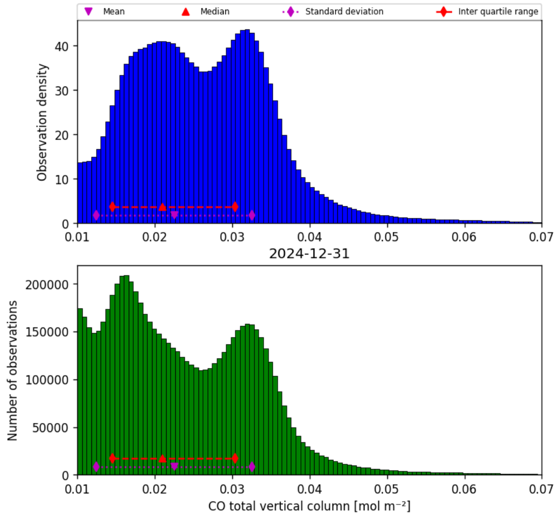
Figure 18: Histogram of “CO total vertical column” for 2024-12-30 to 2025-01-01
