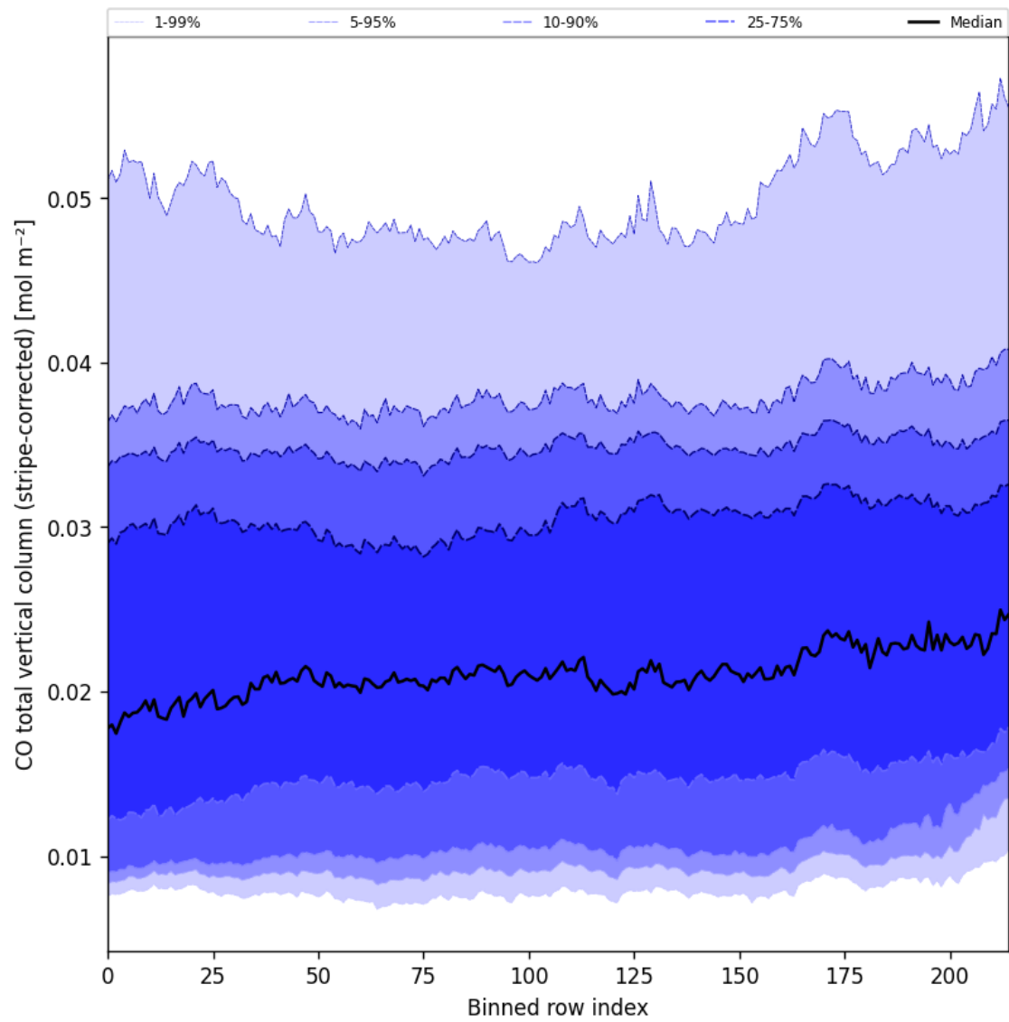
Figure 27: Along track statistics of “CO total vertical column (stripe-corrected)” for 2024-12-30 to 2025-01-01
