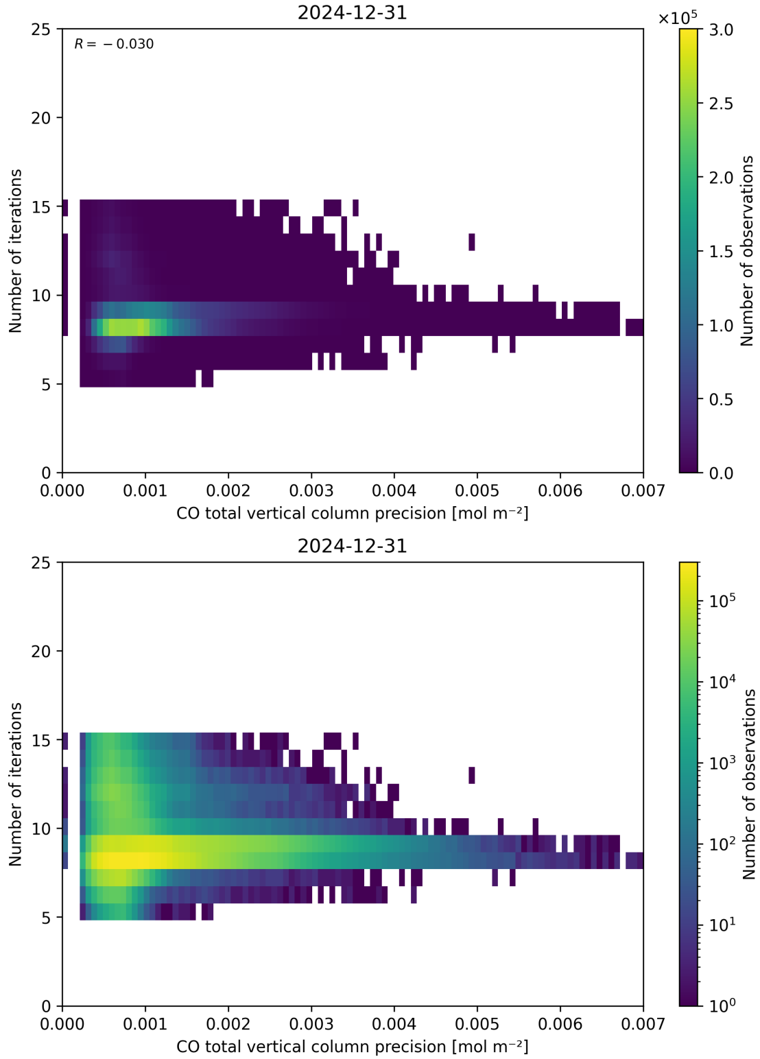
Figure 46: Scatter density plot of “CO total vertical column precision” against “Number of iterations” for 2024-12-30 to 2025-01-01.
