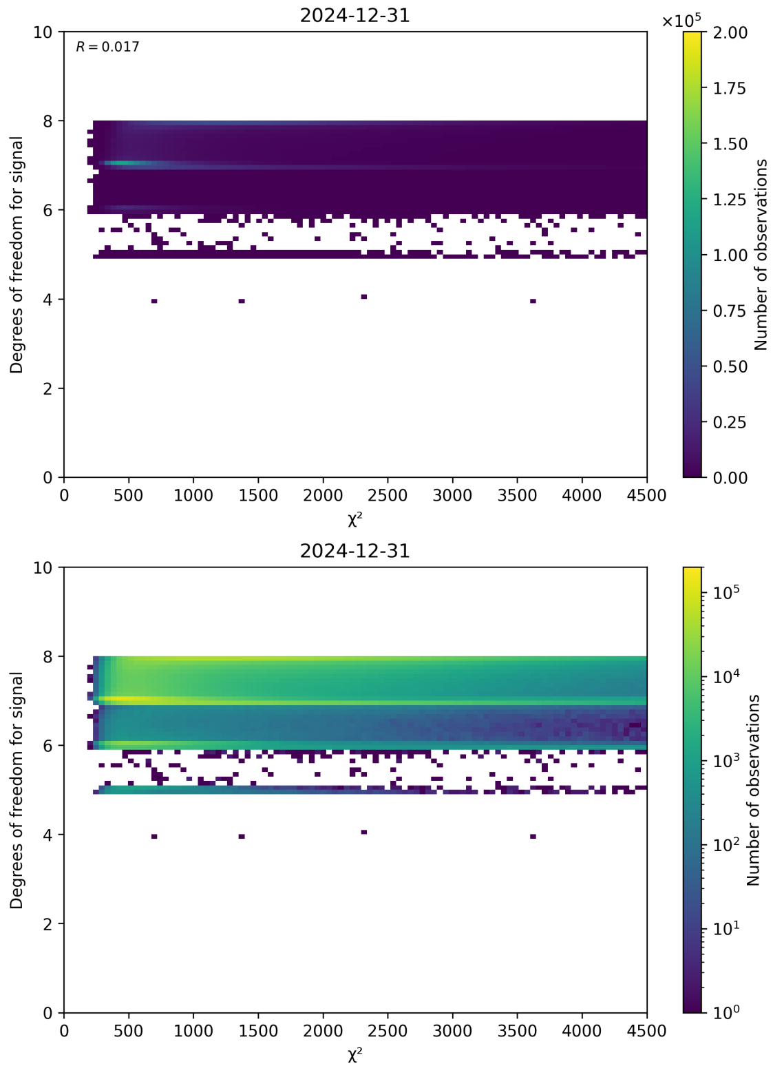
Figure 48: Scatter density plot of “ \chi^2 ” against “Degrees of freedom for signal” for 2024-12-30 to 2025-01-01.
