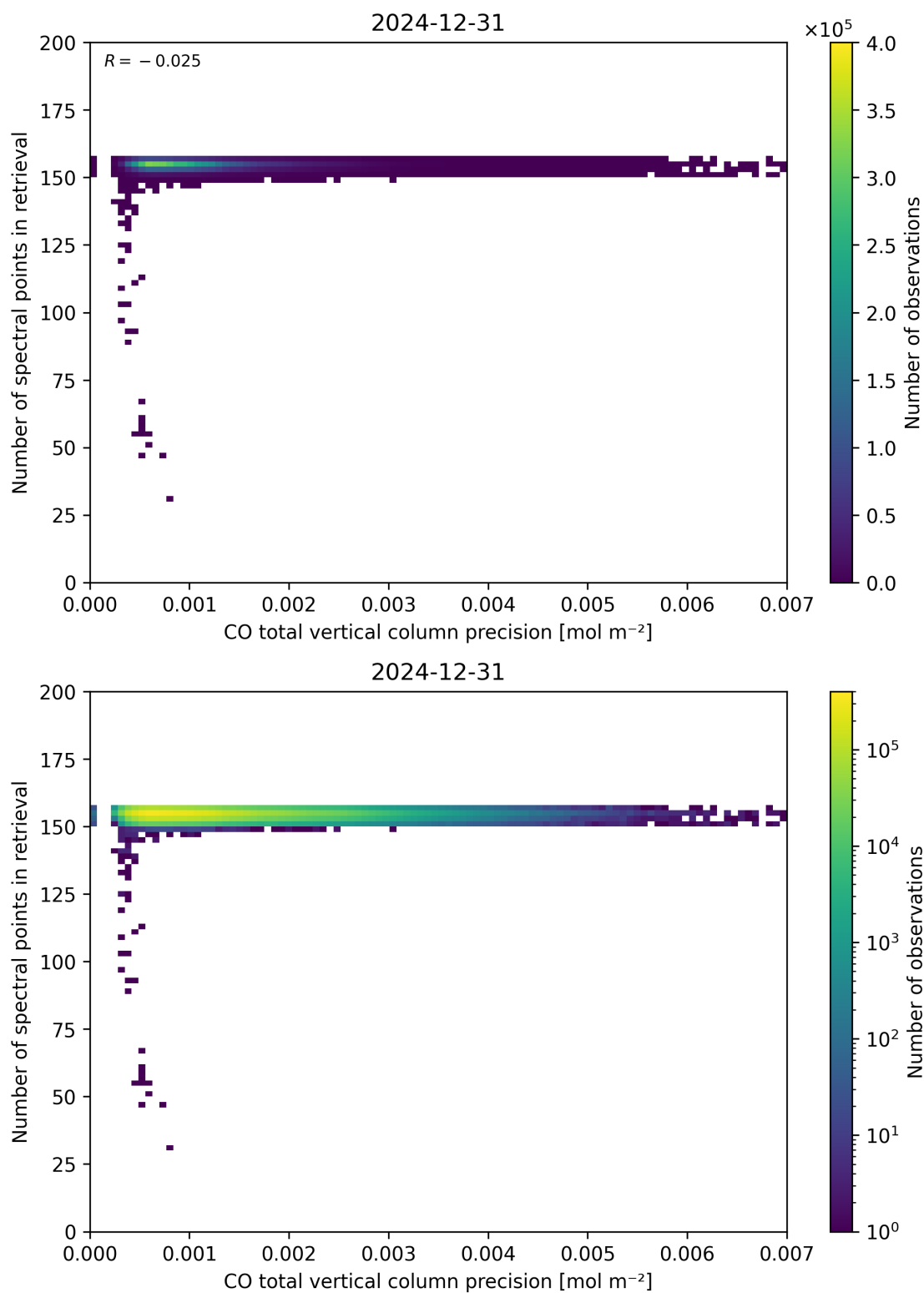
Figure 47: Scatter density plot of “CO total vertical column precision” against “Number of spectral points in retrieval” for 2024-12-30 to 2025-01-01.
