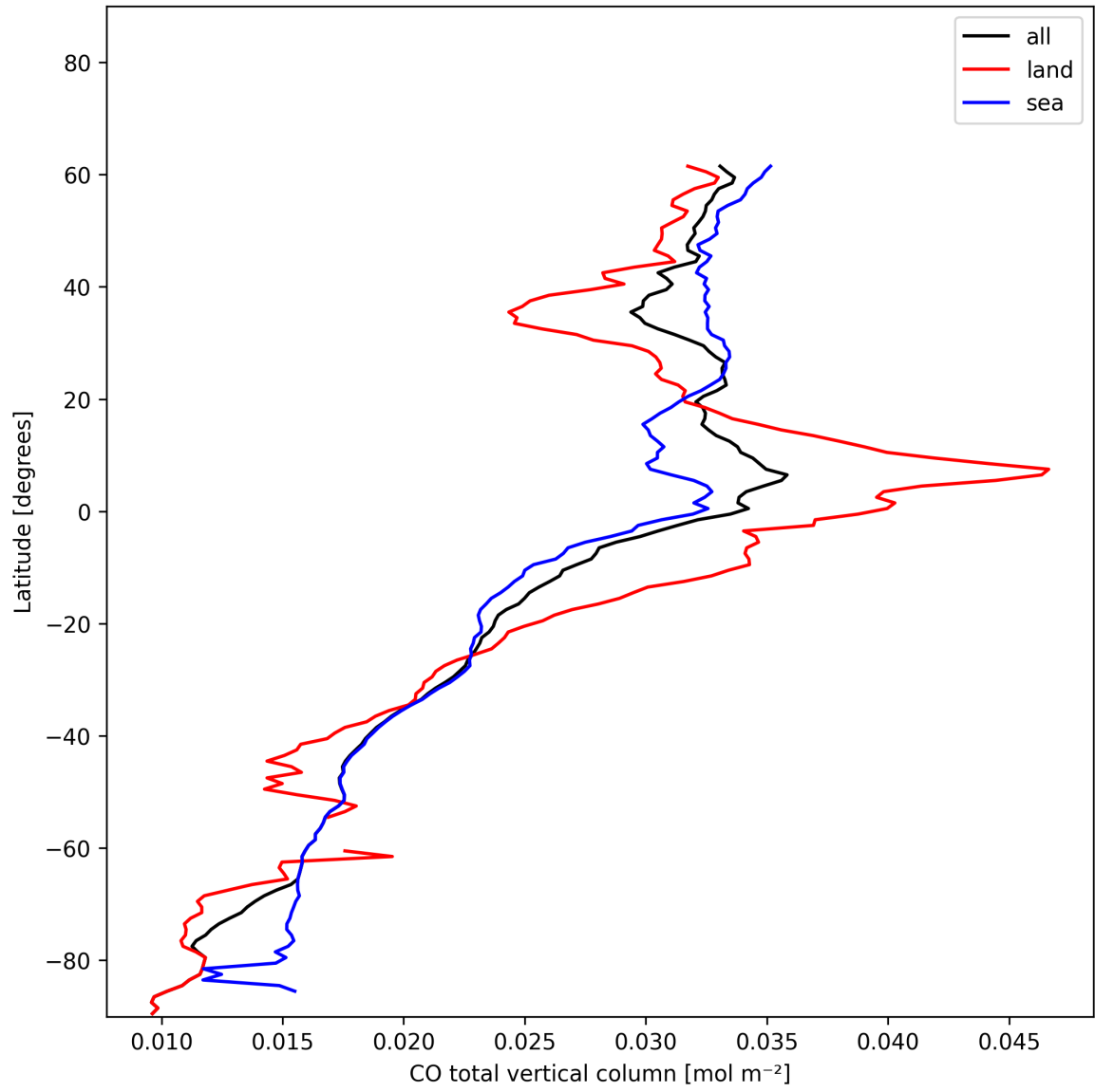
Figure 10: Zonal average of “CO total vertical column” for 2024-12-30 to 2025-01-01.
