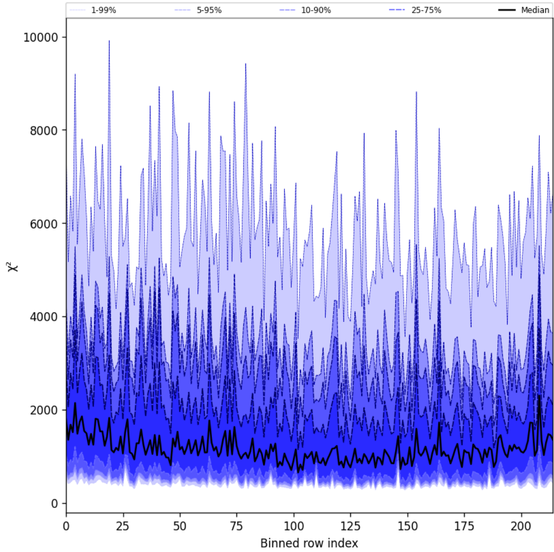
Figure 30: Along track statistics of “ \chi^2 ” for 2024-12-30 to 2025-01-01
