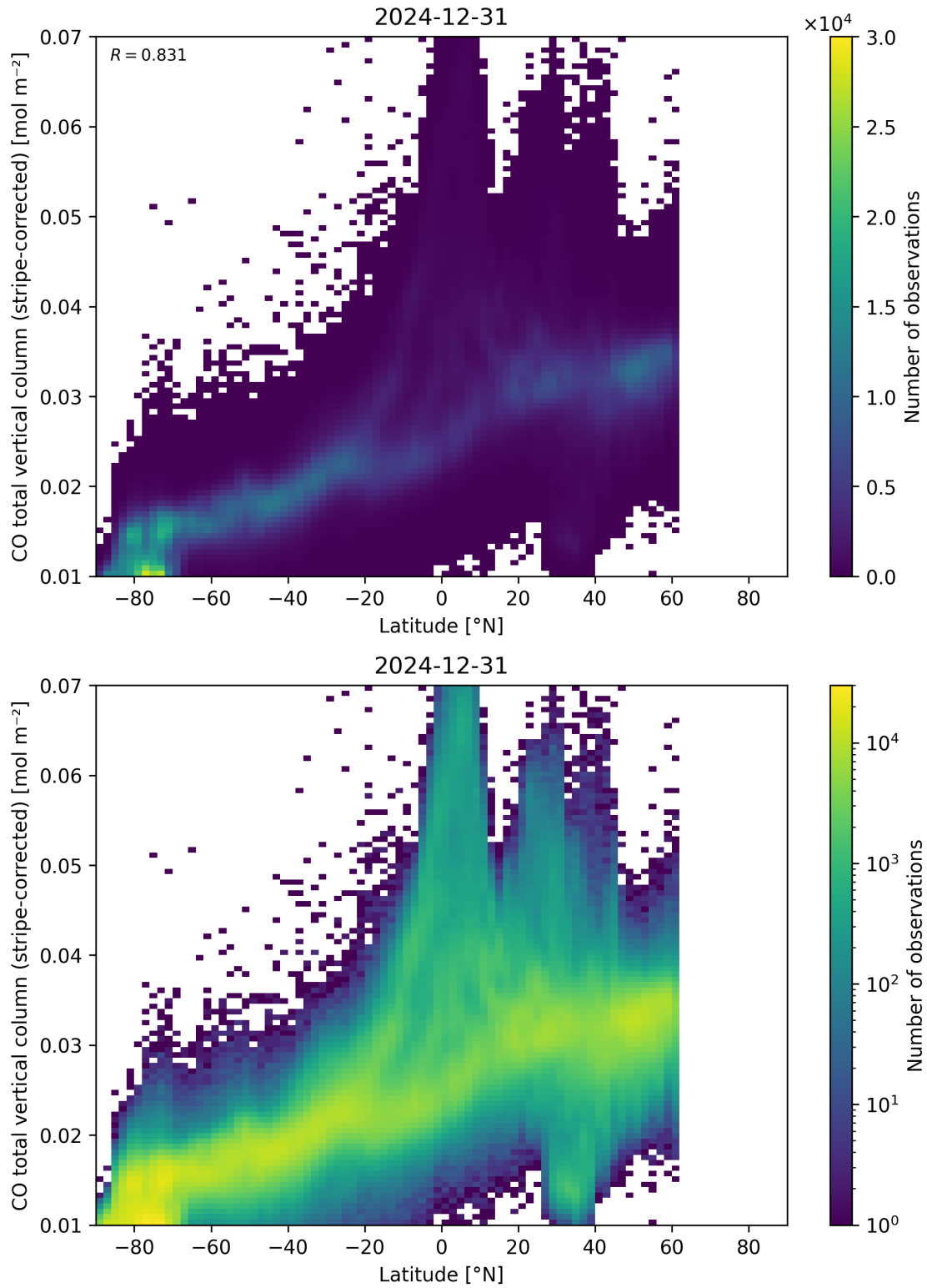
Figure 52: Scatter density plot of “Latitude” against “CO total vertical column (stripe-corrected)” for 2024-12-30 to 2025-01-01.
