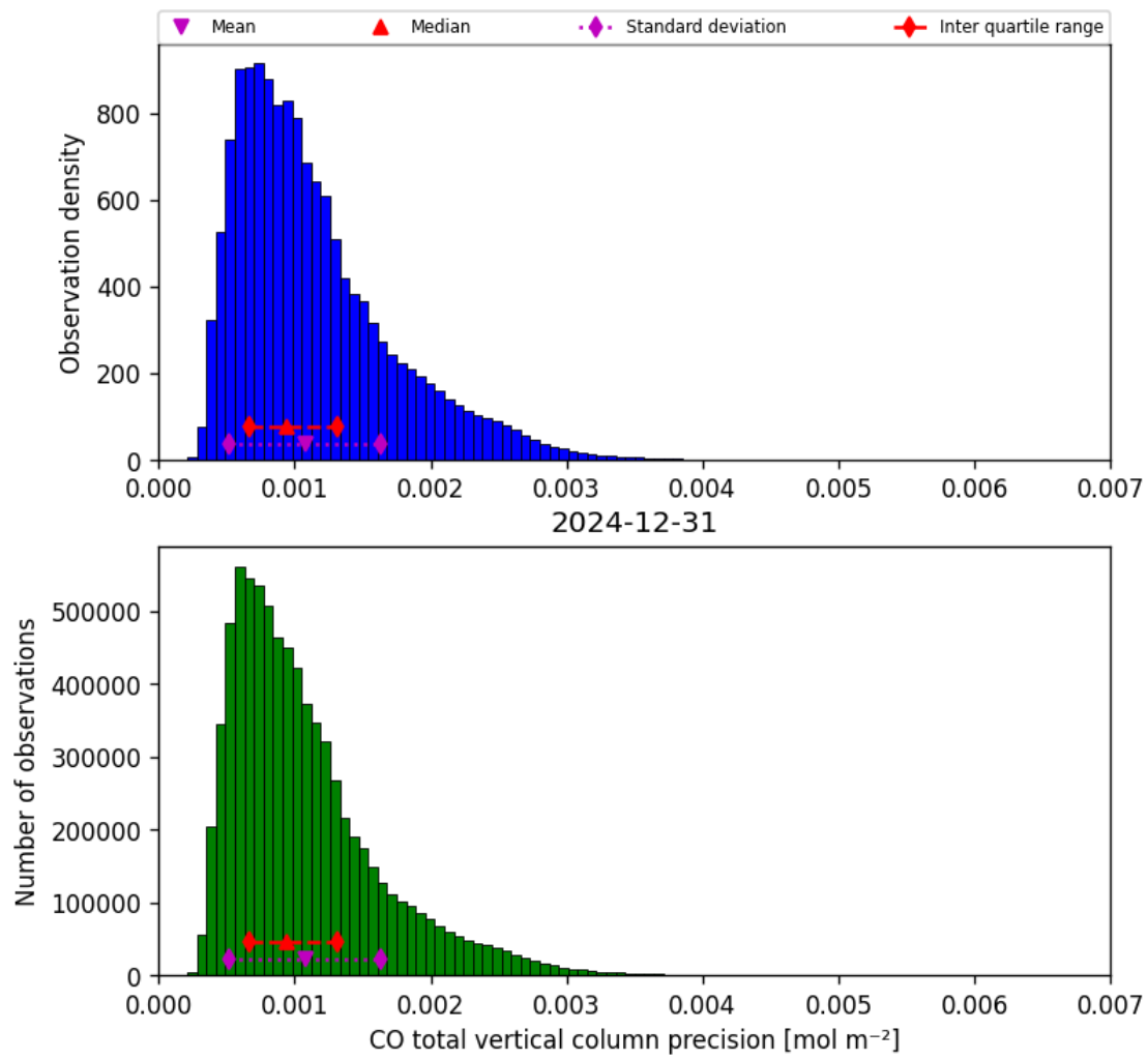
Figure 20: Histogram of “CO total vertical column precision” for 2024-12-30 to 2025-01-01
