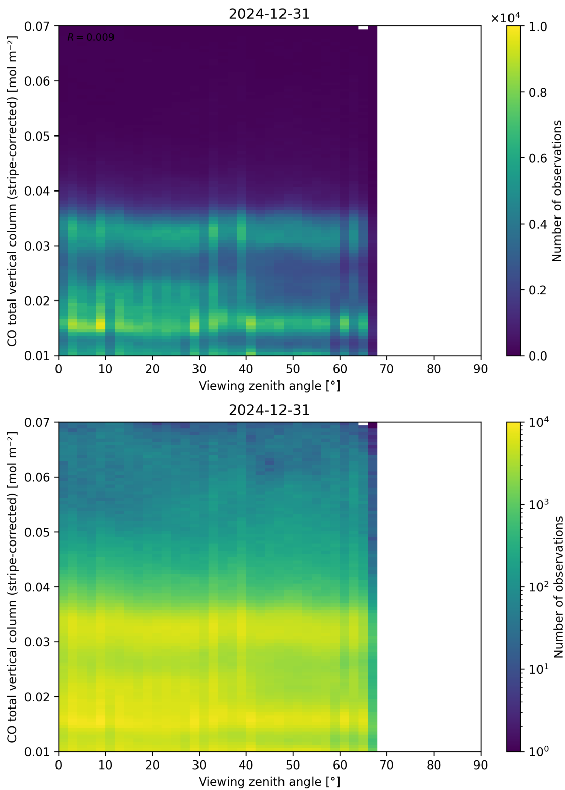
Figure 70: Scatter density plot of “Viewing zenith angle” against “CO total vertical column (stripe-corrected)” for 2024-12-30 to 2025-01-01.
