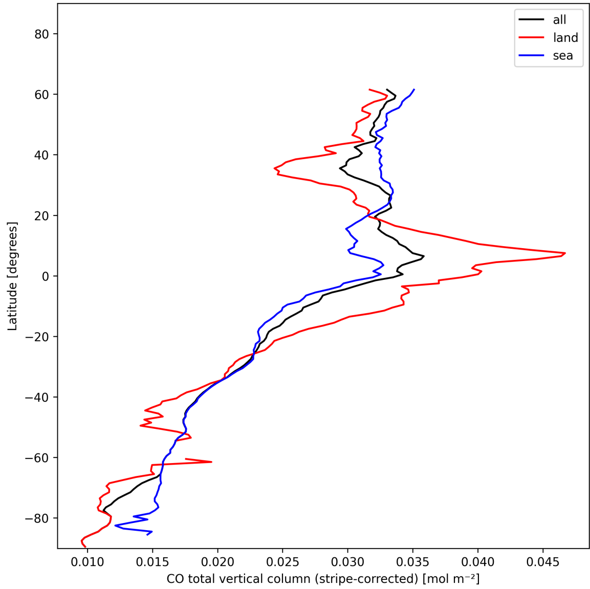
Figure 11: Zonal average of “CO total vertical column (stripe-corrected)” for 2024-12-30 to 2025-01-01.
