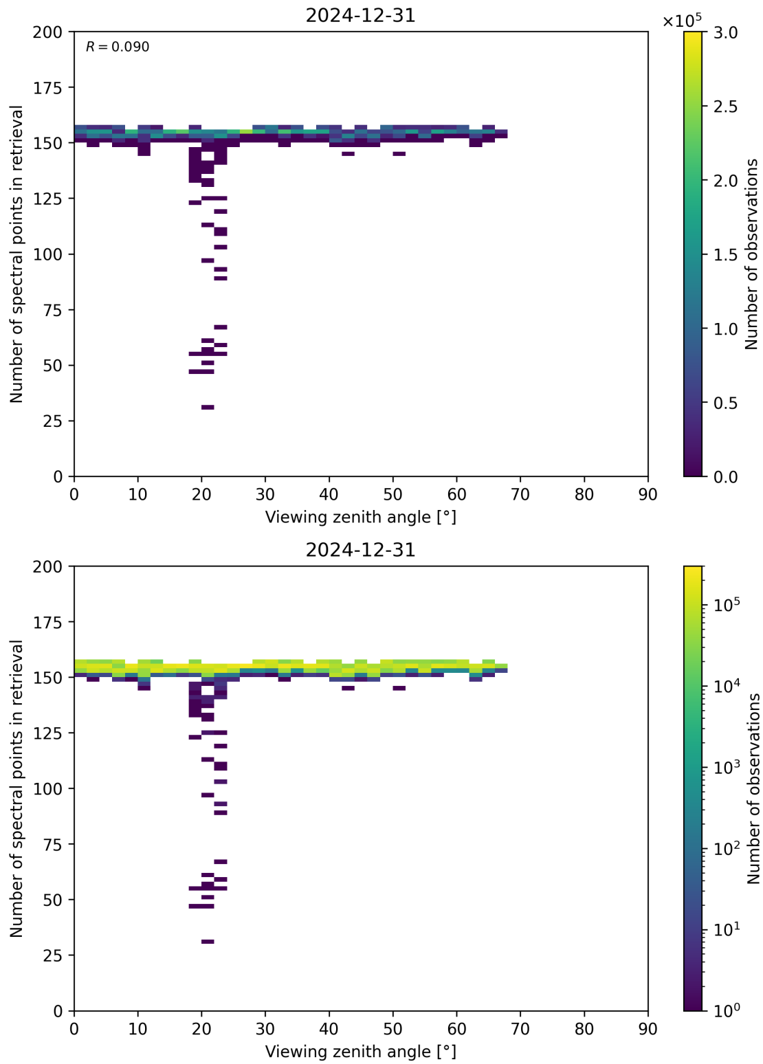
Figure 76: Scatter density plot of “Viewing zenith angle” against “Number of spectral points in retrieval” for 2024-12-30 to 2025-01-01.
