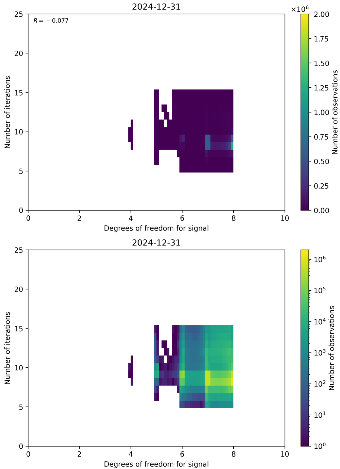
Figure 50: Scatter density plot of “Degrees of freedom for signal” against “Number of iterations” for 2024-12-30 to 2025-01-01.
