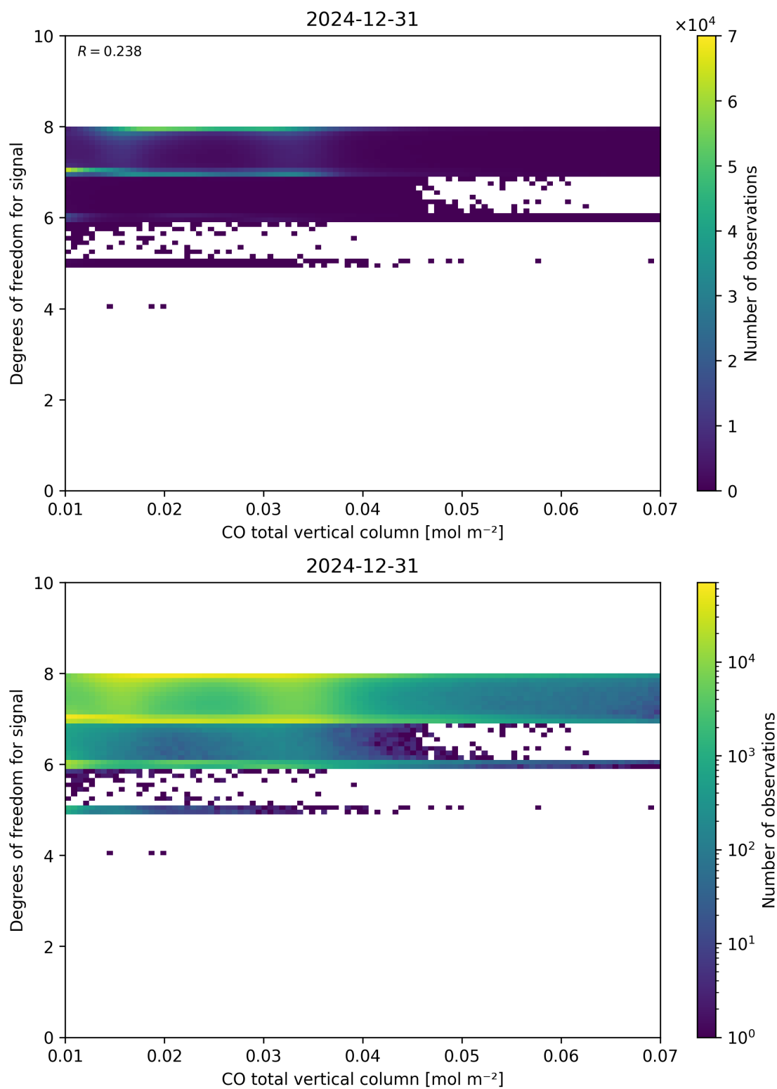
Figure 41: Scatter density plot of “CO total vertical column” against “Degrees of freedom for signal” for 2024-12-30 to 2025-01-01.
