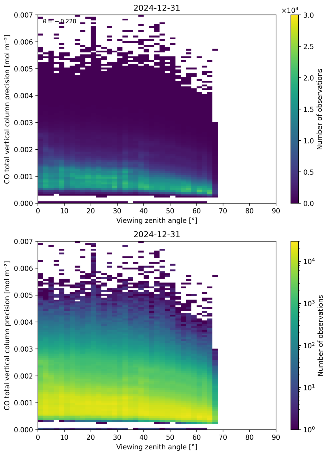
Figure 71: Scatter density plot of “Viewing zenith angle” against “CO total vertical column precision” for 2024-12-30 to 2025-01-01.
