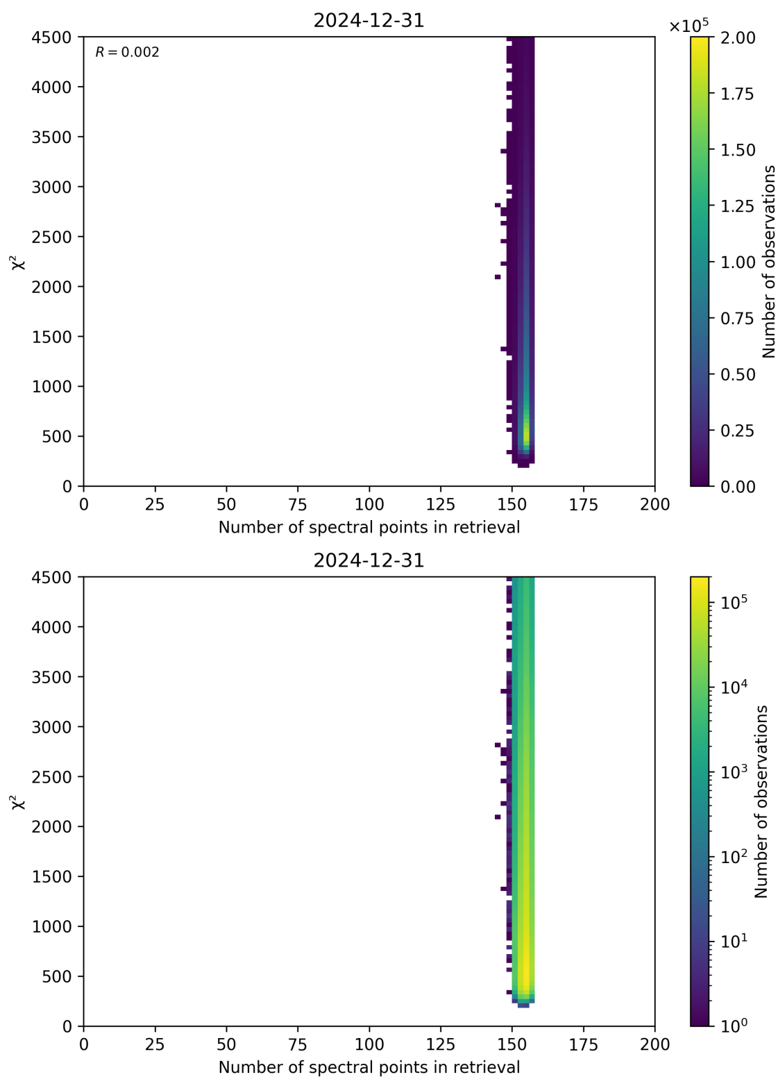
Figure 58: Scatter density plot of “Number of spectral points in retrieval” against “ \chi^2 ” for 2024-12-30 to 2025-01-01.
