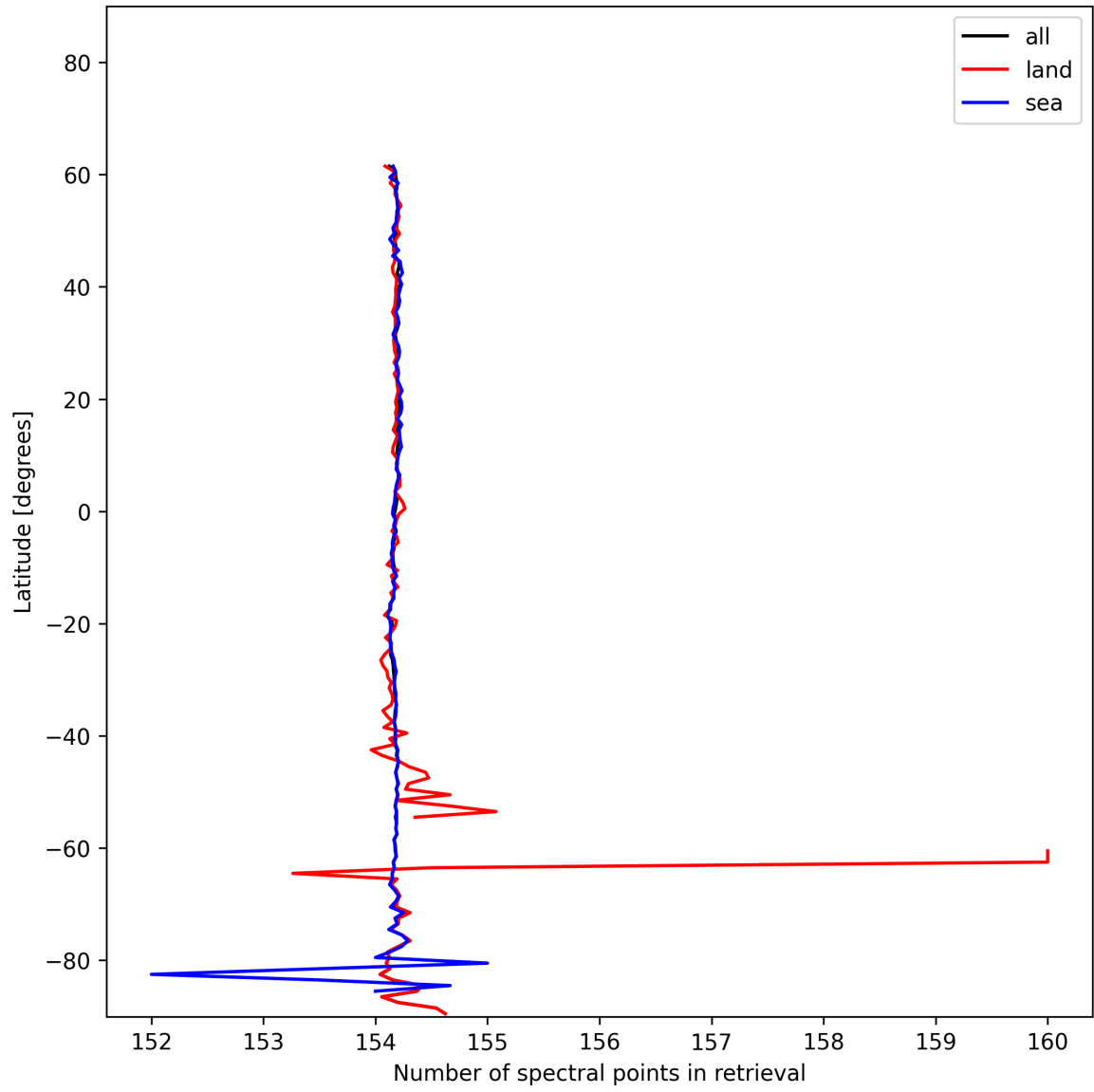
Figure 13: Zonal average of “Number of spectral points in retrieval” for 2024-12-30 to 2025-01-01.
