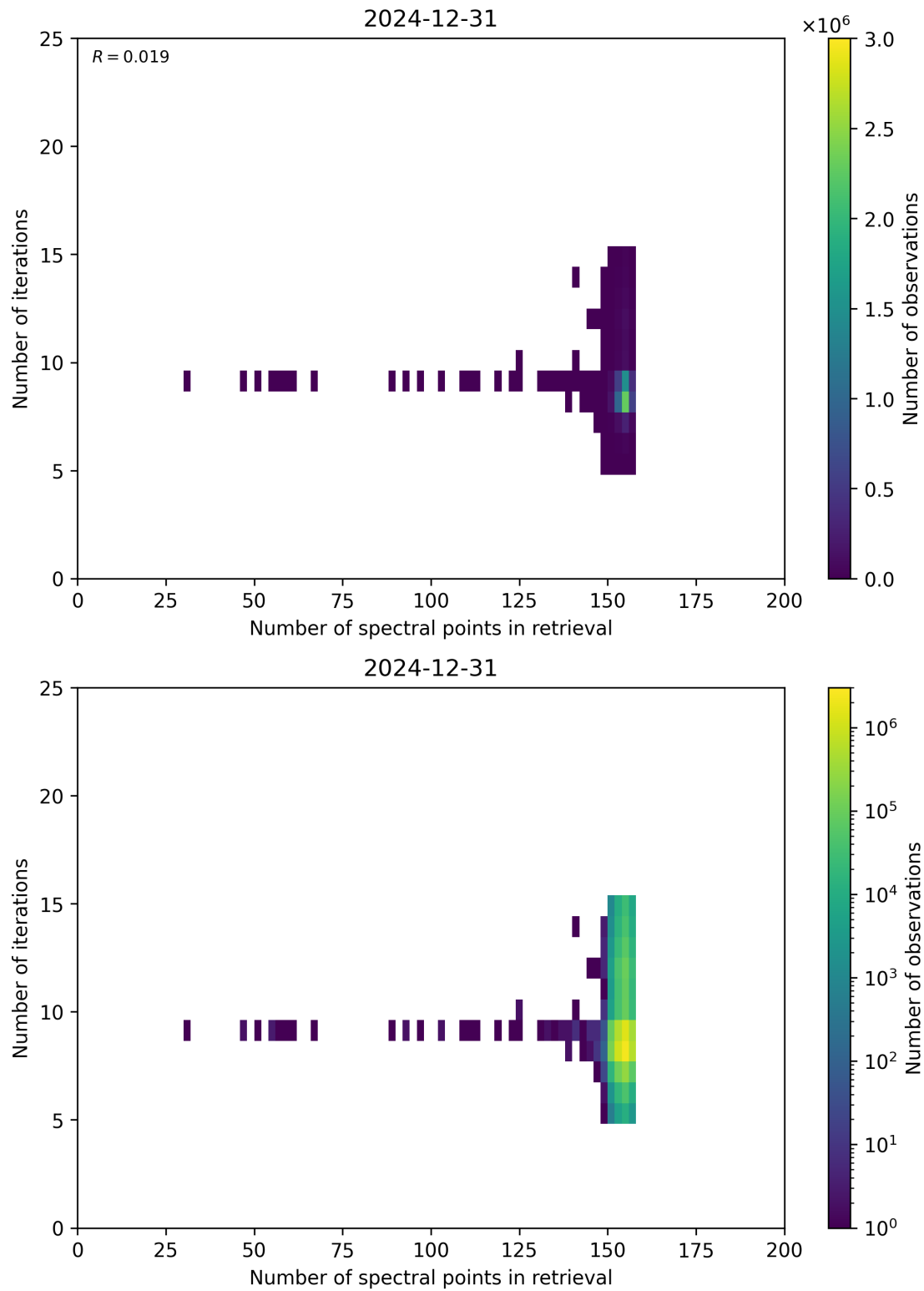
Figure 60: Scatter density plot of “Number of spectral points in retrieval” against “Number of iterations” for 2024-12-30 to 2025-01-01.
