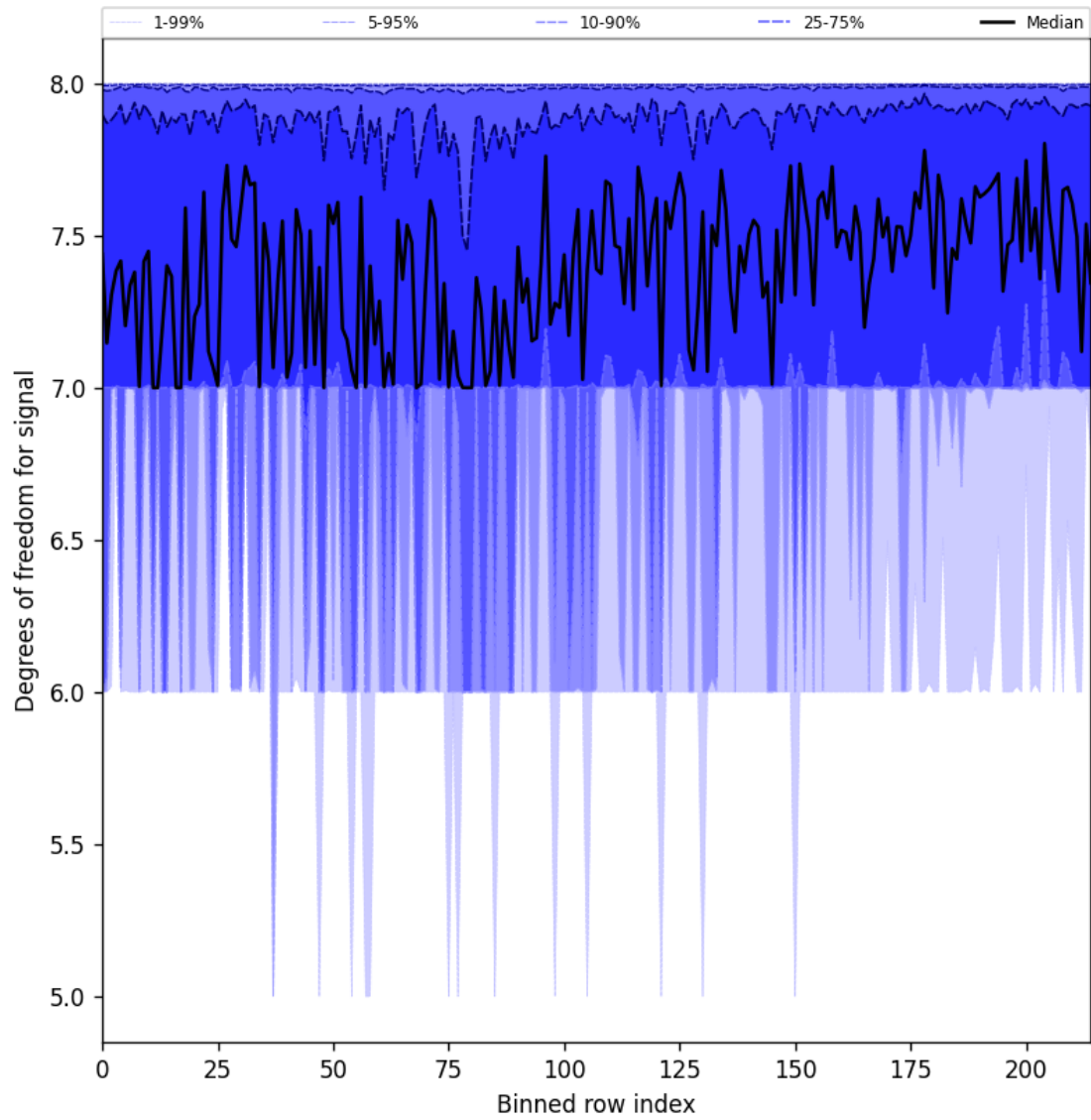
Figure 31: Along track statistics of “Degrees of freedom for signal” for 2024-12-30 to 2025-01-01
