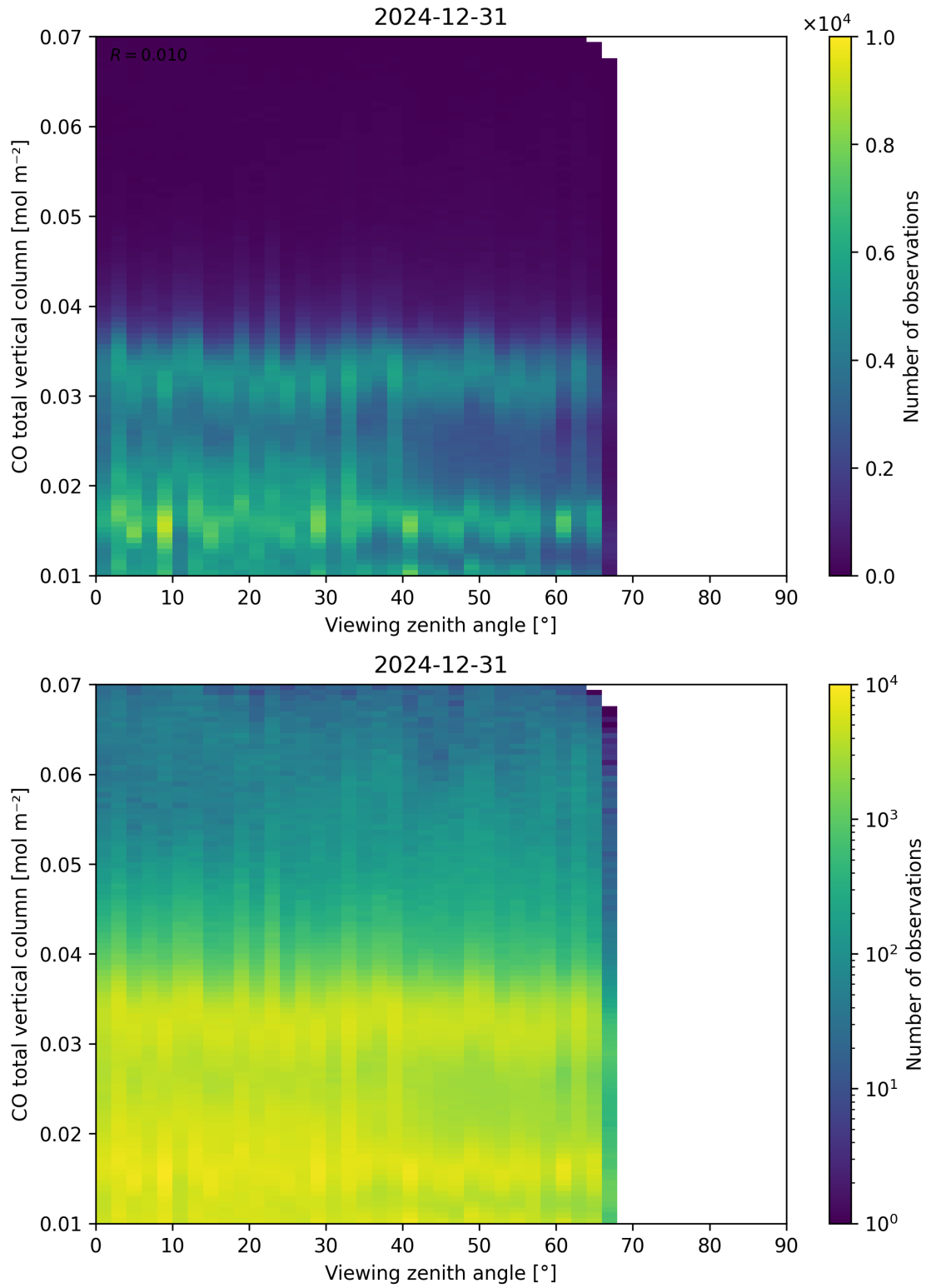
Figure 69: Scatter density plot of “Viewing zenith angle” against “CO total vertical column” for 2024-12-30 to 2025-01-01.
