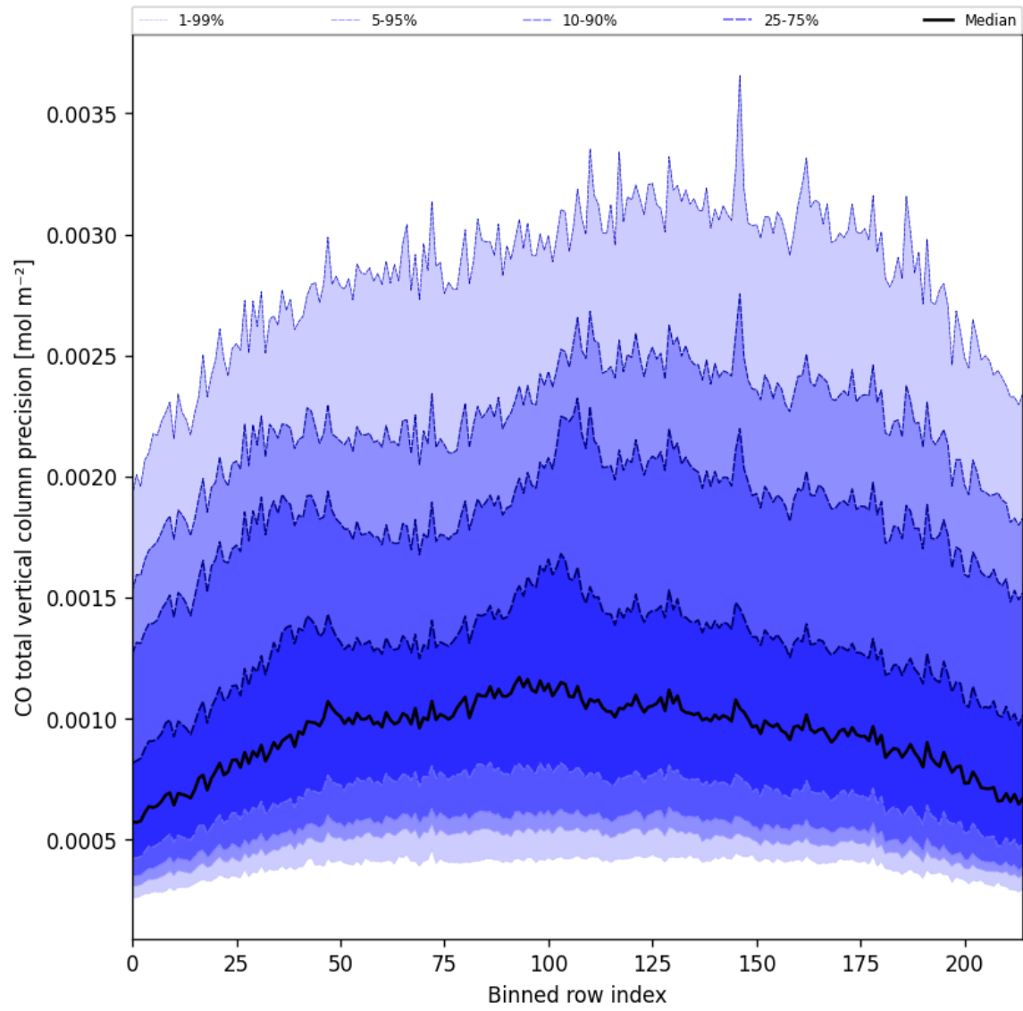
Figure 28: Along track statistics of “CO total vertical column precision” for 2024-12-30 to 2025-01-01
