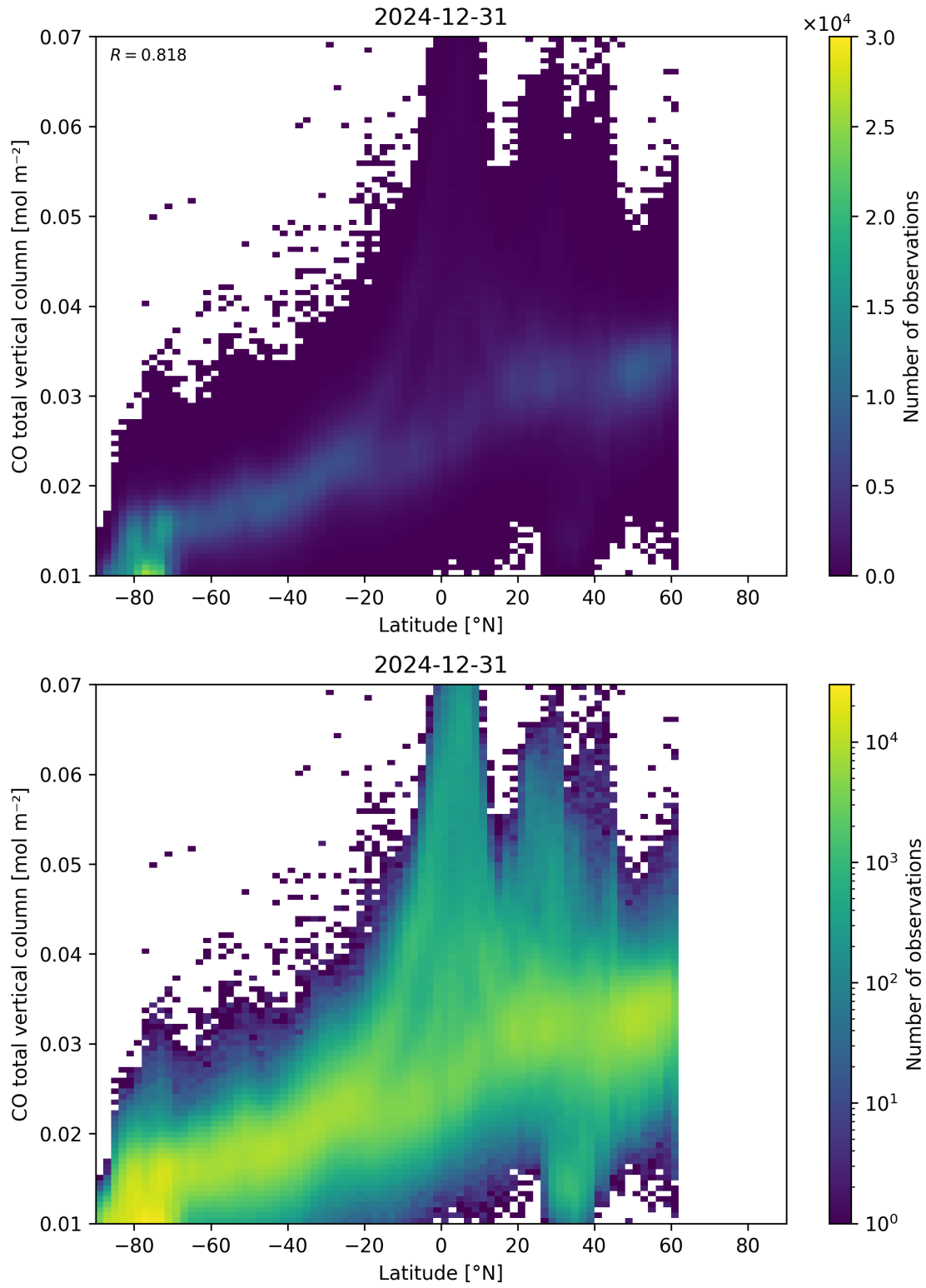
Figure 51: Scatter density plot of “Latitude” against “CO total vertical column” for 2024-12-30 to 2025-01-01.
