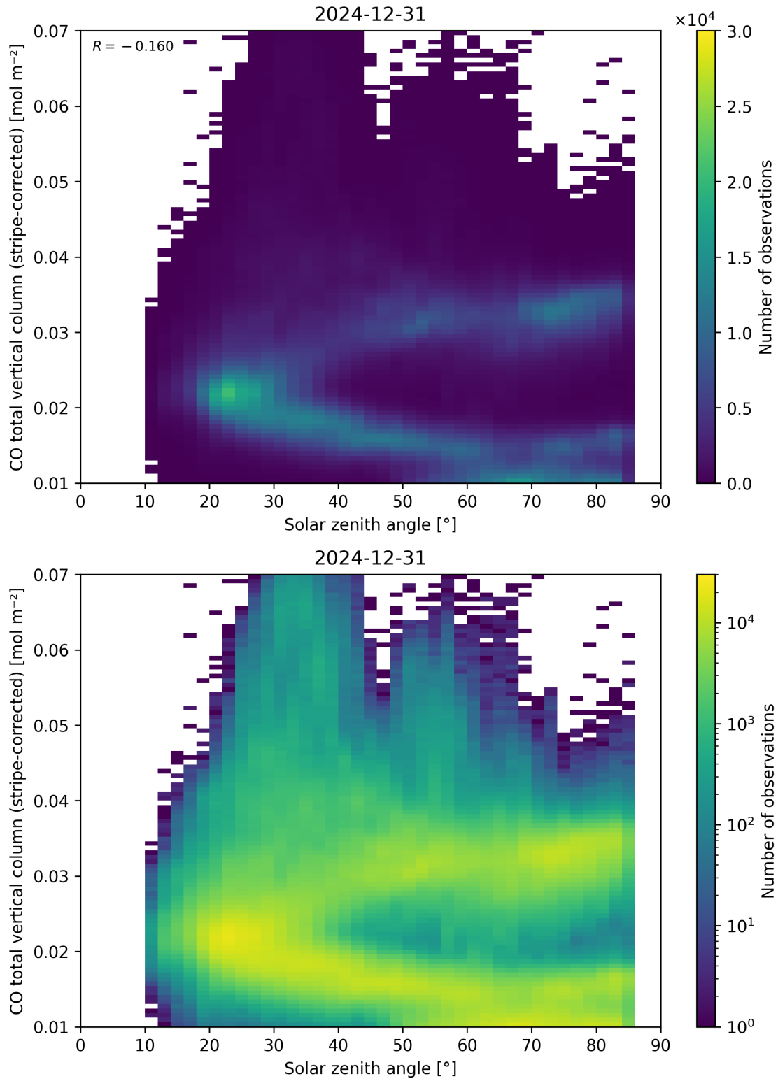
Figure 62: Scatter density plot of “Solar zenith angle” against “CO total vertical column (stripe-corrected)” for 2024-12-30 to 2025-01-01.
