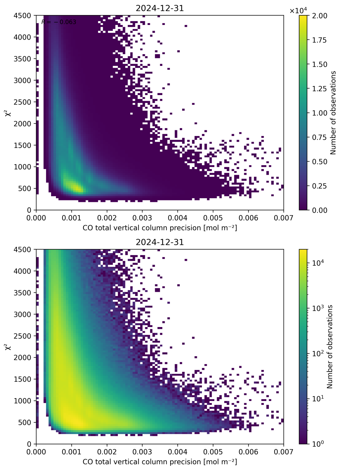
Figure 44: Scatter density plot of “CO total vertical column precision” against “ \chi^2 ” for 2024-12-30 to 2025-01-01.
