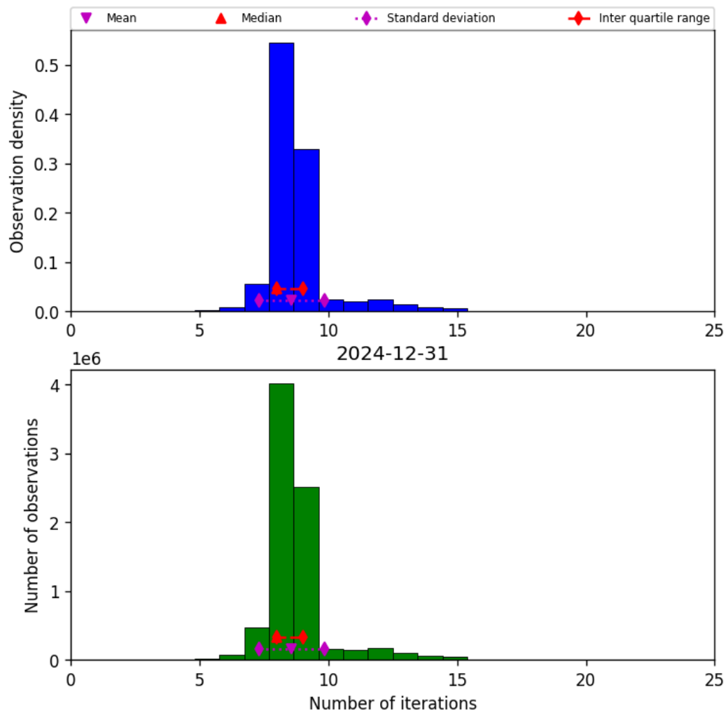
Figure 24: Histogram of “Number of iterations” for 2024-12-30 to 2025-01-01
