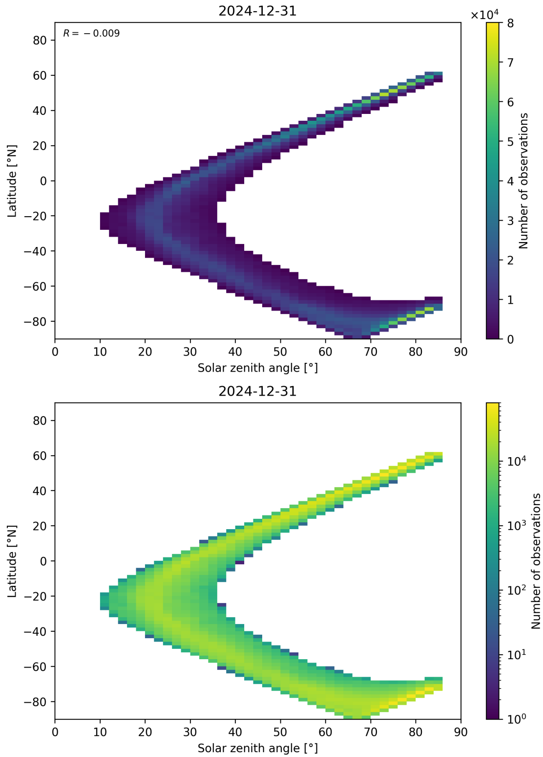
Figure 66: Scatter density plot of “Solar zenith angle” against “Latitude” for 2024-12-30 to 2025-01-01.
