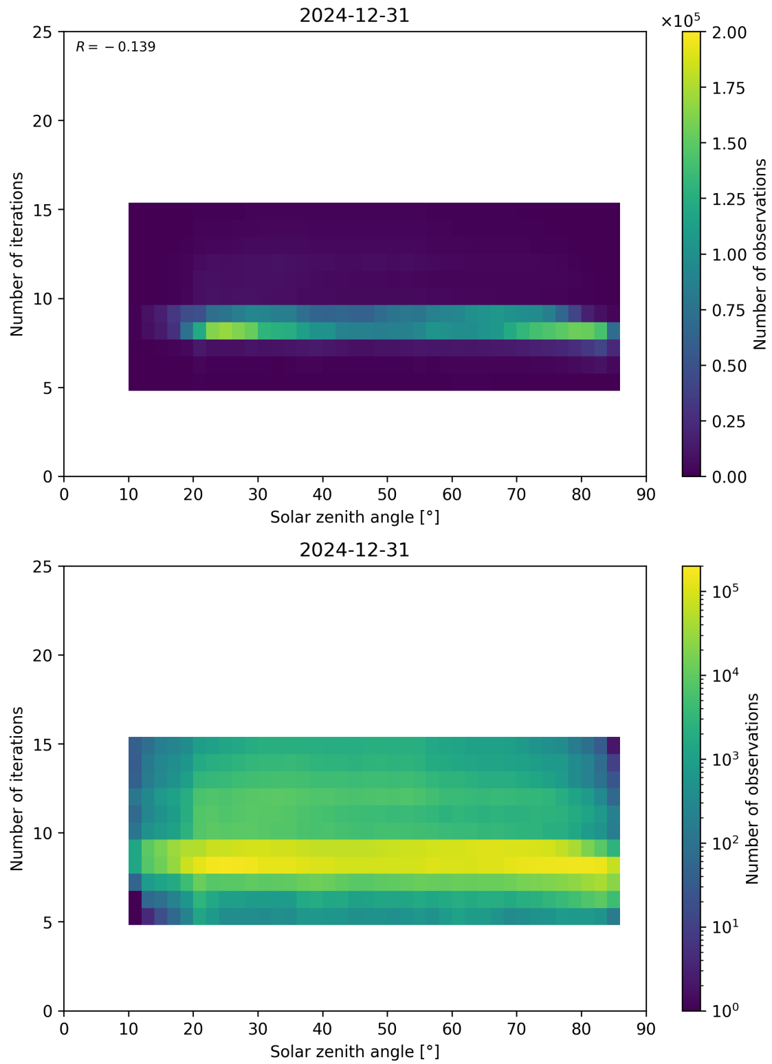
Figure 67: Scatter density plot of “Solar zenith angle” against “Number of iterations” for 2024-12-30 to 2025-01-01.
