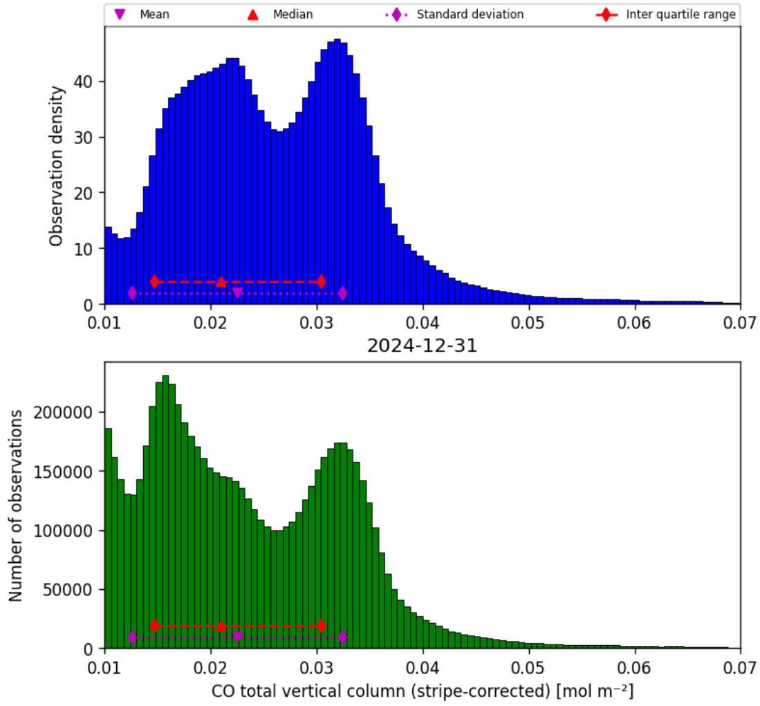
Figure 19: Histogram of “CO total vertical column (stripe-corrected)” for 2024-12-30 to 2025-01-01
