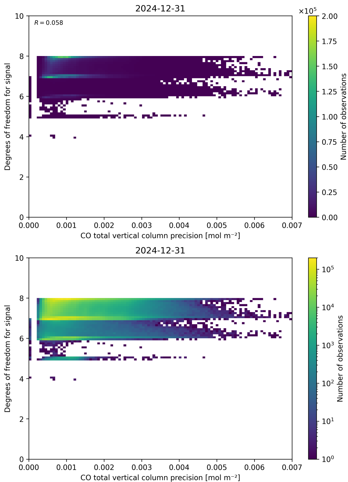
Figure 45: Scatter density plot of “CO total vertical column precision” against “Degrees of freedom for signal” for 2024-12-30 to 2025-01-01.
