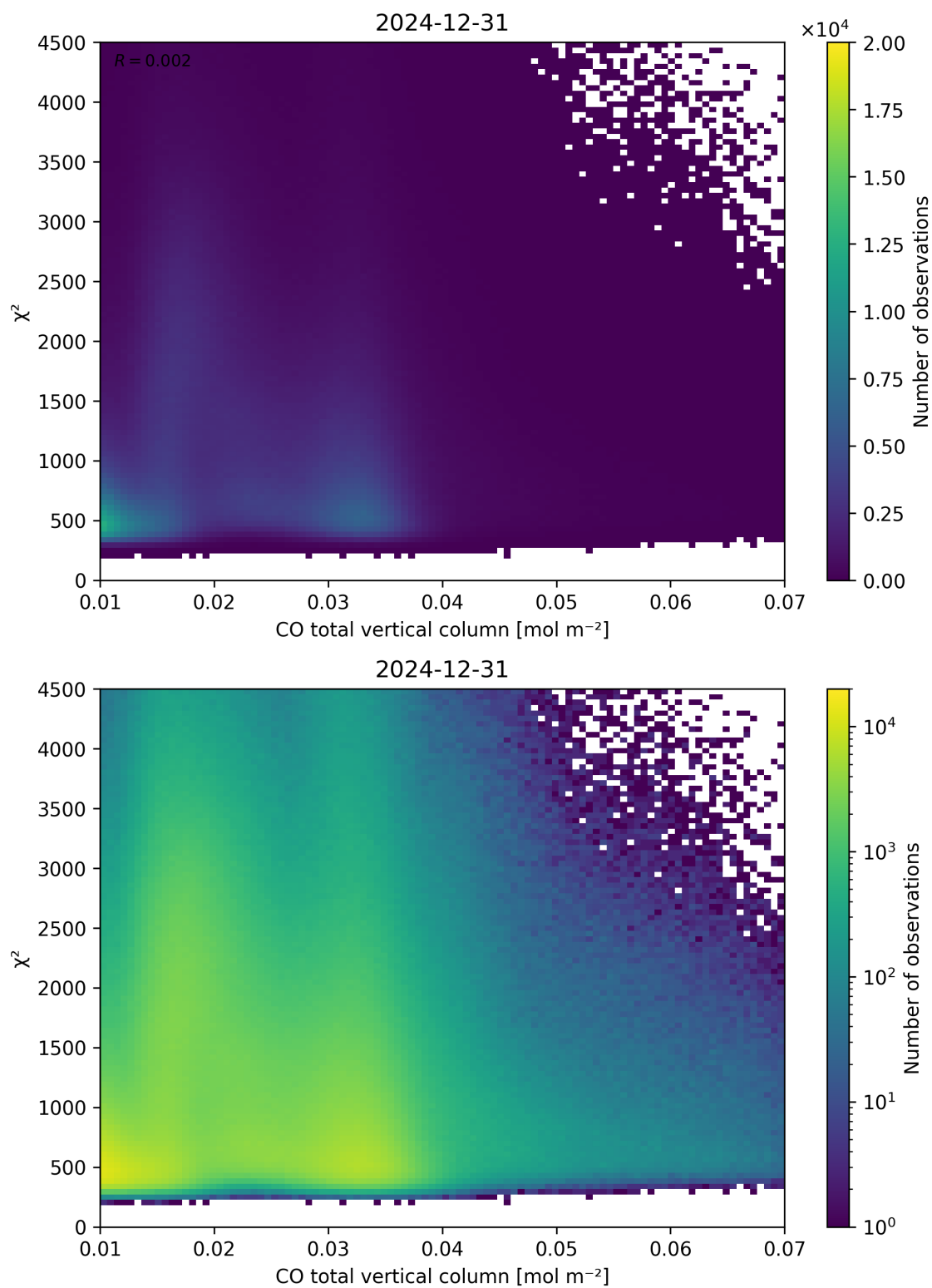
Figure 35: Scatter density plot of “CO total vertical column” against “ \chi^2 ” for 2024-12-30 to 2025-01-01.
