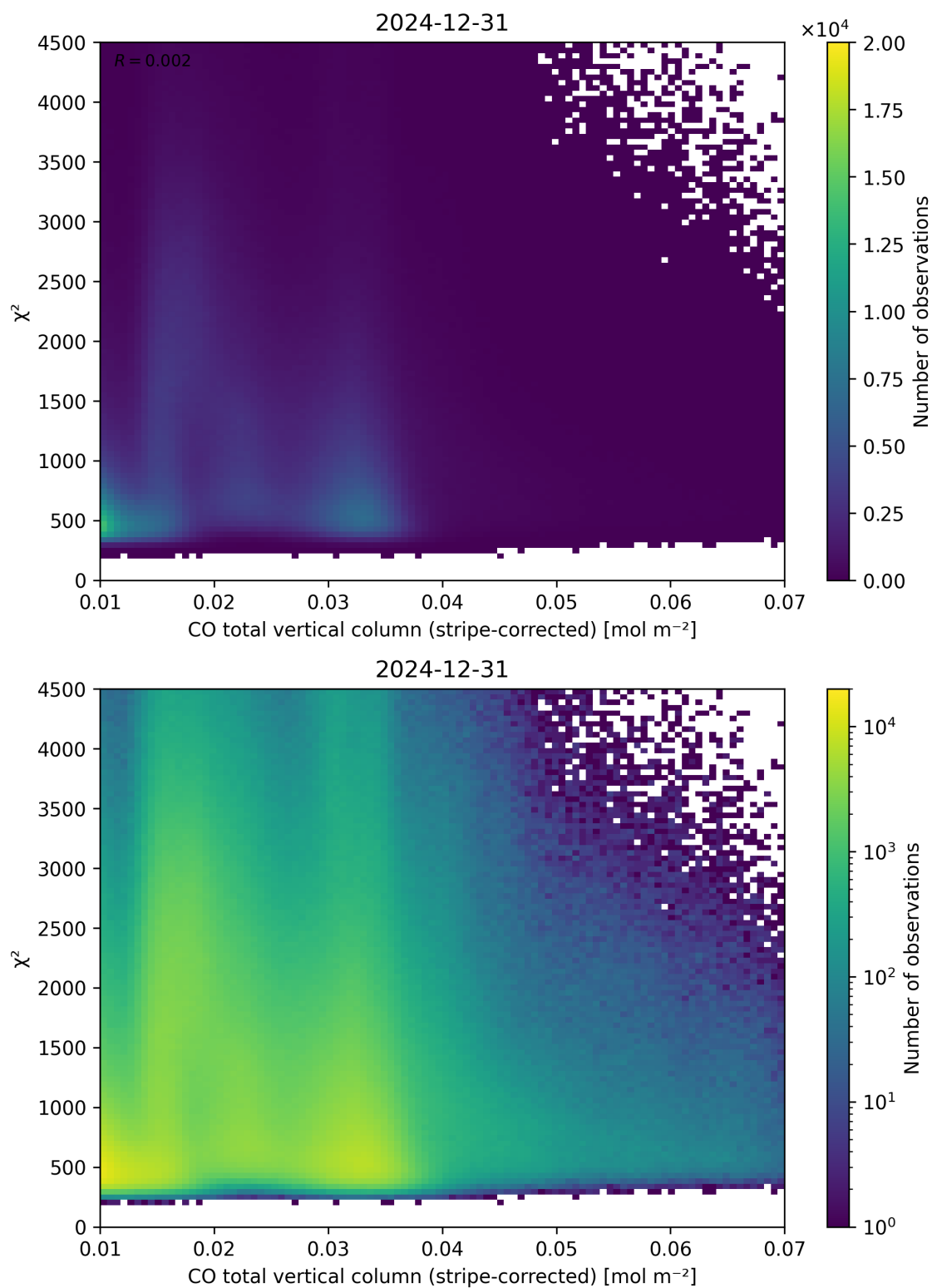
Figure 37: Scatter density plot of “CO total vertical column (stripe-corrected)” against “ \chi^2 ” for 2024-12-30 to 2025-01-01.
