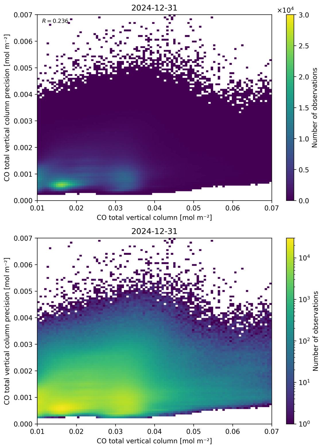
Figure 34: Scatter density plot of “CO total vertical column” against “CO total vertical column precision” for 2024-12-30 to 2025-01-01.
