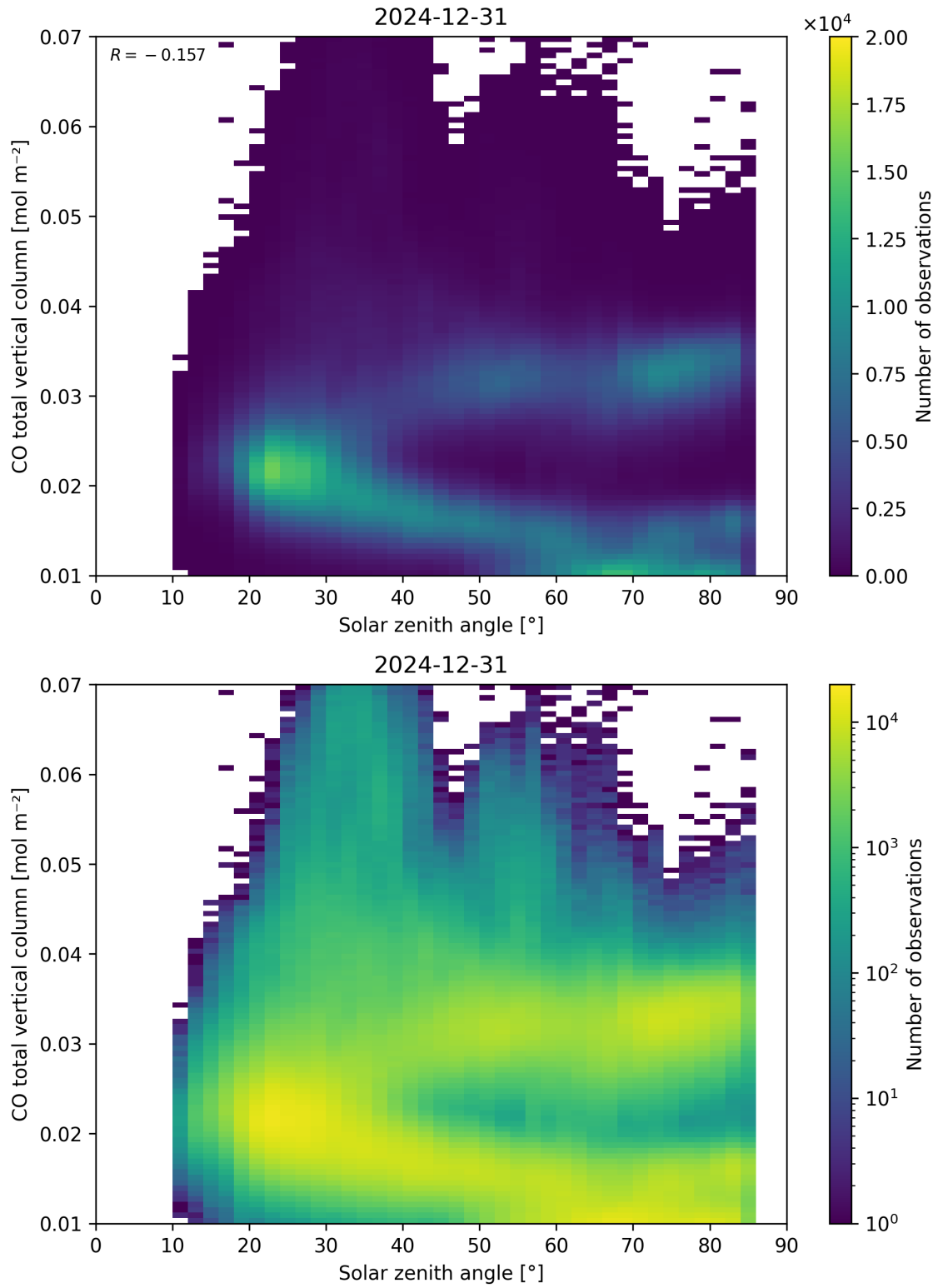
Figure 61: Scatter density plot of “Solar zenith angle” against “CO total vertical column” for 2024-12-30 to 2025-01-01.
