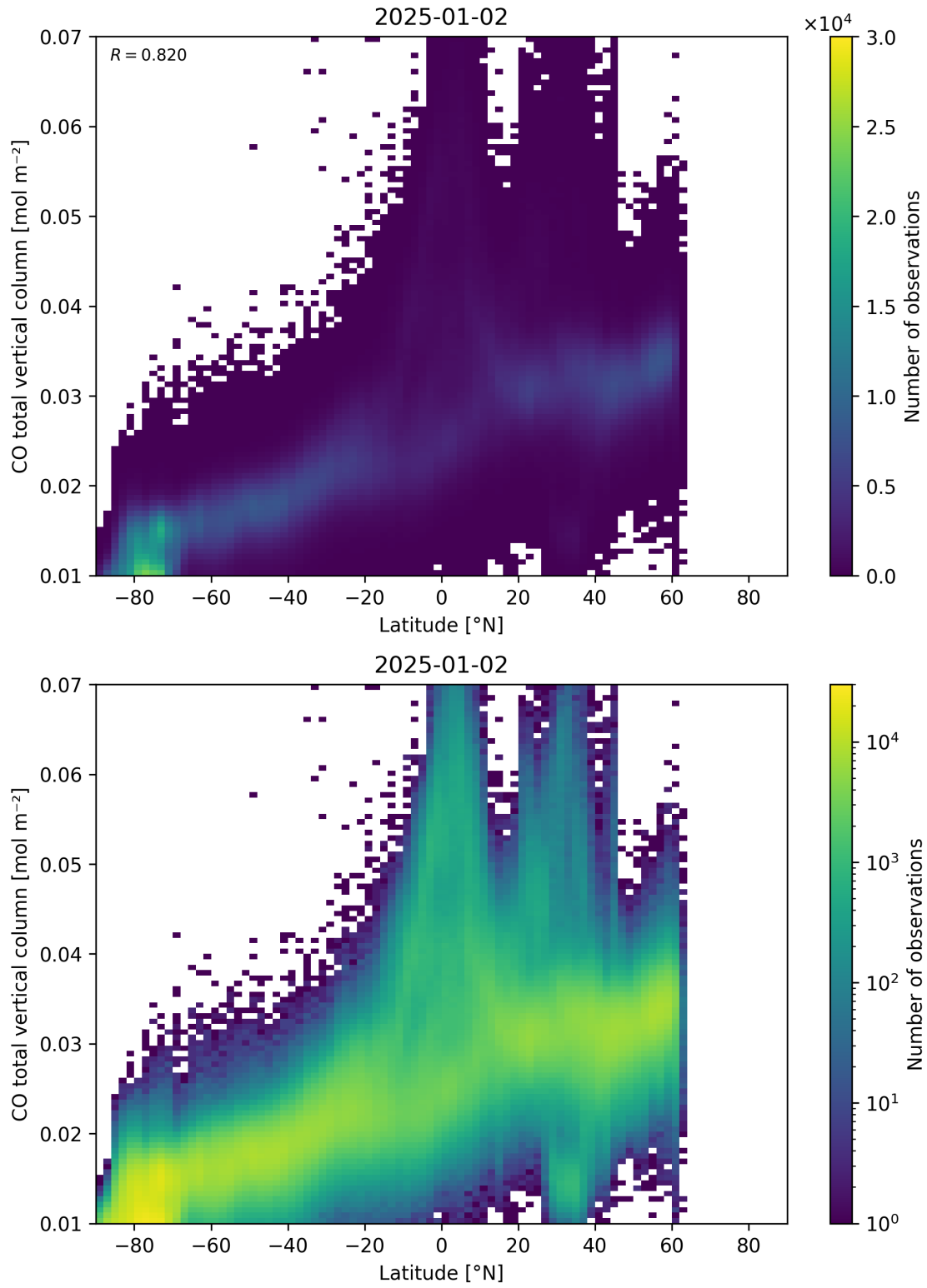
Figure 51: Scatter density plot of “Latitude” against “CO total vertical column” for 2025-01-01 to 2025-01-03.
