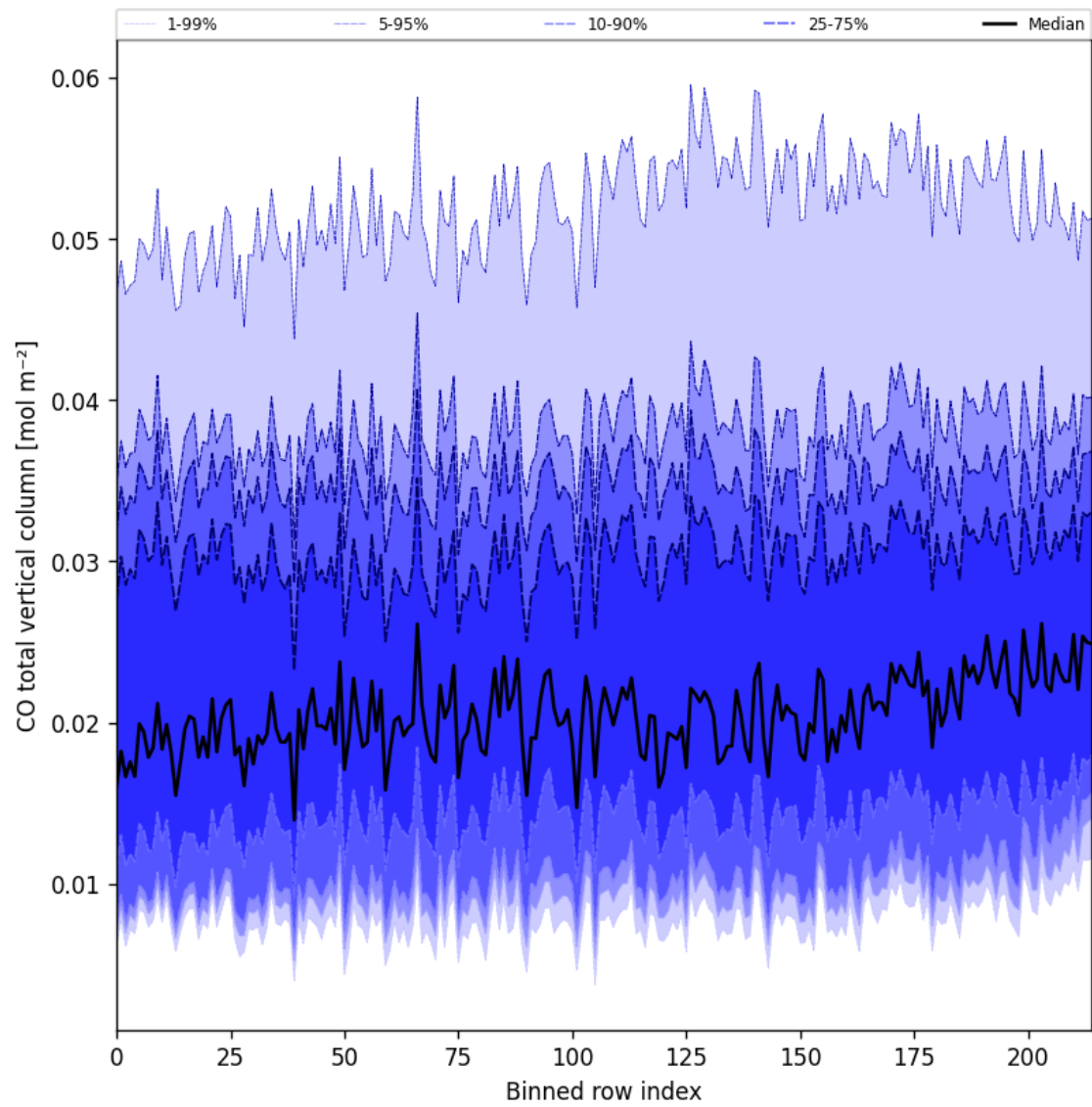
Figure 26: Along track statistics of “CO total vertical column” for 2025-01-01 to 2025-01-03
