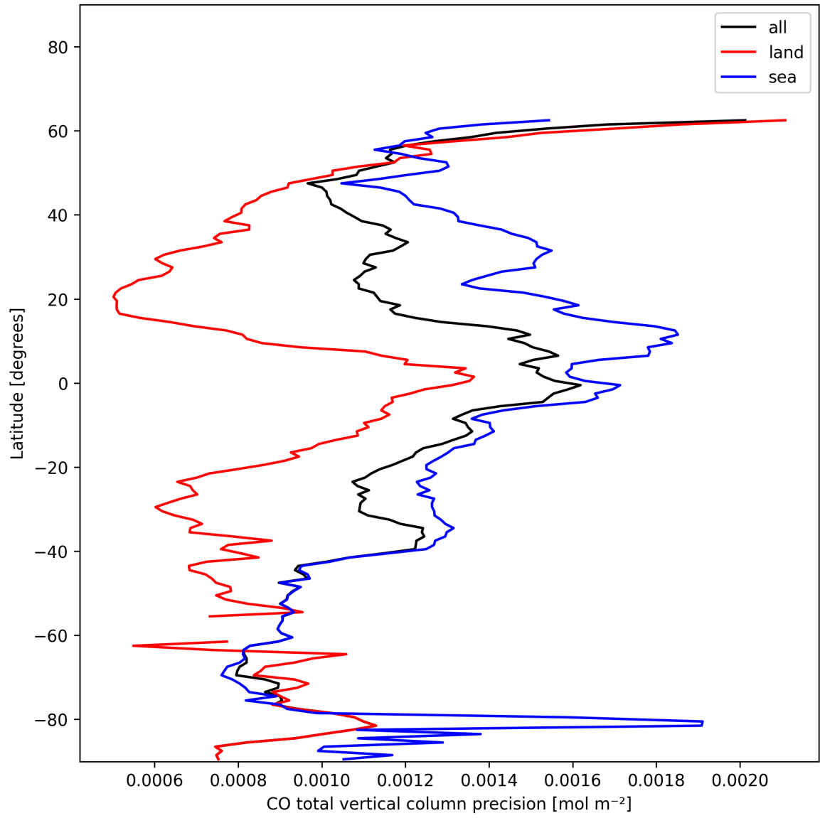
Figure 12: Zonal average of “CO total vertical column precision” for 2025-01-01 to 2025-01-03.
