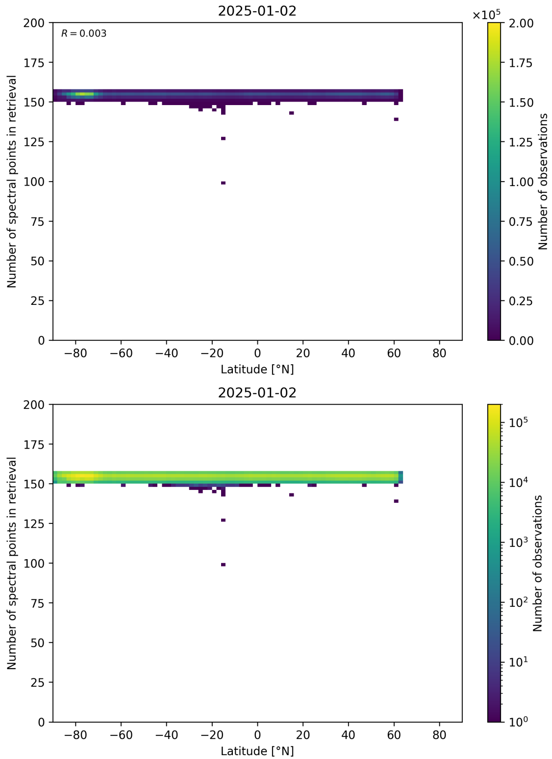
Figure 57: Scatter density plot of “Latitude” against “Number of spectral points in retrieval” for 2025-01-01 to 2025-01-03.
