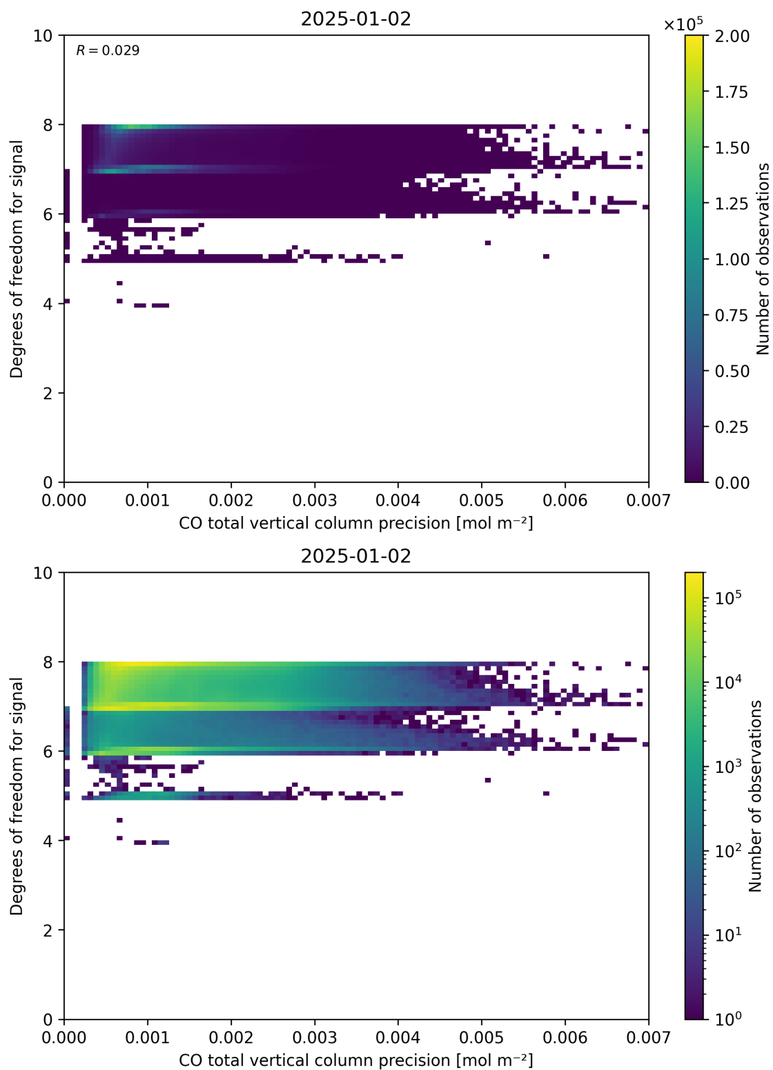
Figure 45: Scatter density plot of “CO total vertical column precision” against “Degrees of freedom for signal” for 2025-01-01 to 2025-01-03.
