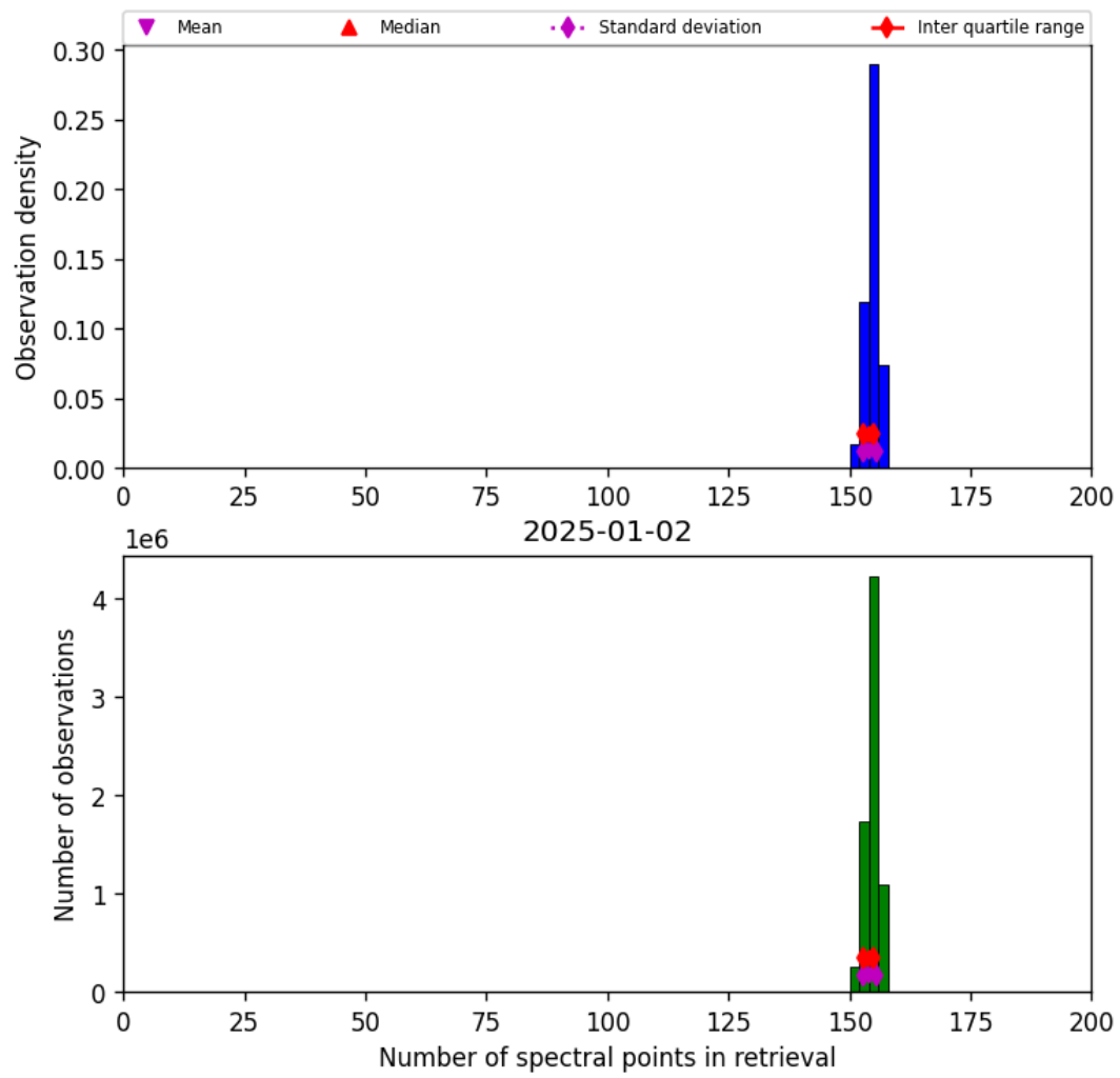
Figure 21: Histogram of “Number of spectral points in retrieval” for 2025-01-01 to 2025-01-03
