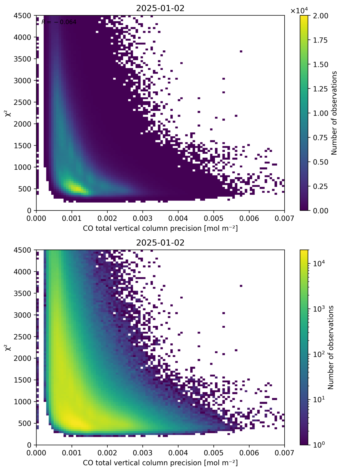
Figure 44: Scatter density plot of “CO total vertical column precision” against “ \chi^2 ” for 2025-01-01 to 2025-01-03.
