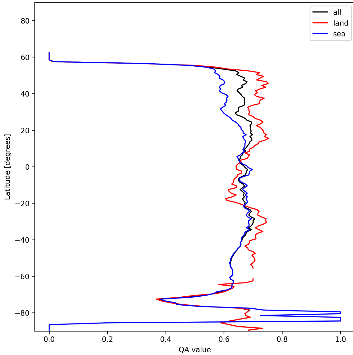
Figure 9: Zonal average of “QA value” for 2025-01-01 to 2025-01-03.
