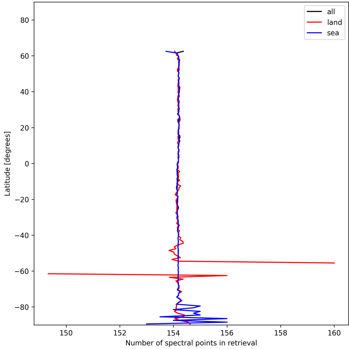
Figure 13: Zonal average of “Number of spectral points in retrieval” for 2025-01-01 to 2025-01-03.
