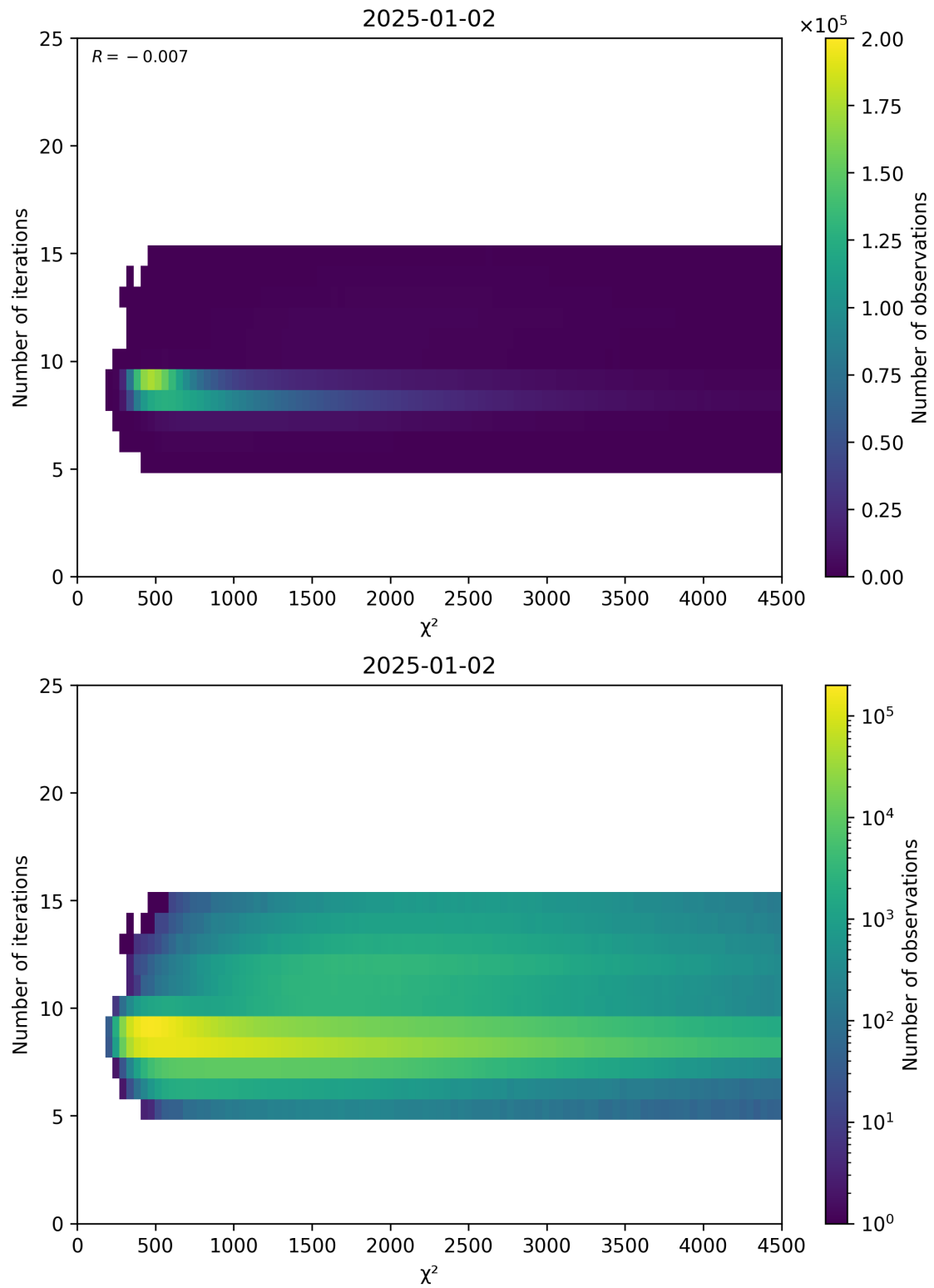
Figure 49: Scatter density plot of “ \chi^2 ” against “Number of iterations” for 2025-01-01 to 2025-01-03.
