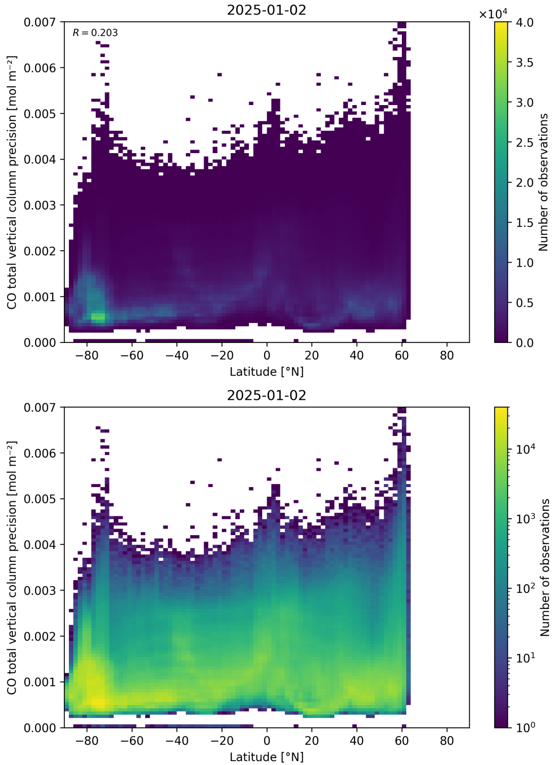
Figure 53: Scatter density plot of “Latitude” against “CO total vertical column precision” for 2025-01-01 to 2025-01-03.
