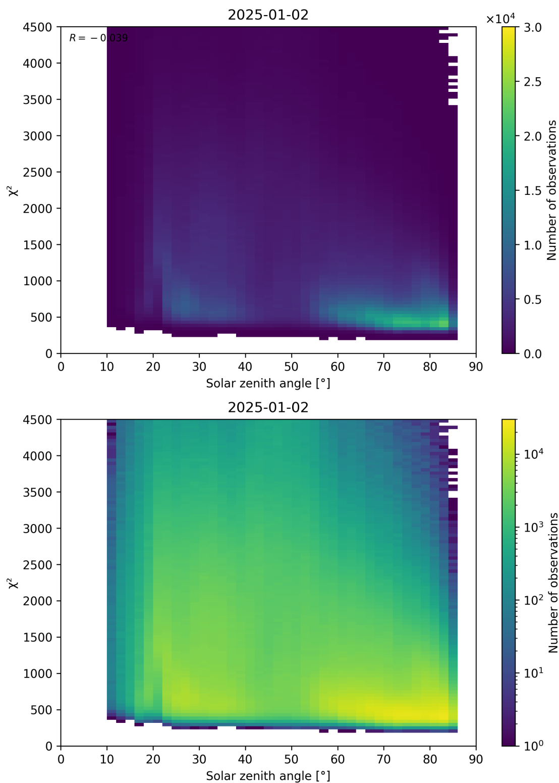
Figure 64: Scatter density plot of “Solar zenith angle” against “ \chi^2 ” for 2025-01-01 to 2025-01-03.
