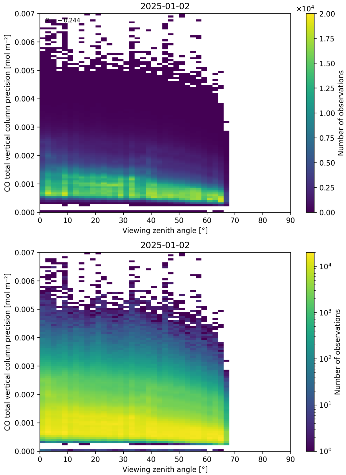
Figure 71: Scatter density plot of “Viewing zenith angle” against “CO total vertical column precision” for 2025-01-01 to 2025-01-03.
