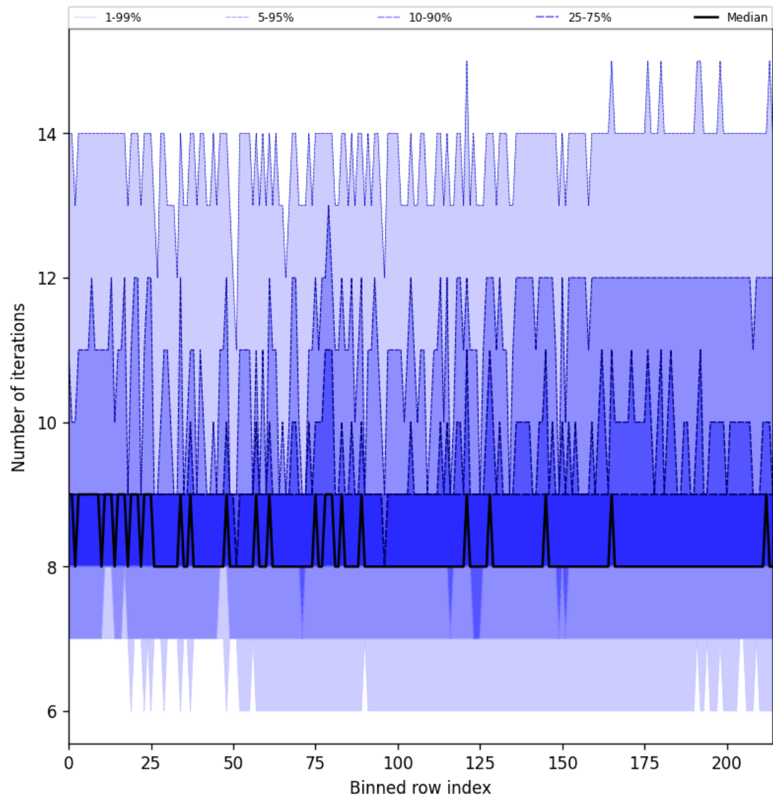
Figure 32: Along track statistics of “Number of iterations” for 2025-01-01 to 2025-01-03
