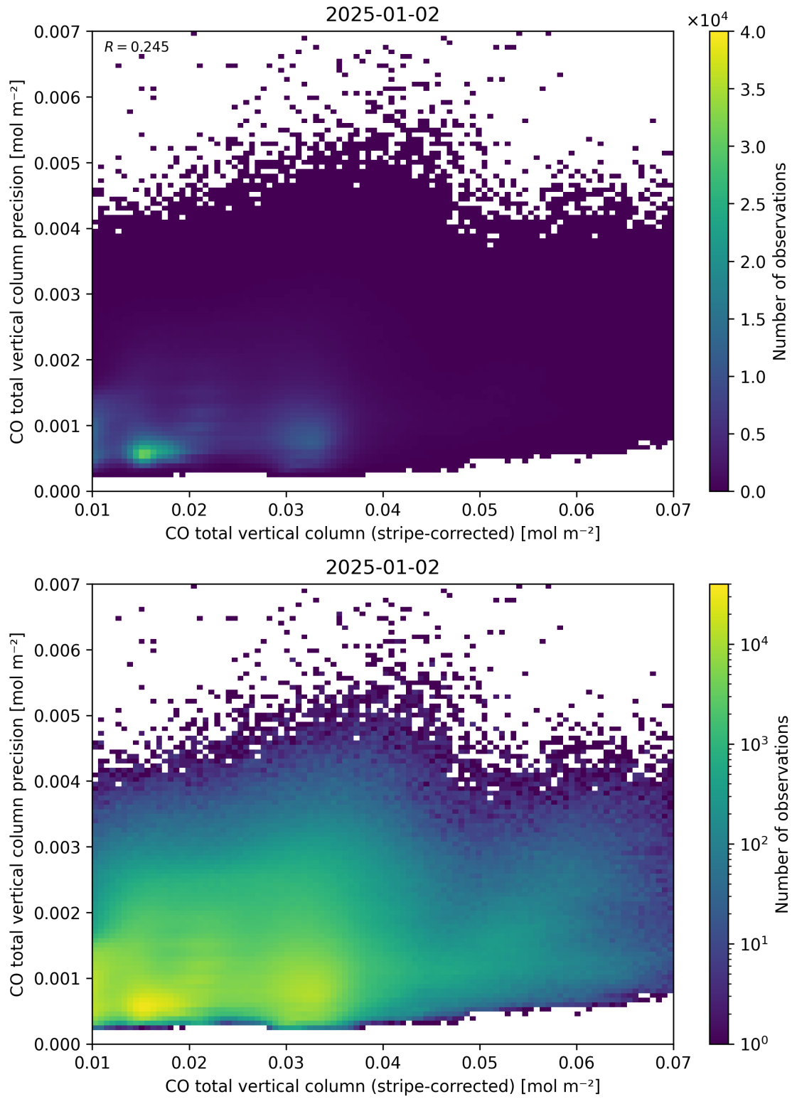
Figure 36: Scatter density plot of “CO total vertical column (stripe-corrected)” against “CO total vertical column precision” for 2025-01-01 to 2025-01-03.
