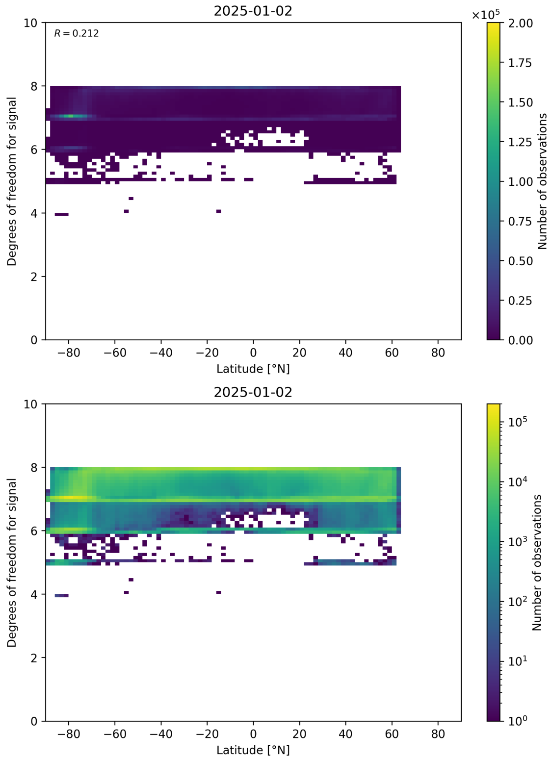
Figure 55: Scatter density plot of “Latitude” against “Degrees of freedom for signal” for 2025-01-01 to 2025-01-03.
