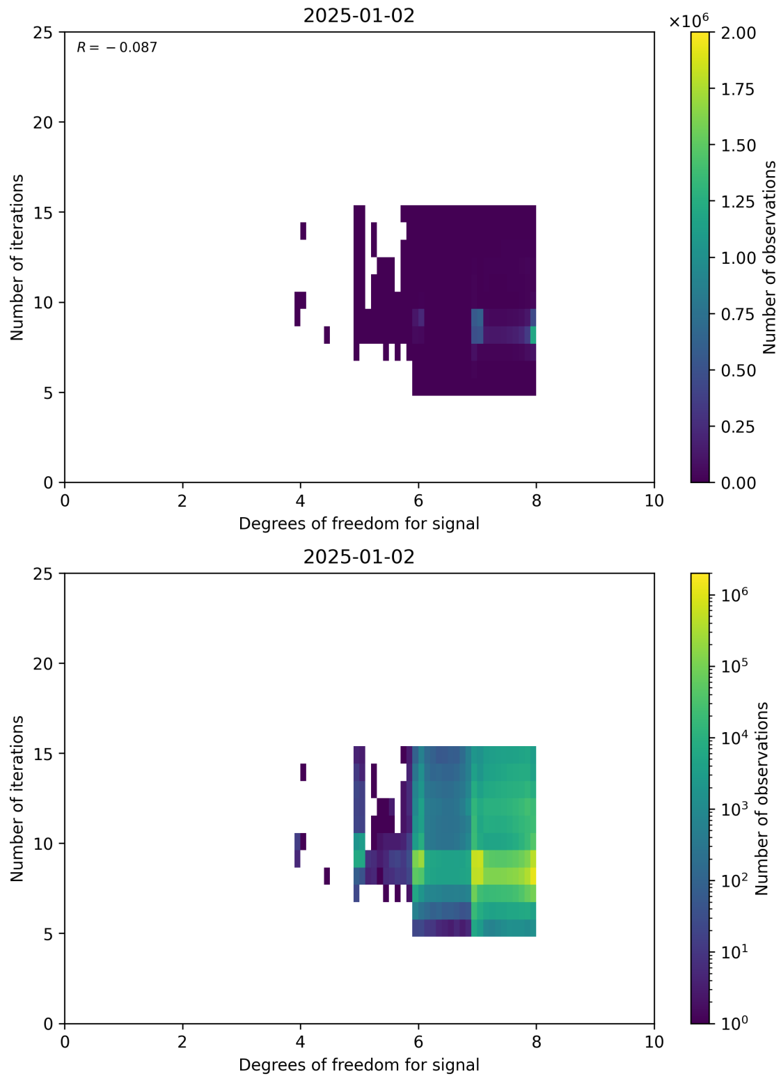
Figure 50: Scatter density plot of “Degrees of freedom for signal” against “Number of iterations” for 2025-01-01 to 2025-01-03.
