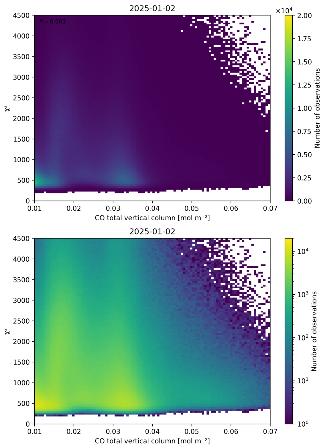
Figure 35: Scatter density plot of “CO total vertical column” against “ \chi^2 ” for 2025-01-01 to 2025-01-03.
