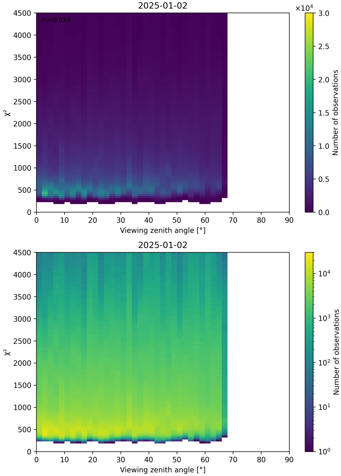
Figure 72: Scatter density plot of “Viewing zenith angle” against “ \chi^2 ” for 2025-01-01 to 2025-01-03.
