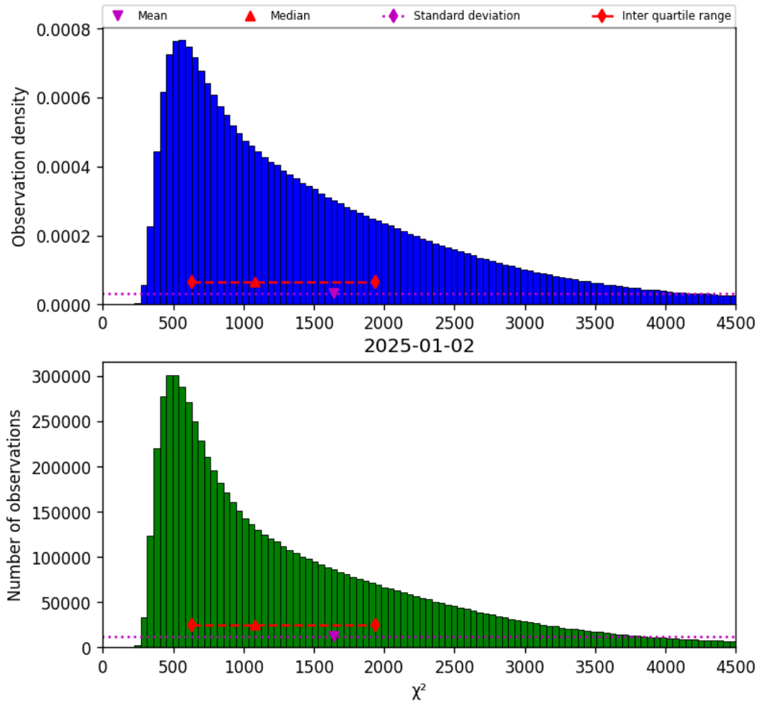
Figure 22: Histogram of " \chi^2 " for 2025-01-01 to 2025-01-03
