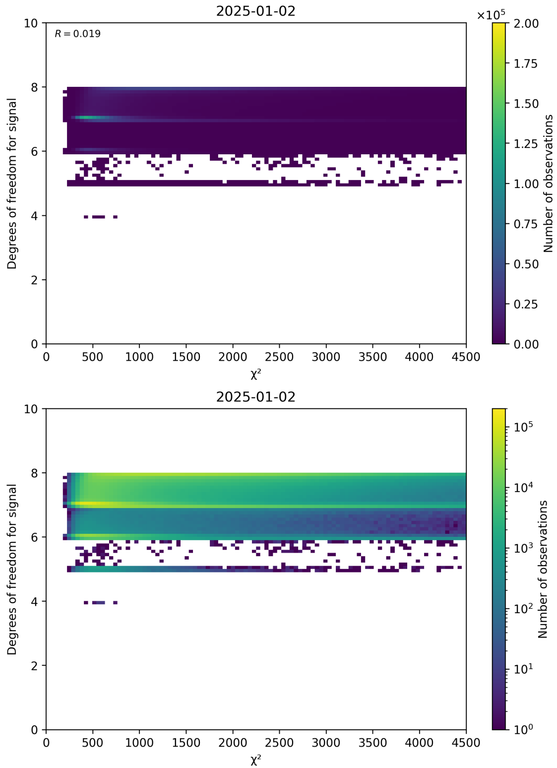
Figure 48: Scatter density plot of “ \chi^2 ” against “Degrees of freedom for signal” for 2025-01-01 to 2025-01-03.
