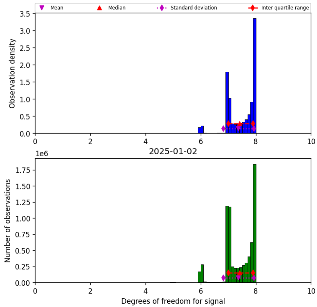
Figure 23: Histogram of “Degrees of freedom for signal” for 2025-01-01 to 2025-01-03
