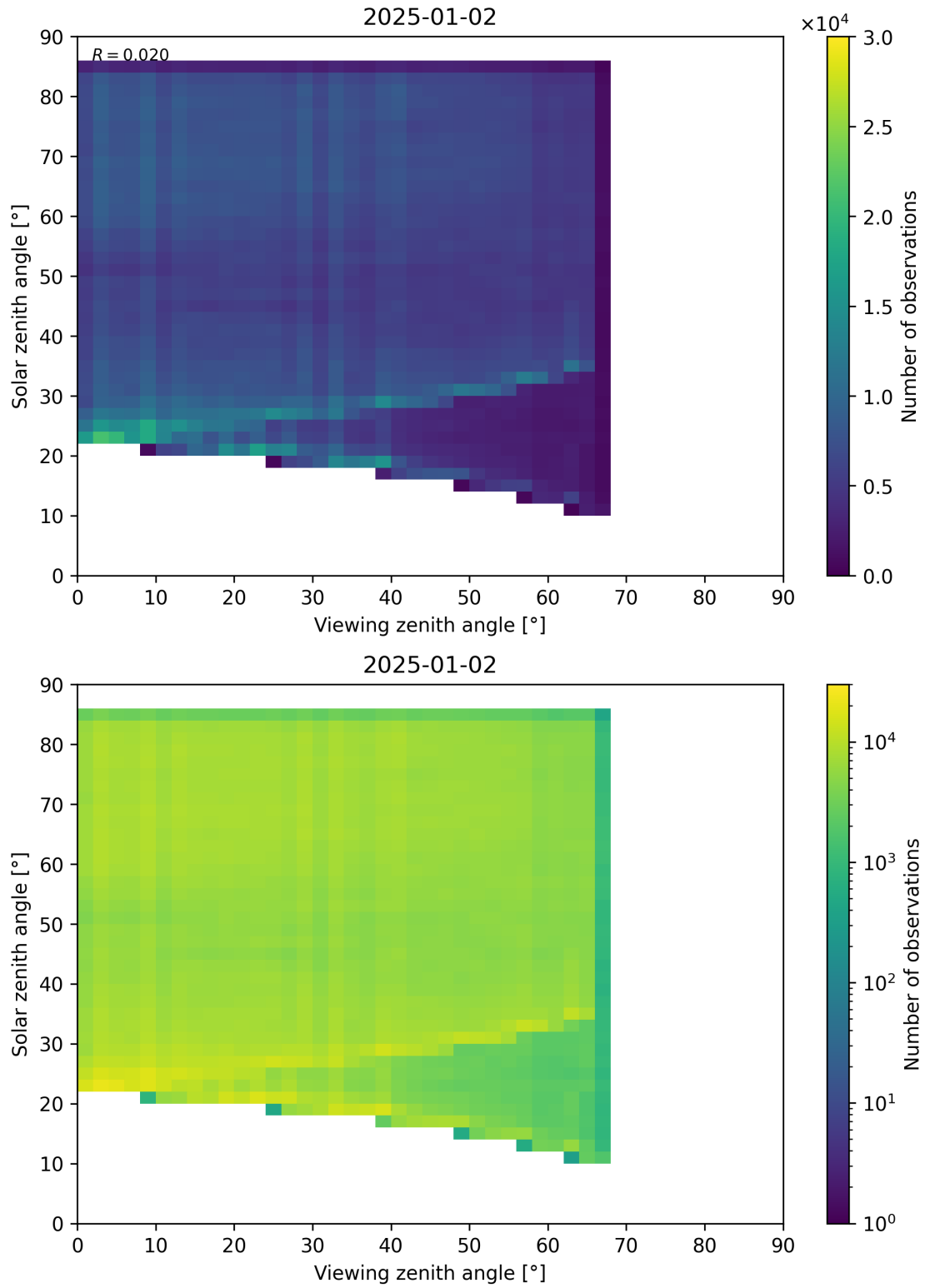
Figure 77: Scatter density plot of “Viewing zenith angle” against “Solar zenith angle” for 2025-01-01 to 2025-01-03.
