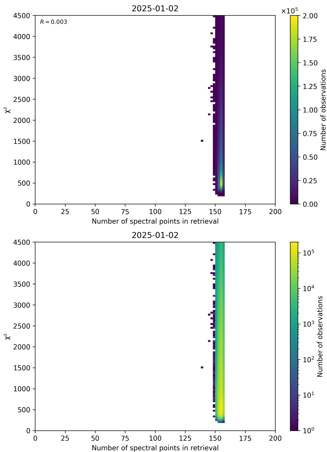
Figure 58: Scatter density plot of “Number of spectral points in retrieval” against “ \chi^2 ” for 2025-01-01 to 2025-01-03.
