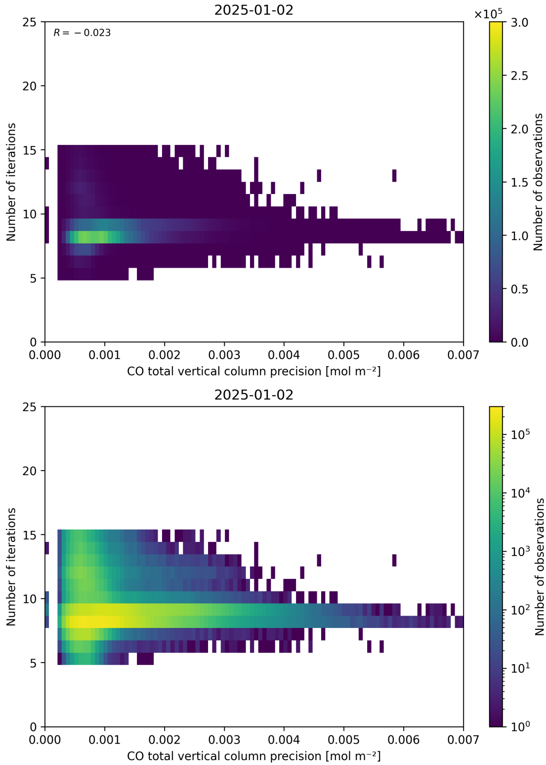
Figure 46: Scatter density plot of “CO total vertical column precision” against “Number of iterations” for 2025-01-01 to 2025-01-03.
