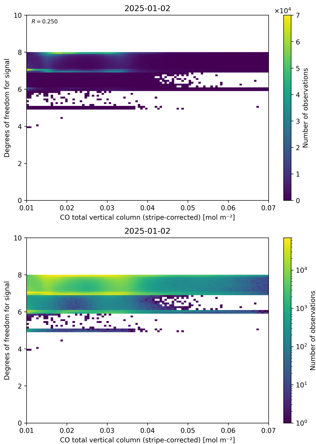
Figure 38: Scatter density plot of “CO total vertical column (stripe-corrected)” against “Degrees of freedom for signal” for 2025-01-01 to 2025-01-03.
