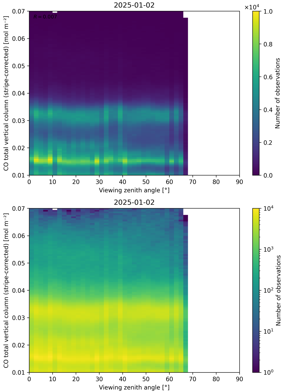
Figure 70: Scatter density plot of “Viewing zenith angle” against “CO total vertical column (stripe-corrected)” for 2025-01-01 to 2025-01-03.
