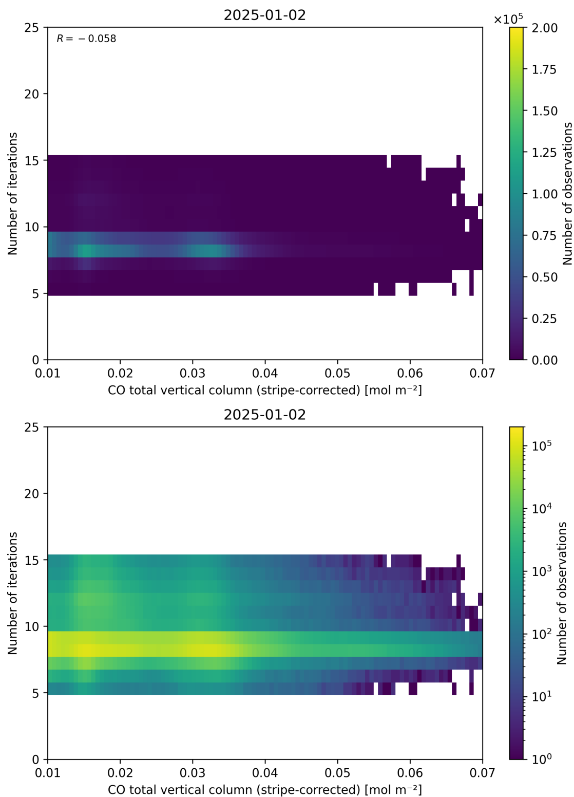
Figure 39: Scatter density plot of “CO total vertical column (stripe-corrected)” against “Number of iterations” for 2025-01-01 to 2025-01-03.
