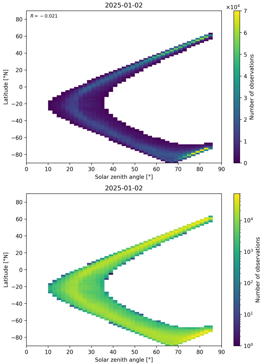
Figure 66: Scatter density plot of “Solar zenith angle” against “Latitude” for 2025-01-01 to 2025-01-03.
