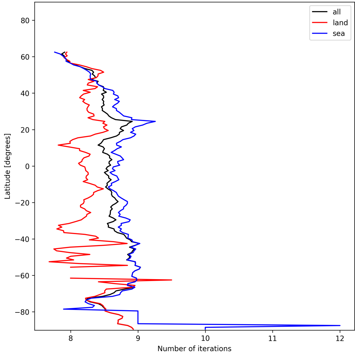
Figure 16: Zonal average of “Number of iterations” for 2025-01-01 to 2025-01-03.
