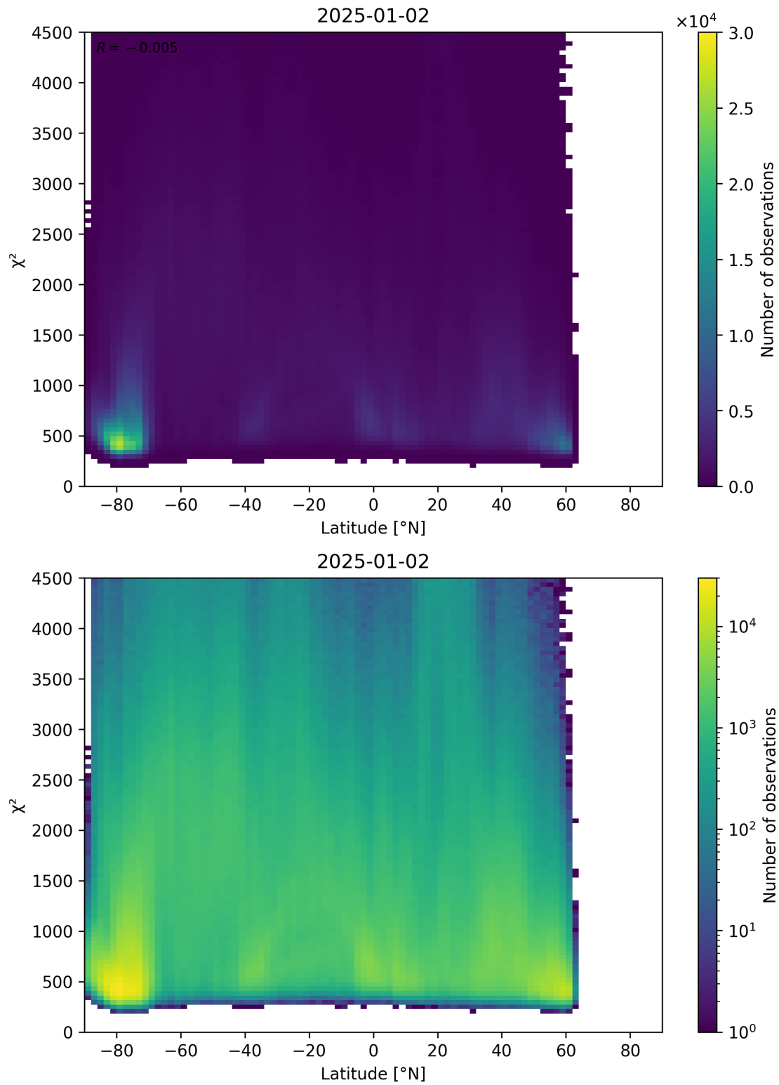
Figure 54: Scatter density plot of “Latitude” against “ \chi^2 ” for 2025-01-01 to 2025-01-03.
