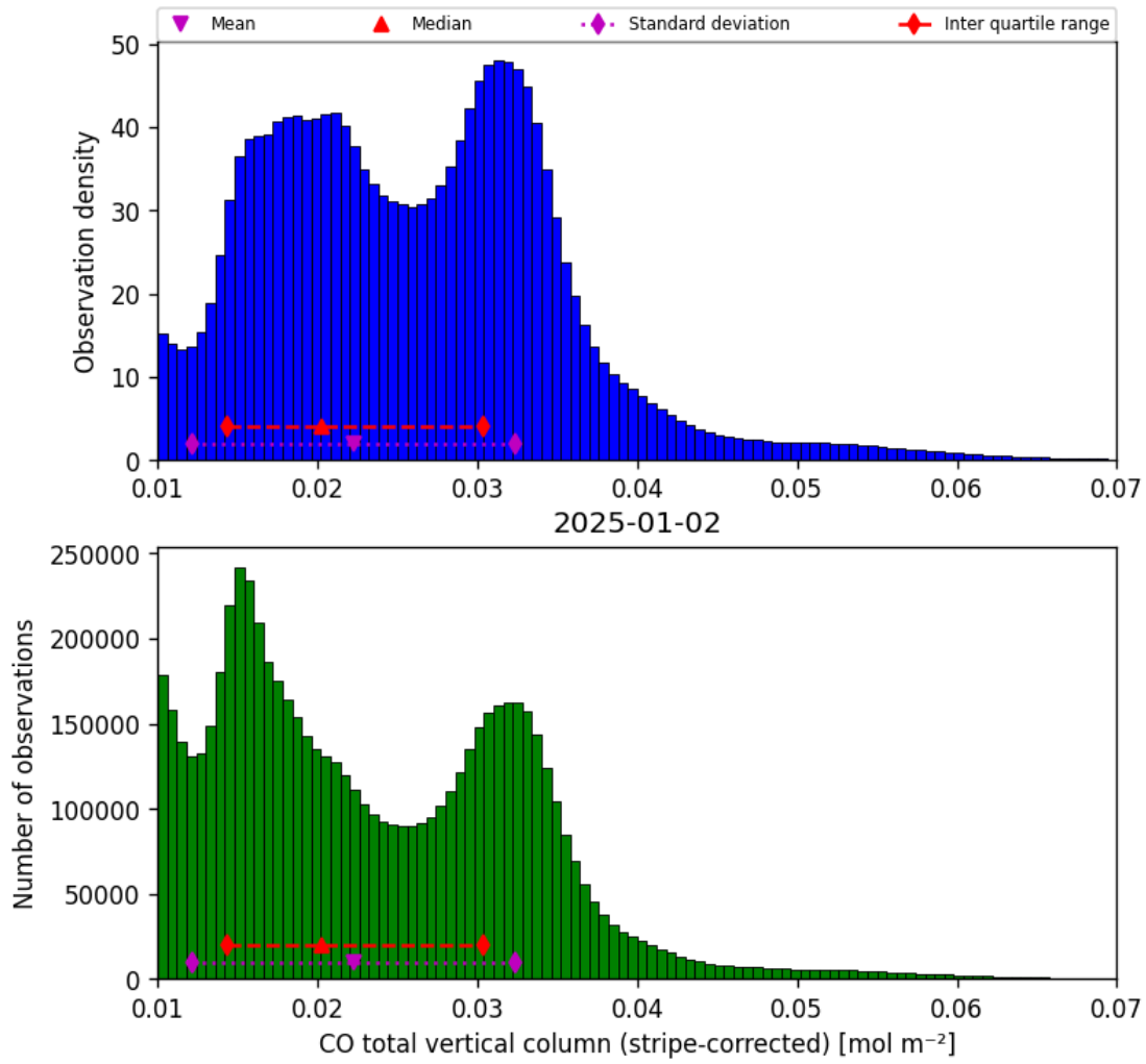
Figure 19: Histogram of “CO total vertical column (stripe-corrected)” for 2025-01-01 to 2025-01-03
