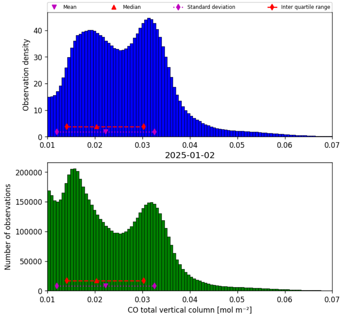
Figure 18: Histogram of “CO total vertical column” for 2025-01-01 to 2025-01-03
