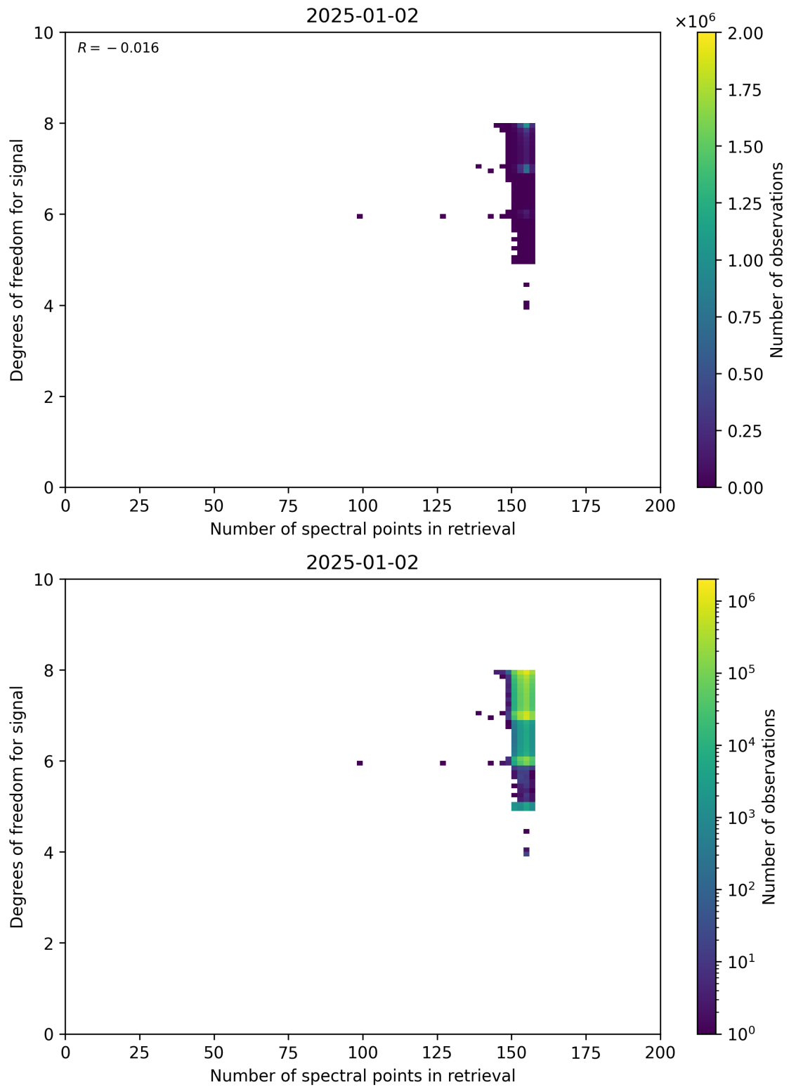
Figure 59: Scatter density plot of “Number of spectral points in retrieval” against “Degrees of freedom for signal” for 2025-01-01 to 2025-01-03.
