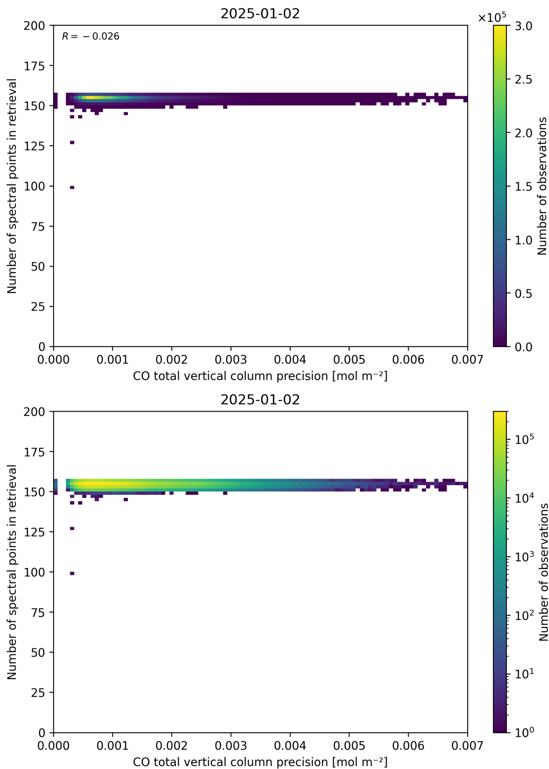
Figure 47: Scatter density plot of “CO total vertical column precision” against “Number of spectral points in retrieval” for 2025-01-01 to 2025-01-03.
