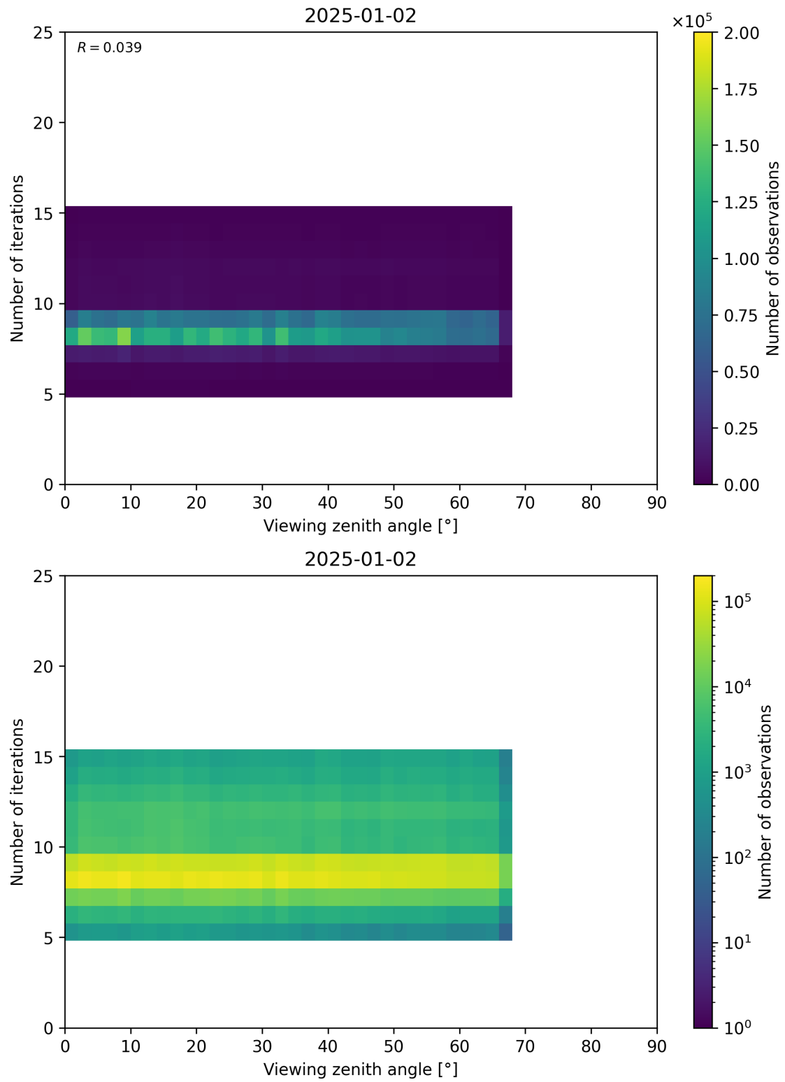
Figure 75: Scatter density plot of “Viewing zenith angle” against “Number of iterations” for 2025-01-01 to 2025-01-03.
