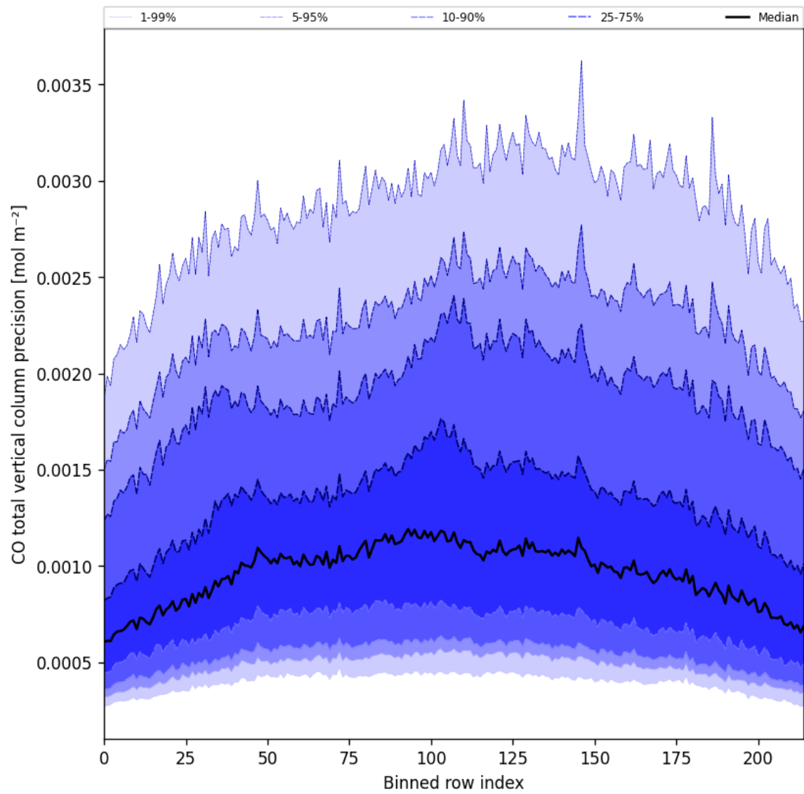
Figure 28: Along track statistics of “CO total vertical column precision” for 2025-01-01 to 2025-01-03
