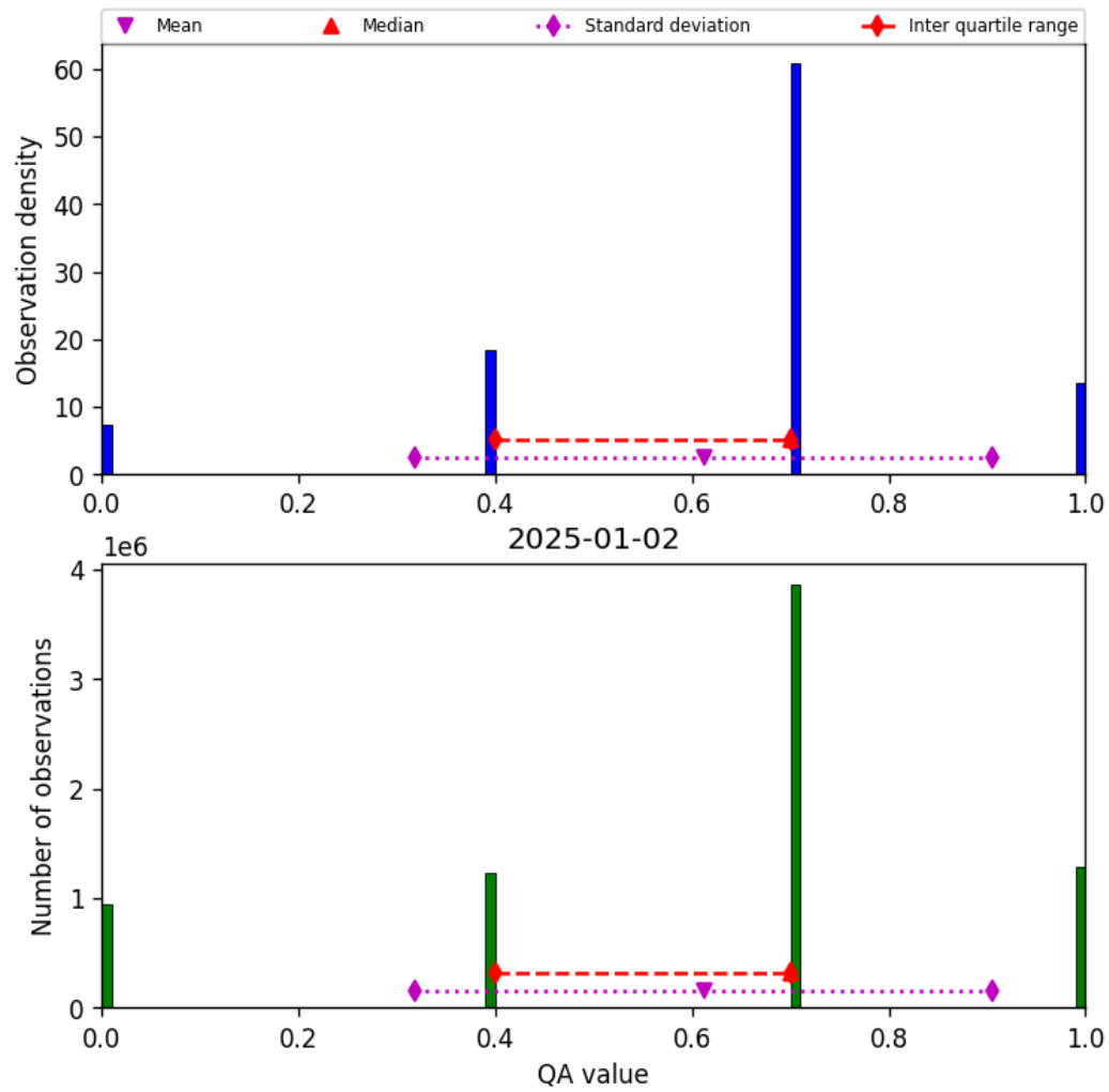
Figure 17: Histogram of "QA value" for 2025-01-01 to 2025-01-03
