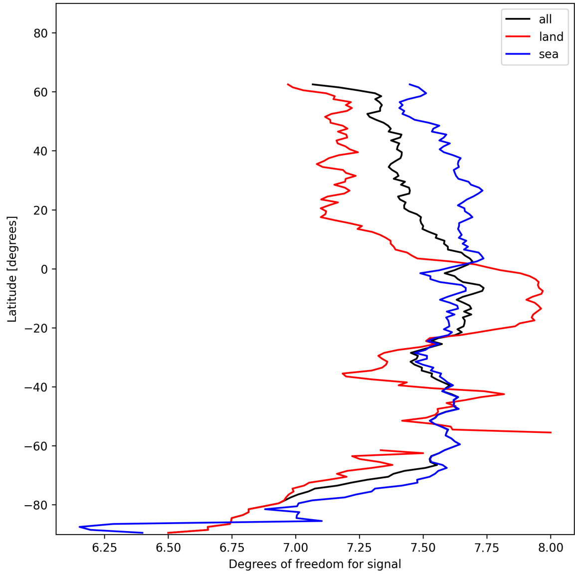
Figure 15: Zonal average of “Degrees of freedom for signal” for 2025-01-01 to 2025-01-03.
