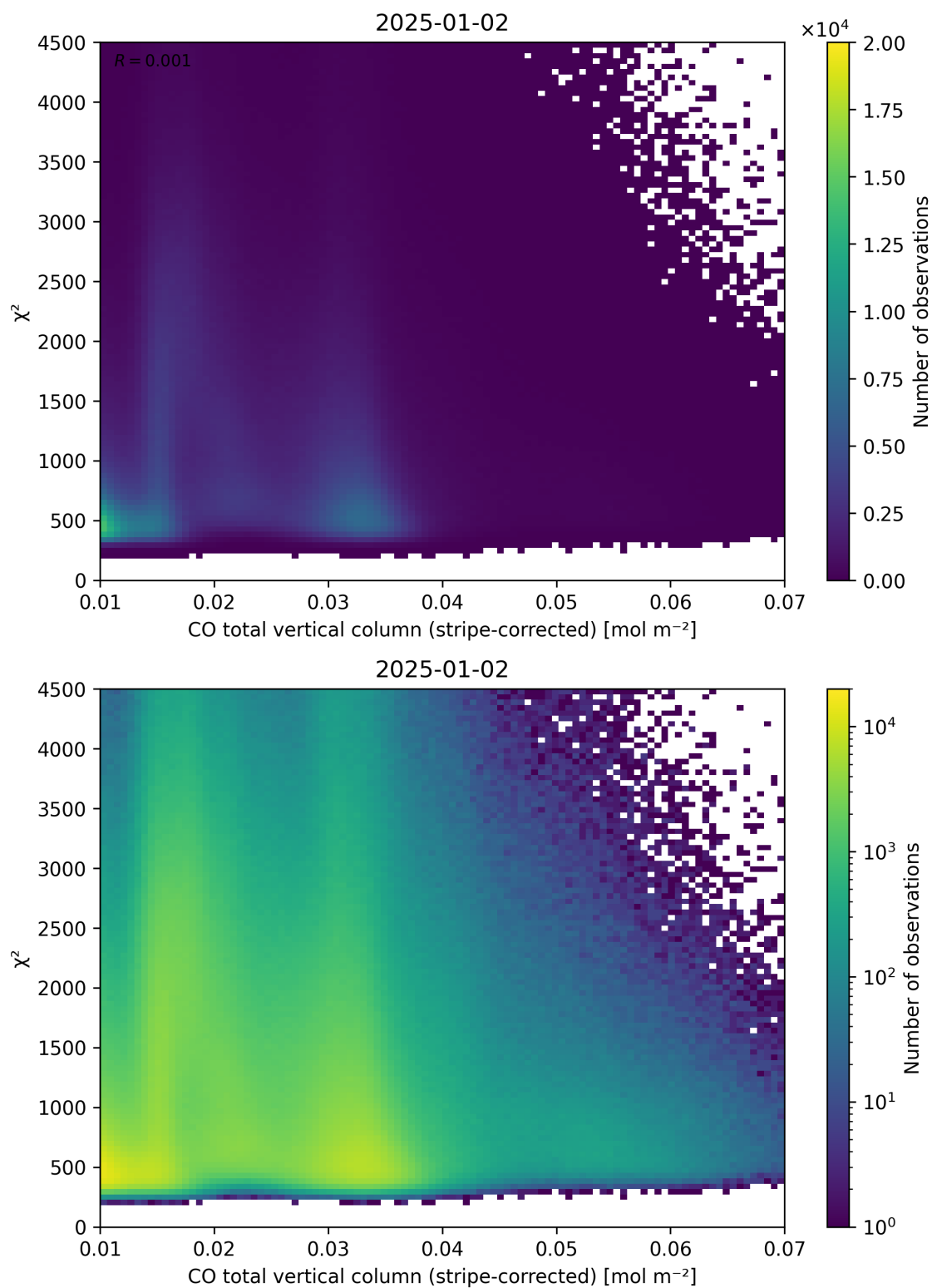
Figure 37: Scatter density plot of “CO total vertical column (stripe-corrected)” against “ \chi^2 ” for 2025-01-01 to 2025-01-03.
