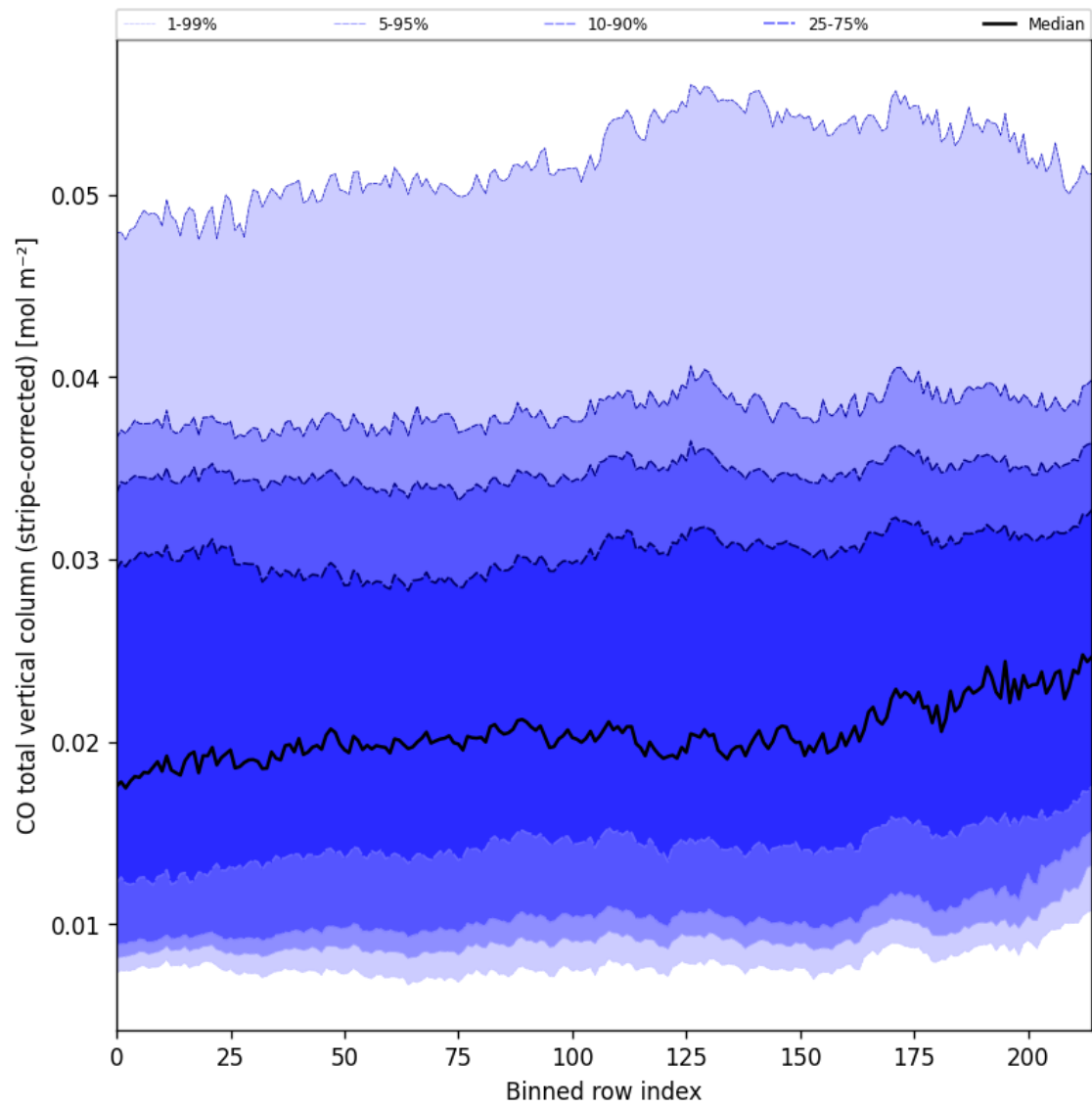
Figure 27: Along track statistics of “CO total vertical column (stripe-corrected)” for 2025-01-01 to 2025-01-03
