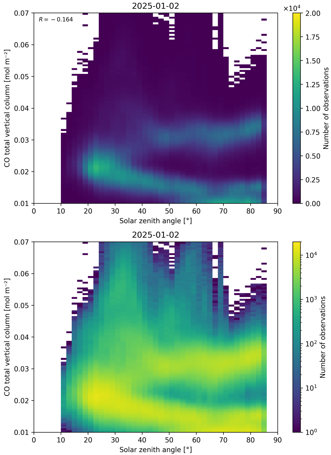
Figure 61: Scatter density plot of “Solar zenith angle” against “CO total vertical column” for 2025-01-01 to 2025-01-03.
