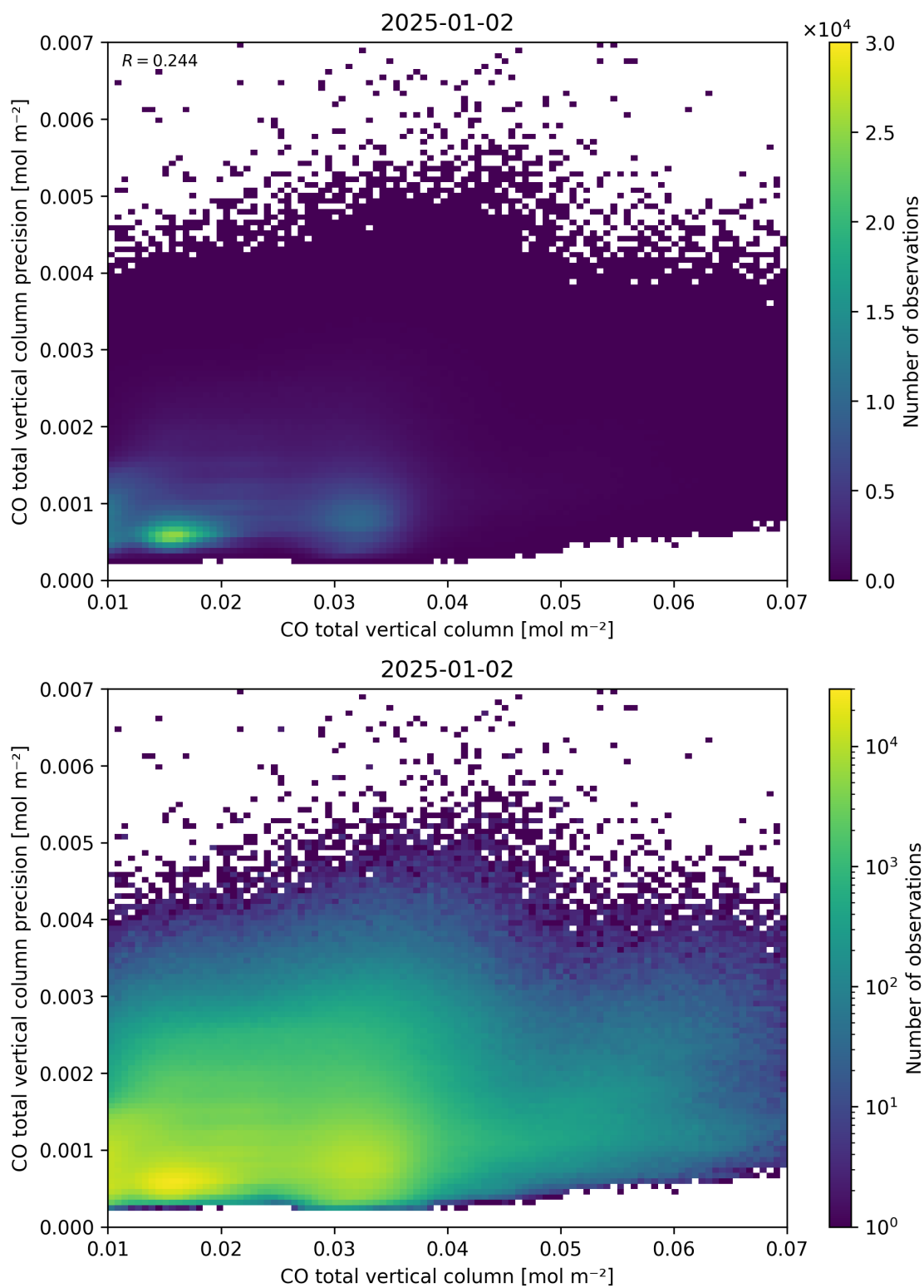
Figure 34: Scatter density plot of “CO total vertical column” against “CO total vertical column precision” for 2025-01-01 to 2025-01-03.
