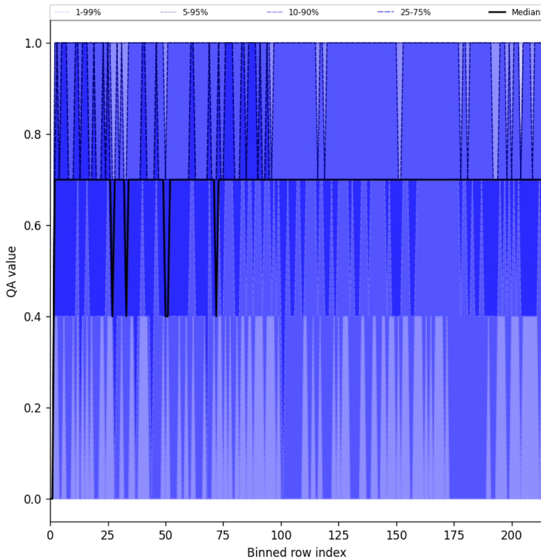
Figure 25: Along track statistics of “QA value” for 2025-01-01 to 2025-01-03
