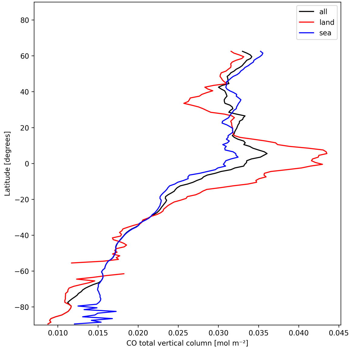
Figure 10: Zonal average of “CO total vertical column” for 2025-01-01 to 2025-01-03.
