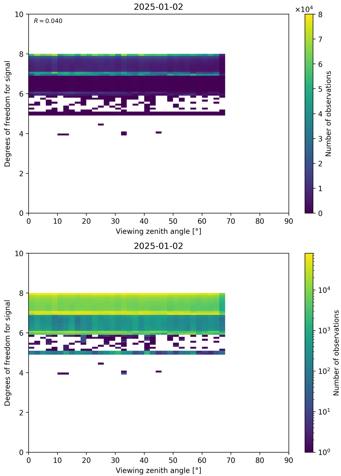
Figure 73: Scatter density plot of “Viewing zenith angle” against “Degrees of freedom for signal” for 2025-01-01 to 2025-01-03.
