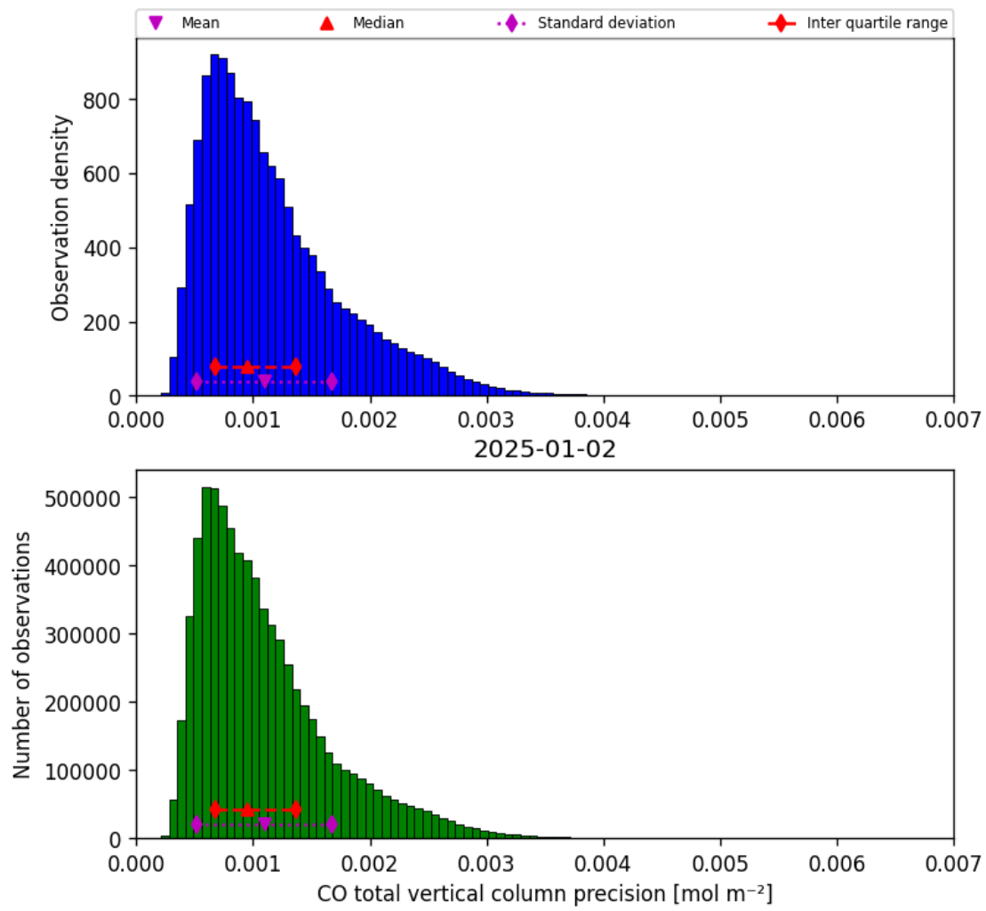
Figure 20: Histogram of “CO total vertical column precision” for 2025-01-01 to 2025-01-03
