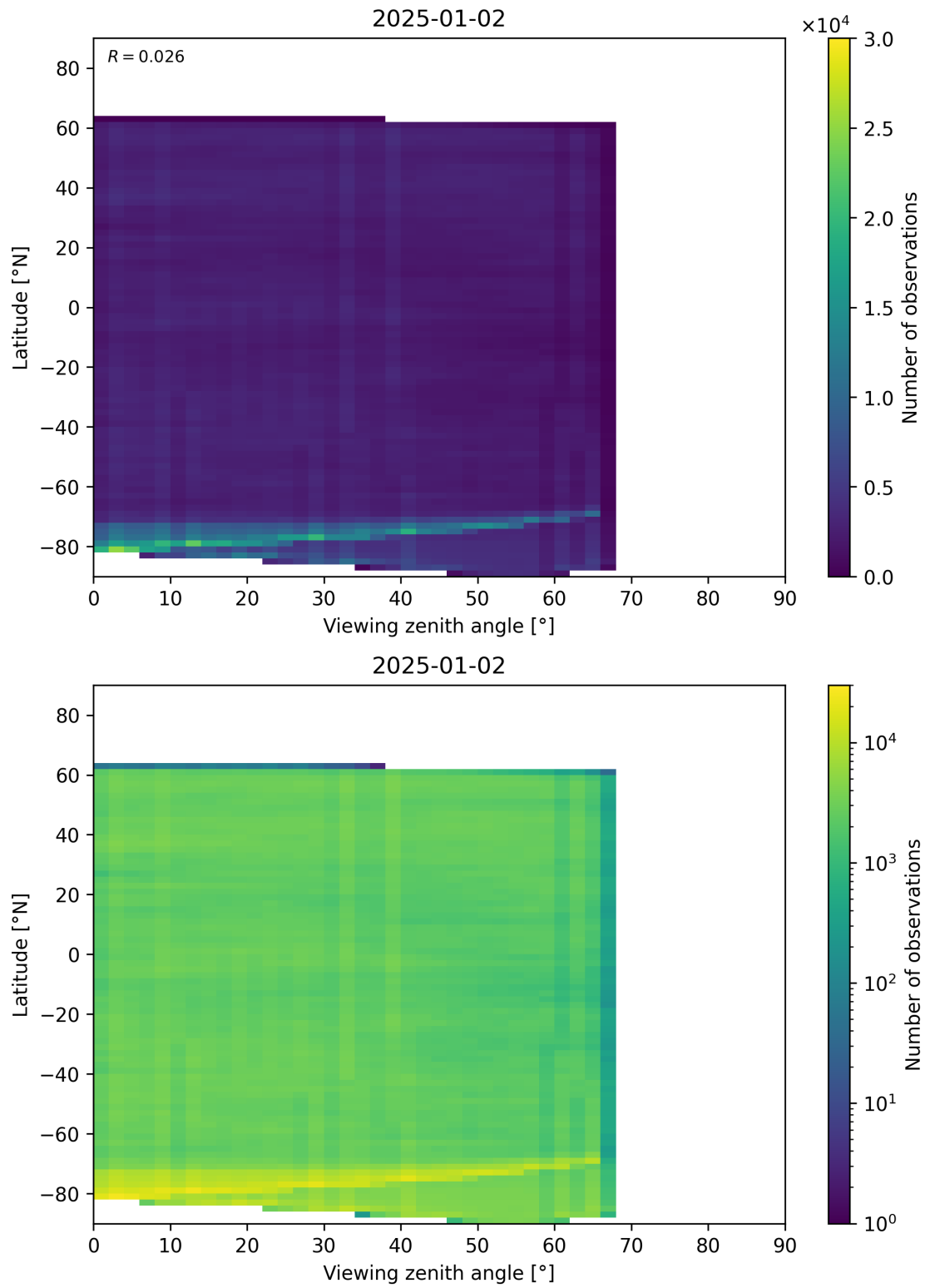
Figure 74: Scatter density plot of “Viewing zenith angle” against “Latitude” for 2025-01-01 to 2025-01-03.
