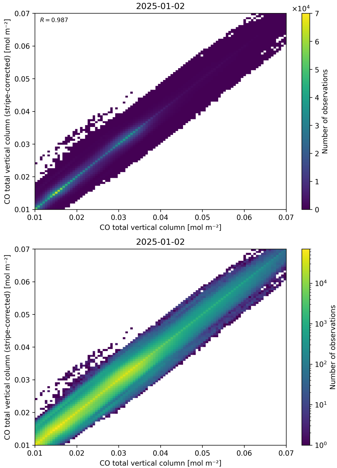
Figure 33: Scatter density plot of “CO total vertical column” against “CO total vertical column (stripe-corrected)” for 2025-01-01 to 2025-01-03.
