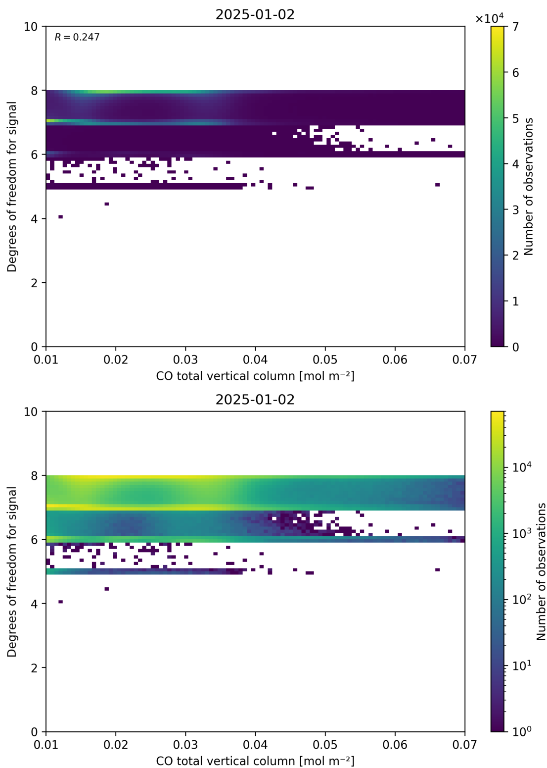
Figure 41: Scatter density plot of “CO total vertical column” against “Degrees of freedom for signal” for 2025-01-01 to 2025-01-03.
