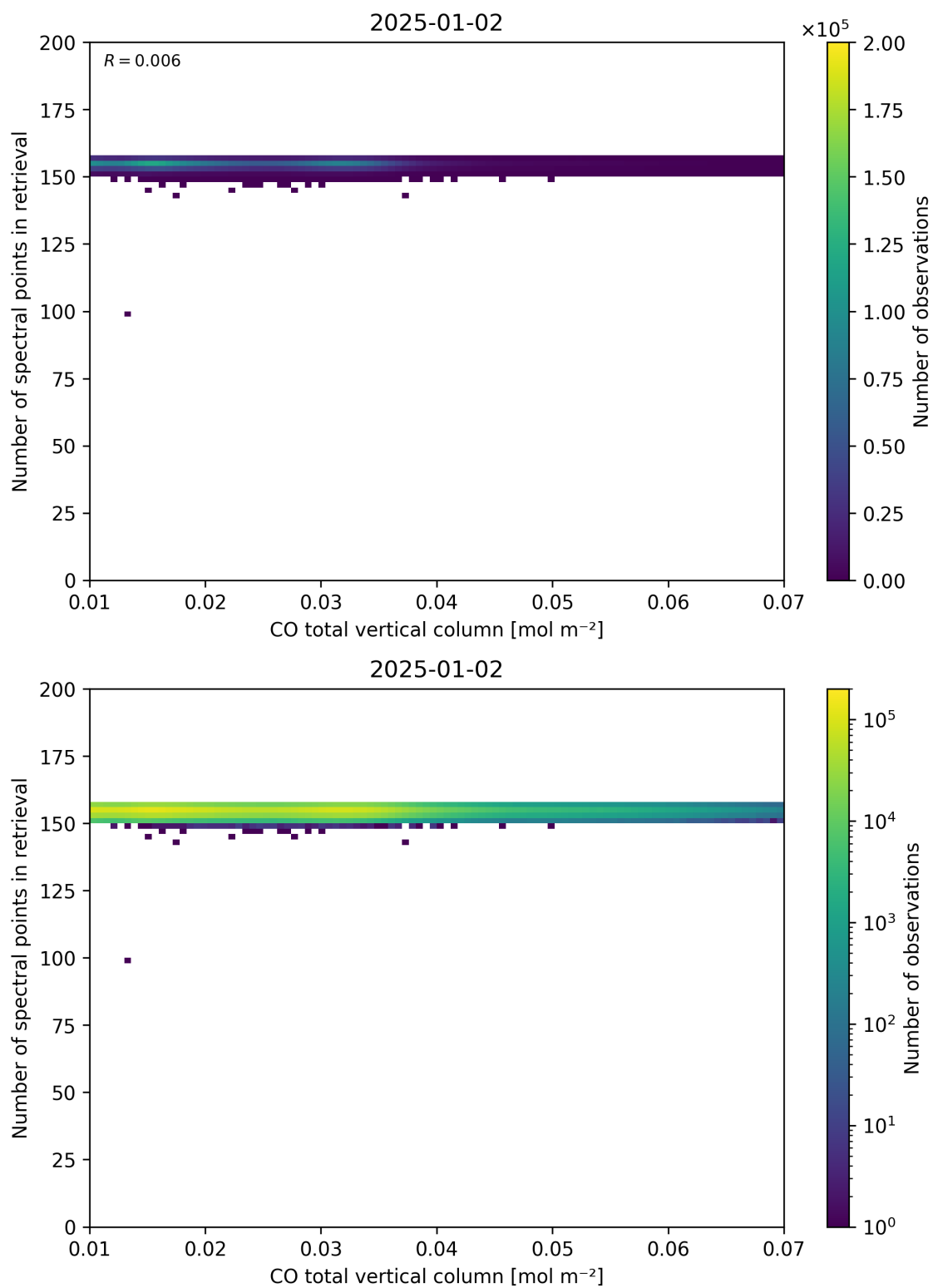
Figure 43: Scatter density plot of “CO total vertical column” against “Number of spectral points in retrieval” for 2025-01-01 to 2025-01-03.
