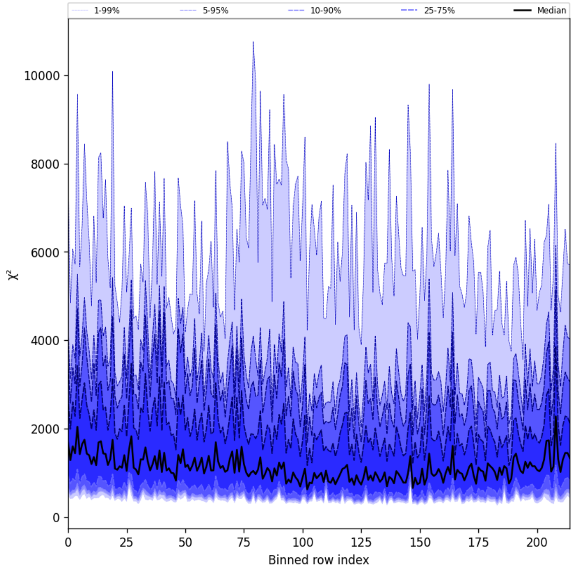
Figure 30: Along track statistics of “ \chi^2 ” for 2025-01-01 to 2025-01-03
