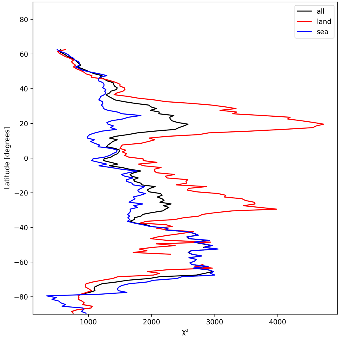
Figure 14: Zonal average of “ \chi^2 ” for 2025-01-01 to 2025-01-03.
