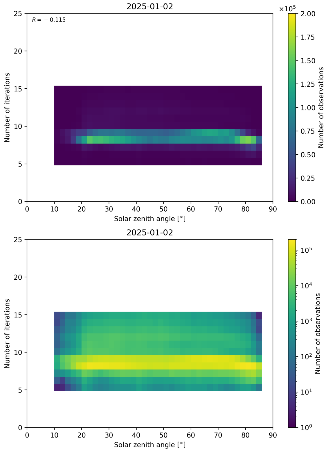
Figure 67: Scatter density plot of “Solar zenith angle” against “Number of iterations” for 2025-01-01 to 2025-01-03.
