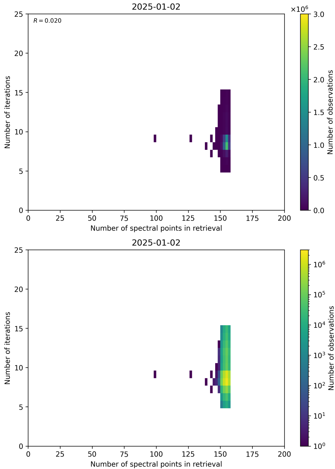
Figure 60: Scatter density plot of “Number of spectral points in retrieval” against “Number of iterations” for 2025-01-01 to 2025-01-03.
