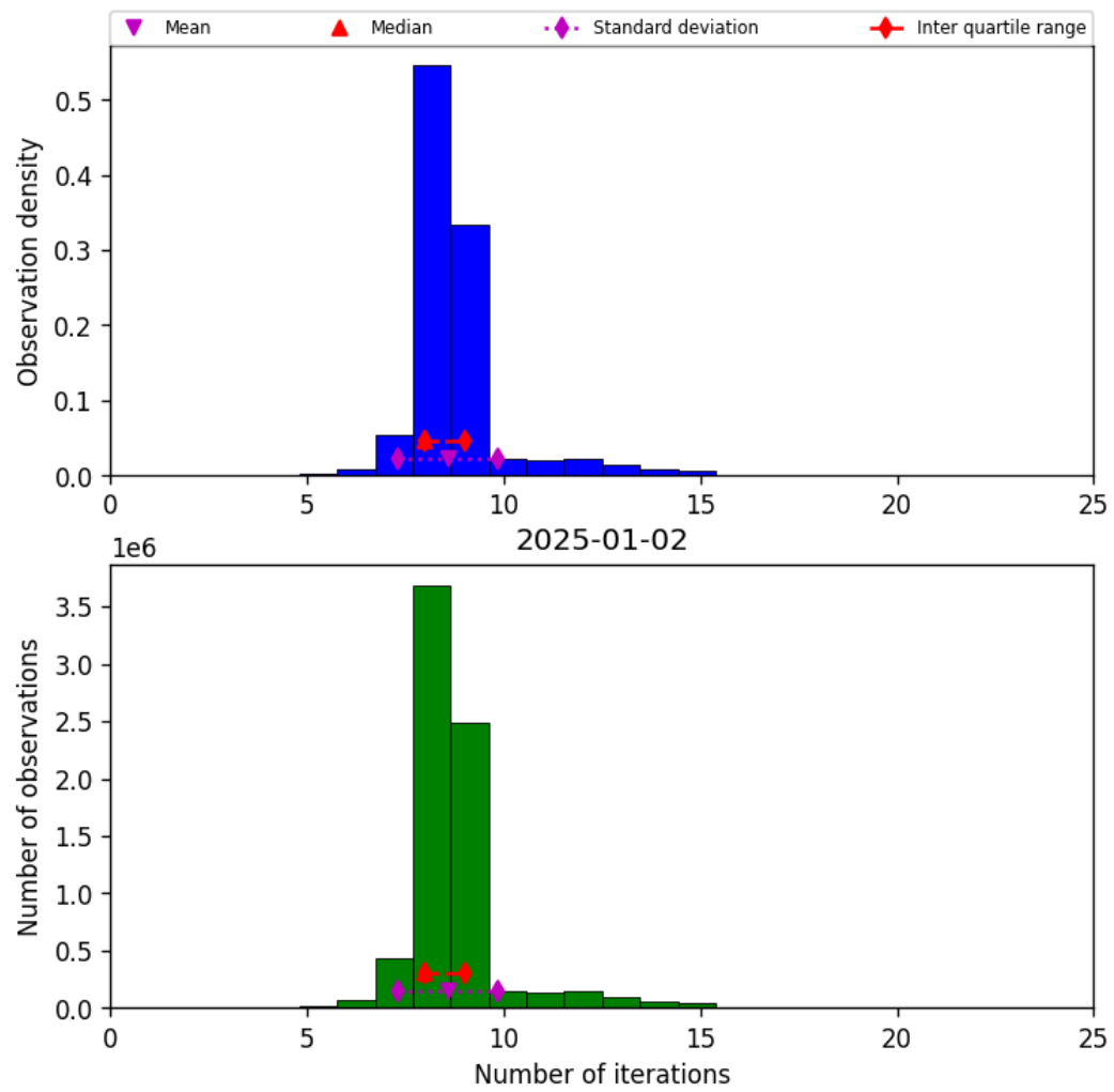
Figure 24: Histogram of “Number of iterations” for 2025-01-01 to 2025-01-03
