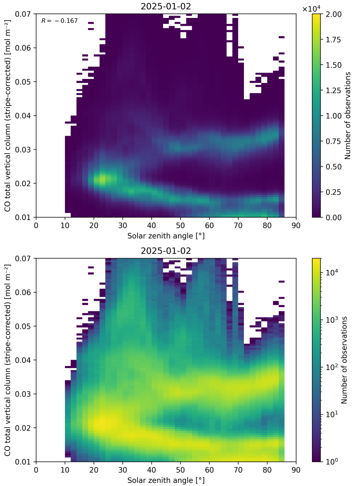
Figure 62: Scatter density plot of “Solar zenith angle” against “CO total vertical column (stripe-corrected)” for 2025-01-01 to 2025-01-03.
