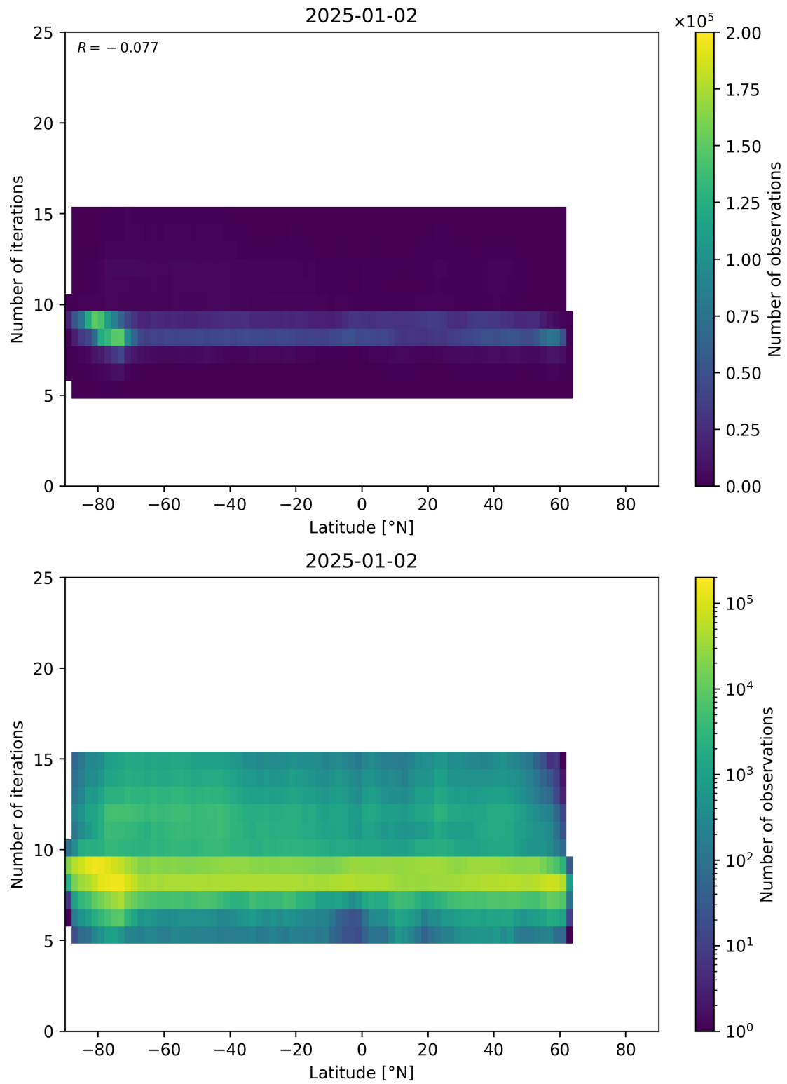
Figure 56: Scatter density plot of “Latitude” against “Number of iterations” for 2025-01-01 to 2025-01-03.
