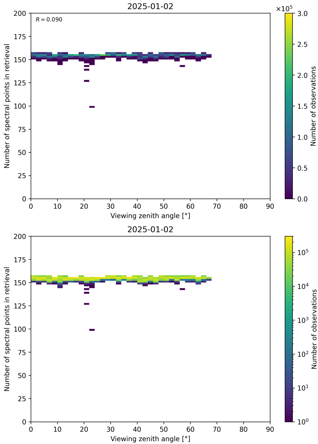
Figure 76: Scatter density plot of “Viewing zenith angle” against “Number of spectral points in retrieval” for 2025-01-01 to 2025-01-03.
