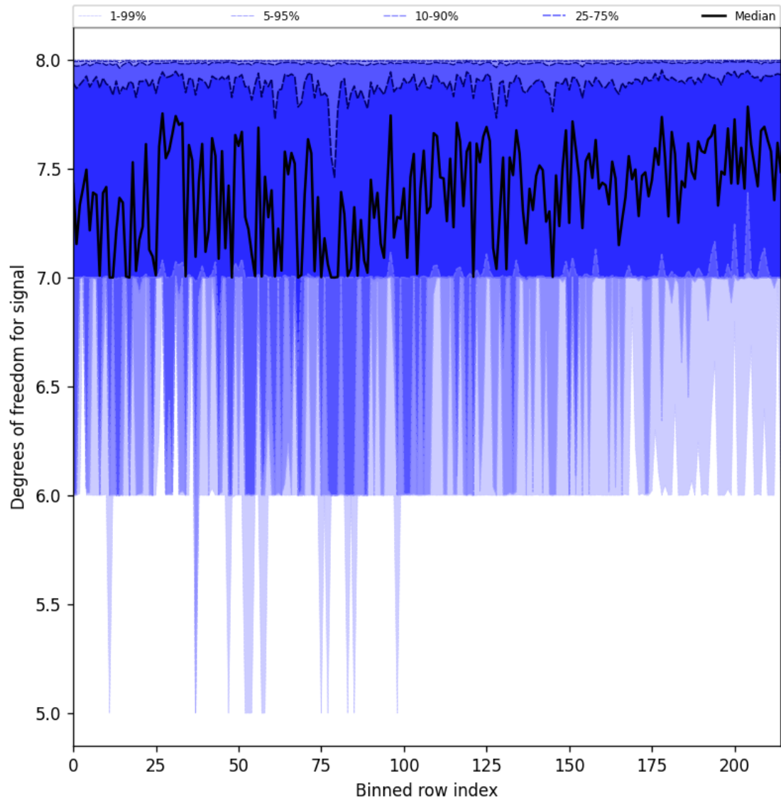
Figure 31: Along track statistics of “Degrees of freedom for signal” for 2025-01-01 to 2025-01-03
