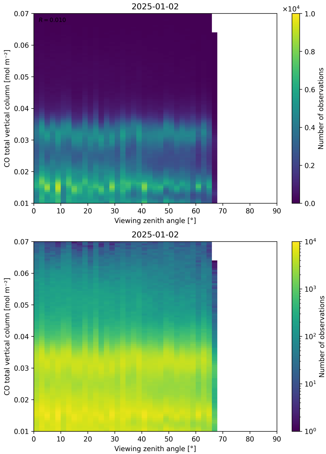
Figure 69: Scatter density plot of “Viewing zenith angle” against “CO total vertical column” for 2025-01-01 to 2025-01-03.
