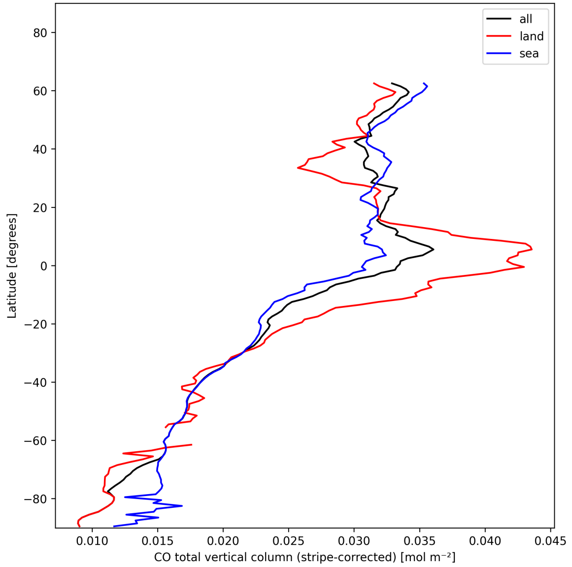
Figure 11: Zonal average of “CO total vertical column (stripe-corrected)” for 2025-01-01 to 2025-01-03.
