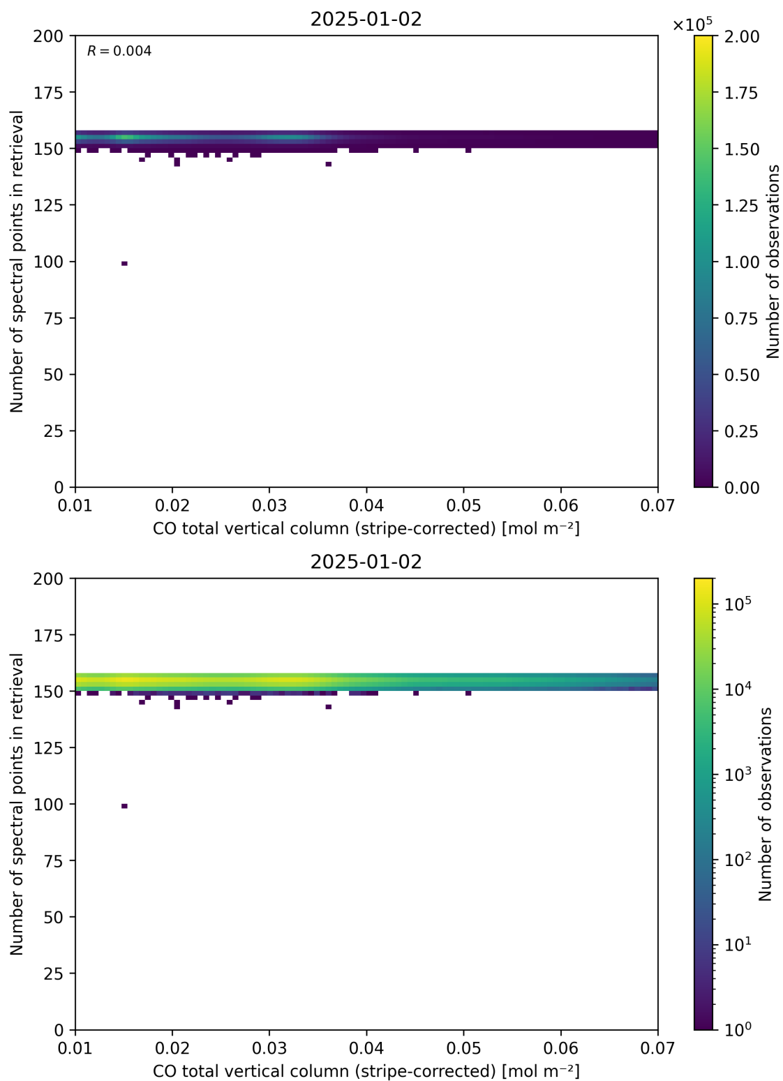
Figure 40: Scatter density plot of “CO total vertical column (stripe-corrected)” against “Number of spectral points in retrieval” for 2025-01-01 to 2025-01-03.
