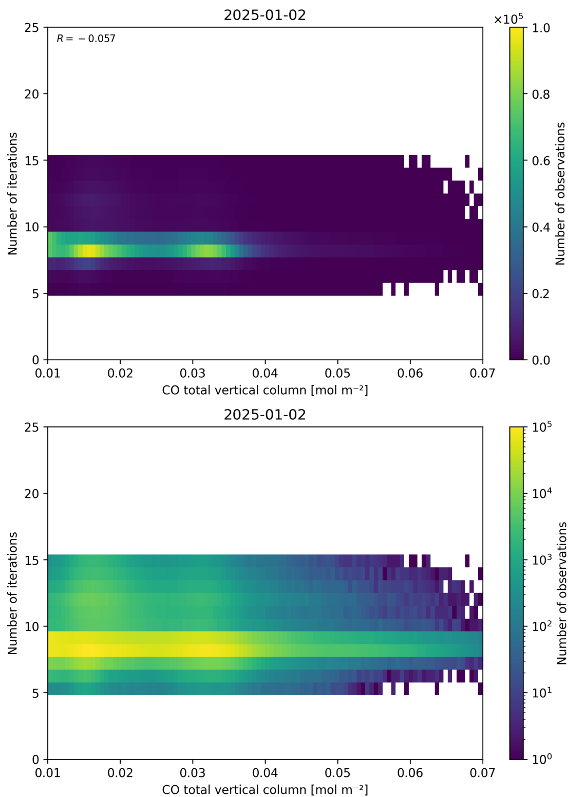
Figure 42: Scatter density plot of “CO total vertical column” against “Number of iterations” for 2025-01-01 to 2025-01-03.
