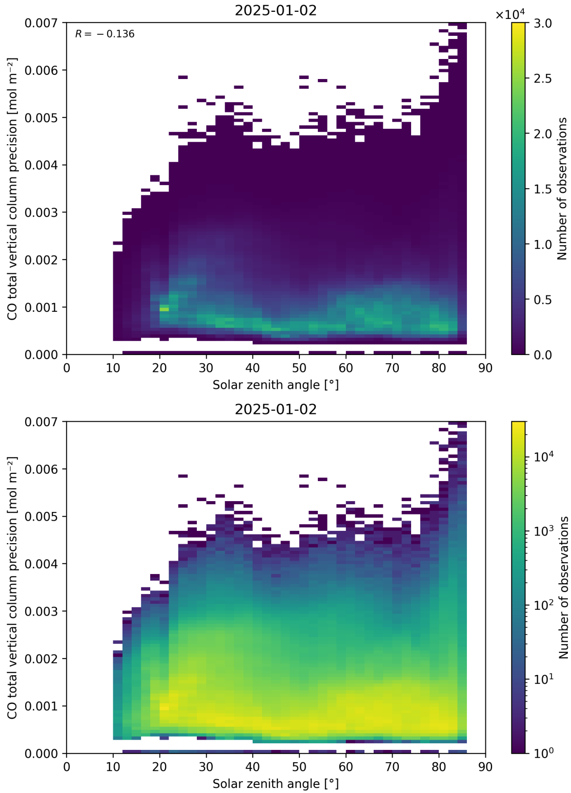
Figure 63: Scatter density plot of “Solar zenith angle” against “CO total vertical column precision” for 2025-01-01 to 2025-01-03.
