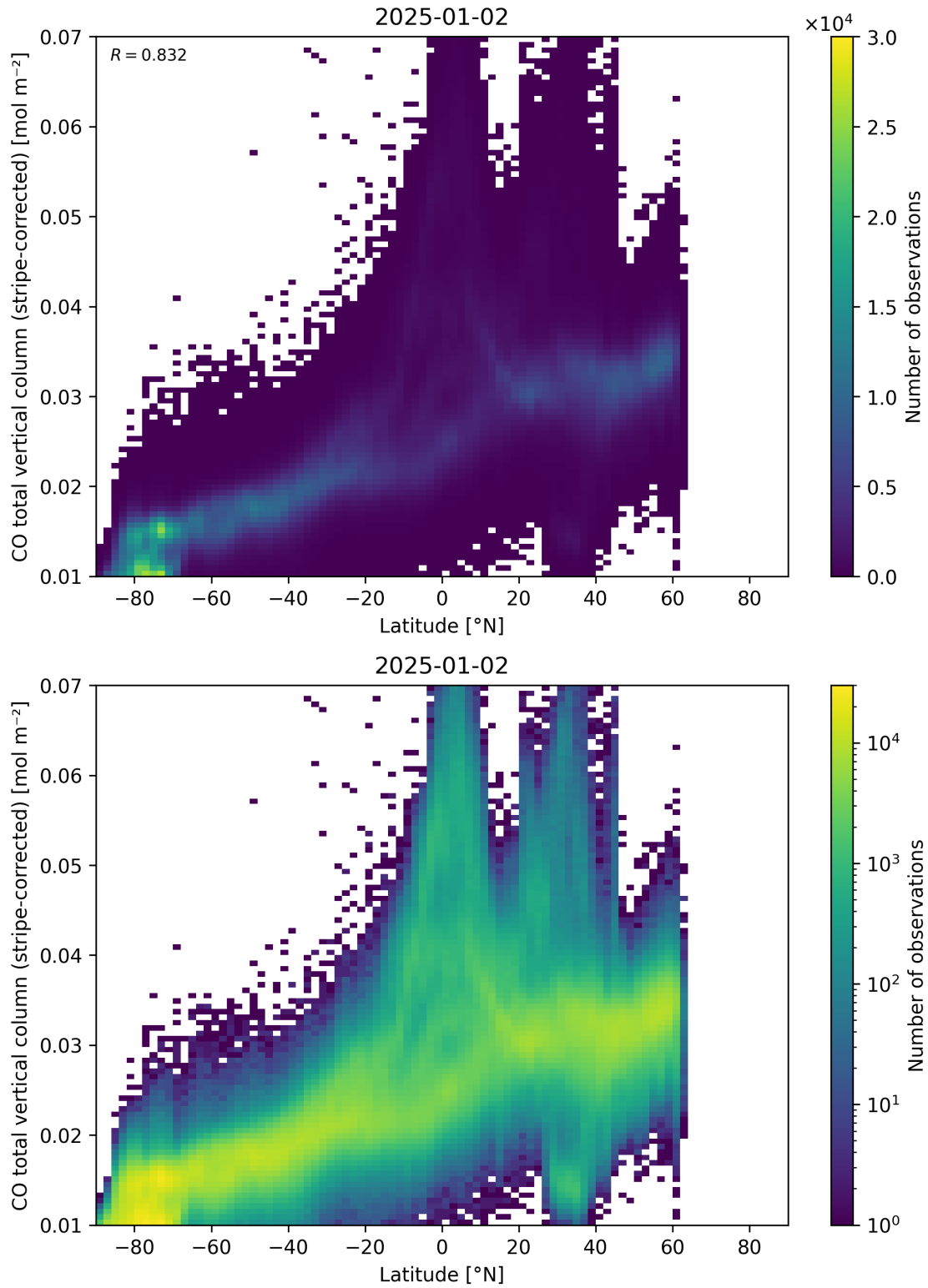
Figure 52: Scatter density plot of “Latitude” against “CO total vertical column (stripe-corrected)” for 2025-01-01 to 2025-01-03.
