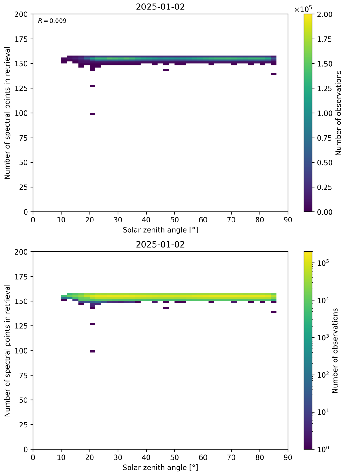
Figure 68: Scatter density plot of “Solar zenith angle” against “Number of spectral points in retrieval” for 2025-01-01 to 2025-01-03.
