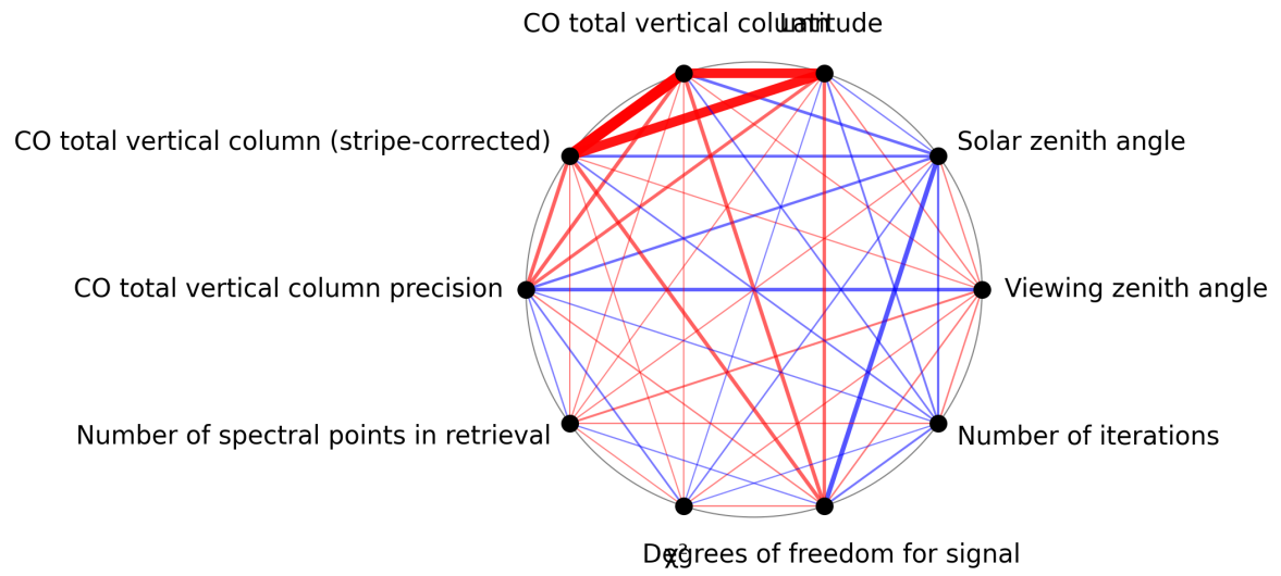
Figure 1: Map of correlation graph for 2025-01-01 to 2025-01-03.
