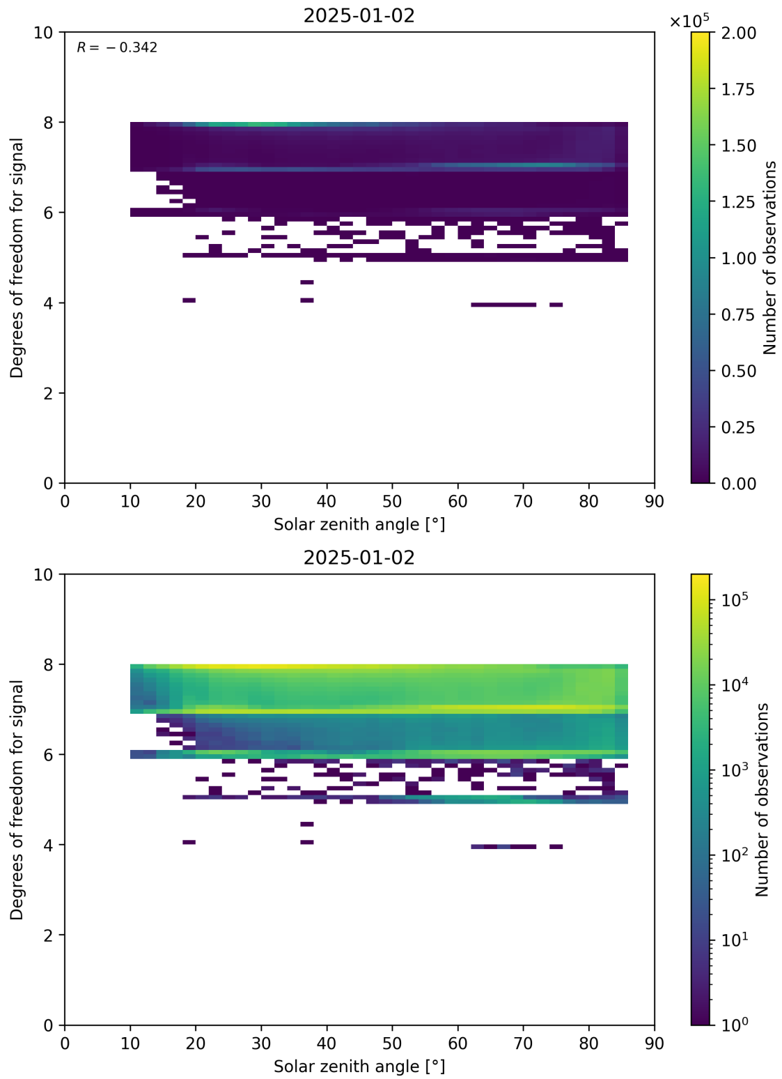
Figure 65: Scatter density plot of “Solar zenith angle” against “Degrees of freedom for signal” for 2025-01-01 to 2025-01-03.
