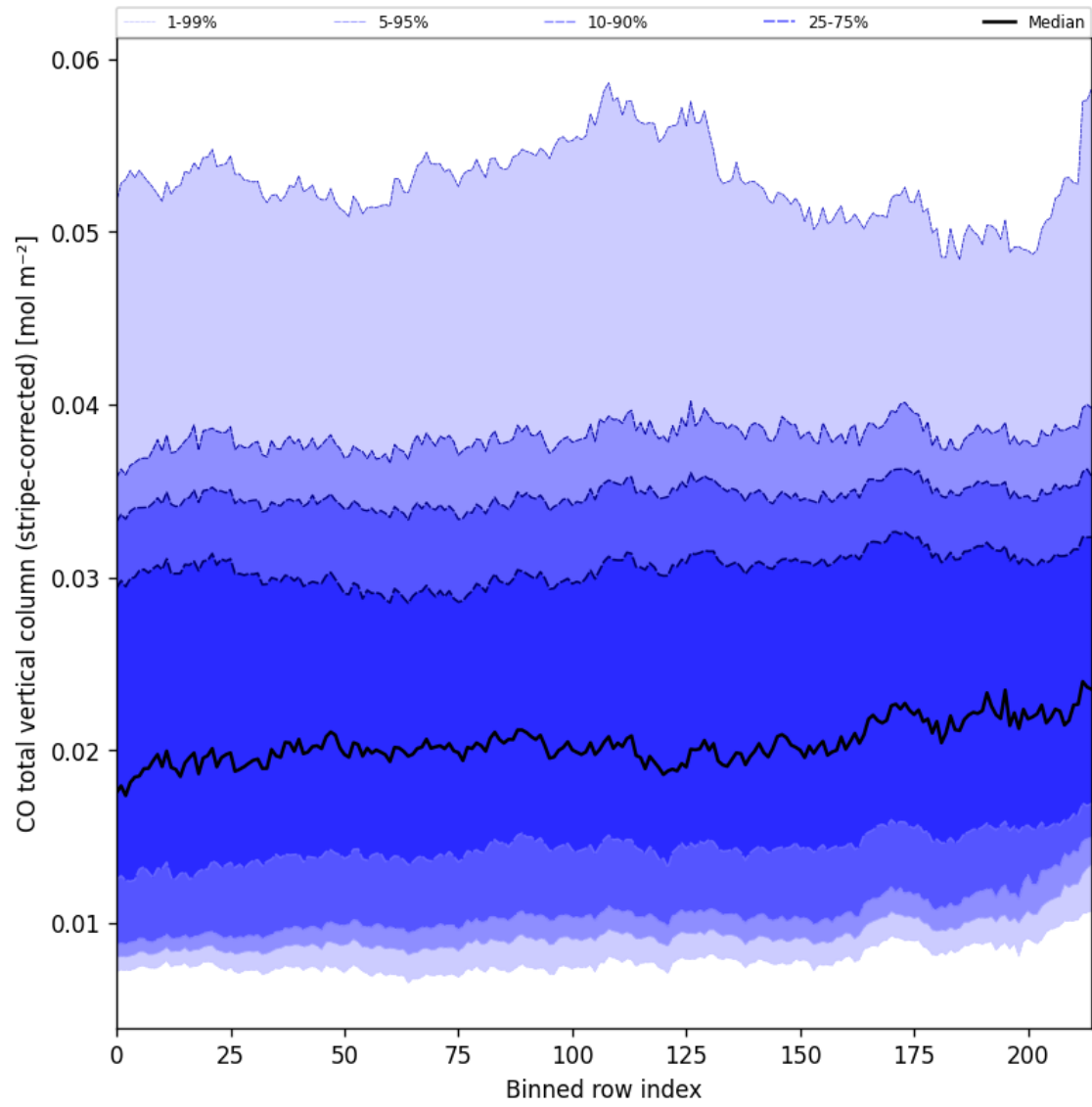
Figure 27: Along track statistics of “CO total vertical column (stripe-corrected)” for 2025-01-02 to 2025-01-04
