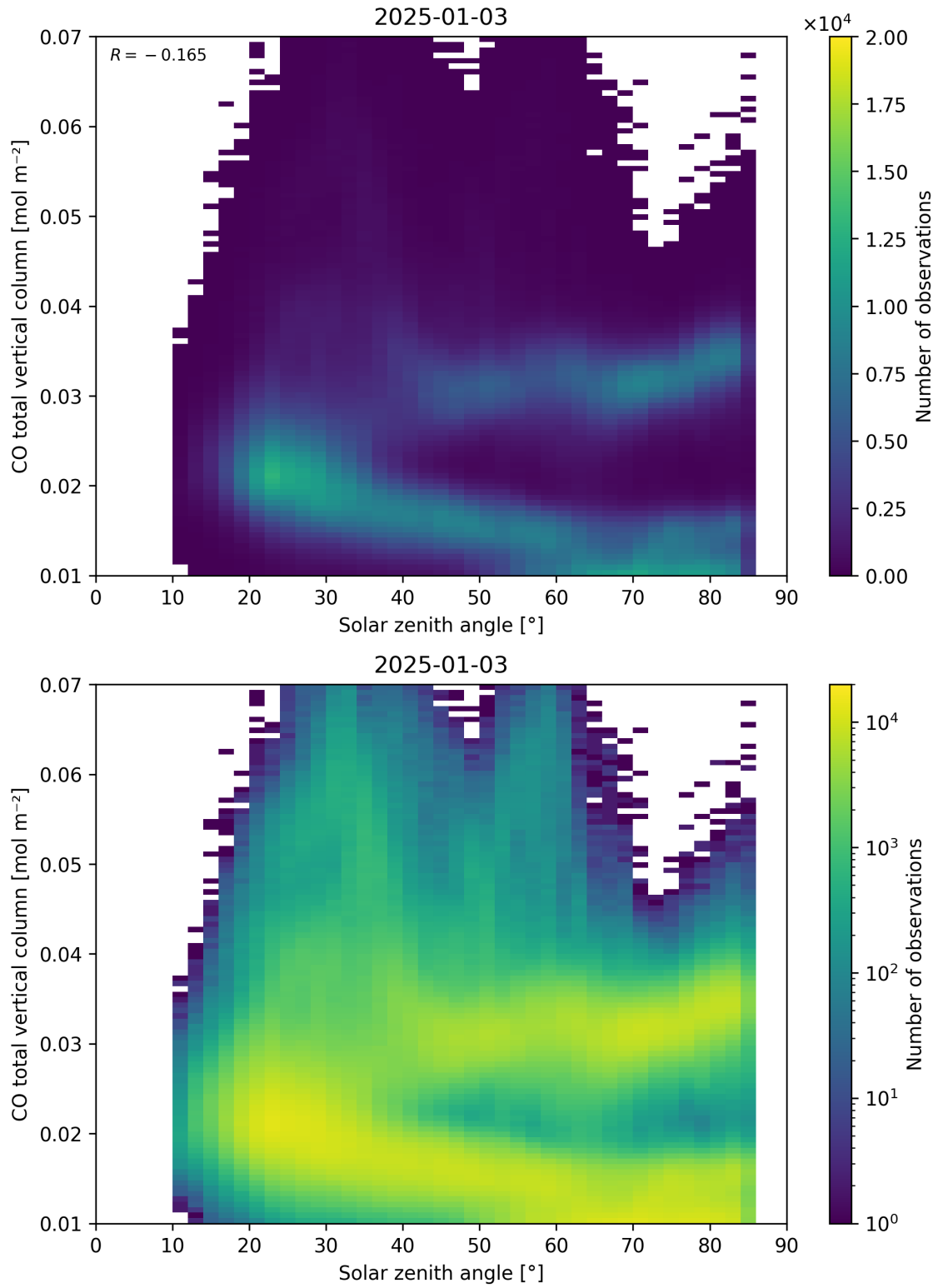
Figure 61: Scatter density plot of “Solar zenith angle” against “CO total vertical column” for 2025-01-02 to 2025-01-04.
