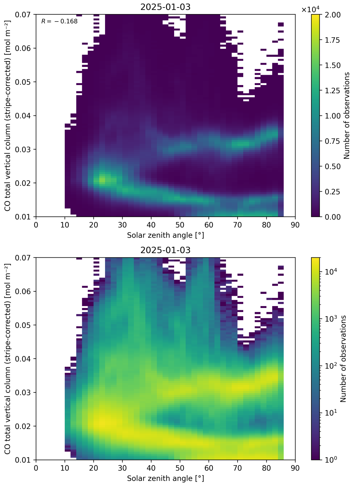
Figure 62: Scatter density plot of “Solar zenith angle” against “CO total vertical column (stripe-corrected)” for 2025-01-02 to 2025-01-04.
