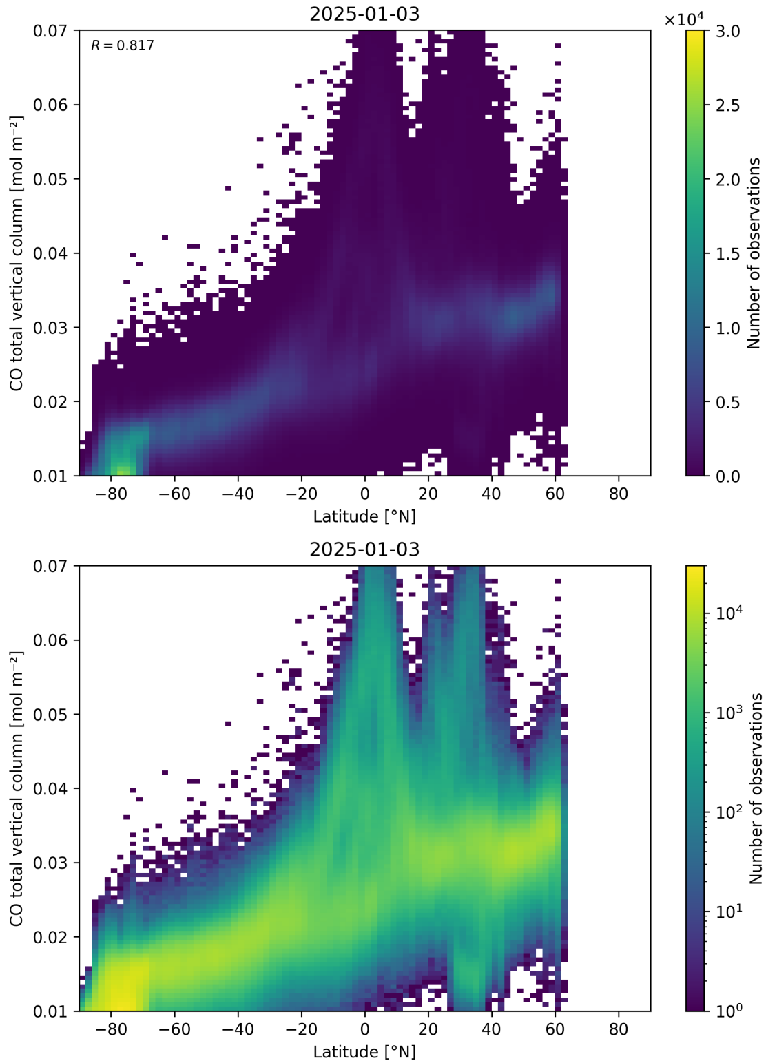
Figure 51: Scatter density plot of “Latitude” against “CO total vertical column” for 2025-01-02 to 2025-01-04.
