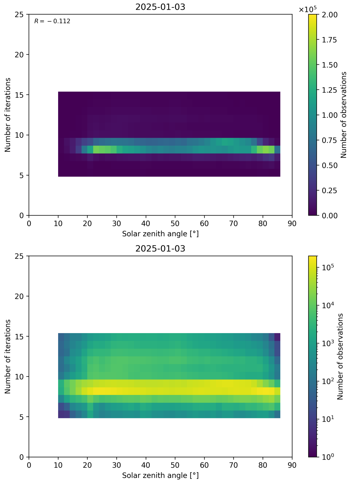
Figure 67: Scatter density plot of “Solar zenith angle” against “Number of iterations” for 2025-01-02 to 2025-01-04.
