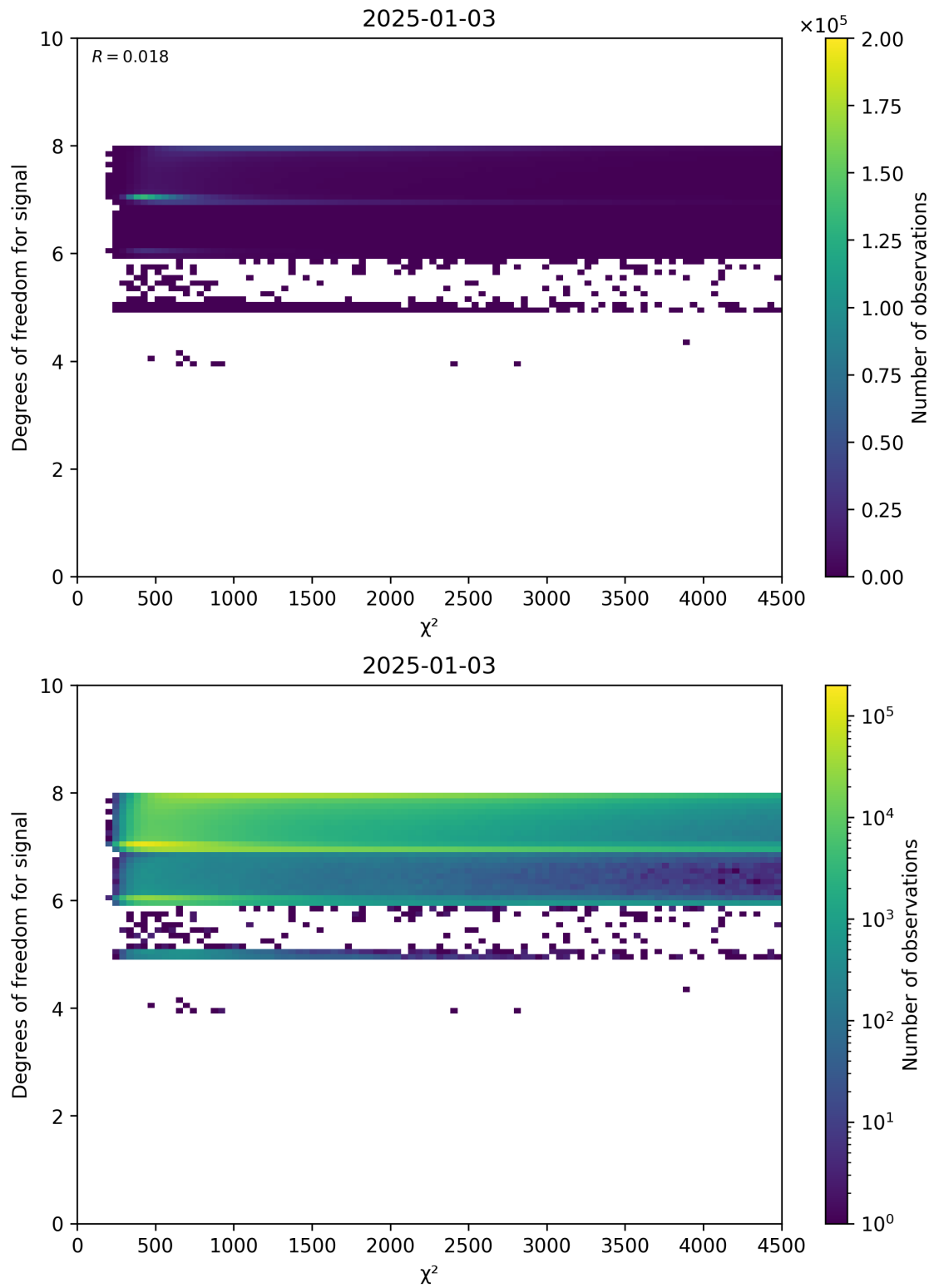
Figure 48: Scatter density plot of “ \chi^2 ” against “Degrees of freedom for signal” for 2025-01-02 to 2025-01-04.
