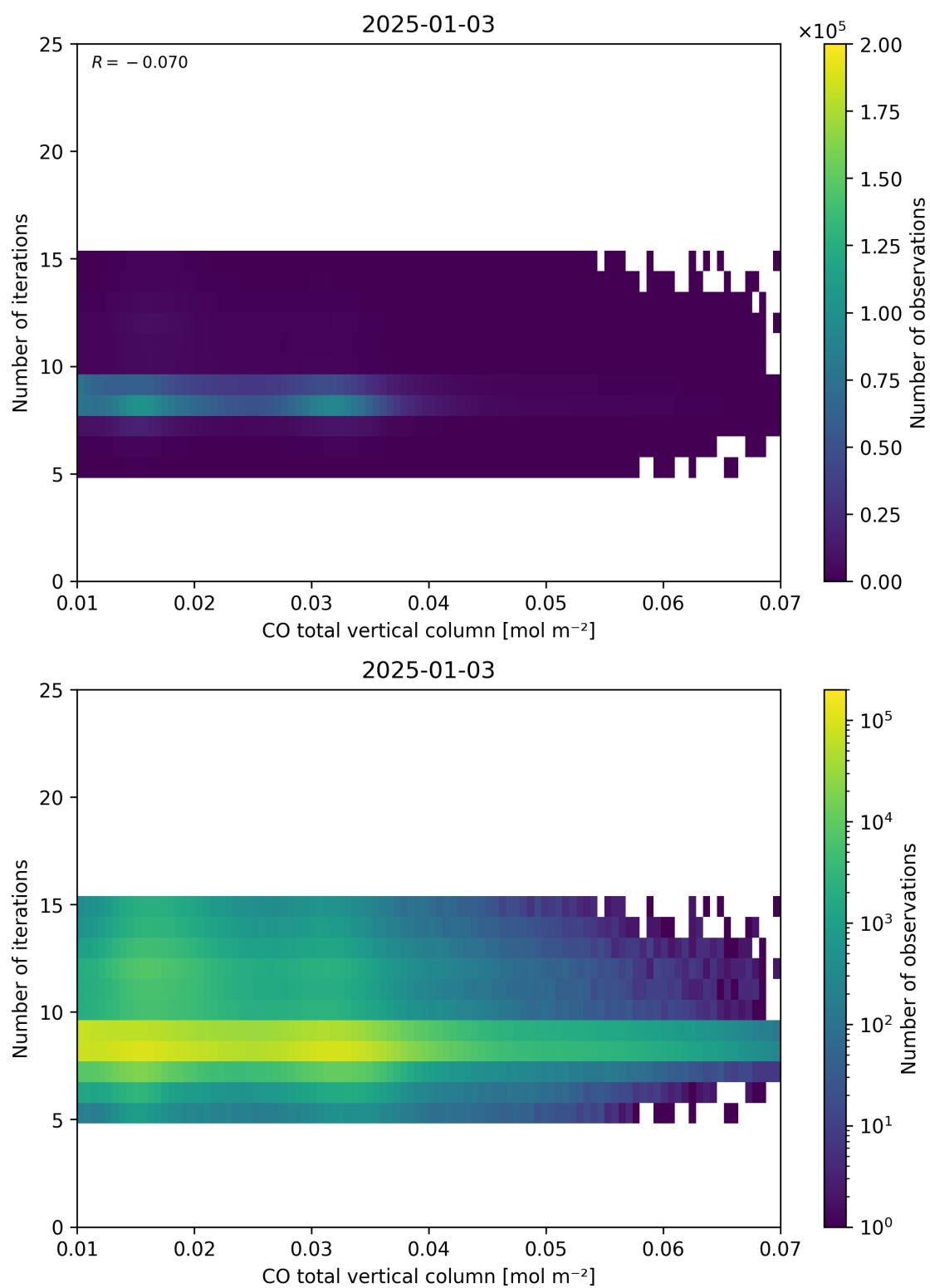
Figure 42: Scatter density plot of “CO total vertical column” against “Number of iterations” for 2025-01-02 to 2025-01-04.
