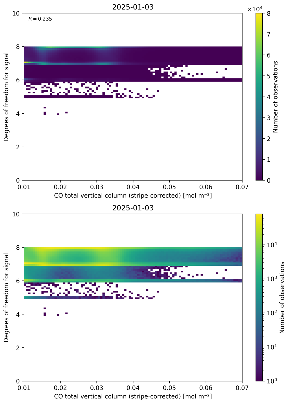
Figure 38: Scatter density plot of “CO total vertical column (stripe-corrected)” against “Degrees of freedom for signal” for 2025-01-02 to 2025-01-04.
