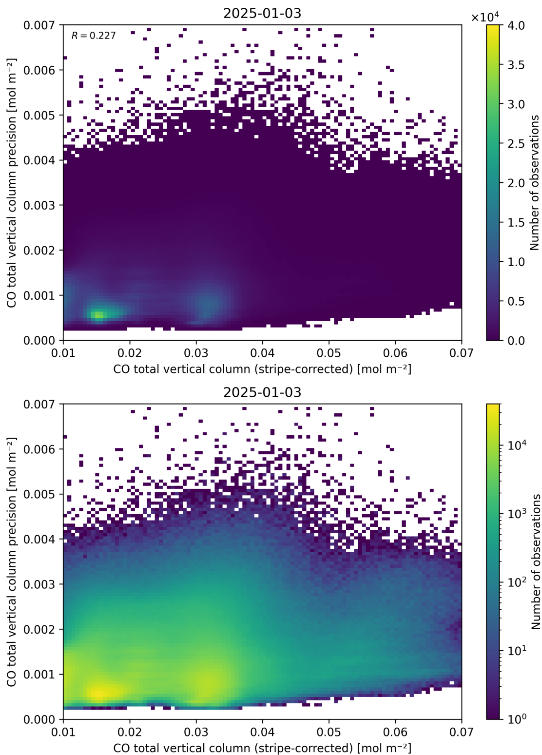
Figure 36: Scatter density plot of “CO total vertical column (stripe-corrected)” against “CO total vertical column precision” for 2025-01-02 to 2025-01-04.
