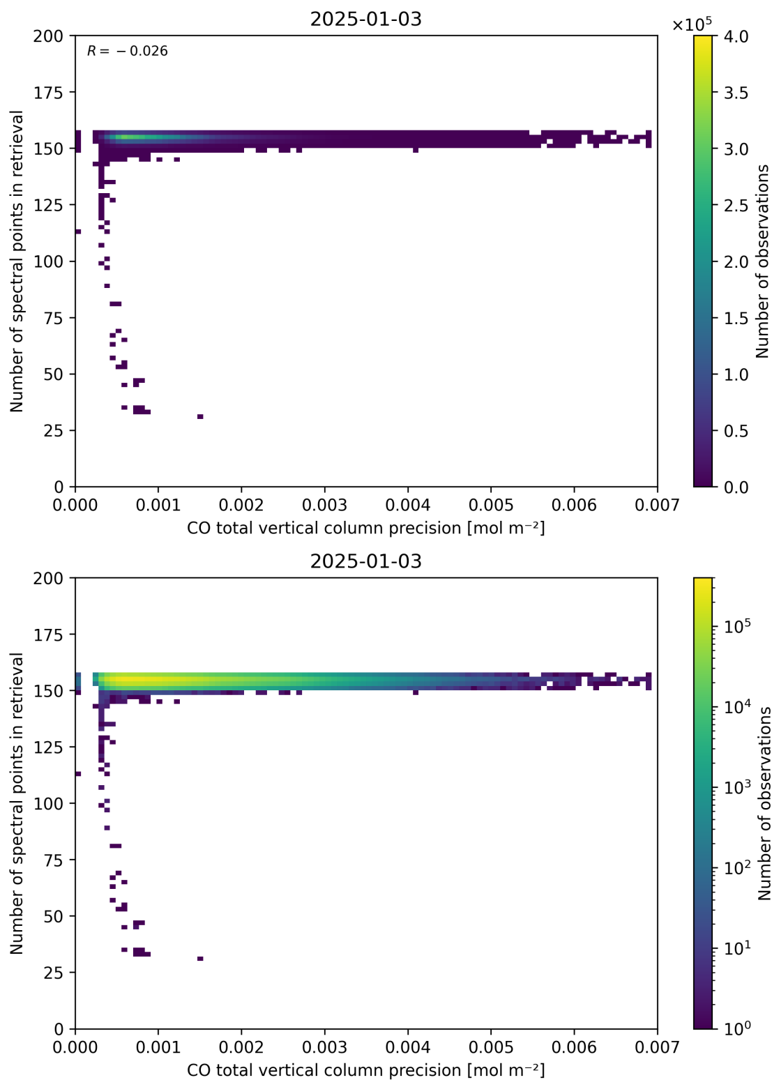
Figure 47: Scatter density plot of “CO total vertical column precision” against “Number of spectral points in retrieval” for 2025-01-02 to 2025-01-04.
