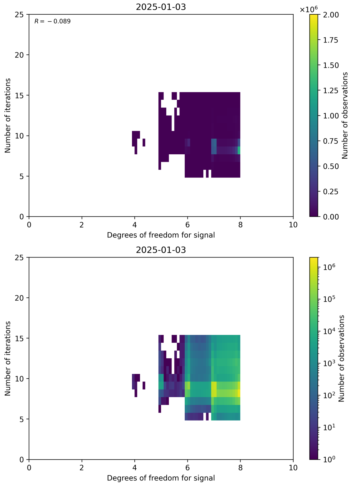
Figure 50: Scatter density plot of “Degrees of freedom for signal” against “Number of iterations” for 2025-01-02 to 2025-01-04.
