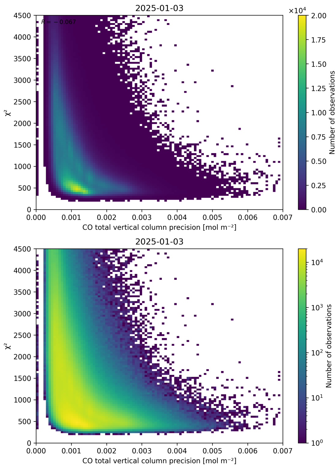
Figure 44: Scatter density plot of “CO total vertical column precision” against “ \chi^2 ” for 2025-01-02 to 2025-01-04.
