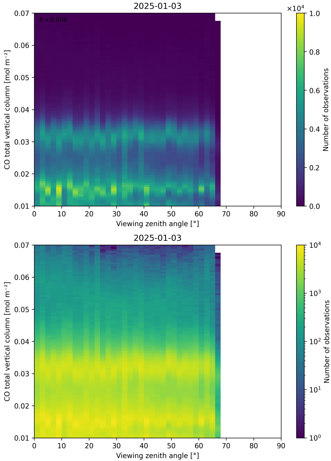
Figure 69: Scatter density plot of “Viewing zenith angle” against “CO total vertical column” for 2025-01-02 to 2025-01-04.
