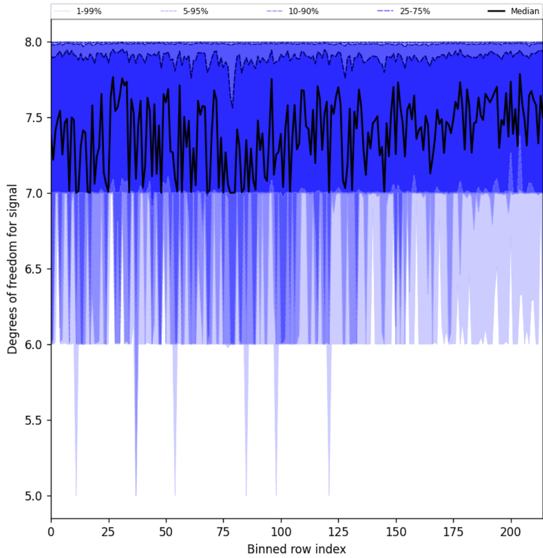
Figure 31: Along track statistics of “Degrees of freedom for signal” for 2025-01-02 to 2025-01-04
