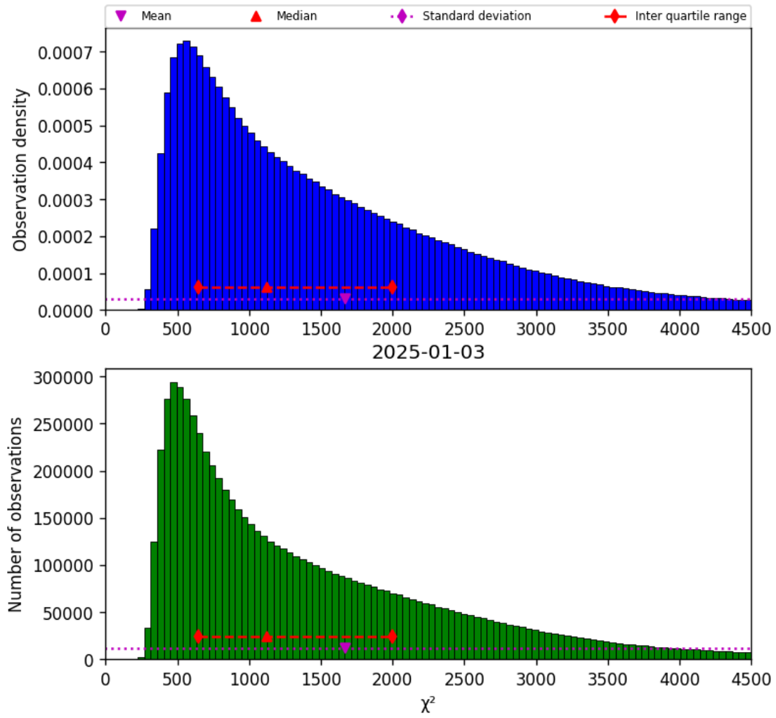
Figure 22: Histogram of “ \chi^2 ” for 2025-01-02 to 2025-01-04
