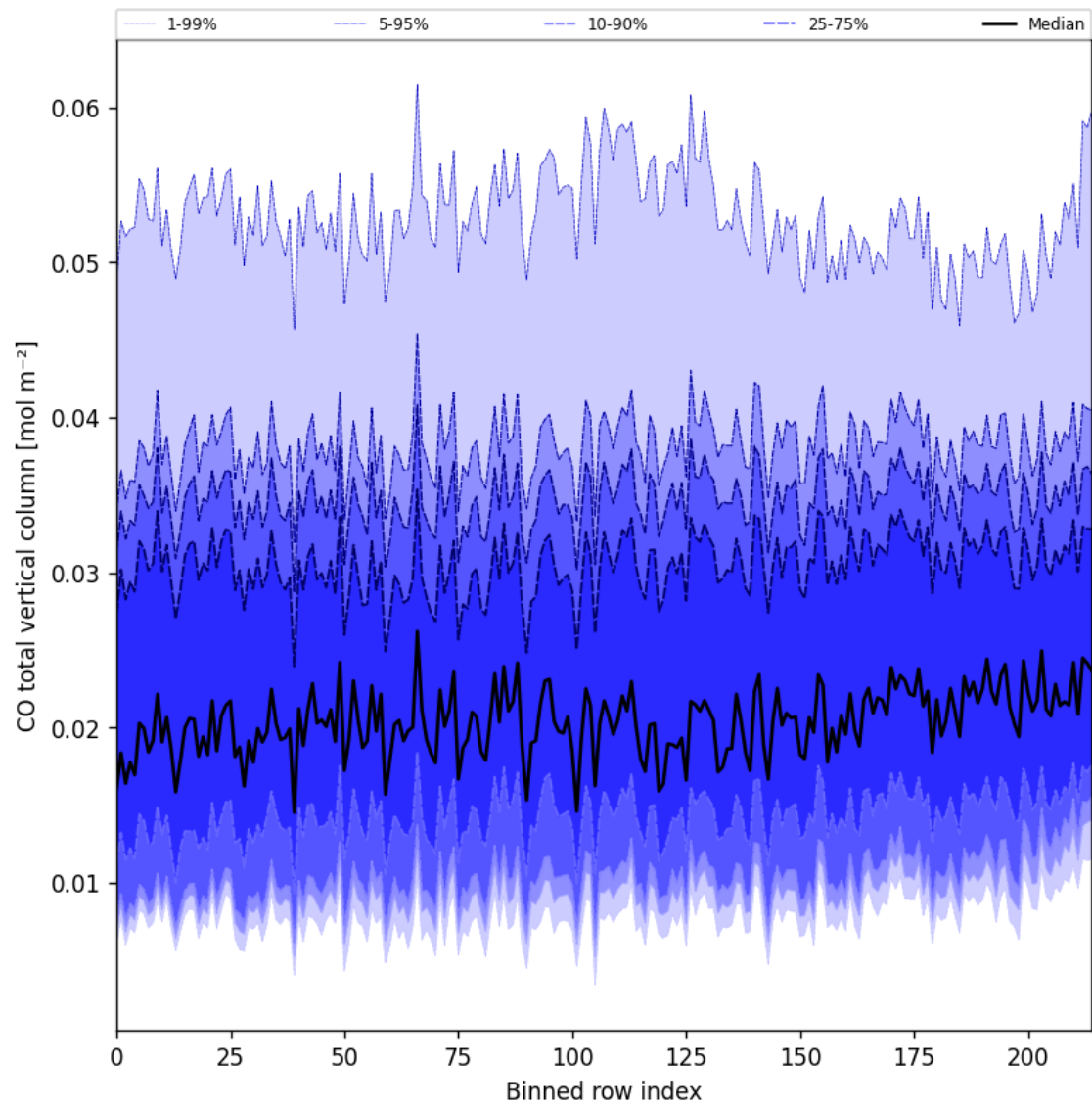
Figure 26: Along track statistics of “CO total vertical column” for 2025-01-02 to 2025-01-04
