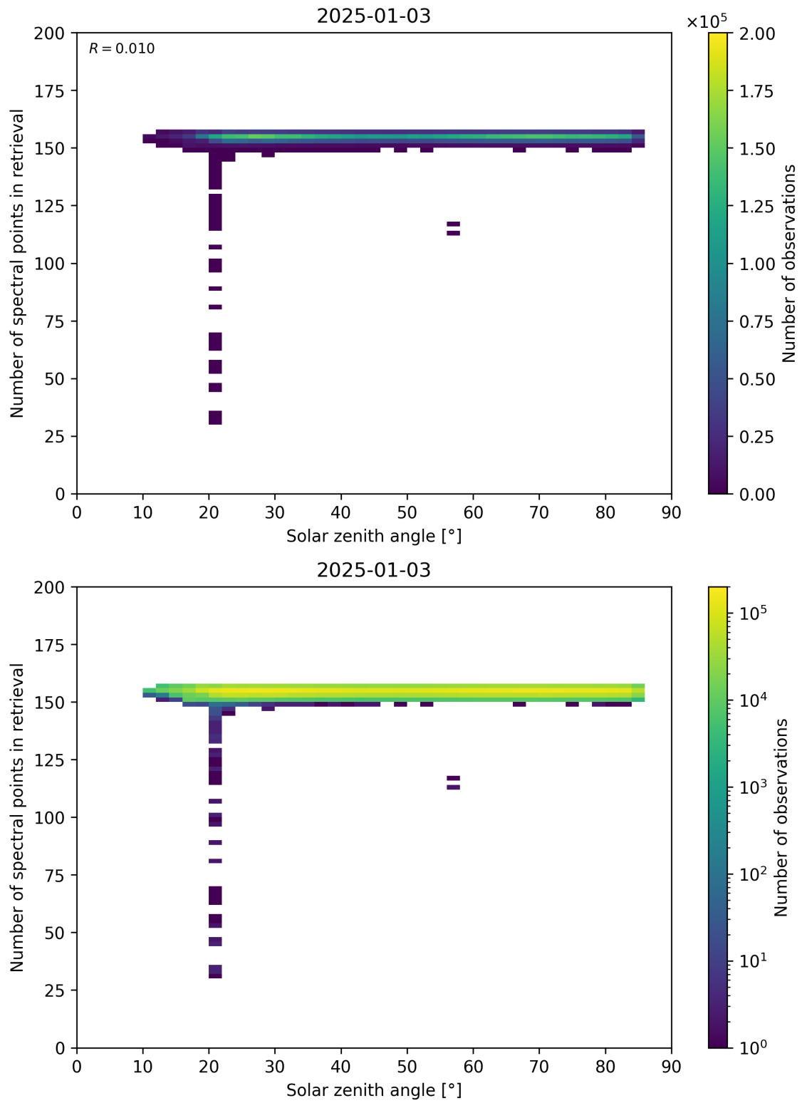
Figure 68: Scatter density plot of “Solar zenith angle” against “Number of spectral points in retrieval” for 2025-01-02 to 2025-01-04.
