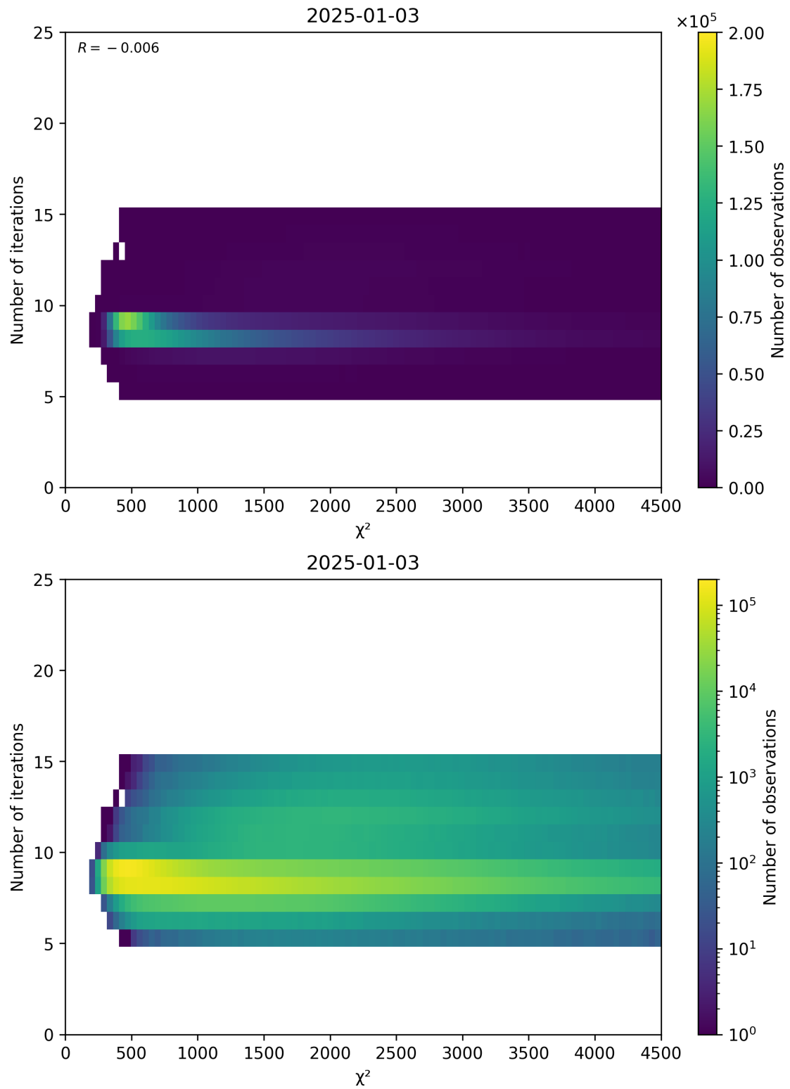
Figure 49: Scatter density plot of “ \chi^2 ” against “Number of iterations” for 2025-01-02 to 2025-01-04.
