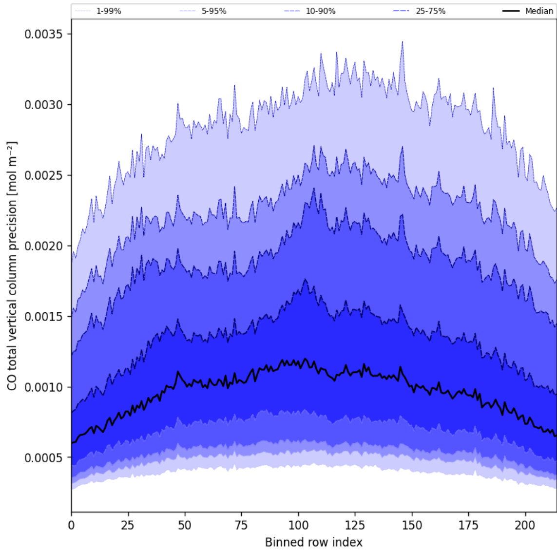
Figure 28: Along track statistics of “CO total vertical column precision” for 2025-01-02 to 2025-01-04
