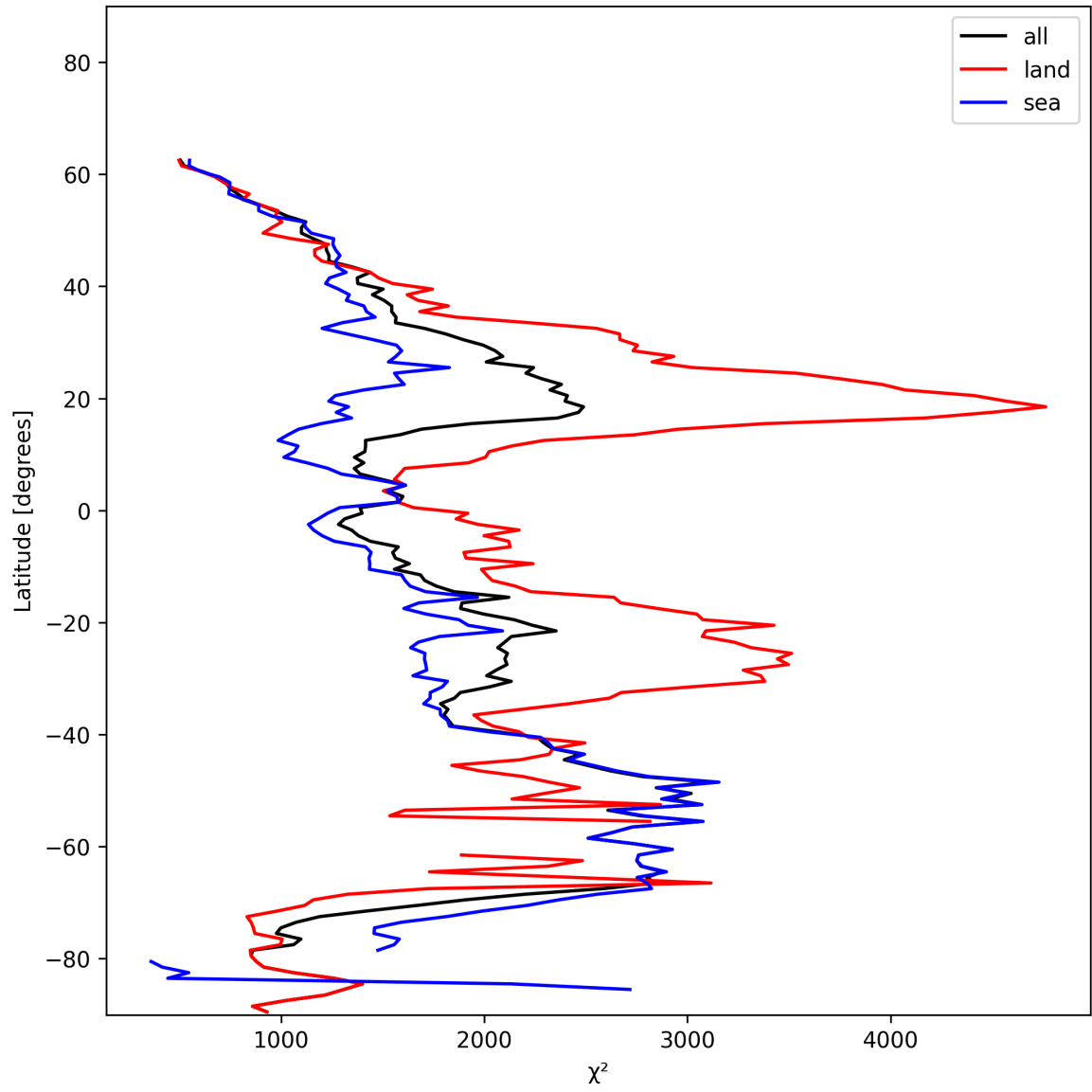
Figure 14: Zonal average of “ \chi^2 ” for 2025-01-02 to 2025-01-04.
