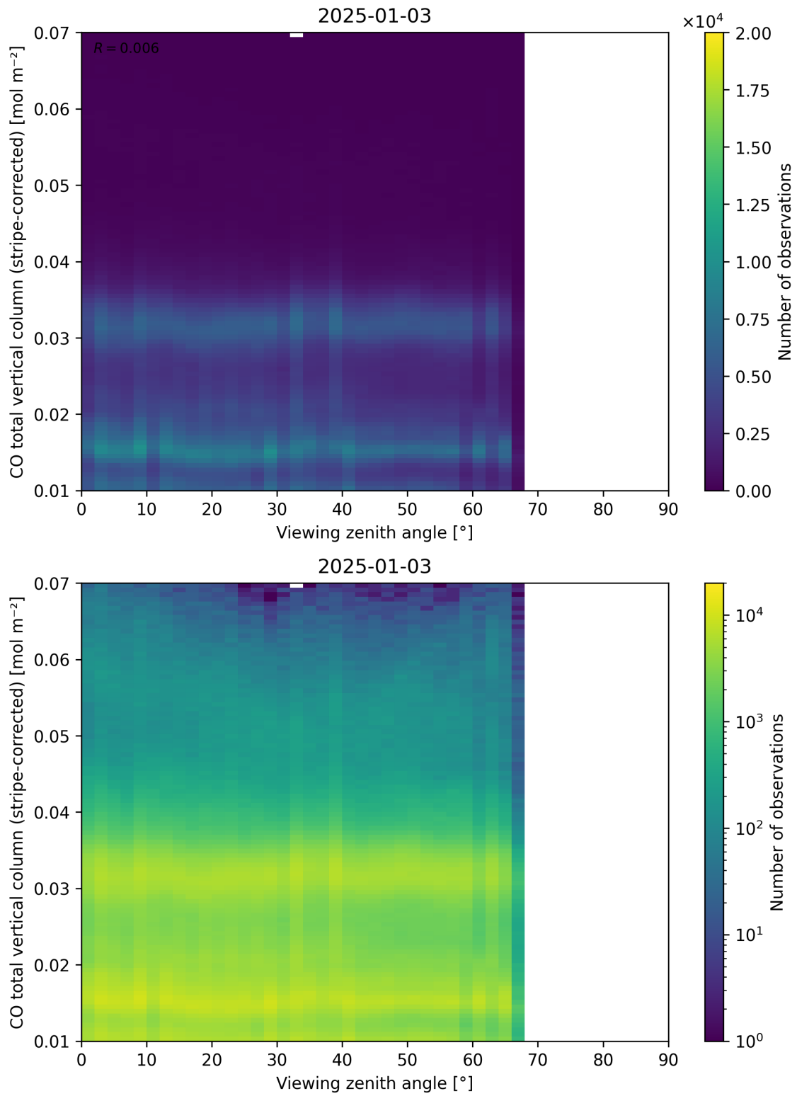
Figure 70: Scatter density plot of “Viewing zenith angle” against “CO total vertical column (stripe-corrected)” for 2025-01-02 to 2025-01-04.
