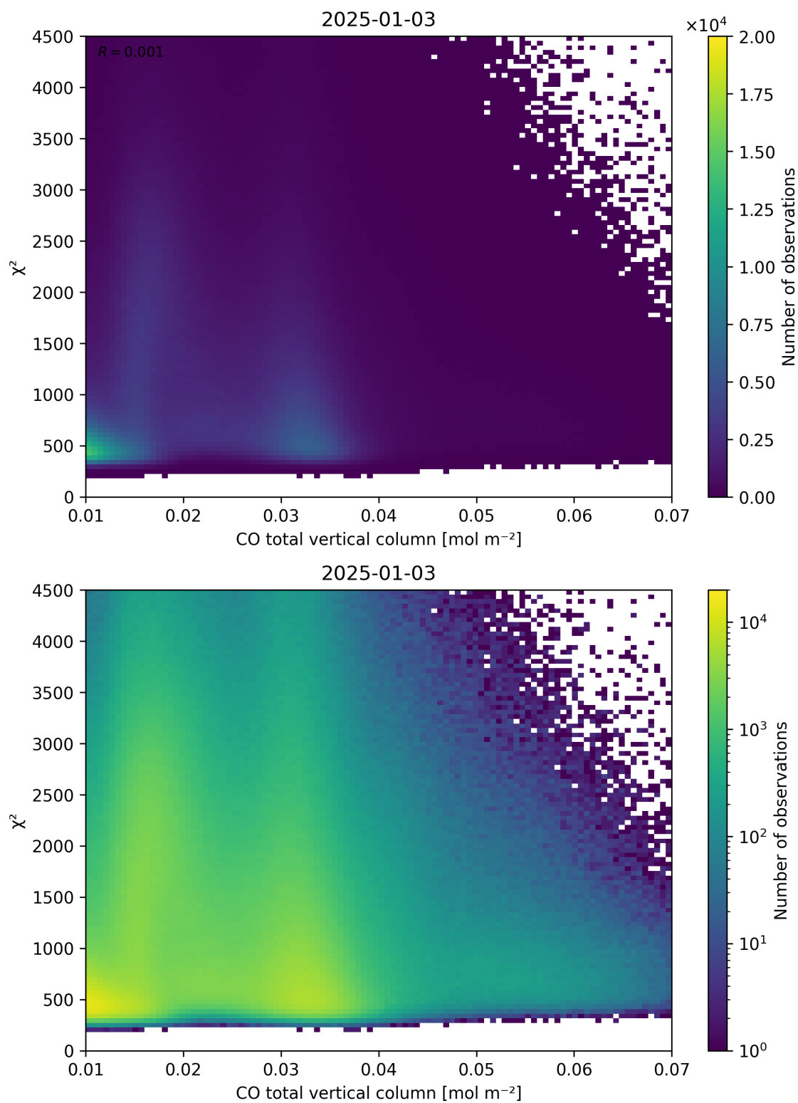
Figure 35: Scatter density plot of “CO total vertical column” against “ \chi^2 ” for 2025-01-02 to 2025-01-04.
