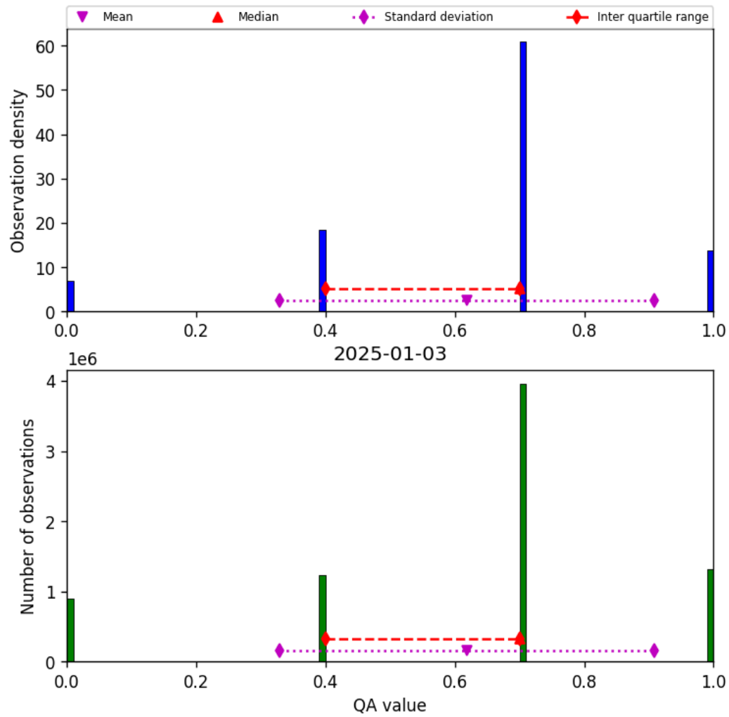
Figure 17: Histogram of “QA value” for 2025-01-02 to 2025-01-04
