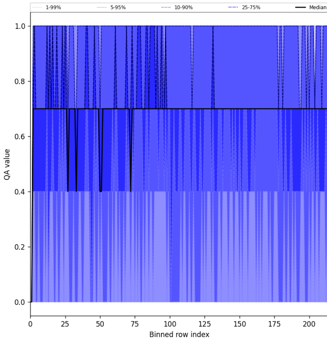
Figure 25: Along track statistics of “QA value” for 2025-01-02 to 2025-01-04
