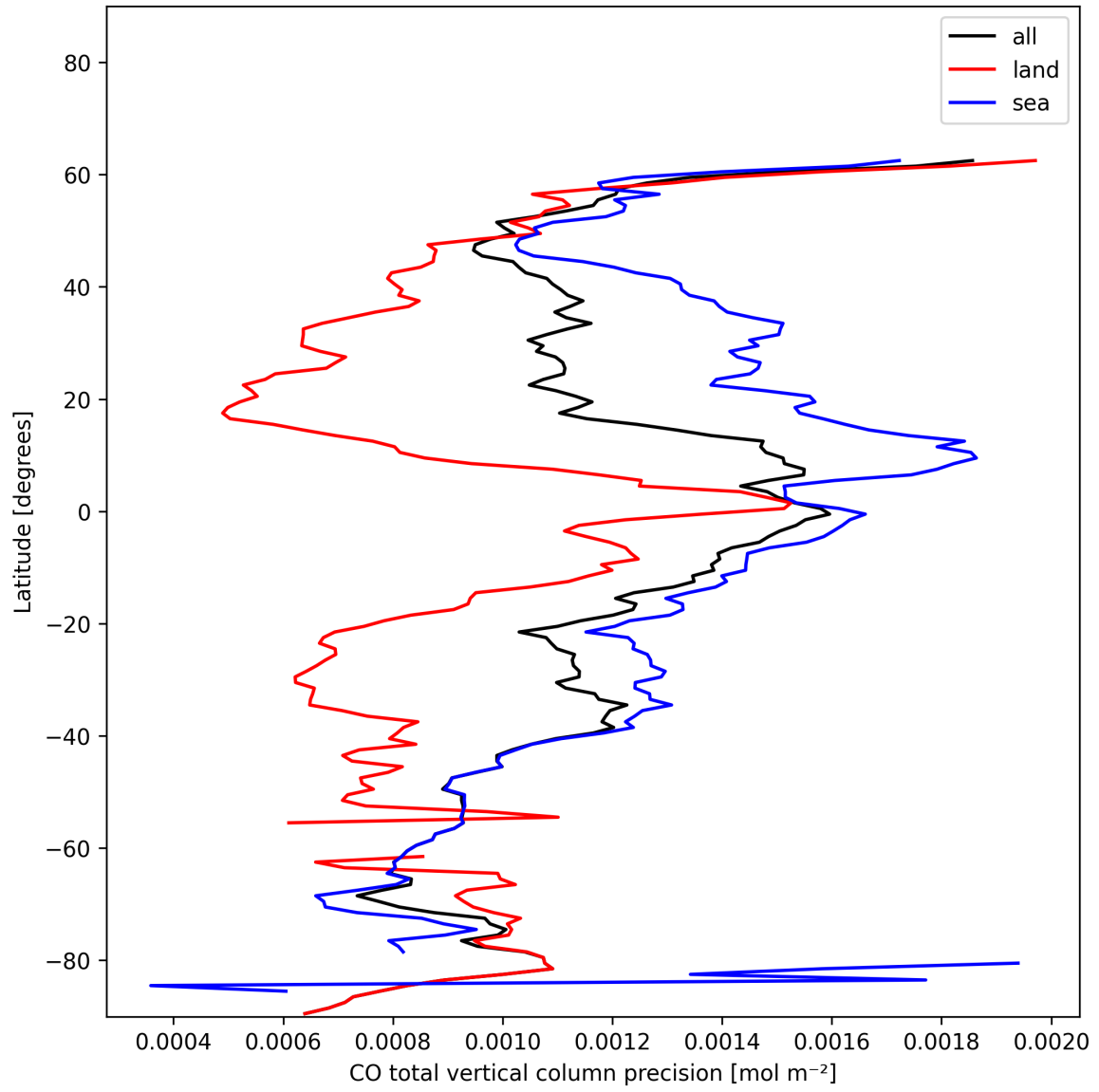
Figure 12: Zonal average of “CO total vertical column precision” for 2025-01-02 to 2025-01-04.
