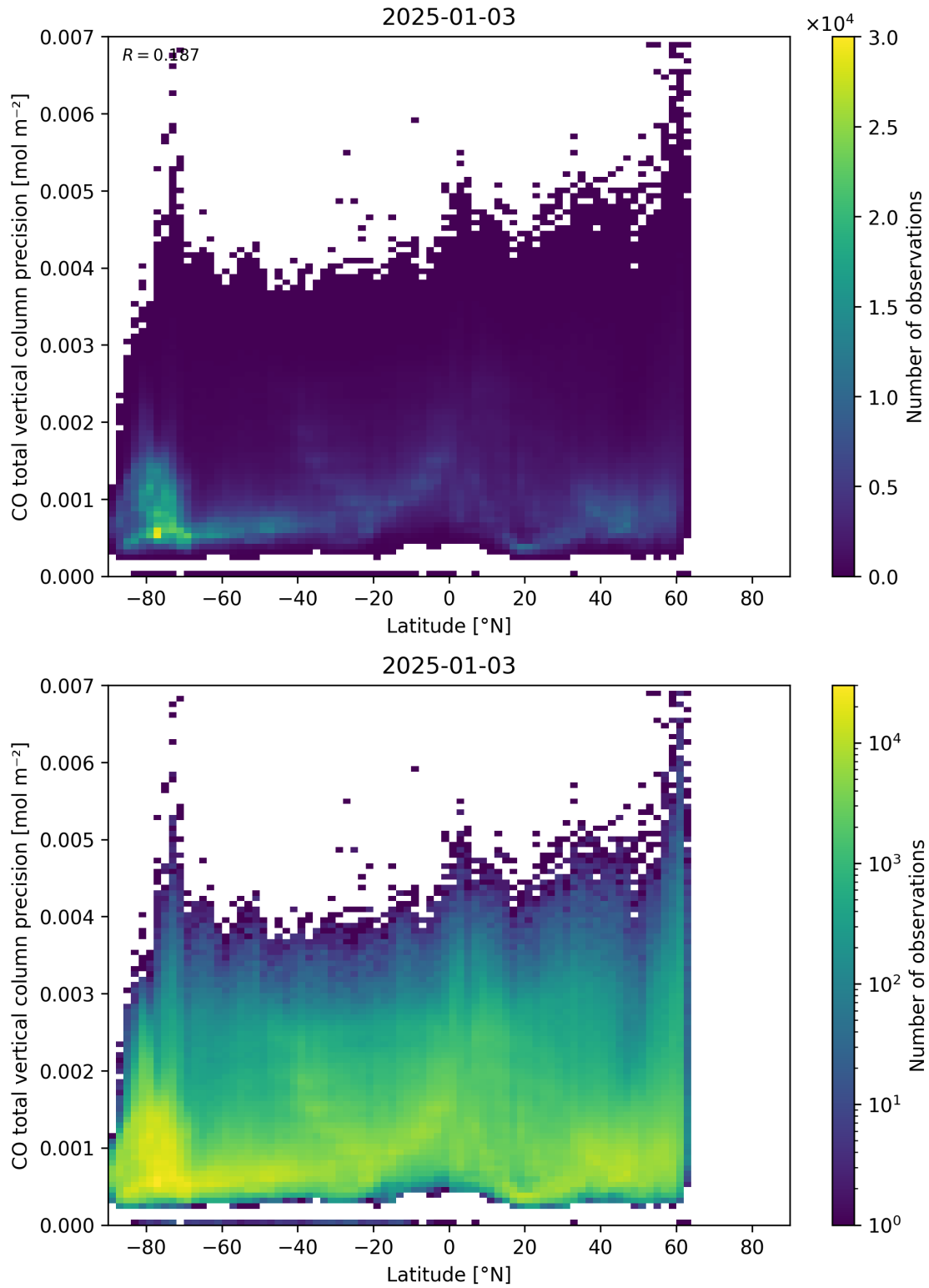
Figure 53: Scatter density plot of “Latitude” against “CO total vertical column precision” for 2025-01-02 to 2025-01-04.
