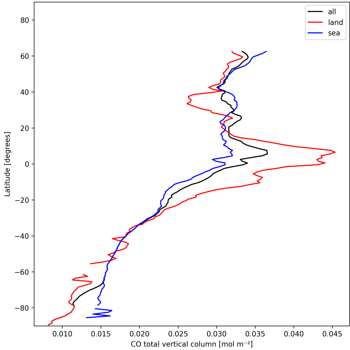
Figure 10: Zonal average of “CO total vertical column” for 2025-01-02 to 2025-01-04.
