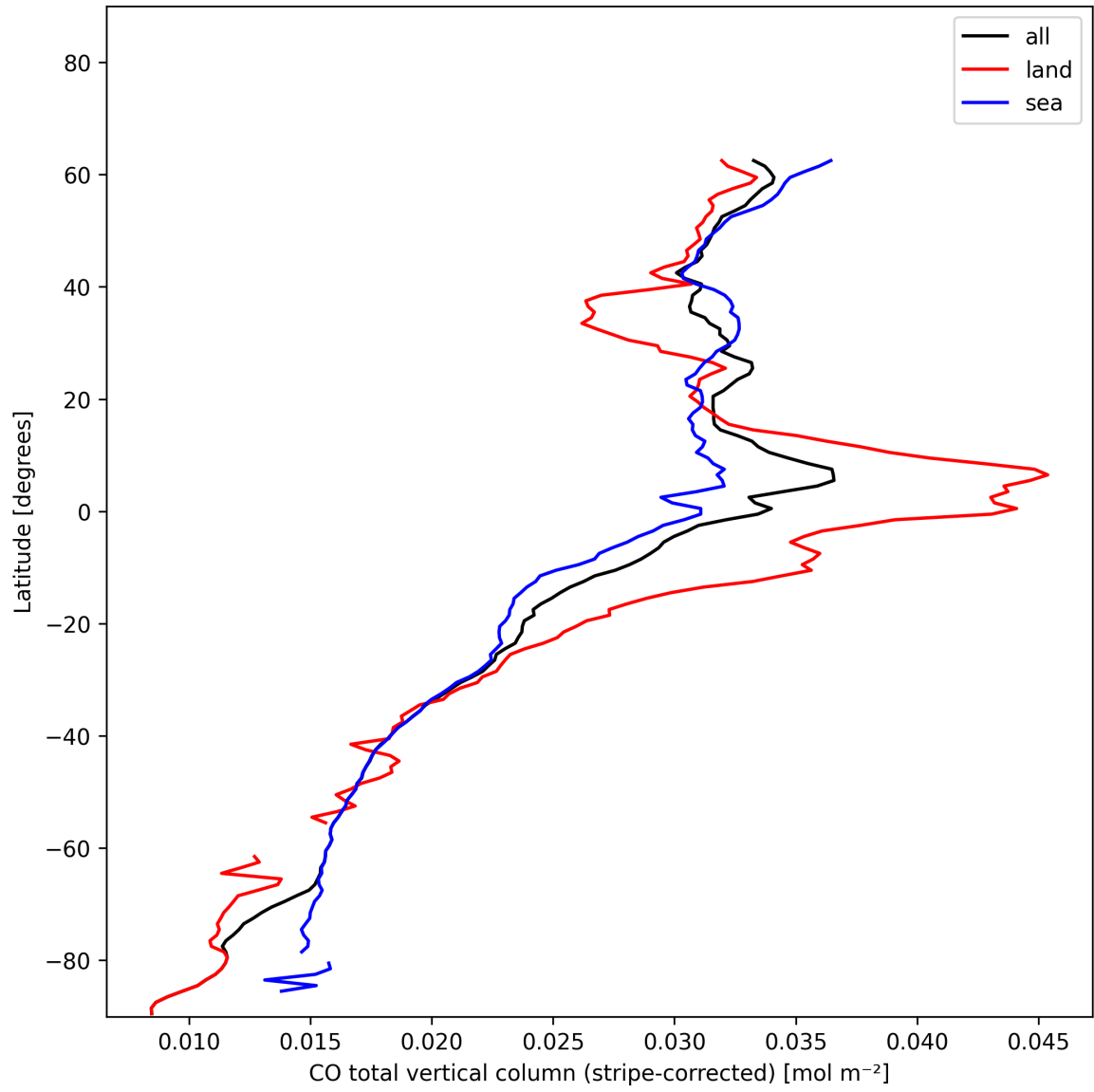
Figure 11: Zonal average of “CO total vertical column (stripe-corrected)” for 2025-01-02 to 2025-01-04.
