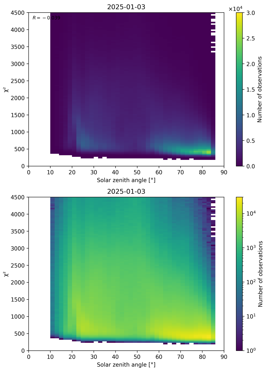
Figure 64: Scatter density plot of “Solar zenith angle” against “ \chi^2 ” for 2025-01-02 to 2025-01-04.
