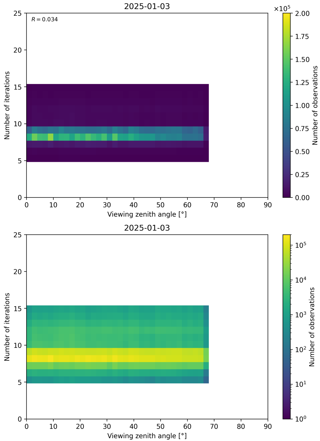
Figure 75: Scatter density plot of “Viewing zenith angle” against “Number of iterations” for 2025-01-02 to 2025-01-04.
