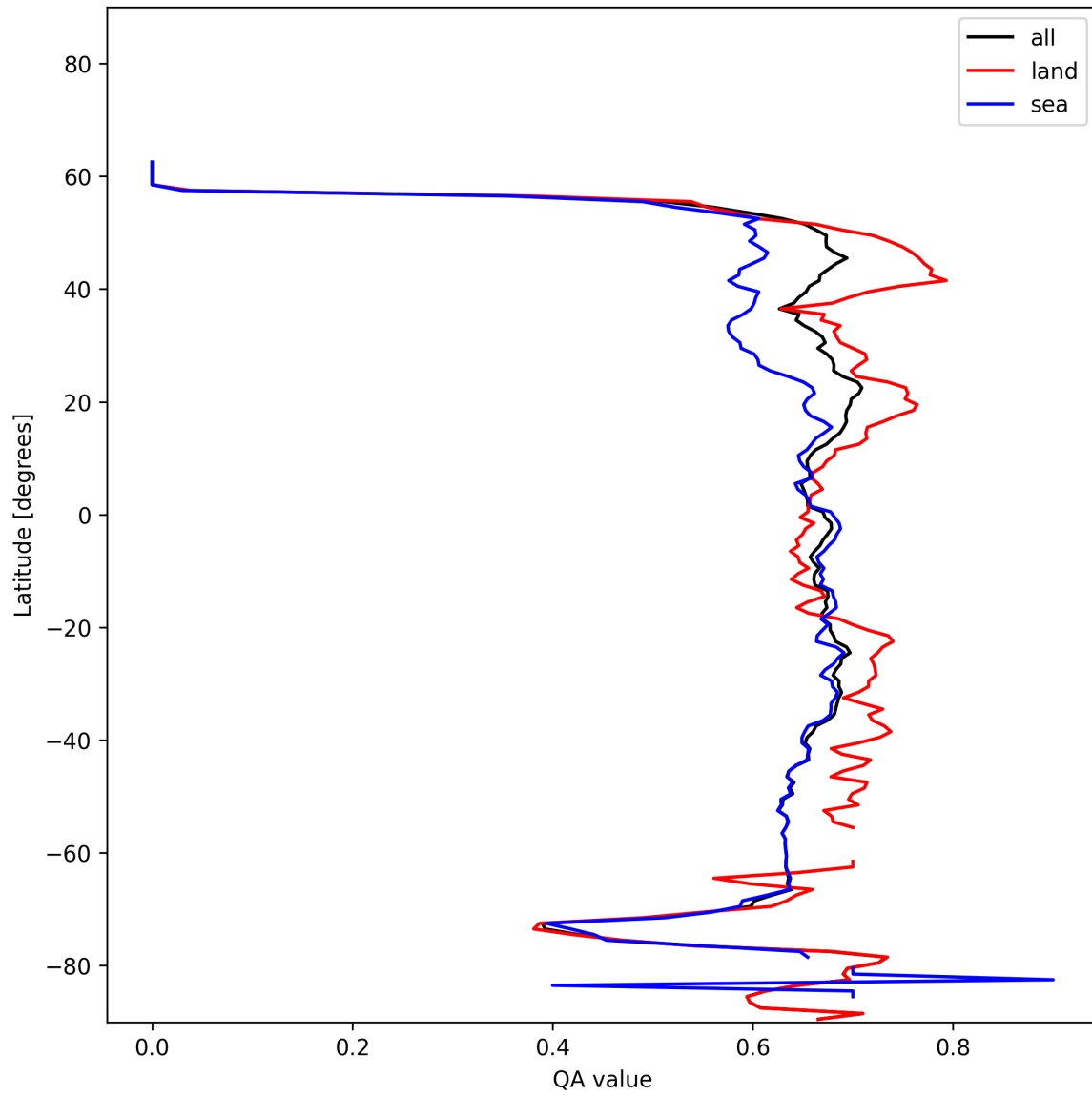
Figure 9: Zonal average of "QA value" for 2025-01-02 to 2025-01-04.
