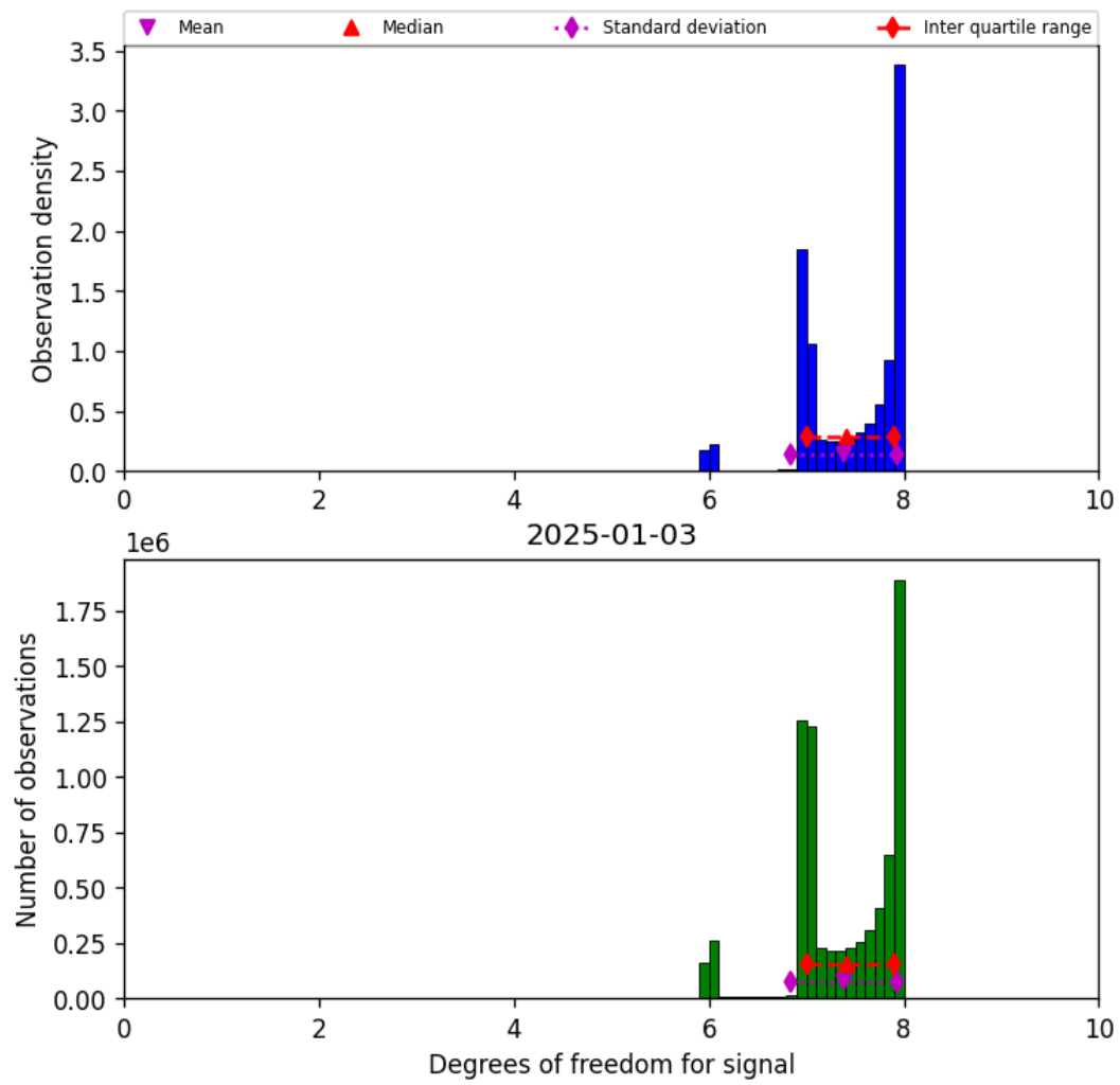
Figure 23: Histogram of “Degrees of freedom for signal” for 2025-01-02 to 2025-01-04
