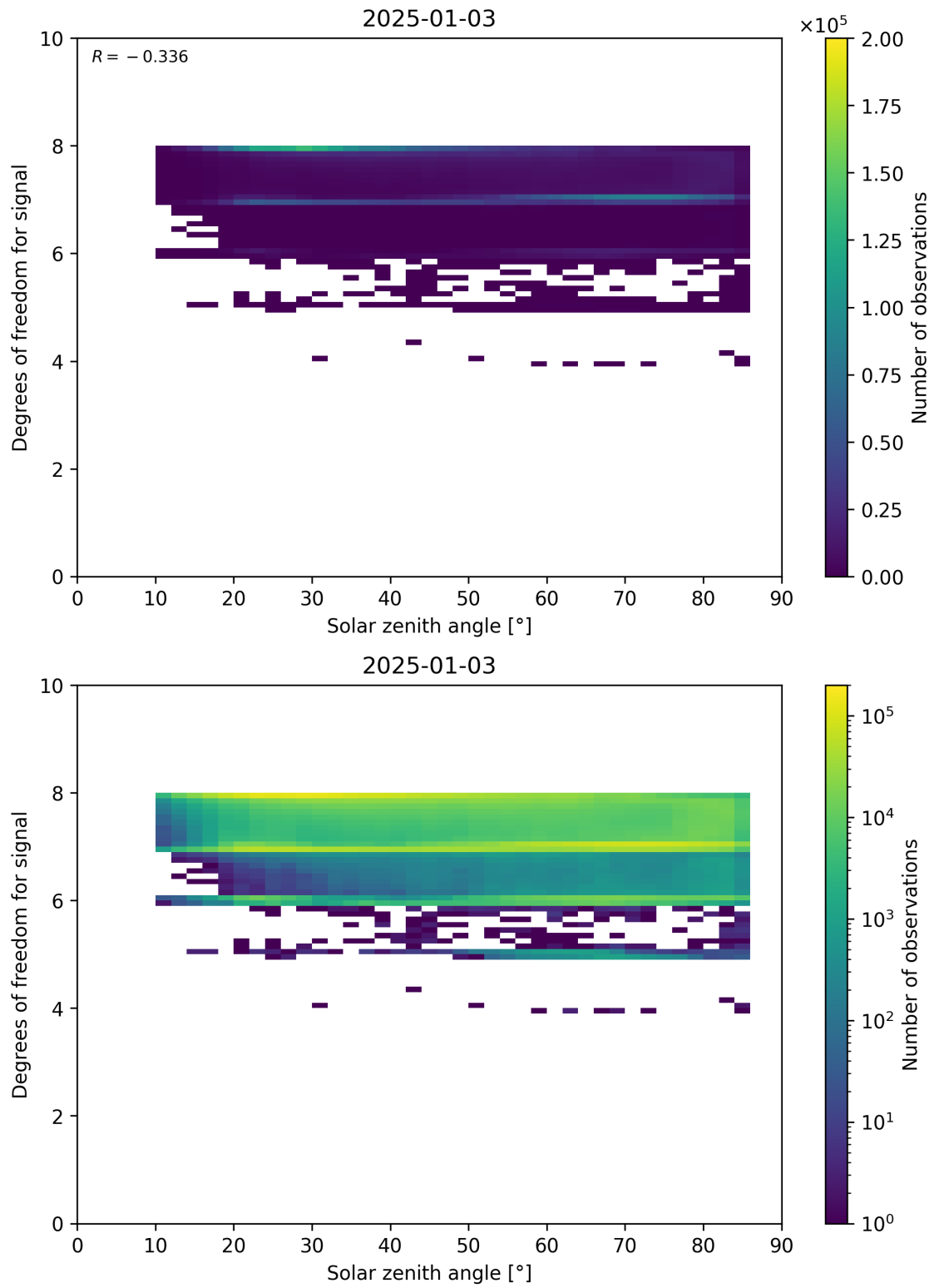
Figure 65: Scatter density plot of “Solar zenith angle” against “Degrees of freedom for signal” for 2025-01-02 to 2025-01-04.
