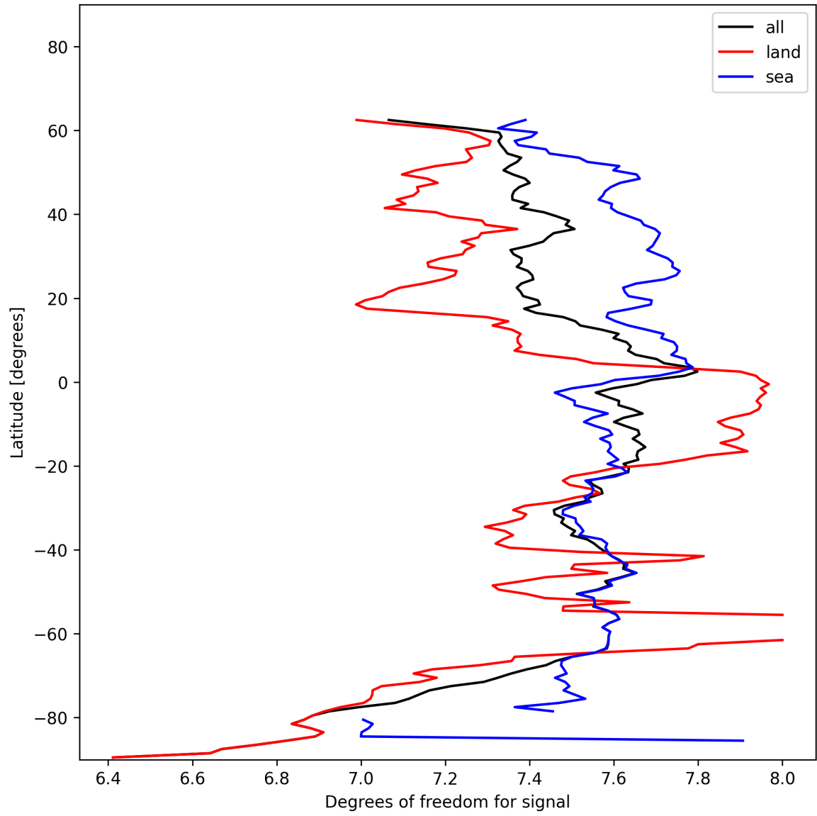
Figure 15: Zonal average of “Degrees of freedom for signal” for 2025-01-02 to 2025-01-04.
