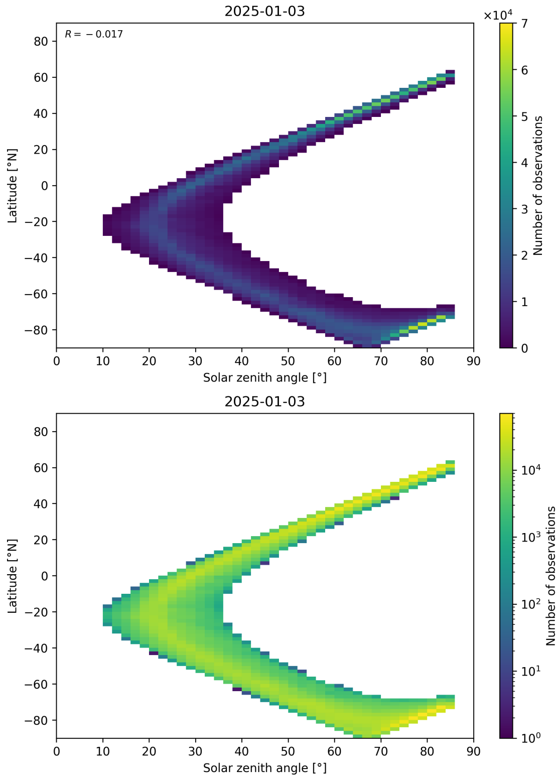
Figure 66: Scatter density plot of “Solar zenith angle” against “Latitude” for 2025-01-02 to 2025-01-04.
