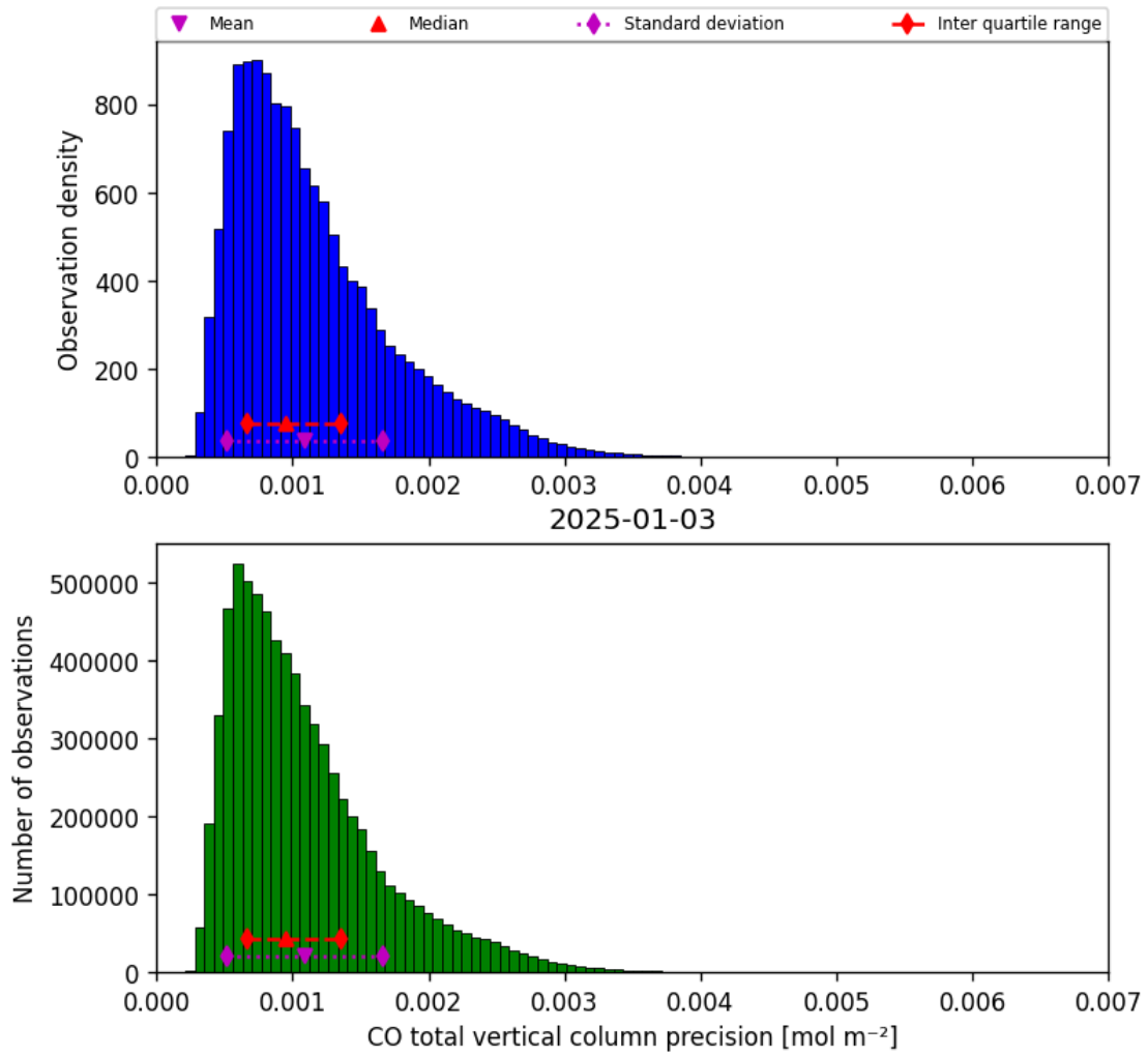
Figure 20: Histogram of “CO total vertical column precision” for 2025-01-02 to 2025-01-04
