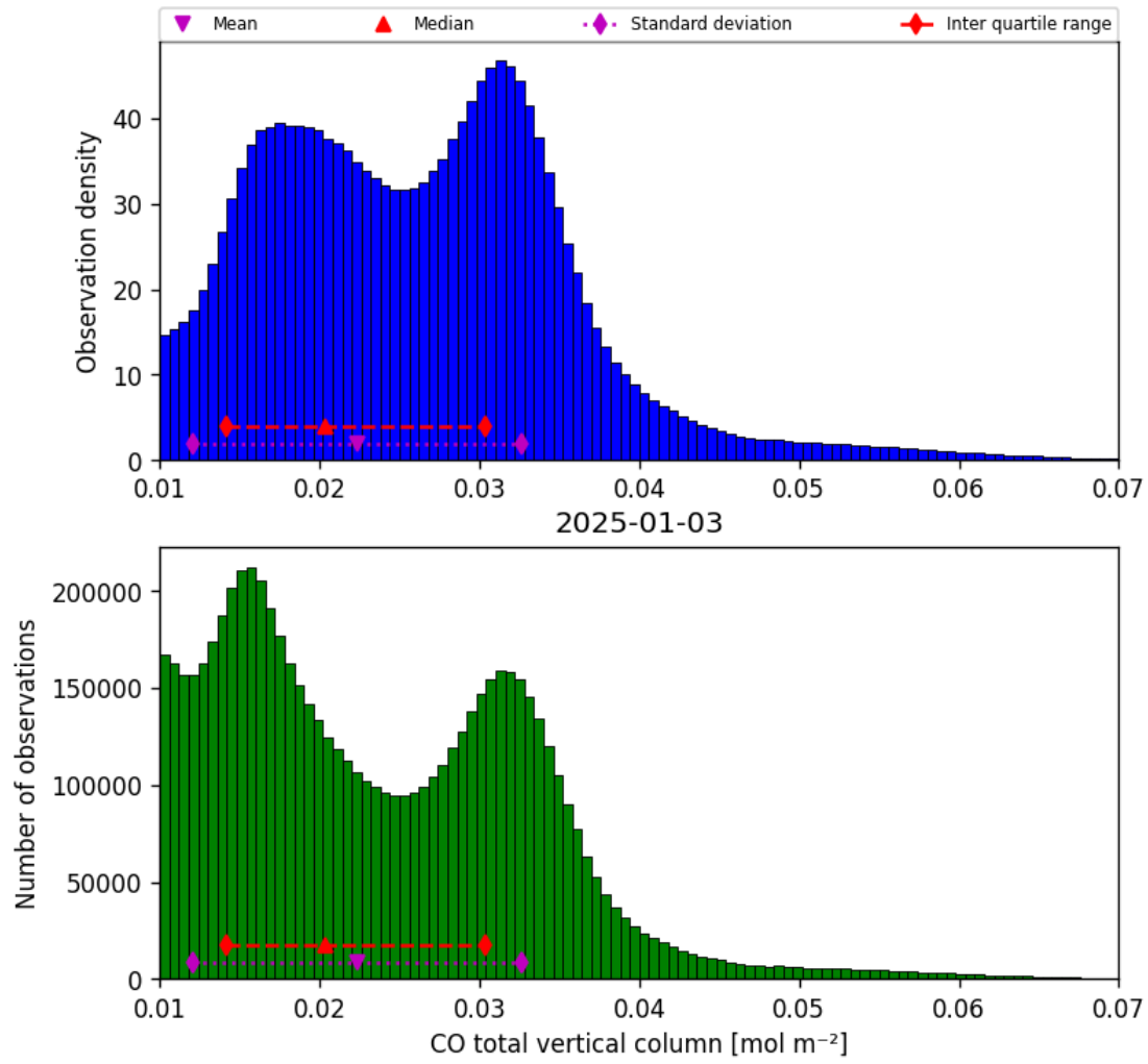
Figure 18: Histogram of “CO total vertical column” for 2025-01-02 to 2025-01-04
