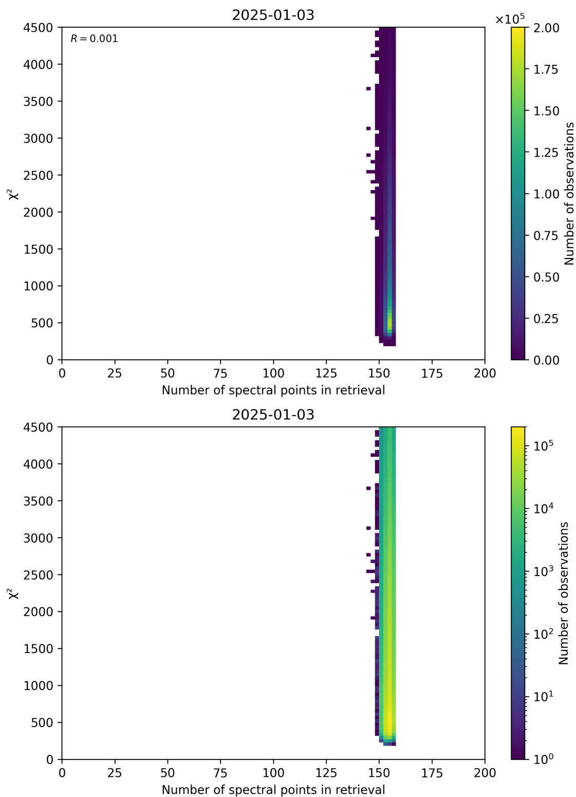
Figure 58: Scatter density plot of “Number of spectral points in retrieval” against “ \chi^2 ” for 2025-01-02 to 2025-01-04.
