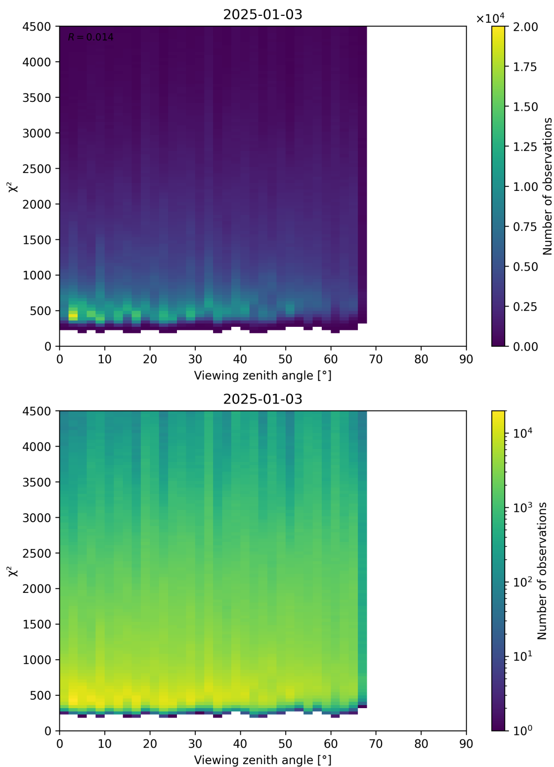
Figure 72: Scatter density plot of “Viewing zenith angle” against “ \chi^2 ” for 2025-01-02 to 2025-01-04.
