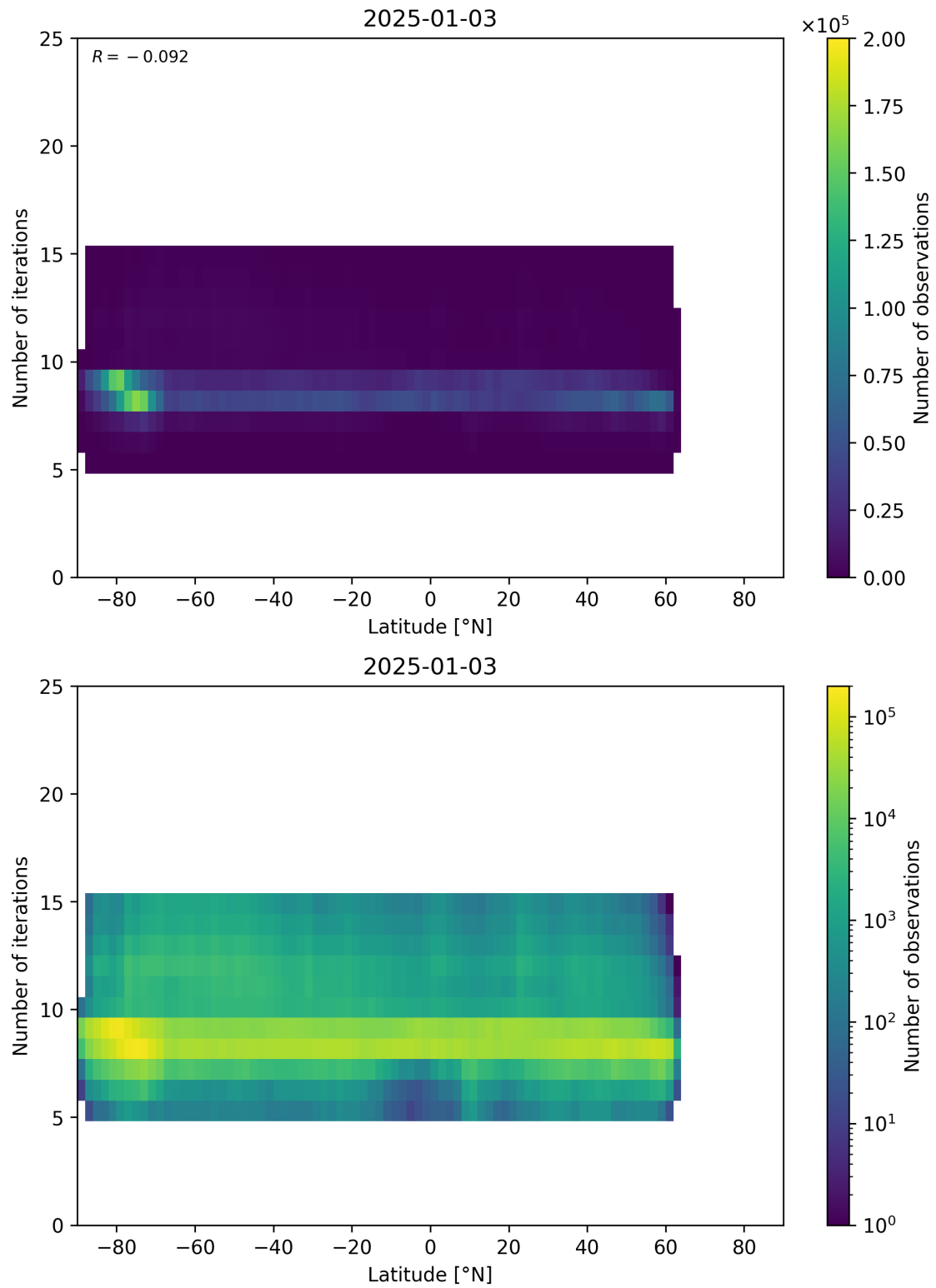
Figure 56: Scatter density plot of “Latitude” against “Number of iterations” for 2025-01-02 to 2025-01-04.
