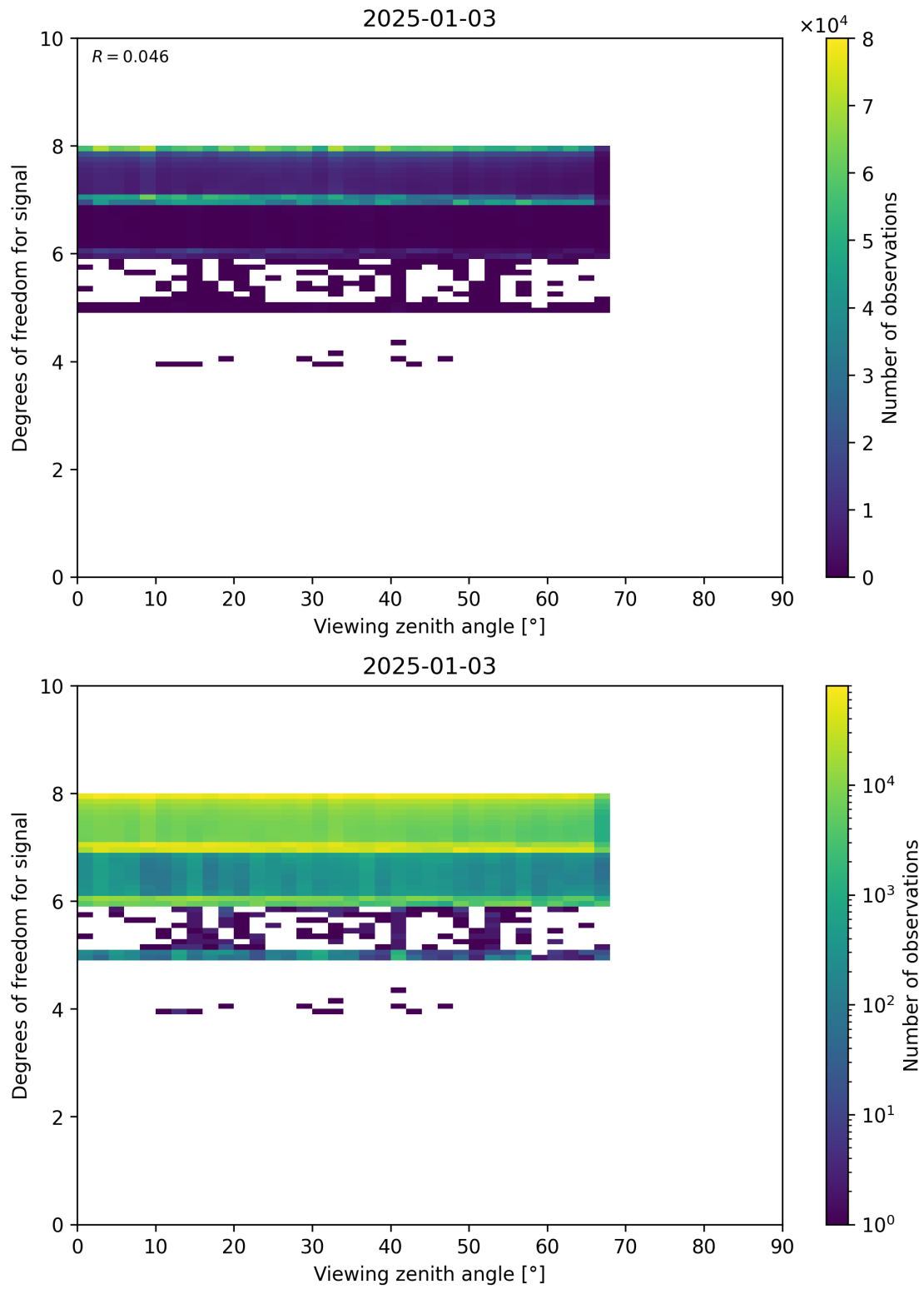
Figure 73: Scatter density plot of “Viewing zenith angle” against “Degrees of freedom for signal” for 2025-01-02 to 2025-01-04.
