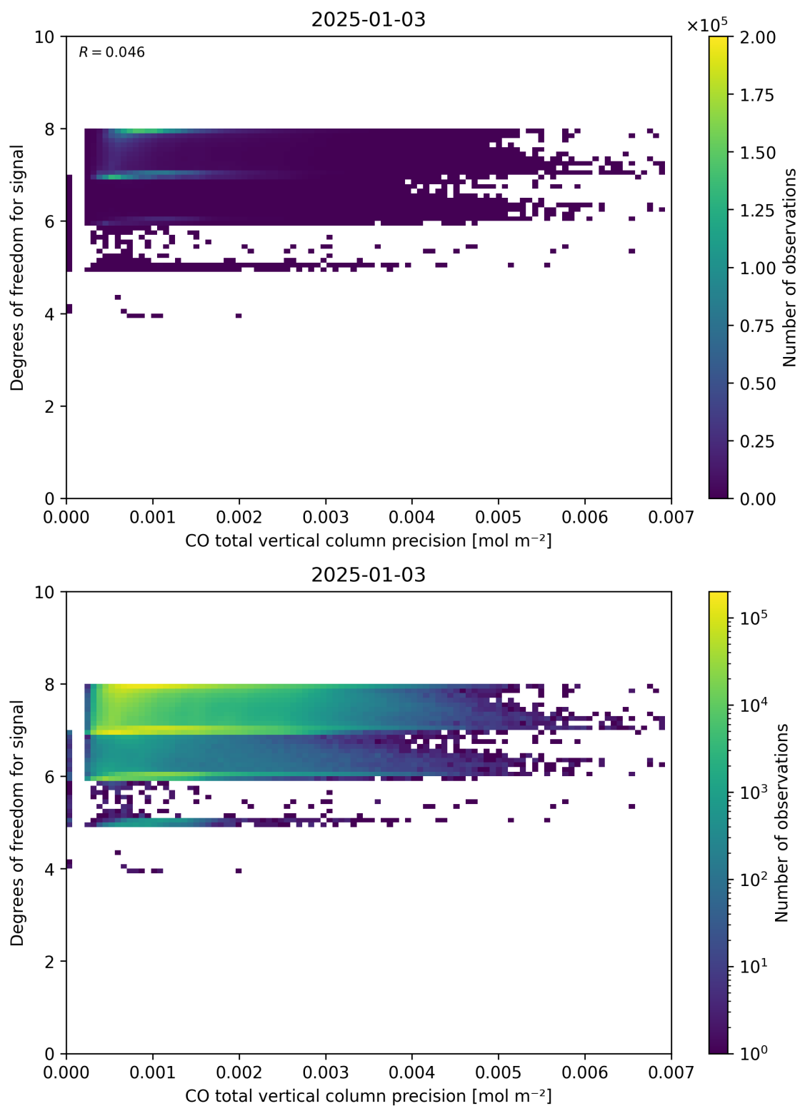
Figure 45: Scatter density plot of “CO total vertical column precision” against “Degrees of freedom for signal” for 2025-01-02 to 2025-01-04.
