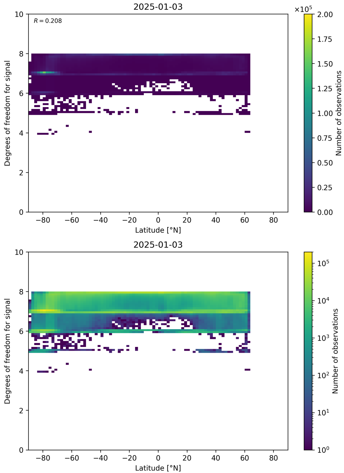
Figure 55: Scatter density plot of “Latitude” against “Degrees of freedom for signal” for 2025-01-02 to 2025-01-04.
