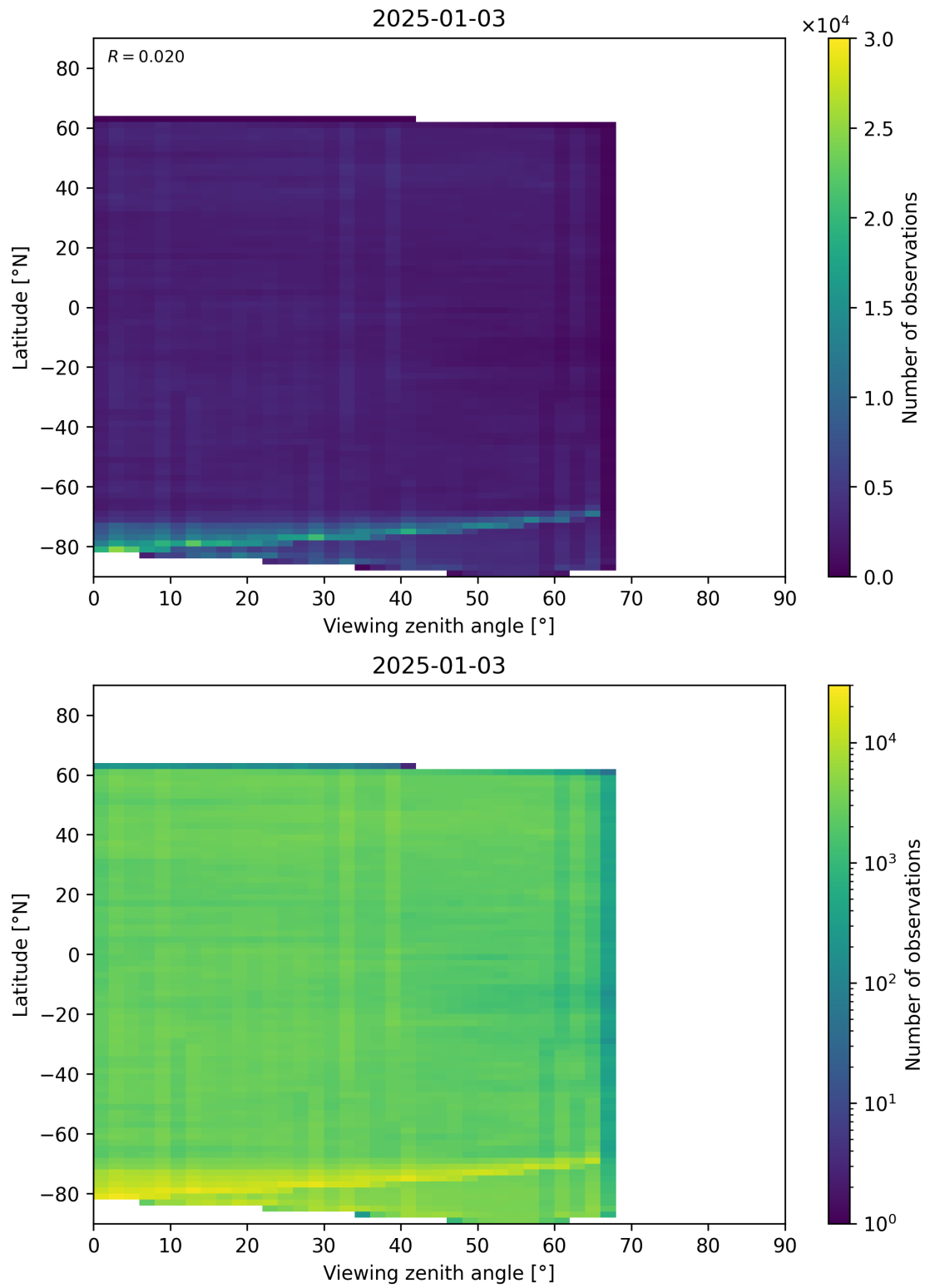
Figure 74: Scatter density plot of “Viewing zenith angle” against “Latitude” for 2025-01-02 to 2025-01-04.
