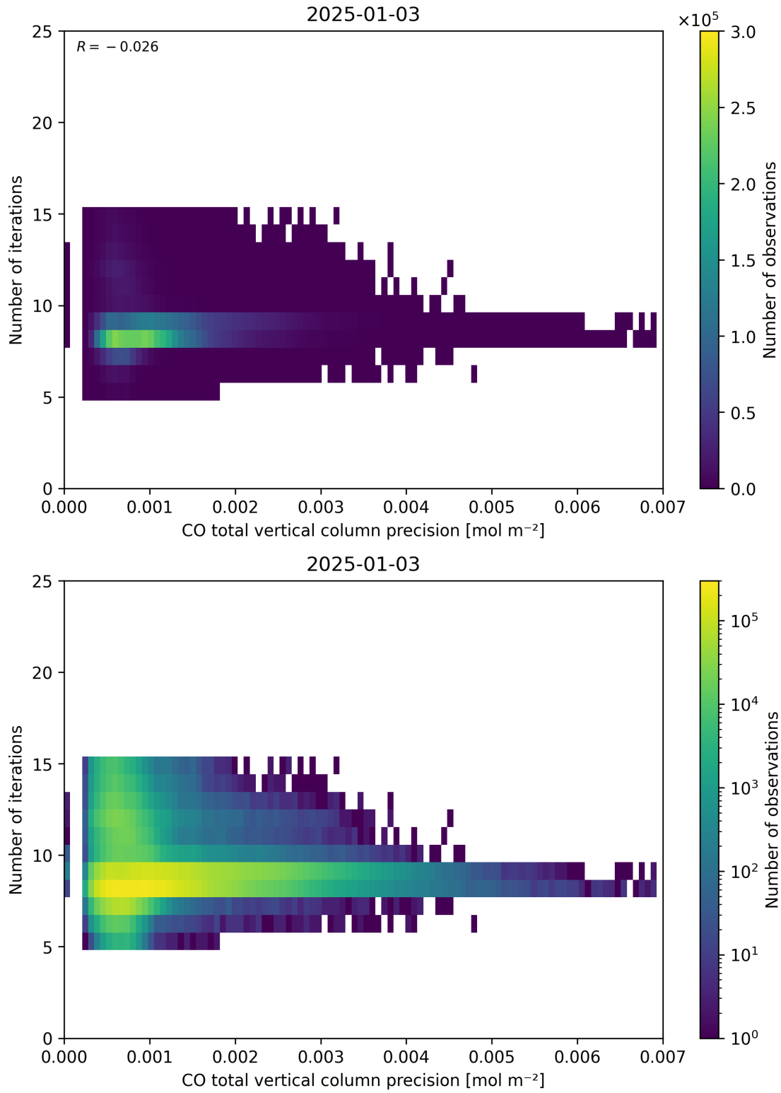
Figure 46: Scatter density plot of “CO total vertical column precision” against “Number of iterations” for 2025-01-02 to 2025-01-04.
