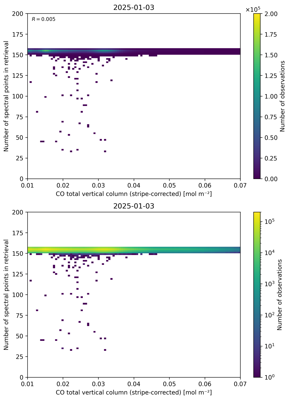
Figure 40: Scatter density plot of “CO total vertical column (stripe-corrected)” against “Number of spectral points in retrieval” for 2025-01-02 to 2025-01-04.
