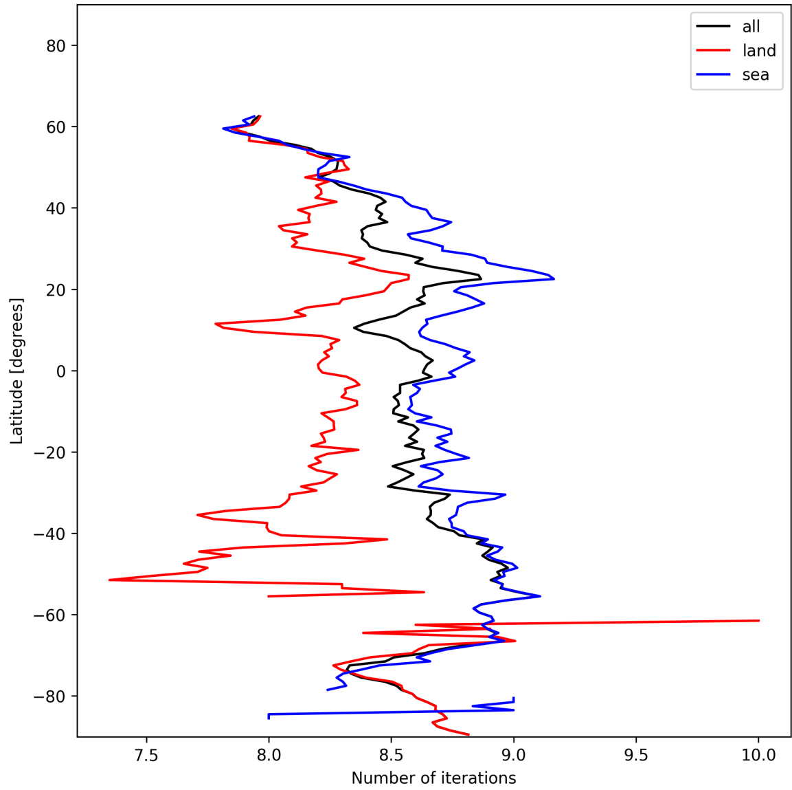
Figure 16: Zonal average of “Number of iterations” for 2025-01-02 to 2025-01-04.
