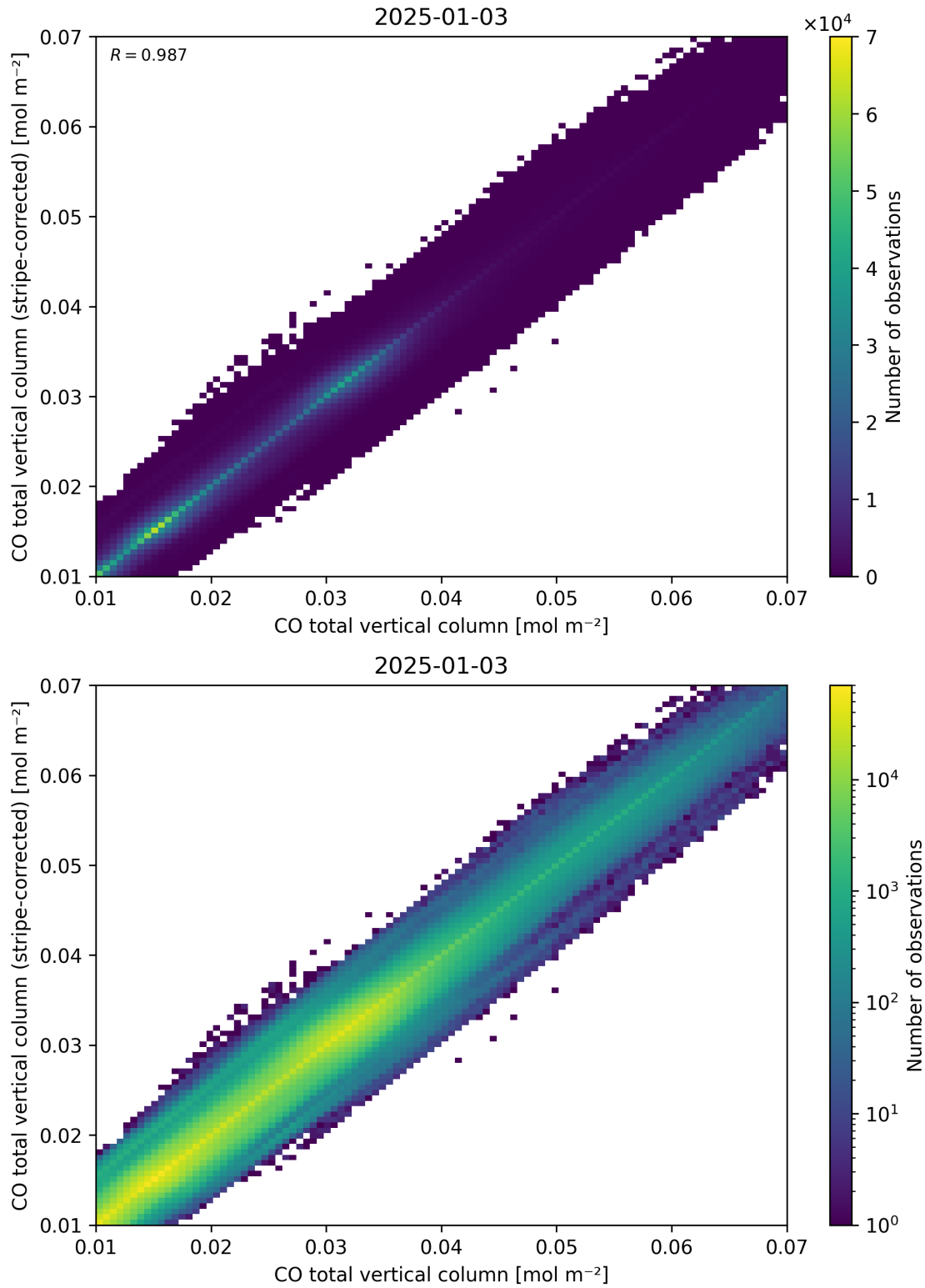
Figure 33: Scatter density plot of “CO total vertical column” against “CO total vertical column (stripe-corrected)” for 2025-01-02 to 2025-01-04.
