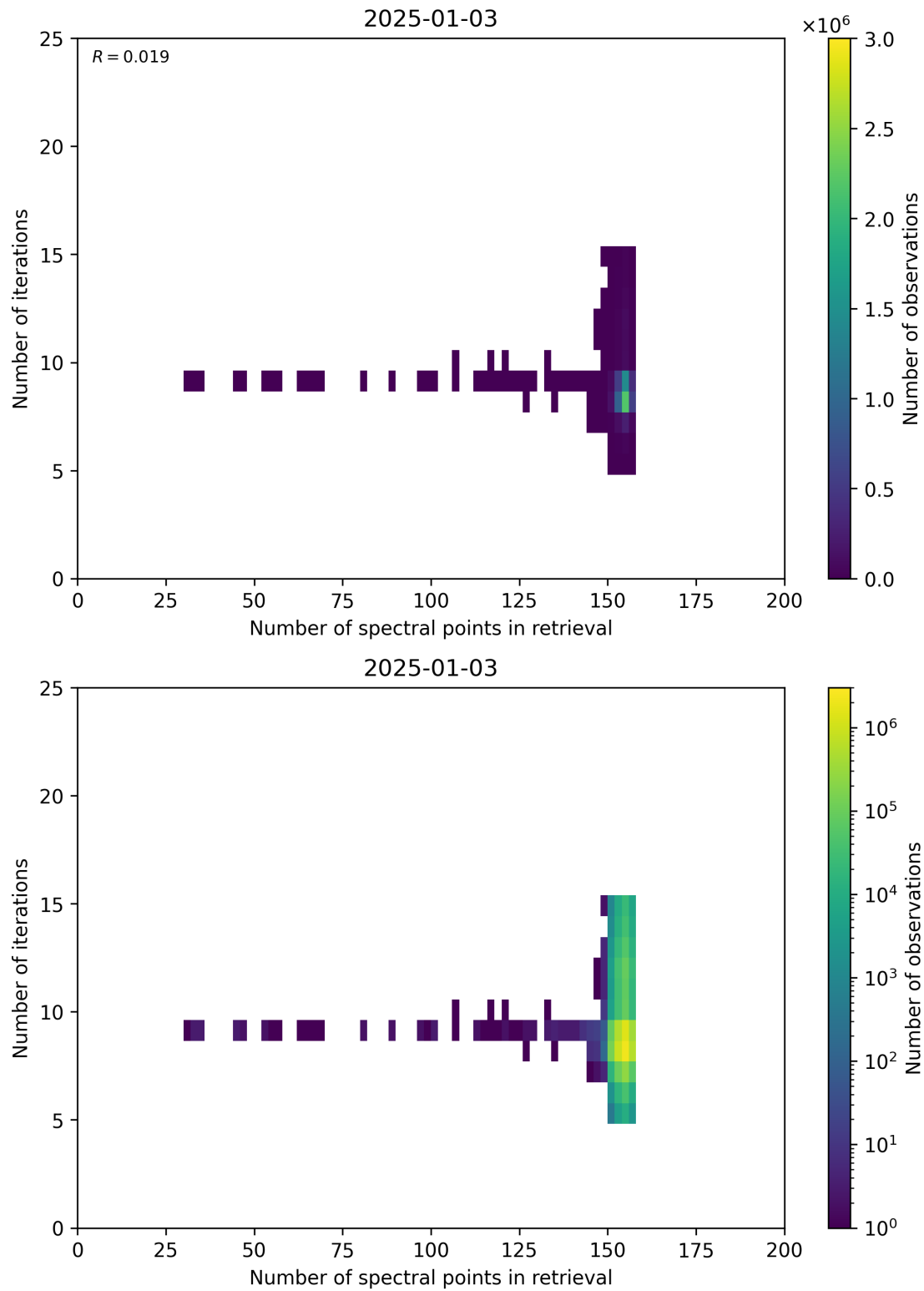
Figure 60: Scatter density plot of “Number of spectral points in retrieval” against “Number of iterations” for 2025-01-02 to 2025-01-04.
