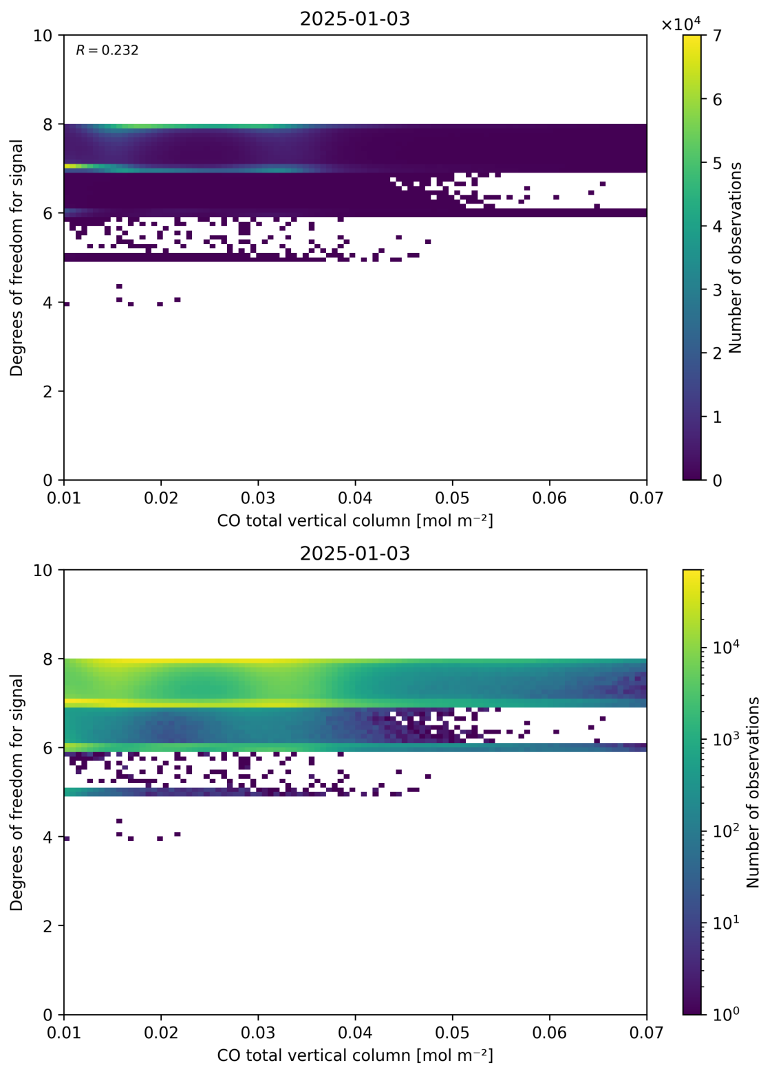
Figure 41: Scatter density plot of “CO total vertical column” against “Degrees of freedom for signal” for 2025-01-02 to 2025-01-04.
