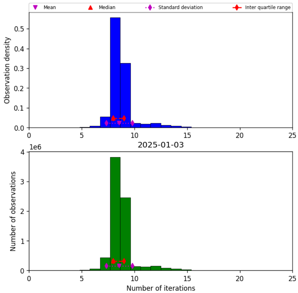
Figure 24: Histogram of “Number of iterations” for 2025-01-02 to 2025-01-04
