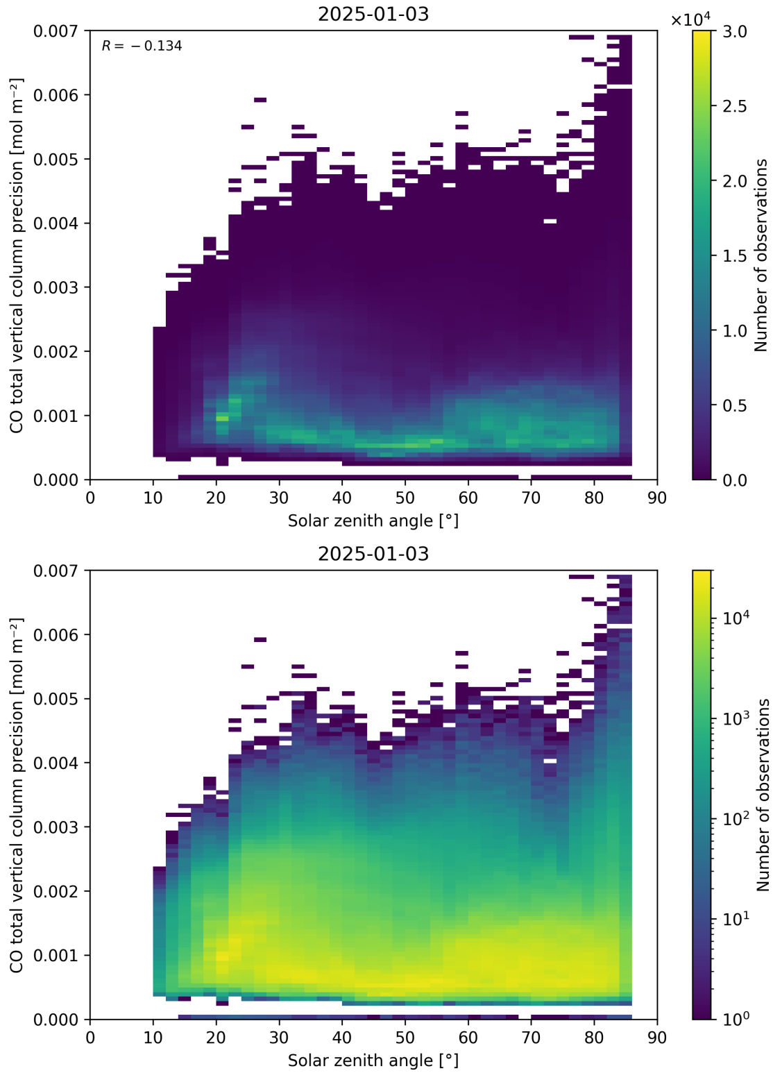
Figure 63: Scatter density plot of “Solar zenith angle” against “CO total vertical column precision” for 2025-01-02 to 2025-01-04.
