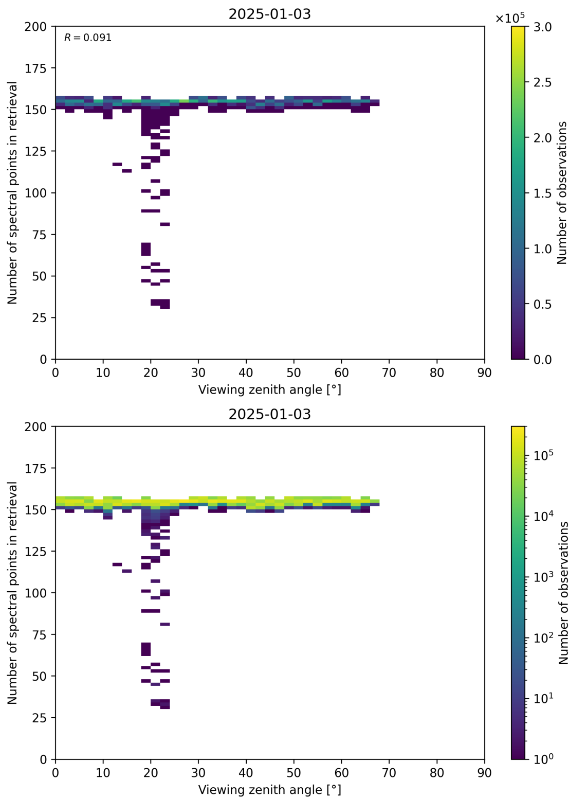
Figure 76: Scatter density plot of “Viewing zenith angle” against “Number of spectral points in retrieval” for 2025-01-02 to 2025-01-04.
