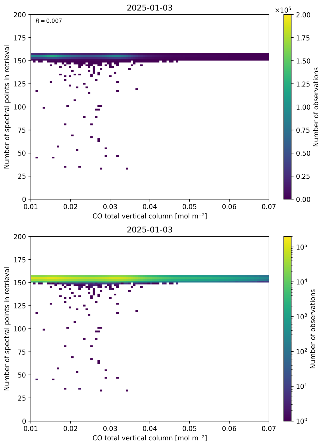
Figure 43: Scatter density plot of “CO total vertical column” against “Number of spectral points in retrieval” for 2025-01-02 to 2025-01-04.
