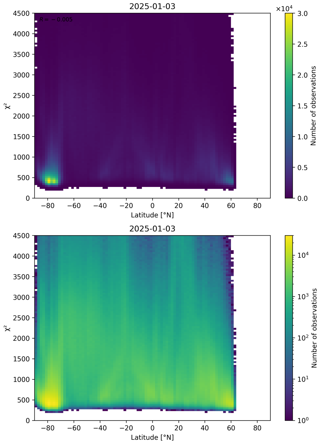
Figure 54: Scatter density plot of “Latitude” against “ \chi^2 ” for 2025-01-02 to 2025-01-04.
