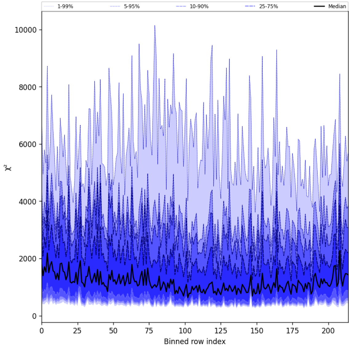
Figure 30: Along track statistics of “ \chi^2 ” for 2025-01-02 to 2025-01-04
