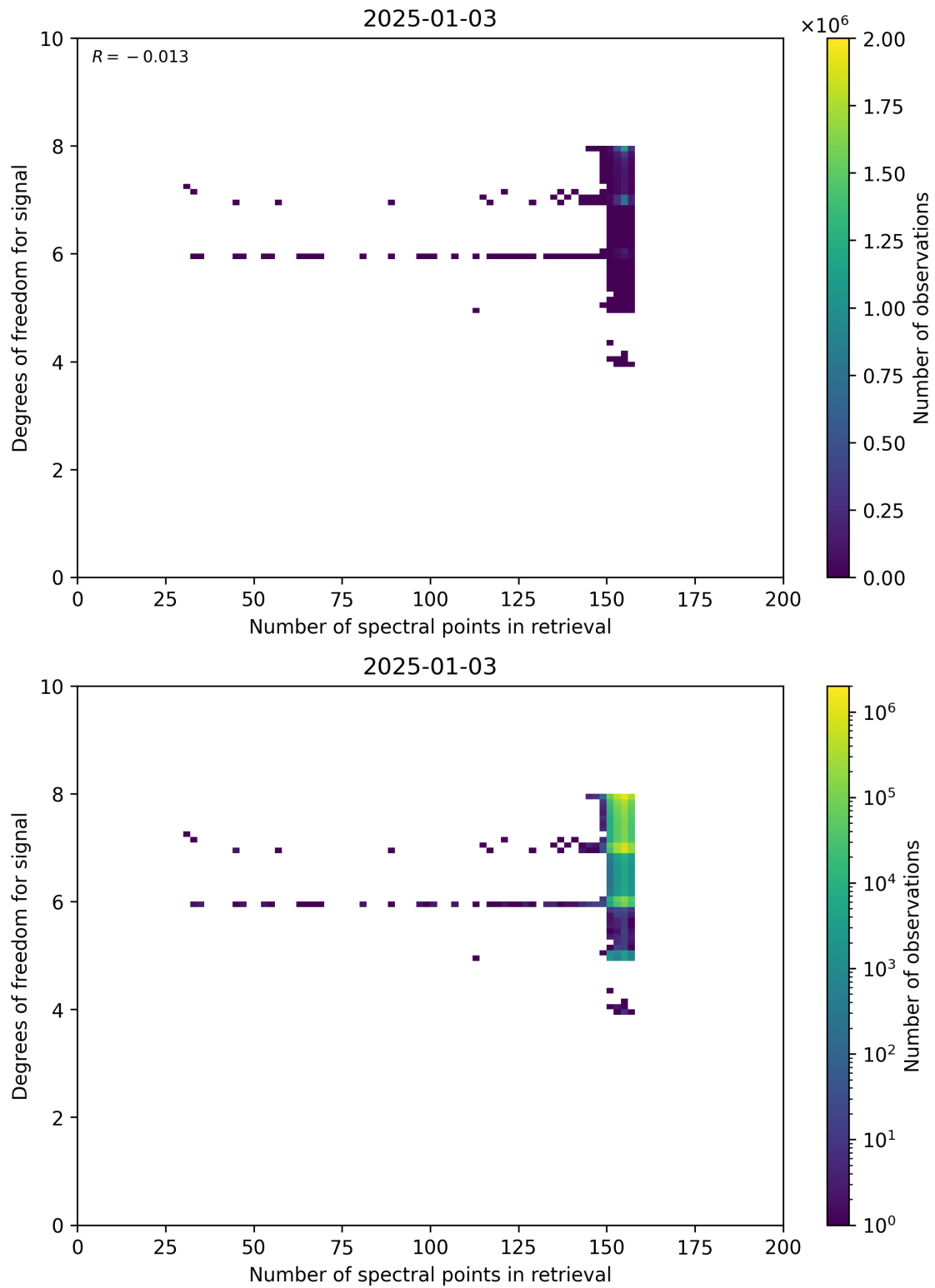
Figure 59: Scatter density plot of “Number of spectral points in retrieval” against “Degrees of freedom for signal” for 2025-01-02 to 2025-01-04.
