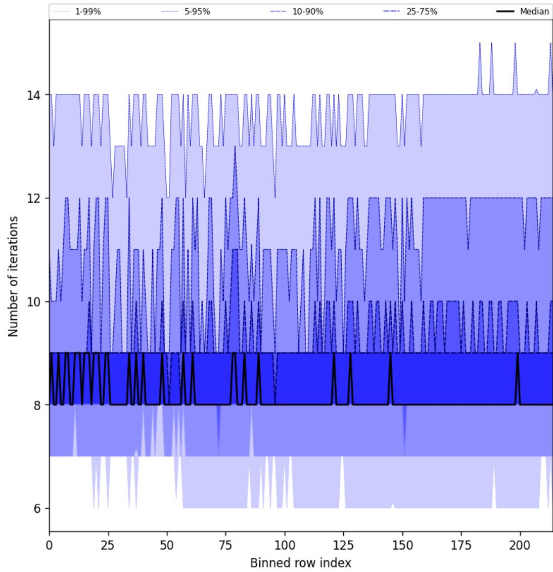
Figure 32: Along track statistics of “Number of iterations” for 2025-01-02 to 2025-01-04
