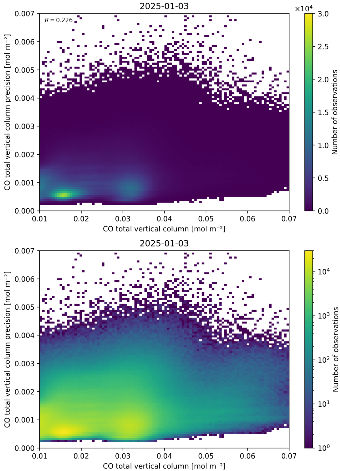
Figure 34: Scatter density plot of “CO total vertical column” against “CO total vertical column precision” for 2025-01-02 to 2025-01-04.
