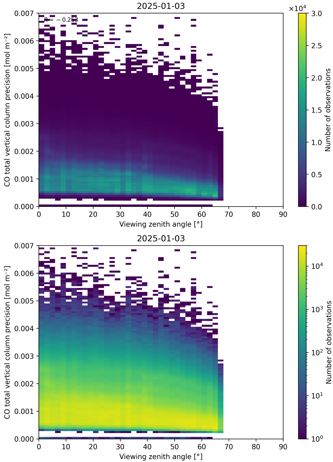
Figure 71: Scatter density plot of “Viewing zenith angle” against “CO total vertical column precision” for 2025-01-02 to 2025-01-04.
