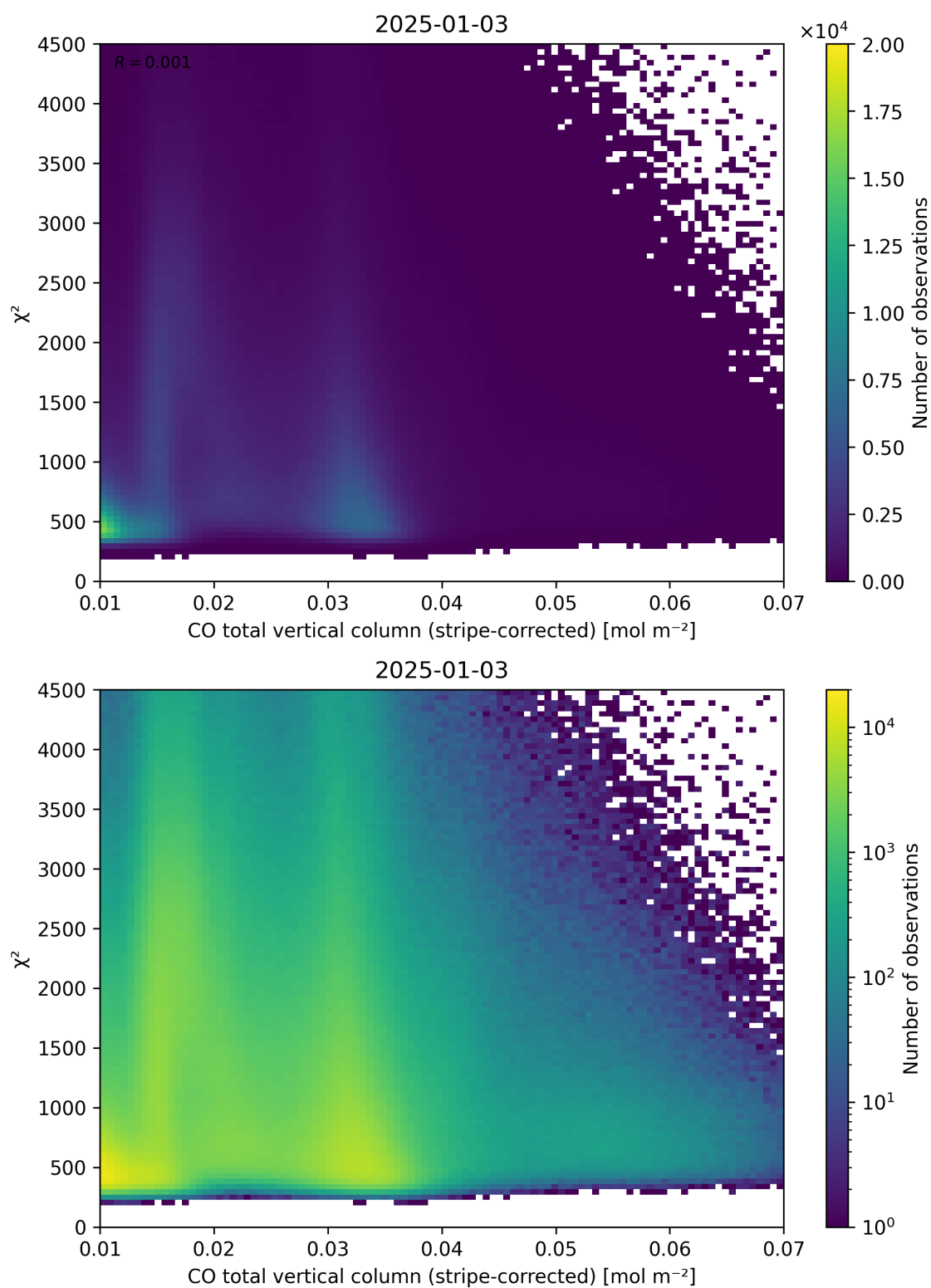
Figure 37: Scatter density plot of “CO total vertical column (stripe-corrected)” against “ \chi^2 ” for 2025-01-02 to 2025-01-04.
