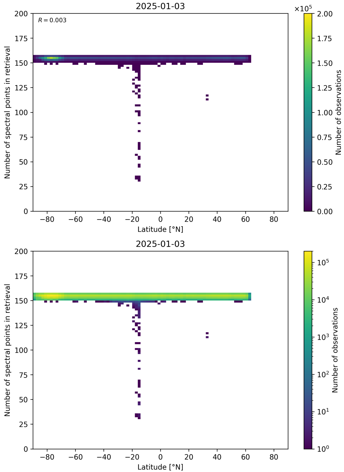
Figure 57: Scatter density plot of “Latitude” against “Number of spectral points in retrieval” for 2025-01-02 to 2025-01-04.
