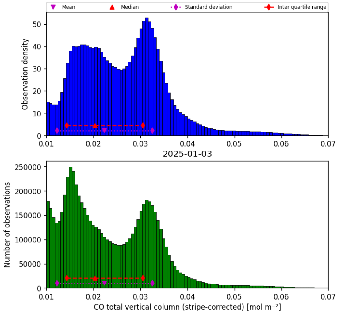
Figure 19: Histogram of “CO total vertical column (stripe-corrected)” for 2025-01-02 to 2025-01-04
