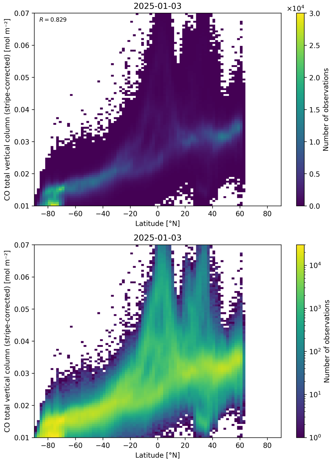
Figure 52: Scatter density plot of “Latitude” against “CO total vertical column (stripe-corrected)” for 2025-01-02 to 2025-01-04.
