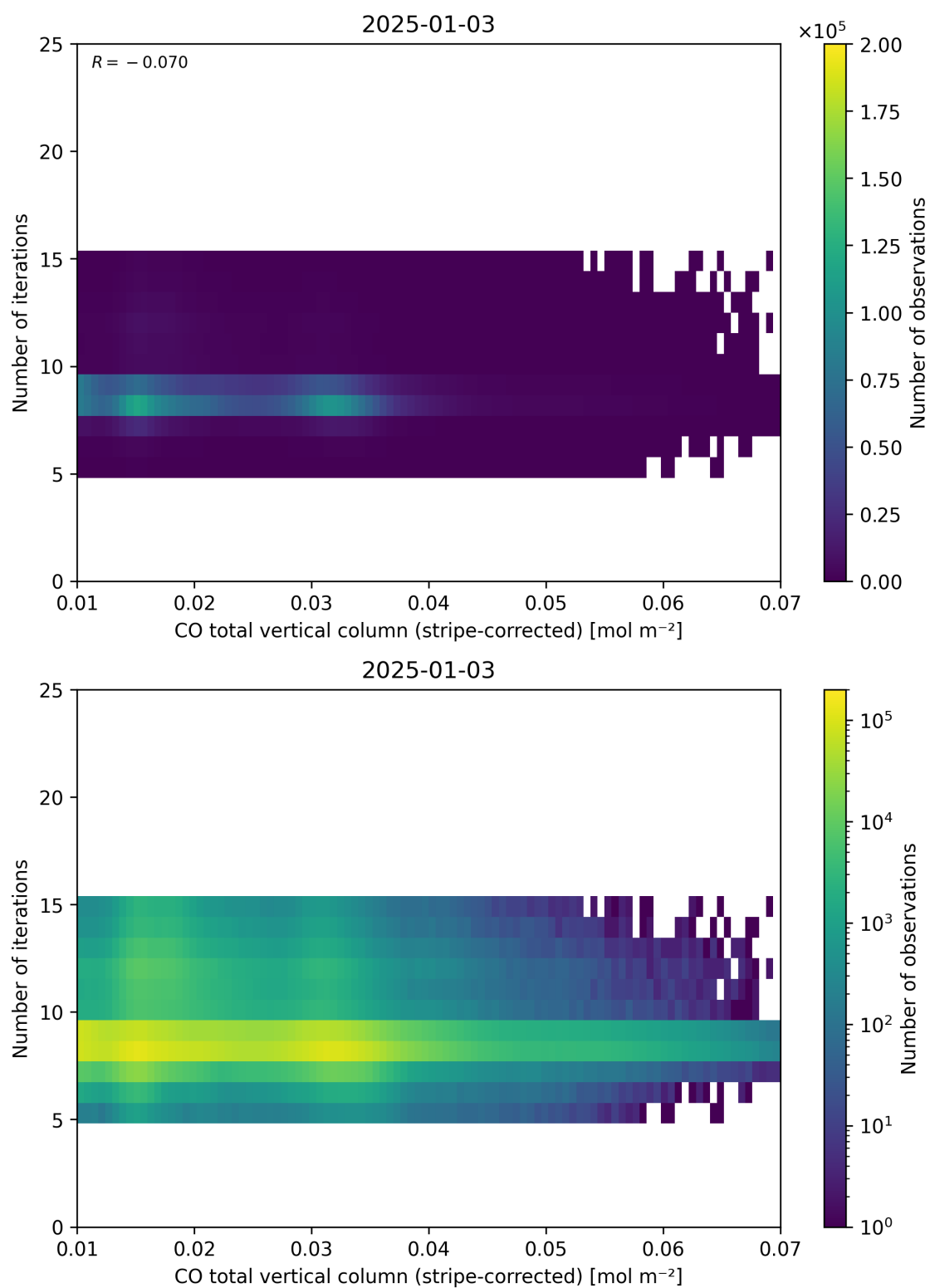
Figure 39: Scatter density plot of “CO total vertical column (stripe-corrected)” against “Number of iterations” for 2025-01-02 to 2025-01-04.
