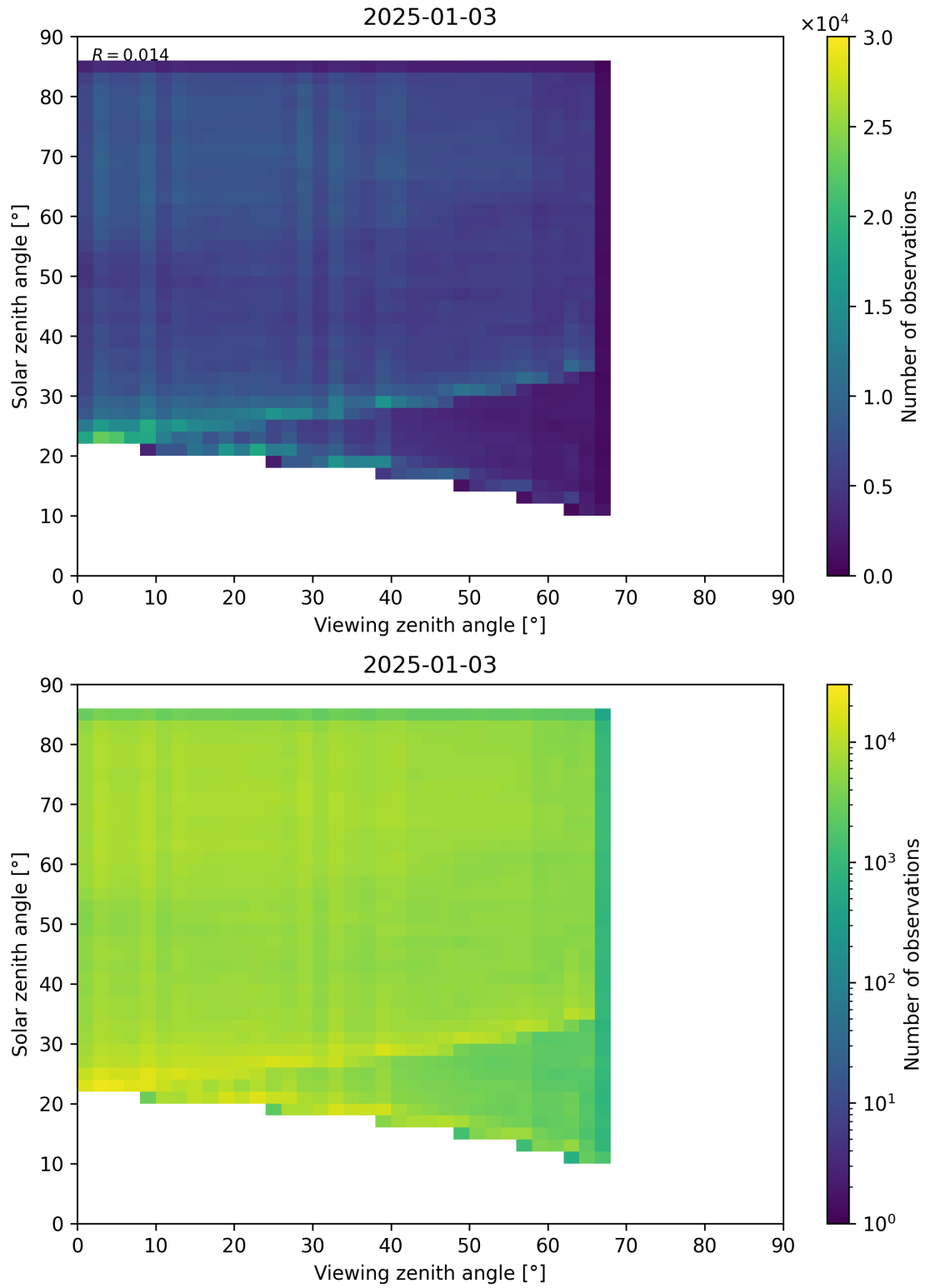
Figure 77: Scatter density plot of “Viewing zenith angle” against “Solar zenith angle” for 2025-01-02 to 2025-01-04.
