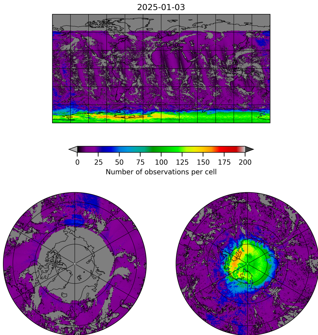
Figure 8: Map of the number of observations for 2025-01-02 to 2025-01-04
