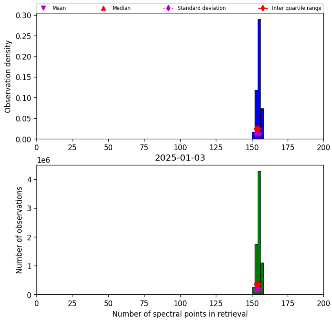
Figure 21: Histogram of “Number of spectral points in retrieval” for 2025-01-02 to 2025-01-04
