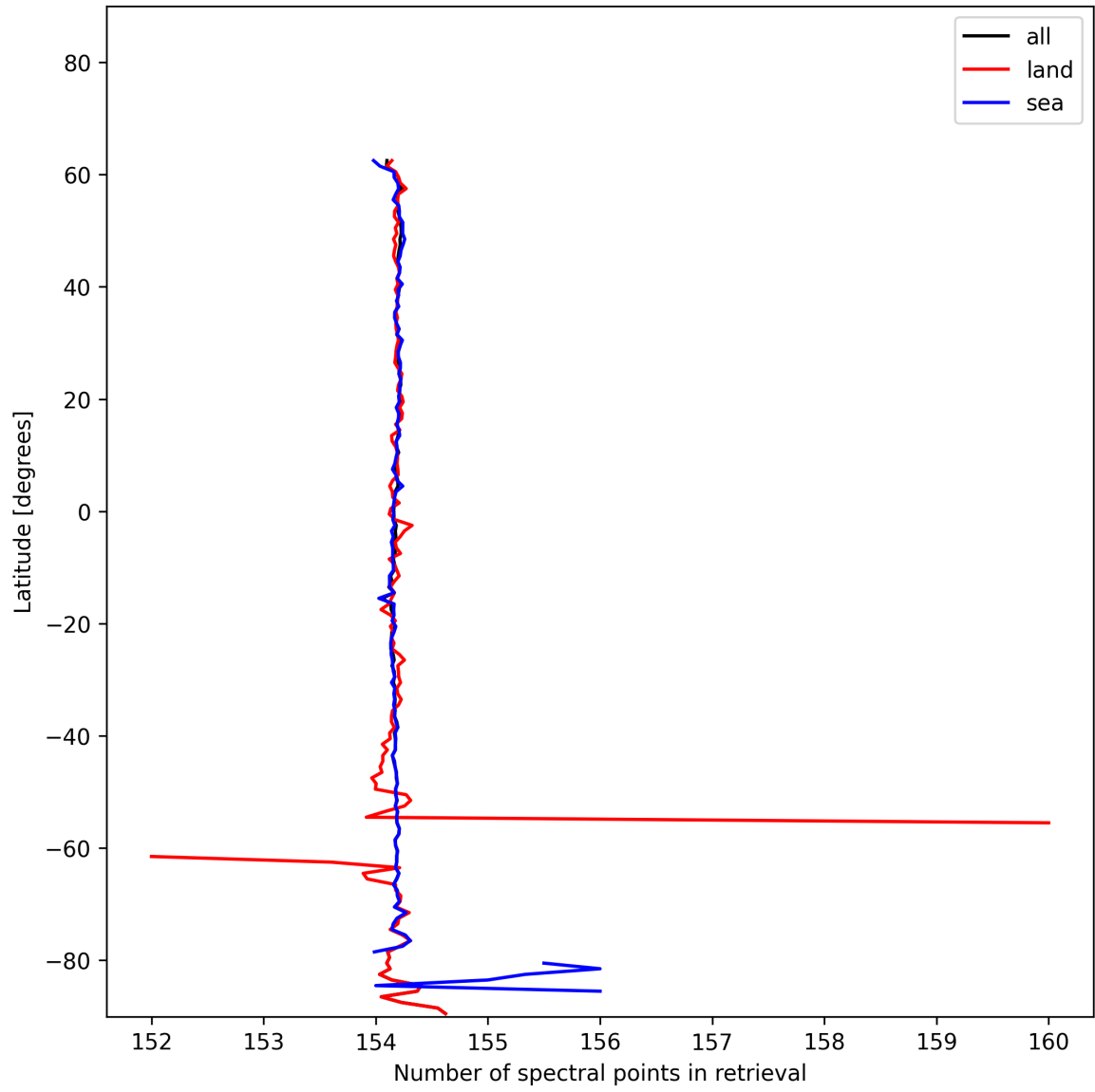
Figure 13: Zonal average of “Number of spectral points in retrieval” for 2025-01-02 to 2025-01-04.
