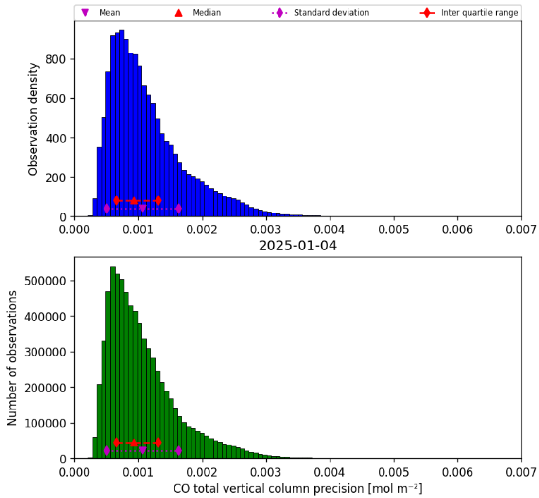
Figure 20: Histogram of “CO total vertical column precision” for 2025-01-03 to 2025-01-05
