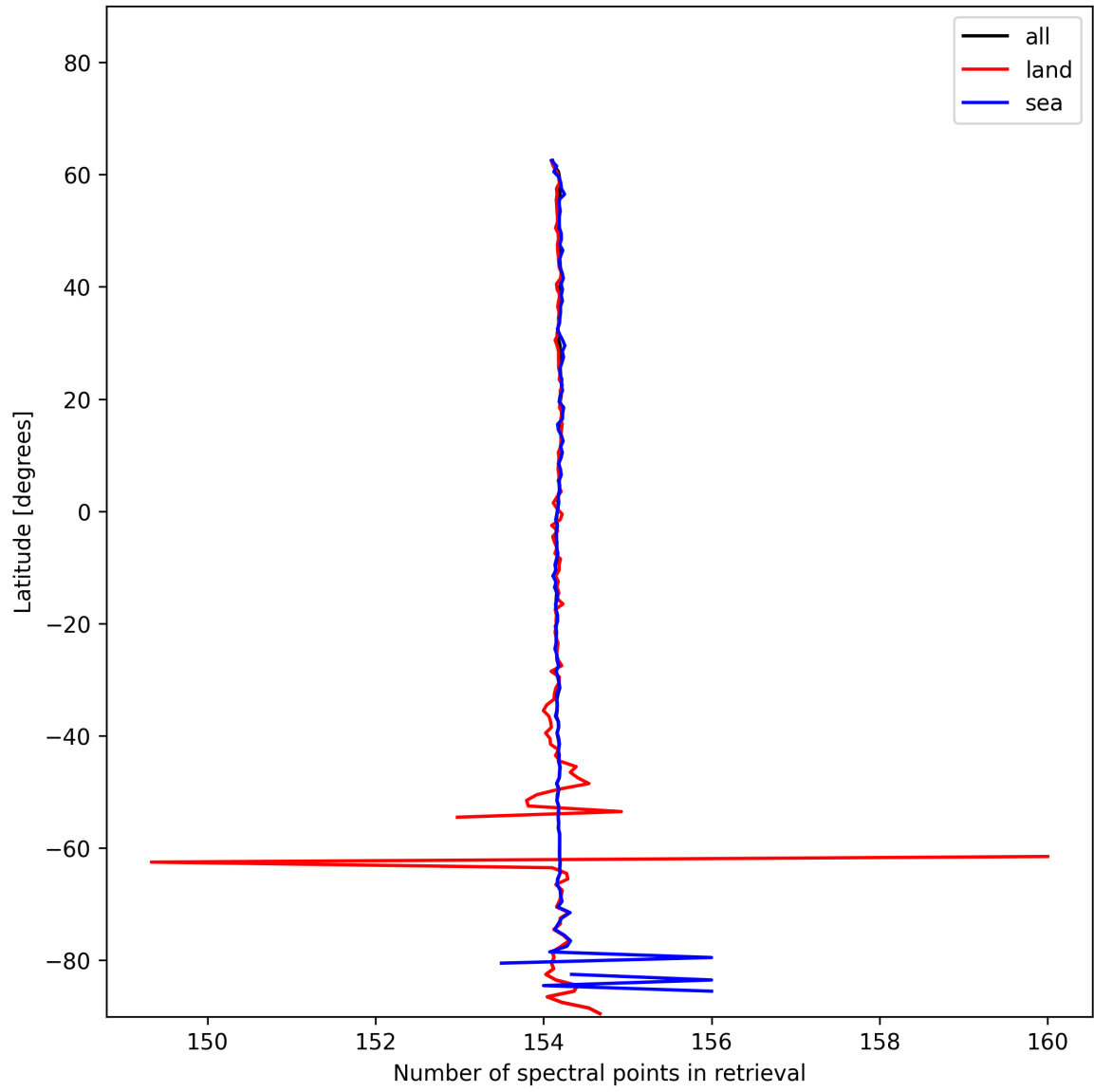
Figure 13: Zonal average of “Number of spectral points in retrieval” for 2025-01-03 to 2025-01-05.
