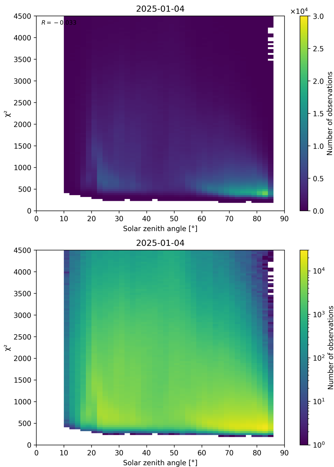
Figure 64: Scatter density plot of “Solar zenith angle” against “ \chi^2 ” for 2025-01-03 to 2025-01-05.
