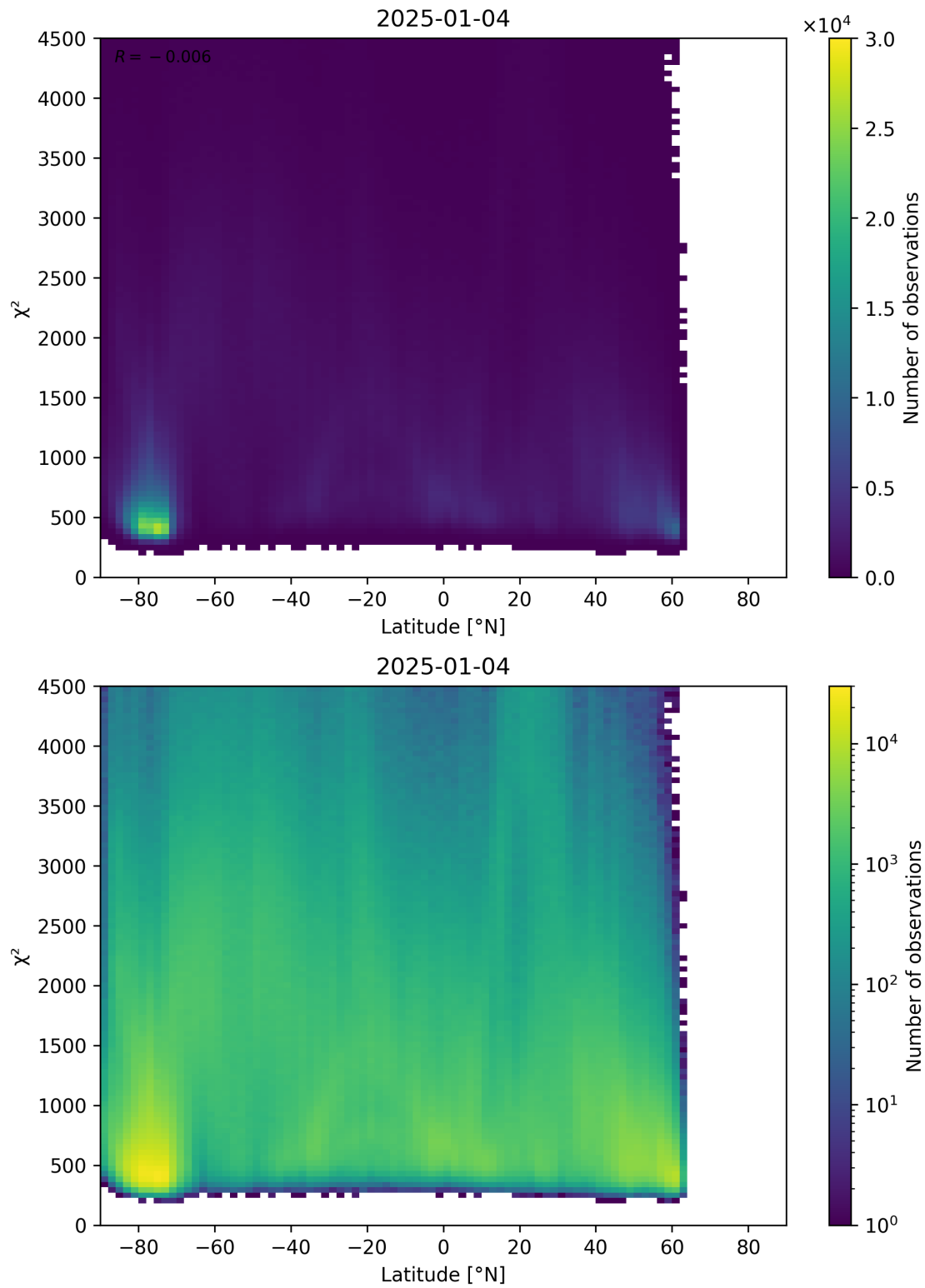
Figure 54: Scatter density plot of “Latitude” against “ \chi^2 ” for 2025-01-03 to 2025-01-05.
