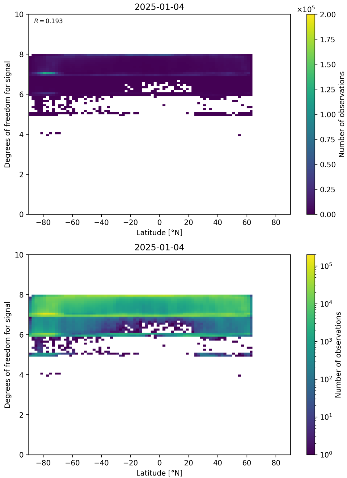
Figure 55: Scatter density plot of “Latitude” against “Degrees of freedom for signal” for 2025-01-03 to 2025-01-05.
