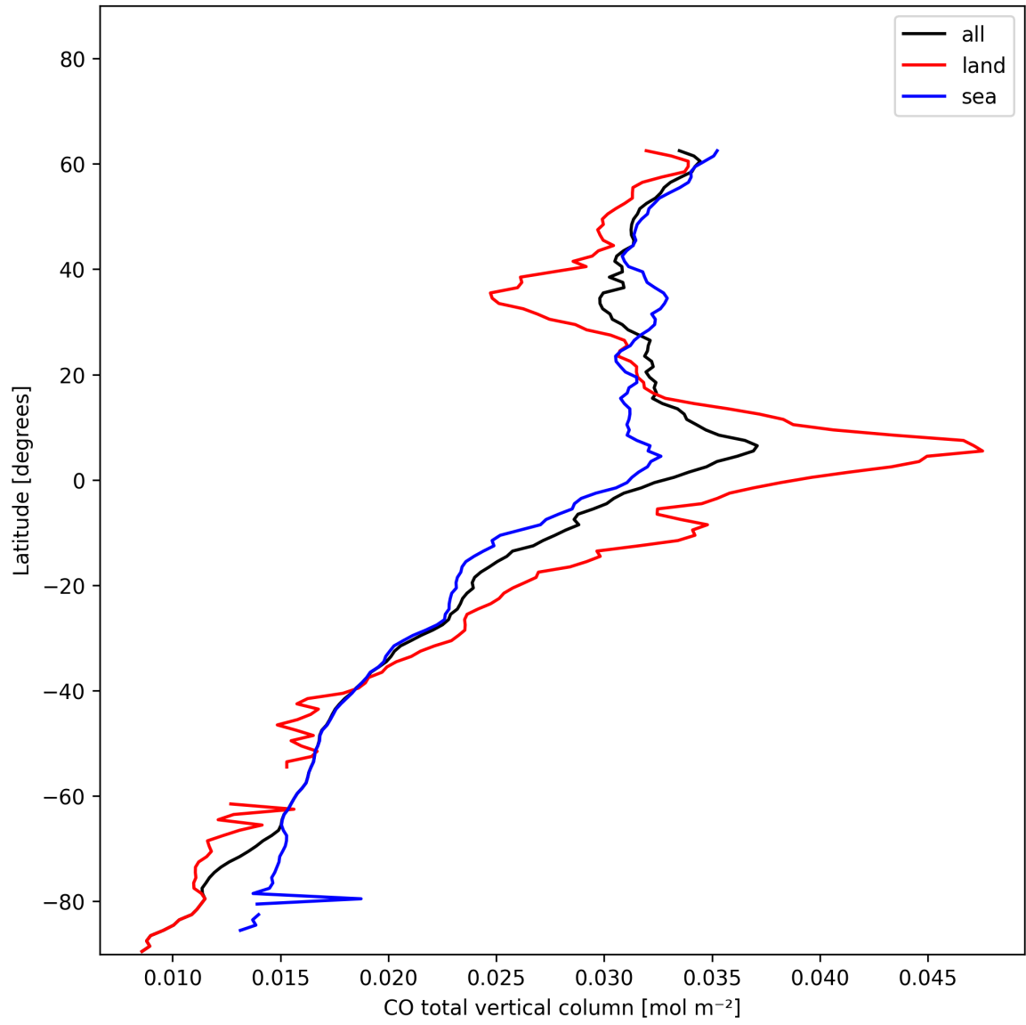
Figure 10: Zonal average of “CO total vertical column” for 2025-01-03 to 2025-01-05.
