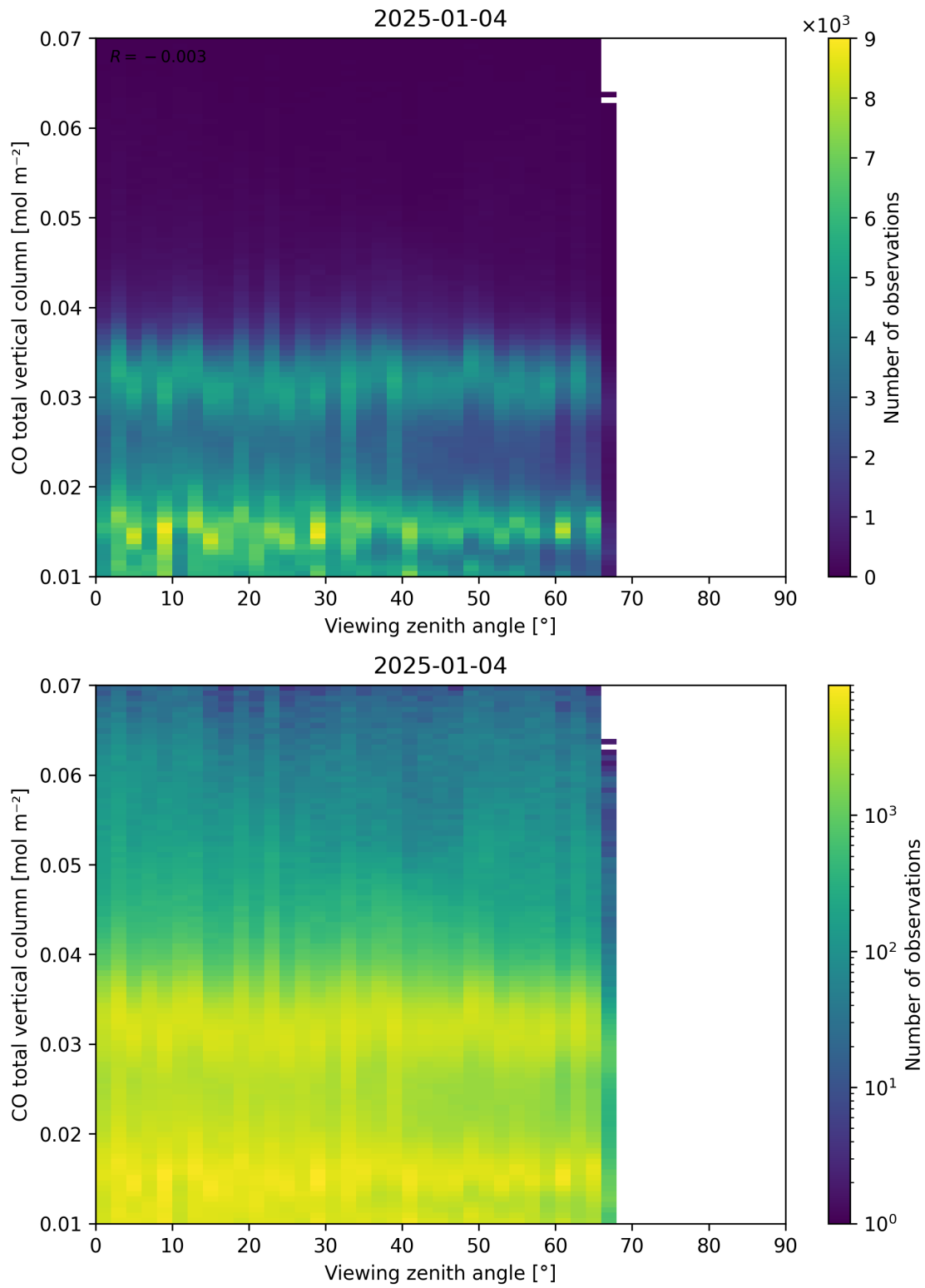
Figure 69: Scatter density plot of “Viewing zenith angle” against “CO total vertical column” for 2025-01-03 to 2025-01-05.
