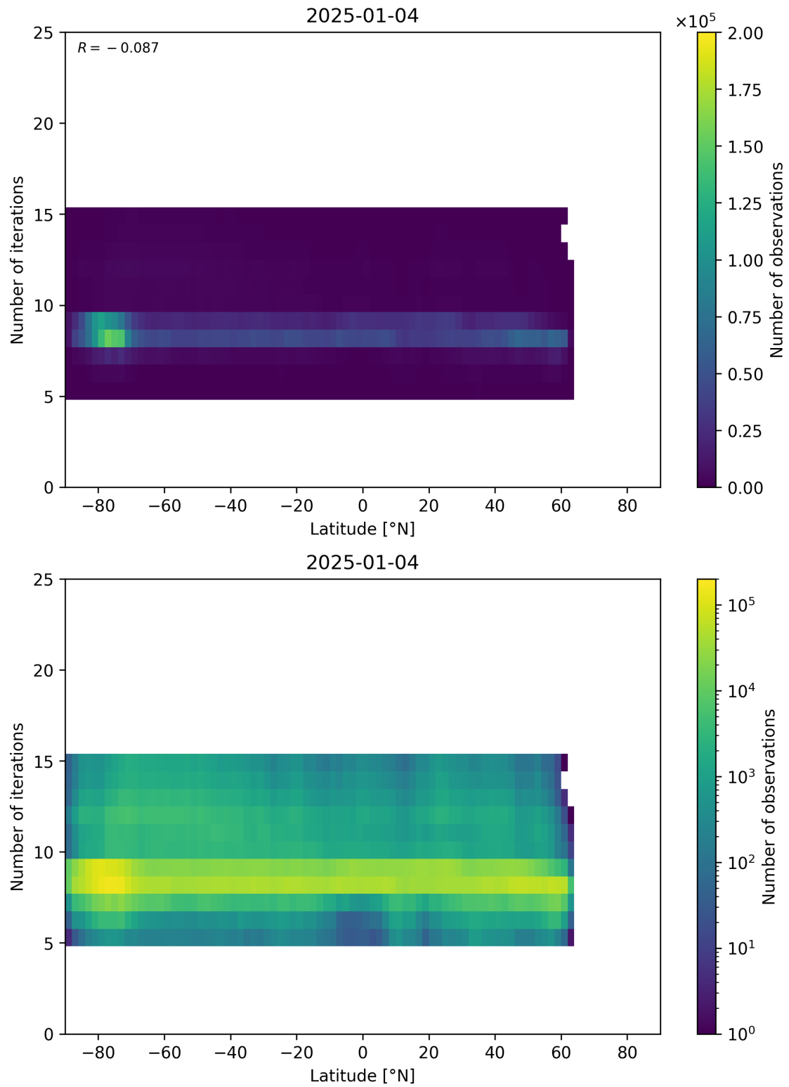
Figure 56: Scatter density plot of “Latitude” against “Number of iterations” for 2025-01-03 to 2025-01-05.
