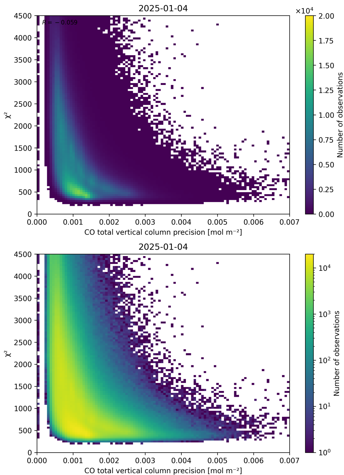
Figure 44: Scatter density plot of “CO total vertical column precision” against “ \chi^2 ” for 2025-01-03 to 2025-01-05.
