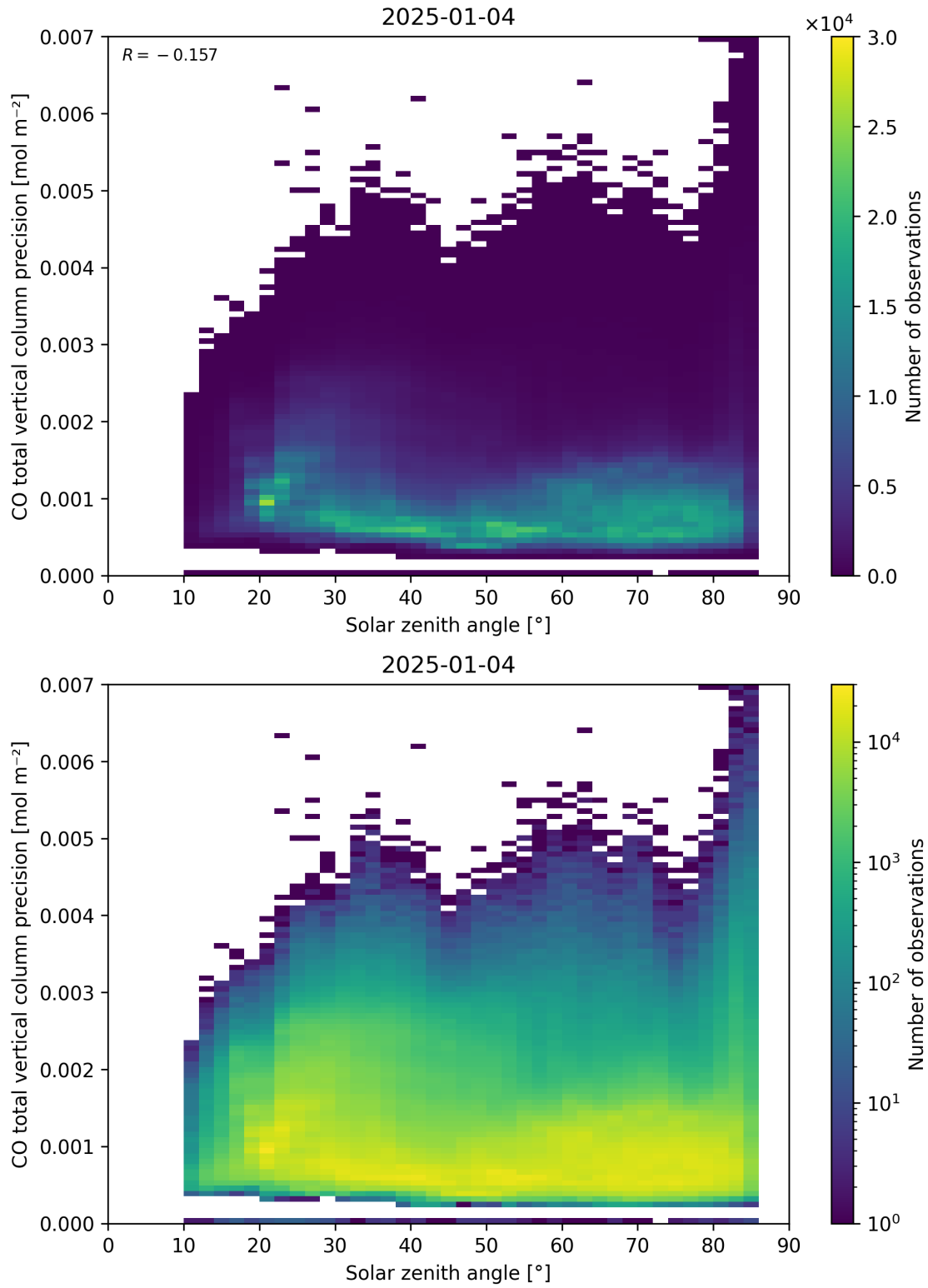
Figure 63: Scatter density plot of “Solar zenith angle” against “CO total vertical column precision” for 2025-01-03 to 2025-01-05.
