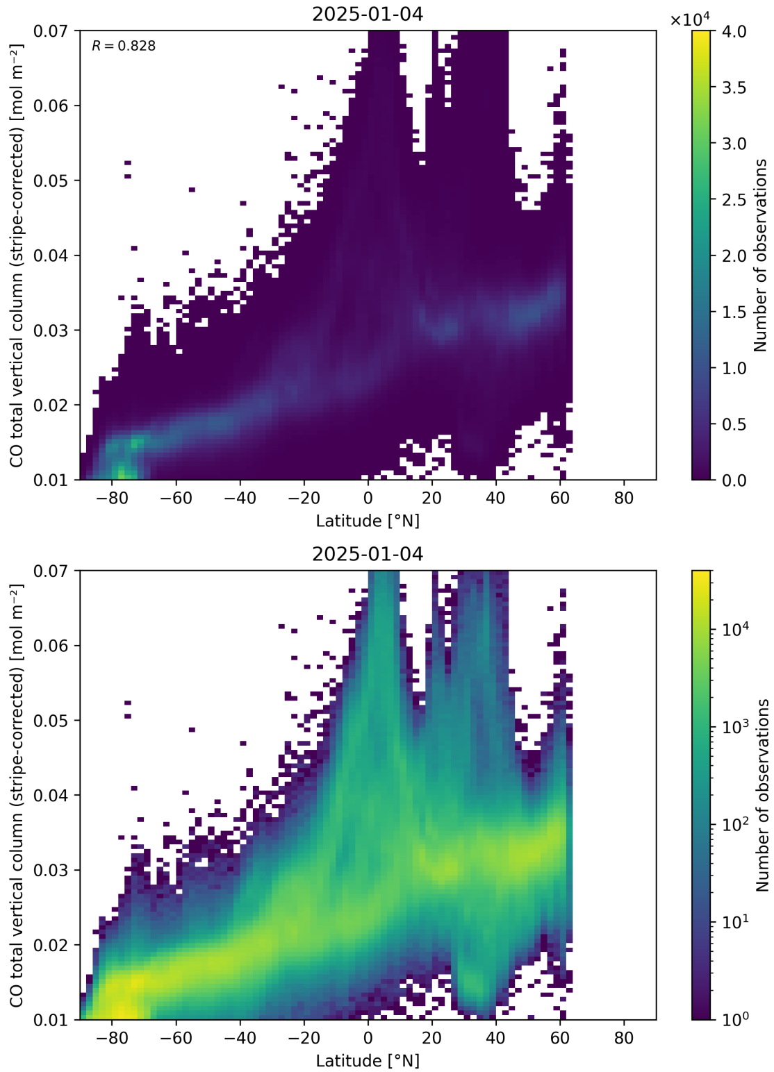
Figure 52: Scatter density plot of “Latitude” against “CO total vertical column (stripe-corrected)” for 2025-01-03 to 2025-01-05.
