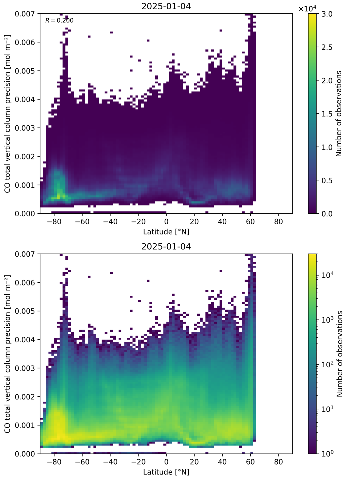
Figure 53: Scatter density plot of “Latitude” against “CO total vertical column precision” for 2025-01-03 to 2025-01-05.
