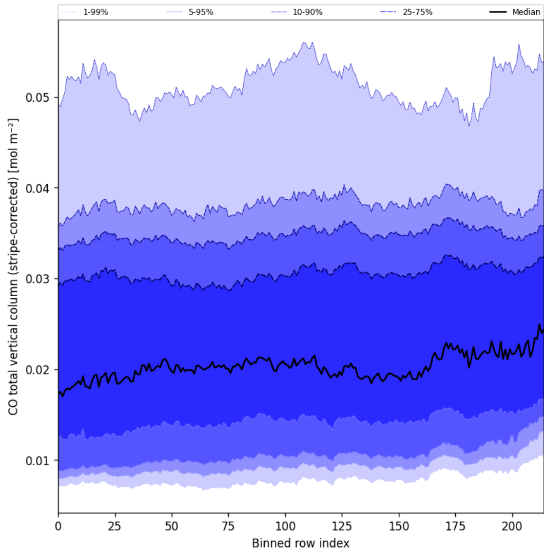
Figure 27: Along track statistics of “CO total vertical column (stripe-corrected)” for 2025-01-03 to 2025-01-05
