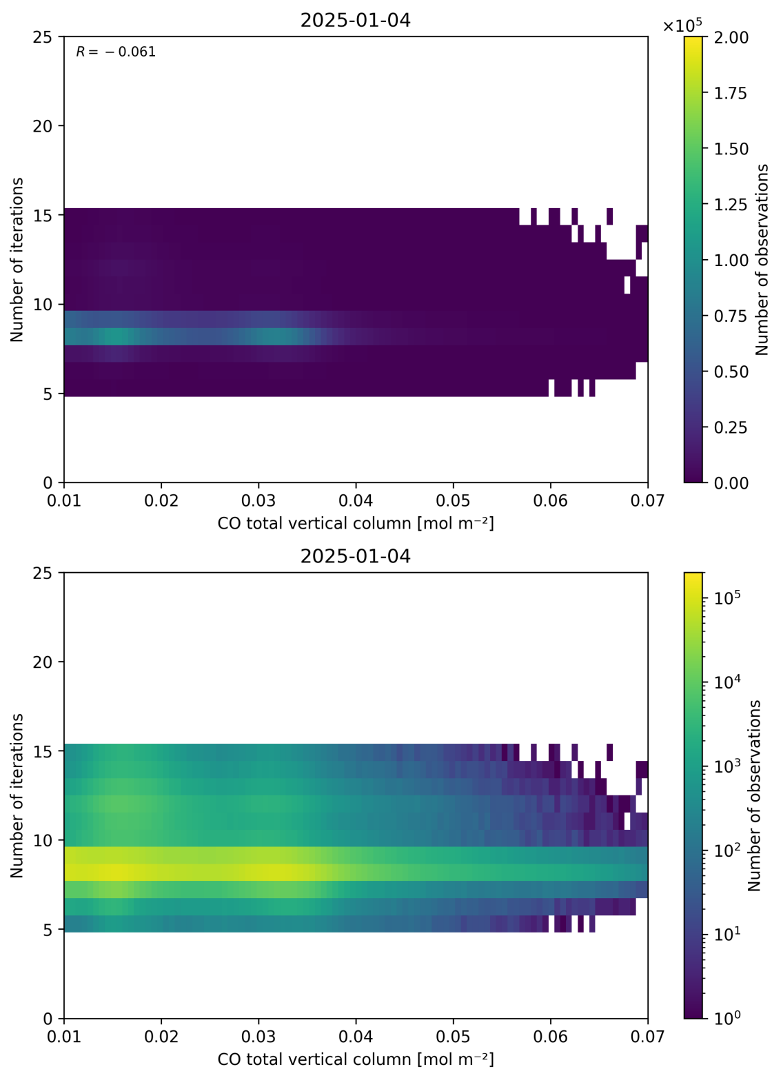
Figure 42: Scatter density plot of “CO total vertical column” against “Number of iterations” for 2025-01-03 to 2025-01-05.
