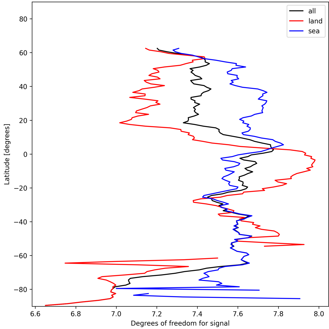
Figure 15: Zonal average of “Degrees of freedom for signal” for 2025-01-03 to 2025-01-05.
