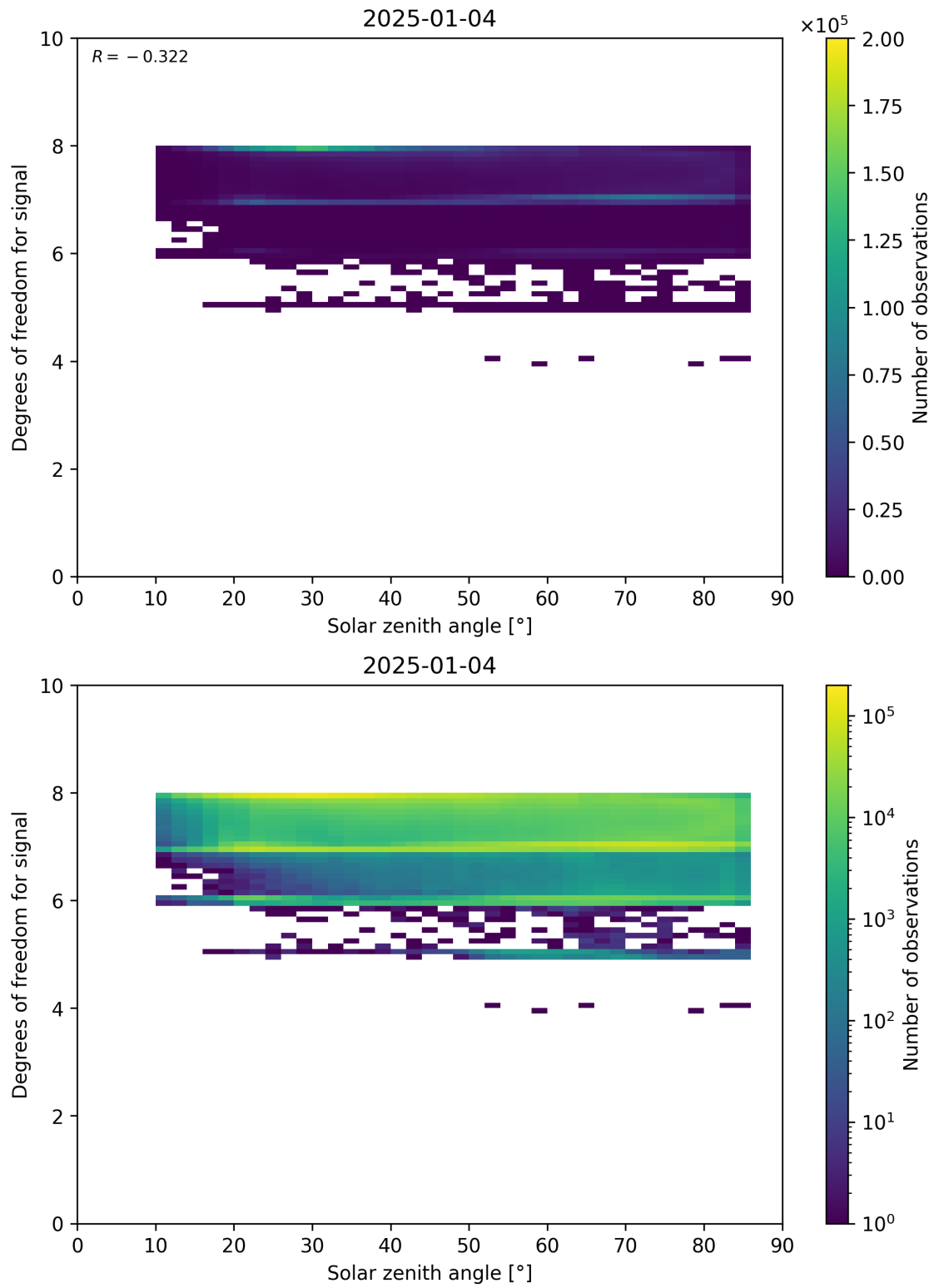
Figure 65: Scatter density plot of “Solar zenith angle” against “Degrees of freedom for signal” for 2025-01-03 to 2025-01-05.
