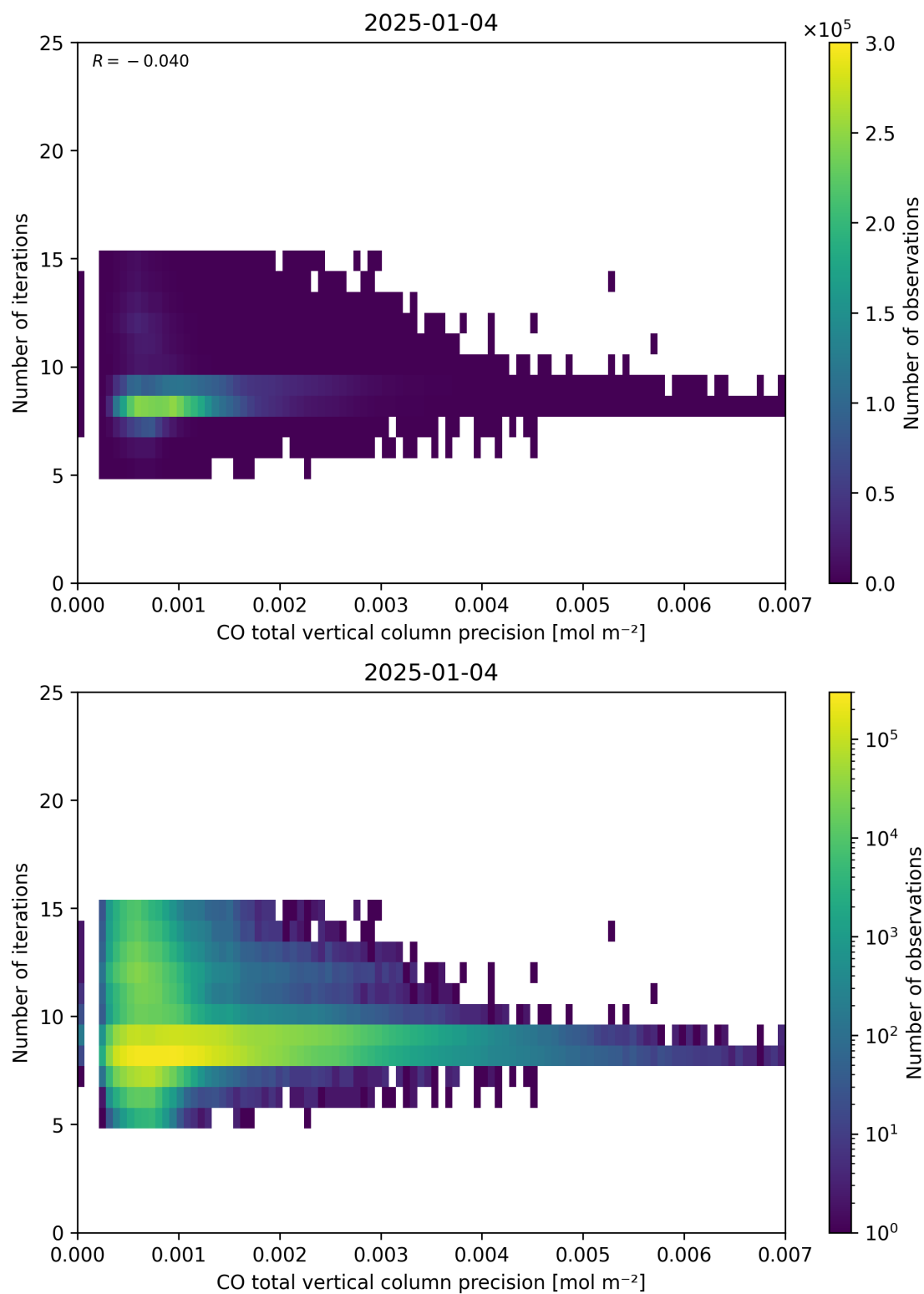
Figure 46: Scatter density plot of “CO total vertical column precision” against “Number of iterations” for 2025-01-03 to 2025-01-05.
