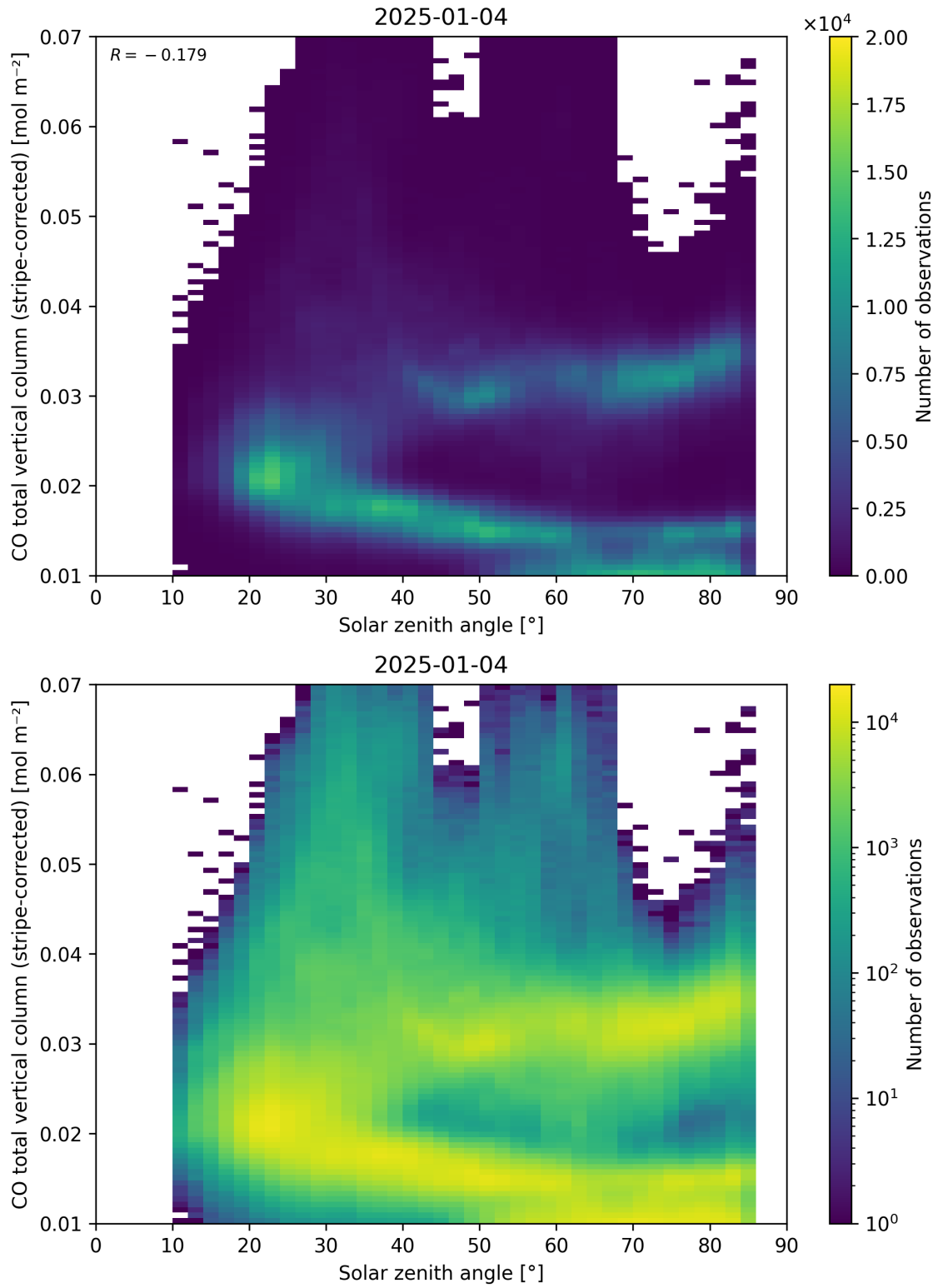
Figure 62: Scatter density plot of “Solar zenith angle” against “CO total vertical column (stripe-corrected)” for 2025-01-03 to 2025-01-05.
