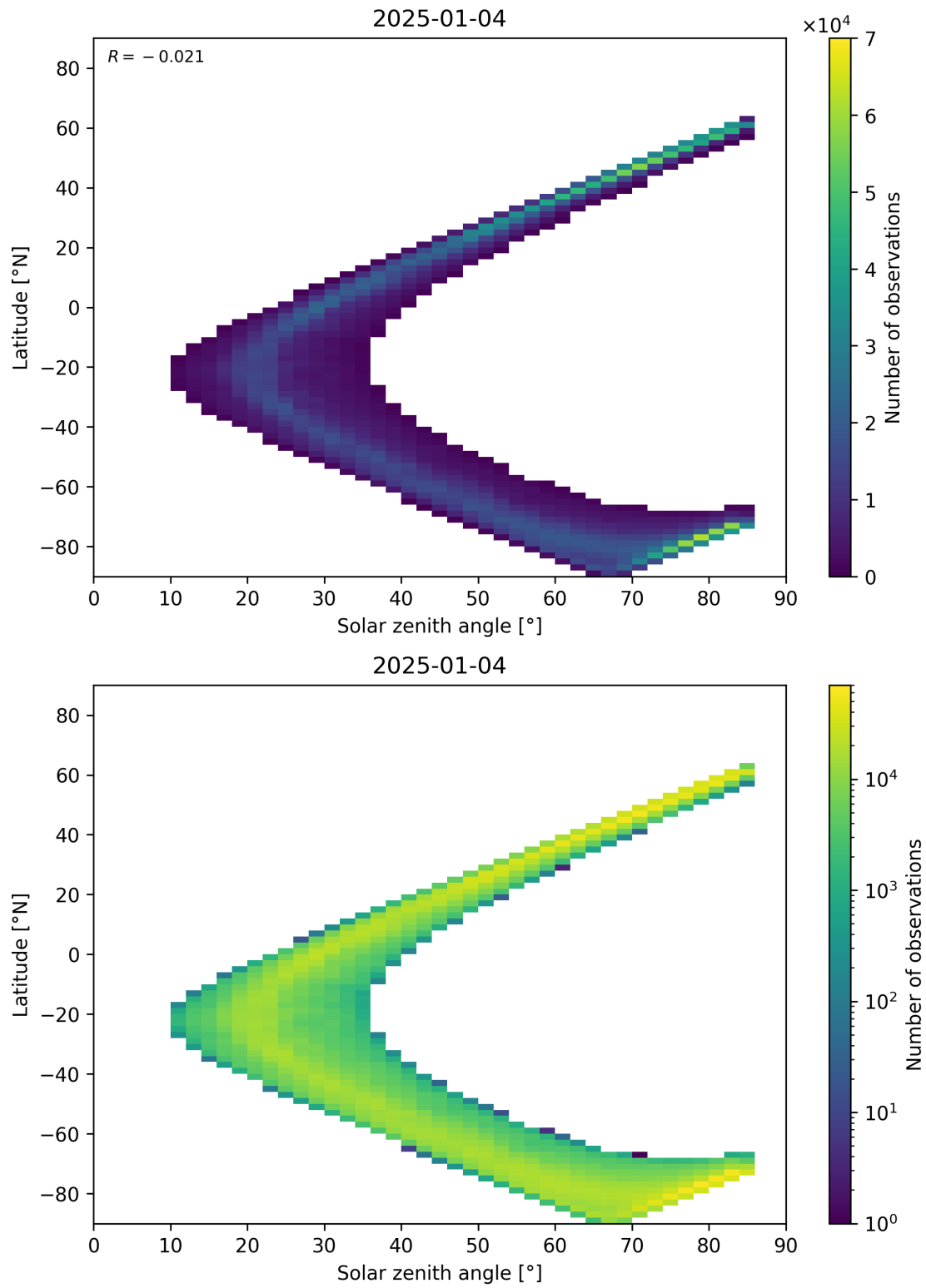
Figure 66: Scatter density plot of “Solar zenith angle” against “Latitude” for 2025-01-03 to 2025-01-05.
