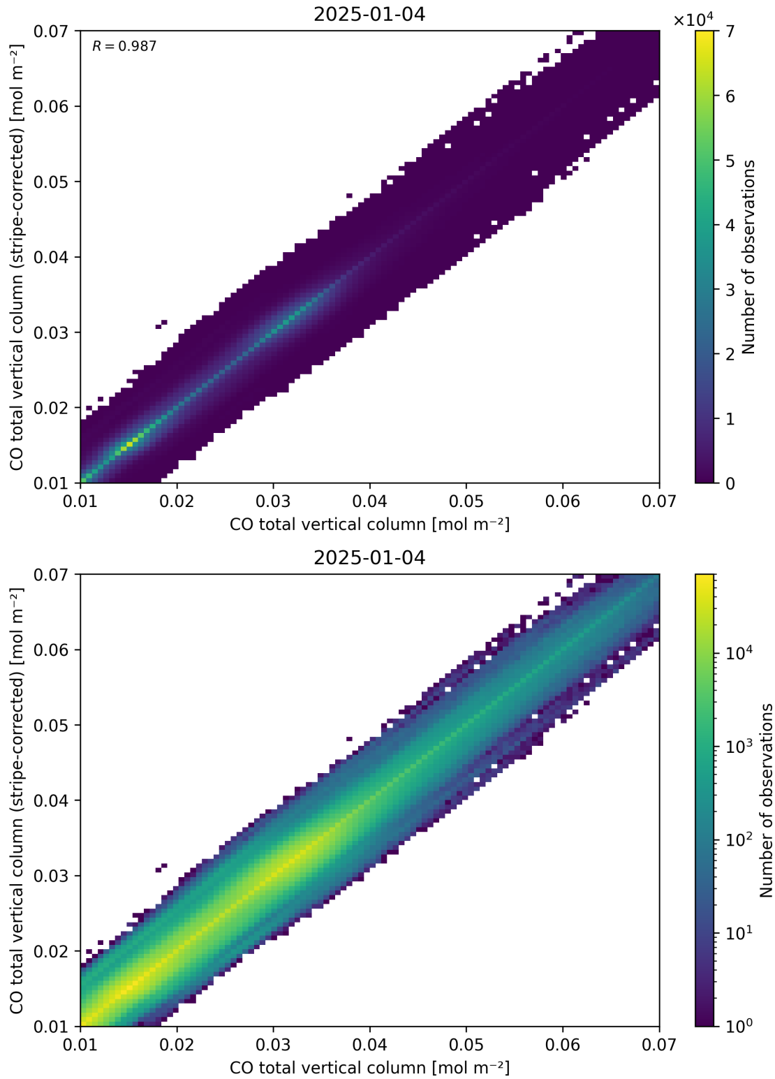
Figure 33: Scatter density plot of “CO total vertical column” against “CO total vertical column (stripe-corrected)” for 2025-01-03 to 2025-01-05.
