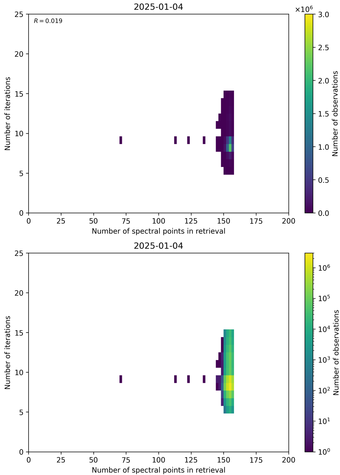
Figure 60: Scatter density plot of “Number of spectral points in retrieval” against “Number of iterations” for 2025-01-03 to 2025-01-05.
