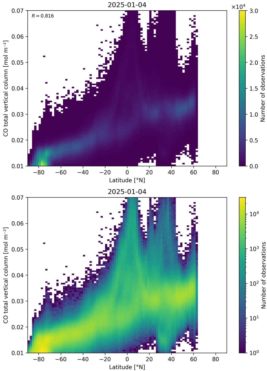
Figure 51: Scatter density plot of “Latitude” against “CO total vertical column” for 2025-01-03 to 2025-01-05.
