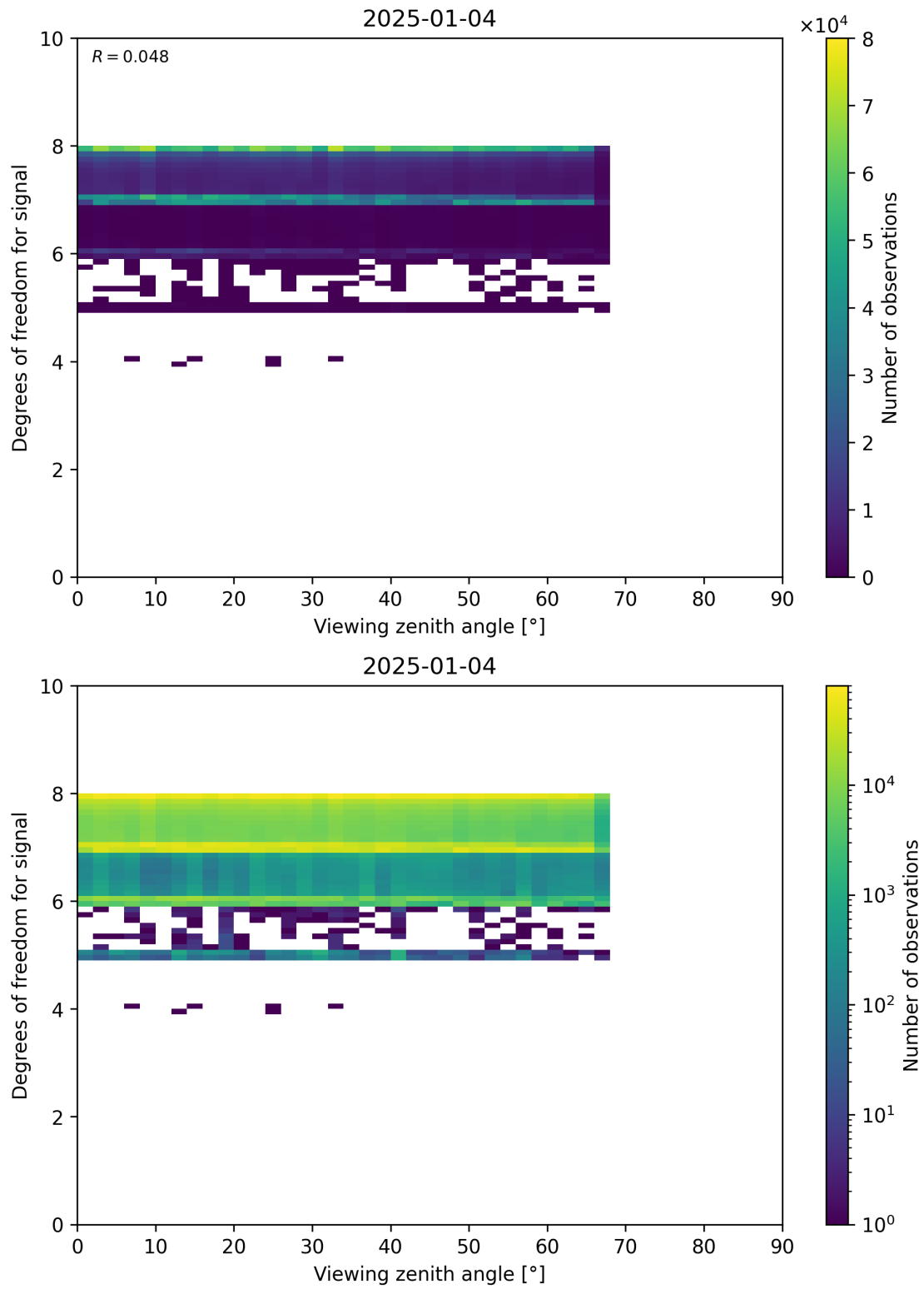
Figure 73: Scatter density plot of “Viewing zenith angle” against “Degrees of freedom for signal” for 2025-01-03 to 2025-01-05.
