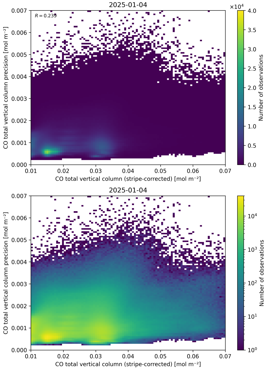
Figure 36: Scatter density plot of “CO total vertical column (stripe-corrected)” against “CO total vertical column precision” for 2025-01-03 to 2025-01-05.
