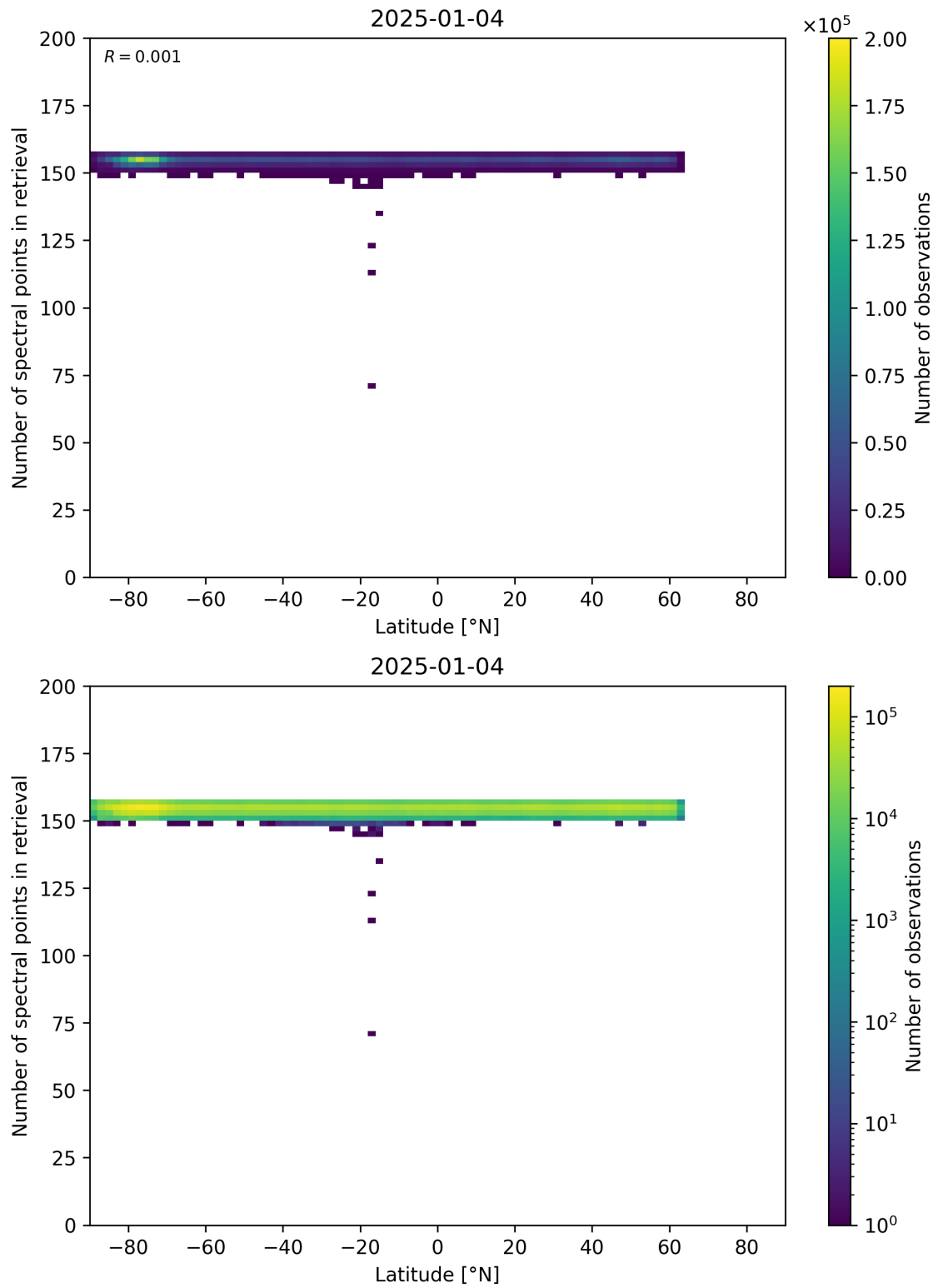
Figure 57: Scatter density plot of “Latitude” against “Number of spectral points in retrieval” for 2025-01-03 to 2025-01-05.
