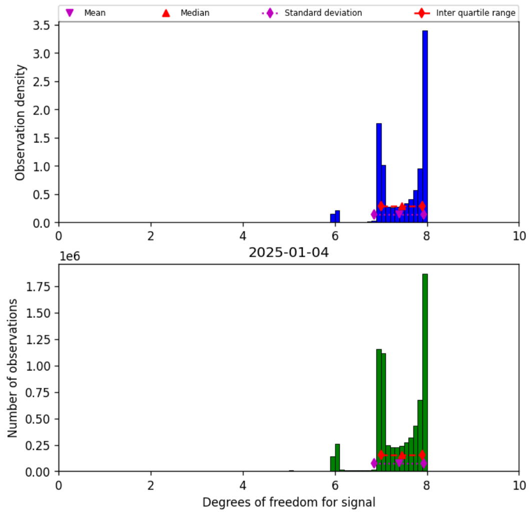
Figure 23: Histogram of “Degrees of freedom for signal” for 2025-01-03 to 2025-01-05
