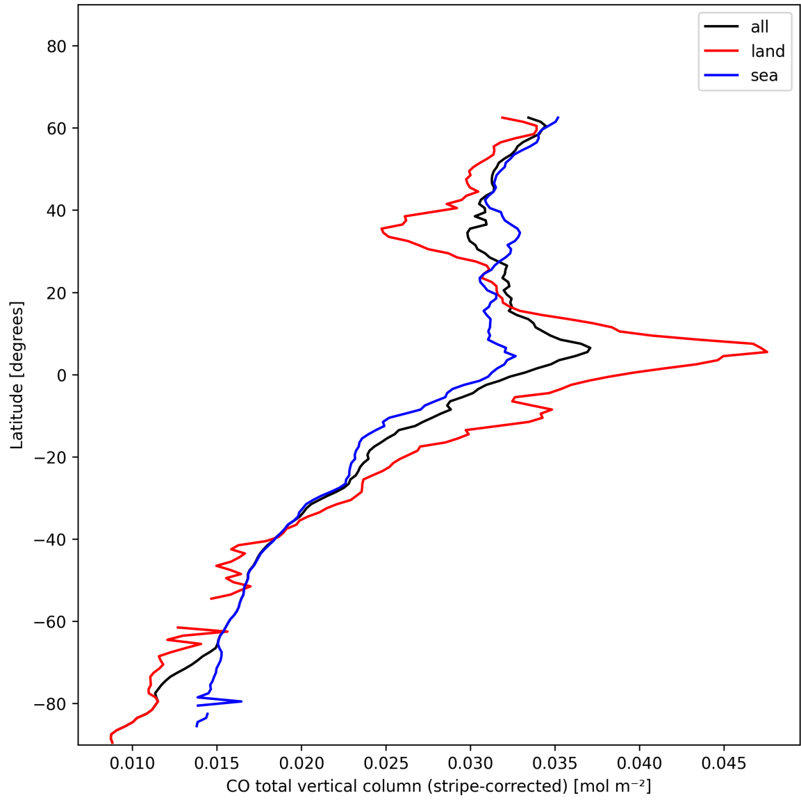
Figure 11: Zonal average of “CO total vertical column (stripe-corrected)” for 2025-01-03 to 2025-01-05.
