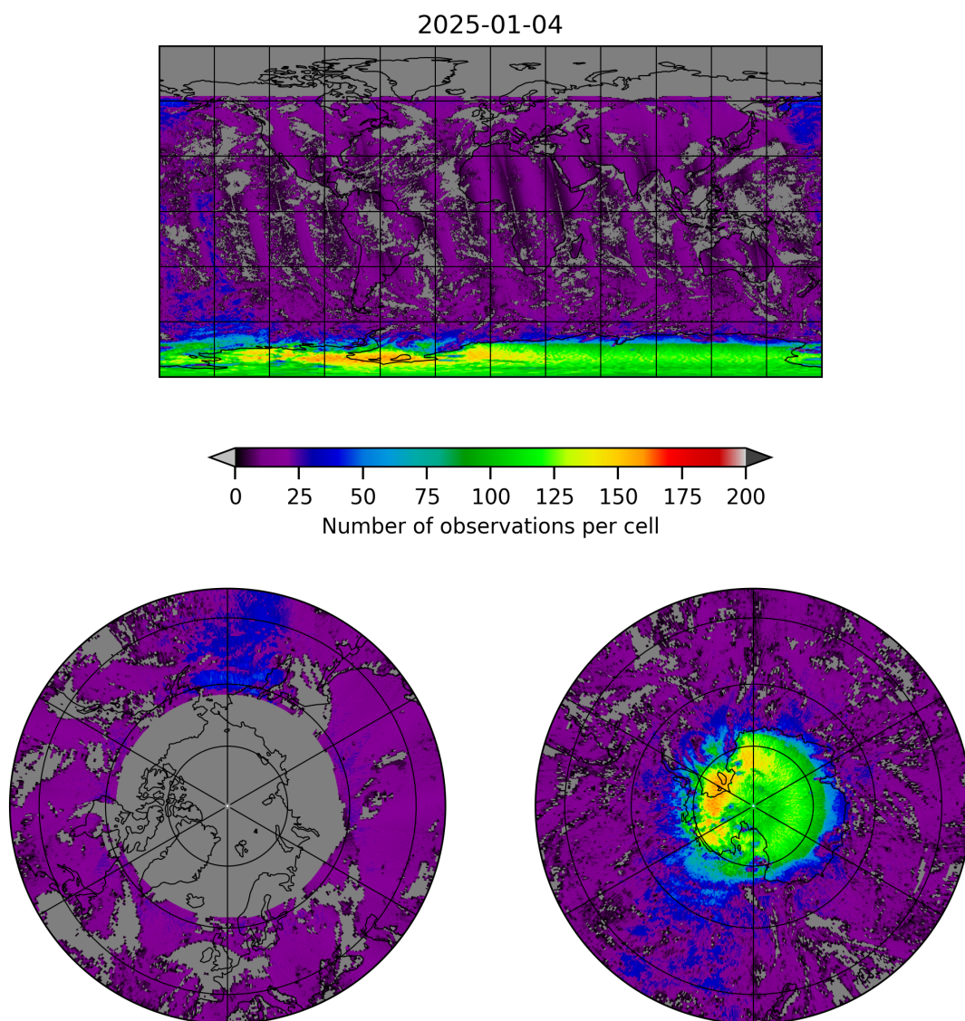
Figure 8: Map of the number of observations for 2025-01-03 to 2025-01-05
