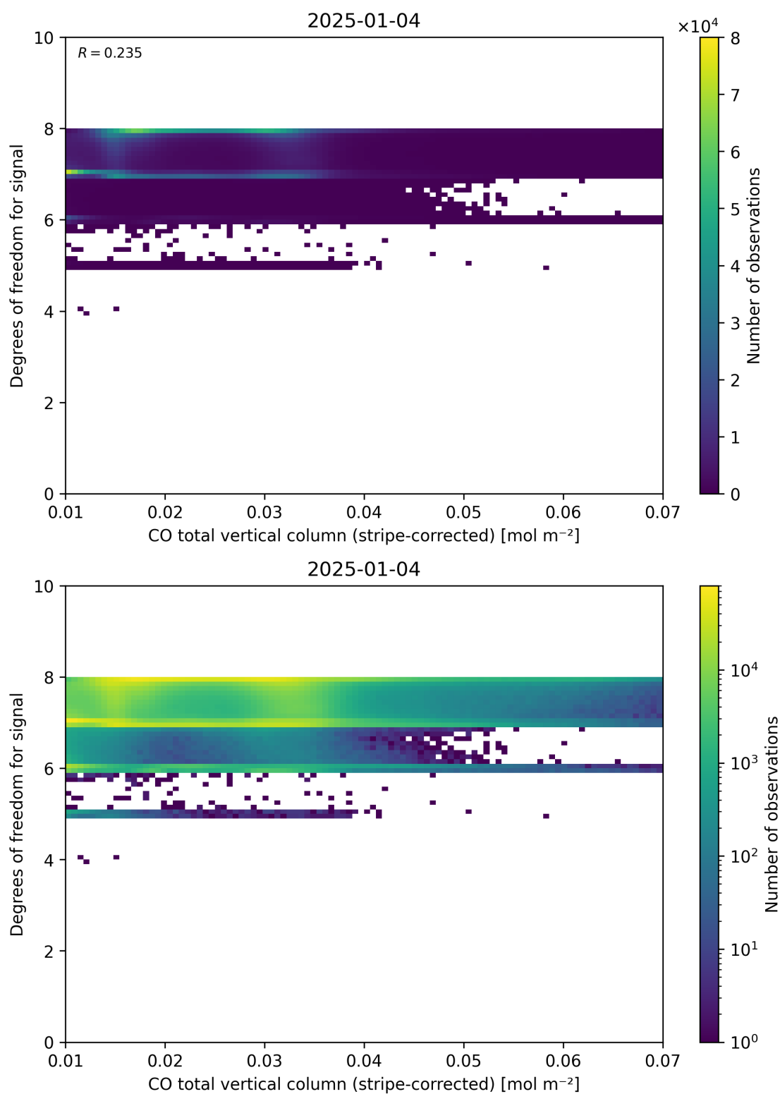
Figure 38: Scatter density plot of “CO total vertical column (stripe-corrected)” against “Degrees of freedom for signal” for 2025-01-03 to 2025-01-05.
