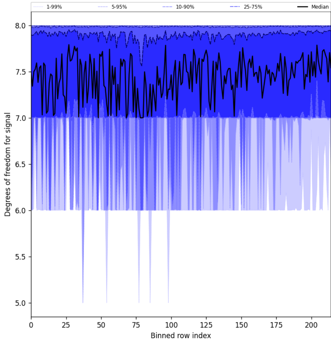
Figure 31: Along track statistics of “Degrees of freedom for signal” for 2025-01-03 to 2025-01-05
