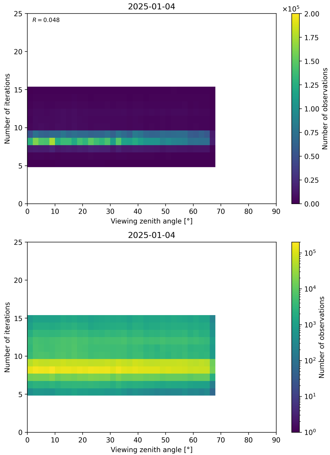
Figure 75: Scatter density plot of “Viewing zenith angle” against “Number of iterations” for 2025-01-03 to 2025-01-05.
