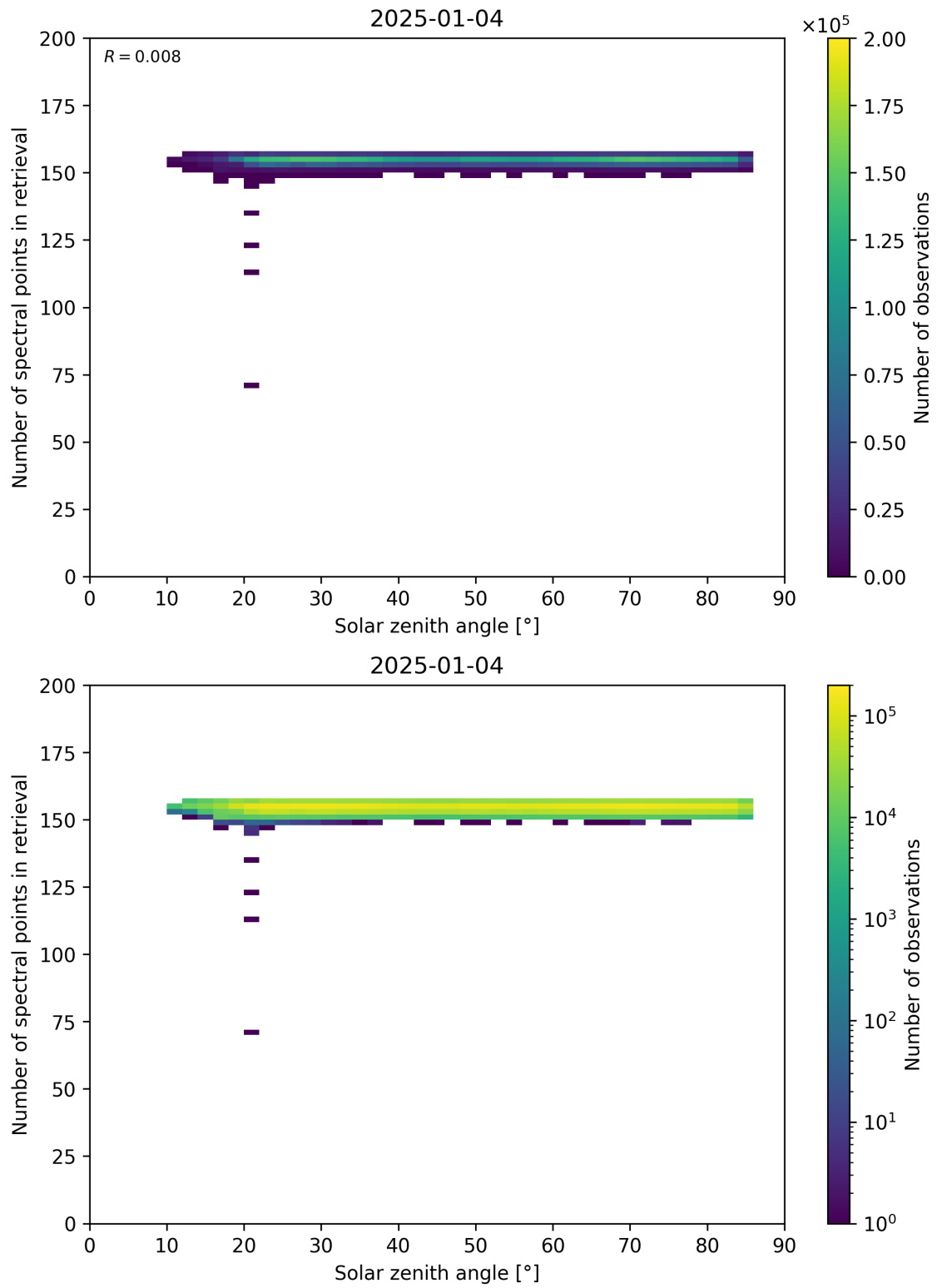
Figure 68: Scatter density plot of “Solar zenith angle” against “Number of spectral points in retrieval” for 2025-01-03 to 2025-01-05.
