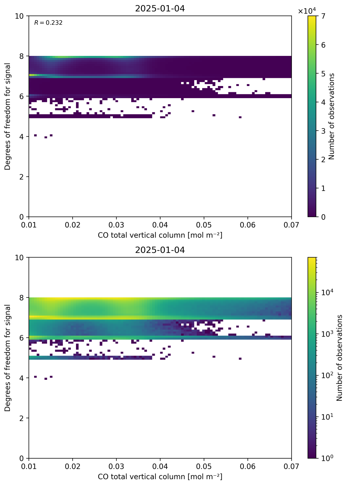
Figure 41: Scatter density plot of “CO total vertical column” against “Degrees of freedom for signal” for 2025-01-03 to 2025-01-05.
