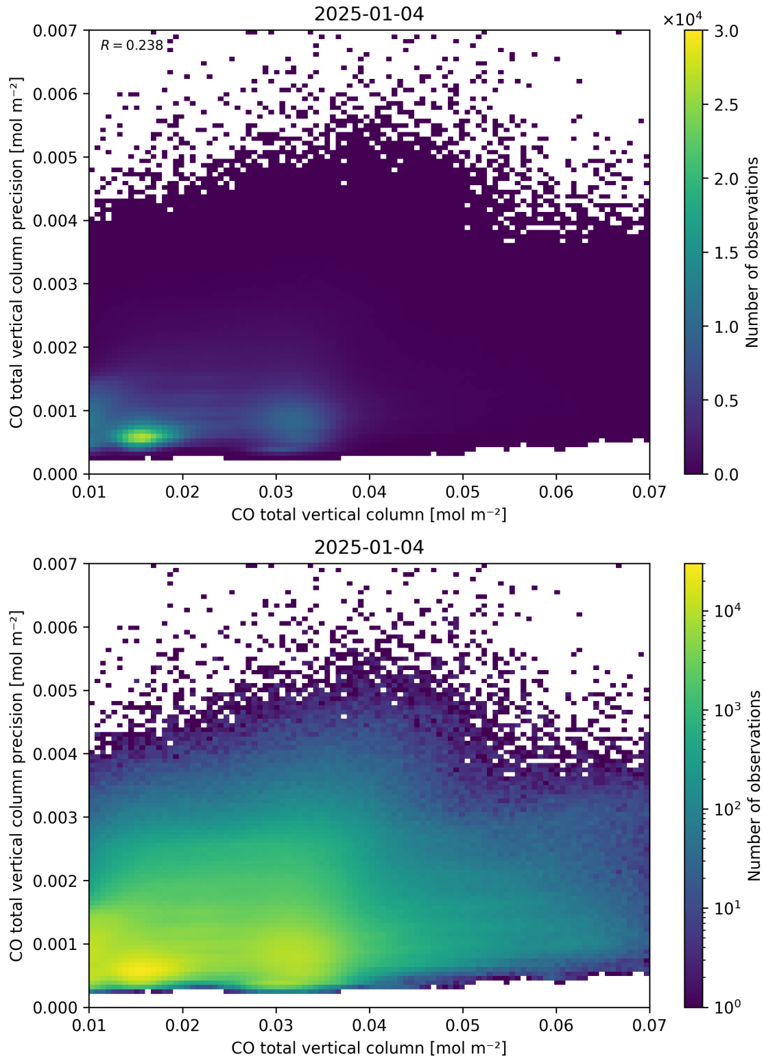
Figure 34: Scatter density plot of “CO total vertical column” against “CO total vertical column precision” for 2025-01-03 to 2025-01-05.
