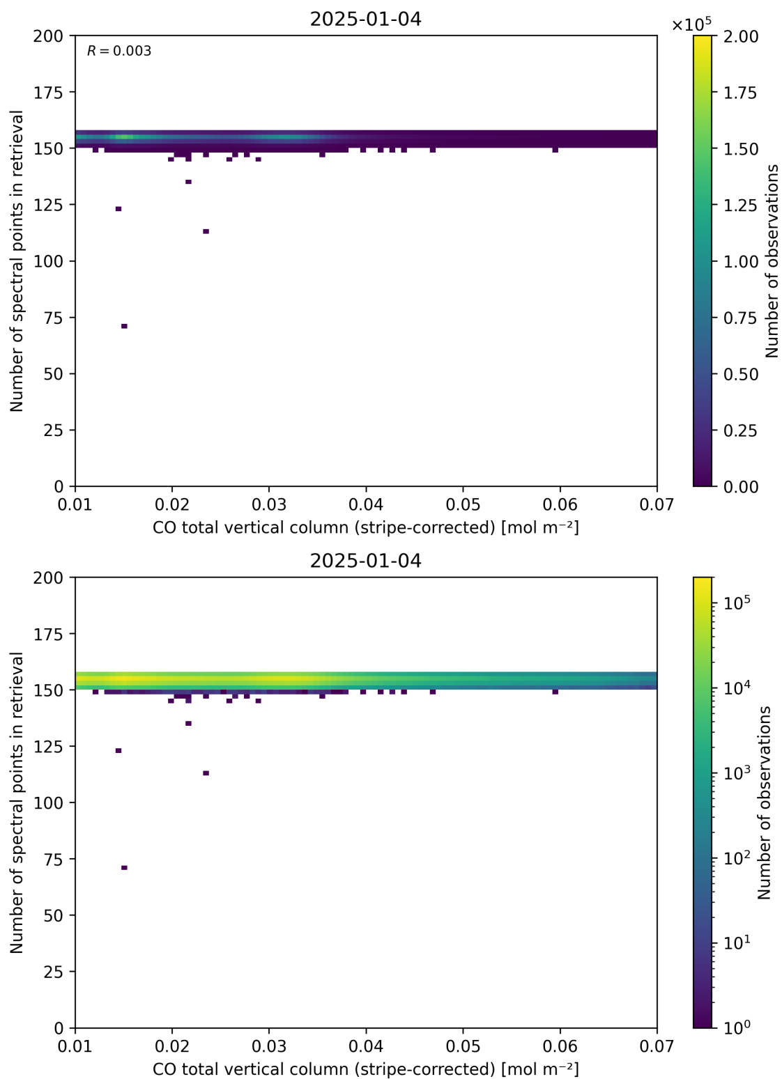
Figure 40: Scatter density plot of “CO total vertical column (stripe-corrected)” against “Number of spectral points in retrieval” for 2025-01-03 to 2025-01-05.
