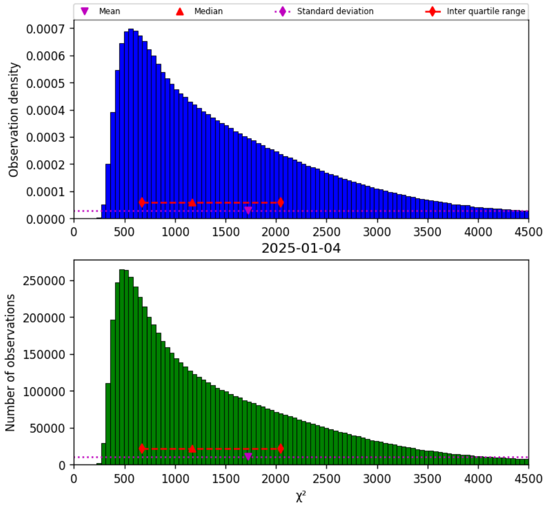
Figure 22: Histogram of “ \chi^2 ” for 2025-01-03 to 2025-01-05
