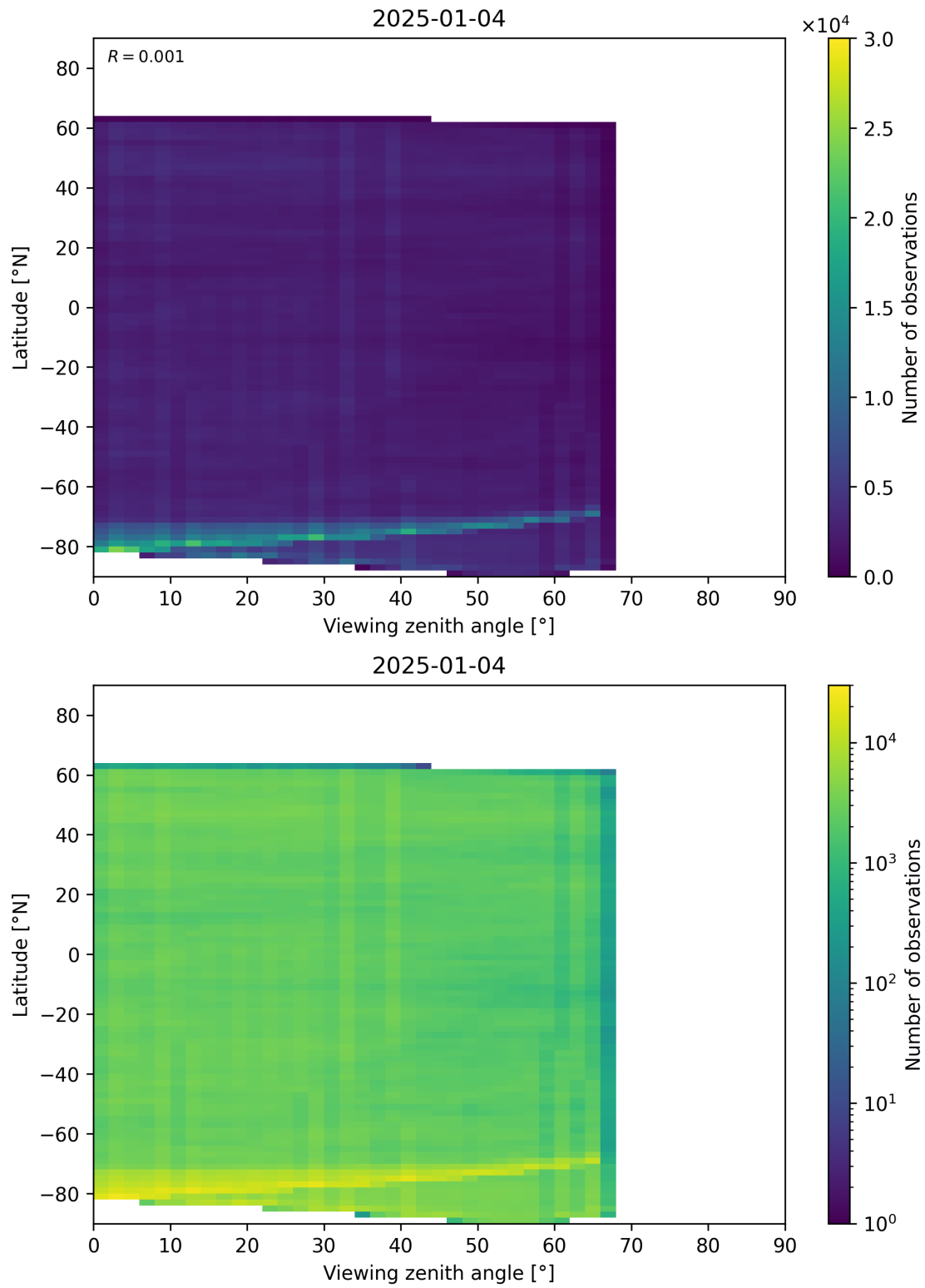
Figure 74: Scatter density plot of “Viewing zenith angle” against “Latitude” for 2025-01-03 to 2025-01-05.
