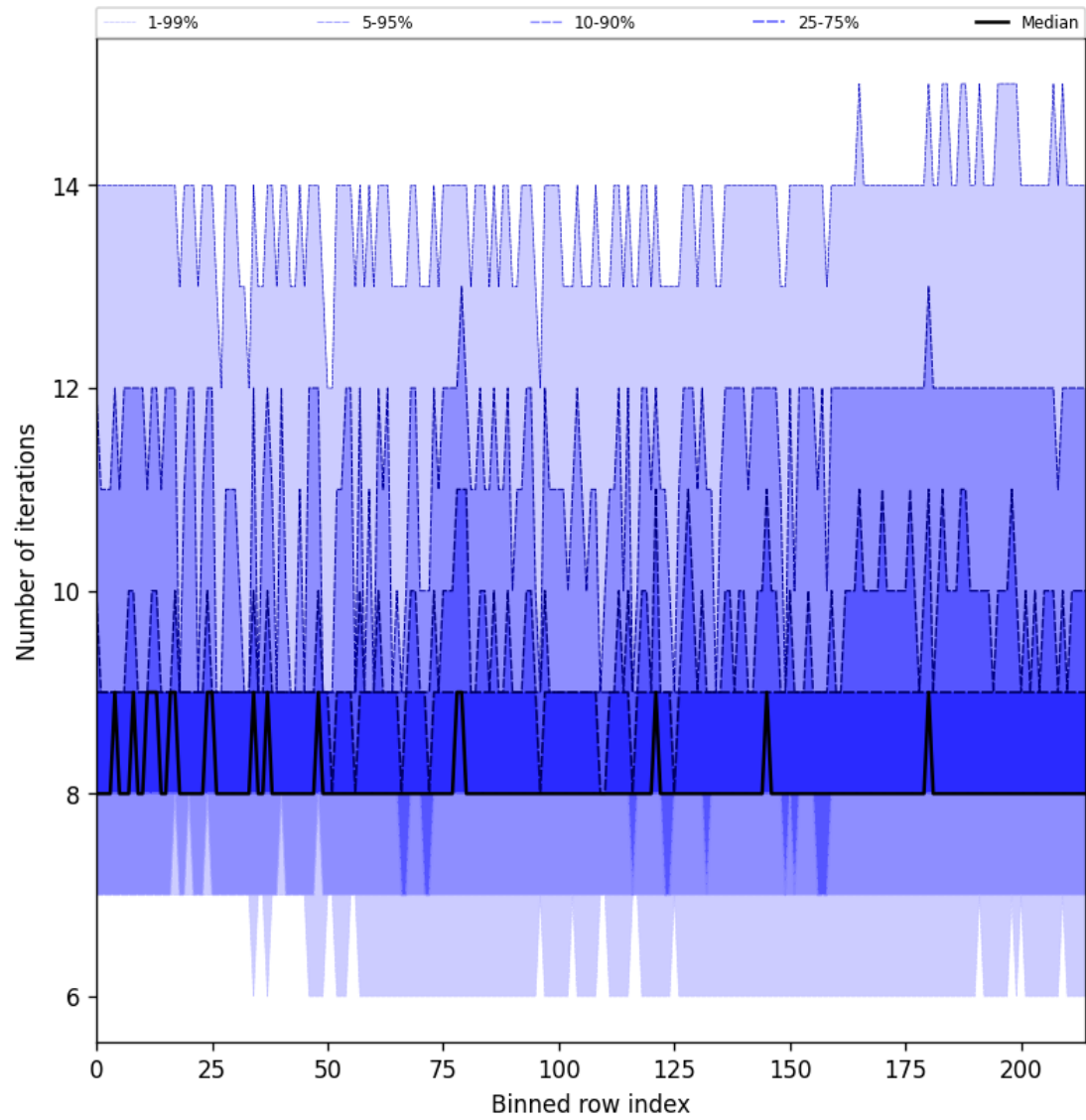
Figure 32: Along track statistics of “Number of iterations” for 2025-01-03 to 2025-01-05
