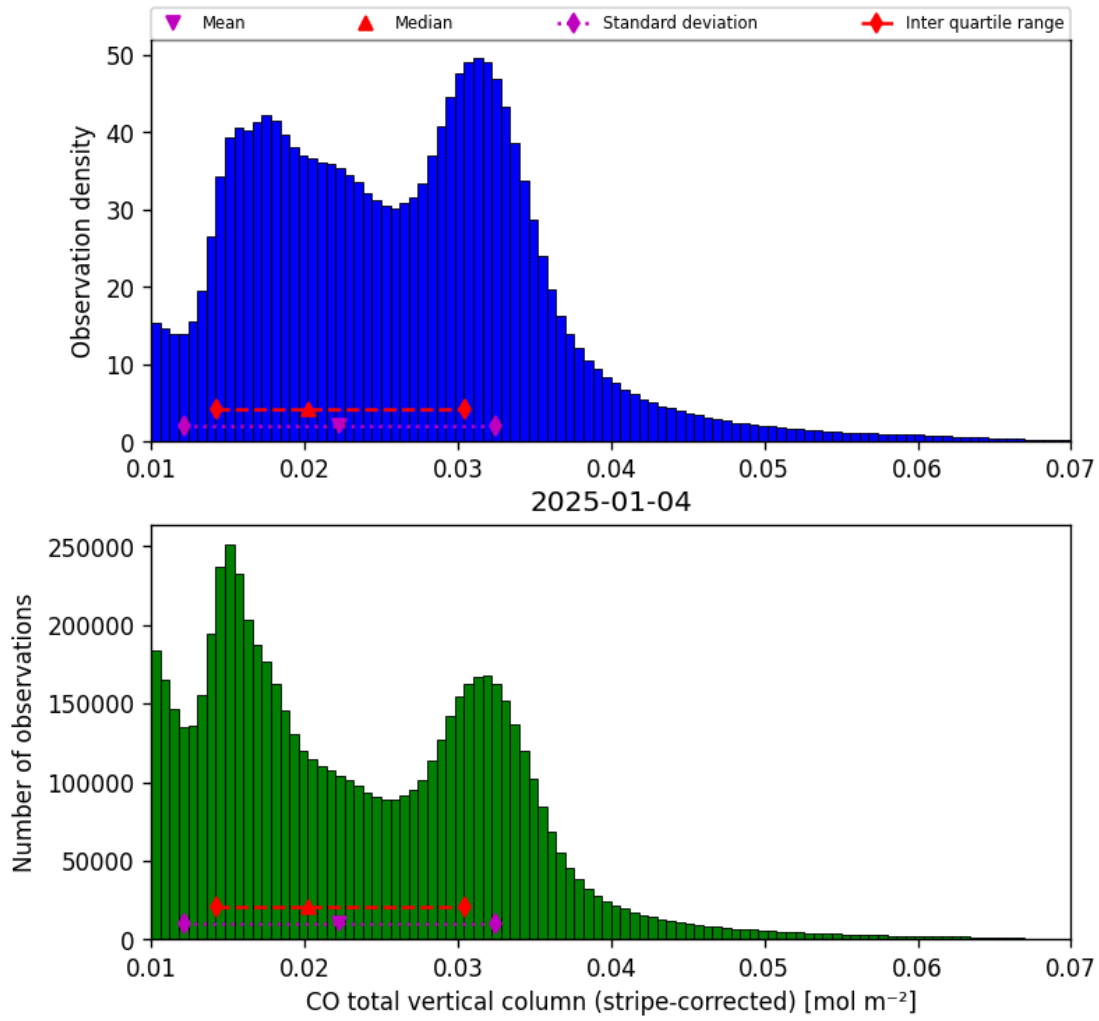
Figure 19: Histogram of “CO total vertical column (stripe-corrected)” for 2025-01-03 to 2025-01-05
