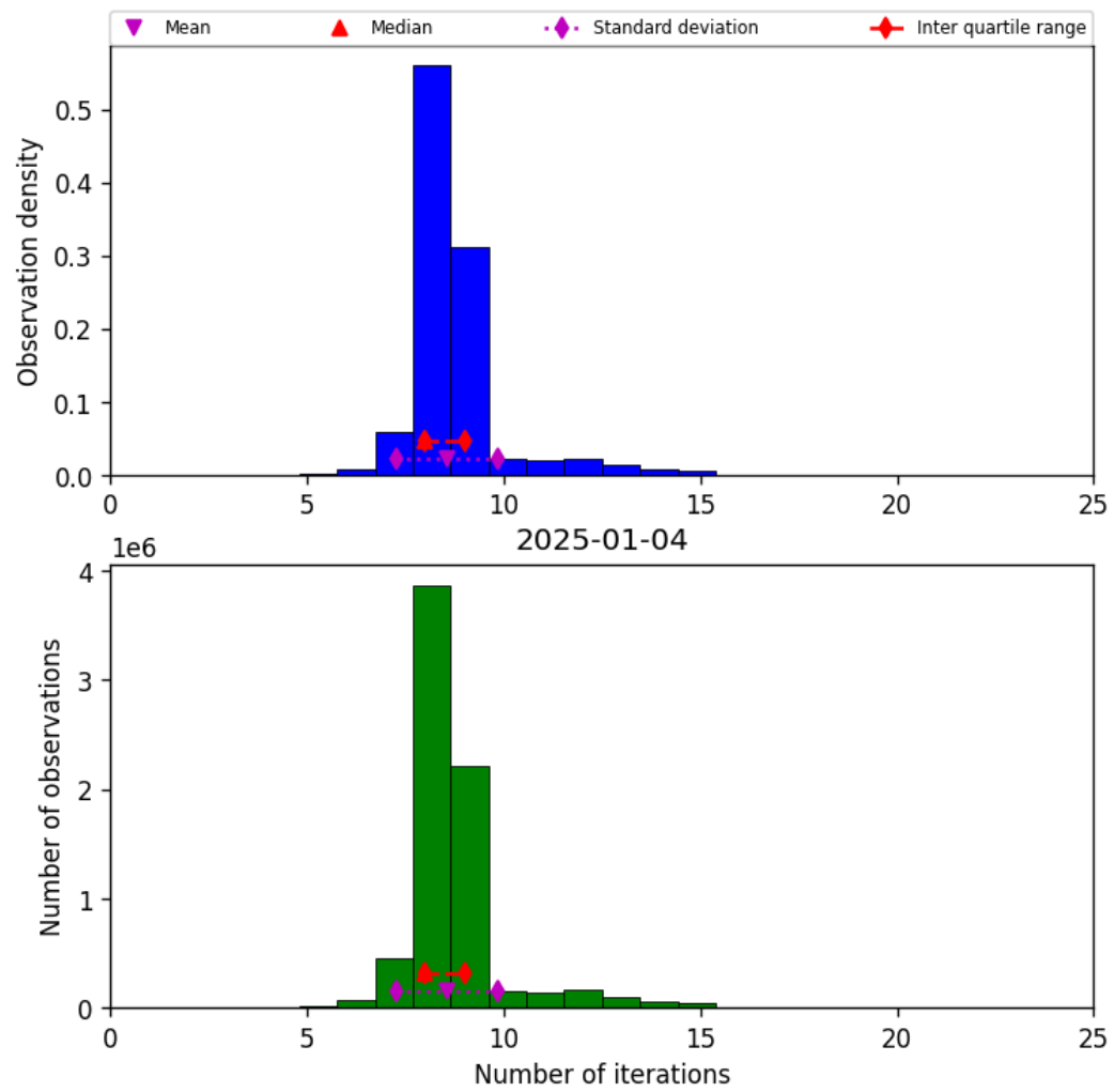
Figure 24: Histogram of “Number of iterations” for 2025-01-03 to 2025-01-05
