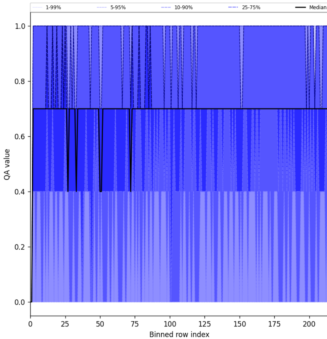
Figure 25: Along track statistics of “QA value” for 2025-01-03 to 2025-01-05
