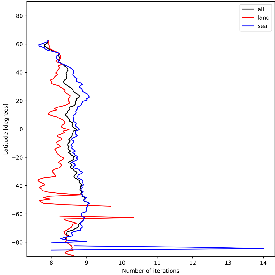
Figure 16: Zonal average of “Number of iterations” for 2025-01-03 to 2025-01-05.
