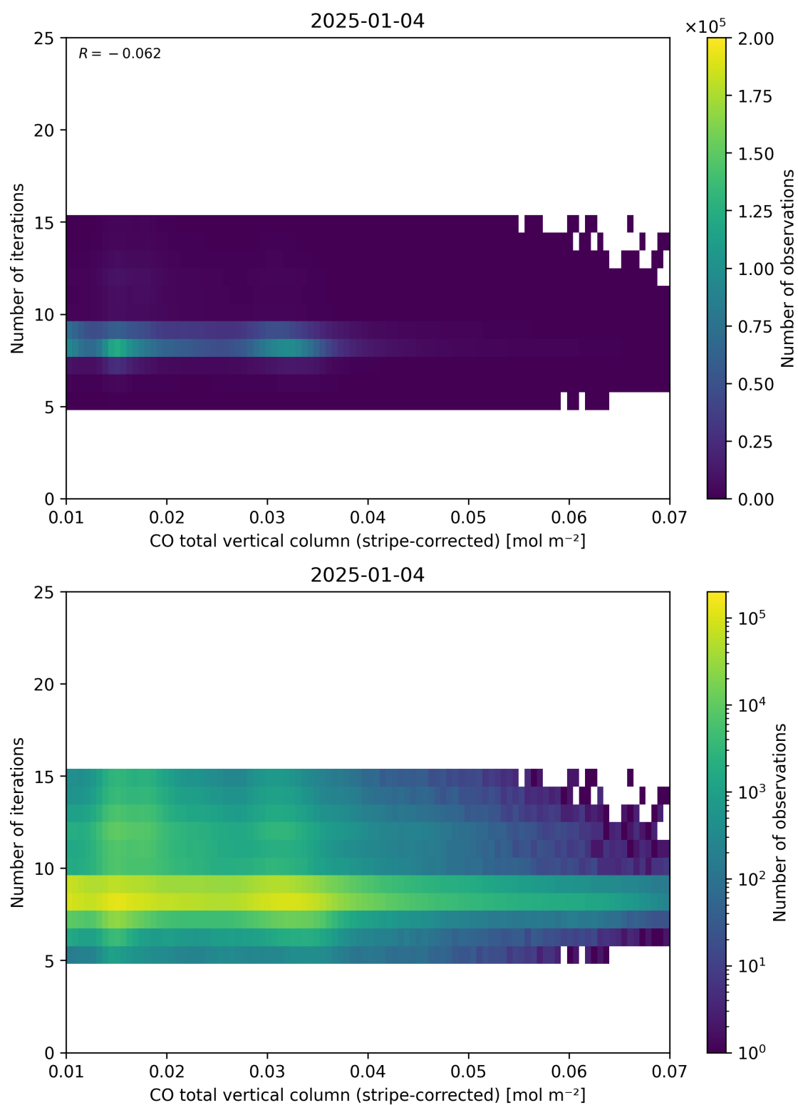
Figure 39: Scatter density plot of “CO total vertical column (stripe-corrected)” against “Number of iterations” for 2025-01-03 to 2025-01-05.
