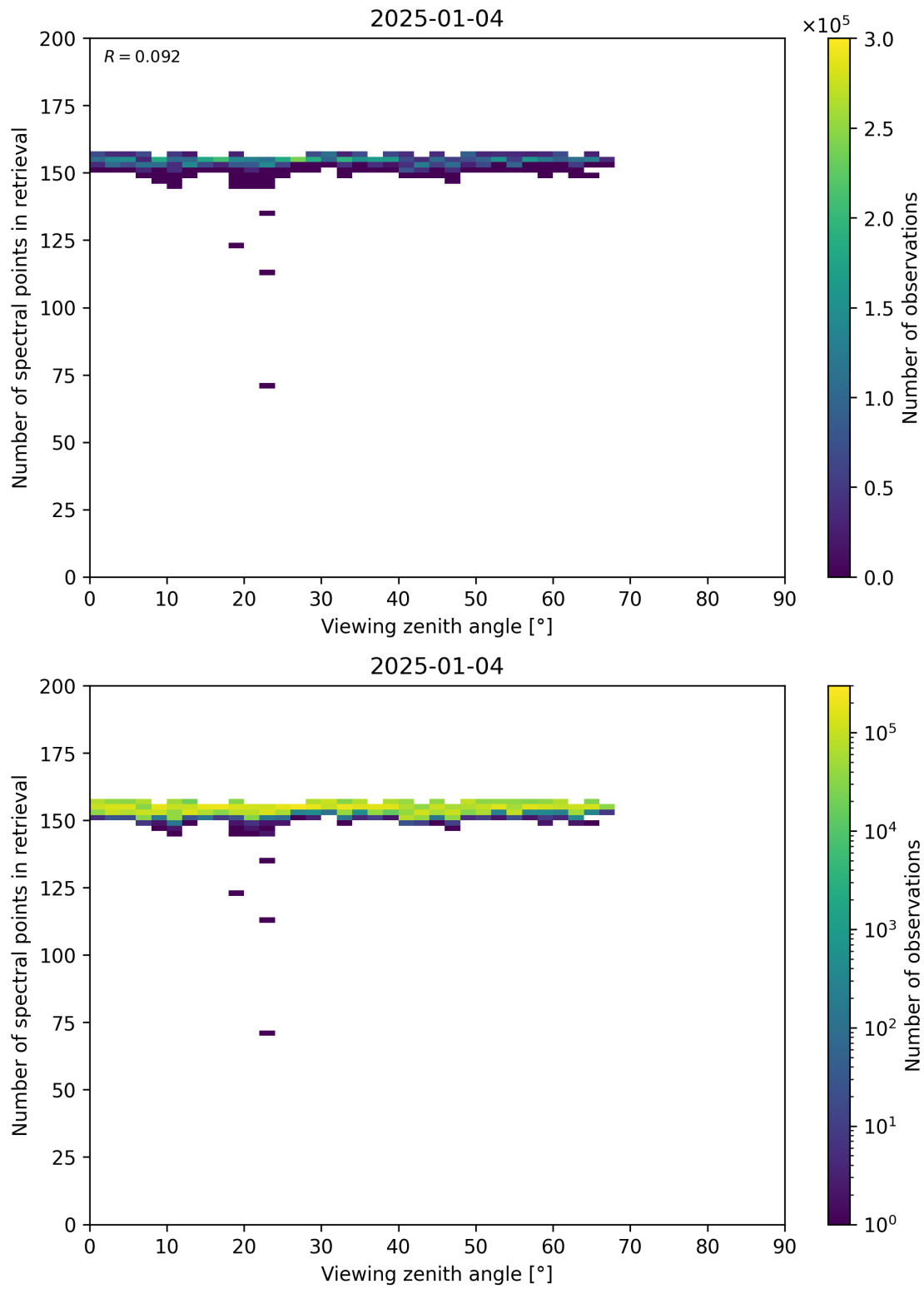
Figure 76: Scatter density plot of “Viewing zenith angle” against “Number of spectral points in retrieval” for 2025-01-03 to 2025-01-05.
