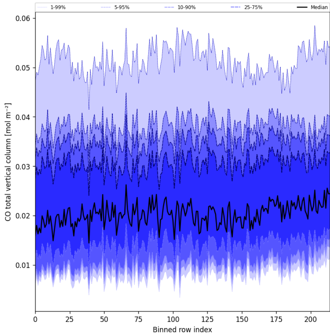
Figure 26: Along track statistics of “CO total vertical column” for 2025-01-03 to 2025-01-05
