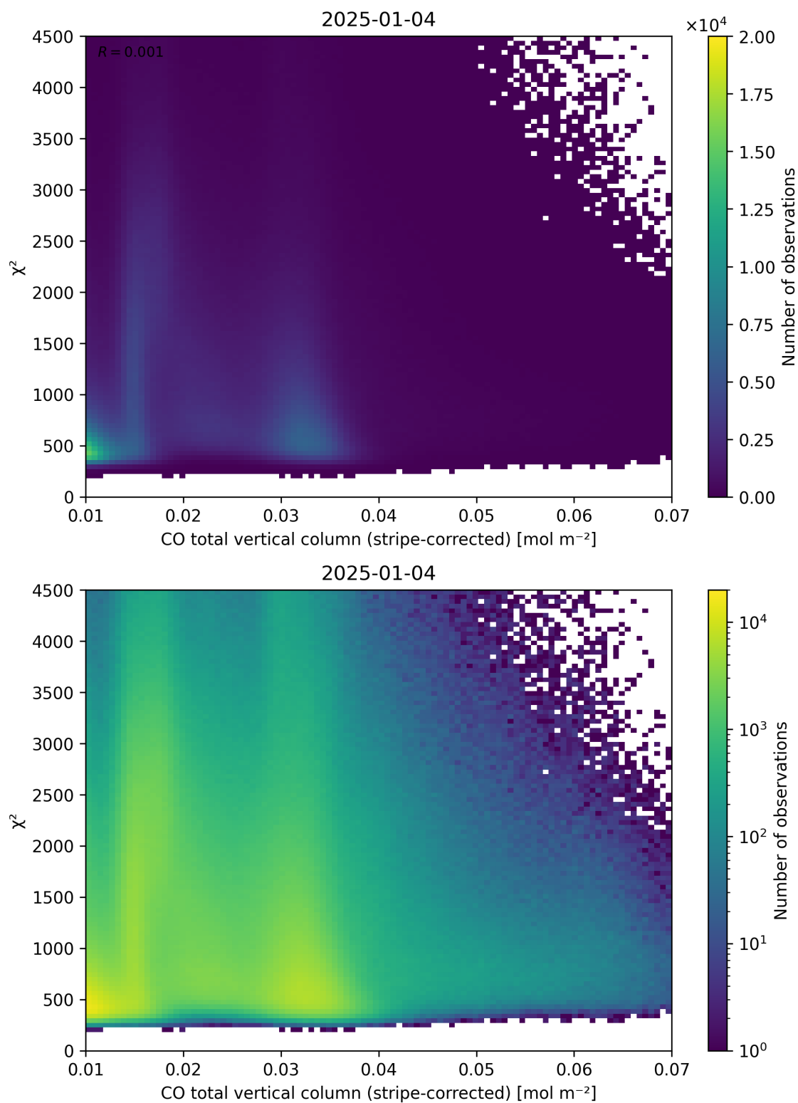
Figure 37: Scatter density plot of “CO total vertical column (stripe-corrected)” against “ \chi^2 ” for 2025-01-03 to 2025-01-05.
