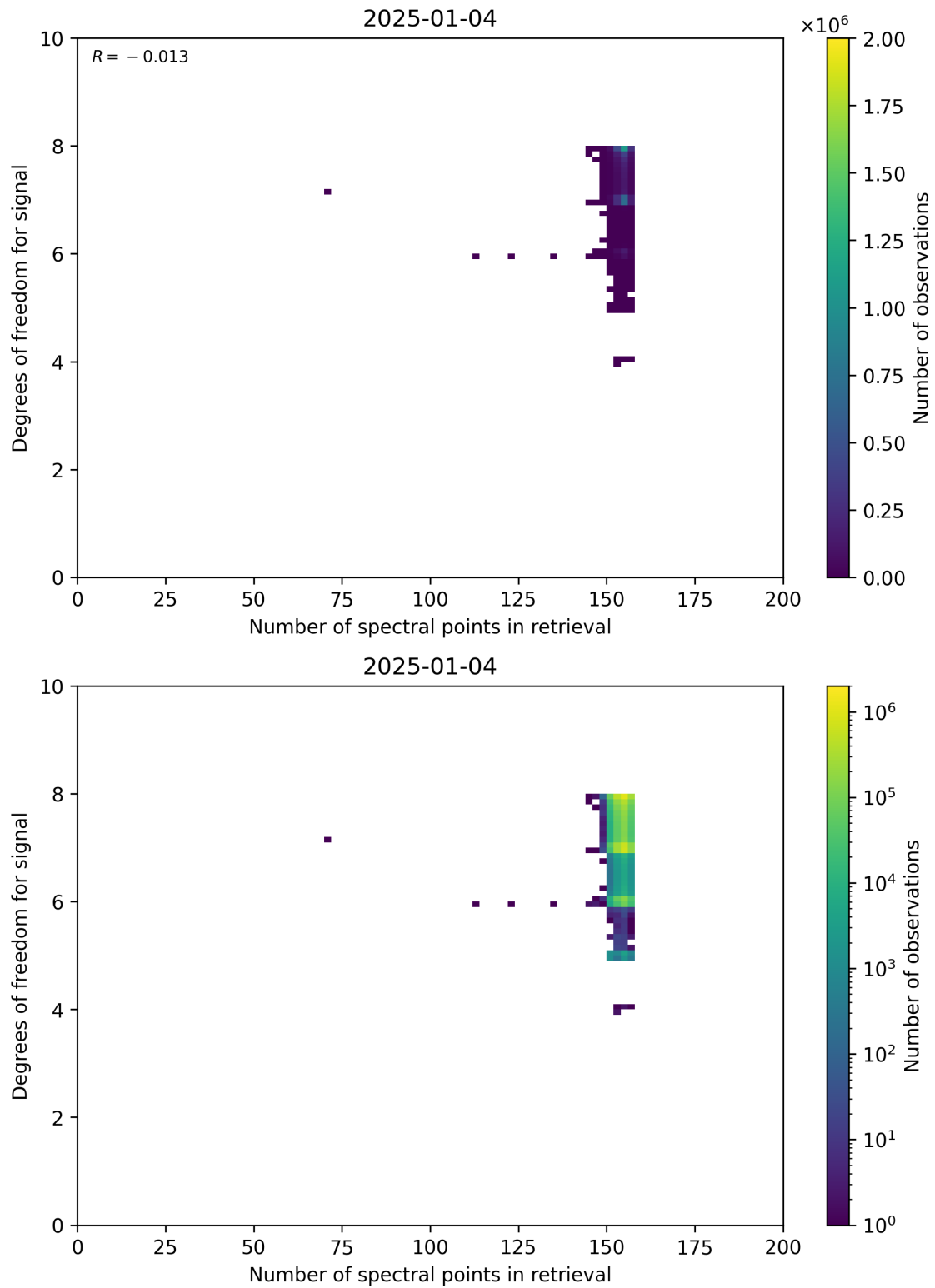
Figure 59: Scatter density plot of “Number of spectral points in retrieval” against “Degrees of freedom for signal” for 2025-01-03 to 2025-01-05.
