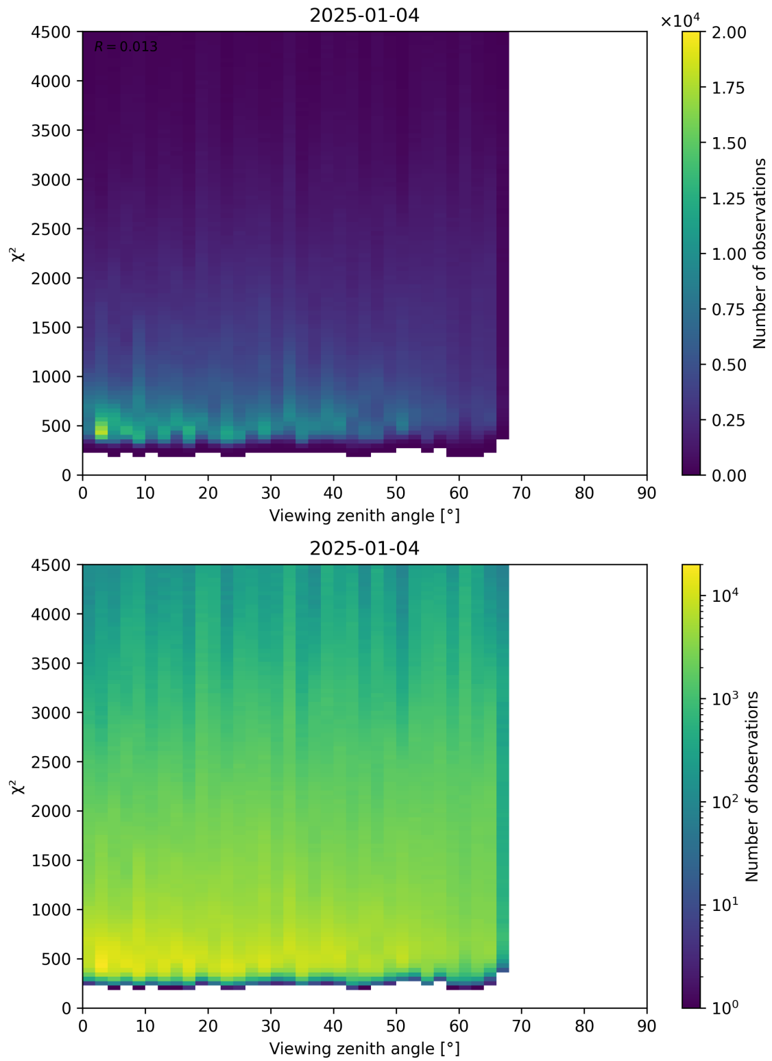
Figure 72: Scatter density plot of “Viewing zenith angle” against “ \chi^2 ” for 2025-01-03 to 2025-01-05.
