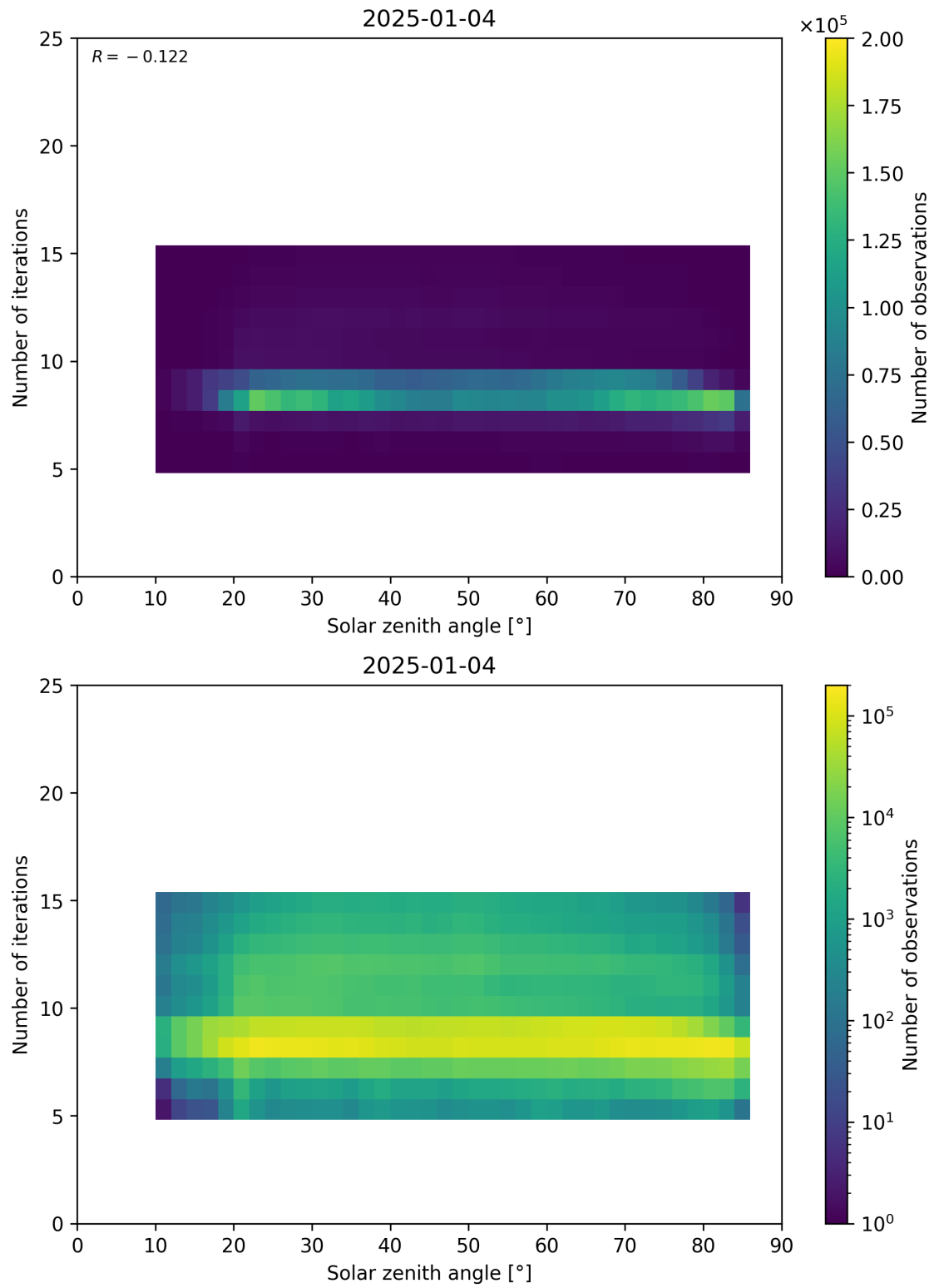
Figure 67: Scatter density plot of “Solar zenith angle” against “Number of iterations” for 2025-01-03 to 2025-01-05.
