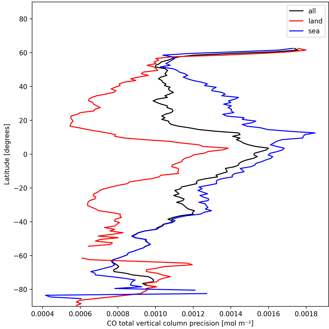
Figure 12: Zonal average of “CO total vertical column precision” for 2025-01-03 to 2025-01-05.
