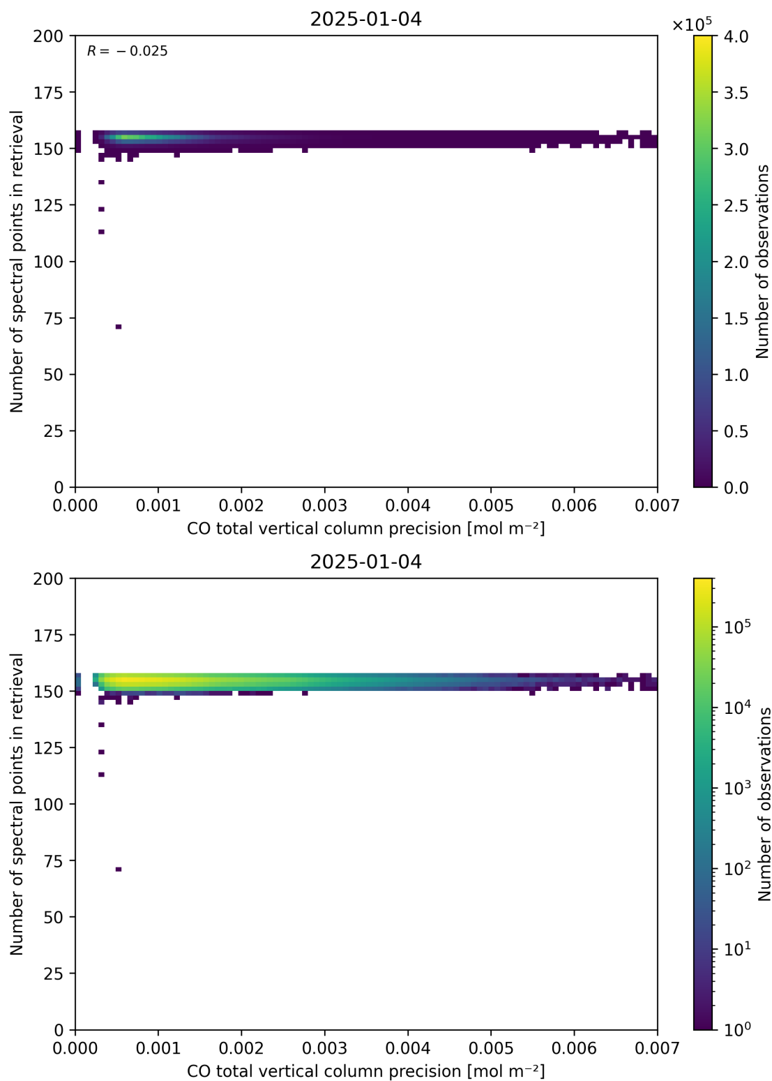
Figure 47: Scatter density plot of “CO total vertical column precision” against “Number of spectral points in retrieval” for 2025-01-03 to 2025-01-05.
