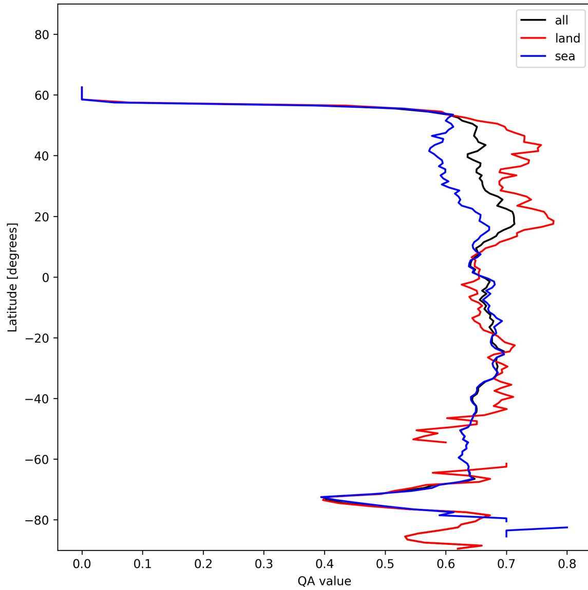
Figure 9: Zonal average of “QA value” for 2025-01-03 to 2025-01-05.
