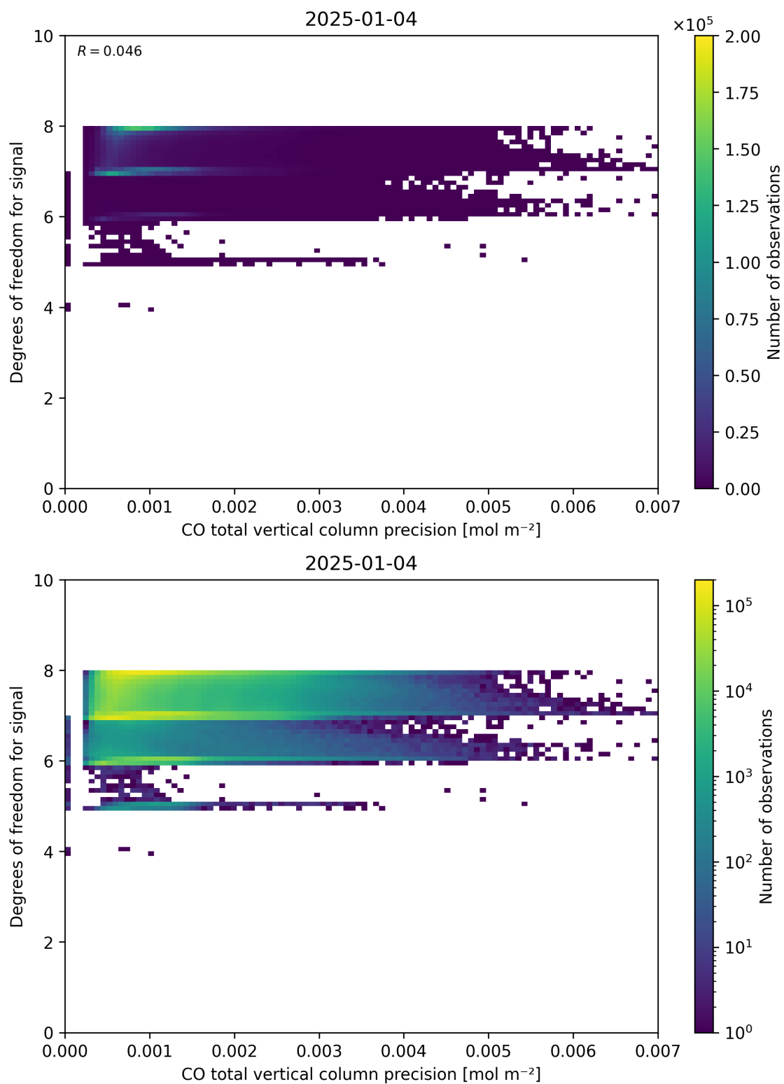
Figure 45: Scatter density plot of “CO total vertical column precision” against “Degrees of freedom for signal” for 2025-01-03 to 2025-01-05.
