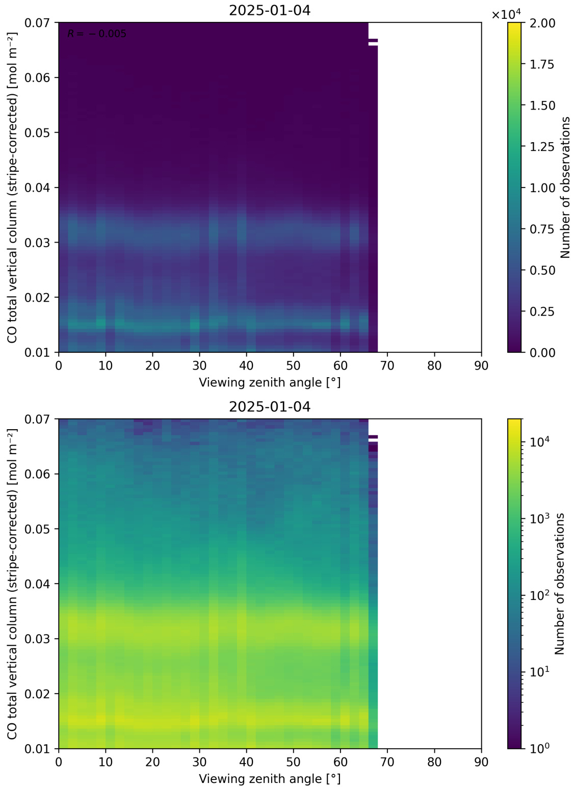
Figure 70: Scatter density plot of “Viewing zenith angle” against “CO total vertical column (stripe-corrected)” for 2025-01-03 to 2025-01-05.
