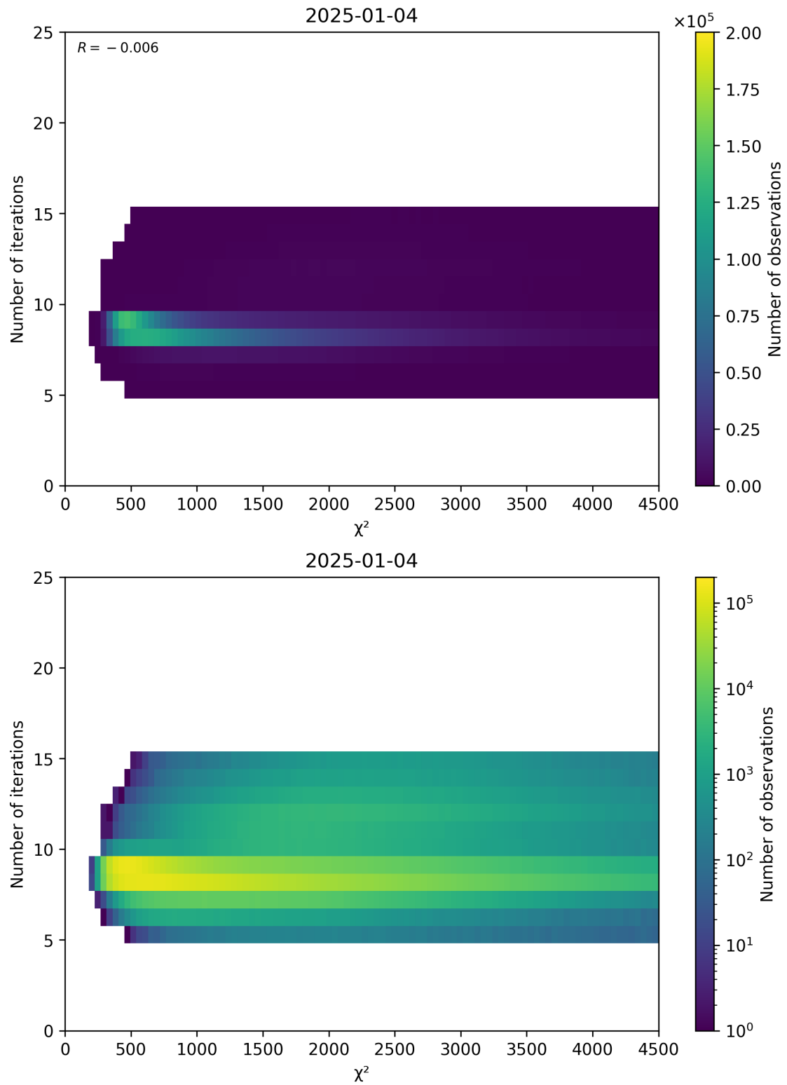
Figure 49: Scatter density plot of “ \chi^2 ” against “Number of iterations” for 2025-01-03 to 2025-01-05.
