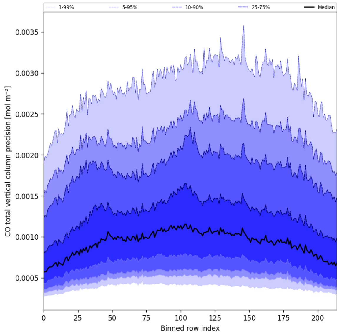
Figure 28: Along track statistics of “CO total vertical column precision” for 2025-01-03 to 2025-01-05
