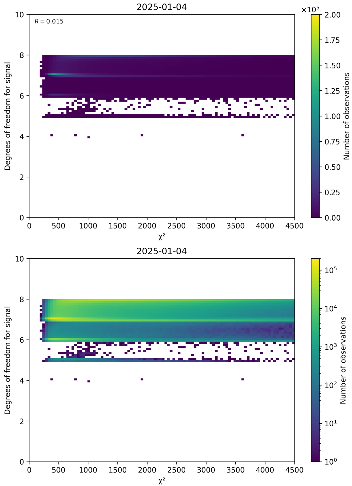
Figure 48: Scatter density plot of “ \chi^2 ” against “Degrees of freedom for signal” for 2025-01-03 to 2025-01-05.
