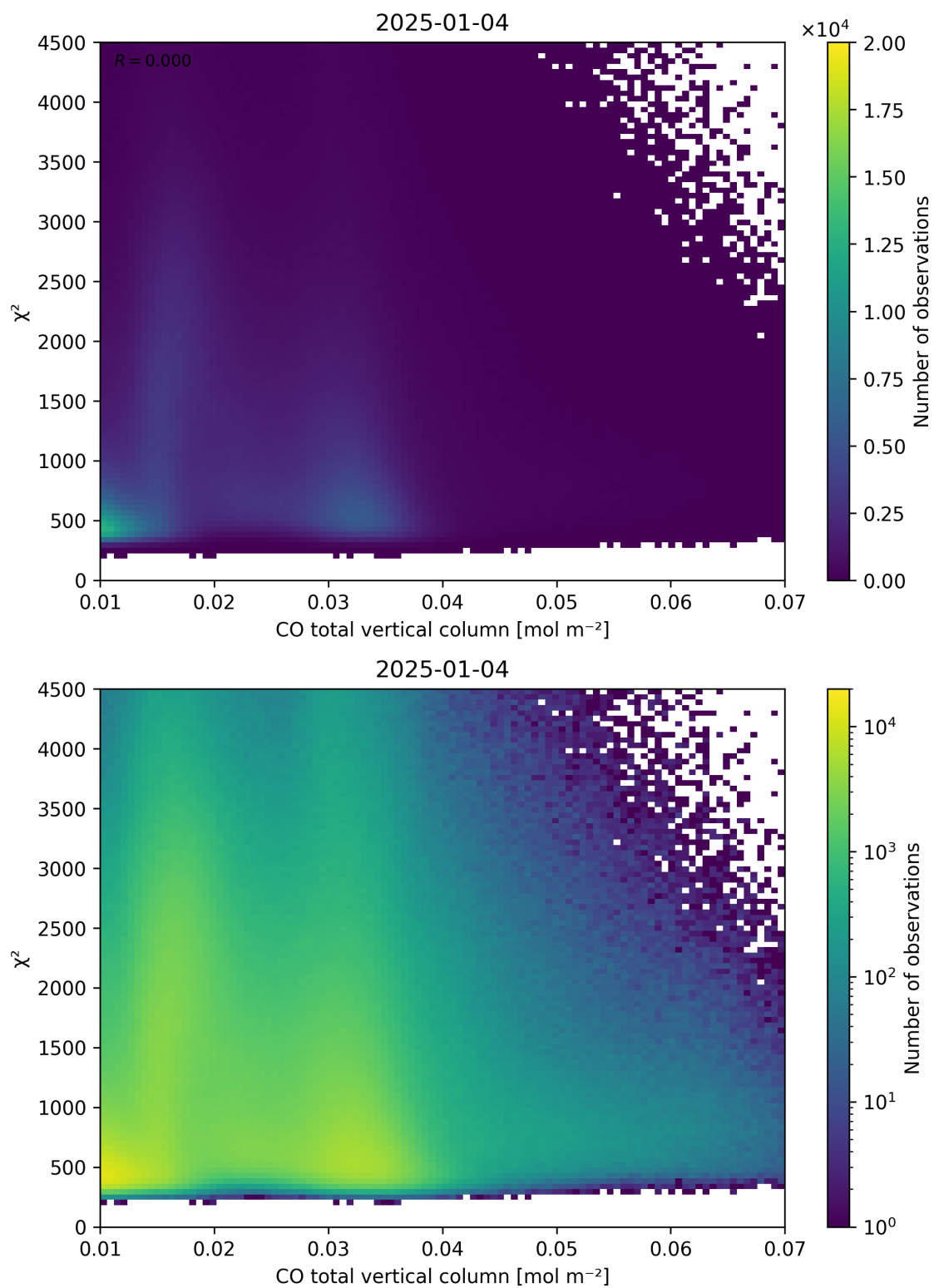
Figure 35: Scatter density plot of “CO total vertical column” against “ \chi^2 ” for 2025-01-03 to 2025-01-05.
