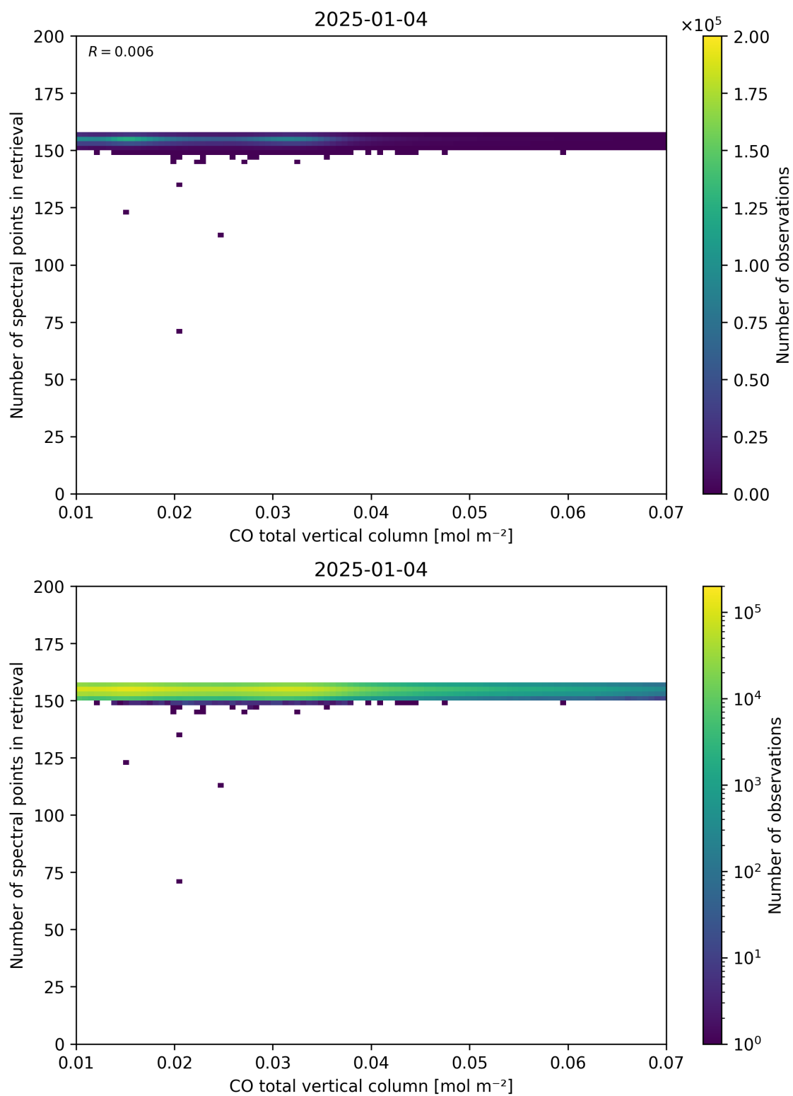
Figure 43: Scatter density plot of “CO total vertical column” against “Number of spectral points in retrieval” for 2025-01-03 to 2025-01-05.
