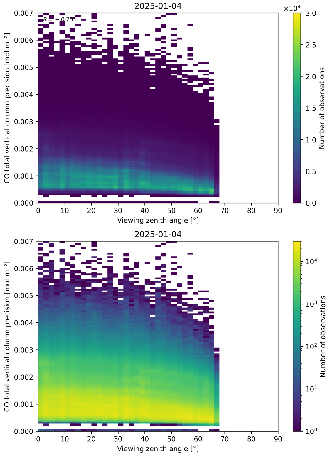
Figure 71: Scatter density plot of “Viewing zenith angle” against “CO total vertical column precision” for 2025-01-03 to 2025-01-05.
