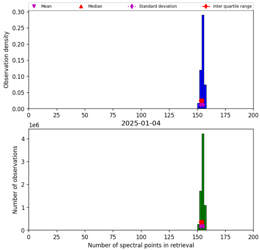
Figure 21: Histogram of “Number of spectral points in retrieval” for 2025-01-03 to 2025-01-05
