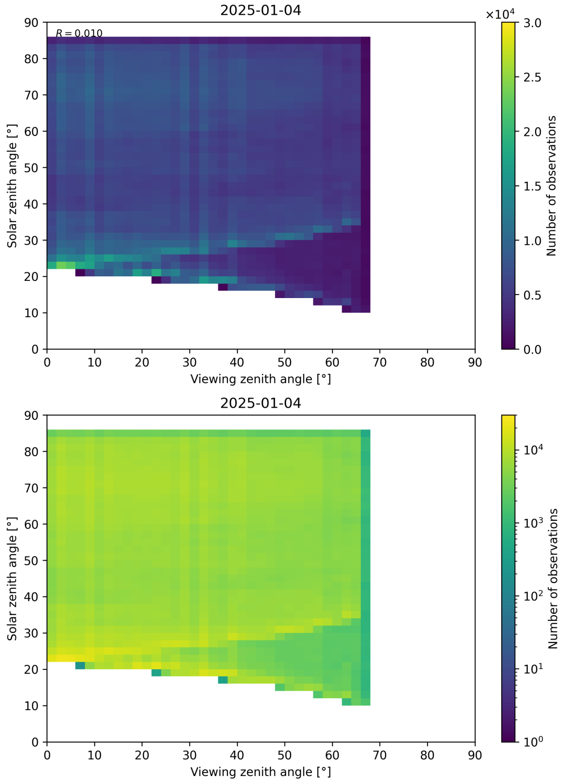
Figure 77: Scatter density plot of “Viewing zenith angle” against “Solar zenith angle” for 2025-01-03 to 2025-01-05.
