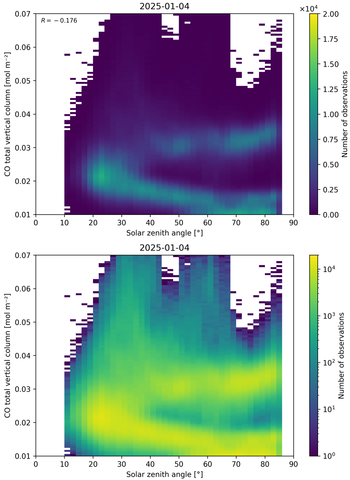
Figure 61: Scatter density plot of “Solar zenith angle” against “CO total vertical column” for 2025-01-03 to 2025-01-05.
