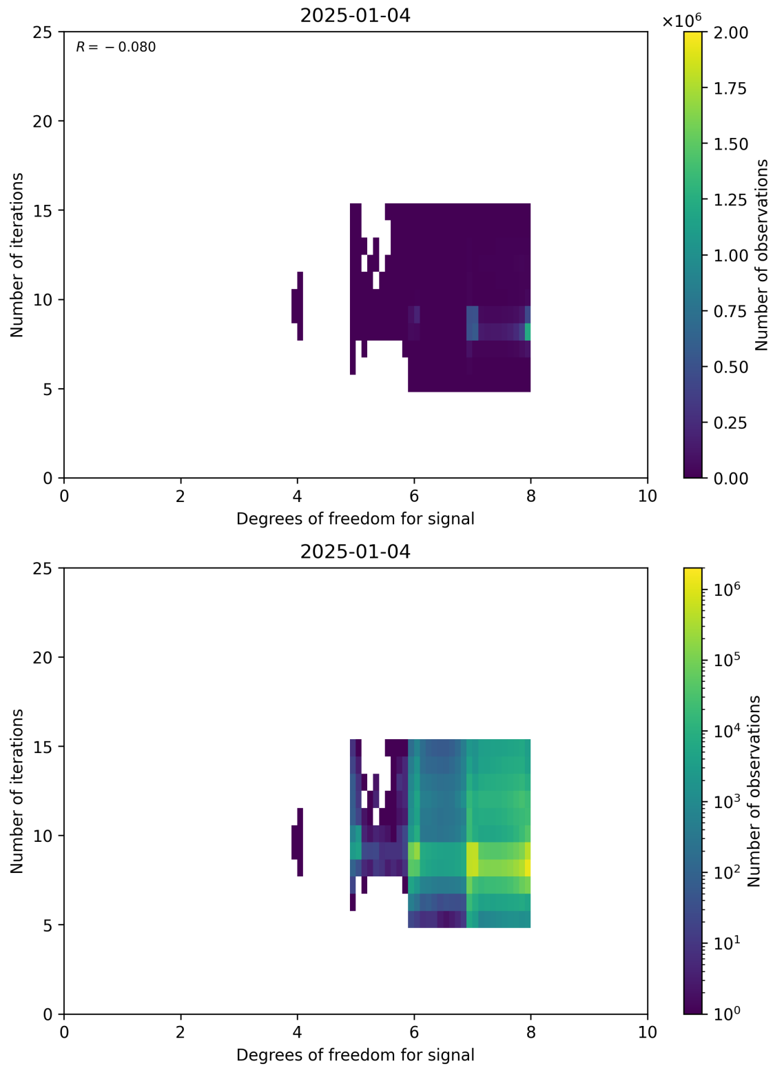
Figure 50: Scatter density plot of “Degrees of freedom for signal” against “Number of iterations” for 2025-01-03 to 2025-01-05.
