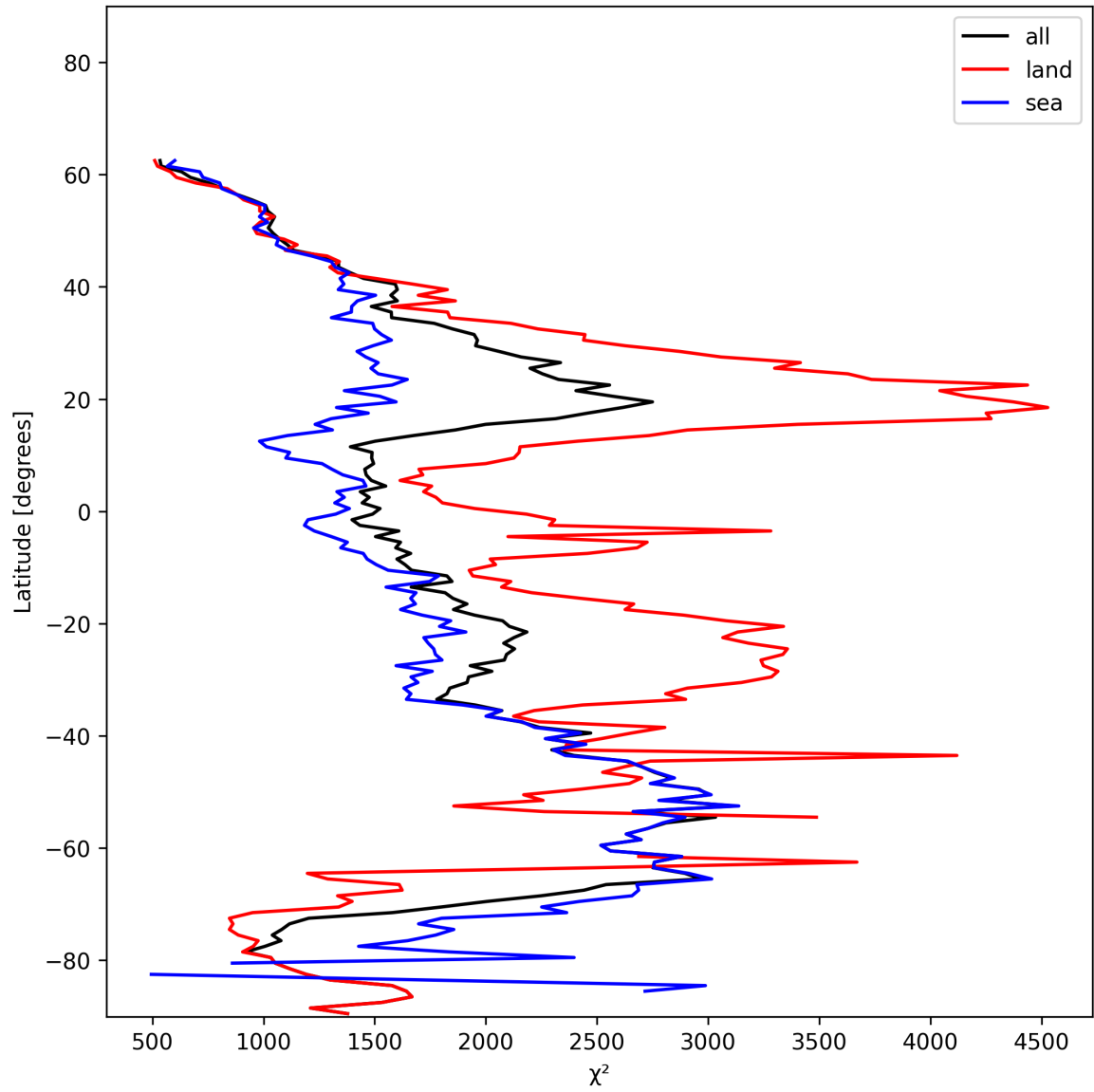
Figure 14: Zonal average of “ \chi^2 ” for 2025-01-03 to 2025-01-05.
