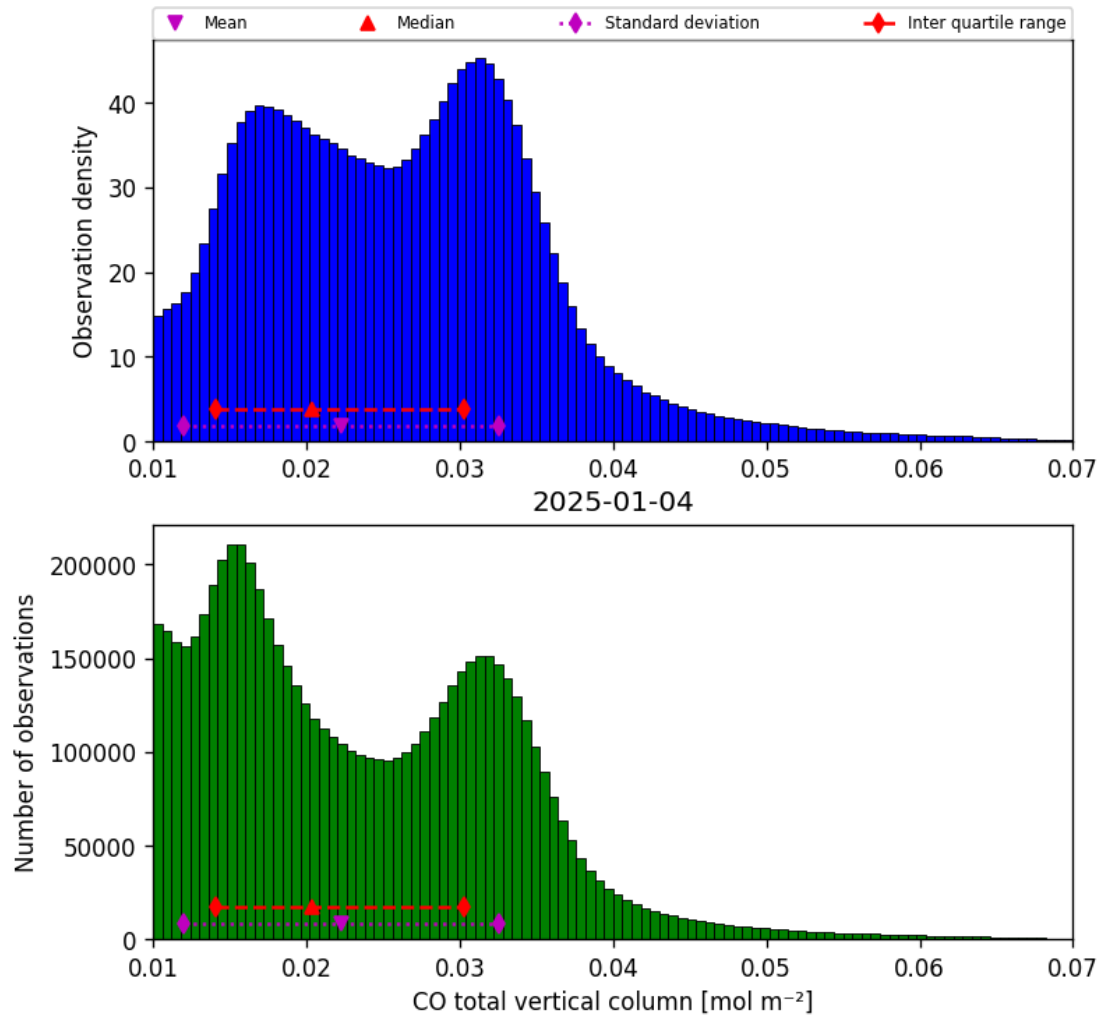
Figure 18: Histogram of “CO total vertical column” for 2025-01-03 to 2025-01-05
