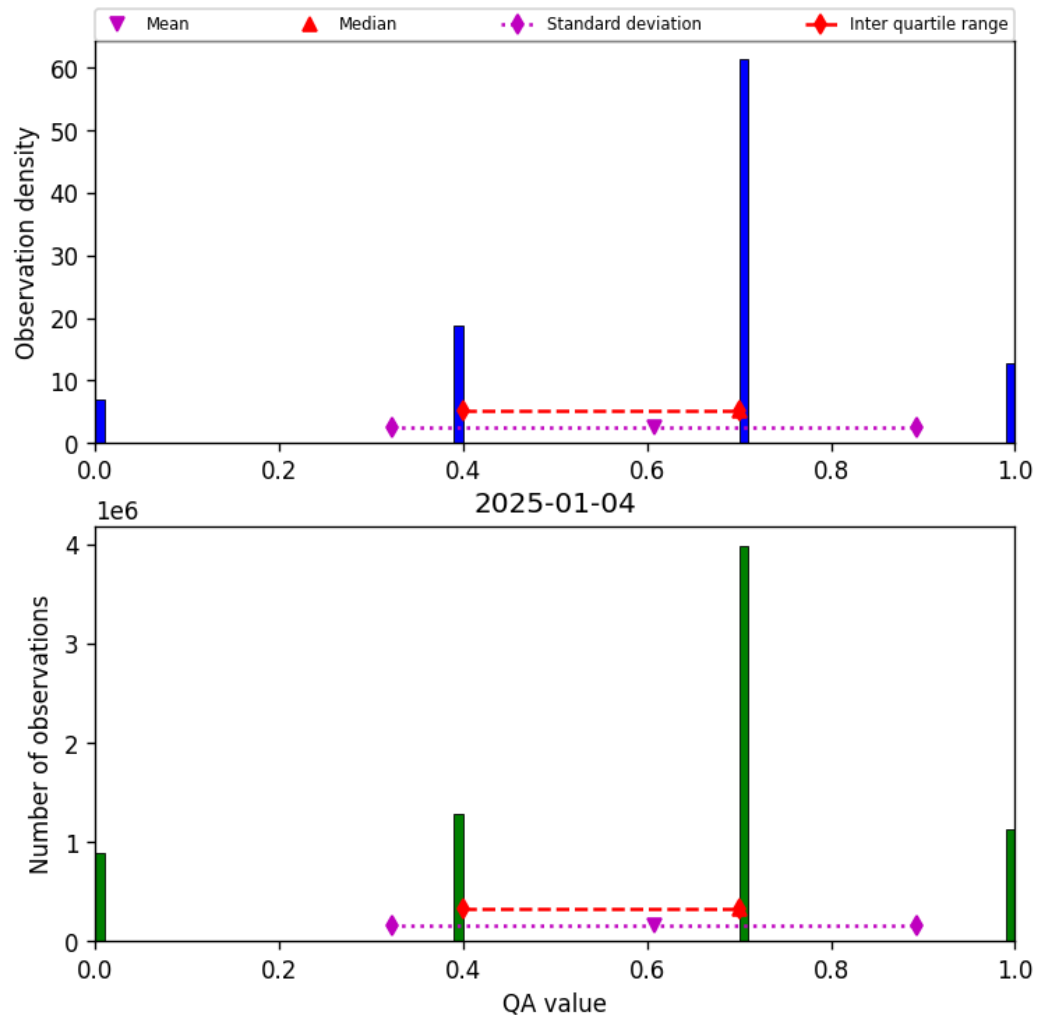
Figure 17: Histogram of “QA value” for 2025-01-03 to 2025-01-05
