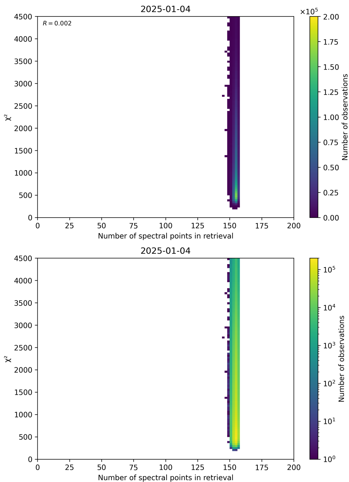
Figure 58: Scatter density plot of “Number of spectral points in retrieval” against “ \chi^2 ” for 2025-01-03 to 2025-01-05.
