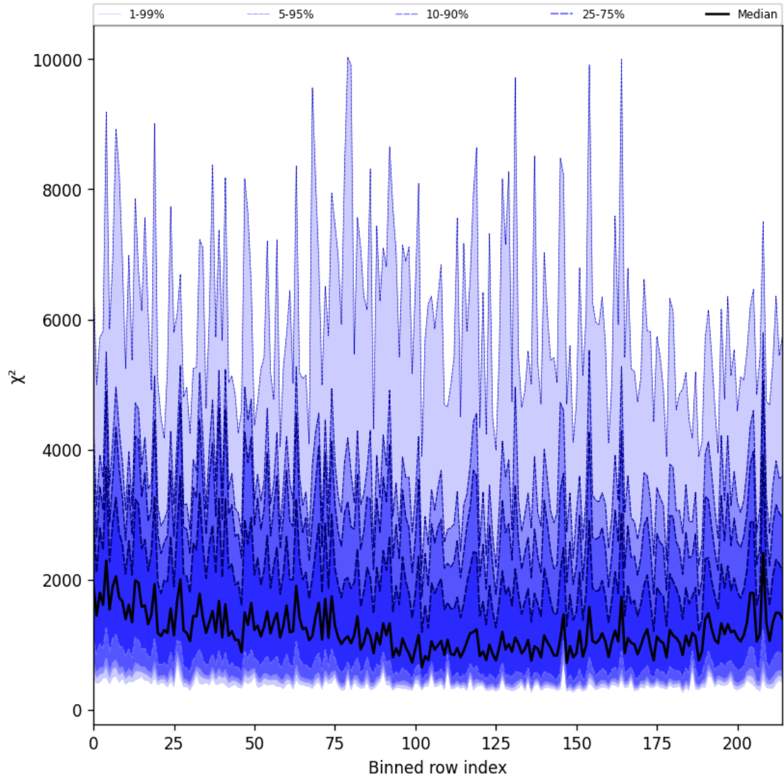
Figure 30: Along track statistics of “ \chi^2 ” for 2025-01-03 to 2025-01-05
