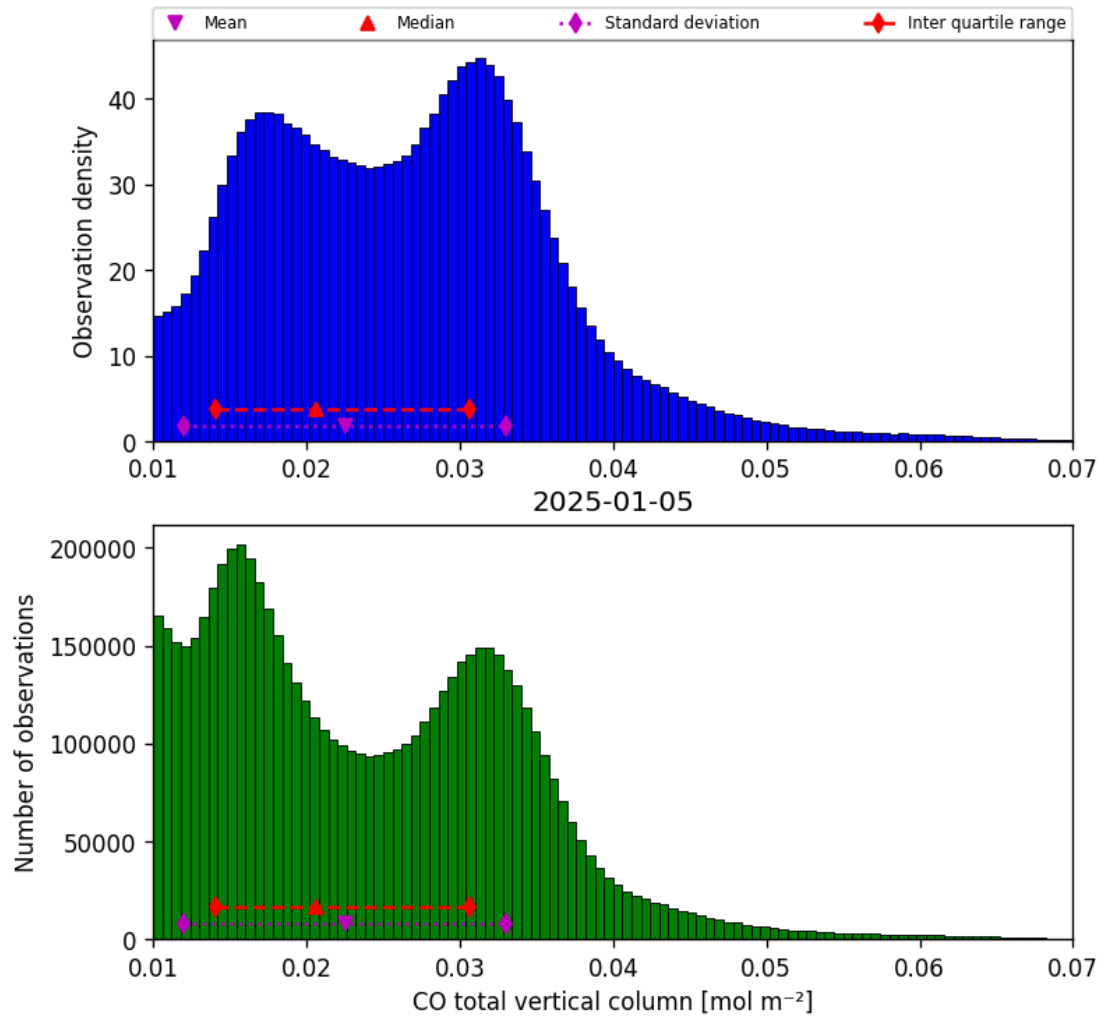
Figure 18: Histogram of “CO total vertical column” for 2025-01-04 to 2025-01-06
