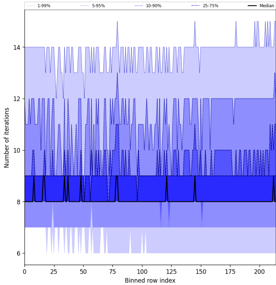
Figure 32: Along track statistics of “Number of iterations” for 2025-01-04 to 2025-01-06
