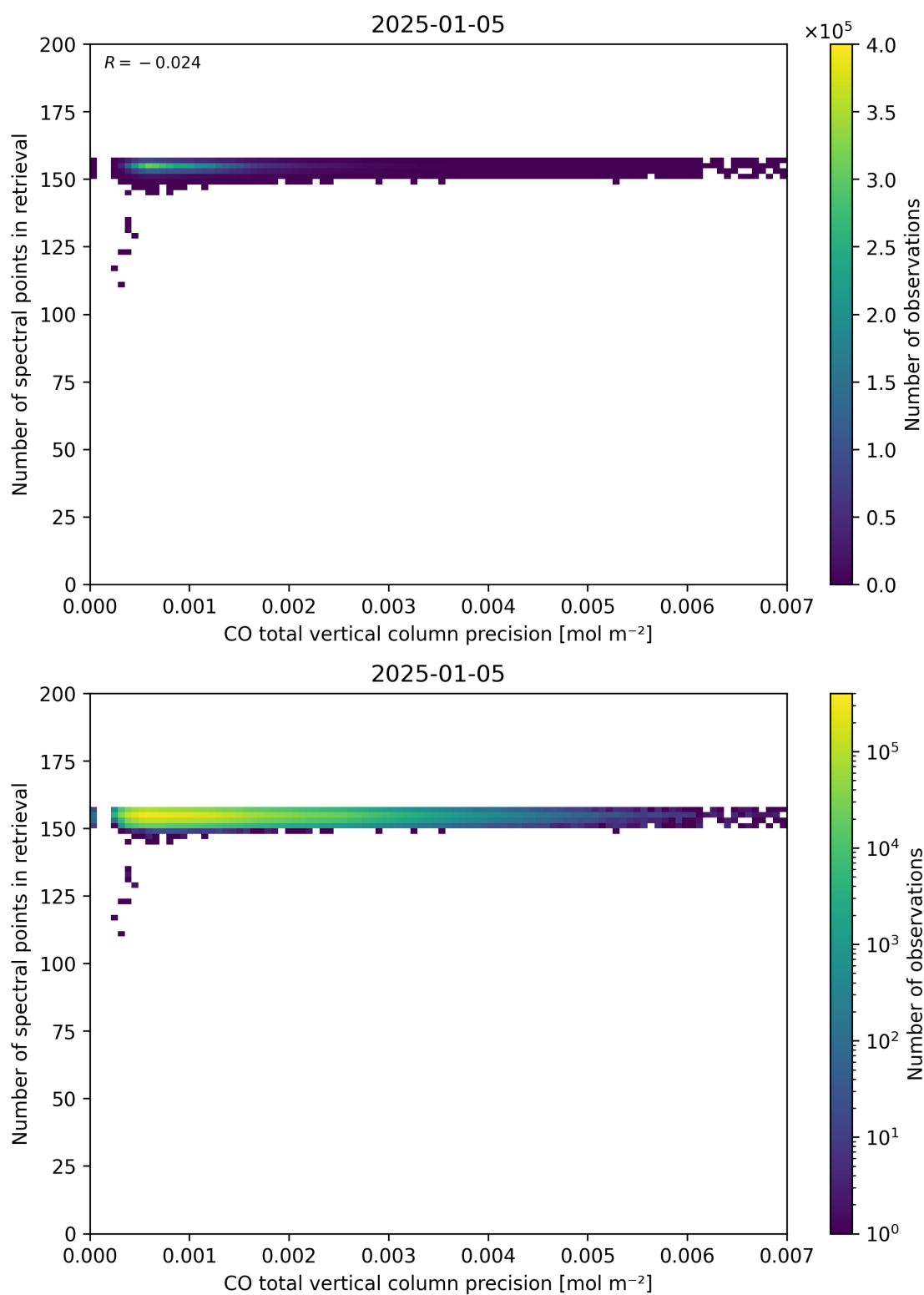
Figure 47: Scatter density plot of “CO total vertical column precision” against “Number of spectral points in retrieval” for 2025-01-04 to 2025-01-06.
