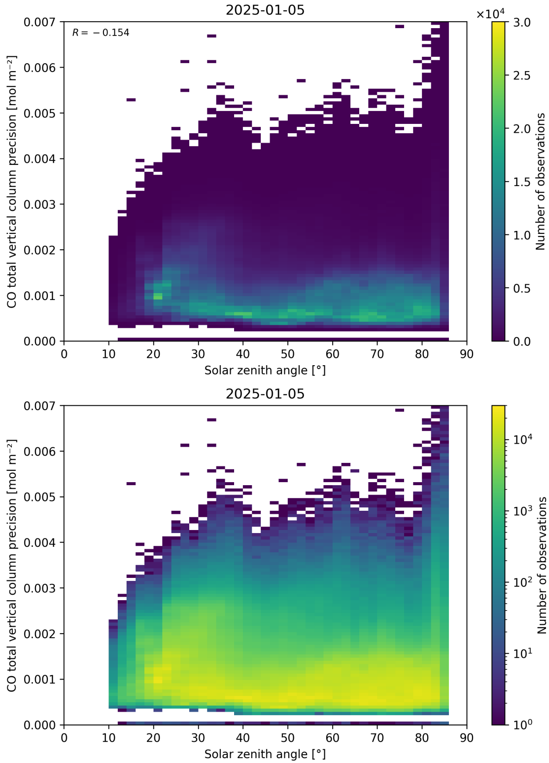
Figure 63: Scatter density plot of “Solar zenith angle” against “CO total vertical column precision” for 2025-01-04 to 2025-01-06.
