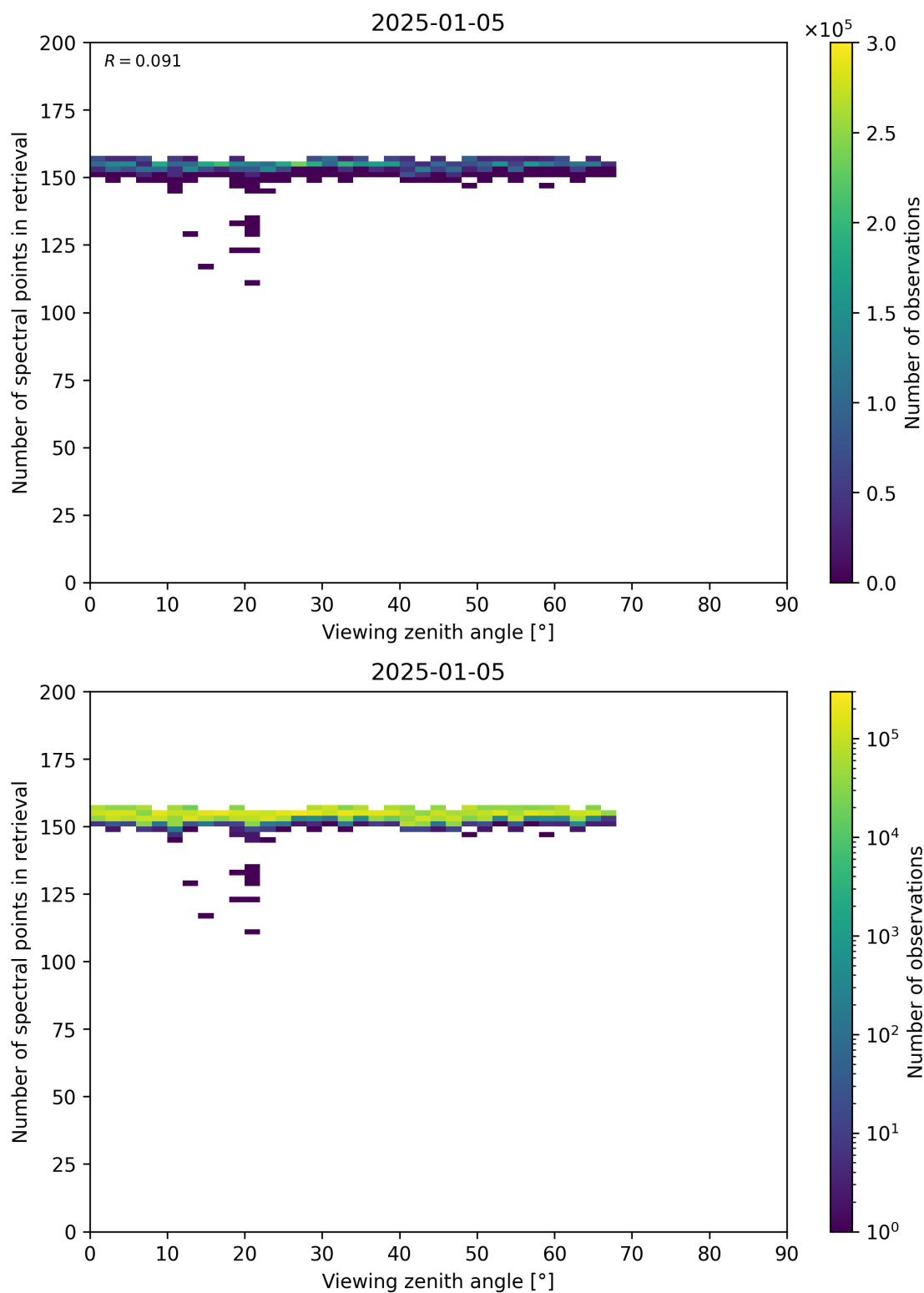
Figure 76: Scatter density plot of “Viewing zenith angle” against “Number of spectral points in retrieval” for 2025-01-04 to 2025-01-06.
