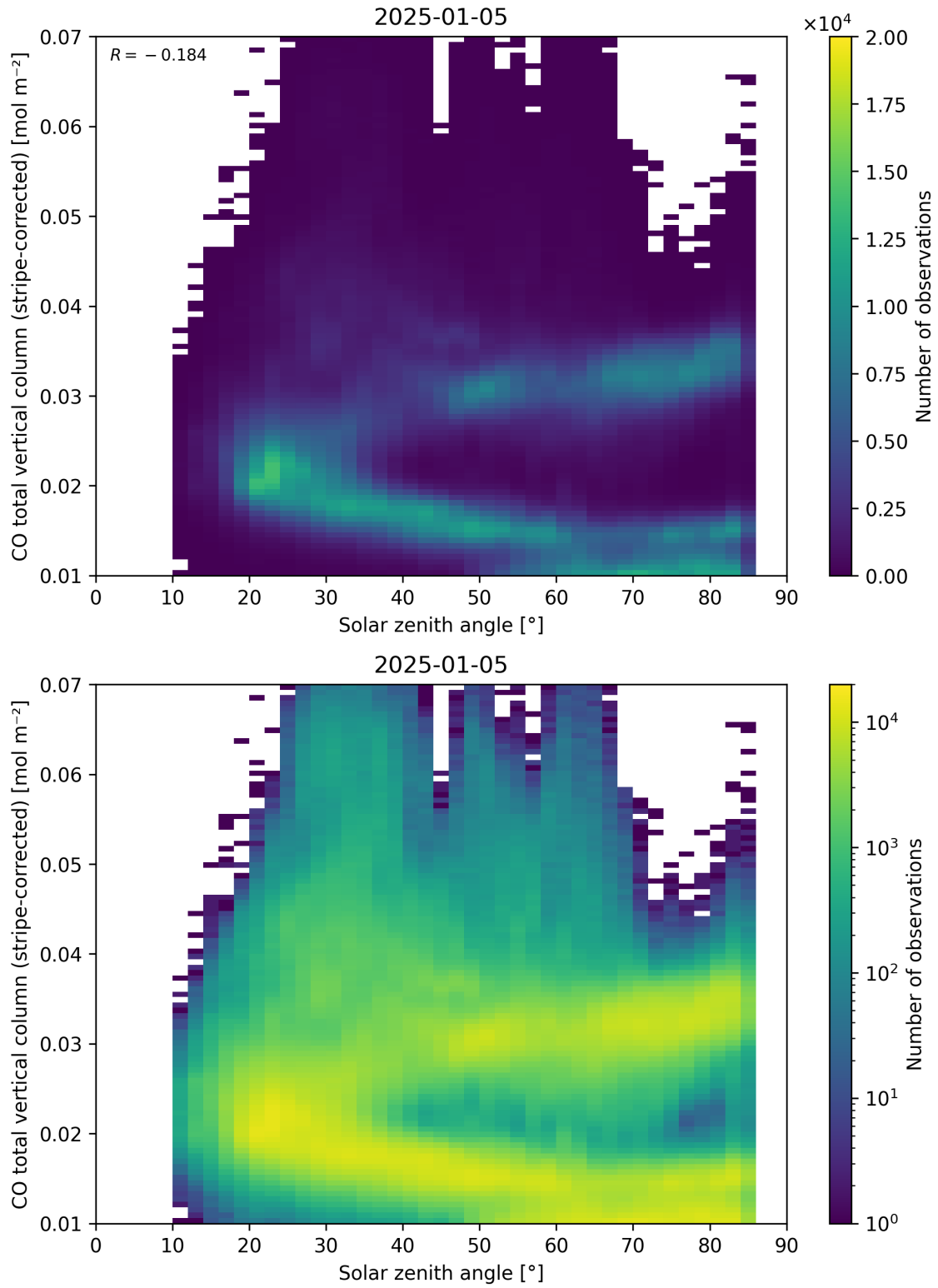
Figure 62: Scatter density plot of “Solar zenith angle” against “CO total vertical column (stripe-corrected)” for 2025-01-04 to 2025-01-06.
