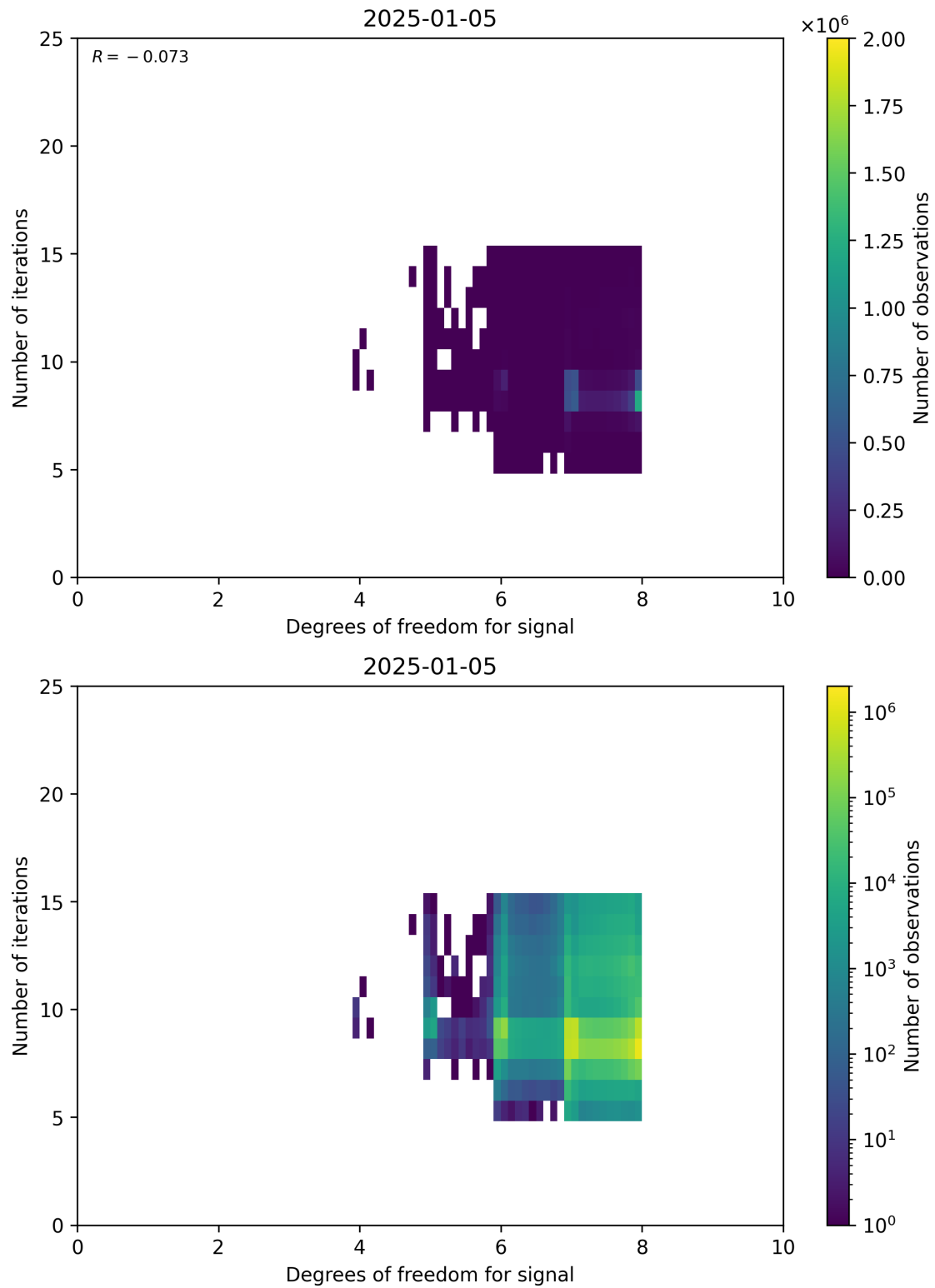
Figure 50: Scatter density plot of “Degrees of freedom for signal” against “Number of iterations” for 2025-01-04 to 2025-01-06.
