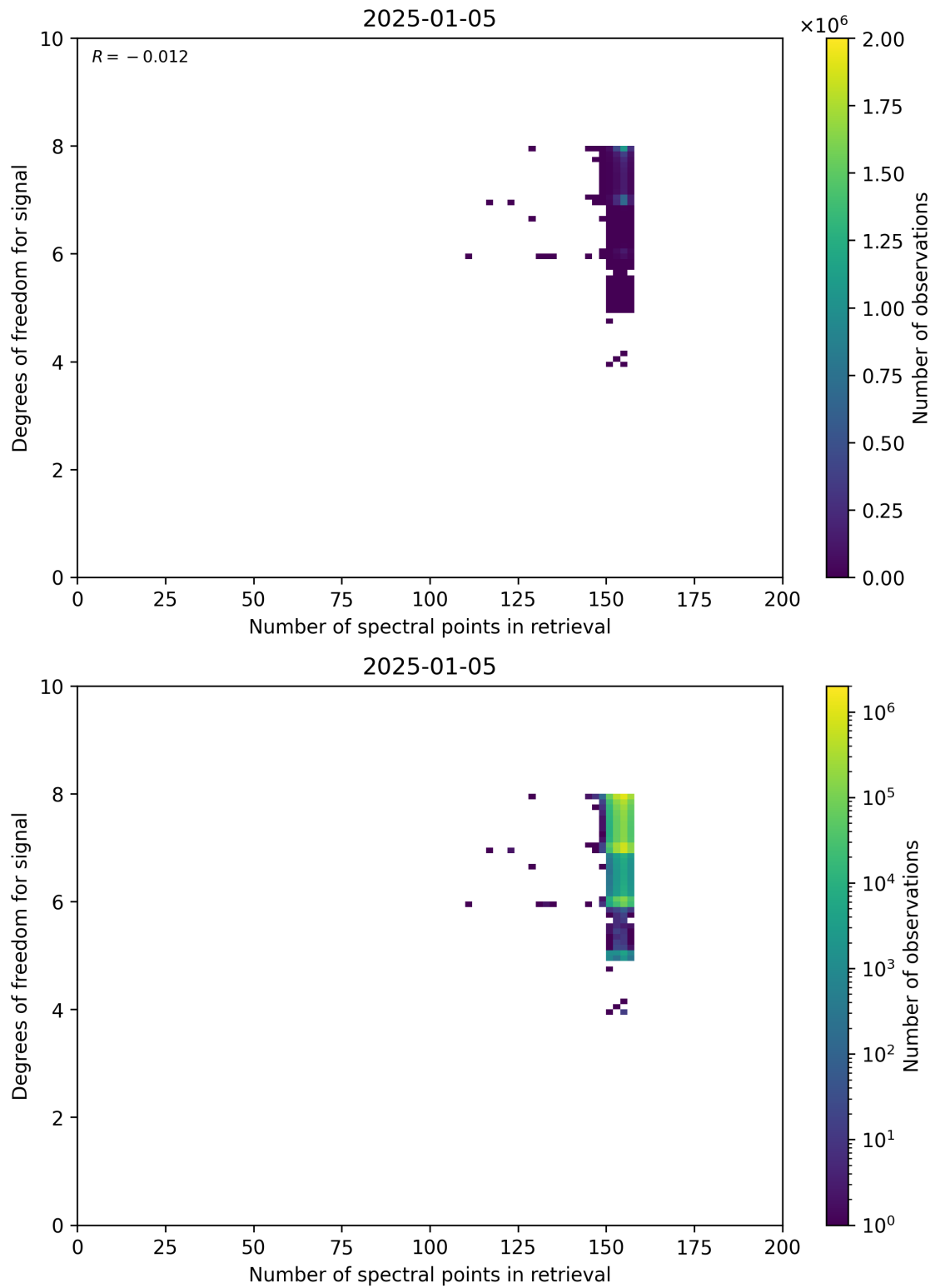
Figure 59: Scatter density plot of “Number of spectral points in retrieval” against “Degrees of freedom for signal” for 2025-01-04 to 2025-01-06.
