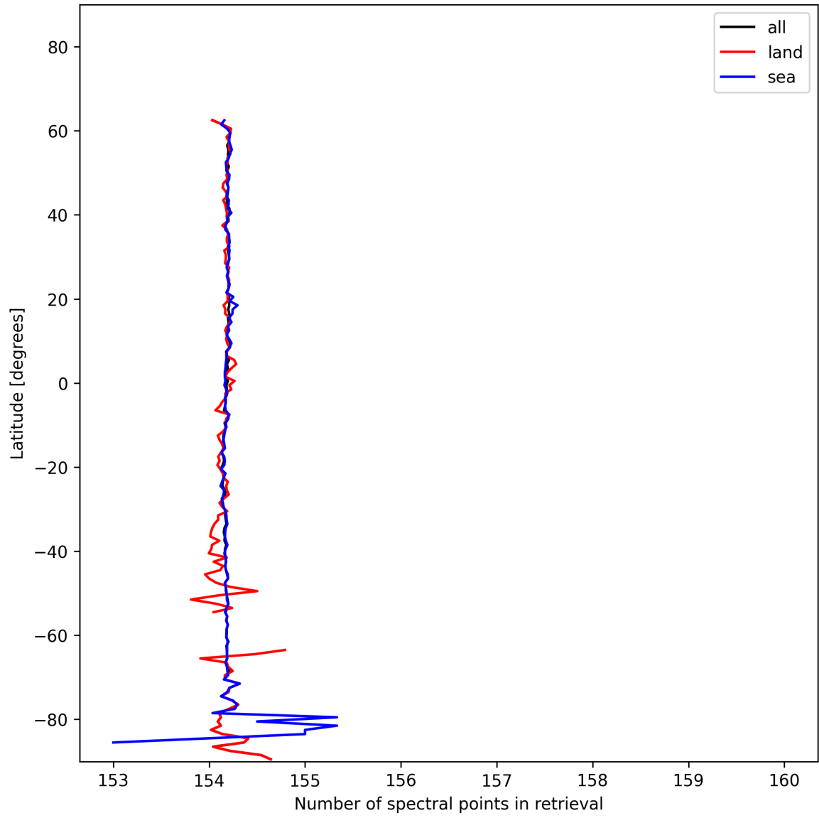
Figure 13: Zonal average of “Number of spectral points in retrieval” for 2025-01-04 to 2025-01-06.
