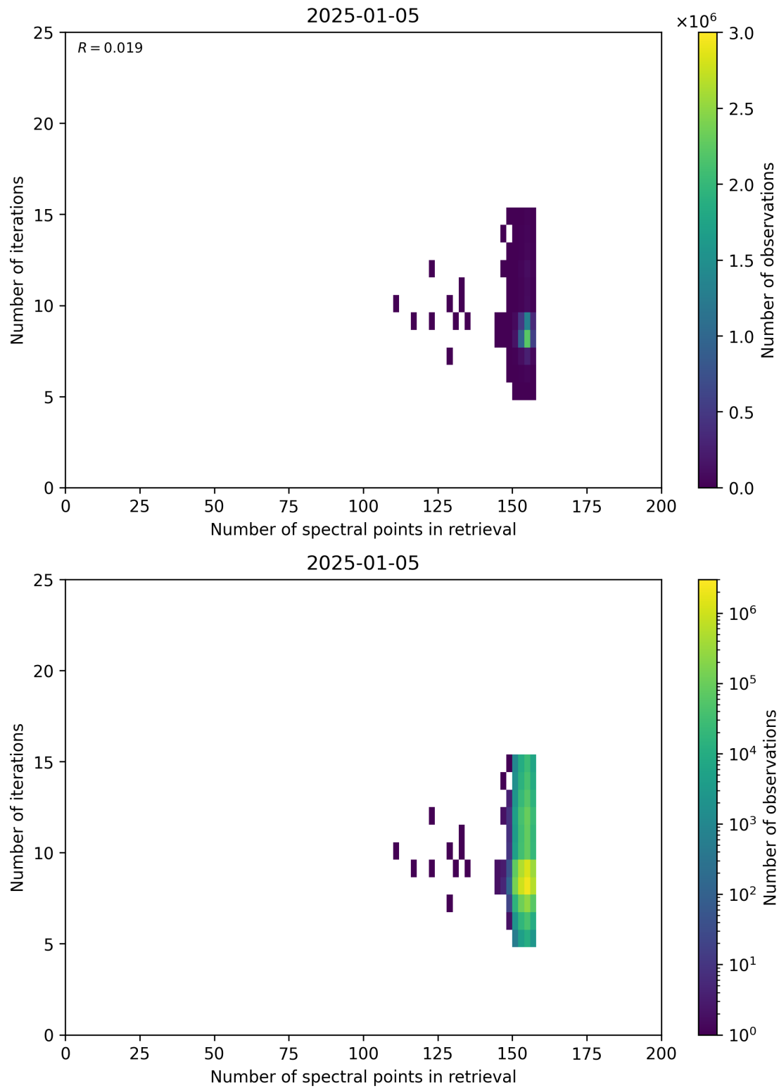
Figure 60: Scatter density plot of “Number of spectral points in retrieval” against “Number of iterations” for 2025-01-04 to 2025-01-06.
