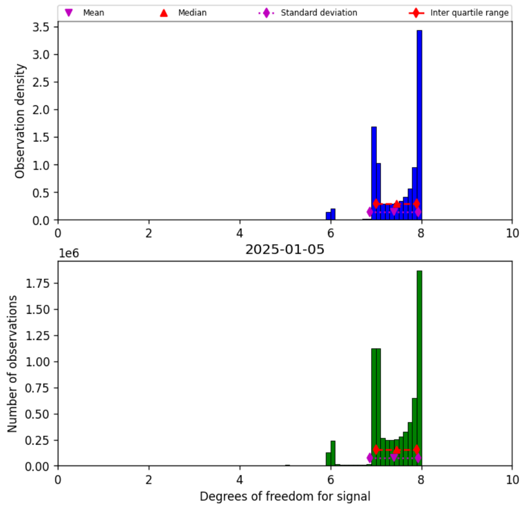
Figure 23: Histogram of “Degrees of freedom for signal” for 2025-01-04 to 2025-01-06
