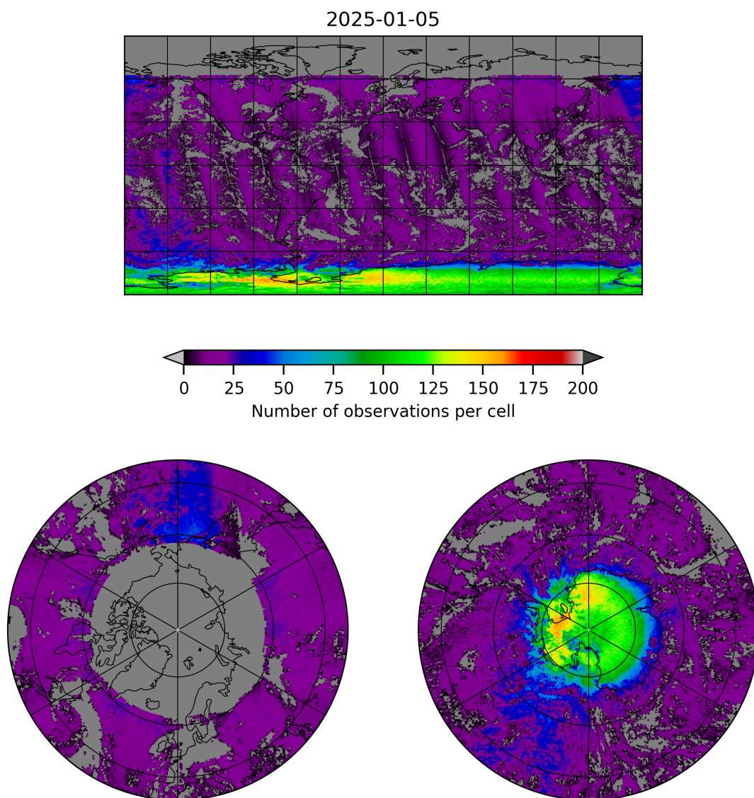
Figure 8: Map of the number of observations for 2025-01-04 to 2025-01-06
