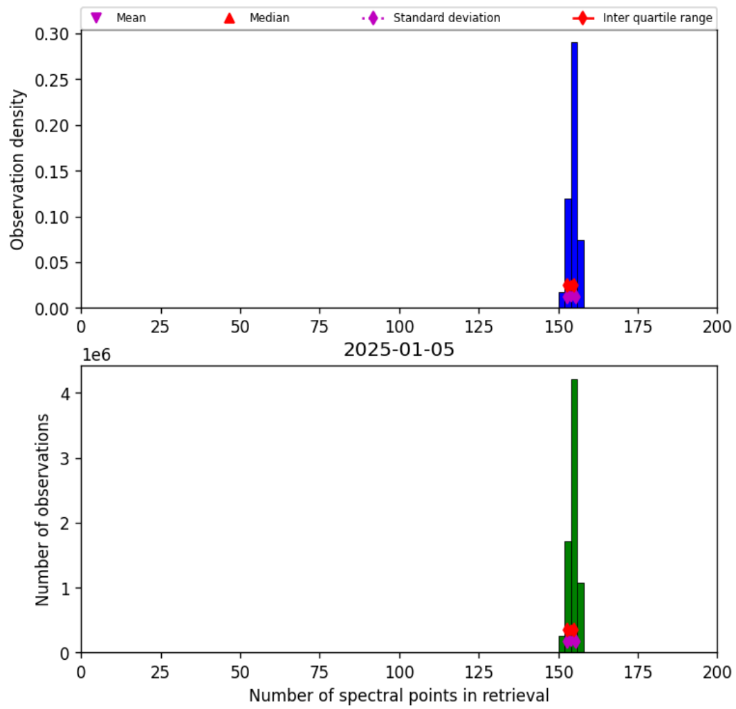
Figure 21: Histogram of “Number of spectral points in retrieval” for 2025-01-04 to 2025-01-06
