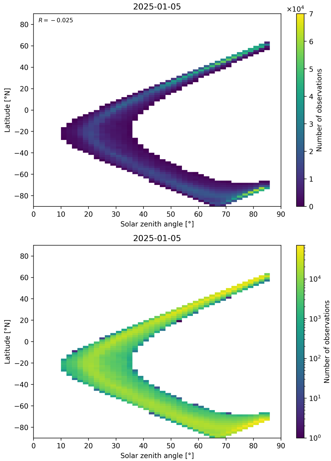
Figure 66: Scatter density plot of “Solar zenith angle” against “Latitude” for 2025-01-04 to 2025-01-06.
