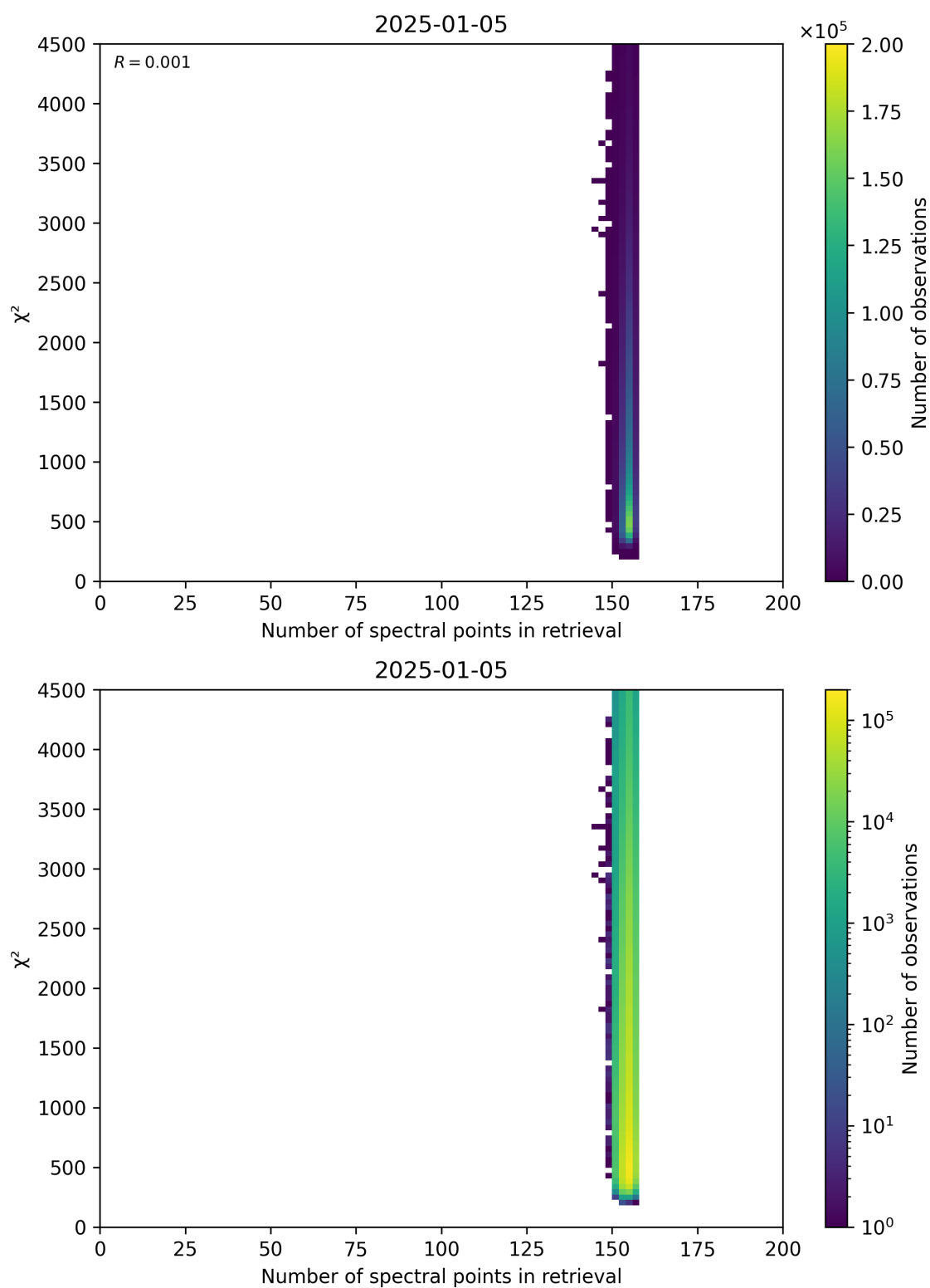
Figure 58: Scatter density plot of “Number of spectral points in retrieval” against “ \chi^2 ” for 2025-01-04 to 2025-01-06.
