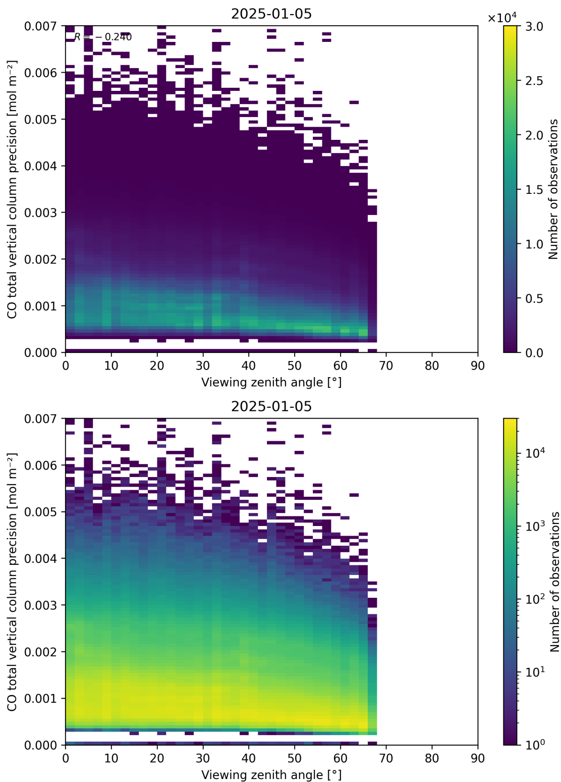
Figure 71: Scatter density plot of “Viewing zenith angle” against “CO total vertical column precision” for 2025-01-04 to 2025-01-06.
