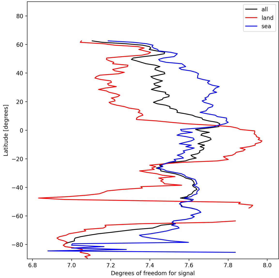
Figure 15: Zonal average of “Degrees of freedom for signal” for 2025-01-04 to 2025-01-06.
