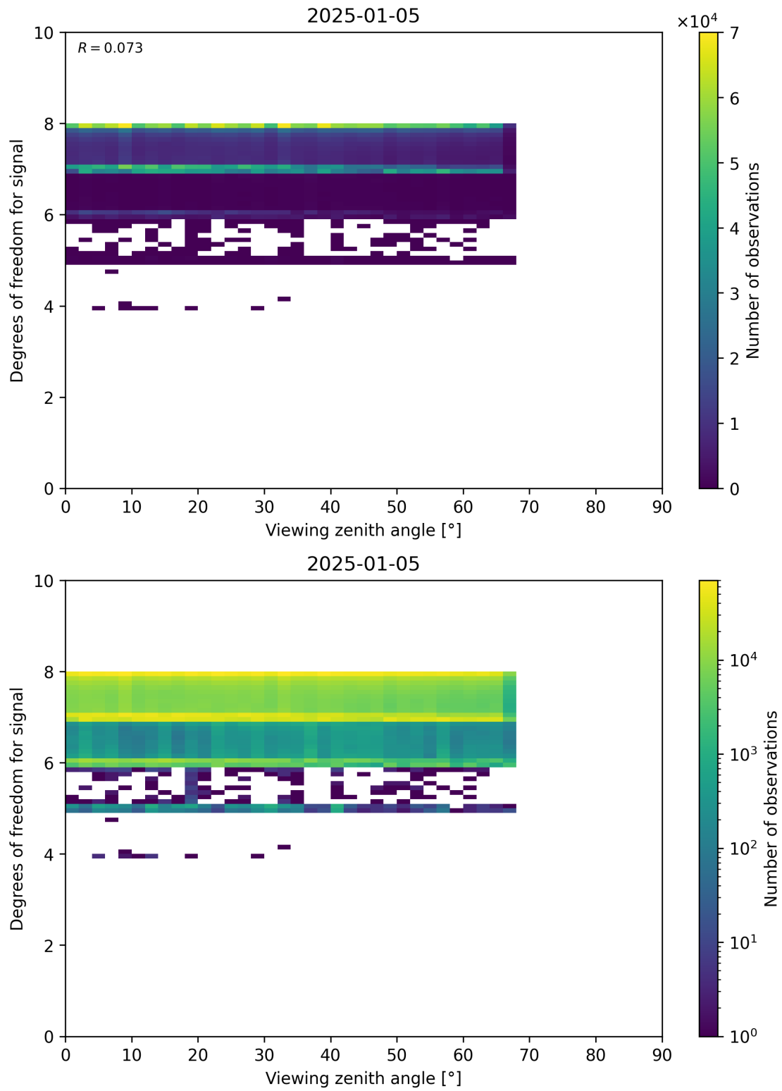
Figure 73: Scatter density plot of “Viewing zenith angle” against “Degrees of freedom for signal” for 2025-01-04 to 2025-01-06.
