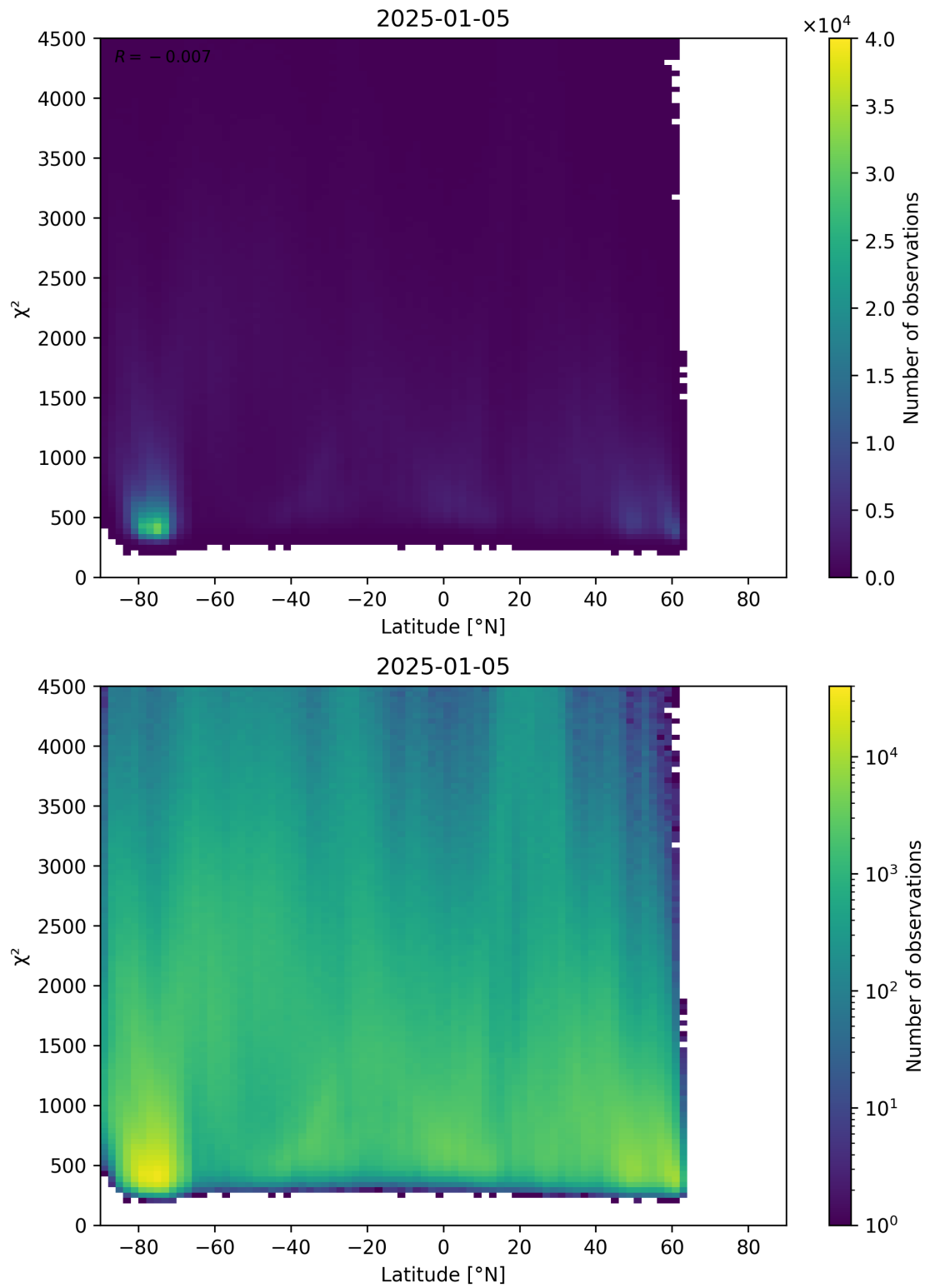
Figure 54: Scatter density plot of “Latitude” against “ \chi^2 ” for 2025-01-04 to 2025-01-06.
