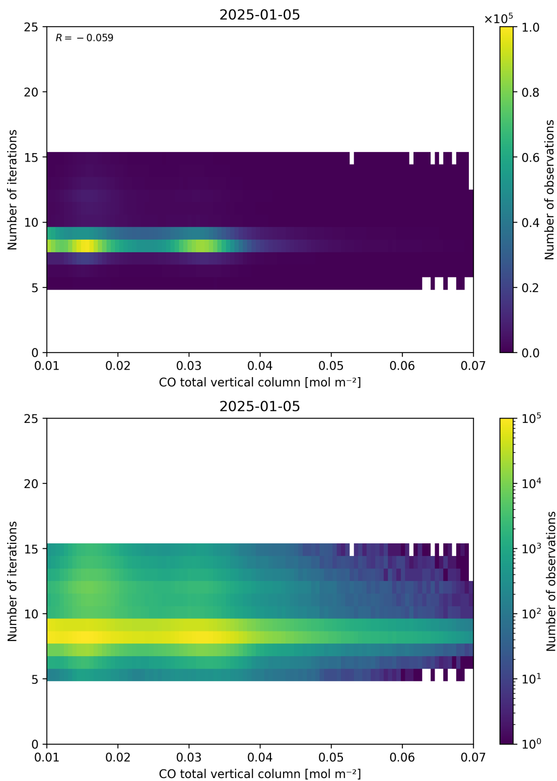
Figure 42: Scatter density plot of “CO total vertical column” against “Number of iterations” for 2025-01-04 to 2025-01-06.
