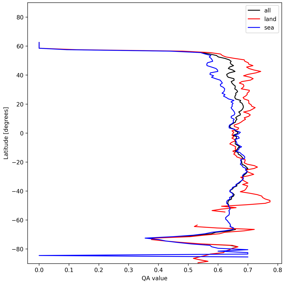
Figure 9: Zonal average of “QA value” for 2025-01-04 to 2025-01-06.
