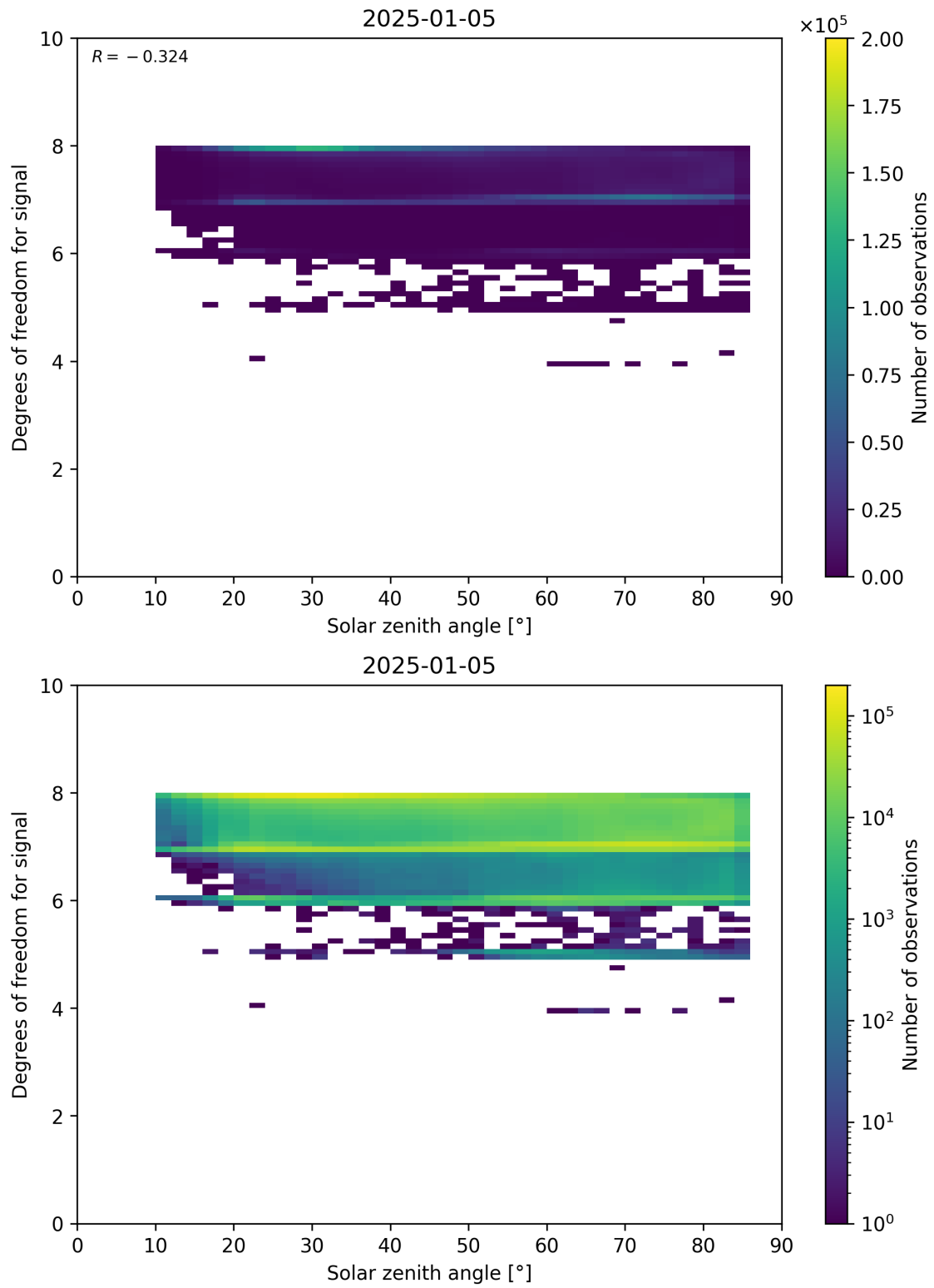
Figure 65: Scatter density plot of “Solar zenith angle” against “Degrees of freedom for signal” for 2025-01-04 to 2025-01-06.
