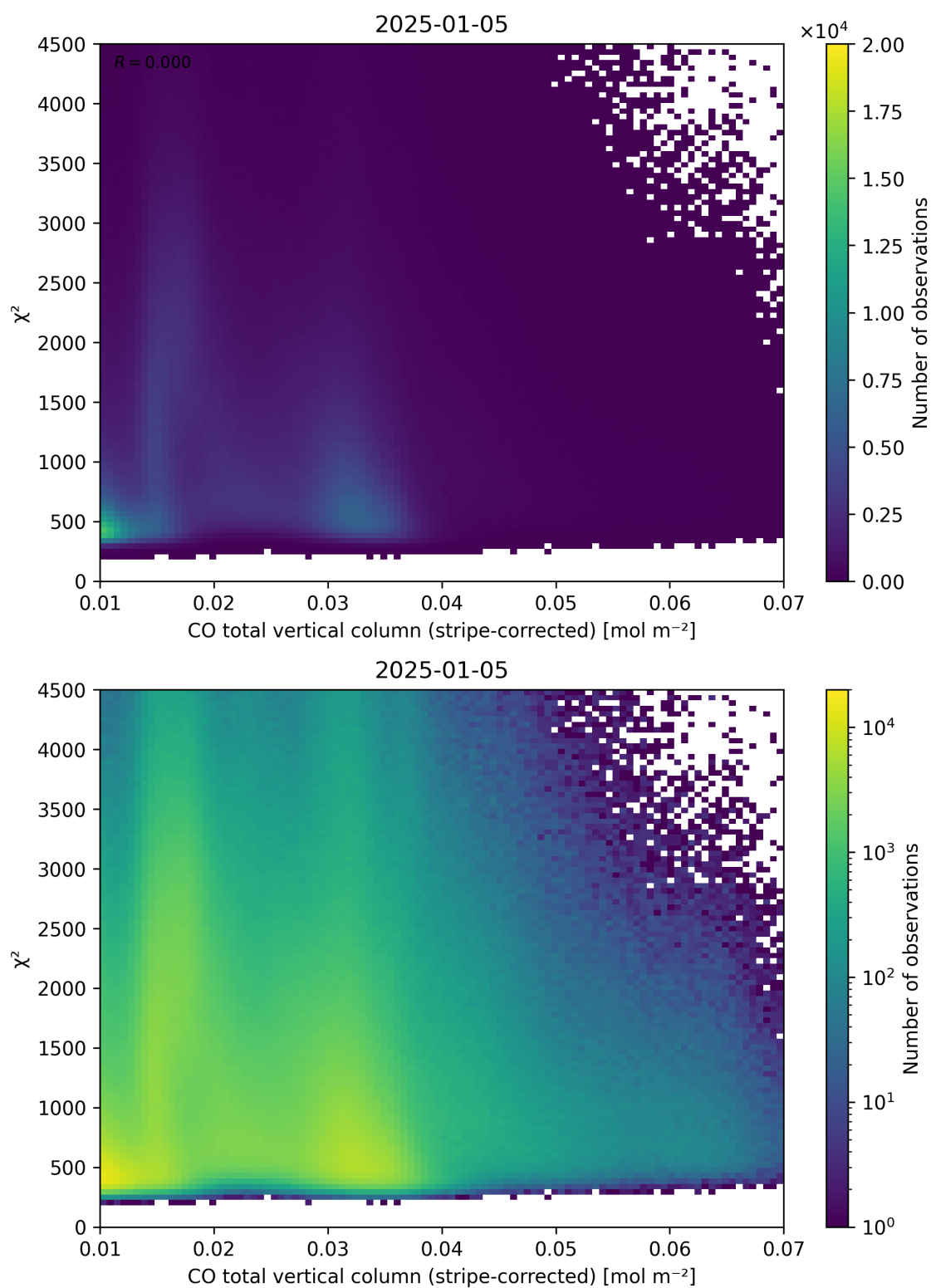
Figure 37: Scatter density plot of “CO total vertical column (stripe-corrected)” against “ \chi^2 ” for 2025-01-04 to 2025-01-06.
