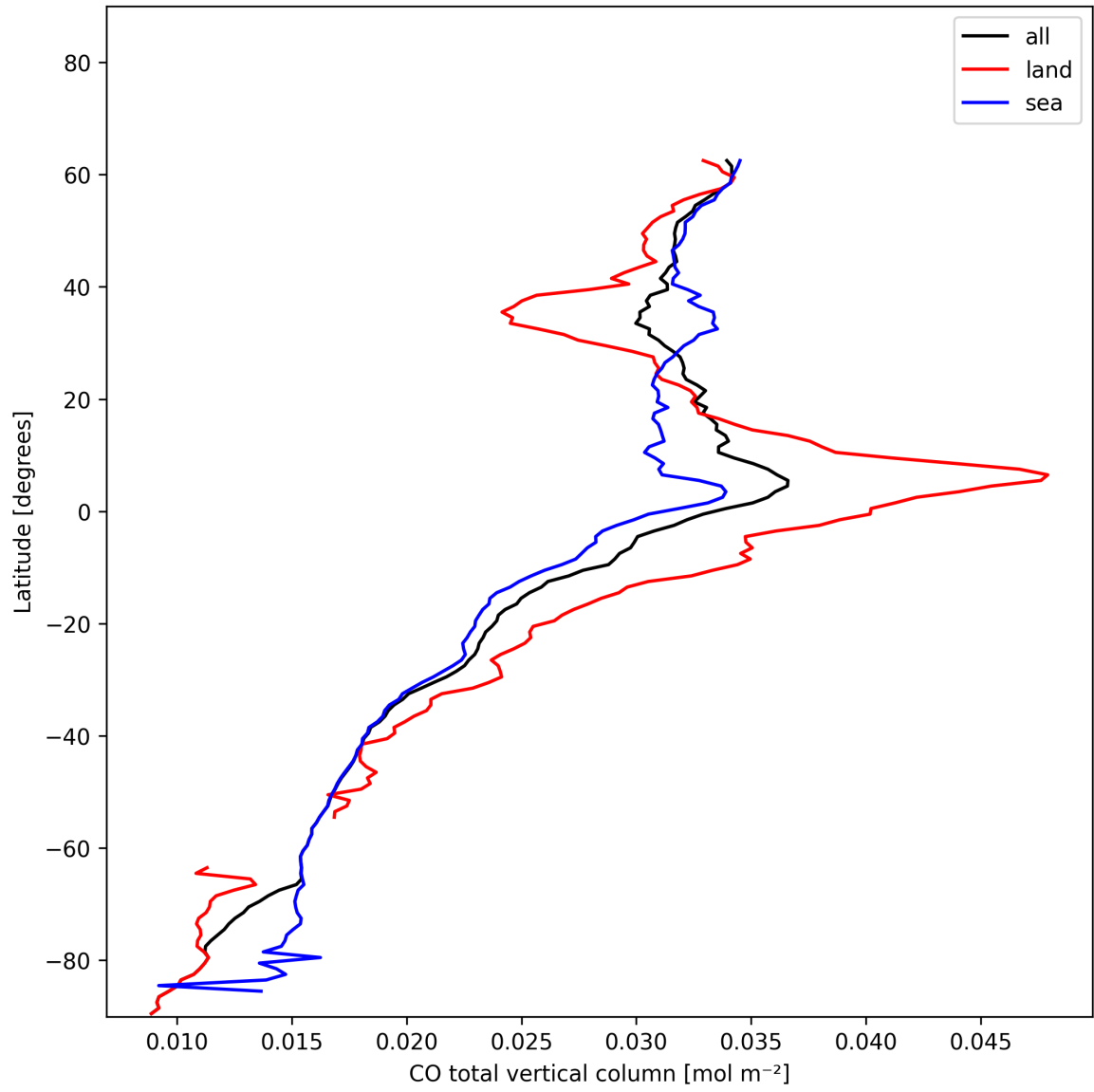
Figure 10: Zonal average of “CO total vertical column” for 2025-01-04 to 2025-01-06.
