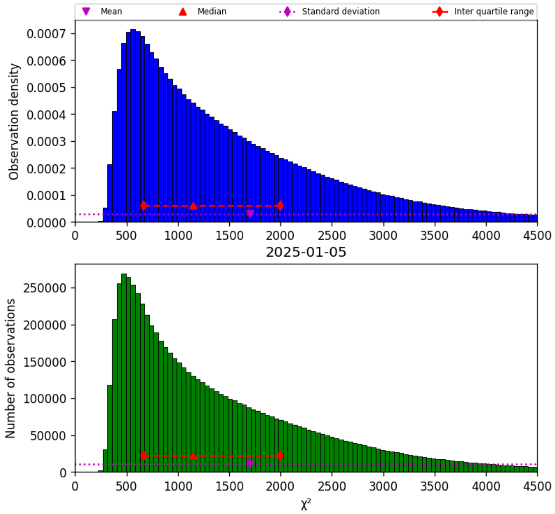
Figure 22: Histogram of “ \chi^2 ” for 2025-01-04 to 2025-01-06
