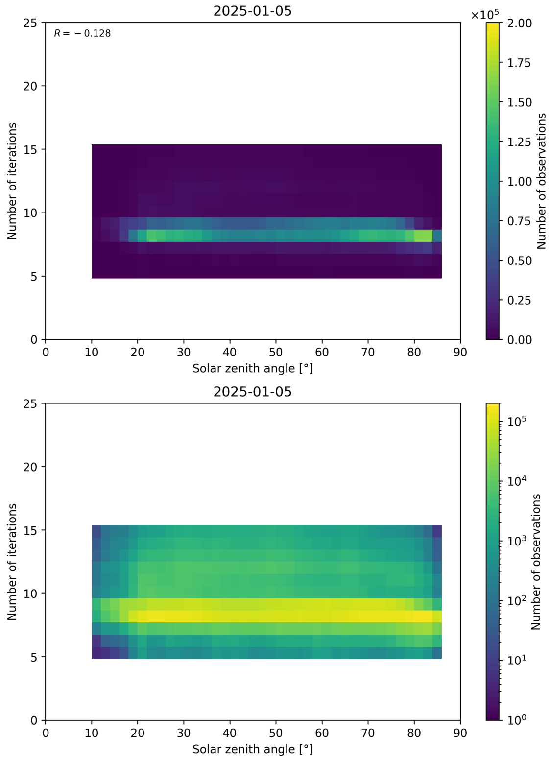
Figure 67: Scatter density plot of “Solar zenith angle” against “Number of iterations” for 2025-01-04 to 2025-01-06.
