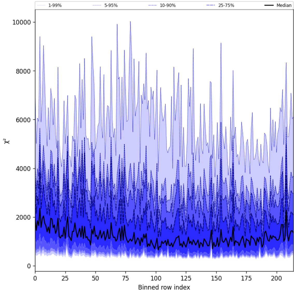
Figure 30: Along track statistics of “ \chi^2 ” for 2025-01-04 to 2025-01-06
