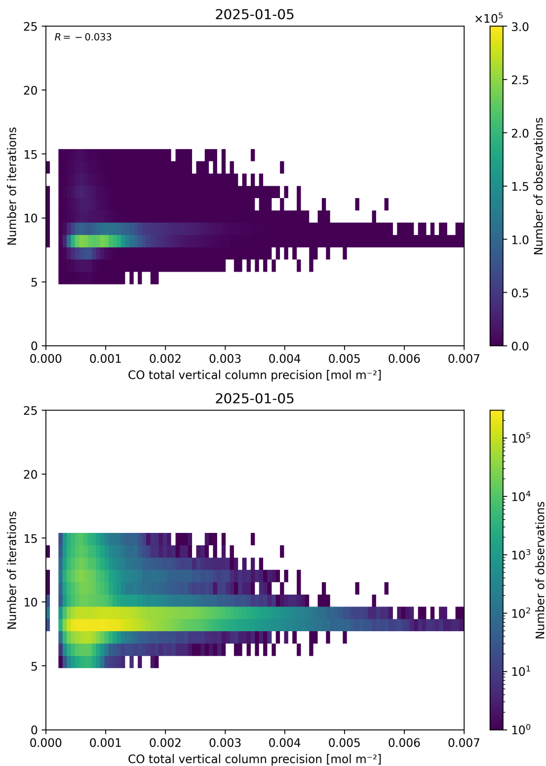
Figure 46: Scatter density plot of “CO total vertical column precision” against “Number of iterations” for 2025-01-04 to 2025-01-06.
