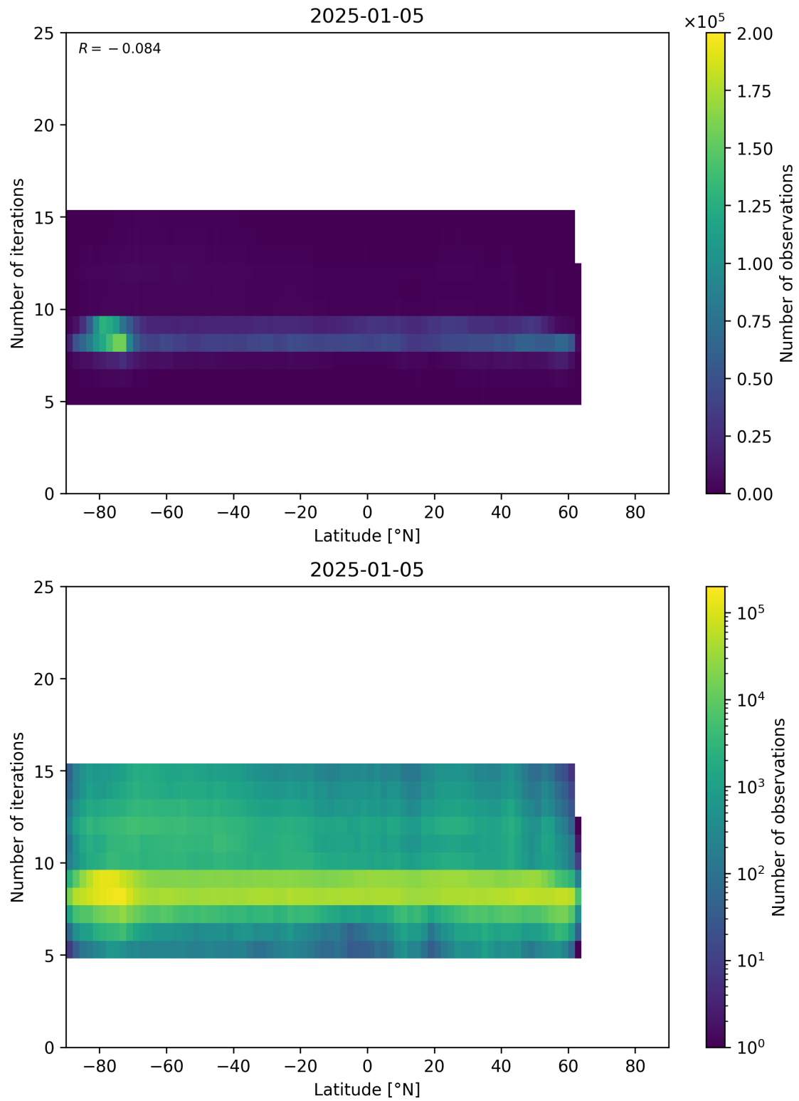
Figure 56: Scatter density plot of “Latitude” against “Number of iterations” for 2025-01-04 to 2025-01-06.
