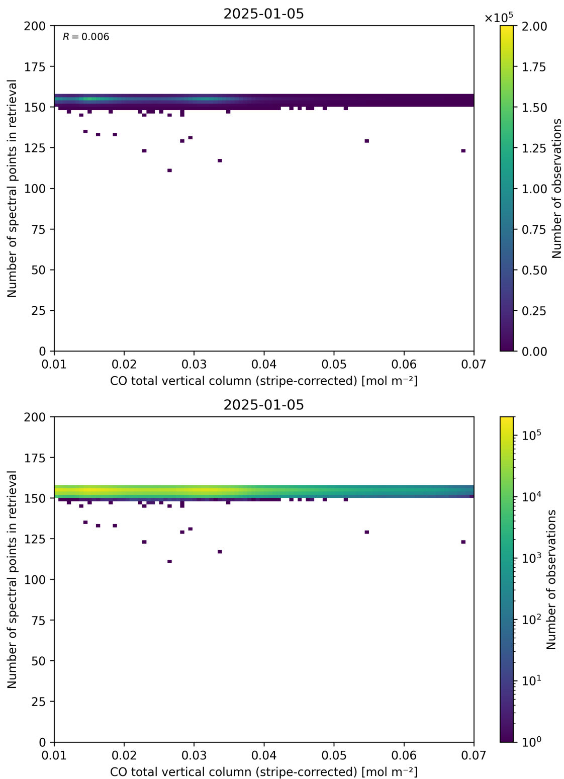
Figure 40: Scatter density plot of “CO total vertical column (stripe-corrected)” against “Number of spectral points in retrieval” for 2025-01-04 to 2025-01-06.
