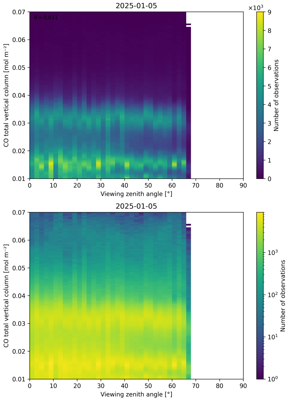
Figure 69: Scatter density plot of “Viewing zenith angle” against “CO total vertical column” for 2025-01-04 to 2025-01-06.
