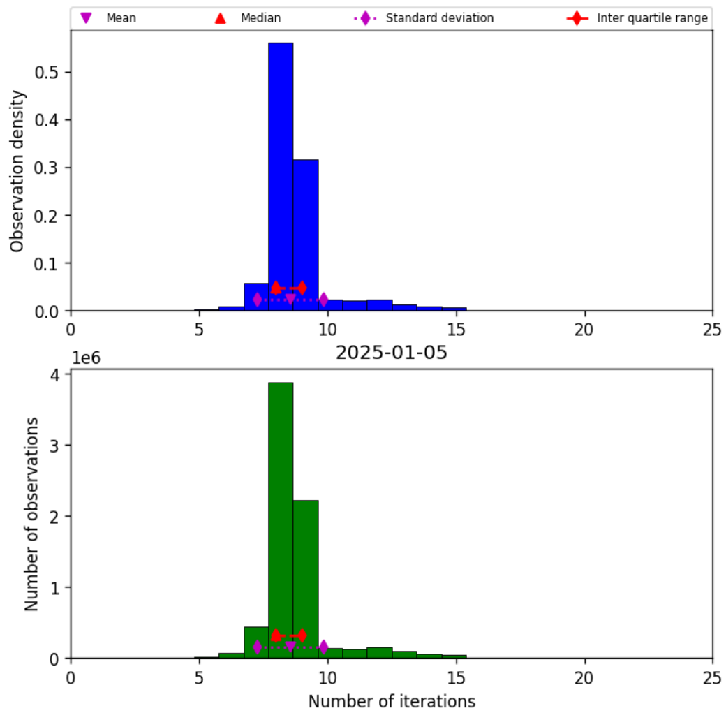
Figure 24: Histogram of “Number of iterations” for 2025-01-04 to 2025-01-06
