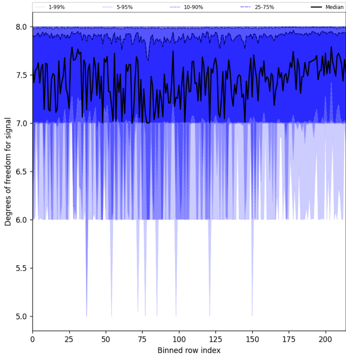
Figure 31: Along track statistics of “Degrees of freedom for signal” for 2025-01-04 to 2025-01-06
