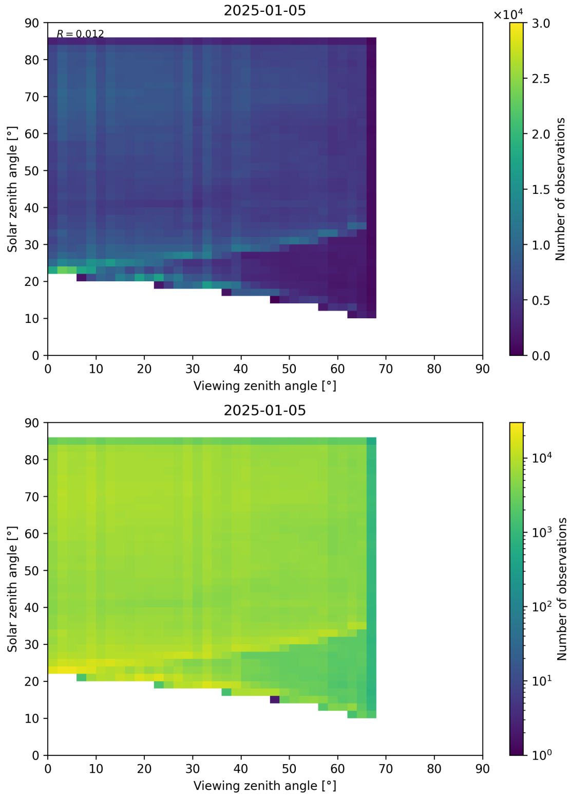
Figure 77: Scatter density plot of “Viewing zenith angle” against “Solar zenith angle” for 2025-01-04 to 2025-01-06.
