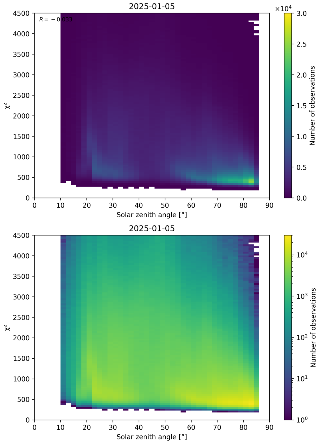
Figure 64: Scatter density plot of “Solar zenith angle” against “ \chi^2 ” for 2025-01-04 to 2025-01-06.
