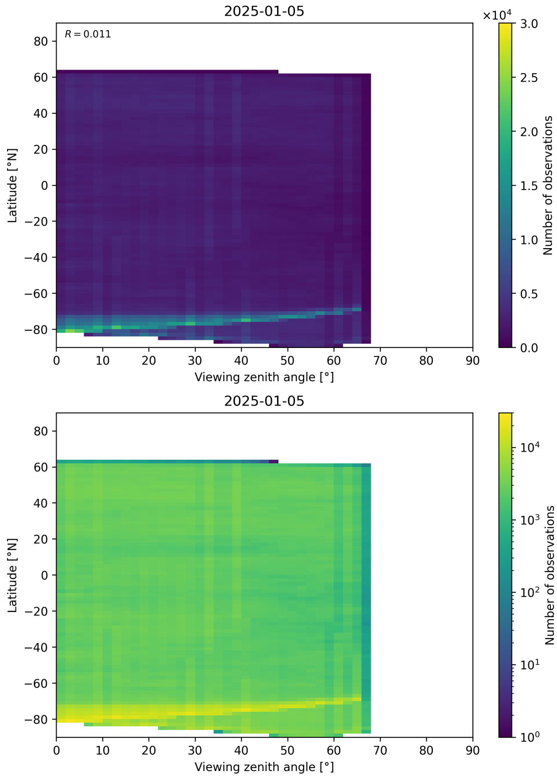
Figure 74: Scatter density plot of “Viewing zenith angle” against “Latitude” for 2025-01-04 to 2025-01-06.
