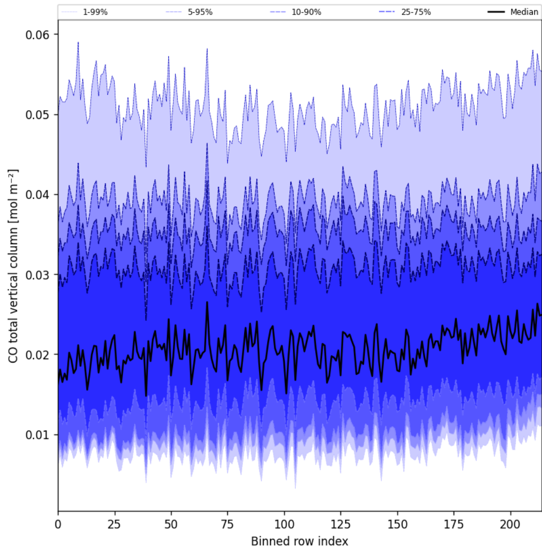
Figure 26: Along track statistics of “CO total vertical column” for 2025-01-04 to 2025-01-06
