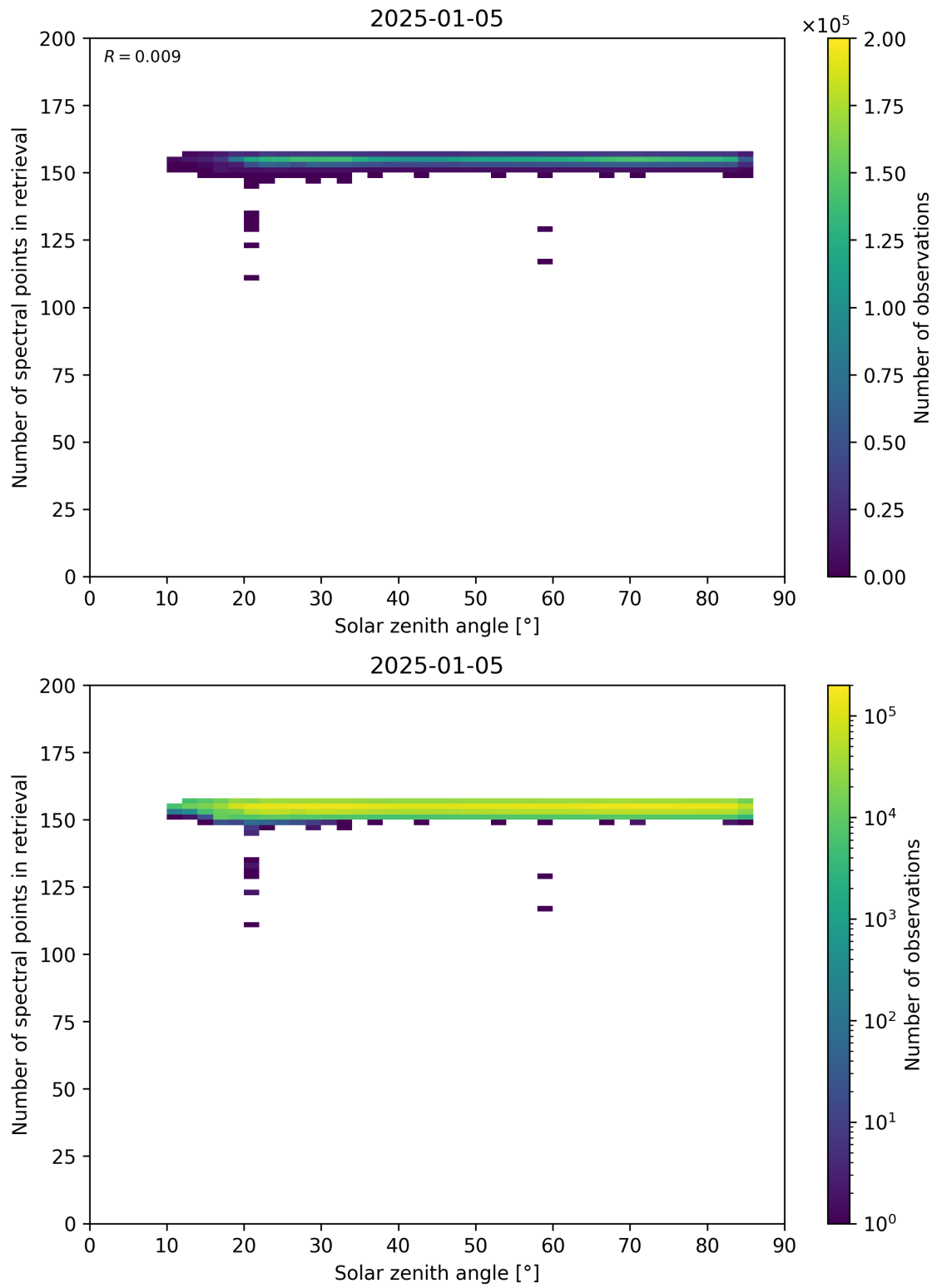
Figure 68: Scatter density plot of “Solar zenith angle” against “Number of spectral points in retrieval” for 2025-01-04 to 2025-01-06.
