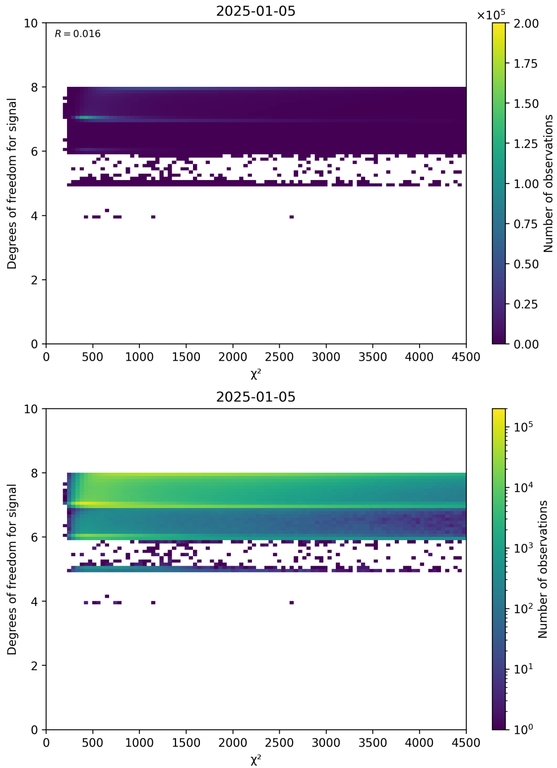
Figure 48: Scatter density plot of “ \chi^2 ” against “Degrees of freedom for signal” for 2025-01-04 to 2025-01-06.
