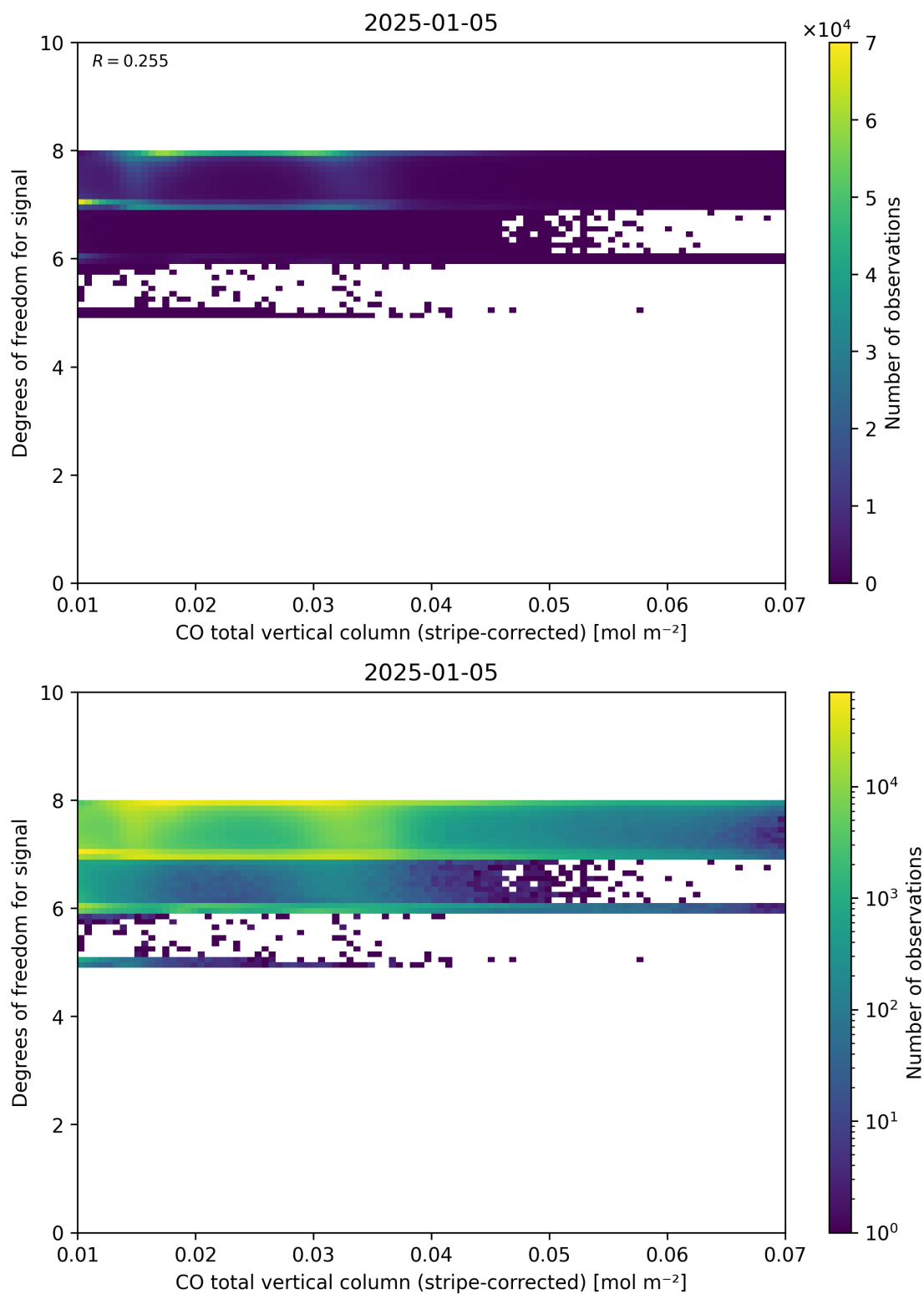
Figure 38: Scatter density plot of “CO total vertical column (stripe-corrected)” against “Degrees of freedom for signal” for 2025-01-04 to 2025-01-06.
