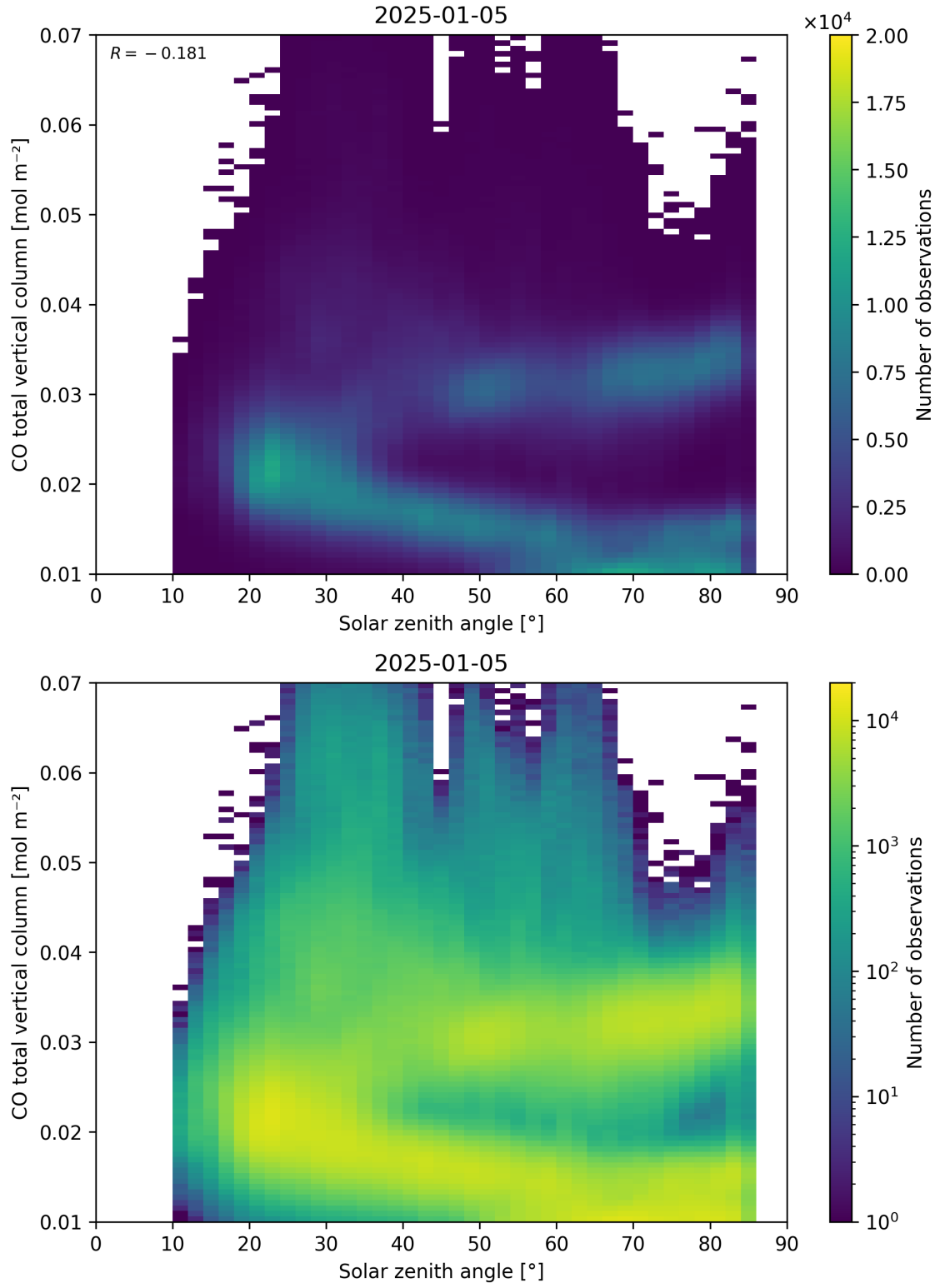
Figure 61: Scatter density plot of “Solar zenith angle” against “CO total vertical column” for 2025-01-04 to 2025-01-06.
