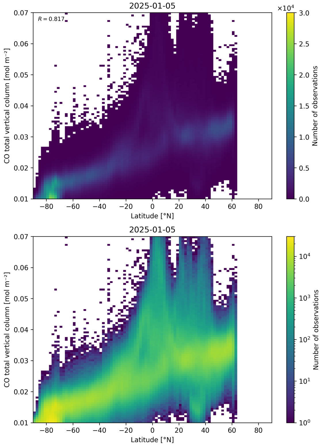
Figure 51: Scatter density plot of “Latitude” against “CO total vertical column” for 2025-01-04 to 2025-01-06.
