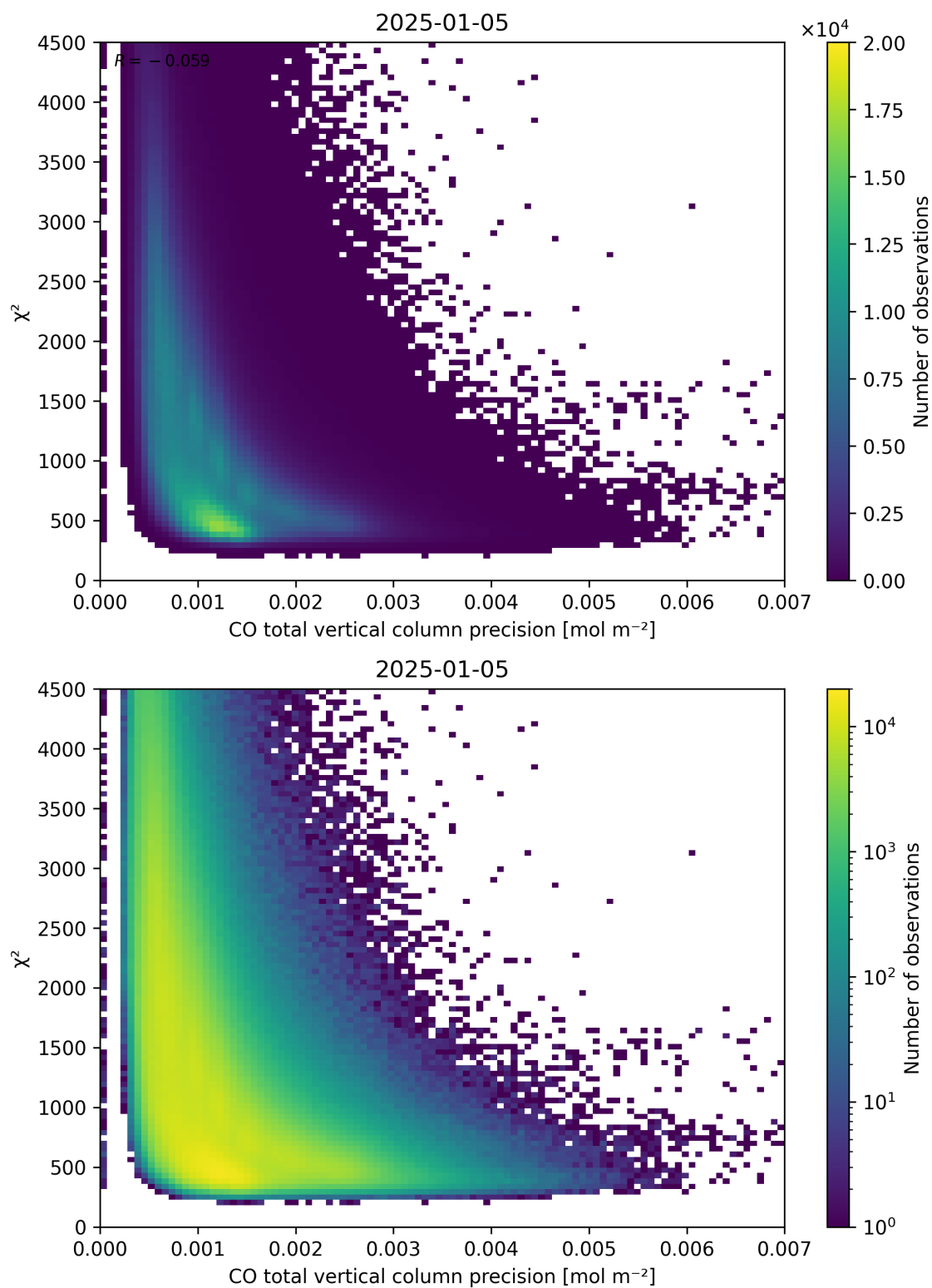
Figure 44: Scatter density plot of “CO total vertical column precision” against “ \chi^2 ” for 2025-01-04 to 2025-01-06.
