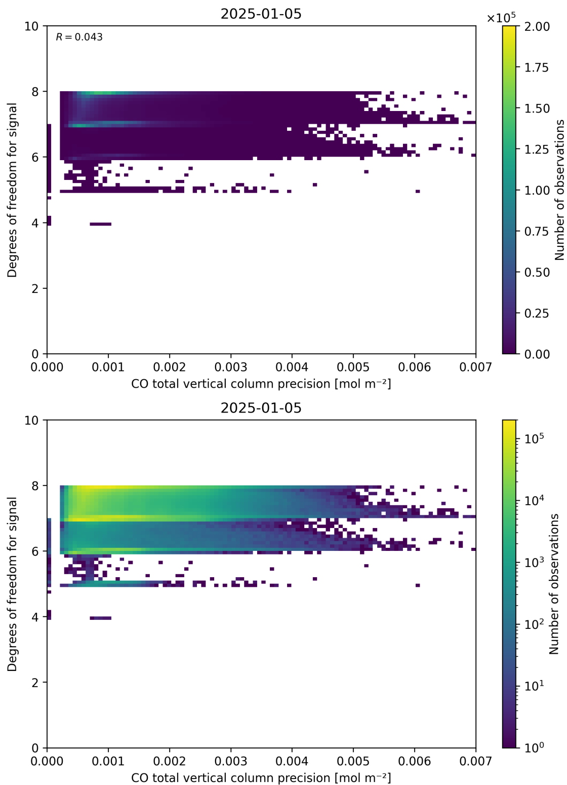
Figure 45: Scatter density plot of “CO total vertical column precision” against “Degrees of freedom for signal” for 2025-01-04 to 2025-01-06.
