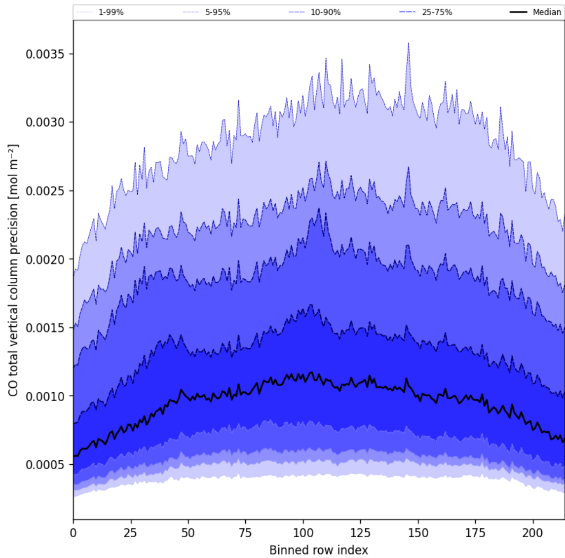
Figure 28: Along track statistics of “CO total vertical column precision” for 2025-01-04 to 2025-01-06
