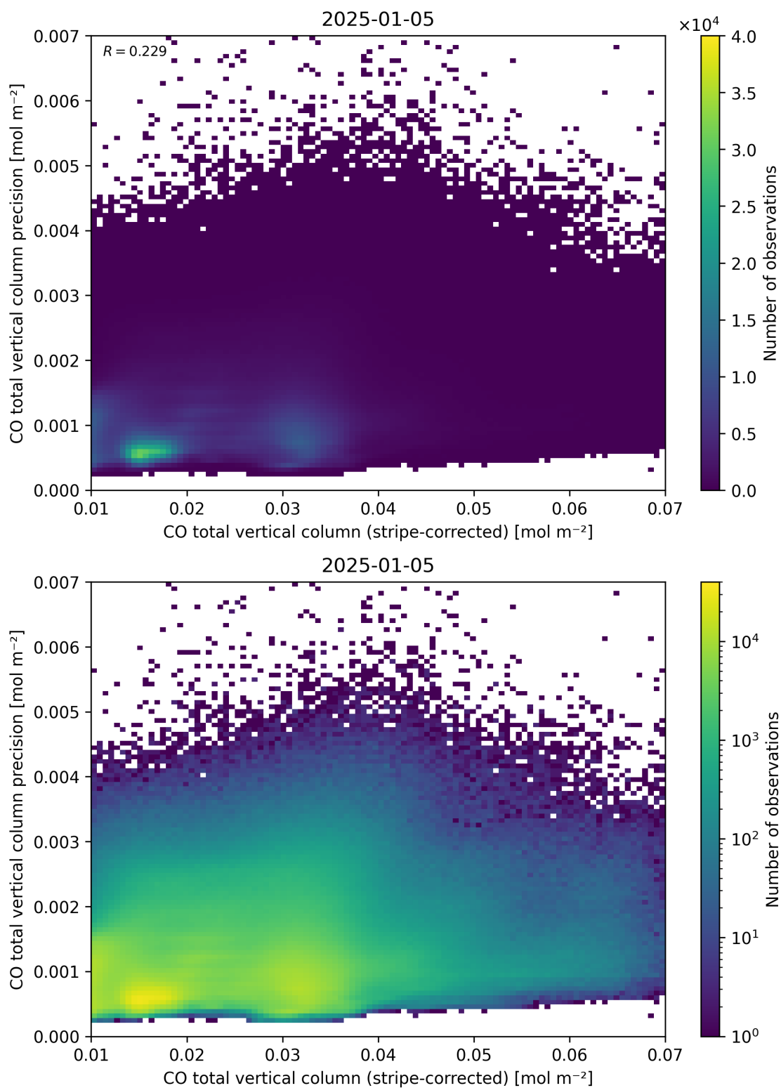
Figure 36: Scatter density plot of “CO total vertical column (stripe-corrected)” against “CO total vertical column precision” for 2025-01-04 to 2025-01-06.
