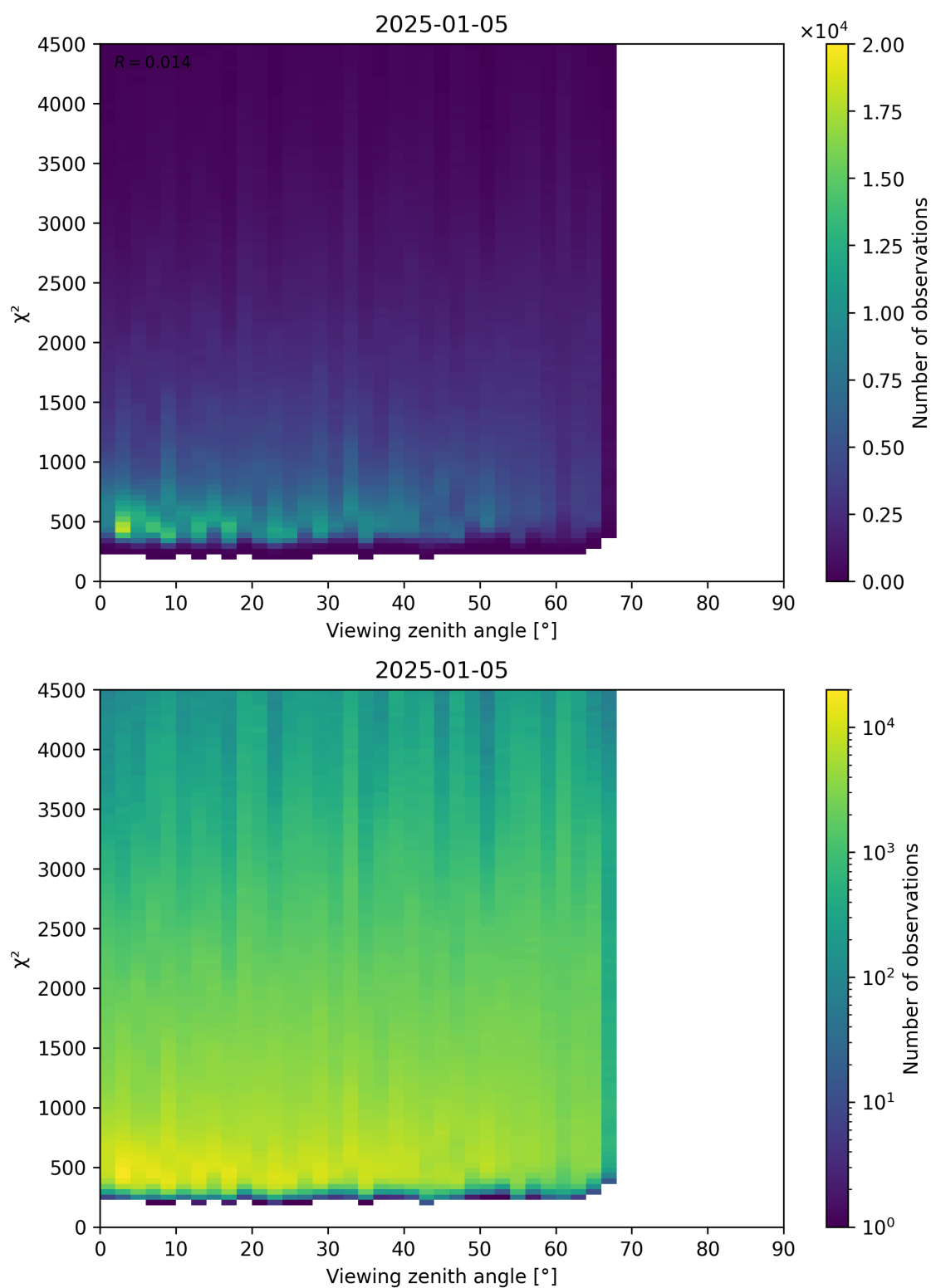
Figure 72: Scatter density plot of “Viewing zenith angle” against “ \chi^2 ” for 2025-01-04 to 2025-01-06.
