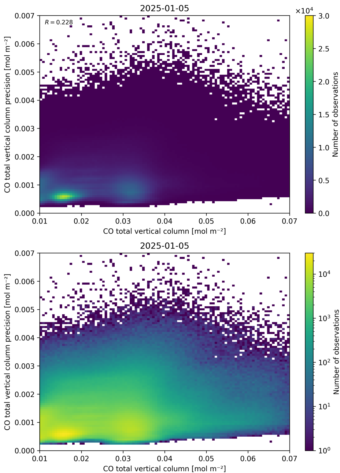
Figure 34: Scatter density plot of “CO total vertical column” against “CO total vertical column precision” for 2025-01-04 to 2025-01-06.
