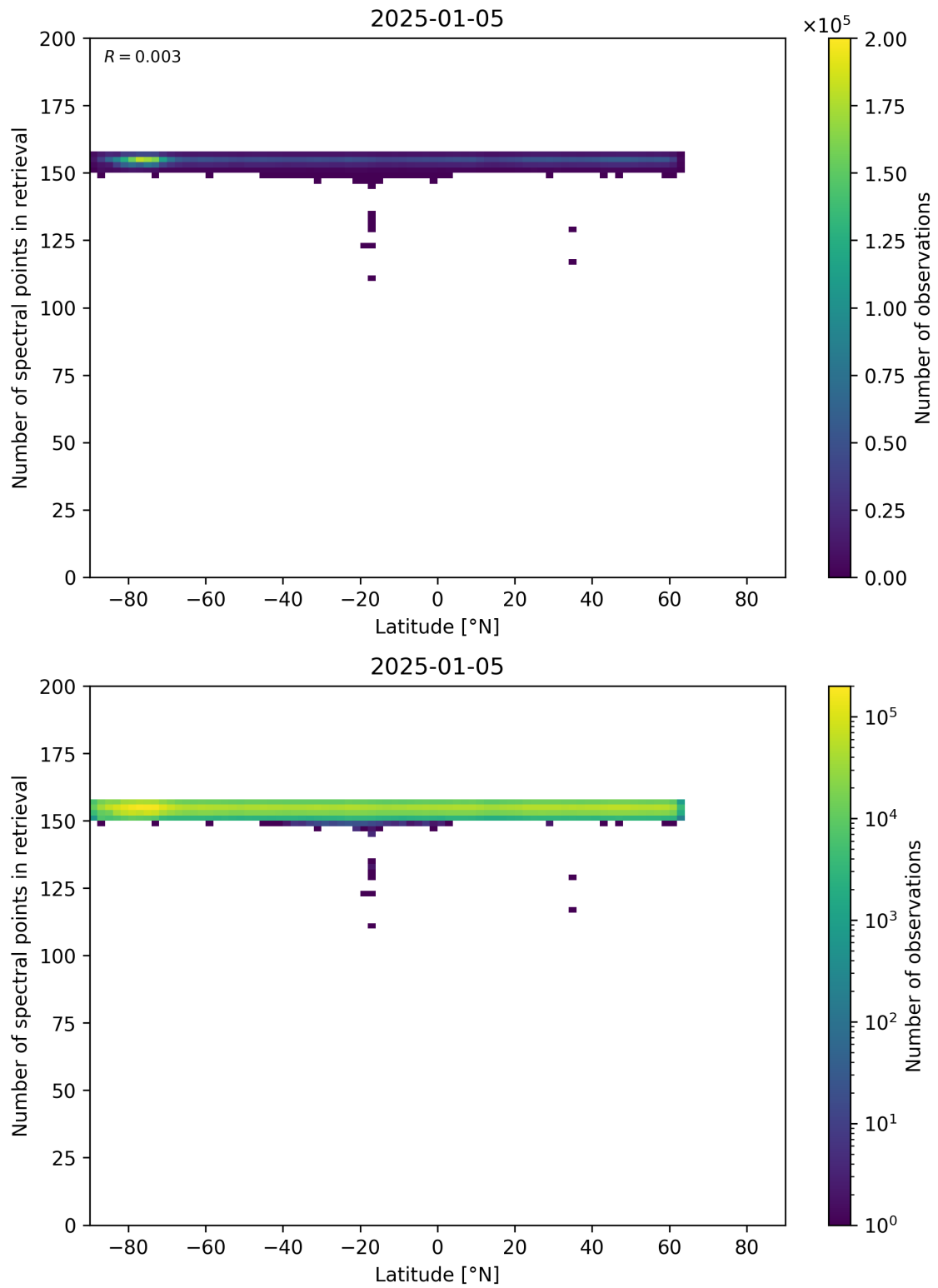
Figure 57: Scatter density plot of “Latitude” against “Number of spectral points in retrieval” for 2025-01-04 to 2025-01-06.
