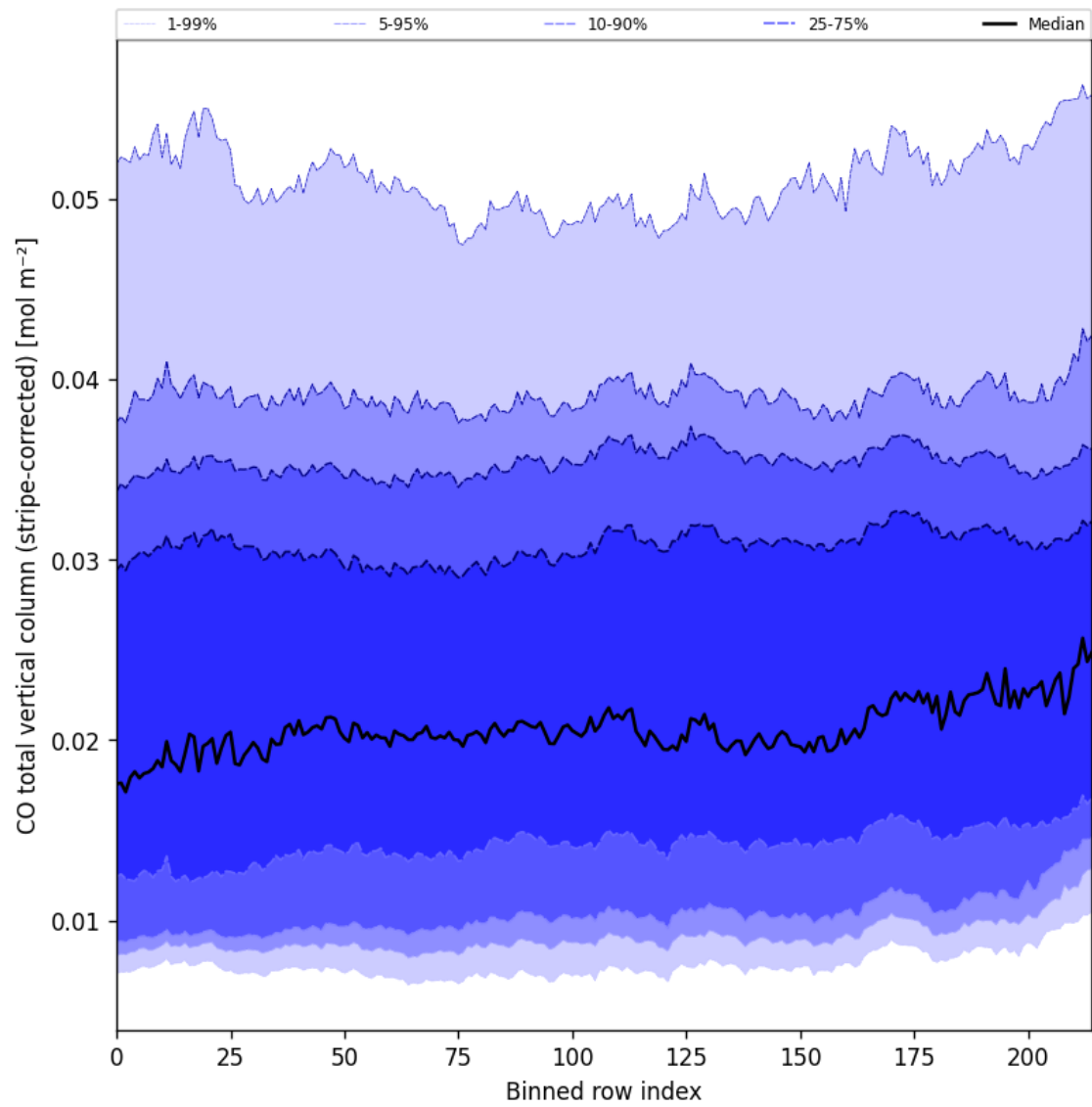
Figure 27: Along track statistics of “CO total vertical column (stripe-corrected)” for 2025-01-04 to 2025-01-06
