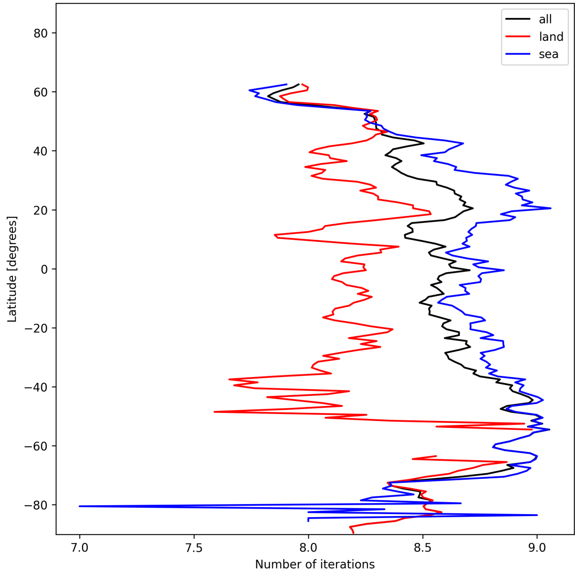
Figure 16: Zonal average of “Number of iterations” for 2025-01-04 to 2025-01-06.
