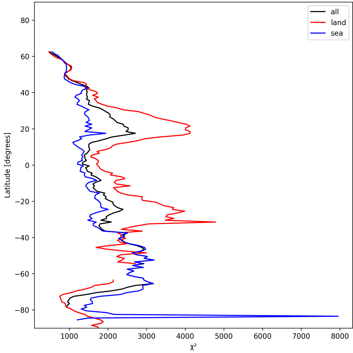
Figure 14: Zonal average of “ \chi^2 ” for 2025-01-04 to 2025-01-06.
