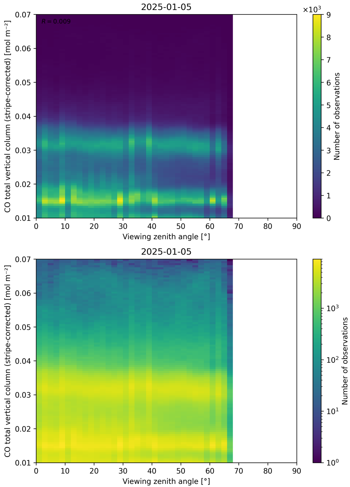
Figure 70: Scatter density plot of “Viewing zenith angle” against “CO total vertical column (stripe-corrected)” for 2025-01-04 to 2025-01-06.
