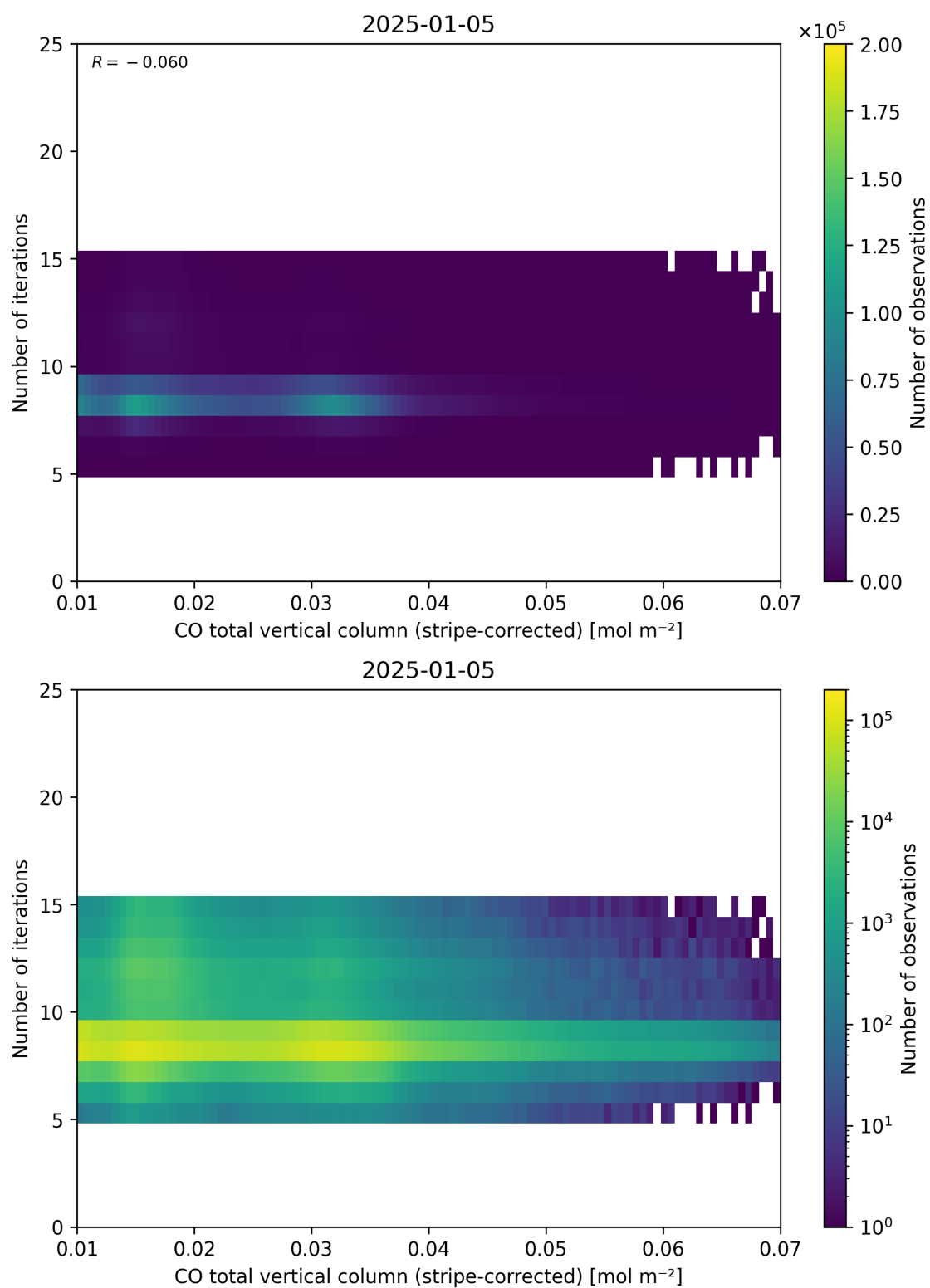
Figure 39: Scatter density plot of “CO total vertical column (stripe-corrected)” against “Number of iterations” for 2025-01-04 to 2025-01-06.
