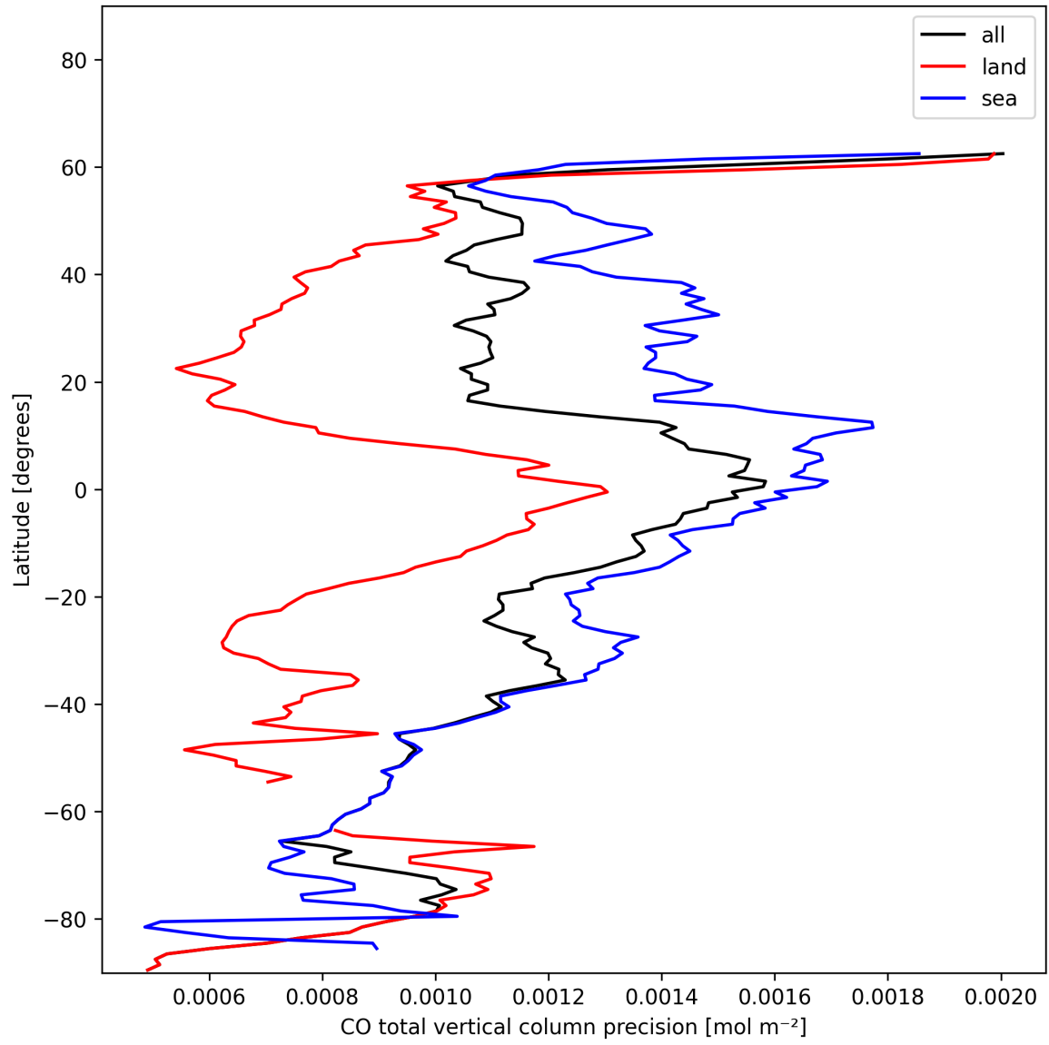
Figure 12: Zonal average of “CO total vertical column precision” for 2025-01-04 to 2025-01-06.
