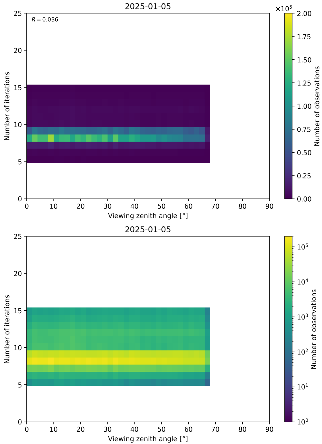
Figure 75: Scatter density plot of “Viewing zenith angle” against “Number of iterations” for 2025-01-04 to 2025-01-06.
