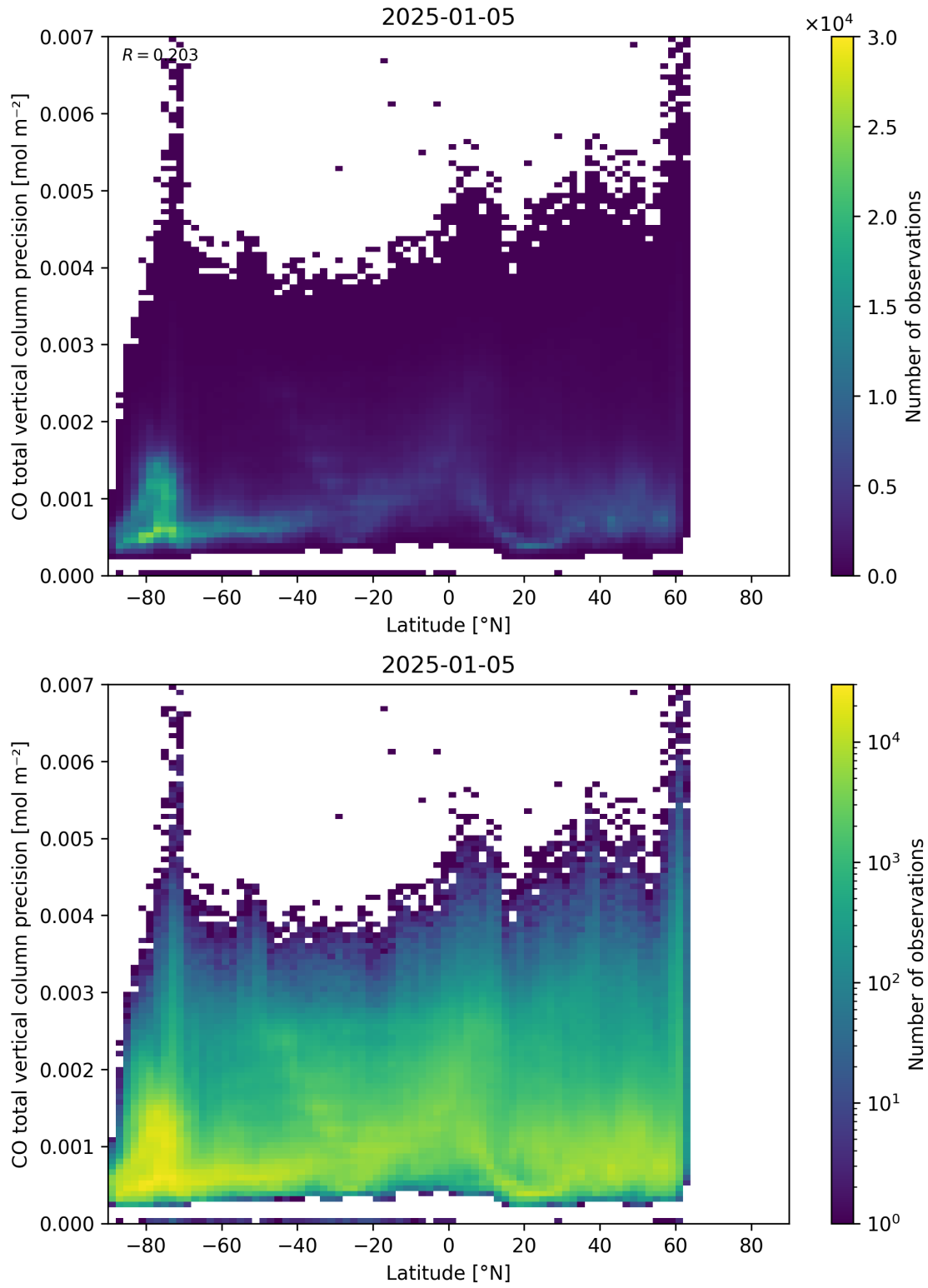
Figure 53: Scatter density plot of “Latitude” against “CO total vertical column precision” for 2025-01-04 to 2025-01-06.
