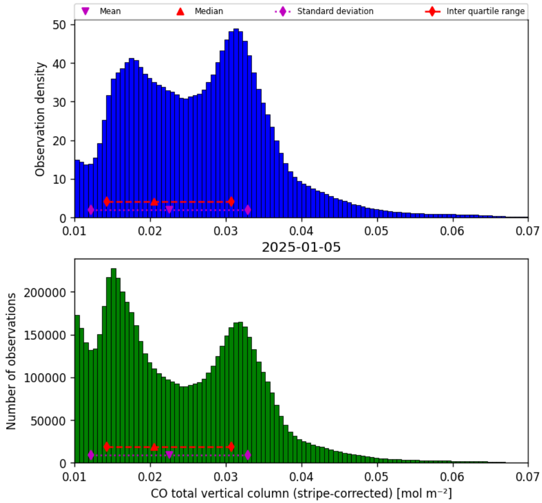
Figure 19: Histogram of “CO total vertical column (stripe-corrected)” for 2025-01-04 to 2025-01-06
