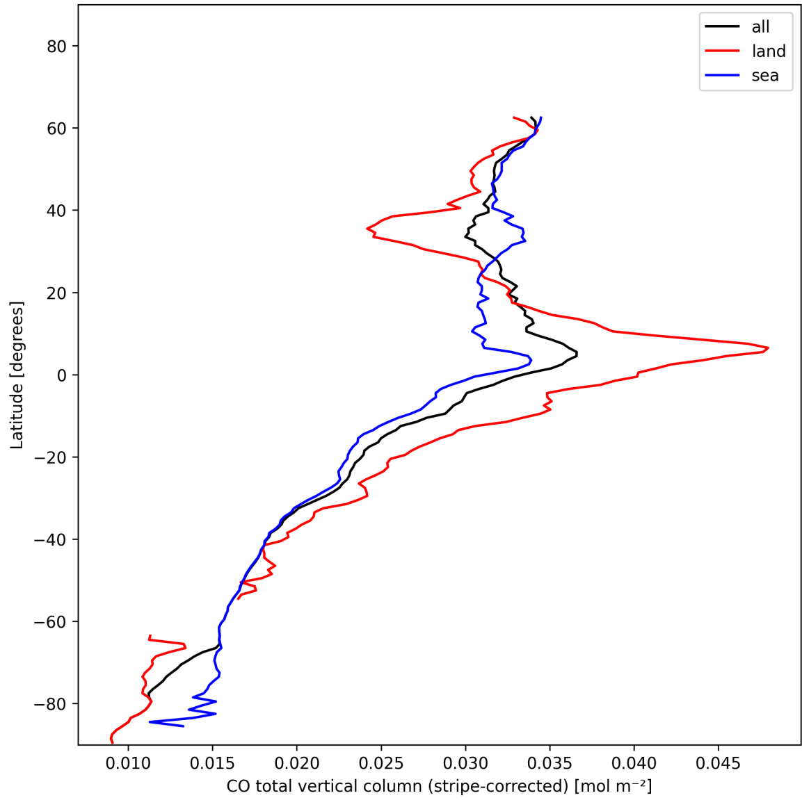
Figure 11: Zonal average of “CO total vertical column (stripe-corrected)” for 2025-01-04 to 2025-01-06.
