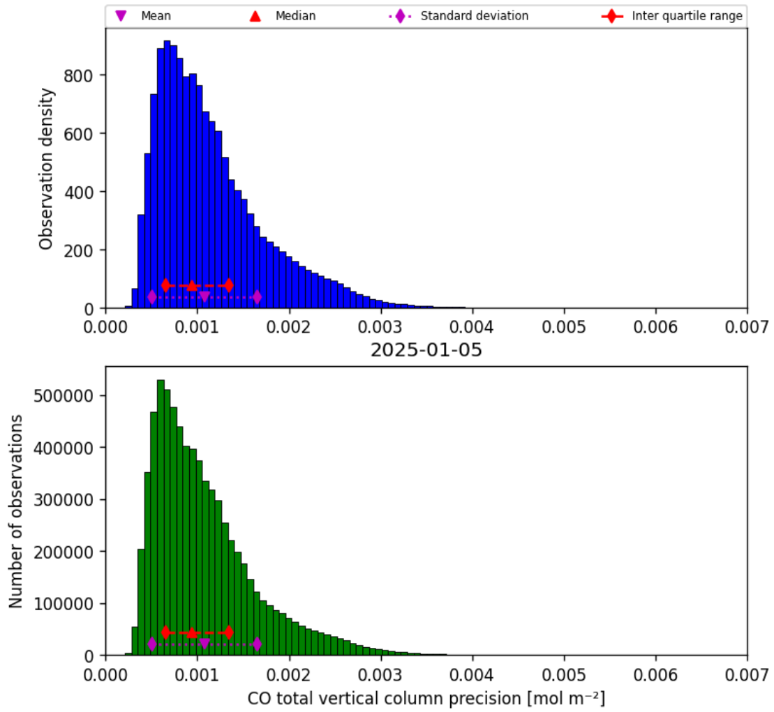
Figure 20: Histogram of “CO total vertical column precision” for 2025-01-04 to 2025-01-06
