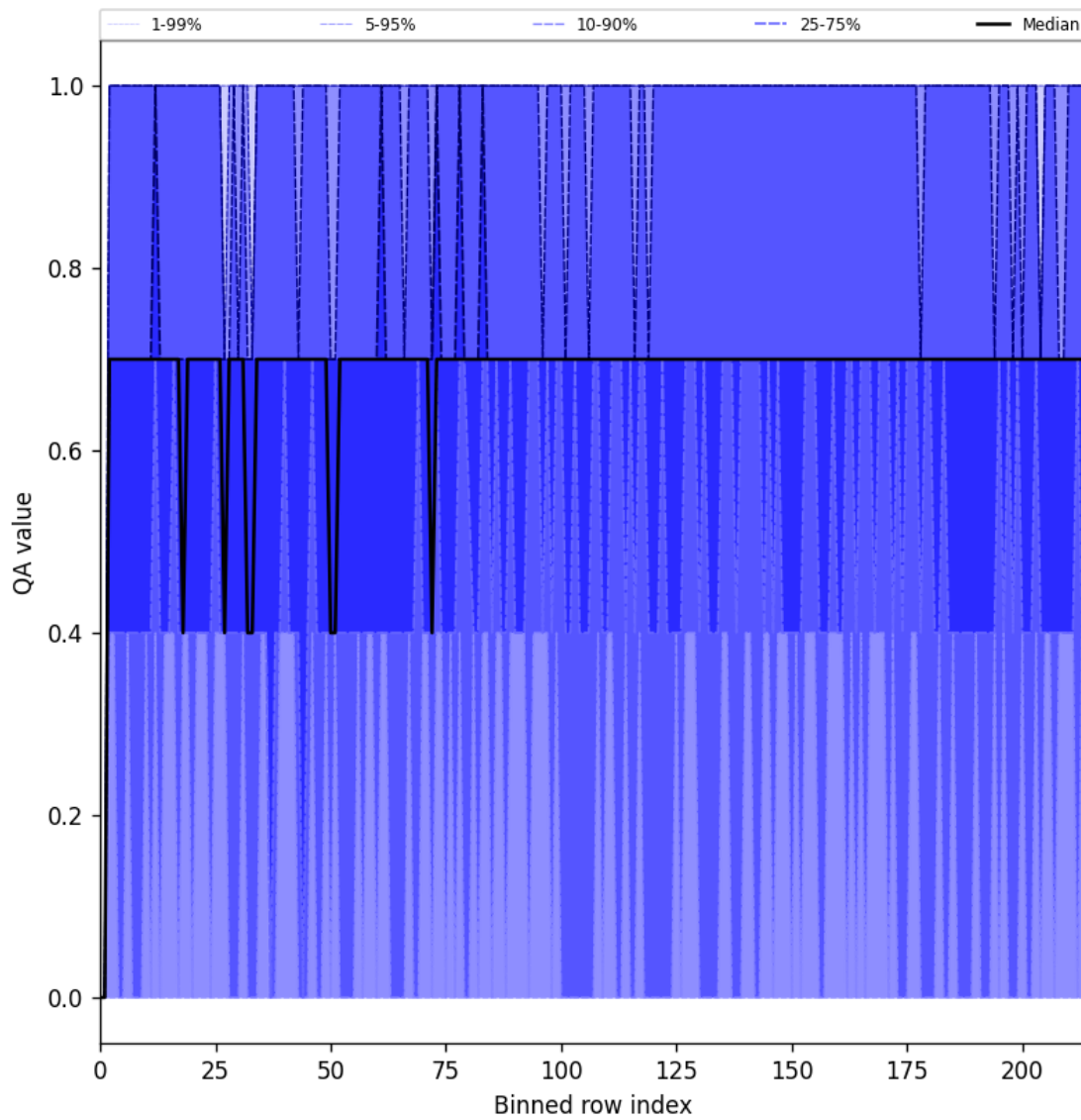
Figure 25: Along track statistics of “QA value” for 2025-01-04 to 2025-01-06
