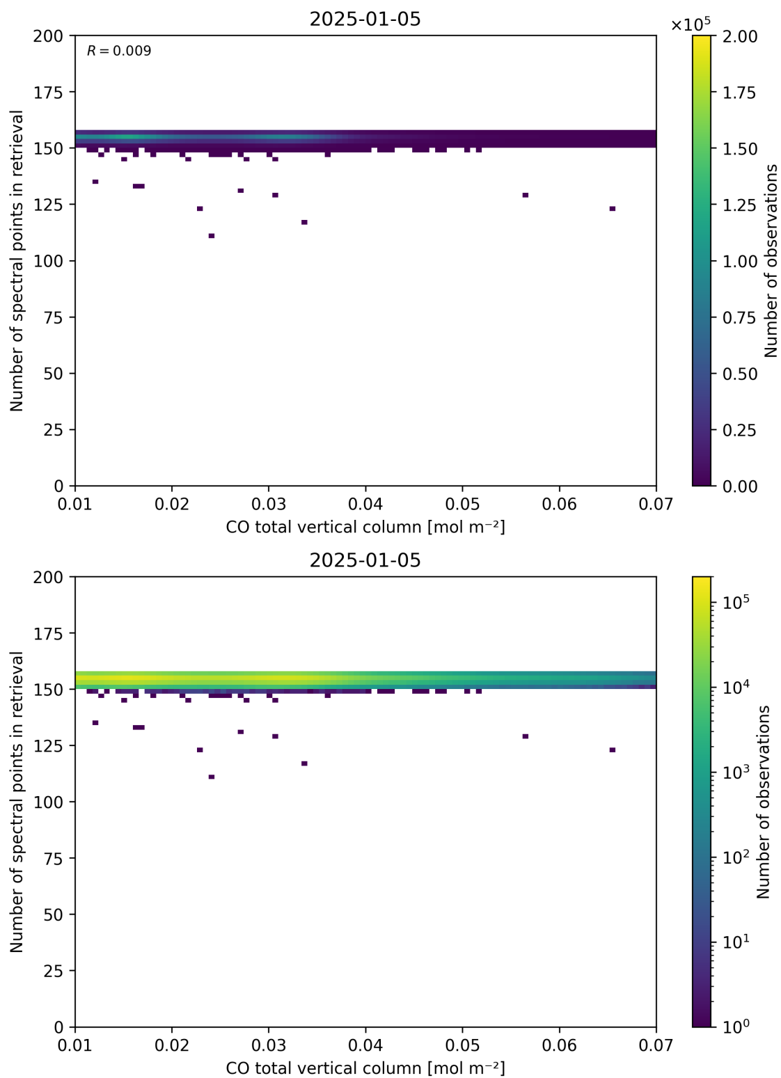
Figure 43: Scatter density plot of “CO total vertical column” against “Number of spectral points in retrieval” for 2025-01-04 to 2025-01-06.
