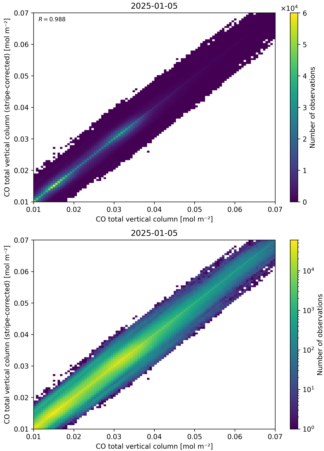
Figure 33: Scatter density plot of “CO total vertical column” against “CO total vertical column (stripe-corrected)” for 2025-01-04 to 2025-01-06.
