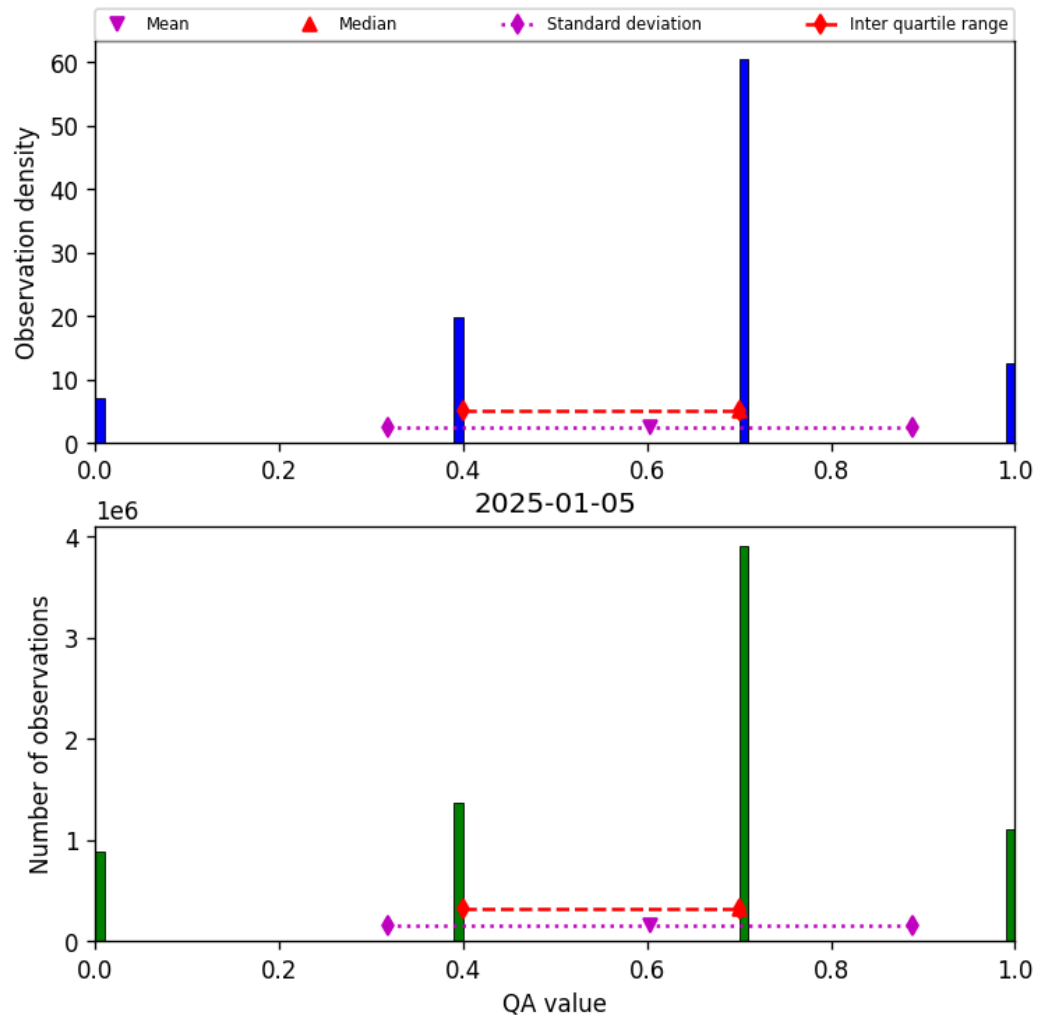
Figure 17: Histogram of "QA value" for 2025-01-04 to 2025-01-06
