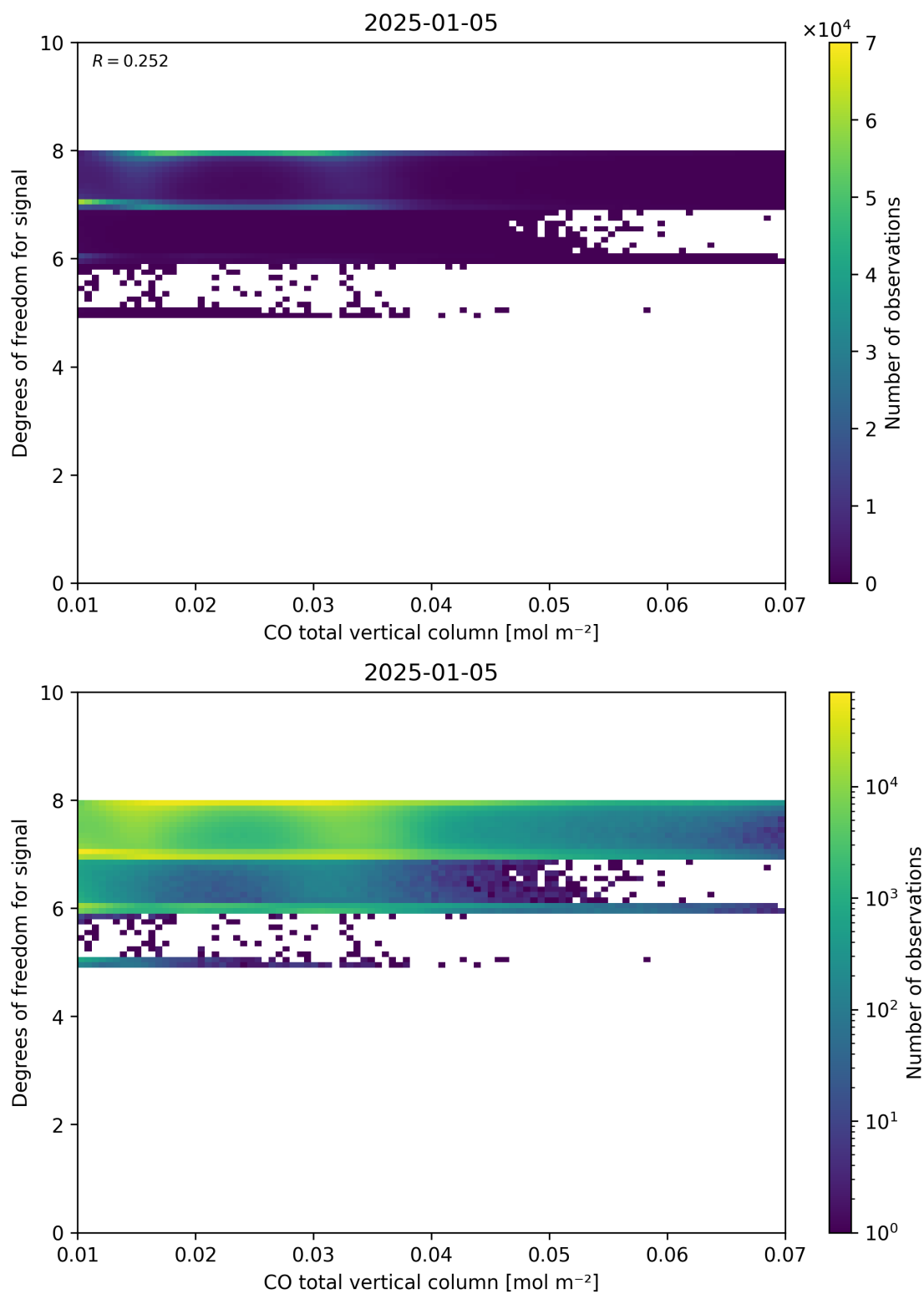
Figure 41: Scatter density plot of “CO total vertical column” against “Degrees of freedom for signal” for 2025-01-04 to 2025-01-06.
