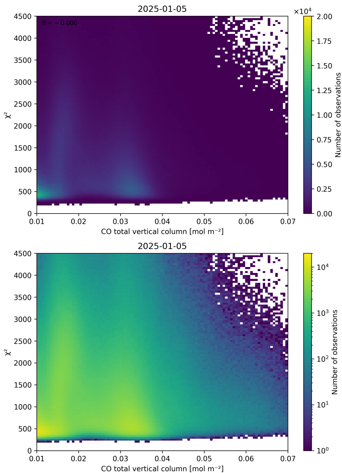
Figure 35: Scatter density plot of “CO total vertical column” against “ \chi^2 ” for 2025-01-04 to 2025-01-06.
