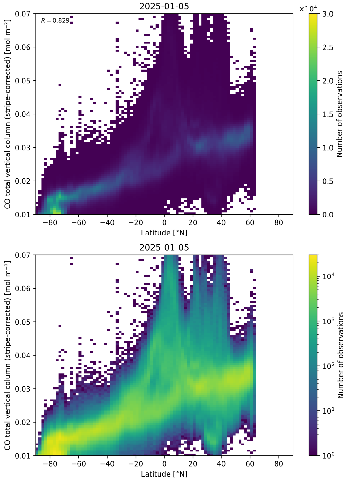
Figure 52: Scatter density plot of “Latitude” against “CO total vertical column (stripe-corrected)” for 2025-01-04 to 2025-01-06.
