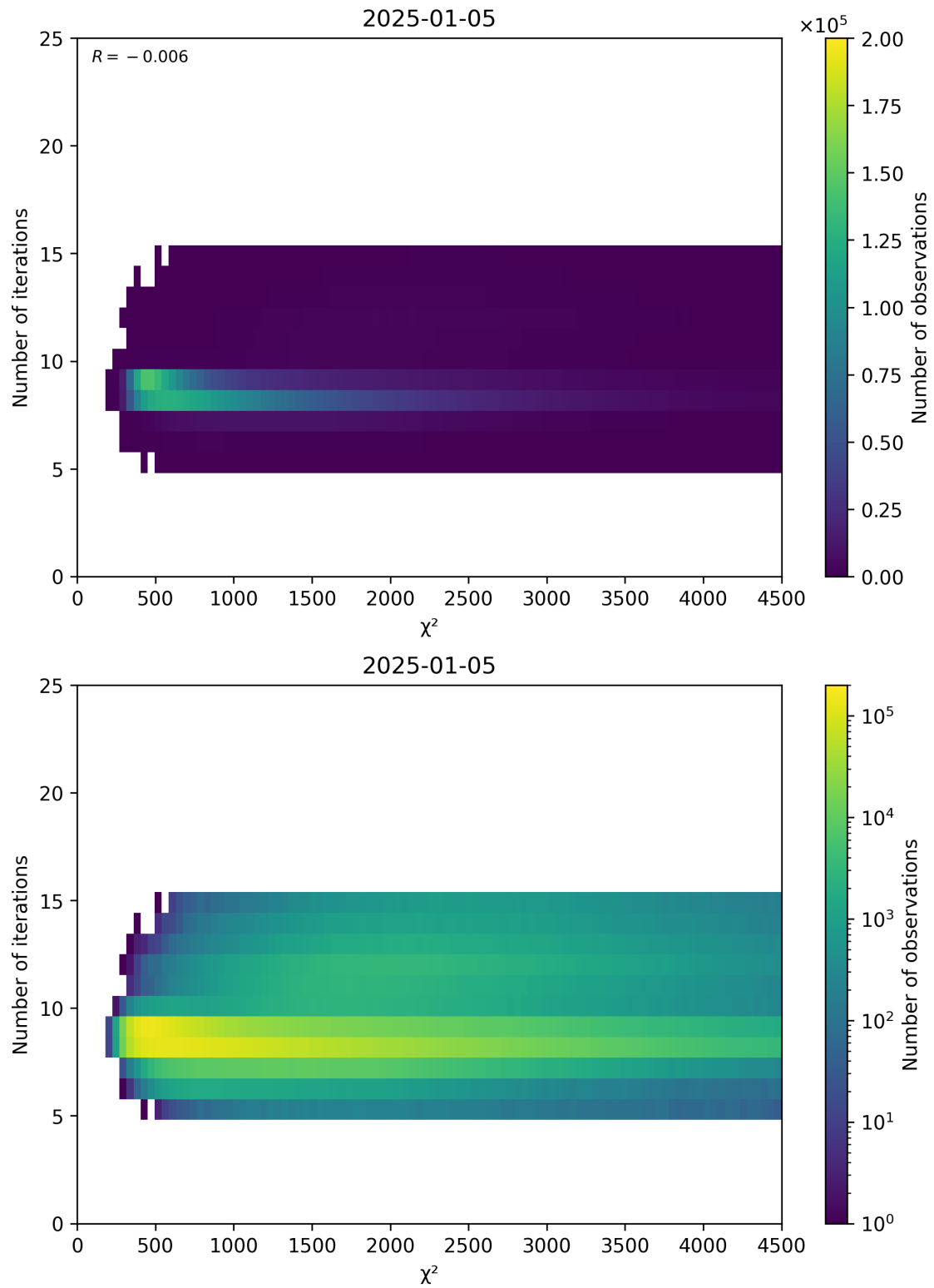
Figure 49: Scatter density plot of “ \chi^2 ” against “Number of iterations” for 2025-01-04 to 2025-01-06.
