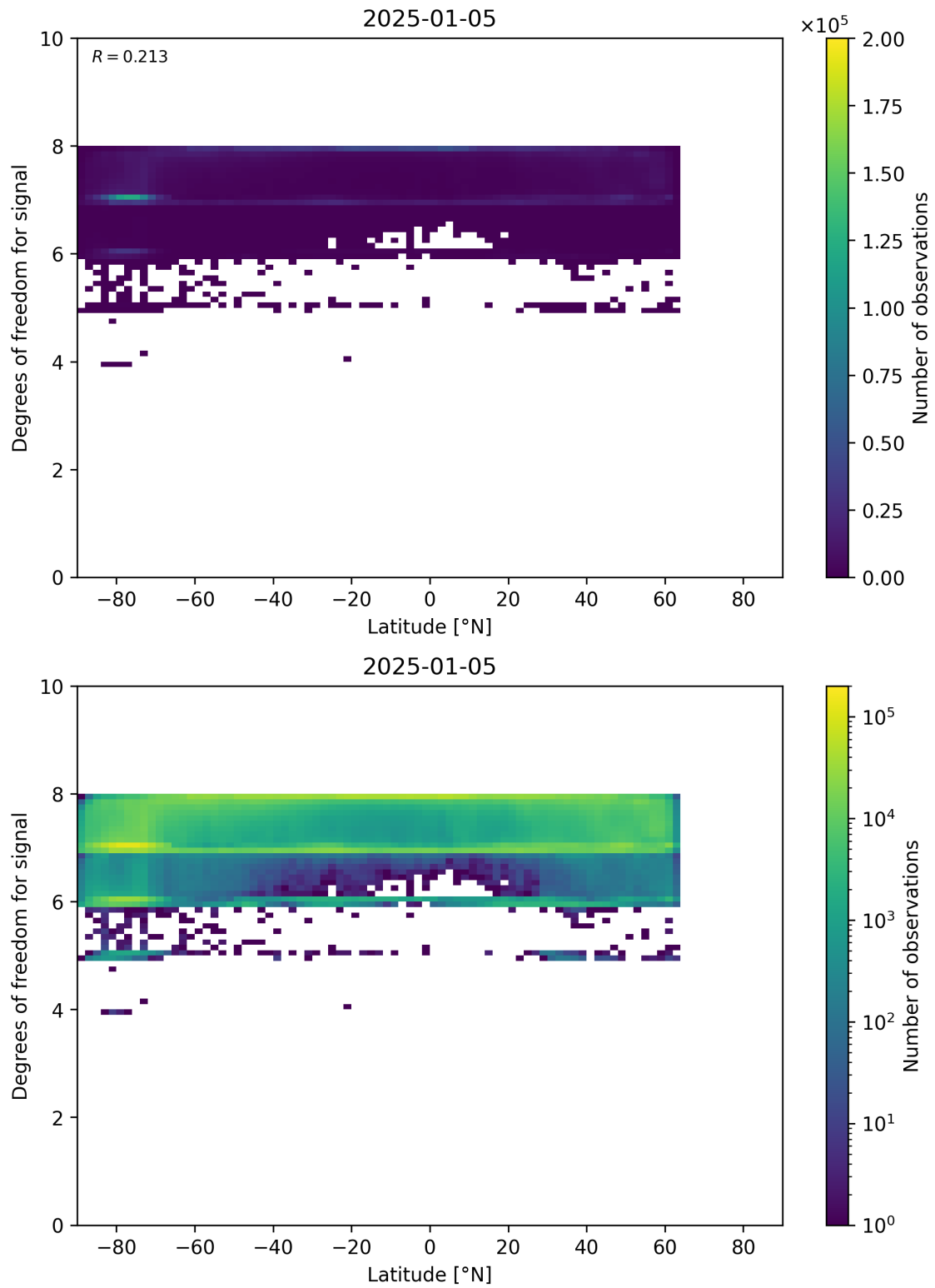
Figure 55: Scatter density plot of “Latitude” against “Degrees of freedom for signal” for 2025-01-04 to 2025-01-06.
