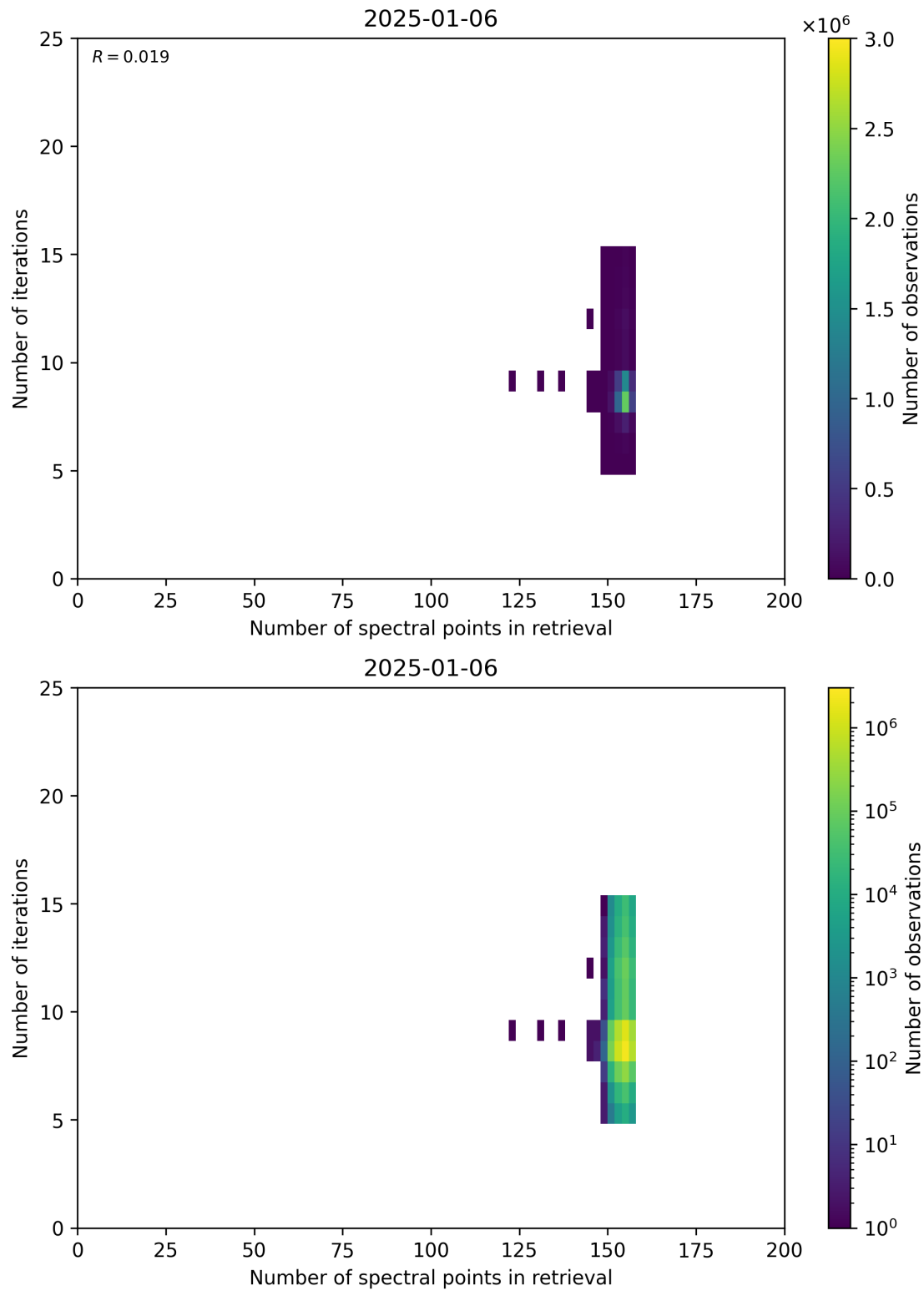
Figure 60: Scatter density plot of “Number of spectral points in retrieval” against “Number of iterations” for 2025-01-05 to 2025-01-07.
