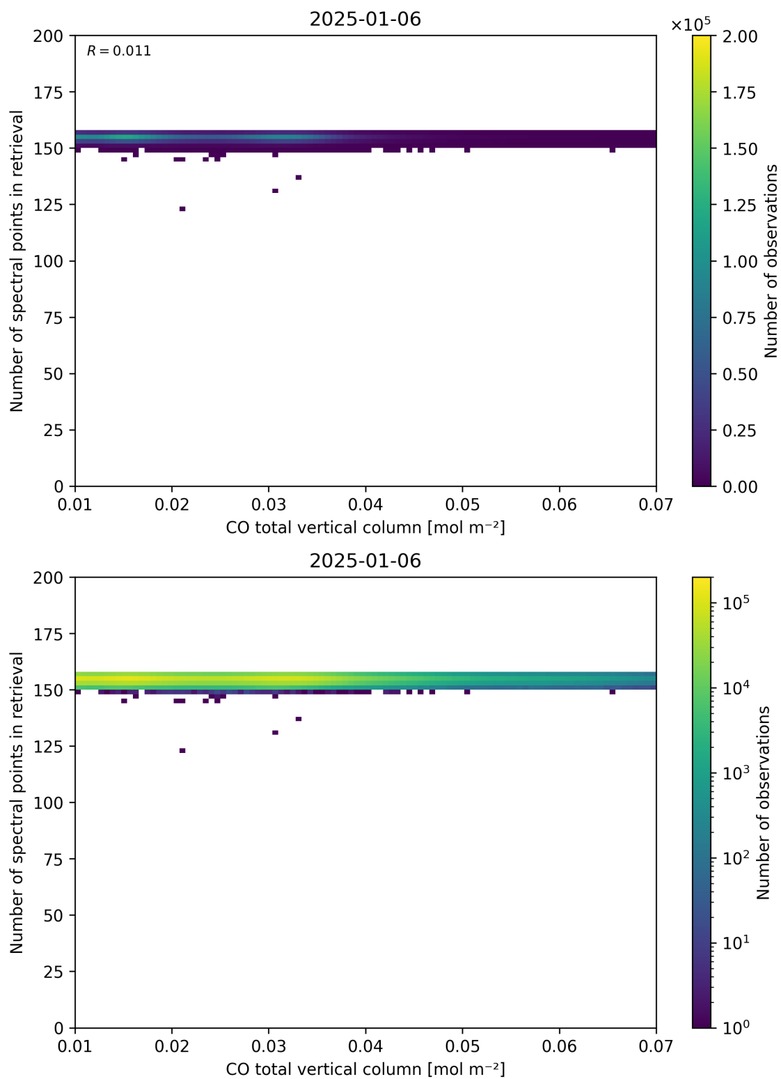
Figure 43: Scatter density plot of “CO total vertical column” against “Number of spectral points in retrieval” for 2025-01-05 to 2025-01-07.
