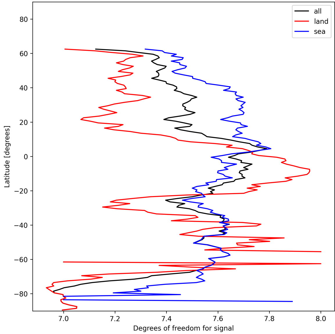
Figure 15: Zonal average of “Degrees of freedom for signal” for 2025-01-05 to 2025-01-07.
