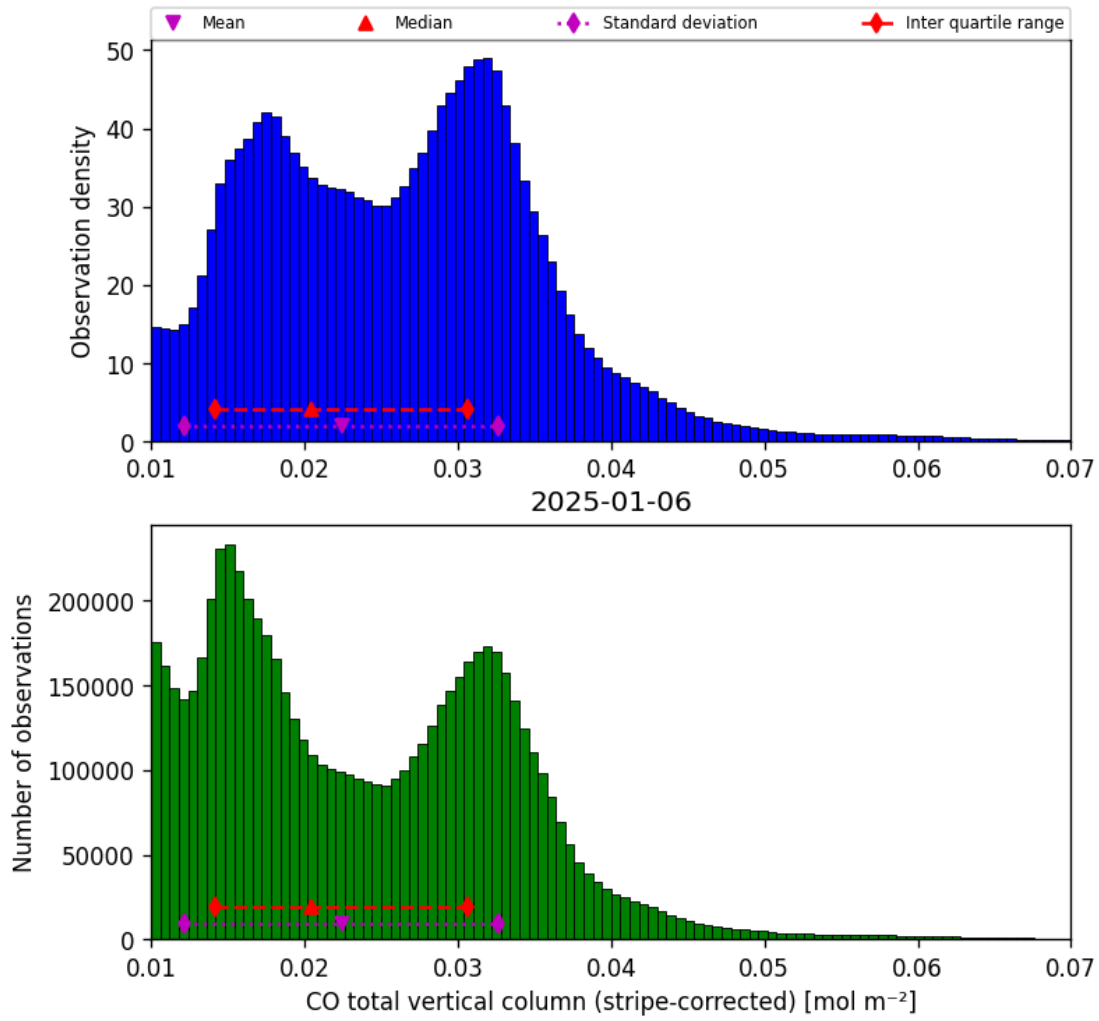
Figure 19: Histogram of “CO total vertical column (stripe-corrected)” for 2025-01-05 to 2025-01-07
