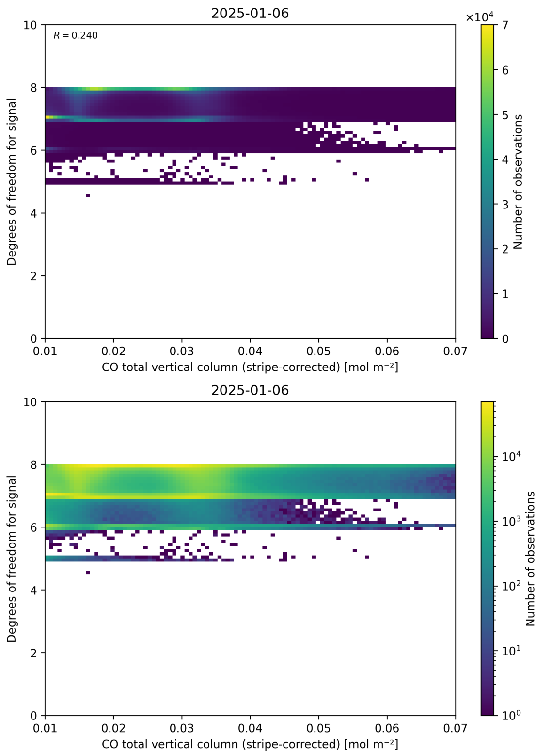
Figure 38: Scatter density plot of “CO total vertical column (stripe-corrected)” against “Degrees of freedom for signal” for 2025-01-05 to 2025-01-07.
