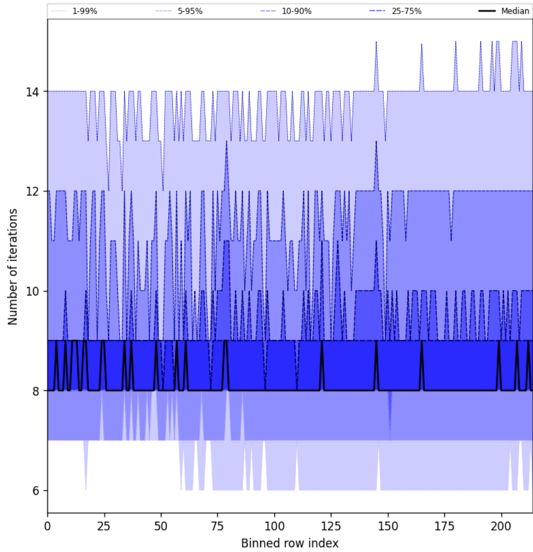
Figure 32: Along track statistics of “Number of iterations” for 2025-01-05 to 2025-01-07
