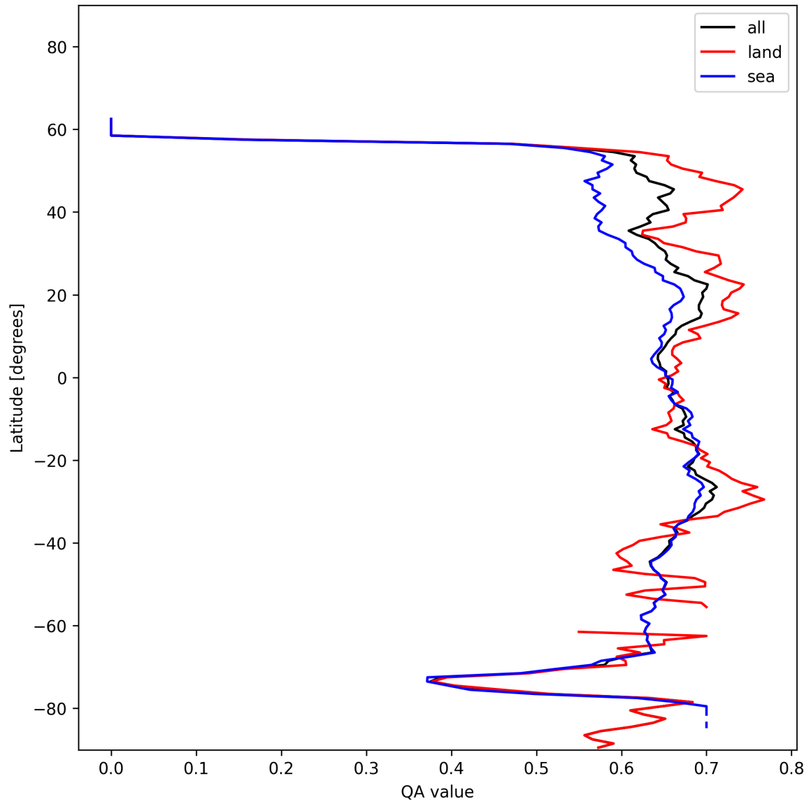
Figure 9: Zonal average of “QA value” for 2025-01-05 to 2025-01-07.
