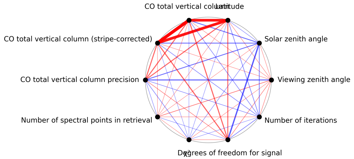
Figure 1: Map of correlation graph for 2025-01-05 to 2025-01-07.
