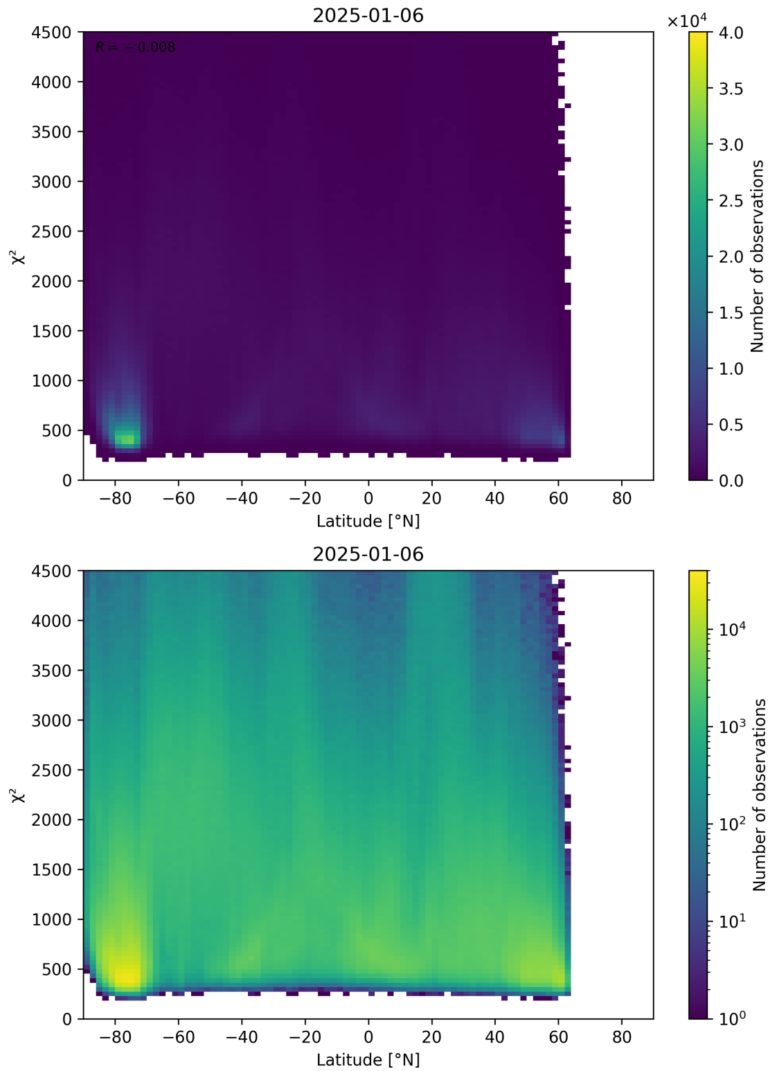
Figure 54: Scatter density plot of “Latitude” against “ \chi^2 ” for 2025-01-05 to 2025-01-07.
