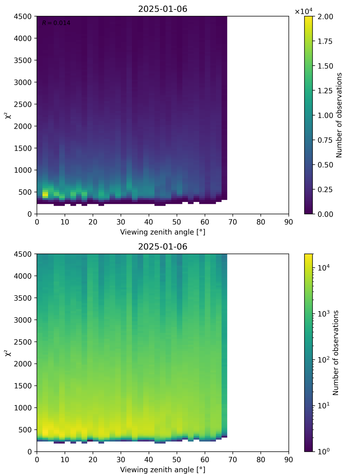
Figure 72: Scatter density plot of “Viewing zenith angle” against “ \chi^2 ” for 2025-01-05 to 2025-01-07.
