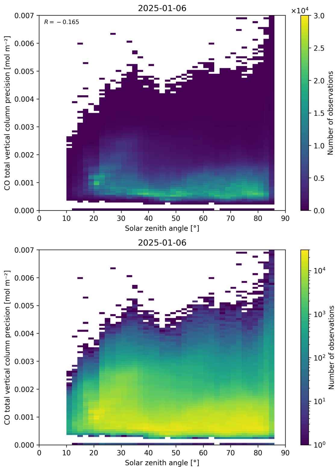
Figure 63: Scatter density plot of “Solar zenith angle” against “CO total vertical column precision” for 2025-01-05 to 2025-01-07.
