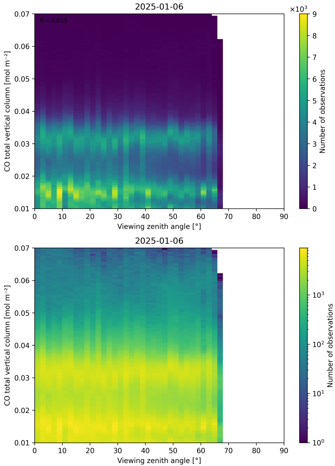
Figure 69: Scatter density plot of “Viewing zenith angle” against “CO total vertical column” for 2025-01-05 to 2025-01-07.
