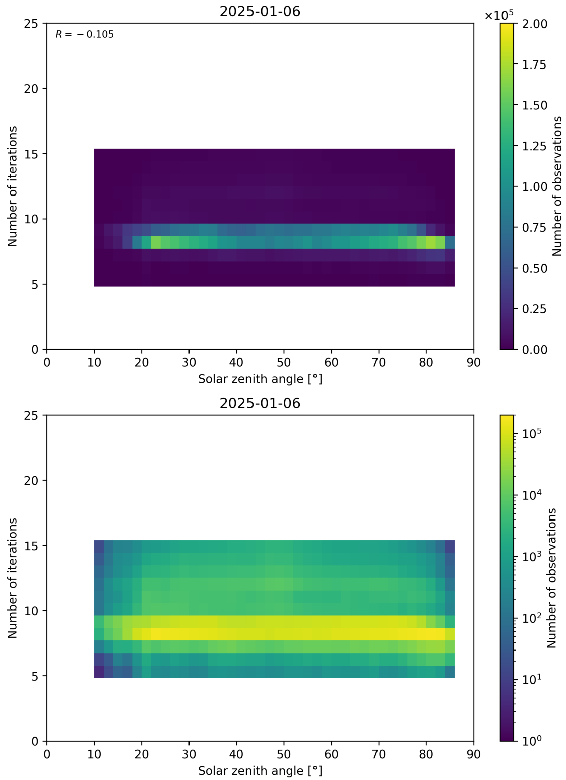
Figure 67: Scatter density plot of “Solar zenith angle” against “Number of iterations” for 2025-01-05 to 2025-01-07.
