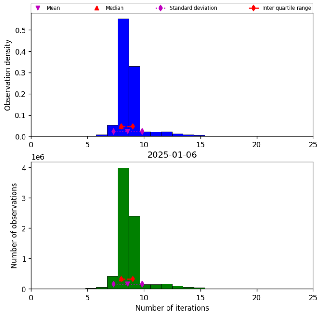
Figure 24: Histogram of “Number of iterations” for 2025-01-05 to 2025-01-07
