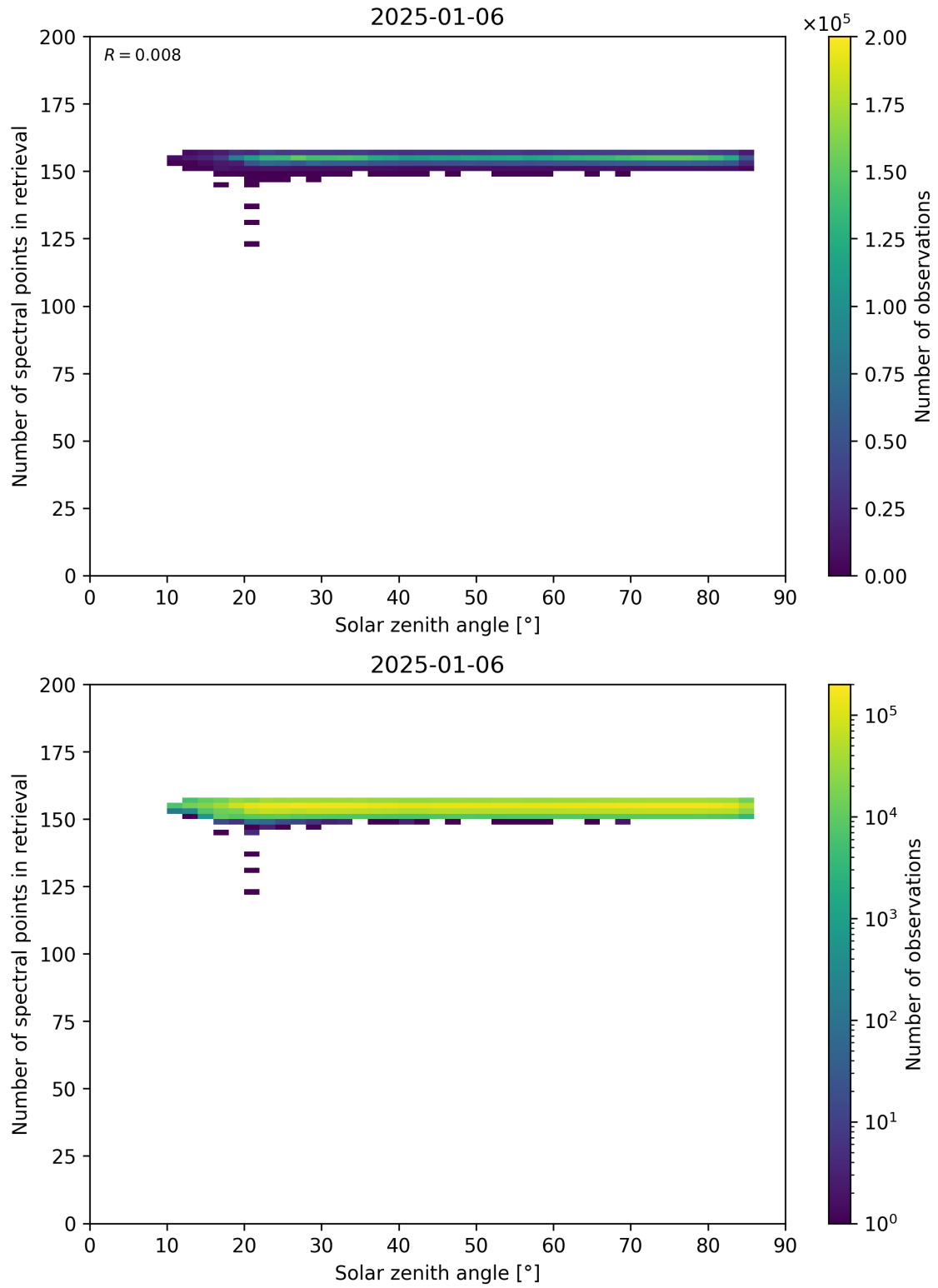
Figure 68: Scatter density plot of “Solar zenith angle” against “Number of spectral points in retrieval” for 2025-01-05 to 2025-01-07.
