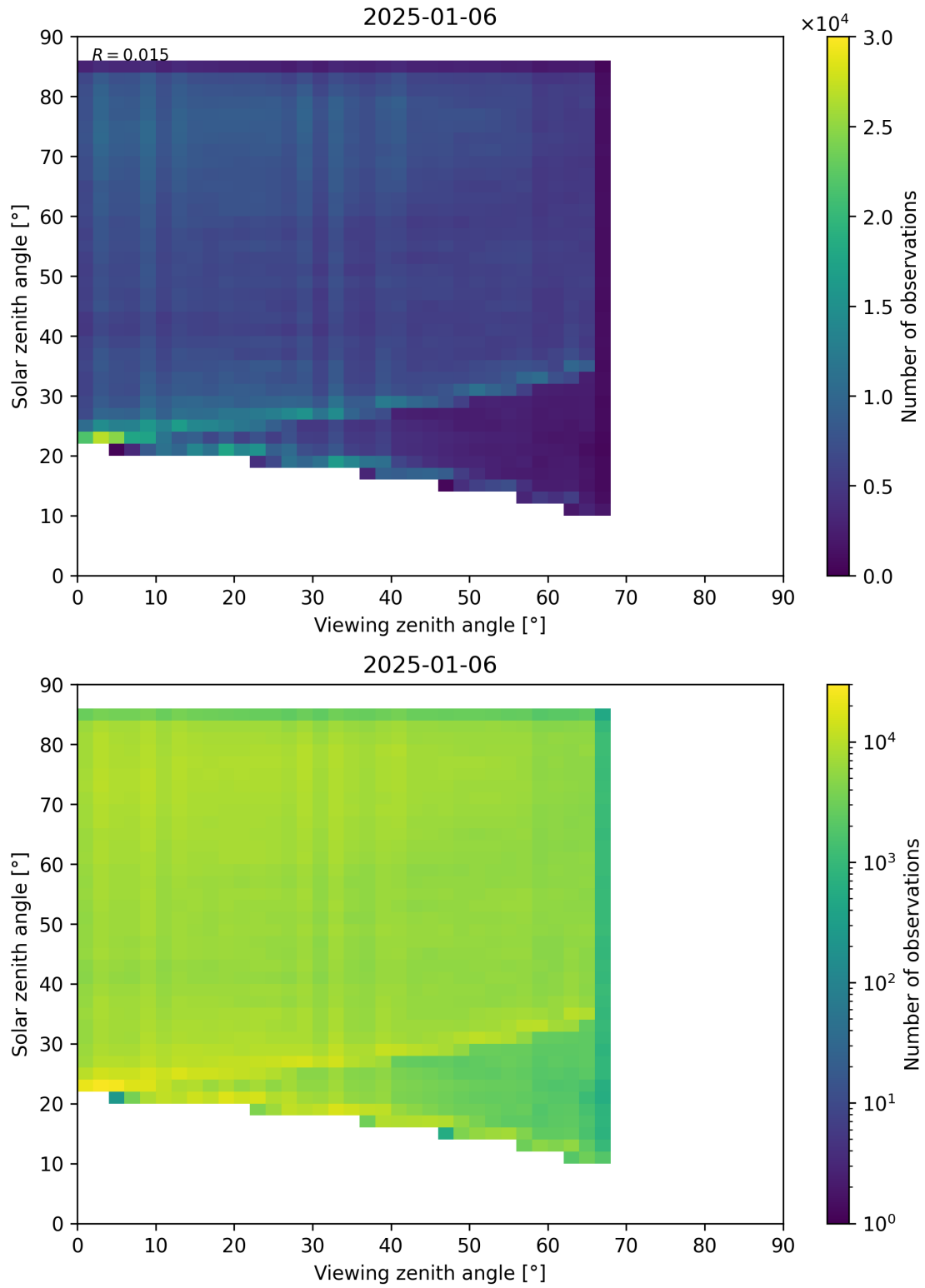
Figure 77: Scatter density plot of “Viewing zenith angle” against “Solar zenith angle” for 2025-01-05 to 2025-01-07.
