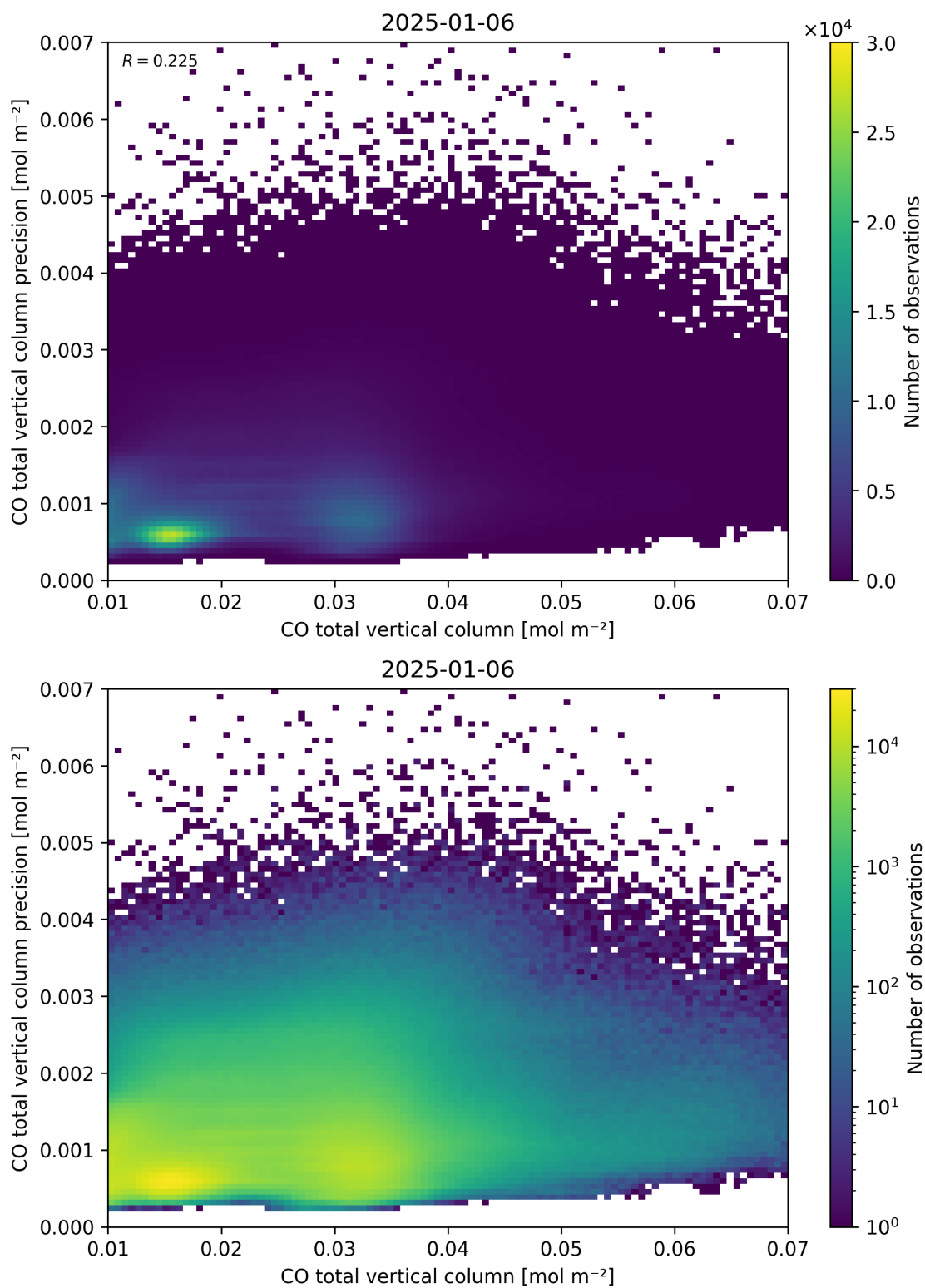
Figure 34: Scatter density plot of “CO total vertical column” against “CO total vertical column precision” for 2025-01-05 to 2025-01-07.
