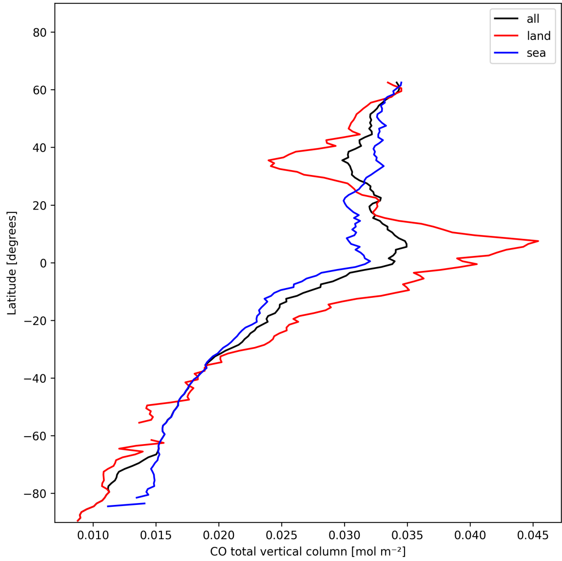
Figure 10: Zonal average of “CO total vertical column” for 2025-01-05 to 2025-01-07.
