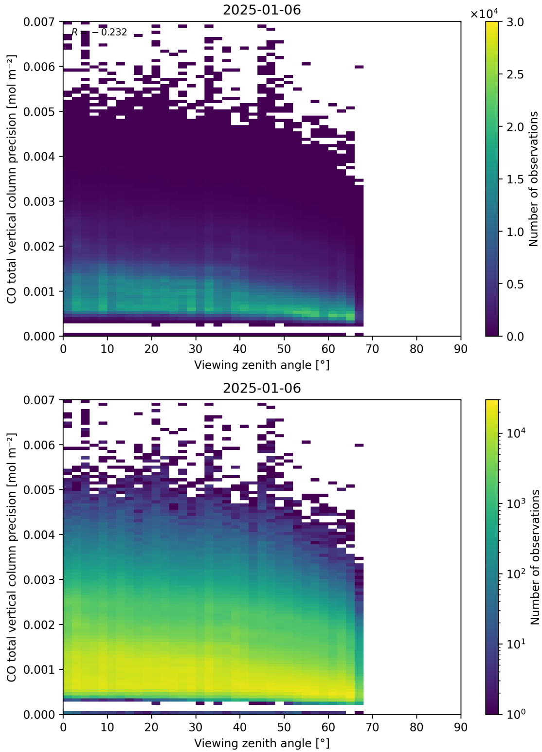
Figure 71: Scatter density plot of “Viewing zenith angle” against “CO total vertical column precision” for 2025-01-05 to 2025-01-07.
