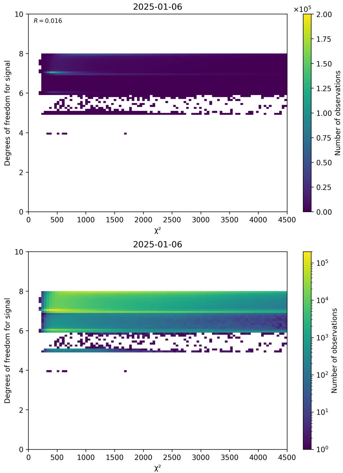
Figure 48: Scatter density plot of “ \chi^2 ” against “Degrees of freedom for signal” for 2025-01-05 to 2025-01-07.
