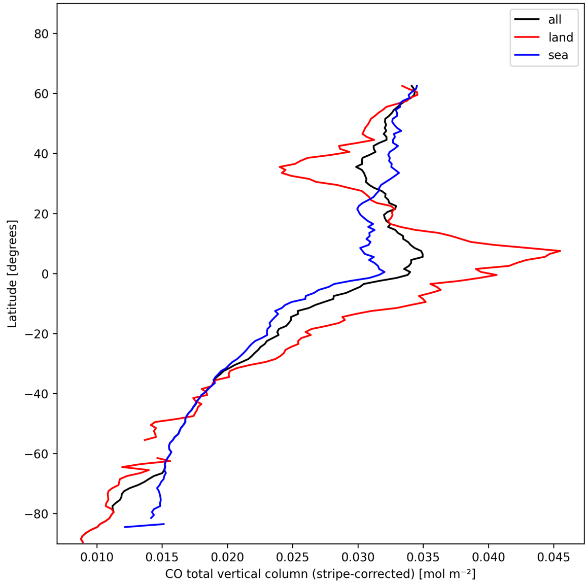
Figure 11: Zonal average of “CO total vertical column (stripe-corrected)” for 2025-01-05 to 2025-01-07.
