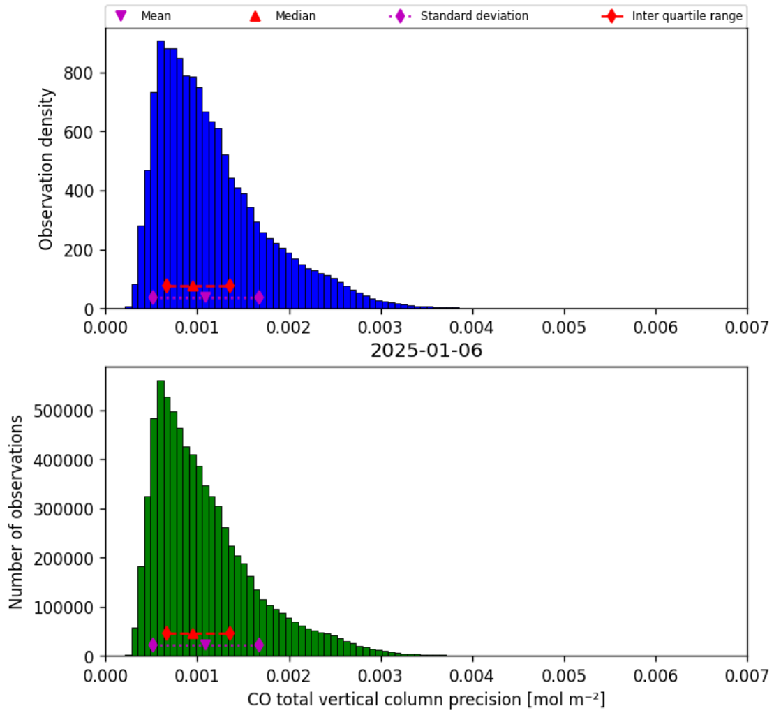
Figure 20: Histogram of “CO total vertical column precision” for 2025-01-05 to 2025-01-07
