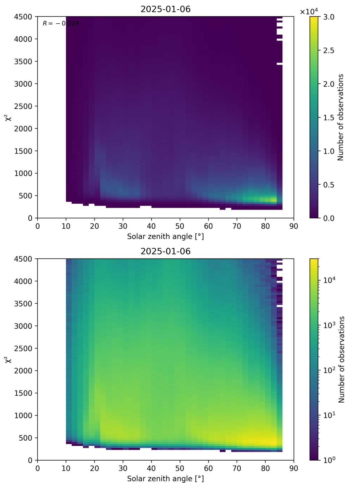
Figure 64: Scatter density plot of “Solar zenith angle” against “ \chi^2 ” for 2025-01-05 to 2025-01-07.
