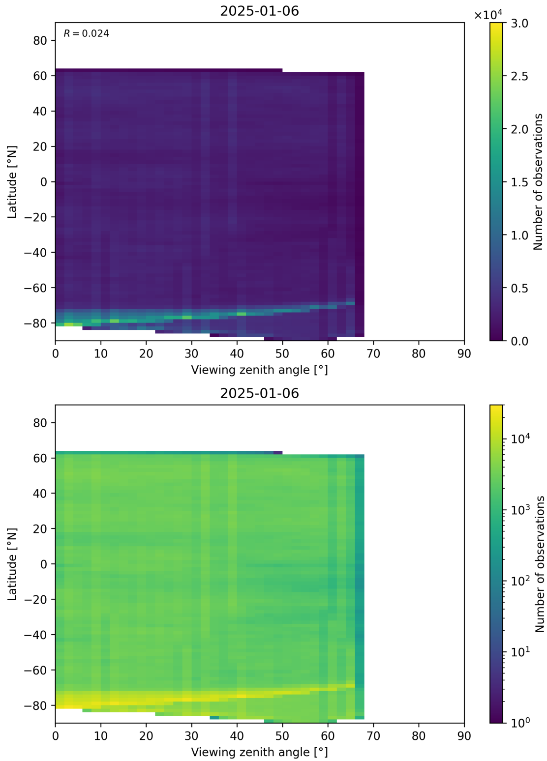
Figure 74: Scatter density plot of “Viewing zenith angle” against “Latitude” for 2025-01-05 to 2025-01-07.
