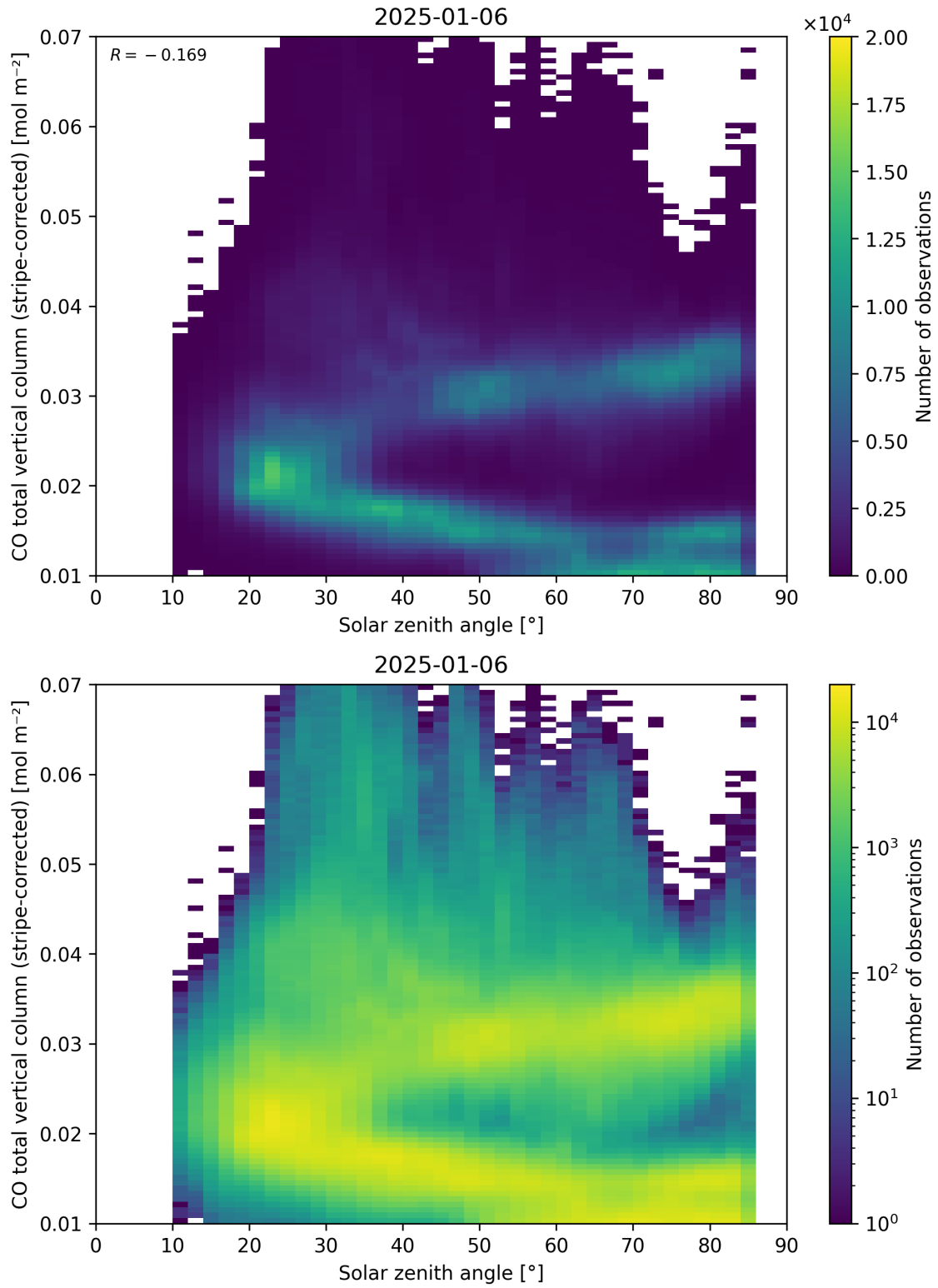
Figure 62: Scatter density plot of “Solar zenith angle” against “CO total vertical column (stripe-corrected)” for 2025-01-05 to 2025-01-07.
