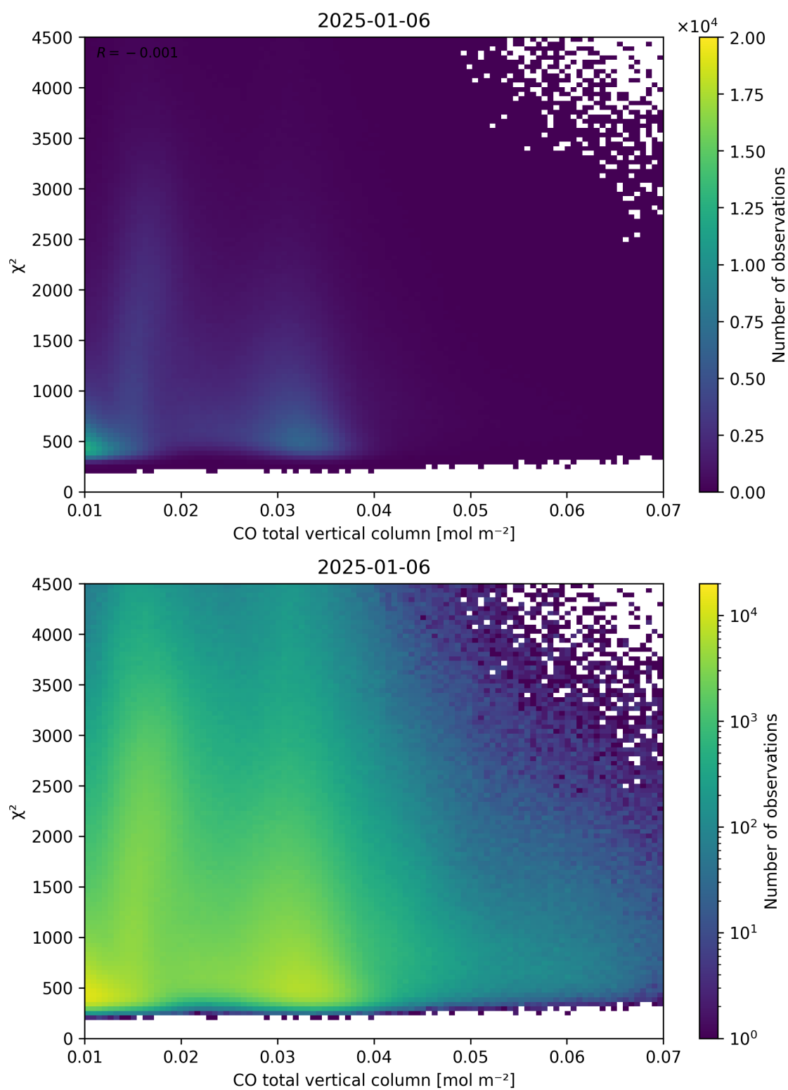
Figure 35: Scatter density plot of “CO total vertical column” against “ \chi^2 ” for 2025-01-05 to 2025-01-07.
