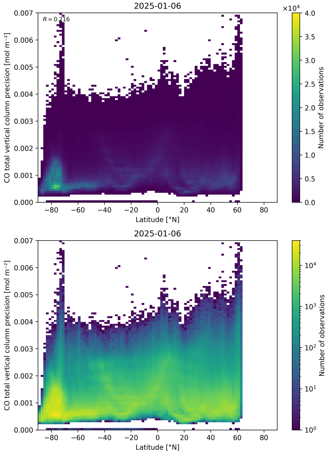
Figure 53: Scatter density plot of “Latitude” against “CO total vertical column precision” for 2025-01-05 to 2025-01-07.
