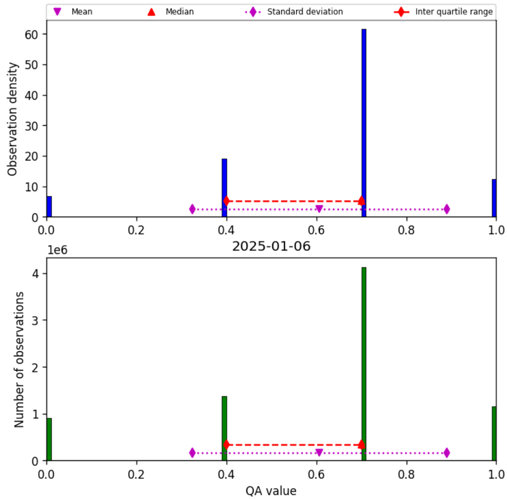
Figure 17: Histogram of “QA value” for 2025-01-05 to 2025-01-07
