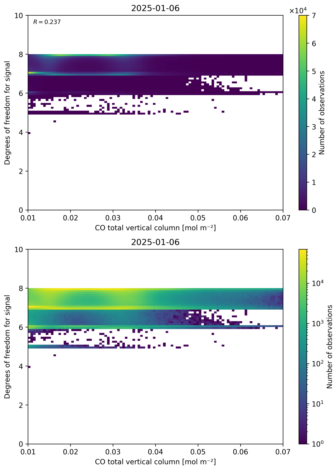
Figure 41: Scatter density plot of “CO total vertical column” against “Degrees of freedom for signal” for 2025-01-05 to 2025-01-07.
