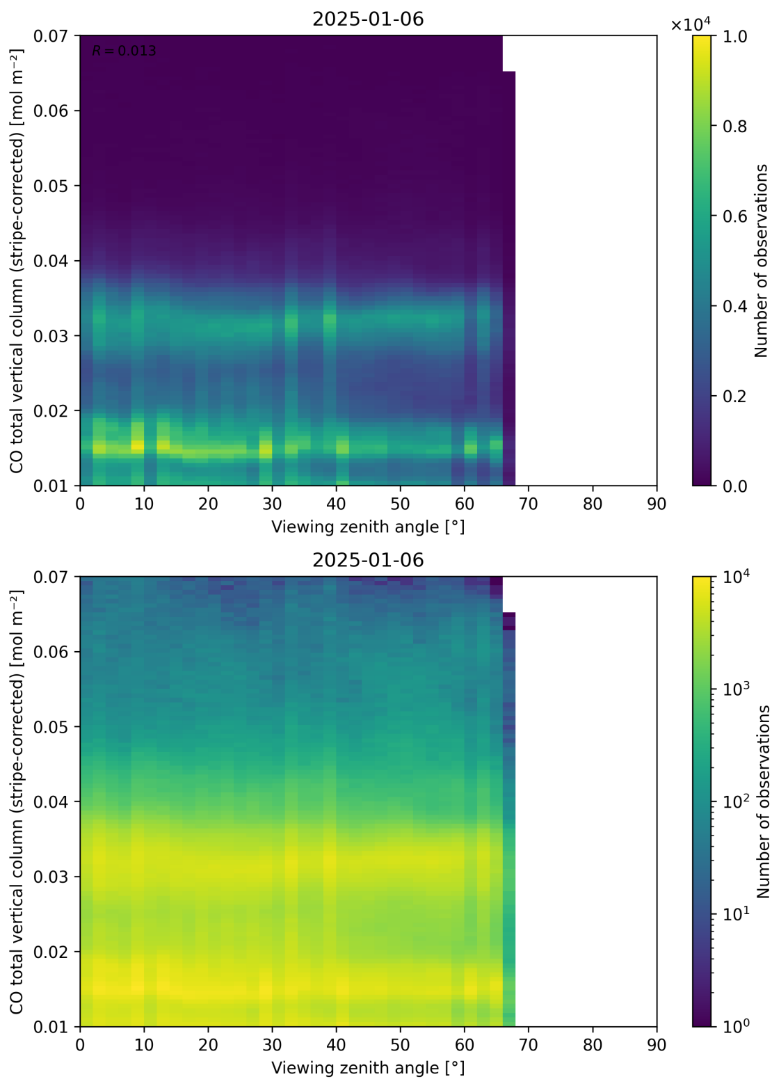
Figure 70: Scatter density plot of “Viewing zenith angle” against “CO total vertical column (stripe-corrected)” for 2025-01-05 to 2025-01-07.
