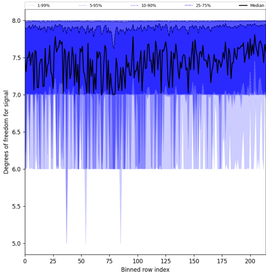
Figure 31: Along track statistics of “Degrees of freedom for signal” for 2025-01-05 to 2025-01-07
