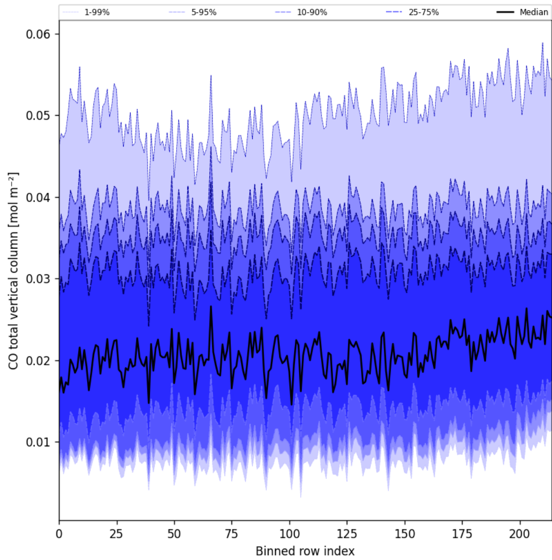
Figure 26: Along track statistics of “CO total vertical column” for 2025-01-05 to 2025-01-07
