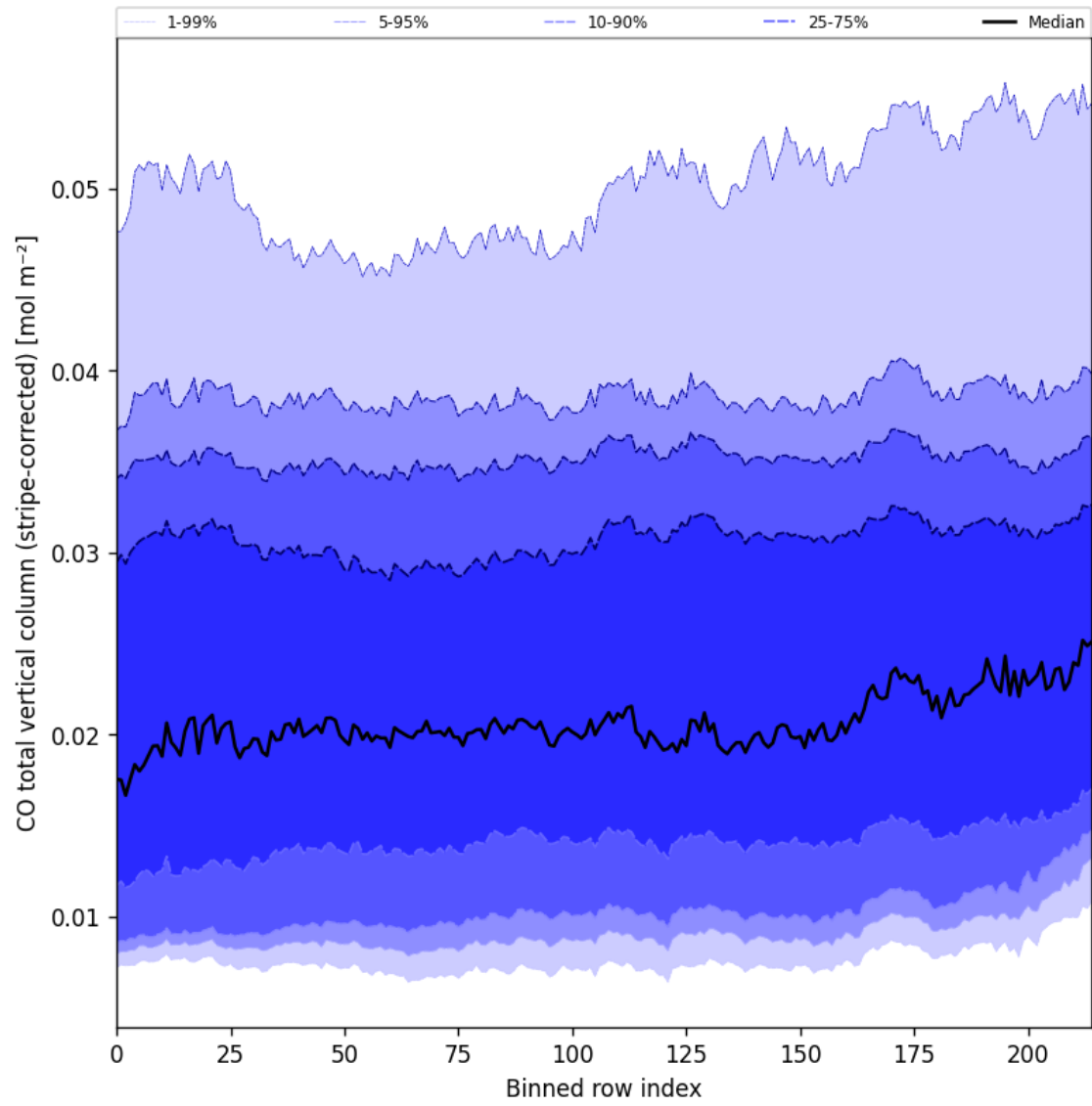
Figure 27: Along track statistics of “CO total vertical column (stripe-corrected)” for 2025-01-05 to 2025-01-07
