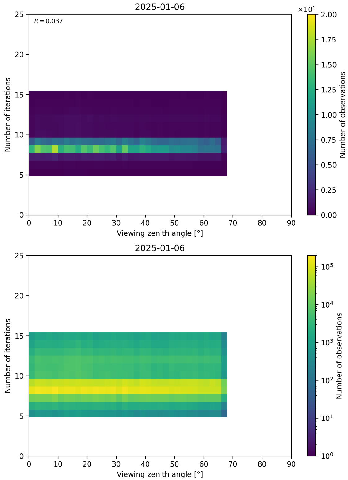
Figure 75: Scatter density plot of “Viewing zenith angle” against “Number of iterations” for 2025-01-05 to 2025-01-07.
