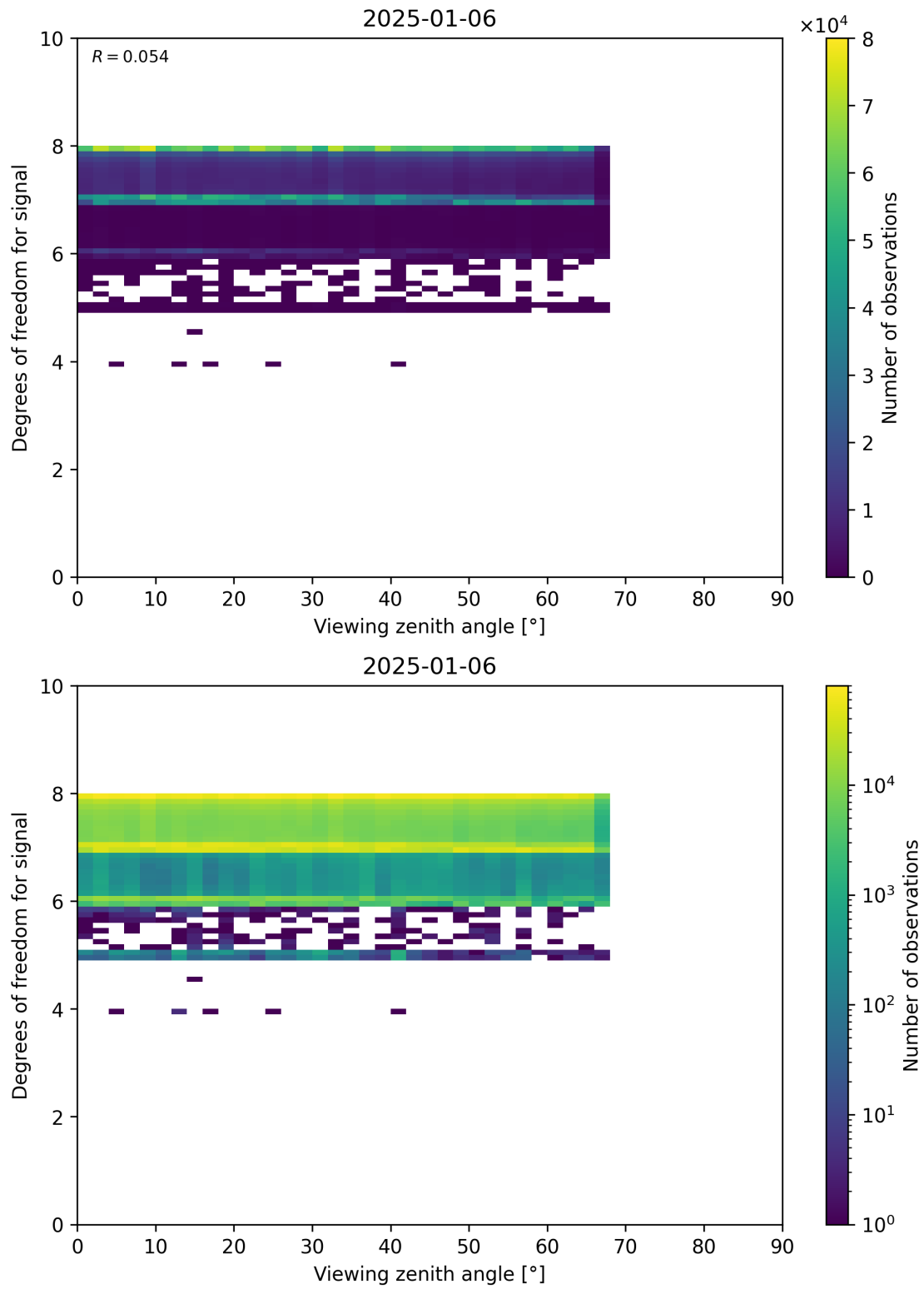
Figure 73: Scatter density plot of “Viewing zenith angle” against “Degrees of freedom for signal” for 2025-01-05 to 2025-01-07.
