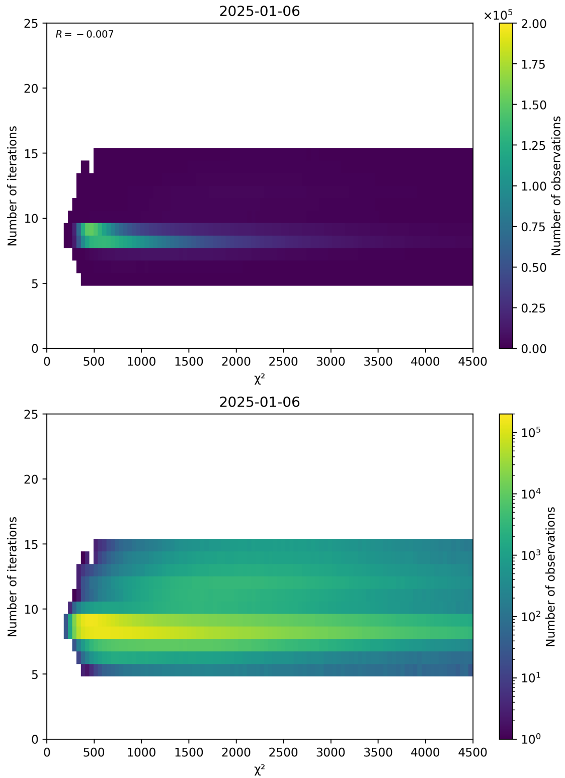
Figure 49: Scatter density plot of “ \chi^2 ” against “Number of iterations” for 2025-01-05 to 2025-01-07.
