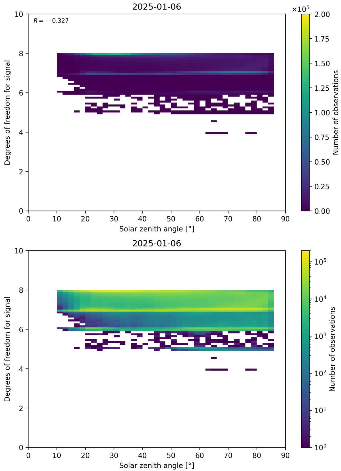
Figure 65: Scatter density plot of “Solar zenith angle” against “Degrees of freedom for signal” for 2025-01-05 to 2025-01-07.
