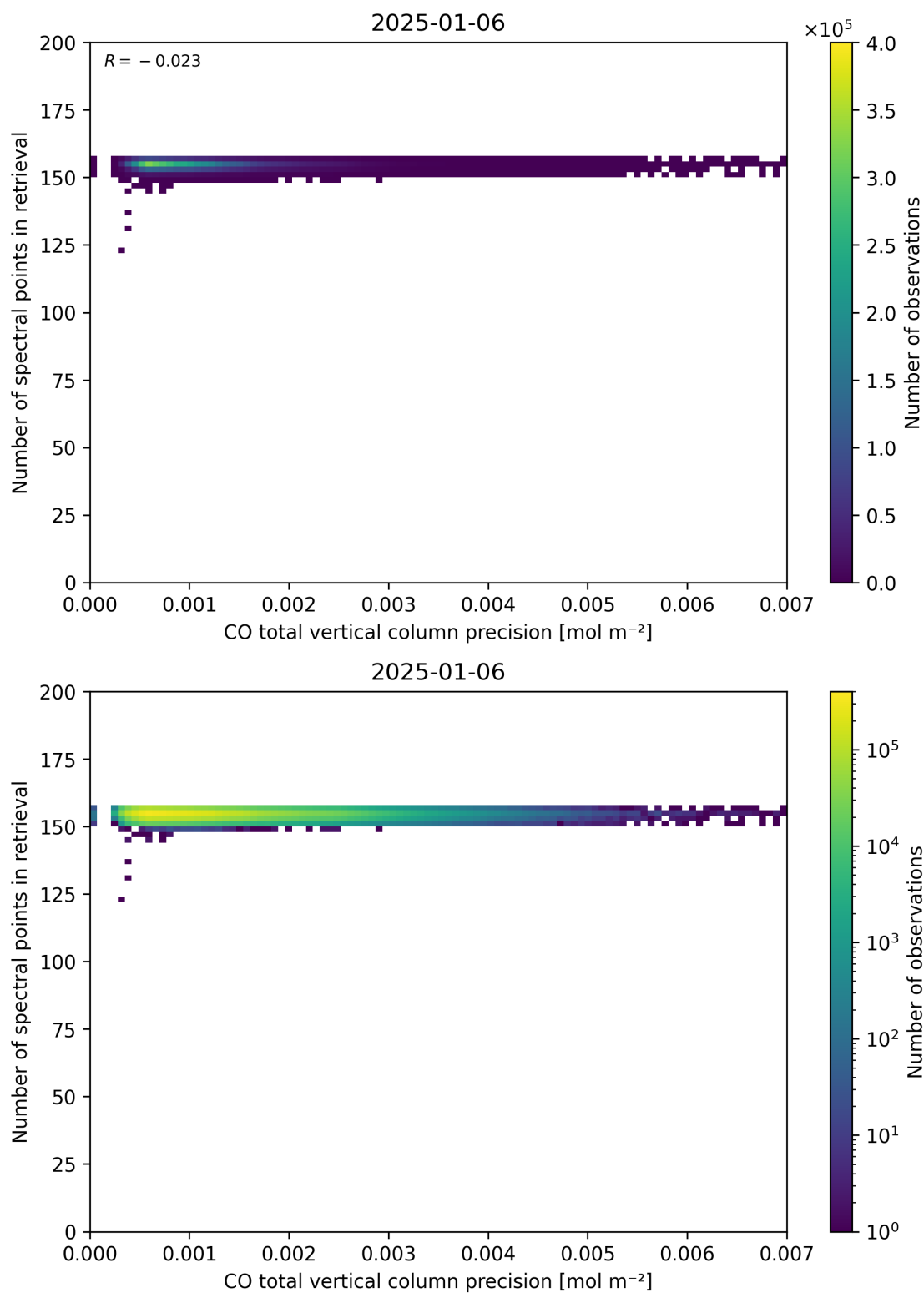
Figure 47: Scatter density plot of “CO total vertical column precision” against “Number of spectral points in retrieval” for 2025-01-05 to 2025-01-07.
