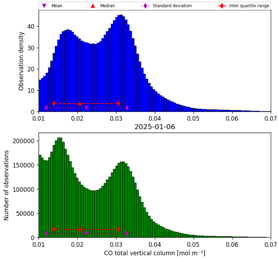
Figure 18: Histogram of “CO total vertical column” for 2025-01-05 to 2025-01-07
