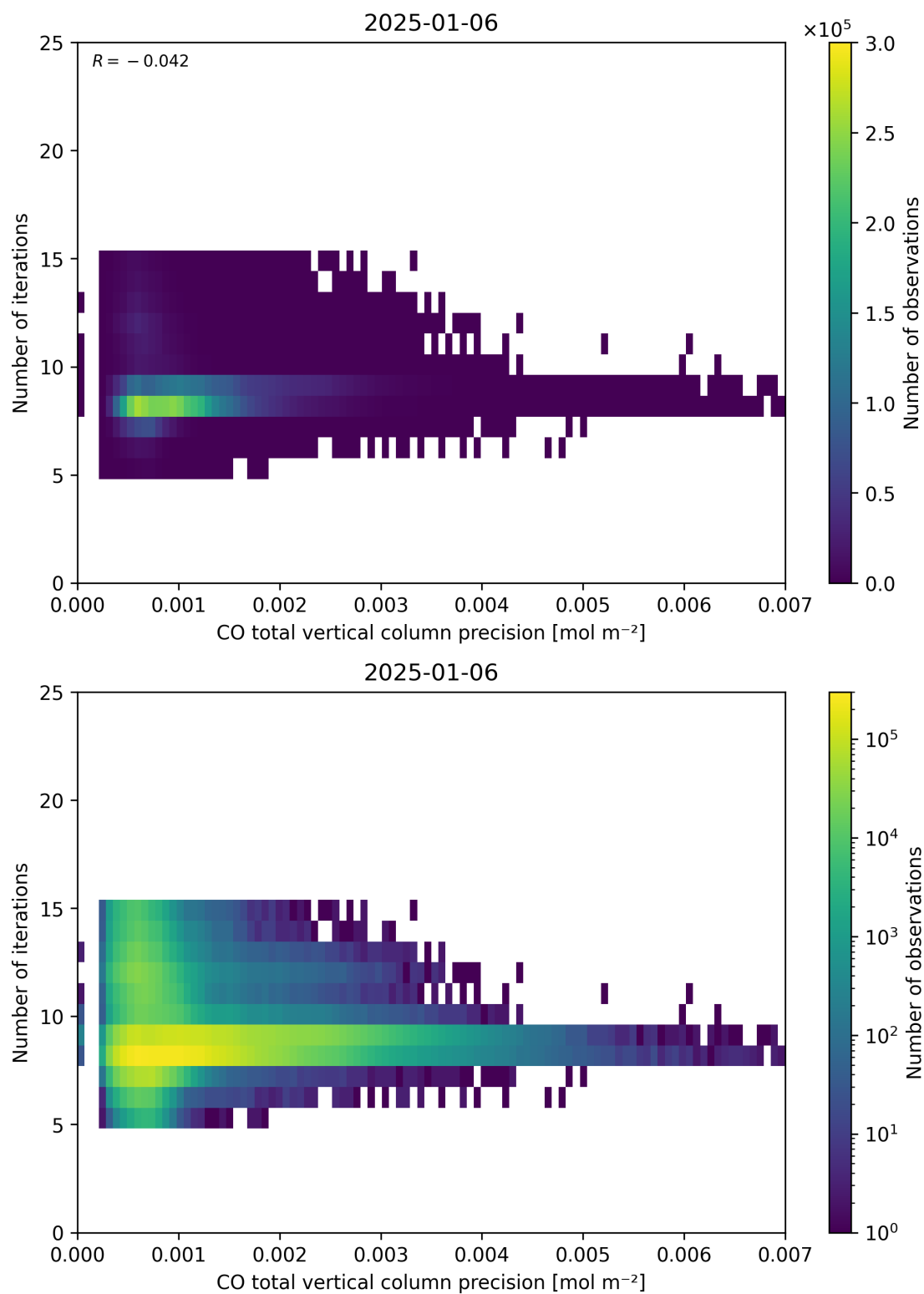
Figure 46: Scatter density plot of “CO total vertical column precision” against “Number of iterations” for 2025-01-05 to 2025-01-07.
