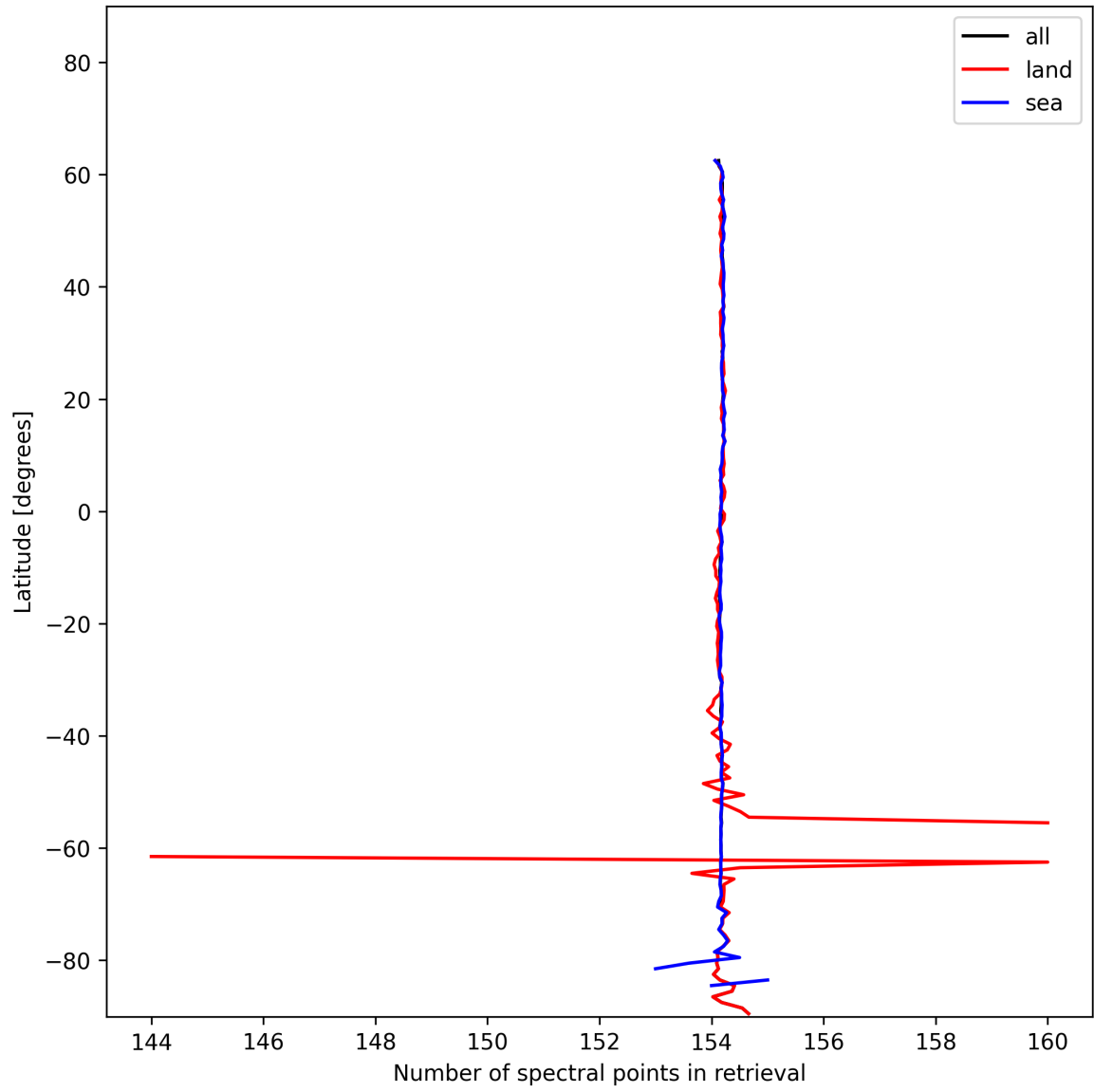
Figure 13: Zonal average of “Number of spectral points in retrieval” for 2025-01-05 to 2025-01-07.
