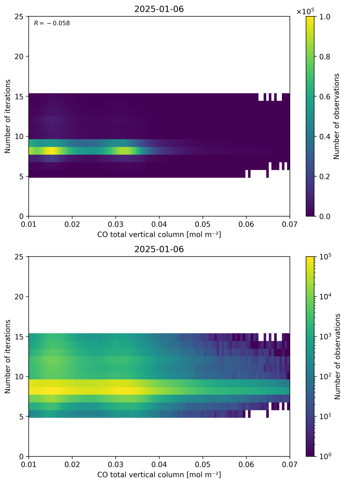
Figure 42: Scatter density plot of “CO total vertical column” against “Number of iterations” for 2025-01-05 to 2025-01-07.
