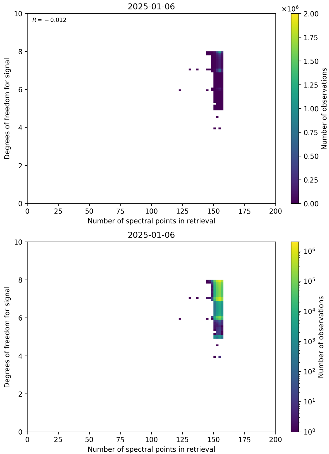
Figure 59: Scatter density plot of “Number of spectral points in retrieval” against “Degrees of freedom for signal” for 2025-01-05 to 2025-01-07.
