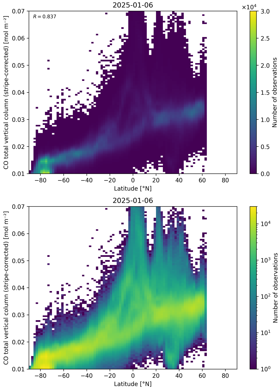
Figure 52: Scatter density plot of “Latitude” against “CO total vertical column (stripe-corrected)” for 2025-01-05 to 2025-01-07.
