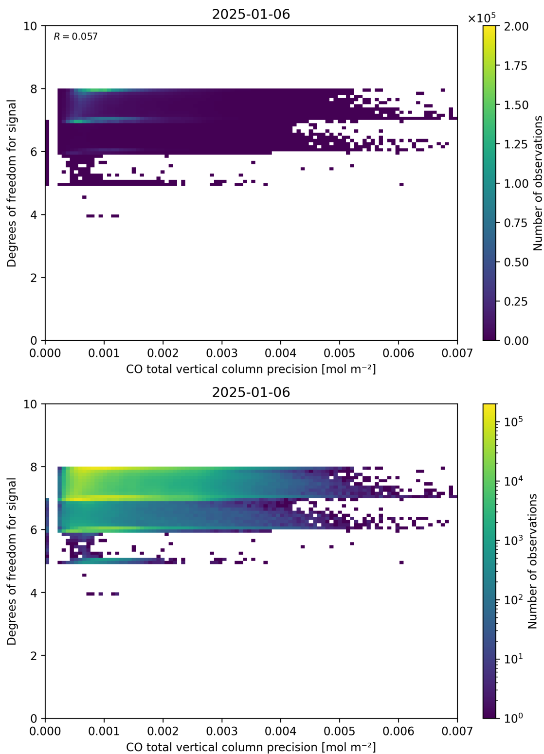
Figure 45: Scatter density plot of “CO total vertical column precision” against “Degrees of freedom for signal” for 2025-01-05 to 2025-01-07.
