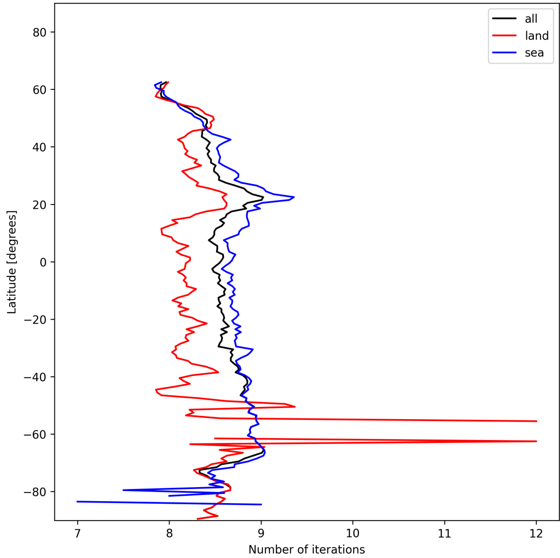
Figure 16: Zonal average of “Number of iterations” for 2025-01-05 to 2025-01-07.
