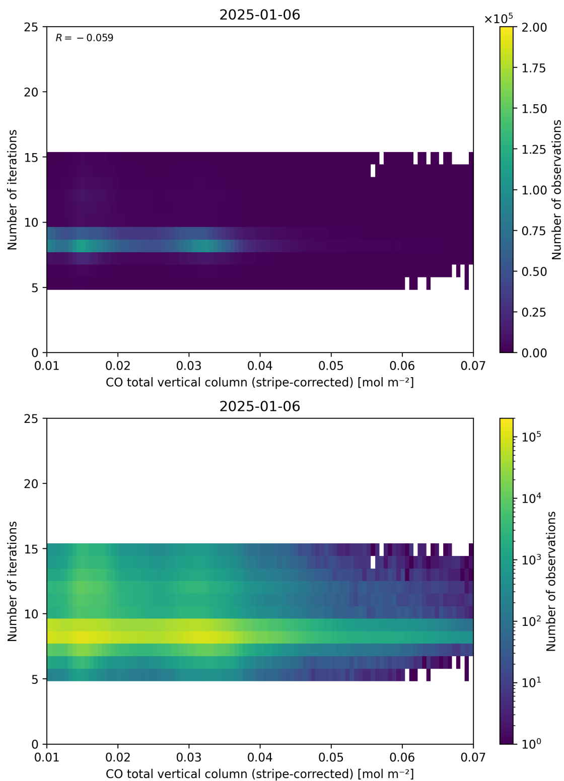
Figure 39: Scatter density plot of “CO total vertical column (stripe-corrected)” against “Number of iterations” for 2025-01-05 to 2025-01-07.
