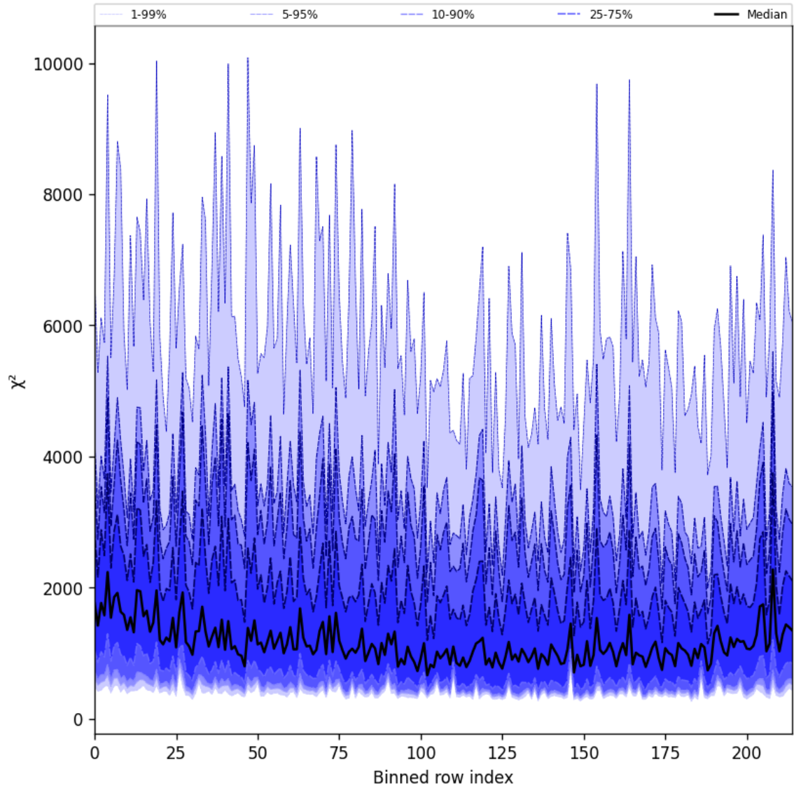
Figure 30: Along track statistics of “ \chi^2 ” for 2025-01-05 to 2025-01-07
