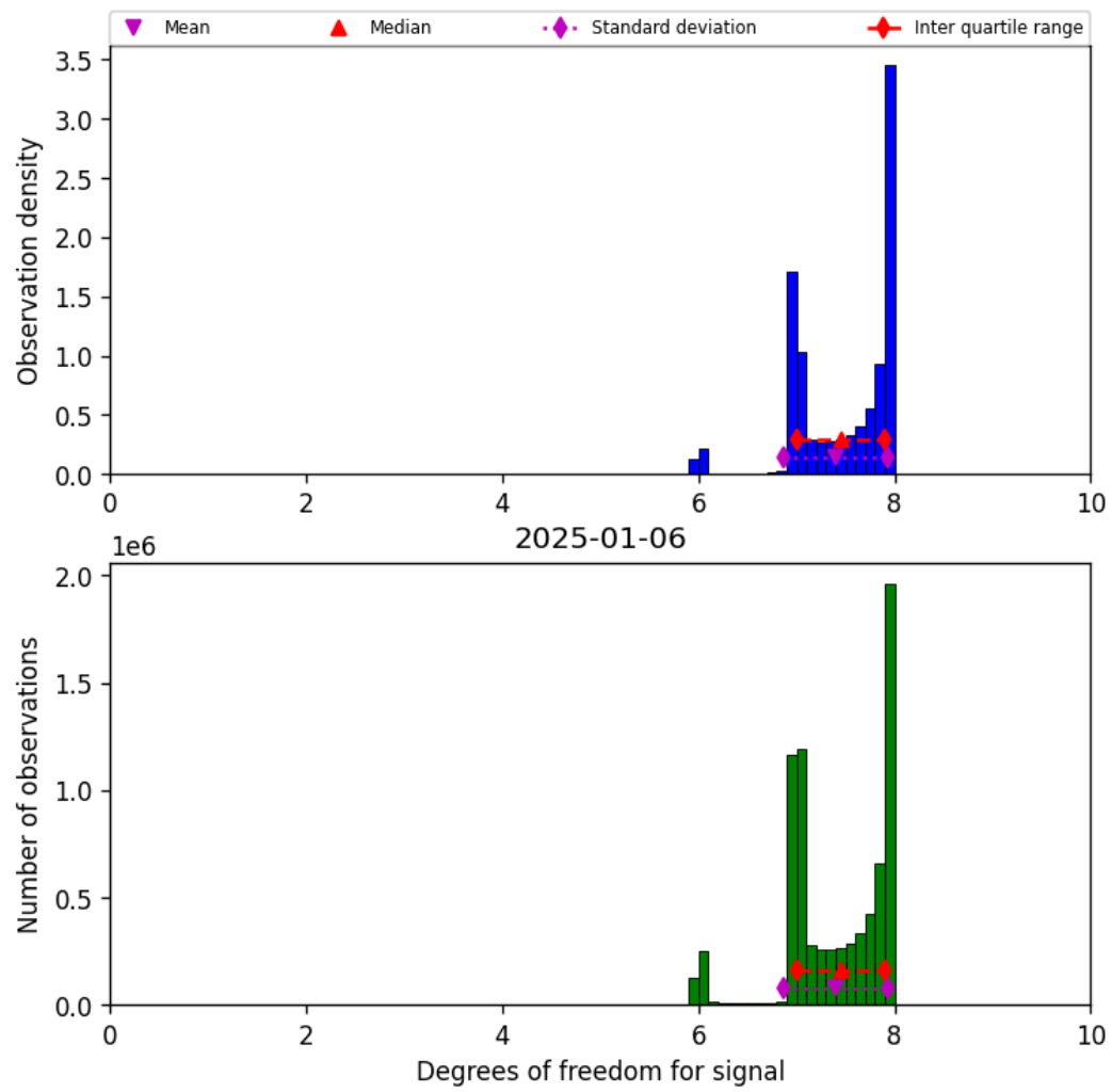
Figure 23: Histogram of “Degrees of freedom for signal” for 2025-01-05 to 2025-01-07
