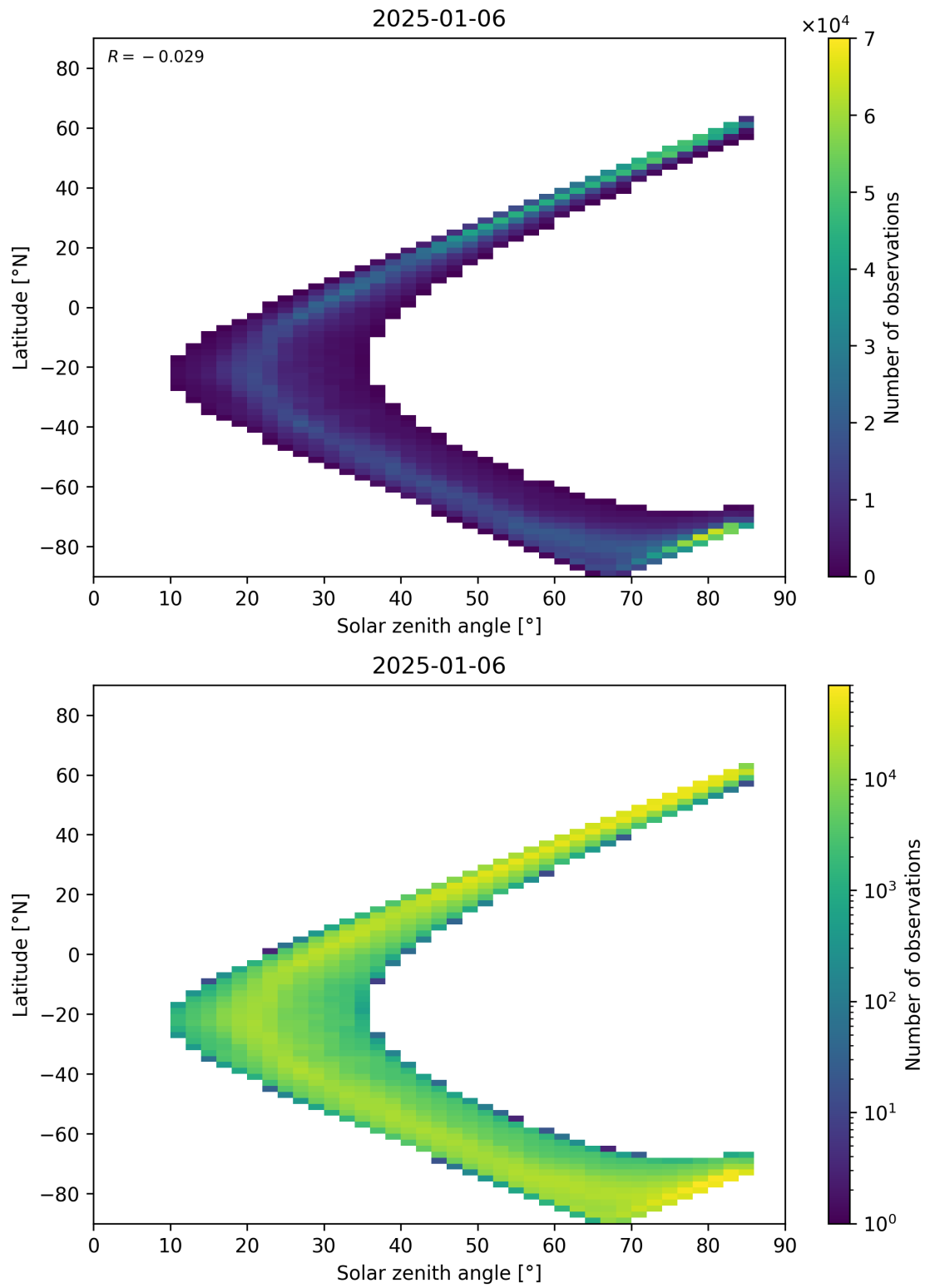
Figure 66: Scatter density plot of “Solar zenith angle” against “Latitude” for 2025-01-05 to 2025-01-07.
