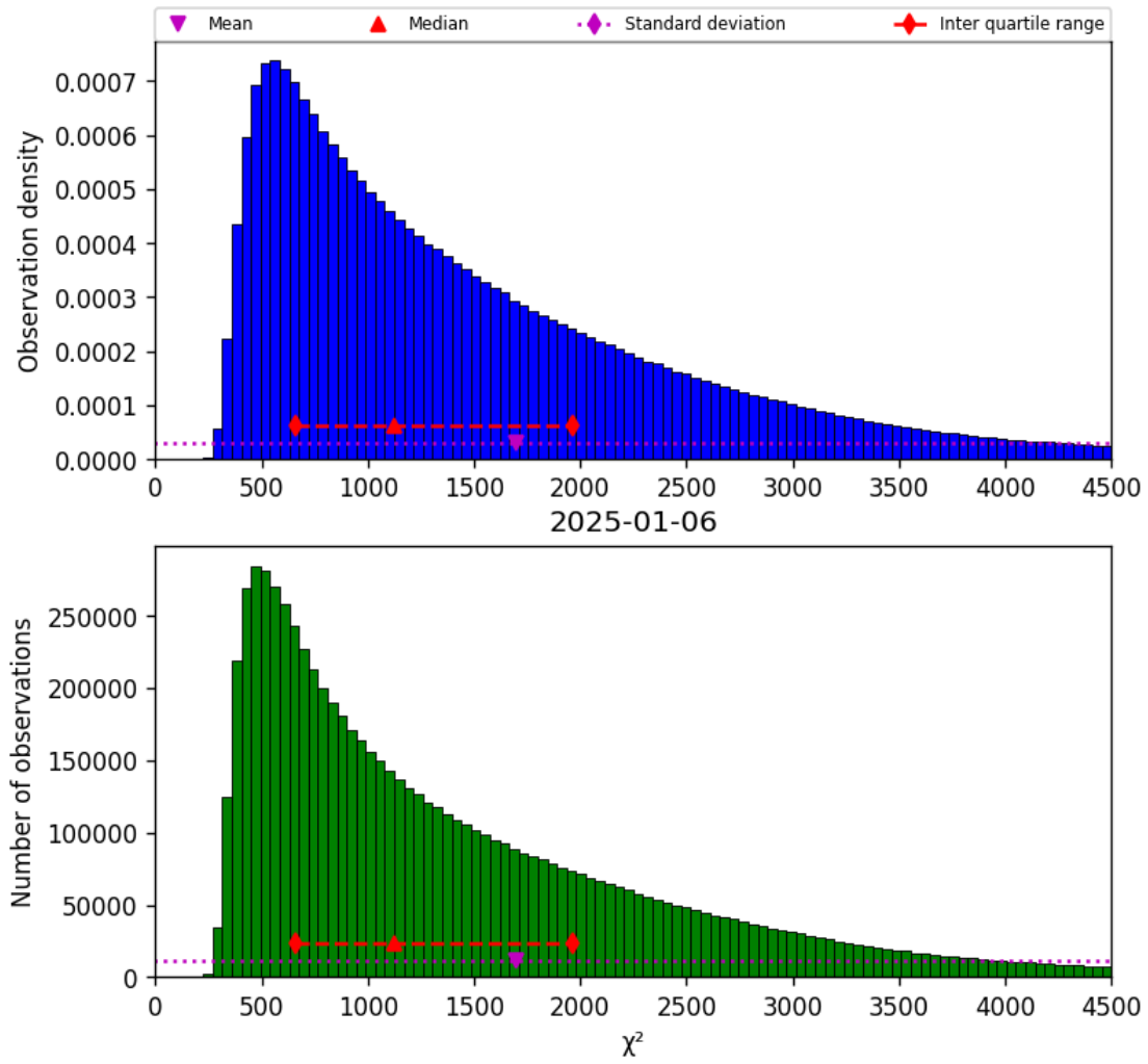
Figure 22: Histogram of “ \chi^2 ” for 2025-01-05 to 2025-01-07
