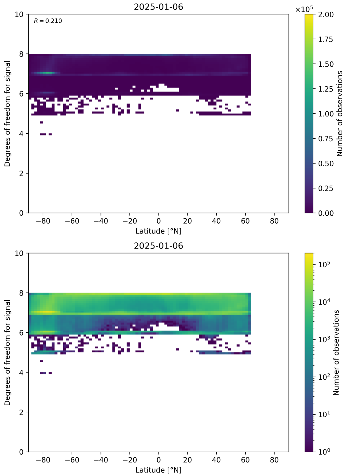
Figure 55: Scatter density plot of “Latitude” against “Degrees of freedom for signal” for 2025-01-05 to 2025-01-07.
