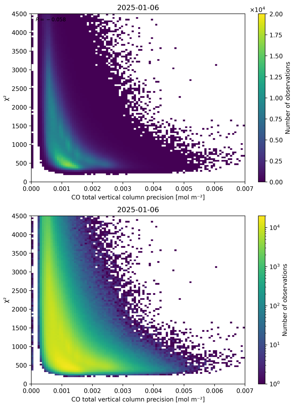
Figure 44: Scatter density plot of “CO total vertical column precision” against “ \chi^2 ” for 2025-01-05 to 2025-01-07.
