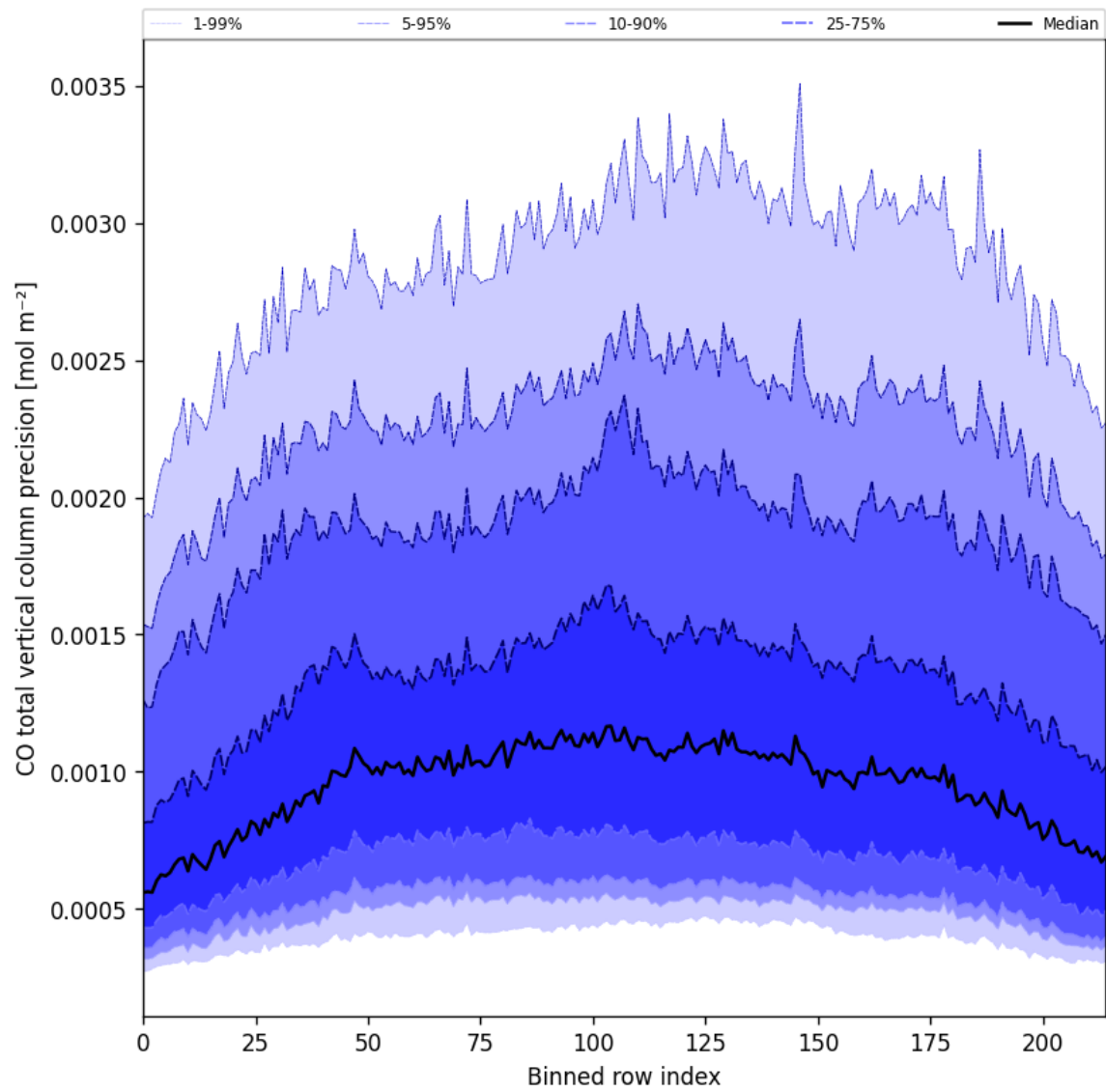
Figure 28: Along track statistics of “CO total vertical column precision” for 2025-01-05 to 2025-01-07
