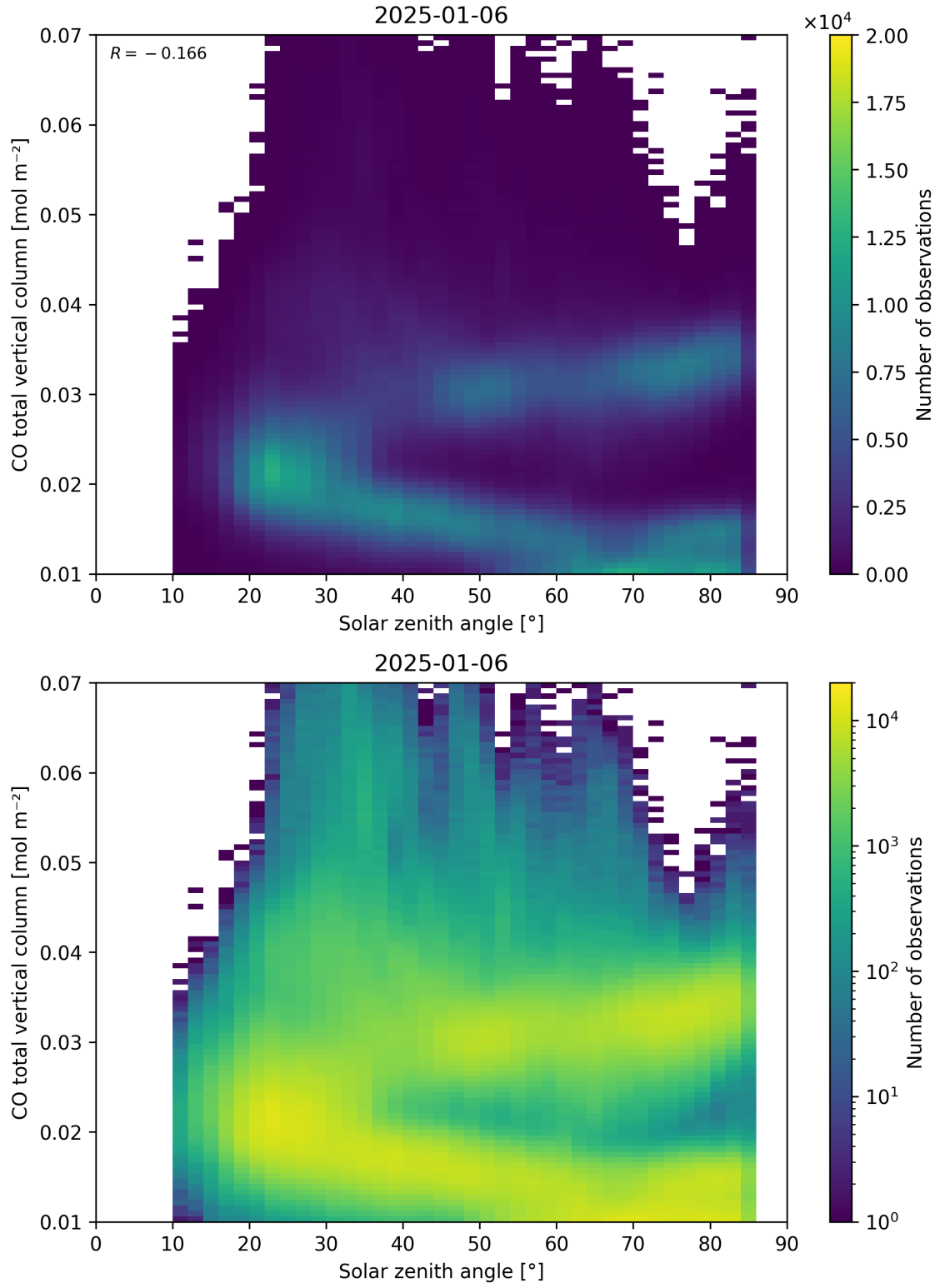
Figure 61: Scatter density plot of “Solar zenith angle” against “CO total vertical column” for 2025-01-05 to 2025-01-07.
