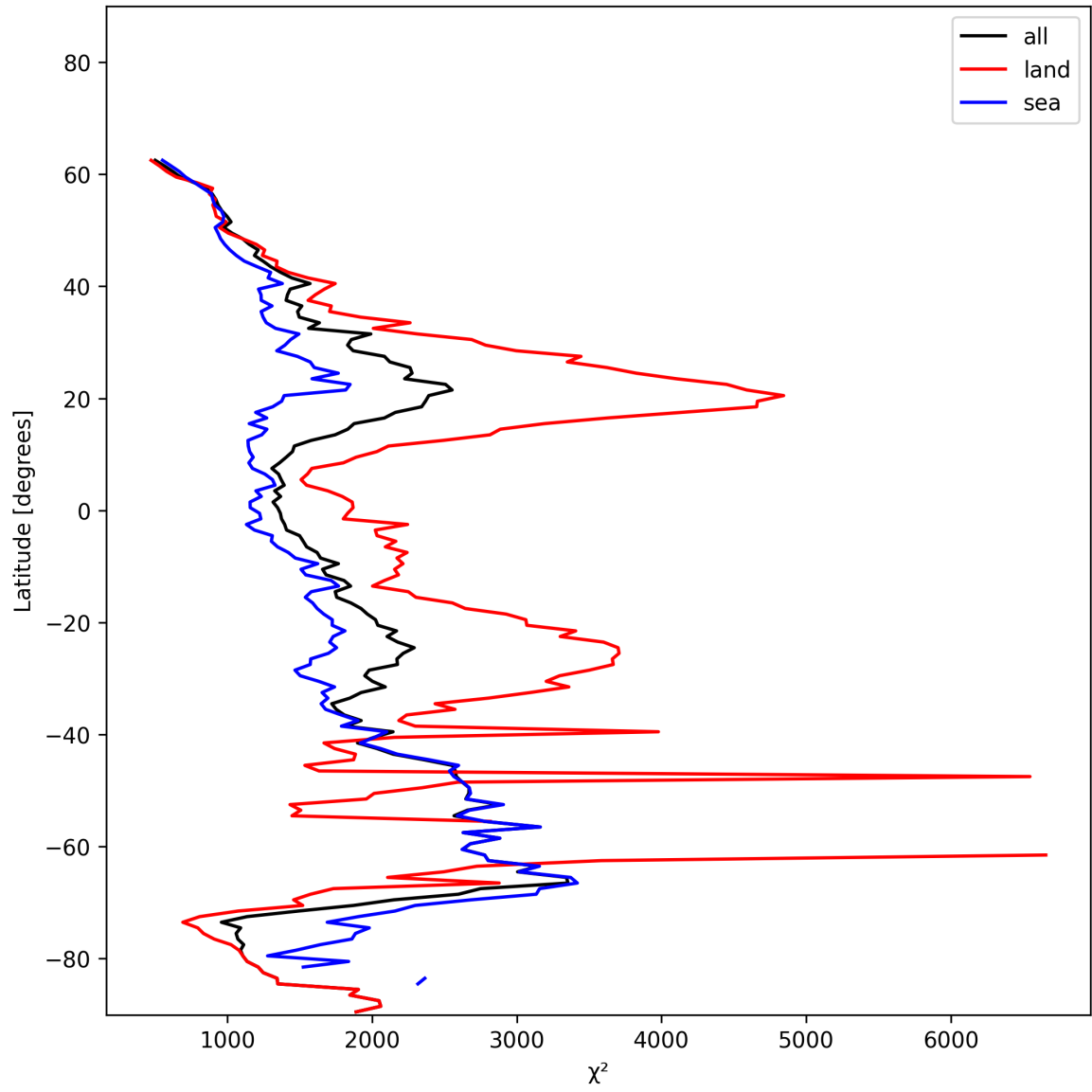
Figure 14: Zonal average of “ \chi^2 ” for 2025-01-05 to 2025-01-07.
