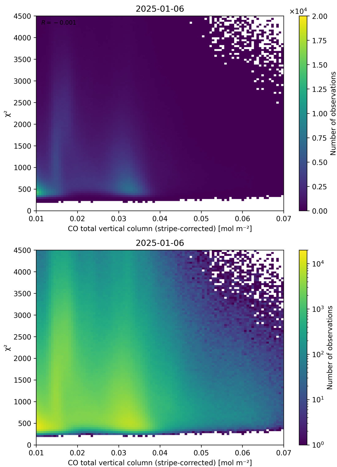
Figure 37: Scatter density plot of “CO total vertical column (stripe-corrected)” against “ \chi^2 ” for 2025-01-05 to 2025-01-07.
