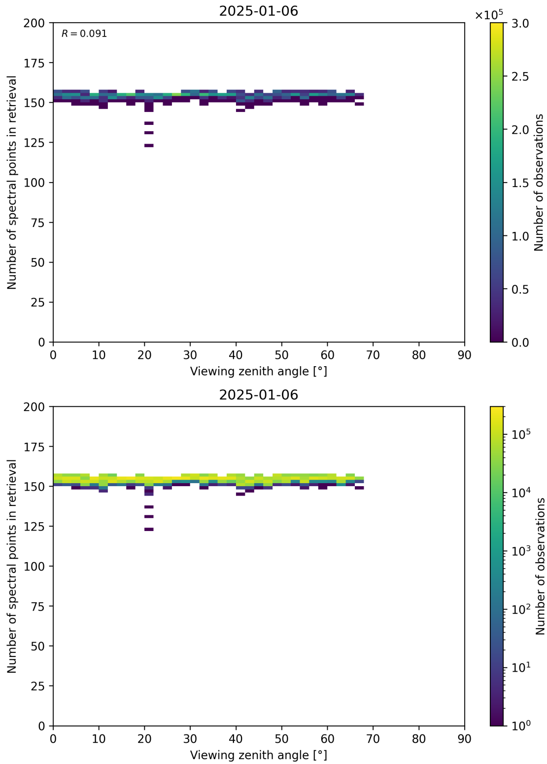
Figure 76: Scatter density plot of “Viewing zenith angle” against “Number of spectral points in retrieval” for 2025-01-05 to 2025-01-07.
