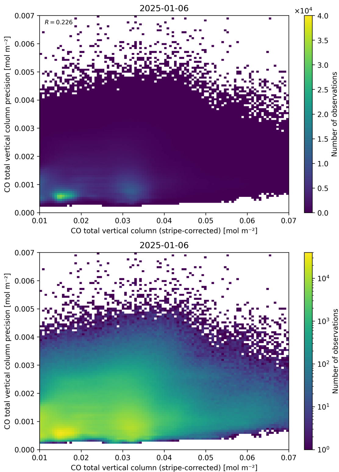
Figure 36: Scatter density plot of “CO total vertical column (stripe-corrected)” against “CO total vertical column precision” for 2025-01-05 to 2025-01-07.
