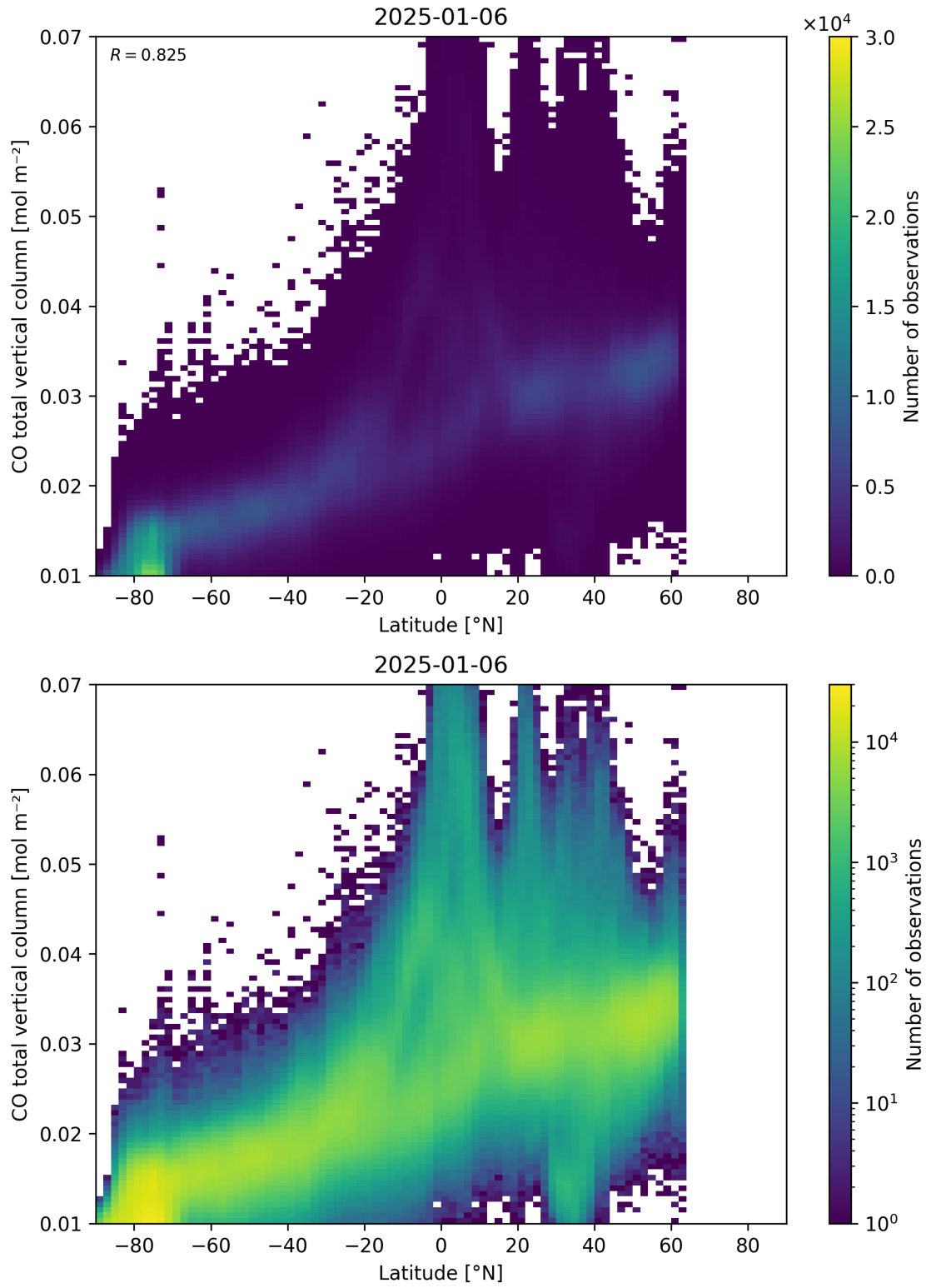
Figure 51: Scatter density plot of “Latitude” against “CO total vertical column” for 2025-01-05 to 2025-01-07.
