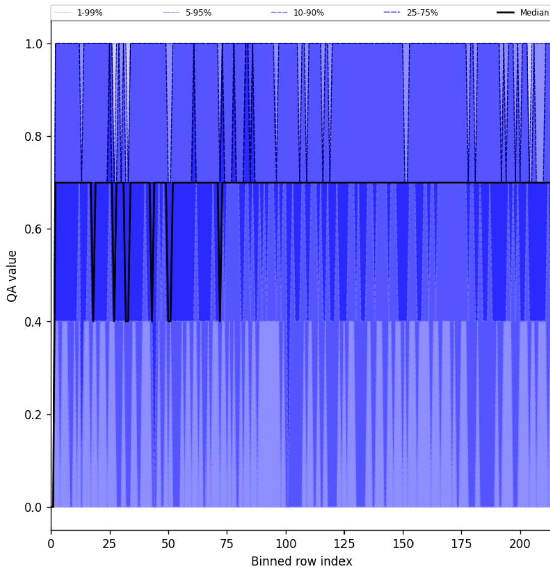
Figure 25: Along track statistics of “QA value” for 2025-01-05 to 2025-01-07
