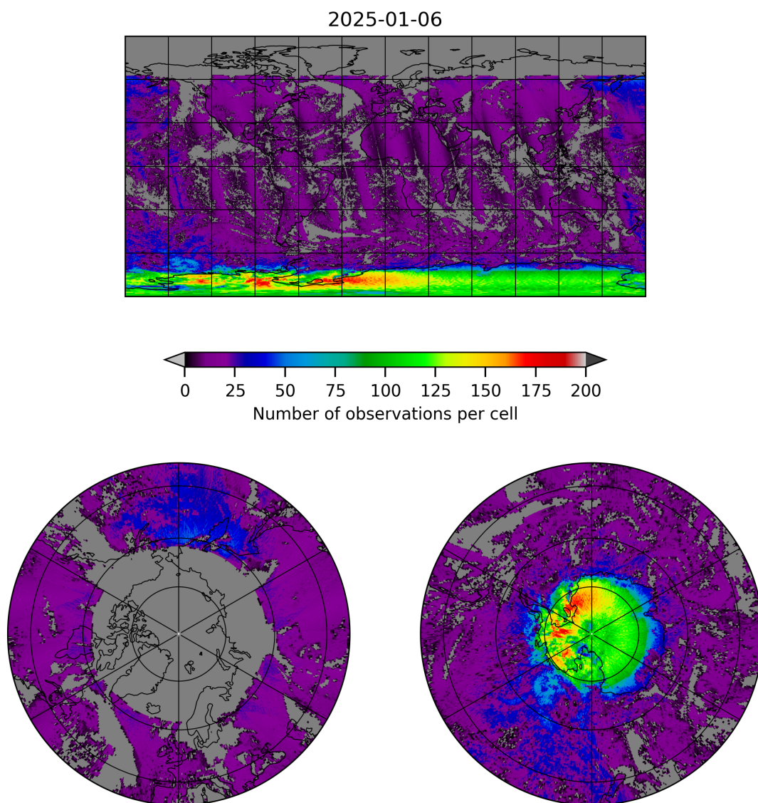
Figure 8: Map of the number of observations for 2025-01-05 to 2025-01-07
