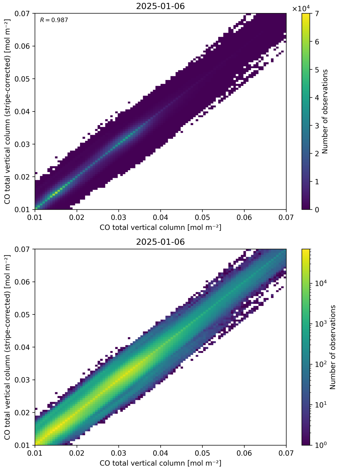
Figure 33: Scatter density plot of “CO total vertical column” against “CO total vertical column (stripe-corrected)” for 2025-01-05 to 2025-01-07.
