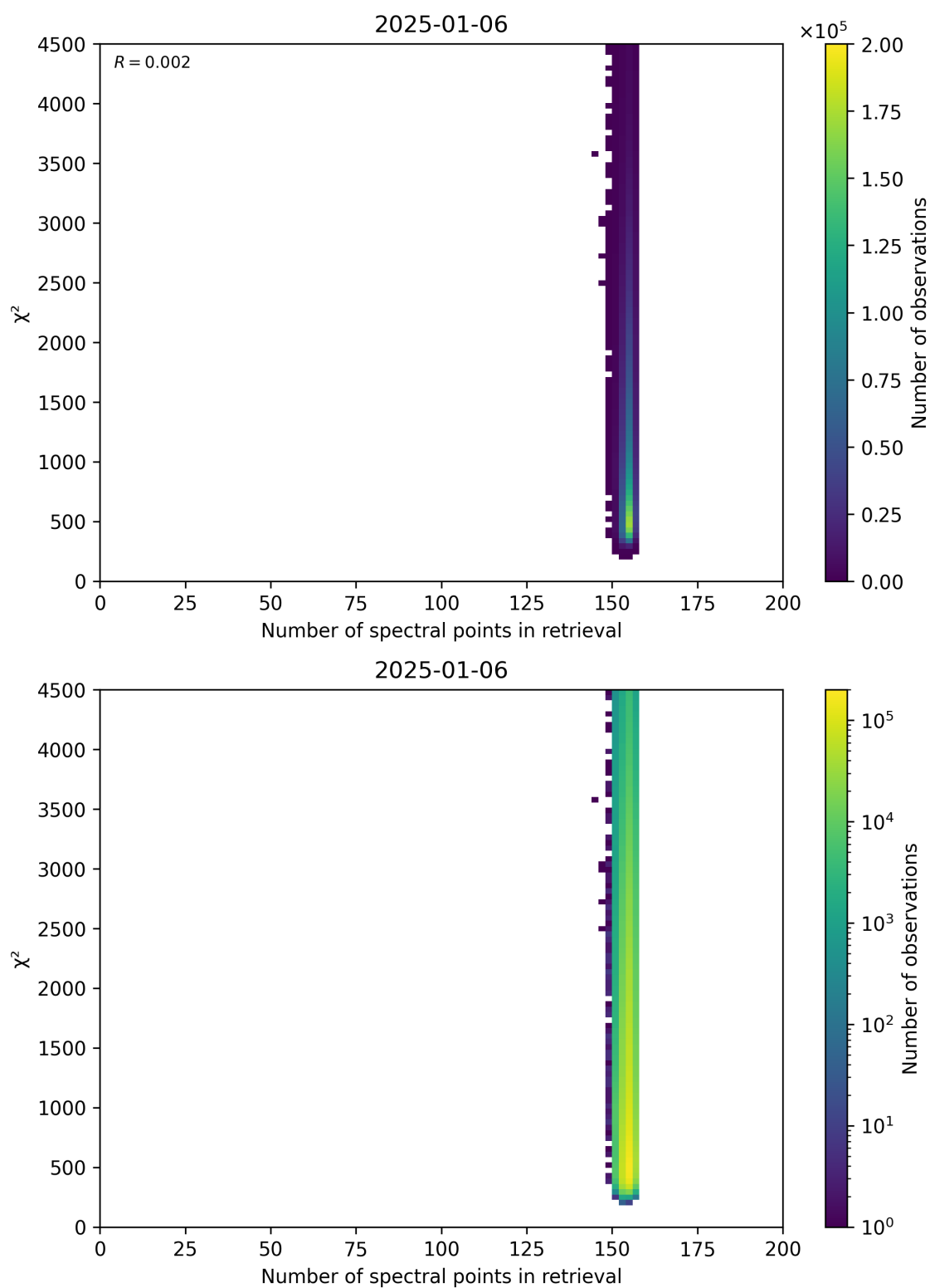
Figure 58: Scatter density plot of “Number of spectral points in retrieval” against “ \chi^2 ” for 2025-01-05 to 2025-01-07.
