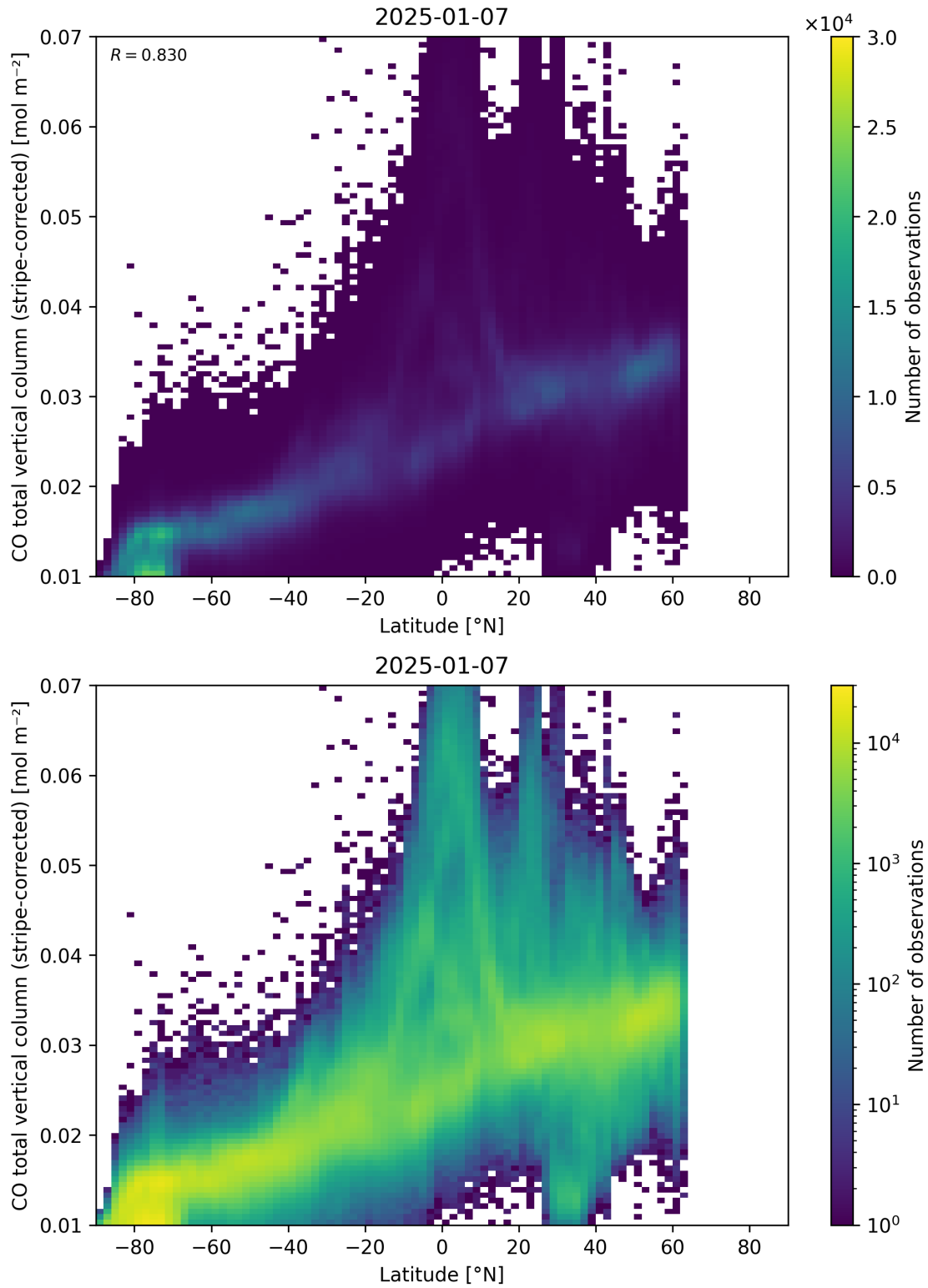
Figure 52: Scatter density plot of “Latitude” against “CO total vertical column (stripe-corrected)” for 2025-01-07 to 2025-01-08.
