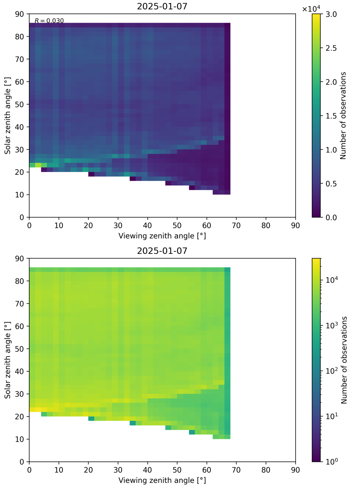
Figure 77: Scatter density plot of “Viewing zenith angle” against “Solar zenith angle” for 2025-01-07 to 2025-01-08.
