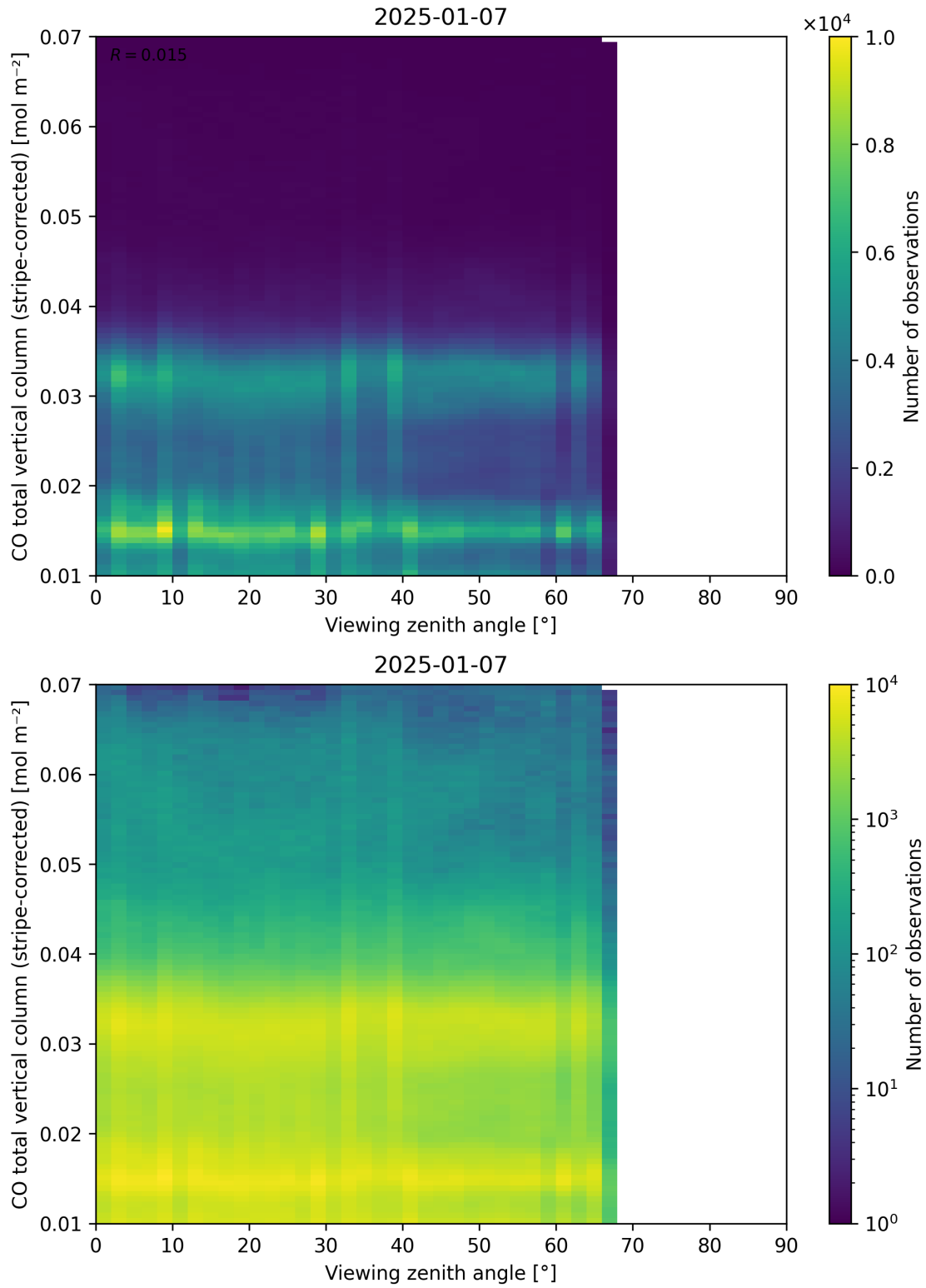
Figure 70: Scatter density plot of “Viewing zenith angle” against “CO total vertical column (stripe-corrected)” for 2025-01-07 to 2025-01-08.
