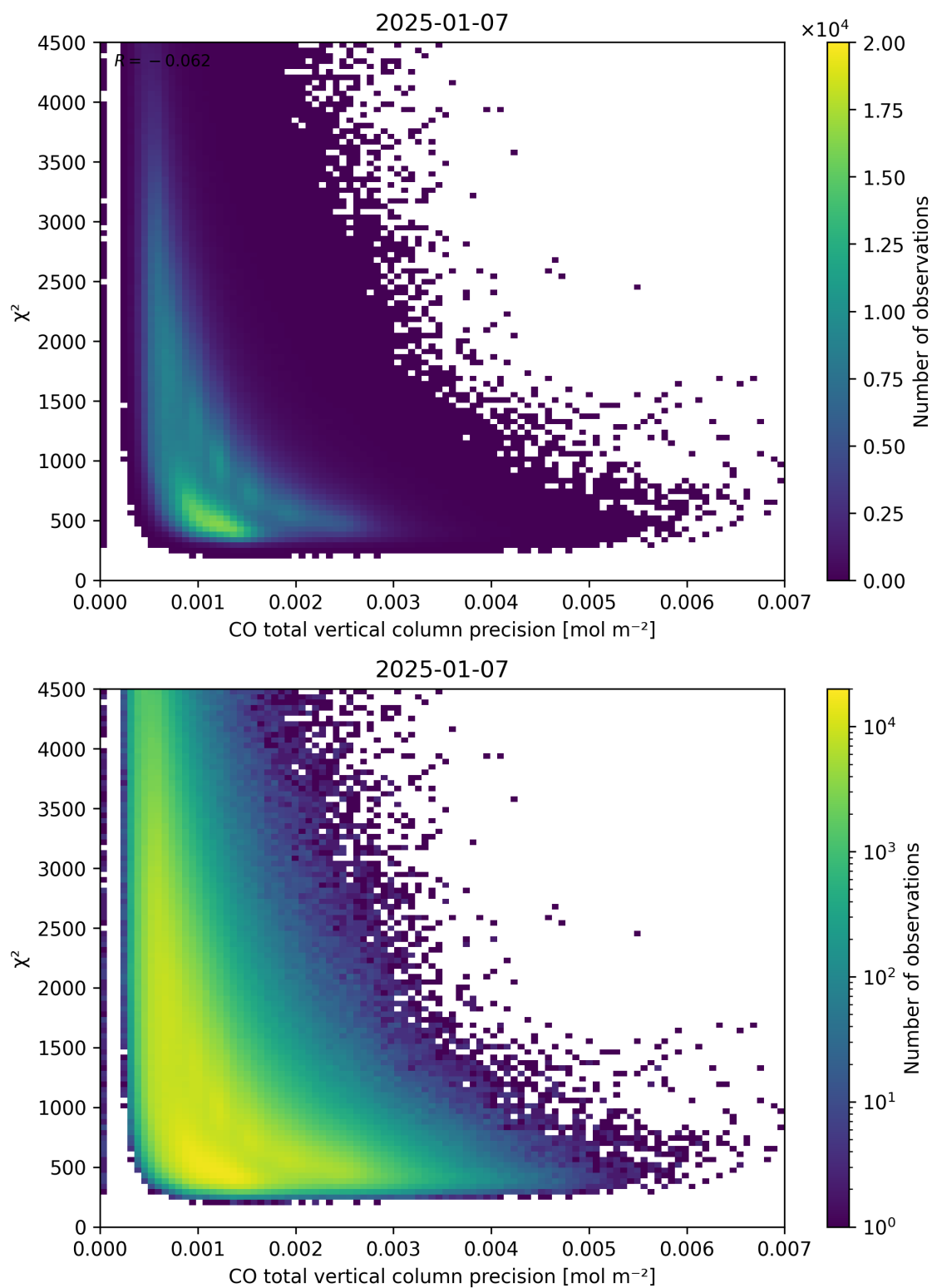
Figure 44: Scatter density plot of “CO total vertical column precision” against “ \chi^2 ” for 2025-01-07 to 2025-01-08.
