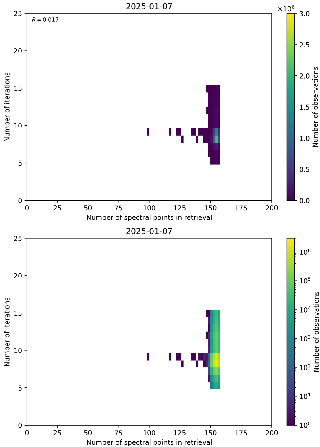
Figure 60: Scatter density plot of “Number of spectral points in retrieval” against “Number of iterations” for 2025-01-07 to 2025-01-08.
