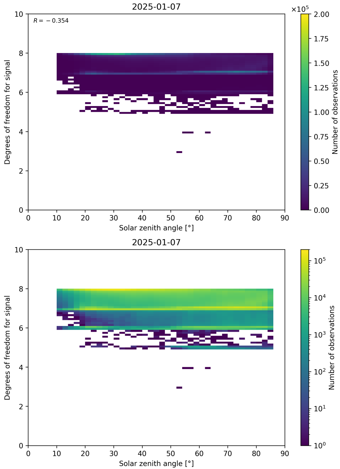
Figure 65: Scatter density plot of “Solar zenith angle” against “Degrees of freedom for signal” for 2025-01-07 to 2025-01-08.
