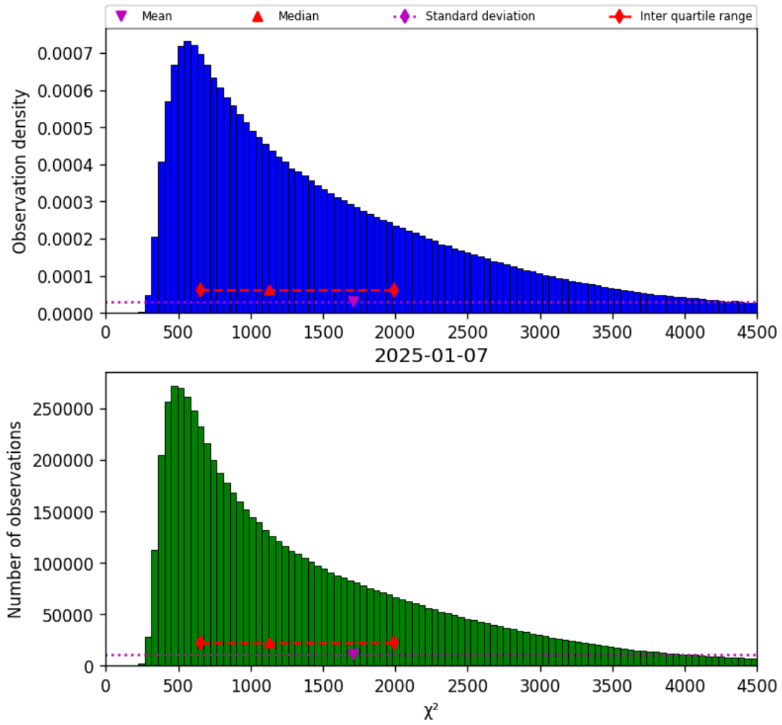
Figure 22: Histogram of “ \chi^2 ” for 2025-01-07 to 2025-01-08
