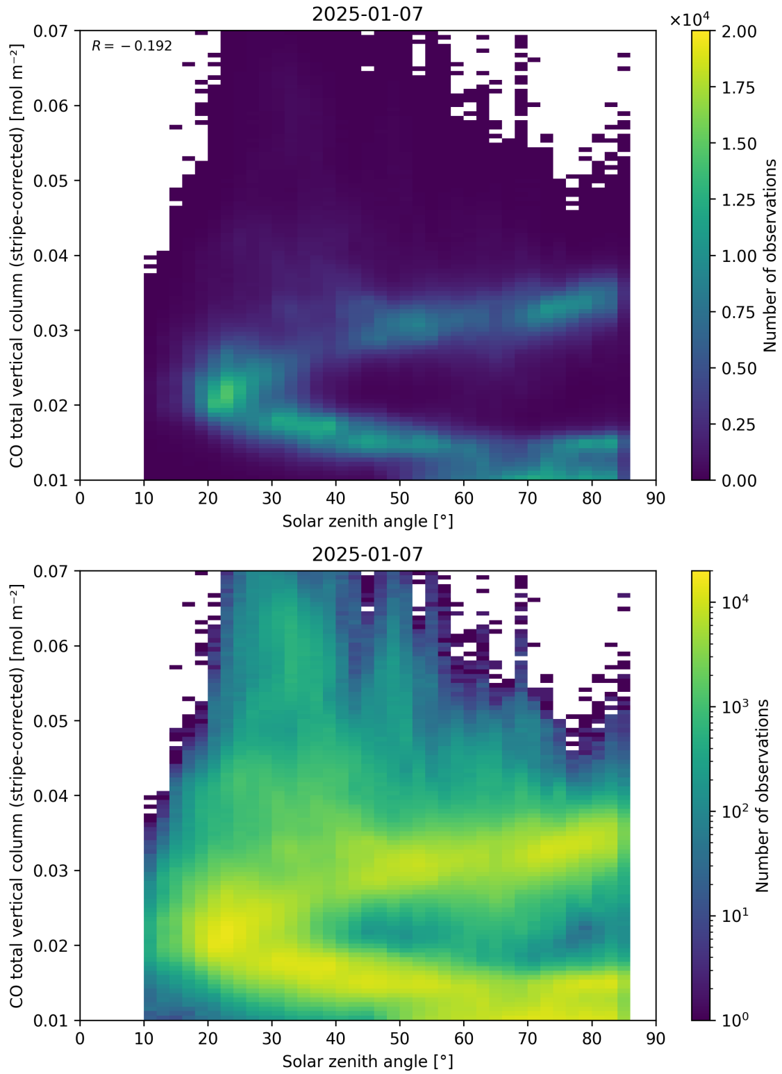
Figure 62: Scatter density plot of “Solar zenith angle” against “CO total vertical column (stripe-corrected)” for 2025-01-07 to 2025-01-08.
