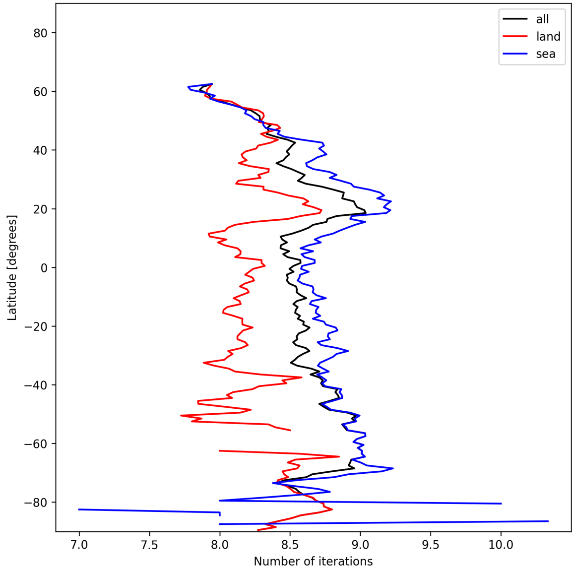
Figure 16: Zonal average of “Number of iterations” for 2025-01-07 to 2025-01-08.
