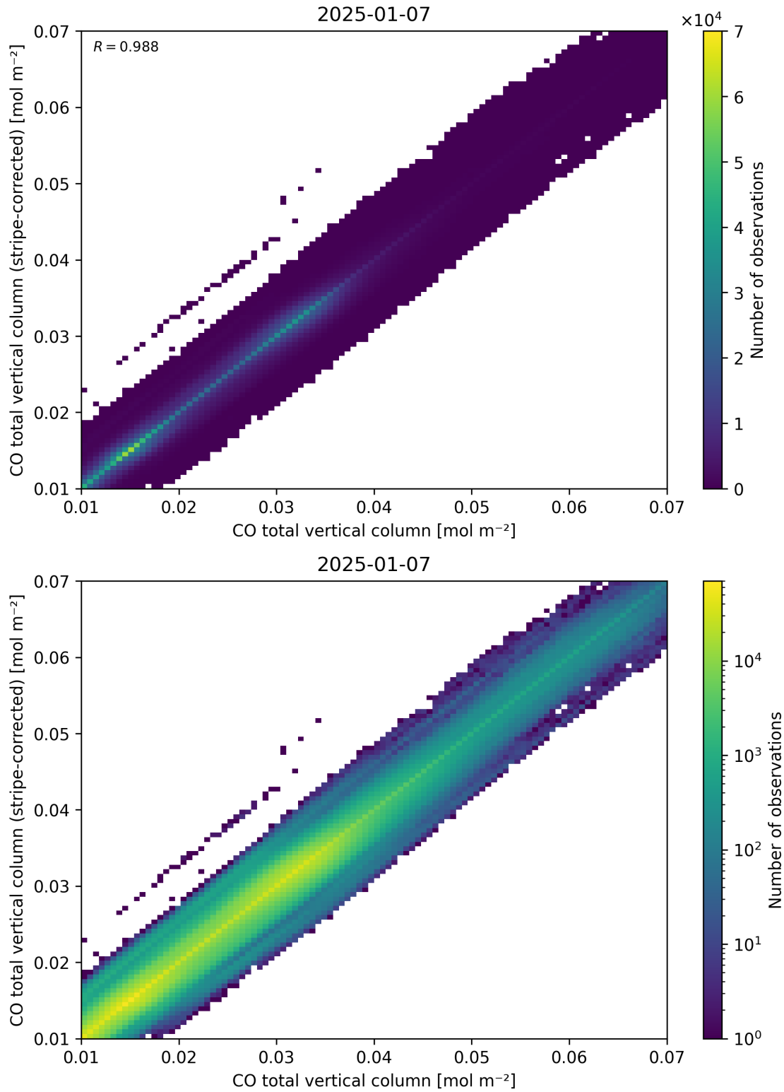
Figure 33: Scatter density plot of “CO total vertical column” against “CO total vertical column (stripe-corrected)” for 2025-01-07 to 2025-01-08.
