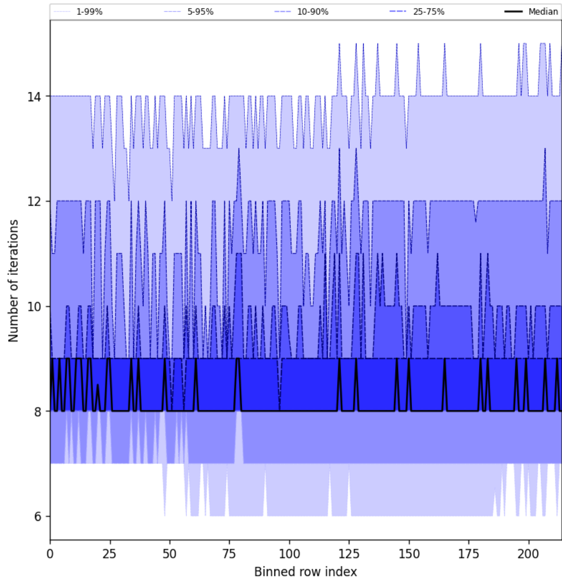
Figure 32: Along track statistics of “Number of iterations” for 2025-01-07 to 2025-01-08
