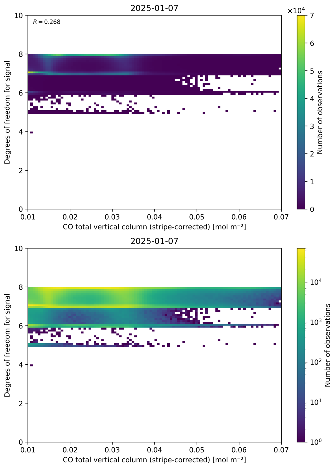
Figure 38: Scatter density plot of “CO total vertical column (stripe-corrected)” against “Degrees of freedom for signal” for 2025-01-07 to 2025-01-08.
