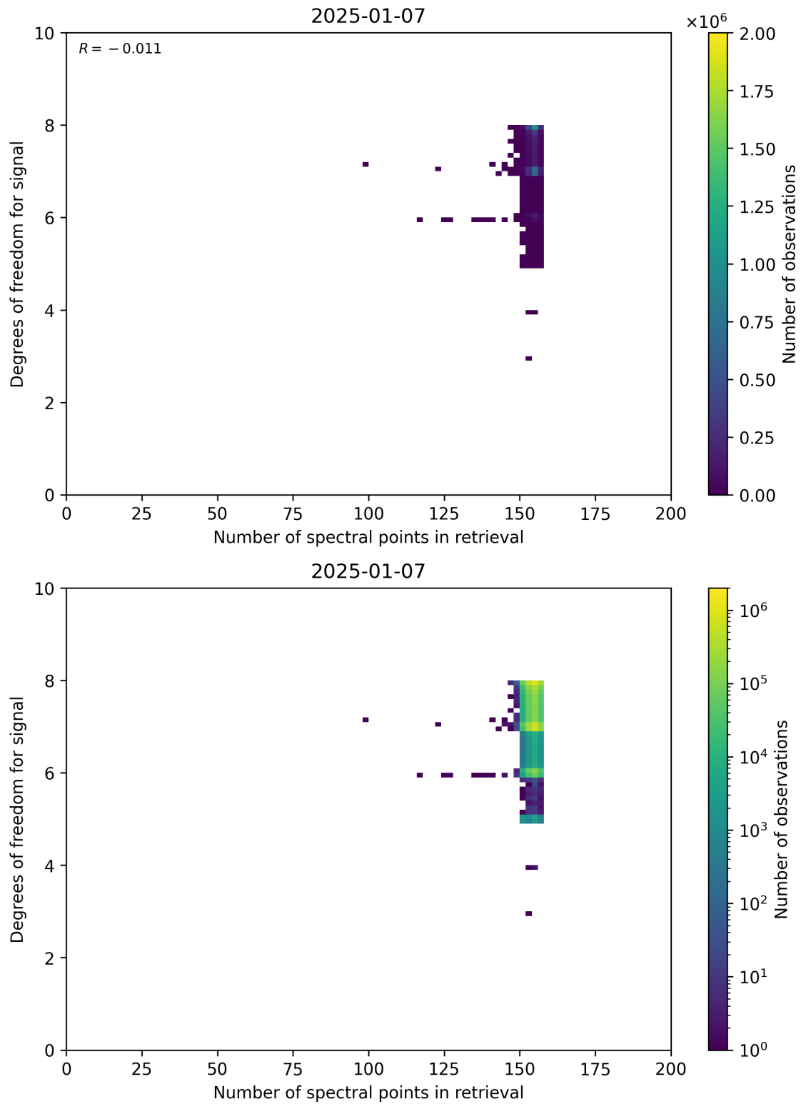
Figure 59: Scatter density plot of “Number of spectral points in retrieval” against “Degrees of freedom for signal” for 2025-01-07 to 2025-01-08.
