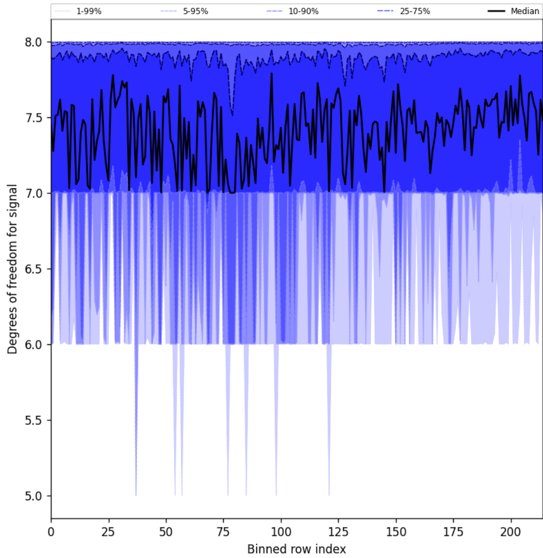
Figure 31: Along track statistics of “Degrees of freedom for signal” for 2025-01-07 to 2025-01-08
