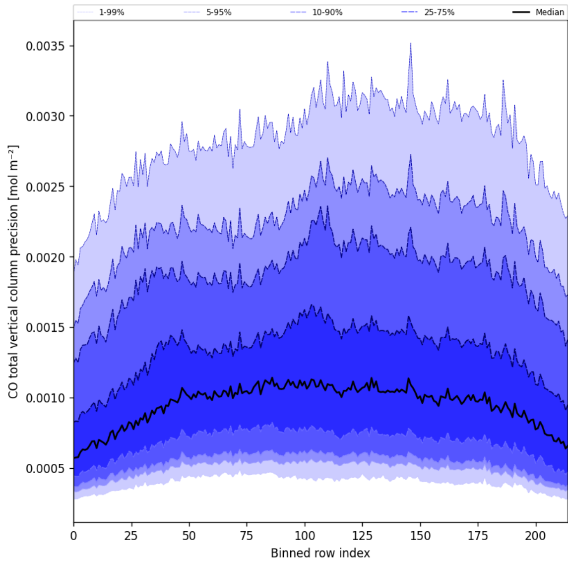
Figure 28: Along track statistics of “CO total vertical column precision” for 2025-01-07 to 2025-01-08
