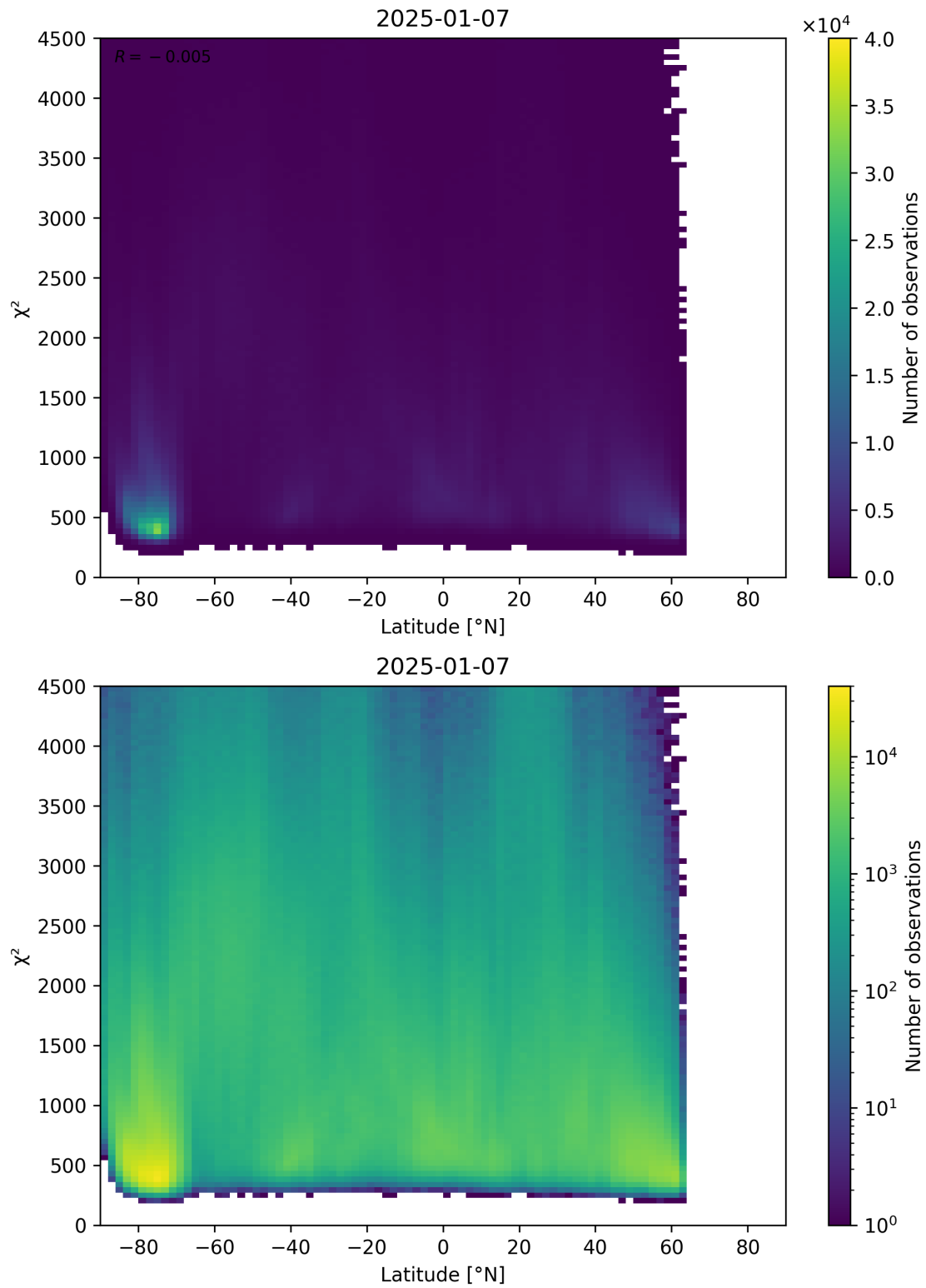
Figure 54: Scatter density plot of “Latitude” against “ \chi^2 ” for 2025-01-07 to 2025-01-08.
