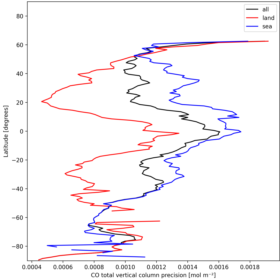
Figure 12: Zonal average of “CO total vertical column precision” for 2025-01-07 to 2025-01-08.
