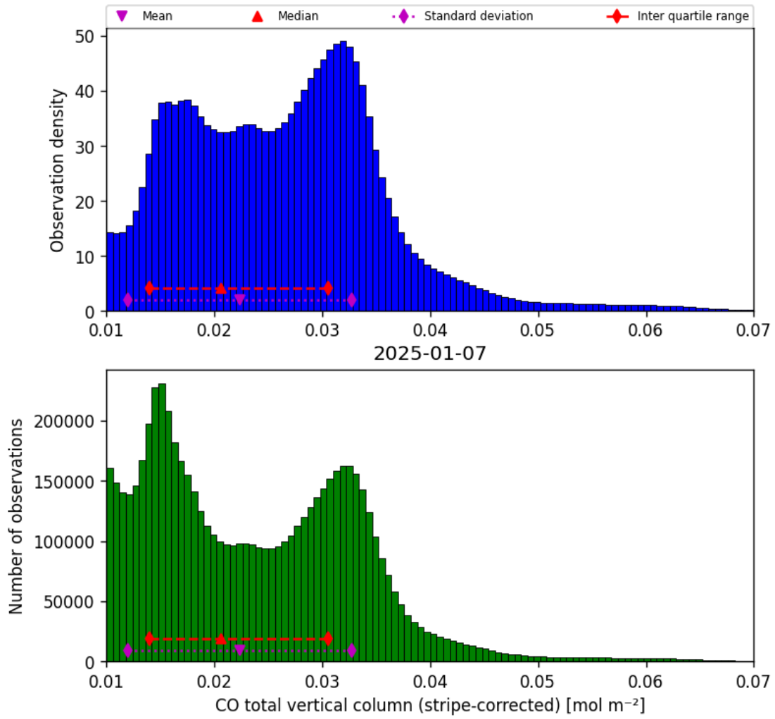
Figure 19: Histogram of “CO total vertical column (stripe-corrected)” for 2025-01-07 to 2025-01-08
