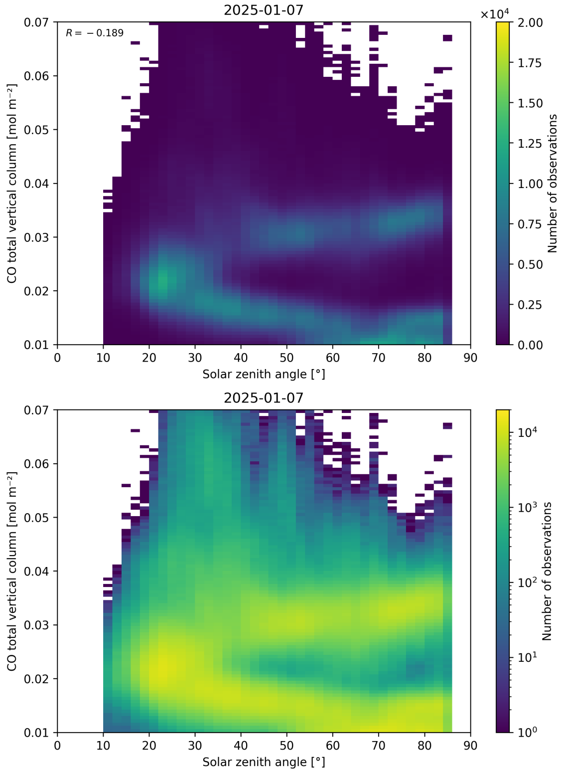
Figure 61: Scatter density plot of “Solar zenith angle” against “CO total vertical column” for 2025-01-07 to 2025-01-08.
