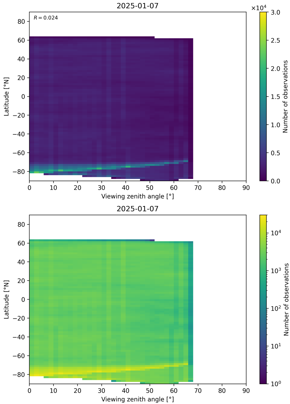
Figure 74: Scatter density plot of “Viewing zenith angle” against “Latitude” for 2025-01-07 to 2025-01-08.
