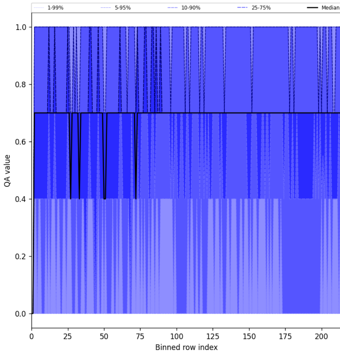
Figure 25: Along track statistics of “QA value” for 2025-01-07 to 2025-01-08
