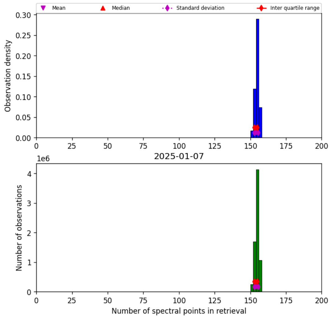
Figure 21: Histogram of “Number of spectral points in retrieval” for 2025-01-07 to 2025-01-08
