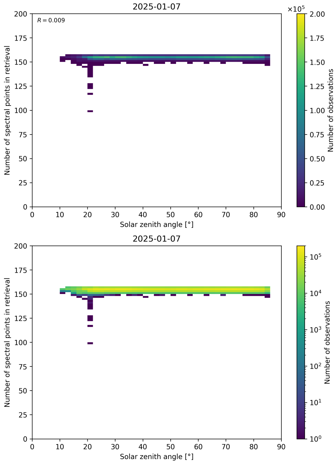
Figure 68: Scatter density plot of “Solar zenith angle” against “Number of spectral points in retrieval” for 2025-01-07 to 2025-01-08.
