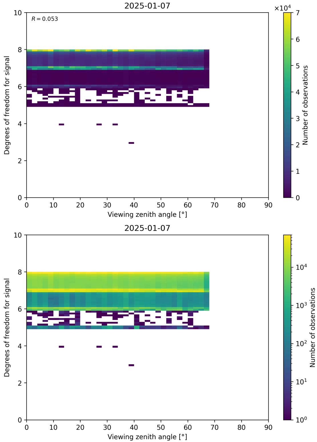
Figure 73: Scatter density plot of “Viewing zenith angle” against “Degrees of freedom for signal” for 2025-01-07 to 2025-01-08.
