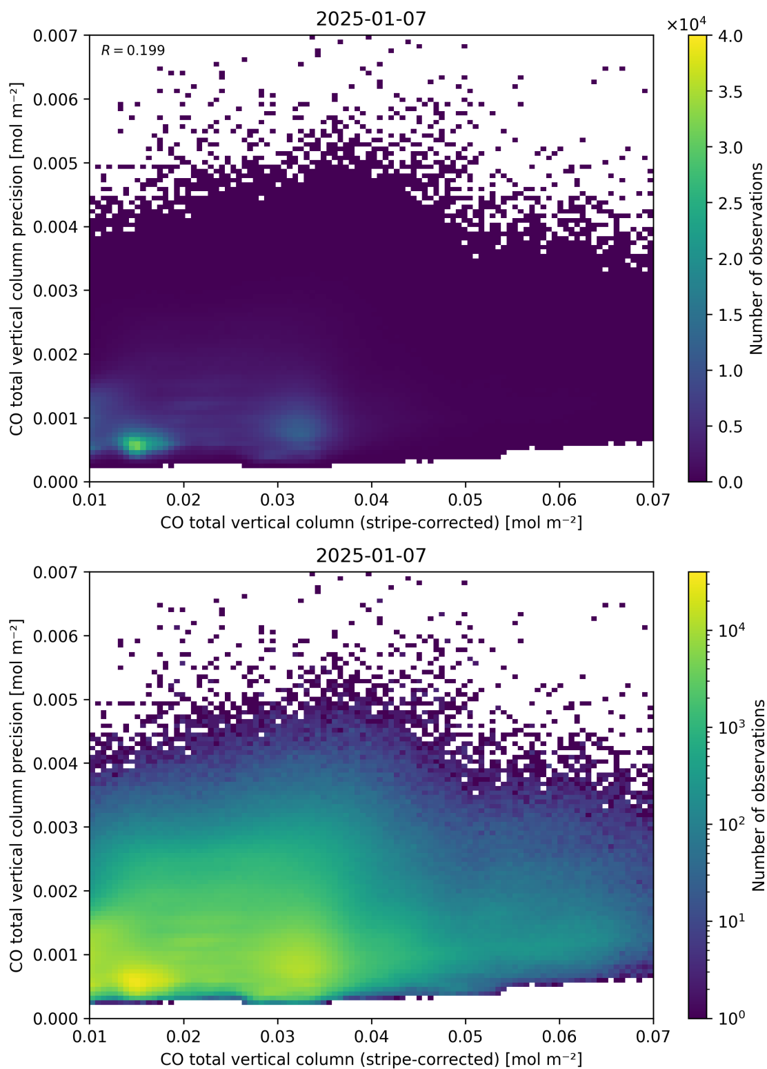
Figure 36: Scatter density plot of “CO total vertical column (stripe-corrected)” against “CO total vertical column precision” for 2025-01-07 to 2025-01-08.
