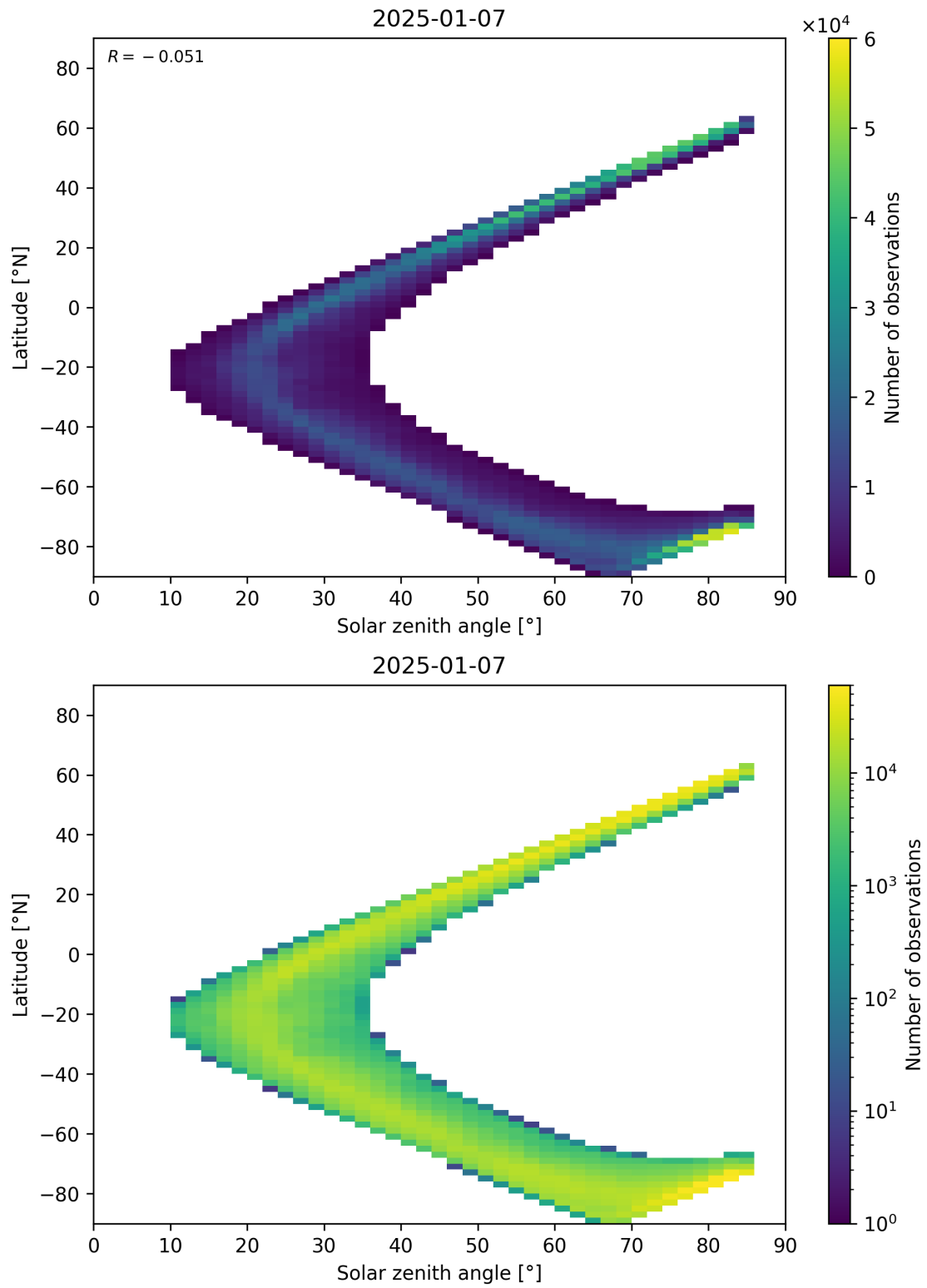
Figure 66: Scatter density plot of “Solar zenith angle” against “Latitude” for 2025-01-07 to 2025-01-08.
