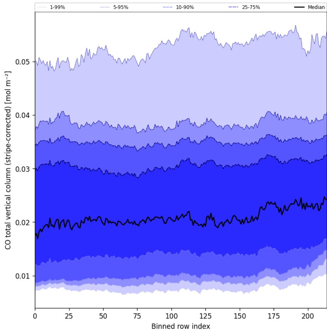
Figure 27: Along track statistics of “CO total vertical column (stripe-corrected)” for 2025-01-07 to 2025-01-08
