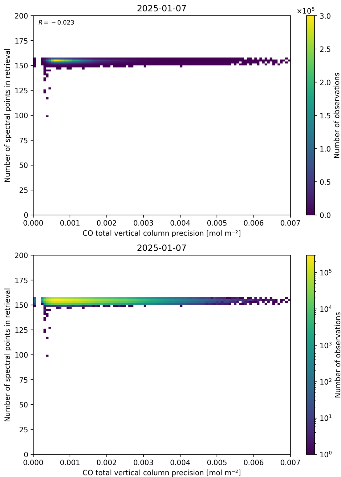
Figure 47: Scatter density plot of “CO total vertical column precision” against “Number of spectral points in retrieval” for 2025-01-07 to 2025-01-08.
