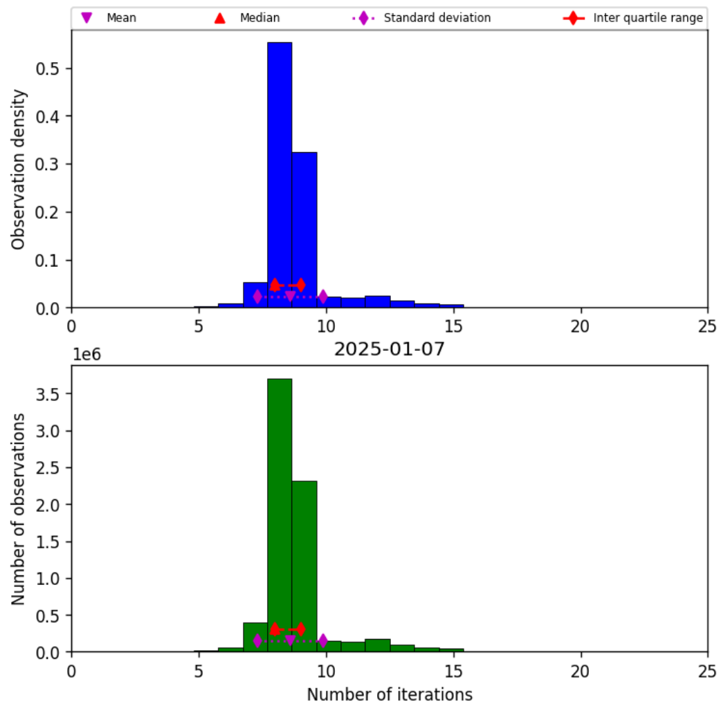
Figure 24: Histogram of “Number of iterations” for 2025-01-07 to 2025-01-08
