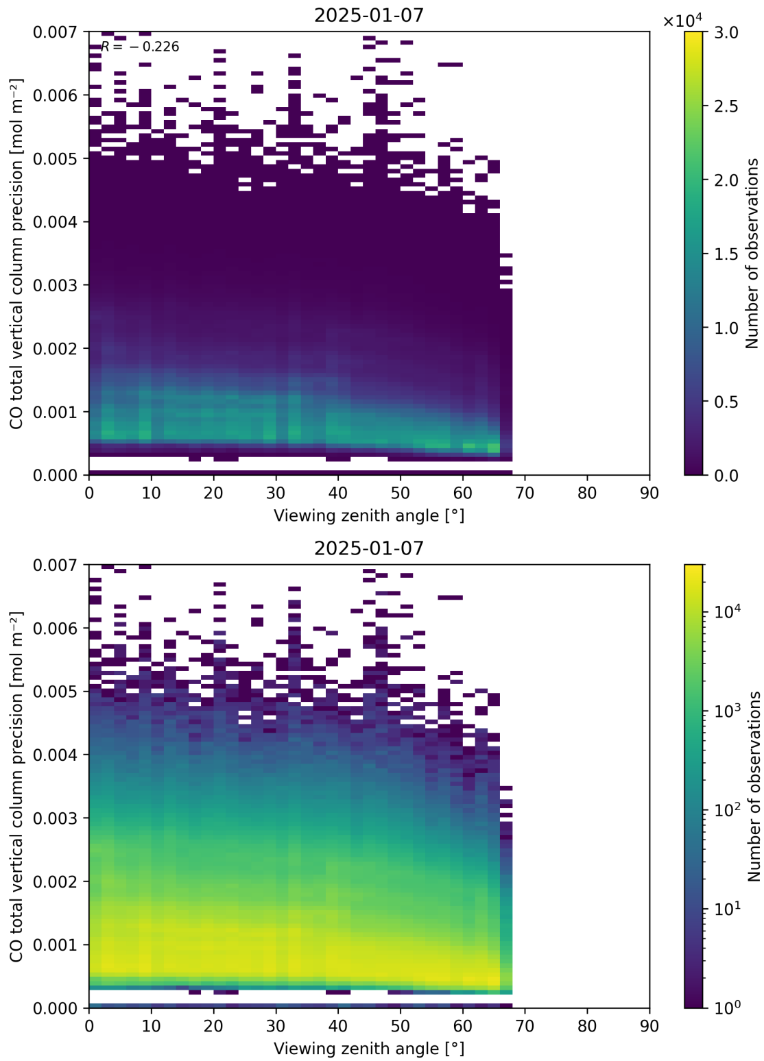
Figure 71: Scatter density plot of “Viewing zenith angle” against “CO total vertical column precision” for 2025-01-07 to 2025-01-08.
