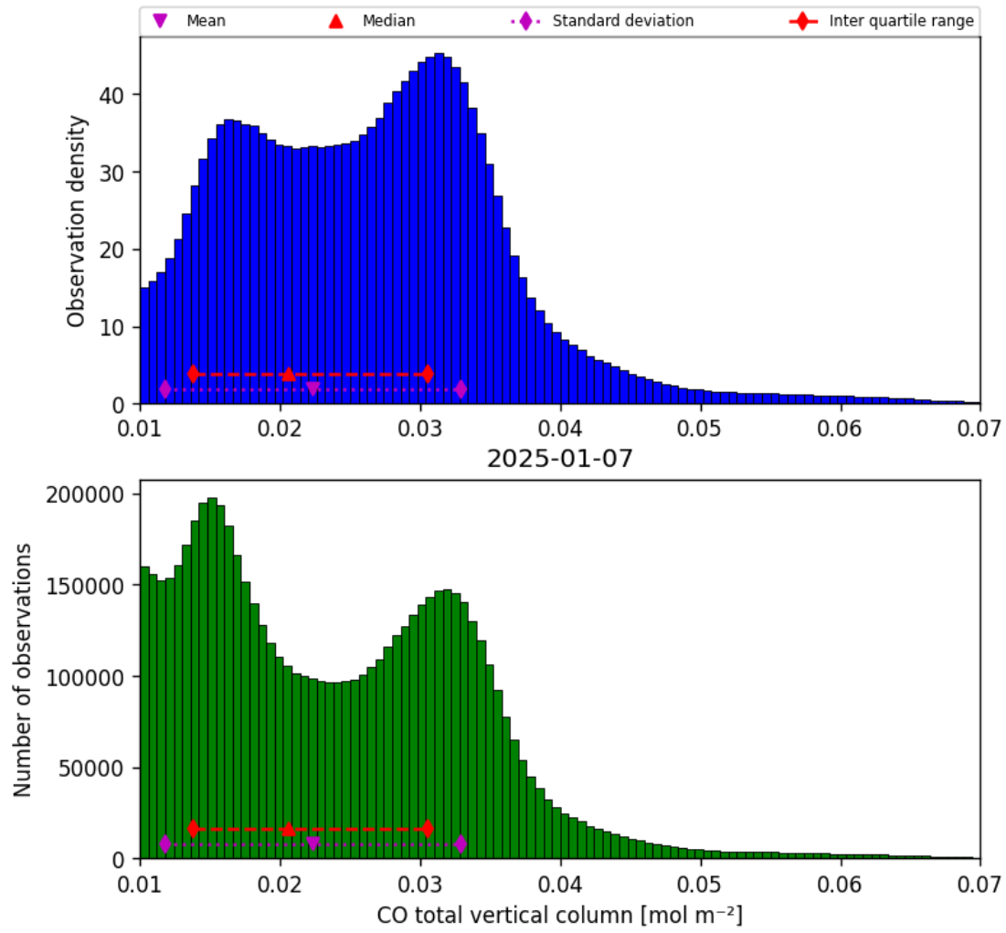
Figure 18: Histogram of “CO total vertical column” for 2025-01-07 to 2025-01-08
