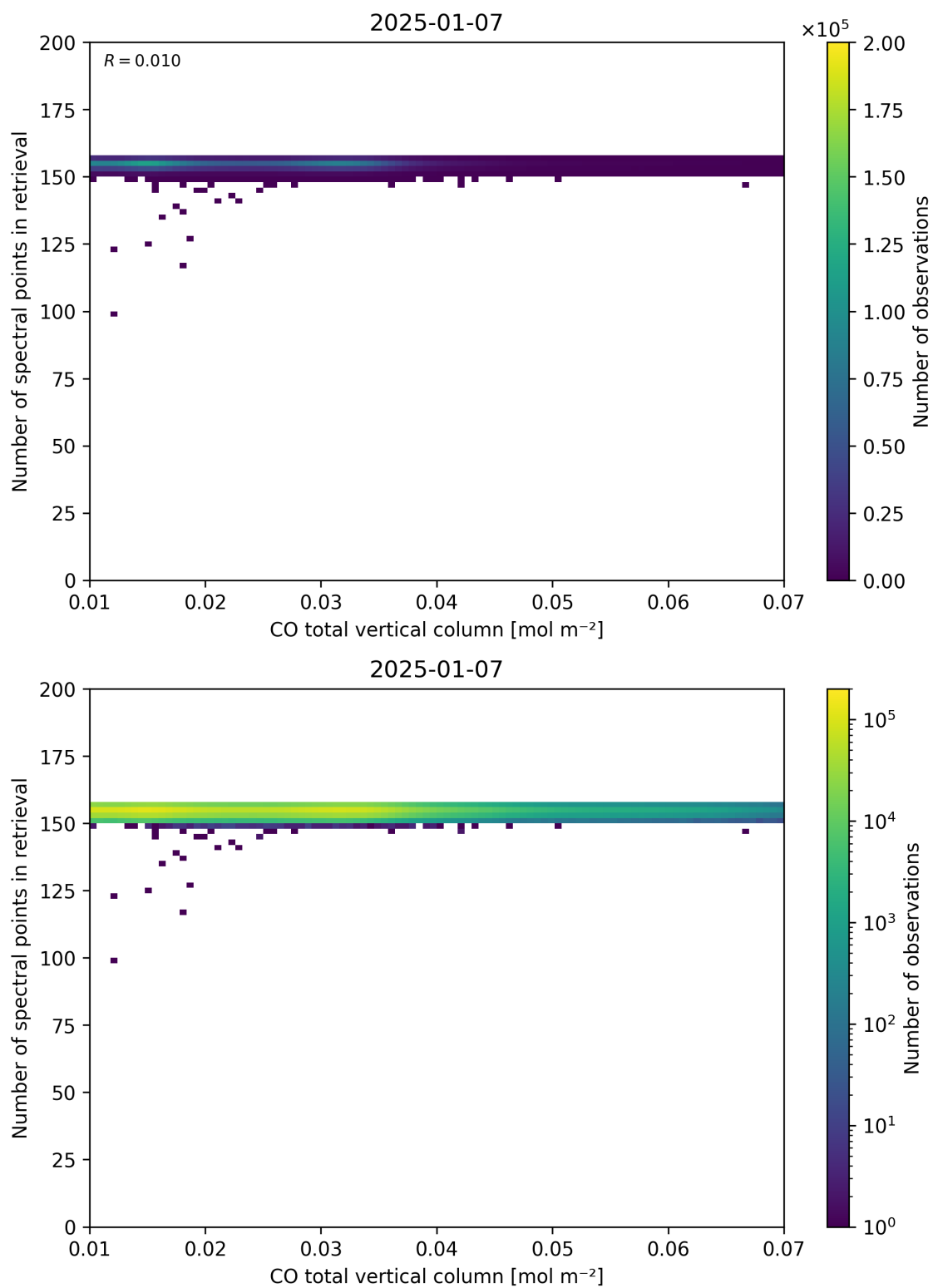
Figure 43: Scatter density plot of “CO total vertical column” against “Number of spectral points in retrieval” for 2025-01-07 to 2025-01-08.
