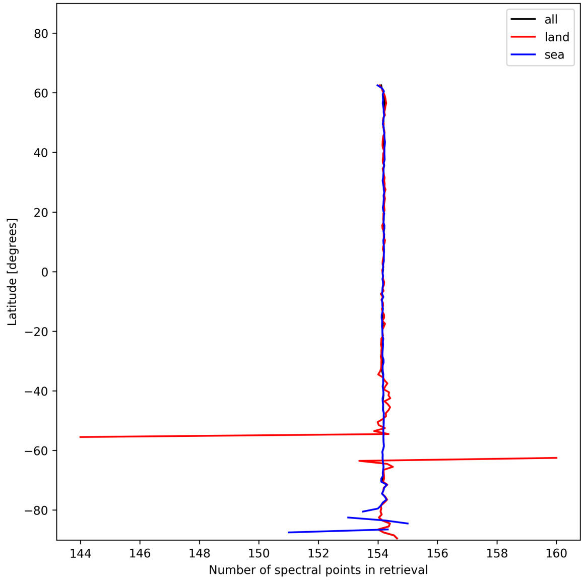
Figure 13: Zonal average of “Number of spectral points in retrieval” for 2025-01-07 to 2025-01-08.
