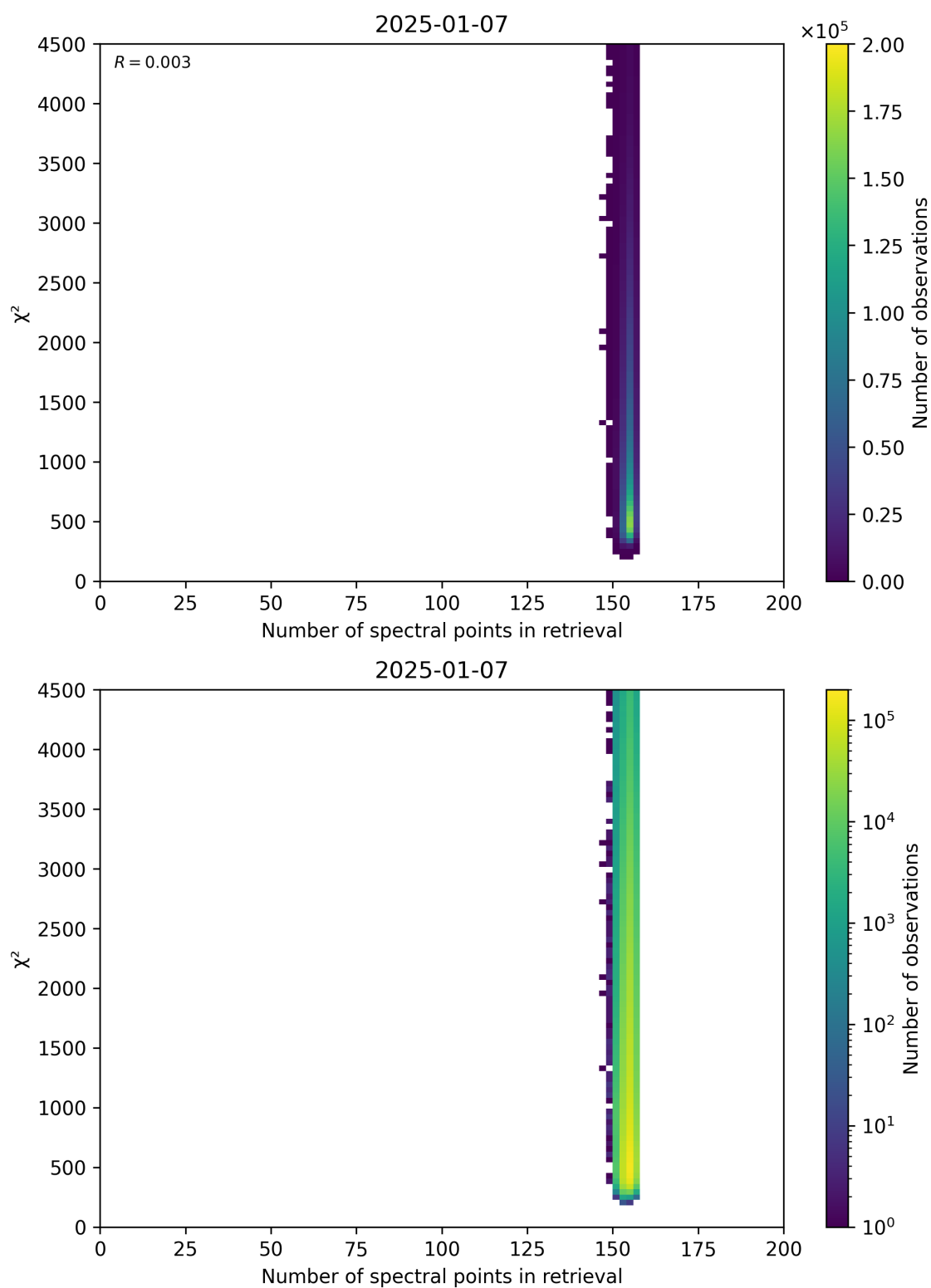
Figure 58: Scatter density plot of “Number of spectral points in retrieval” against “ \chi^2 ” for 2025-01-07 to 2025-01-08.
