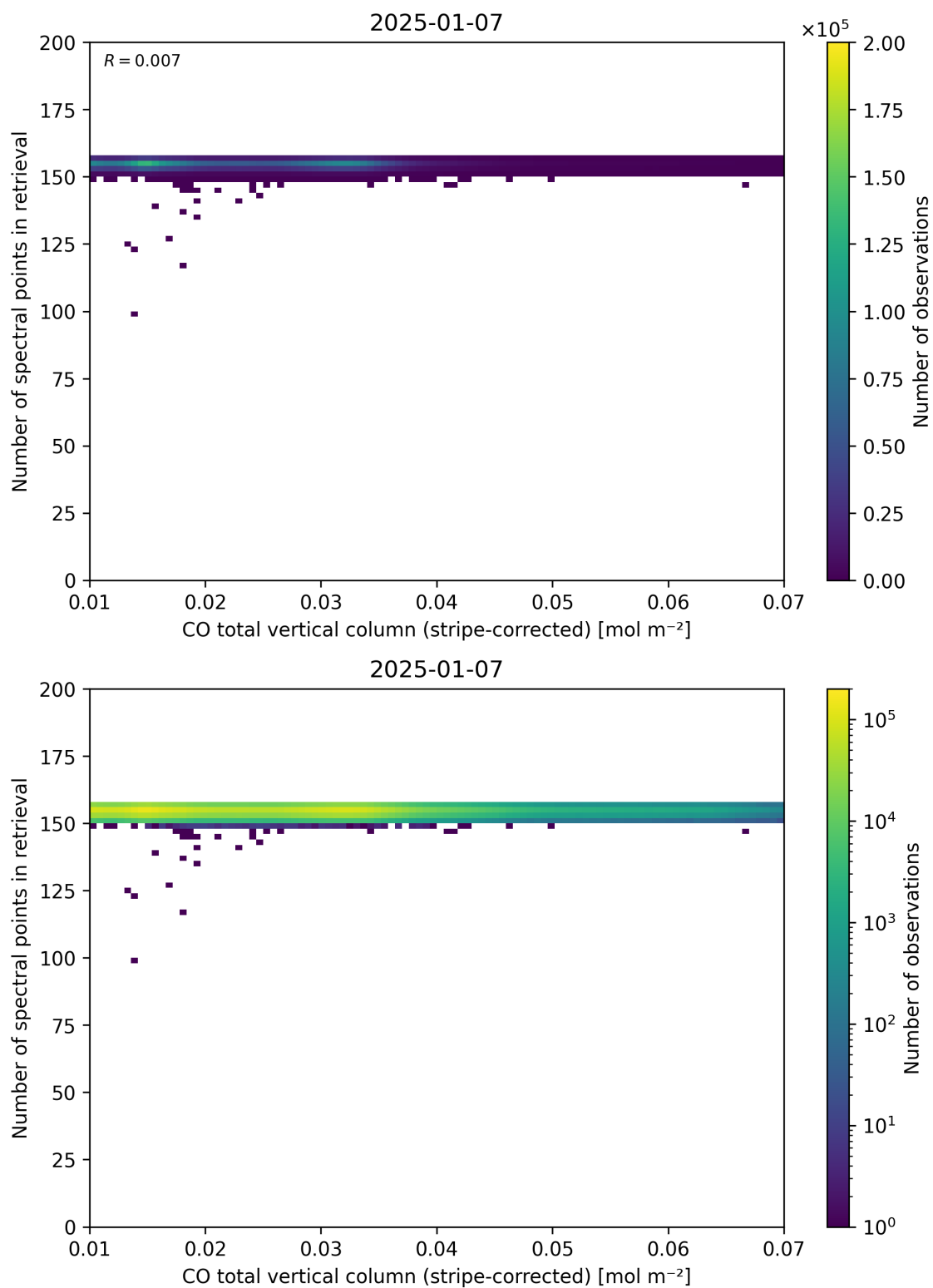
Figure 40: Scatter density plot of “CO total vertical column (stripe-corrected)” against “Number of spectral points in retrieval” for 2025-01-07 to 2025-01-08.
