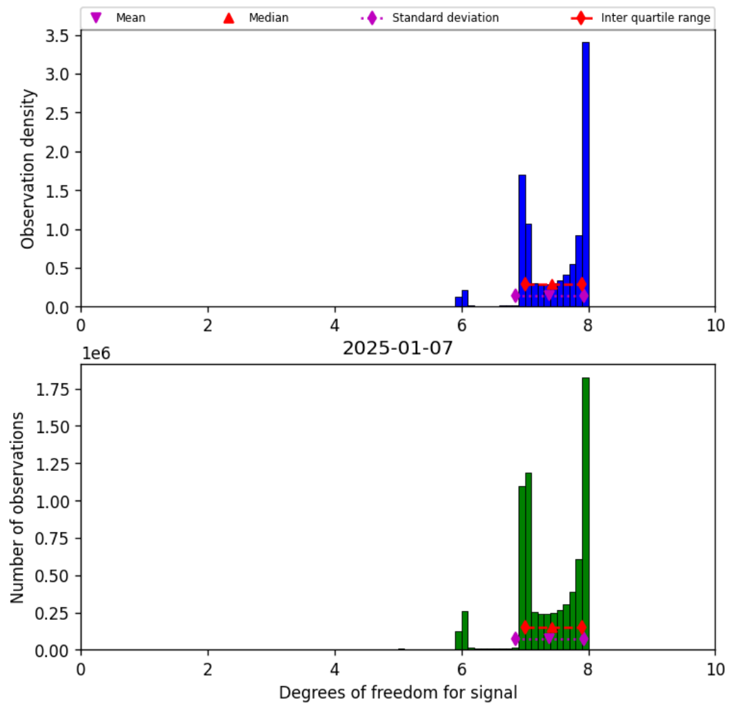
Figure 23: Histogram of “Degrees of freedom for signal” for 2025-01-07 to 2025-01-08
