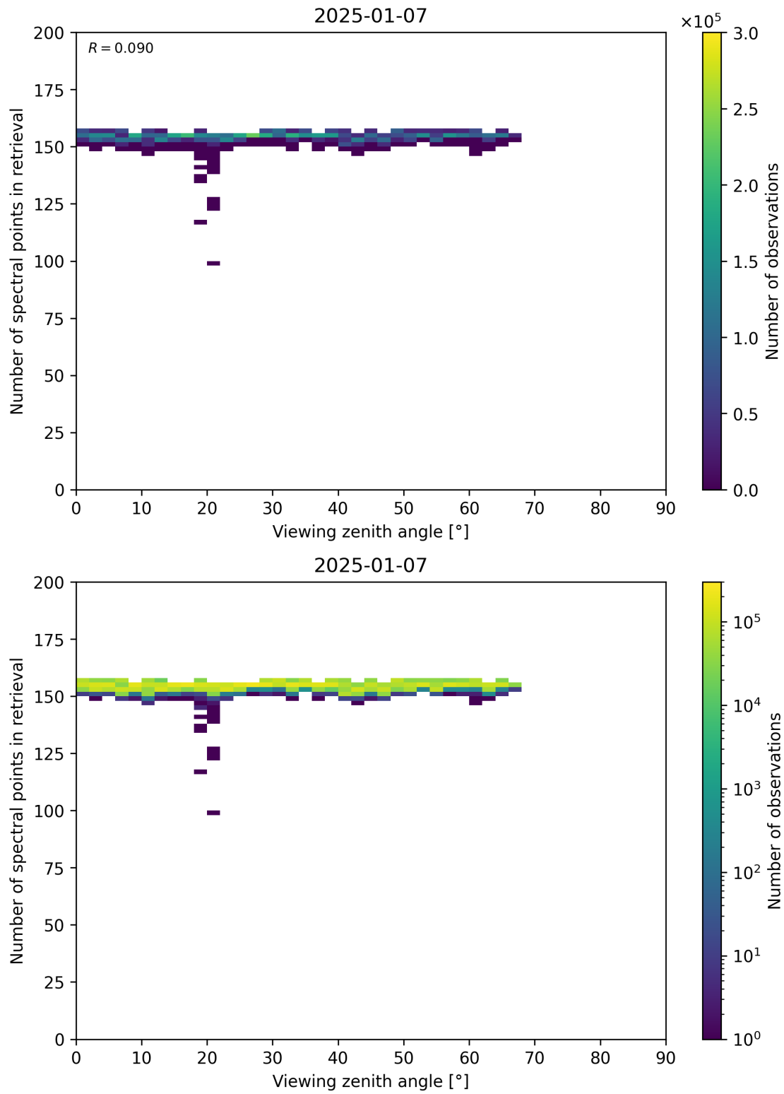
Figure 76: Scatter density plot of “Viewing zenith angle” against “Number of spectral points in retrieval” for 2025-01-07 to 2025-01-08.
