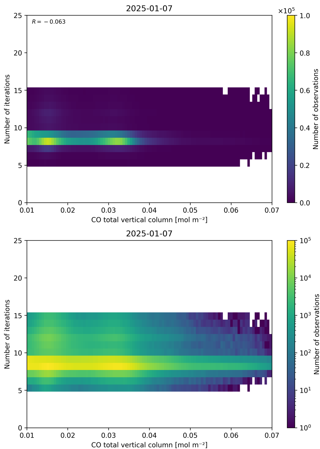
Figure 42: Scatter density plot of “CO total vertical column” against “Number of iterations” for 2025-01-07 to 2025-01-08.
