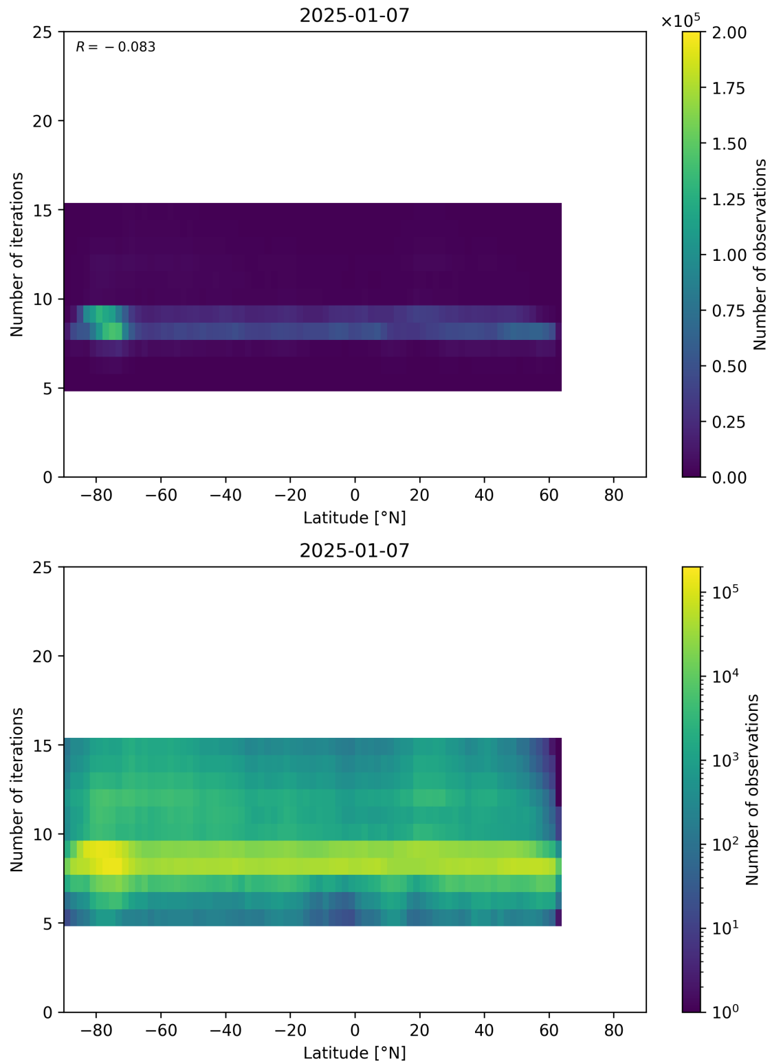
Figure 56: Scatter density plot of “Latitude” against “Number of iterations” for 2025-01-07 to 2025-01-08.
