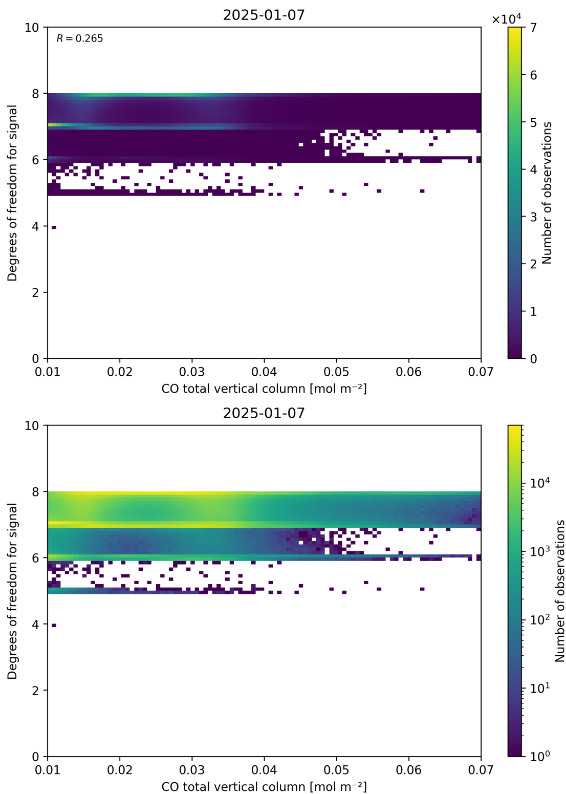
Figure 41: Scatter density plot of “CO total vertical column” against “Degrees of freedom for signal” for 2025-01-07 to 2025-01-08.
