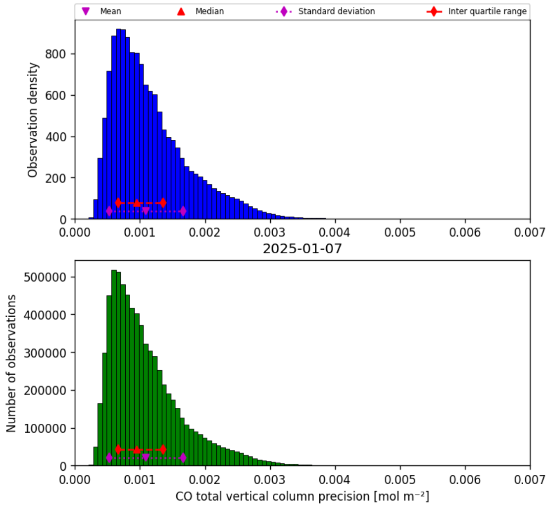
Figure 20: Histogram of “CO total vertical column precision” for 2025-01-07 to 2025-01-08
