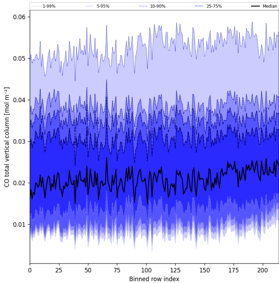
Figure 26: Along track statistics of “CO total vertical column” for 2025-01-07 to 2025-01-08
