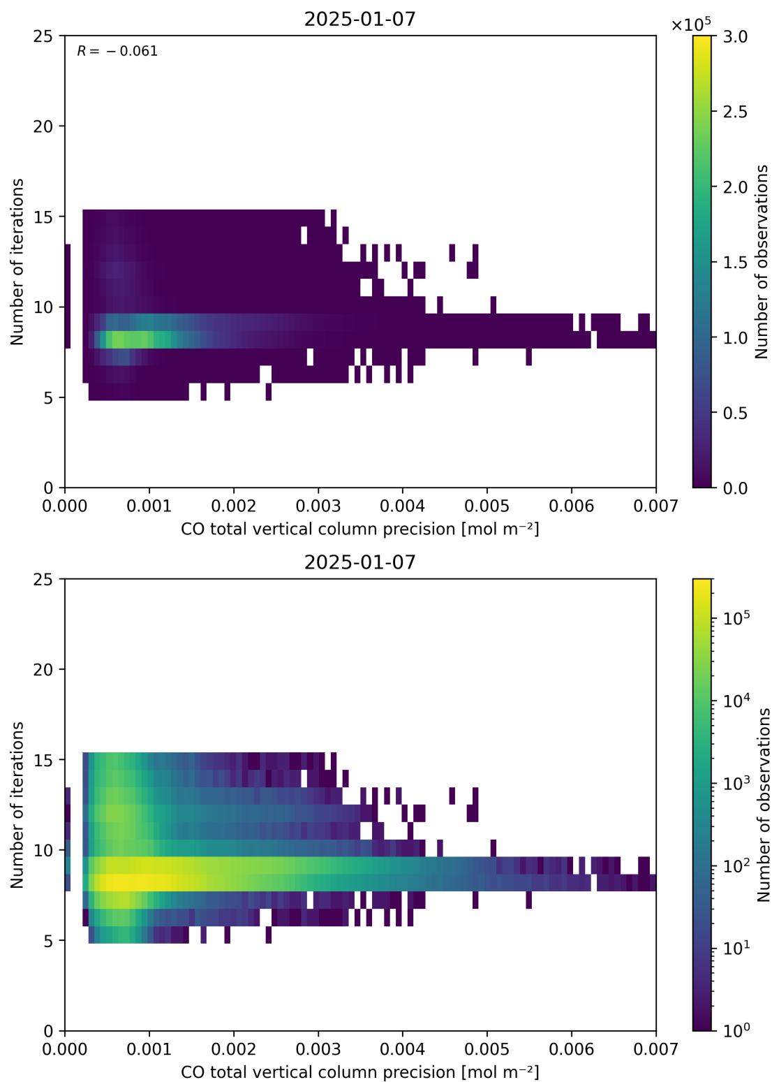
Figure 46: Scatter density plot of “CO total vertical column precision” against “Number of iterations” for 2025-01-07 to 2025-01-08.
