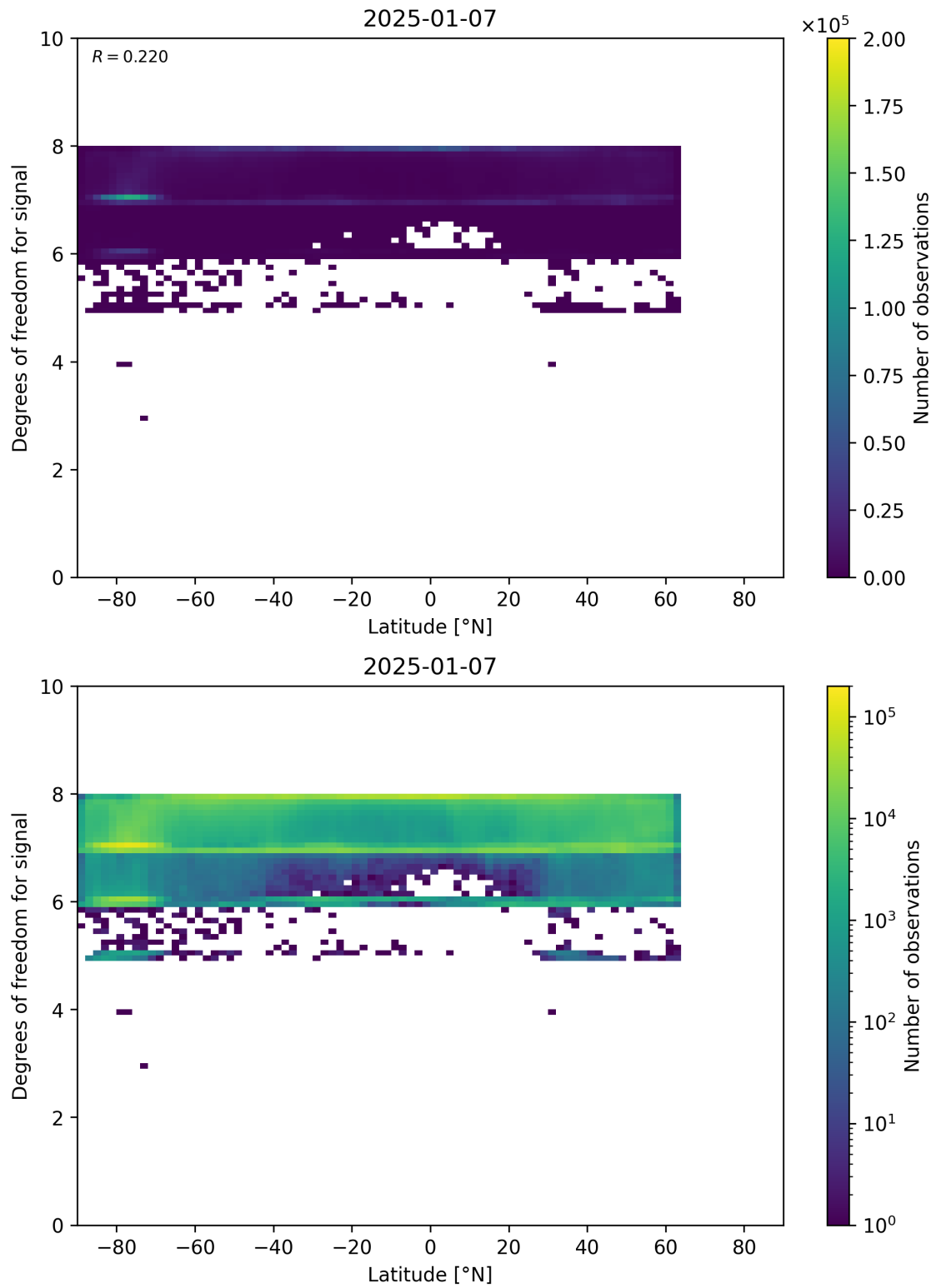
Figure 55: Scatter density plot of “Latitude” against “Degrees of freedom for signal” for 2025-01-07 to 2025-01-08.
