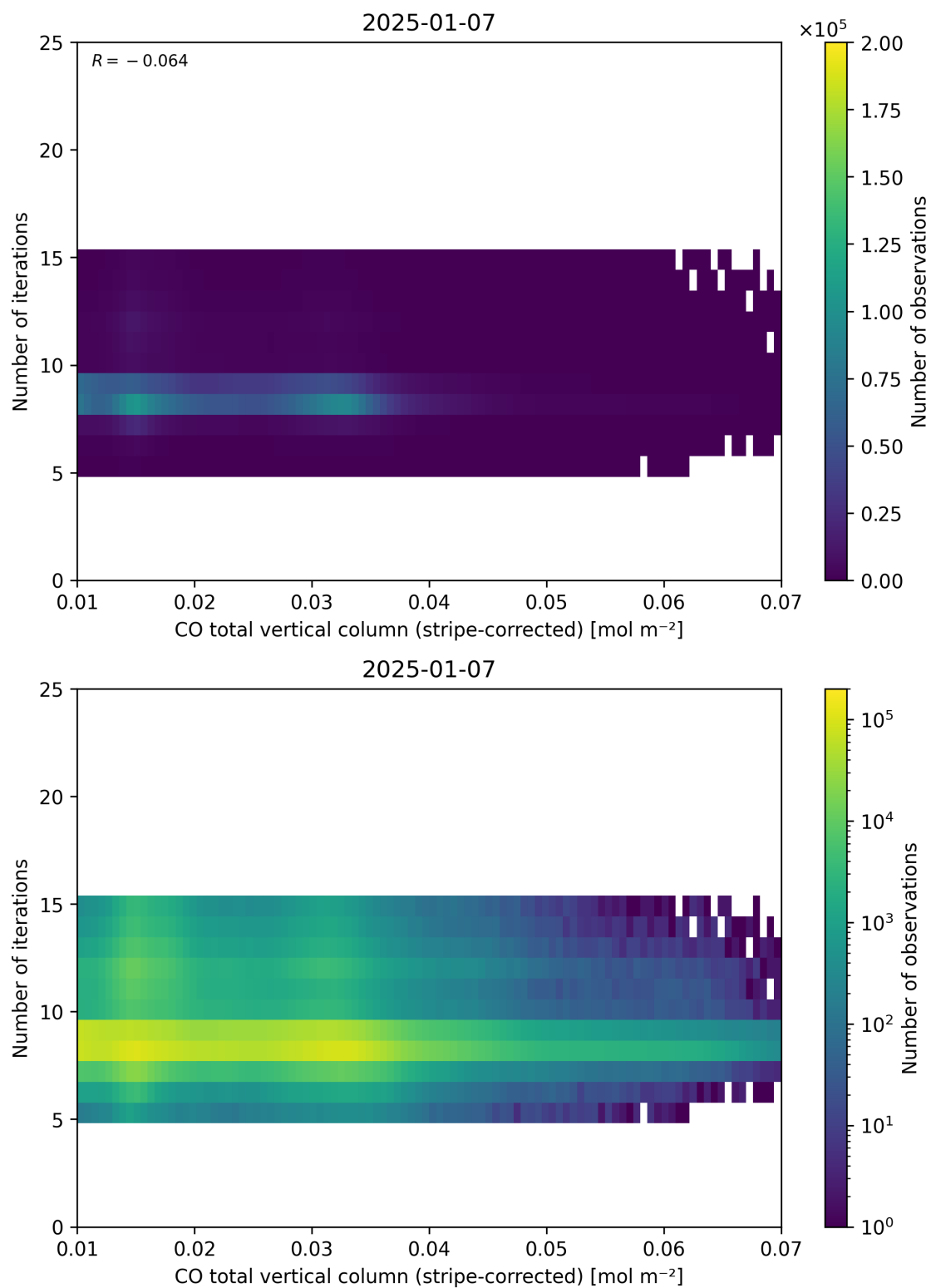
Figure 39: Scatter density plot of “CO total vertical column (stripe-corrected)” against “Number of iterations” for 2025-01-07 to 2025-01-08.
