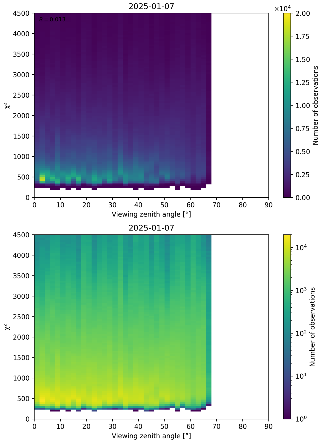
Figure 72: Scatter density plot of “Viewing zenith angle” against “ \chi^2 ” for 2025-01-07 to 2025-01-08.
