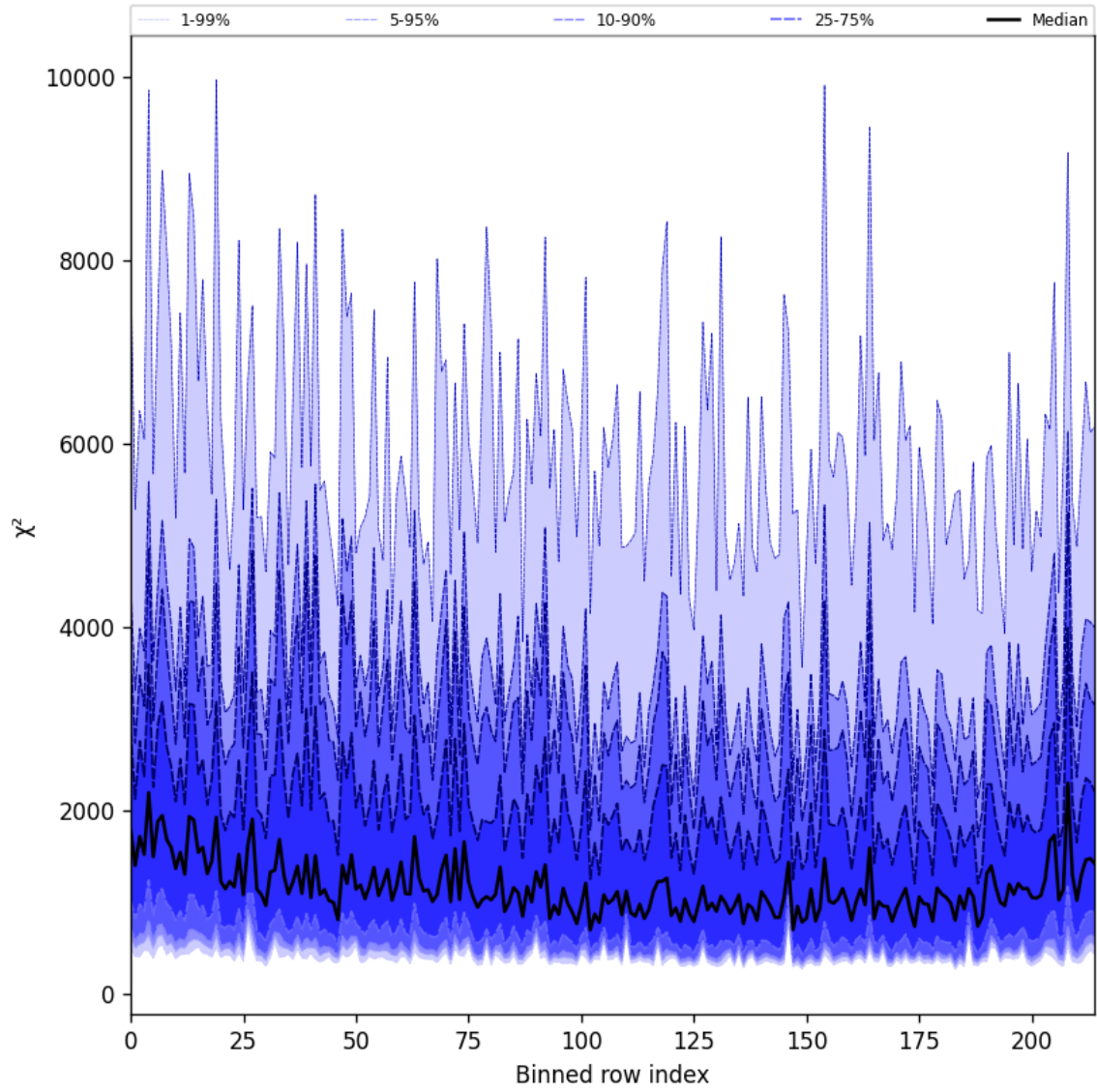
Figure 30: Along track statistics of “ \chi^2 ” for 2025-01-07 to 2025-01-08
