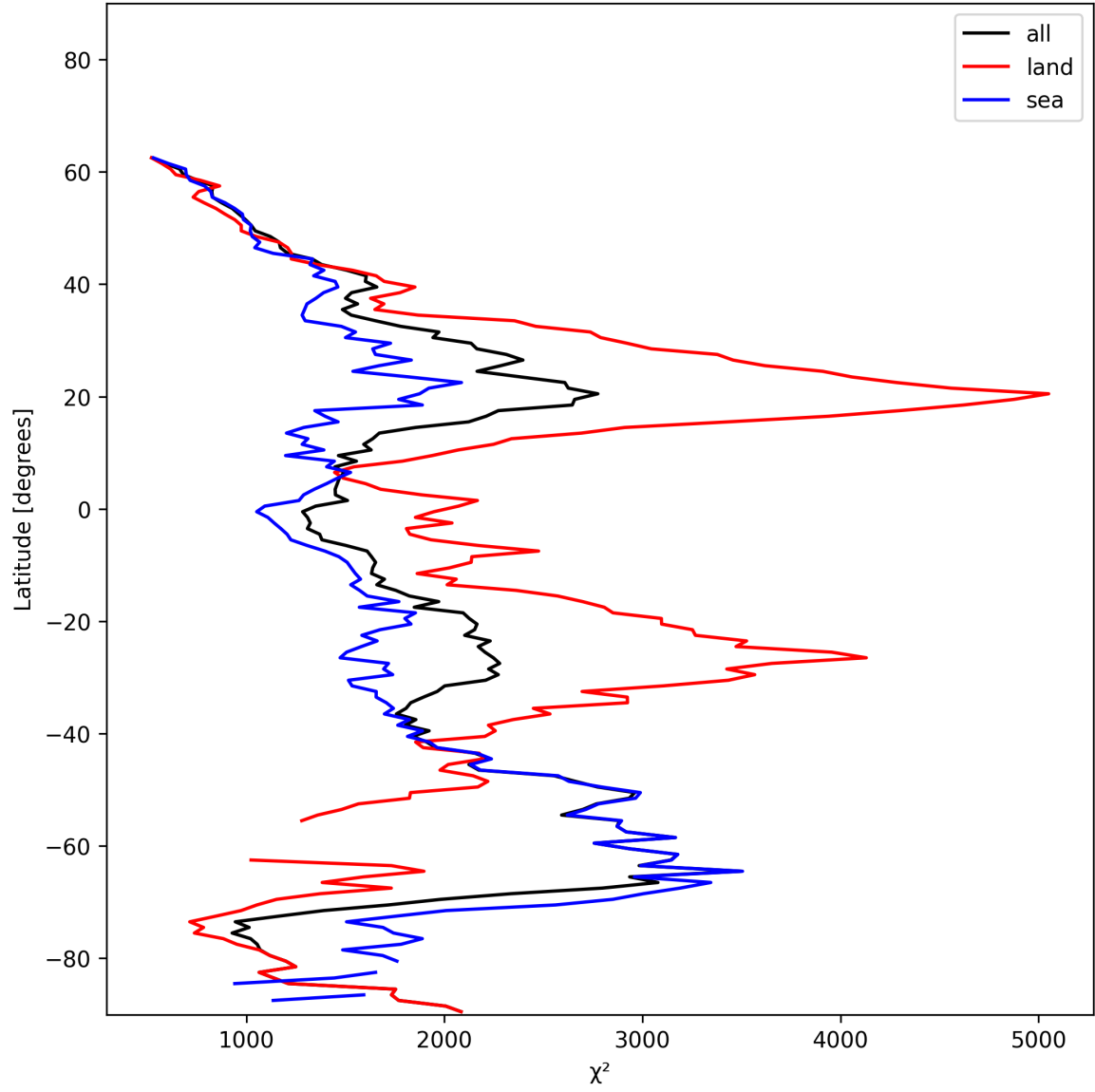
Figure 14: Zonal average of “ \chi^2 ” for 2025-01-07 to 2025-01-08.
