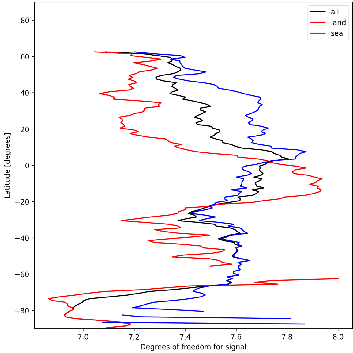
Figure 15: Zonal average of “Degrees of freedom for signal” for 2025-01-07 to 2025-01-08.
