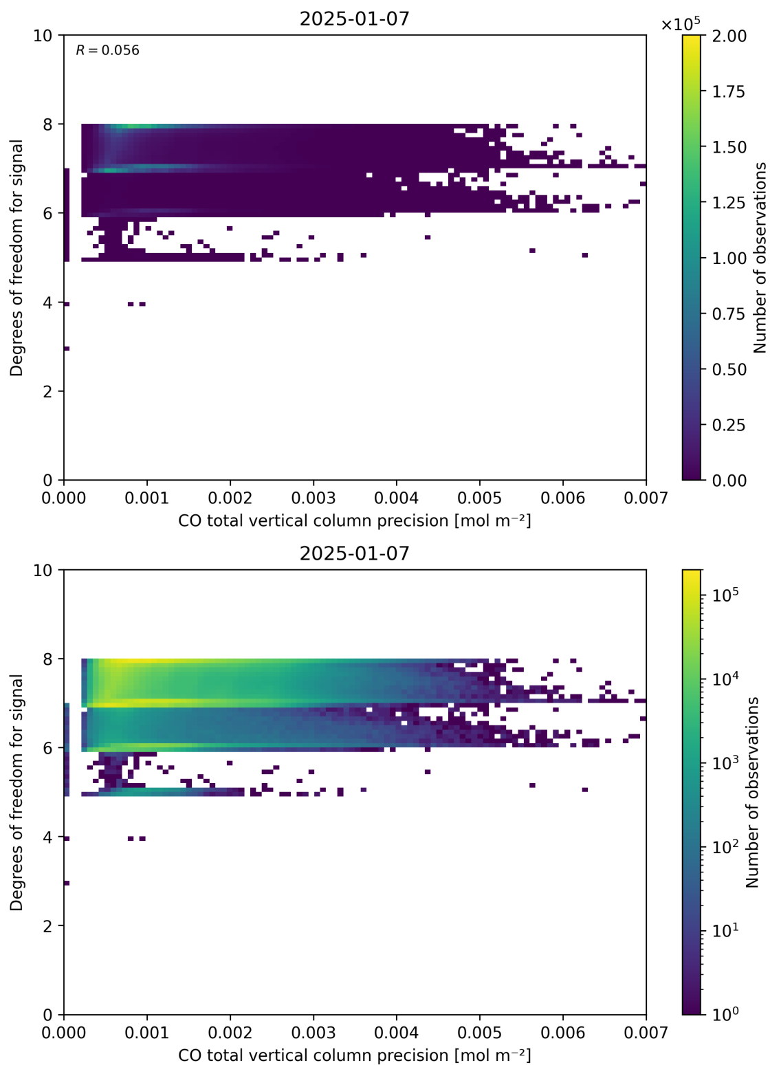
Figure 45: Scatter density plot of “CO total vertical column precision” against “Degrees of freedom for signal” for 2025-01-07 to 2025-01-08.
