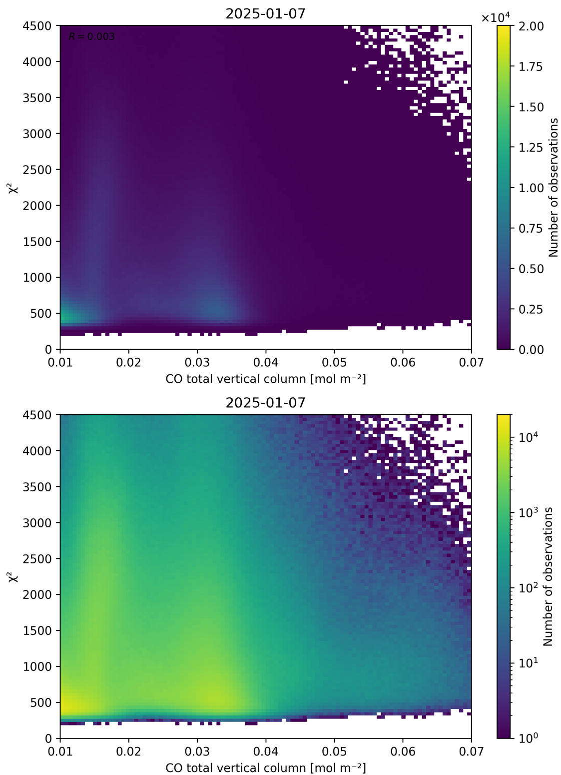
Figure 35: Scatter density plot of “CO total vertical column” against “ \chi^2 ” for 2025-01-07 to 2025-01-08.
