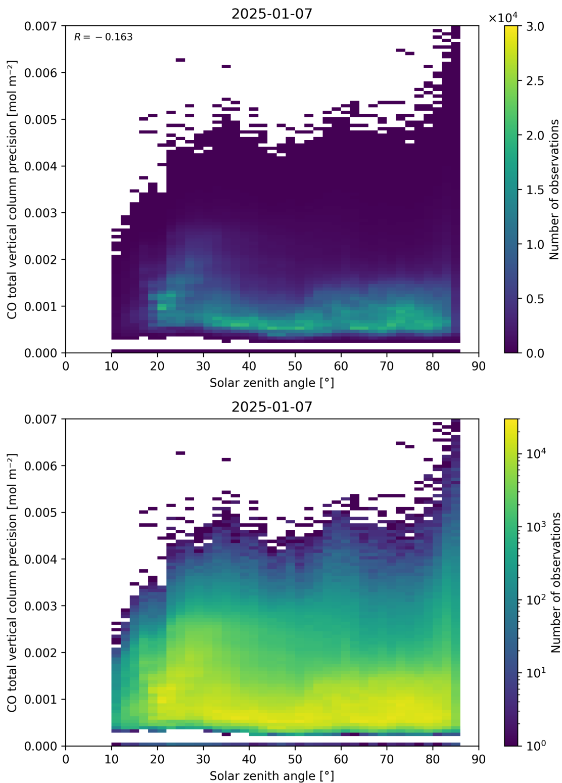
Figure 63: Scatter density plot of “Solar zenith angle” against “CO total vertical column precision” for 2025-01-07 to 2025-01-08.
