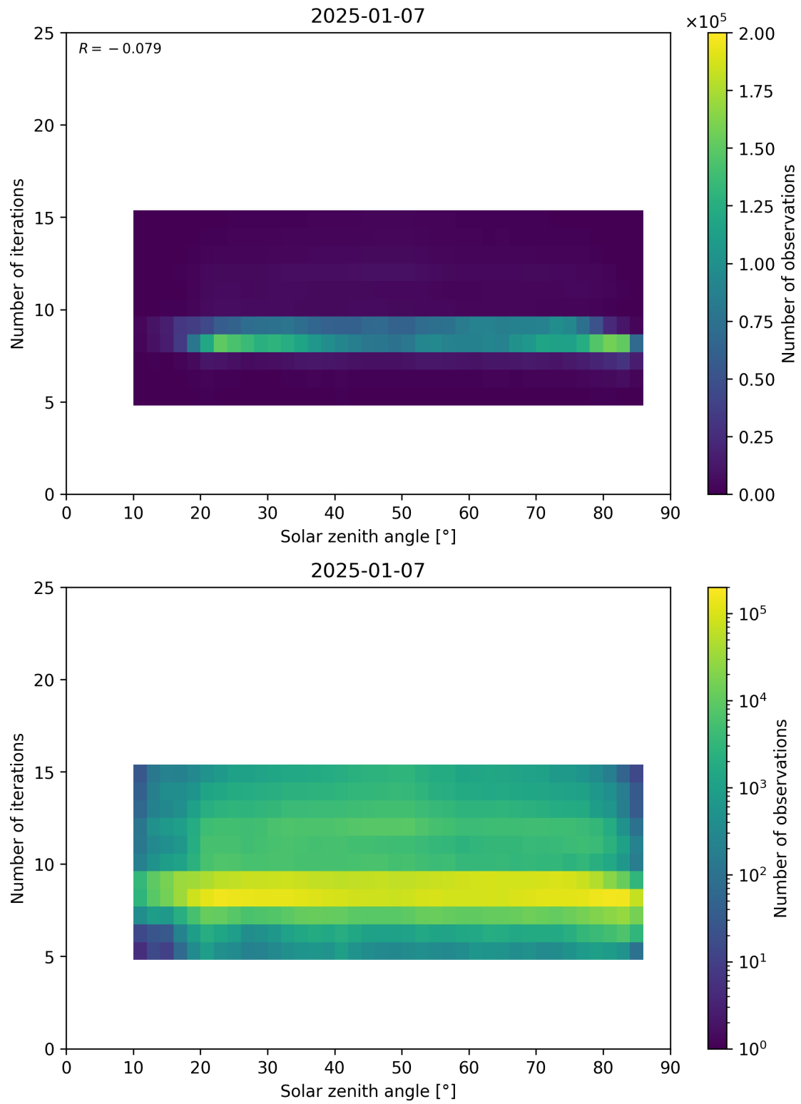
Figure 67: Scatter density plot of “Solar zenith angle” against “Number of iterations” for 2025-01-07 to 2025-01-08.
