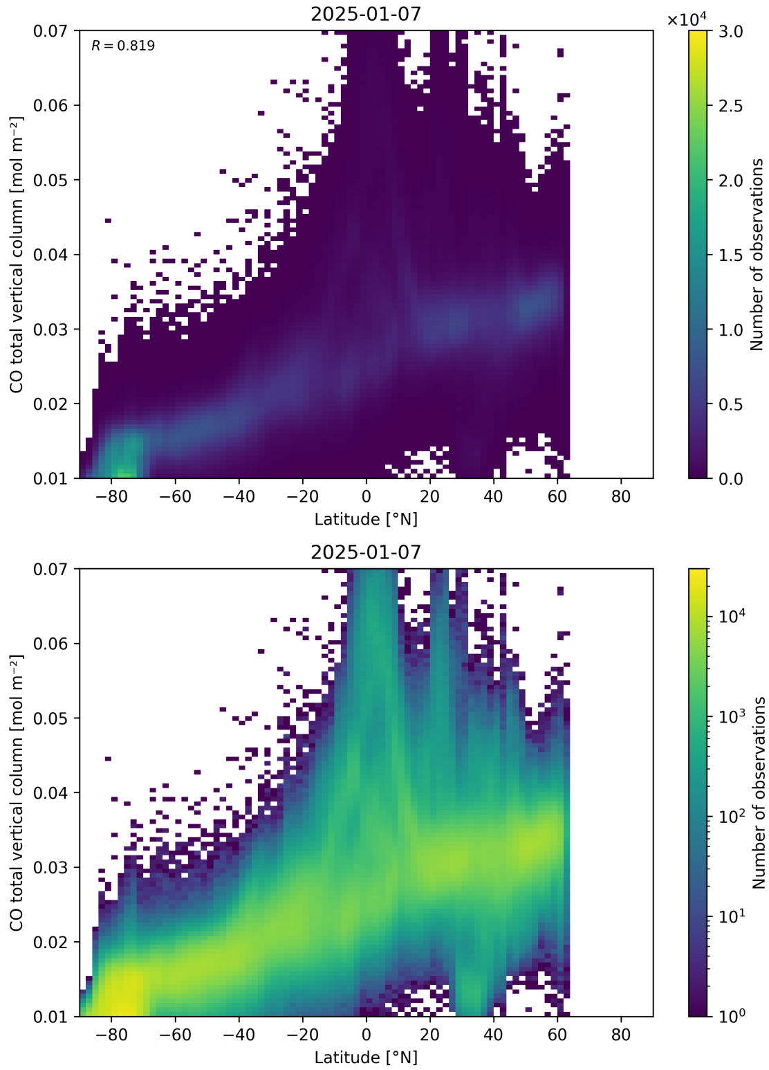
Figure 51: Scatter density plot of “Latitude” against “CO total vertical column” for 2025-01-07 to 2025-01-08.
