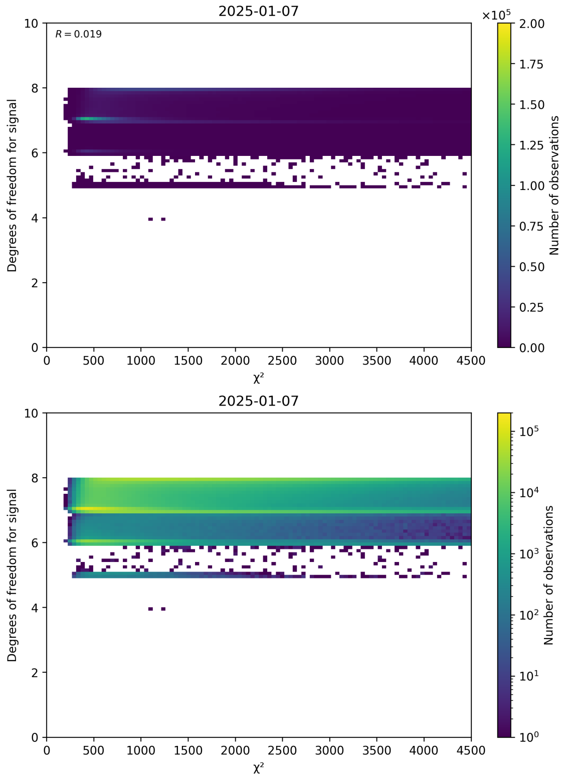
Figure 48: Scatter density plot of “ \chi^2 ” against “Degrees of freedom for signal” for 2025-01-07 to 2025-01-08.
