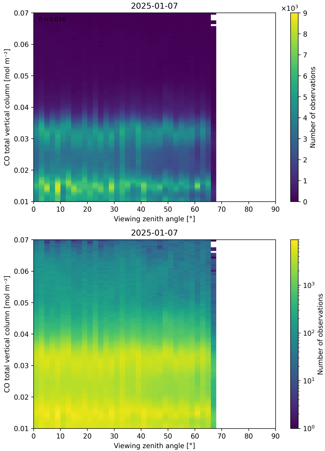
Figure 69: Scatter density plot of “Viewing zenith angle” against “CO total vertical column” for 2025-01-07 to 2025-01-08.
