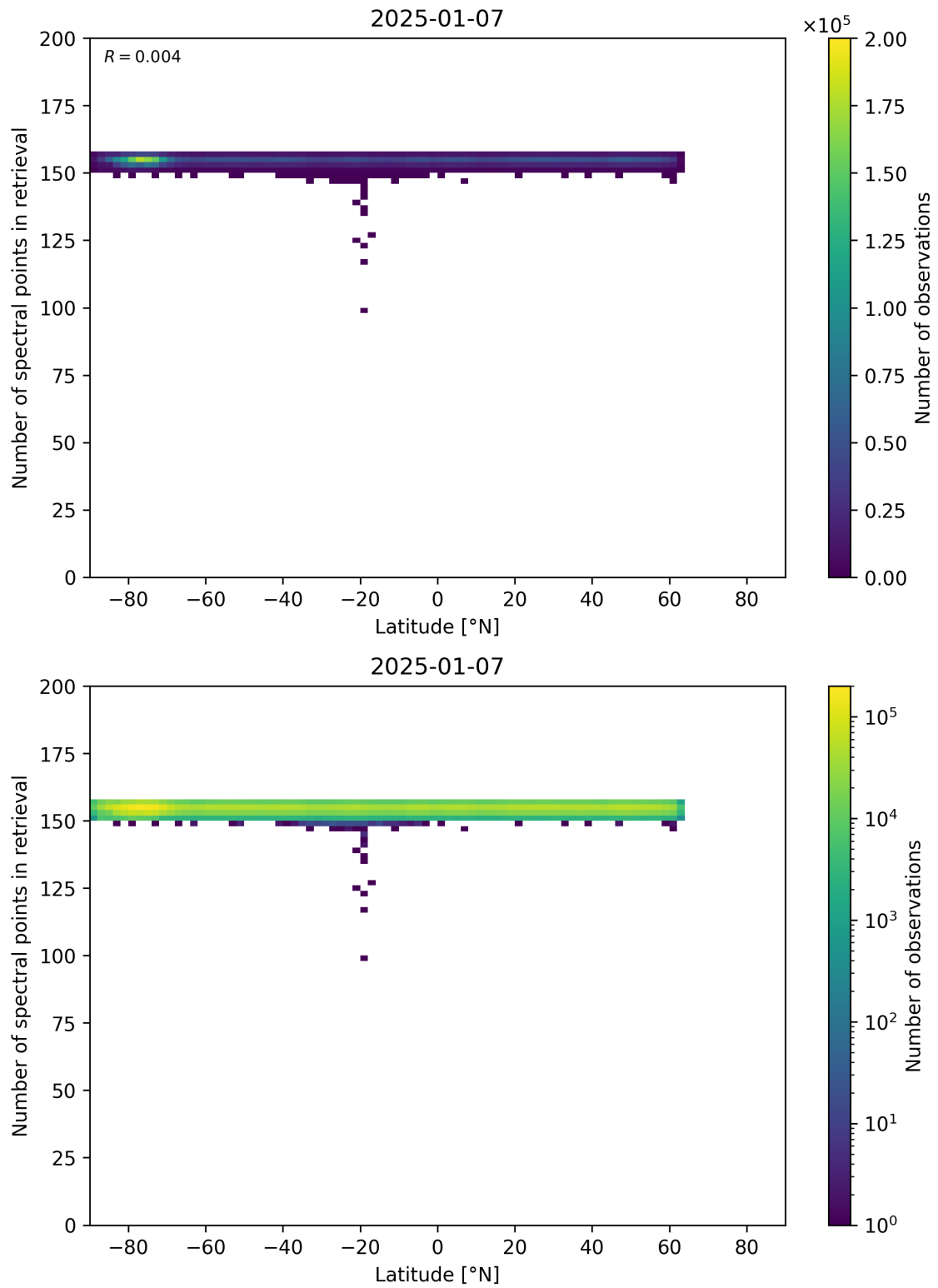
Figure 57: Scatter density plot of “Latitude” against “Number of spectral points in retrieval” for 2025-01-07 to 2025-01-08.
