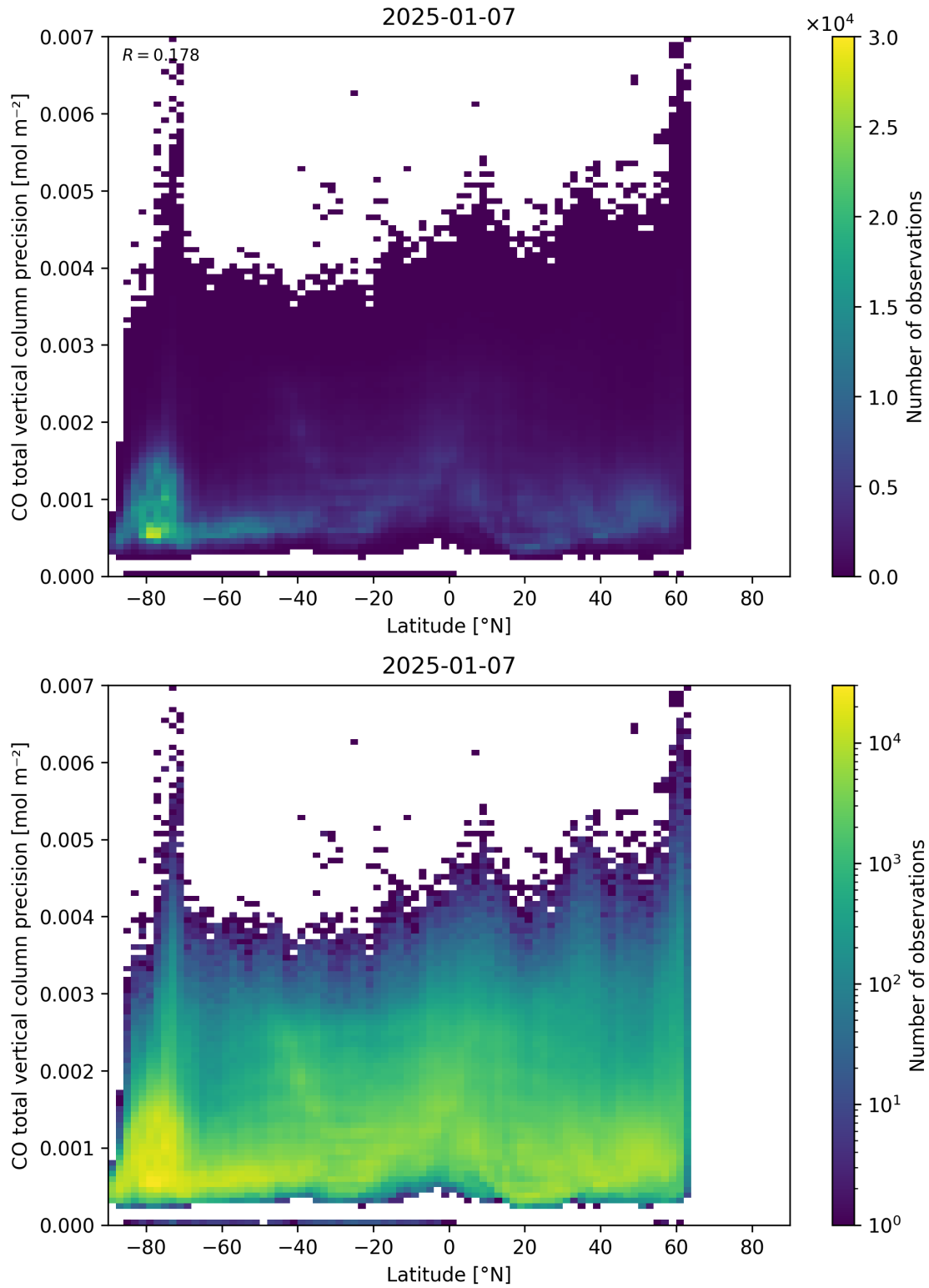
Figure 53: Scatter density plot of “Latitude” against “CO total vertical column precision” for 2025-01-07 to 2025-01-08.
