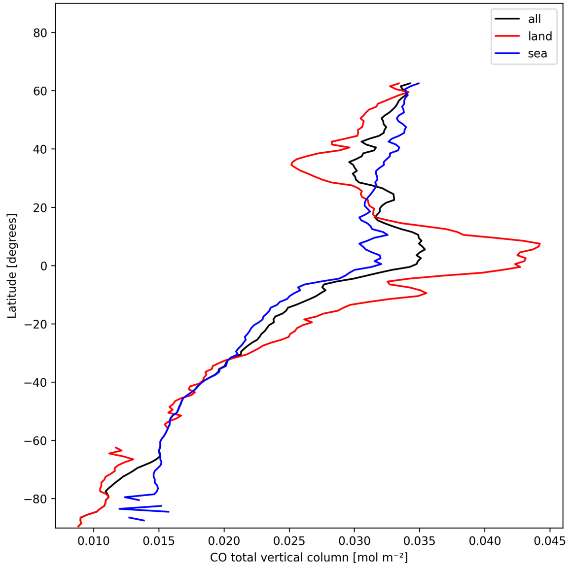
Figure 10: Zonal average of “CO total vertical column” for 2025-01-07 to 2025-01-08.
