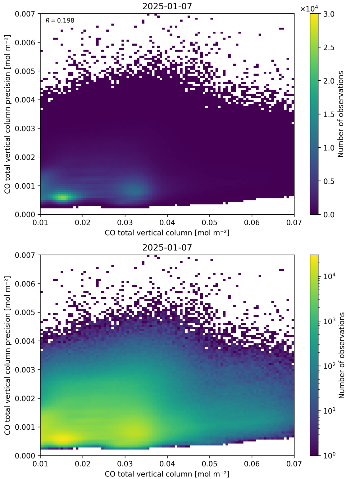
Figure 34: Scatter density plot of “CO total vertical column” against “CO total vertical column precision” for 2025-01-07 to 2025-01-08.
