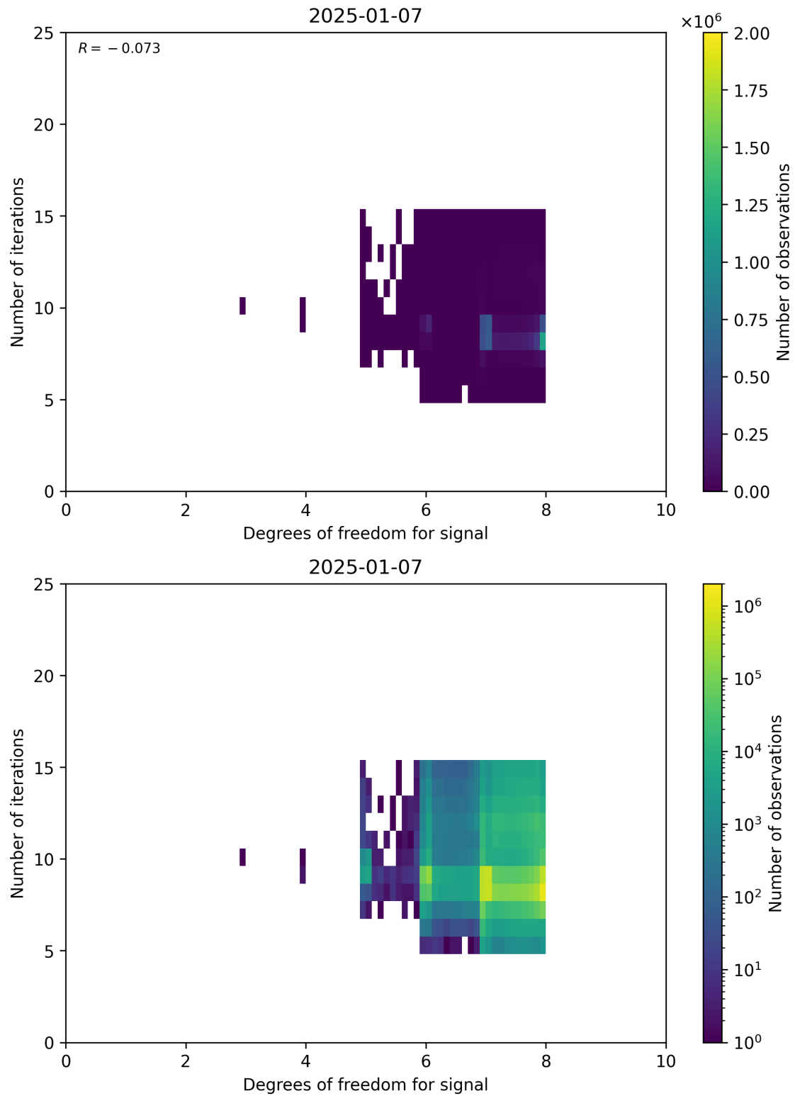
Figure 50: Scatter density plot of “Degrees of freedom for signal” against “Number of iterations” for 2025-01-07 to 2025-01-08.
