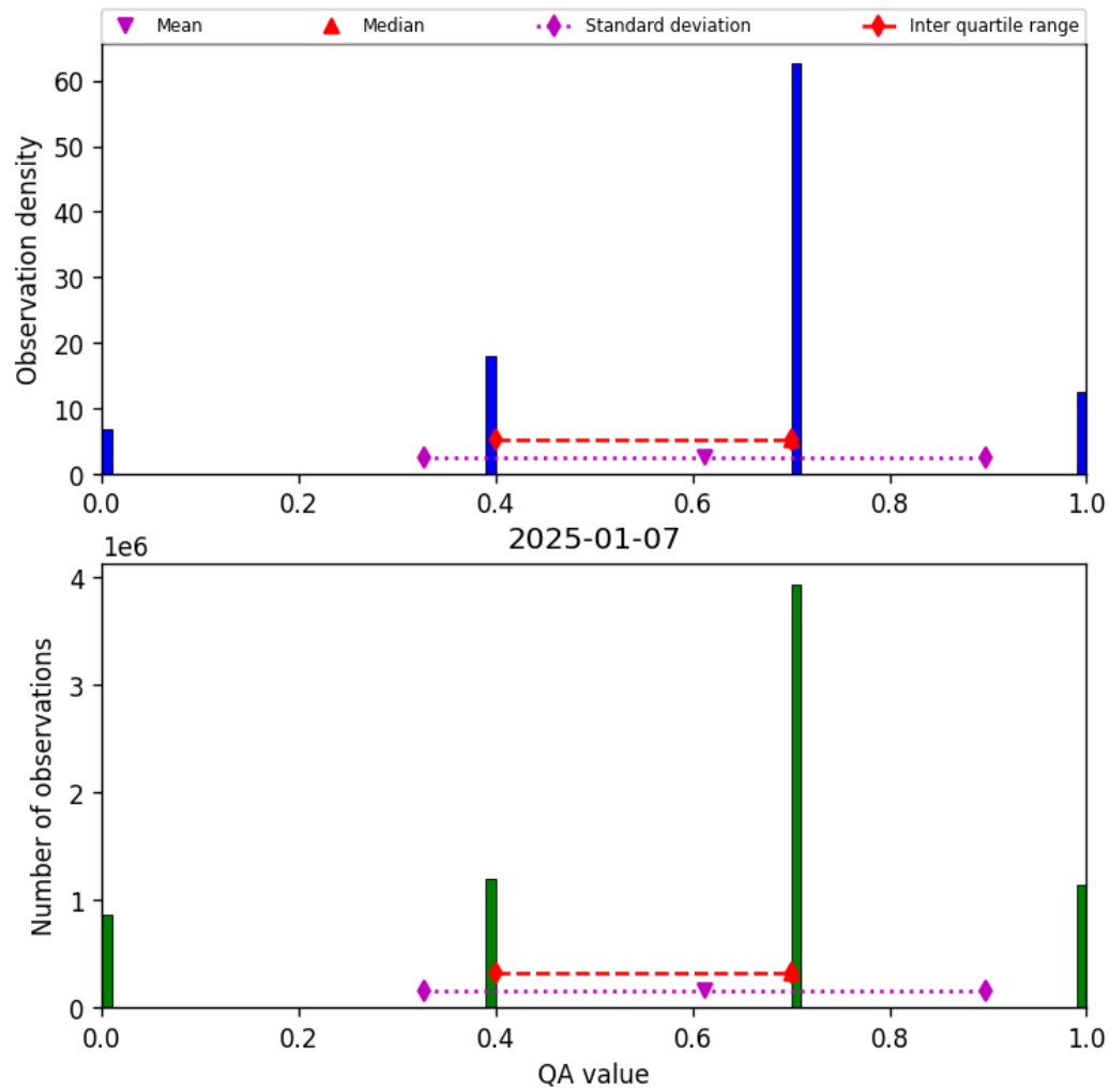
Figure 17: Histogram of “QA value” for 2025-01-07 to 2025-01-08
