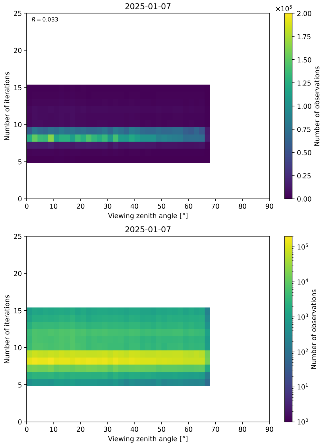
Figure 75: Scatter density plot of “Viewing zenith angle” against “Number of iterations” for 2025-01-07 to 2025-01-08.
