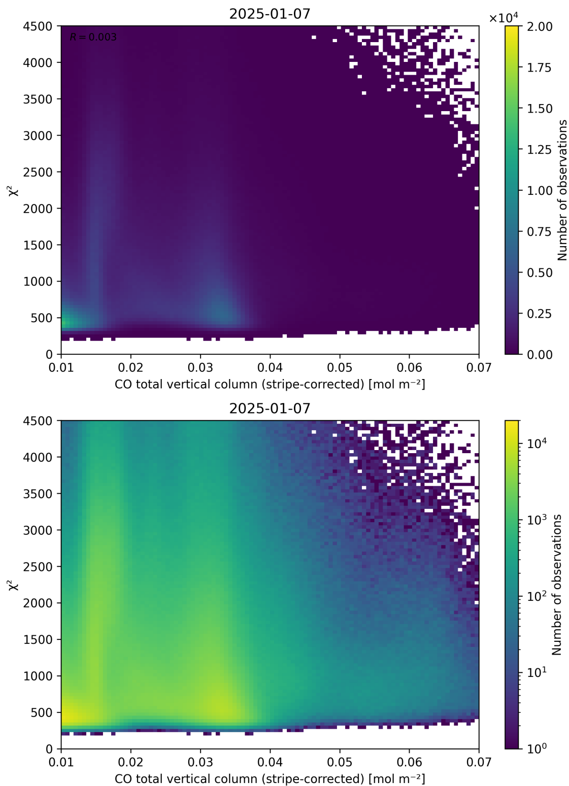
Figure 37: Scatter density plot of “CO total vertical column (stripe-corrected)” against “ \chi^2 ” for 2025-01-07 to 2025-01-08.
