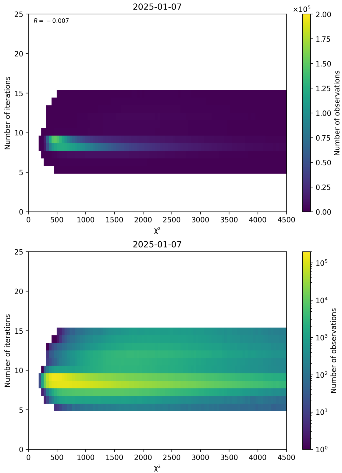
Figure 49: Scatter density plot of “ \chi^2 ” against “Number of iterations” for 2025-01-07 to 2025-01-08.
