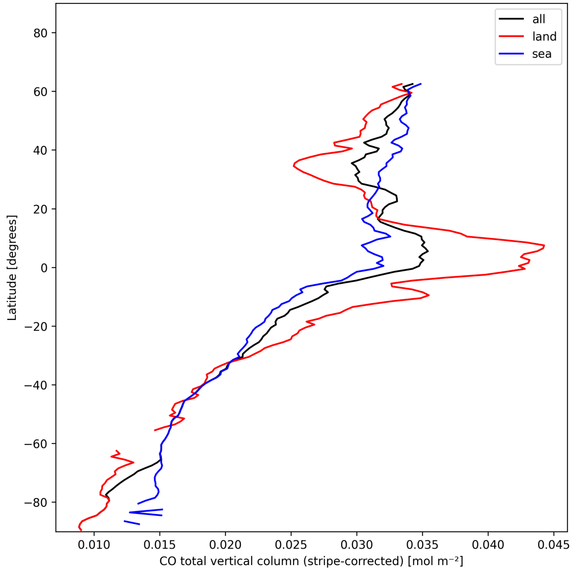
Figure 11: Zonal average of “CO total vertical column (stripe-corrected)” for 2025-01-07 to 2025-01-08.
