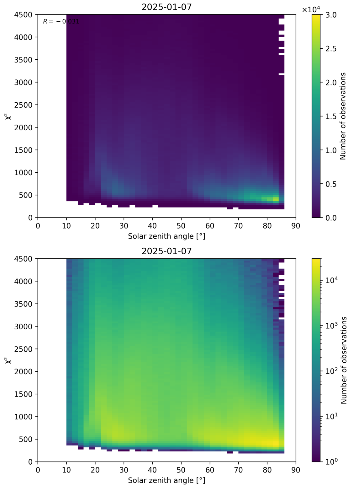
Figure 64: Scatter density plot of “Solar zenith angle” against “ \chi^2 ” for 2025-01-07 to 2025-01-08.
