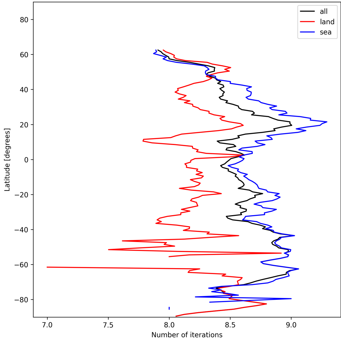
Figure 16: Zonal average of “Number of iterations” for 2025-01-07 to 2025-01-09.
