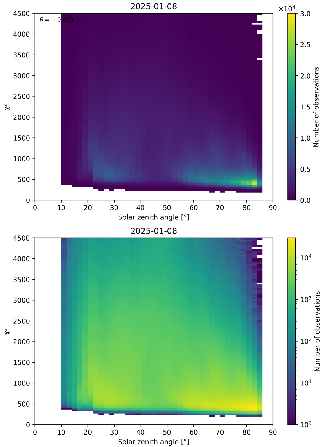
Figure 64: Scatter density plot of “Solar zenith angle” against “ \chi^2 ” for 2025-01-07 to 2025-01-09.
