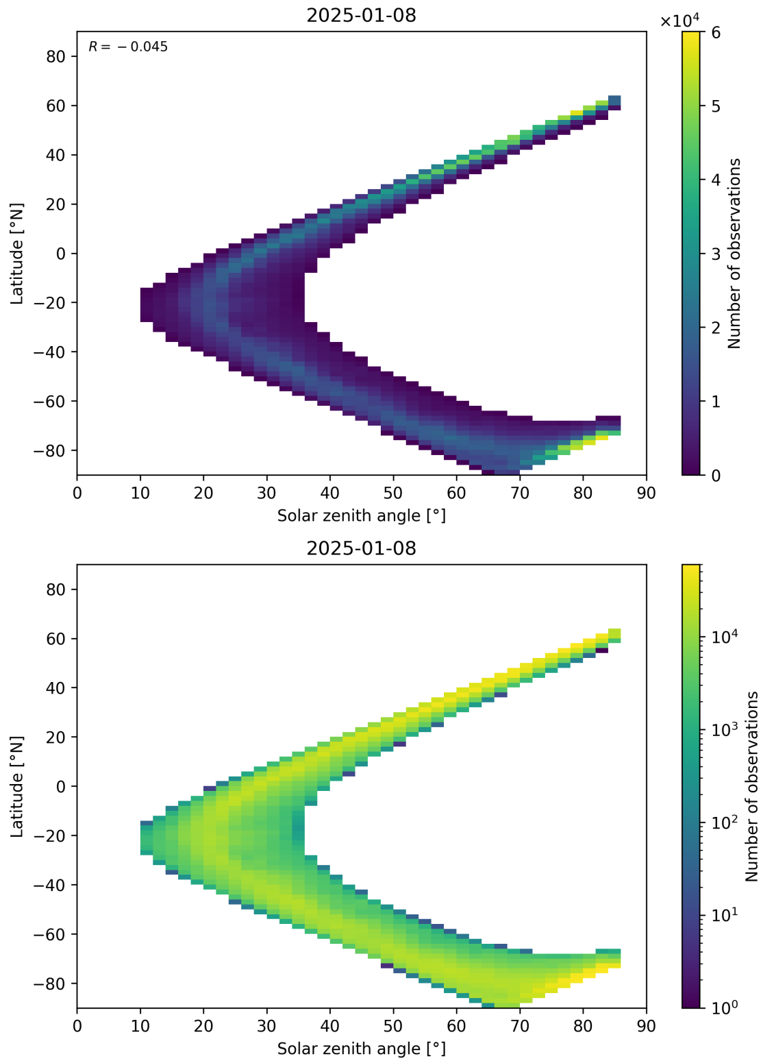
Figure 66: Scatter density plot of “Solar zenith angle” against “Latitude” for 2025-01-07 to 2025-01-09.
