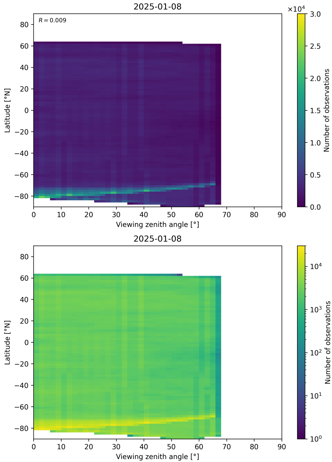
Figure 74: Scatter density plot of “Viewing zenith angle” against “Latitude” for 2025-01-07 to 2025-01-09.
