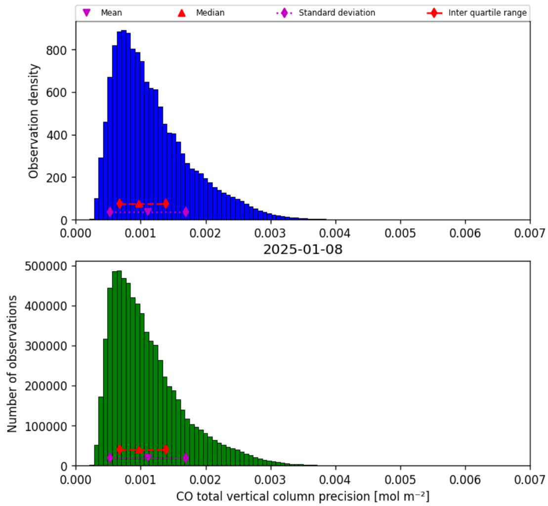
Figure 20: Histogram of “CO total vertical column precision” for 2025-01-07 to 2025-01-09
