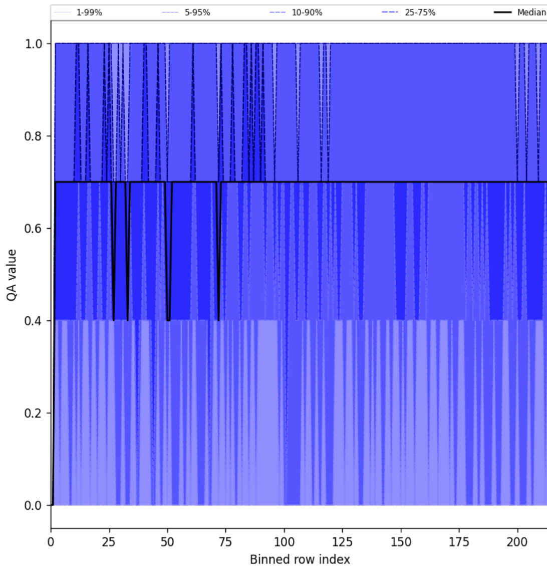
Figure 25: Along track statistics of “QA value” for 2025-01-07 to 2025-01-09
