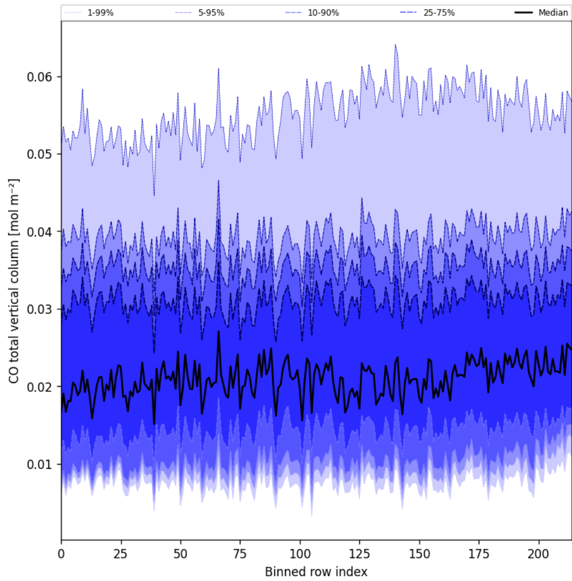
Figure 26: Along track statistics of “CO total vertical column” for 2025-01-07 to 2025-01-09
