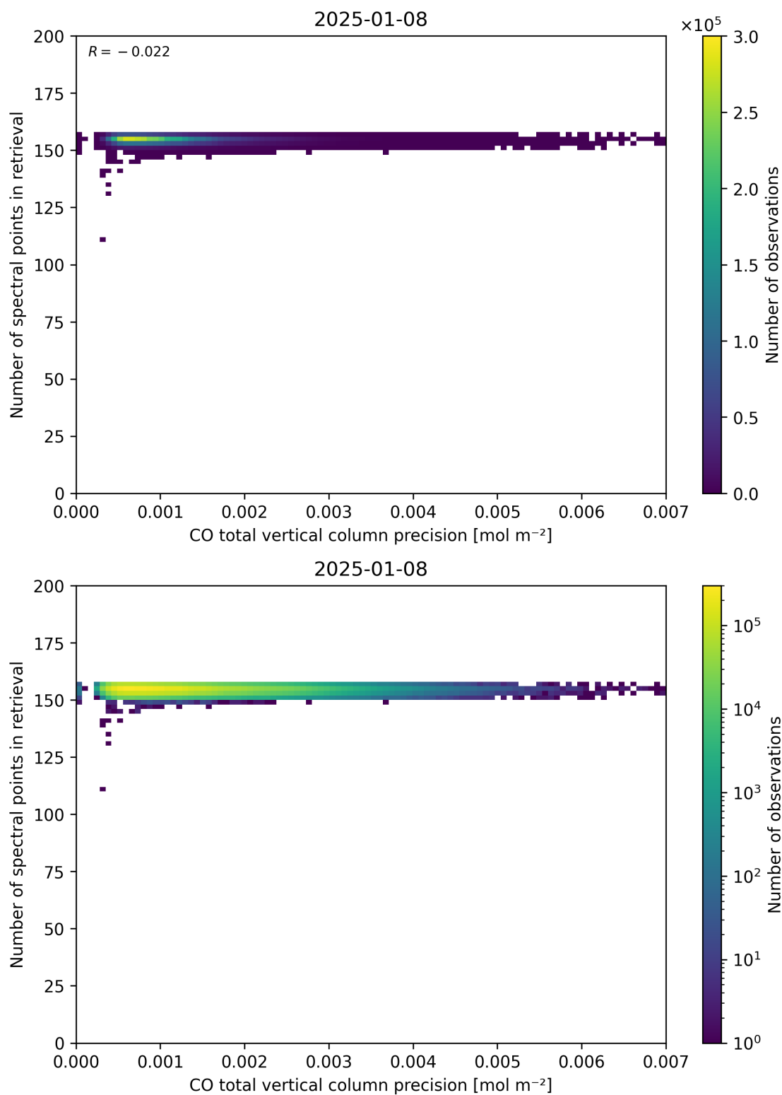
Figure 47: Scatter density plot of “CO total vertical column precision” against “Number of spectral points in retrieval” for 2025-01-07 to 2025-01-09.
