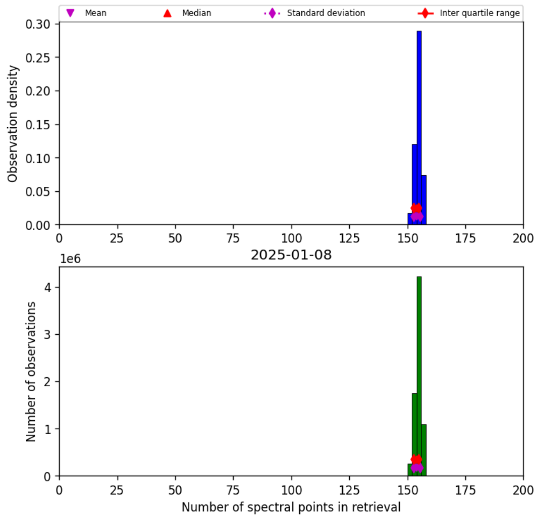
Figure 21: Histogram of “Number of spectral points in retrieval” for 2025-01-07 to 2025-01-09
