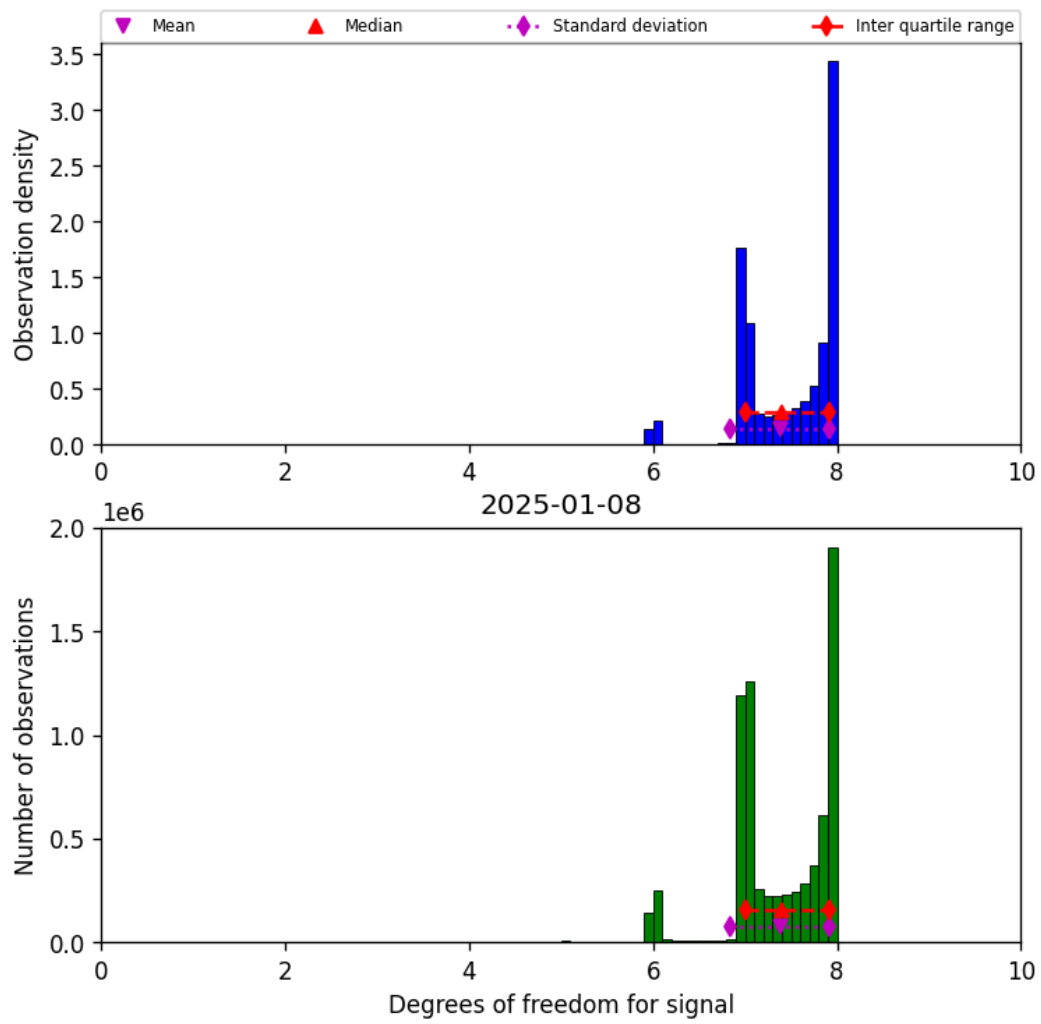
Figure 23: Histogram of “Degrees of freedom for signal” for 2025-01-07 to 2025-01-09
