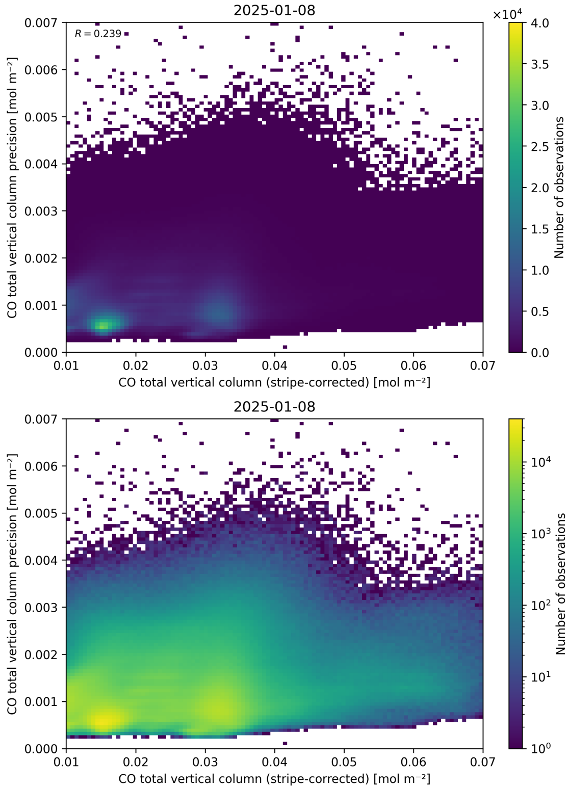
Figure 36: Scatter density plot of “CO total vertical column (stripe-corrected)” against “CO total vertical column precision” for 2025-01-07 to 2025-01-09.
