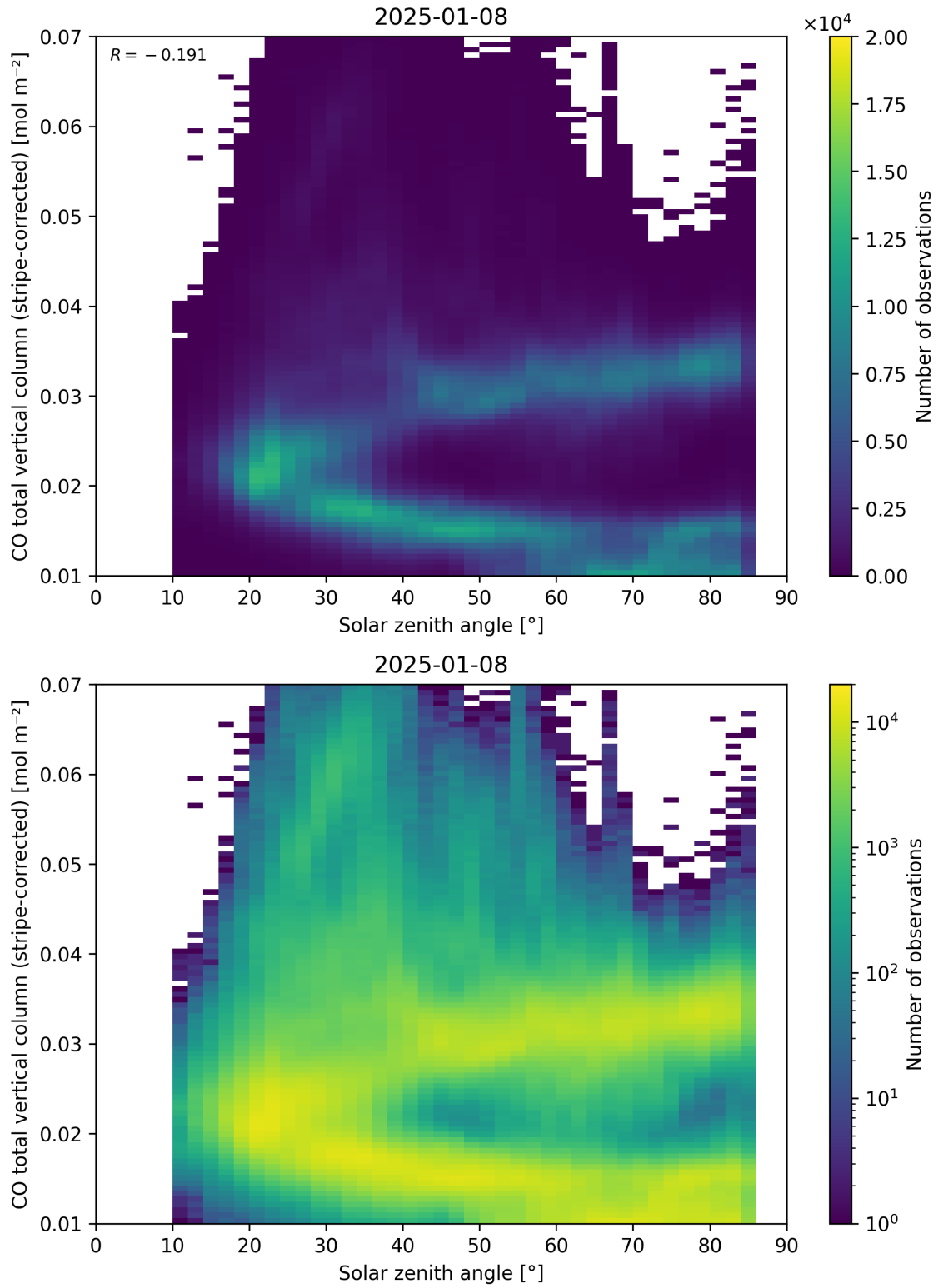
Figure 62: Scatter density plot of “Solar zenith angle” against “CO total vertical column (stripe-corrected)” for 2025-01-07 to 2025-01-09.
