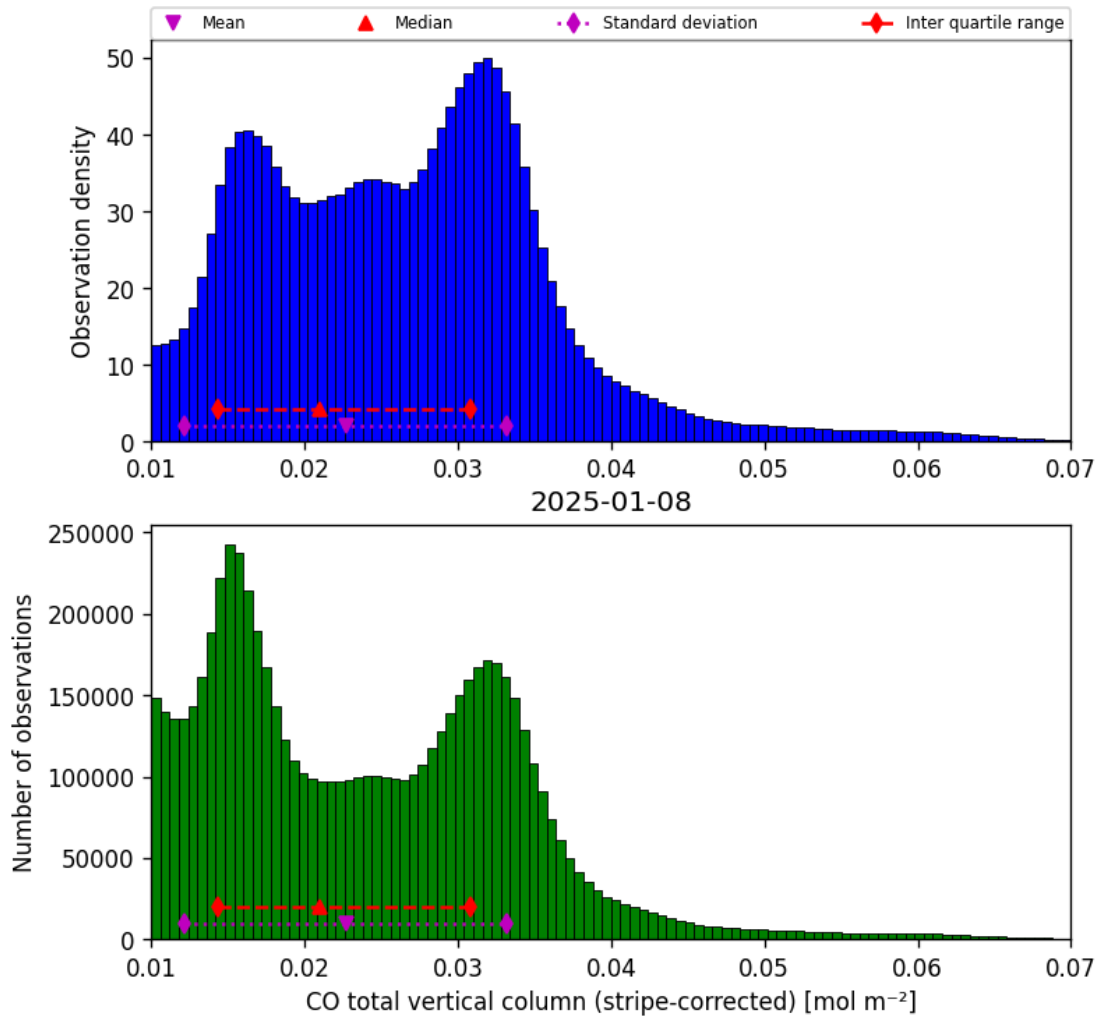
Figure 19: Histogram of “CO total vertical column (stripe-corrected)” for 2025-01-07 to 2025-01-09
