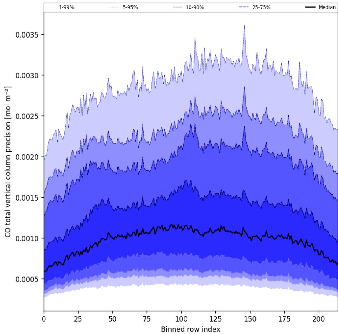
Figure 28: Along track statistics of “CO total vertical column precision” for 2025-01-07 to 2025-01-09
