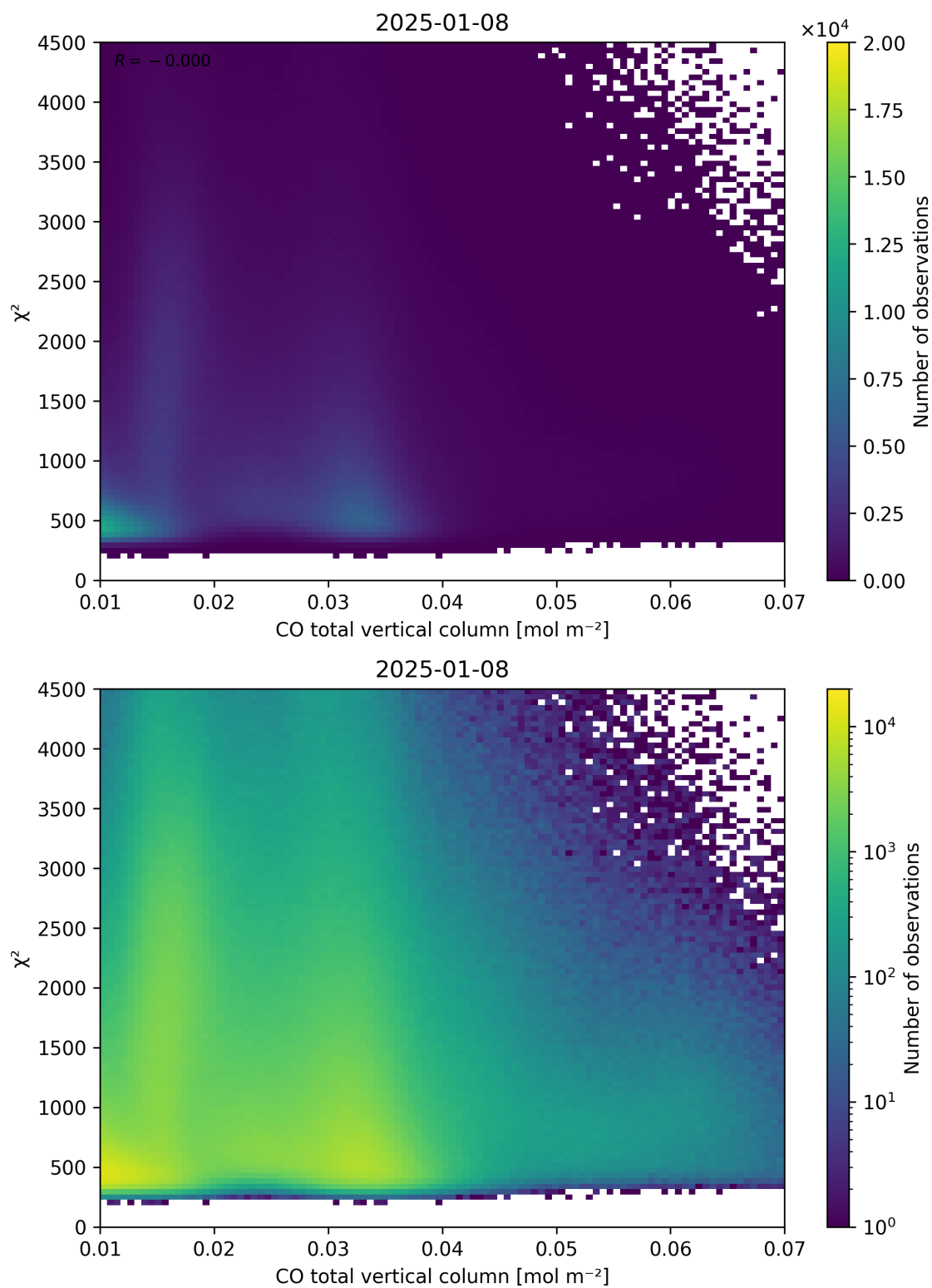
Figure 35: Scatter density plot of “CO total vertical column” against “ \chi^2 ” for 2025-01-07 to 2025-01-09.
