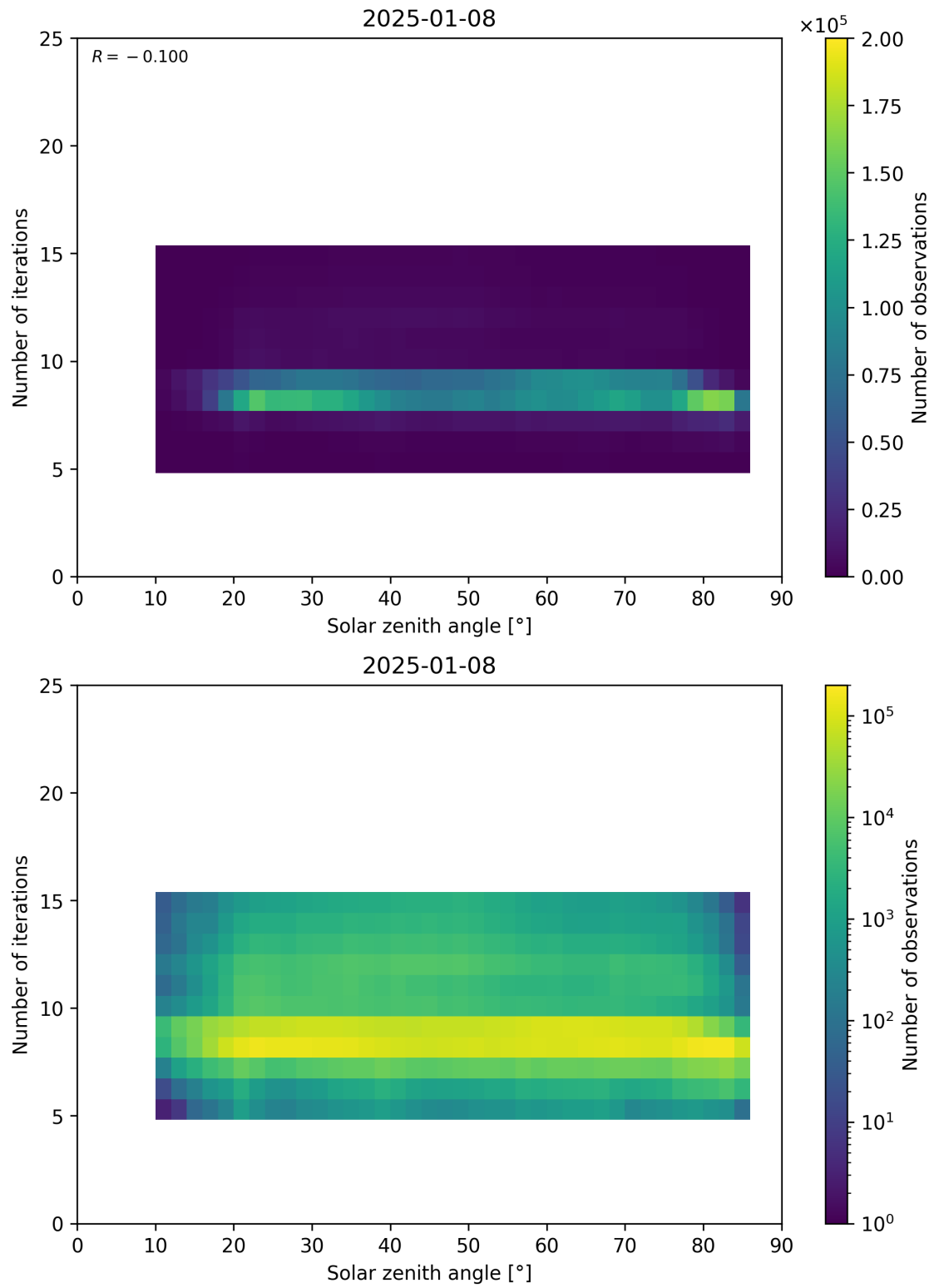
Figure 67: Scatter density plot of “Solar zenith angle” against “Number of iterations” for 2025-01-07 to 2025-01-09.
