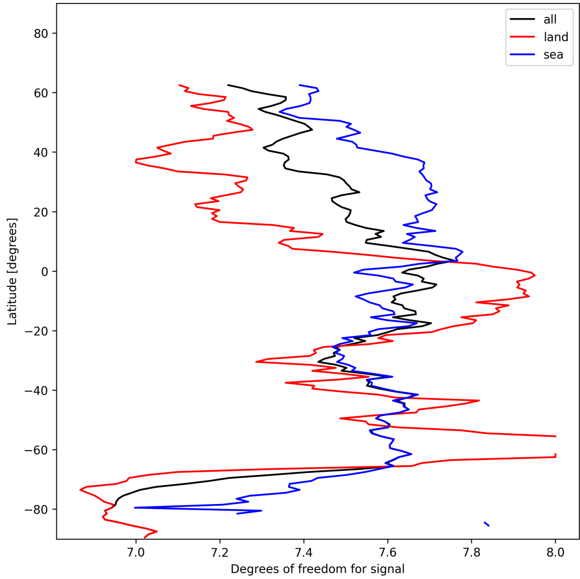
Figure 15: Zonal average of “Degrees of freedom for signal” for 2025-01-07 to 2025-01-09.
