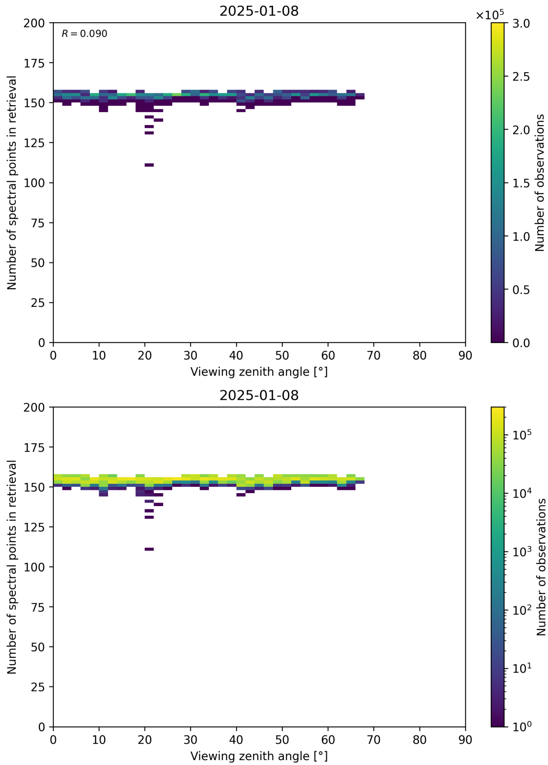
Figure 76: Scatter density plot of “Viewing zenith angle” against “Number of spectral points in retrieval” for 2025-01-07 to 2025-01-09.
