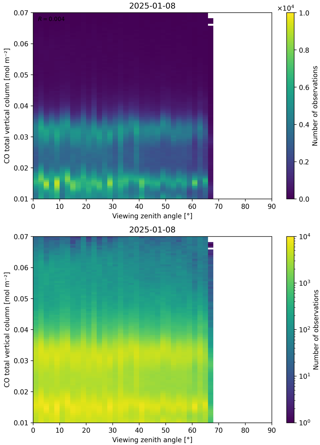
Figure 69: Scatter density plot of “Viewing zenith angle” against “CO total vertical column” for 2025-01-07 to 2025-01-09.
