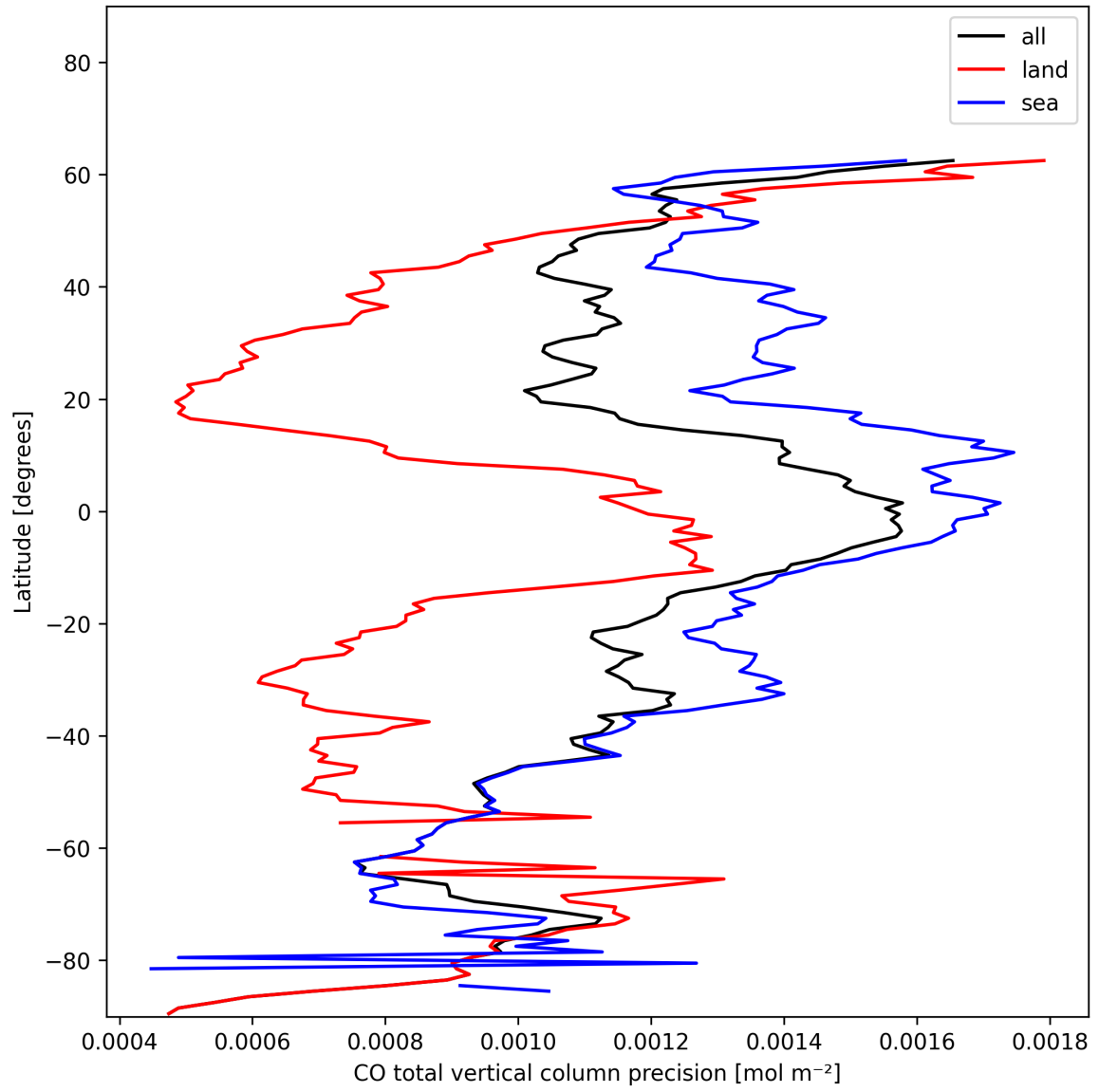
Figure 12: Zonal average of “CO total vertical column precision” for 2025-01-07 to 2025-01-09.
