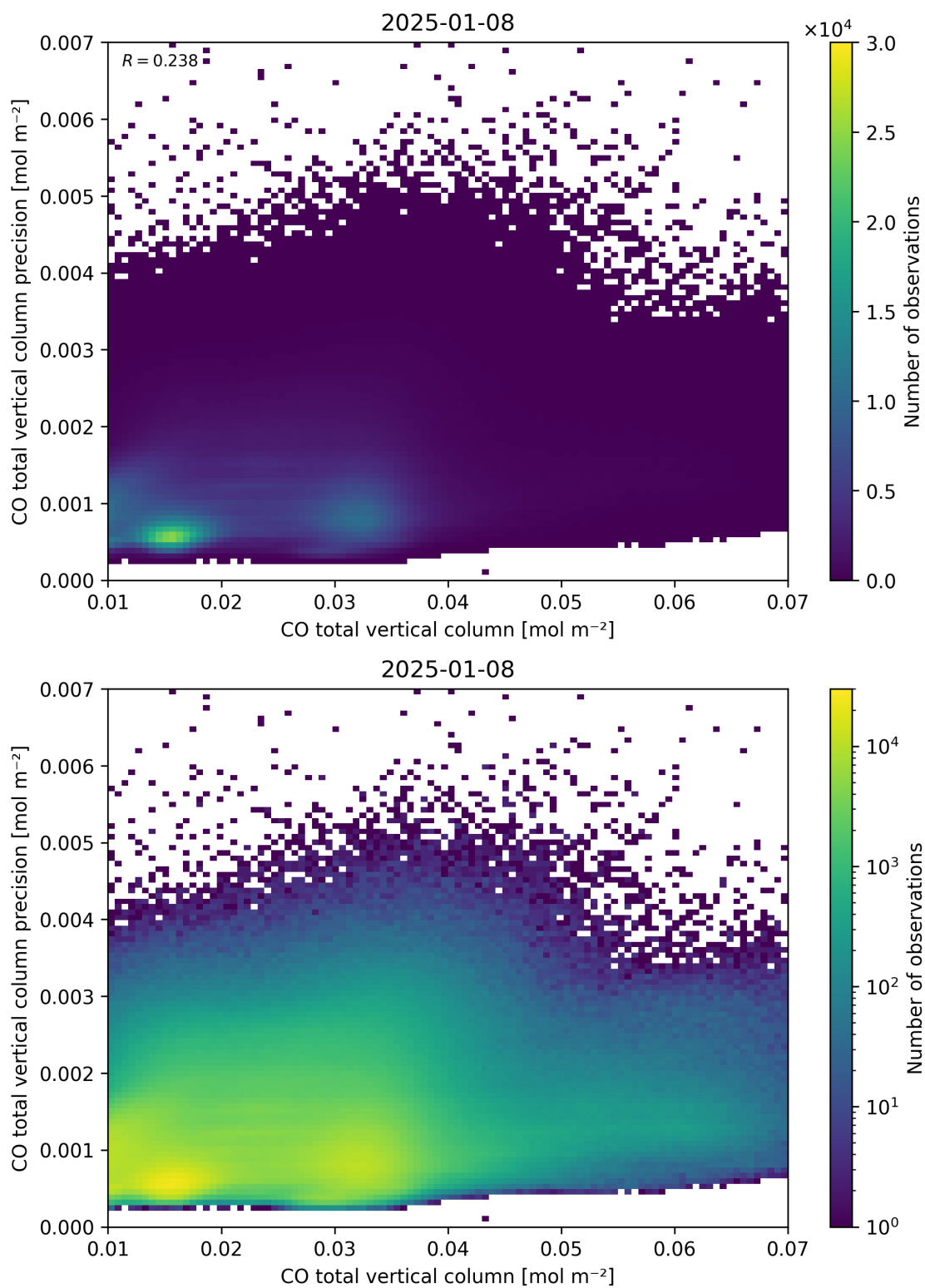
Figure 34: Scatter density plot of “CO total vertical column” against “CO total vertical column precision” for 2025-01-07 to 2025-01-09.
