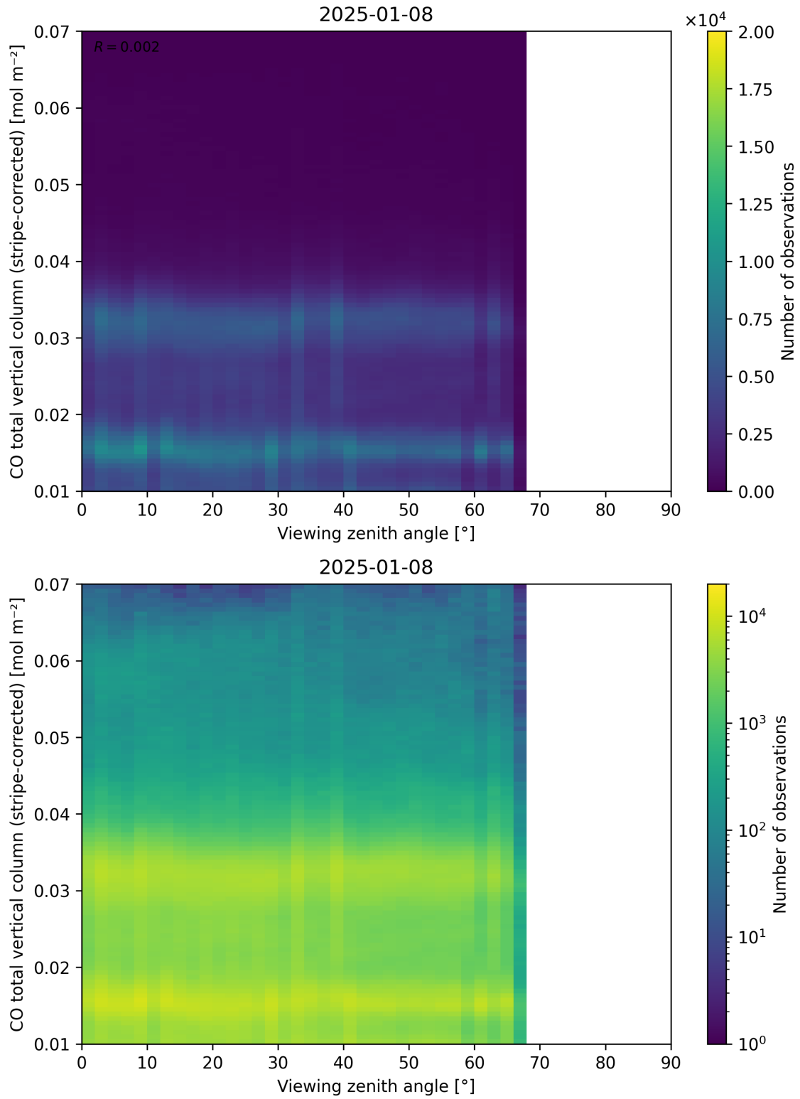
Figure 70: Scatter density plot of “Viewing zenith angle” against “CO total vertical column (stripe-corrected)” for 2025-01-07 to 2025-01-09.
