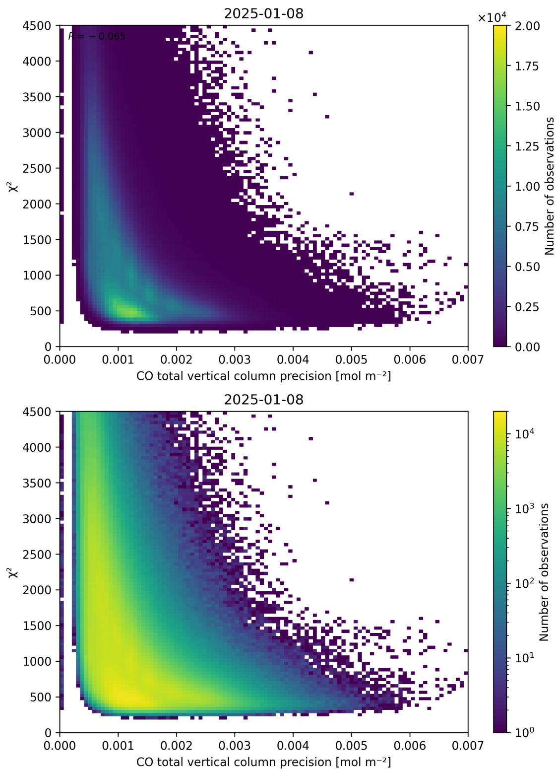
Figure 44: Scatter density plot of “CO total vertical column precision” against “ \chi^2 ” for 2025-01-07 to 2025-01-09.
