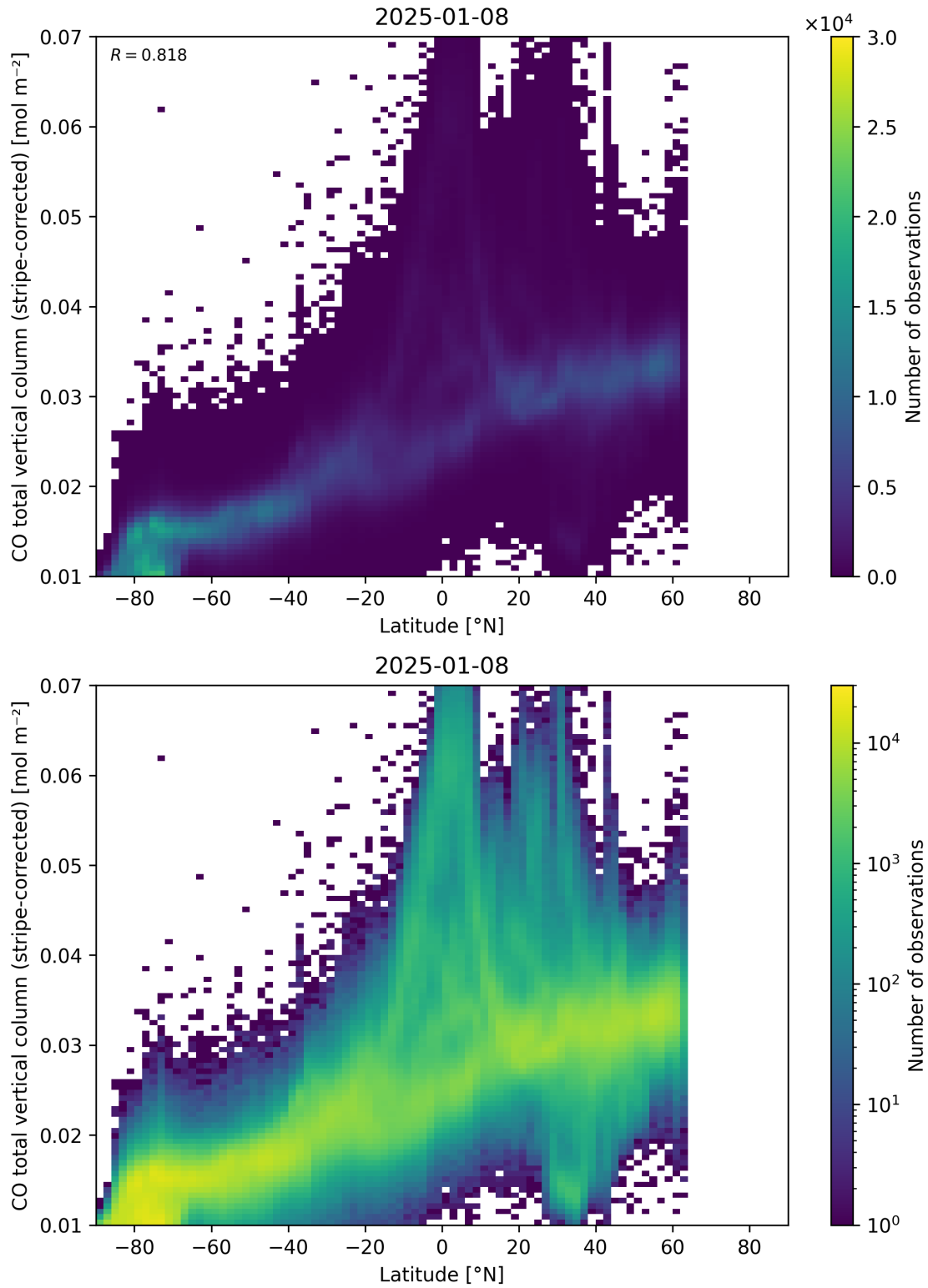
Figure 52: Scatter density plot of “Latitude” against “CO total vertical column (stripe-corrected)” for 2025-01-07 to 2025-01-09.
