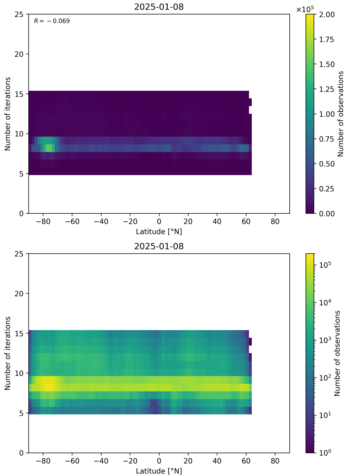
Figure 56: Scatter density plot of “Latitude” against “Number of iterations” for 2025-01-07 to 2025-01-09.
