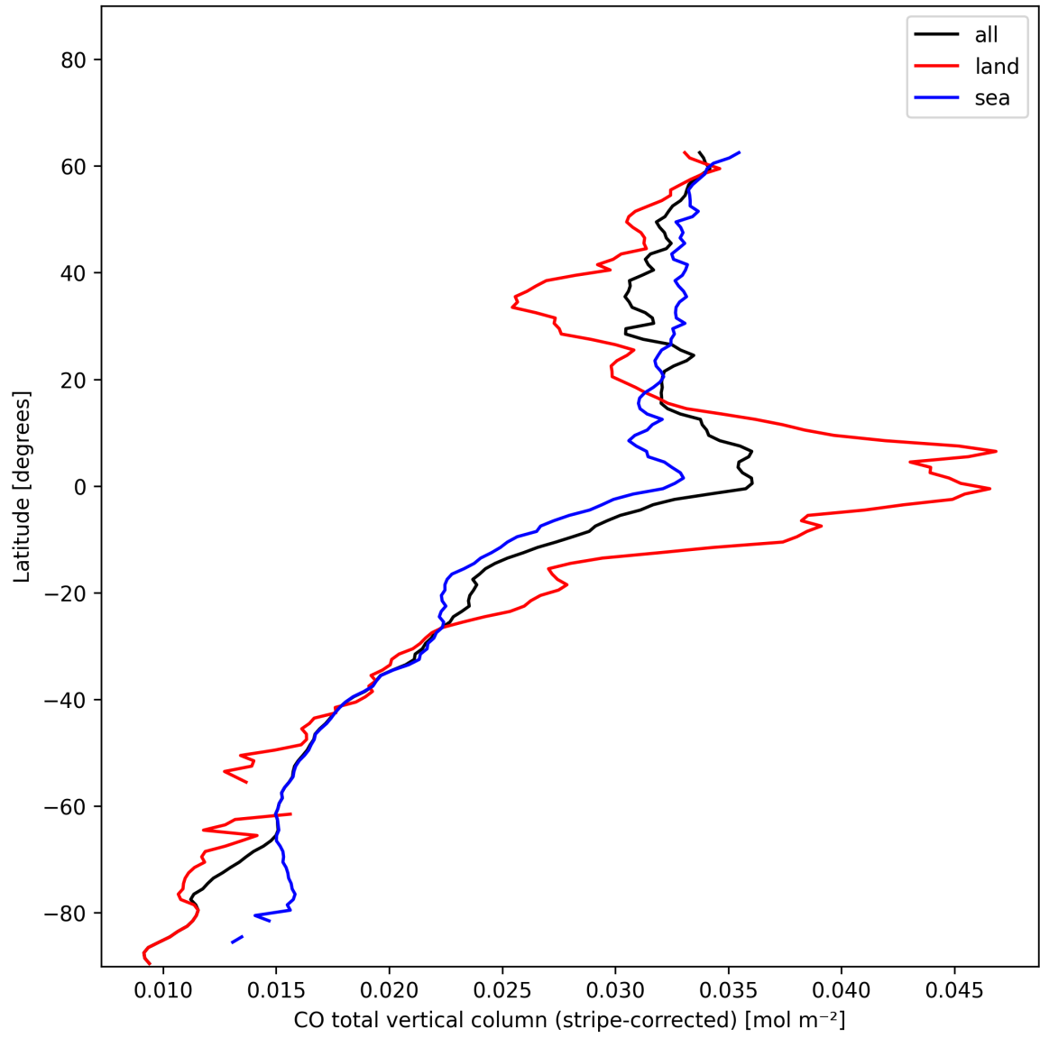
Figure 11: Zonal average of “CO total vertical column (stripe-corrected)” for 2025-01-07 to 2025-01-09.
