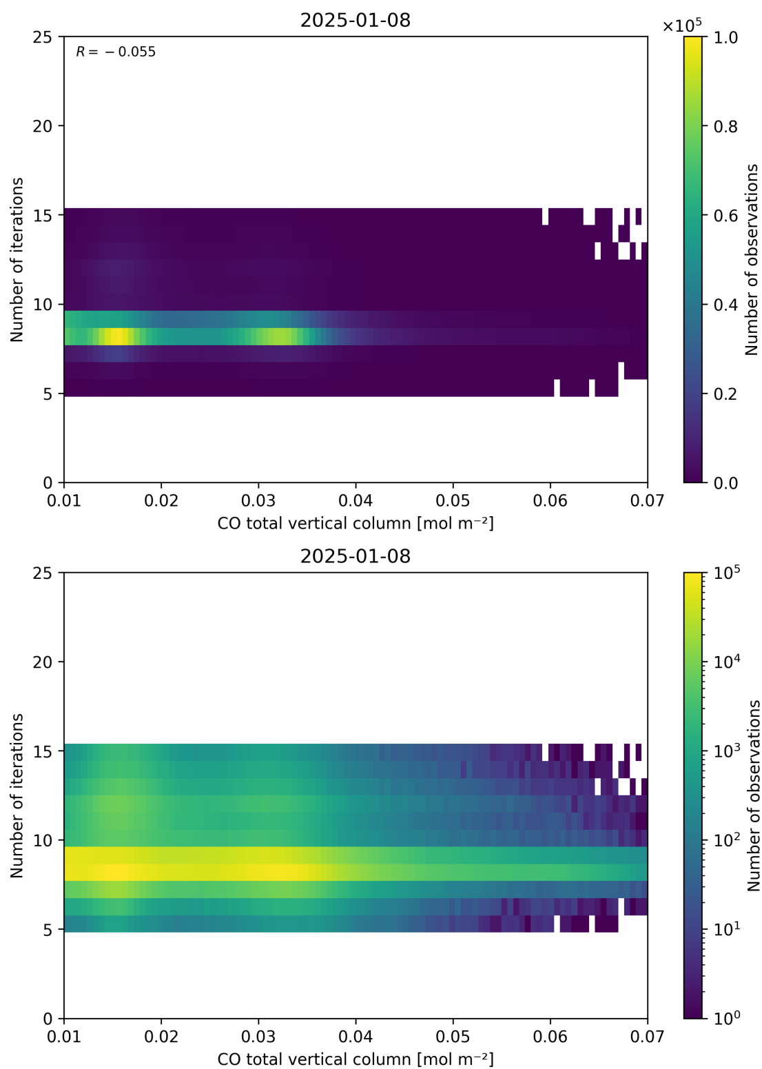
Figure 42: Scatter density plot of “CO total vertical column” against “Number of iterations” for 2025-01-07 to 2025-01-09.
