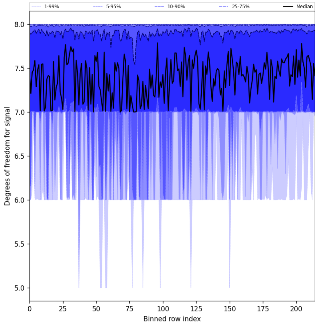
Figure 31: Along track statistics of “Degrees of freedom for signal” for 2025-01-07 to 2025-01-09
