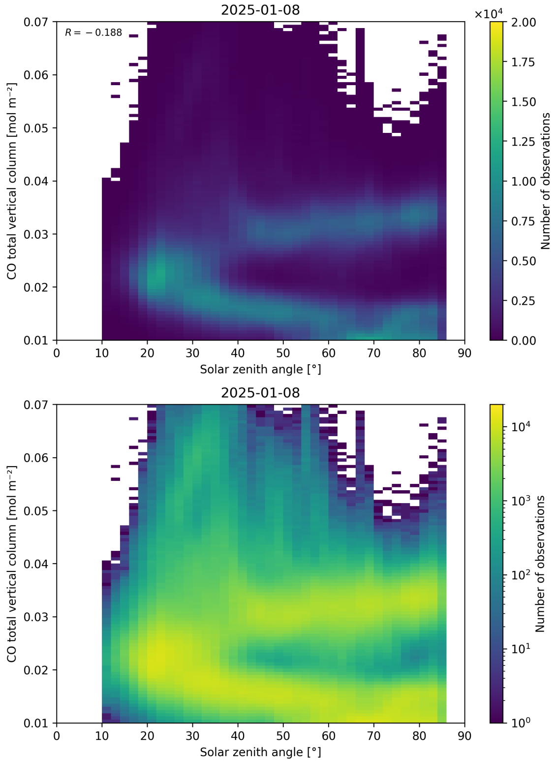
Figure 61: Scatter density plot of “Solar zenith angle” against “CO total vertical column” for 2025-01-07 to 2025-01-09.
