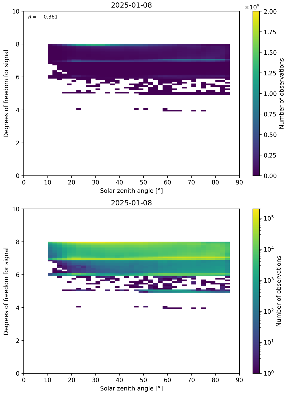
Figure 65: Scatter density plot of “Solar zenith angle” against “Degrees of freedom for signal” for 2025-01-07 to 2025-01-09.
