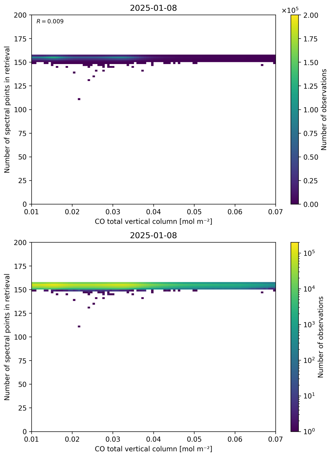
Figure 43: Scatter density plot of “CO total vertical column” against “Number of spectral points in retrieval” for 2025-01-07 to 2025-01-09.
