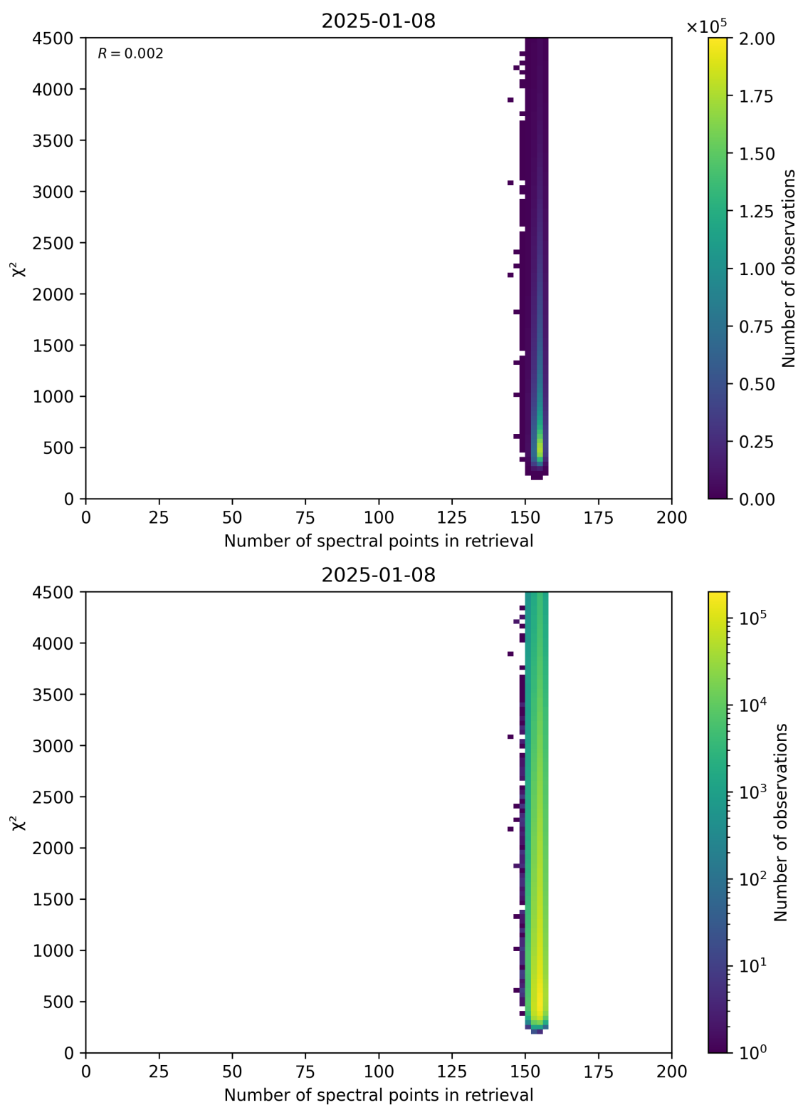
Figure 58: Scatter density plot of “Number of spectral points in retrieval” against “ \chi^2 ” for 2025-01-07 to 2025-01-09.
