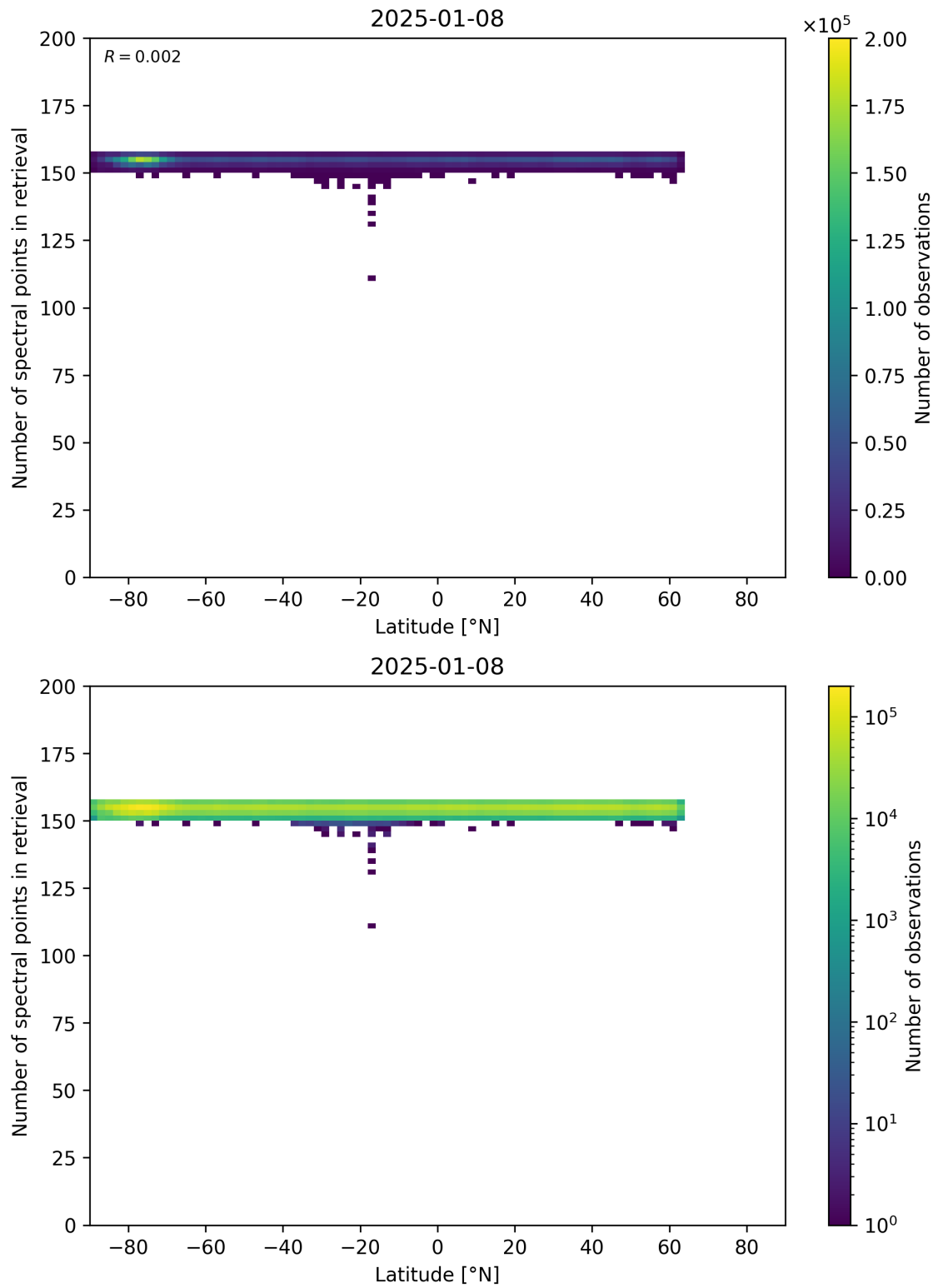
Figure 57: Scatter density plot of “Latitude” against “Number of spectral points in retrieval” for 2025-01-07 to 2025-01-09.
