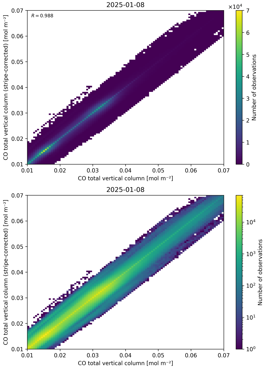
Figure 33: Scatter density plot of “CO total vertical column” against “CO total vertical column (stripe-corrected)” for 2025-01-07 to 2025-01-09.
