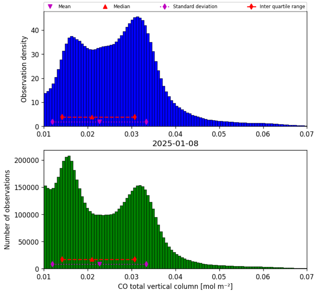
Figure 18: Histogram of “CO total vertical column” for 2025-01-07 to 2025-01-09
