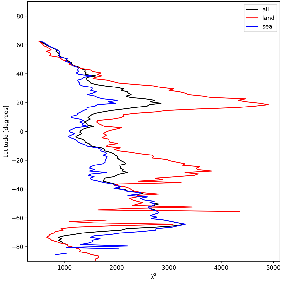
Figure 14: Zonal average of “ \chi^2 ” for 2025-01-07 to 2025-01-09.
