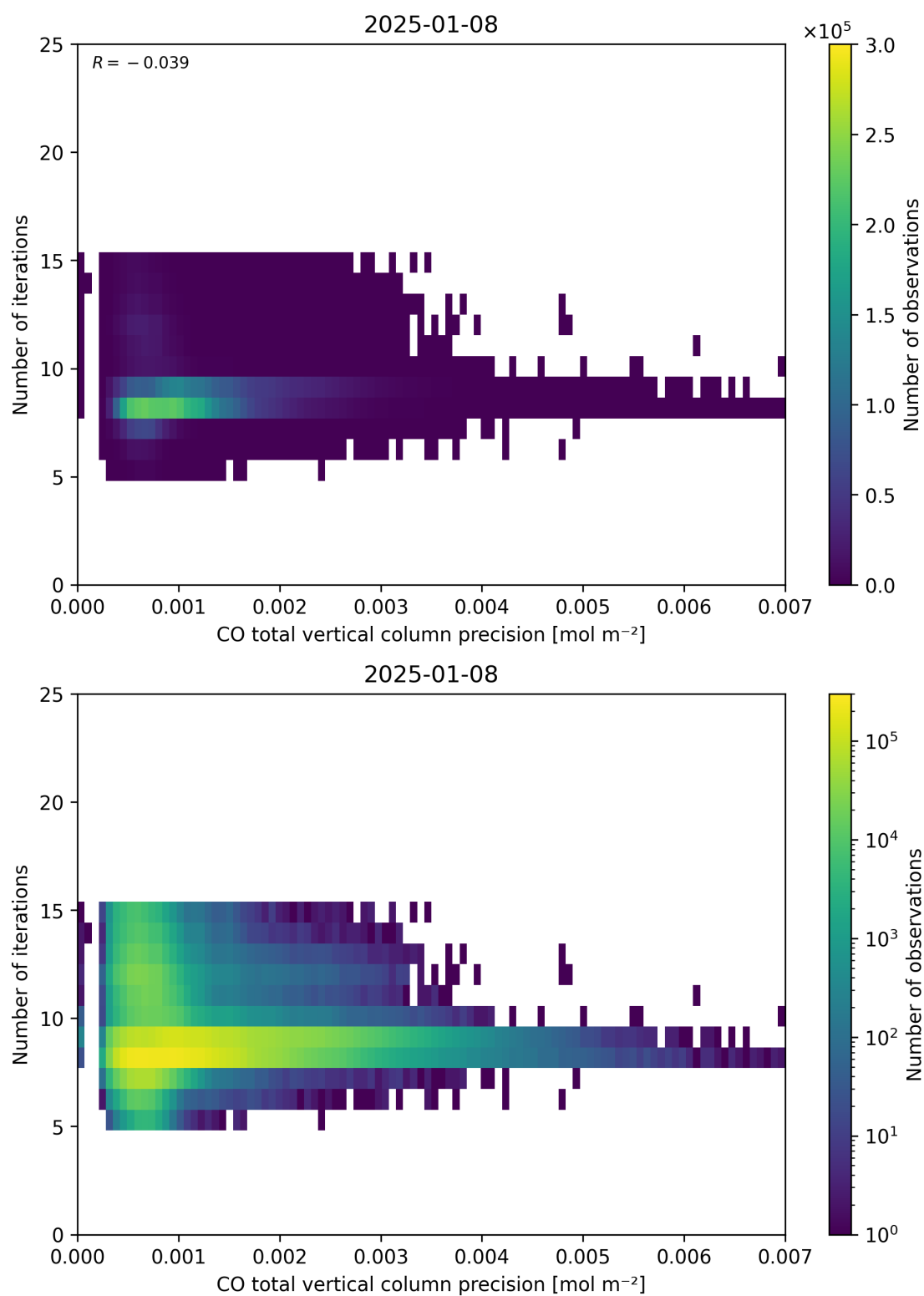
Figure 46: Scatter density plot of “CO total vertical column precision” against “Number of iterations” for 2025-01-07 to 2025-01-09.
