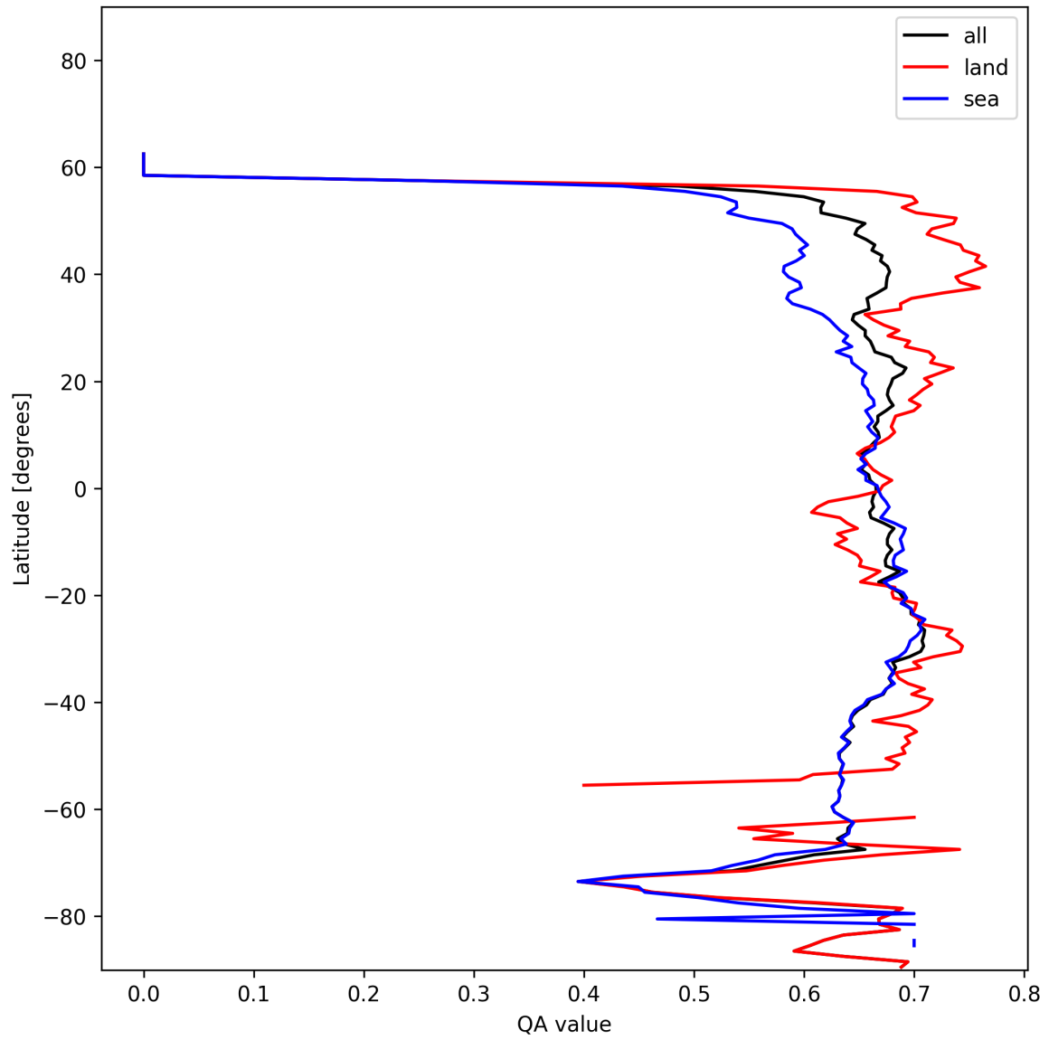
Figure 9: Zonal average of “QA value” for 2025-01-07 to 2025-01-09.
