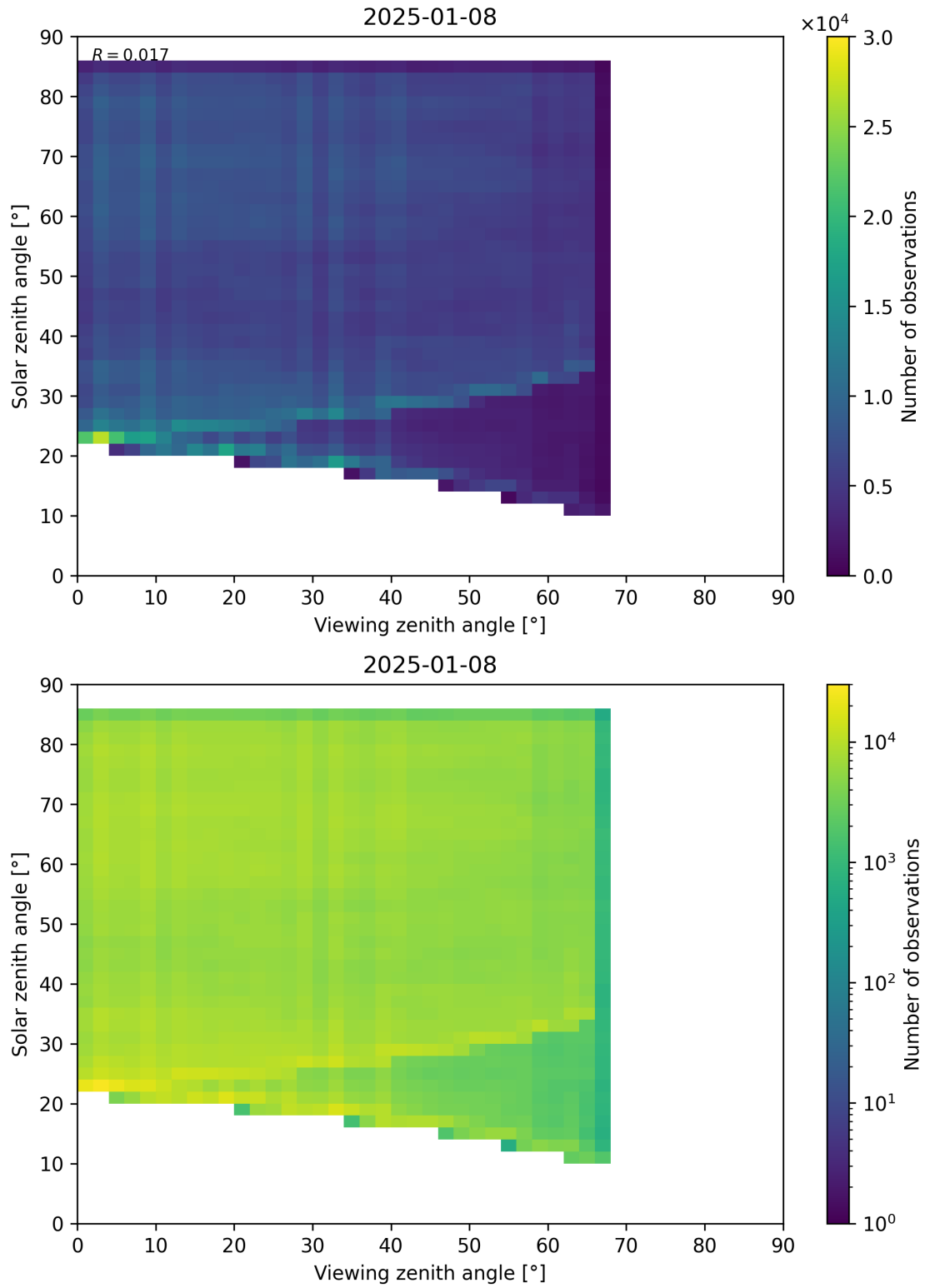
Figure 77: Scatter density plot of “Viewing zenith angle” against “Solar zenith angle” for 2025-01-07 to 2025-01-09.
