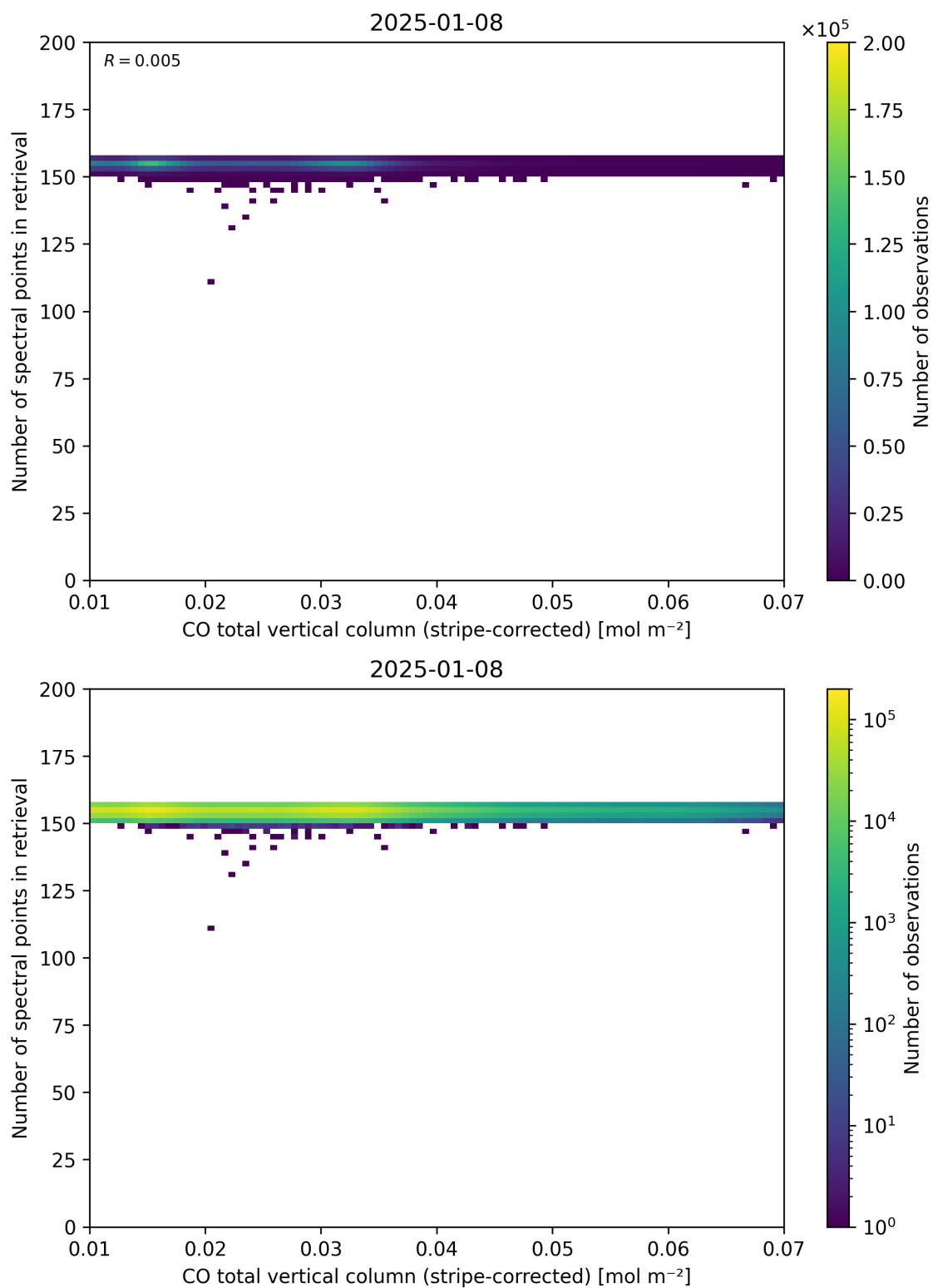
Figure 40: Scatter density plot of “CO total vertical column (stripe-corrected)” against “Number of spectral points in retrieval” for 2025-01-07 to 2025-01-09.
