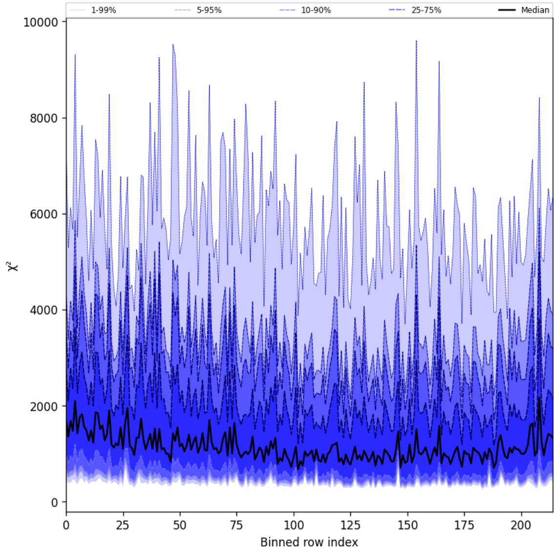
Figure 30: Along track statistics of “ \chi^2 ” for 2025-01-07 to 2025-01-09
