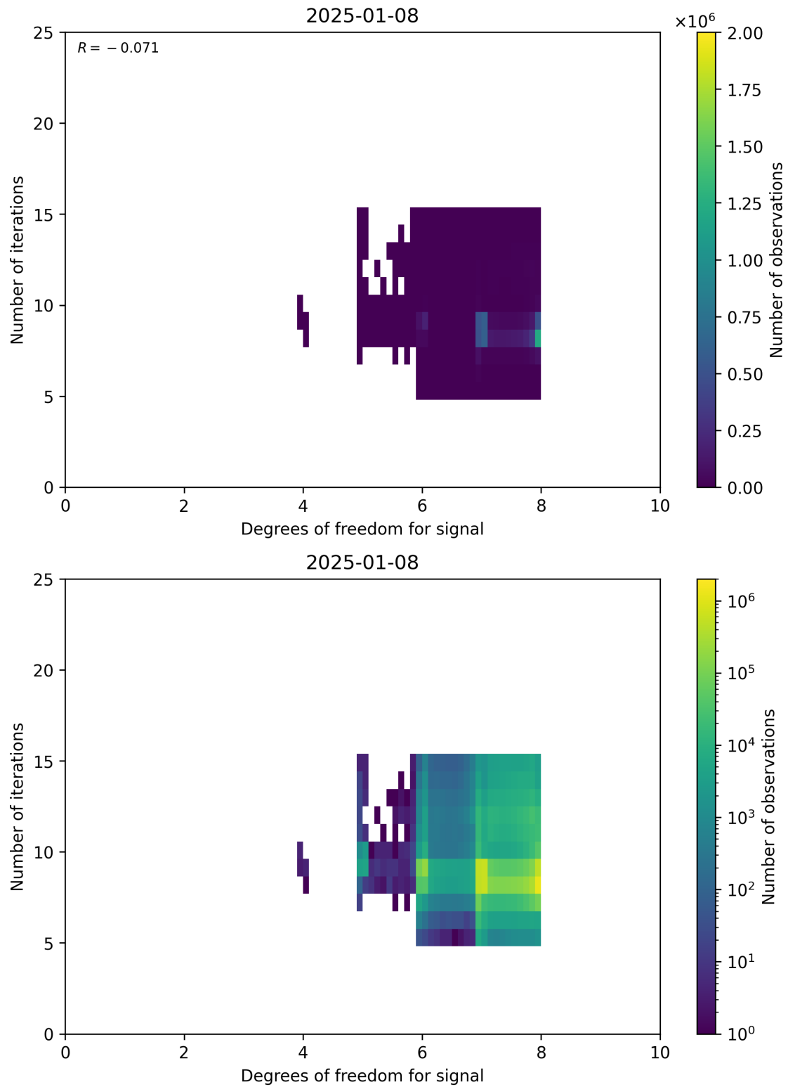
Figure 50: Scatter density plot of “Degrees of freedom for signal” against “Number of iterations” for 2025-01-07 to 2025-01-09.
