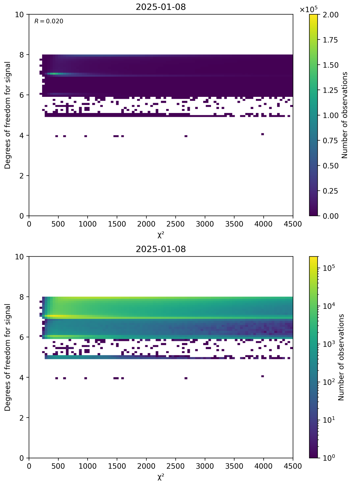
Figure 48: Scatter density plot of “ \chi^2 ” against “Degrees of freedom for signal” for 2025-01-07 to 2025-01-09.
