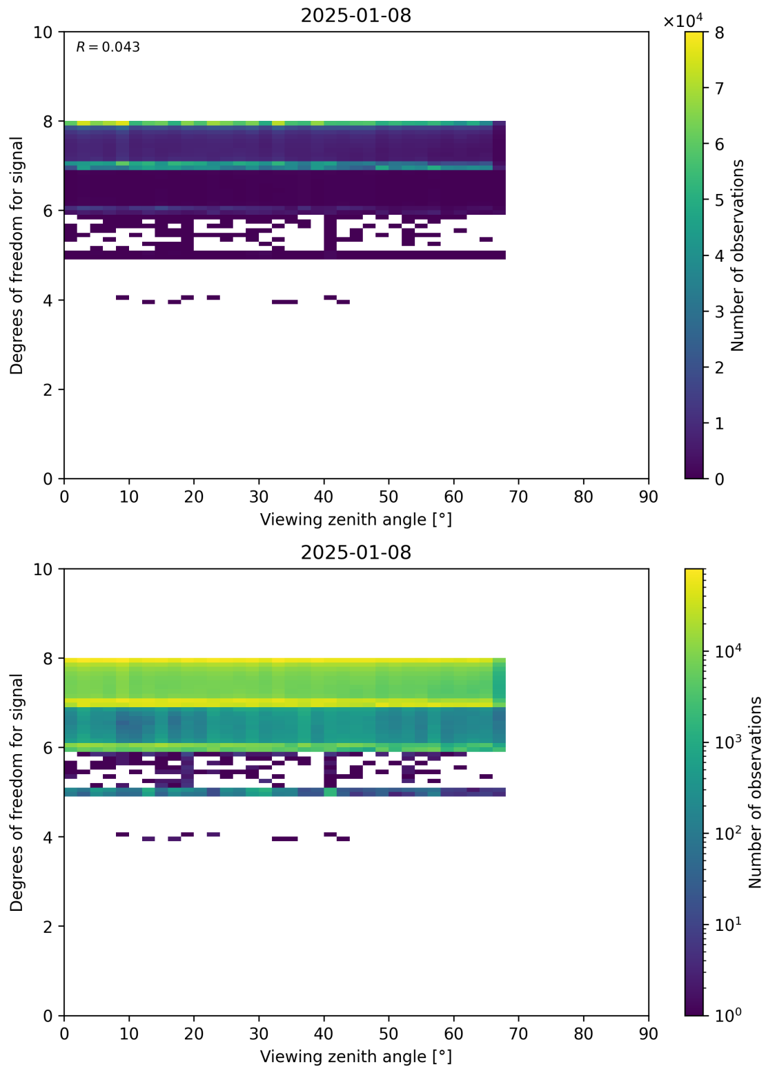
Figure 73: Scatter density plot of “Viewing zenith angle” against “Degrees of freedom for signal” for 2025-01-07 to 2025-01-09.
