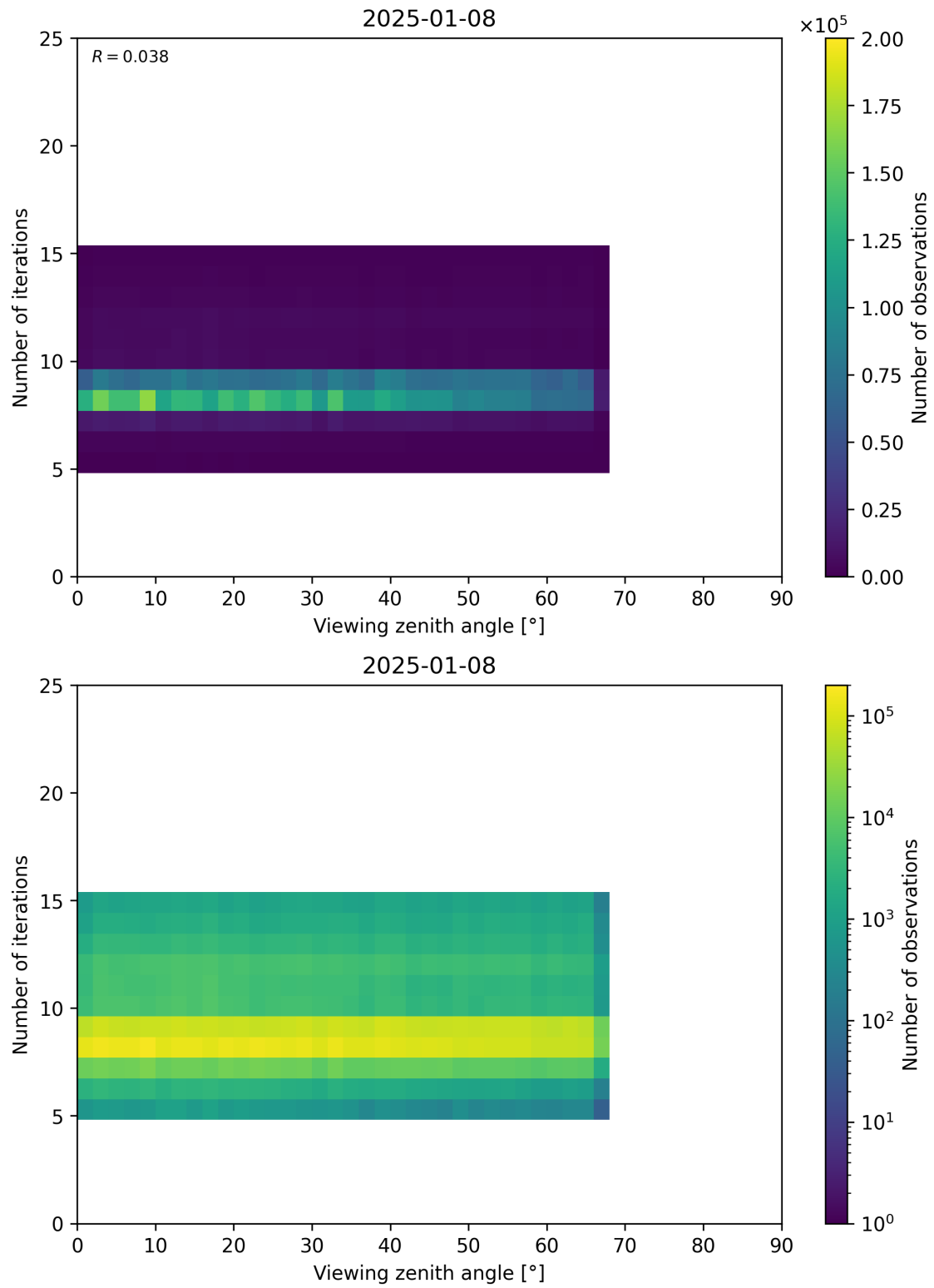
Figure 75: Scatter density plot of “Viewing zenith angle” against “Number of iterations” for 2025-01-07 to 2025-01-09.
