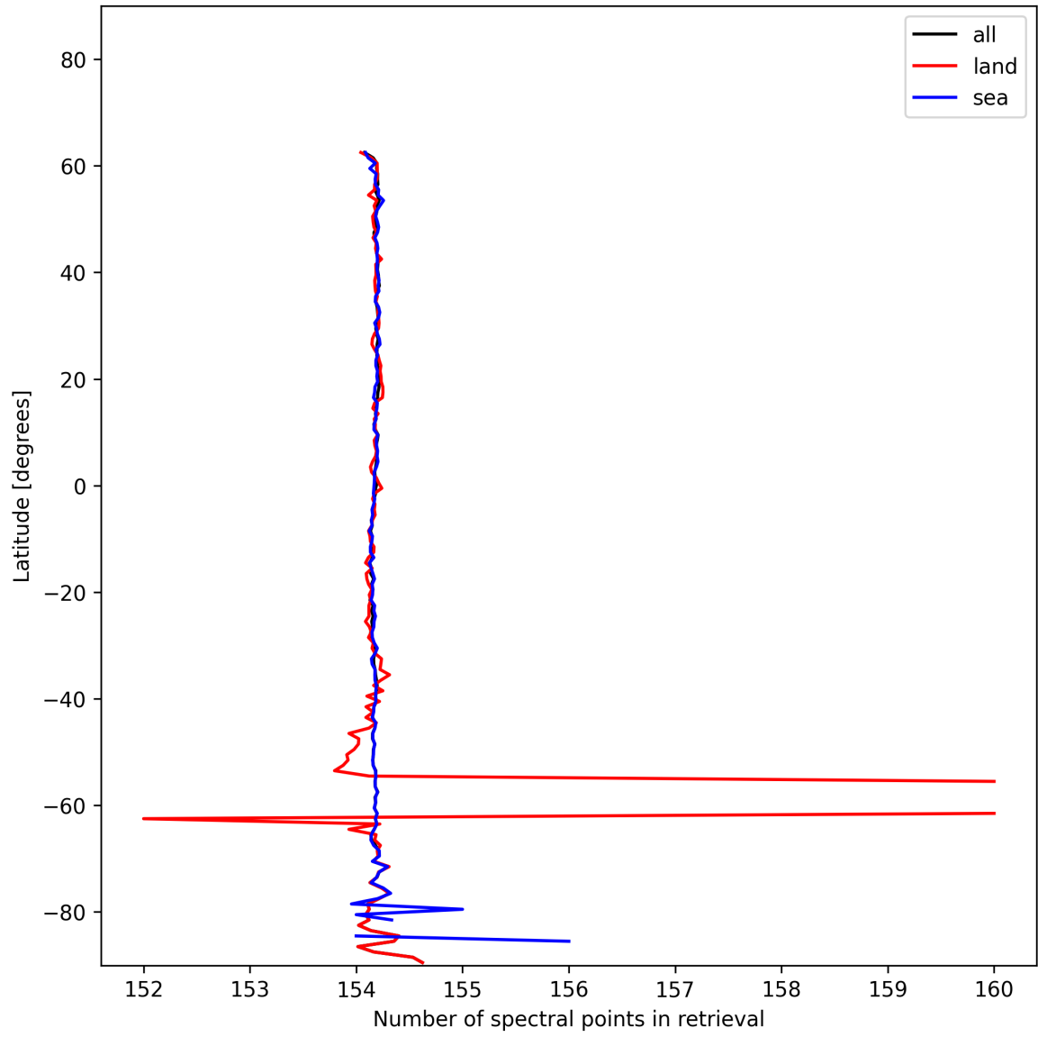
Figure 13: Zonal average of “Number of spectral points in retrieval” for 2025-01-07 to 2025-01-09.
