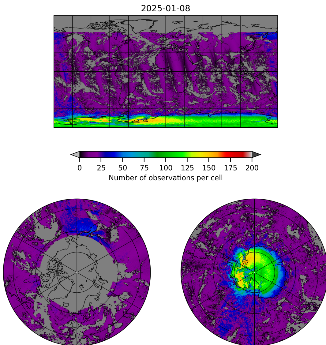
Figure 8: Map of the number of observations for 2025-01-07 to 2025-01-09
