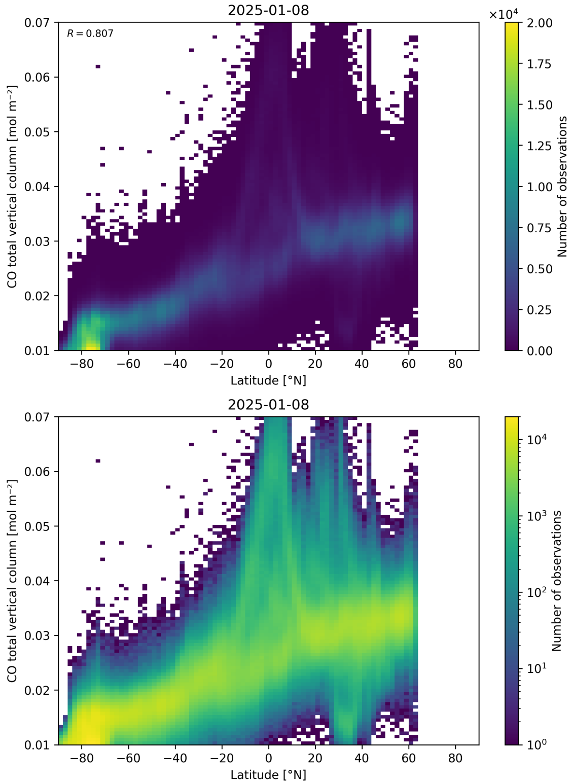
Figure 51: Scatter density plot of “Latitude” against “CO total vertical column” for 2025-01-07 to 2025-01-09.
