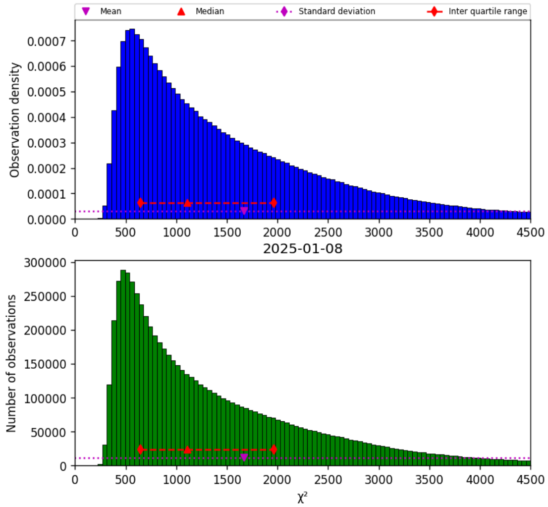
Figure 22: Histogram of “ \chi^2 ” for 2025-01-07 to 2025-01-09
