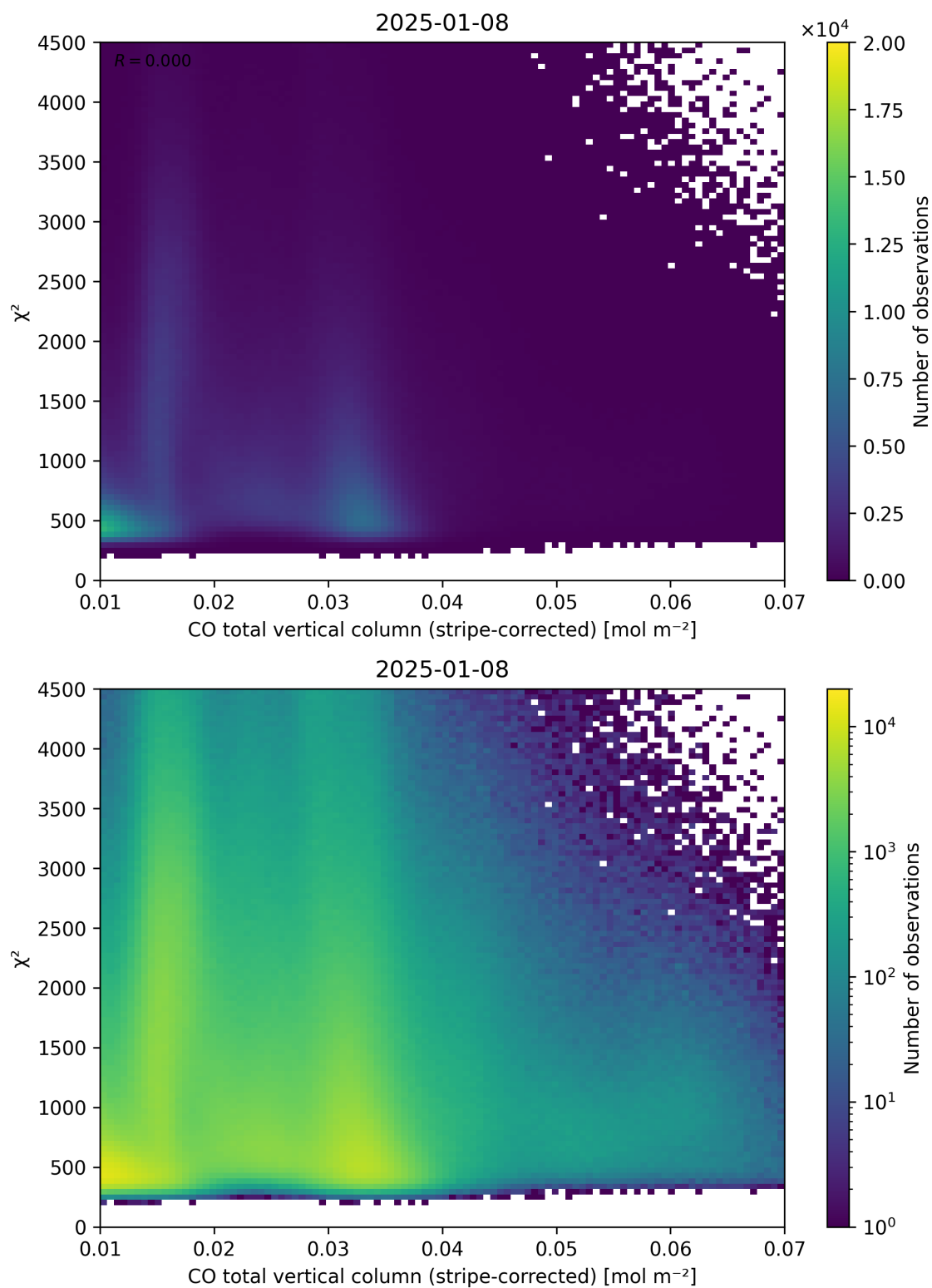
Figure 37: Scatter density plot of “CO total vertical column (stripe-corrected)” against “ \chi^2 ” for 2025-01-07 to 2025-01-09.
