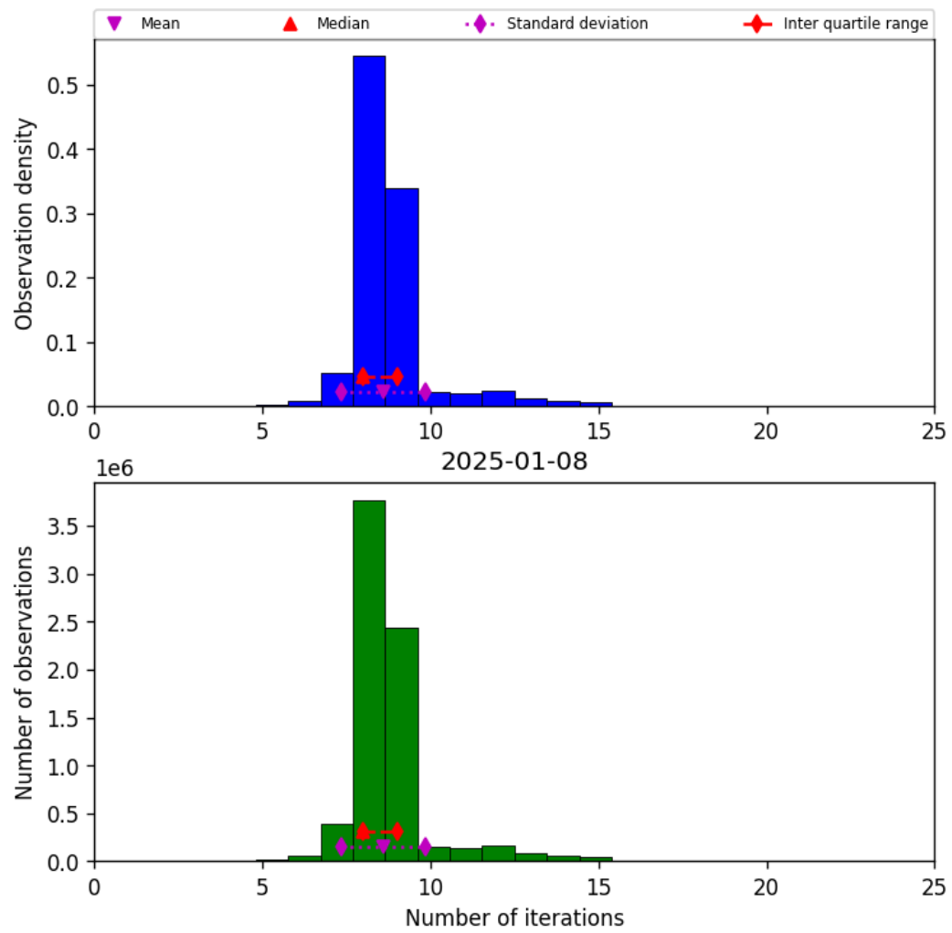
Figure 24: Histogram of “Number of iterations” for 2025-01-07 to 2025-01-09
