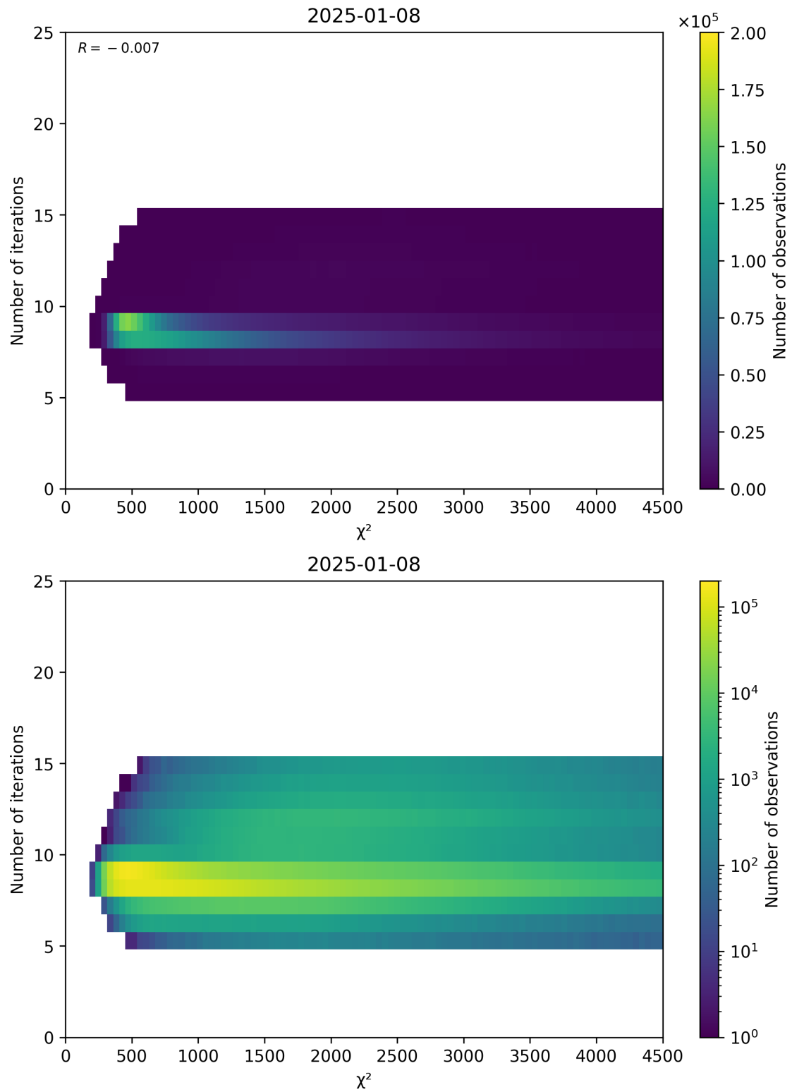
Figure 49: Scatter density plot of “ \chi^2 ” against “Number of iterations” for 2025-01-07 to 2025-01-09.
