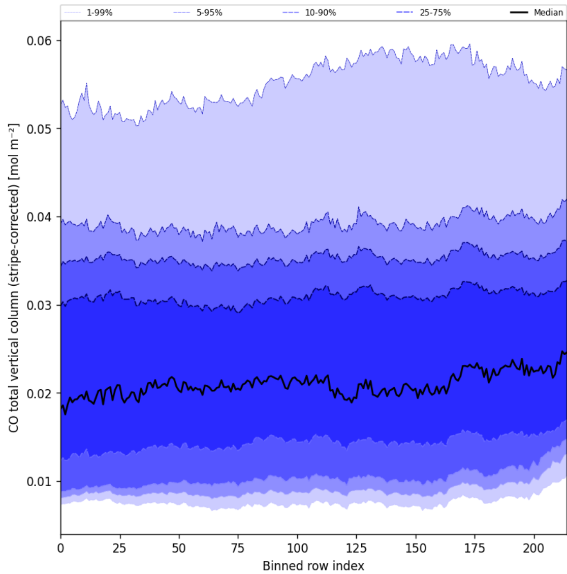
Figure 27: Along track statistics of “CO total vertical column (stripe-corrected)” for 2025-01-07 to 2025-01-09
