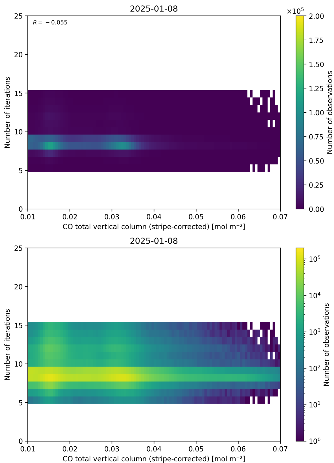
Figure 39: Scatter density plot of “CO total vertical column (stripe-corrected)” against “Number of iterations” for 2025-01-07 to 2025-01-09.
