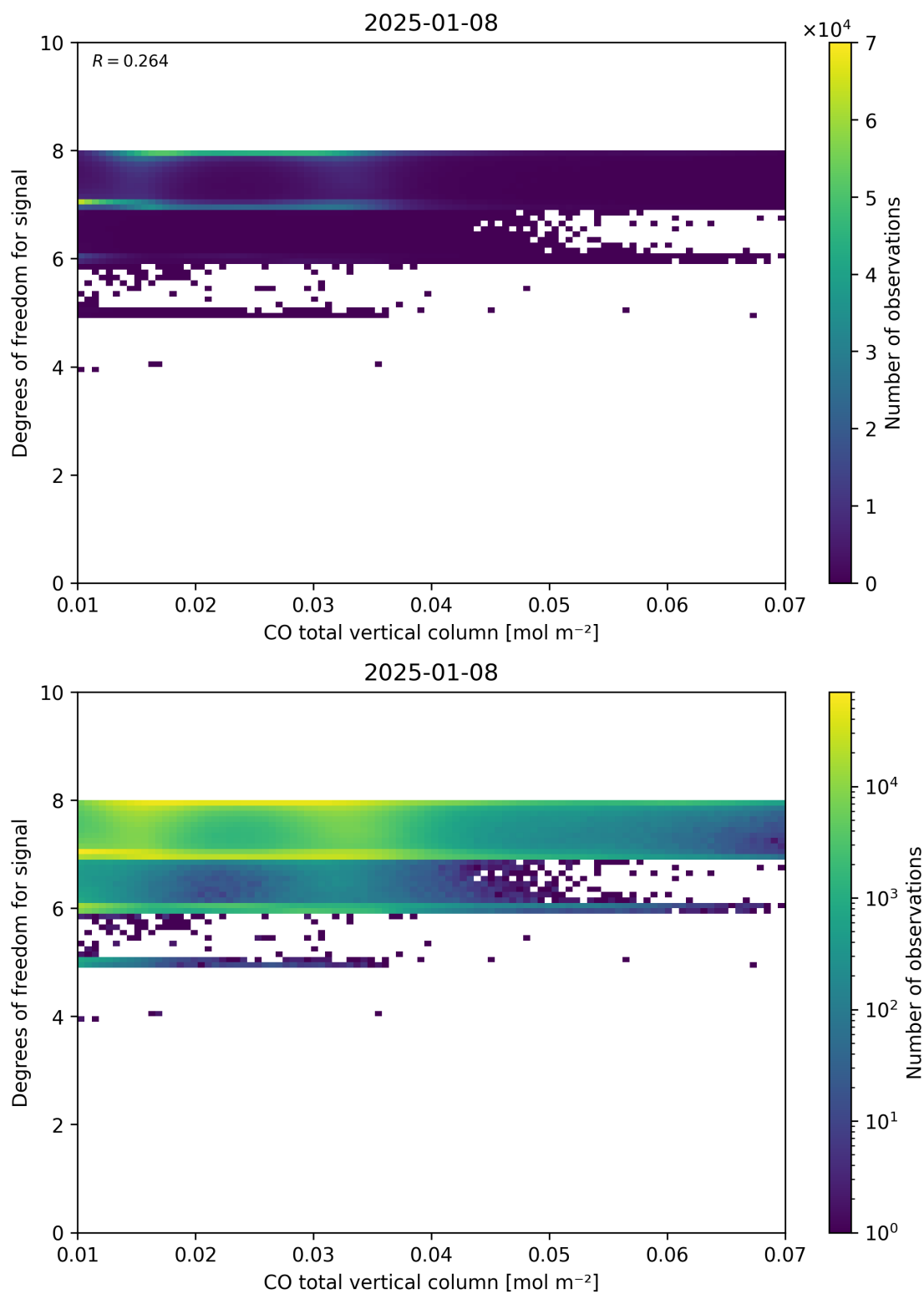
Figure 41: Scatter density plot of “CO total vertical column” against “Degrees of freedom for signal” for 2025-01-07 to 2025-01-09.
