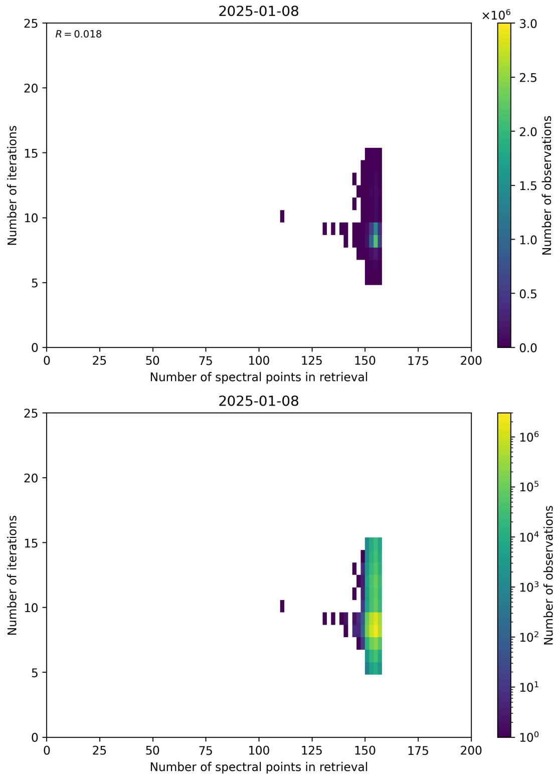
Figure 60: Scatter density plot of “Number of spectral points in retrieval” against “Number of iterations” for 2025-01-07 to 2025-01-09.
