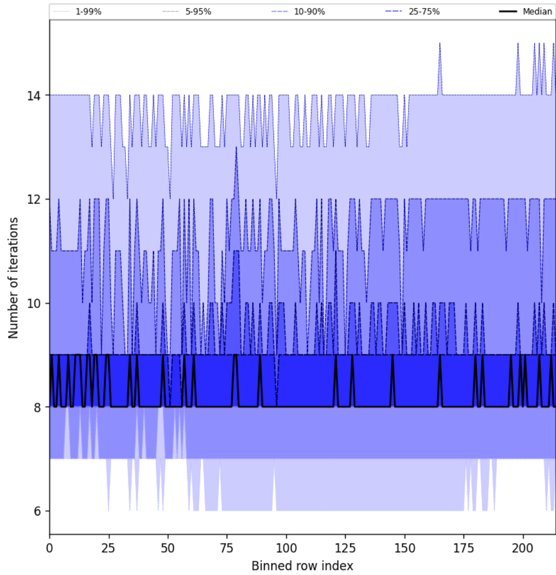
Figure 32: Along track statistics of “Number of iterations” for 2025-01-07 to 2025-01-09
