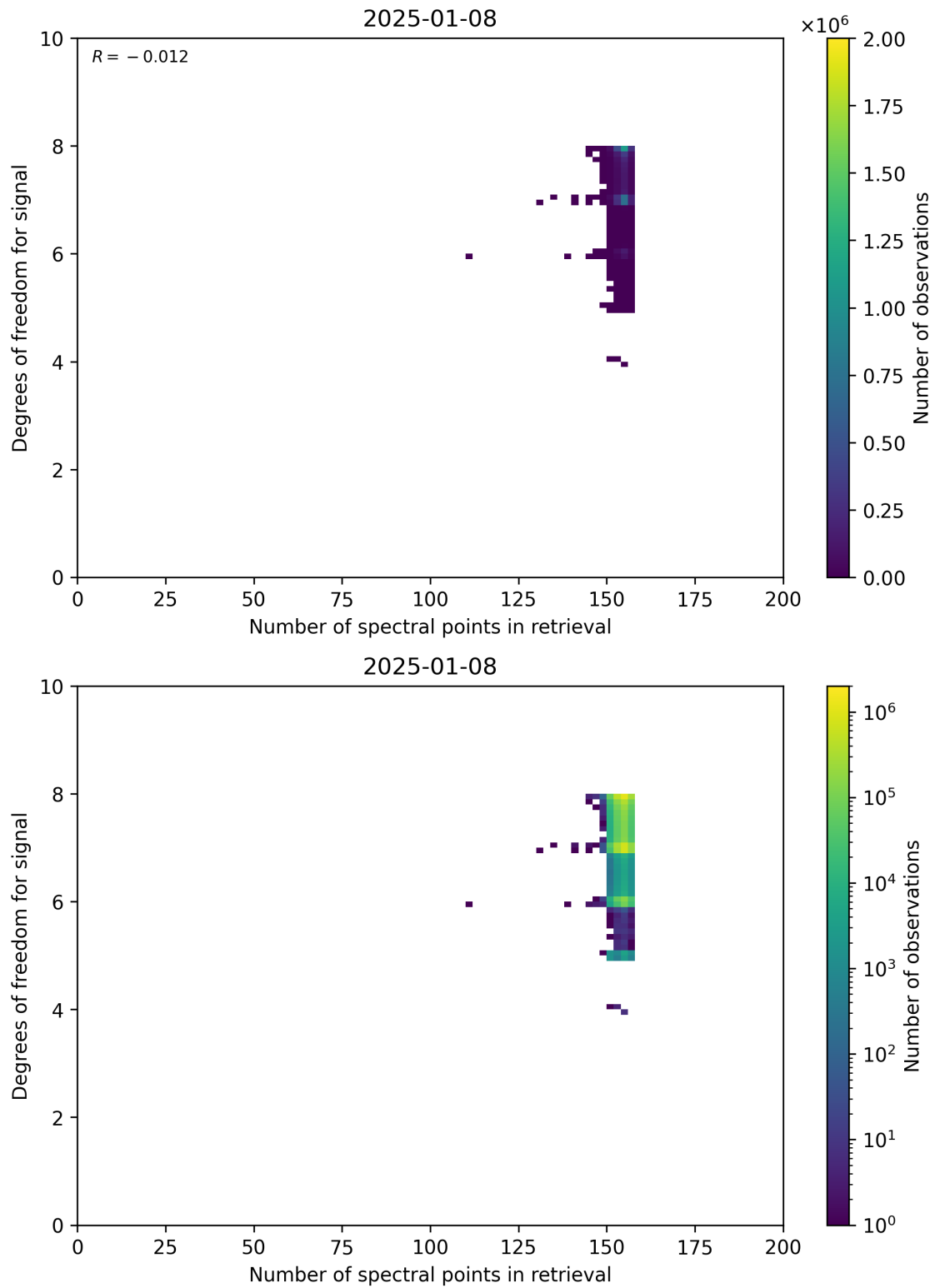
Figure 59: Scatter density plot of “Number of spectral points in retrieval” against “Degrees of freedom for signal” for 2025-01-07 to 2025-01-09.
