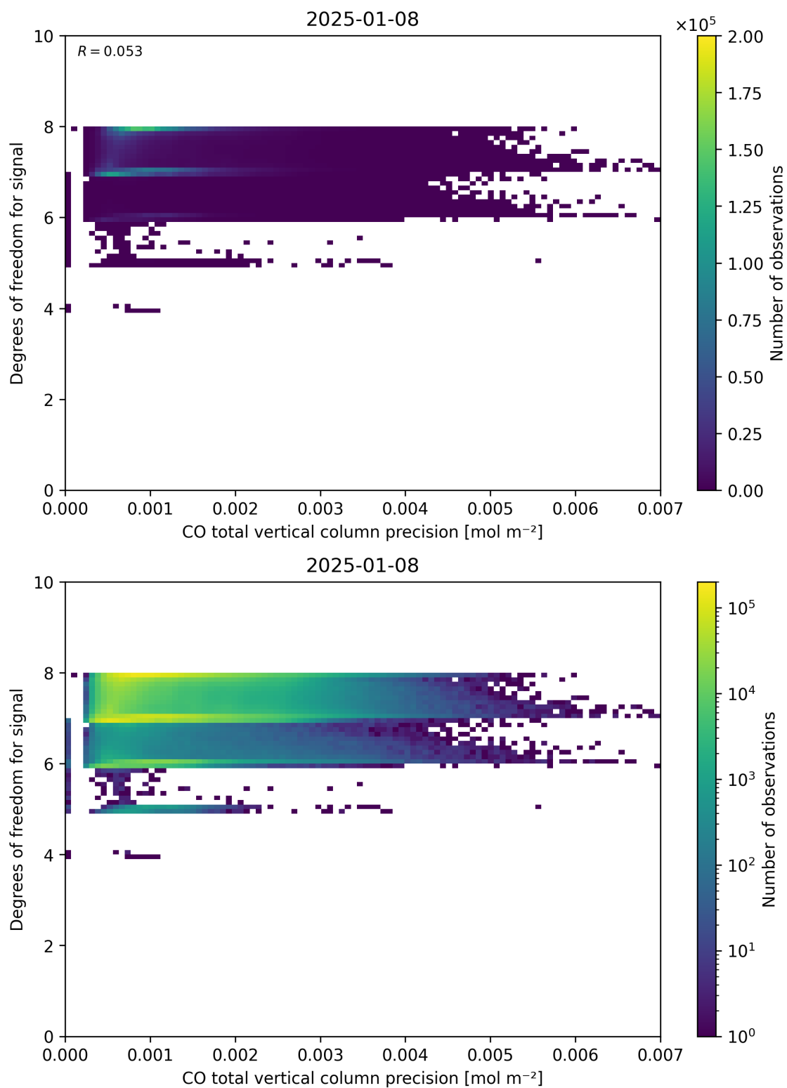
Figure 45: Scatter density plot of “CO total vertical column precision” against “Degrees of freedom for signal” for 2025-01-07 to 2025-01-09.
