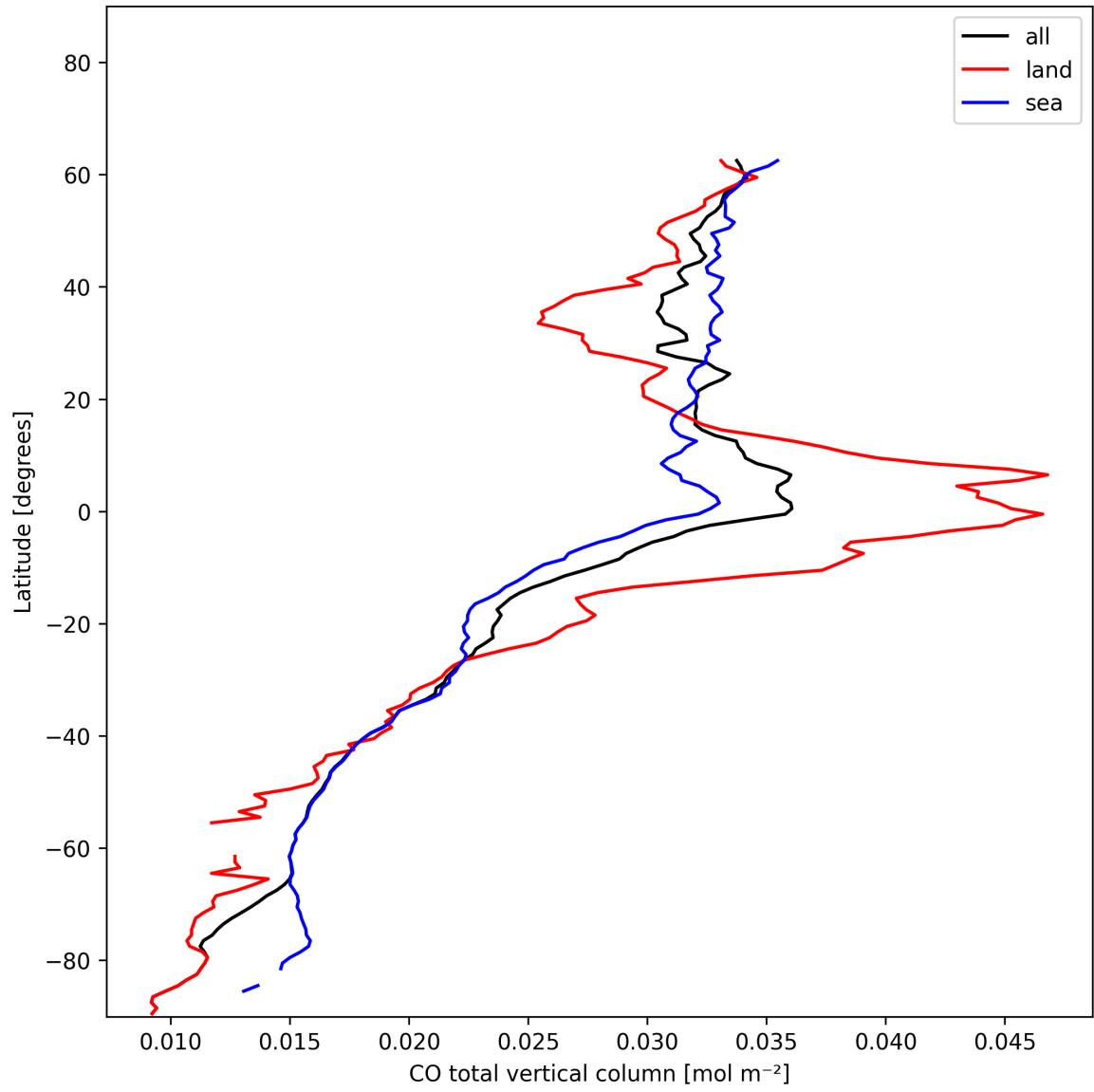
Figure 10: Zonal average of “CO total vertical column” for 2025-01-07 to 2025-01-09.
