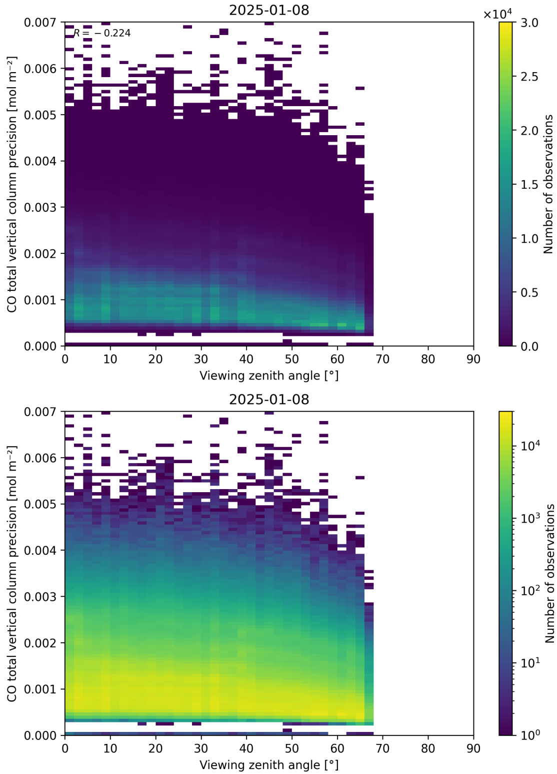
Figure 71: Scatter density plot of “Viewing zenith angle” against “CO total vertical column precision” for 2025-01-07 to 2025-01-09.
