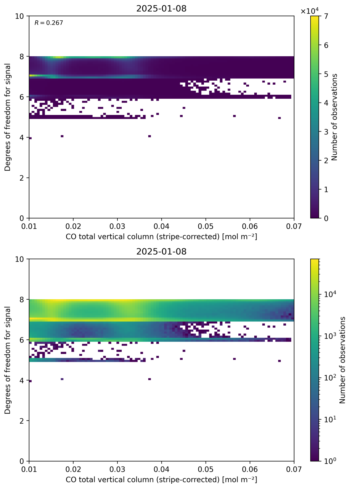
Figure 38: Scatter density plot of “CO total vertical column (stripe-corrected)” against “Degrees of freedom for signal” for 2025-01-07 to 2025-01-09.
