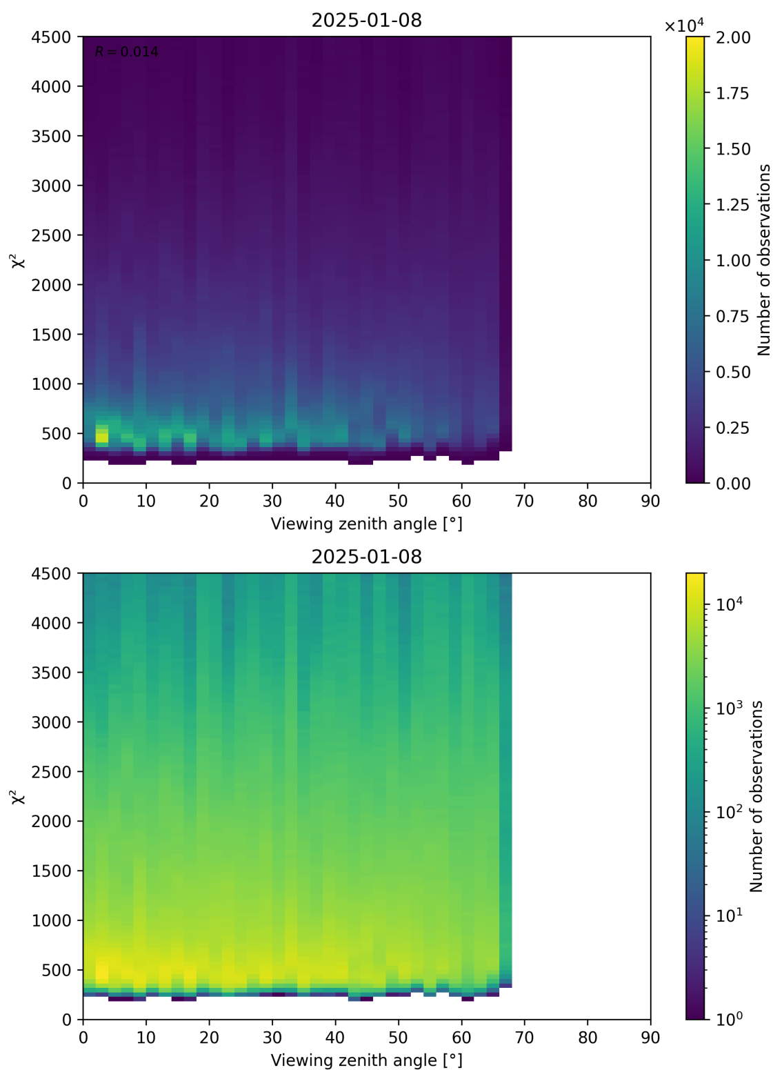
Figure 72: Scatter density plot of “Viewing zenith angle” against “ \chi^2 ” for 2025-01-07 to 2025-01-09.
