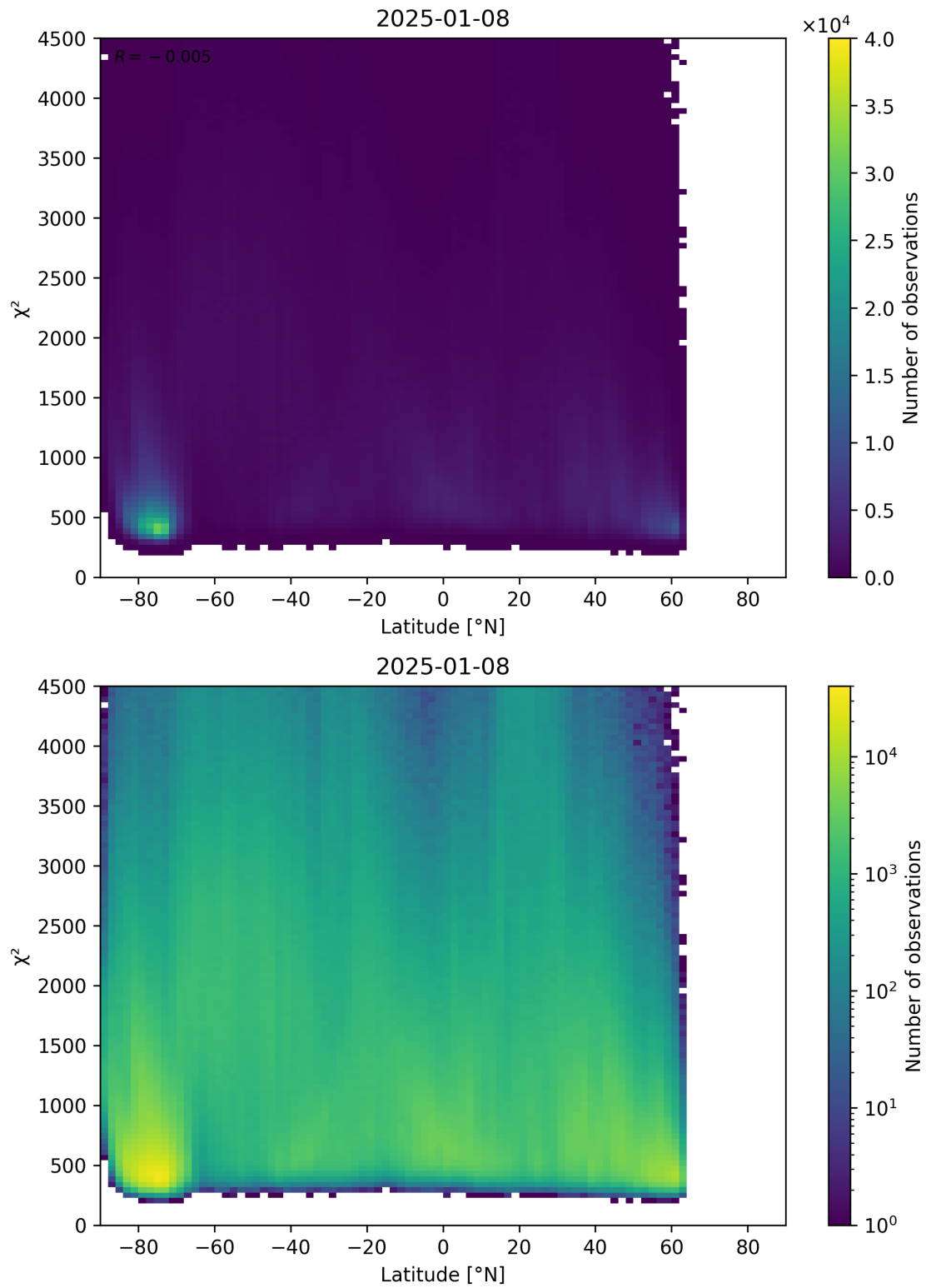
Figure 54: Scatter density plot of “Latitude” against “ \chi^2 ” for 2025-01-07 to 2025-01-09.
