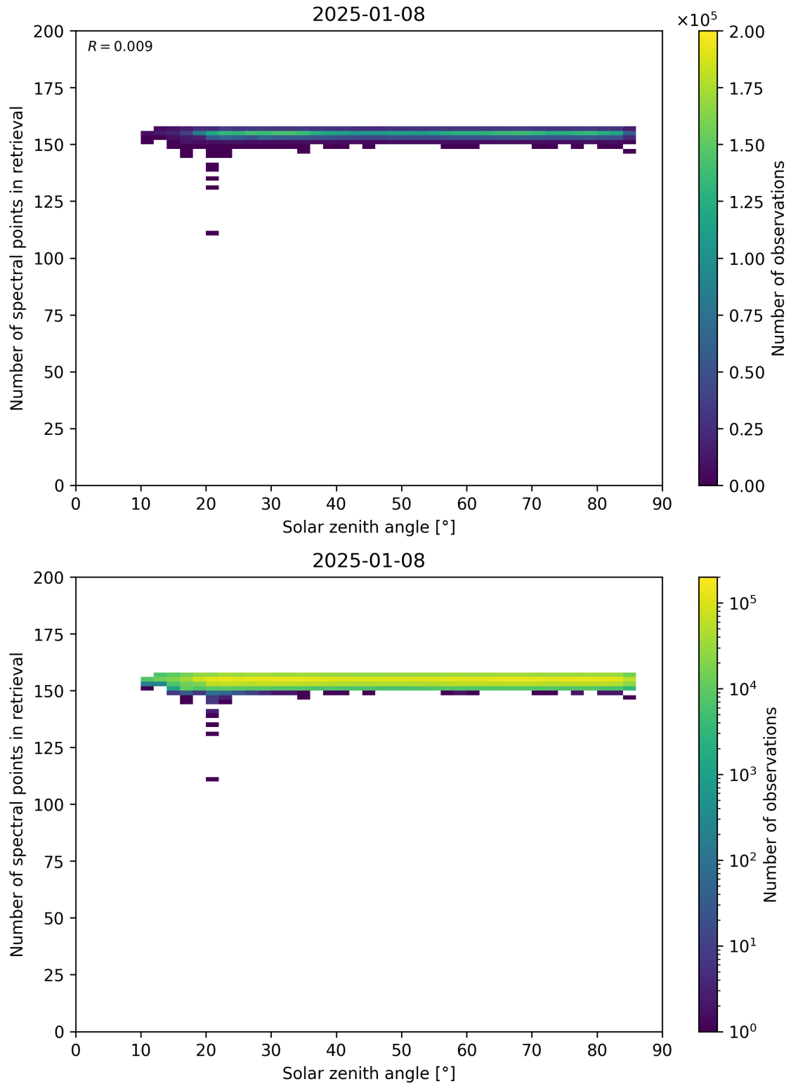
Figure 68: Scatter density plot of “Solar zenith angle” against “Number of spectral points in retrieval” for 2025-01-07 to 2025-01-09.
