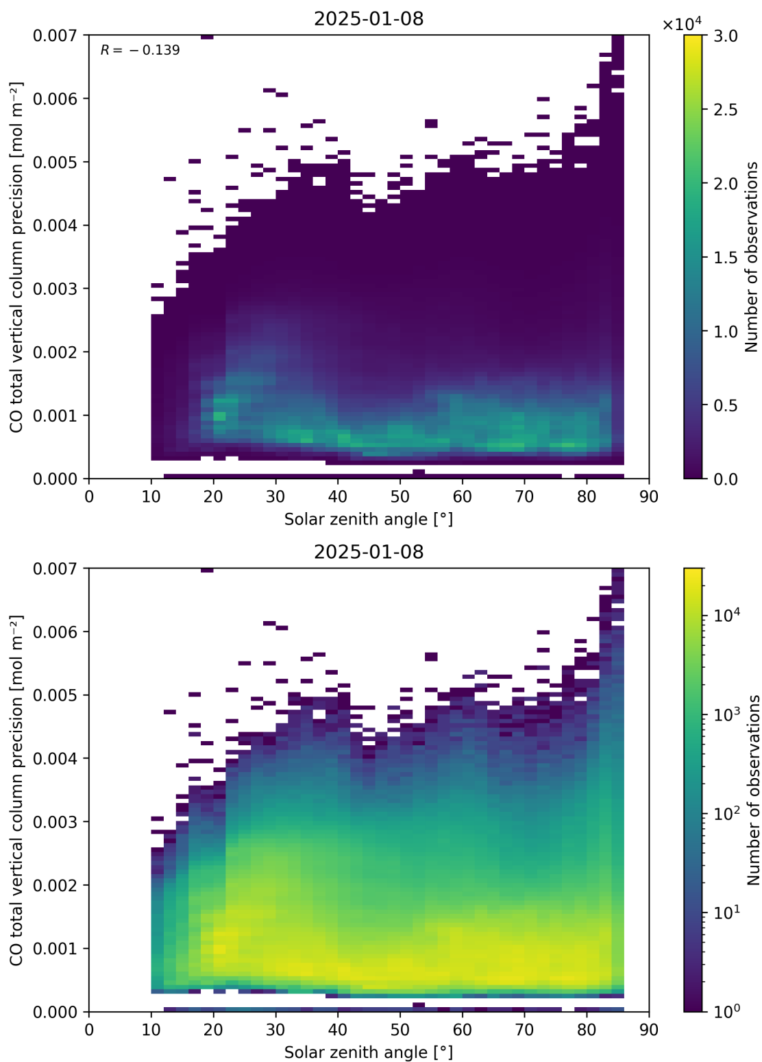
Figure 63: Scatter density plot of “Solar zenith angle” against “CO total vertical column precision” for 2025-01-07 to 2025-01-09.
