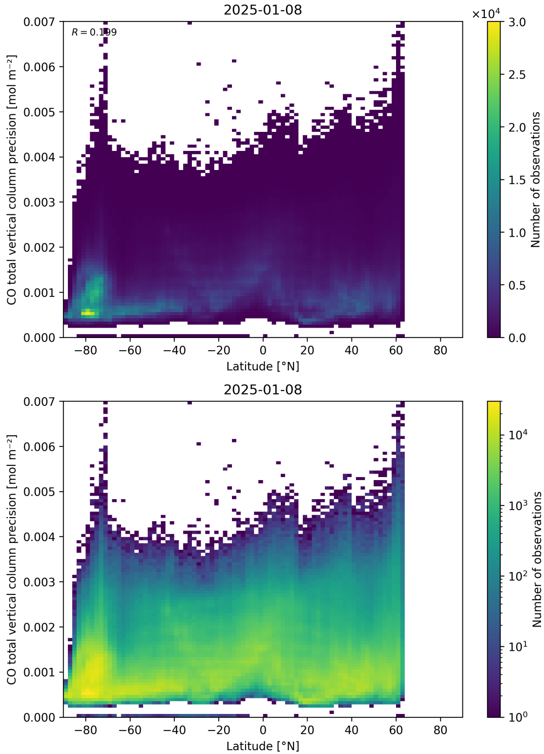
Figure 53: Scatter density plot of “Latitude” against “CO total vertical column precision” for 2025-01-07 to 2025-01-09.
