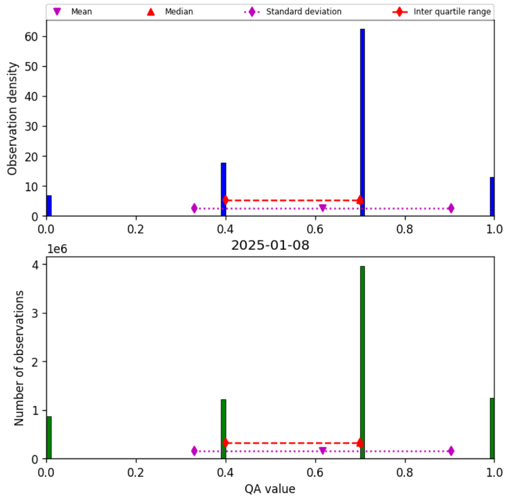
Figure 17: Histogram of “QA value” for 2025-01-07 to 2025-01-09
