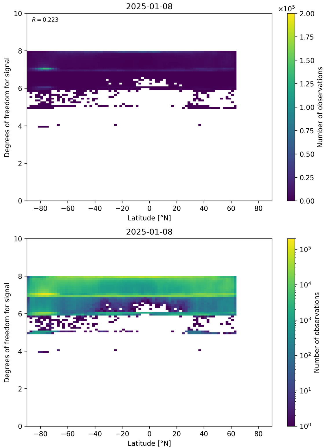
Figure 55: Scatter density plot of “Latitude” against “Degrees of freedom for signal” for 2025-01-07 to 2025-01-09.
