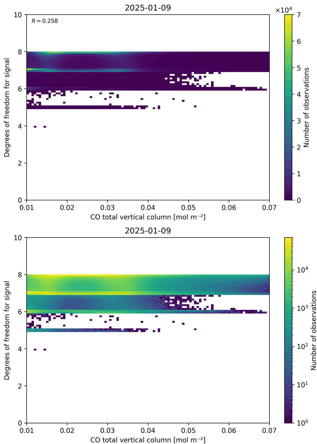
Figure 41: Scatter density plot of “CO total vertical column” against “Degrees of freedom for signal” for 2025-01-08 to 2025-01-10.
