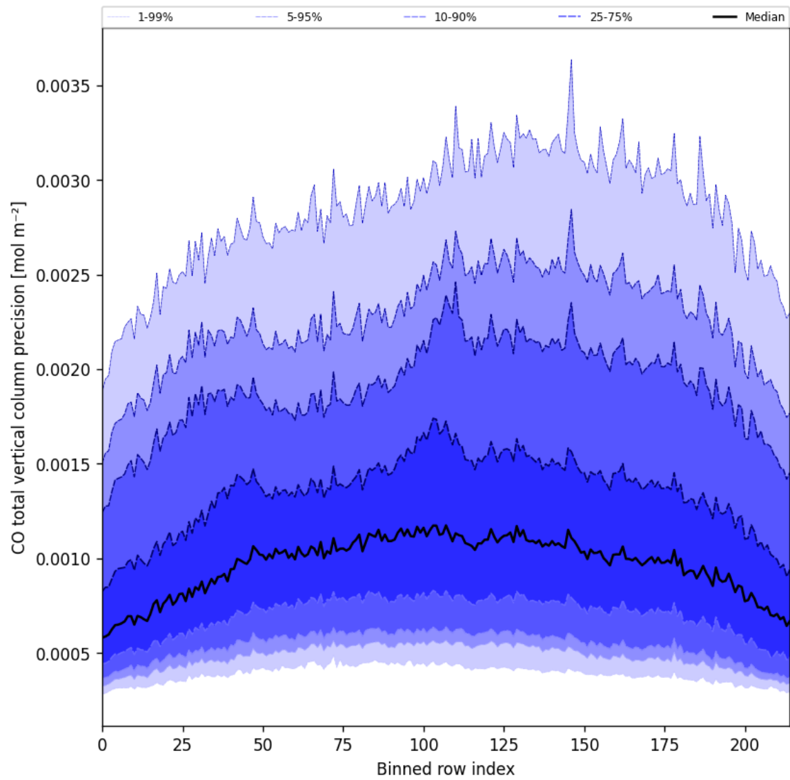
Figure 28: Along track statistics of “CO total vertical column precision” for 2025-01-08 to 2025-01-10
