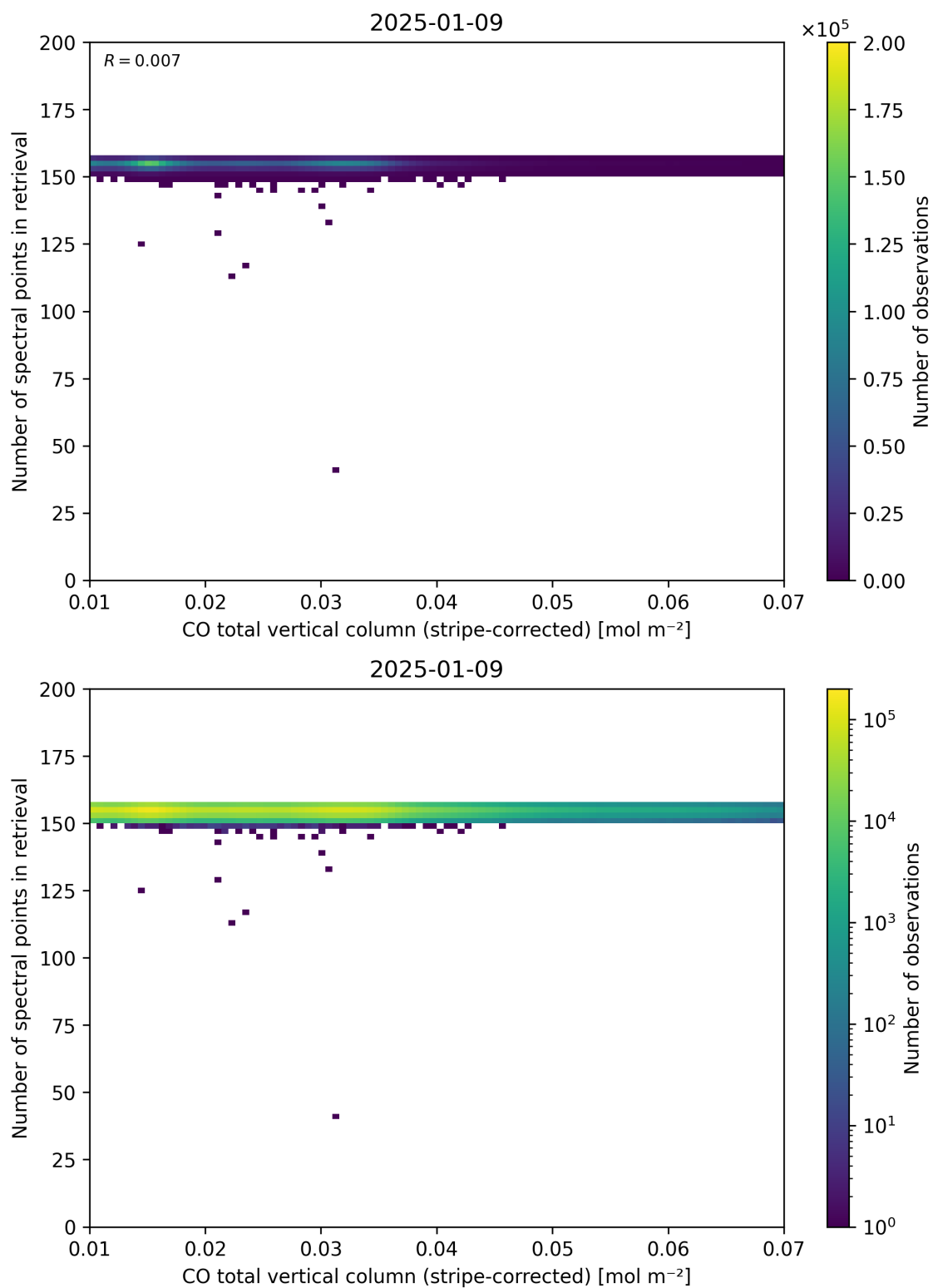
Figure 40: Scatter density plot of “CO total vertical column (stripe-corrected)” against “Number of spectral points in retrieval” for 2025-01-08 to 2025-01-10.
