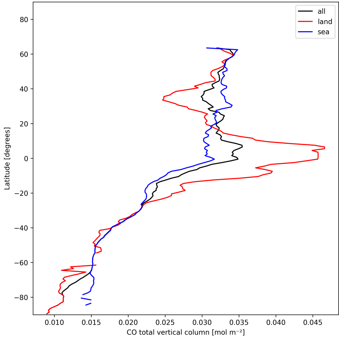
Figure 10: Zonal average of “CO total vertical column” for 2025-01-08 to 2025-01-10.
