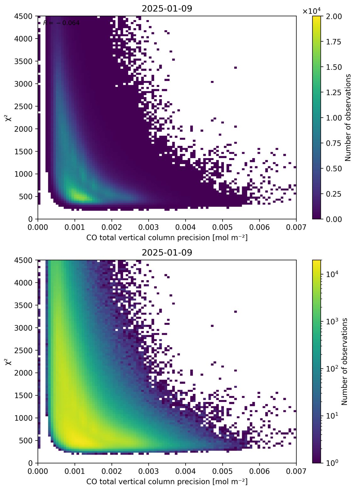
Figure 44: Scatter density plot of “CO total vertical column precision” against “ \chi^2 ” for 2025-01-08 to 2025-01-10.
