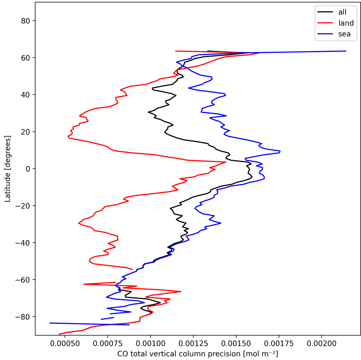
Figure 12: Zonal average of “CO total vertical column precision” for 2025-01-08 to 2025-01-10.
