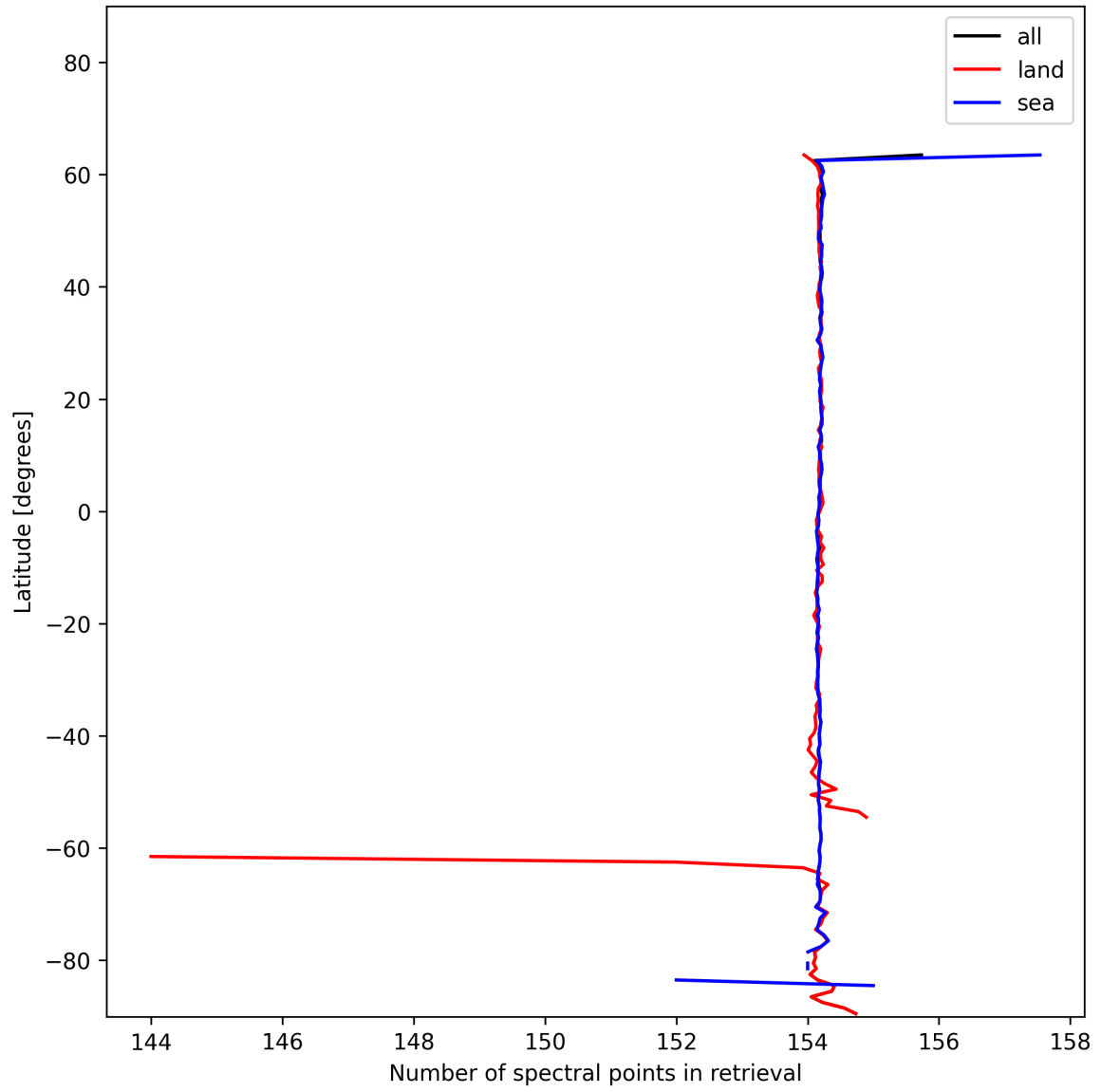
Figure 13: Zonal average of “Number of spectral points in retrieval” for 2025-01-08 to 2025-01-10.
