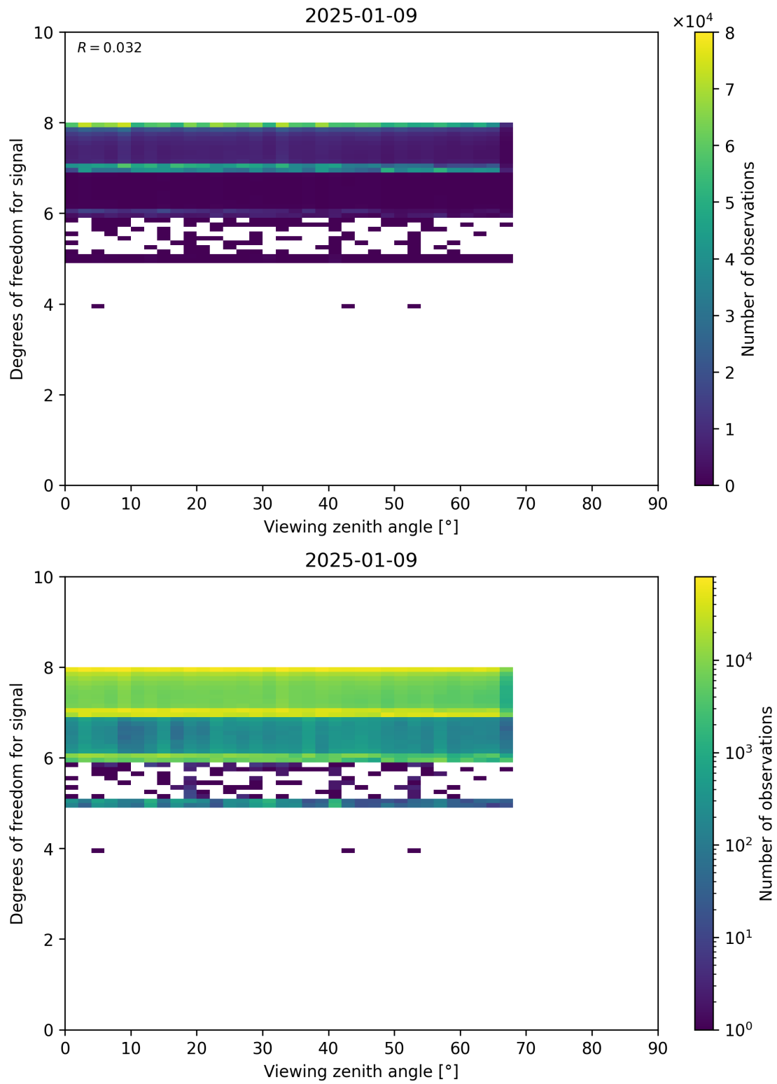
Figure 73: Scatter density plot of “Viewing zenith angle” against “Degrees of freedom for signal” for 2025-01-08 to 2025-01-10.
