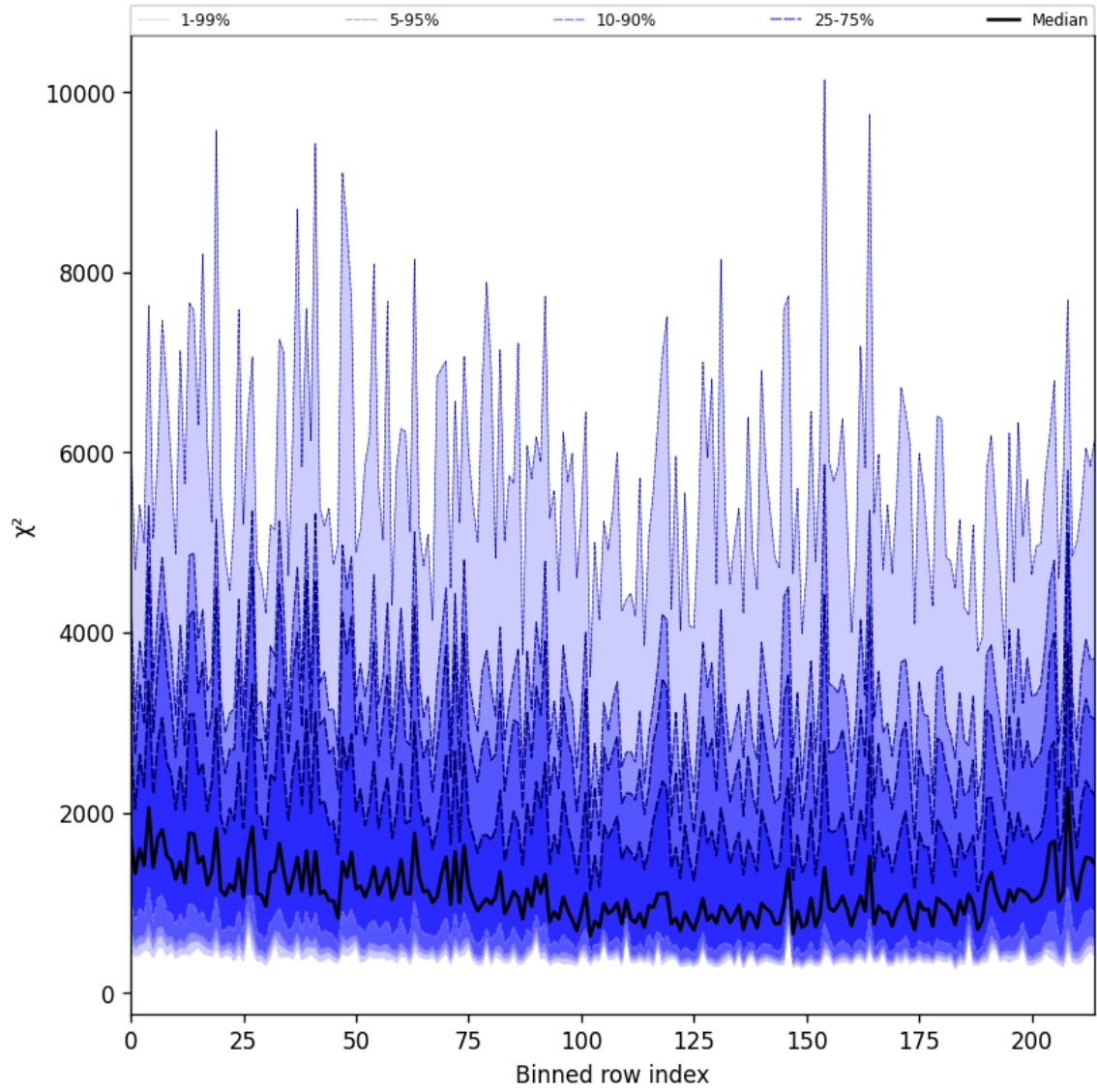
Figure 30: Along track statistics of “ \chi^2 ” for 2025-01-08 to 2025-01-10
