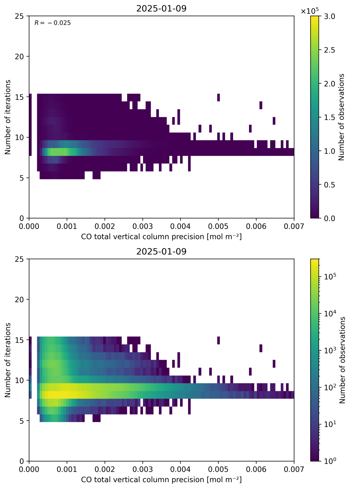
Figure 46: Scatter density plot of “CO total vertical column precision” against “Number of iterations” for 2025-01-08 to 2025-01-10.
