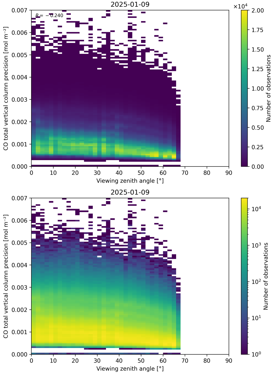
Figure 71: Scatter density plot of “Viewing zenith angle” against “CO total vertical column precision” for 2025-01-08 to 2025-01-10.
