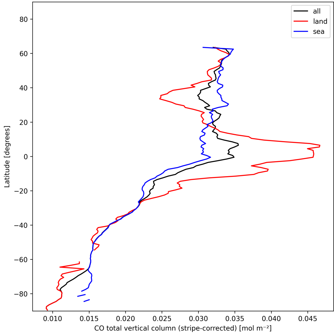
Figure 11: Zonal average of “CO total vertical column (stripe-corrected)” for 2025-01-08 to 2025-01-10.
