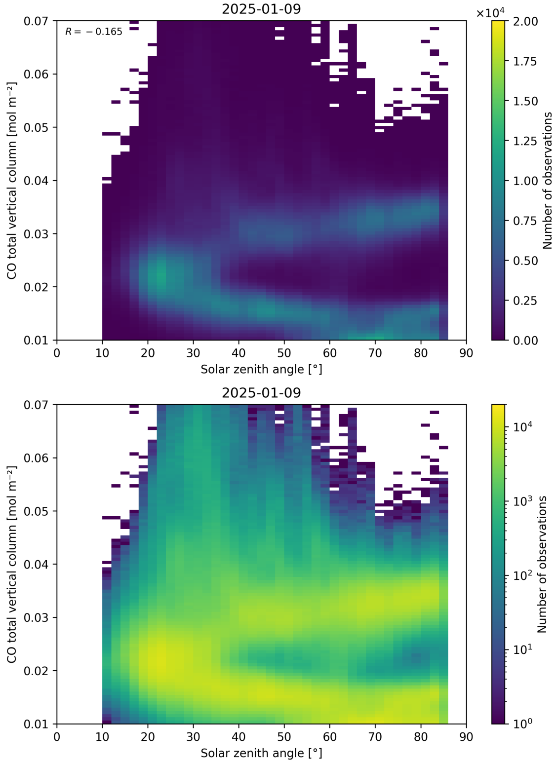
Figure 61: Scatter density plot of “Solar zenith angle” against “CO total vertical column” for 2025-01-08 to 2025-01-10.
