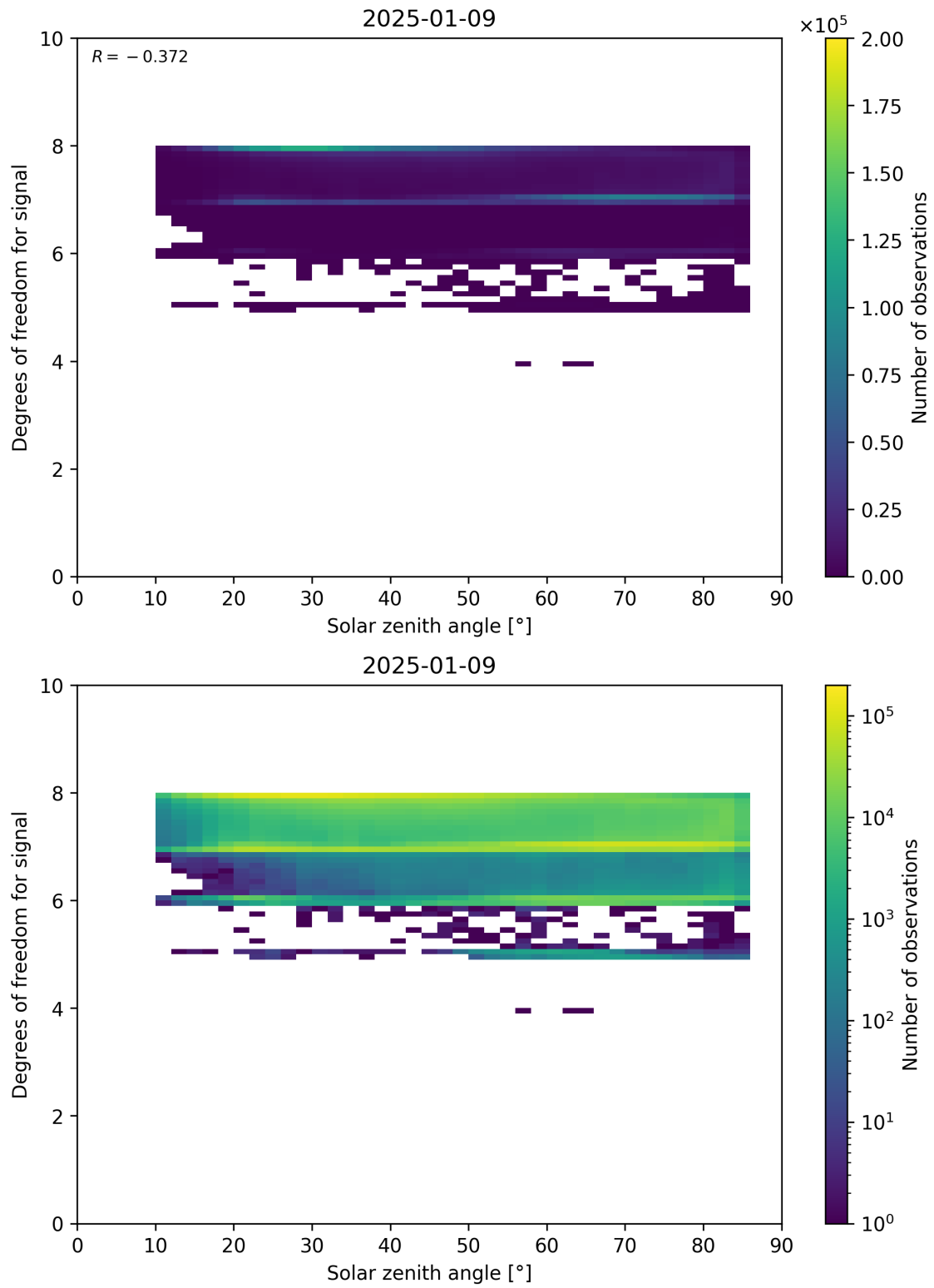
Figure 65: Scatter density plot of “Solar zenith angle” against “Degrees of freedom for signal” for 2025-01-08 to 2025-01-10.
