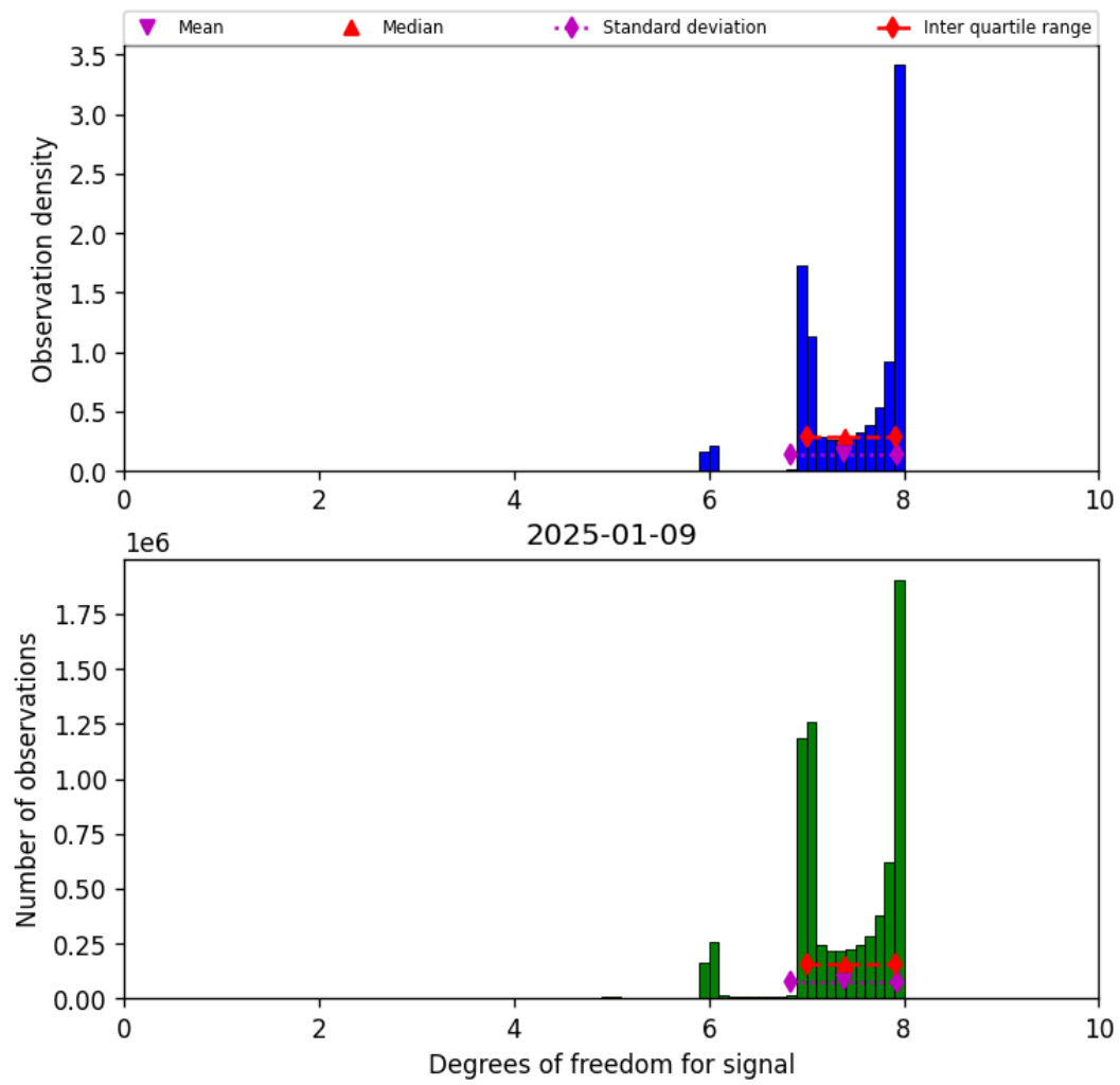
Figure 23: Histogram of “Degrees of freedom for signal” for 2025-01-08 to 2025-01-10
