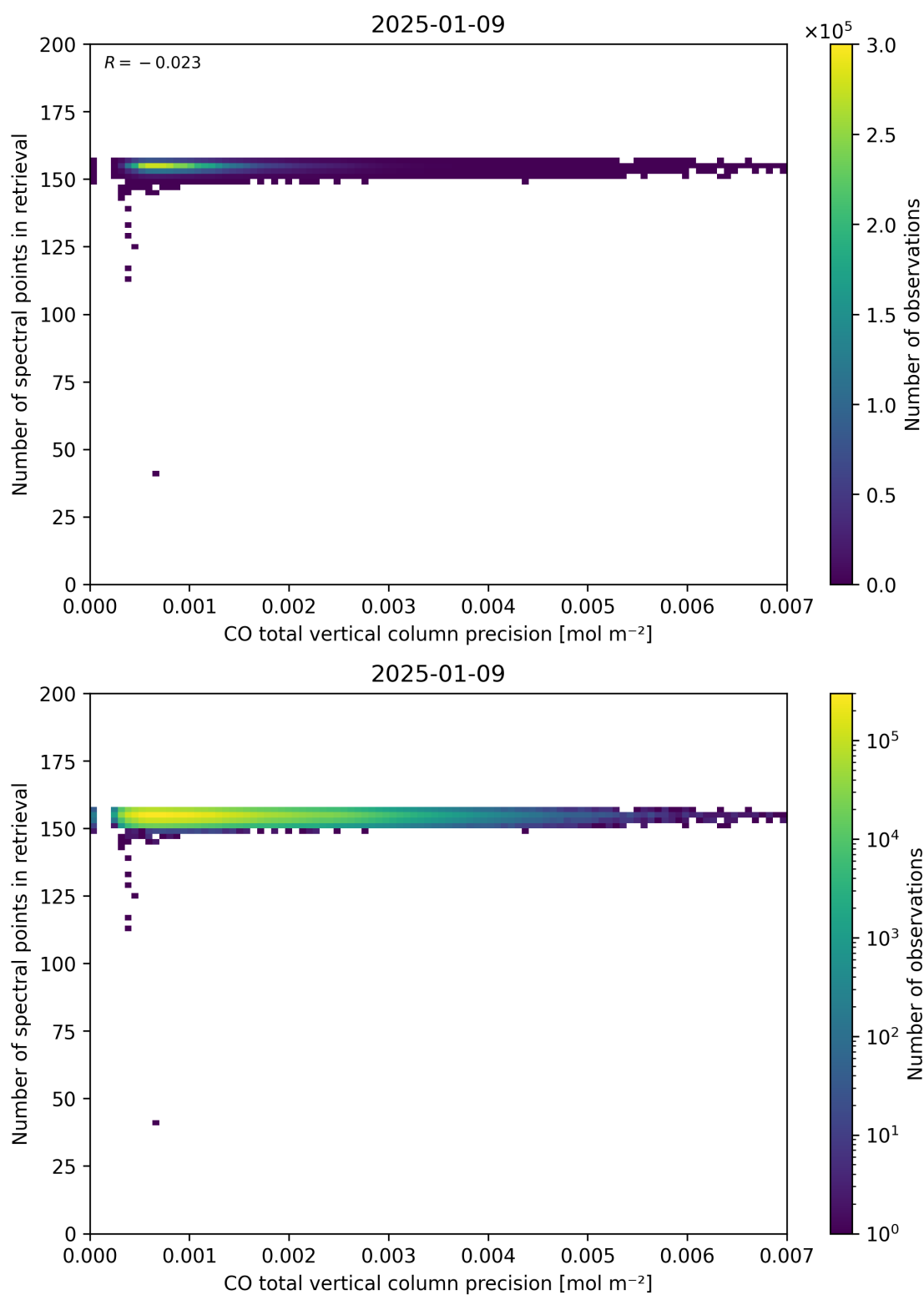
Figure 47: Scatter density plot of “CO total vertical column precision” against “Number of spectral points in retrieval” for 2025-01-08 to 2025-01-10.
