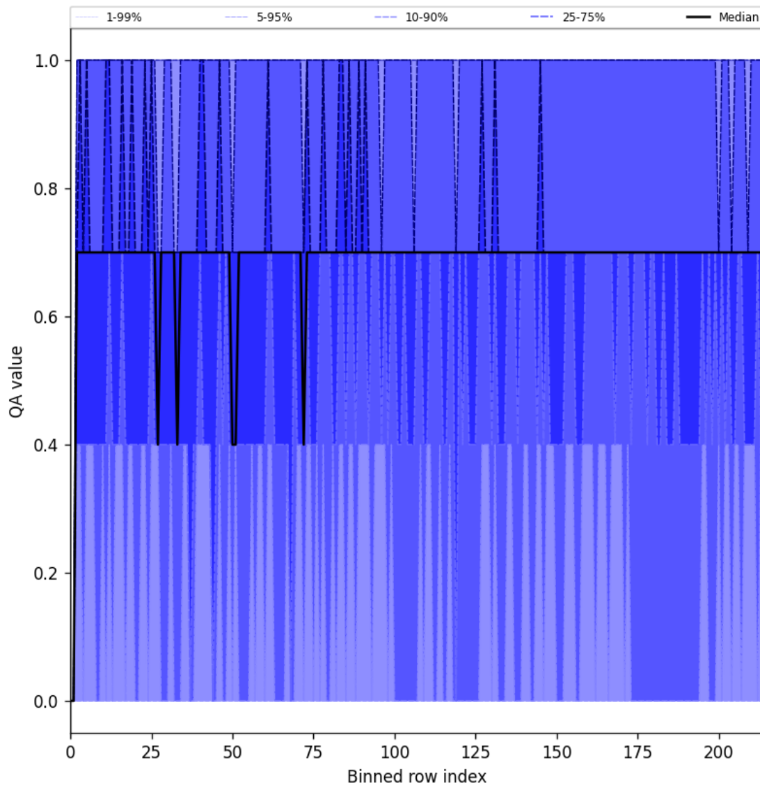
Figure 25: Along track statistics of “QA value” for 2025-01-08 to 2025-01-10
