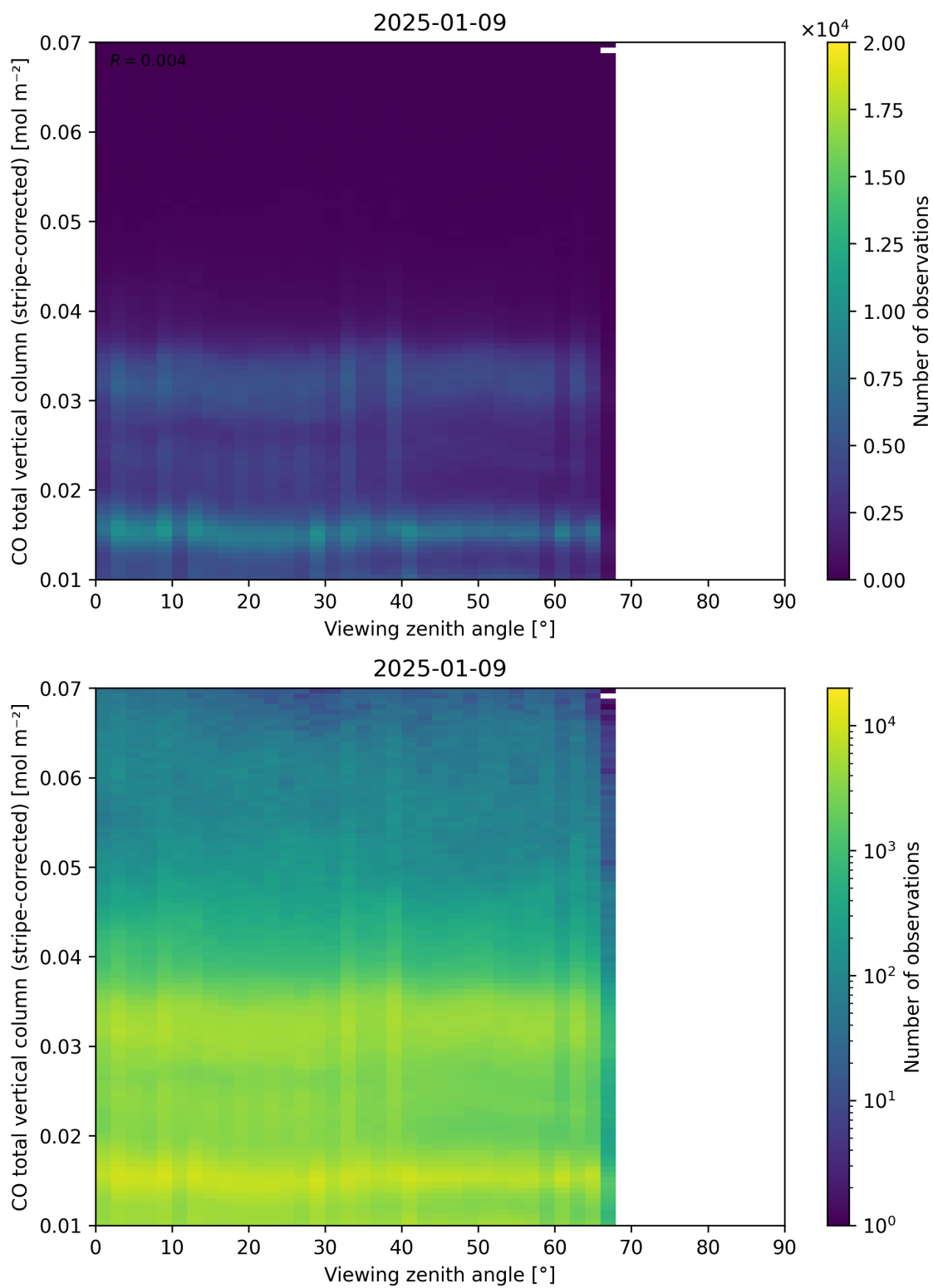
Figure 70: Scatter density plot of “Viewing zenith angle” against “CO total vertical column (stripe-corrected)” for 2025-01-08 to 2025-01-10.
