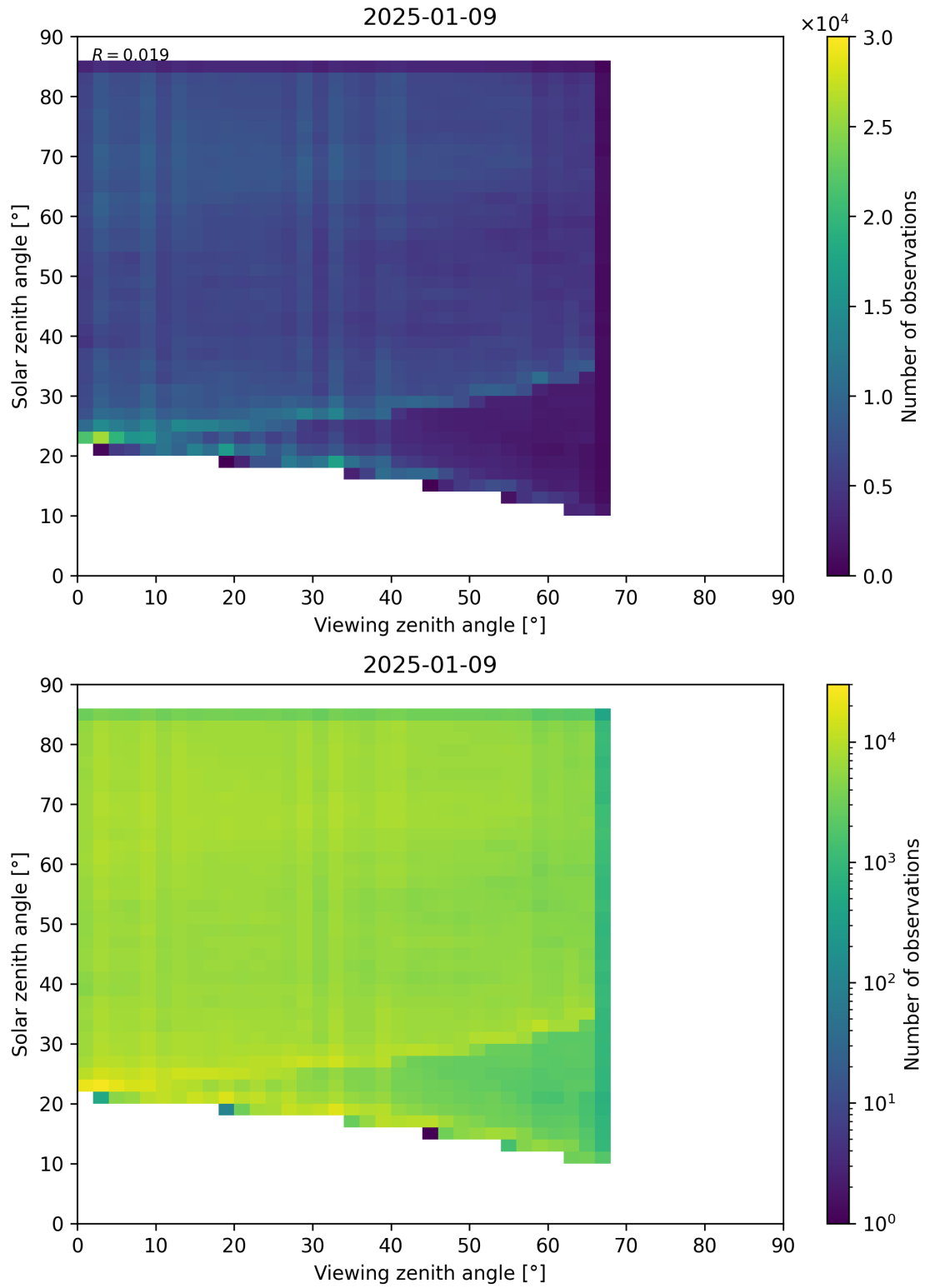
Figure 77: Scatter density plot of “Viewing zenith angle” against “Solar zenith angle” for 2025-01-08 to 2025-01-10.
