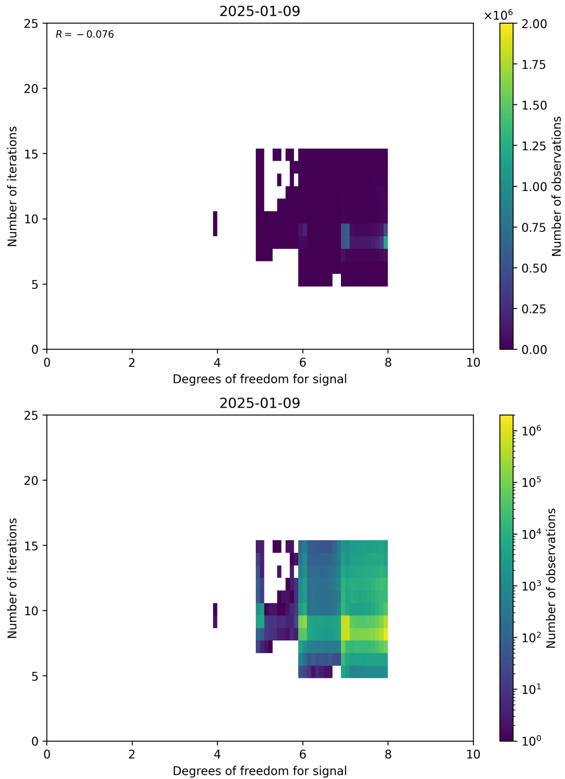
Figure 50: Scatter density plot of “Degrees of freedom for signal” against “Number of iterations” for 2025-01-08 to 2025-01-10.
