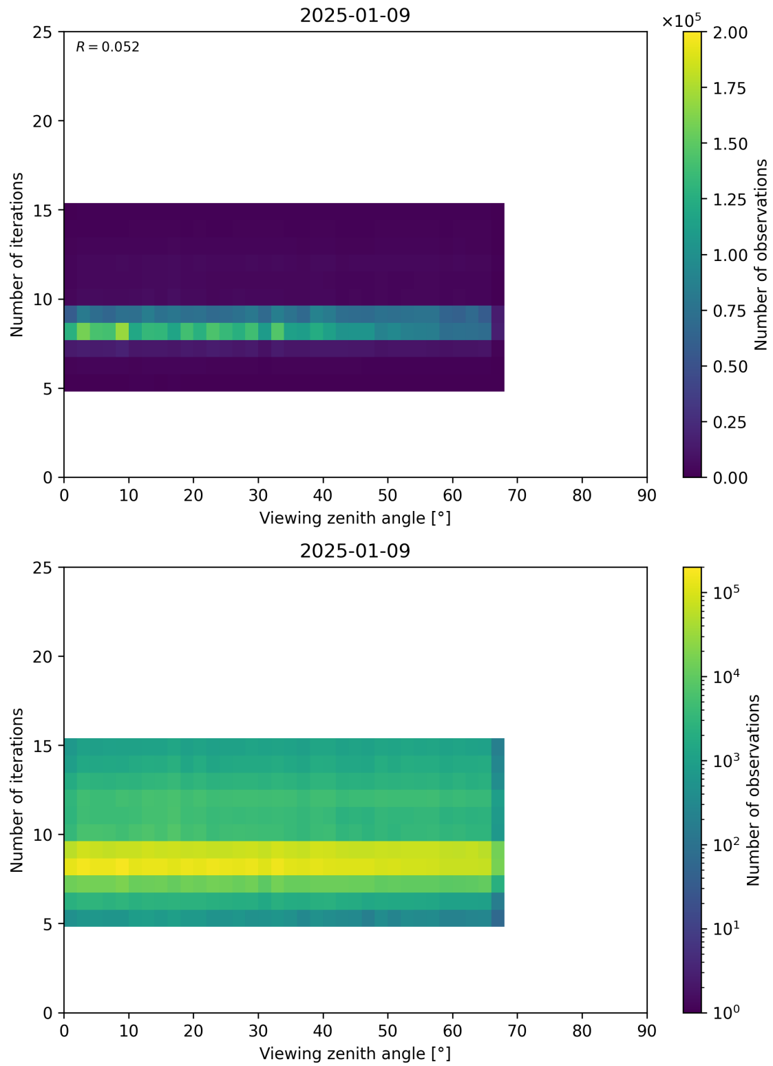
Figure 75: Scatter density plot of “Viewing zenith angle” against “Number of iterations” for 2025-01-08 to 2025-01-10.
