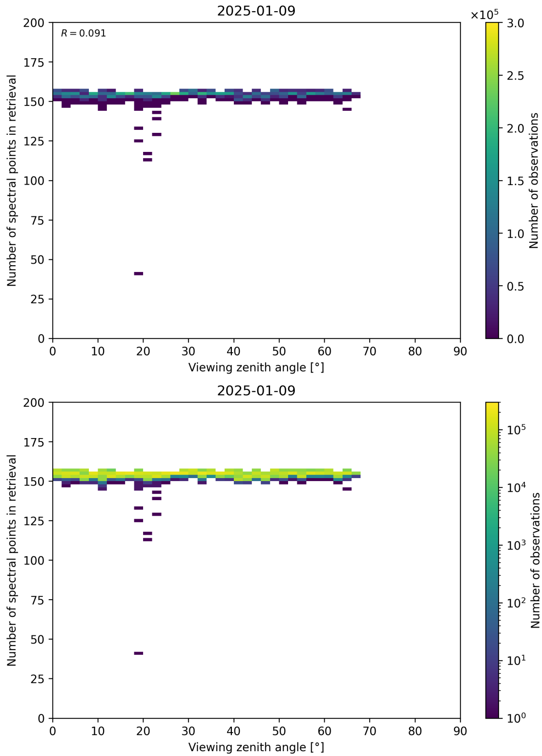
Figure 76: Scatter density plot of “Viewing zenith angle” against “Number of spectral points in retrieval” for 2025-01-08 to 2025-01-10.
