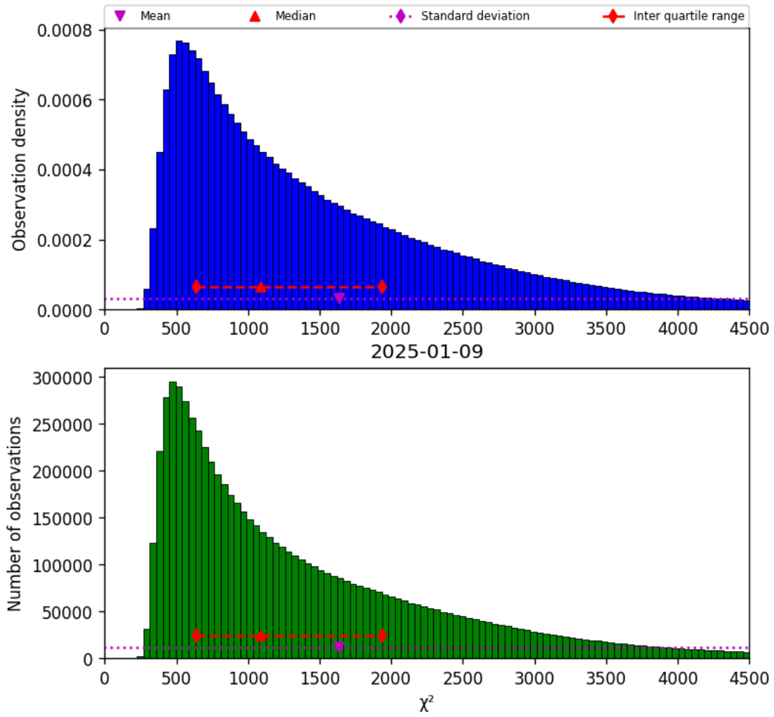
Figure 22: Histogram of “ \chi^2 ” for 2025-01-08 to 2025-01-10
