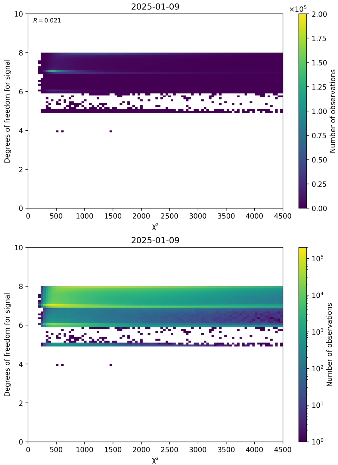
Figure 48: Scatter density plot of “ \chi^2 ” against “Degrees of freedom for signal” for 2025-01-08 to 2025-01-10.
