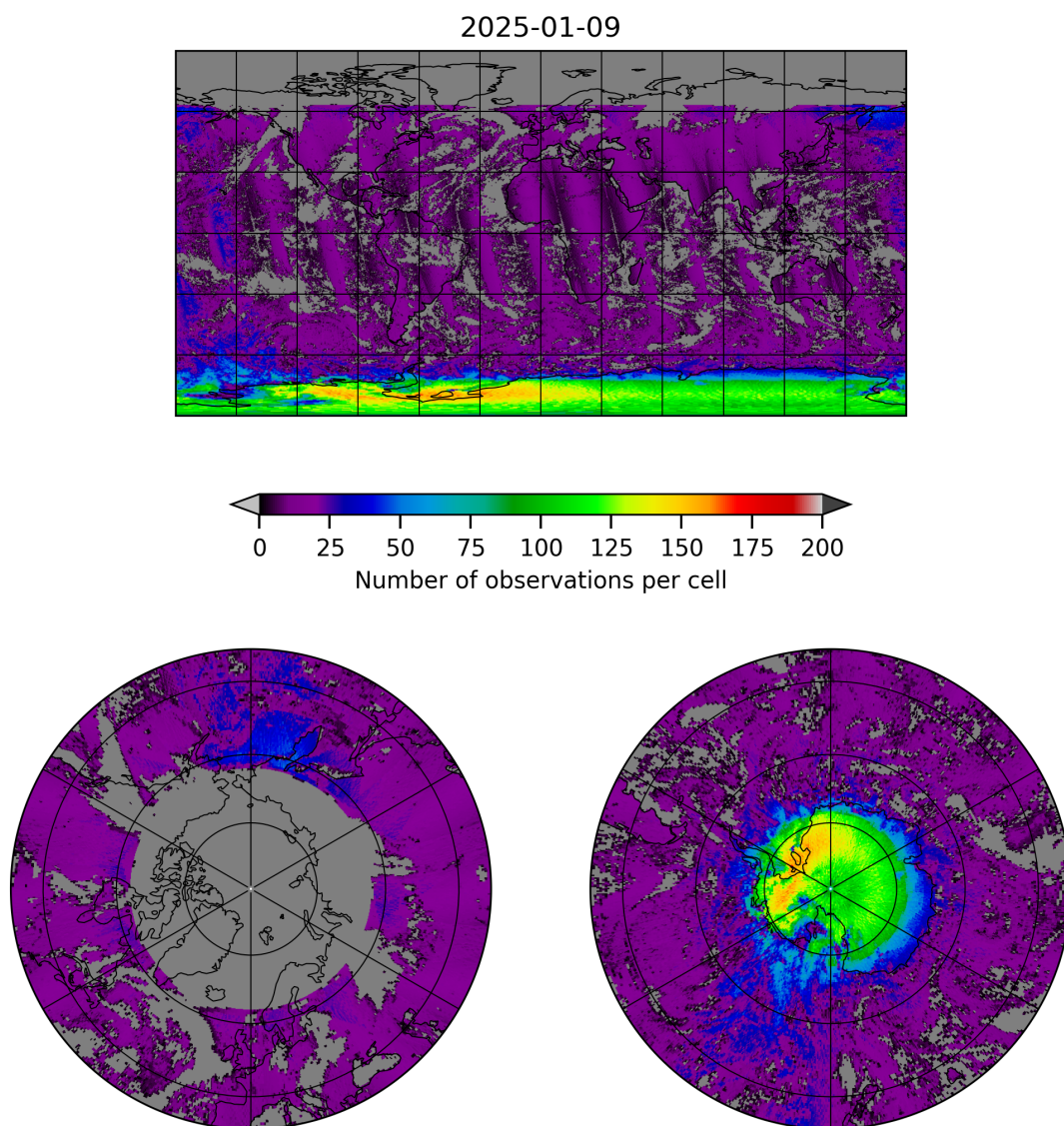
Figure 8: Map of the number of observations for 2025-01-08 to 2025-01-10
