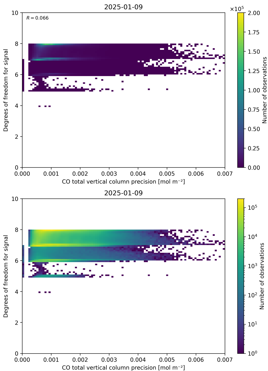
Figure 45: Scatter density plot of “CO total vertical column precision” against “Degrees of freedom for signal” for 2025-01-08 to 2025-01-10.
