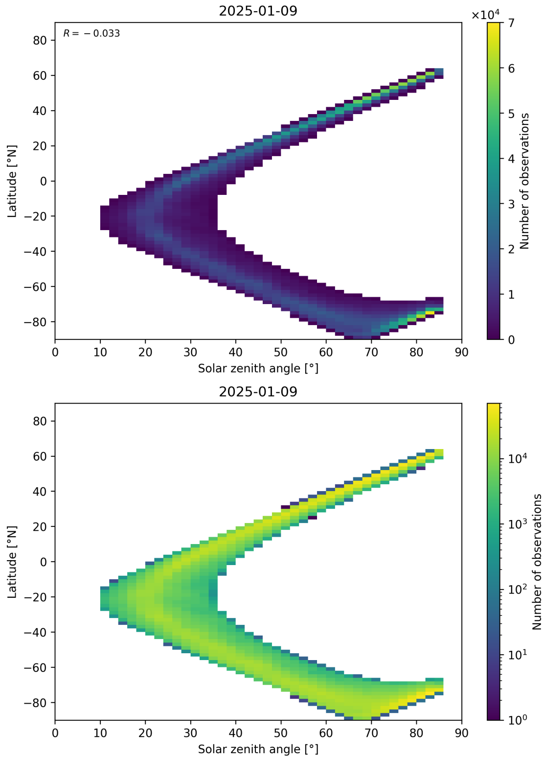
Figure 66: Scatter density plot of “Solar zenith angle” against “Latitude” for 2025-01-08 to 2025-01-10.
