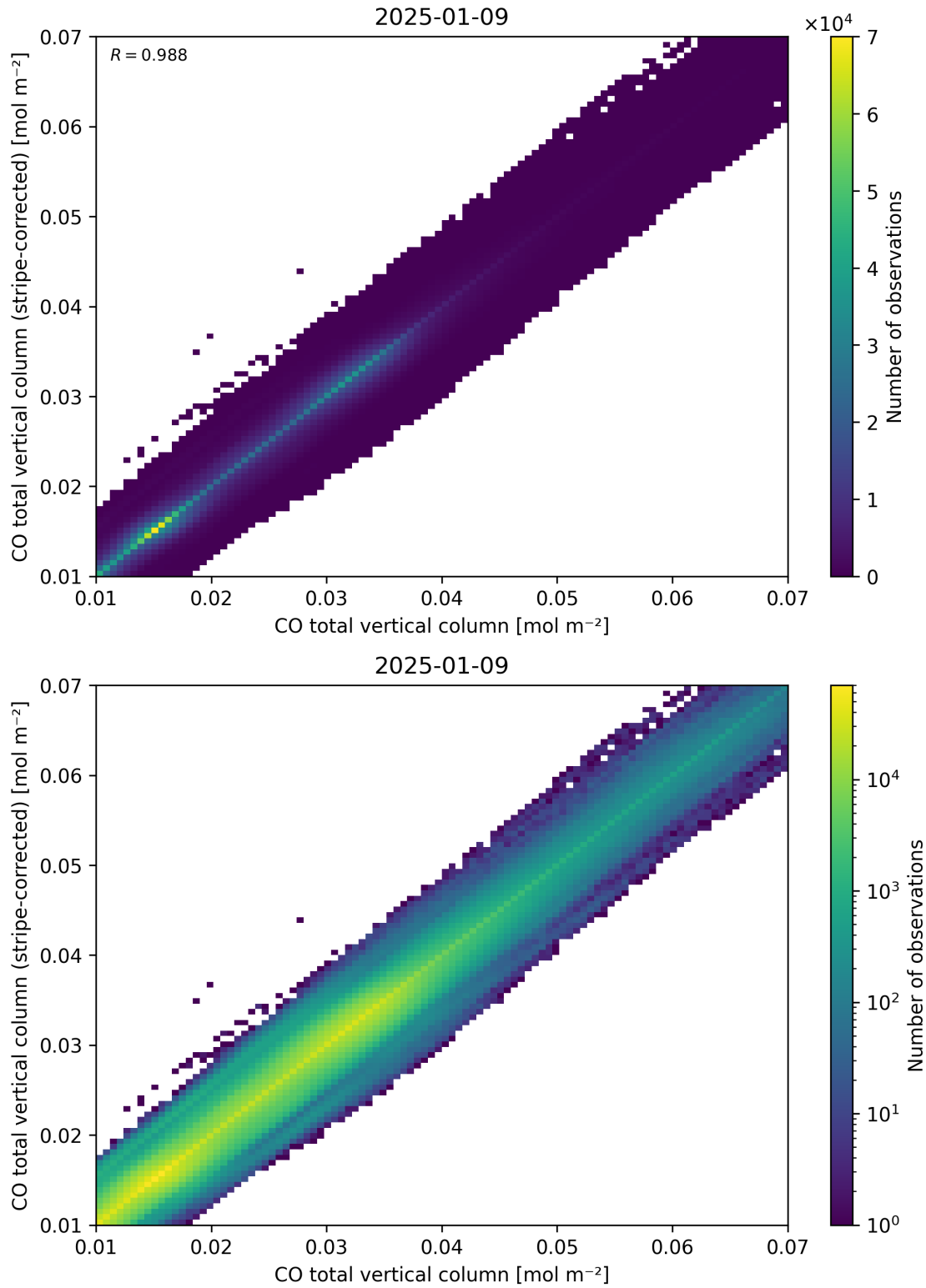
Figure 33: Scatter density plot of “CO total vertical column” against “CO total vertical column (stripe-corrected)” for 2025-01-08 to 2025-01-10.
