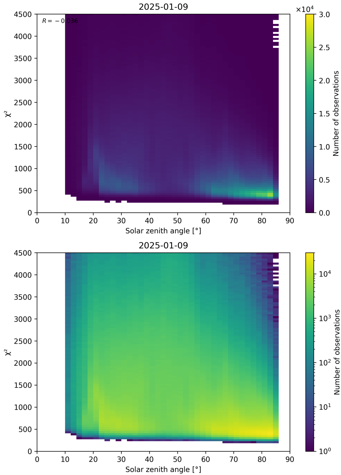
Figure 64: Scatter density plot of “Solar zenith angle” against “ \chi^2 ” for 2025-01-08 to 2025-01-10.
