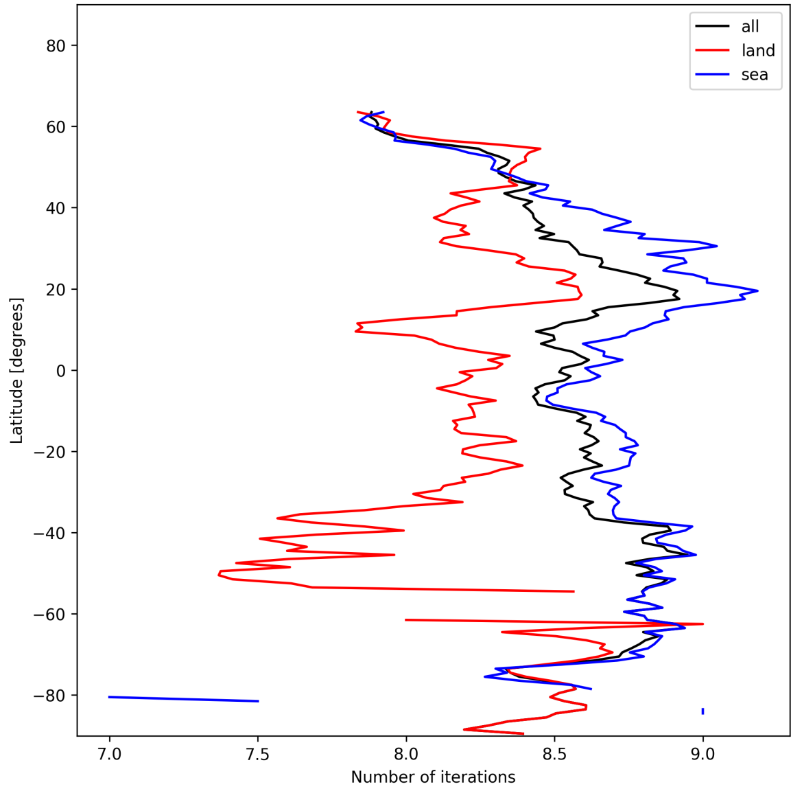
Figure 16: Zonal average of “Number of iterations” for 2025-01-08 to 2025-01-10.
