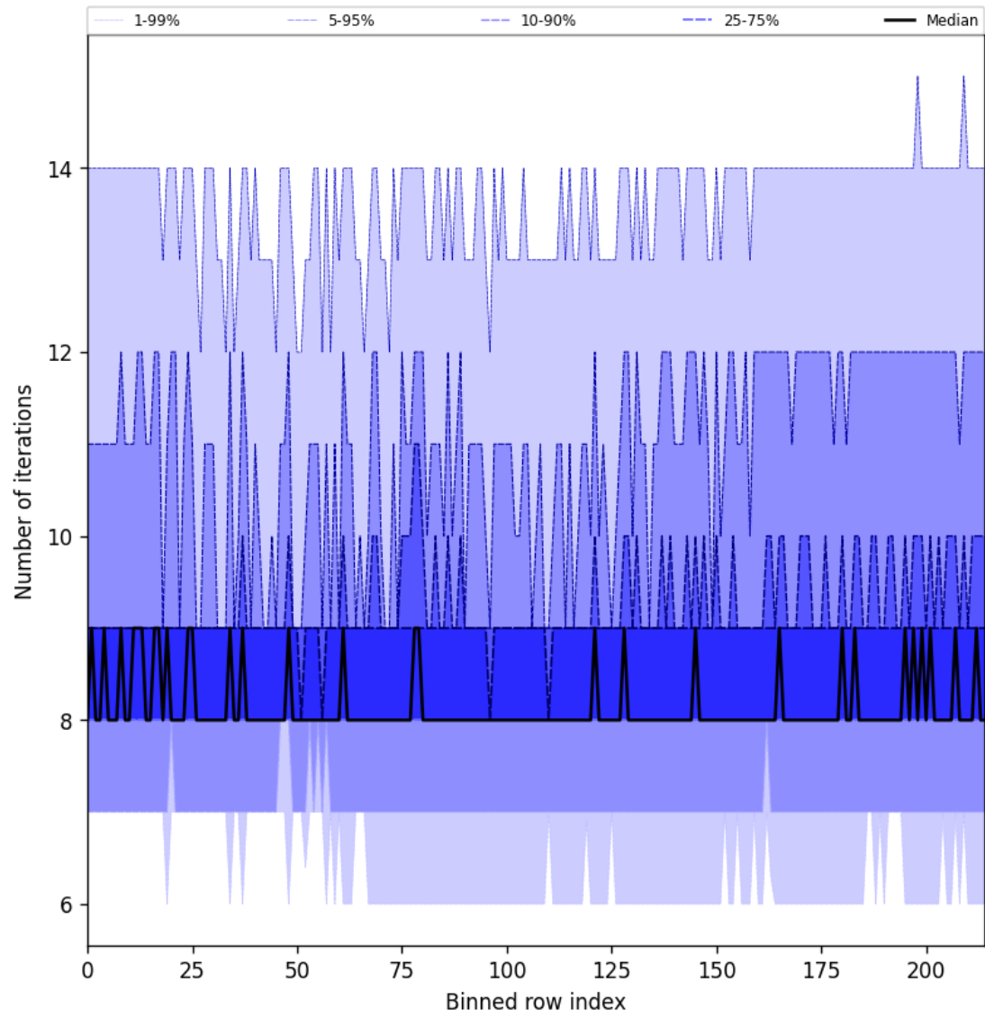
Figure 32: Along track statistics of “Number of iterations” for 2025-01-08 to 2025-01-10
