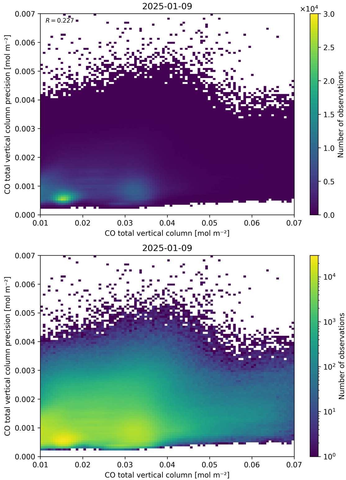
Figure 34: Scatter density plot of “CO total vertical column” against “CO total vertical column precision” for 2025-01-08 to 2025-01-10.
