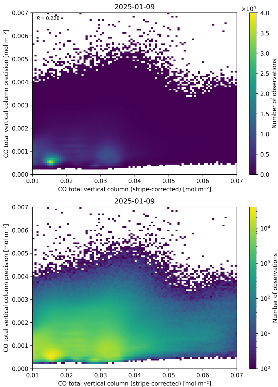
Figure 36: Scatter density plot of “CO total vertical column (stripe-corrected)” against “CO total vertical column precision” for 2025-01-08 to 2025-01-10.
