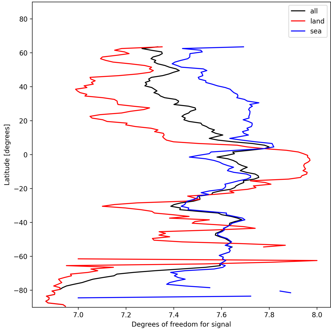
Figure 15: Zonal average of “Degrees of freedom for signal” for 2025-01-08 to 2025-01-10.
