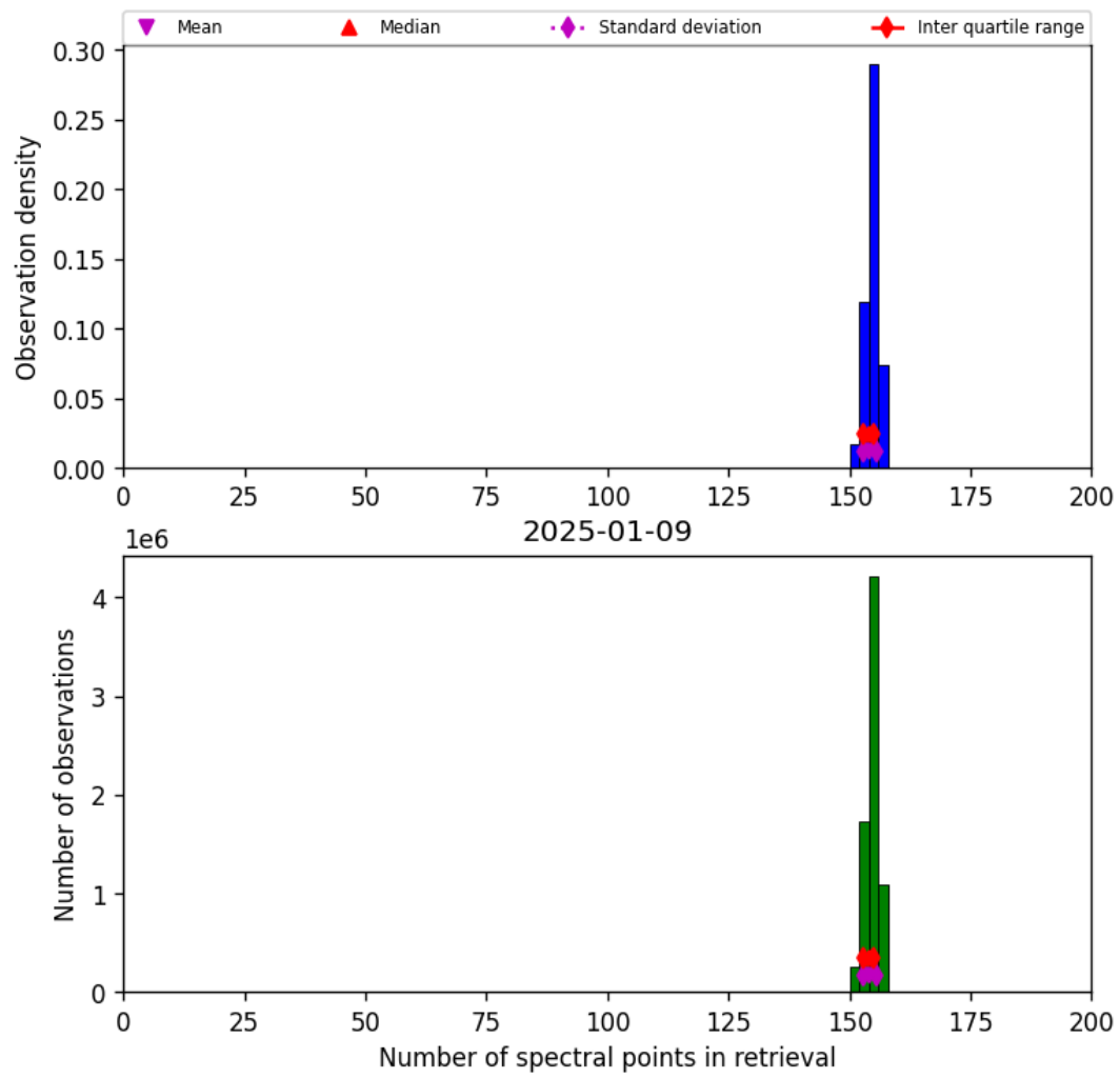
Figure 21: Histogram of “Number of spectral points in retrieval” for 2025-01-08 to 2025-01-10
