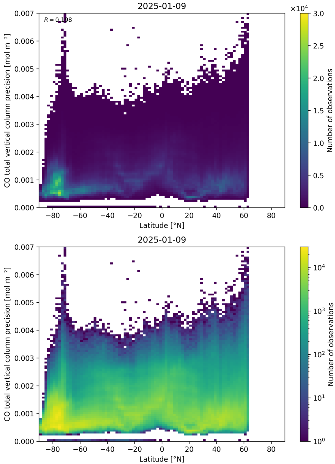
Figure 53: Scatter density plot of “Latitude” against “CO total vertical column precision” for 2025-01-08 to 2025-01-10.
