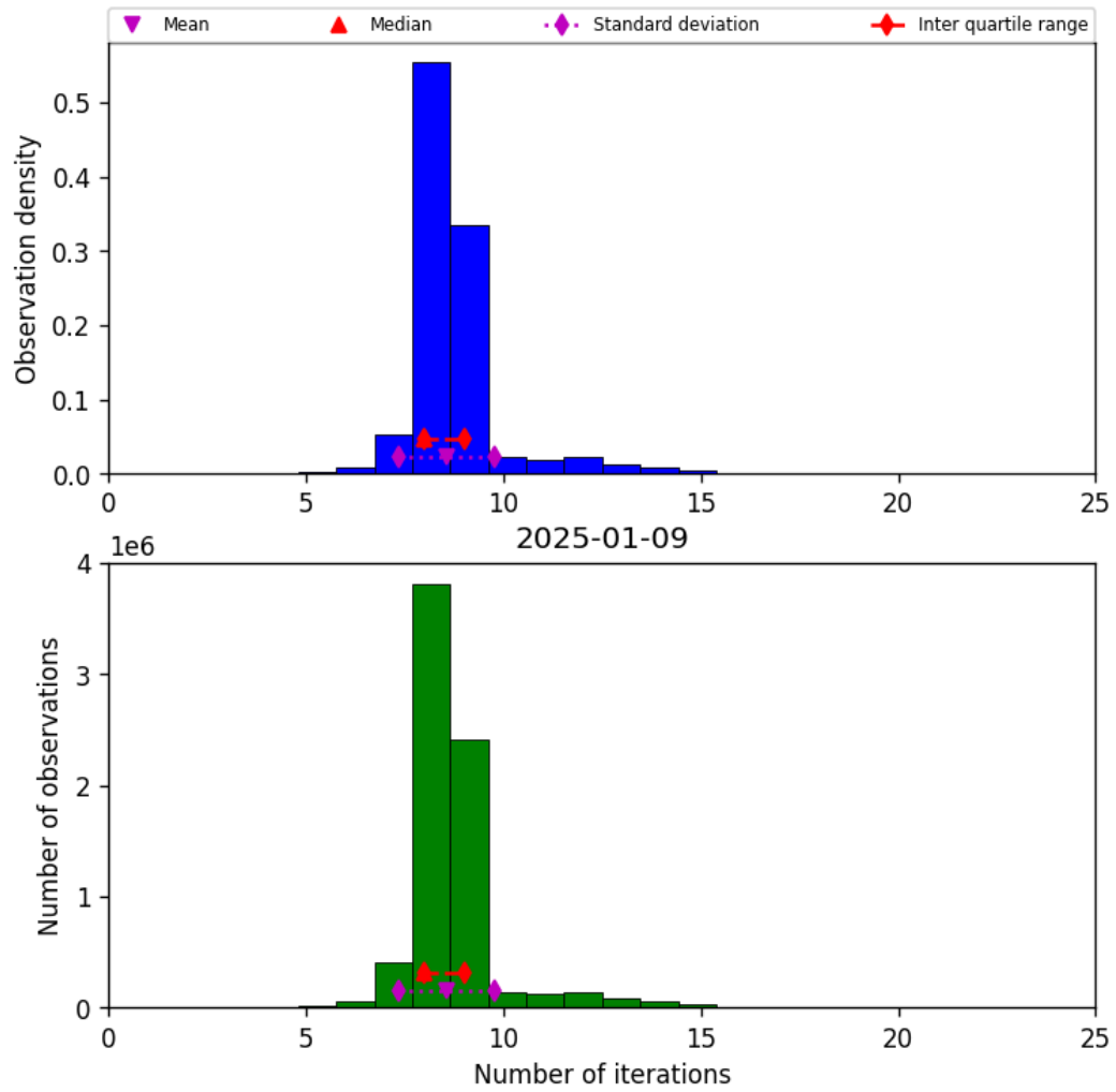
Figure 24: Histogram of “Number of iterations” for 2025-01-08 to 2025-01-10
