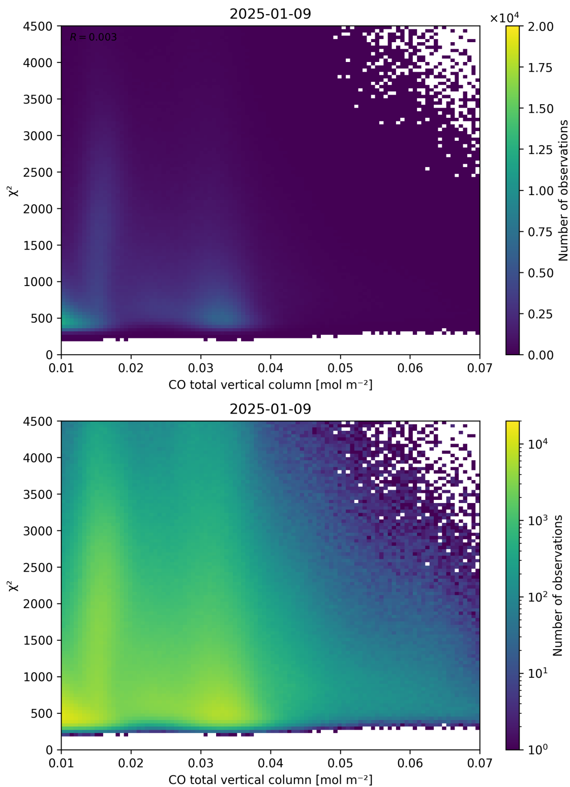
Figure 35: Scatter density plot of “CO total vertical column” against “ \chi^2 ” for 2025-01-08 to 2025-01-10.
