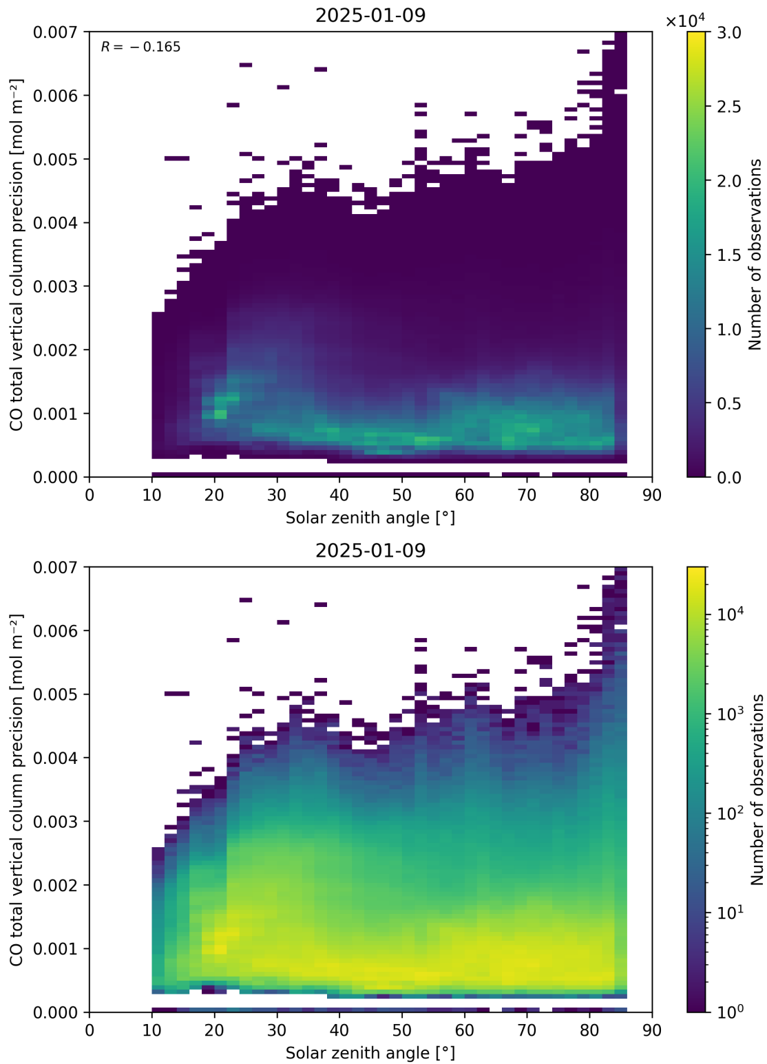
Figure 63: Scatter density plot of “Solar zenith angle” against “CO total vertical column precision” for 2025-01-08 to 2025-01-10.
