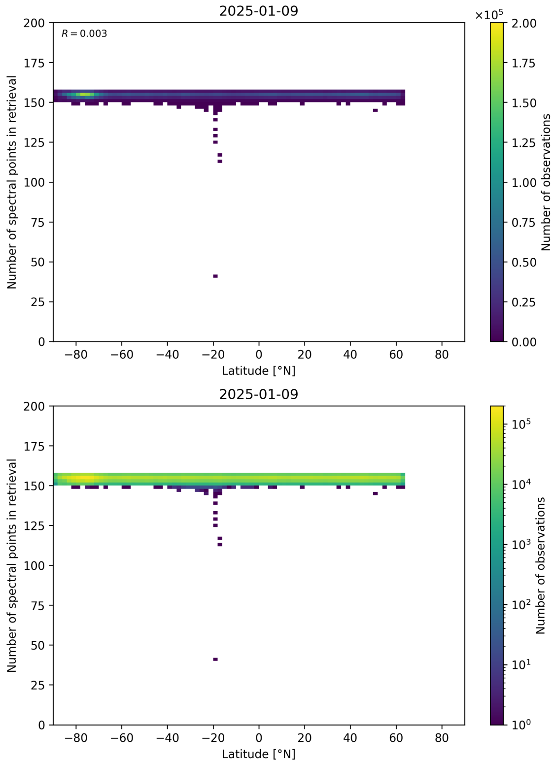
Figure 57: Scatter density plot of “Latitude” against “Number of spectral points in retrieval” for 2025-01-08 to 2025-01-10.
