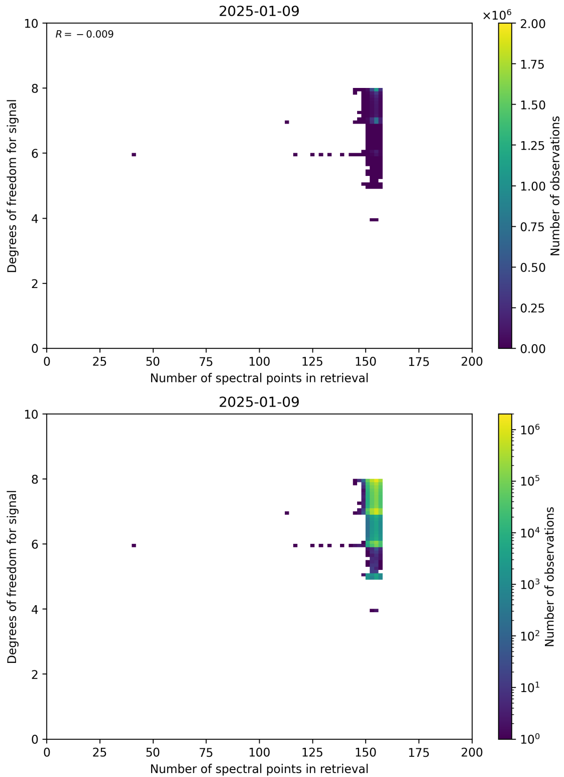
Figure 59: Scatter density plot of “Number of spectral points in retrieval” against “Degrees of freedom for signal” for 2025-01-08 to 2025-01-10.
