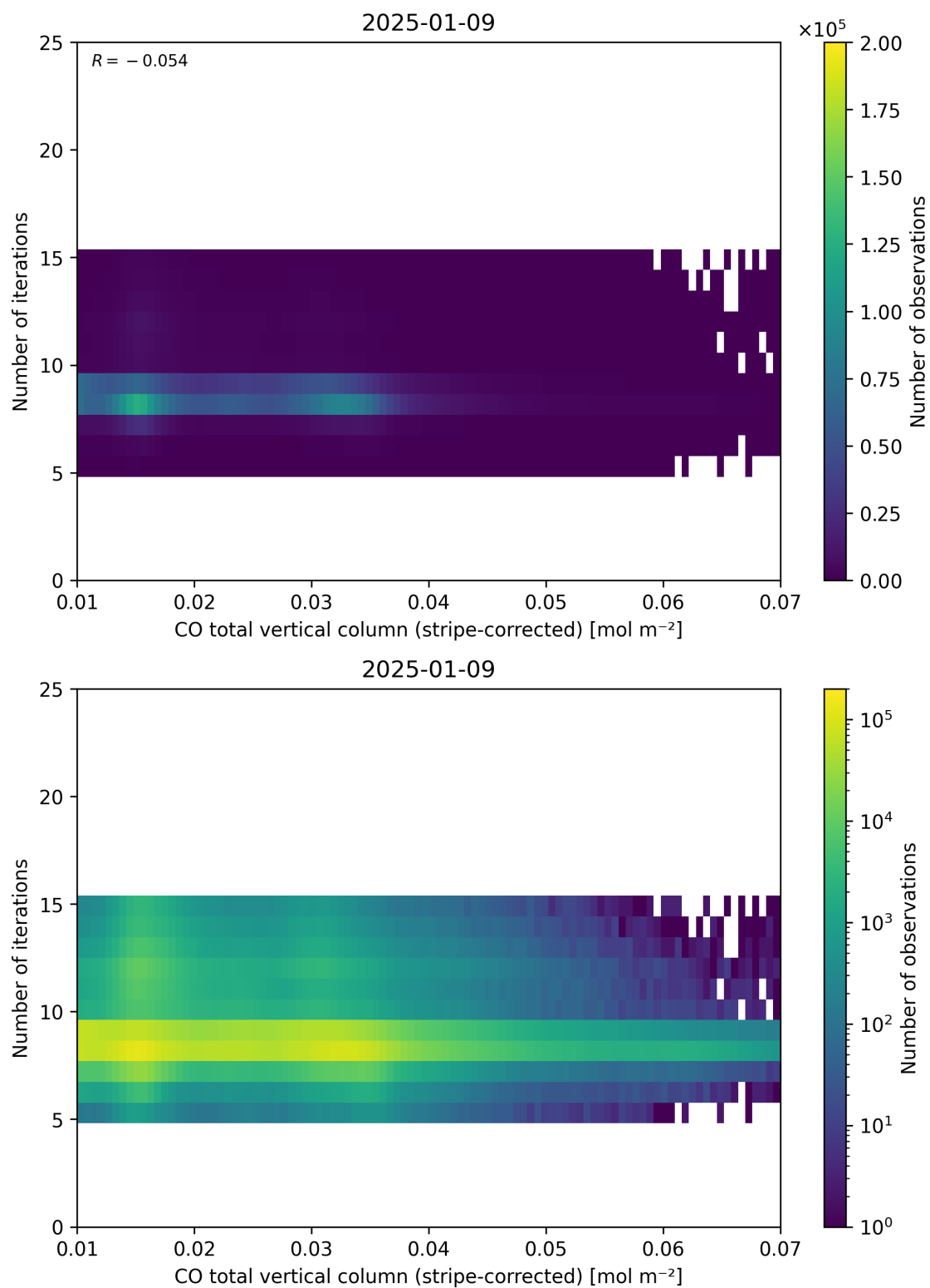
Figure 39: Scatter density plot of “CO total vertical column (stripe-corrected)” against “Number of iterations” for 2025-01-08 to 2025-01-10.
