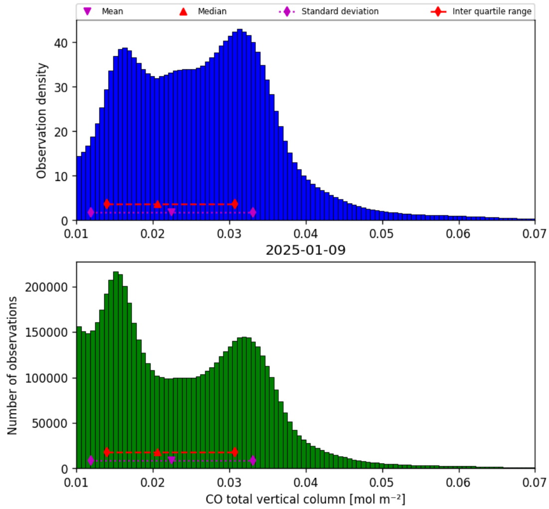
Figure 18: Histogram of “CO total vertical column” for 2025-01-08 to 2025-01-10
