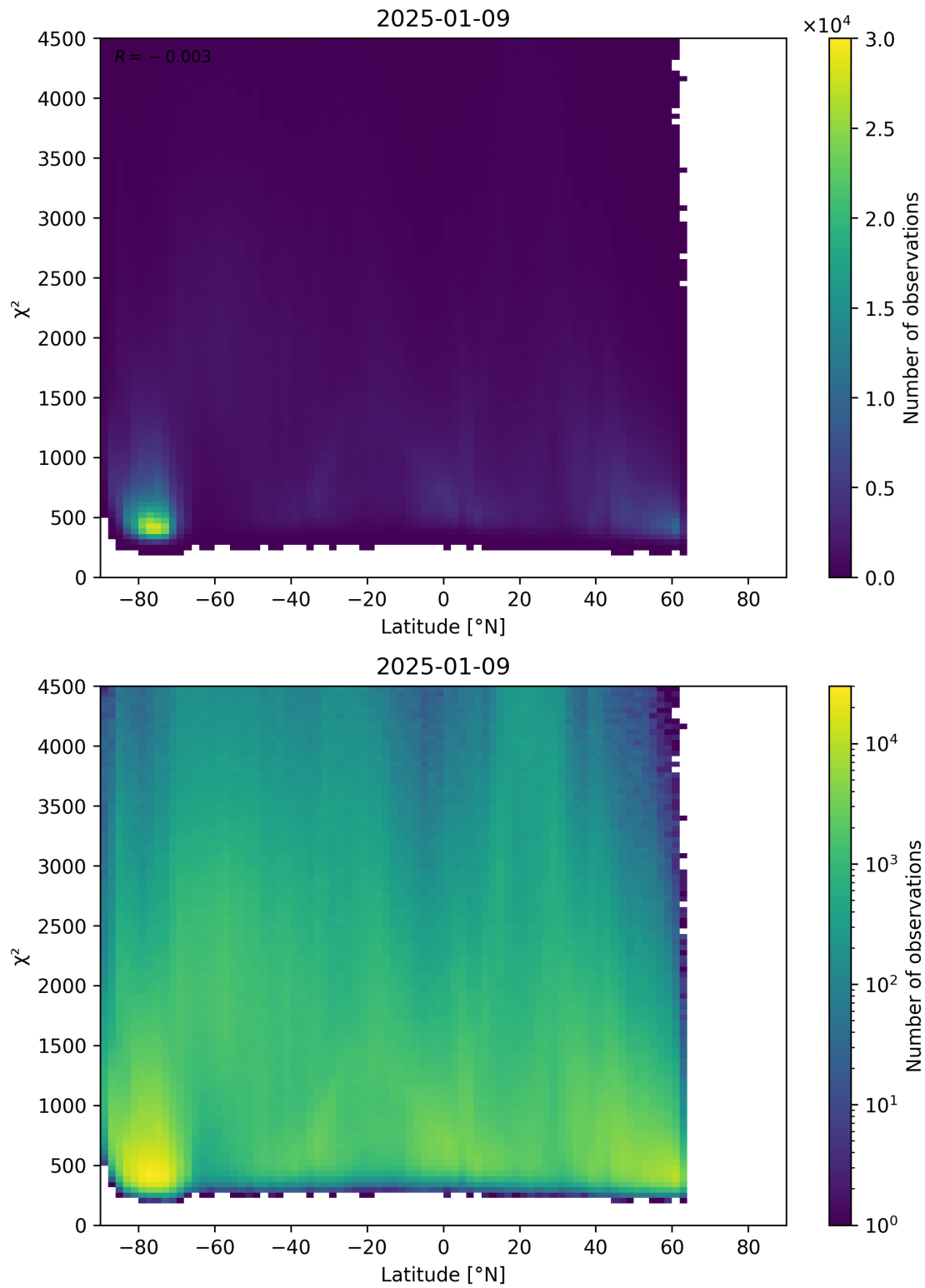
Figure 54: Scatter density plot of “Latitude” against “ \chi^2 ” for 2025-01-08 to 2025-01-10.
