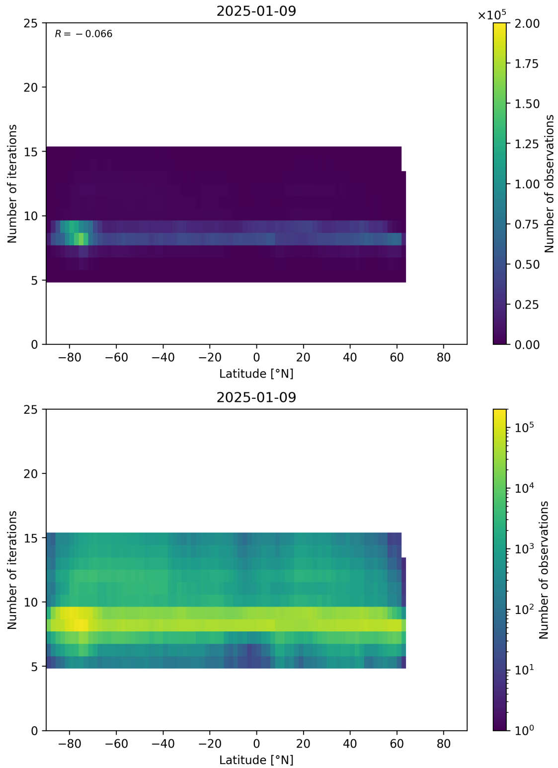
Figure 56: Scatter density plot of “Latitude” against “Number of iterations” for 2025-01-08 to 2025-01-10.
