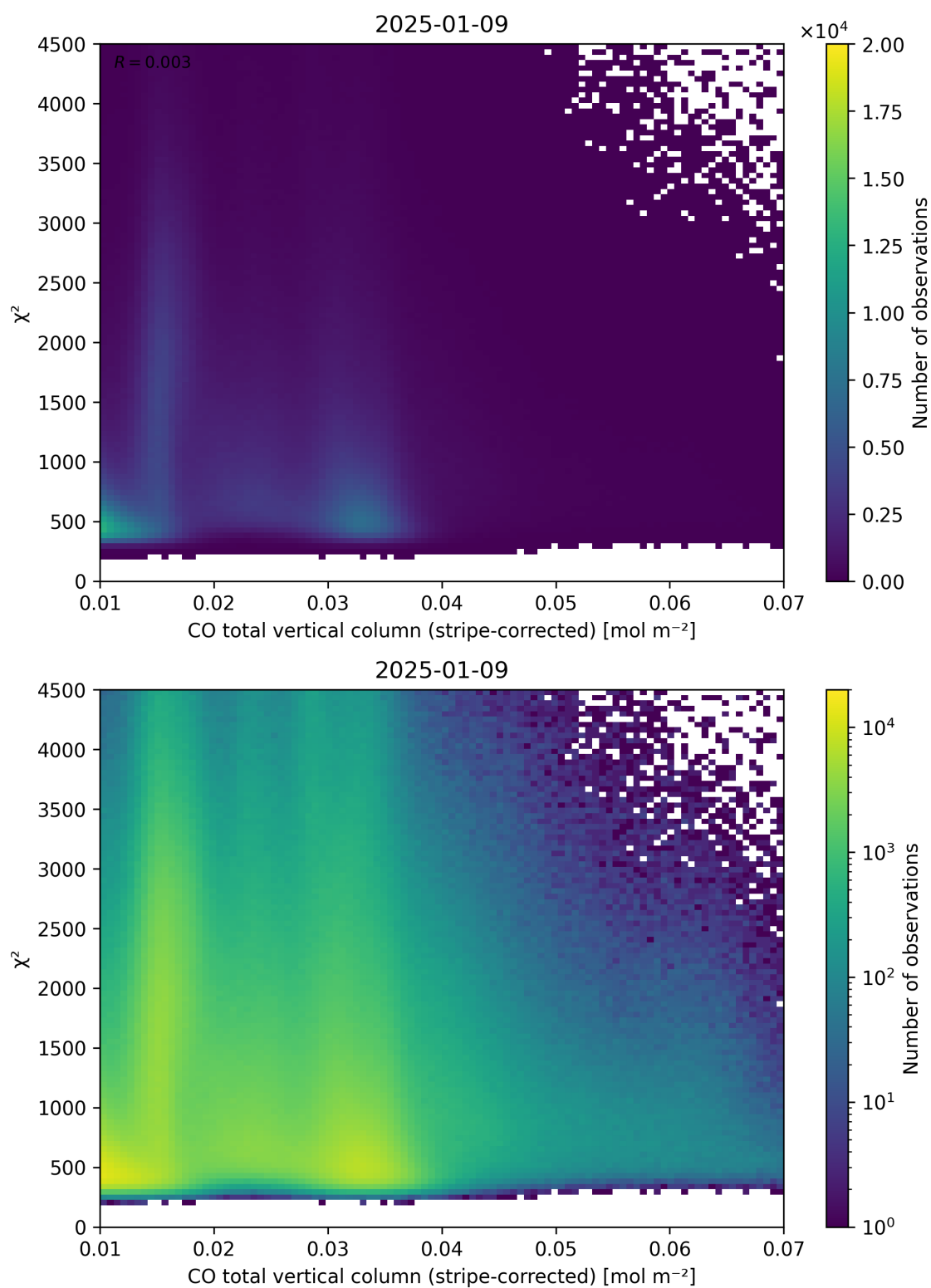
Figure 37: Scatter density plot of “CO total vertical column (stripe-corrected)” against “ \chi^2 ” for 2025-01-08 to 2025-01-10.
