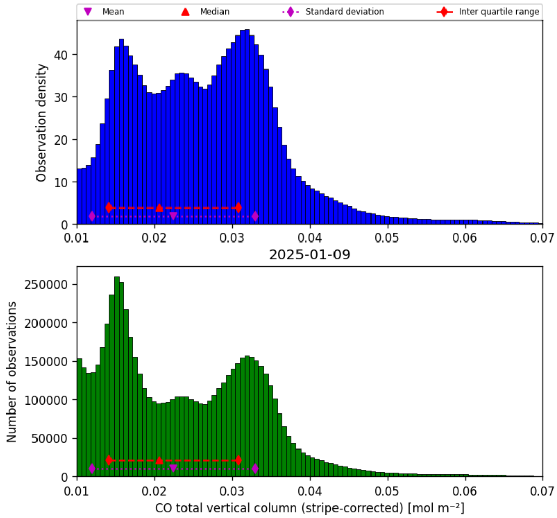
Figure 19: Histogram of “CO total vertical column (stripe-corrected)” for 2025-01-08 to 2025-01-10
