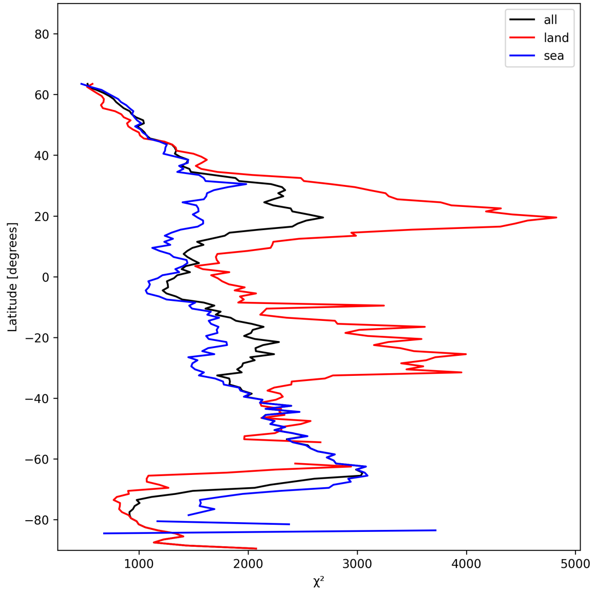
Figure 14: Zonal average of “ \chi^2 ” for 2025-01-08 to 2025-01-10.
