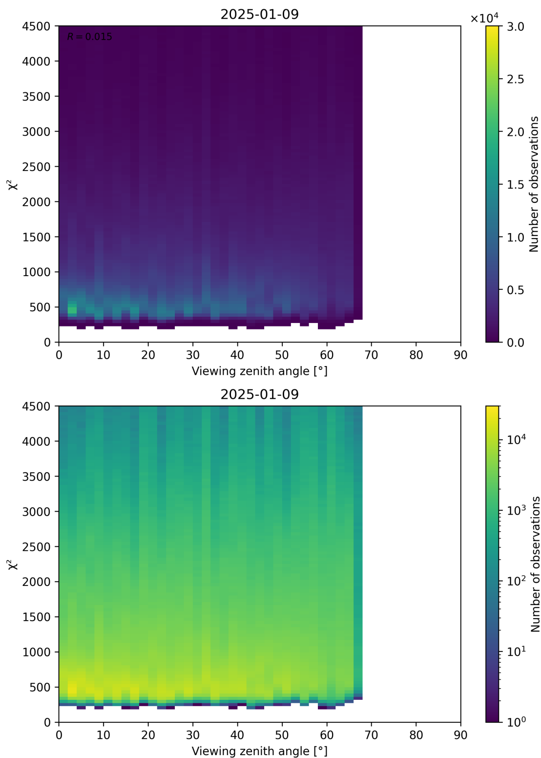
Figure 72: Scatter density plot of “Viewing zenith angle” against “ \chi^2 ” for 2025-01-08 to 2025-01-10.
