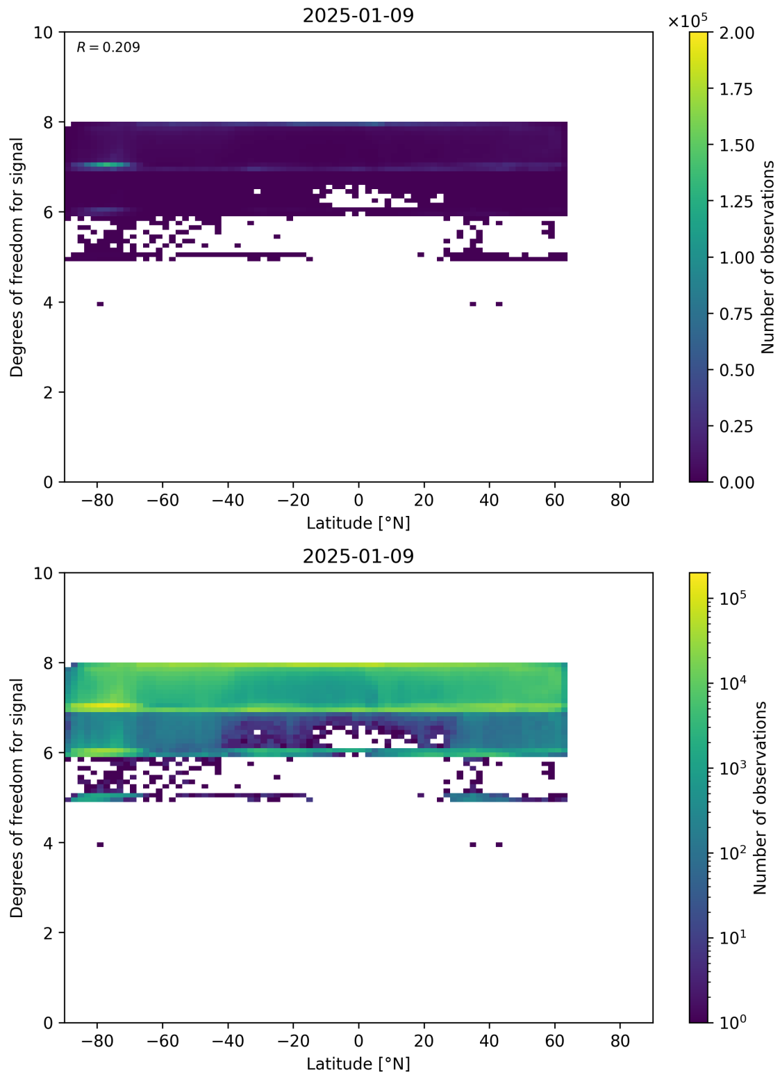
Figure 55: Scatter density plot of “Latitude” against “Degrees of freedom for signal” for 2025-01-08 to 2025-01-10.
