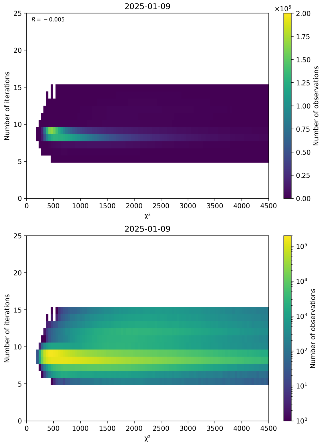
Figure 49: Scatter density plot of “ \chi^2 ” against “Number of iterations” for 2025-01-08 to 2025-01-10.
