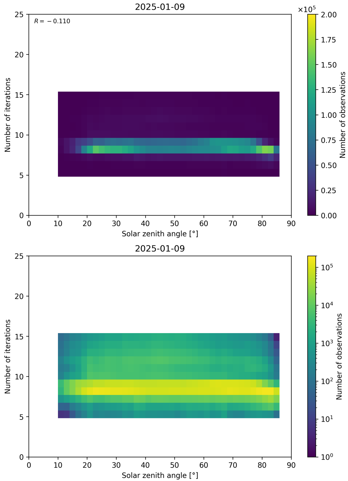
Figure 67: Scatter density plot of “Solar zenith angle” against “Number of iterations” for 2025-01-08 to 2025-01-10.
