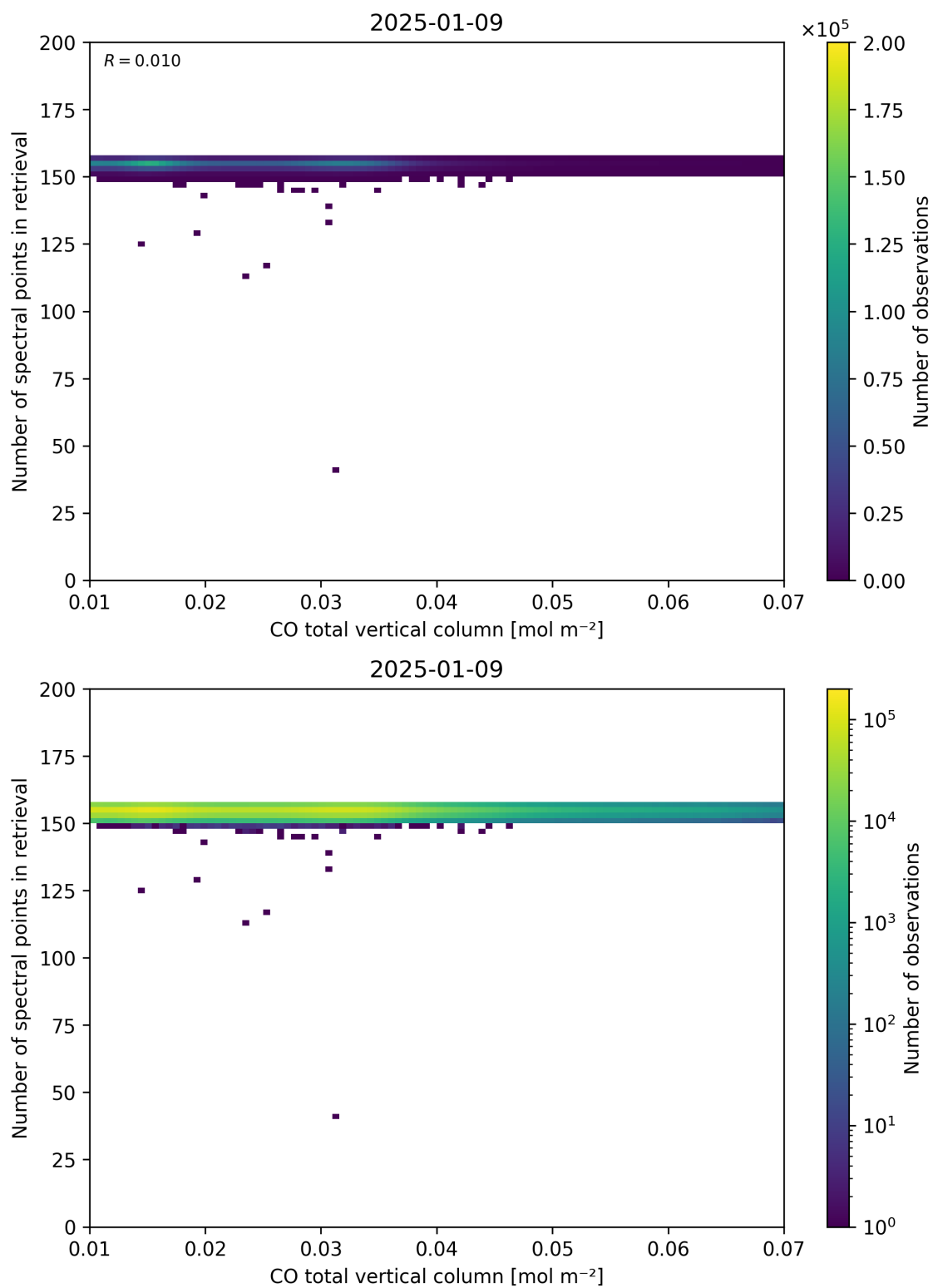
Figure 43: Scatter density plot of “CO total vertical column” against “Number of spectral points in retrieval” for 2025-01-08 to 2025-01-10.
