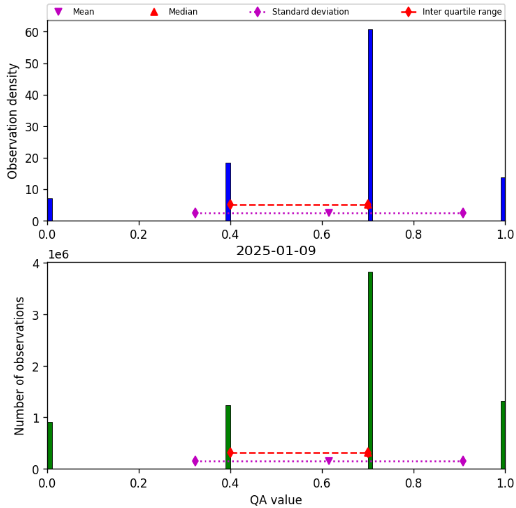
Figure 17: Histogram of “QA value” for 2025-01-08 to 2025-01-10
