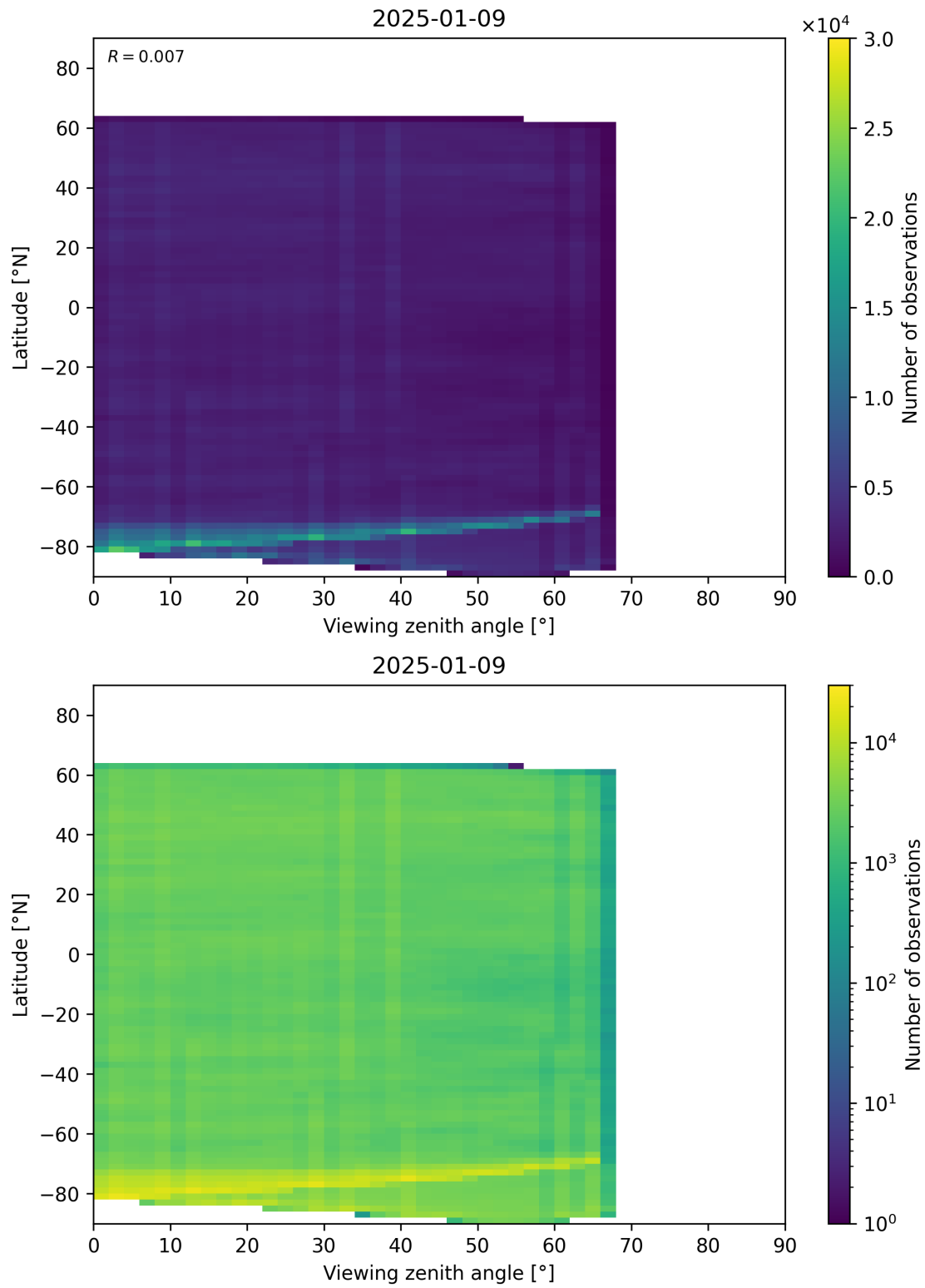
Figure 74: Scatter density plot of “Viewing zenith angle” against “Latitude” for 2025-01-08 to 2025-01-10.
