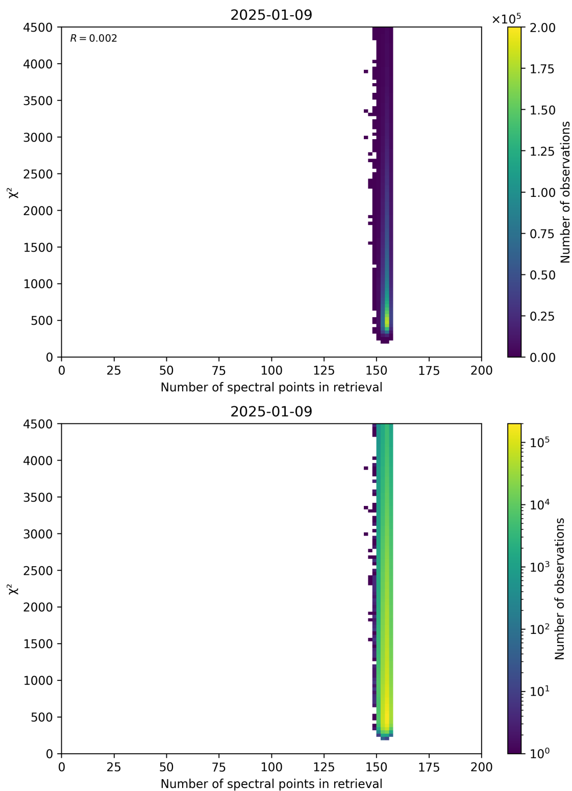
Figure 58: Scatter density plot of “Number of spectral points in retrieval” against “ \chi^2 ” for 2025-01-08 to 2025-01-10.
