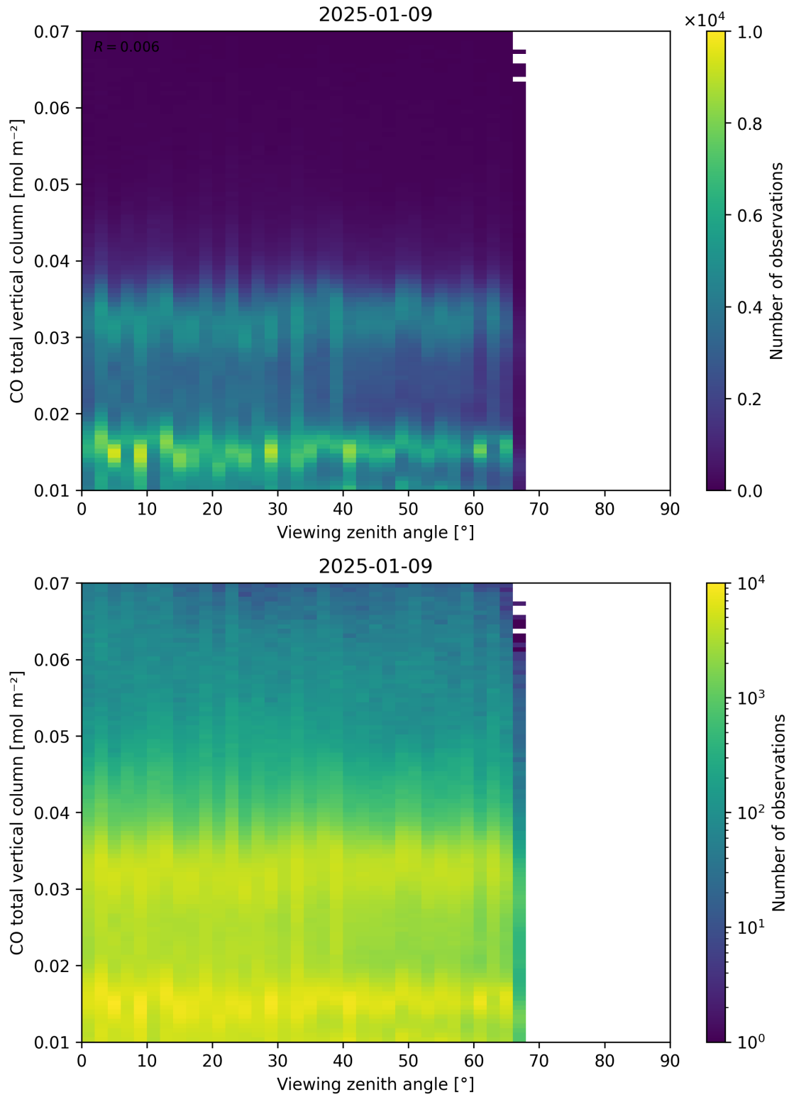
Figure 69: Scatter density plot of “Viewing zenith angle” against “CO total vertical column” for 2025-01-08 to 2025-01-10.
