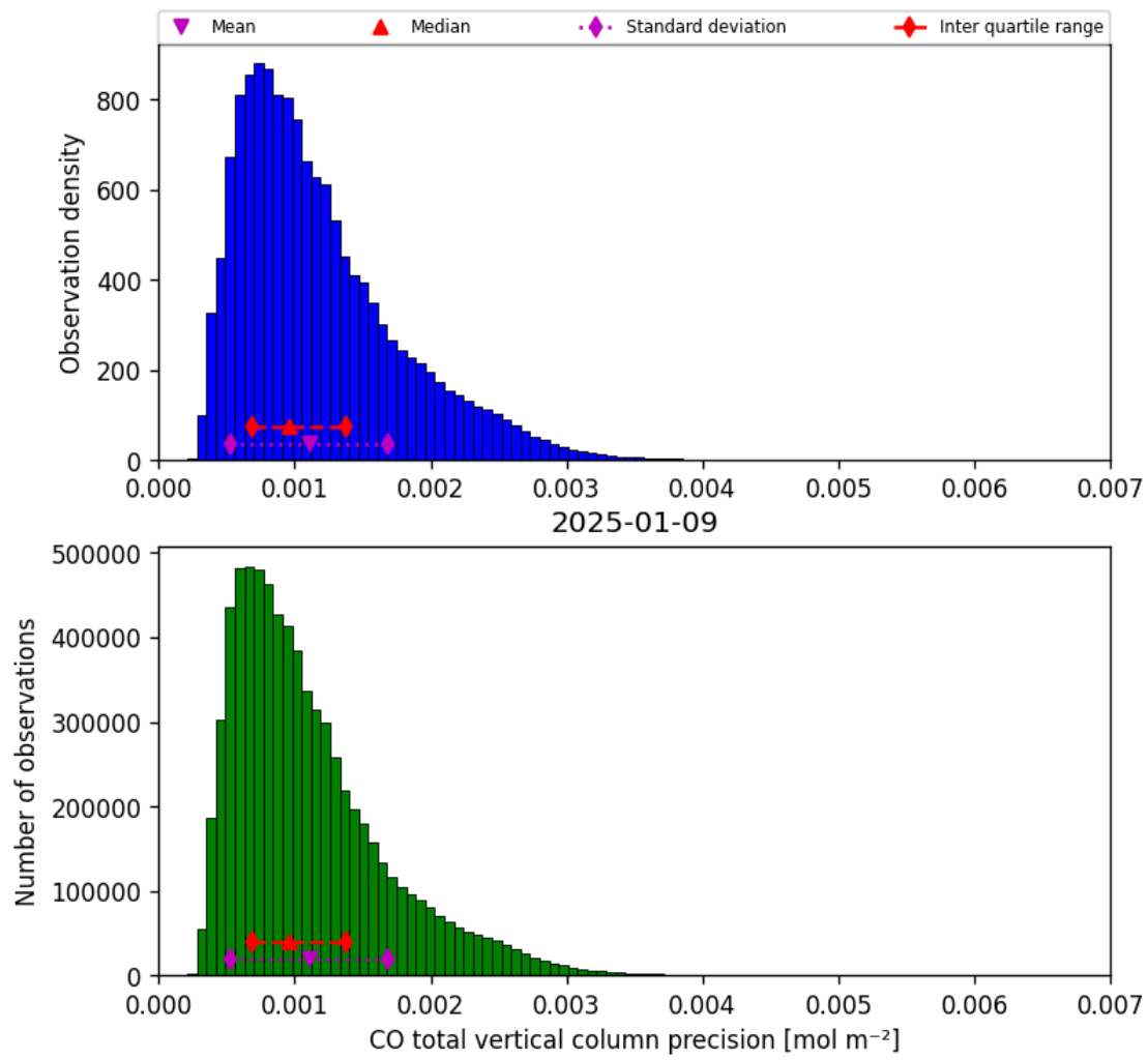
Figure 20: Histogram of “CO total vertical column precision” for 2025-01-08 to 2025-01-10
