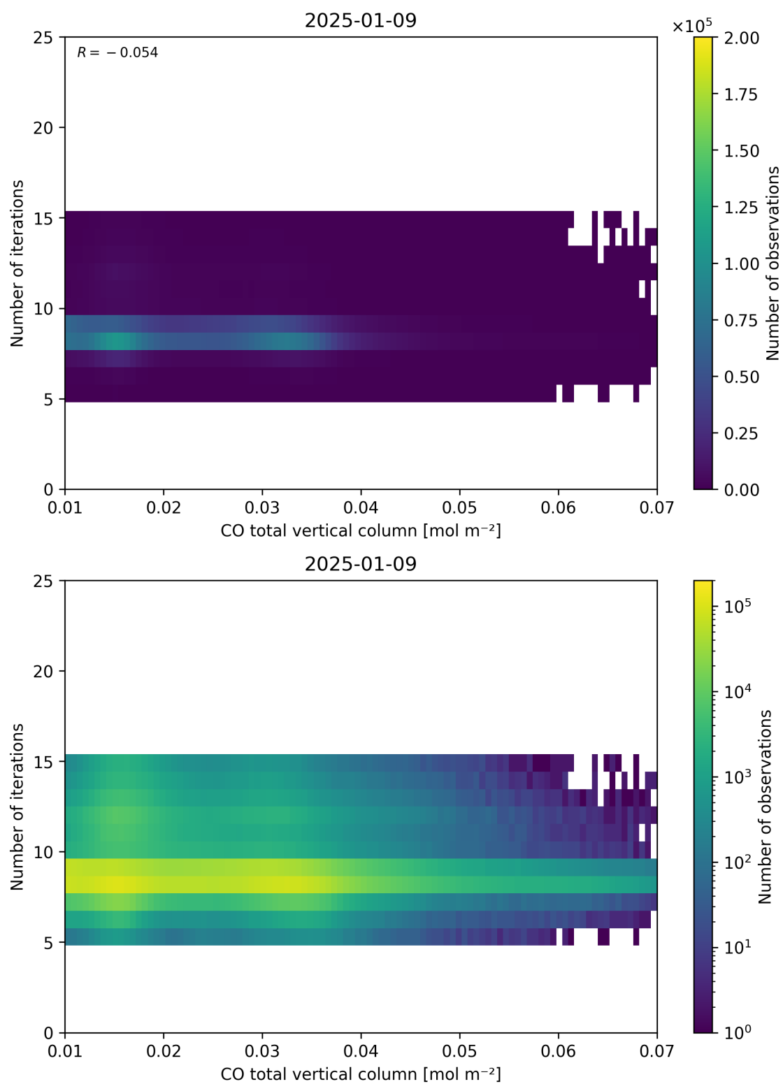
Figure 42: Scatter density plot of “CO total vertical column” against “Number of iterations” for 2025-01-08 to 2025-01-10.
