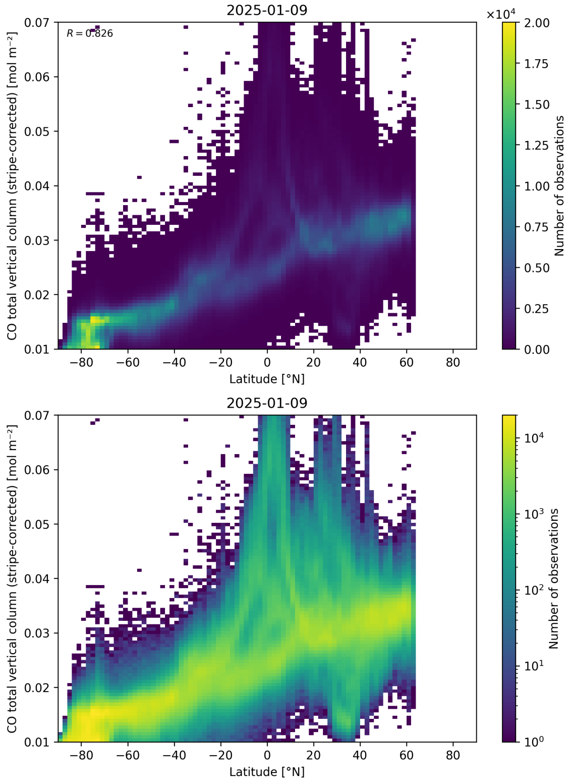
Figure 52: Scatter density plot of “Latitude” against “CO total vertical column (stripe-corrected)” for 2025-01-08 to 2025-01-10.
