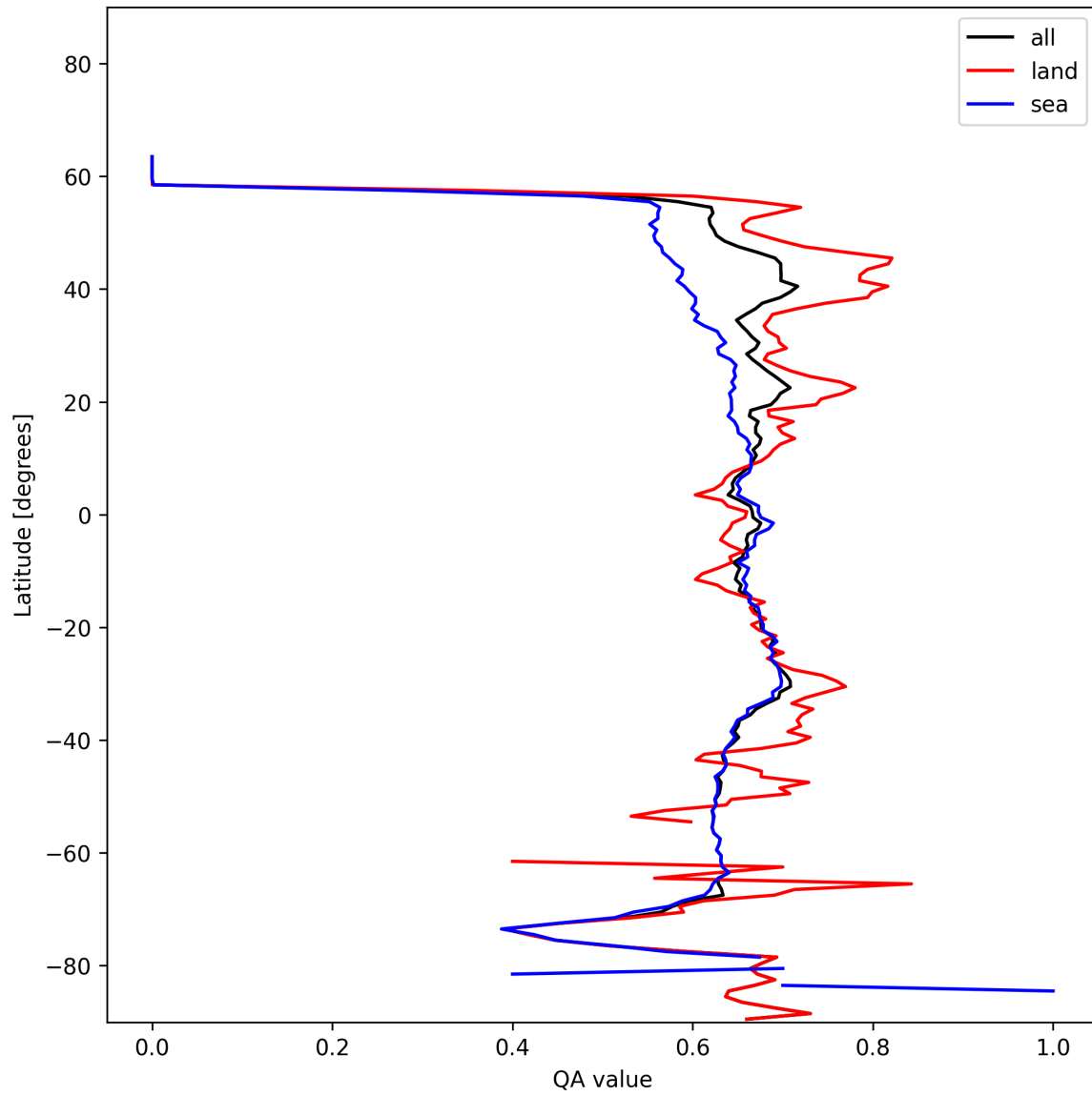
Figure 9: Zonal average of “QA value” for 2025-01-08 to 2025-01-10.
