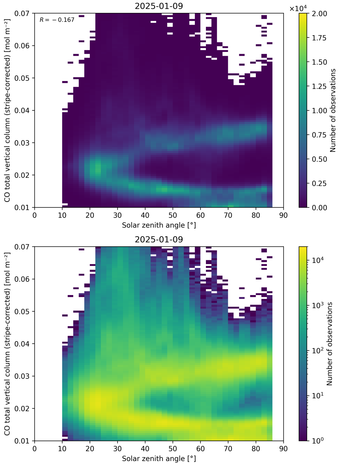
Figure 62: Scatter density plot of “Solar zenith angle” against “CO total vertical column (stripe-corrected)” for 2025-01-08 to 2025-01-10.
