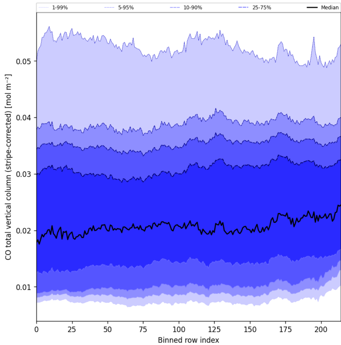
Figure 27: Along track statistics of “CO total vertical column (stripe-corrected)” for 2025-01-08 to 2025-01-10
