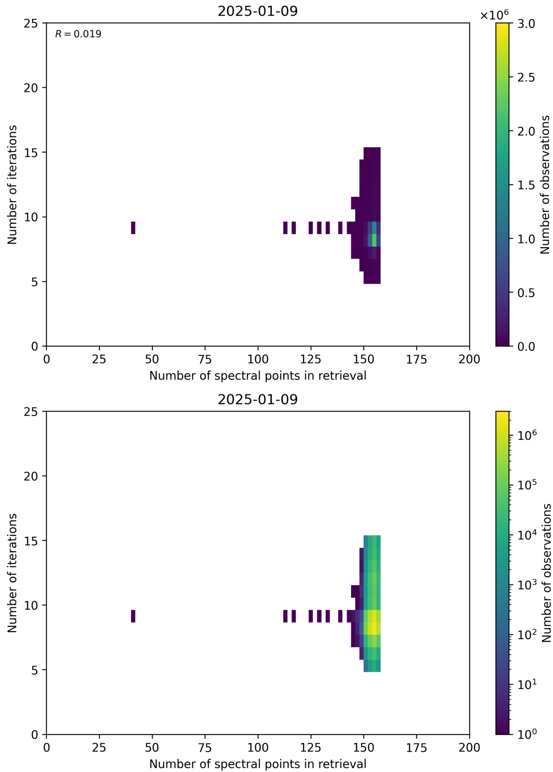
Figure 60: Scatter density plot of “Number of spectral points in retrieval” against “Number of iterations” for 2025-01-08 to 2025-01-10.
