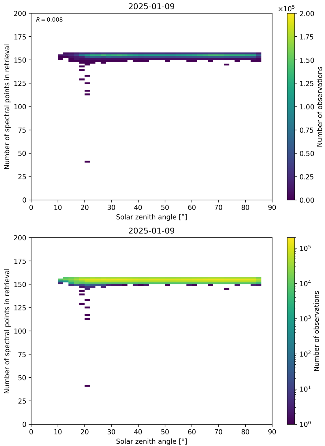
Figure 68: Scatter density plot of “Solar zenith angle” against “Number of spectral points in retrieval” for 2025-01-08 to 2025-01-10.
