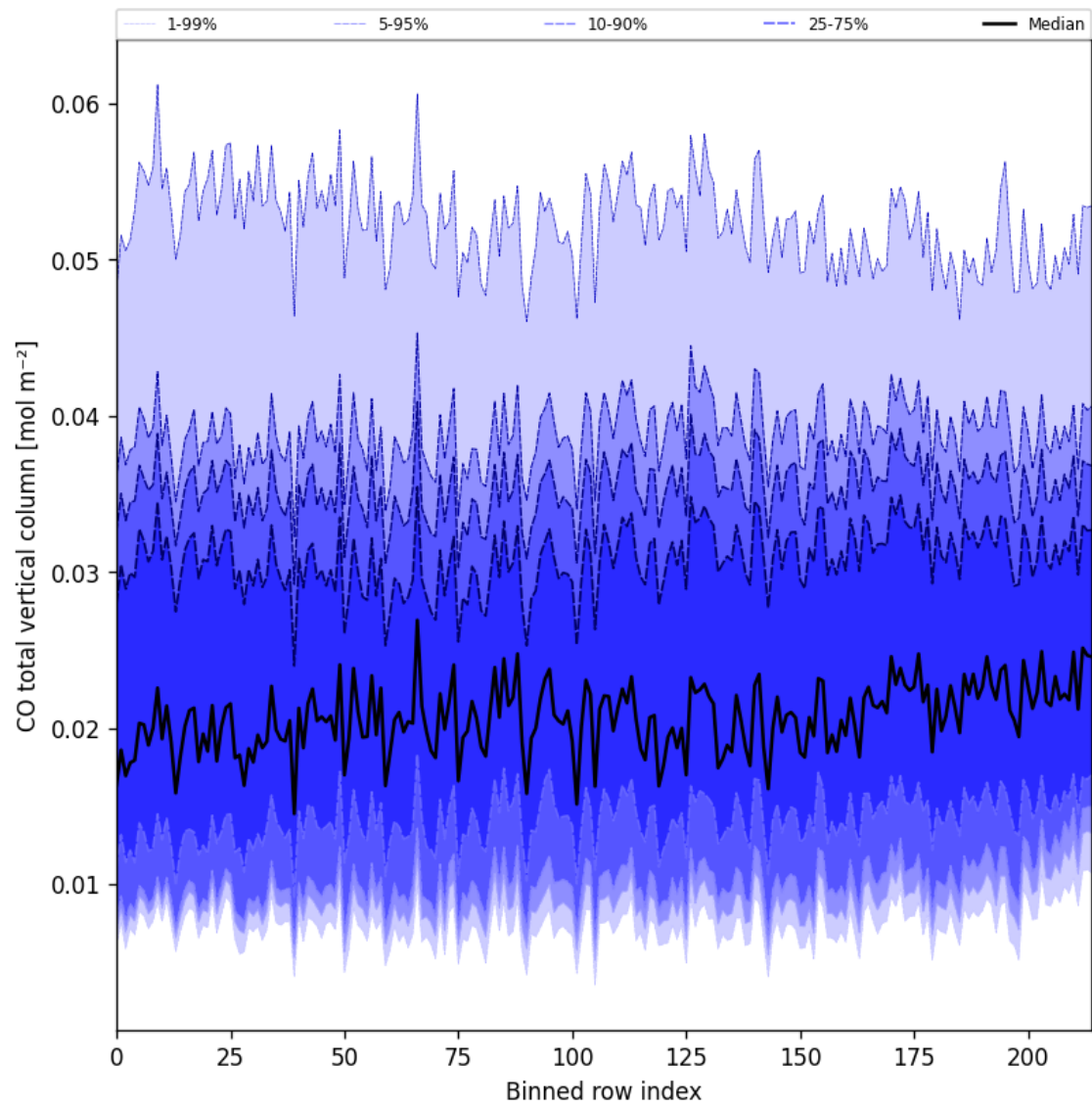
Figure 26: Along track statistics of “CO total vertical column” for 2025-01-08 to 2025-01-10
