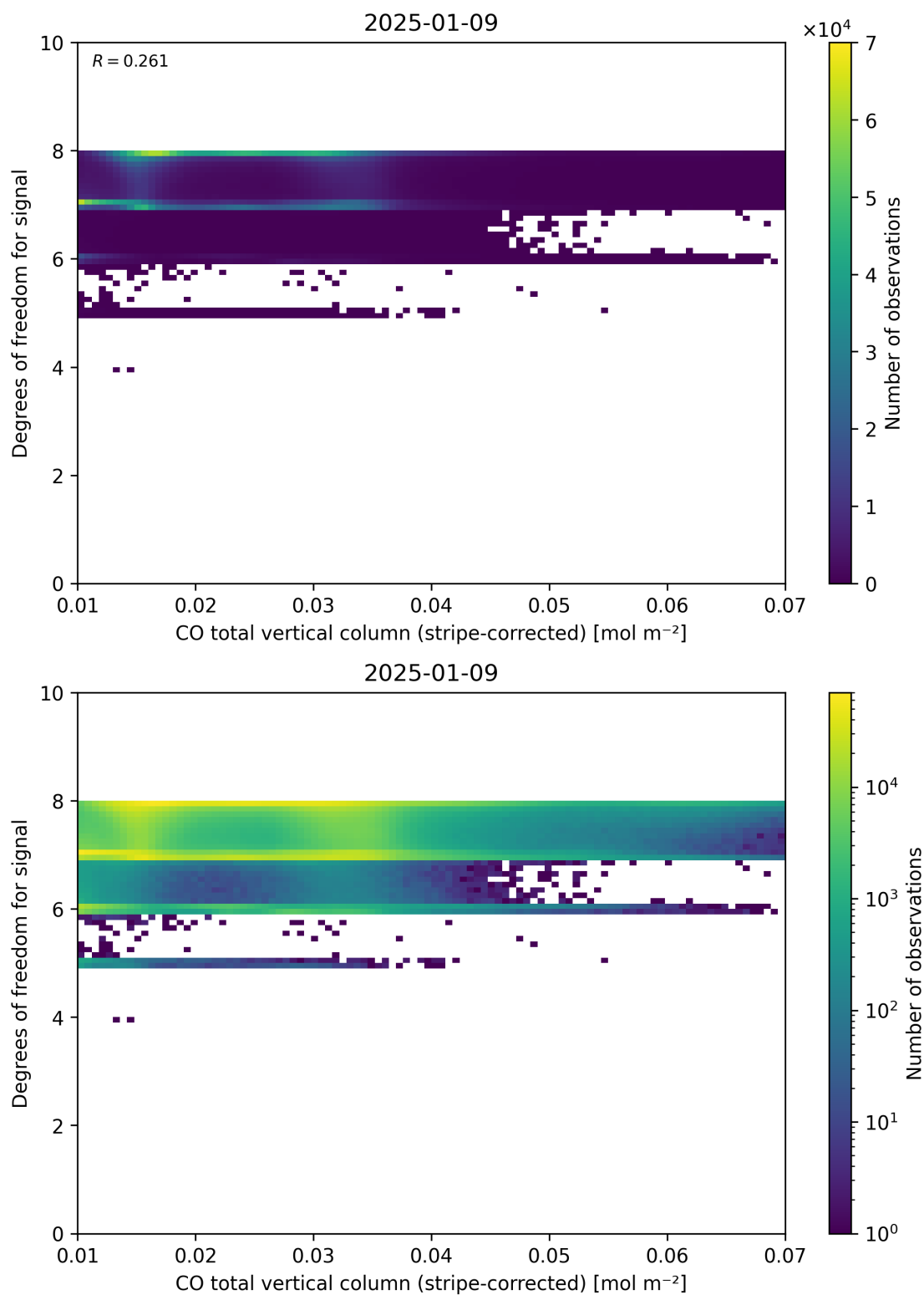
Figure 38: Scatter density plot of “CO total vertical column (stripe-corrected)” against “Degrees of freedom for signal” for 2025-01-08 to 2025-01-10.
