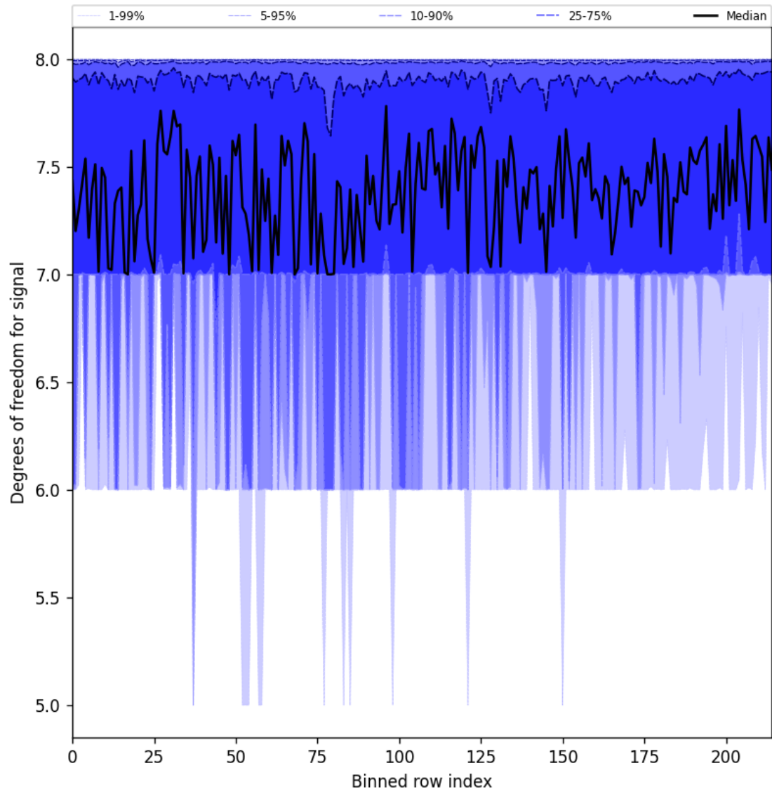
Figure 31: Along track statistics of “Degrees of freedom for signal” for 2025-01-08 to 2025-01-10
