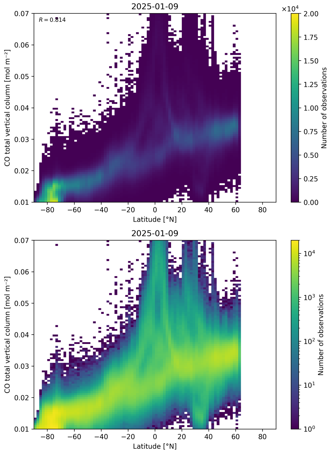
Figure 51: Scatter density plot of “Latitude” against “CO total vertical column” for 2025-01-08 to 2025-01-10.
