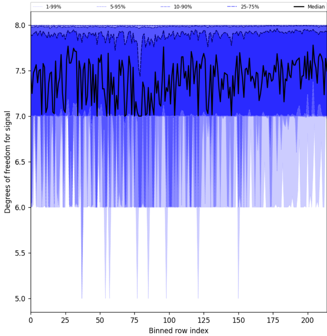
Figure 31: Along track statistics of “Degrees of freedom for signal” for 2025-01-09 to 2025-01-11
