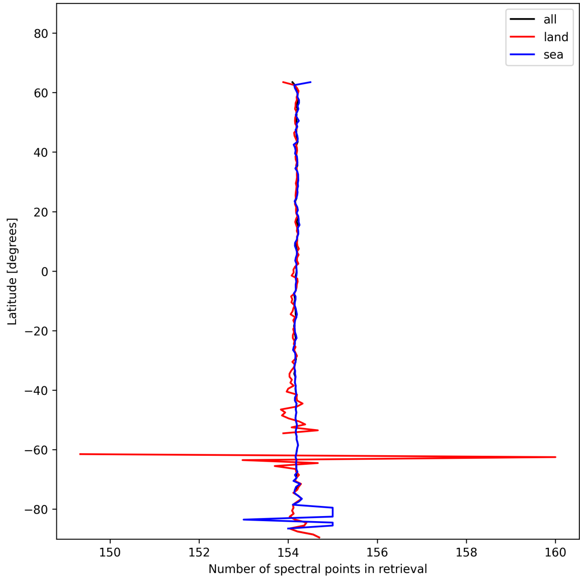
Figure 13: Zonal average of “Number of spectral points in retrieval” for 2025-01-09 to 2025-01-11.
