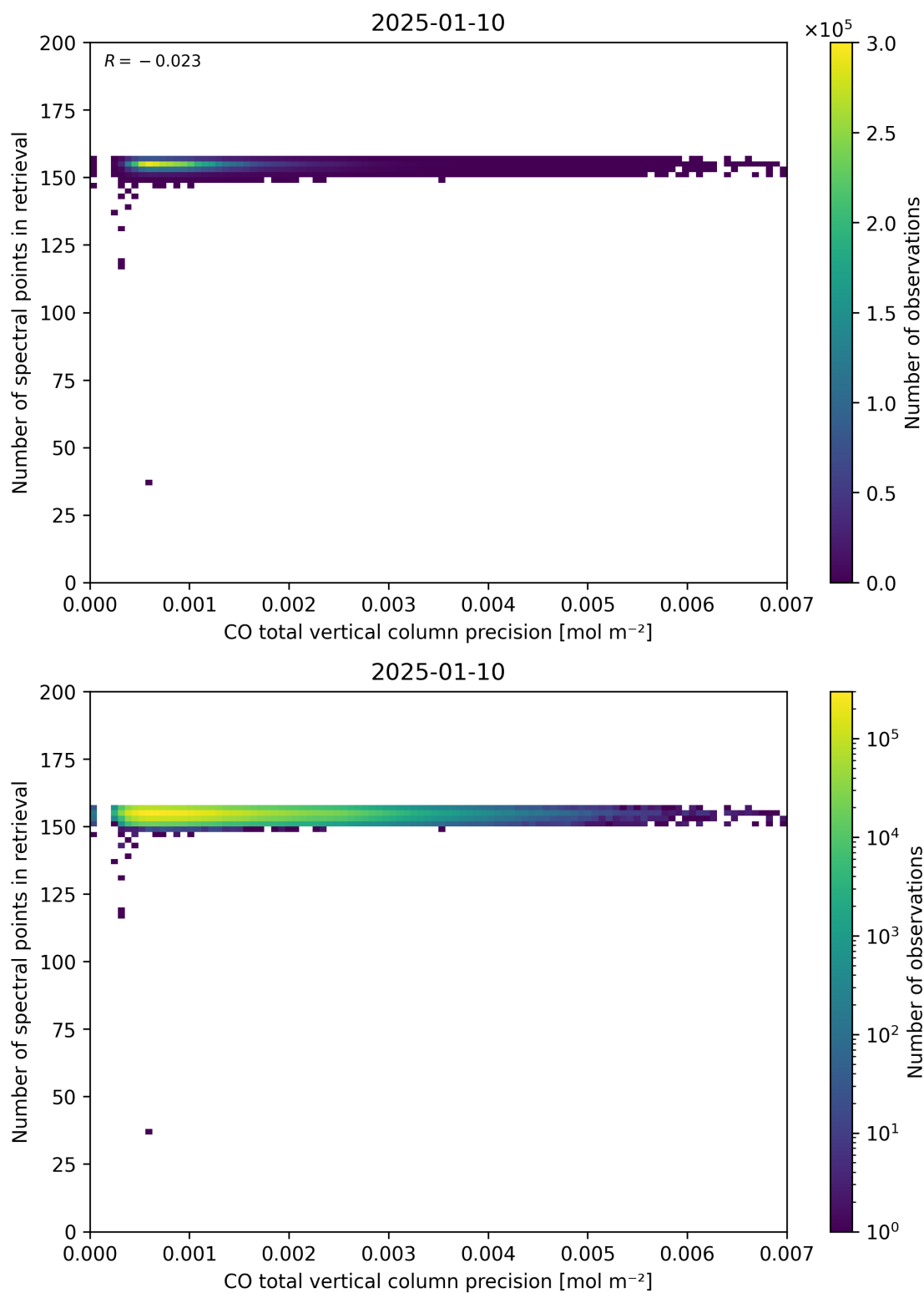
Figure 47: Scatter density plot of “CO total vertical column precision” against “Number of spectral points in retrieval” for 2025-01-09 to 2025-01-11.
