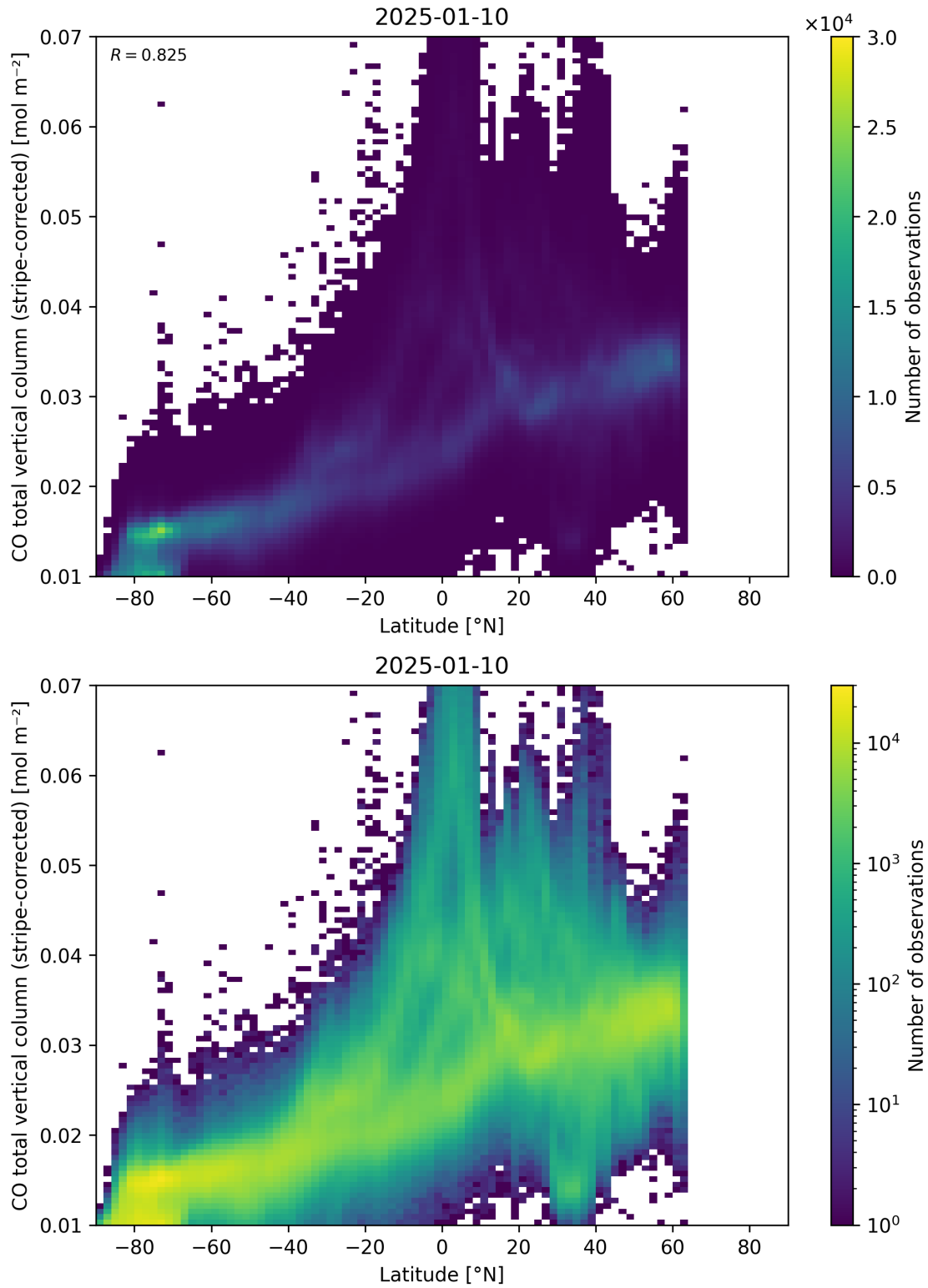
Figure 52: Scatter density plot of “Latitude” against “CO total vertical column (stripe-corrected)” for 2025-01-09 to 2025-01-11.
