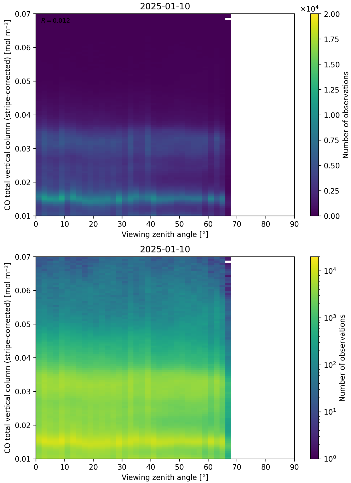
Figure 70: Scatter density plot of “Viewing zenith angle” against “CO total vertical column (stripe-corrected)” for 2025-01-09 to 2025-01-11.
