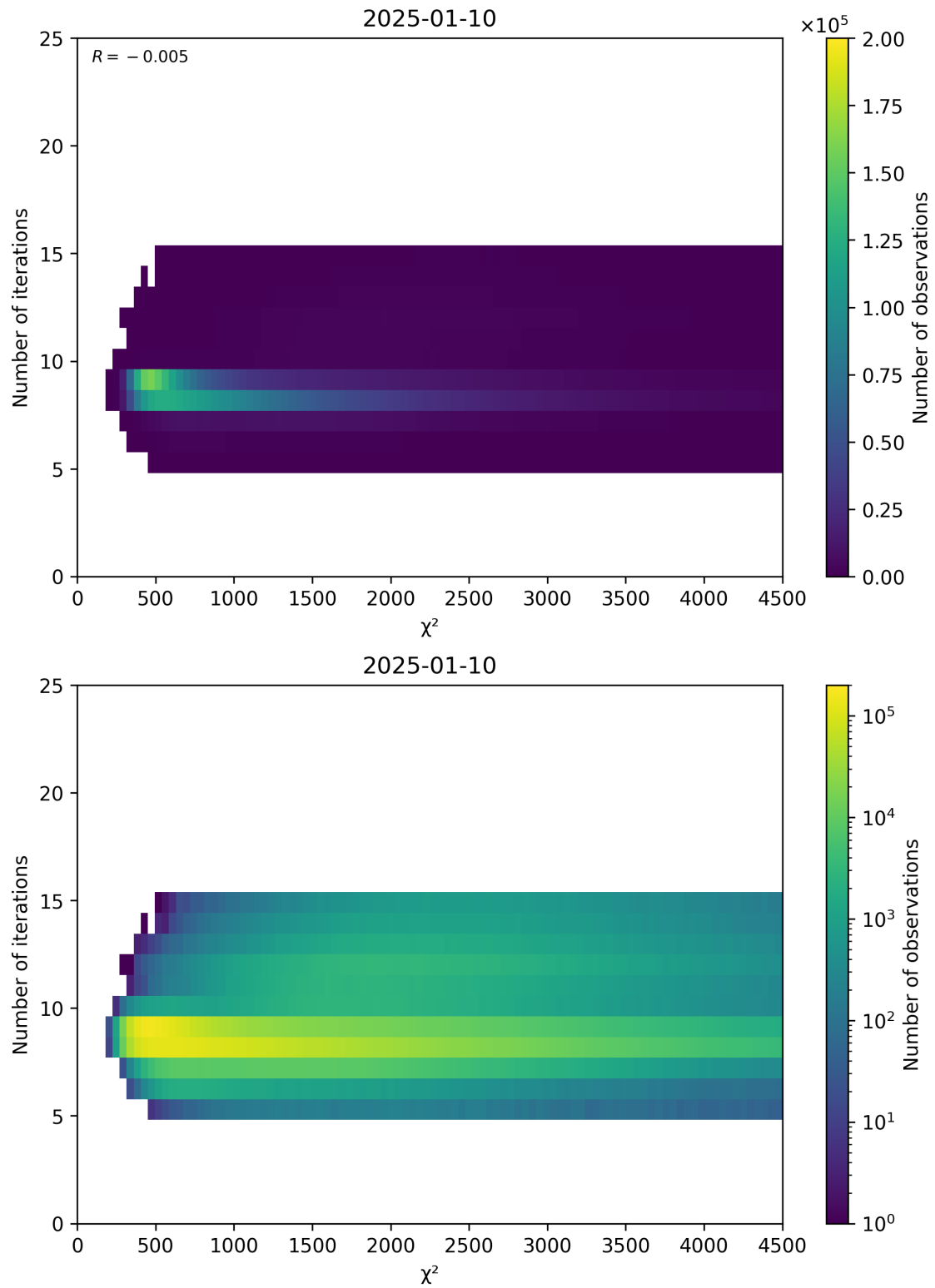
Figure 49: Scatter density plot of “ \chi^2 ” against “Number of iterations” for 2025-01-09 to 2025-01-11.
