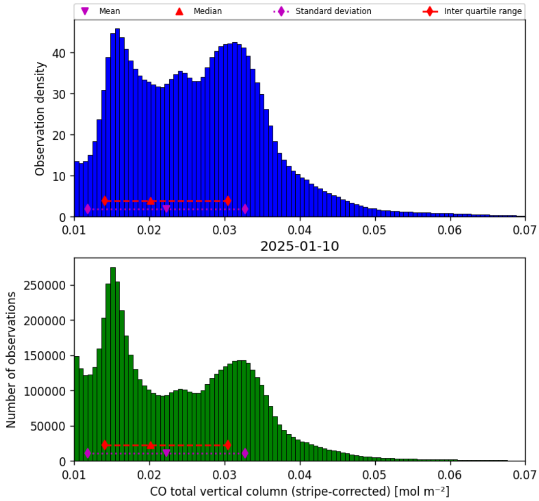
Figure 19: Histogram of “CO total vertical column (stripe-corrected)” for 2025-01-09 to 2025-01-11
