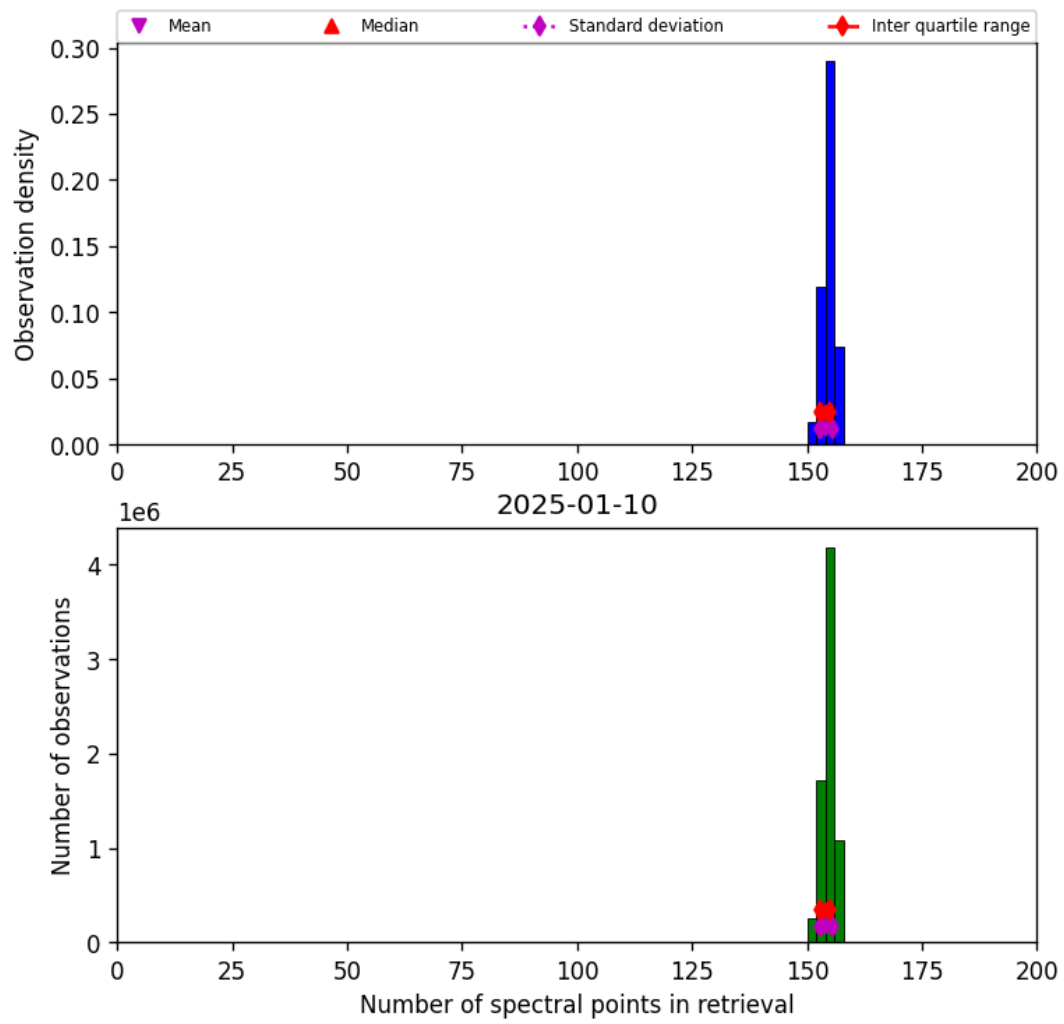
Figure 21: Histogram of “Number of spectral points in retrieval” for 2025-01-09 to 2025-01-11
