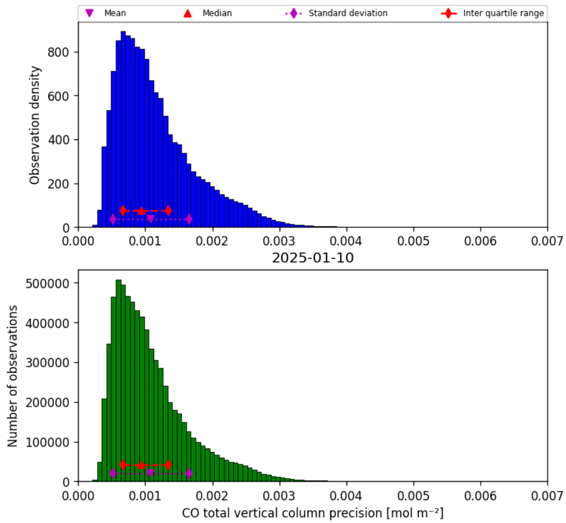
Figure 20: Histogram of “CO total vertical column precision” for 2025-01-09 to 2025-01-11
