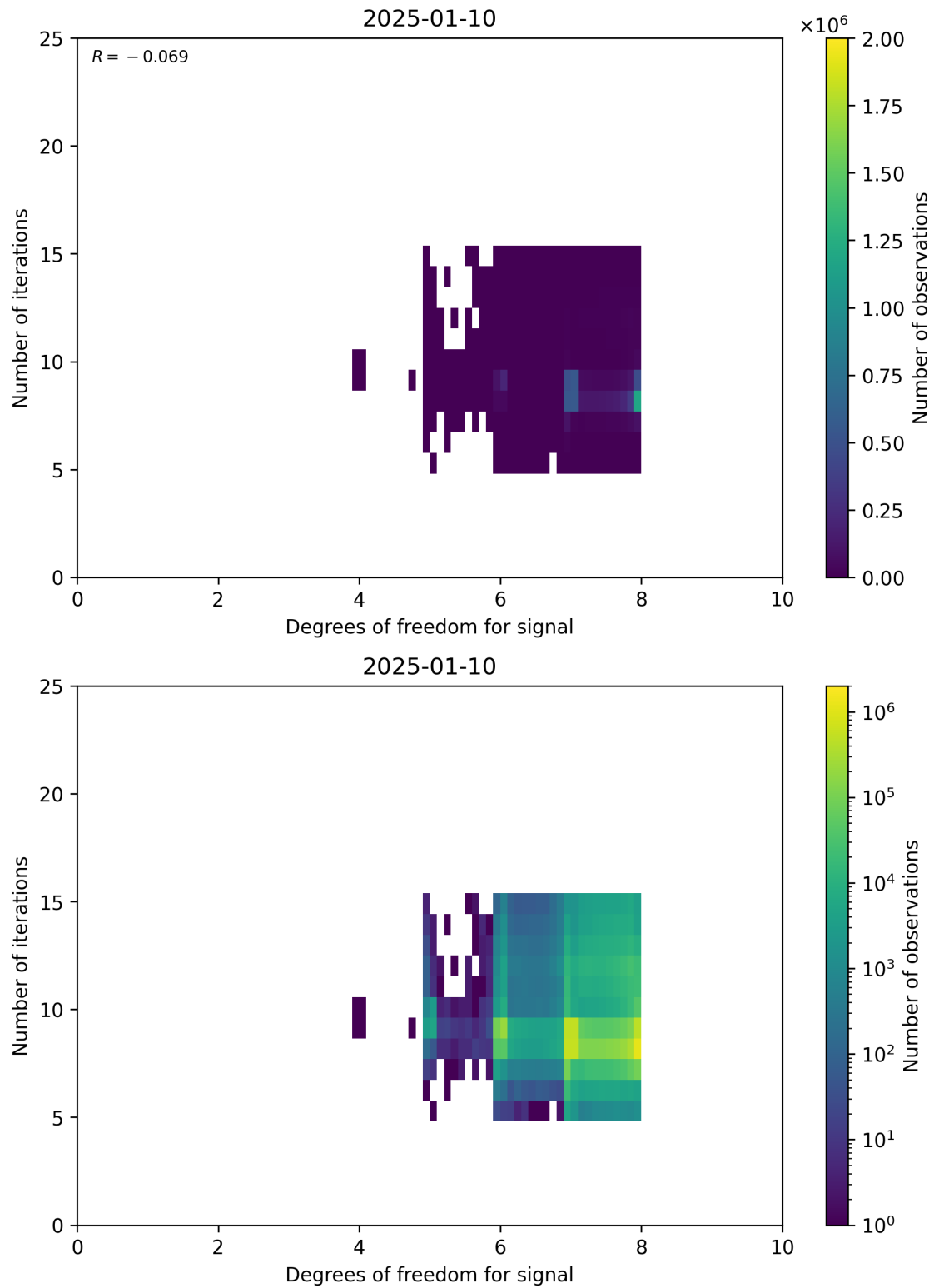
Figure 50: Scatter density plot of “Degrees of freedom for signal” against “Number of iterations” for 2025-01-09 to 2025-01-11.
