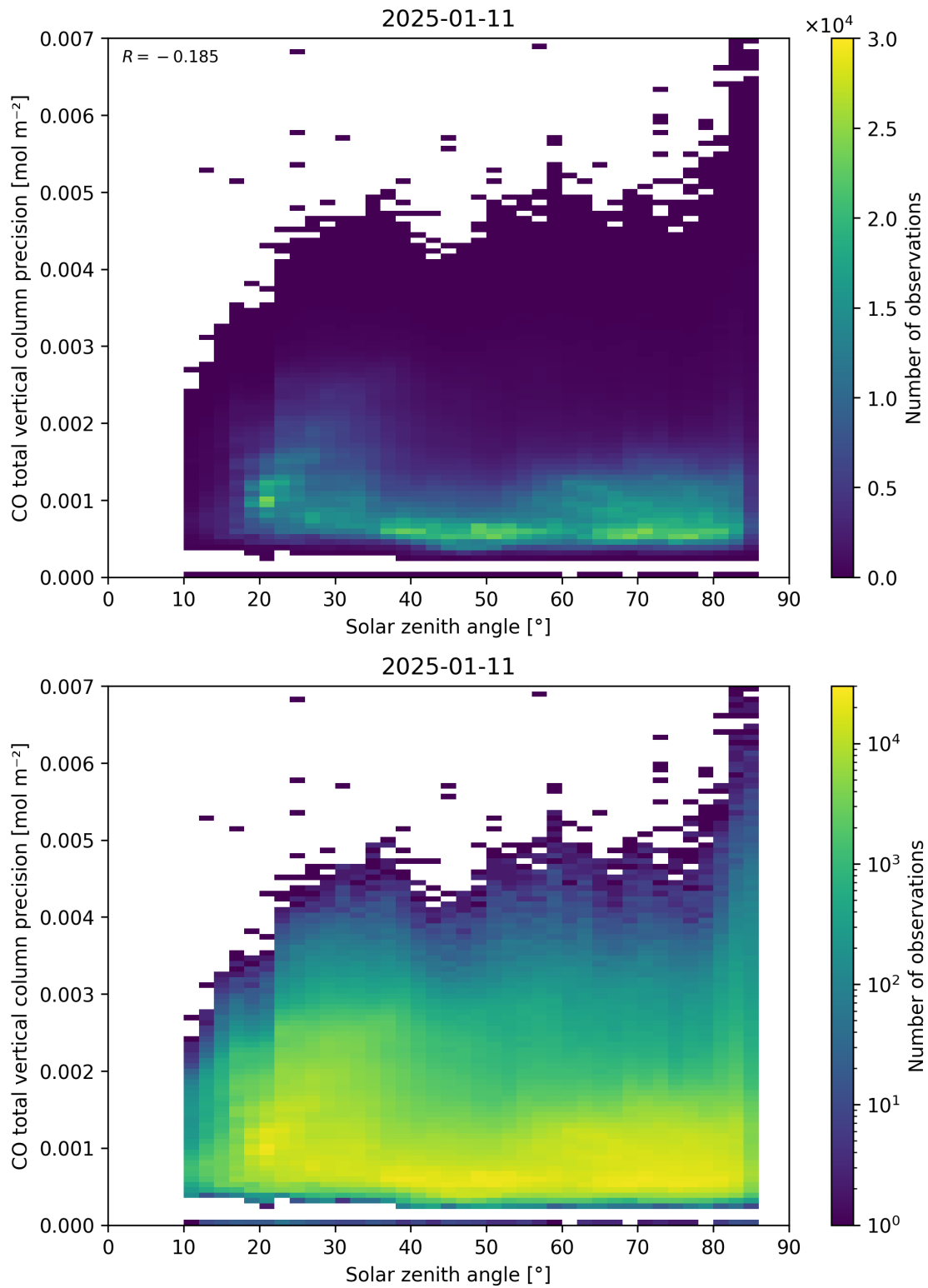
Figure 63: Scatter density plot of “Solar zenith angle” against “CO total vertical column precision” for 2025-01-10 to 2025-01-12.
