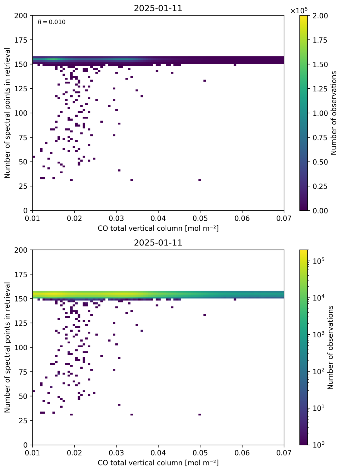
Figure 43: Scatter density plot of “CO total vertical column” against “Number of spectral points in retrieval” for 2025-01-10 to 2025-01-12.
