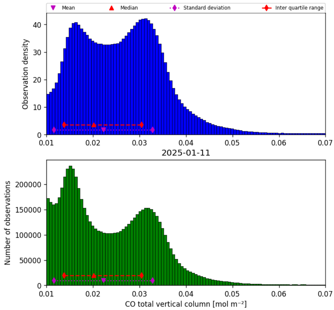
Figure 18: Histogram of “CO total vertical column” for 2025-01-10 to 2025-01-12
