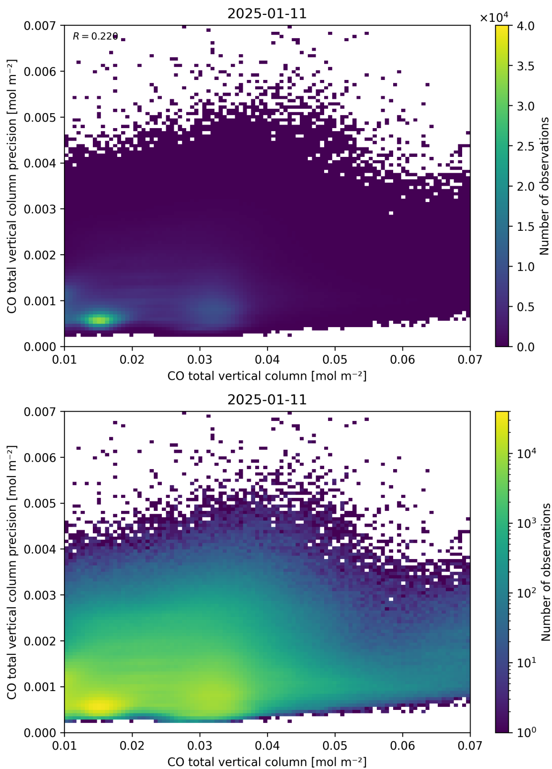
Figure 34: Scatter density plot of “CO total vertical column” against “CO total vertical column precision” for 2025-01-10 to 2025-01-12.
