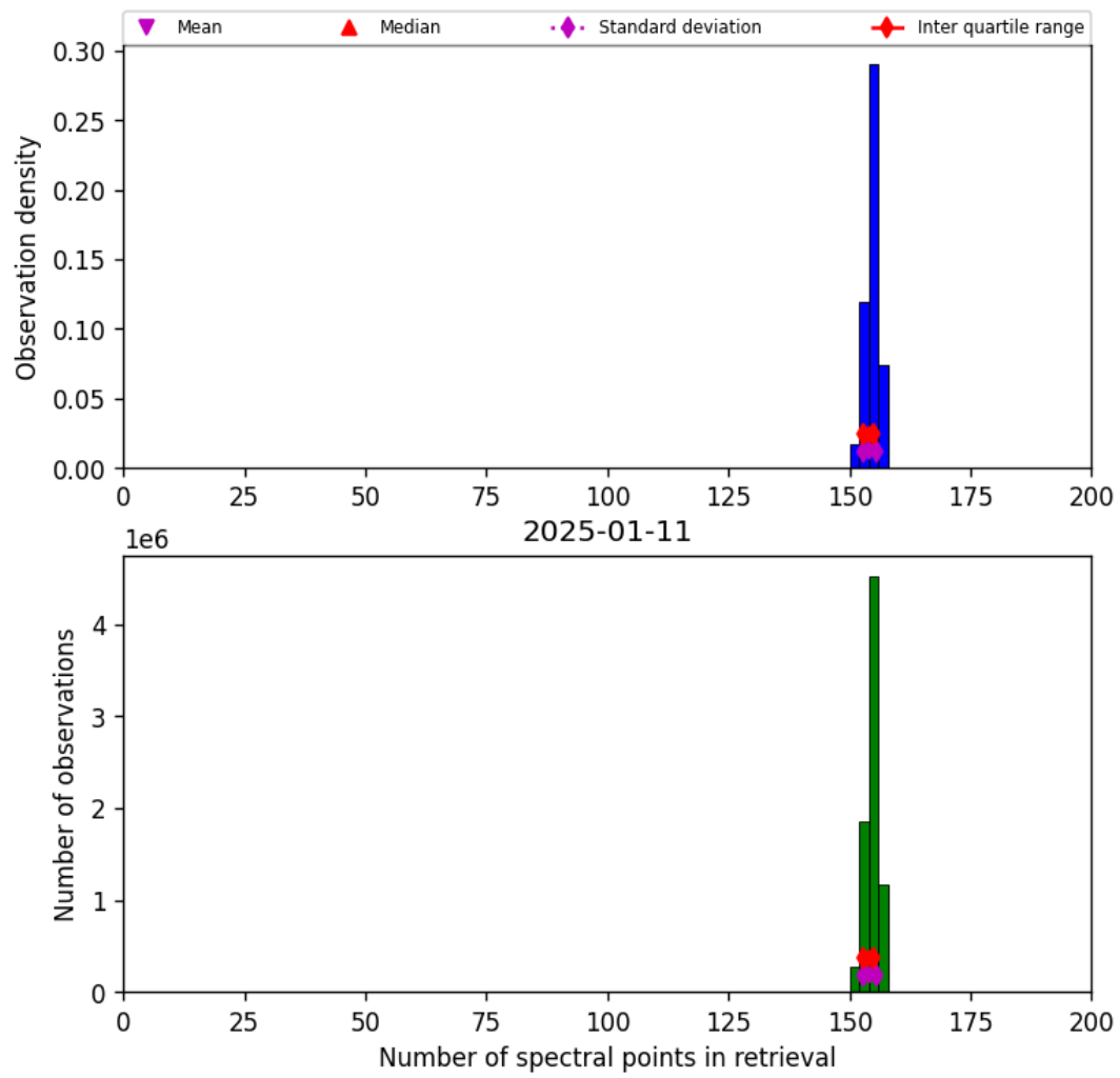
Figure 21: Histogram of “Number of spectral points in retrieval” for 2025-01-10 to 2025-01-12
