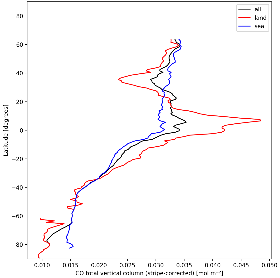
Figure 11: Zonal average of “CO total vertical column (stripe-corrected)” for 2025-01-10 to 2025-01-12.
