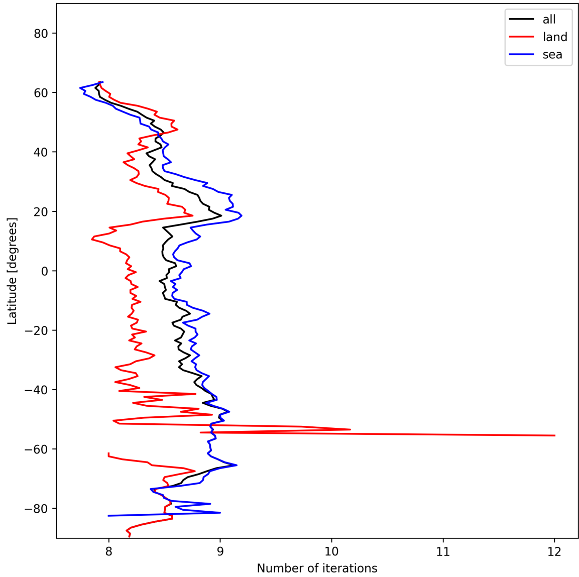
Figure 16: Zonal average of “Number of iterations” for 2025-01-10 to 2025-01-12.
