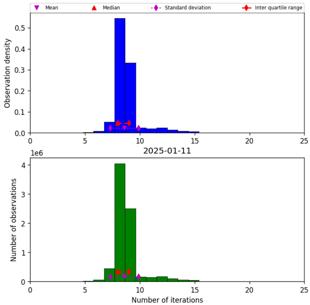
Figure 24: Histogram of “Number of iterations” for 2025-01-10 to 2025-01-12
