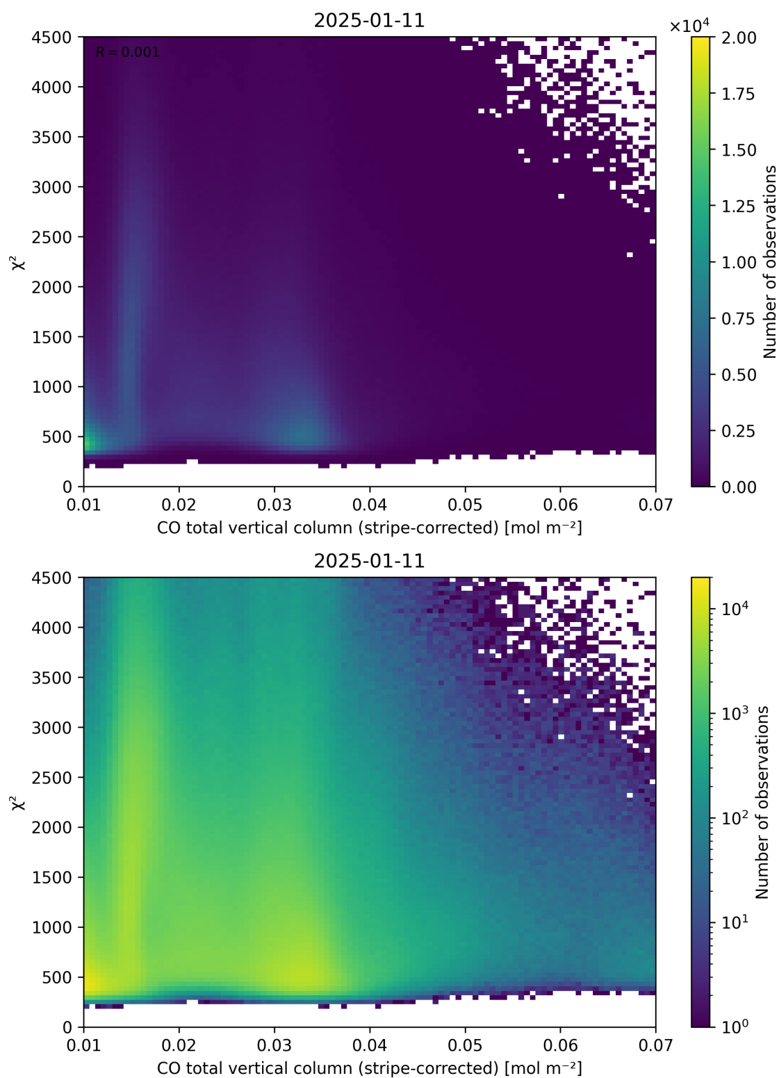
Figure 37: Scatter density plot of “CO total vertical column (stripe-corrected)” against “ \chi^2 ” for 2025-01-10 to 2025-01-12.
