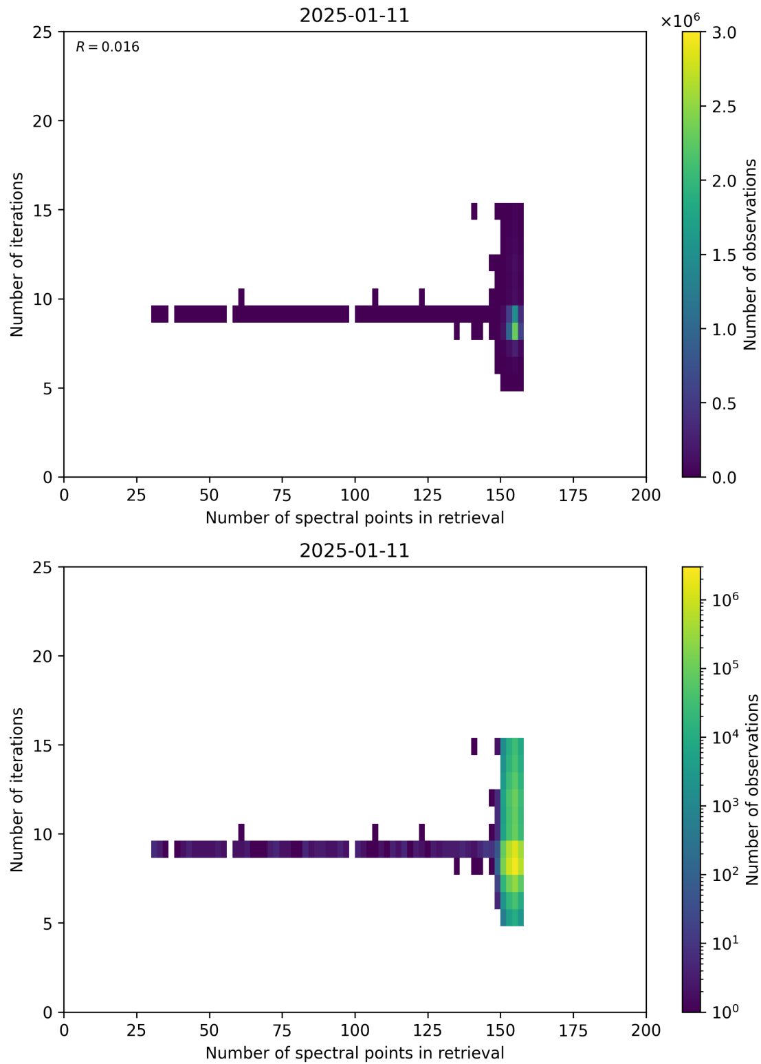
Figure 60: Scatter density plot of “Number of spectral points in retrieval” against “Number of iterations” for 2025-01-10 to 2025-01-12.
