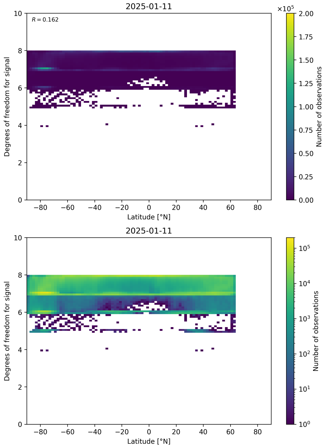
Figure 55: Scatter density plot of “Latitude” against “Degrees of freedom for signal” for 2025-01-10 to 2025-01-12.
