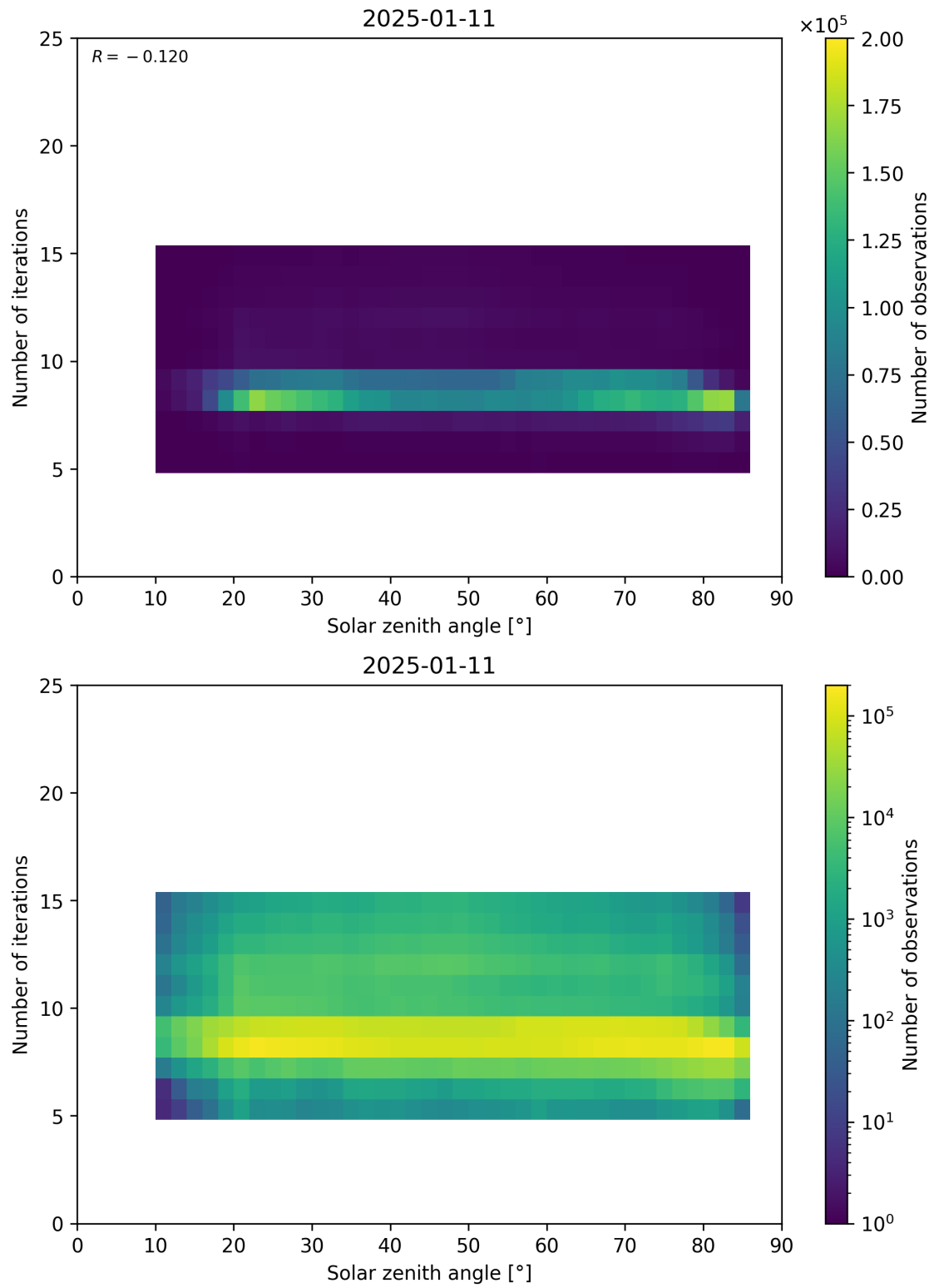
Figure 67: Scatter density plot of “Solar zenith angle” against “Number of iterations” for 2025-01-10 to 2025-01-12.
