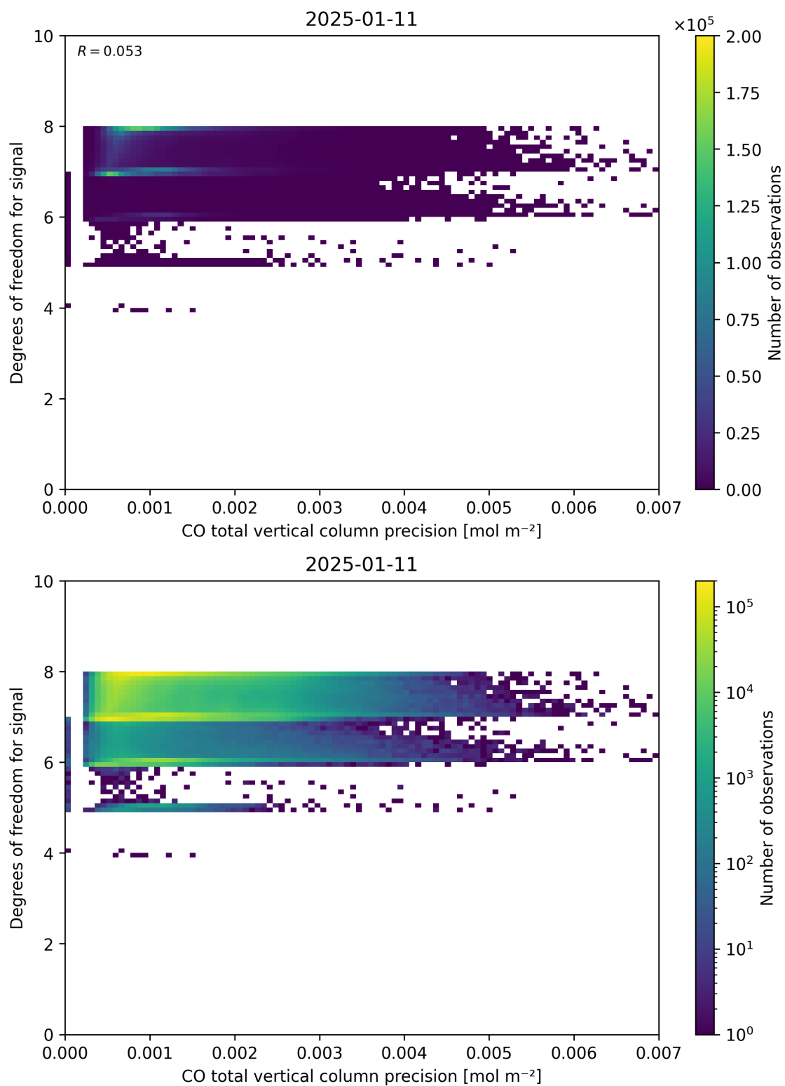
Figure 45: Scatter density plot of “CO total vertical column precision” against “Degrees of freedom for signal” for 2025-01-10 to 2025-01-12.
