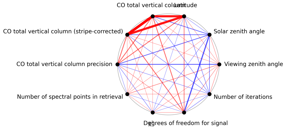
Figure 1: Map of correlation graph for 2025-01-10 to 2025-01-12.
