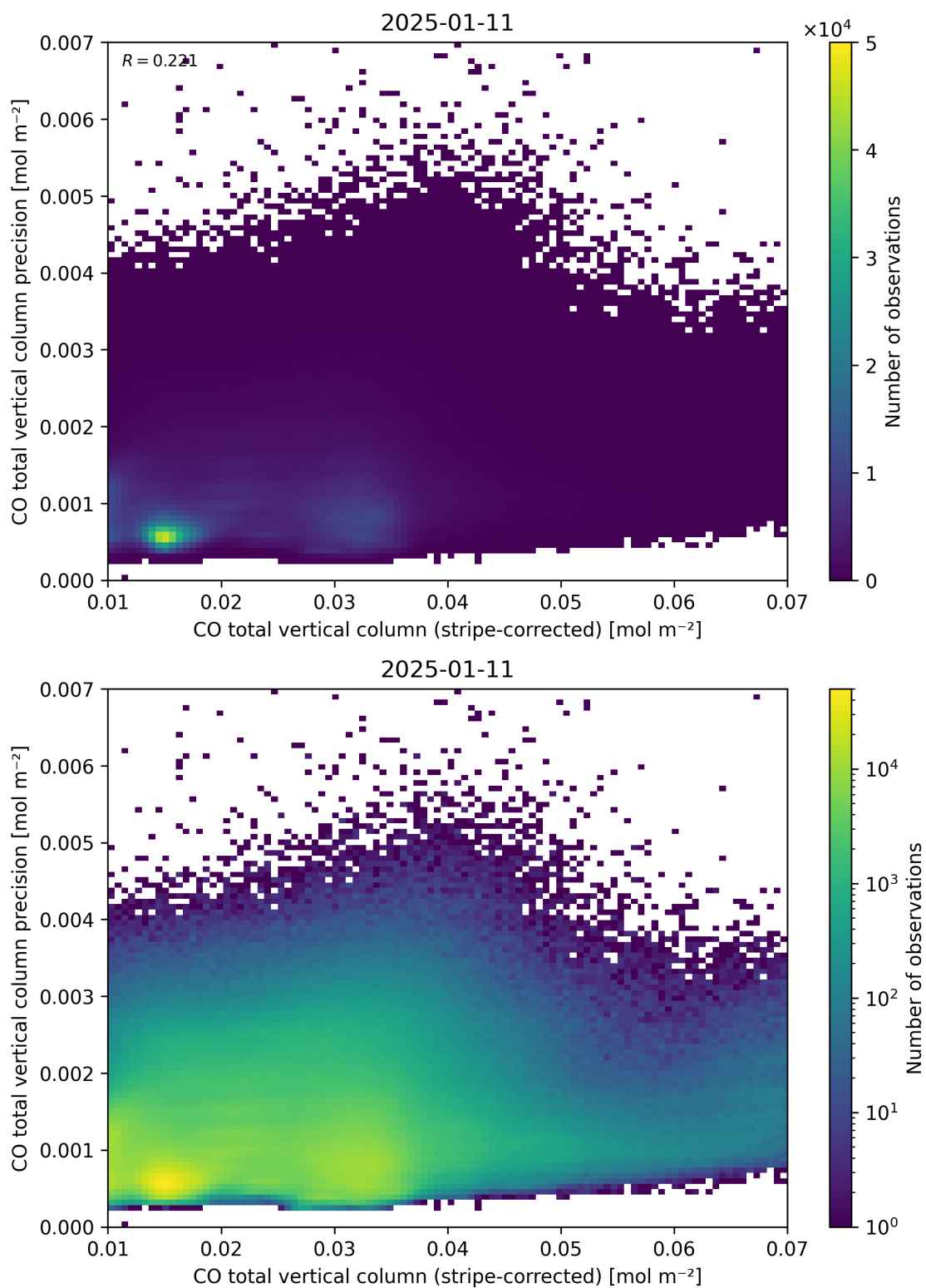
Figure 36: Scatter density plot of “CO total vertical column (stripe-corrected)” against “CO total vertical column precision” for 2025-01-10 to 2025-01-12.
