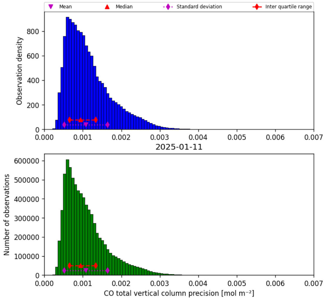
Figure 20: Histogram of “CO total vertical column precision” for 2025-01-10 to 2025-01-12
