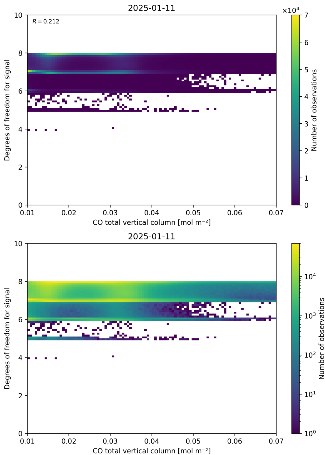
Figure 41: Scatter density plot of “CO total vertical column” against “Degrees of freedom for signal” for 2025-01-10 to 2025-01-12.
