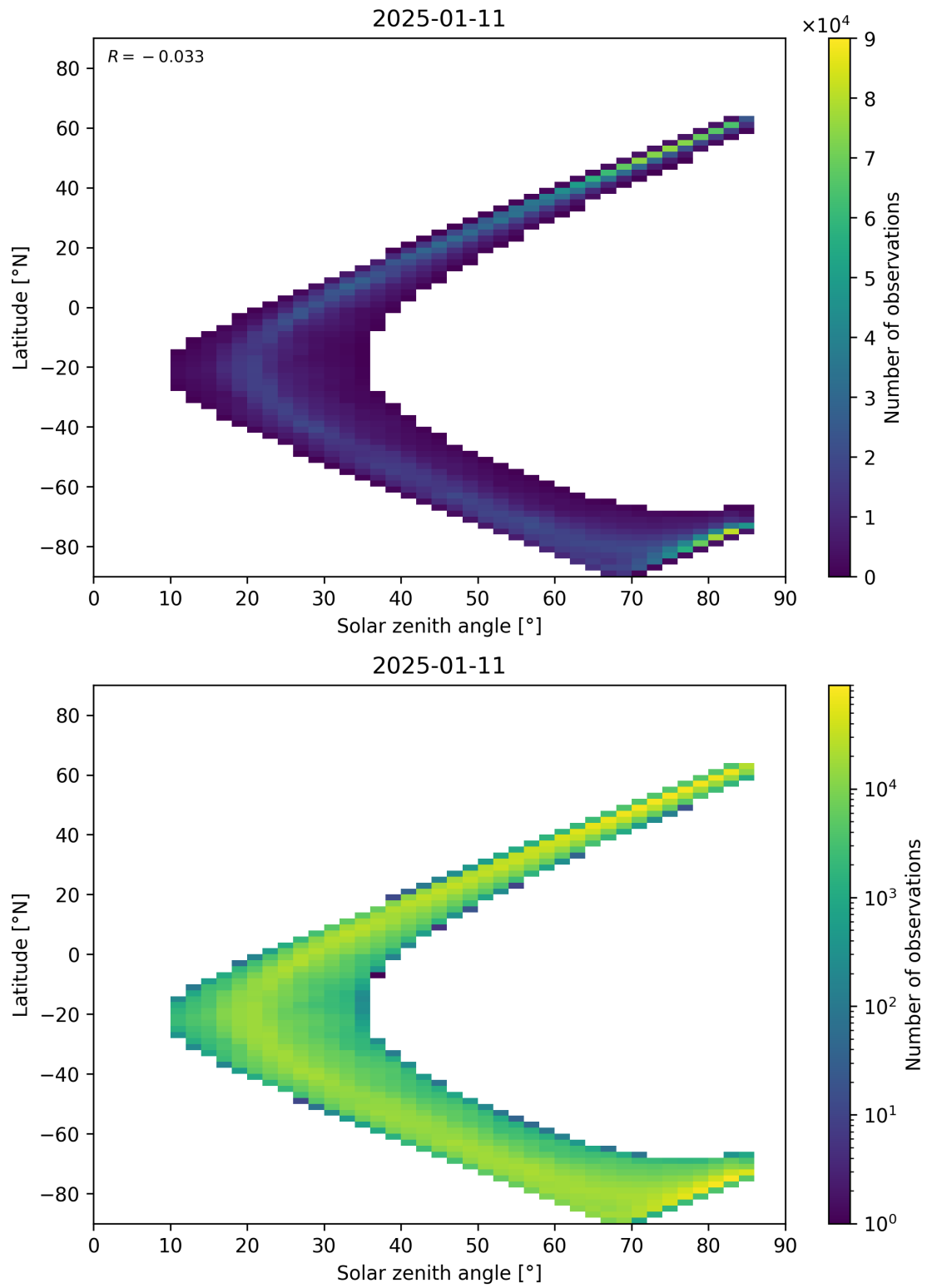
Figure 66: Scatter density plot of “Solar zenith angle” against “Latitude” for 2025-01-10 to 2025-01-12.
