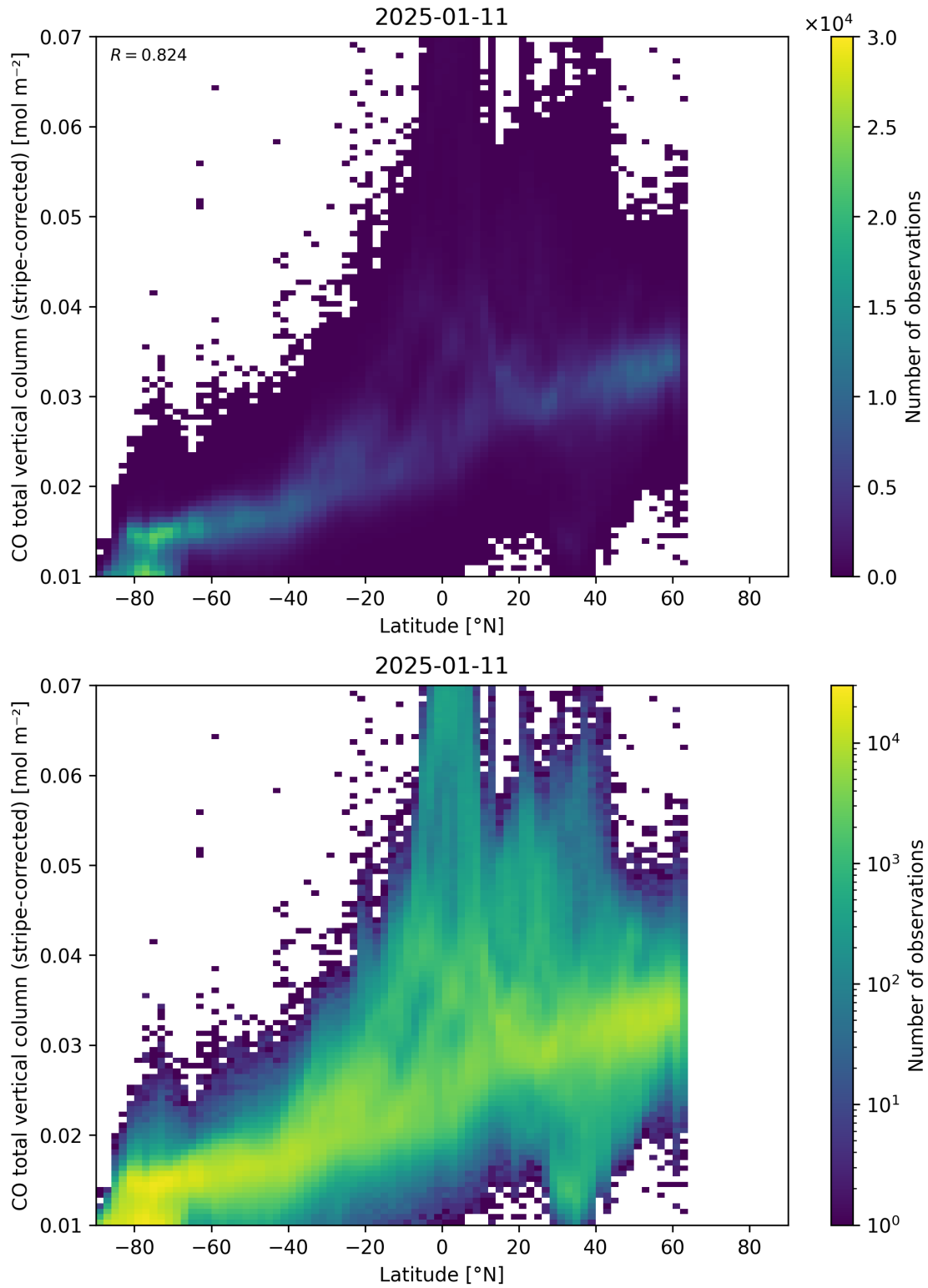
Figure 52: Scatter density plot of “Latitude” against “CO total vertical column (stripe-corrected)” for 2025-01-10 to 2025-01-12.
