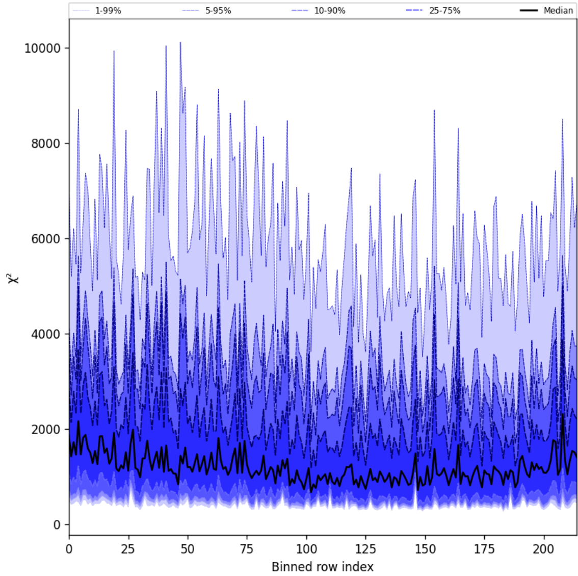
Figure 30: Along track statistics of “ \chi^2 ” for 2025-01-10 to 2025-01-12
