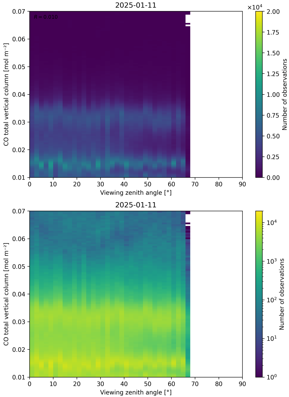
Figure 69: Scatter density plot of “Viewing zenith angle” against “CO total vertical column” for 2025-01-10 to 2025-01-12.
