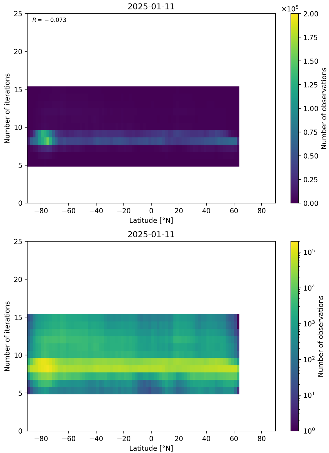
Figure 56: Scatter density plot of “Latitude” against “Number of iterations” for 2025-01-10 to 2025-01-12.
