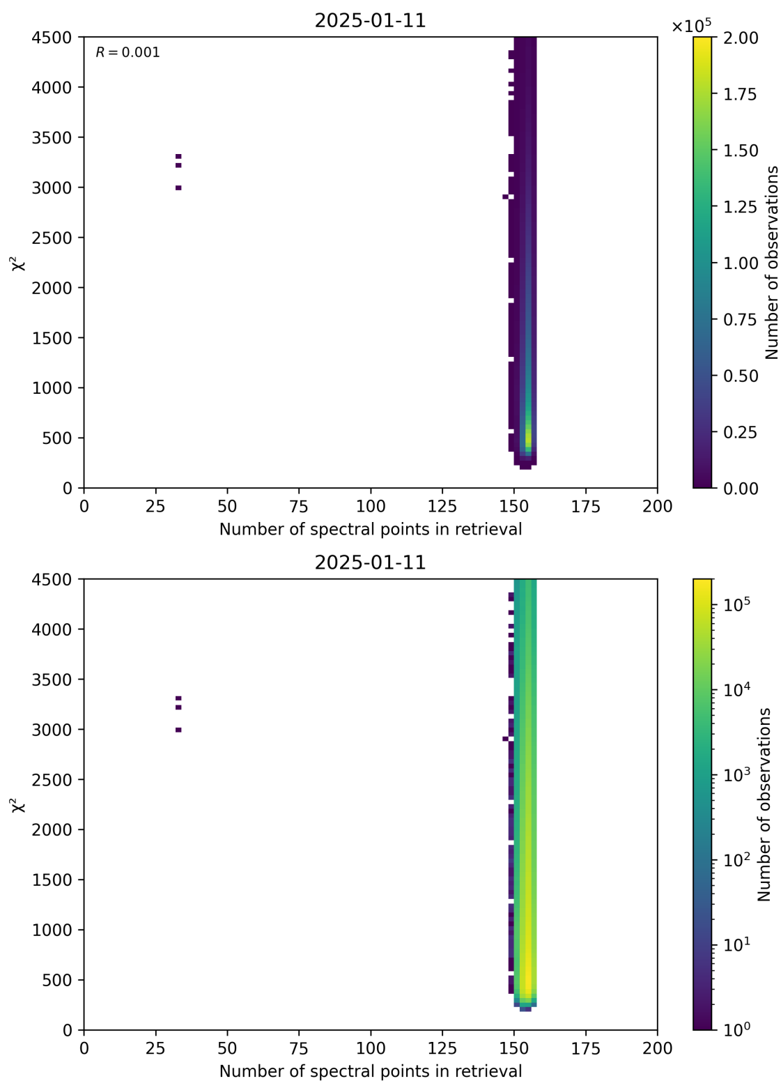
Figure 58: Scatter density plot of “Number of spectral points in retrieval” against “ \chi^2 ” for 2025-01-10 to 2025-01-12.
