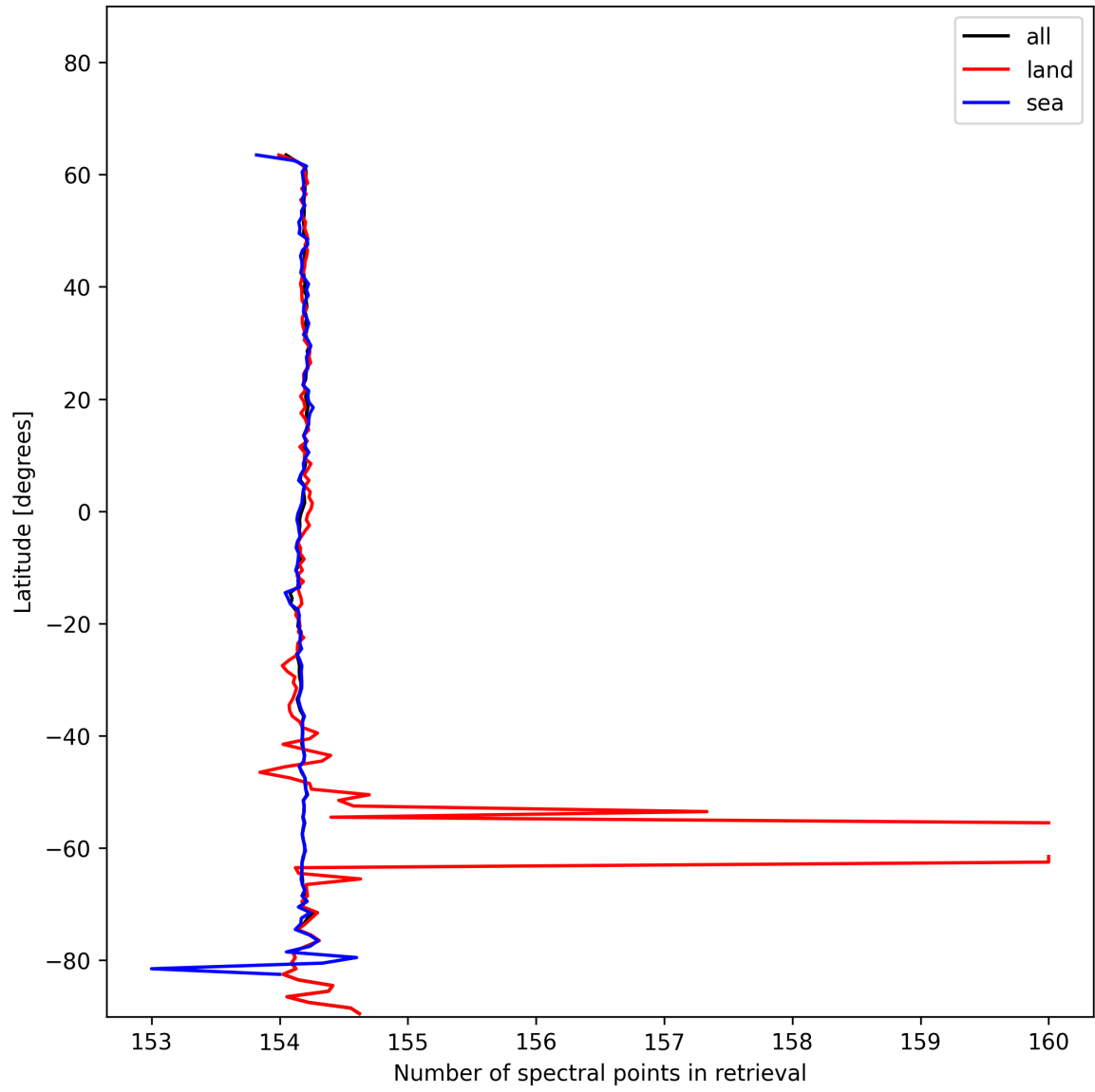
Figure 13: Zonal average of “Number of spectral points in retrieval” for 2025-01-10 to 2025-01-12.
