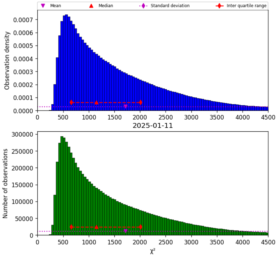
Figure 22: Histogram of “ \chi^2 ” for 2025-01-10 to 2025-01-12
