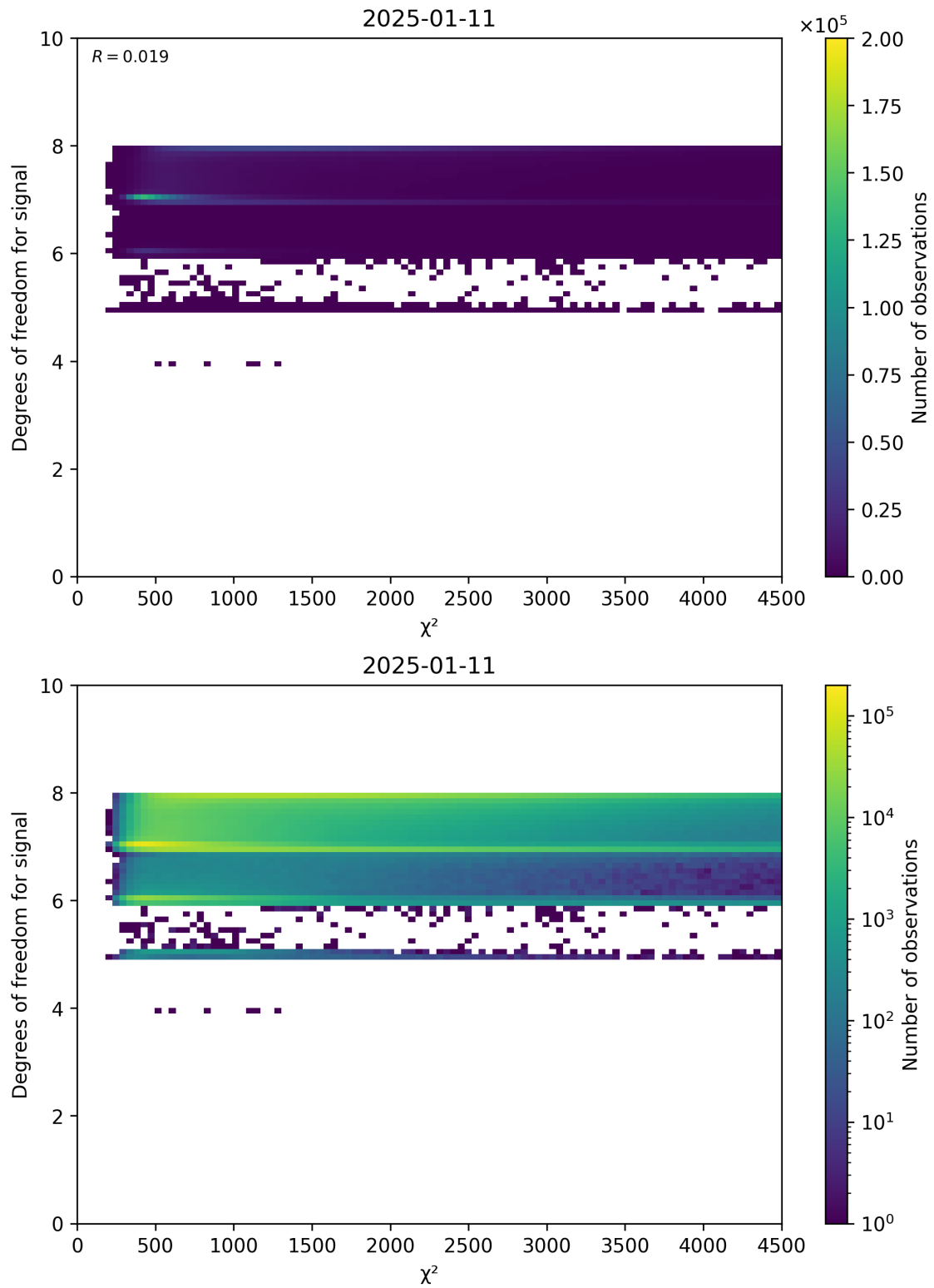
Figure 48: Scatter density plot of “ \chi^2 ” against “Degrees of freedom for signal” for 2025-01-10 to 2025-01-12.
