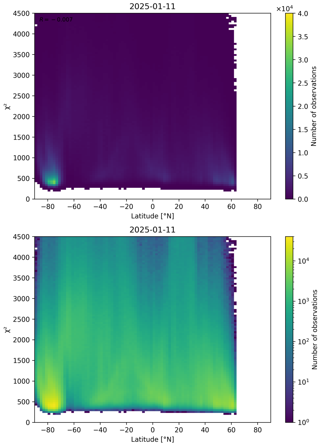
Figure 54: Scatter density plot of “Latitude” against “ \chi^2 ” for 2025-01-10 to 2025-01-12.
