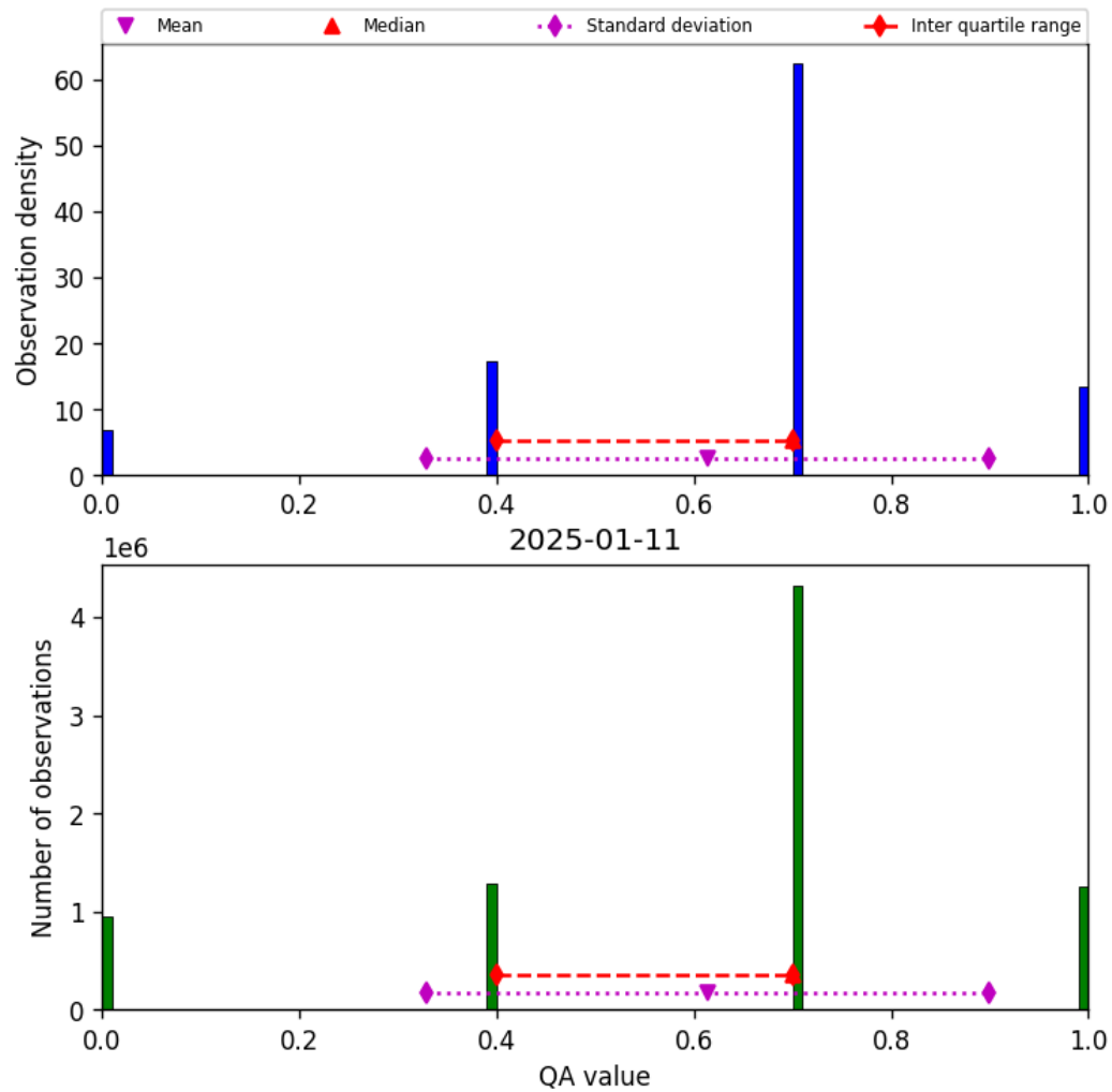
Figure 17: Histogram of “QA value” for 2025-01-10 to 2025-01-12
