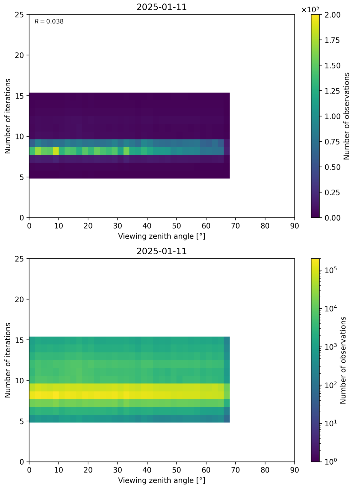
Figure 75: Scatter density plot of “Viewing zenith angle” against “Number of iterations” for 2025-01-10 to 2025-01-12.
