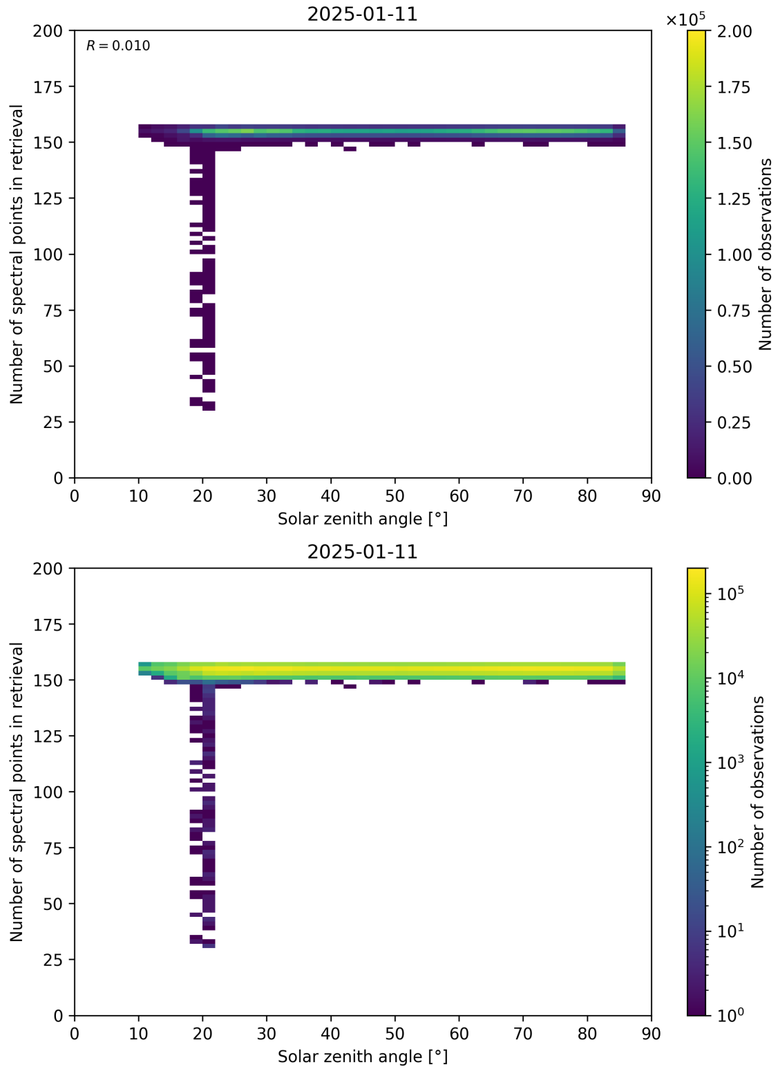
Figure 68: Scatter density plot of “Solar zenith angle” against “Number of spectral points in retrieval” for 2025-01-10 to 2025-01-12.
