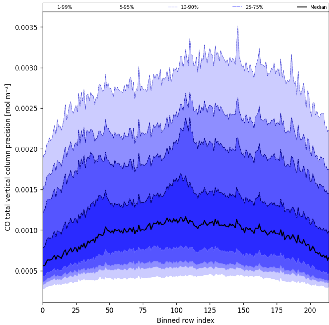
Figure 28: Along track statistics of “CO total vertical column precision” for 2025-01-10 to 2025-01-12
