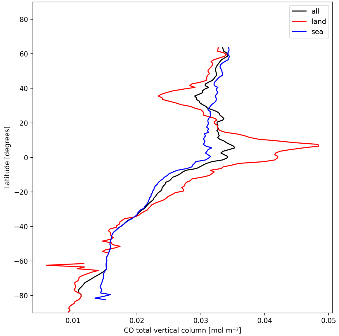
Figure 10: Zonal average of “CO total vertical column” for 2025-01-10 to 2025-01-12.
