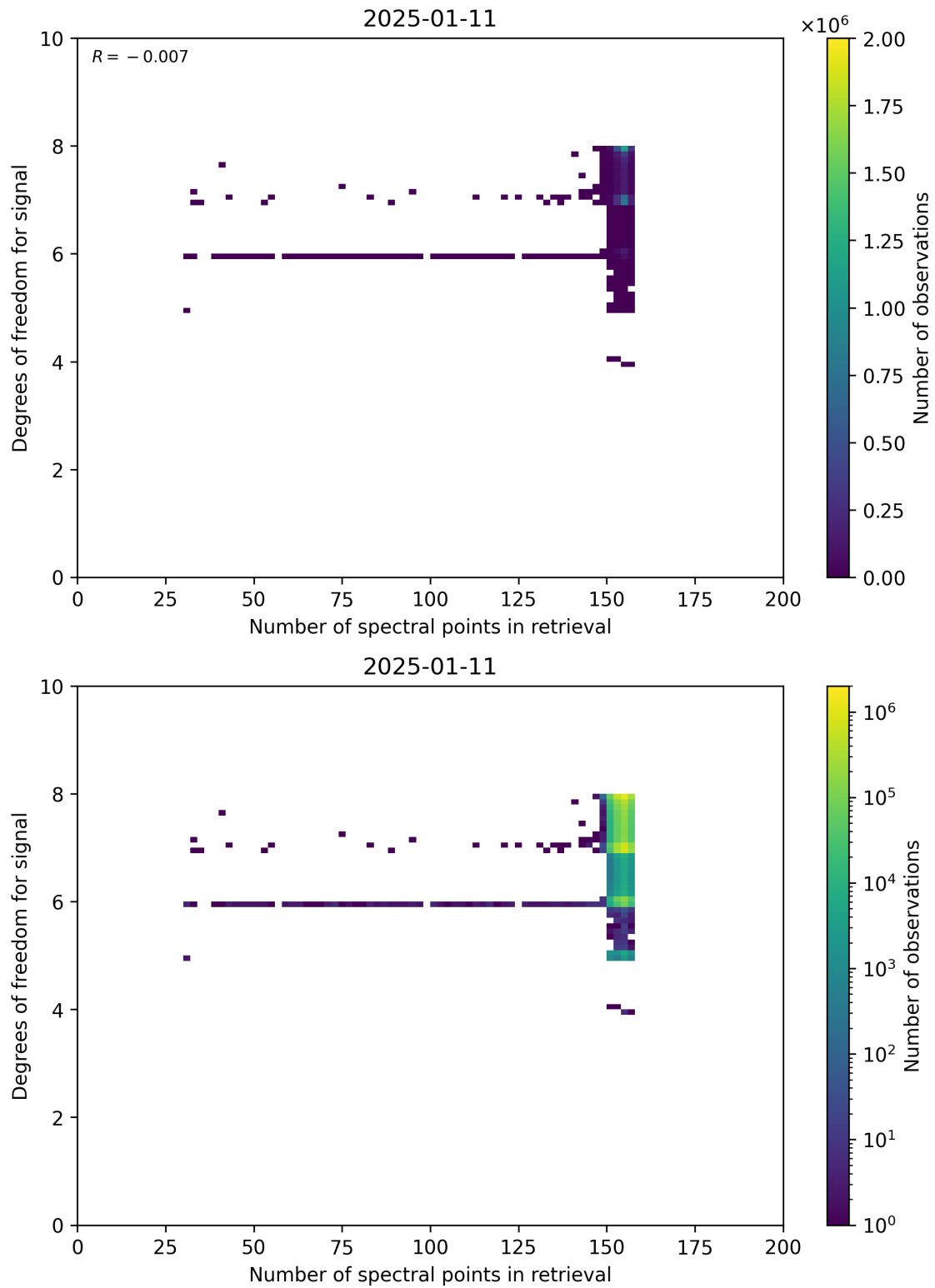
Figure 59: Scatter density plot of “Number of spectral points in retrieval” against “Degrees of freedom for signal” for 2025-01-10 to 2025-01-12.
