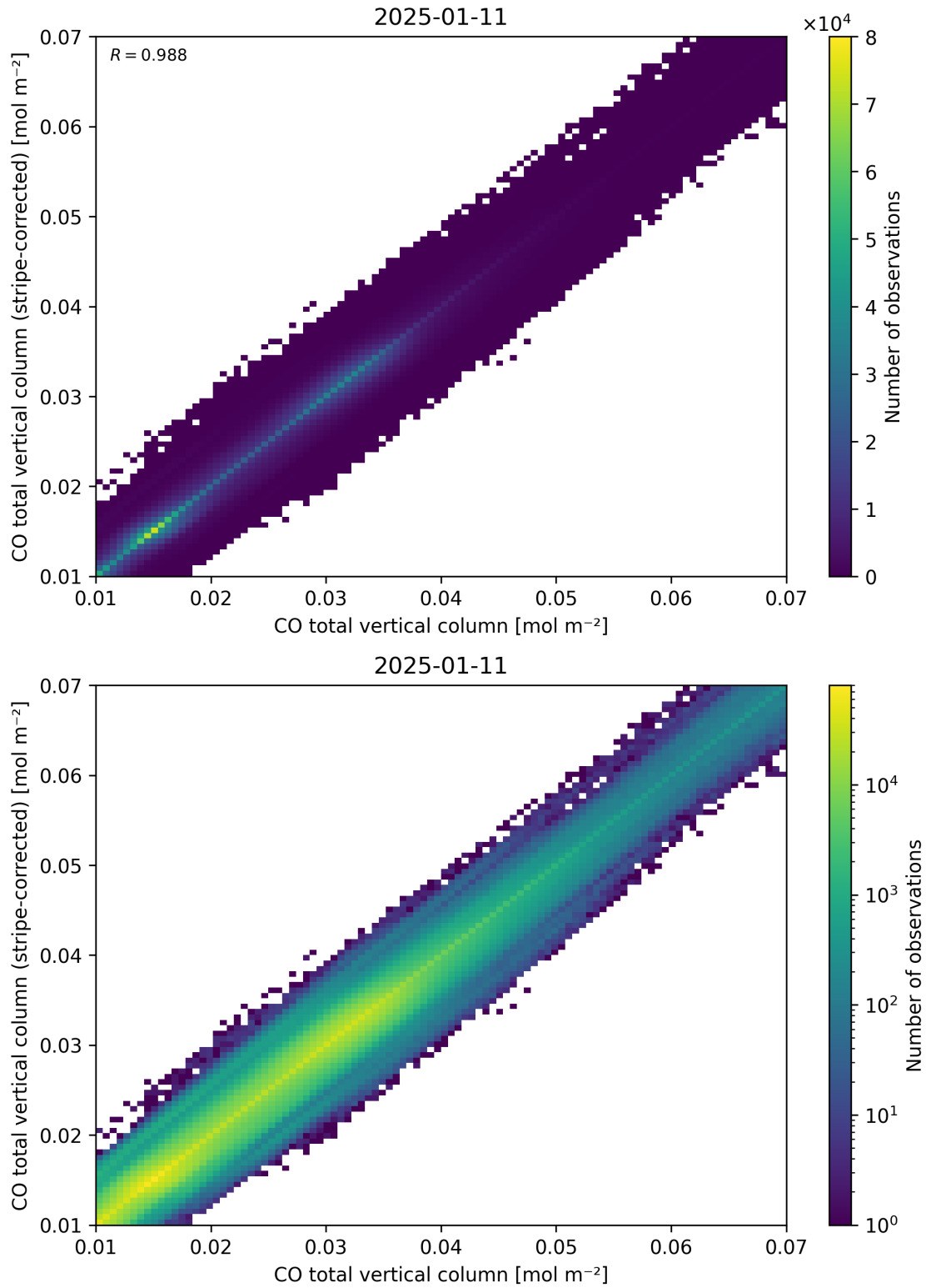
Figure 33: Scatter density plot of “CO total vertical column” against “CO total vertical column (stripe-corrected)” for 2025-01-10 to 2025-01-12.
