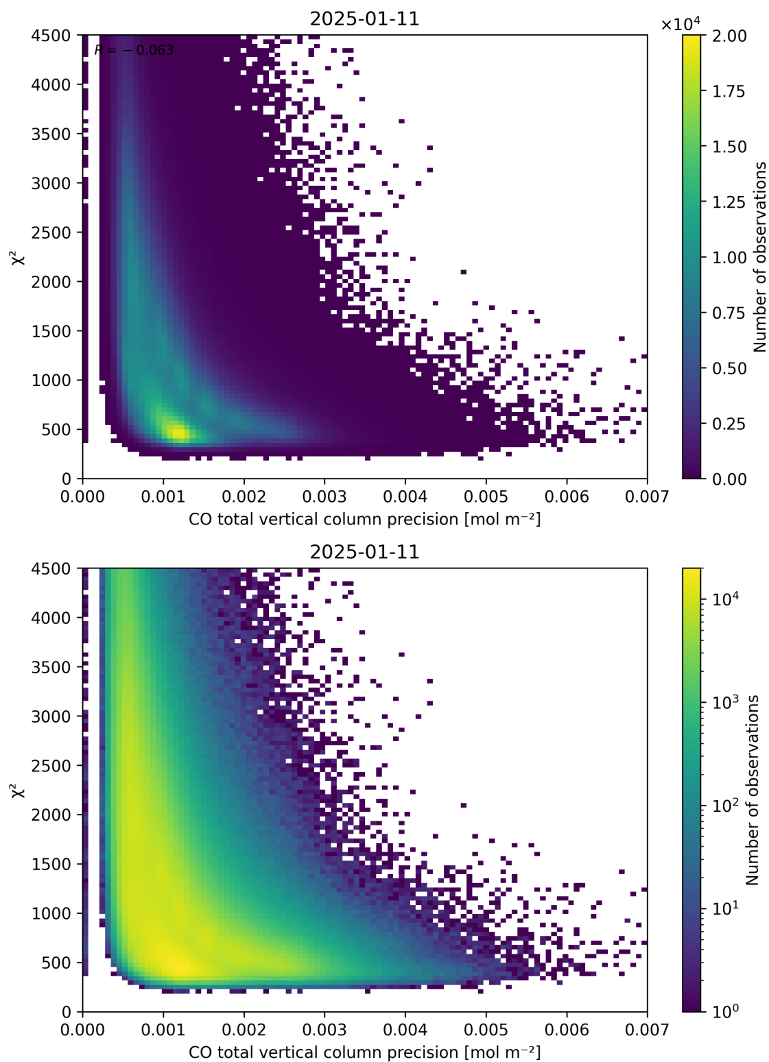
Figure 44: Scatter density plot of “CO total vertical column precision” against “ \chi^2 ” for 2025-01-10 to 2025-01-12.
