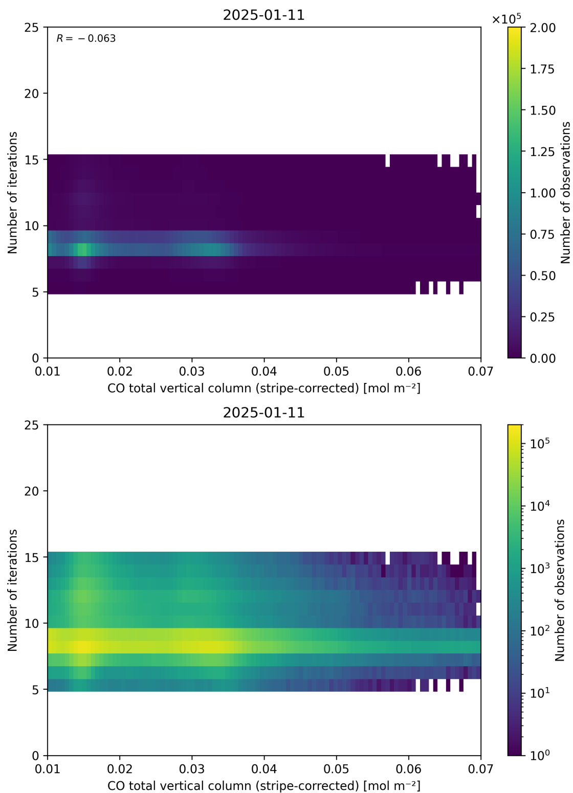
Figure 39: Scatter density plot of “CO total vertical column (stripe-corrected)” against “Number of iterations” for 2025-01-10 to 2025-01-12.
