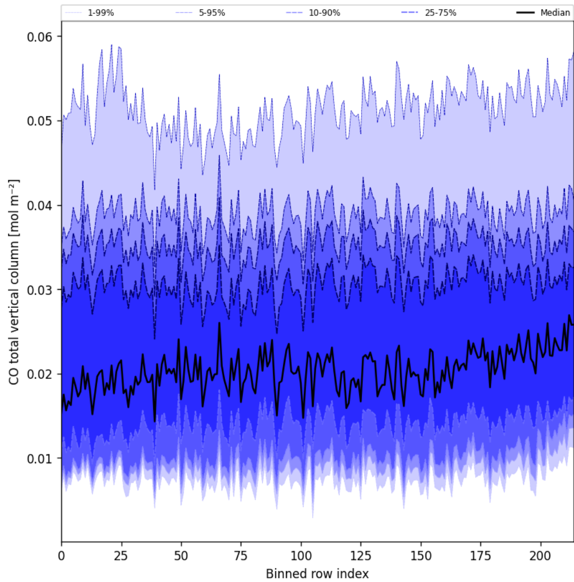
Figure 26: Along track statistics of “CO total vertical column” for 2025-01-10 to 2025-01-12
