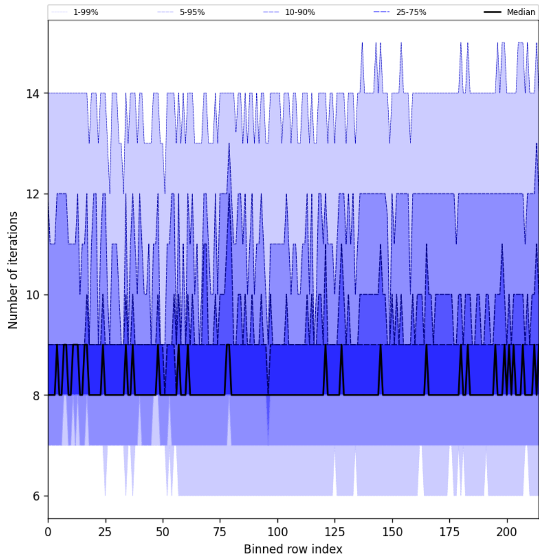
Figure 32: Along track statistics of “Number of iterations” for 2025-01-10 to 2025-01-12
