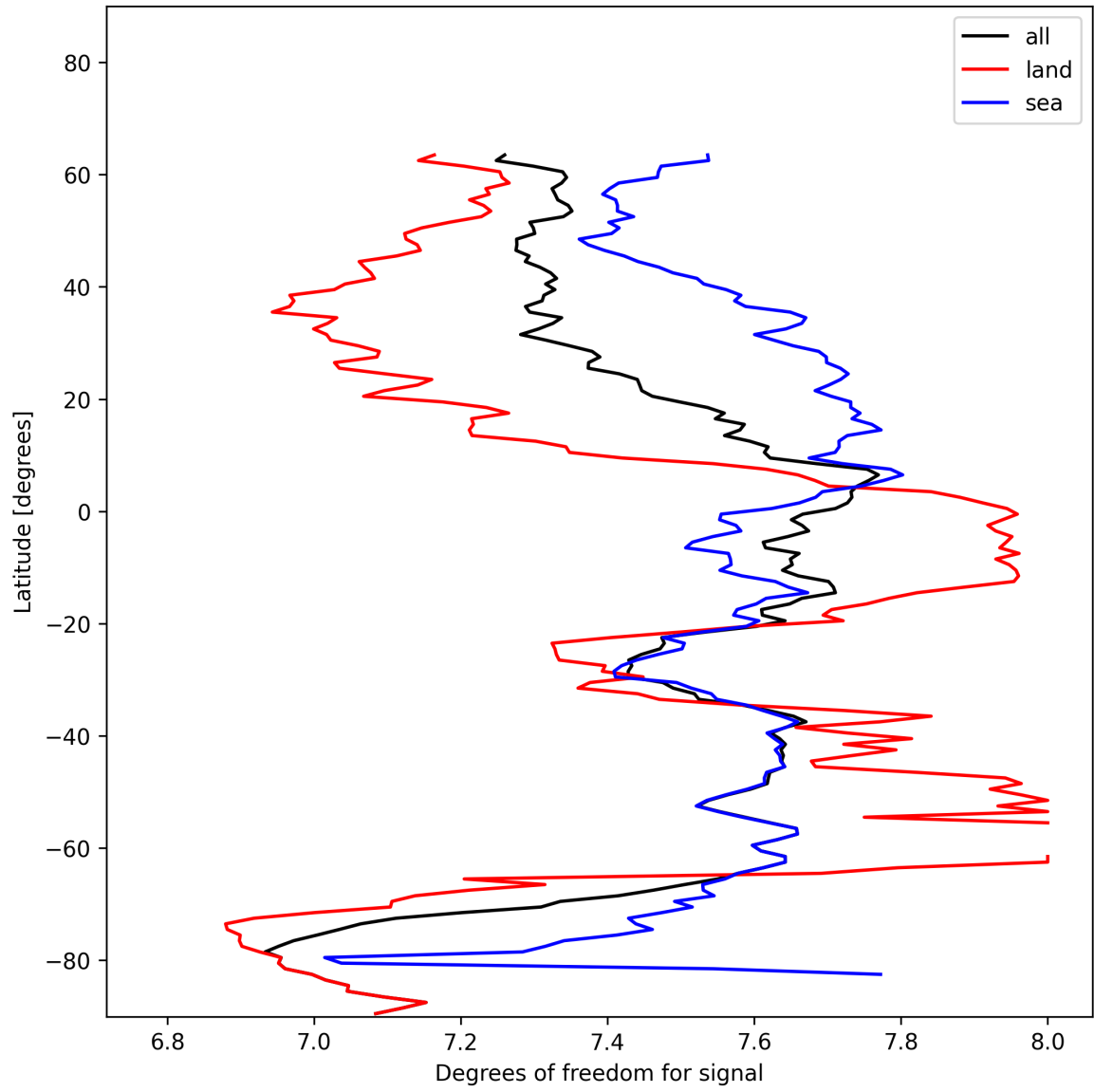
Figure 15: Zonal average of “Degrees of freedom for signal” for 2025-01-10 to 2025-01-12.
