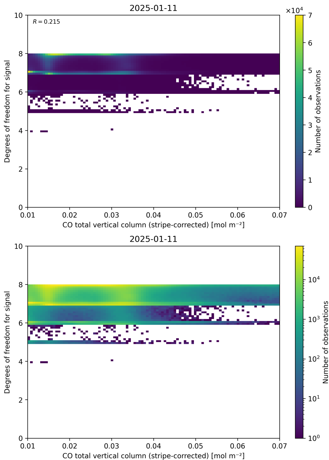
Figure 38: Scatter density plot of “CO total vertical column (stripe-corrected)” against “Degrees of freedom for signal” for 2025-01-10 to 2025-01-12.
