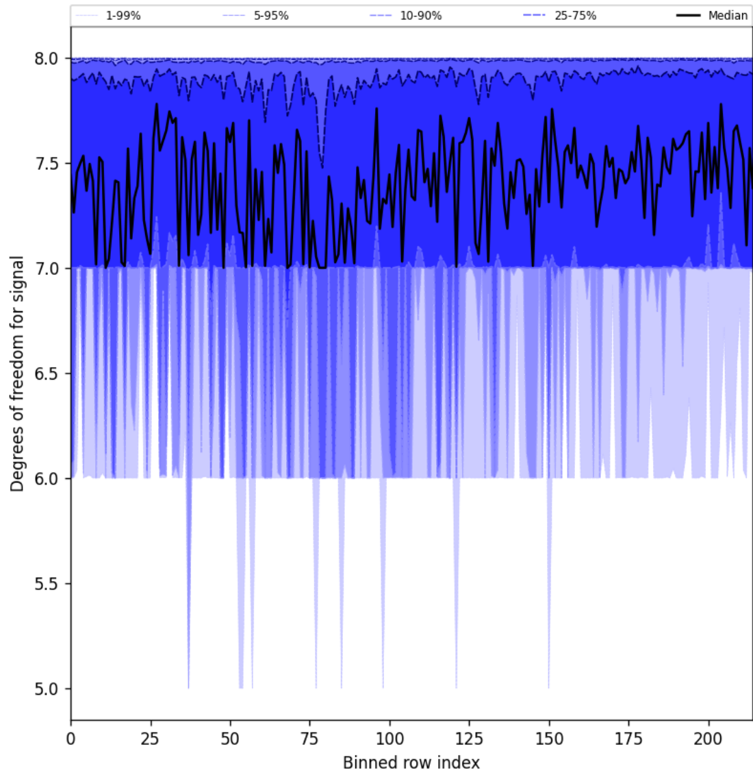
Figure 31: Along track statistics of “Degrees of freedom for signal” for 2025-01-10 to 2025-01-12
