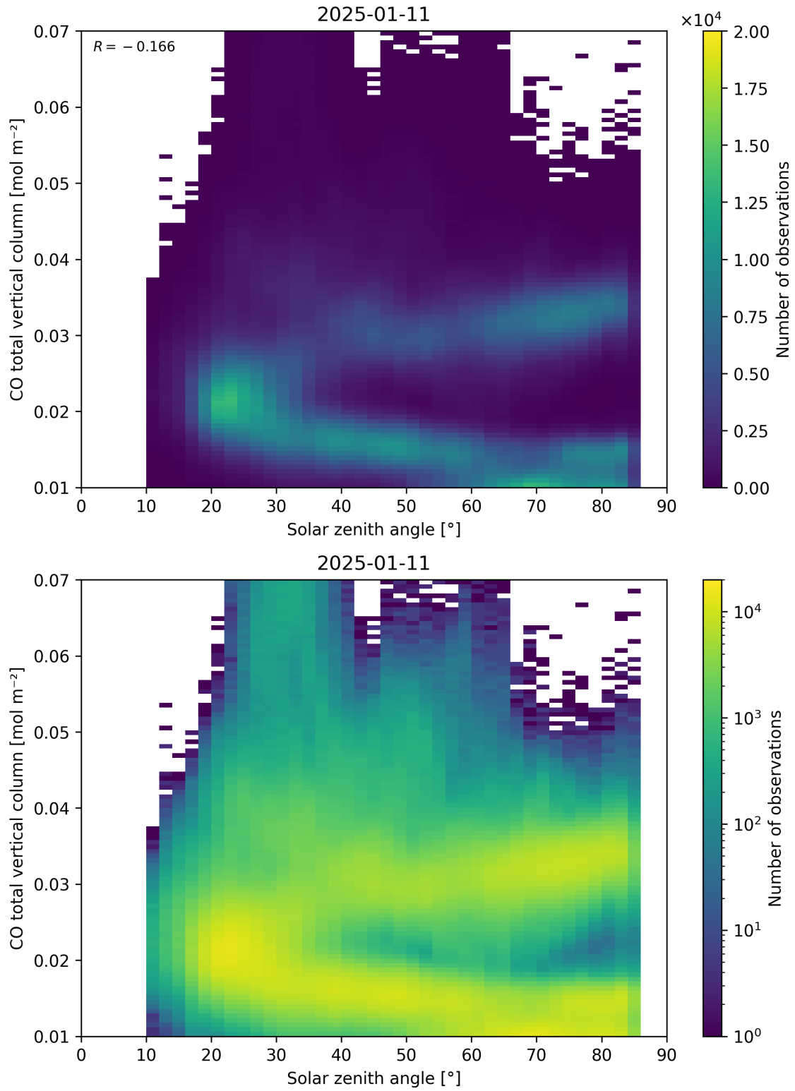
Figure 61: Scatter density plot of “Solar zenith angle” against “CO total vertical column” for 2025-01-10 to 2025-01-12.
