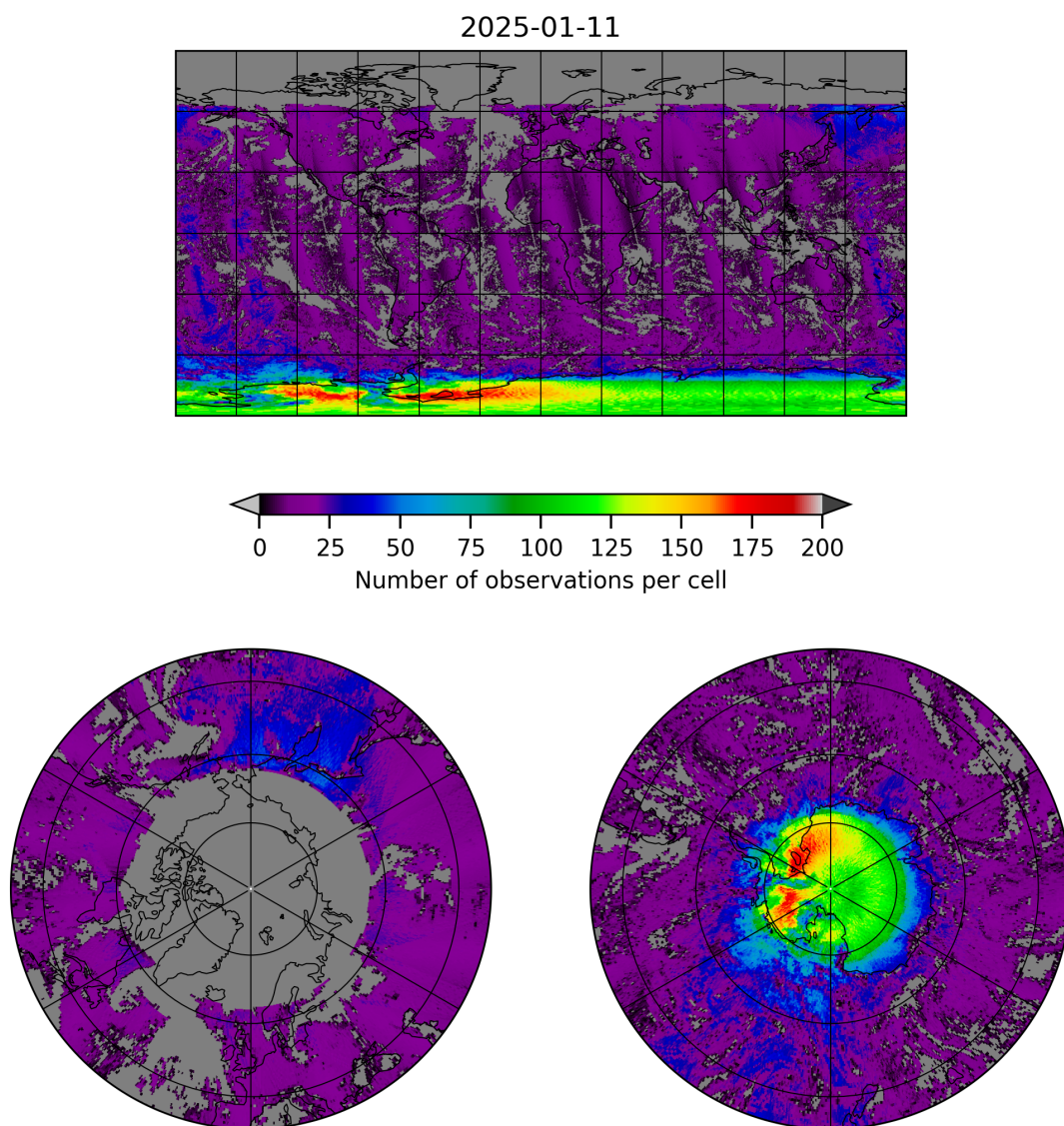
Figure 8: Map of the number of observations for 2025-01-10 to 2025-01-12
