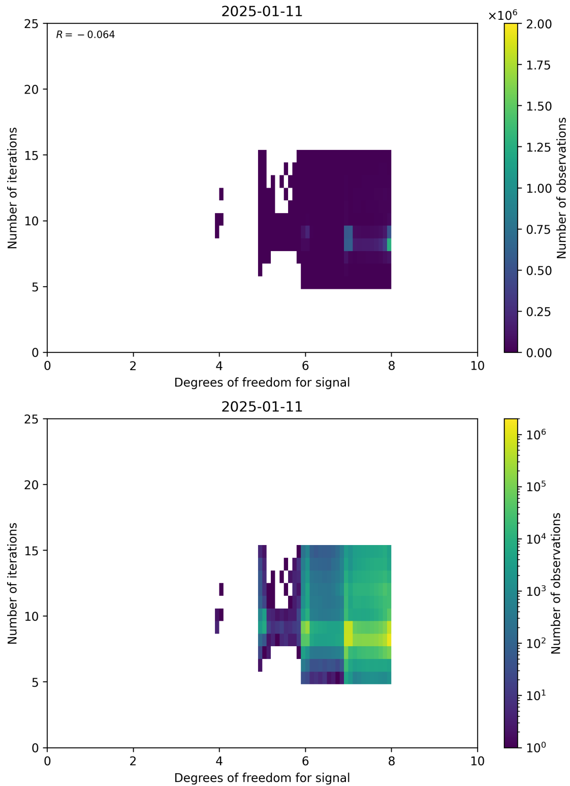
Figure 50: Scatter density plot of “Degrees of freedom for signal” against “Number of iterations” for 2025-01-10 to 2025-01-12.
