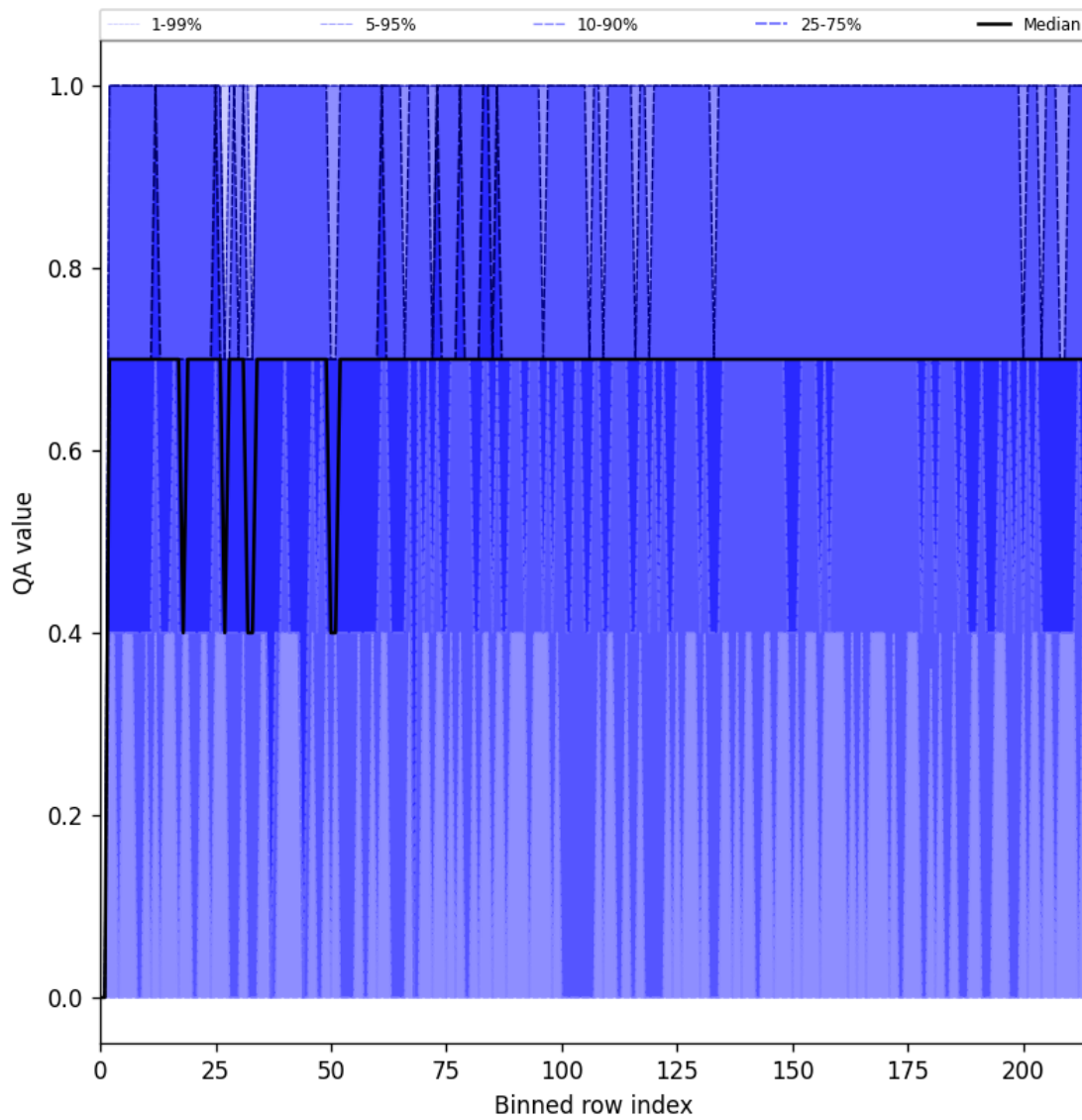
Figure 25: Along track statistics of “QA value” for 2025-01-10 to 2025-01-12
