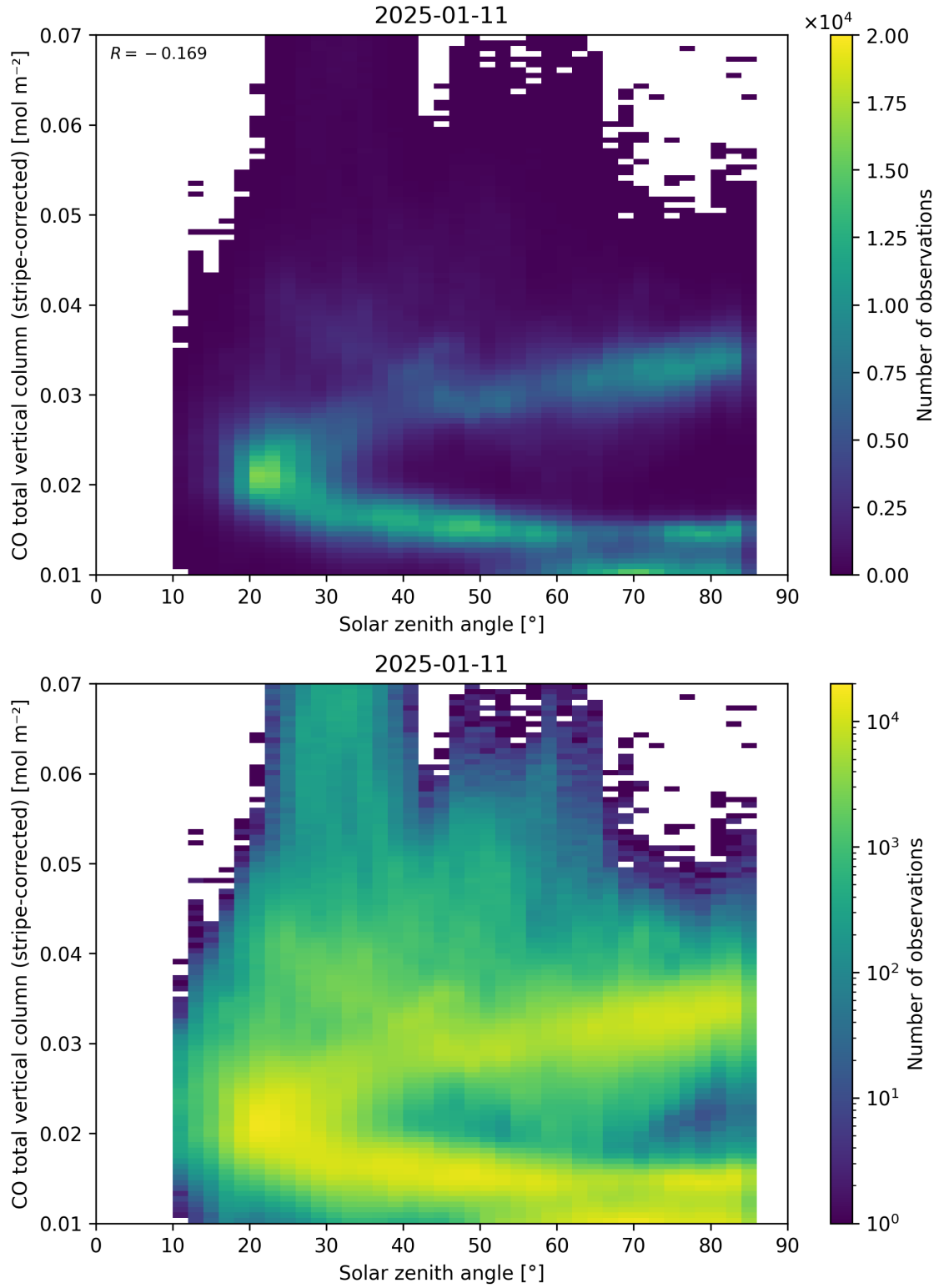
Figure 62: Scatter density plot of “Solar zenith angle” against “CO total vertical column (stripe-corrected)” for 2025-01-10 to 2025-01-12.
