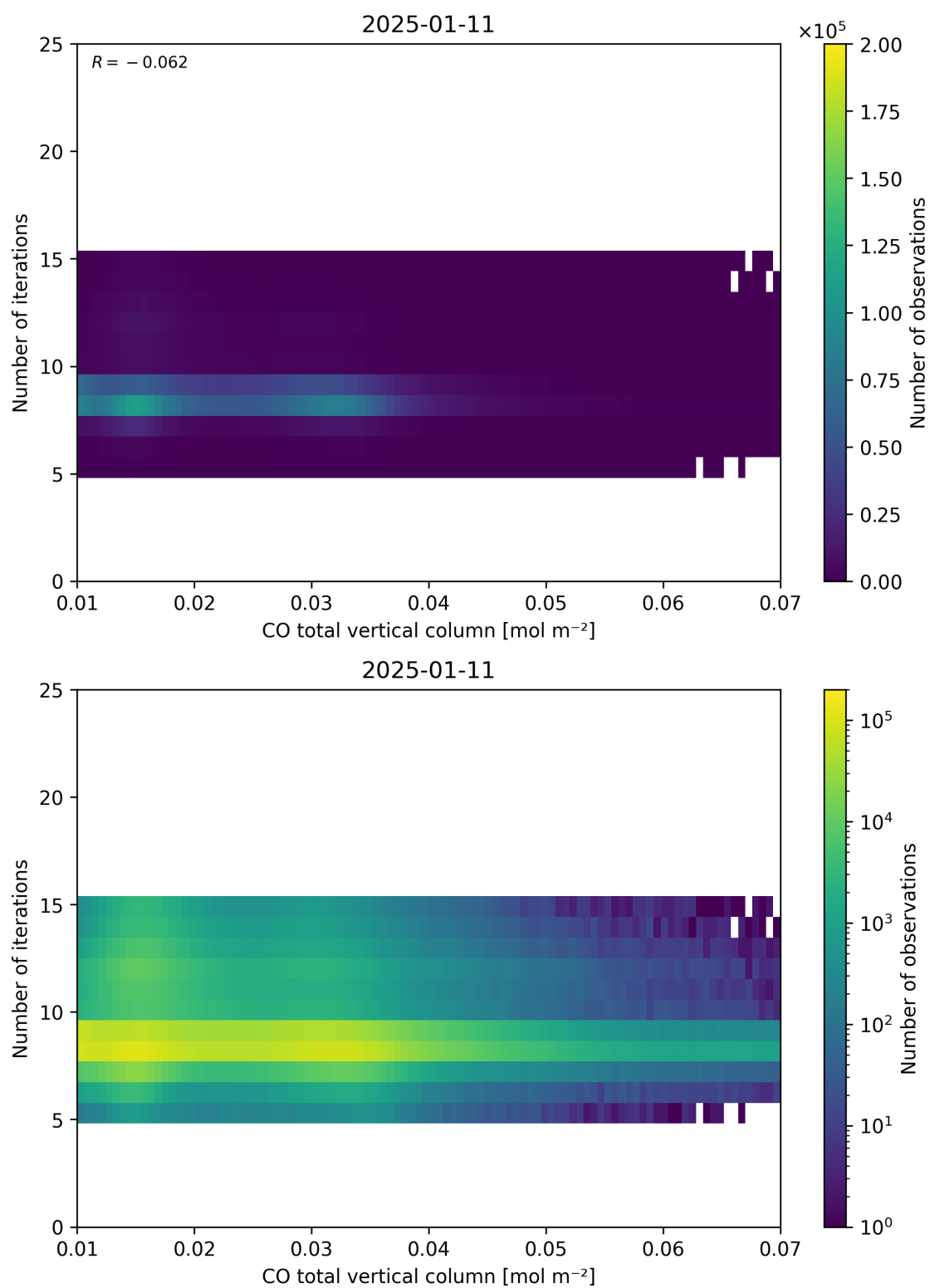
Figure 42: Scatter density plot of “CO total vertical column” against “Number of iterations” for 2025-01-10 to 2025-01-12.
