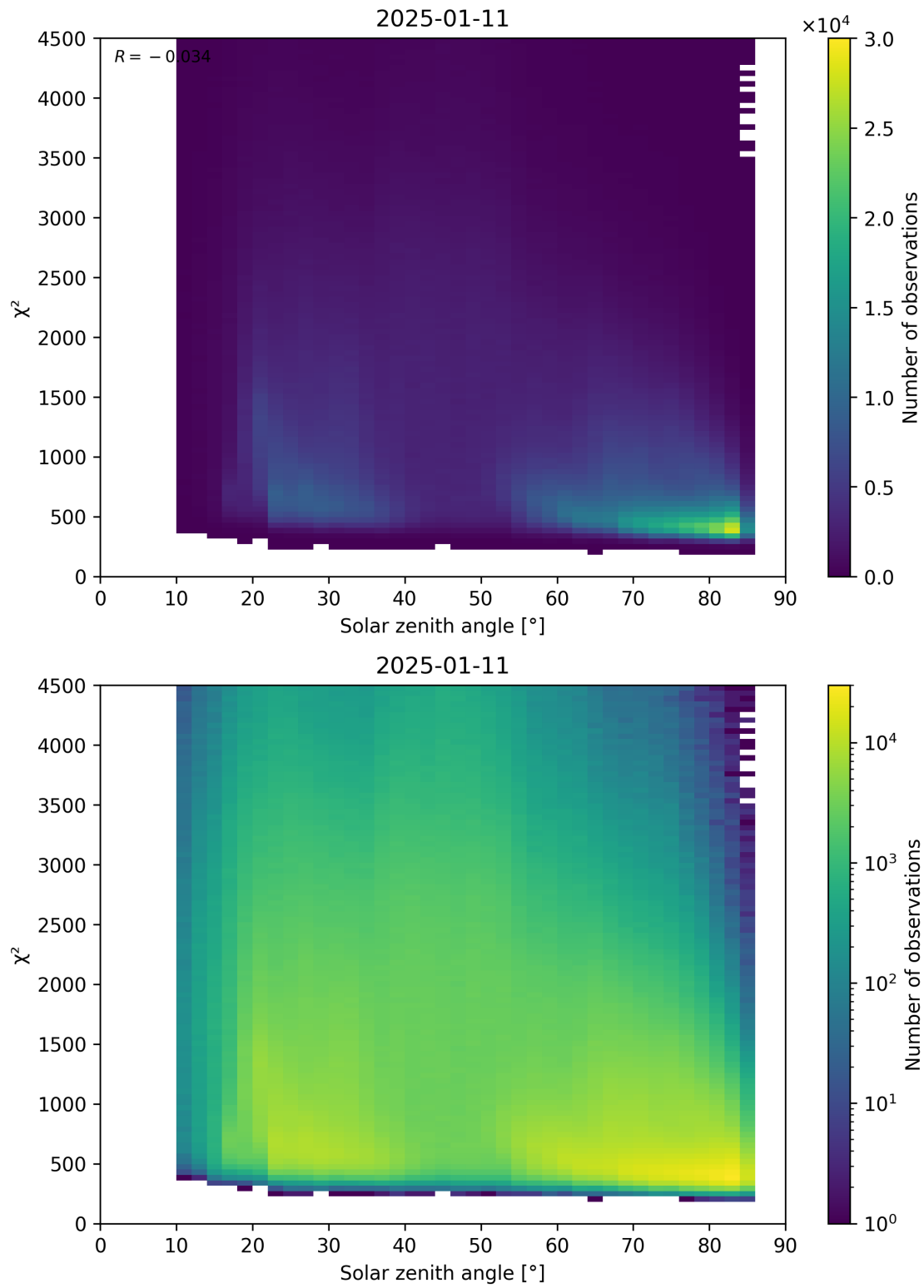
Figure 64: Scatter density plot of “Solar zenith angle” against “ \chi^2 ” for 2025-01-10 to 2025-01-12.
