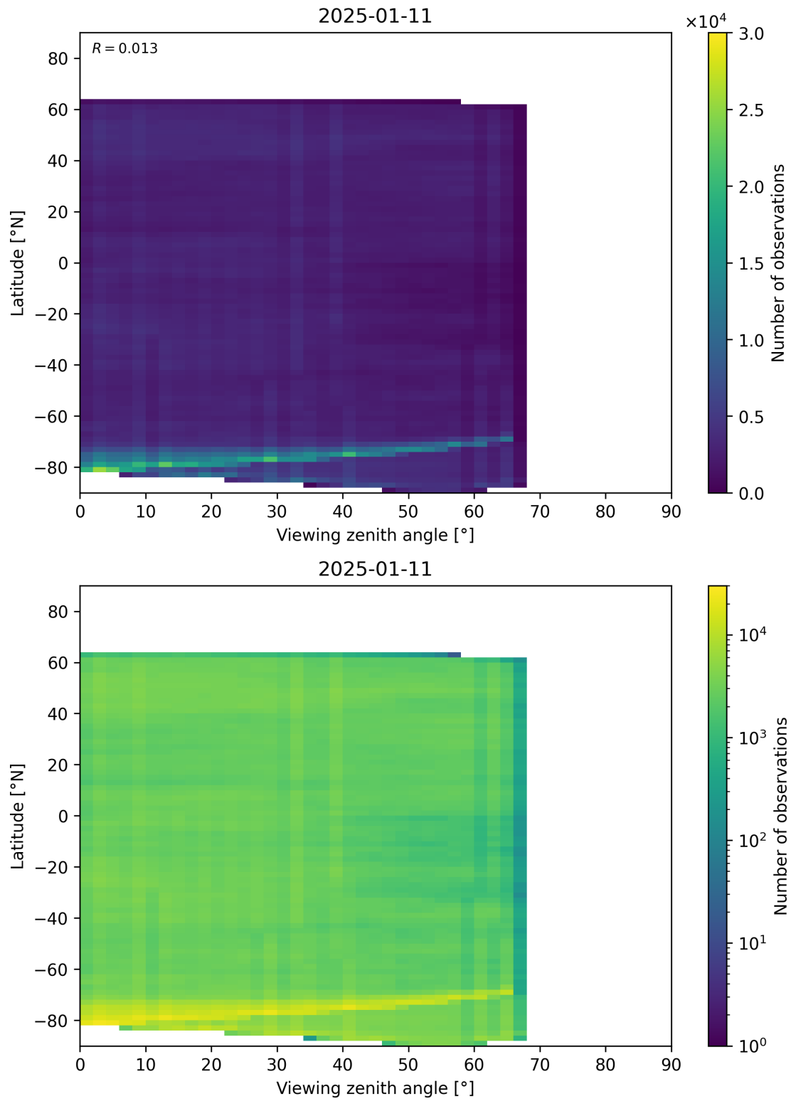
Figure 74: Scatter density plot of “Viewing zenith angle” against “Latitude” for 2025-01-10 to 2025-01-12.
