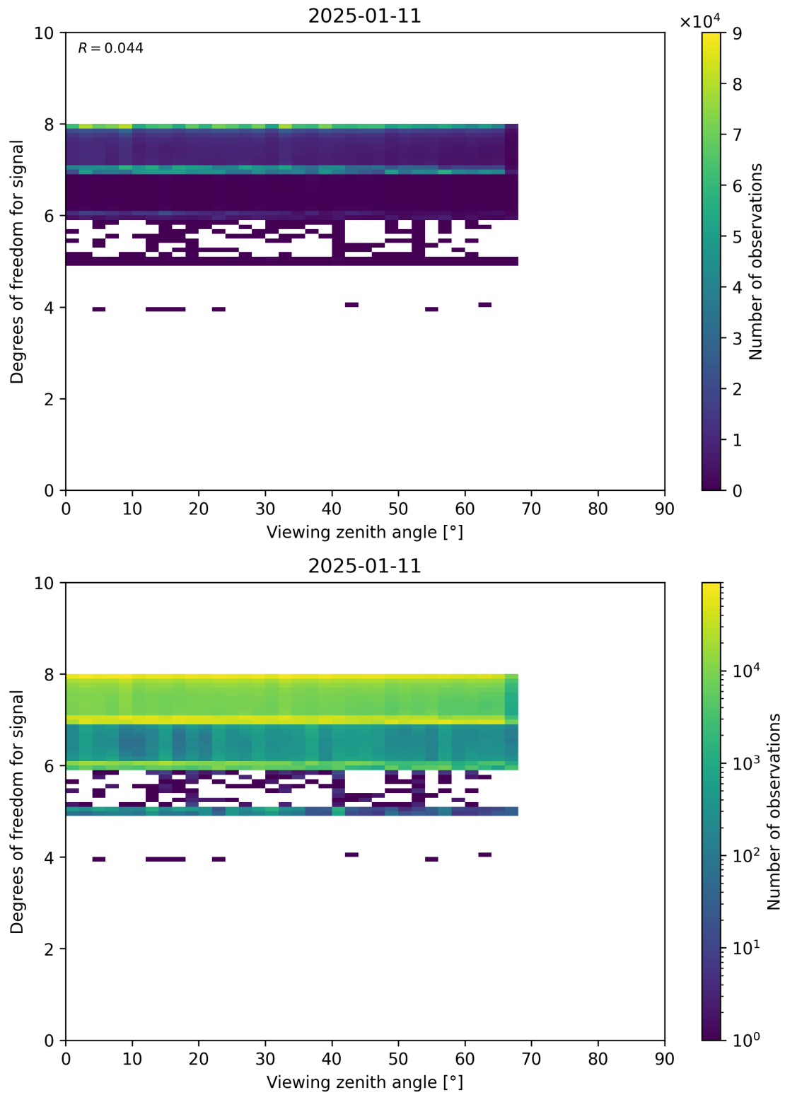
Figure 73: Scatter density plot of “Viewing zenith angle” against “Degrees of freedom for signal” for 2025-01-10 to 2025-01-12.
