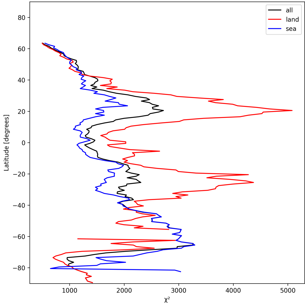
Figure 14: Zonal average of “ \chi^2 ” for 2025-01-10 to 2025-01-12.
