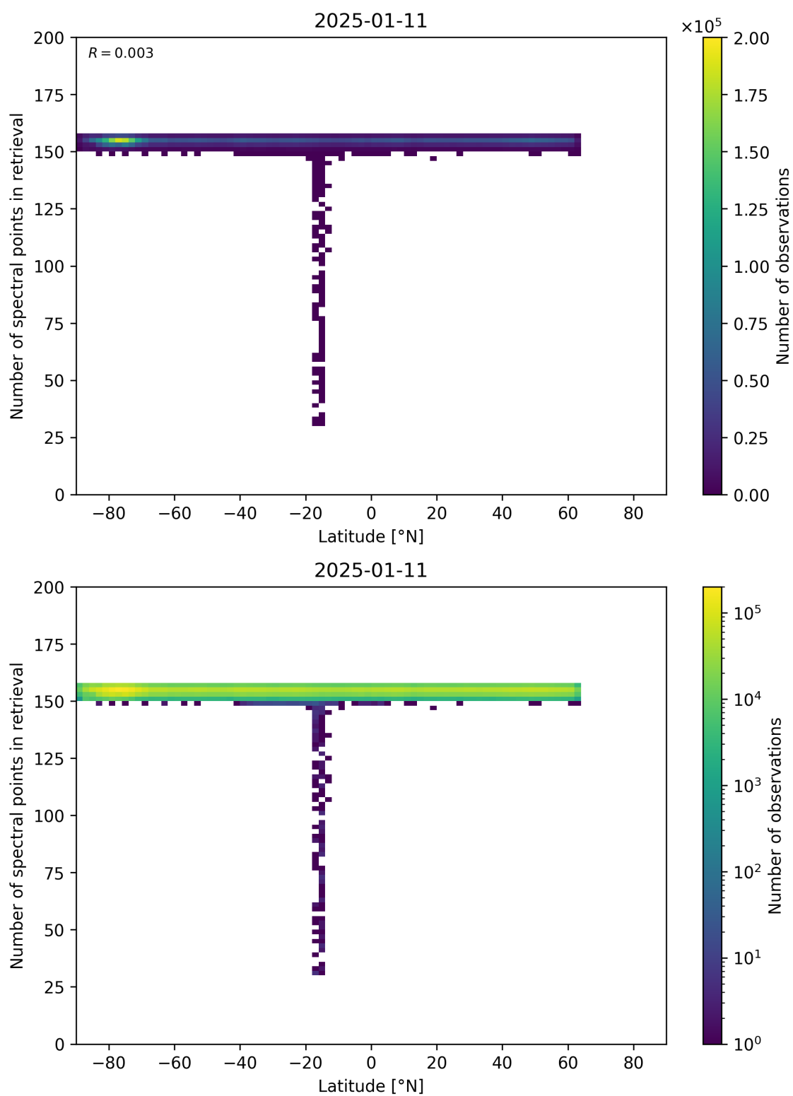
Figure 57: Scatter density plot of “Latitude” against “Number of spectral points in retrieval” for 2025-01-10 to 2025-01-12.
