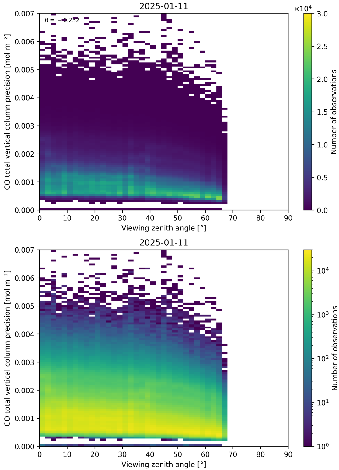
Figure 71: Scatter density plot of “Viewing zenith angle” against “CO total vertical column precision” for 2025-01-10 to 2025-01-12.
