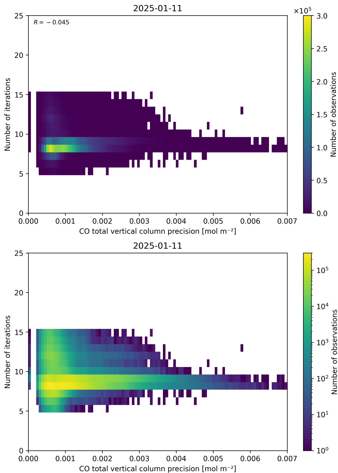
Figure 46: Scatter density plot of “CO total vertical column precision” against “Number of iterations” for 2025-01-10 to 2025-01-12.
