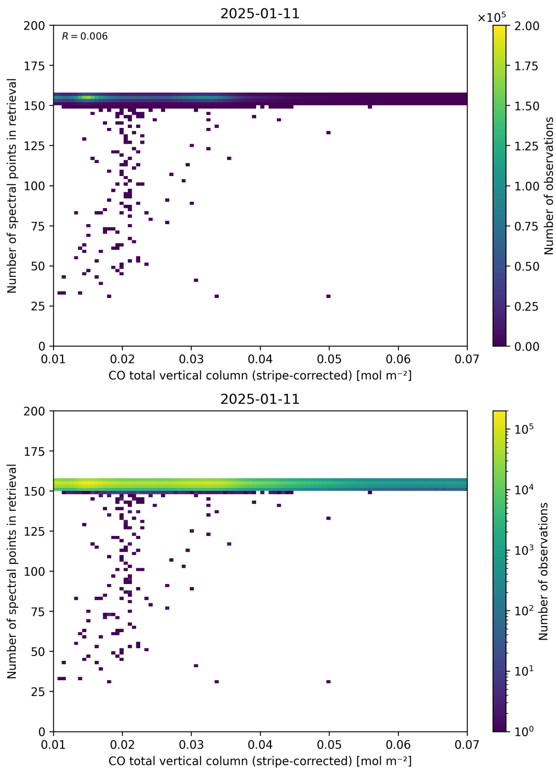
Figure 40: Scatter density plot of “CO total vertical column (stripe-corrected)” against “Number of spectral points in retrieval” for 2025-01-10 to 2025-01-12.
