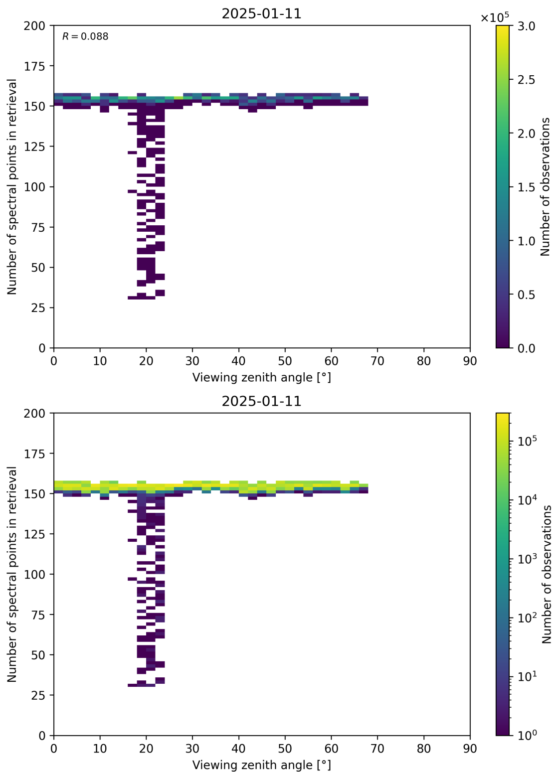
Figure 76: Scatter density plot of “Viewing zenith angle” against “Number of spectral points in retrieval” for 2025-01-10 to 2025-01-12.
