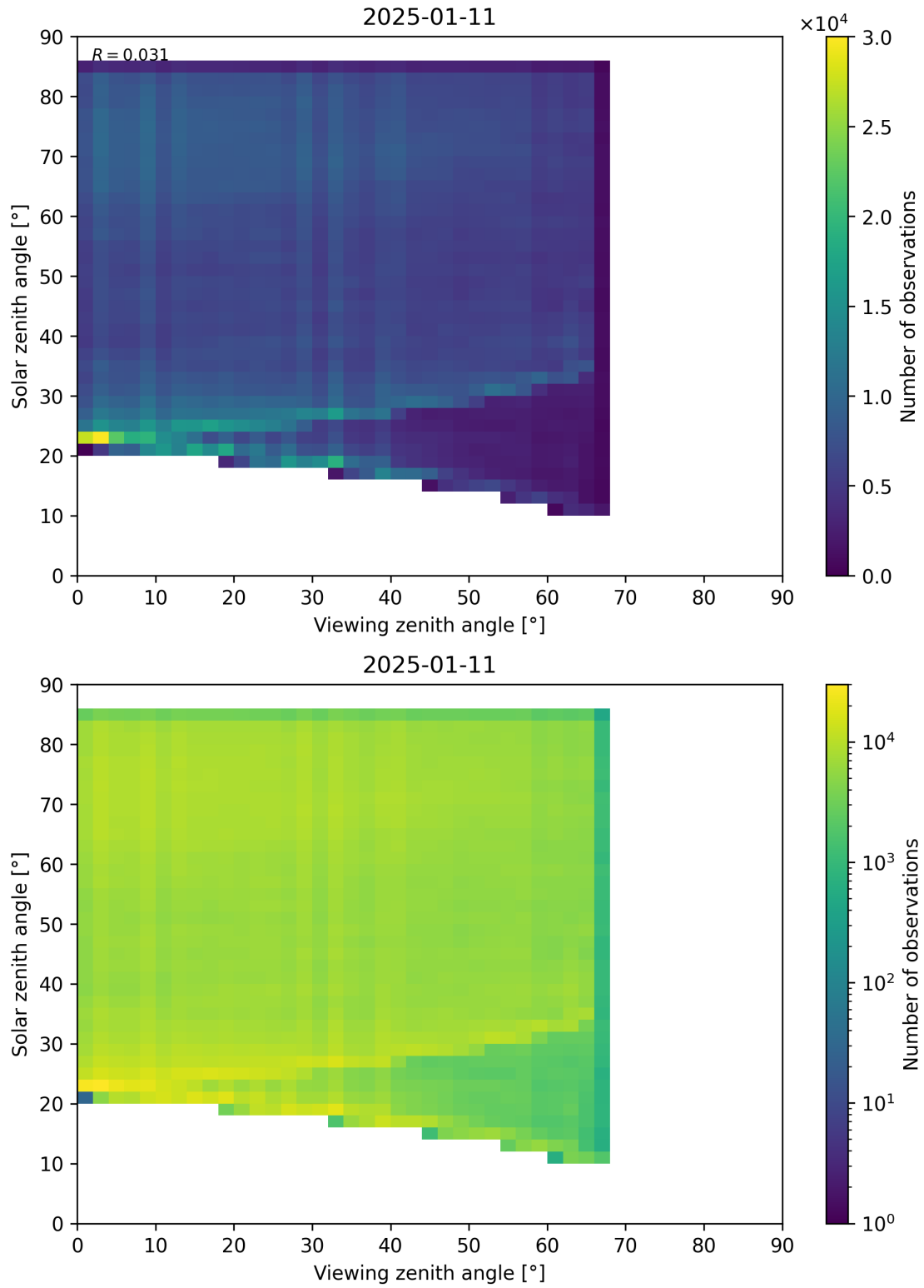
Figure 77: Scatter density plot of “Viewing zenith angle” against “Solar zenith angle” for 2025-01-10 to 2025-01-12.
