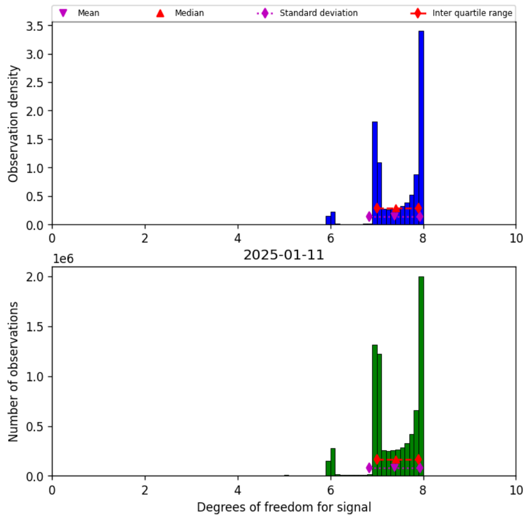
Figure 23: Histogram of “Degrees of freedom for signal” for 2025-01-10 to 2025-01-12
