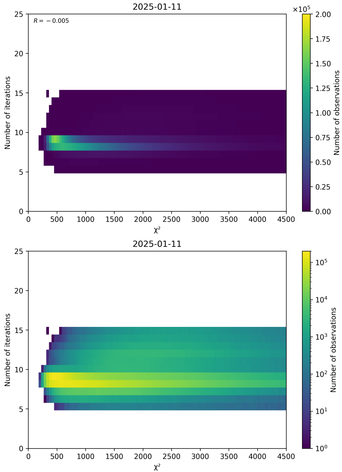
Figure 49: Scatter density plot of “ \chi^2 ” against “Number of iterations” for 2025-01-10 to 2025-01-12.
