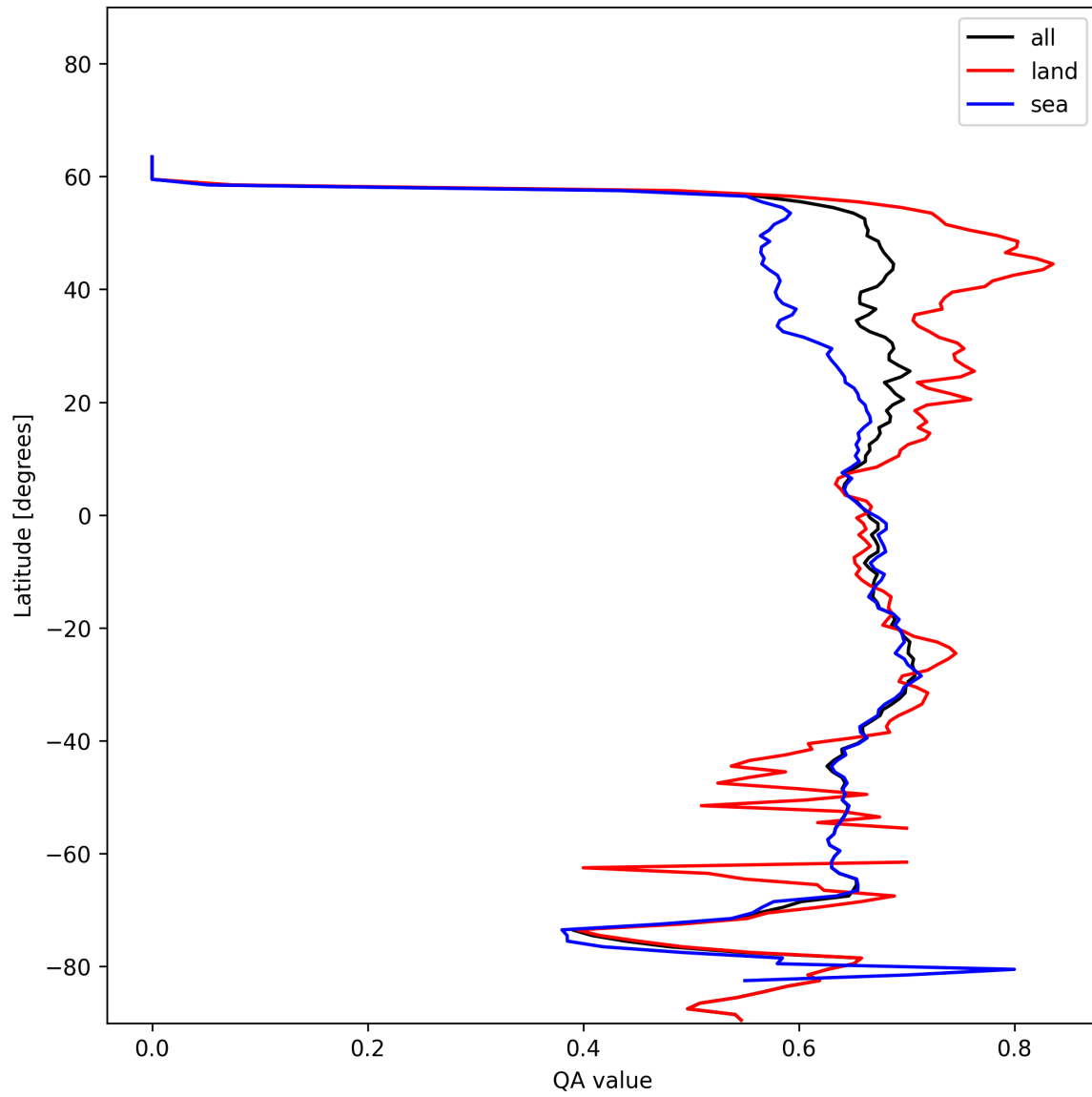
Figure 9: Zonal average of “QA value” for 2025-01-10 to 2025-01-12.
