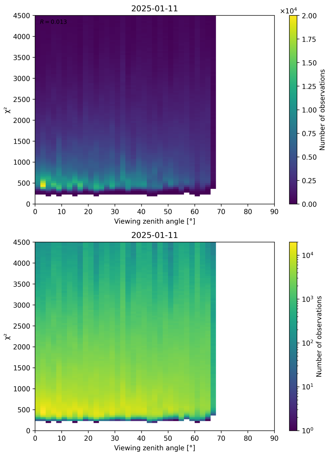
Figure 72: Scatter density plot of “Viewing zenith angle” against “ \chi^2 ” for 2025-01-10 to 2025-01-12.
