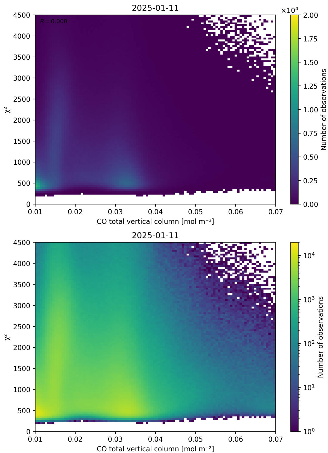
Figure 35: Scatter density plot of “CO total vertical column” against “ \chi^2 ” for 2025-01-10 to 2025-01-12.
