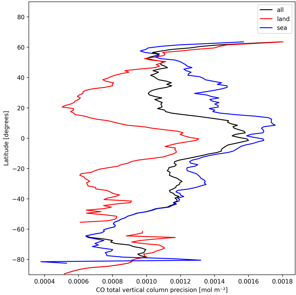
Figure 12: Zonal average of “CO total vertical column precision” for 2025-01-10 to 2025-01-12.
