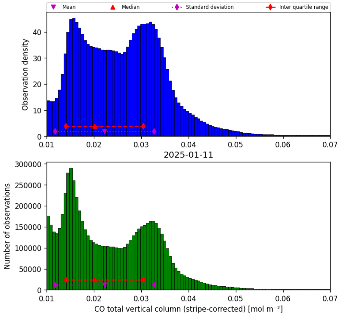
Figure 19: Histogram of “CO total vertical column (stripe-corrected)” for 2025-01-10 to 2025-01-12
