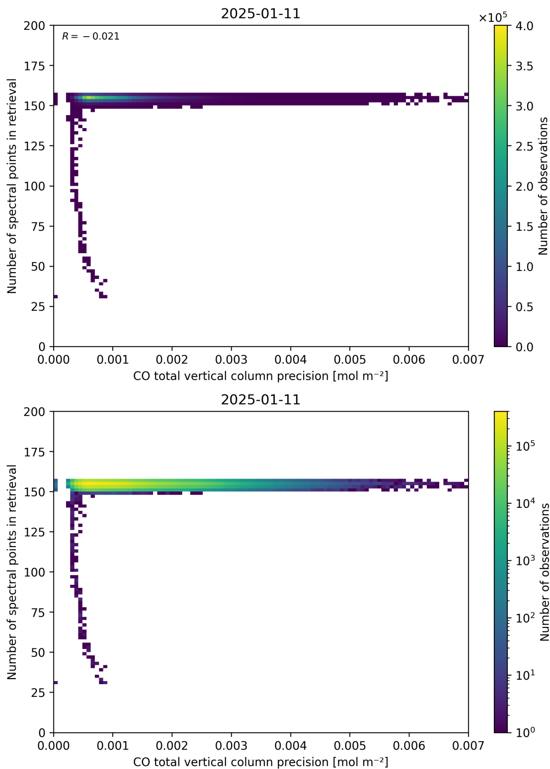
Figure 47: Scatter density plot of “CO total vertical column precision” against “Number of spectral points in retrieval” for 2025-01-10 to 2025-01-12.
