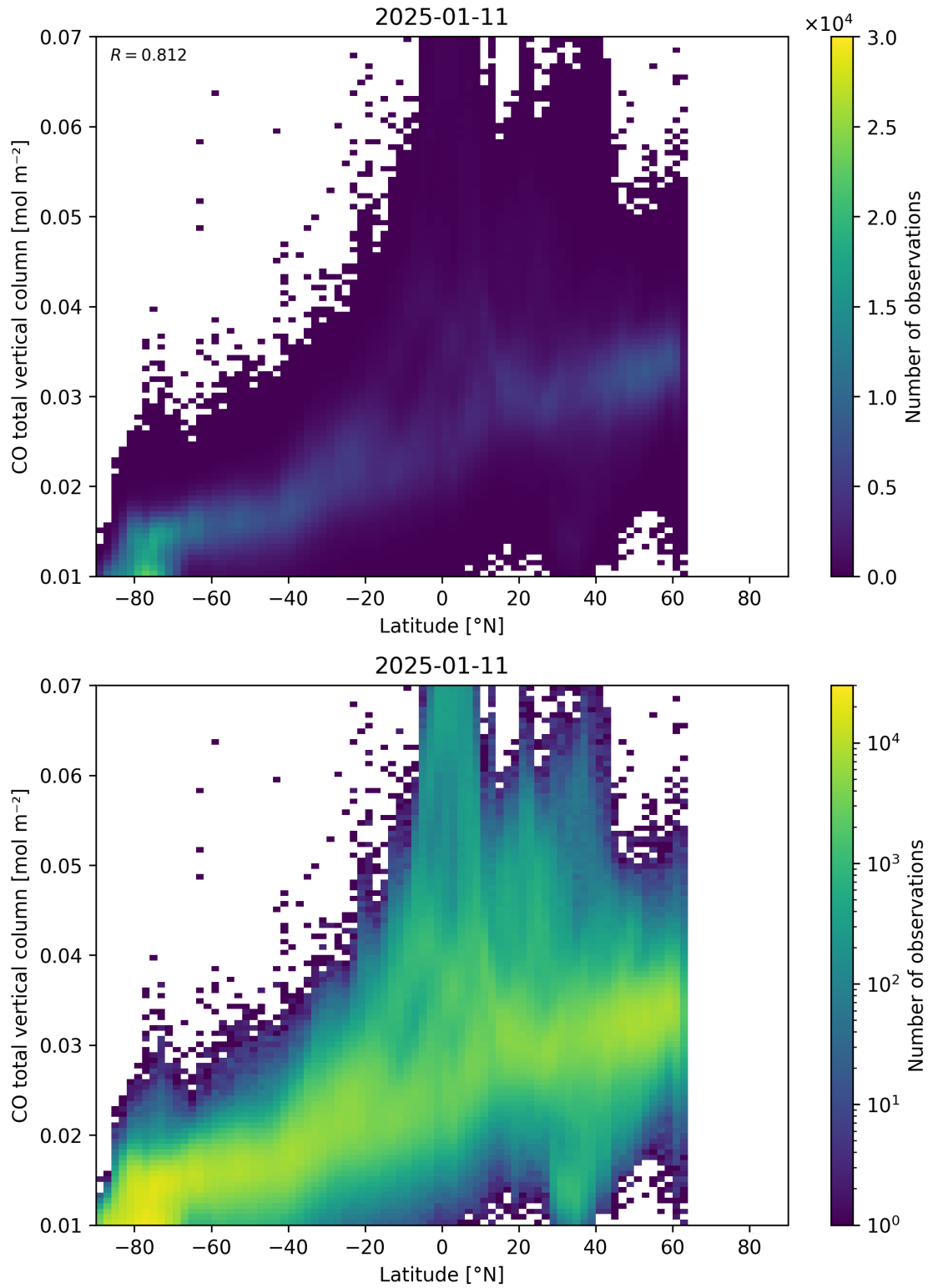
Figure 51: Scatter density plot of “Latitude” against “CO total vertical column” for 2025-01-10 to 2025-01-12.
