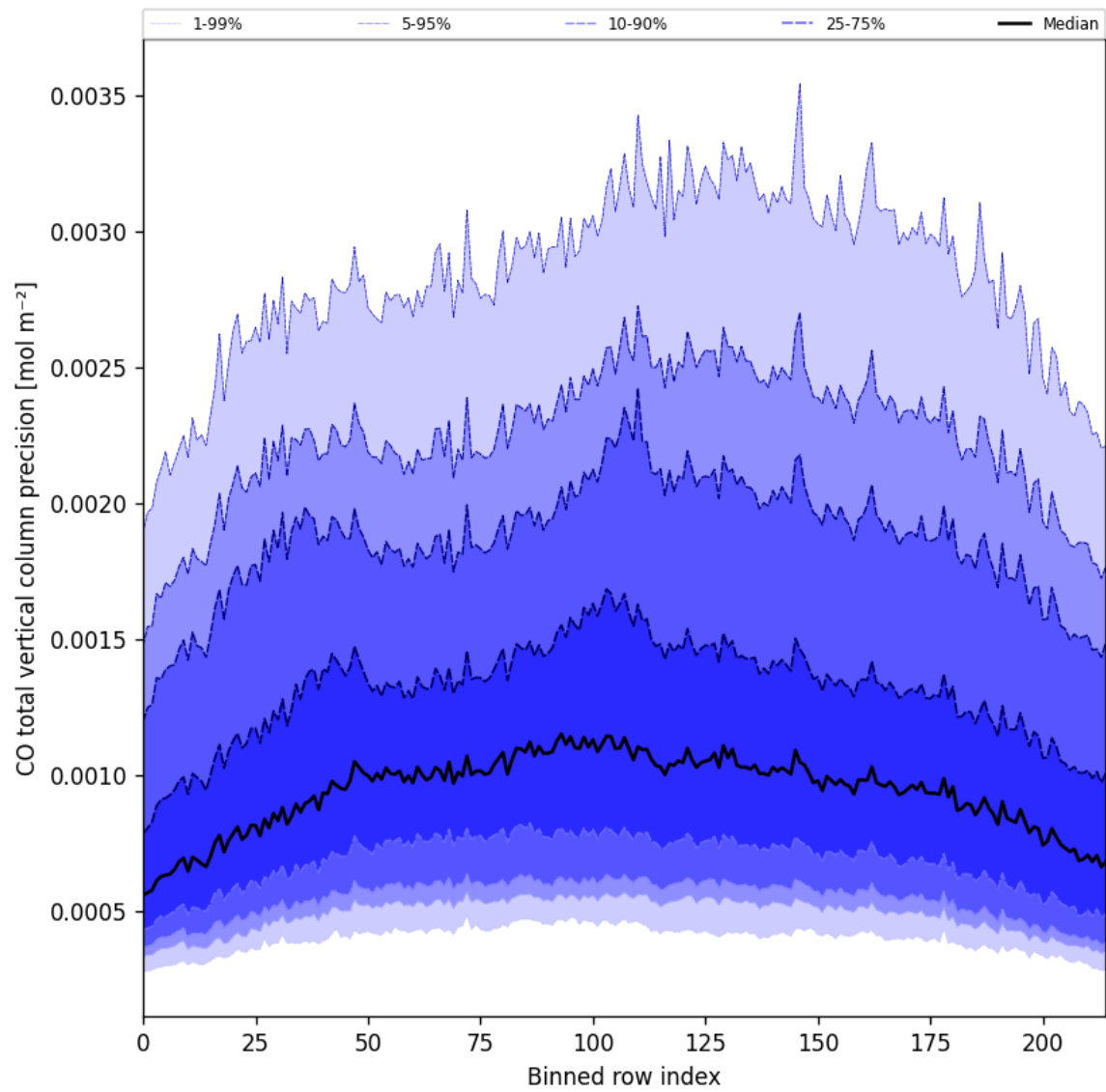
Figure 28: Along track statistics of “CO total vertical column precision” for 2025-01-12 to 2025-01-13
