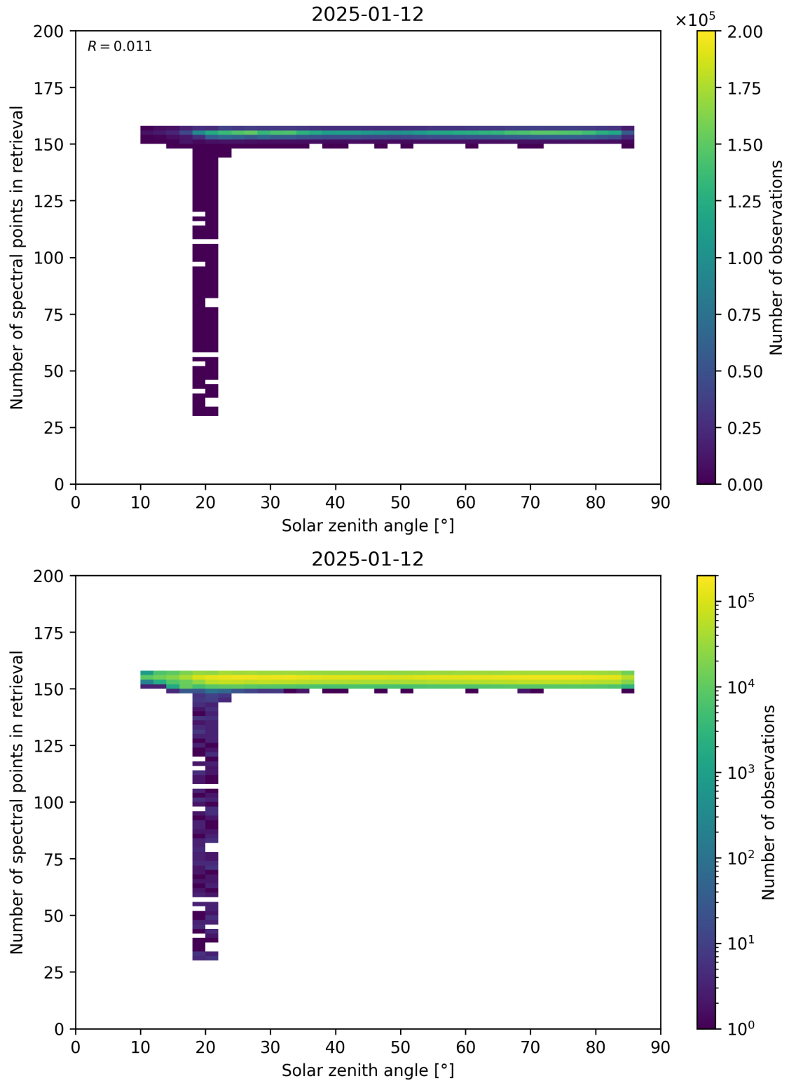
Figure 68: Scatter density plot of “Solar zenith angle” against “Number of spectral points in retrieval” for 2025-01-12 to 2025-01-13.
