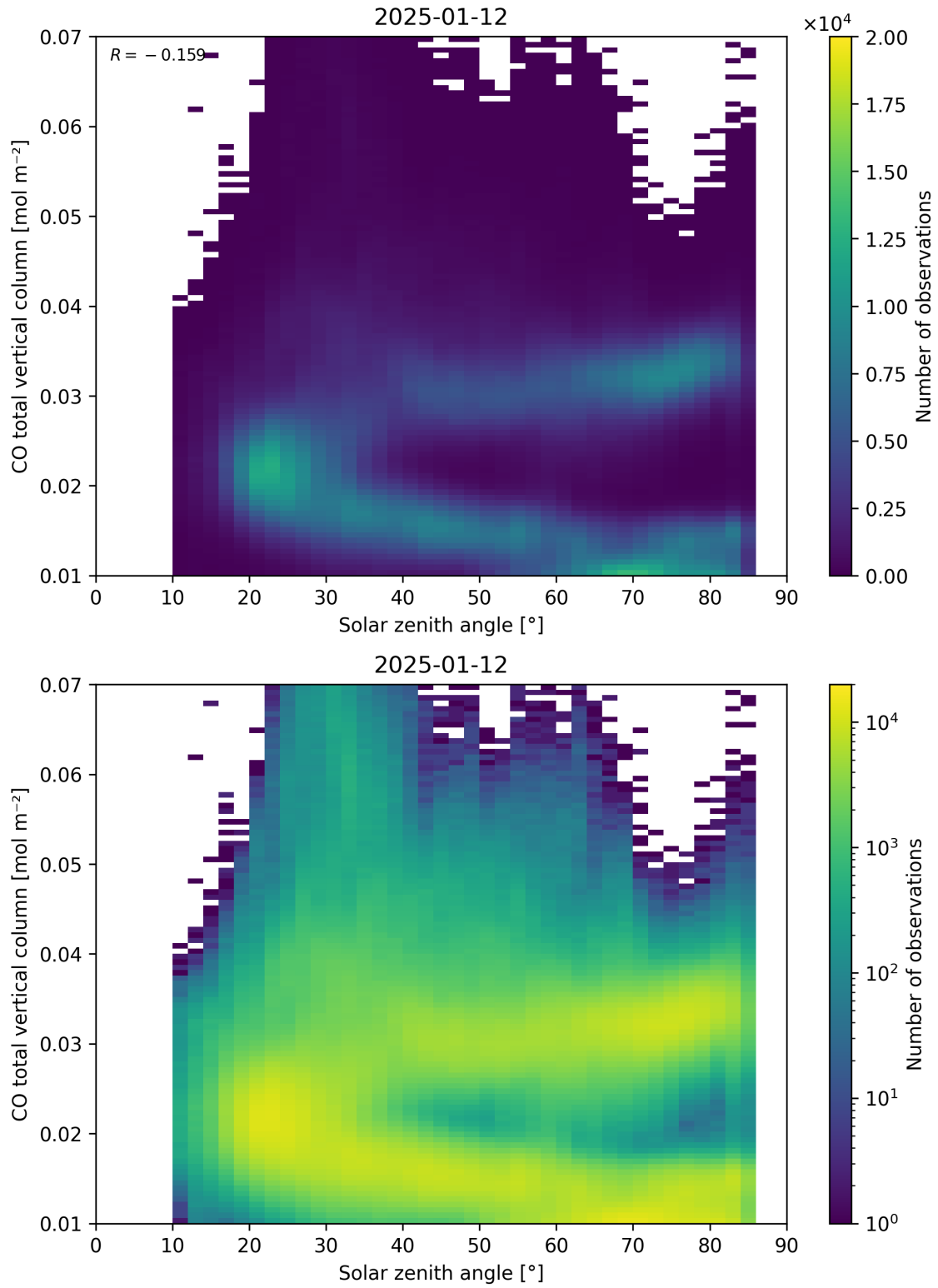
Figure 61: Scatter density plot of “Solar zenith angle” against “CO total vertical column” for 2025-01-12 to 2025-01-13.
