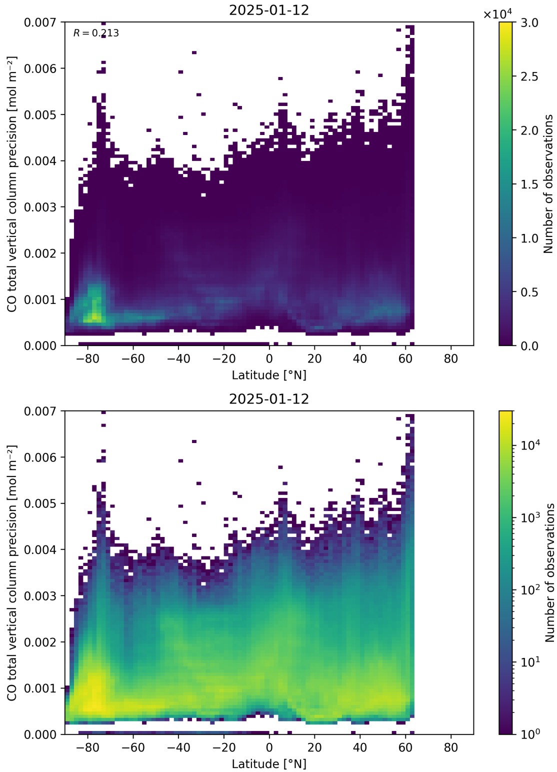
Figure 53: Scatter density plot of “Latitude” against “CO total vertical column precision” for 2025-01-12 to 2025-01-13.
