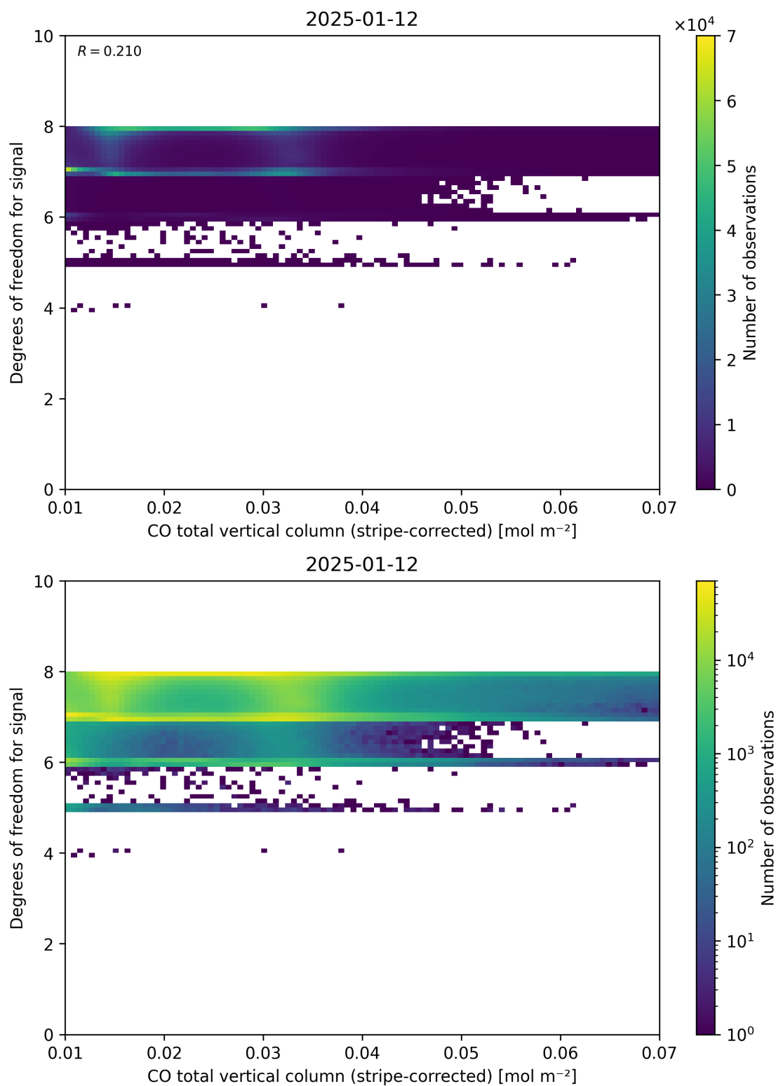
Figure 38: Scatter density plot of “CO total vertical column (stripe-corrected)” against “Degrees of freedom for signal” for 2025-01-12 to 2025-01-13.
