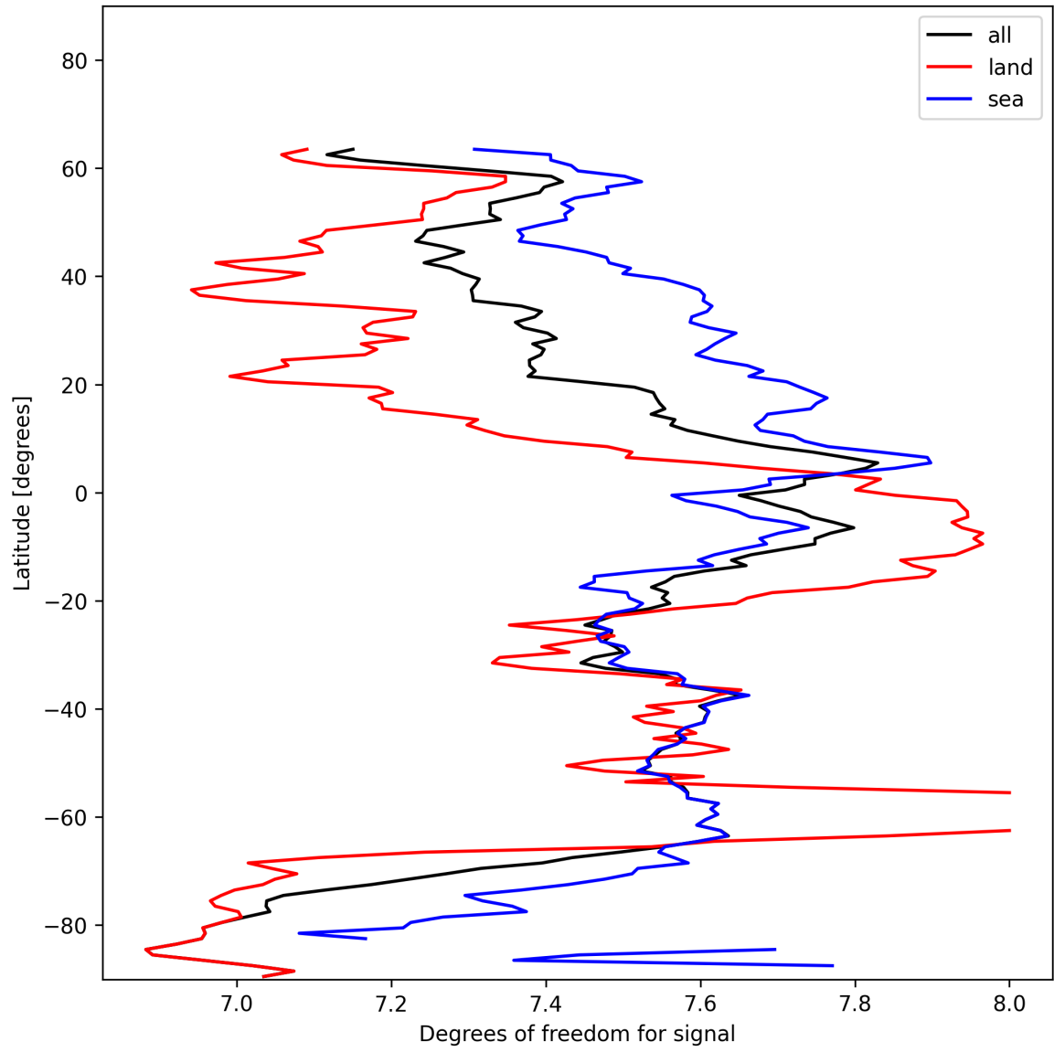
Figure 15: Zonal average of “Degrees of freedom for signal” for 2025-01-12 to 2025-01-13.
