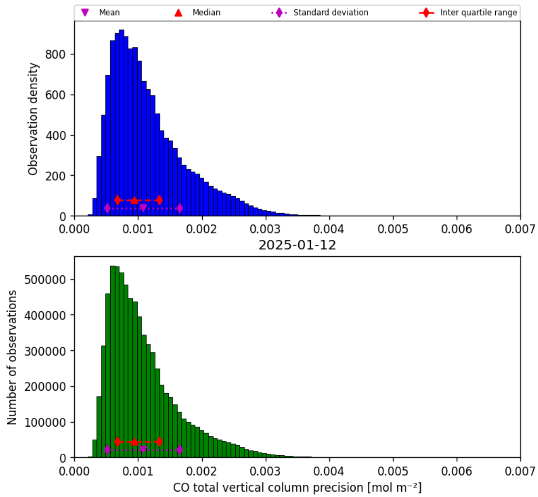
Figure 20: Histogram of “CO total vertical column precision” for 2025-01-12 to 2025-01-13
