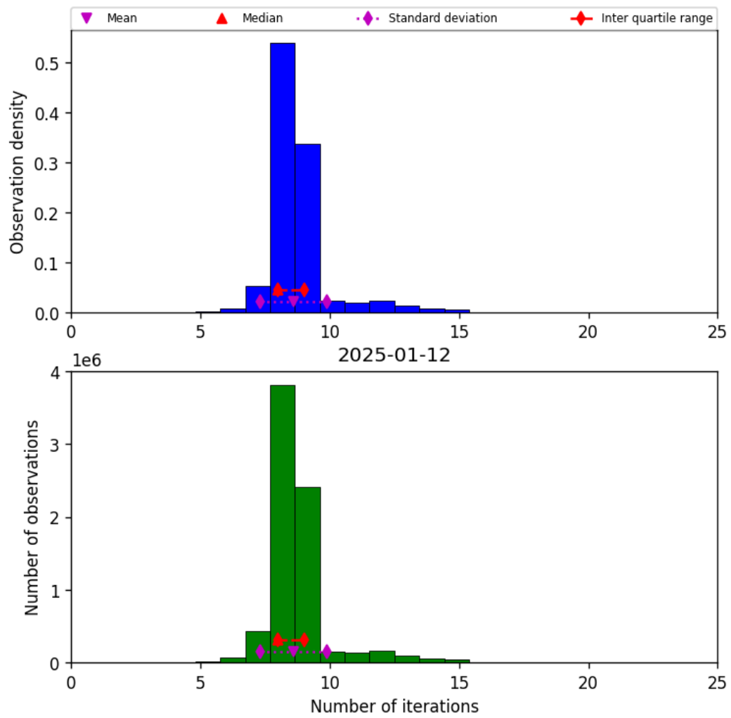
Figure 24: Histogram of “Number of iterations” for 2025-01-12 to 2025-01-13
