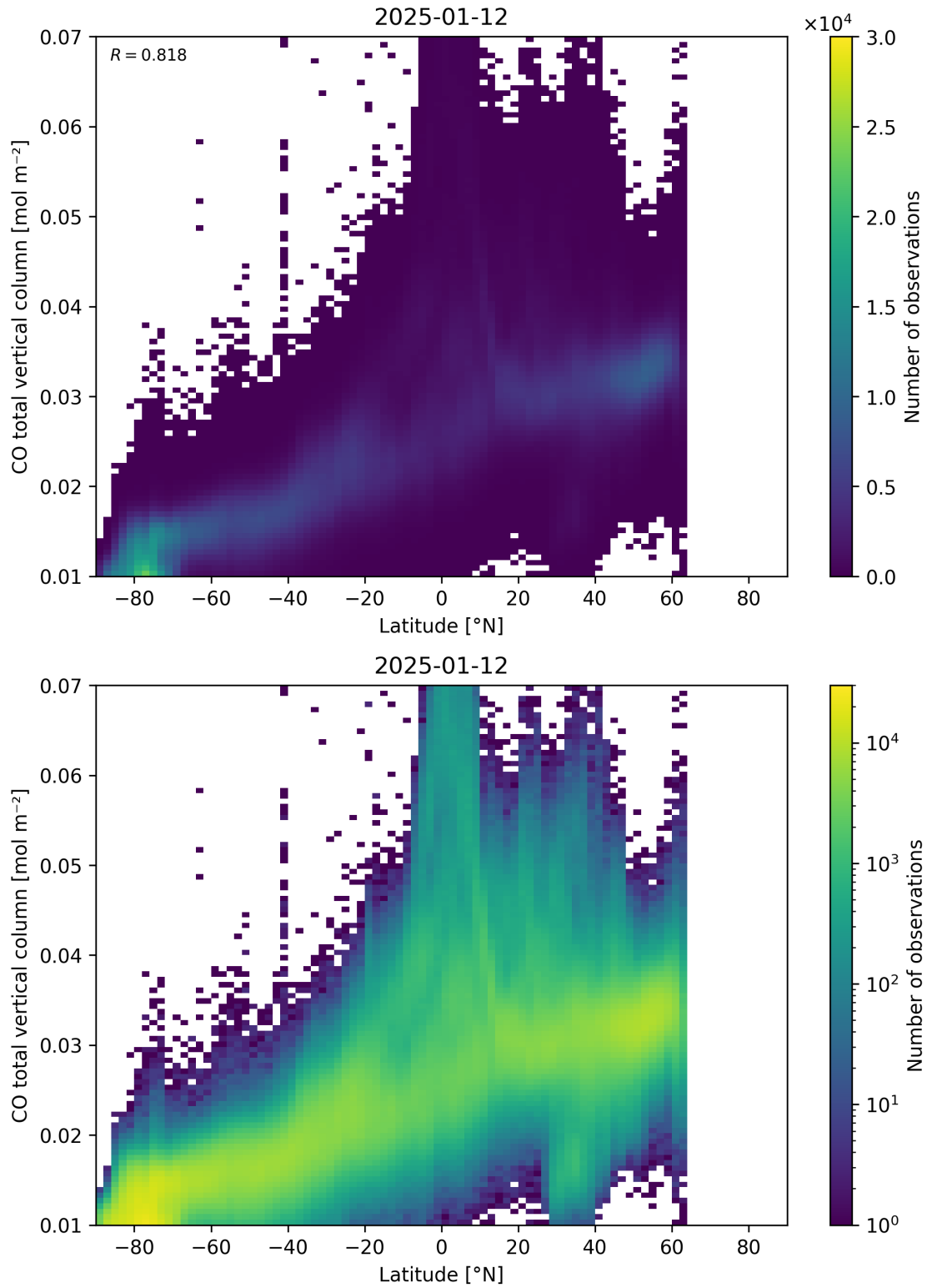
Figure 51: Scatter density plot of “Latitude” against “CO total vertical column” for 2025-01-12 to 2025-01-13.
