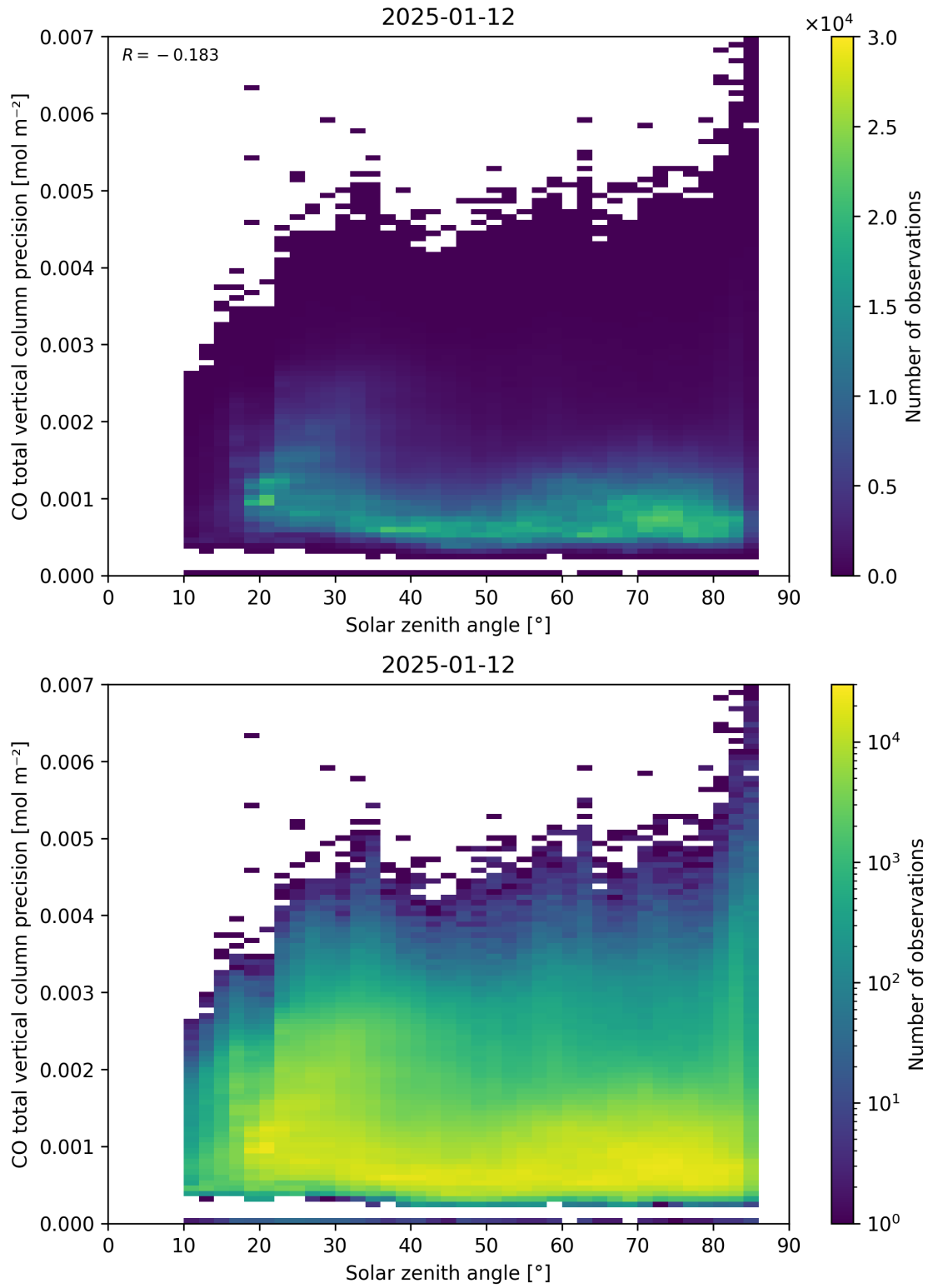
Figure 63: Scatter density plot of “Solar zenith angle” against “CO total vertical column precision” for 2025-01-12 to 2025-01-13.
