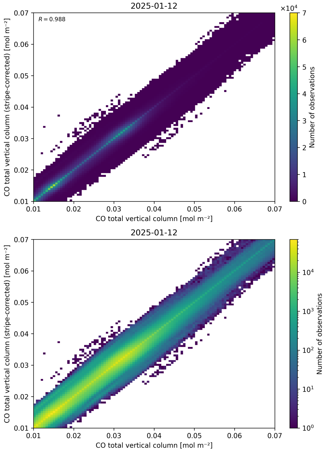
Figure 33: Scatter density plot of “CO total vertical column” against “CO total vertical column (stripe-corrected)” for 2025-01-12 to 2025-01-13.
