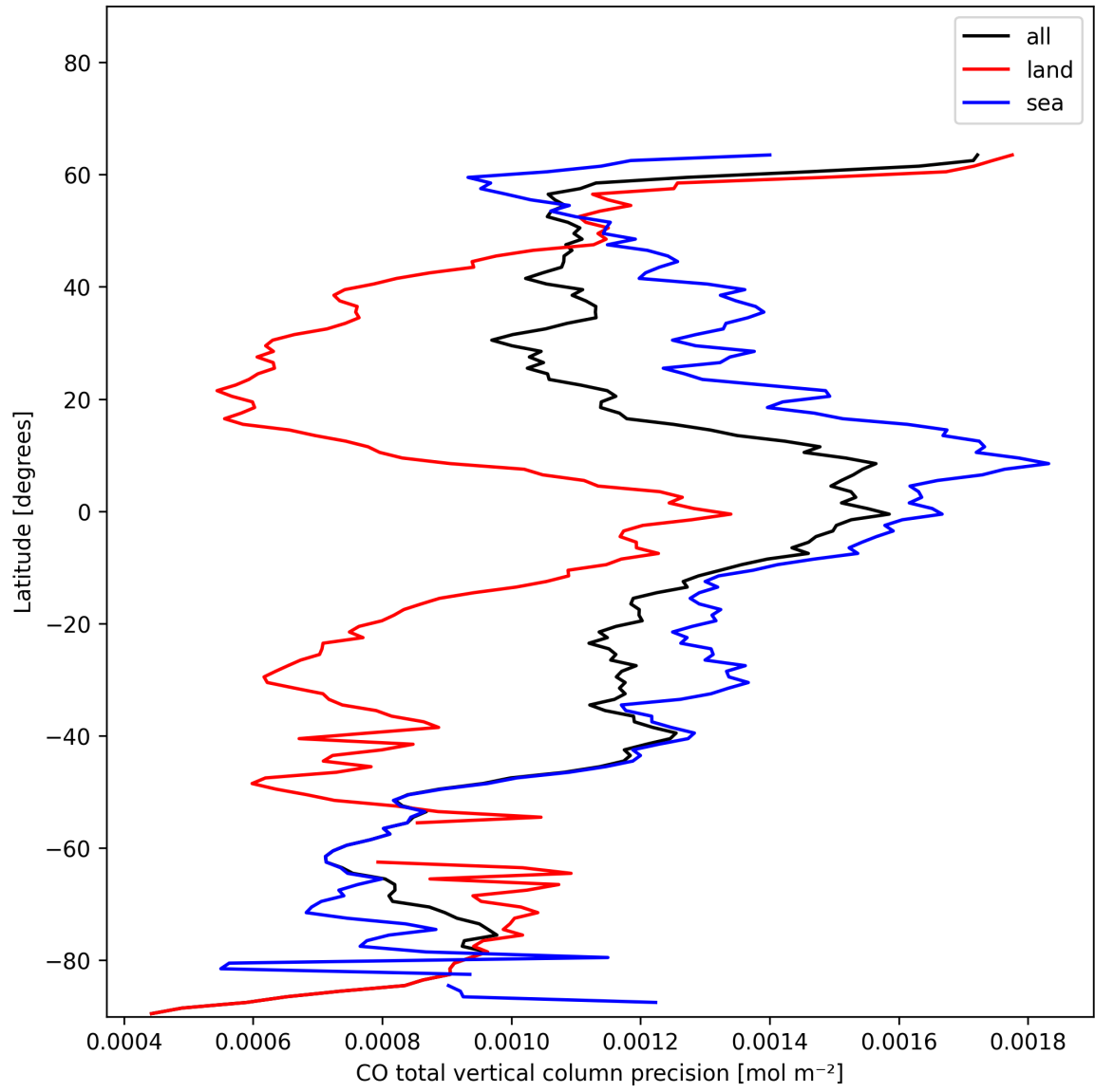
Figure 12: Zonal average of "CO total vertical column precision" for 2025-01-12 to 2025-01-13.
