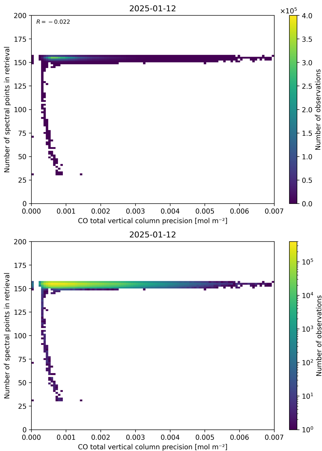
Figure 47: Scatter density plot of “CO total vertical column precision” against “Number of spectral points in retrieval” for 2025-01-12 to 2025-01-13.
