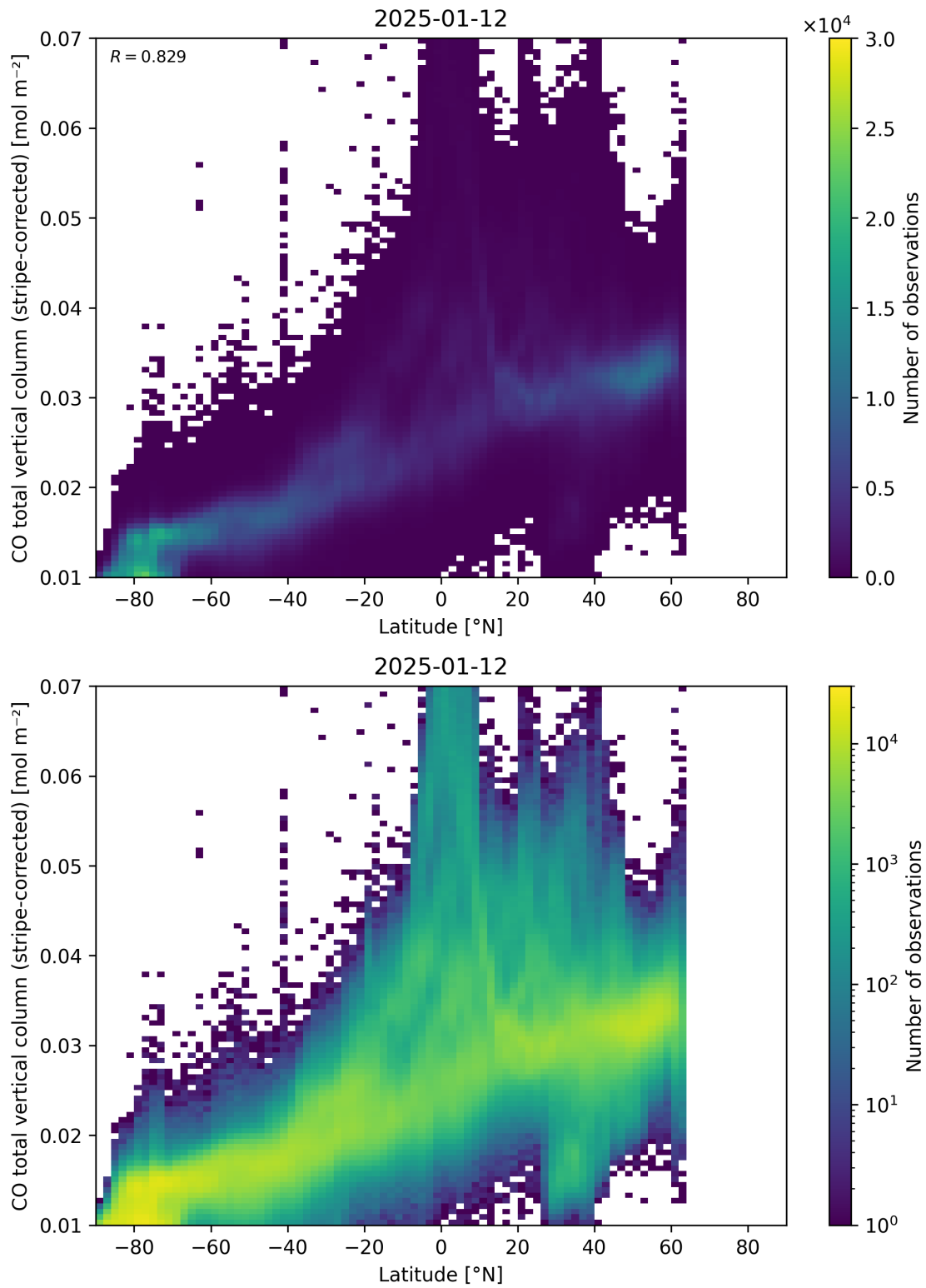
Figure 52: Scatter density plot of “Latitude” against “CO total vertical column (stripe-corrected)” for 2025-01-12 to 2025-01-13.
