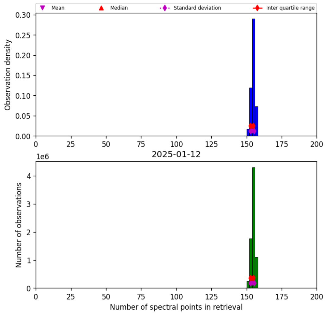
Figure 21: Histogram of “Number of spectral points in retrieval” for 2025-01-12 to 2025-01-13
