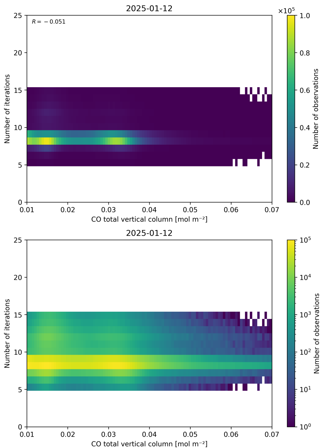
Figure 42: Scatter density plot of “CO total vertical column” against “Number of iterations” for 2025-01-12 to 2025-01-13.
