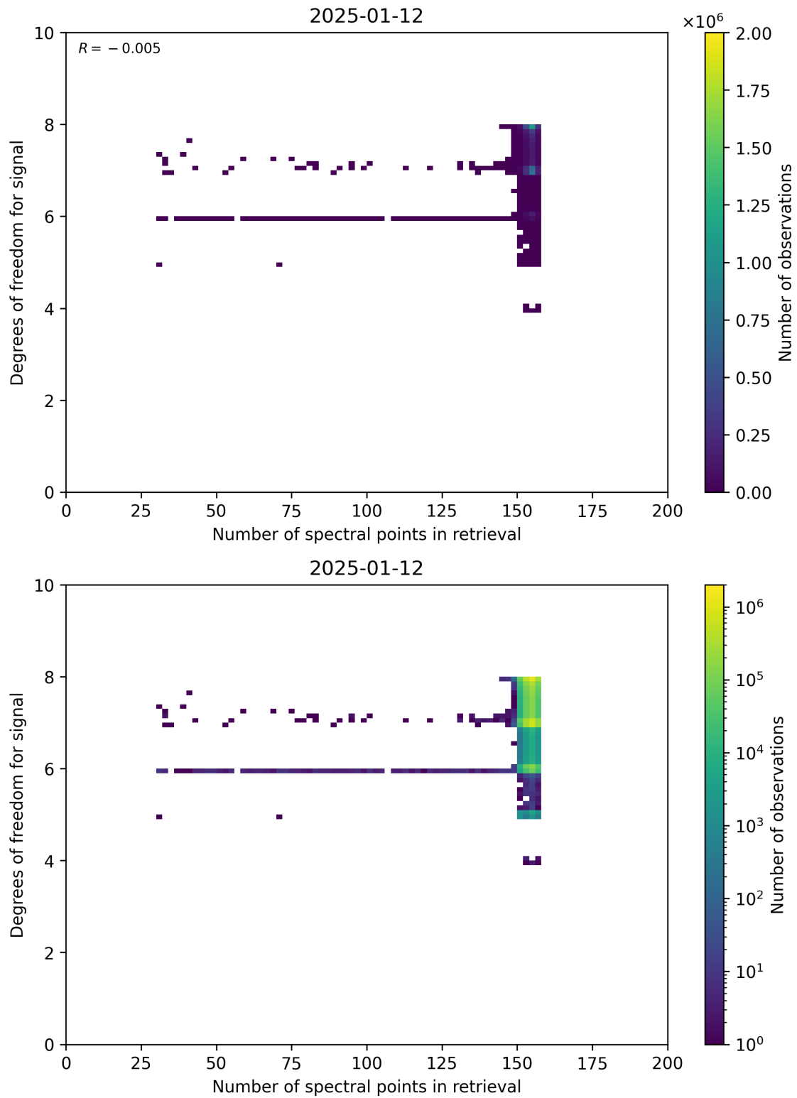
Figure 59: Scatter density plot of “Number of spectral points in retrieval” against “Degrees of freedom for signal” for 2025-01-12 to 2025-01-13.
