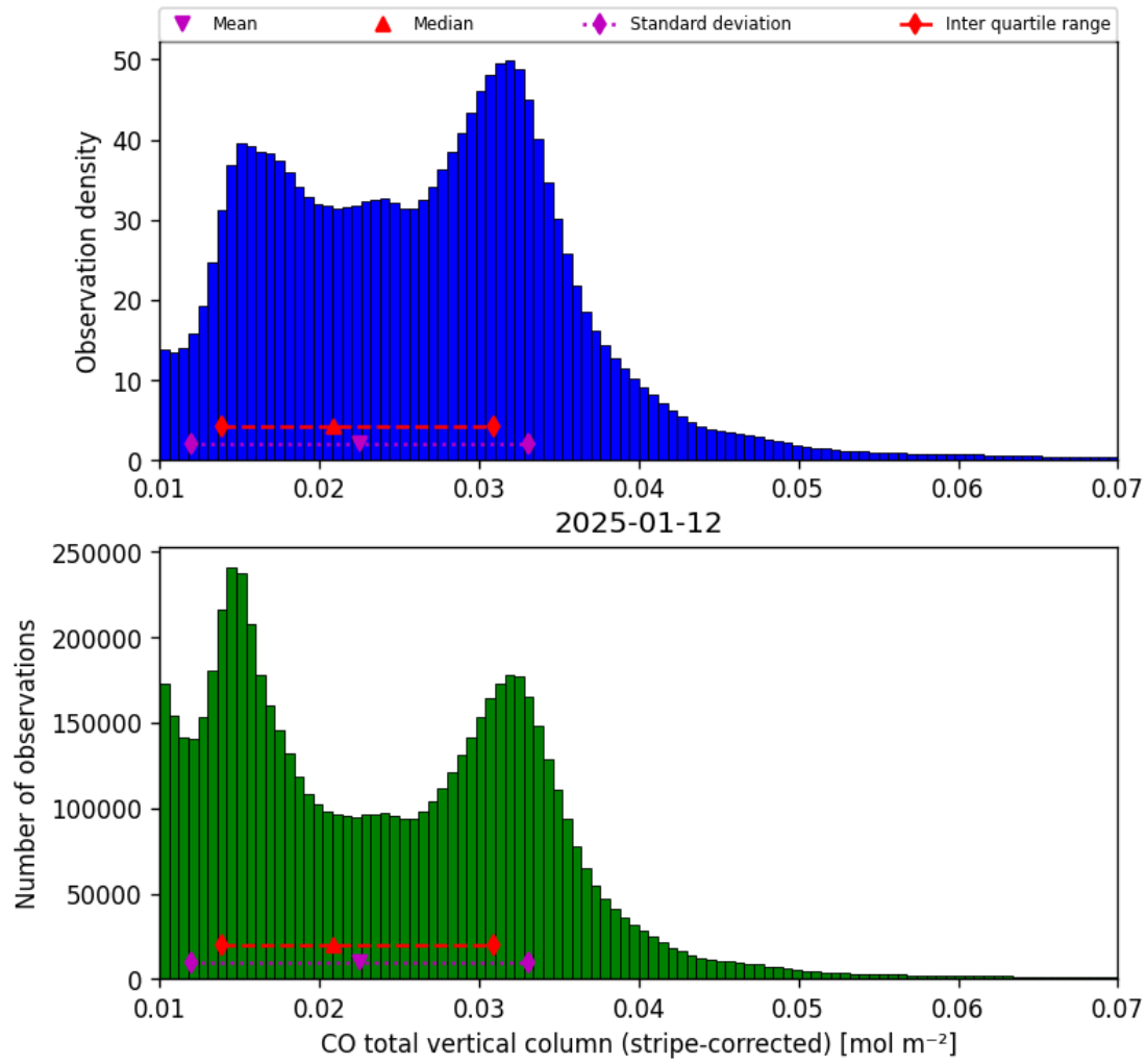
Figure 19: Histogram of “CO total vertical column (stripe-corrected)” for 2025-01-12 to 2025-01-13
