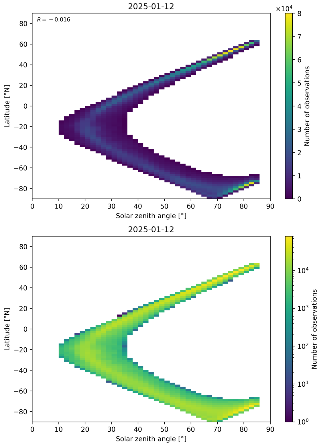
Figure 66: Scatter density plot of “Solar zenith angle” against “Latitude” for 2025-01-12 to 2025-01-13.
