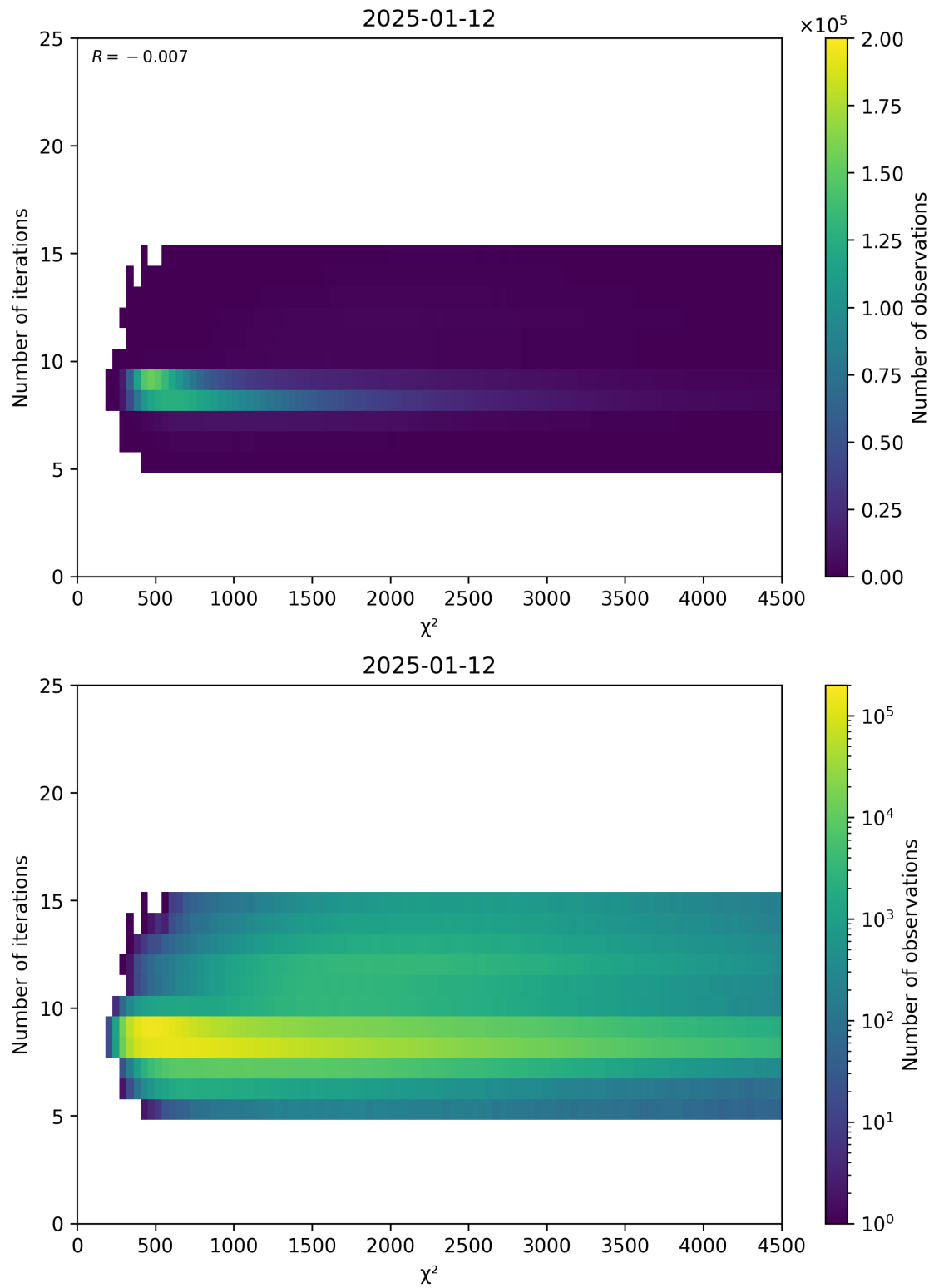
Figure 49: Scatter density plot of “ \chi^2 ” against “Number of iterations” for 2025-01-12 to 2025-01-13.
