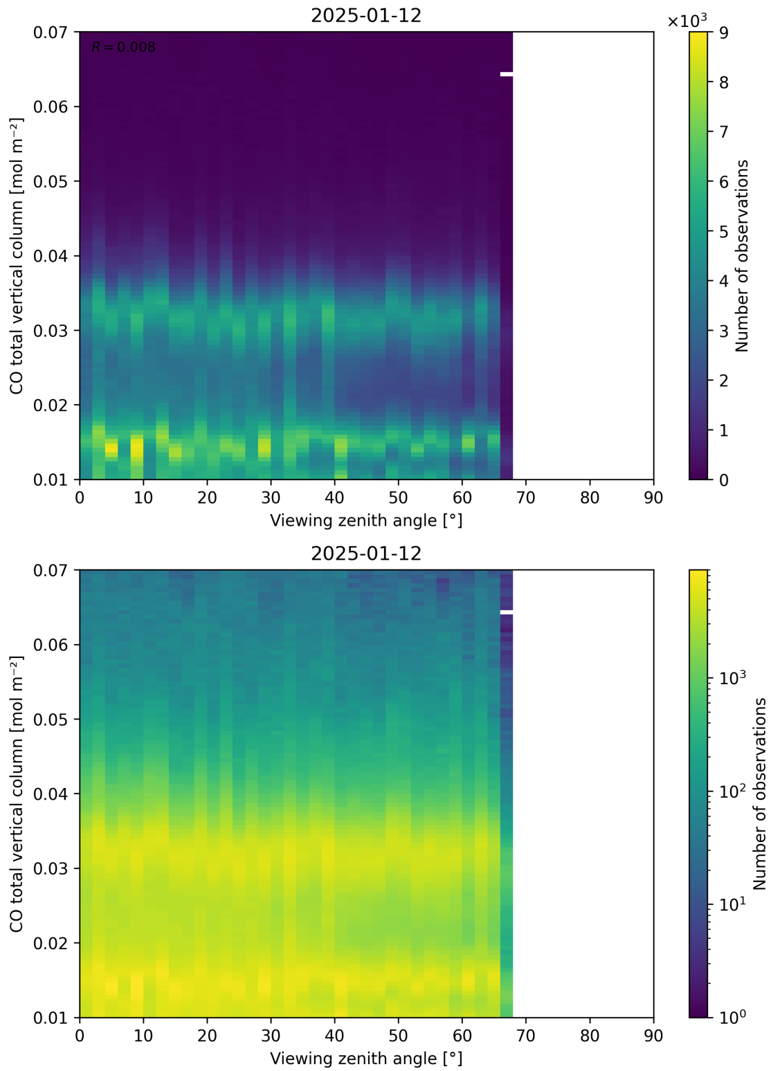
Figure 69: Scatter density plot of “Viewing zenith angle” against “CO total vertical column” for 2025-01-12 to 2025-01-13.
