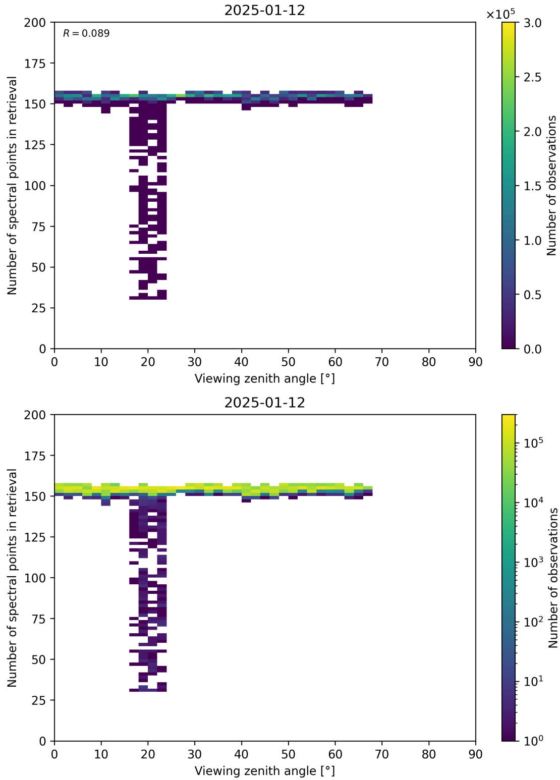
Figure 76: Scatter density plot of “Viewing zenith angle” against “Number of spectral points in retrieval” for 2025-01-12 to 2025-01-13.
