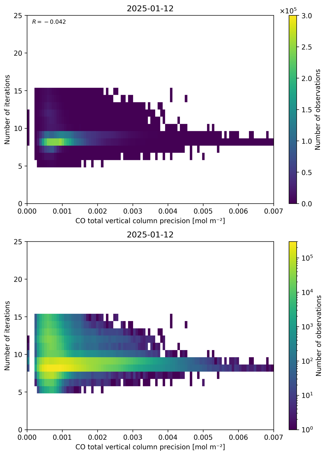
Figure 46: Scatter density plot of “CO total vertical column precision” against “Number of iterations” for 2025-01-12 to 2025-01-13.
