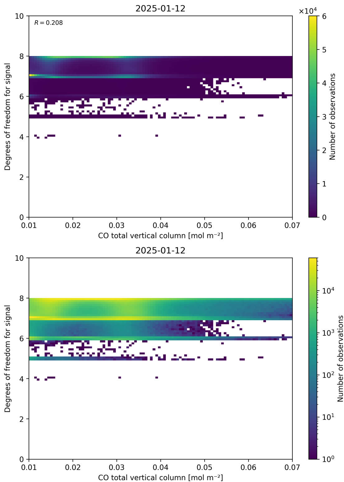
Figure 41: Scatter density plot of “CO total vertical column” against “Degrees of freedom for signal” for 2025-01-12 to 2025-01-13.
