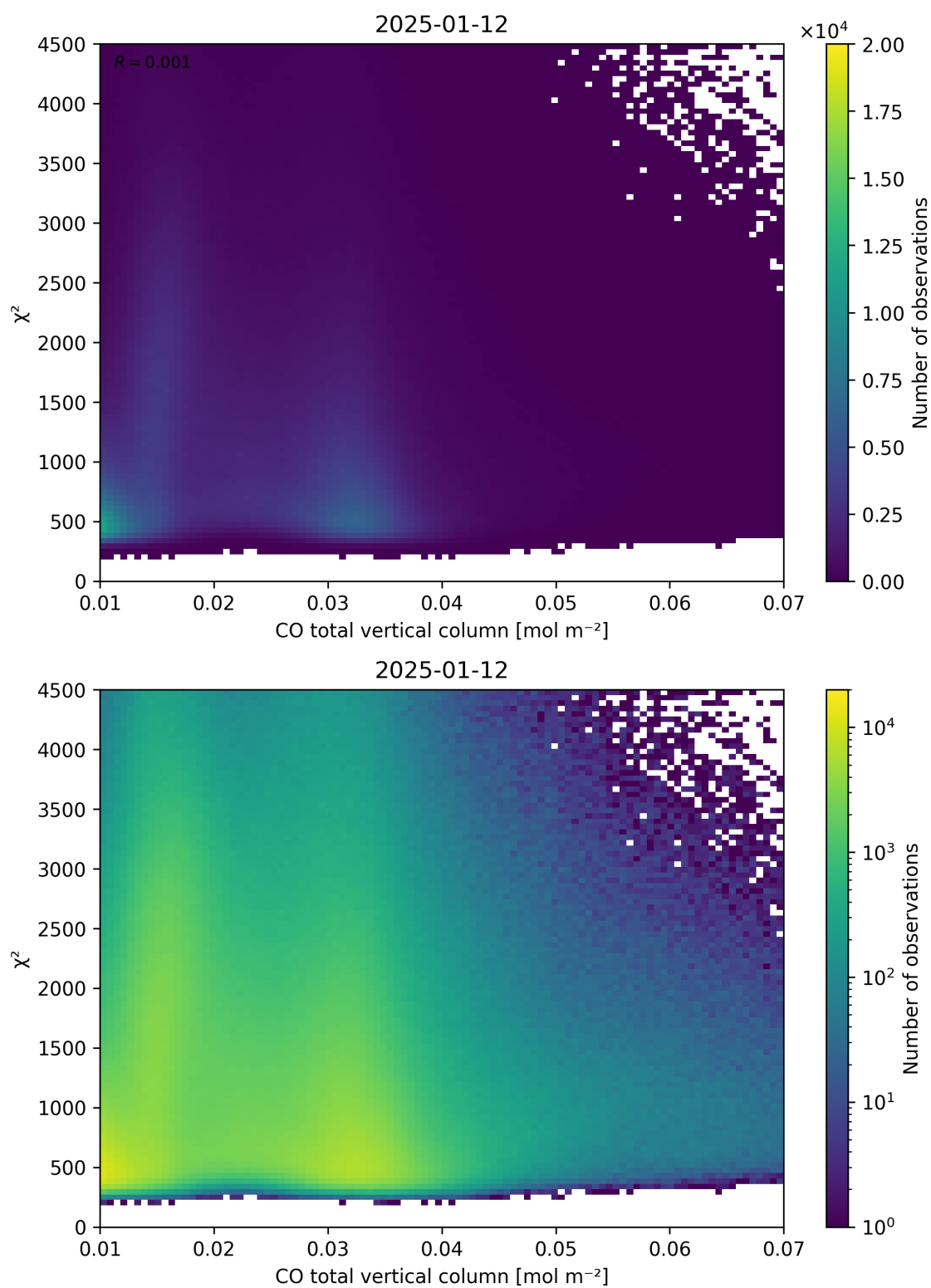
Figure 35: Scatter density plot of “CO total vertical column” against “ \chi^2 ” for 2025-01-12 to 2025-01-13.
