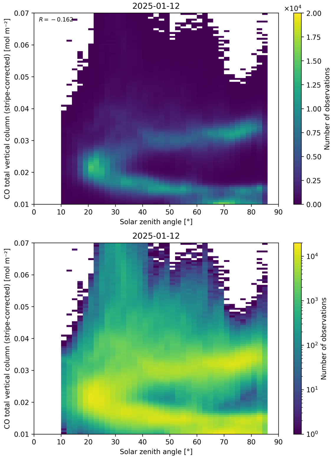
Figure 62: Scatter density plot of “Solar zenith angle” against “CO total vertical column (stripe-corrected)” for 2025-01-12 to 2025-01-13.
