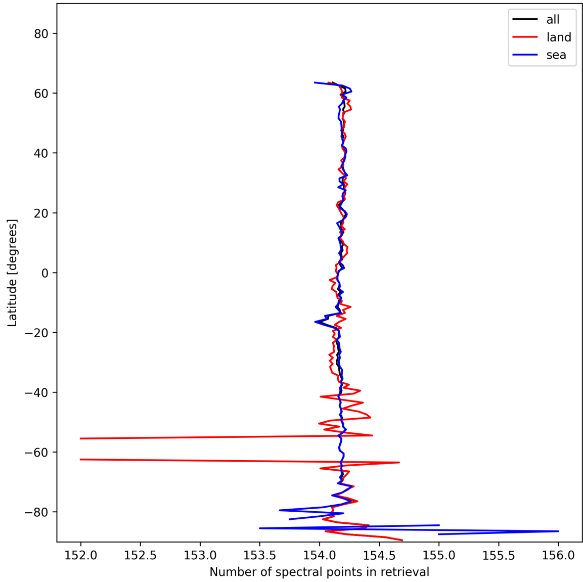
Figure 13: Zonal average of “Number of spectral points in retrieval” for 2025-01-12 to 2025-01-13.
