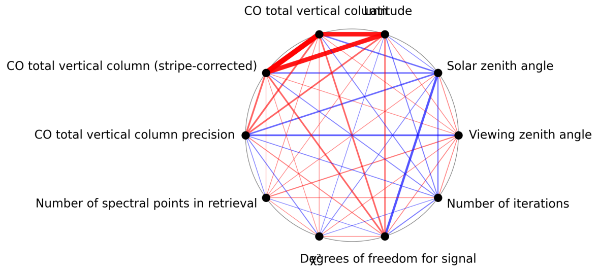
Figure 1: Map of correlation graph for 2025-01-12 to 2025-01-13.
