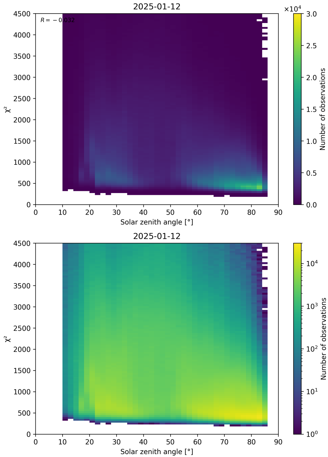
Figure 64: Scatter density plot of “Solar zenith angle” against “ \chi^2 ” for 2025-01-12 to 2025-01-13.
