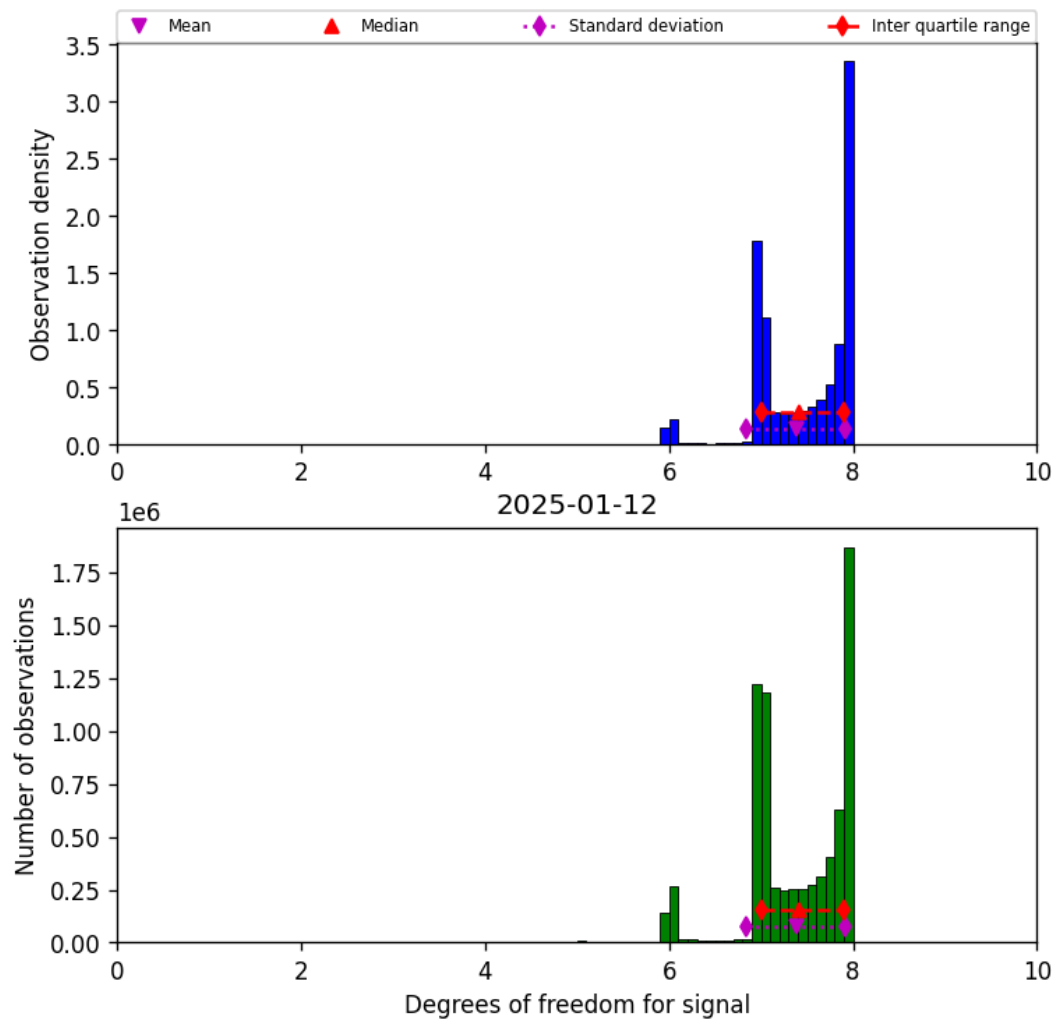
Figure 23: Histogram of “Degrees of freedom for signal” for 2025-01-12 to 2025-01-13
