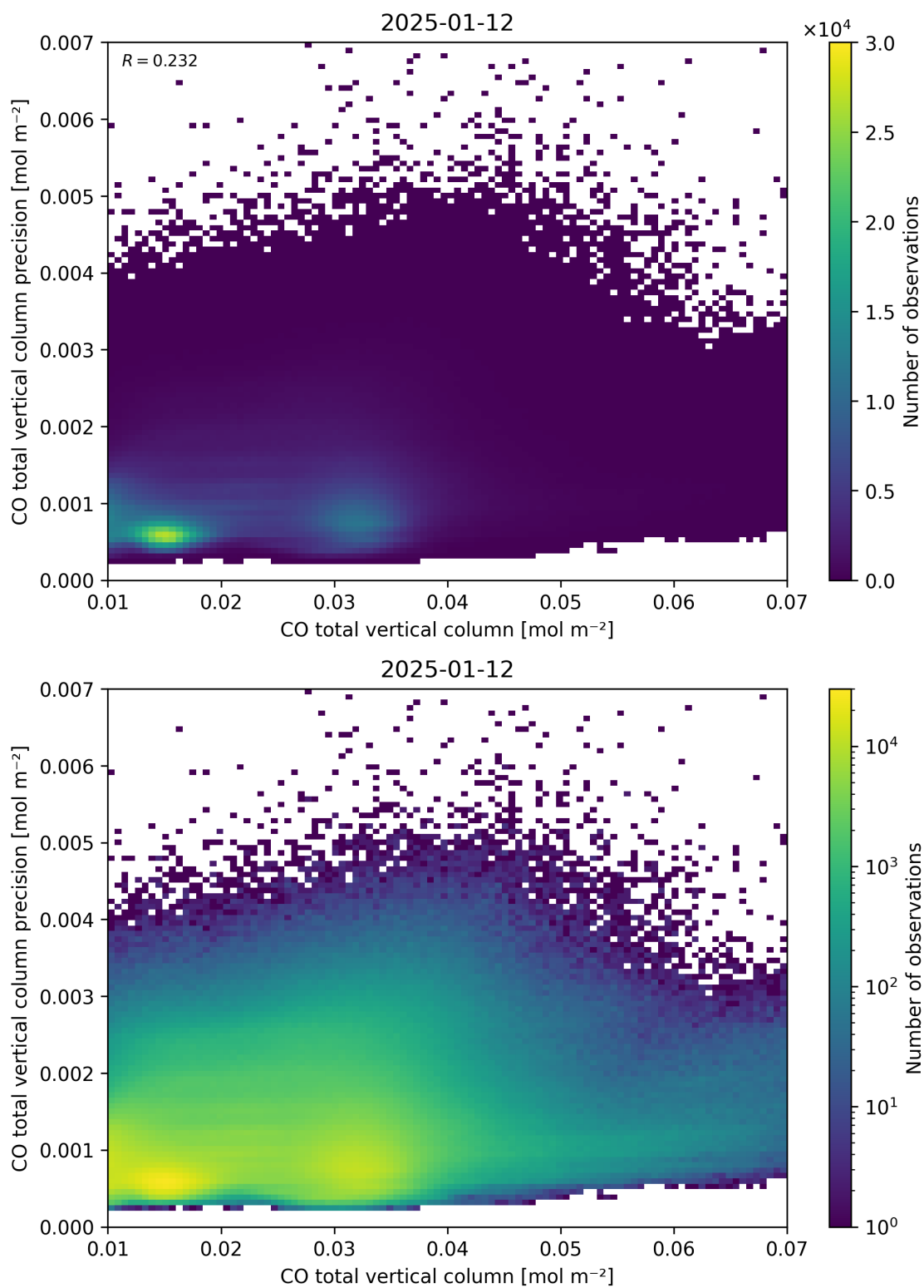
Figure 34: Scatter density plot of “CO total vertical column” against “CO total vertical column precision” for 2025-01-12 to 2025-01-13.
