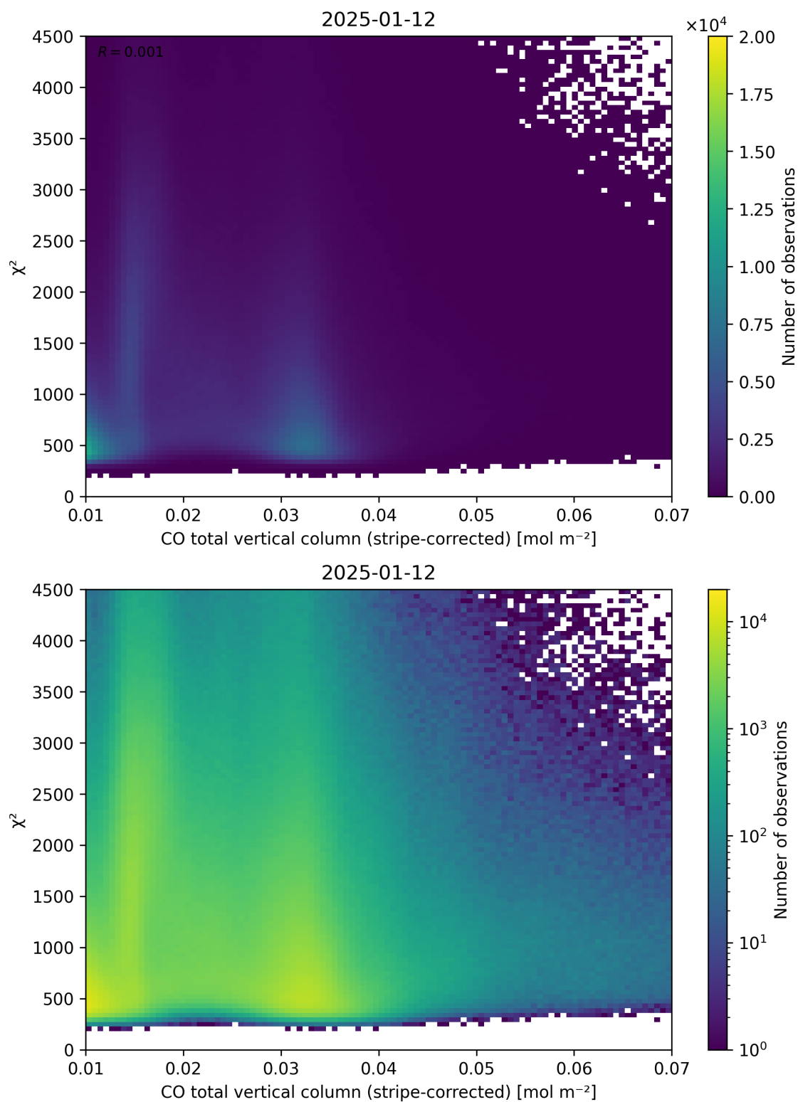
Figure 37: Scatter density plot of “CO total vertical column (stripe-corrected)” against “ \chi^2 ” for 2025-01-12 to 2025-01-13.
