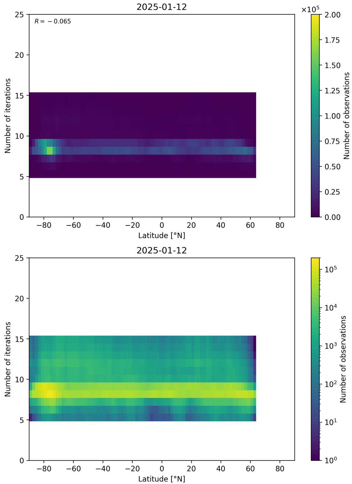
Figure 56: Scatter density plot of “Latitude” against “Number of iterations” for 2025-01-12 to 2025-01-13.
