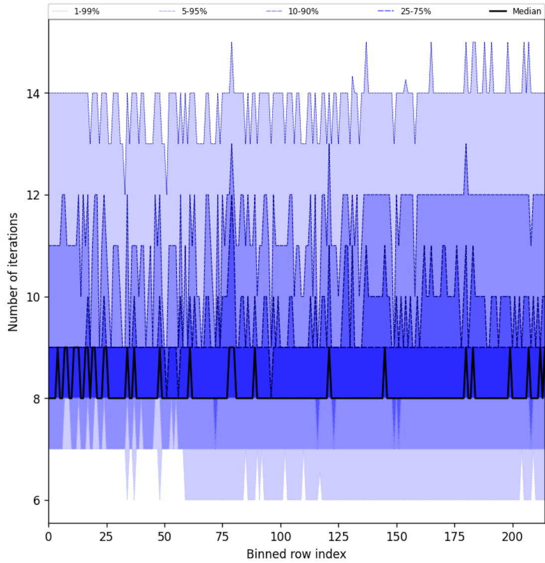
Figure 32: Along track statistics of “Number of iterations” for 2025-01-12 to 2025-01-13
