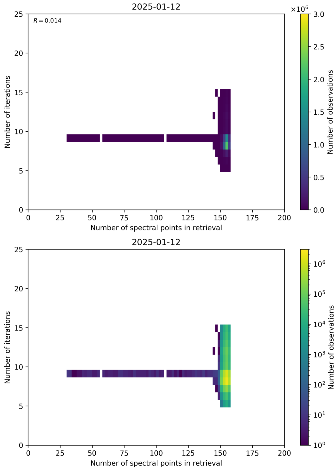
Figure 60: Scatter density plot of “Number of spectral points in retrieval” against “Number of iterations” for 2025-01-12 to 2025-01-13.
