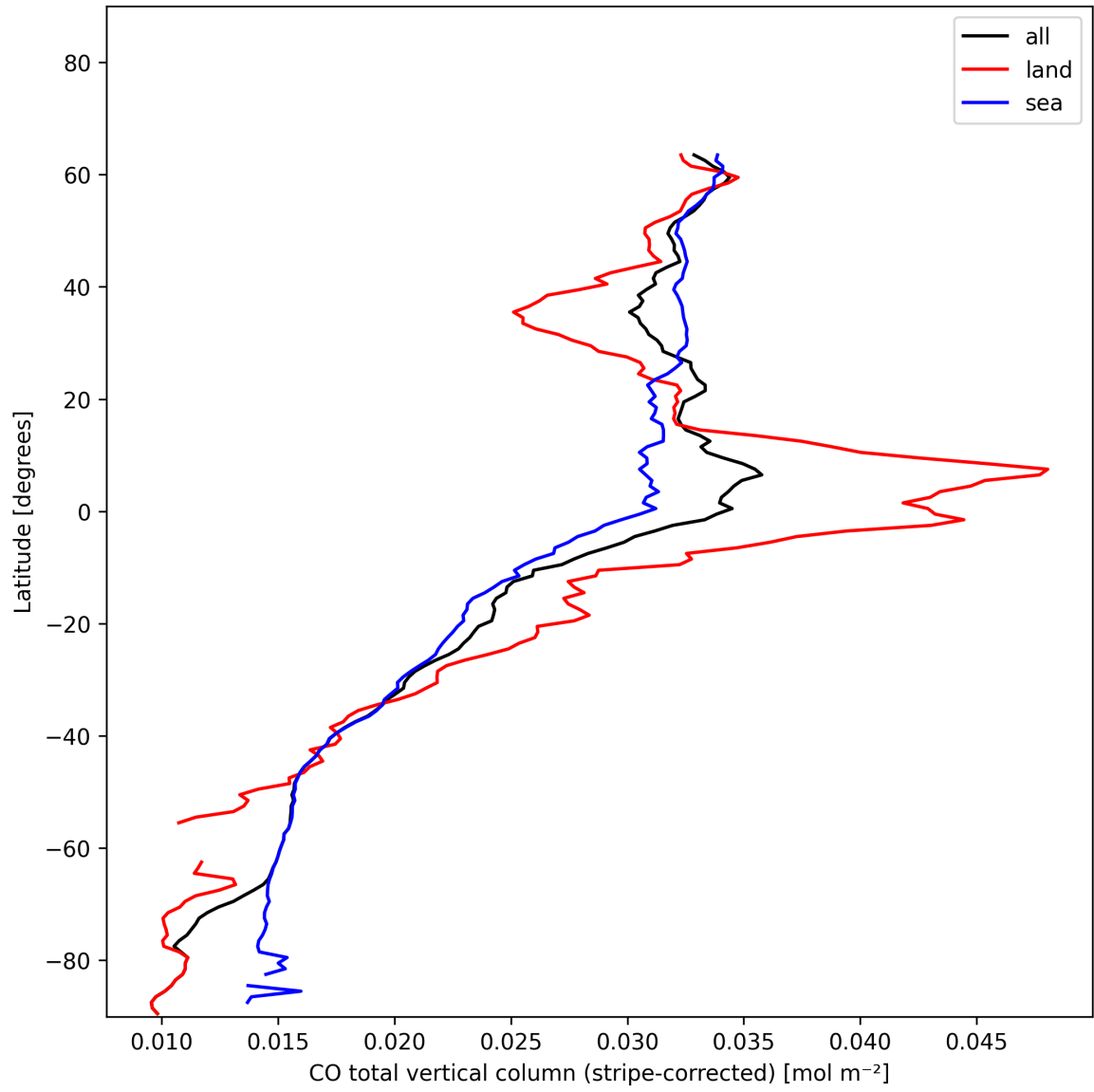
Figure 11: Zonal average of “CO total vertical column (stripe-corrected)” for 2025-01-12 to 2025-01-13.
