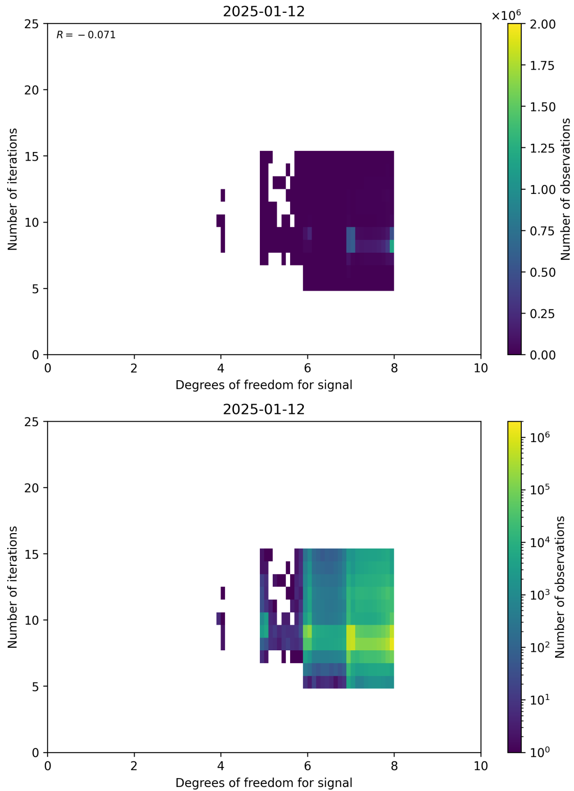
Figure 50: Scatter density plot of “Degrees of freedom for signal” against “Number of iterations” for 2025-01-12 to 2025-01-13.
