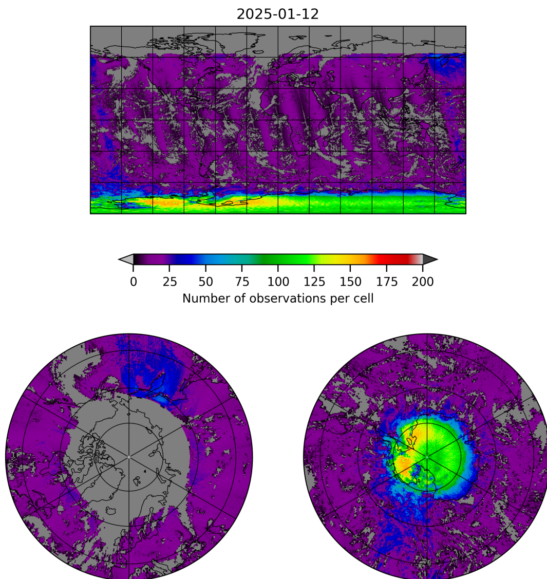
Figure 8: Map of the number of observations for 2025-01-12 to 2025-01-13
