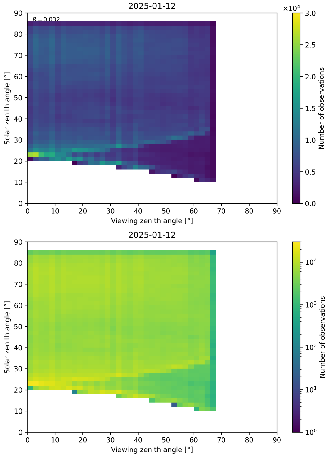
Figure 77: Scatter density plot of “Viewing zenith angle” against “Solar zenith angle” for 2025-01-12 to 2025-01-13.
