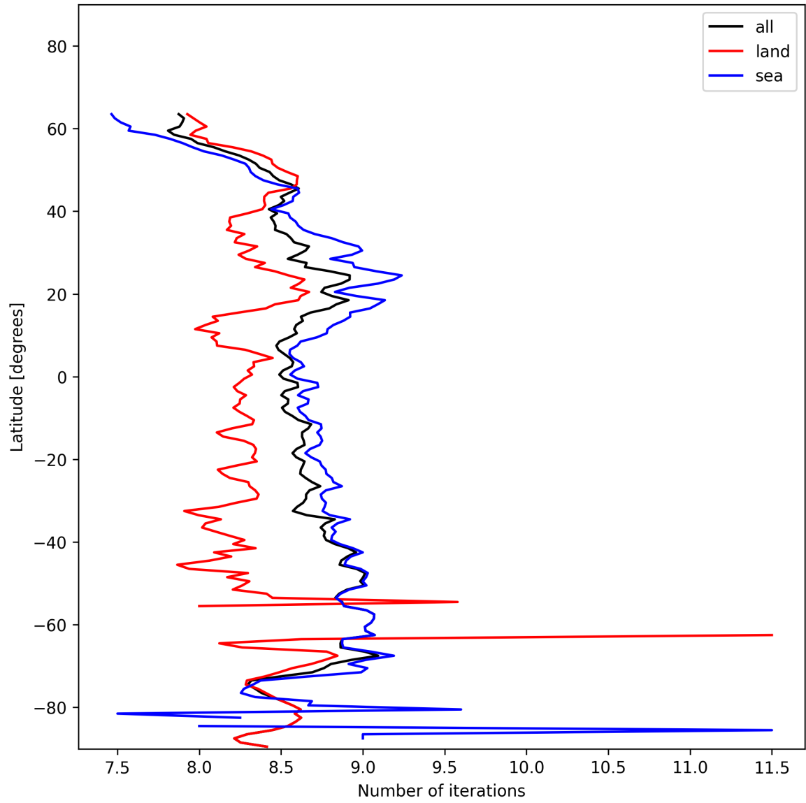
Figure 16: Zonal average of “Number of iterations” for 2025-01-12 to 2025-01-13.
