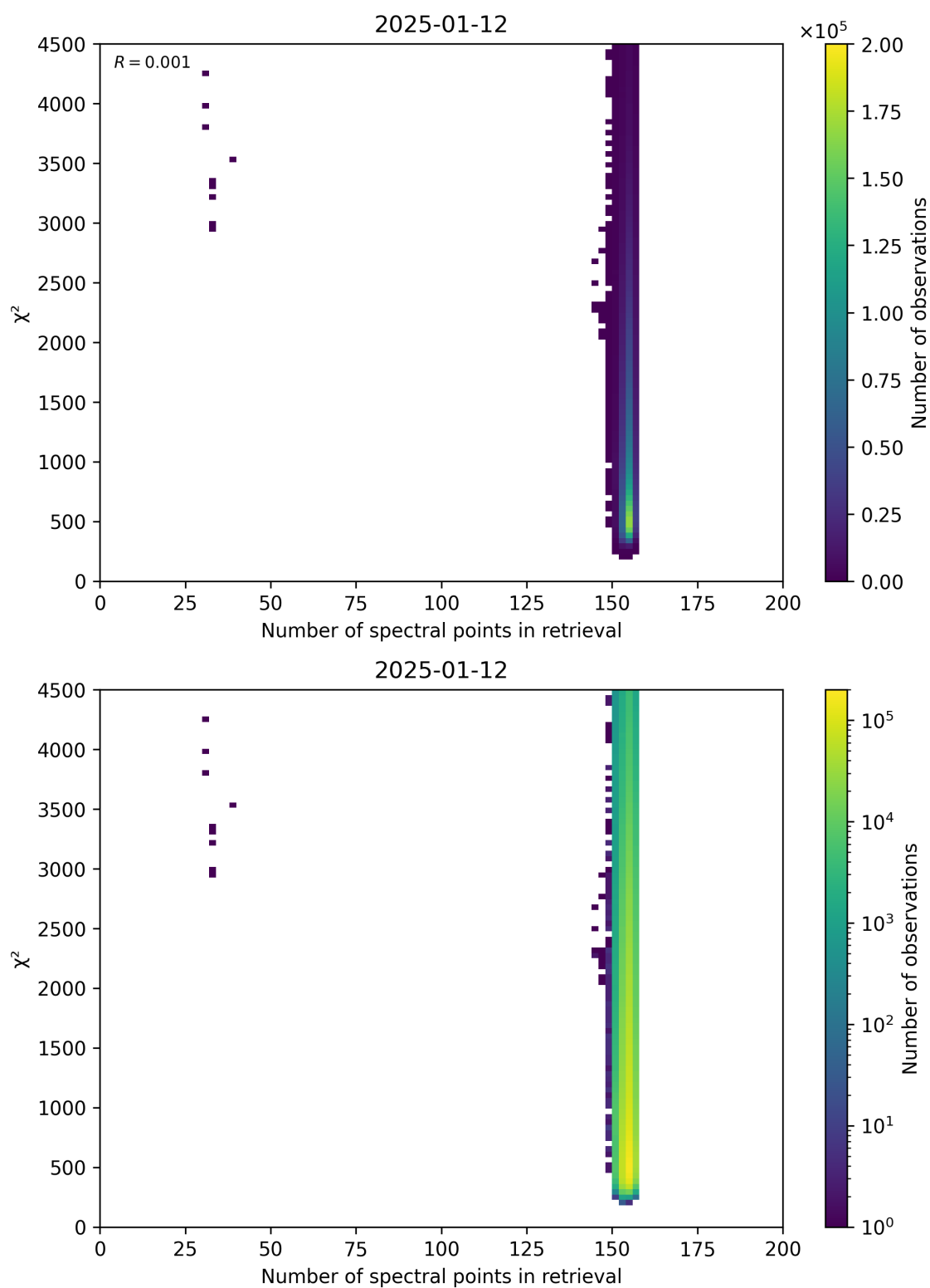
Figure 58: Scatter density plot of “Number of spectral points in retrieval” against “ \chi^2 ” for 2025-01-12 to 2025-01-13.
