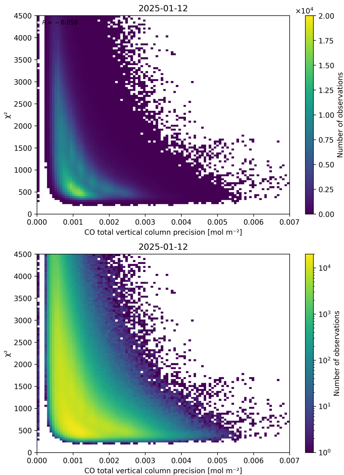
Figure 44: Scatter density plot of “CO total vertical column precision” against “ \chi^2 ” for 2025-01-12 to 2025-01-13.
