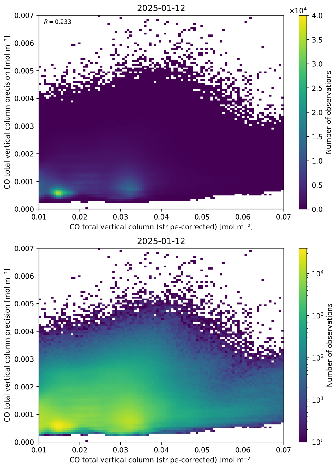
Figure 36: Scatter density plot of “CO total vertical column (stripe-corrected)” against “CO total vertical column precision” for 2025-01-12 to 2025-01-13.
