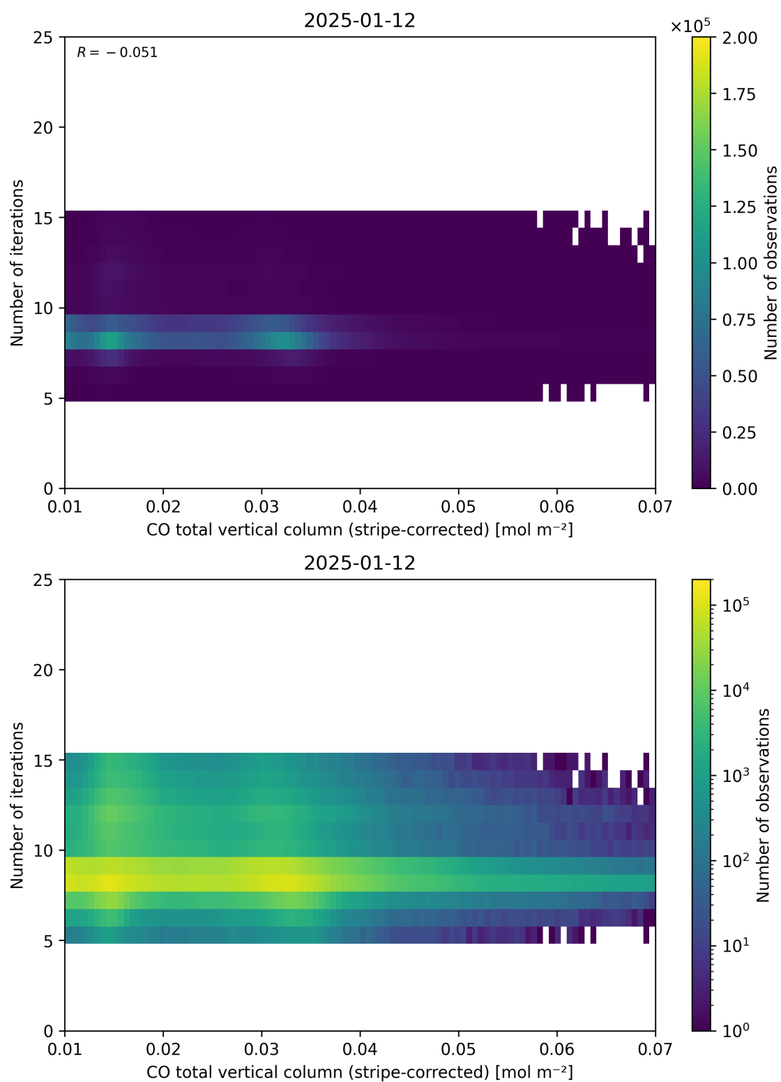
Figure 39: Scatter density plot of “CO total vertical column (stripe-corrected)” against “Number of iterations” for 2025-01-12 to 2025-01-13.
