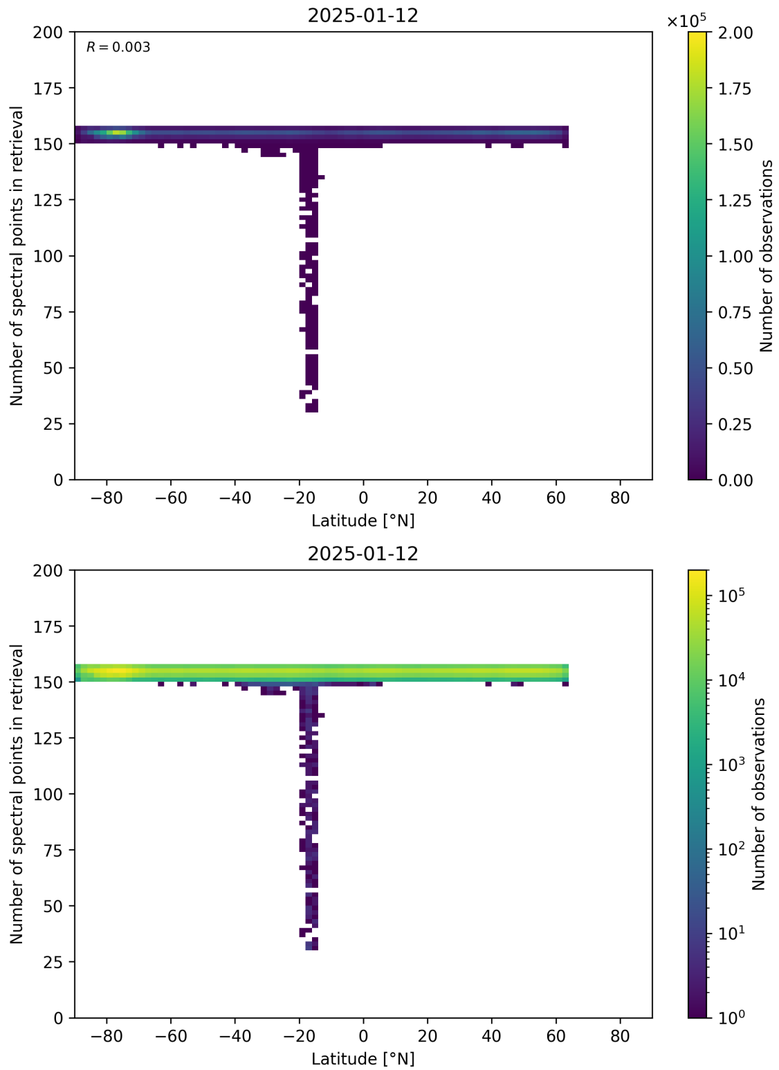
Figure 57: Scatter density plot of “Latitude” against “Number of spectral points in retrieval” for 2025-01-12 to 2025-01-13.
