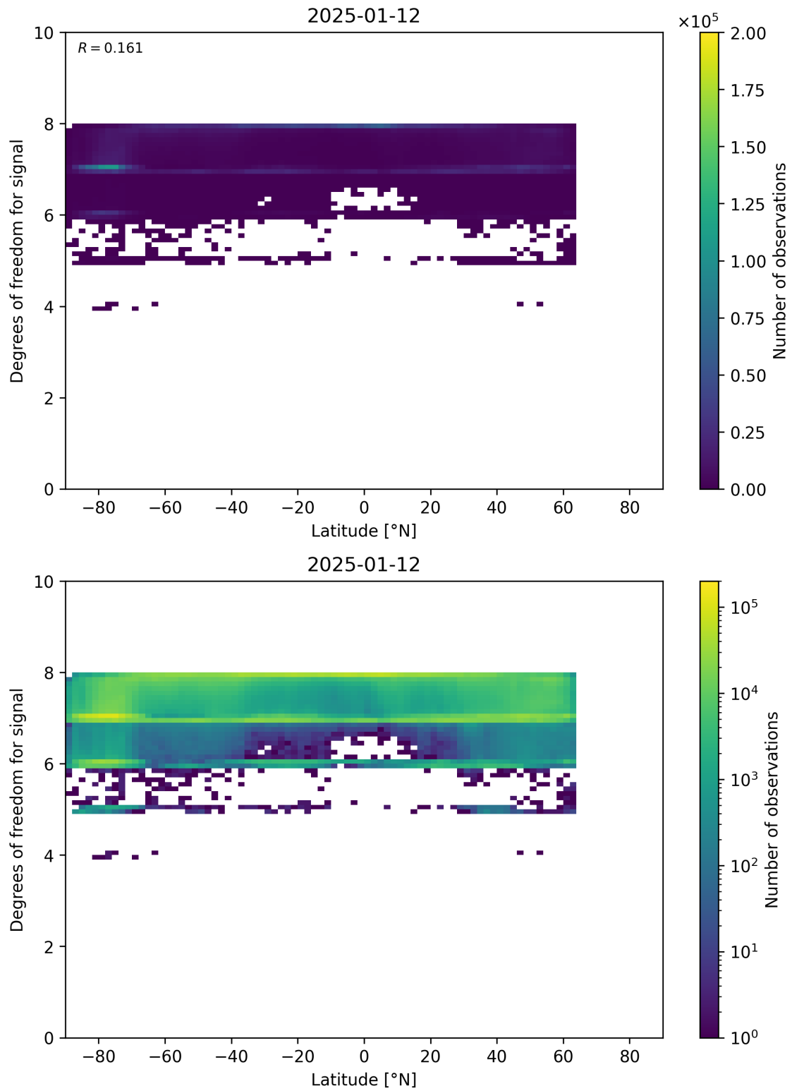
Figure 55: Scatter density plot of “Latitude” against “Degrees of freedom for signal” for 2025-01-12 to 2025-01-13.
