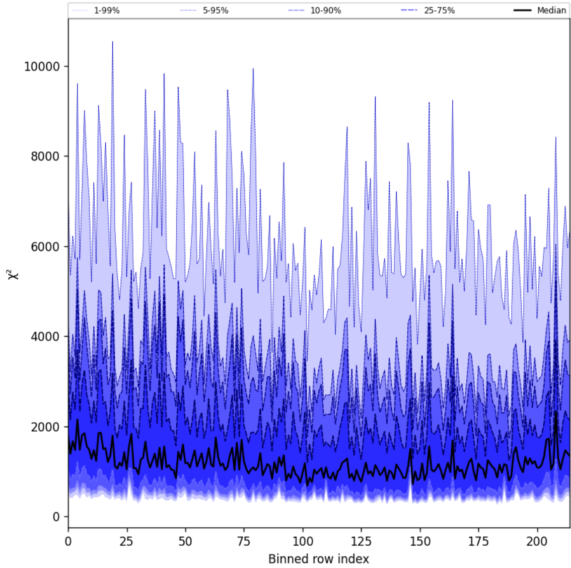
Figure 30: Along track statistics of “ \chi^2 ” for 2025-01-12 to 2025-01-13
