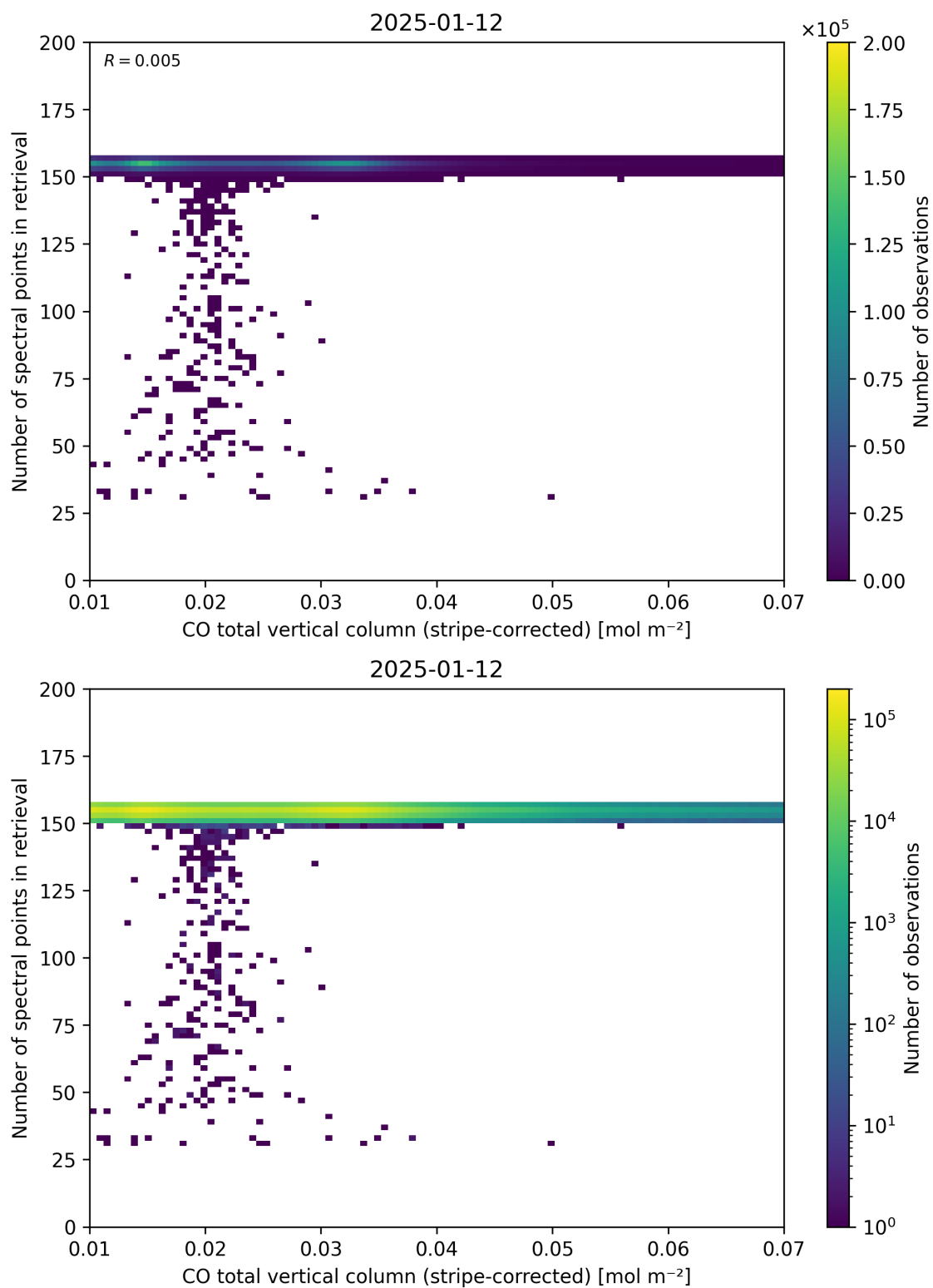
Figure 40: Scatter density plot of “CO total vertical column (stripe-corrected)” against “Number of spectral points in retrieval” for 2025-01-12 to 2025-01-13.
