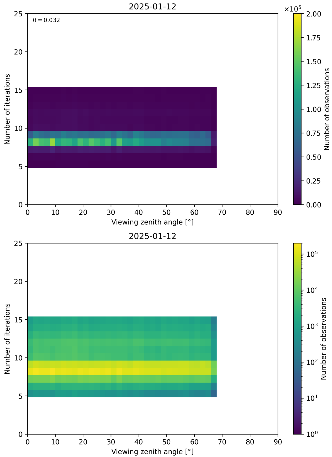
Figure 75: Scatter density plot of “Viewing zenith angle” against “Number of iterations” for 2025-01-12 to 2025-01-13.
