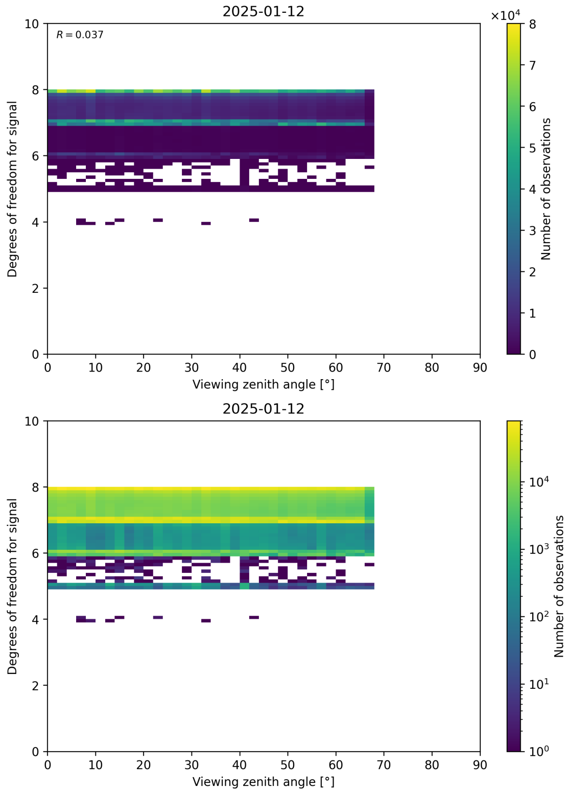
Figure 73: Scatter density plot of “Viewing zenith angle” against “Degrees of freedom for signal” for 2025-01-12 to 2025-01-13.
