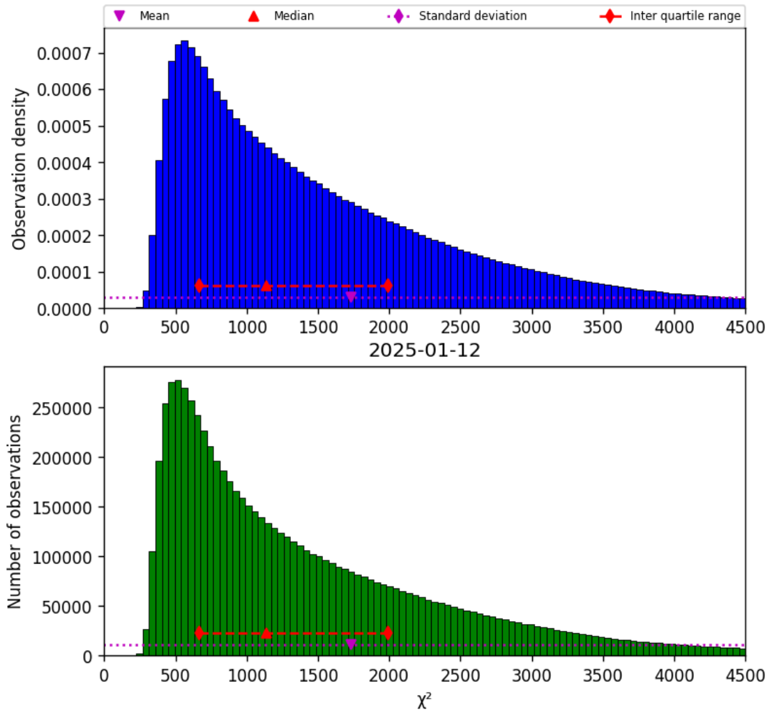
Figure 22: Histogram of “ \chi^2 ” for 2025-01-12 to 2025-01-13
