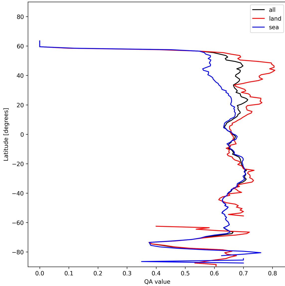
Figure 9: Zonal average of “QA value” for 2025-01-12 to 2025-01-13.
