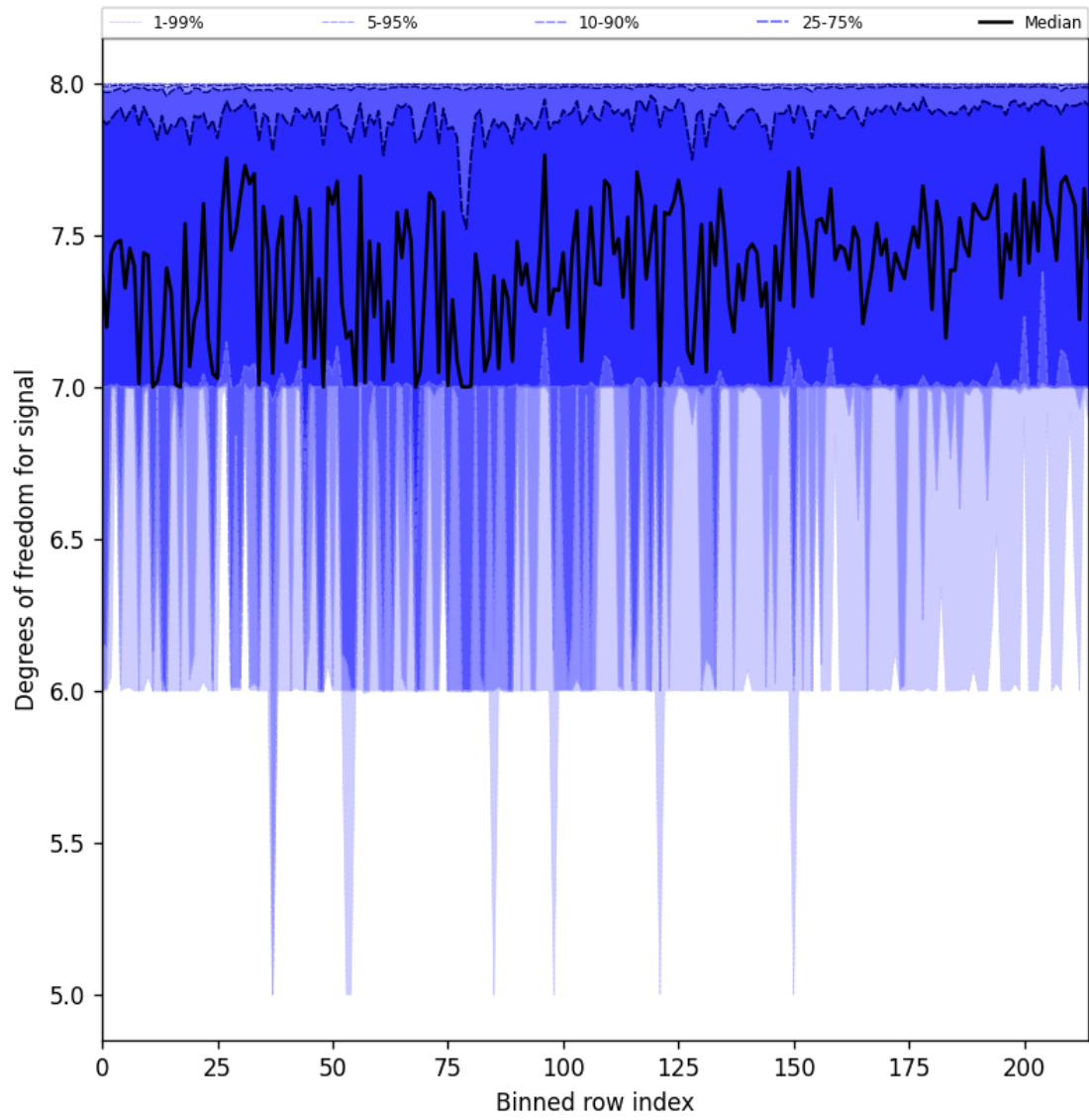
Figure 31: Along track statistics of “Degrees of freedom for signal” for 2025-01-12 to 2025-01-13
