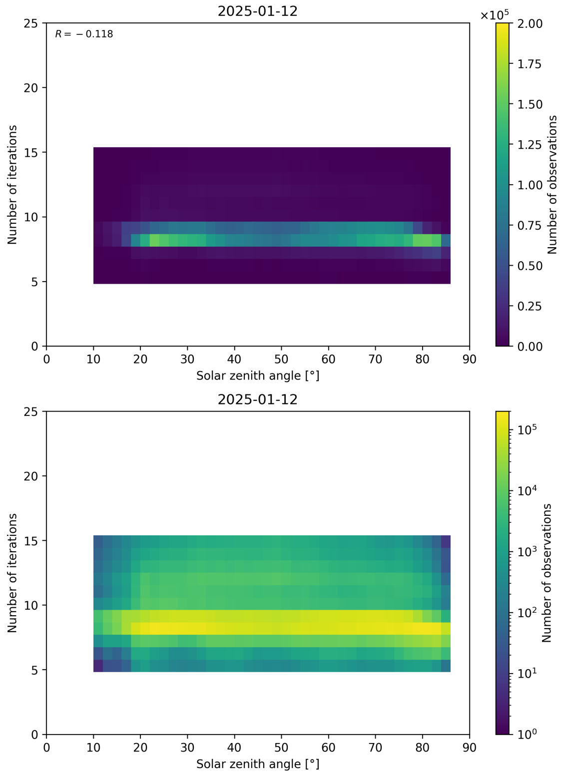
Figure 67: Scatter density plot of “Solar zenith angle” against “Number of iterations” for 2025-01-12 to 2025-01-13.
