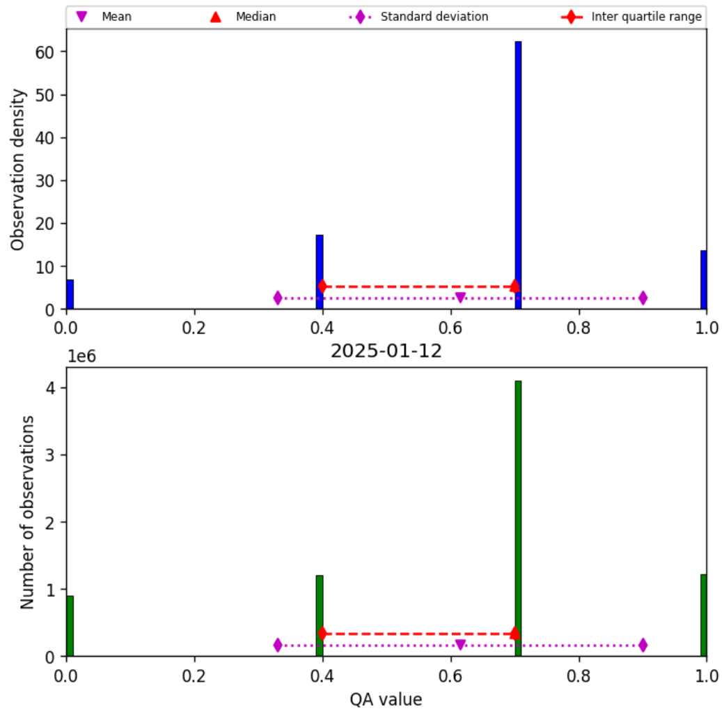
Figure 17: Histogram of “QA value” for 2025-01-12 to 2025-01-13
