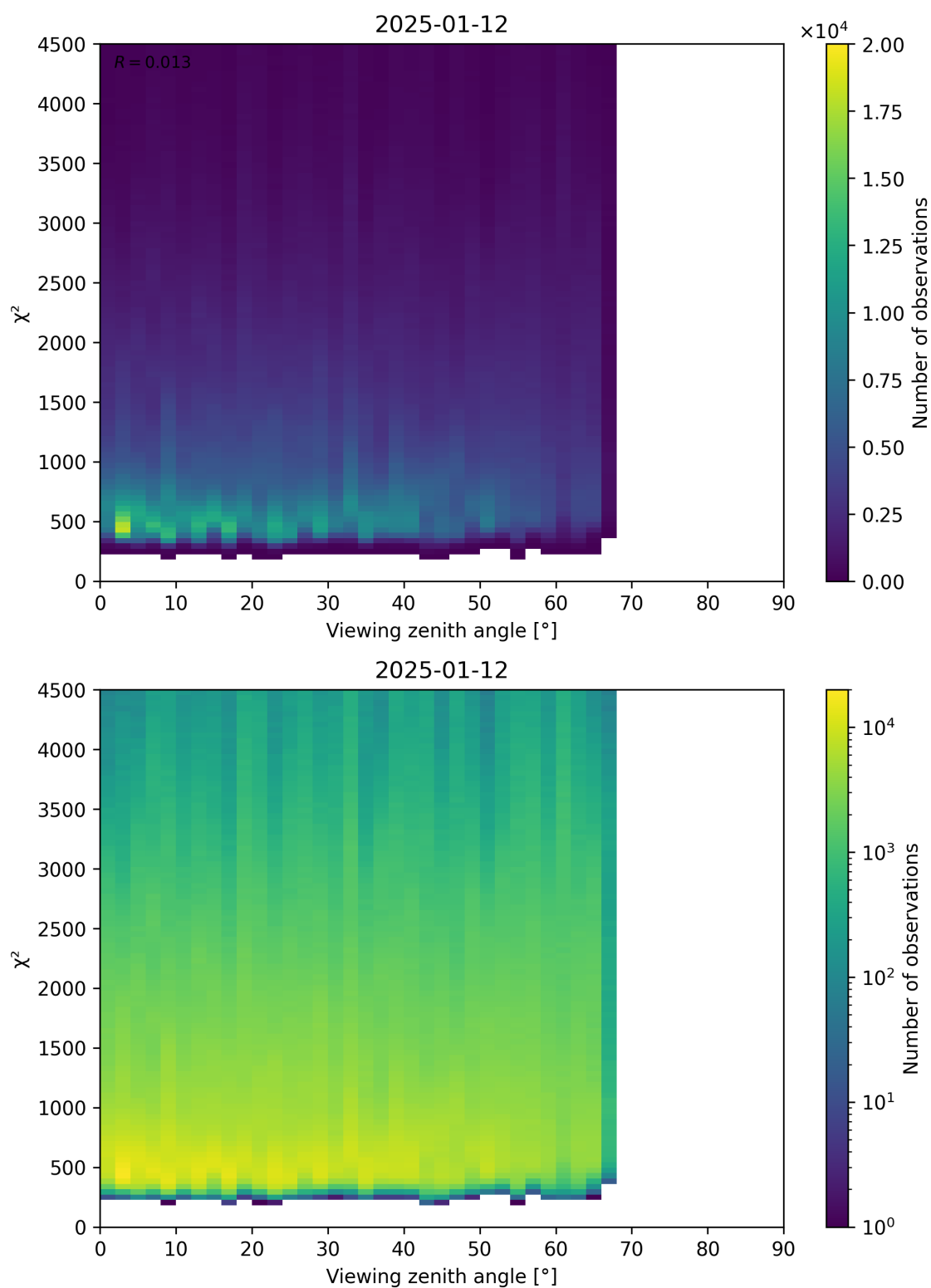
Figure 72: Scatter density plot of “Viewing zenith angle” against “ \chi^2 ” for 2025-01-12 to 2025-01-13.
