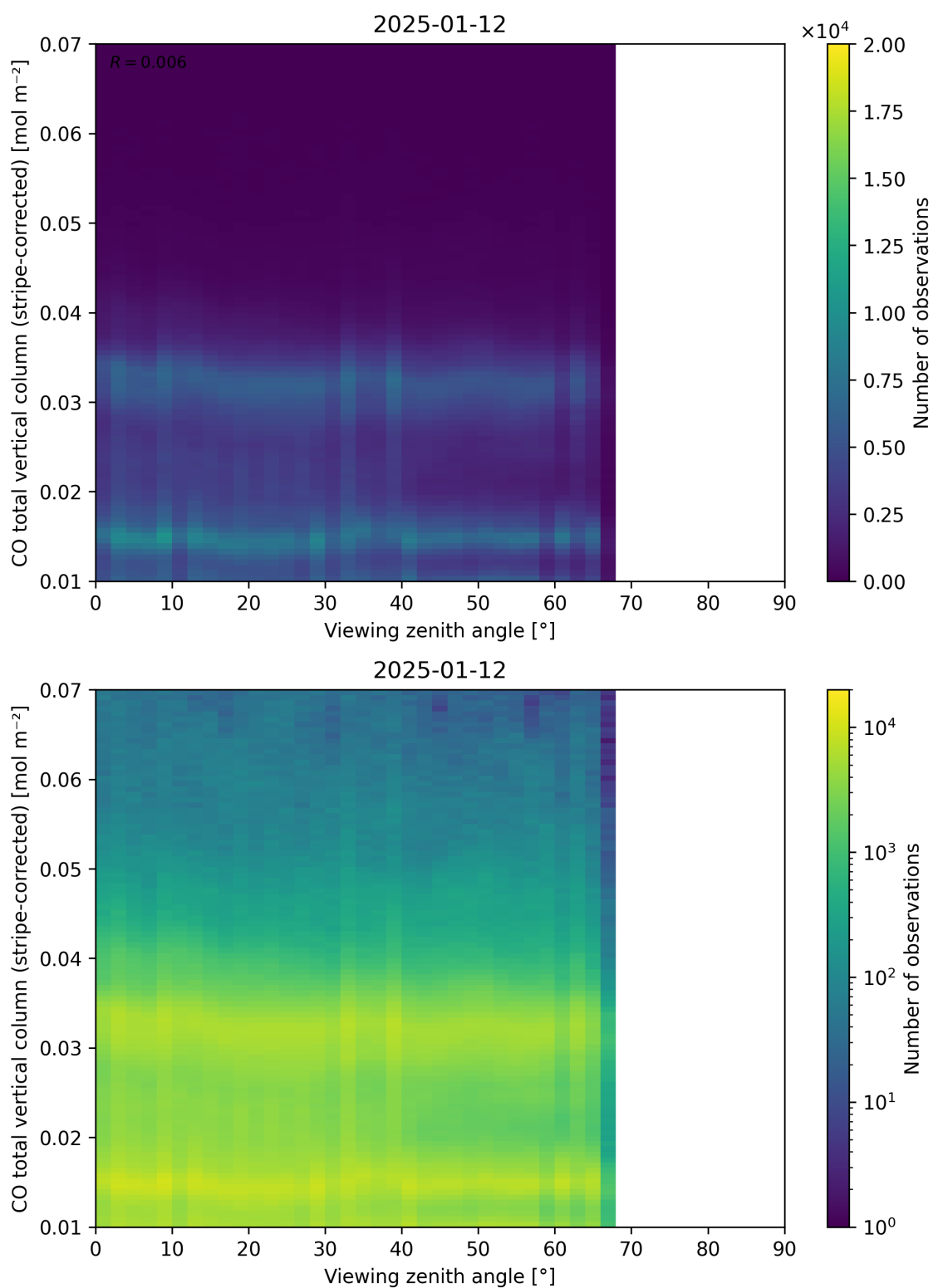
Figure 70: Scatter density plot of “Viewing zenith angle” against “CO total vertical column (stripe-corrected)” for 2025-01-12 to 2025-01-13.
