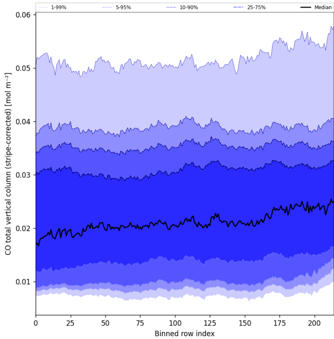
Figure 27: Along track statistics of “CO total vertical column (stripe-corrected)” for 2025-01-12 to 2025-01-13
