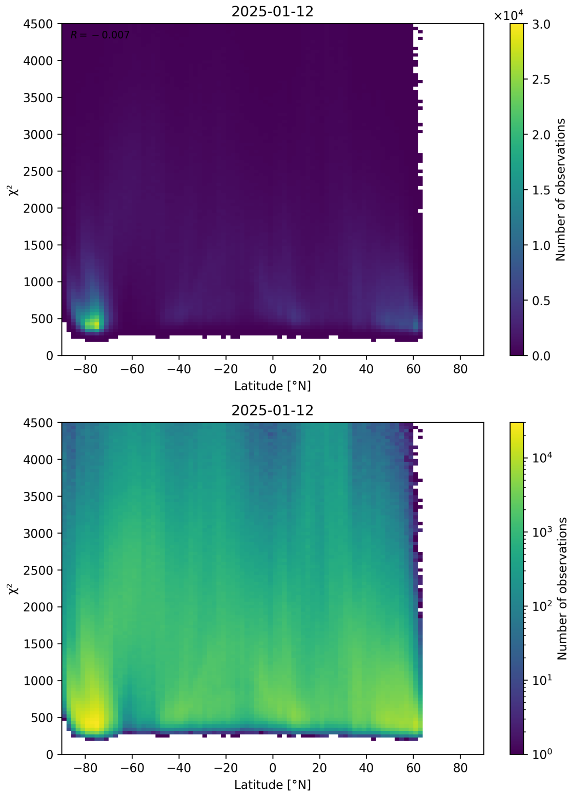
Figure 54: Scatter density plot of “Latitude” against “ \chi^2 ” for 2025-01-12 to 2025-01-13.
