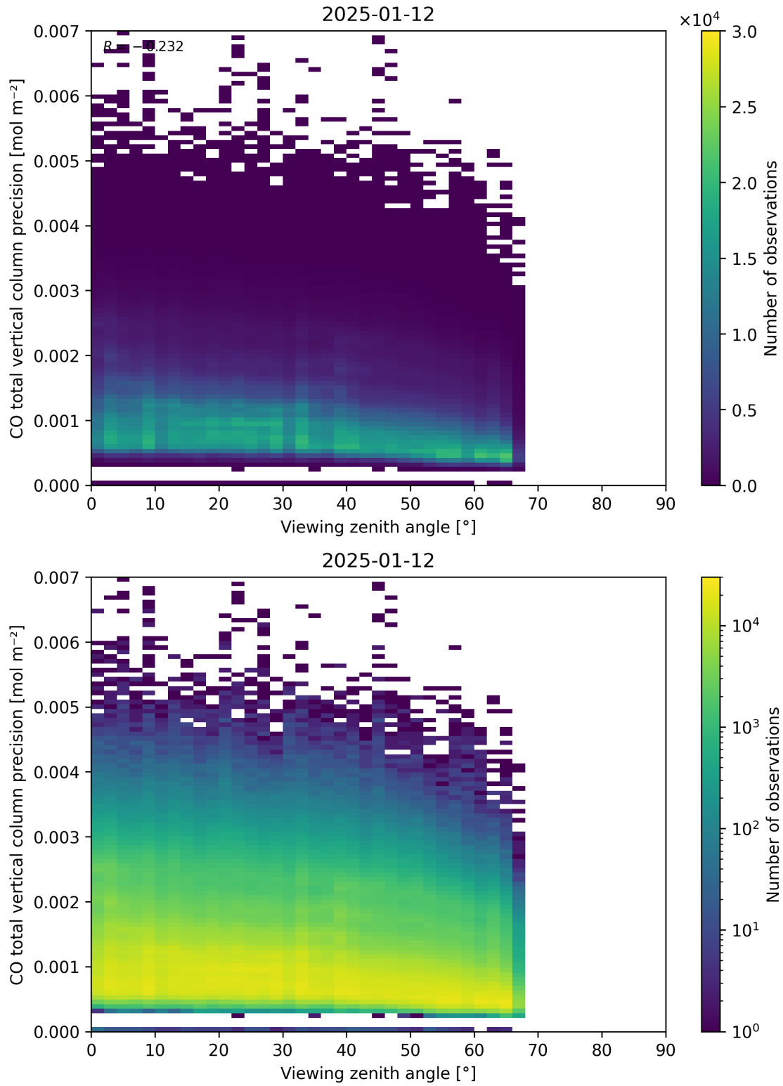
Figure 71: Scatter density plot of “Viewing zenith angle” against “CO total vertical column precision” for 2025-01-12 to 2025-01-13.
