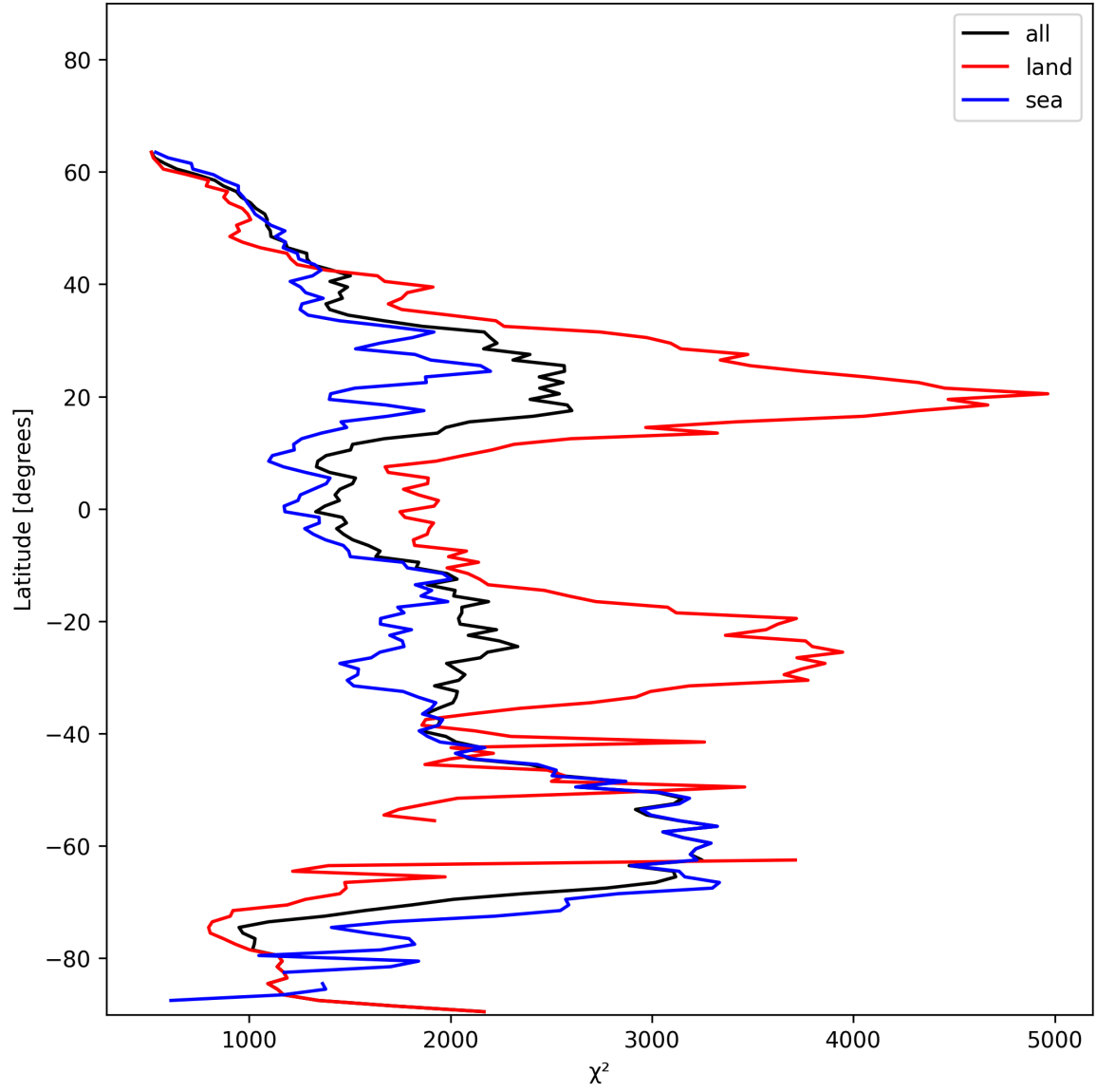
Figure 14: Zonal average of “ \chi^2 ” for 2025-01-12 to 2025-01-13.
