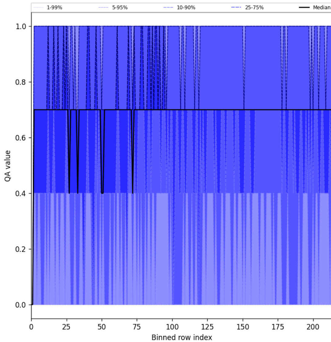
Figure 25: Along track statistics of “QA value” for 2025-01-12 to 2025-01-13
