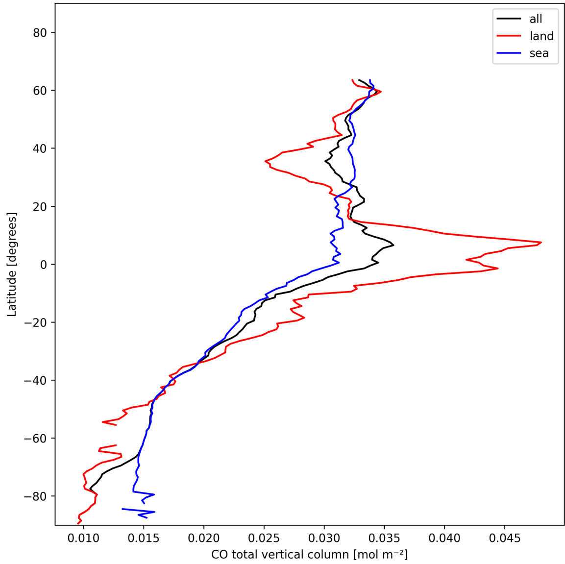
Figure 10: Zonal average of “CO total vertical column” for 2025-01-12 to 2025-01-13.
