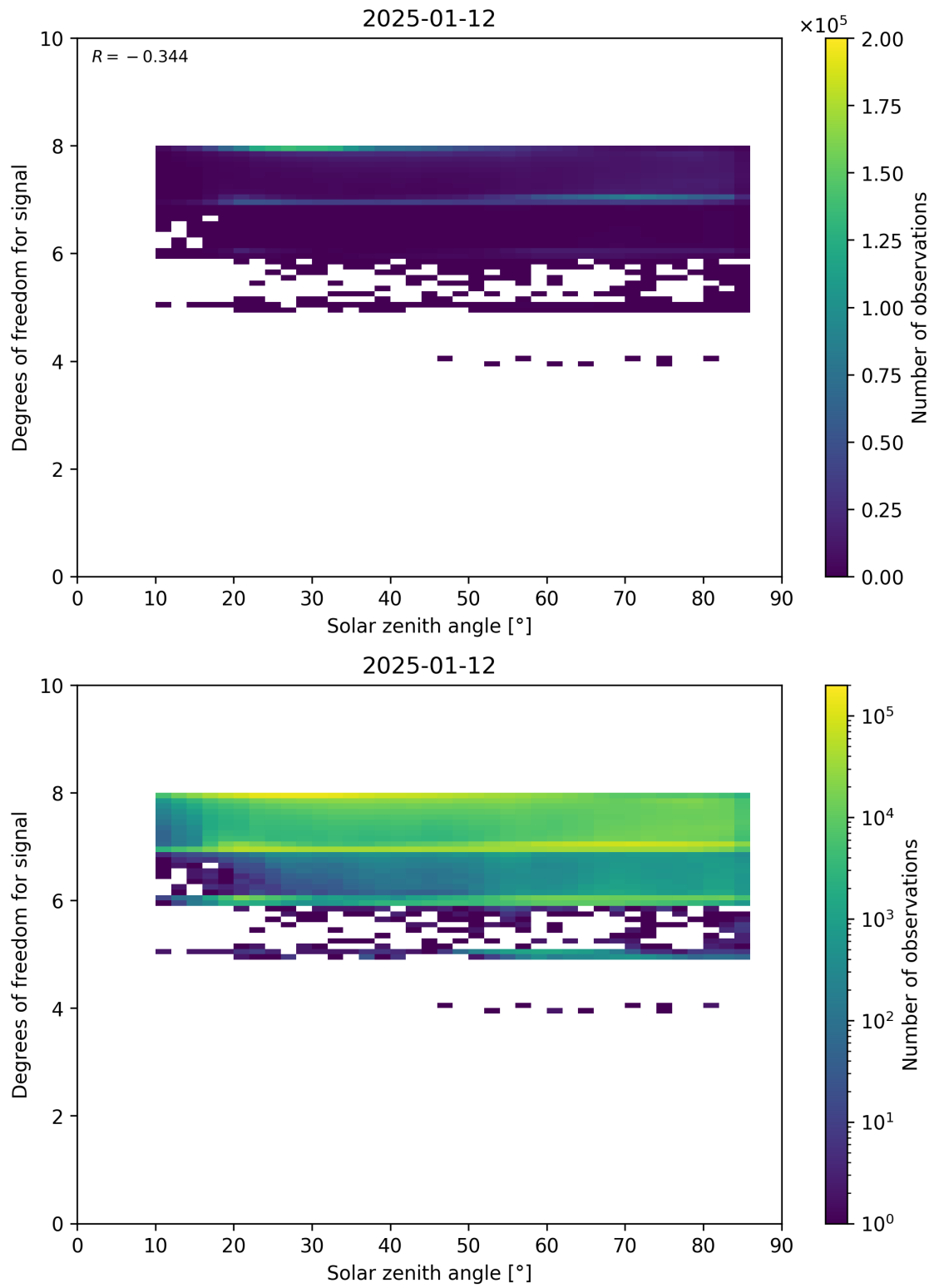
Figure 65: Scatter density plot of “Solar zenith angle” against “Degrees of freedom for signal” for 2025-01-12 to 2025-01-13.
