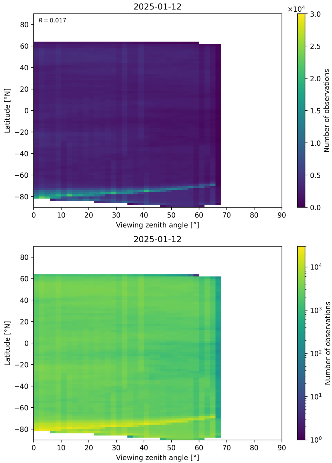
Figure 74: Scatter density plot of “Viewing zenith angle” against “Latitude” for 2025-01-12 to 2025-01-13.
