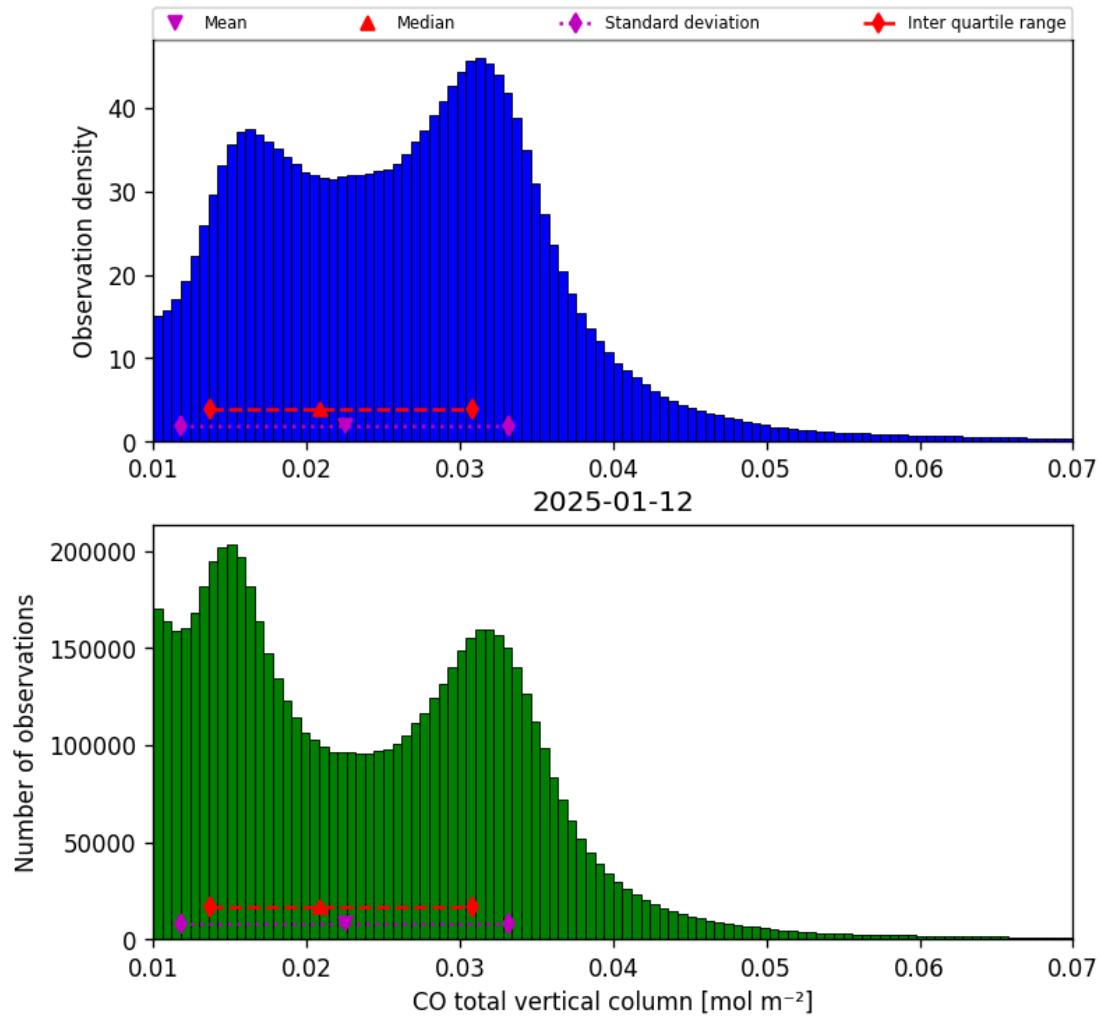
Figure 18: Histogram of “CO total vertical column” for 2025-01-12 to 2025-01-13
