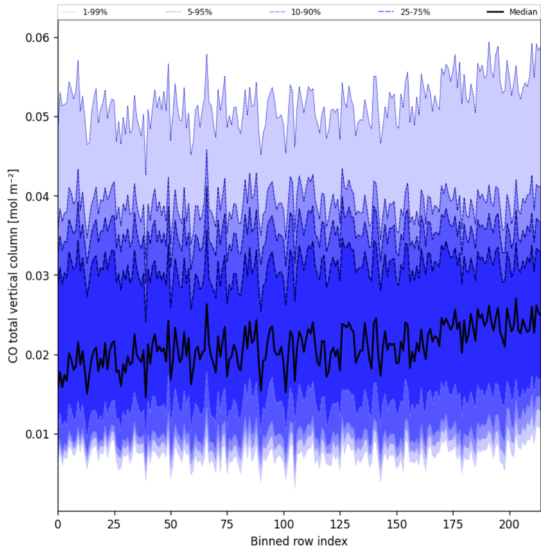
Figure 26: Along track statistics of “CO total vertical column” for 2025-01-12 to 2025-01-13
