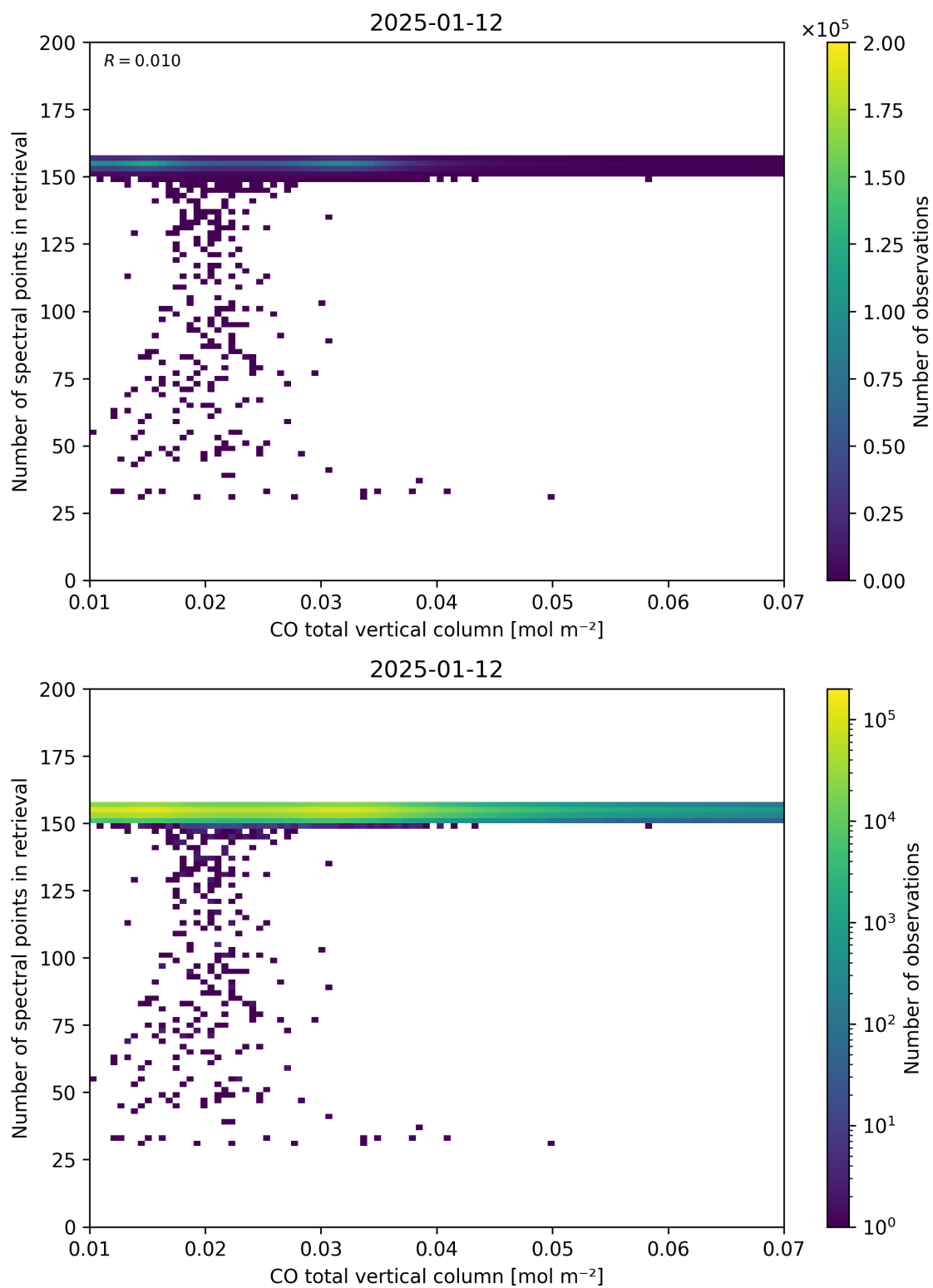
Figure 43: Scatter density plot of “CO total vertical column” against “Number of spectral points in retrieval” for 2025-01-12 to 2025-01-13.
