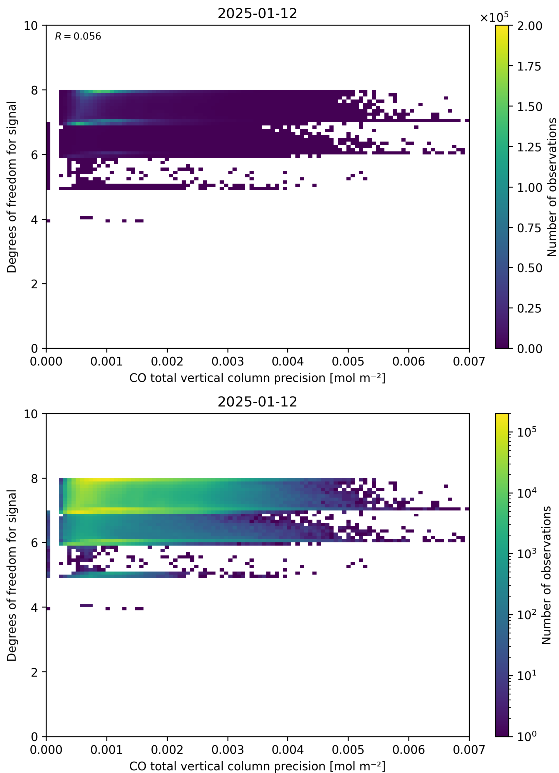
Figure 45: Scatter density plot of “CO total vertical column precision” against “Degrees of freedom for signal” for 2025-01-12 to 2025-01-13.
