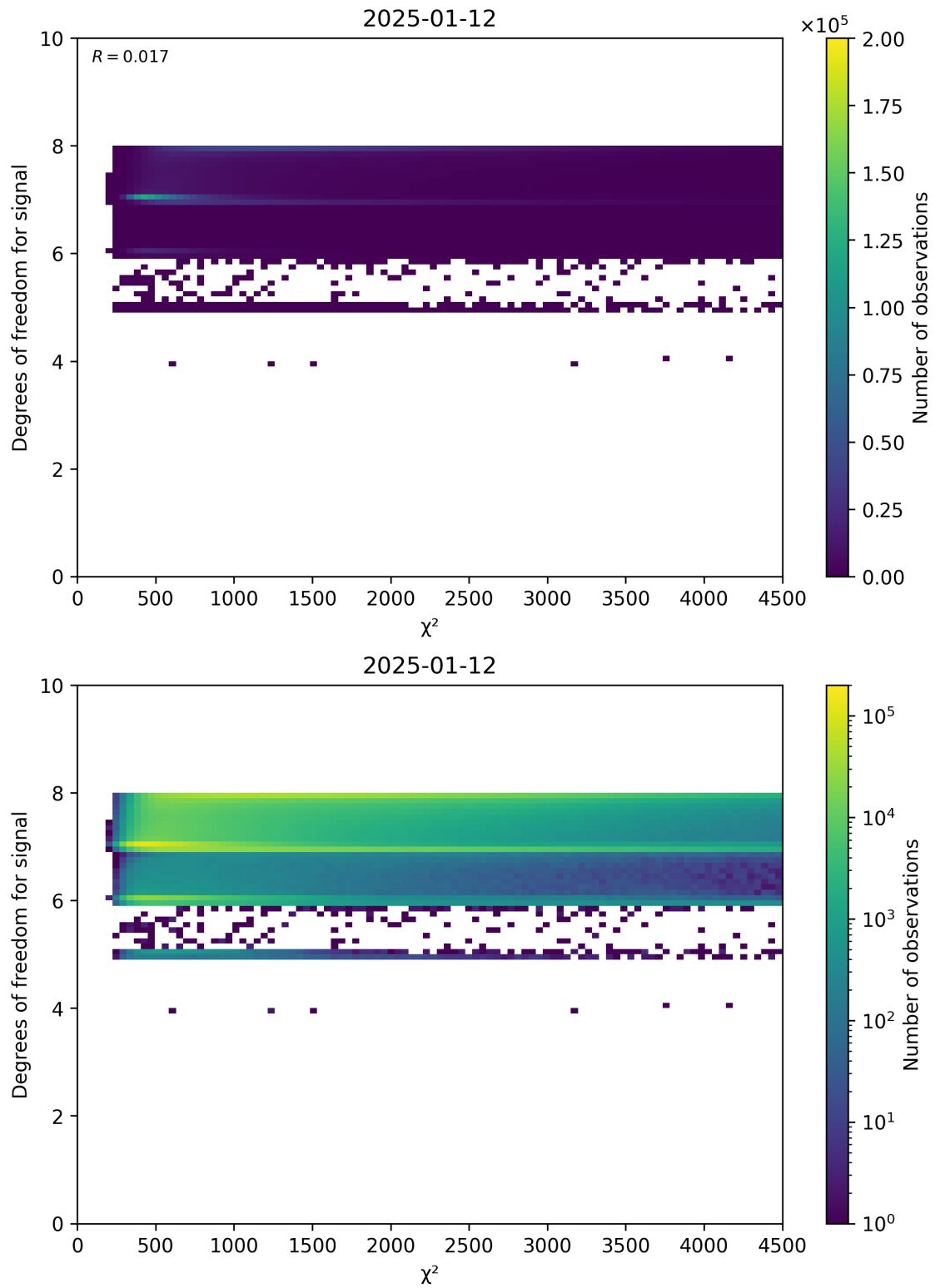
Figure 48: Scatter density plot of “ \chi^2 ” against “Degrees of freedom for signal” for 2025-01-12 to 2025-01-13.
