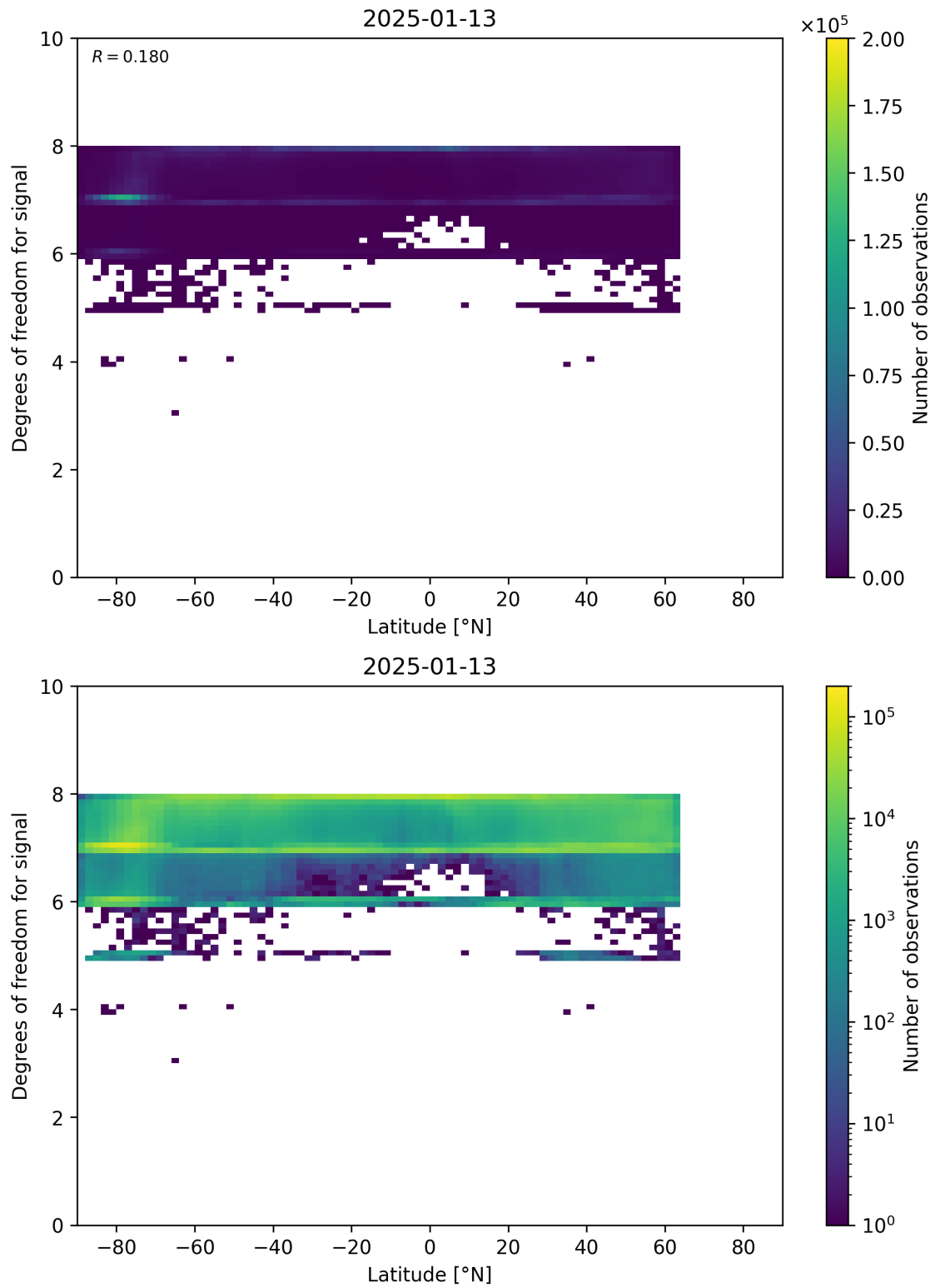
Figure 55: Scatter density plot of “Latitude” against “Degrees of freedom for signal” for 2025-01-12 to 2025-01-14.
