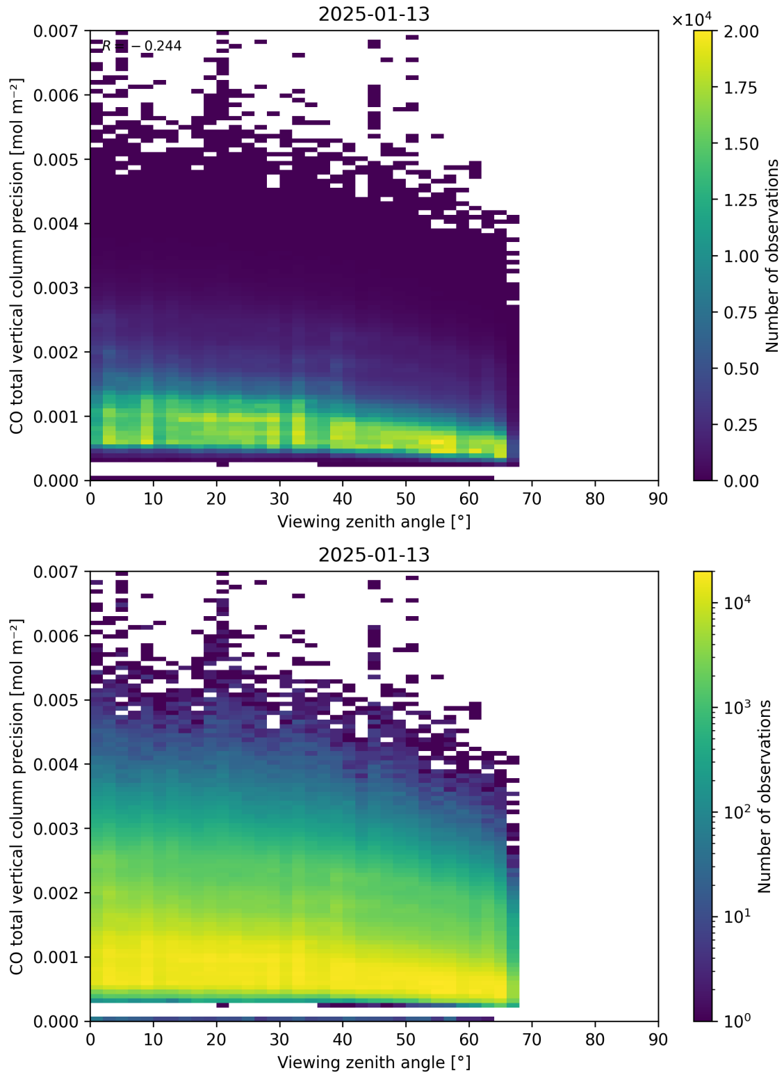
Figure 71: Scatter density plot of “Viewing zenith angle” against “CO total vertical column precision” for 2025-01-12 to 2025-01-14.
