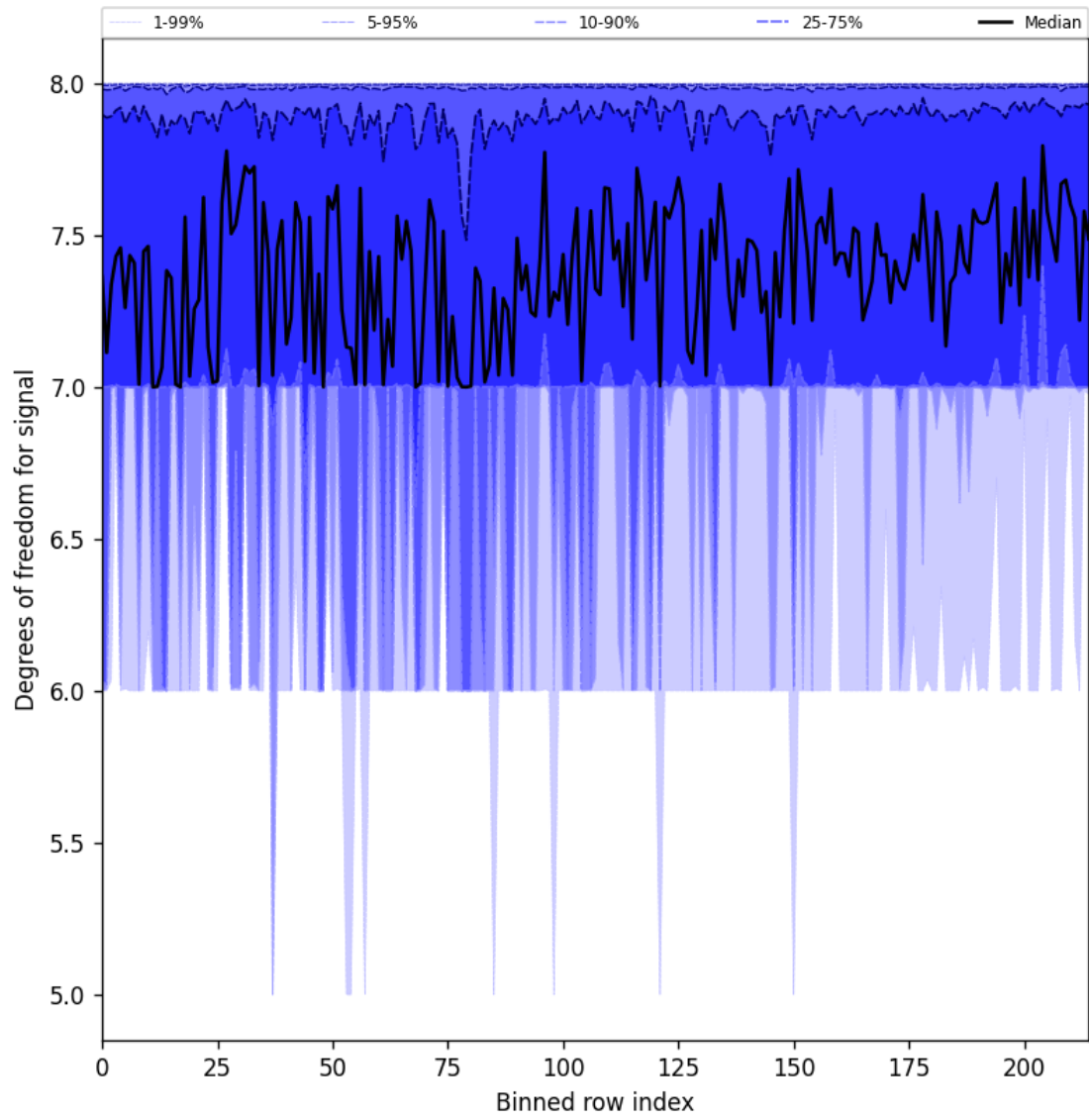
Figure 31: Along track statistics of “Degrees of freedom for signal” for 2025-01-12 to 2025-01-14
