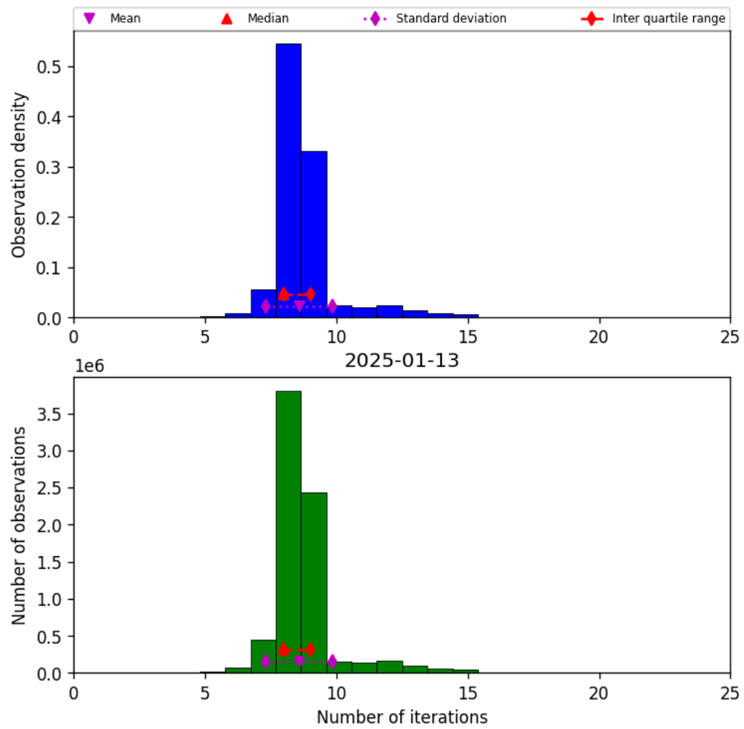
Figure 24: Histogram of “Number of iterations” for 2025-01-12 to 2025-01-14
