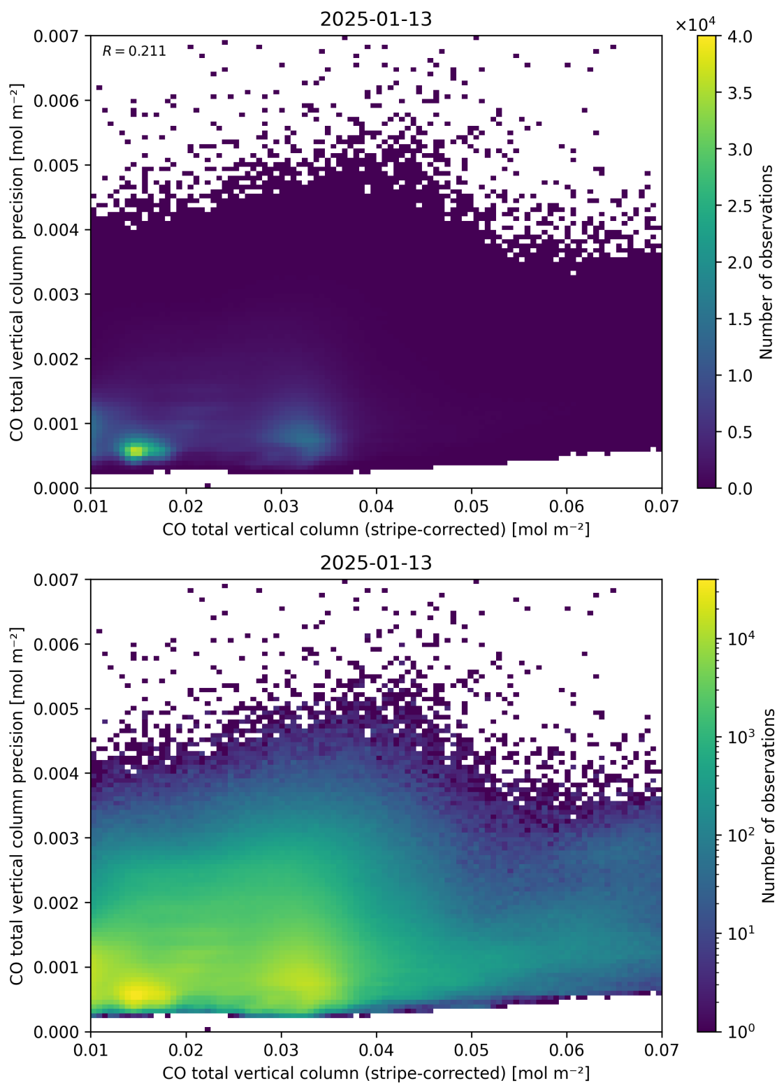
Figure 36: Scatter density plot of “CO total vertical column (stripe-corrected)” against “CO total vertical column precision” for 2025-01-12 to 2025-01-14.
