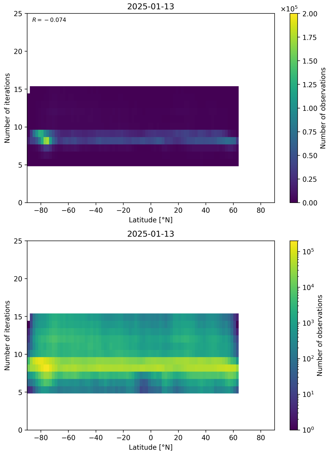
Figure 56: Scatter density plot of “Latitude” against “Number of iterations” for 2025-01-12 to 2025-01-14.
