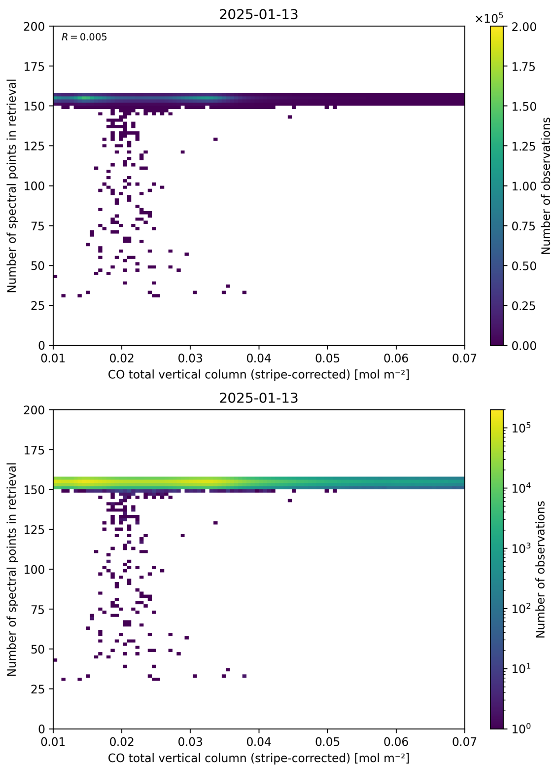
Figure 40: Scatter density plot of “CO total vertical column (stripe-corrected)” against “Number of spectral points in retrieval” for 2025-01-12 to 2025-01-14.
