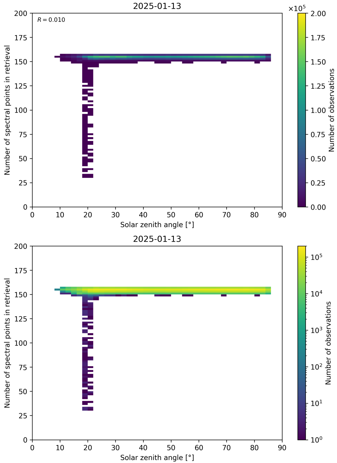
Figure 68: Scatter density plot of “Solar zenith angle” against “Number of spectral points in retrieval” for 2025-01-12 to 2025-01-14.
