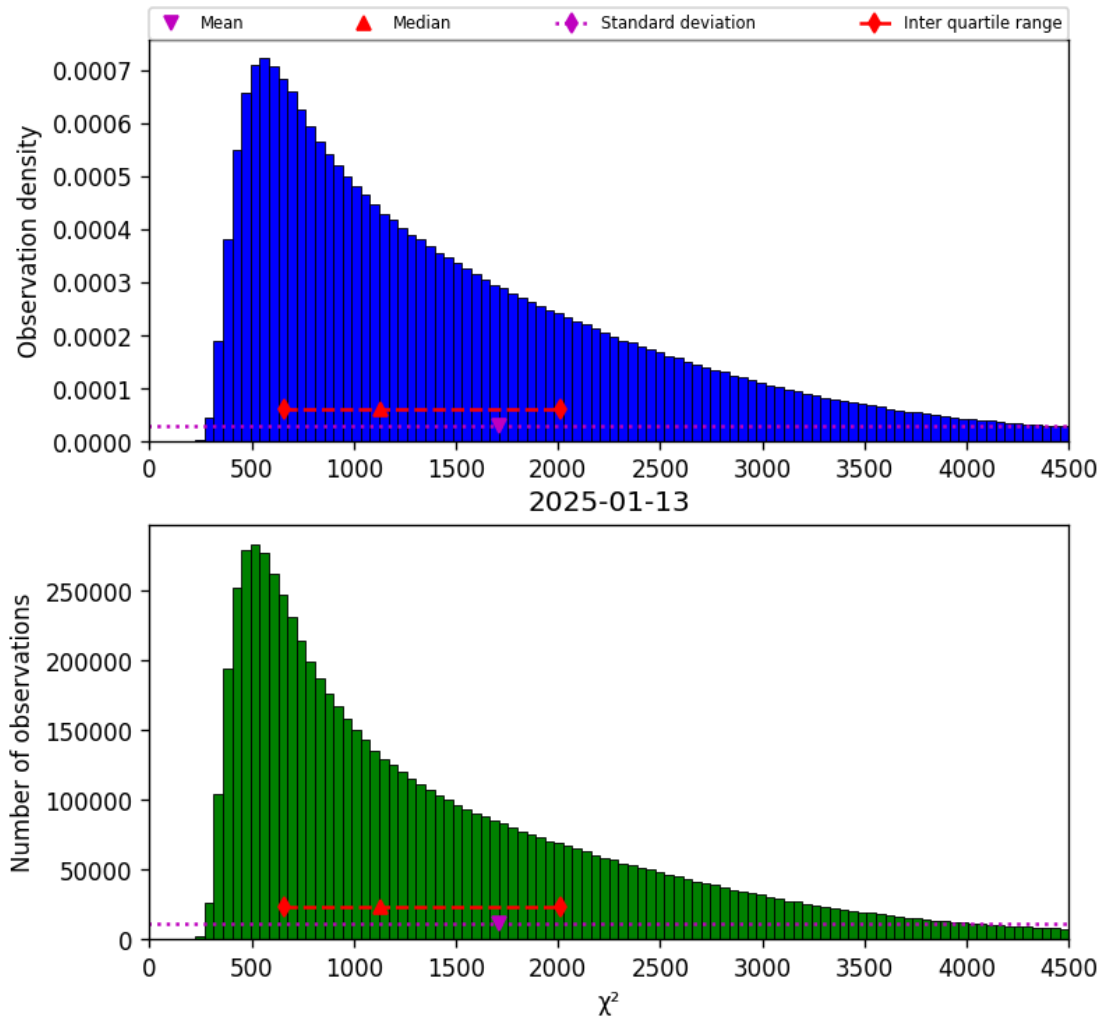
Figure 22: Histogram of “ \chi^2 ” for 2025-01-12 to 2025-01-14
