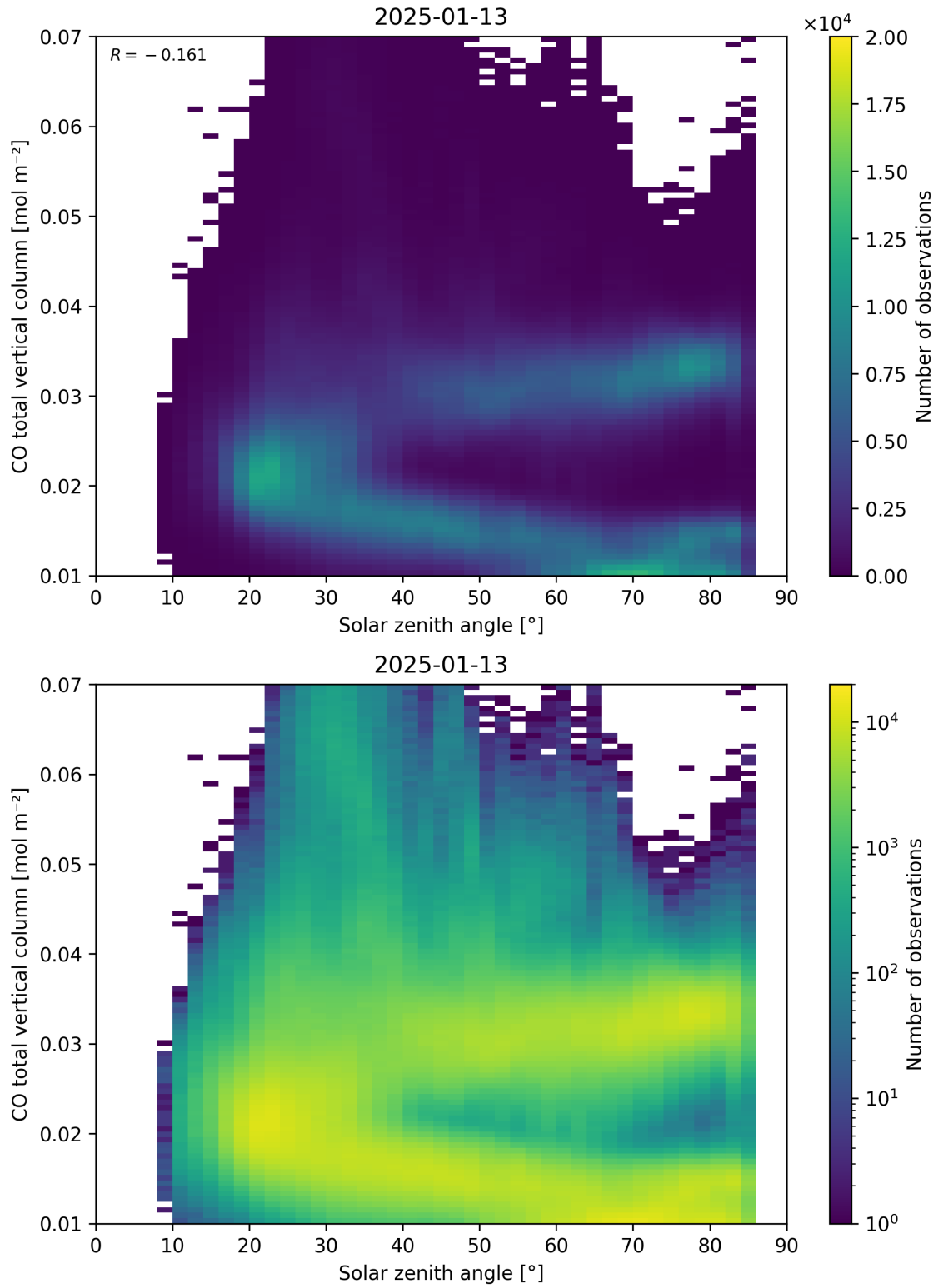
Figure 61: Scatter density plot of “Solar zenith angle” against “CO total vertical column” for 2025-01-12 to 2025-01-14.
