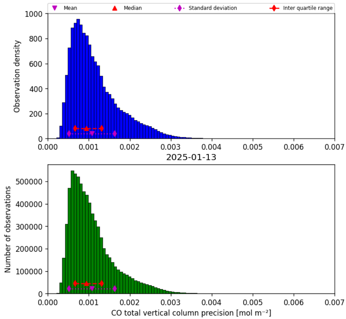
Figure 20: Histogram of “CO total vertical column precision” for 2025-01-12 to 2025-01-14
