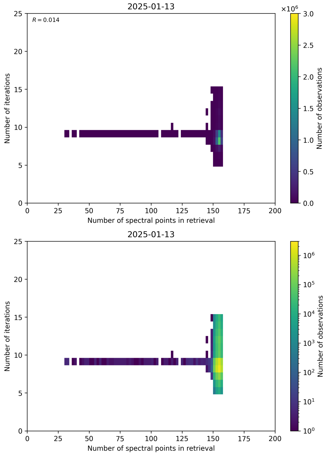
Figure 60: Scatter density plot of “Number of spectral points in retrieval” against “Number of iterations” for 2025-01-12 to 2025-01-14.
