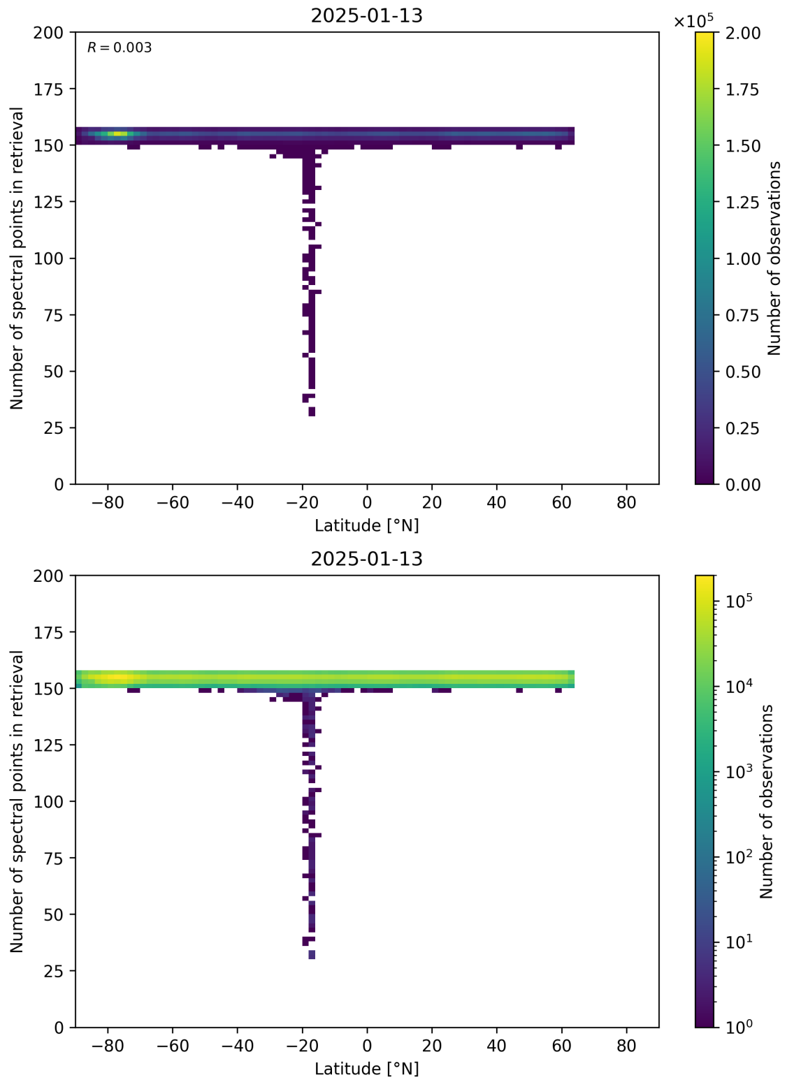
Figure 57: Scatter density plot of “Latitude” against “Number of spectral points in retrieval” for 2025-01-12 to 2025-01-14.
