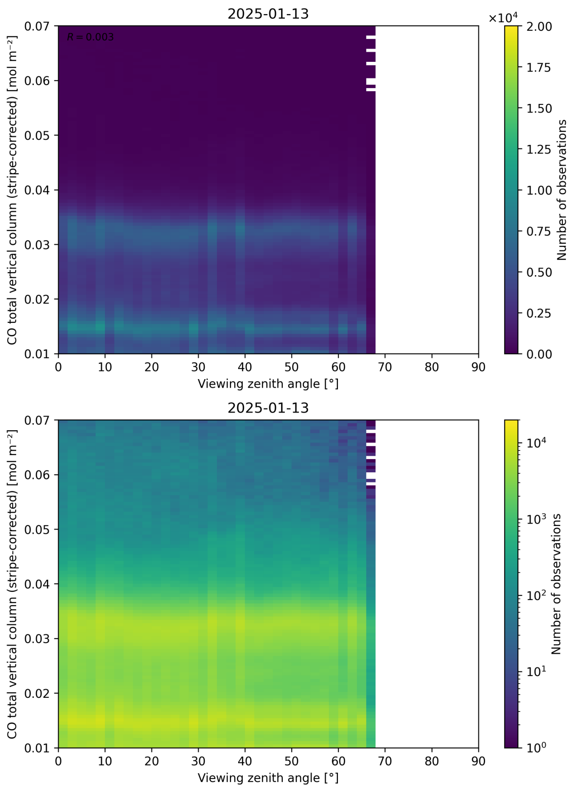
Figure 70: Scatter density plot of “Viewing zenith angle” against “CO total vertical column (stripe-corrected)” for 2025-01-12 to 2025-01-14.
