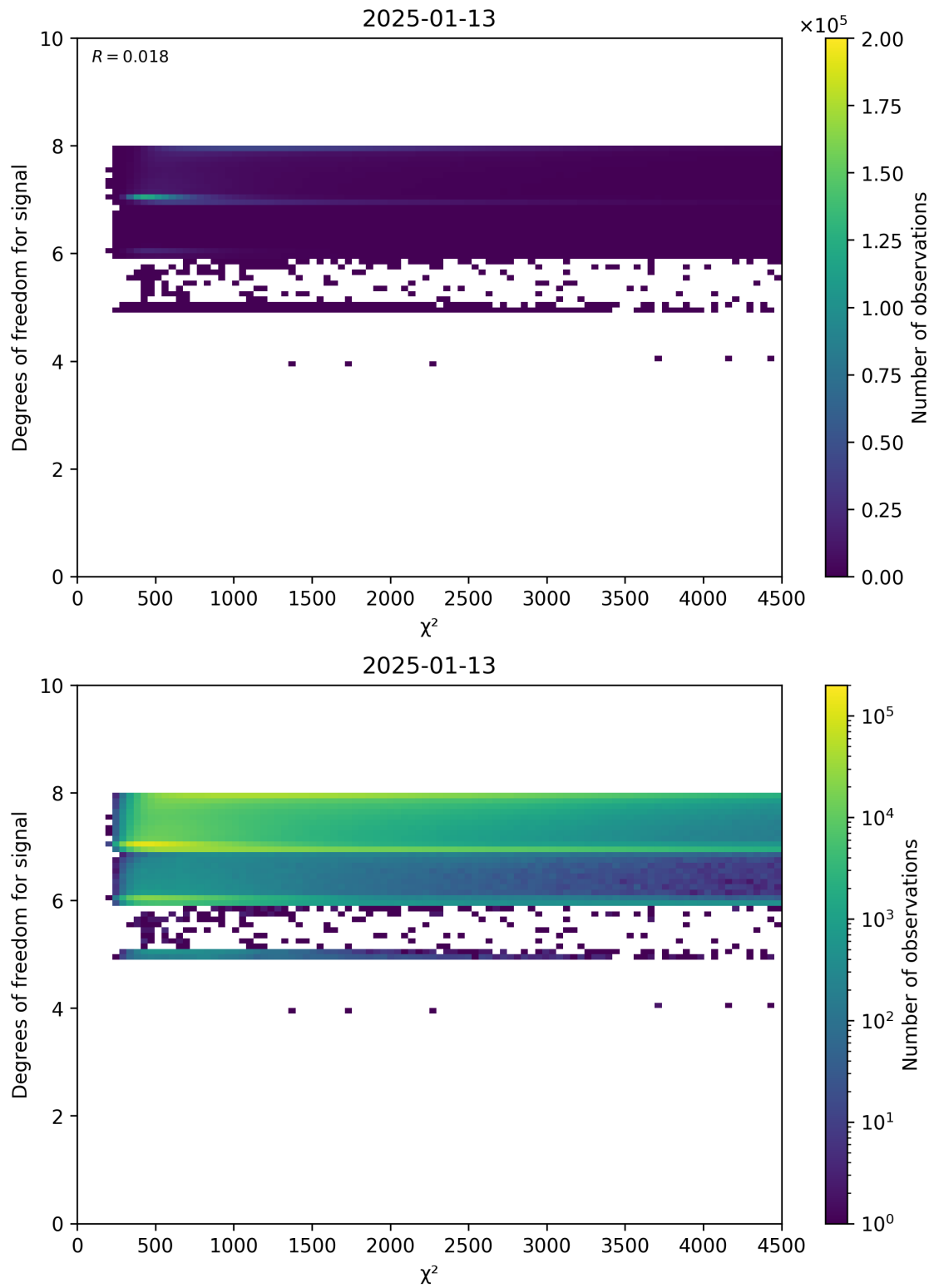
Figure 48: Scatter density plot of “ \chi^2 ” against “Degrees of freedom for signal” for 2025-01-12 to 2025-01-14.
