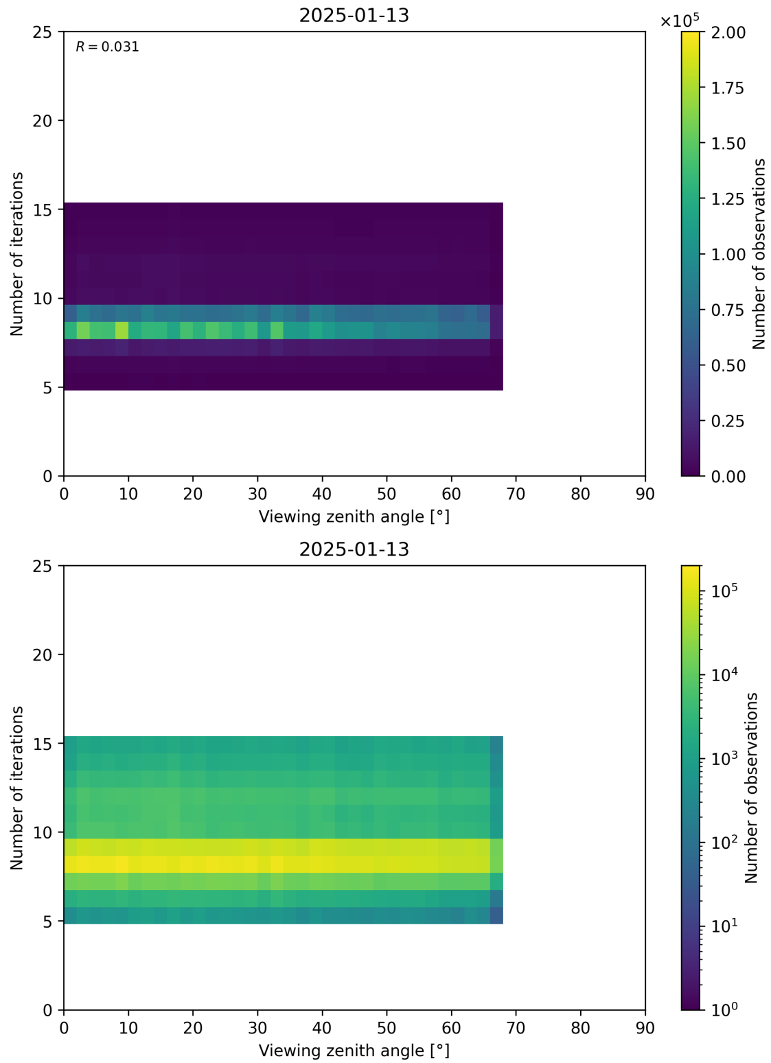
Figure 75: Scatter density plot of “Viewing zenith angle” against “Number of iterations” for 2025-01-12 to 2025-01-14.
