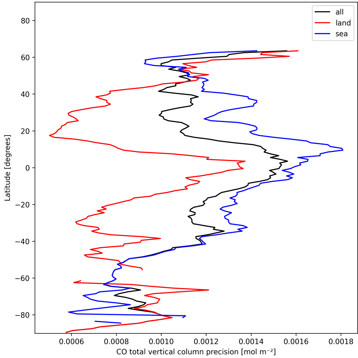
Figure 12: Zonal average of “CO total vertical column precision” for 2025-01-12 to 2025-01-14.
