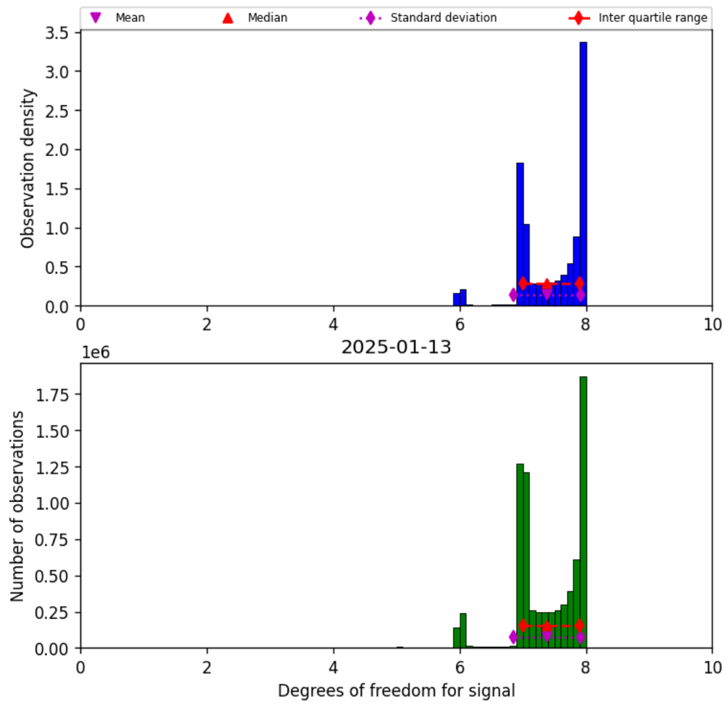
Figure 23: Histogram of “Degrees of freedom for signal” for 2025-01-12 to 2025-01-14
