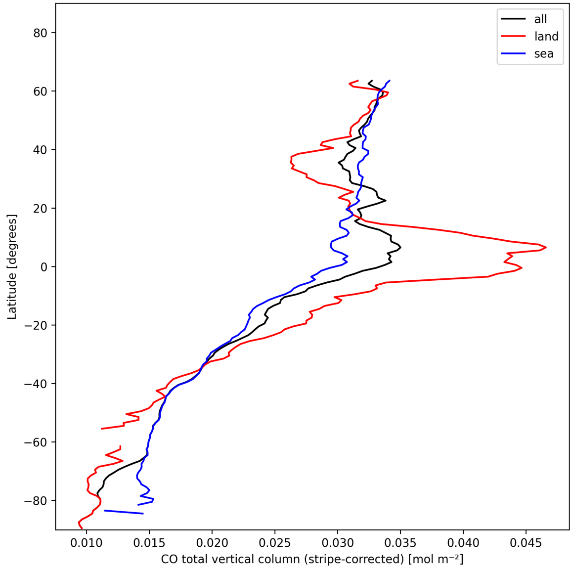
Figure 11: Zonal average of “CO total vertical column (stripe-corrected)” for 2025-01-12 to 2025-01-14.
