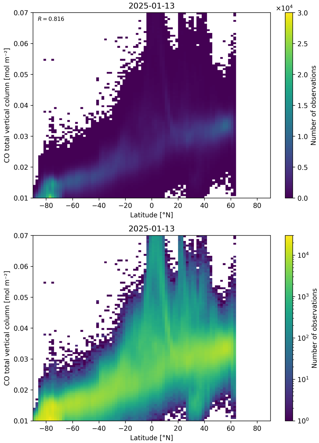
Figure 51: Scatter density plot of “Latitude” against “CO total vertical column” for 2025-01-12 to 2025-01-14.
