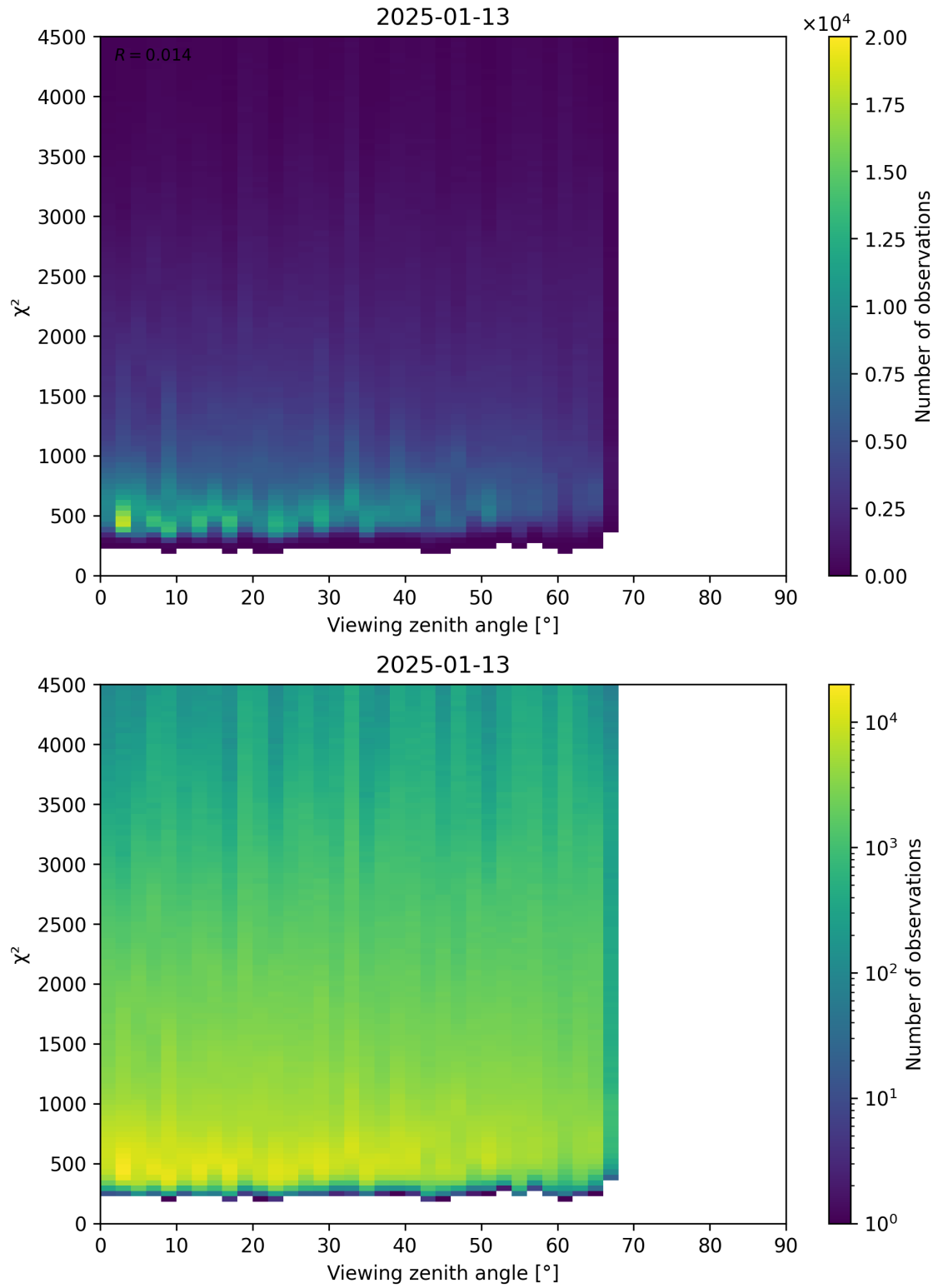
Figure 72: Scatter density plot of “Viewing zenith angle” against “ \chi^2 ” for 2025-01-12 to 2025-01-14.
