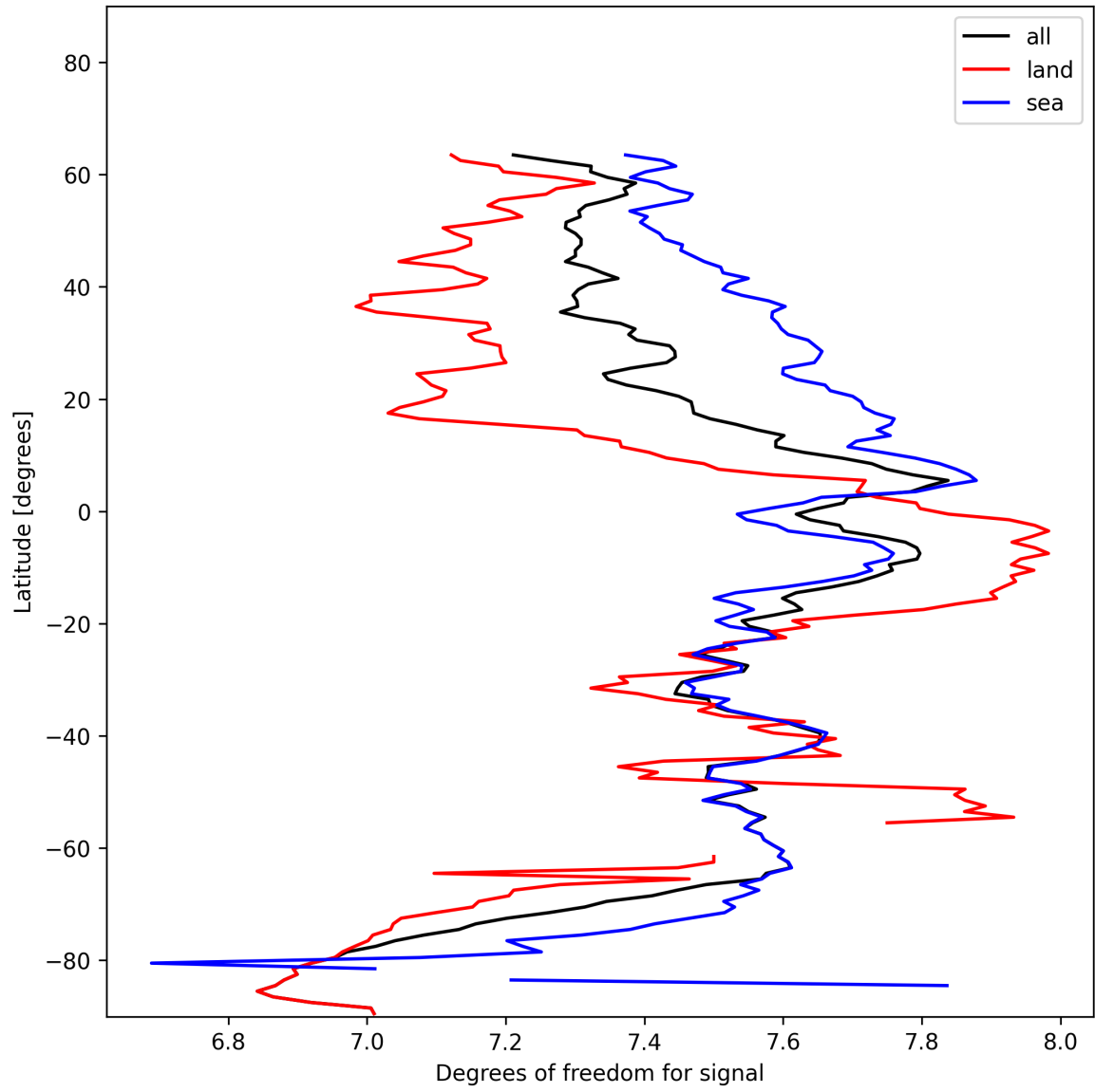
Figure 15: Zonal average of “Degrees of freedom for signal” for 2025-01-12 to 2025-01-14.
