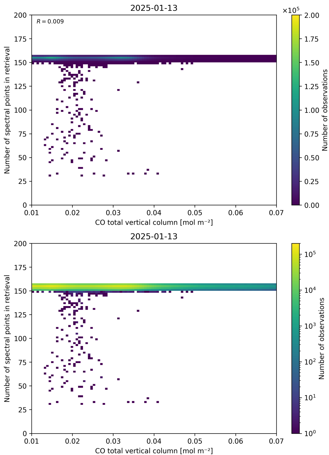
Figure 43: Scatter density plot of “CO total vertical column” against “Number of spectral points in retrieval” for 2025-01-12 to 2025-01-14.
