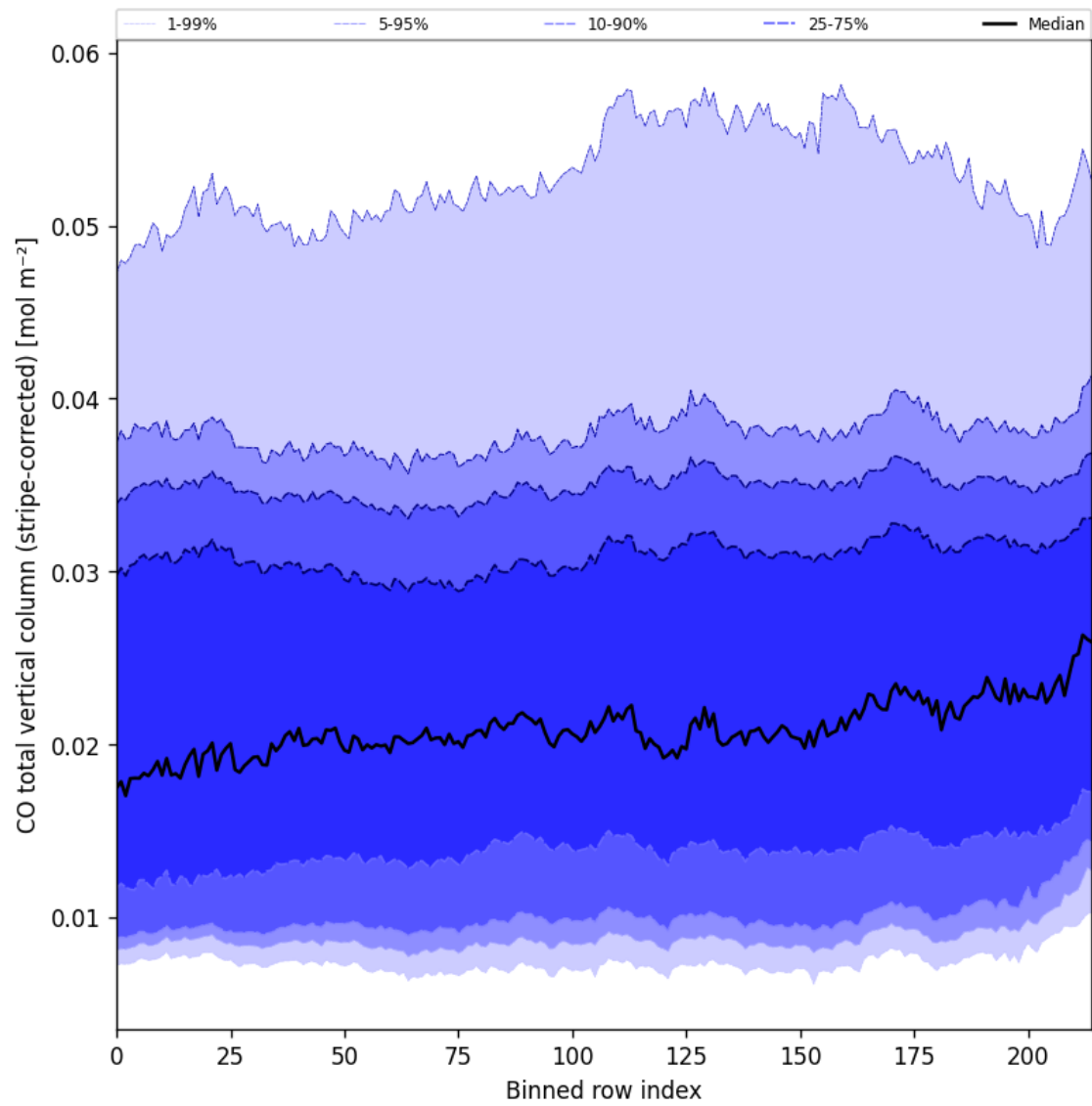
Figure 27: Along track statistics of “CO total vertical column (stripe-corrected)” for 2025-01-12 to 2025-01-14
