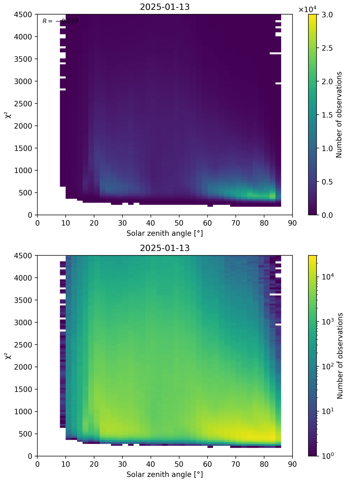
Figure 64: Scatter density plot of “Solar zenith angle” against “ \chi^2 ” for 2025-01-12 to 2025-01-14.
