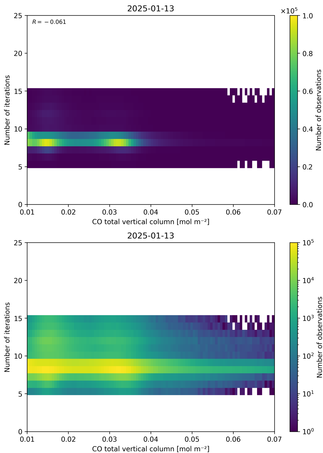
Figure 42: Scatter density plot of “CO total vertical column” against “Number of iterations” for 2025-01-12 to 2025-01-14.
