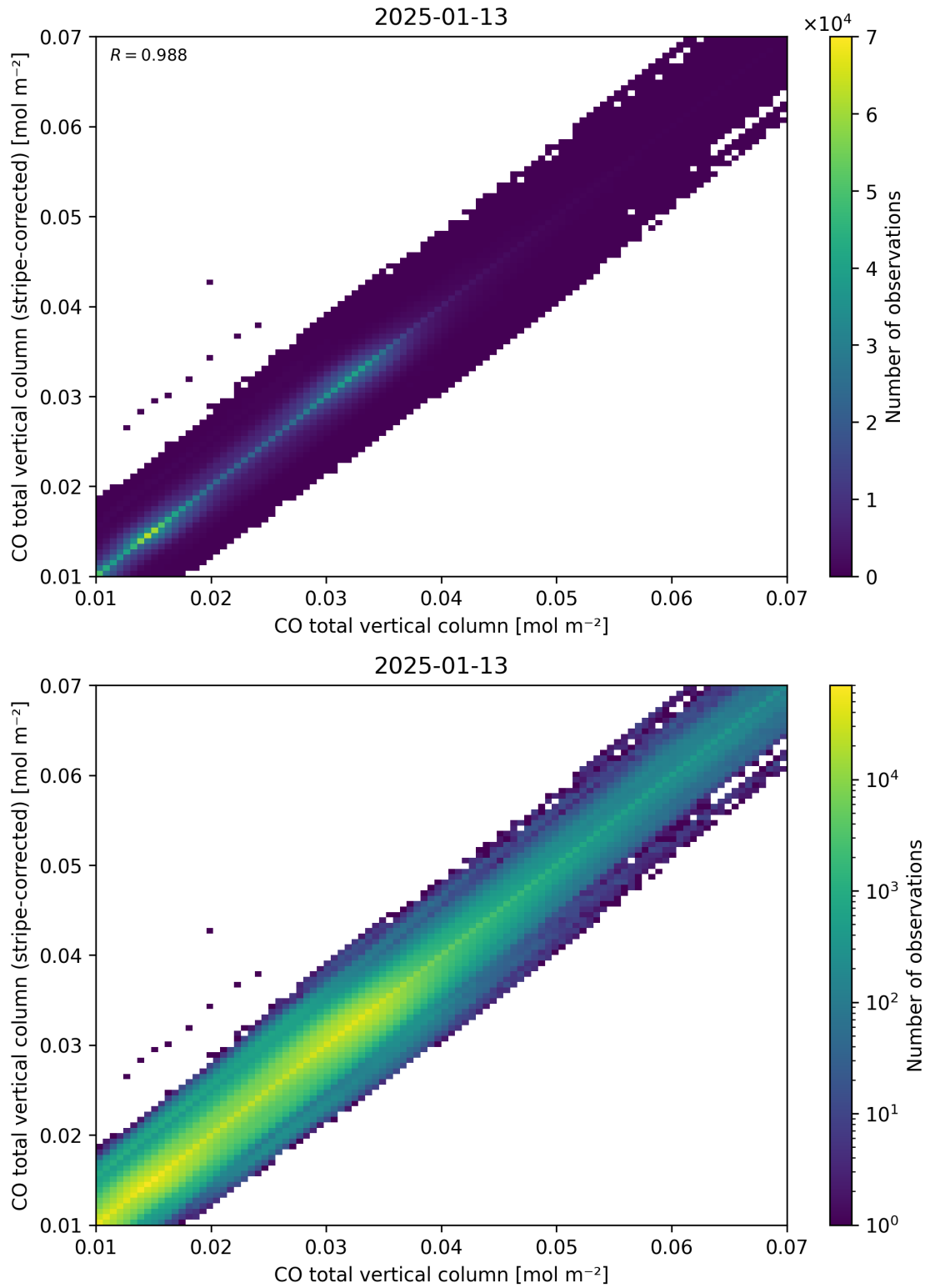
Figure 33: Scatter density plot of “CO total vertical column” against “CO total vertical column (stripe-corrected)” for 2025-01-12 to 2025-01-14.
