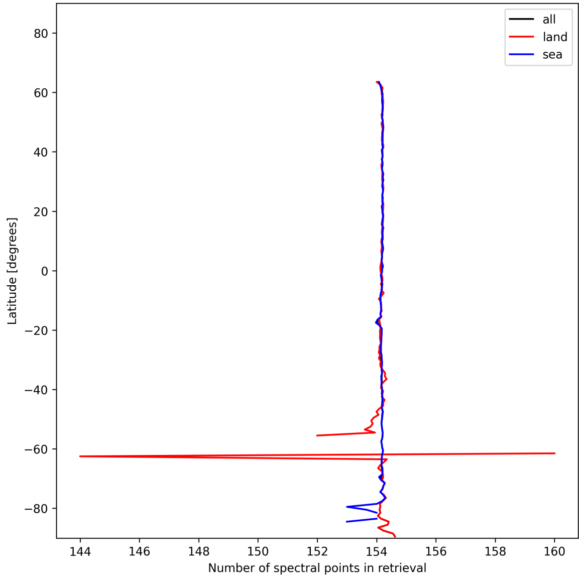
Figure 13: Zonal average of “Number of spectral points in retrieval” for 2025-01-12 to 2025-01-14.
