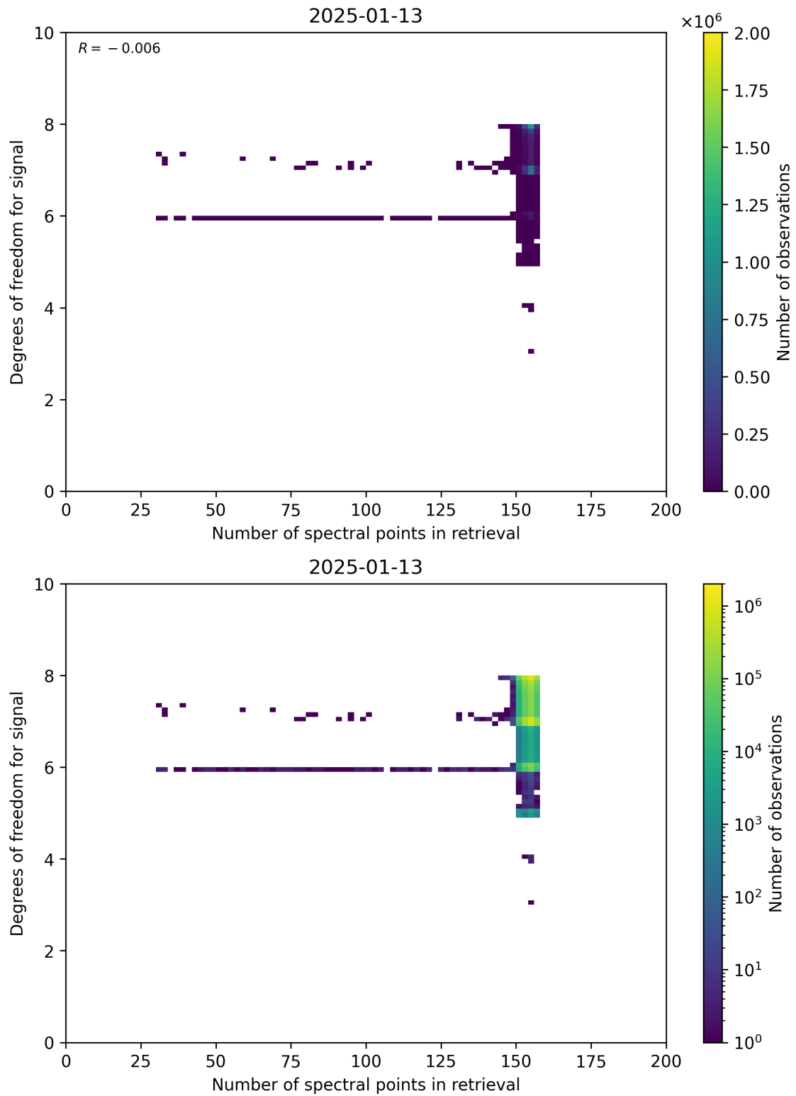
Figure 59: Scatter density plot of “Number of spectral points in retrieval” against “Degrees of freedom for signal” for 2025-01-12 to 2025-01-14.
