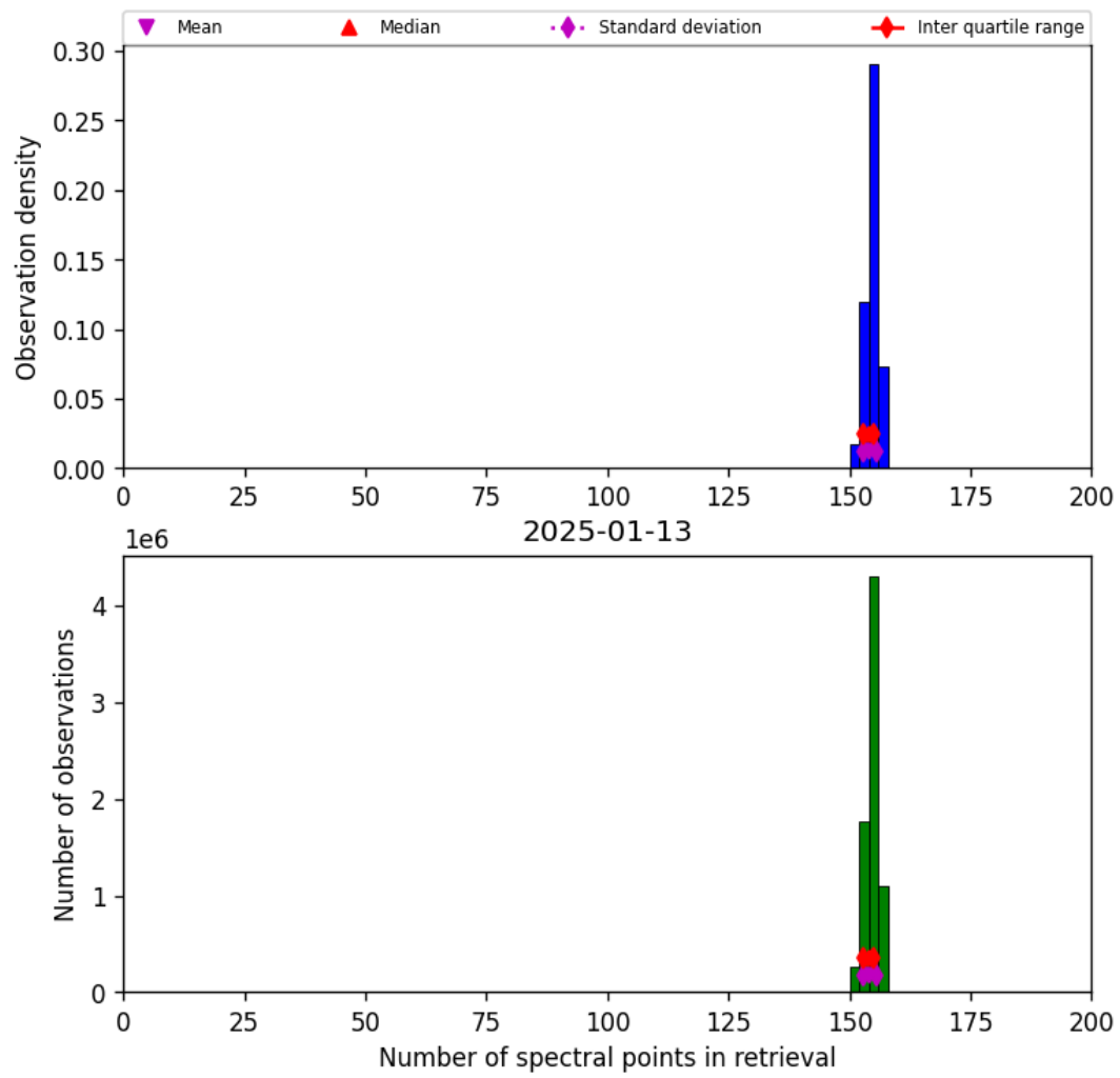
Figure 21: Histogram of “Number of spectral points in retrieval” for 2025-01-12 to 2025-01-14
