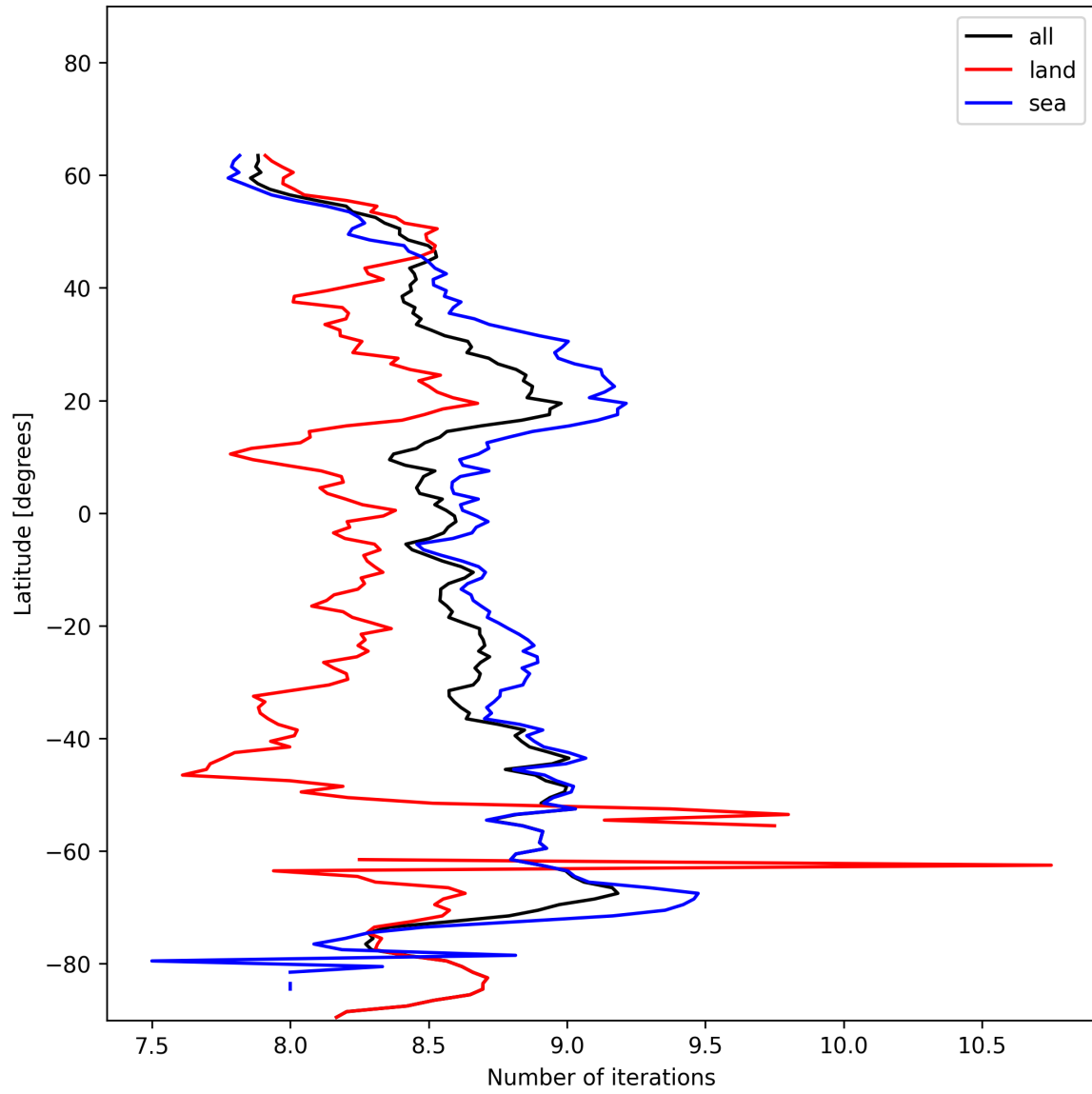
Figure 16: Zonal average of “Number of iterations” for 2025-01-12 to 2025-01-14.
