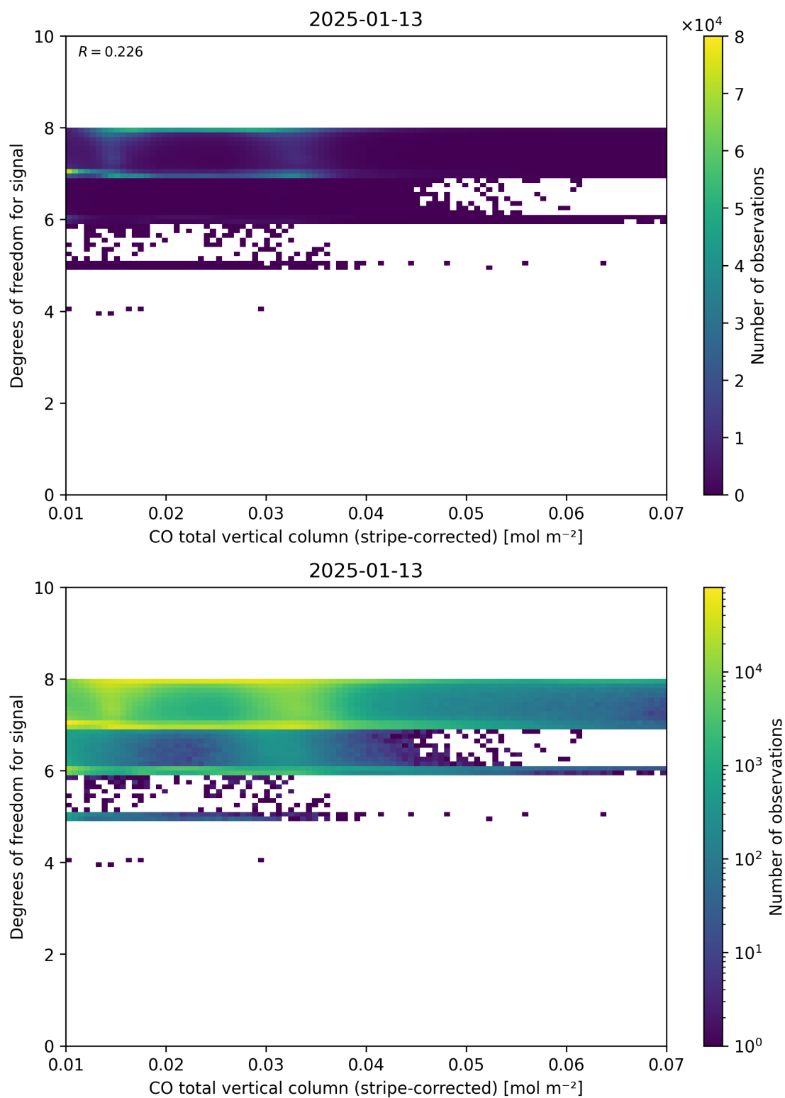
Figure 38: Scatter density plot of “CO total vertical column (stripe-corrected)” against “Degrees of freedom for signal” for 2025-01-12 to 2025-01-14.
