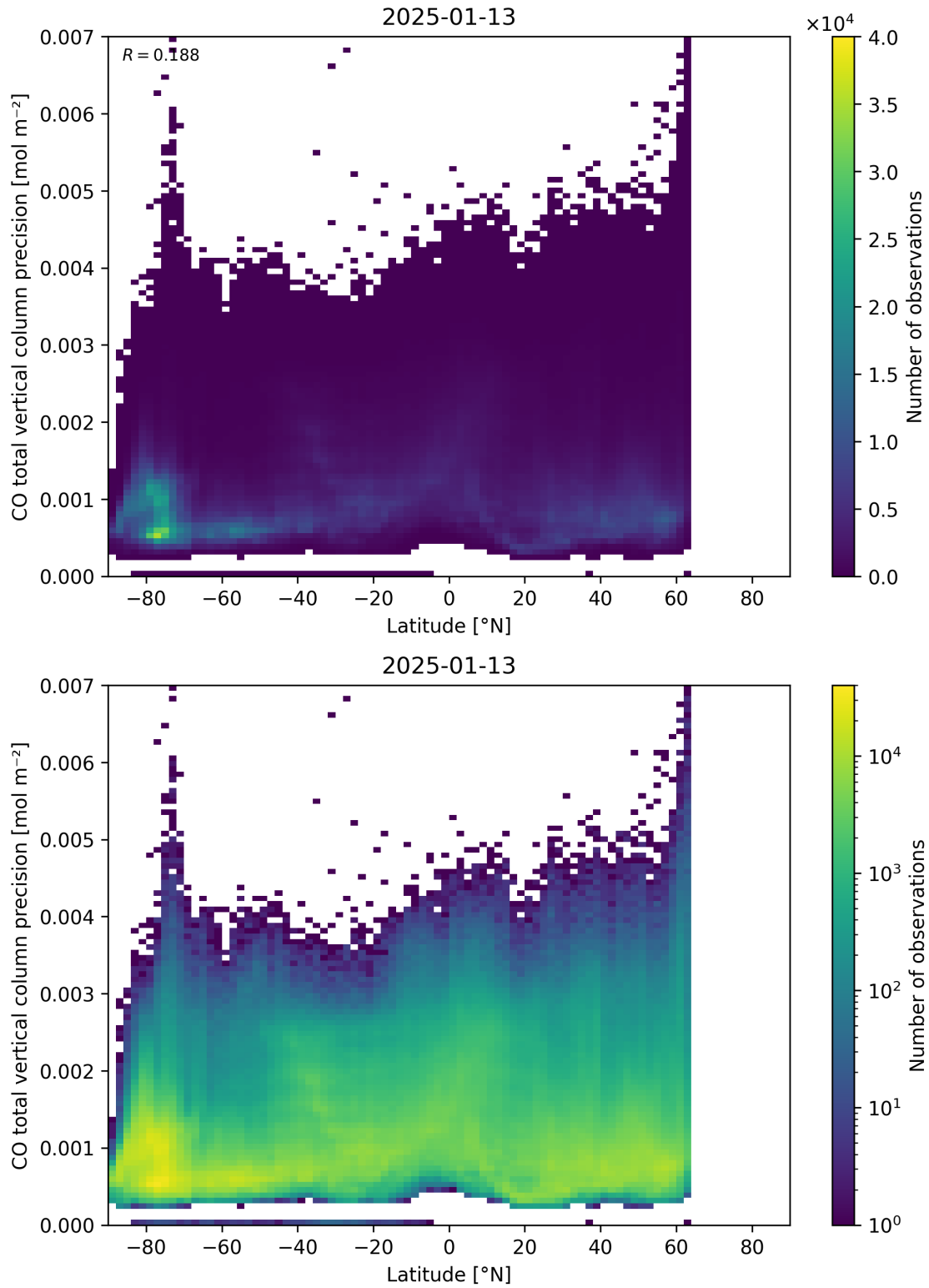
Figure 53: Scatter density plot of “Latitude” against “CO total vertical column precision” for 2025-01-12 to 2025-01-14.
