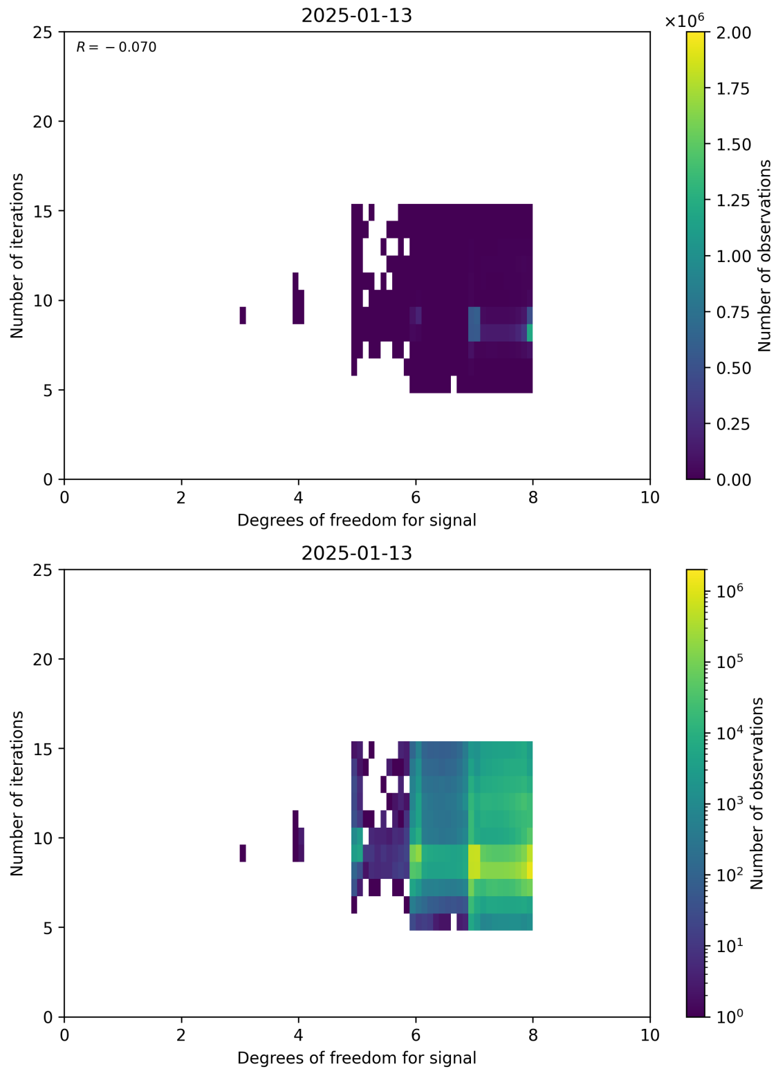
Figure 50: Scatter density plot of “Degrees of freedom for signal” against “Number of iterations” for 2025-01-12 to 2025-01-14.
