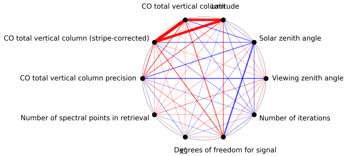
Figure 1: Map of correlation graph for 2025-01-12 to 2025-01-14.
