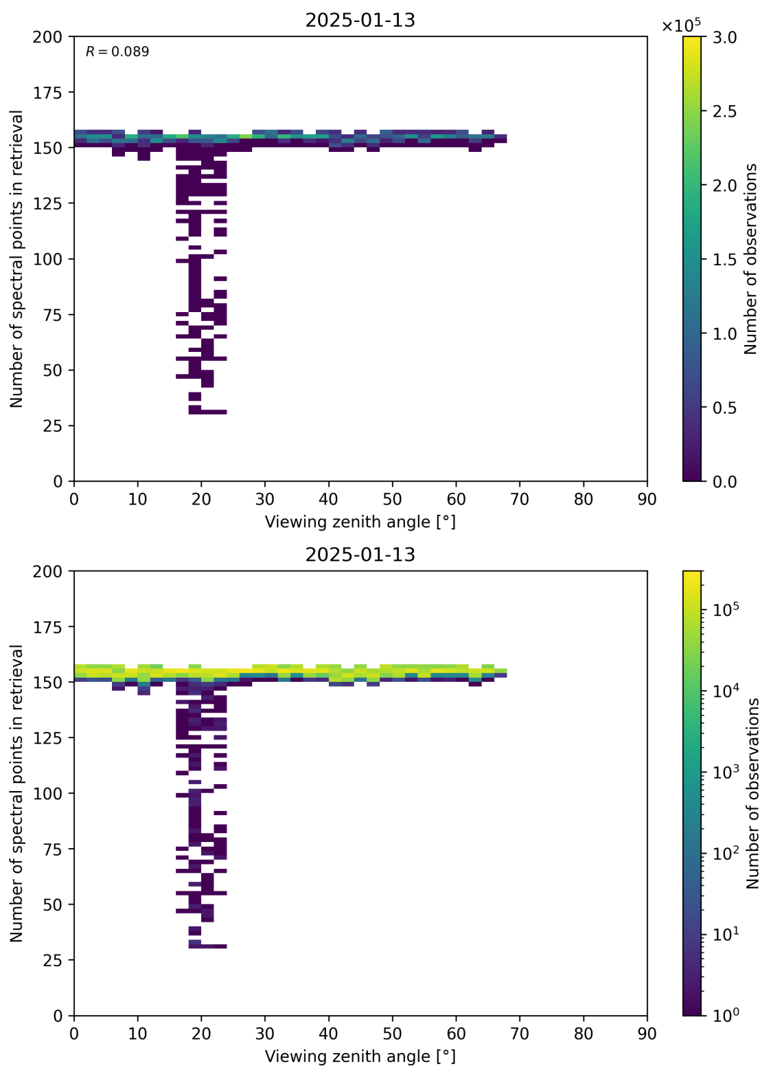
Figure 76: Scatter density plot of “Viewing zenith angle” against “Number of spectral points in retrieval” for 2025-01-12 to 2025-01-14.
