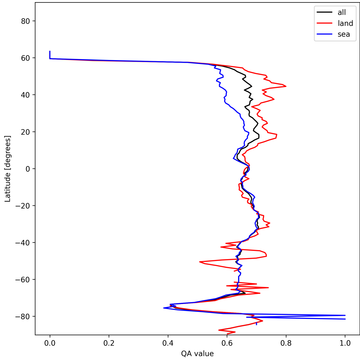
Figure 9: Zonal average of “QA value” for 2025-01-12 to 2025-01-14.
