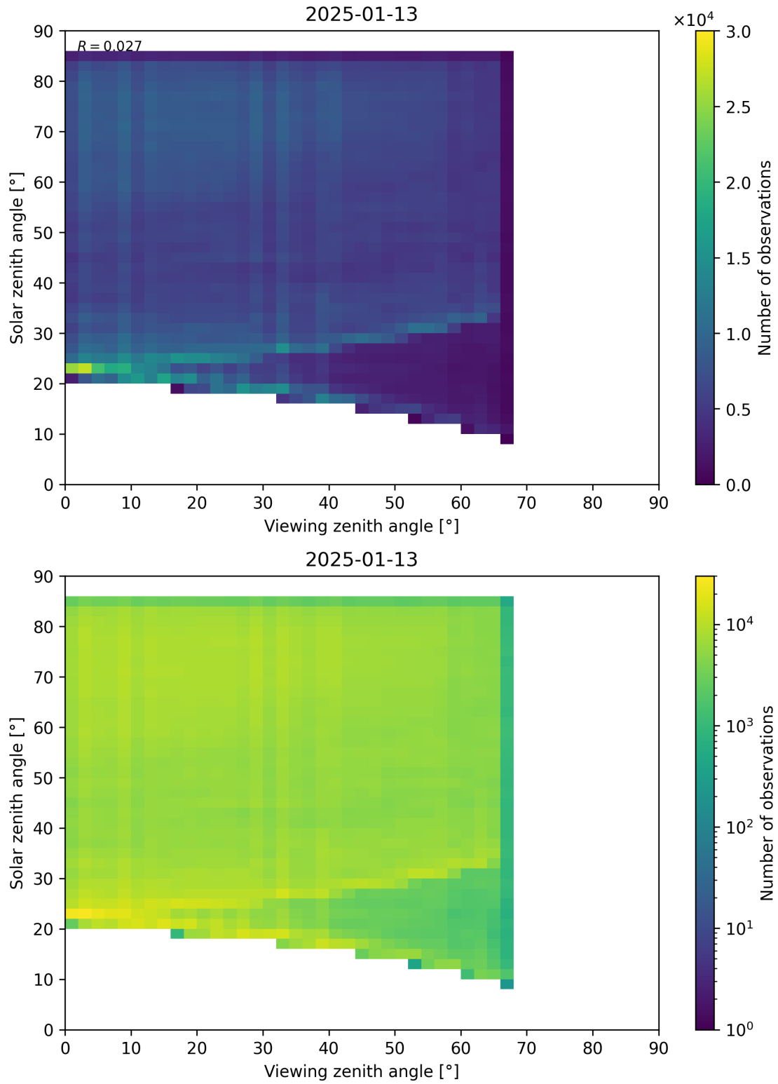
Figure 77: Scatter density plot of “Viewing zenith angle” against “Solar zenith angle” for 2025-01-12 to 2025-01-14.
