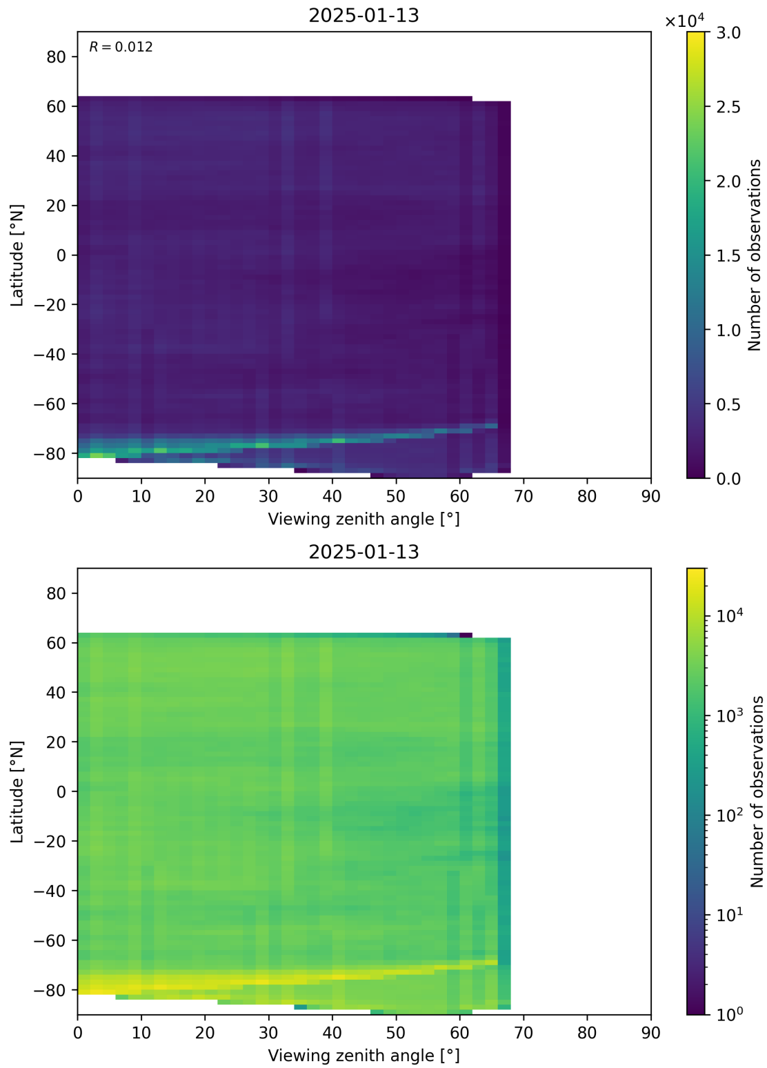
Figure 74: Scatter density plot of “Viewing zenith angle” against “Latitude” for 2025-01-12 to 2025-01-14.
