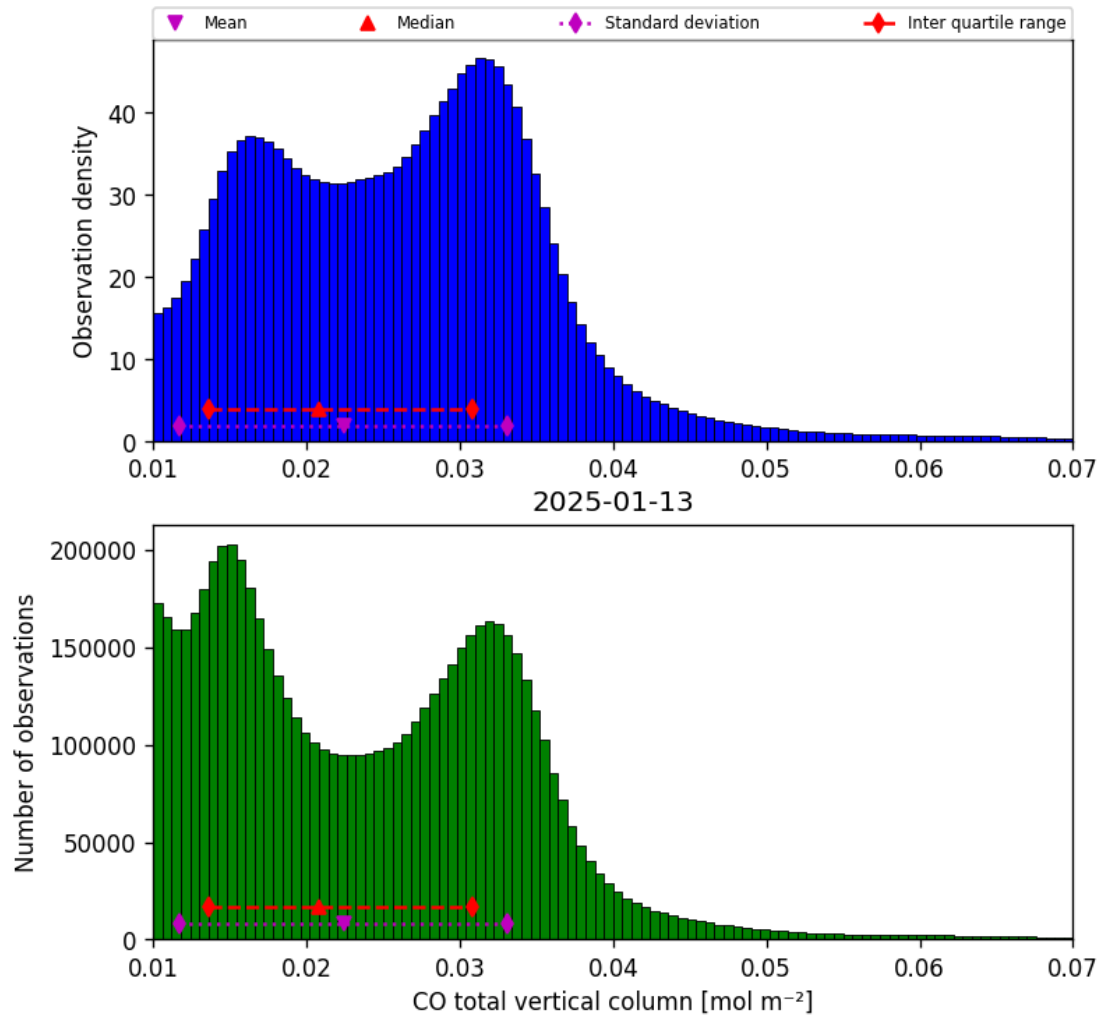
Figure 18: Histogram of “CO total vertical column” for 2025-01-12 to 2025-01-14
