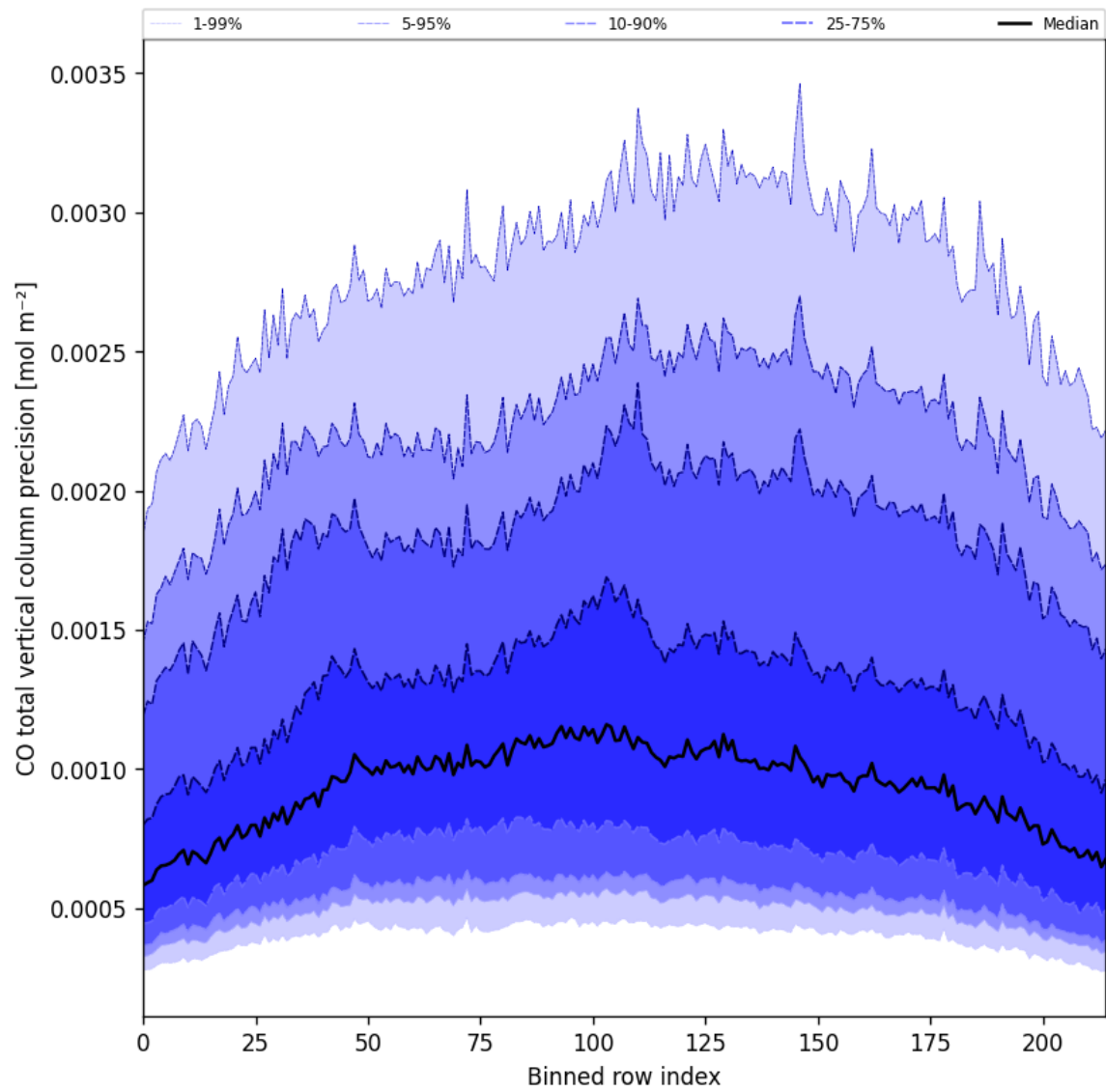
Figure 28: Along track statistics of “CO total vertical column precision” for 2025-01-12 to 2025-01-14
