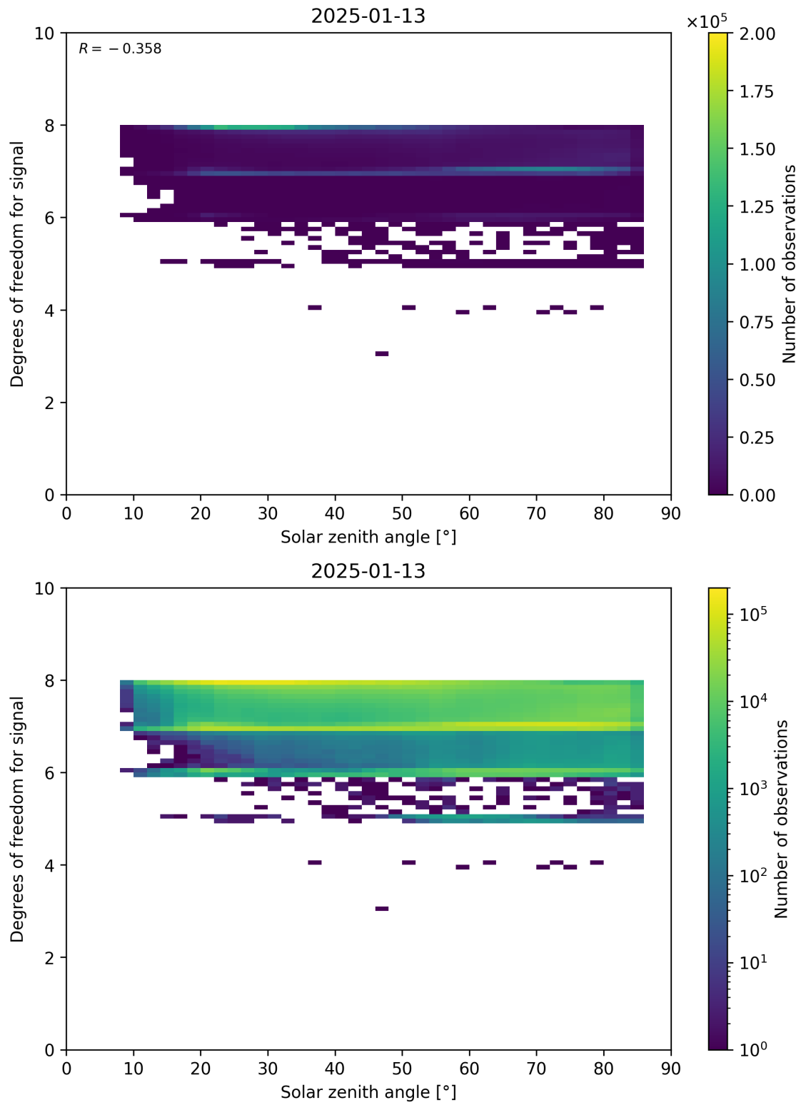
Figure 65: Scatter density plot of “Solar zenith angle” against “Degrees of freedom for signal” for 2025-01-12 to 2025-01-14.
