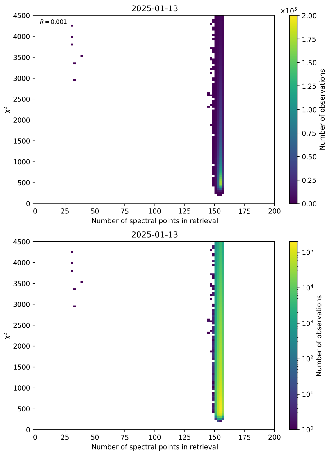
Figure 58: Scatter density plot of “Number of spectral points in retrieval” against “ \chi^2 ” for 2025-01-12 to 2025-01-14.
