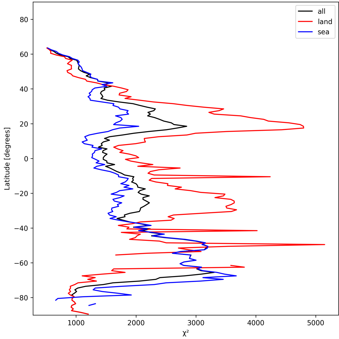
Figure 14: Zonal average of “ \chi^2 ” for 2025-01-12 to 2025-01-14.
