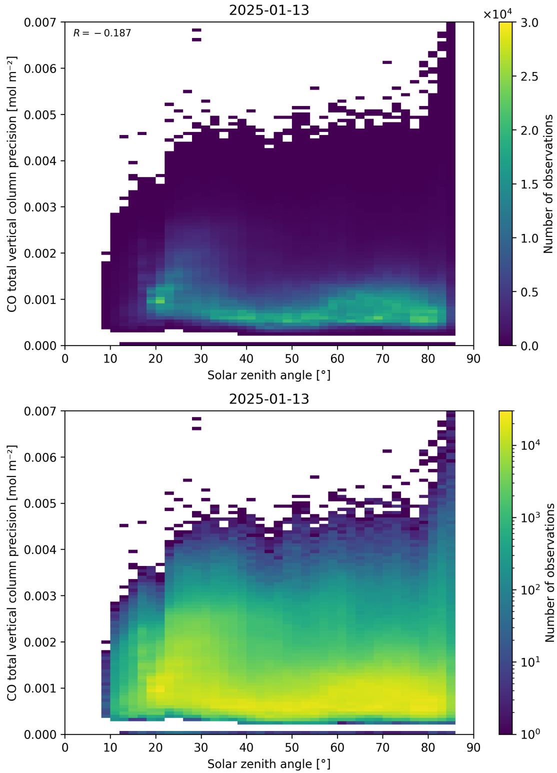
Figure 63: Scatter density plot of “Solar zenith angle” against “CO total vertical column precision” for 2025-01-12 to 2025-01-14.
