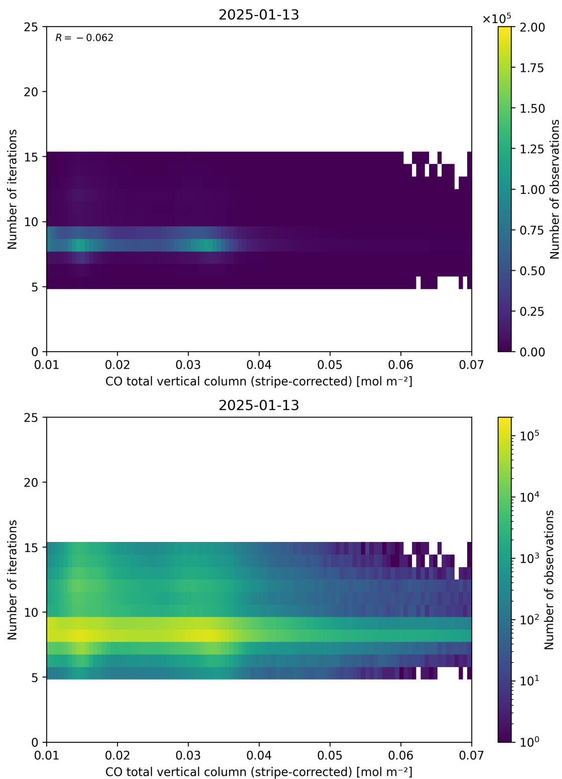
Figure 39: Scatter density plot of “CO total vertical column (stripe-corrected)” against “Number of iterations” for 2025-01-12 to 2025-01-14.
