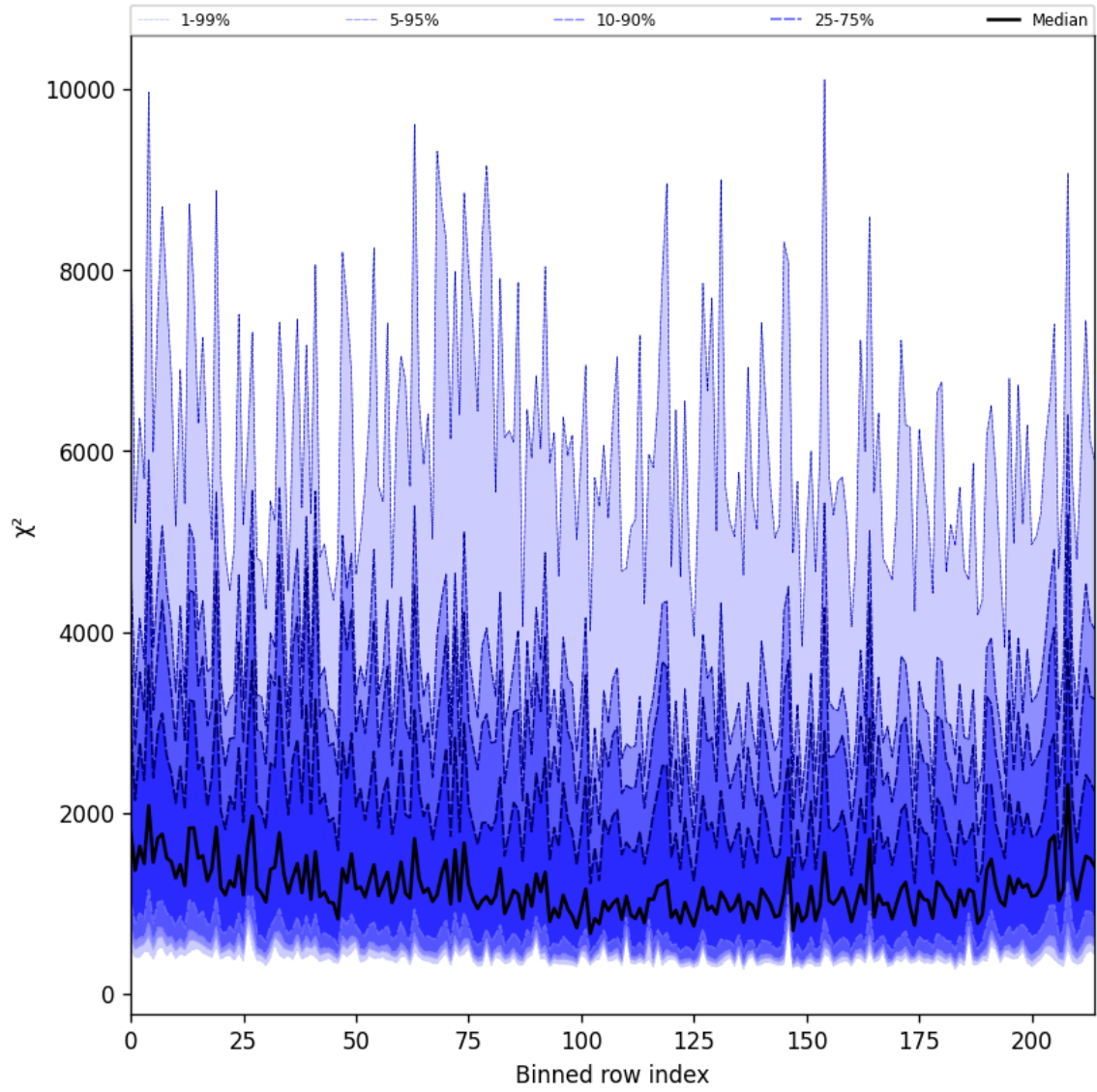
Figure 30: Along track statistics of “ \chi^2 ” for 2025-01-12 to 2025-01-14
