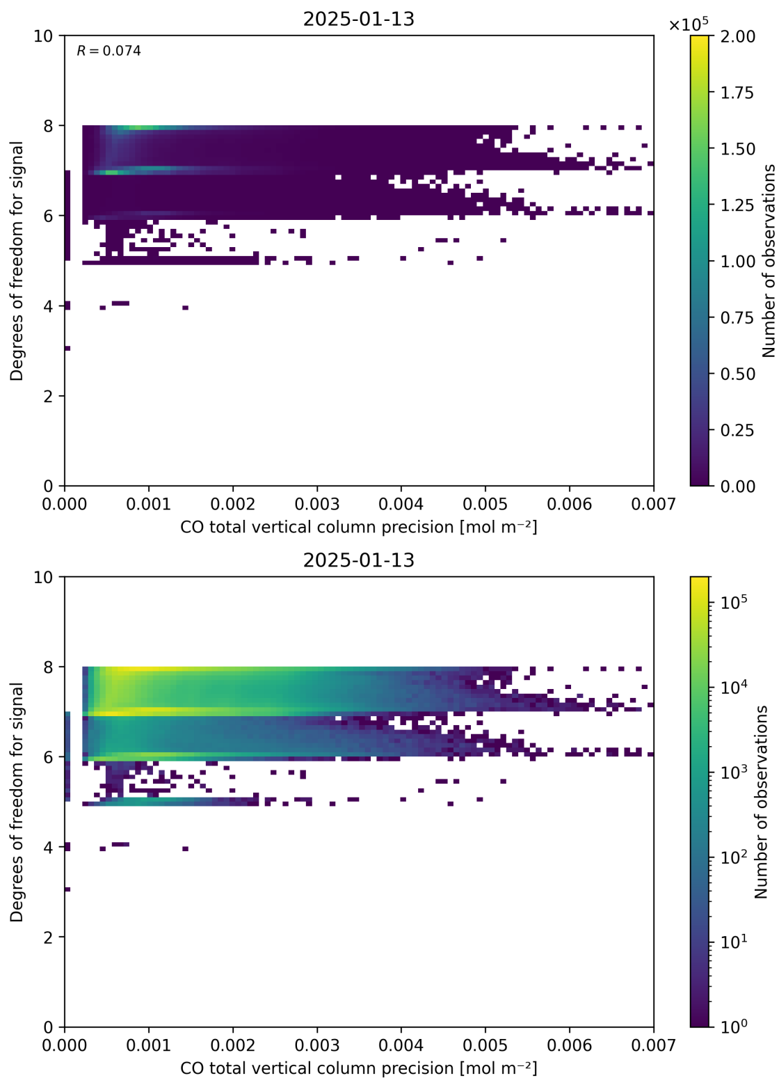
Figure 45: Scatter density plot of “CO total vertical column precision” against “Degrees of freedom for signal” for 2025-01-12 to 2025-01-14.
