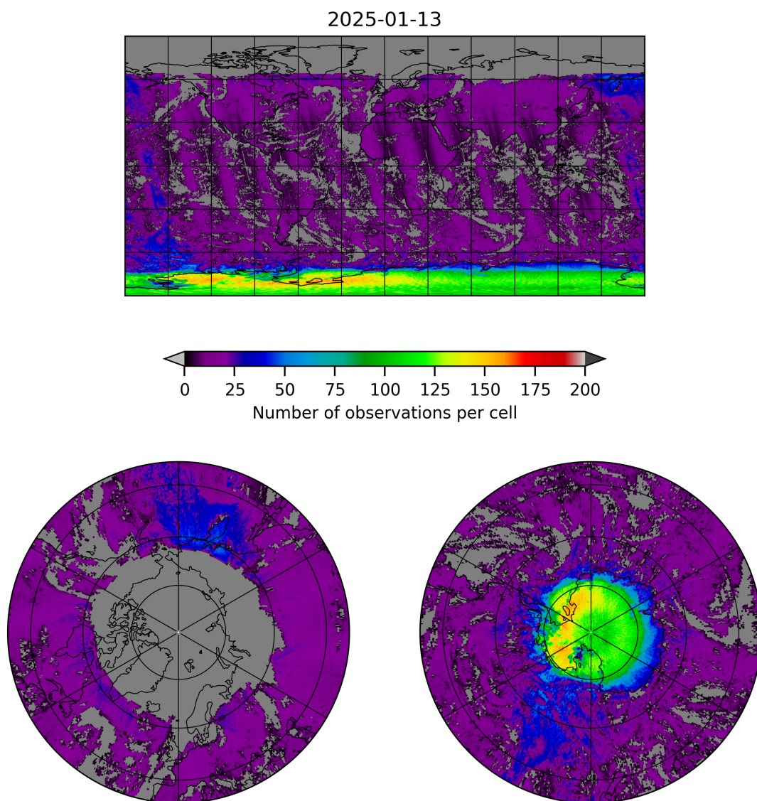
Figure 8: Map of the number of observations for 2025-01-12 to 2025-01-14
