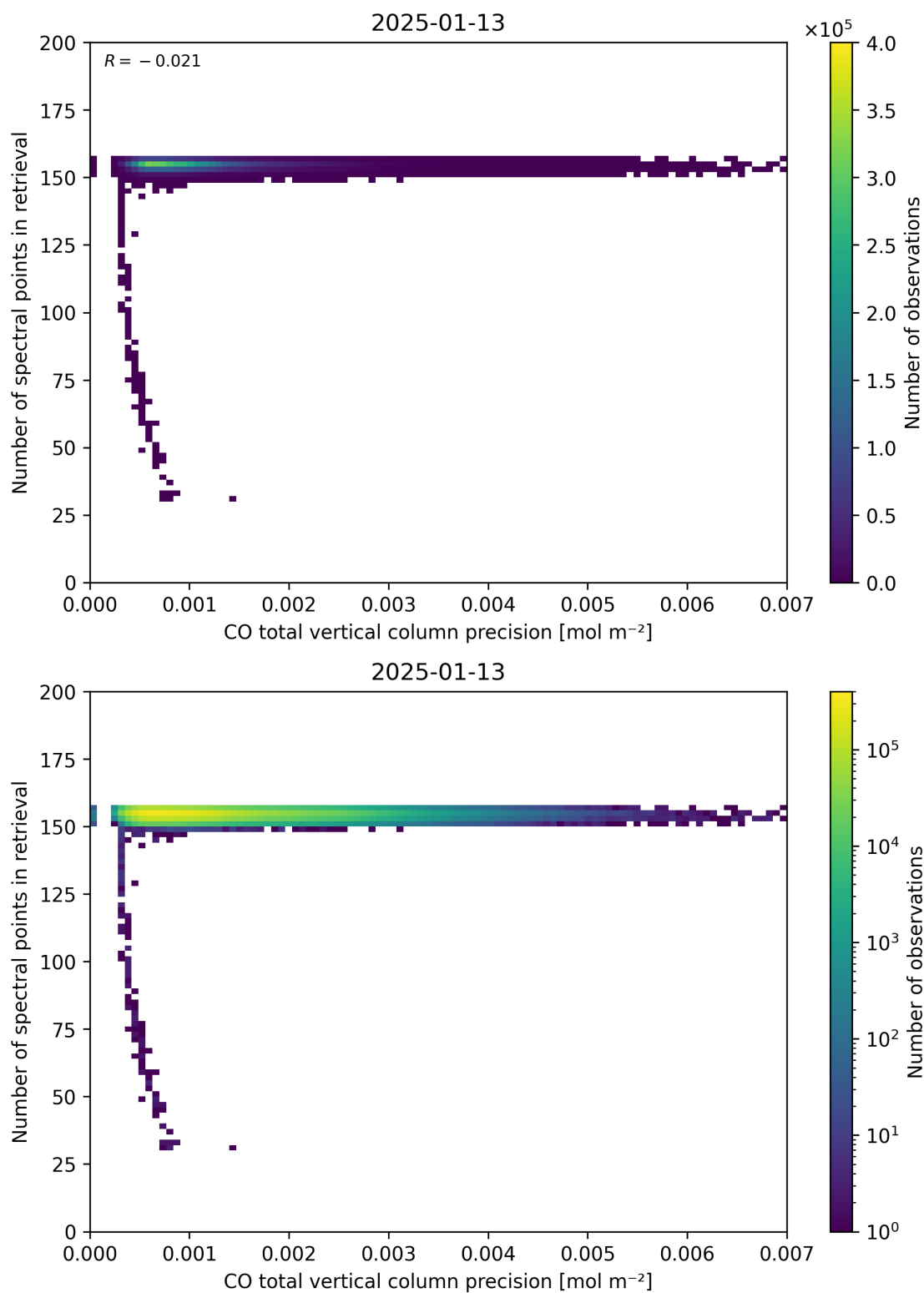
Figure 47: Scatter density plot of “CO total vertical column precision” against “Number of spectral points in retrieval” for 2025-01-12 to 2025-01-14.
