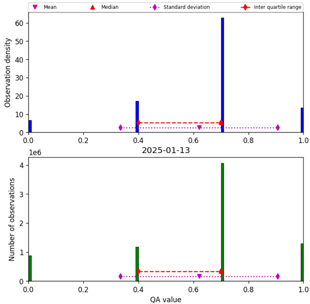
Figure 17: Histogram of “QA value” for 2025-01-12 to 2025-01-14
