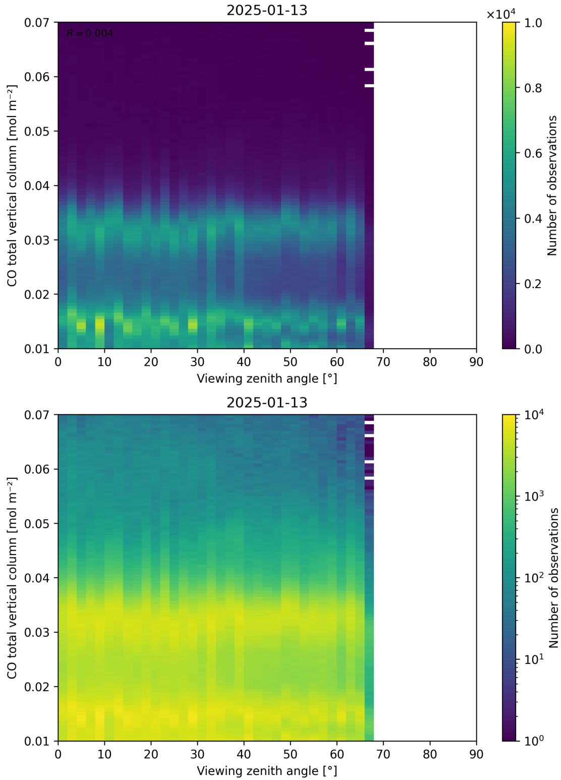
Figure 69: Scatter density plot of “Viewing zenith angle” against “CO total vertical column” for 2025-01-12 to 2025-01-14.
