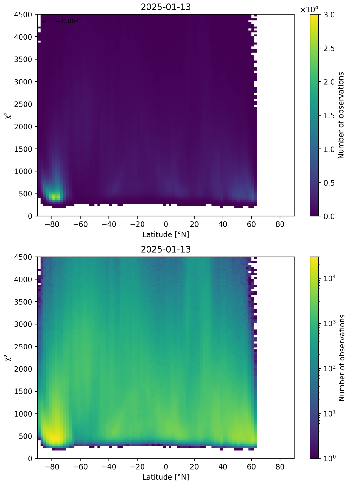
Figure 54: Scatter density plot of “Latitude” against “ \chi^2 ” for 2025-01-12 to 2025-01-14.
