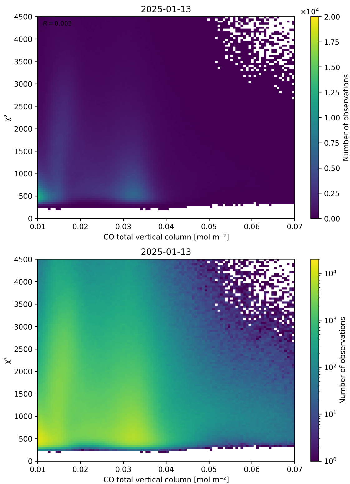
Figure 35: Scatter density plot of “CO total vertical column” against “ \chi^2 ” for 2025-01-12 to 2025-01-14.
