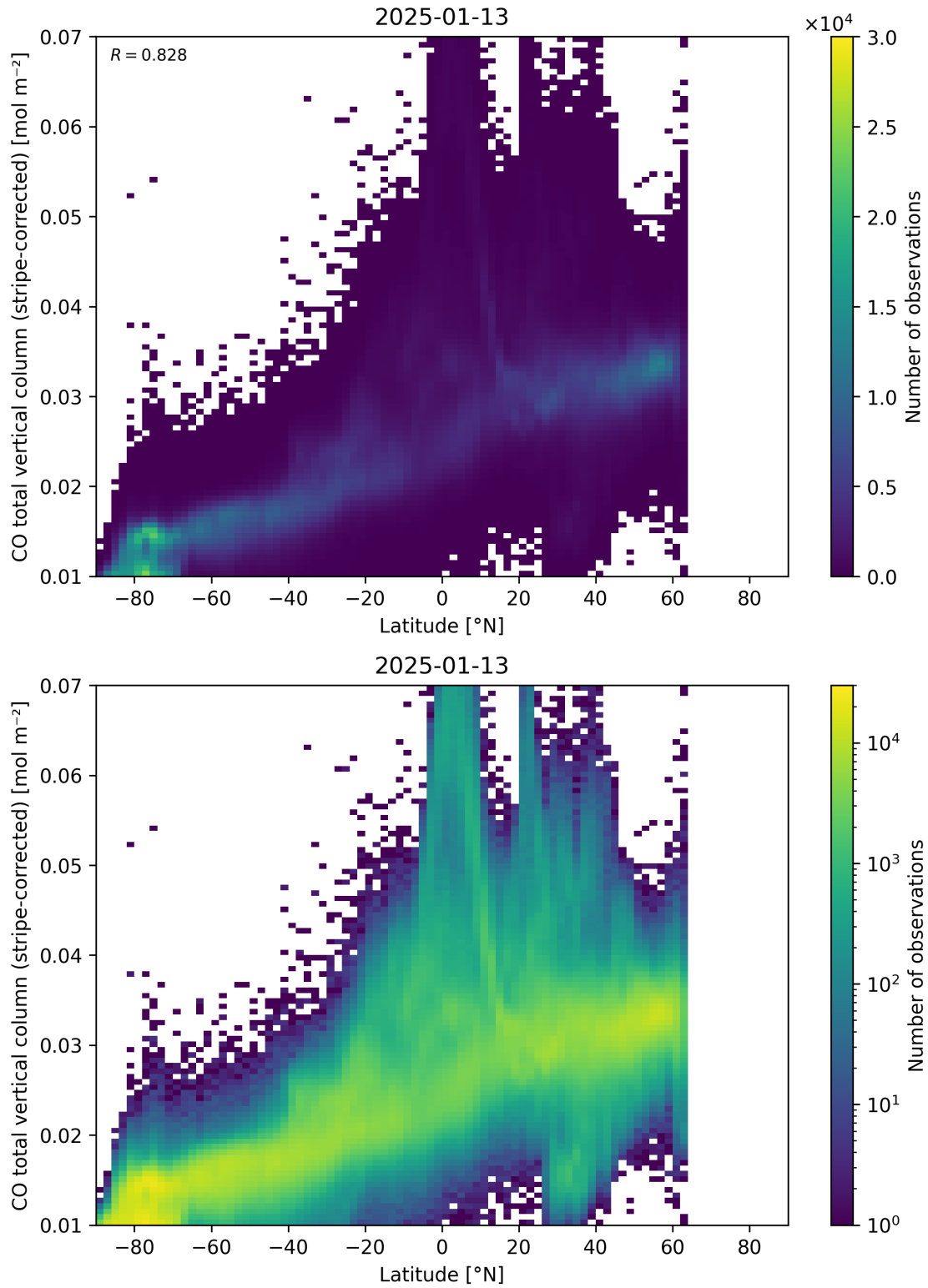
Figure 52: Scatter density plot of “Latitude” against “CO total vertical column (stripe-corrected)” for 2025-01-12 to 2025-01-14.
