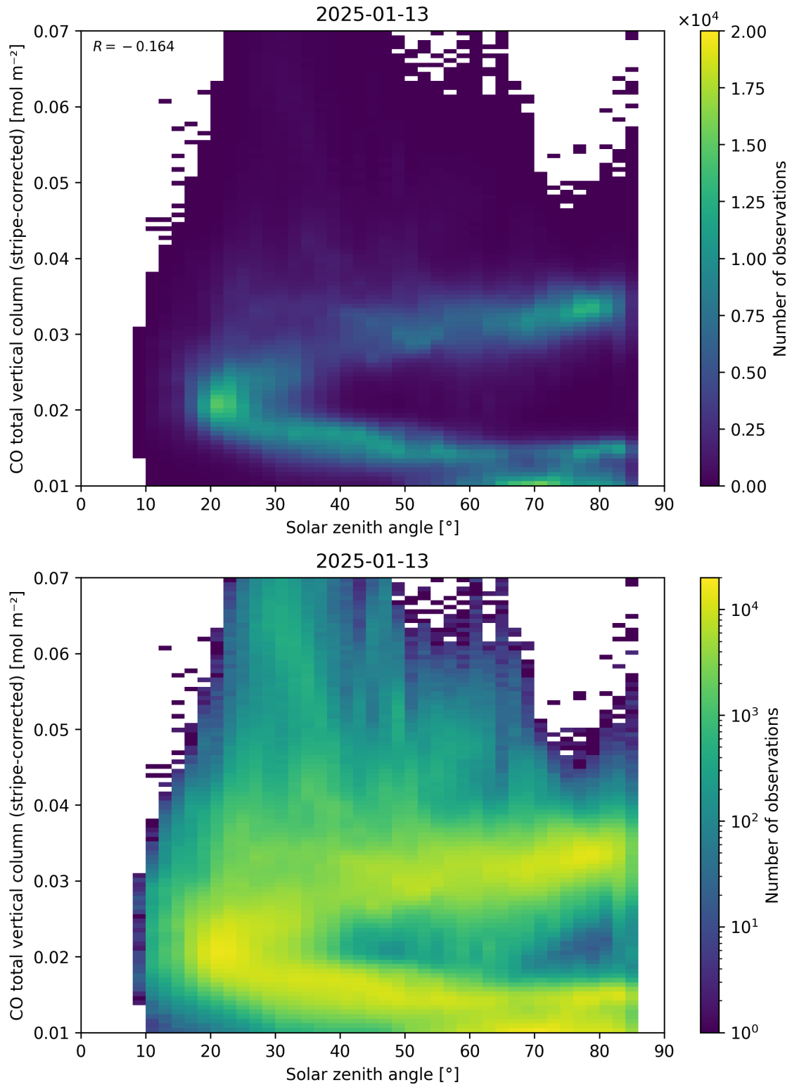
Figure 62: Scatter density plot of “Solar zenith angle” against “CO total vertical column (stripe-corrected)” for 2025-01-12 to 2025-01-14.
