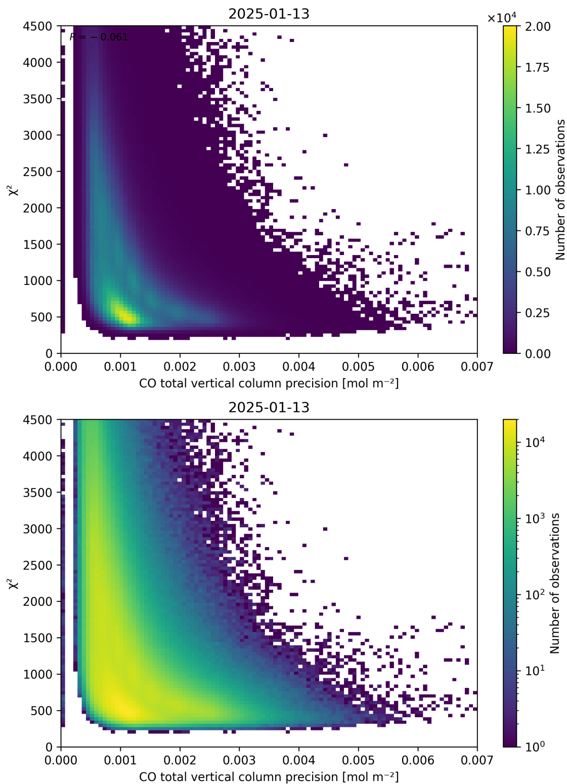
Figure 44: Scatter density plot of “CO total vertical column precision” against “ \chi^2 ” for 2025-01-12 to 2025-01-14.
