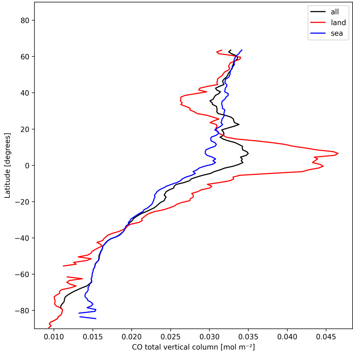
Figure 10: Zonal average of “CO total vertical column” for 2025-01-12 to 2025-01-14.
