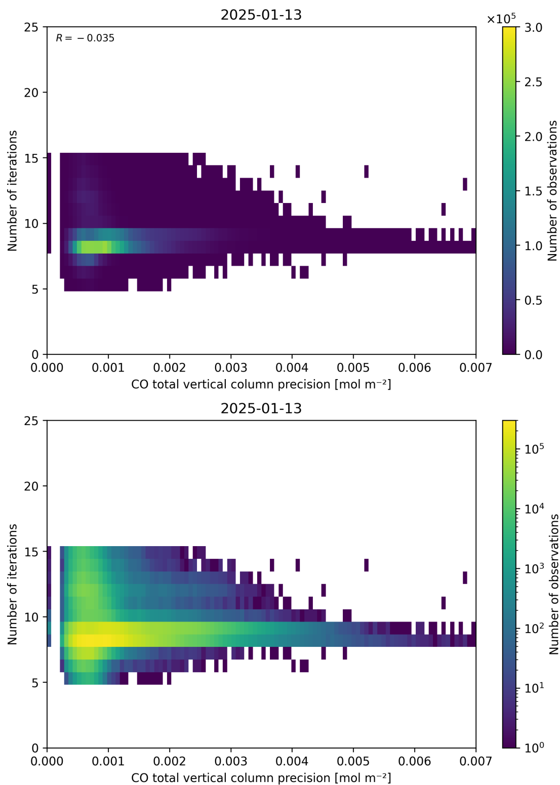
Figure 46: Scatter density plot of “CO total vertical column precision” against “Number of iterations” for 2025-01-12 to 2025-01-14.
