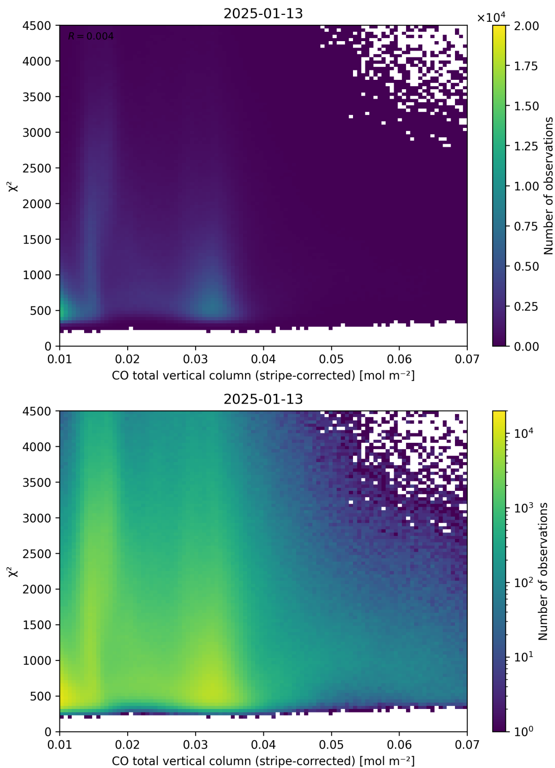
Figure 37: Scatter density plot of “CO total vertical column (stripe-corrected)” against “ \chi^2 ” for 2025-01-12 to 2025-01-14.
