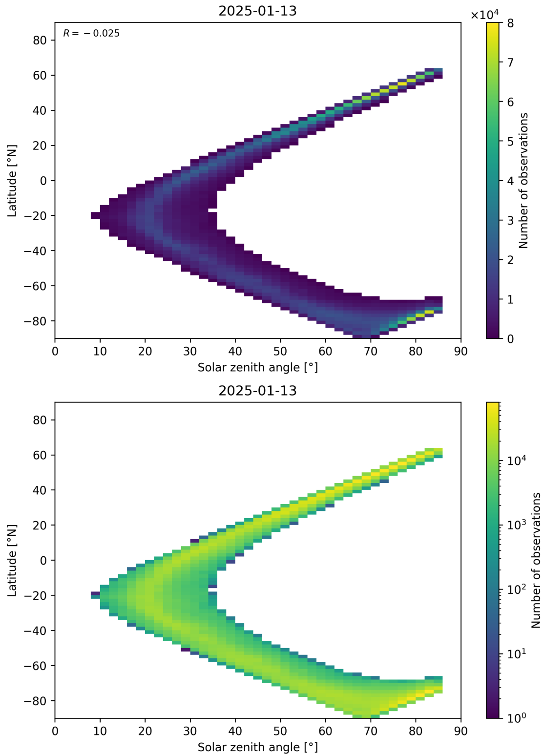
Figure 66: Scatter density plot of “Solar zenith angle” against “Latitude” for 2025-01-12 to 2025-01-14.
