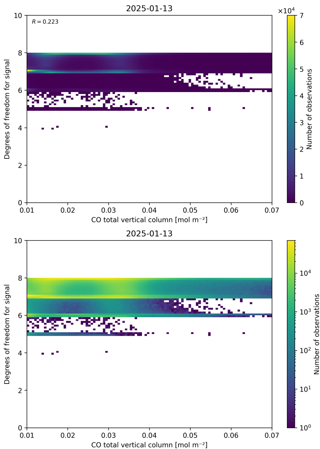
Figure 41: Scatter density plot of “CO total vertical column” against “Degrees of freedom for signal” for 2025-01-12 to 2025-01-14.
