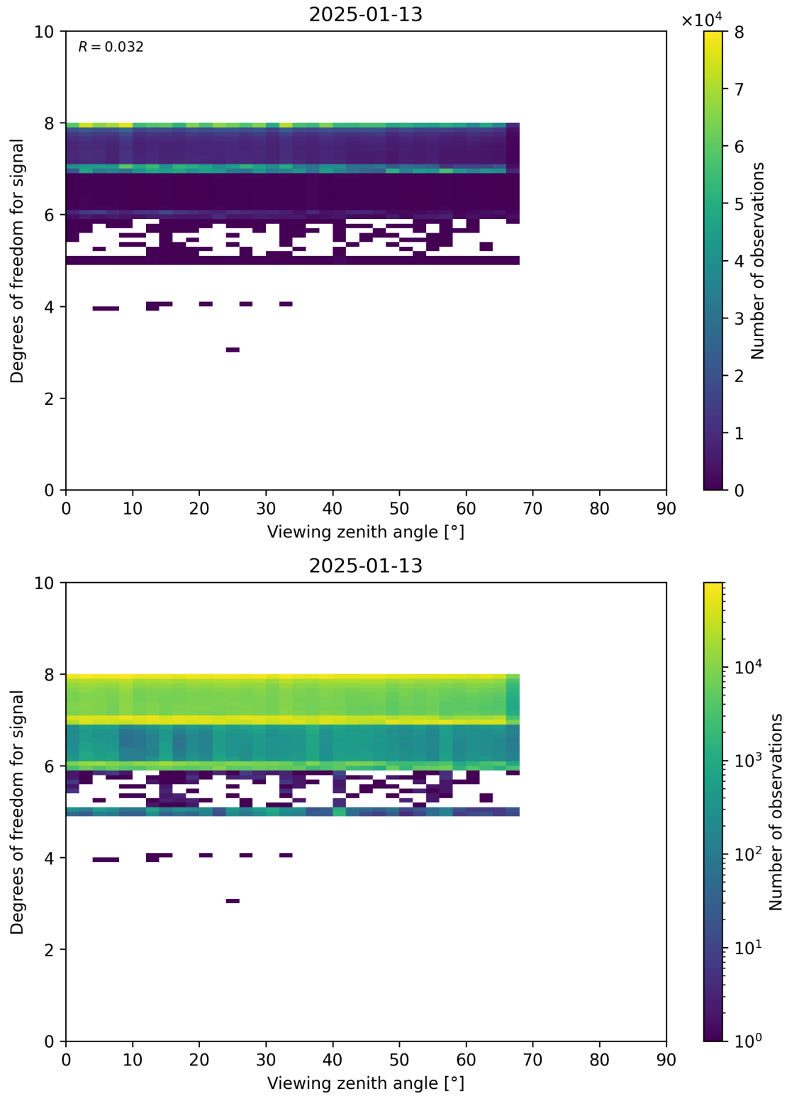
Figure 73: Scatter density plot of “Viewing zenith angle” against “Degrees of freedom for signal” for 2025-01-12 to 2025-01-14.
