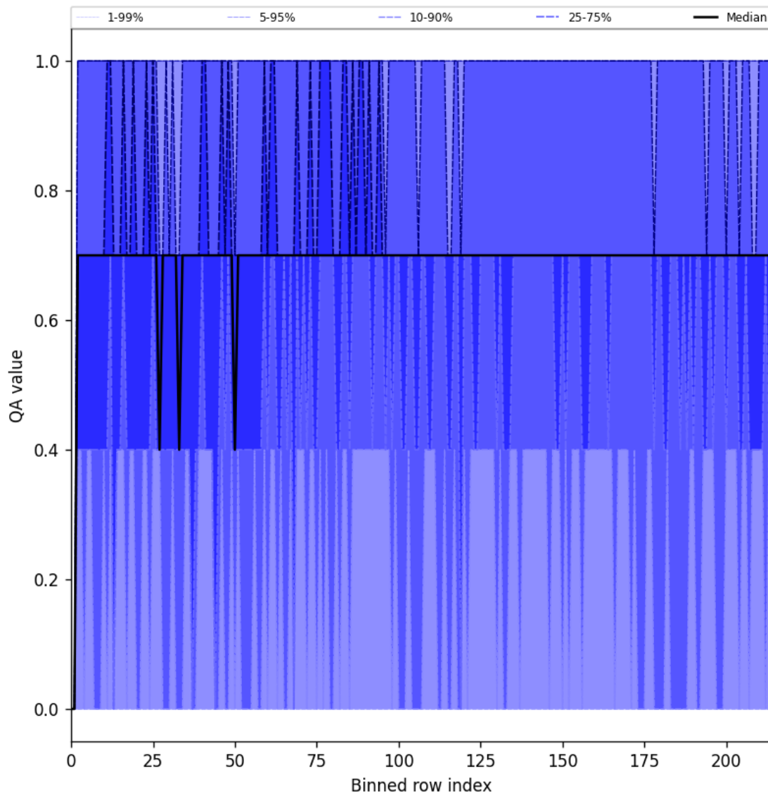
Figure 25: Along track statistics of “QA value” for 2025-01-12 to 2025-01-14
