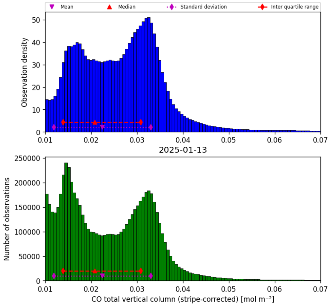
Figure 19: Histogram of “CO total vertical column (stripe-corrected)” for 2025-01-12 to 2025-01-14
