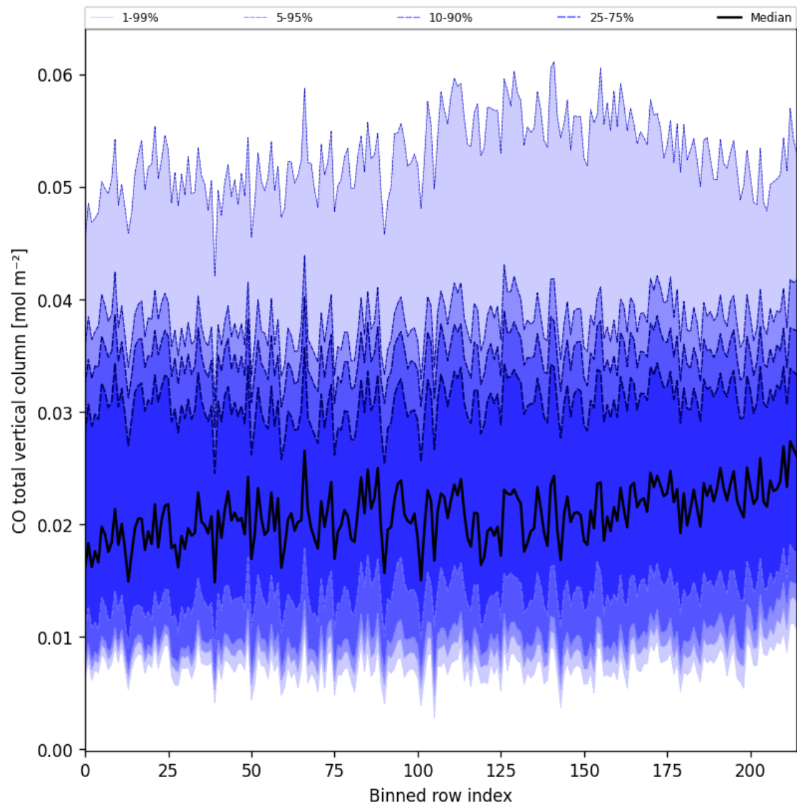
Figure 26: Along track statistics of “CO total vertical column” for 2025-01-12 to 2025-01-14
