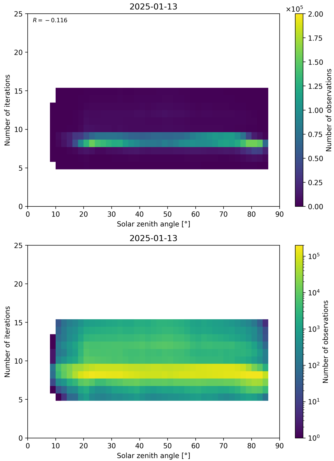
Figure 67: Scatter density plot of “Solar zenith angle” against “Number of iterations” for 2025-01-12 to 2025-01-14.
