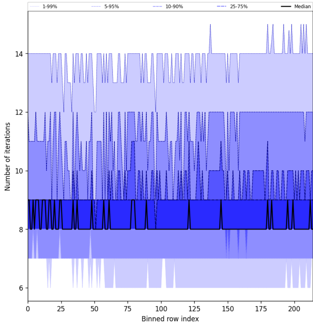
Figure 32: Along track statistics of “Number of iterations” for 2025-01-12 to 2025-01-14
