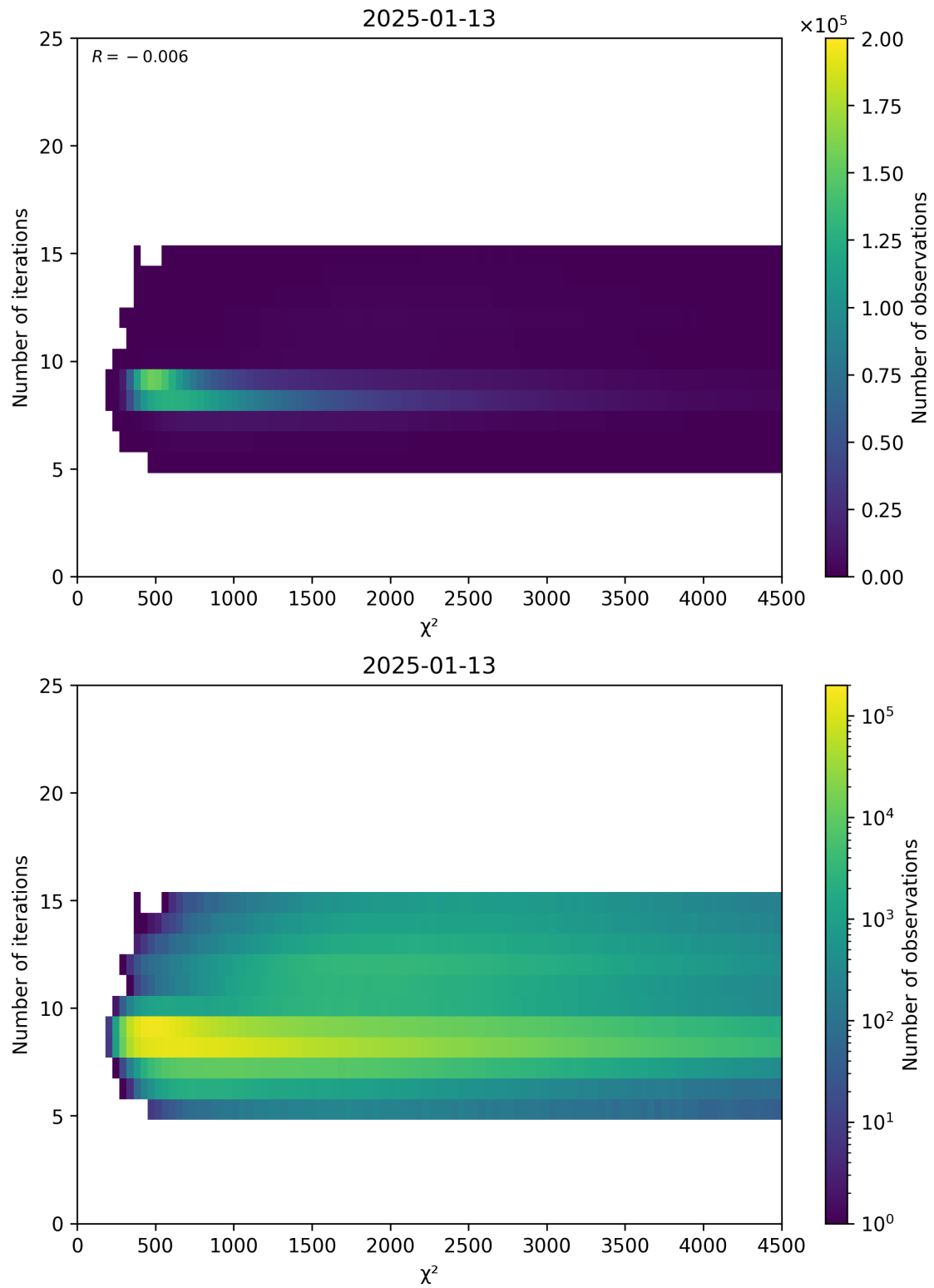
Figure 49: Scatter density plot of “ \chi^2 ” against “Number of iterations” for 2025-01-12 to 2025-01-14.
