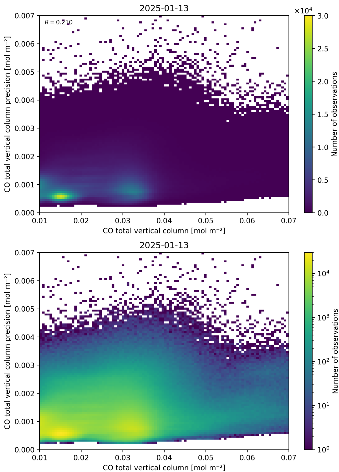
Figure 34: Scatter density plot of “CO total vertical column” against “CO total vertical column precision” for 2025-01-12 to 2025-01-14.
