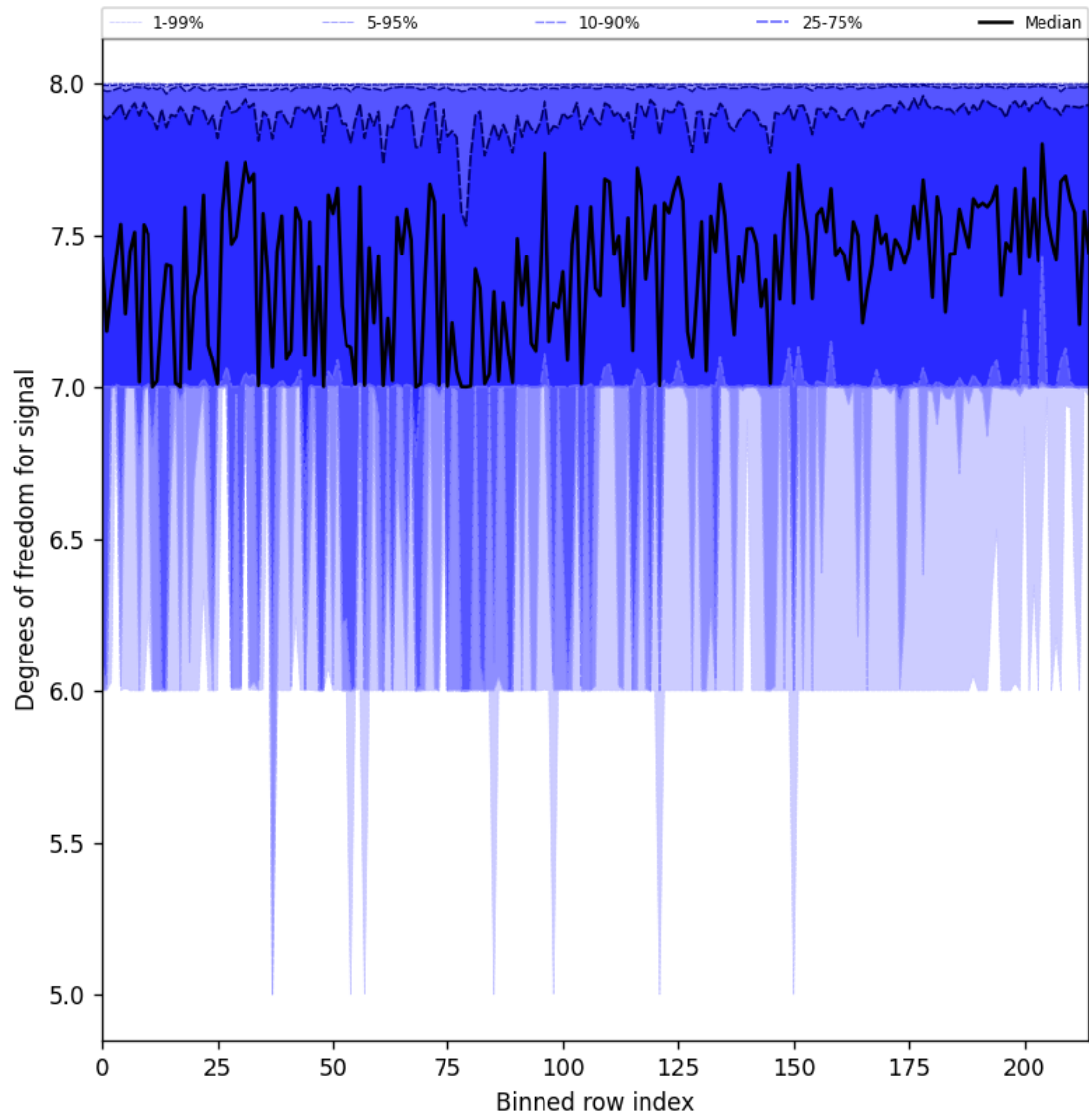
Figure 31: Along track statistics of “Degrees of freedom for signal” for 2025-01-13 to 2025-01-15
