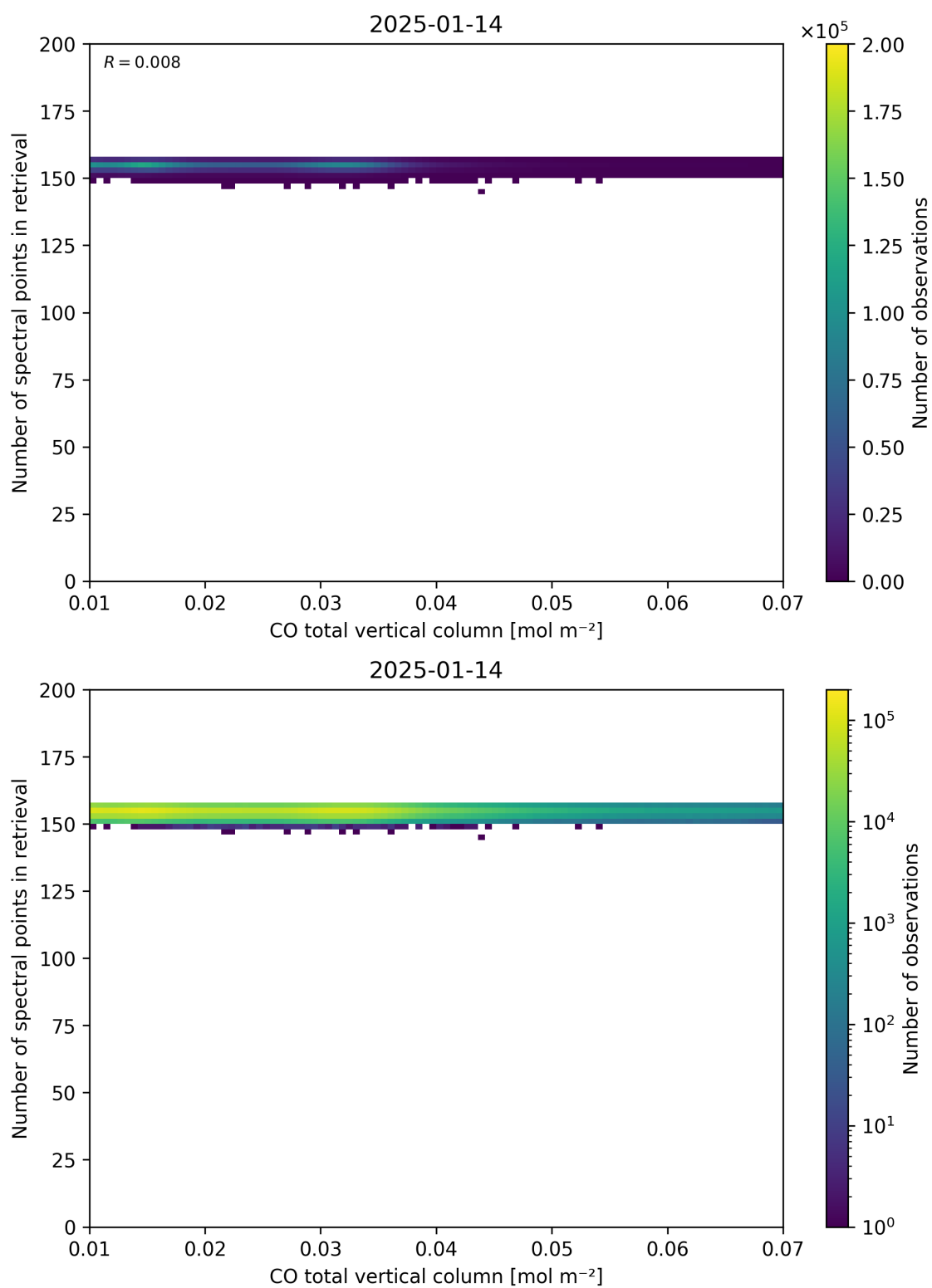
Figure 43: Scatter density plot of “CO total vertical column” against “Number of spectral points in retrieval” for 2025-01-13 to 2025-01-15.
