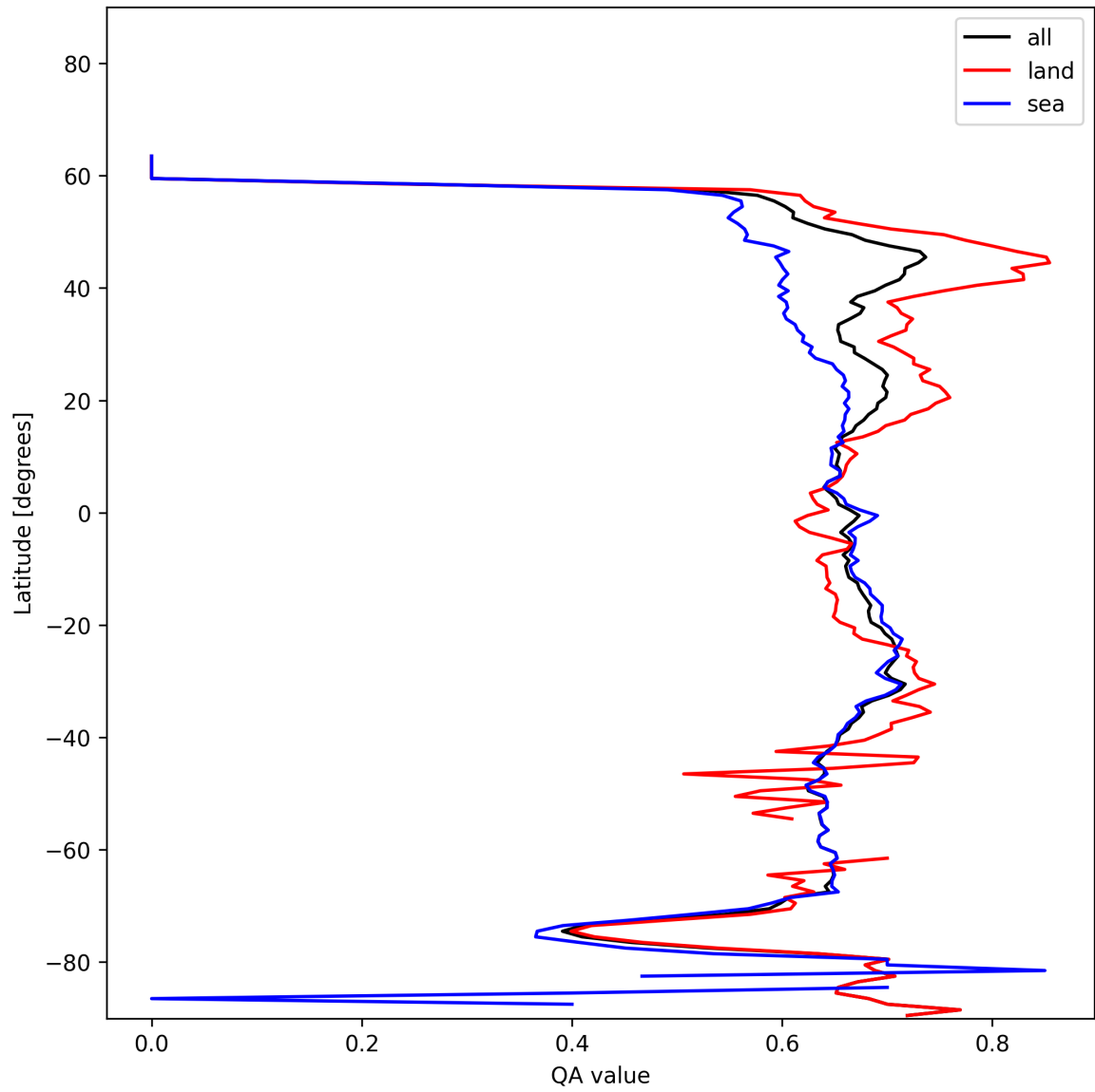
Figure 9: Zonal average of “QA value” for 2025-01-13 to 2025-01-15.
