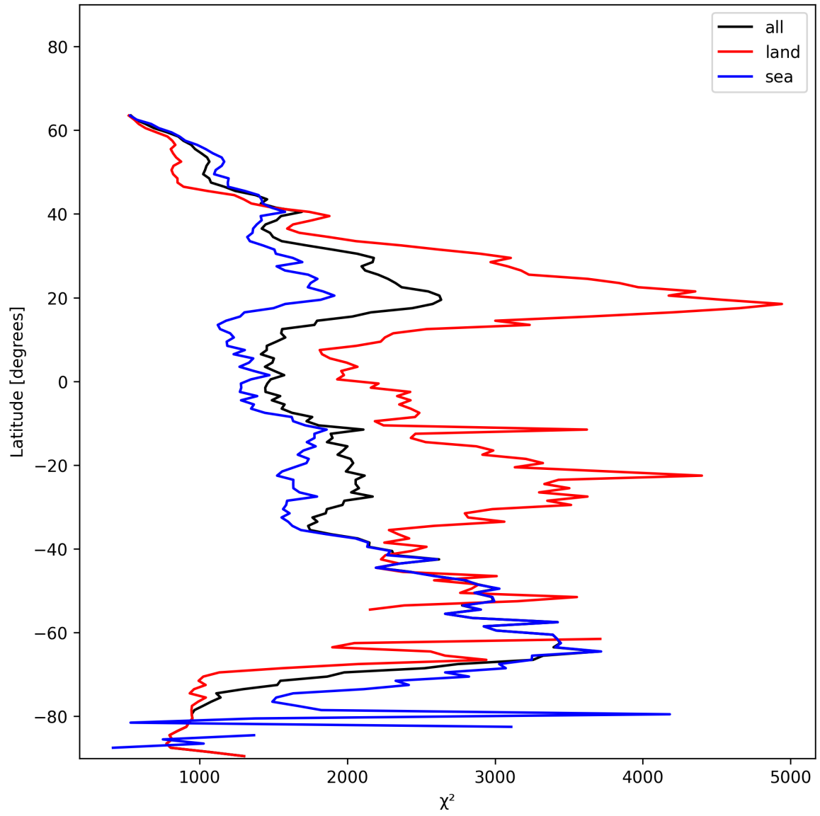
Figure 14: Zonal average of “ \chi^2 ” for 2025-01-13 to 2025-01-15.
