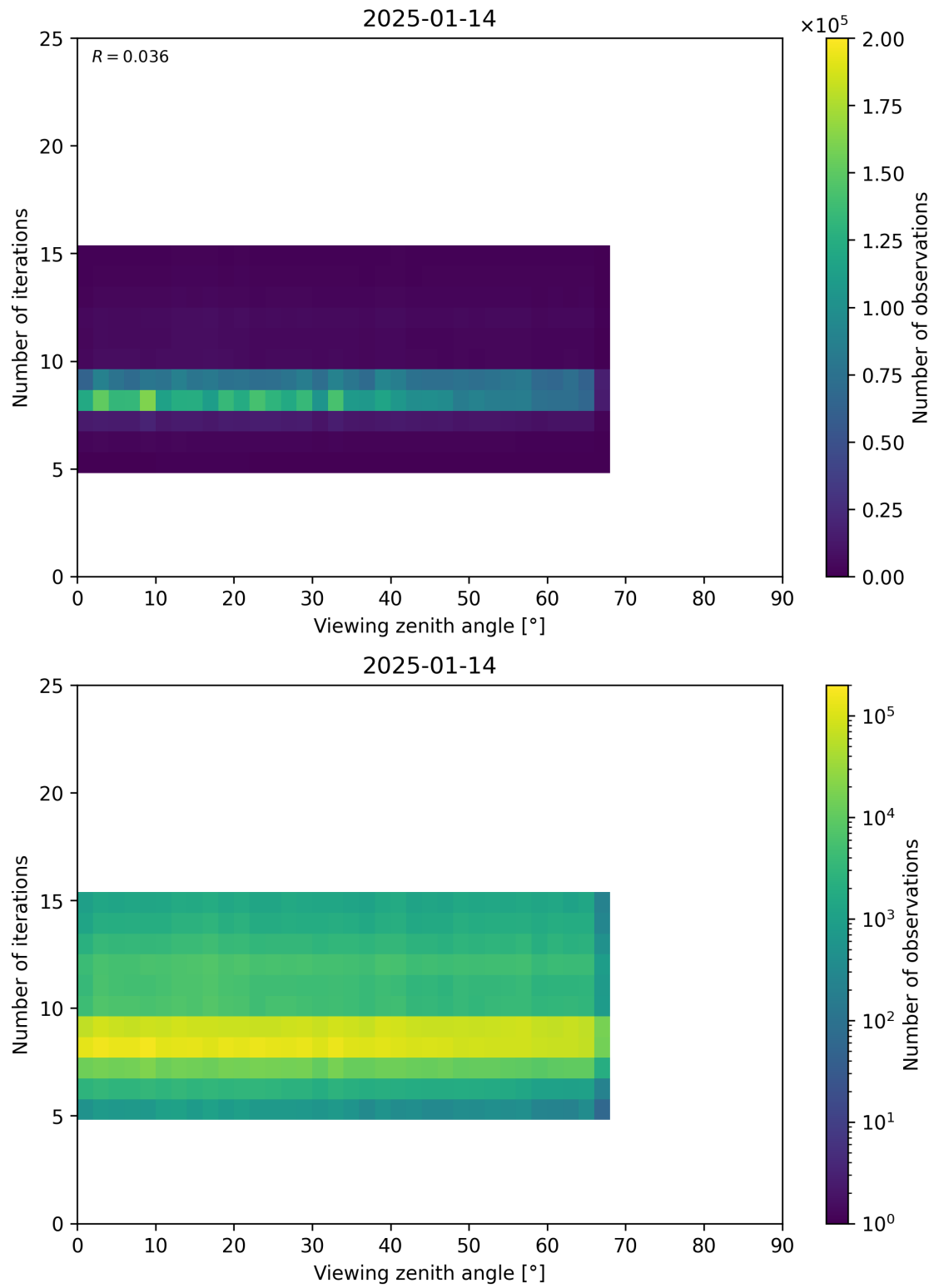
Figure 75: Scatter density plot of “Viewing zenith angle” against “Number of iterations” for 2025-01-13 to 2025-01-15.
