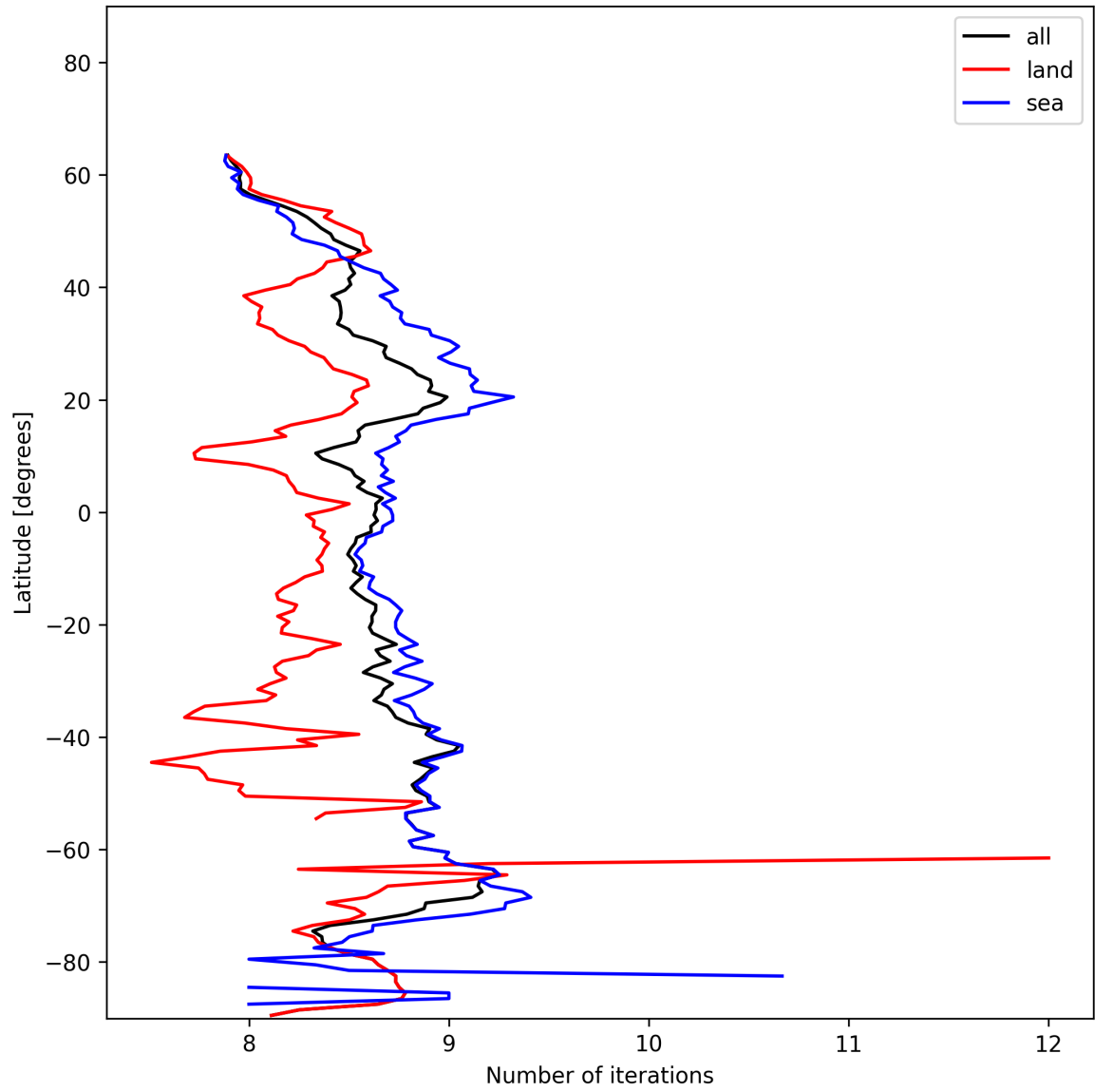
Figure 16: Zonal average of “Number of iterations” for 2025-01-13 to 2025-01-15.
