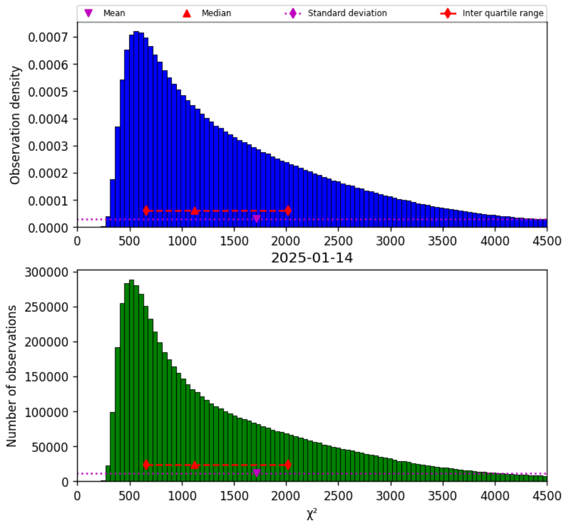
Figure 22: Histogram of “ \chi^2 ” for 2025-01-13 to 2025-01-15
