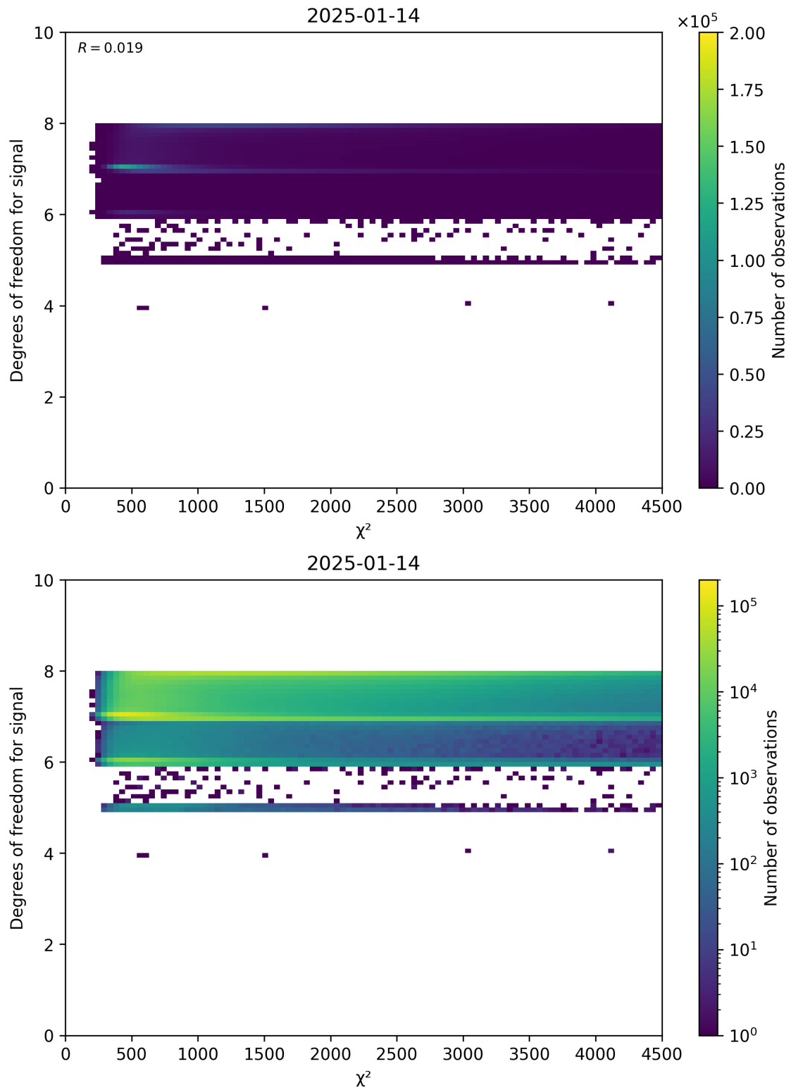
Figure 48: Scatter density plot of “ \chi^2 ” against “Degrees of freedom for signal” for 2025-01-13 to 2025-01-15.
