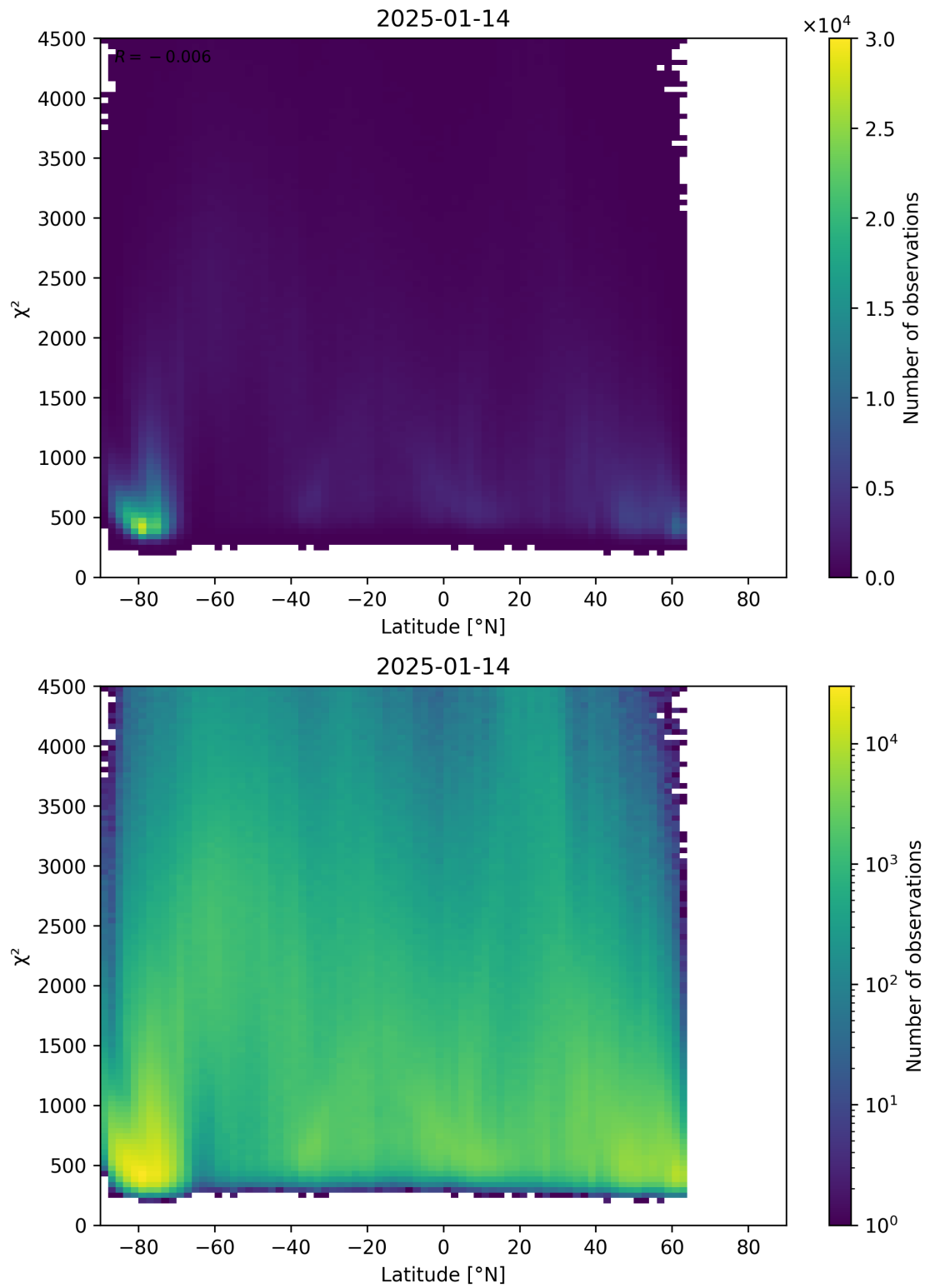
Figure 54: Scatter density plot of “Latitude” against “ \chi^2 ” for 2025-01-13 to 2025-01-15.
