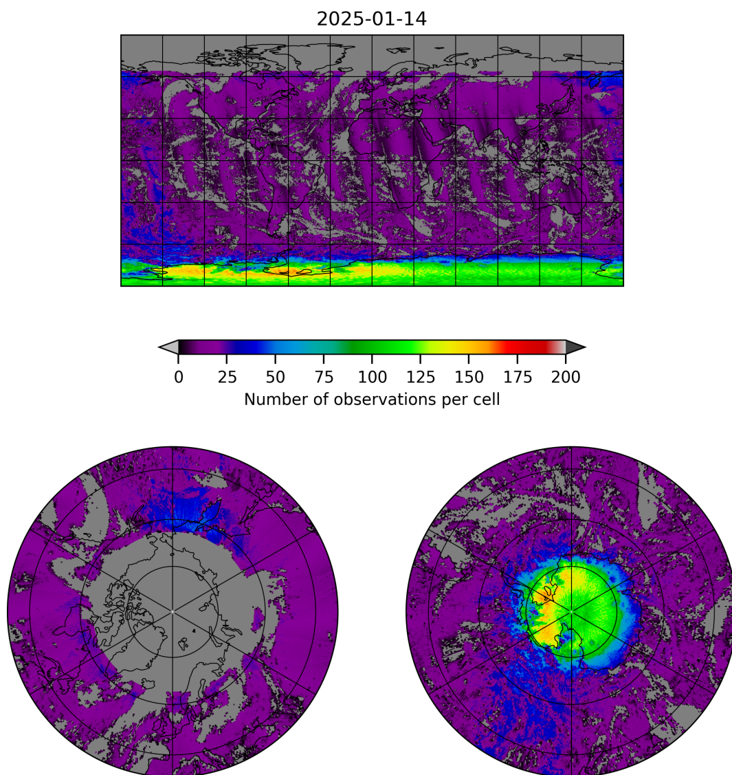
Figure 8: Map of the number of observations for 2025-01-13 to 2025-01-15
