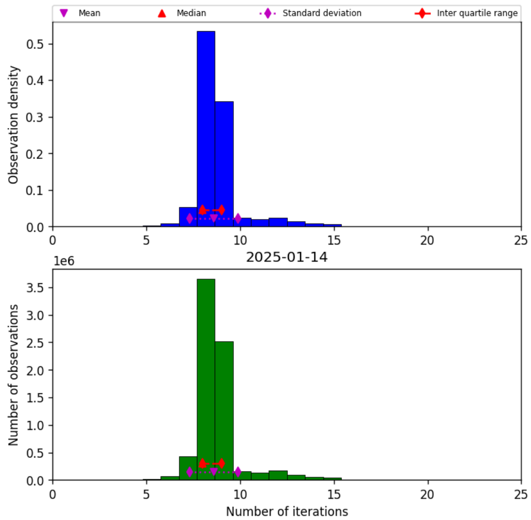
Figure 24: Histogram of “Number of iterations” for 2025-01-13 to 2025-01-15
