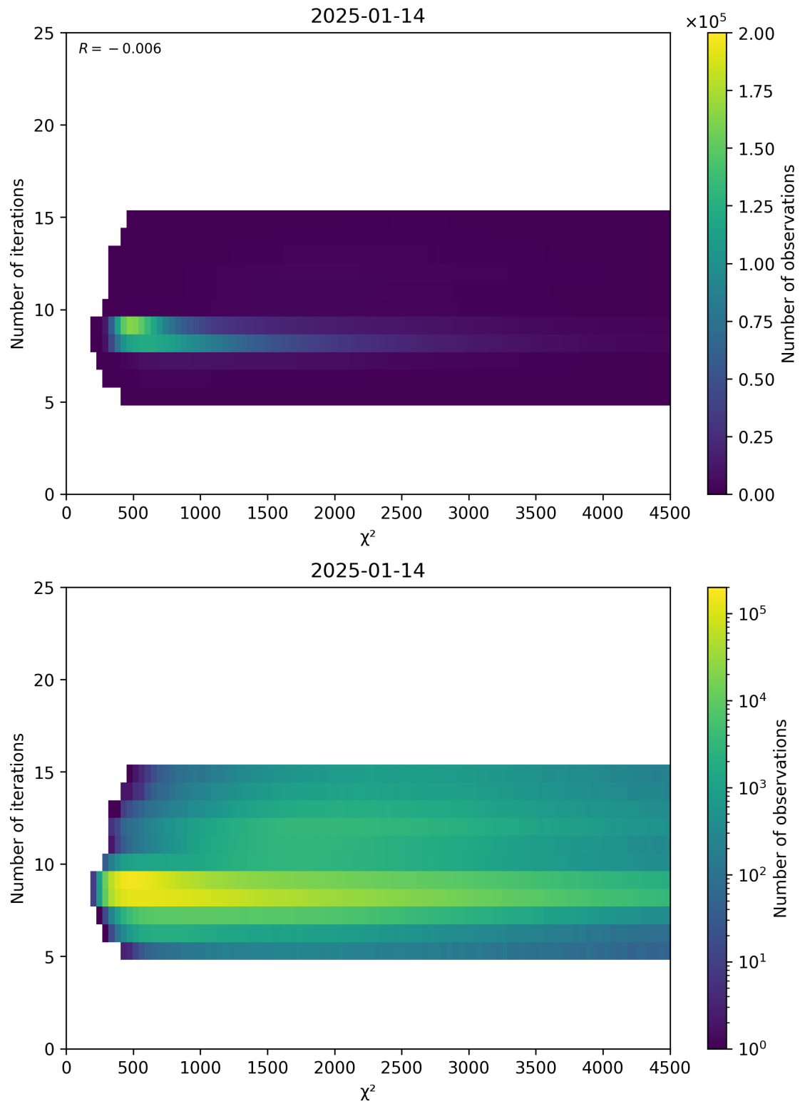
Figure 49: Scatter density plot of “ \chi^2 ” against “Number of iterations” for 2025-01-13 to 2025-01-15.
