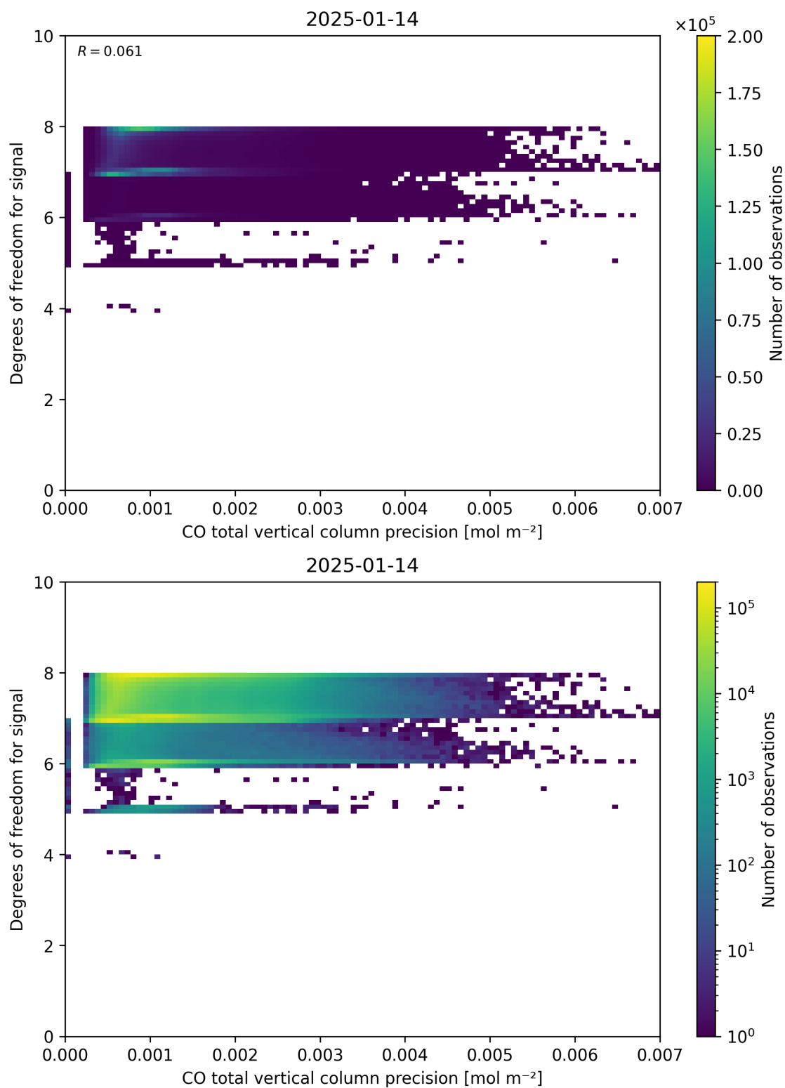
Figure 45: Scatter density plot of “CO total vertical column precision” against “Degrees of freedom for signal” for 2025-01-13 to 2025-01-15.
