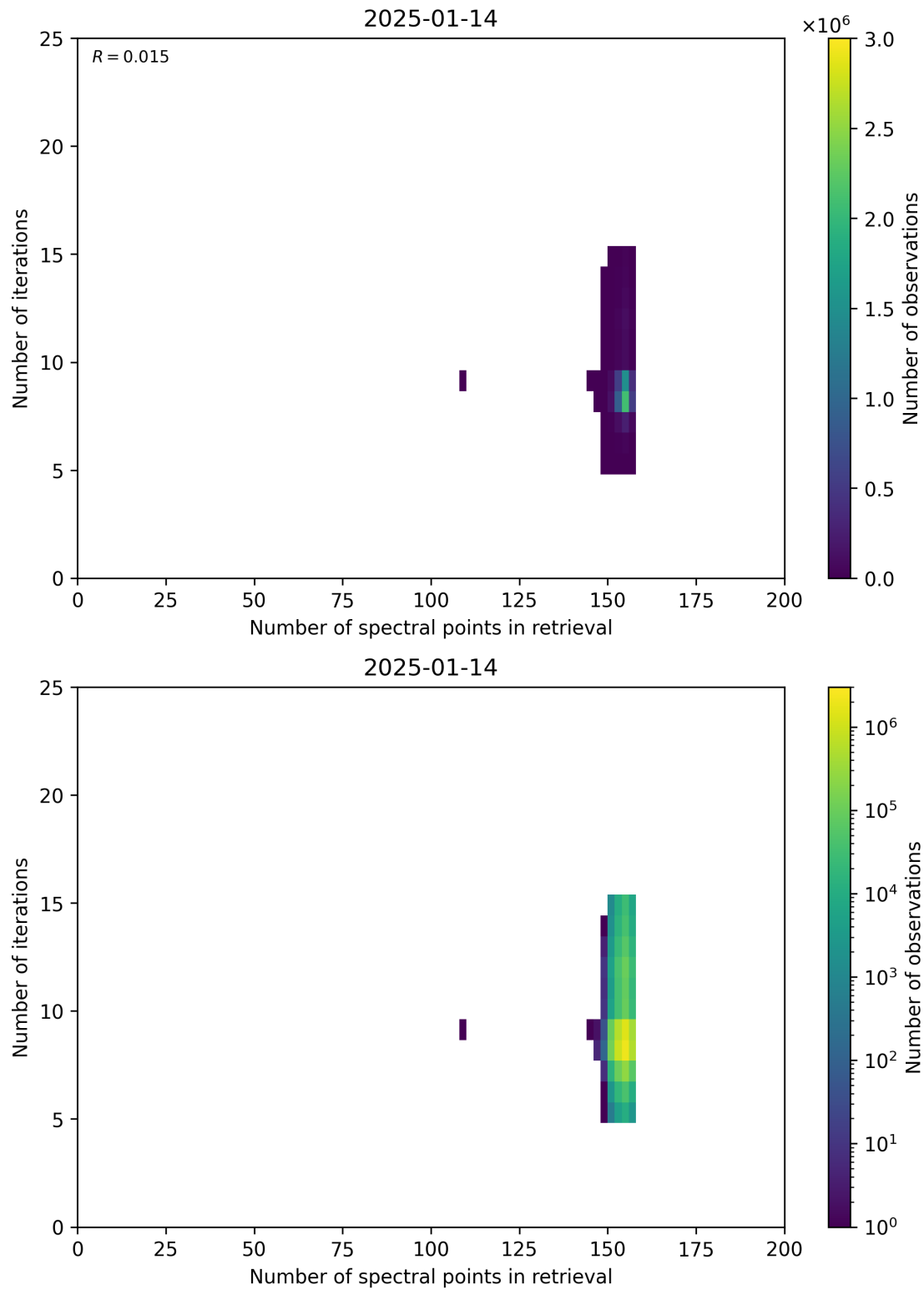
Figure 60: Scatter density plot of “Number of spectral points in retrieval” against “Number of iterations” for 2025-01-13 to 2025-01-15.
