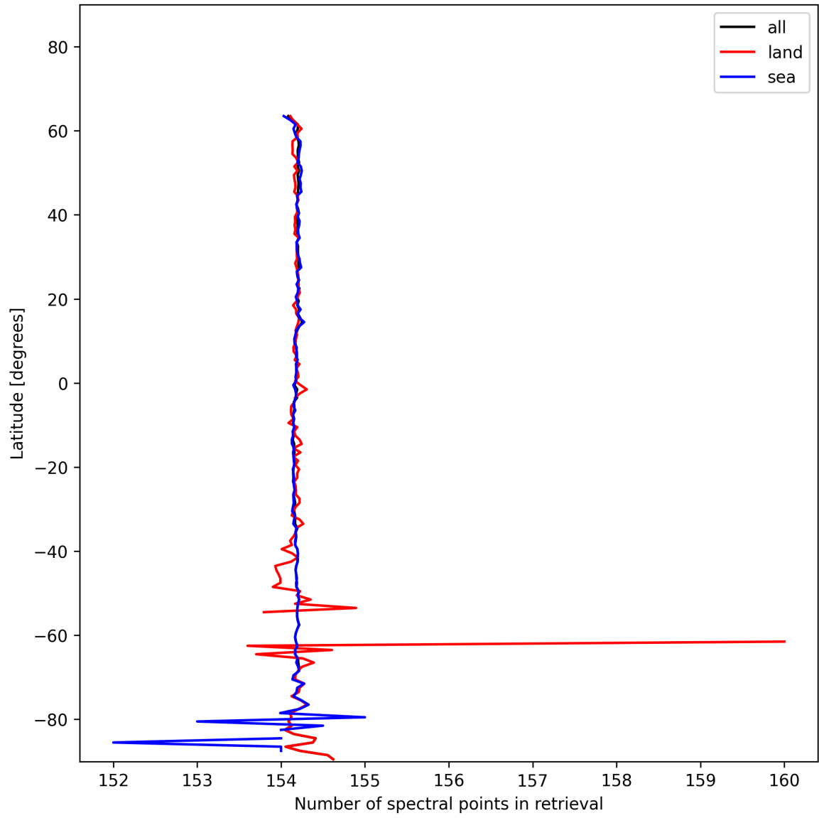
Figure 13: Zonal average of “Number of spectral points in retrieval” for 2025-01-13 to 2025-01-15.
