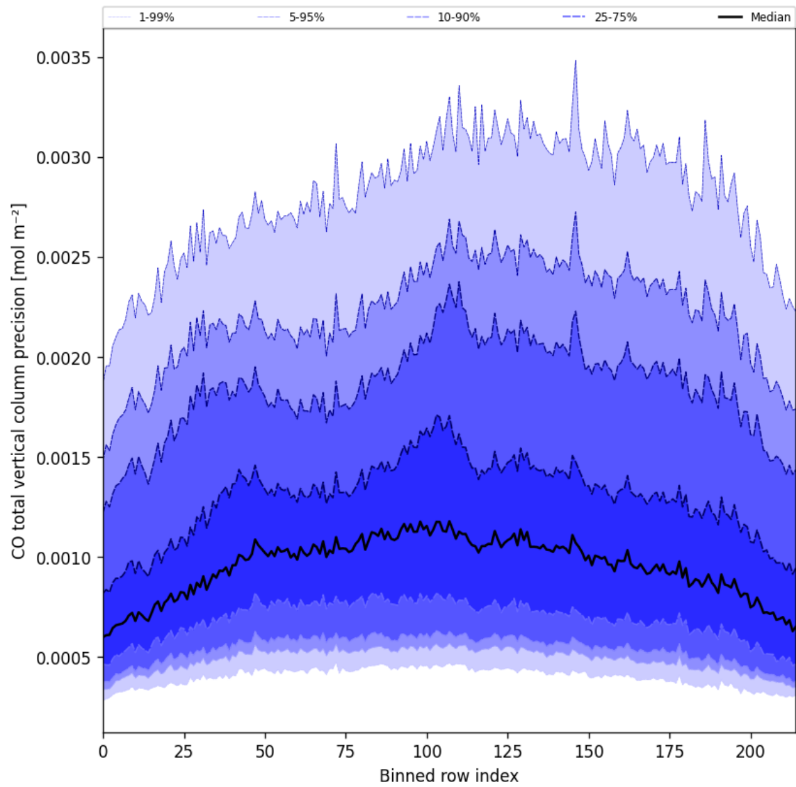
Figure 28: Along track statistics of “CO total vertical column precision” for 2025-01-13 to 2025-01-15
