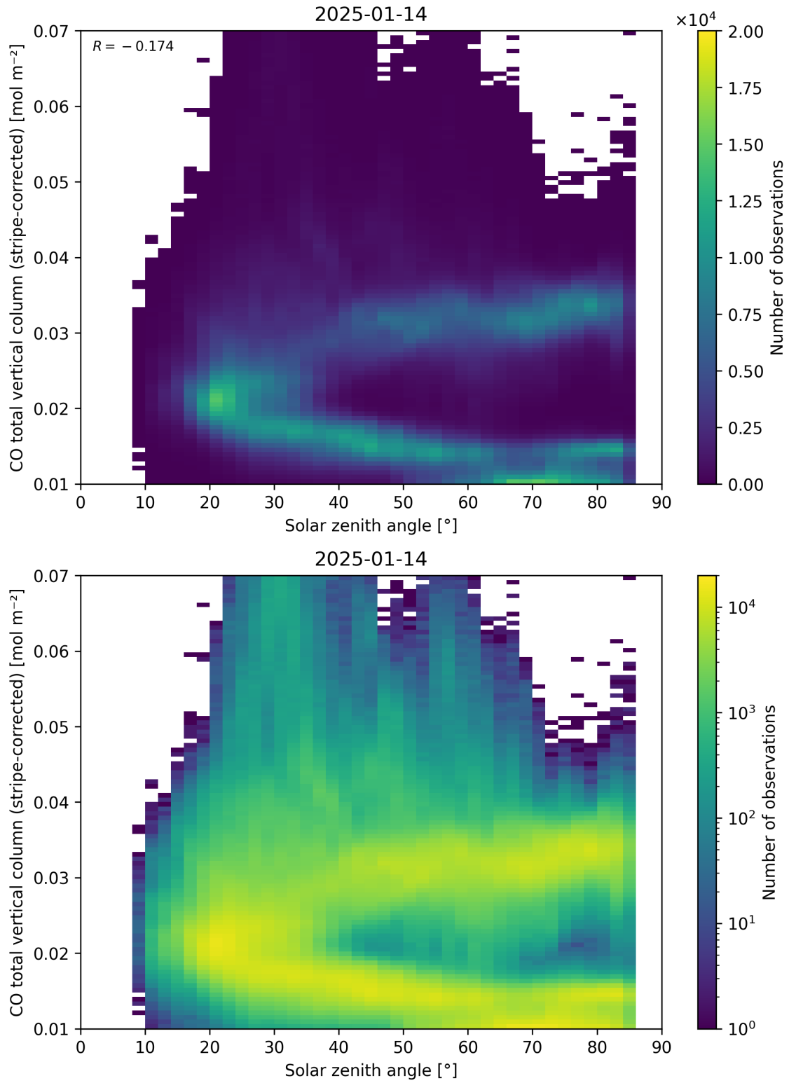
Figure 62: Scatter density plot of “Solar zenith angle” against “CO total vertical column (stripe-corrected)” for 2025-01-13 to 2025-01-15.
