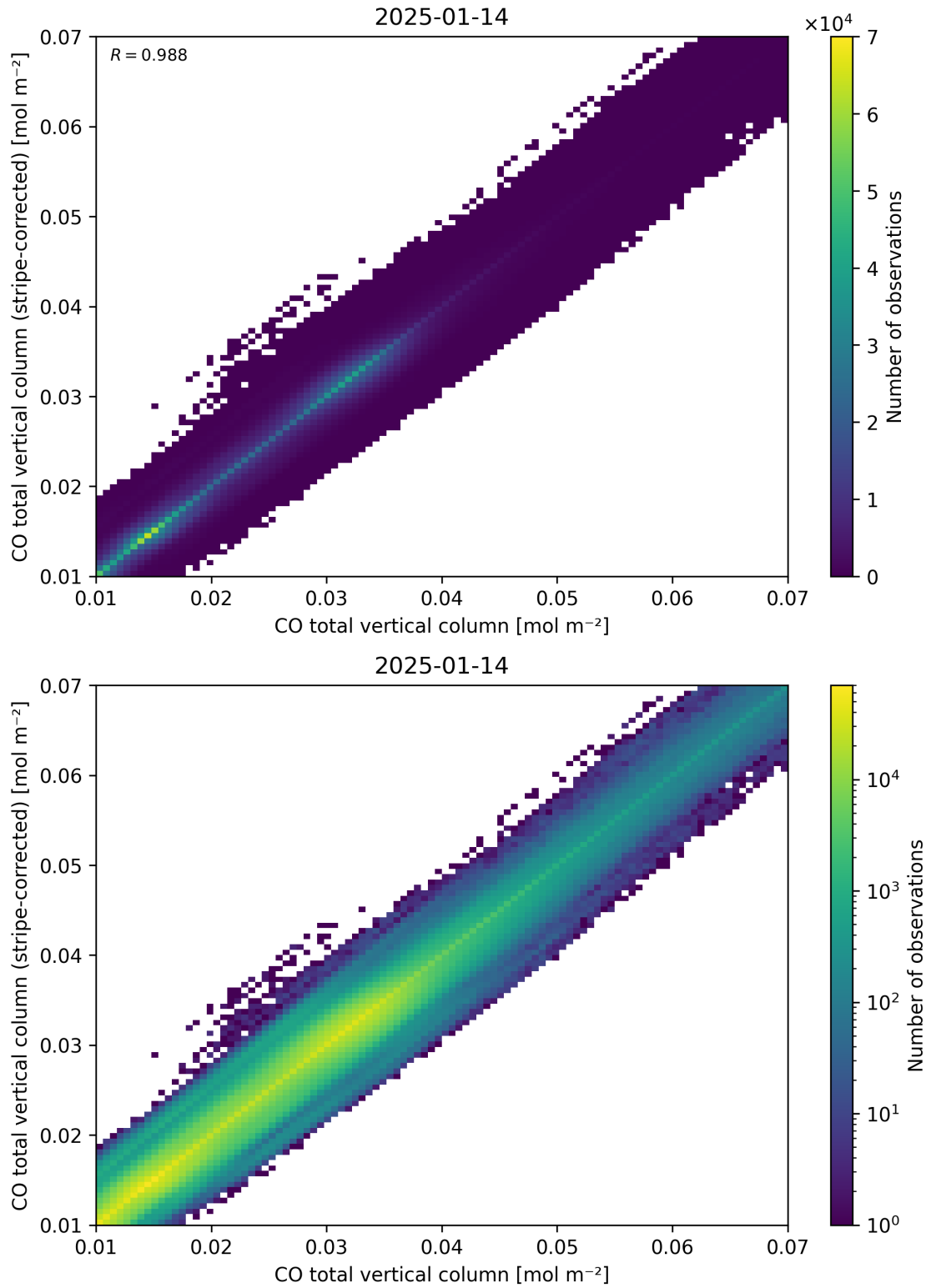
Figure 33: Scatter density plot of “CO total vertical column” against “CO total vertical column (stripe-corrected)” for 2025-01-13 to 2025-01-15.
