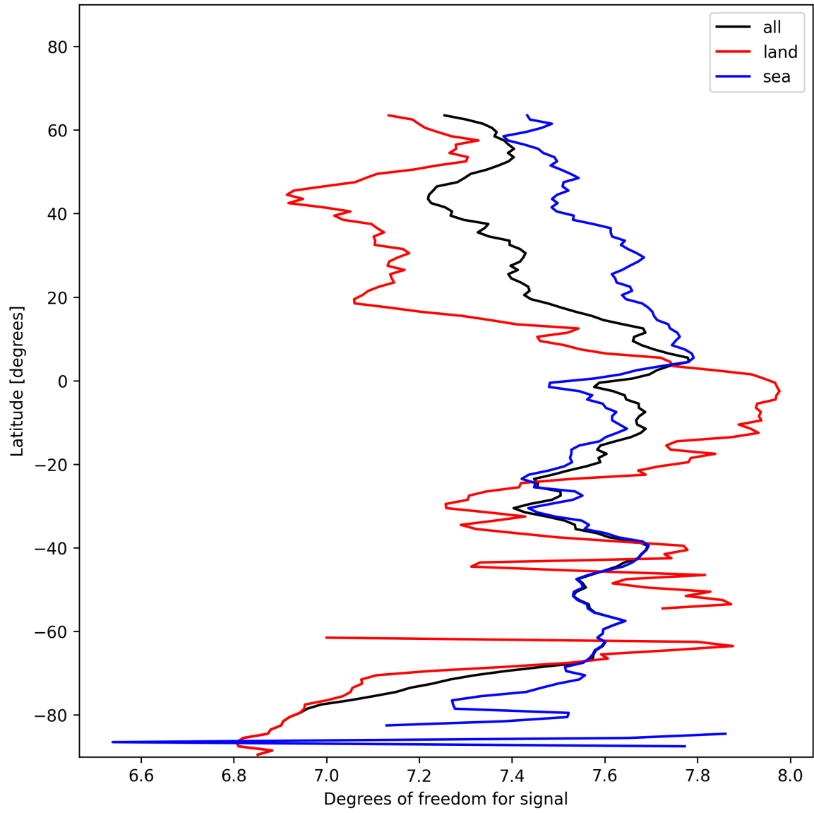
Figure 15: Zonal average of “Degrees of freedom for signal” for 2025-01-13 to 2025-01-15.
