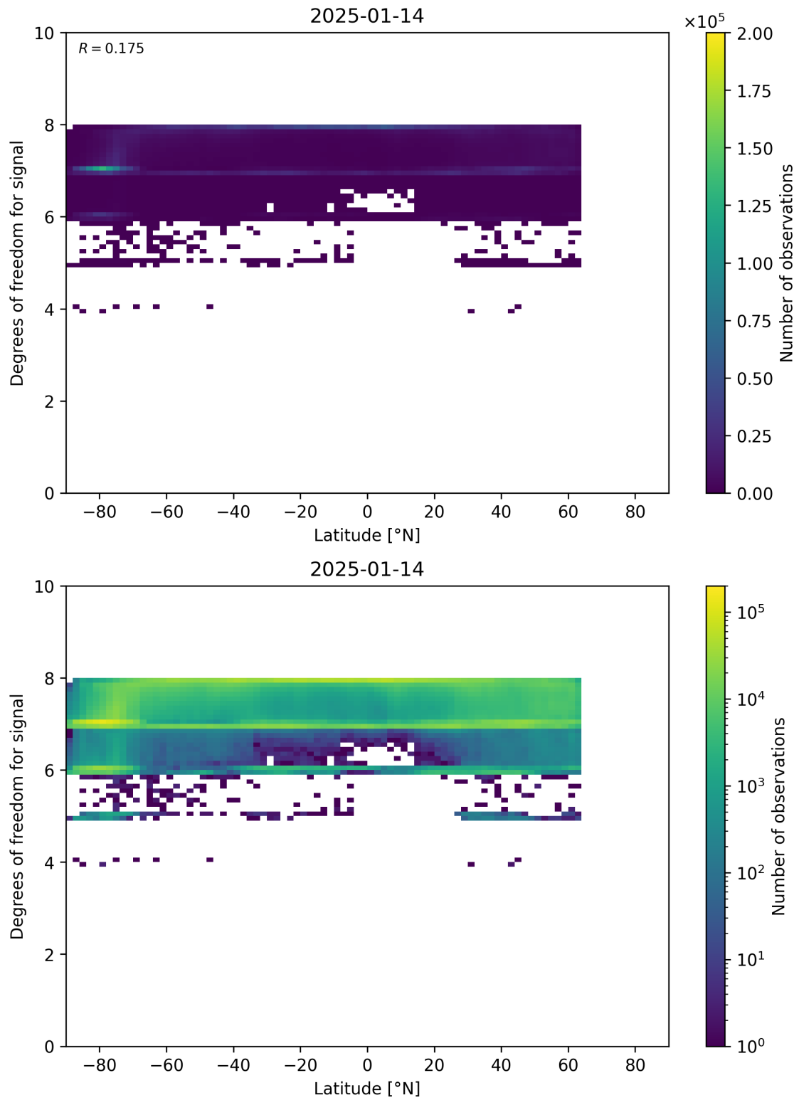
Figure 55: Scatter density plot of “Latitude” against “Degrees of freedom for signal” for 2025-01-13 to 2025-01-15.
