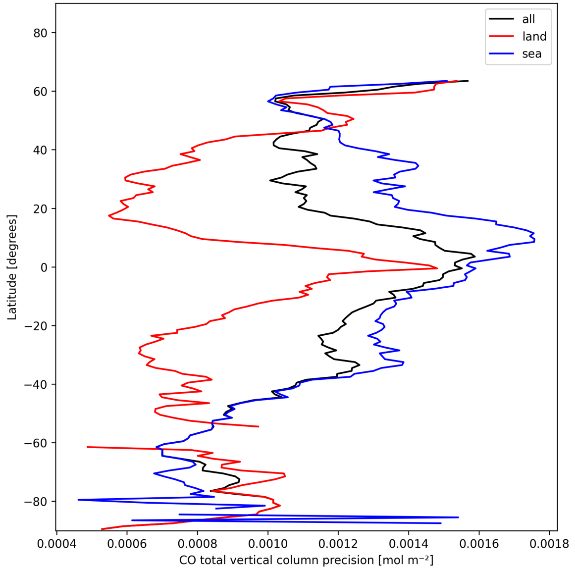
Figure 12: Zonal average of “CO total vertical column precision” for 2025-01-13 to 2025-01-15.
