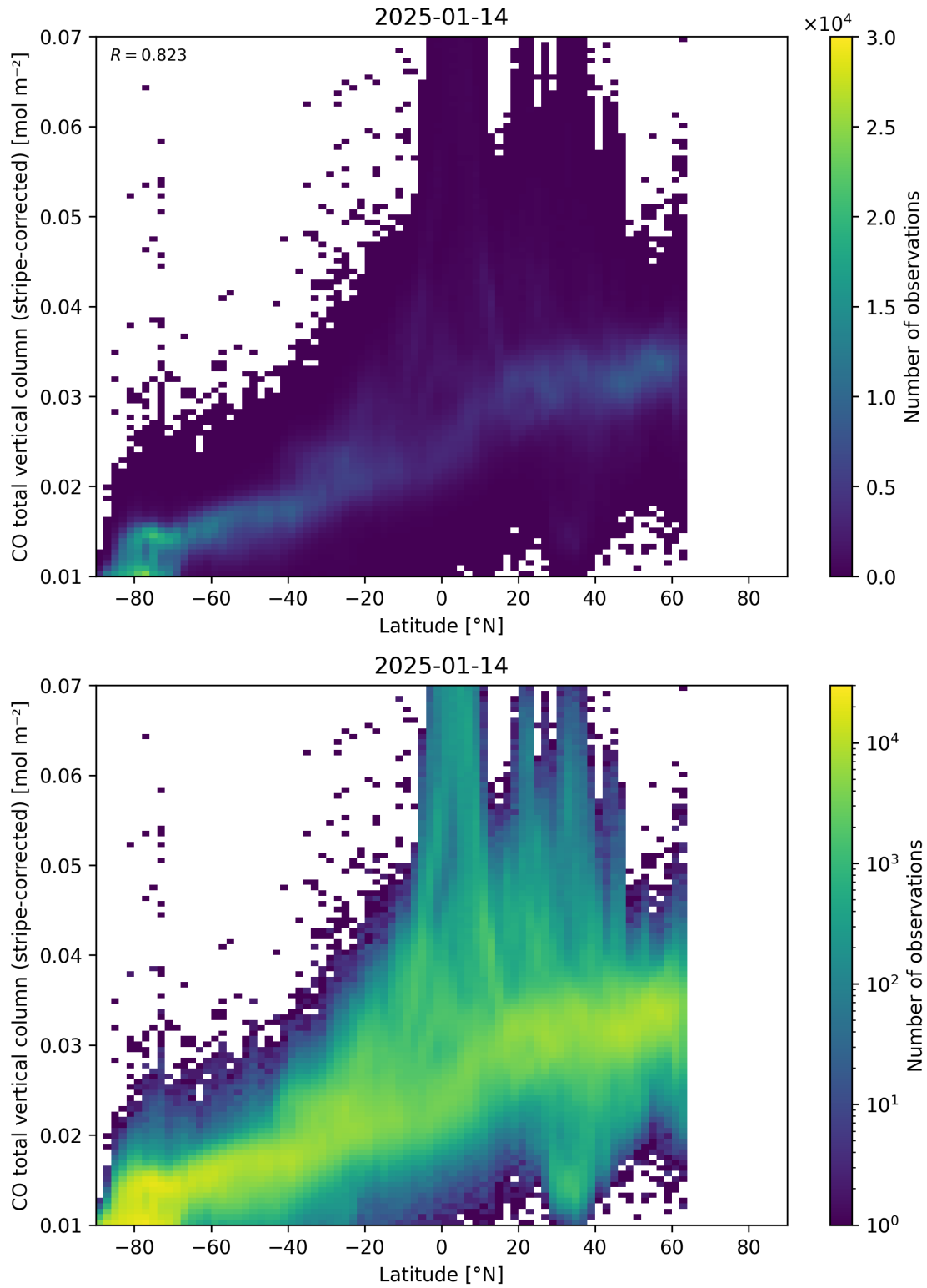
Figure 52: Scatter density plot of “Latitude” against “CO total vertical column (stripe-corrected)” for 2025-01-13 to 2025-01-15.
