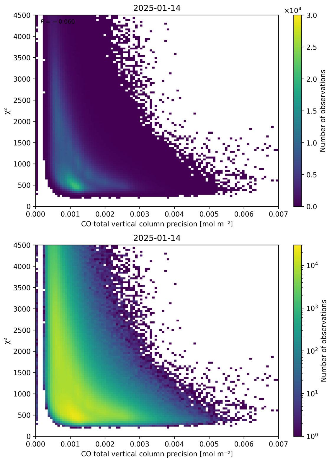
Figure 44: Scatter density plot of “CO total vertical column precision” against “ \chi^2 ” for 2025-01-13 to 2025-01-15.
