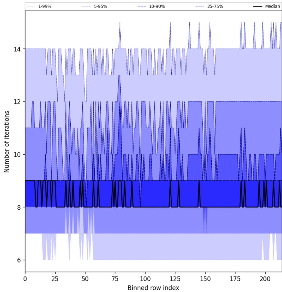
Figure 32: Along track statistics of “Number of iterations” for 2025-01-13 to 2025-01-15
