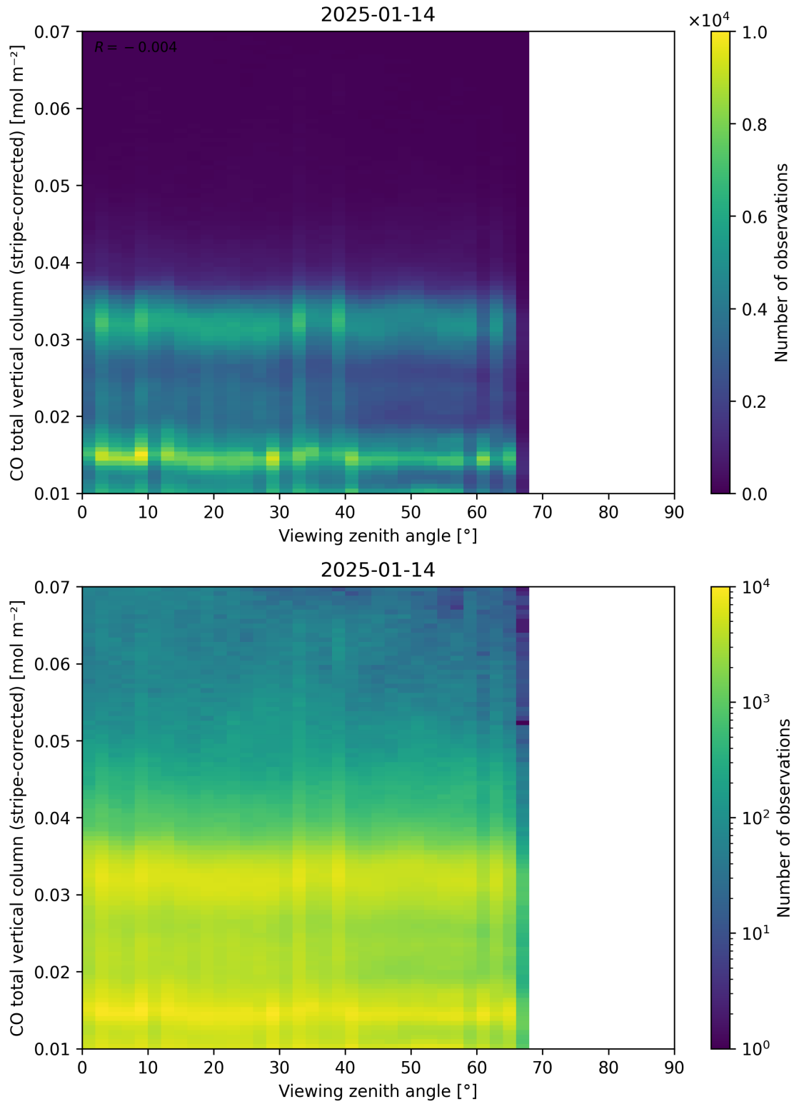
Figure 70: Scatter density plot of “Viewing zenith angle” against “CO total vertical column (stripe-corrected)” for 2025-01-13 to 2025-01-15.
