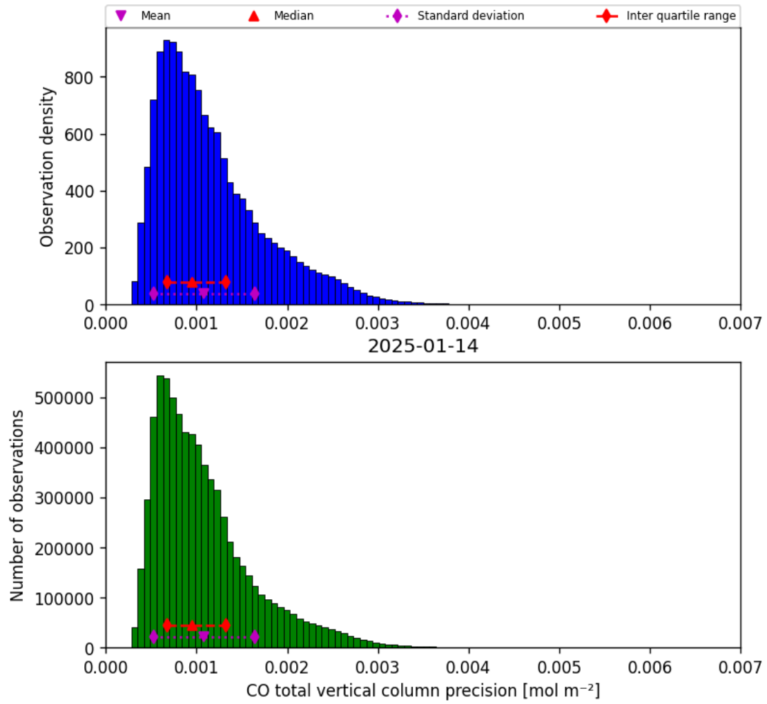
Figure 20: Histogram of “CO total vertical column precision” for 2025-01-13 to 2025-01-15
