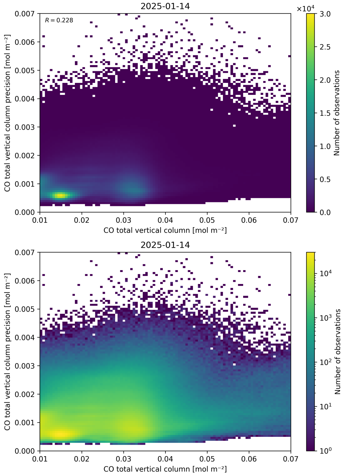
Figure 34: Scatter density plot of “CO total vertical column” against “CO total vertical column precision” for 2025-01-13 to 2025-01-15.
