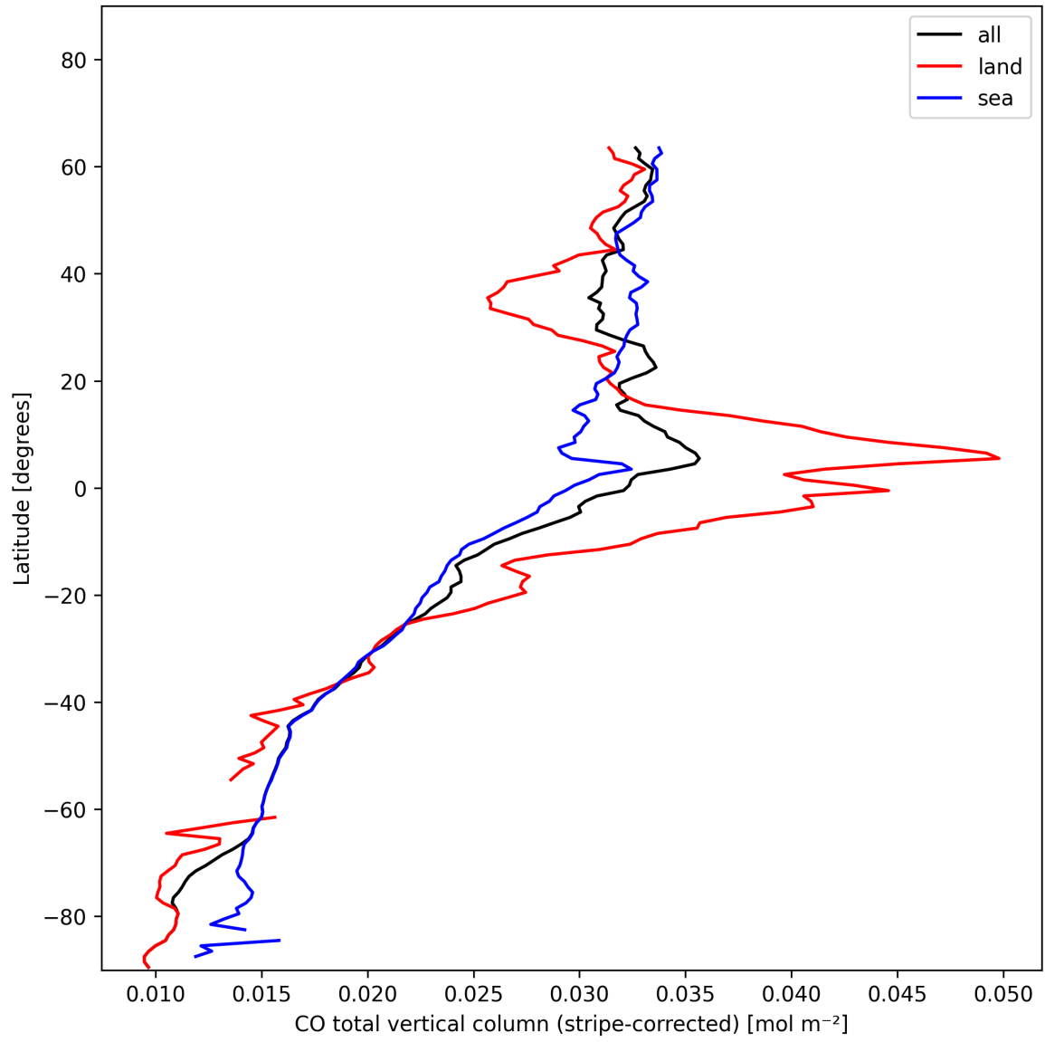
Figure 11: Zonal average of “CO total vertical column (stripe-corrected)” for 2025-01-13 to 2025-01-15.
