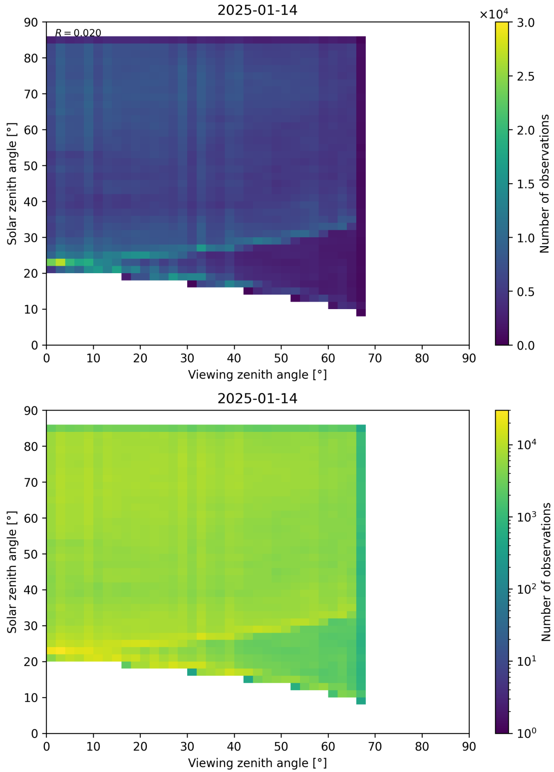
Figure 77: Scatter density plot of “Viewing zenith angle” against “Solar zenith angle” for 2025-01-13 to 2025-01-15.
