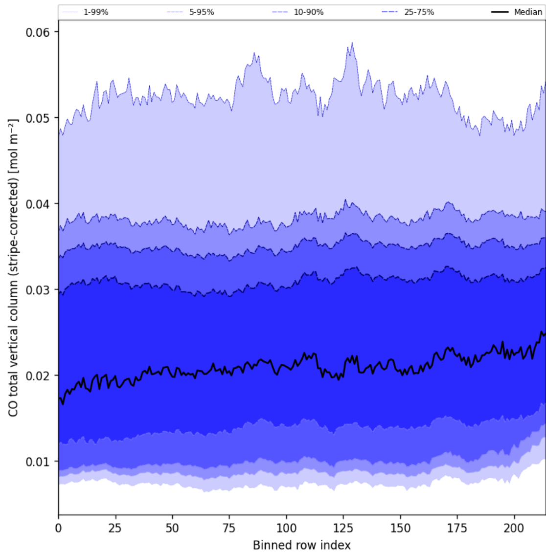
Figure 27: Along track statistics of “CO total vertical column (stripe-corrected)” for 2025-01-13 to 2025-01-15
