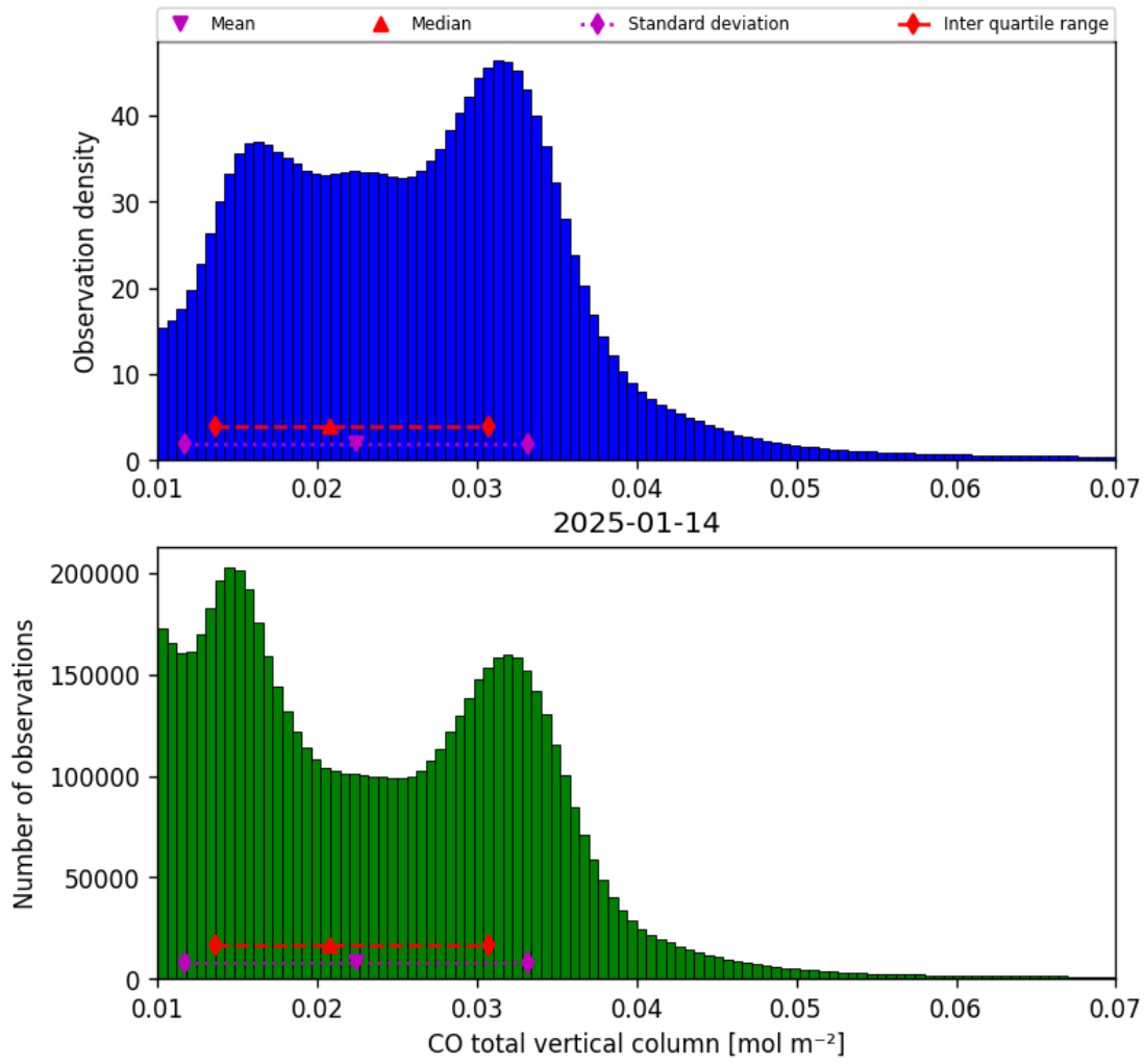
Figure 18: Histogram of “CO total vertical column” for 2025-01-13 to 2025-01-15
