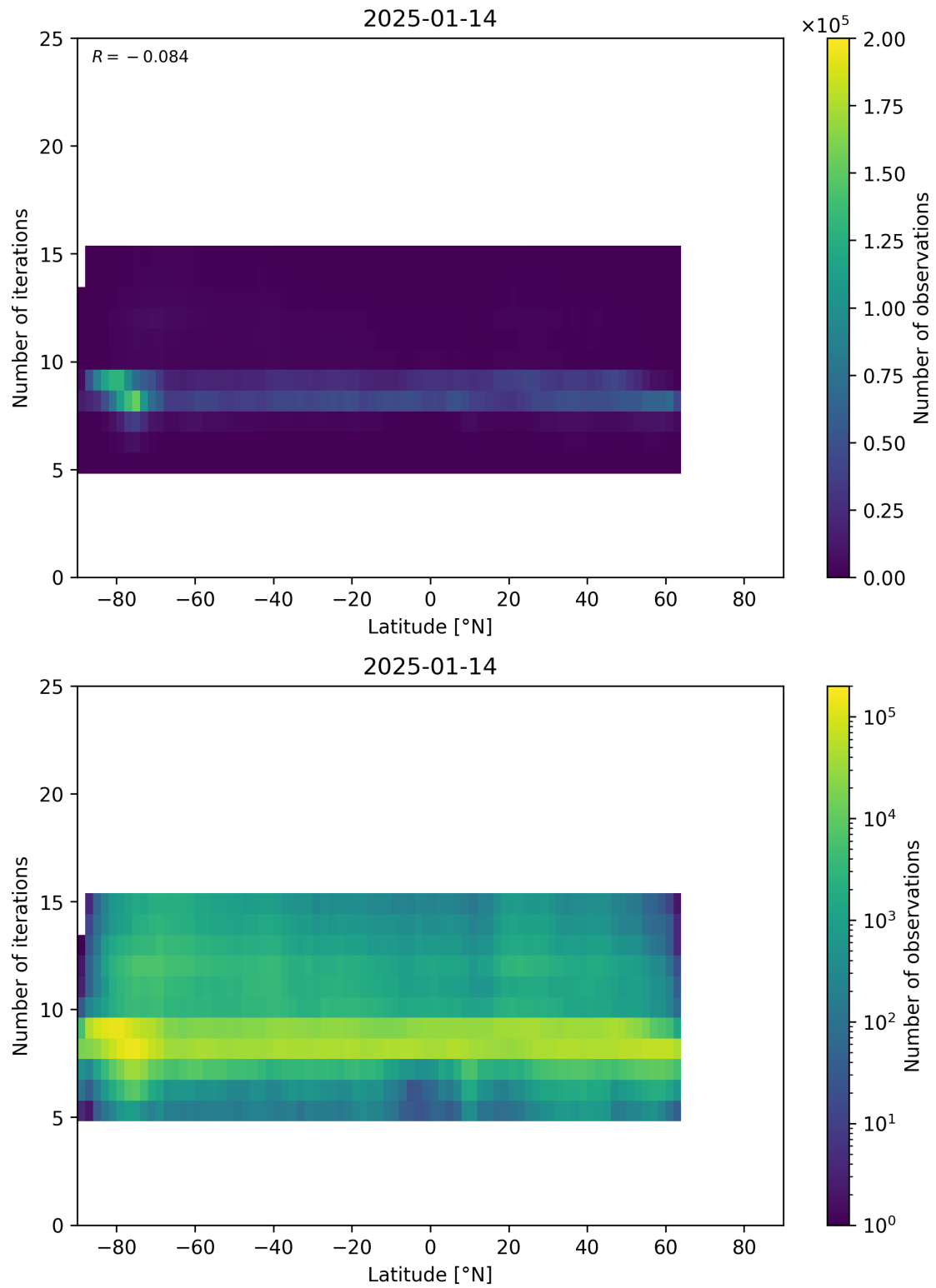
Figure 56: Scatter density plot of “Latitude” against “Number of iterations” for 2025-01-13 to 2025-01-15.
