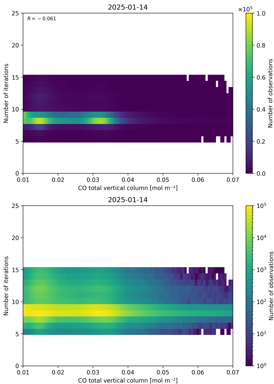
Figure 42: Scatter density plot of “CO total vertical column” against “Number of iterations” for 2025-01-13 to 2025-01-15.
