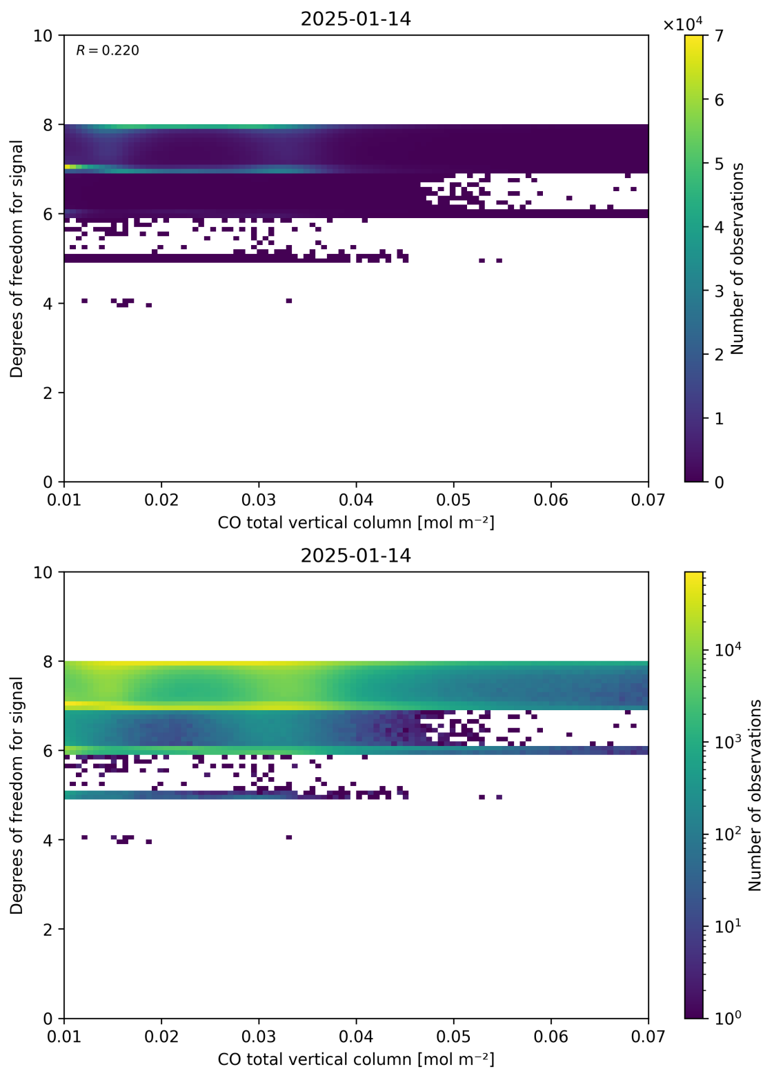
Figure 41: Scatter density plot of “CO total vertical column” against “Degrees of freedom for signal” for 2025-01-13 to 2025-01-15.
