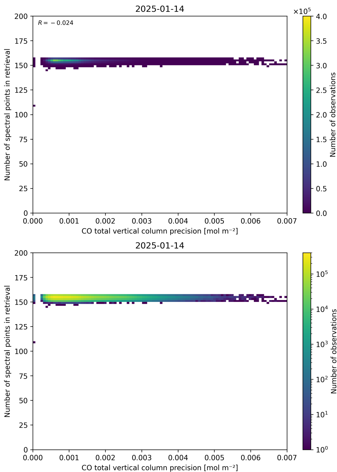
Figure 47: Scatter density plot of “CO total vertical column precision” against “Number of spectral points in retrieval” for 2025-01-13 to 2025-01-15.
