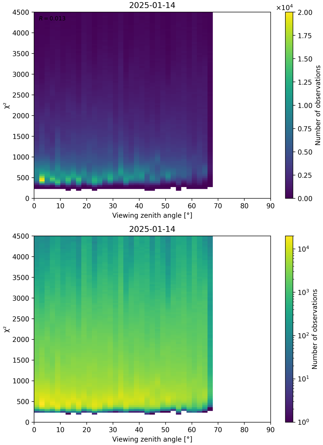
Figure 72: Scatter density plot of “Viewing zenith angle” against “ \chi^2 ” for 2025-01-13 to 2025-01-15.
