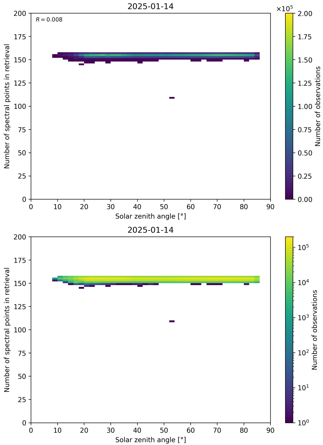
Figure 68: Scatter density plot of “Solar zenith angle” against “Number of spectral points in retrieval” for 2025-01-13 to 2025-01-15.
