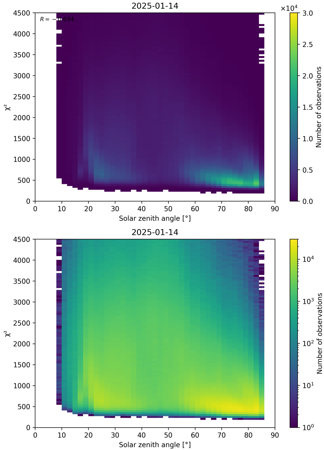
Figure 64: Scatter density plot of “Solar zenith angle” against “ \chi^2 ” for 2025-01-13 to 2025-01-15.
