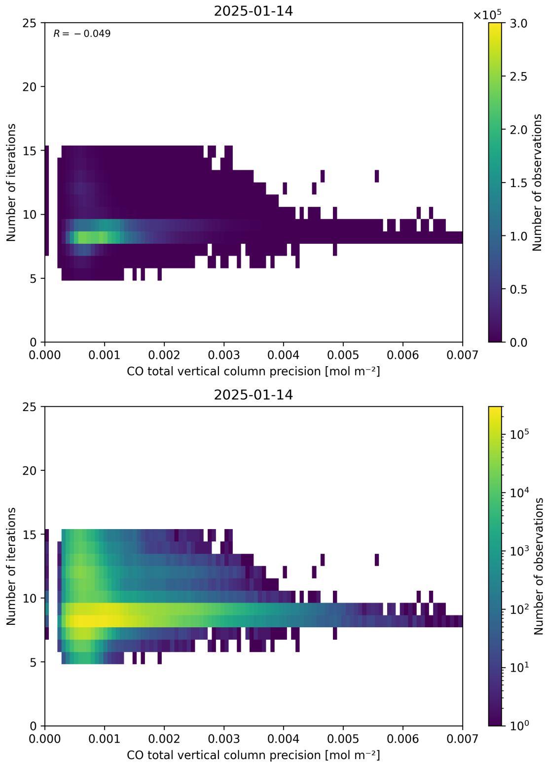
Figure 46: Scatter density plot of “CO total vertical column precision” against “Number of iterations” for 2025-01-13 to 2025-01-15.
