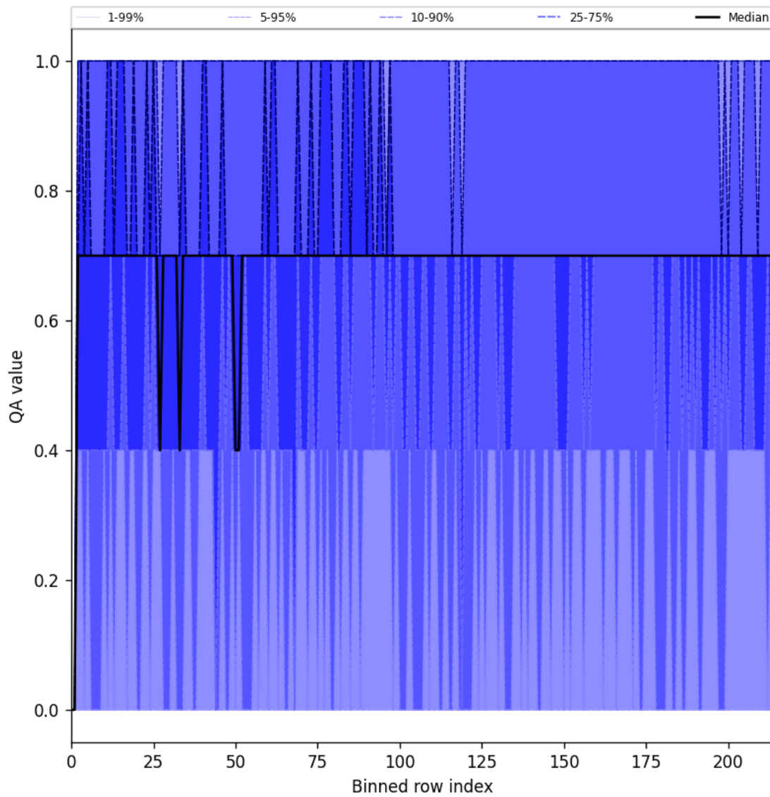
Figure 25: Along track statistics of “QA value” for 2025-01-13 to 2025-01-15
