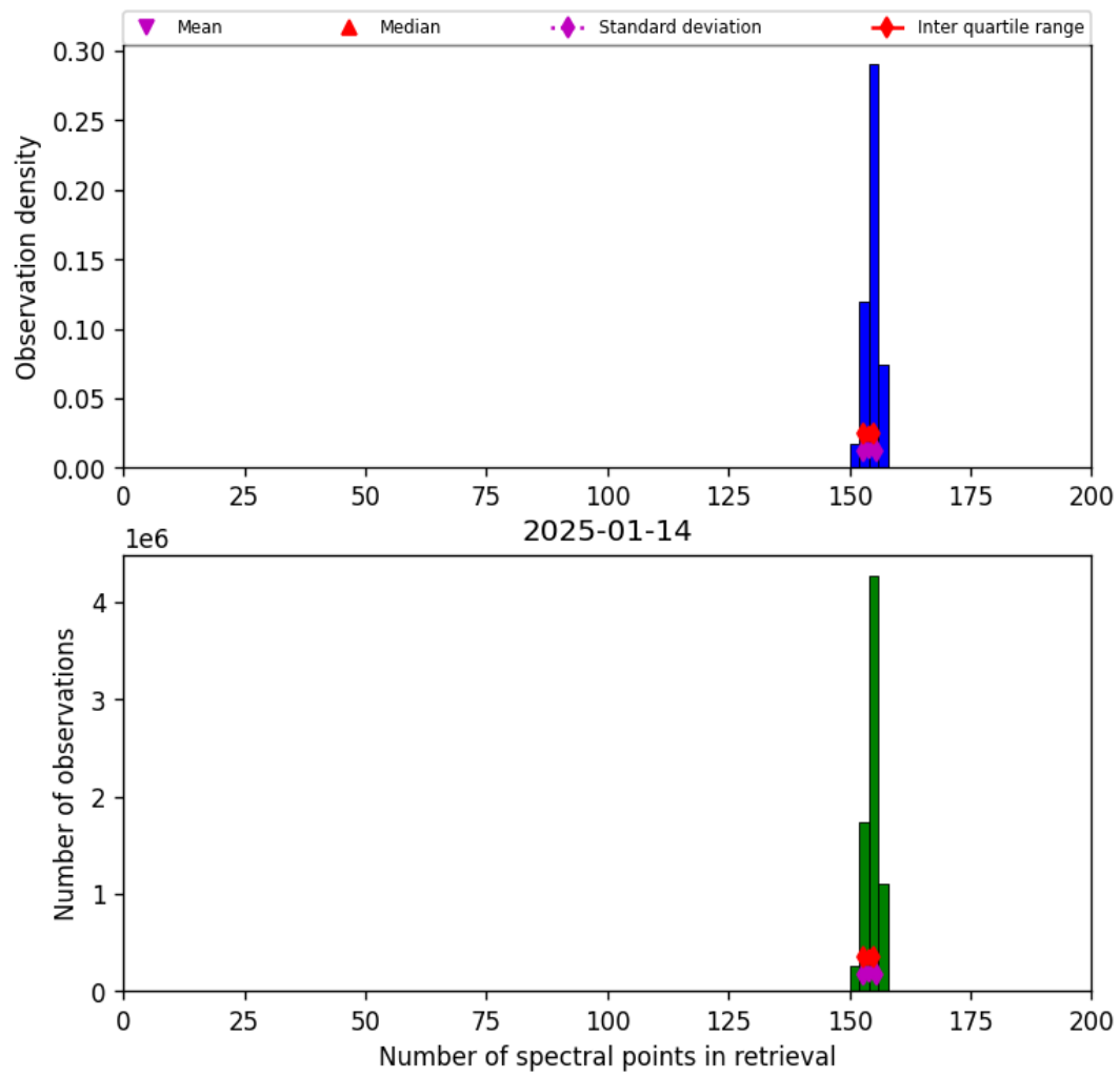
Figure 21: Histogram of “Number of spectral points in retrieval” for 2025-01-13 to 2025-01-15
