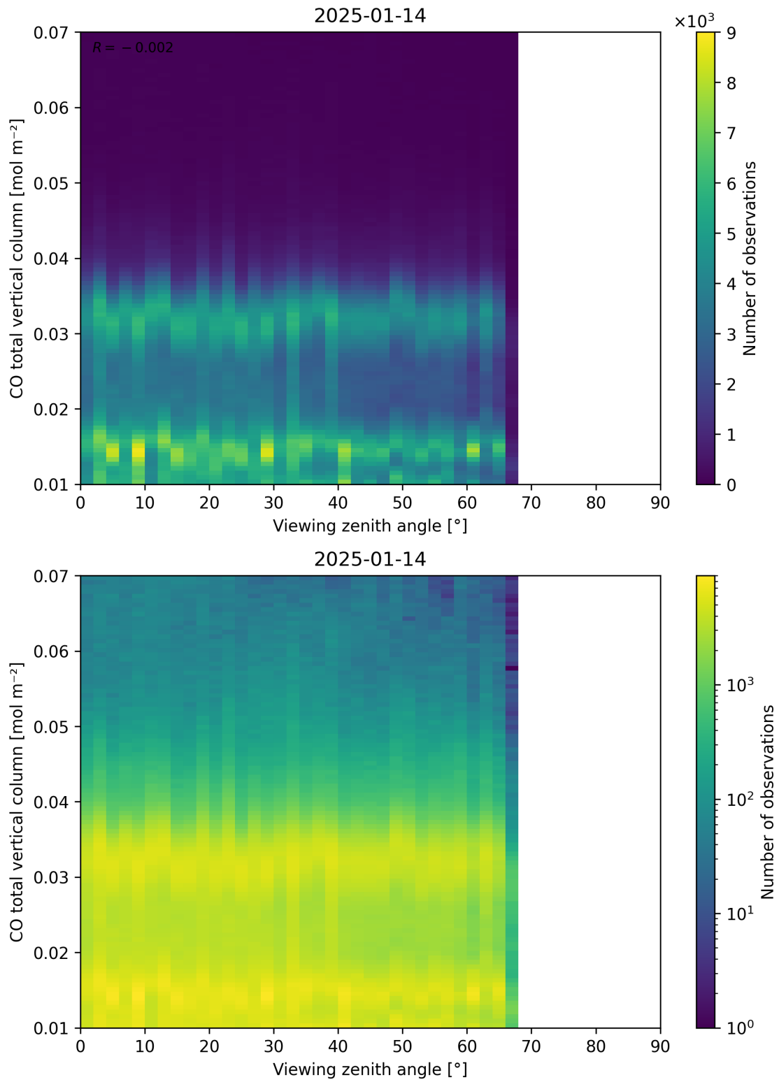
Figure 69: Scatter density plot of “Viewing zenith angle” against “CO total vertical column” for 2025-01-13 to 2025-01-15.
