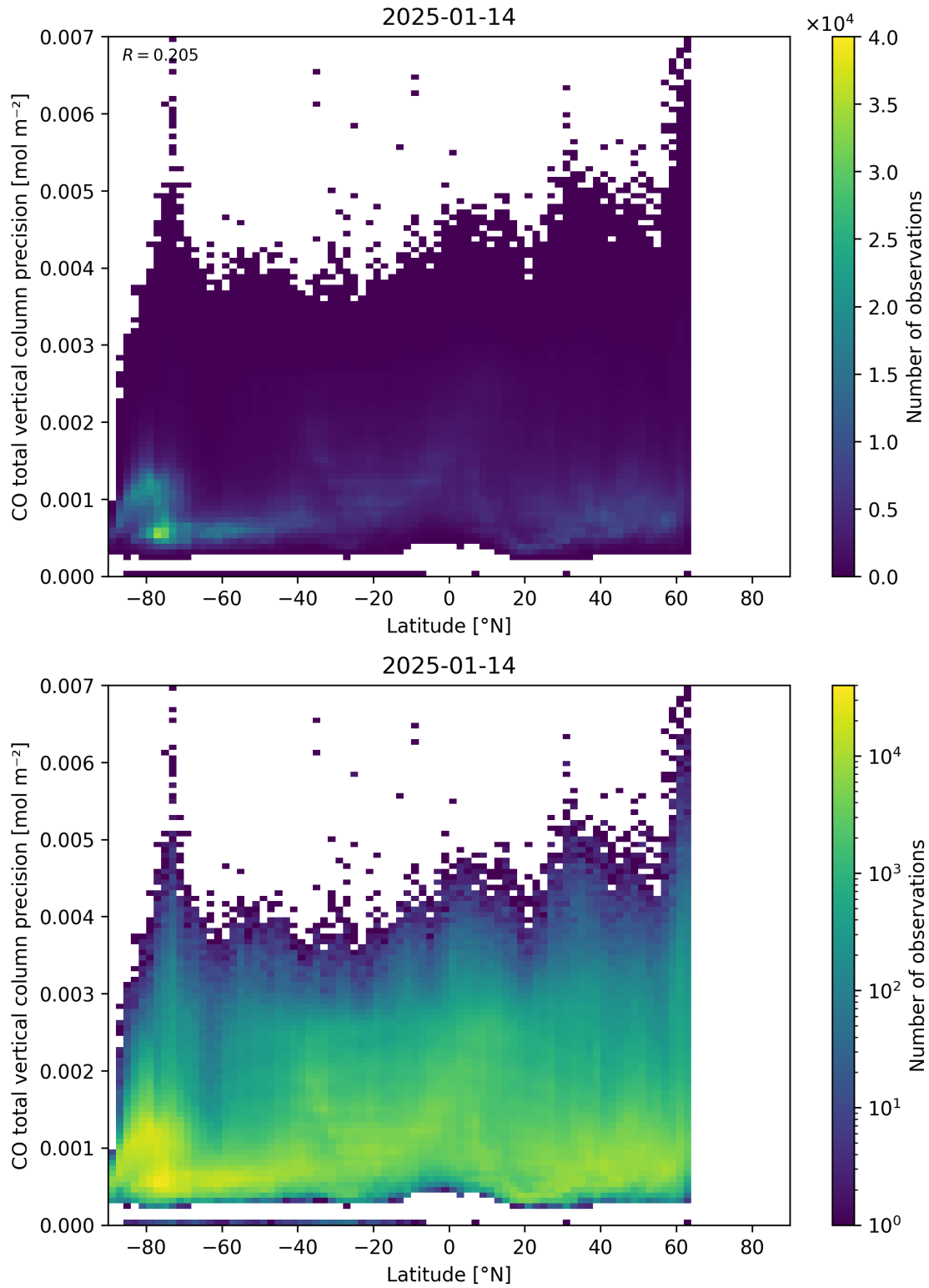
Figure 53: Scatter density plot of “Latitude” against “CO total vertical column precision” for 2025-01-13 to 2025-01-15.
