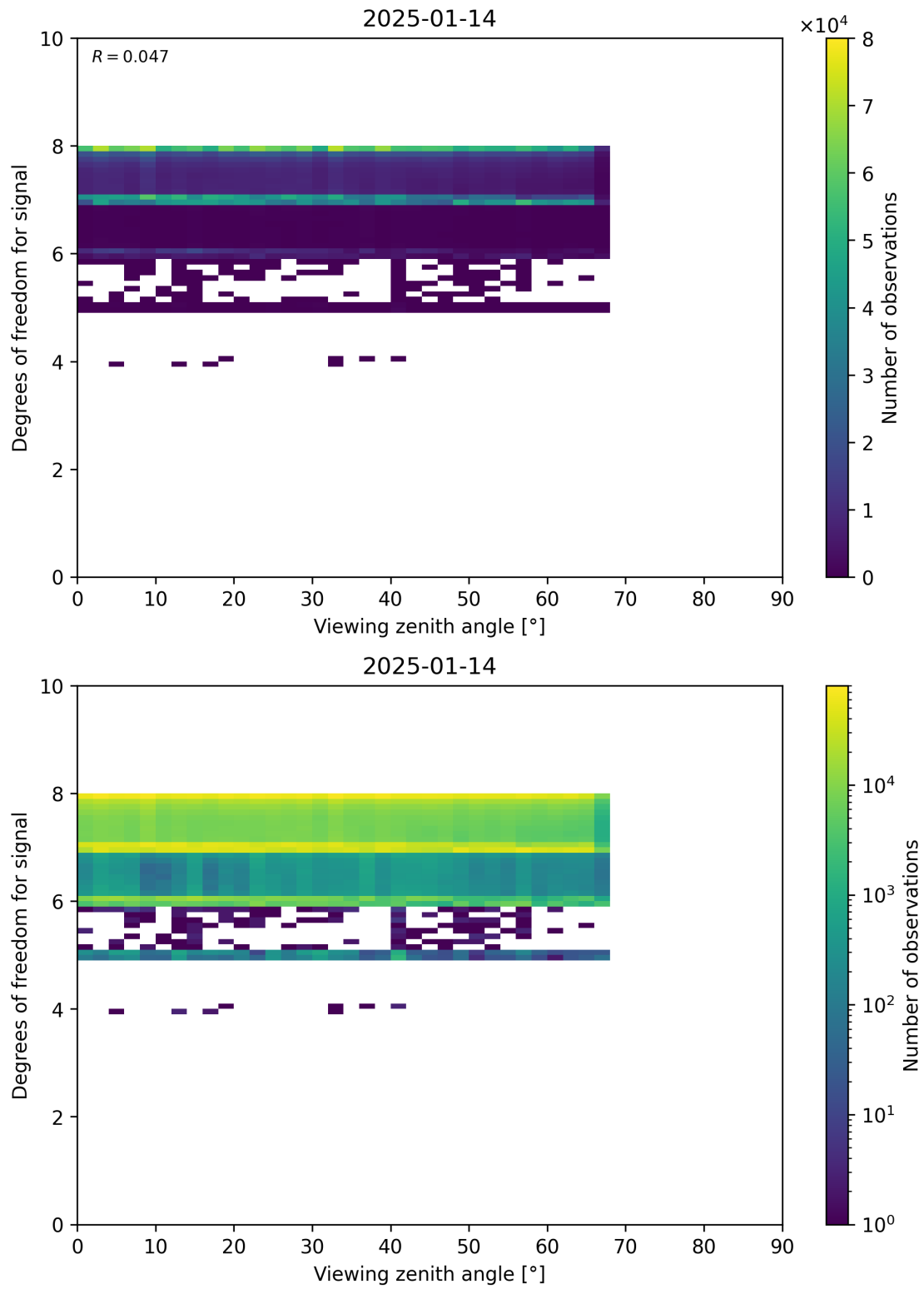
Figure 73: Scatter density plot of “Viewing zenith angle” against “Degrees of freedom for signal” for 2025-01-13 to 2025-01-15.
