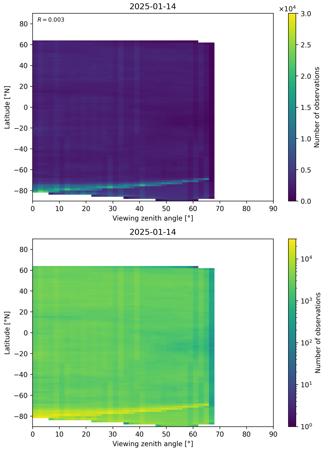
Figure 74: Scatter density plot of “Viewing zenith angle” against “Latitude” for 2025-01-13 to 2025-01-15.
