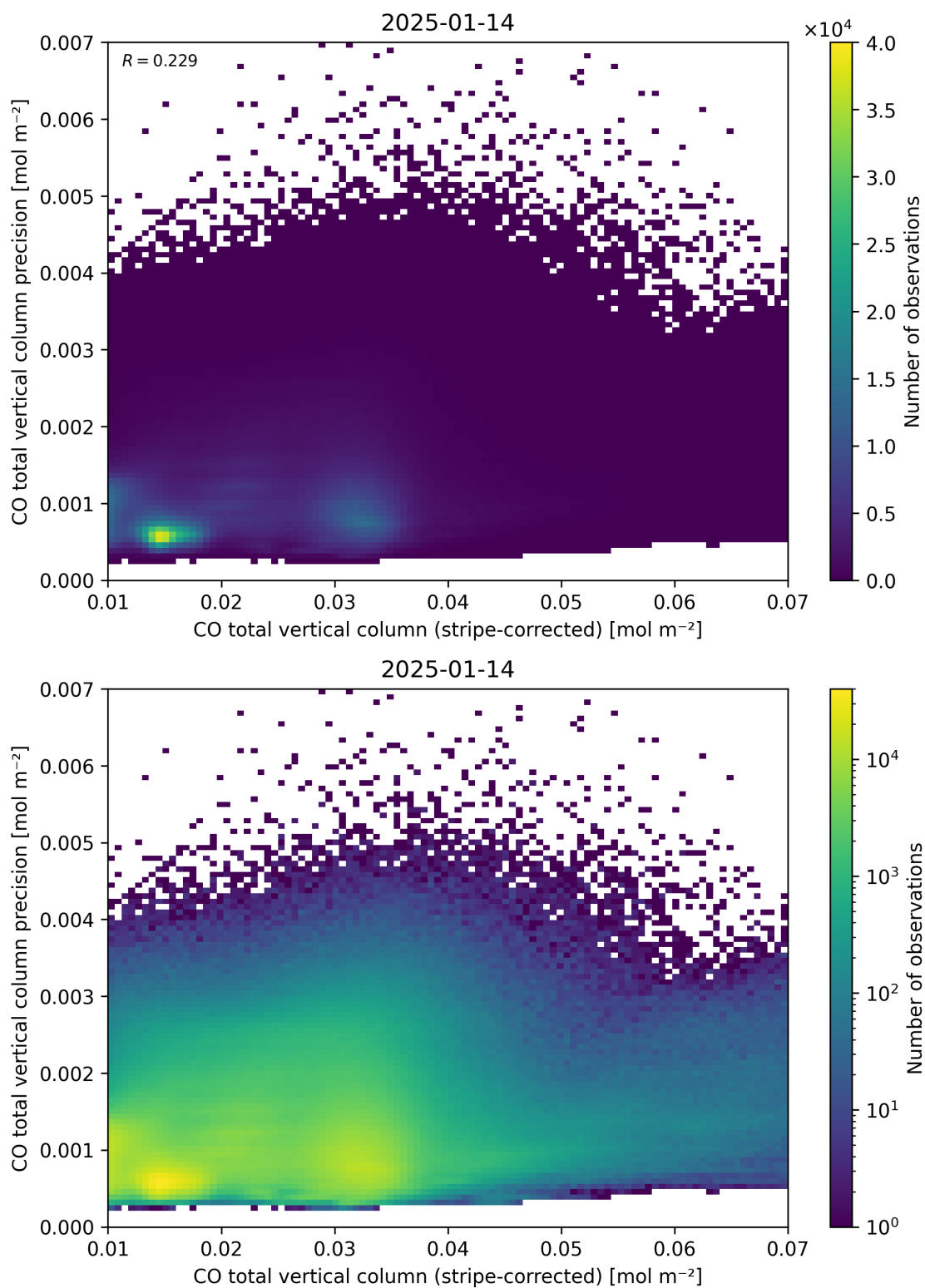
Figure 36: Scatter density plot of “CO total vertical column (stripe-corrected)” against “CO total vertical column precision” for 2025-01-13 to 2025-01-15.
