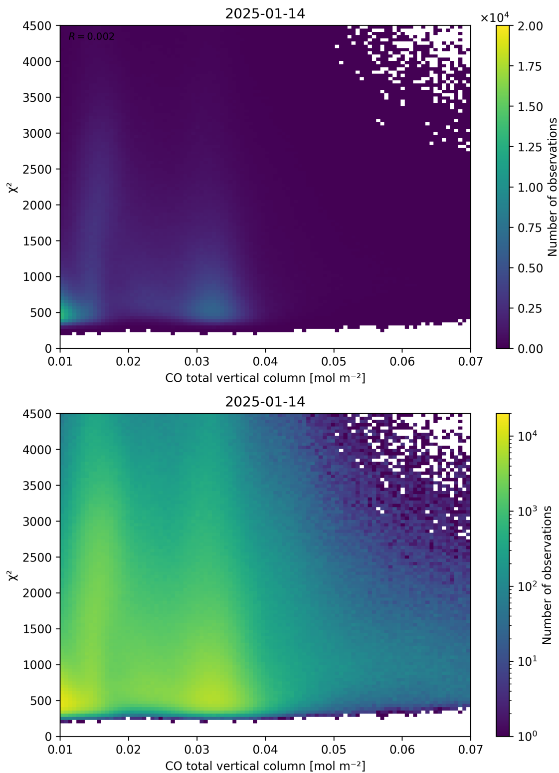
Figure 35: Scatter density plot of “CO total vertical column” against “ \chi^2 ” for 2025-01-13 to 2025-01-15.
