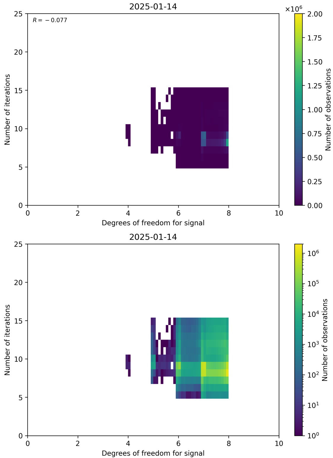
Figure 50: Scatter density plot of “Degrees of freedom for signal” against “Number of iterations” for 2025-01-13 to 2025-01-15.
