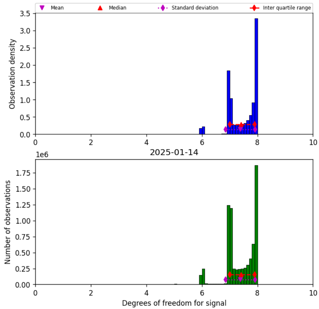
Figure 23: Histogram of “Degrees of freedom for signal” for 2025-01-13 to 2025-01-15
