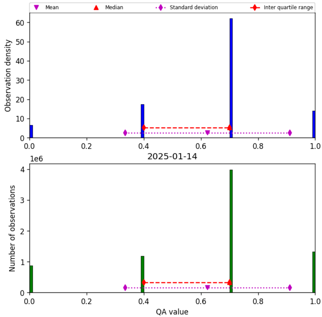
Figure 17: Histogram of “QA value” for 2025-01-13 to 2025-01-15
