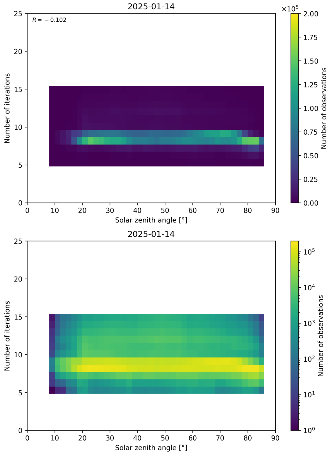
Figure 67: Scatter density plot of “Solar zenith angle” against “Number of iterations” for 2025-01-13 to 2025-01-15.
