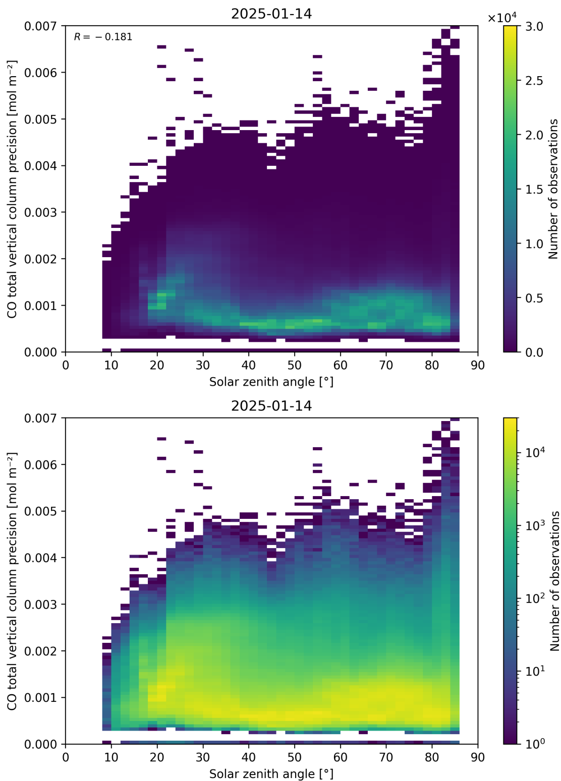
Figure 63: Scatter density plot of “Solar zenith angle” against “CO total vertical column precision” for 2025-01-13 to 2025-01-15.
