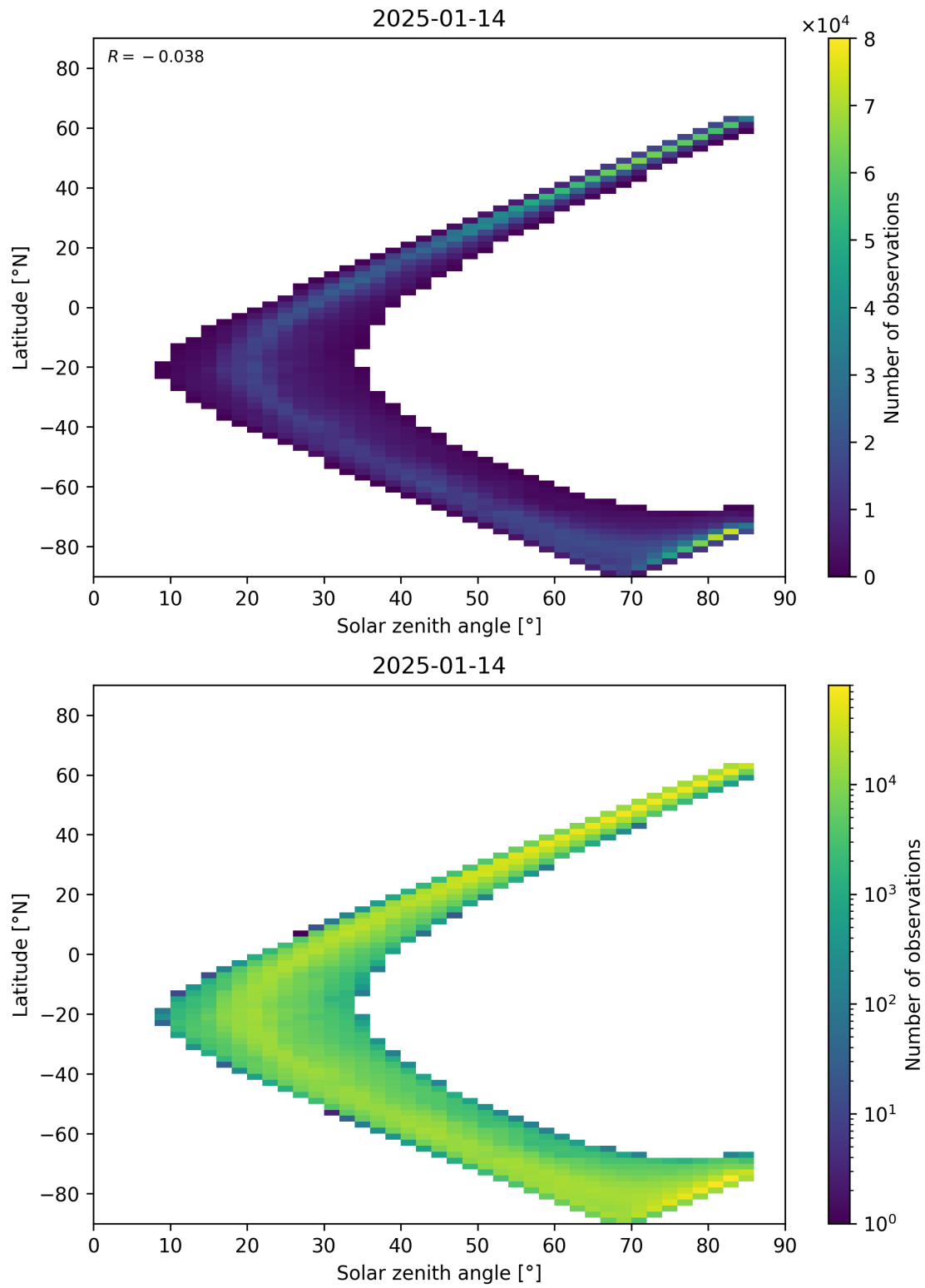
Figure 66: Scatter density plot of “Solar zenith angle” against “Latitude” for 2025-01-13 to 2025-01-15.
