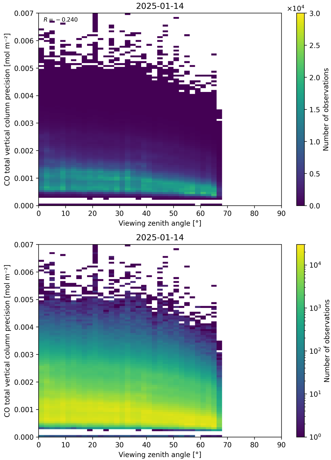
Figure 71: Scatter density plot of “Viewing zenith angle” against “CO total vertical column precision” for 2025-01-13 to 2025-01-15.
