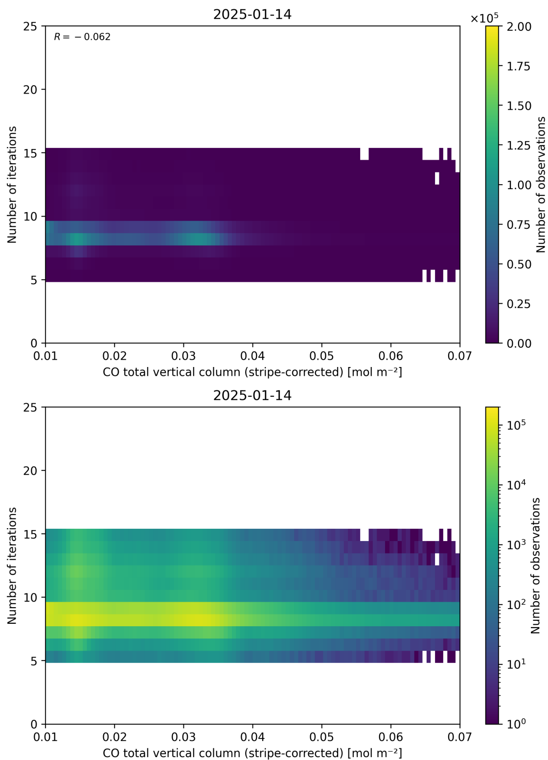
Figure 39: Scatter density plot of “CO total vertical column (stripe-corrected)” against “Number of iterations” for 2025-01-13 to 2025-01-15.
