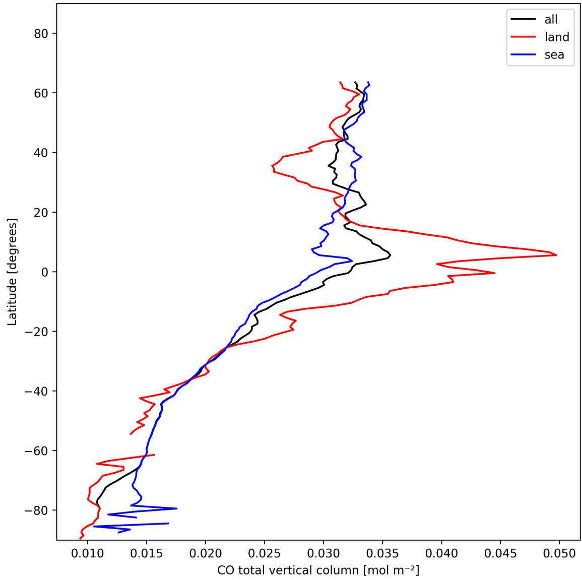
Figure 10: Zonal average of “CO total vertical column” for 2025-01-13 to 2025-01-15.
