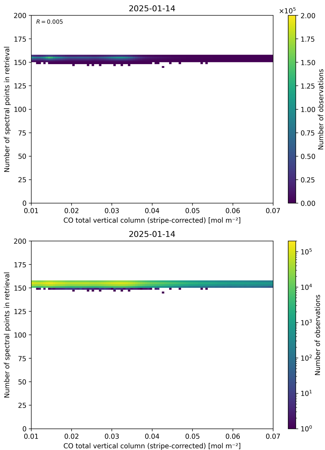
Figure 40: Scatter density plot of “CO total vertical column (stripe-corrected)” against “Number of spectral points in retrieval” for 2025-01-13 to 2025-01-15.
