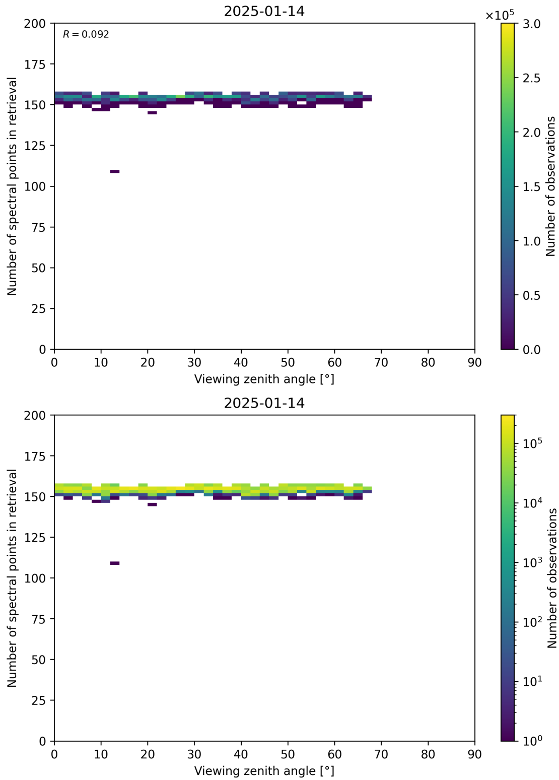
Figure 76: Scatter density plot of “Viewing zenith angle” against “Number of spectral points in retrieval” for 2025-01-13 to 2025-01-15.
