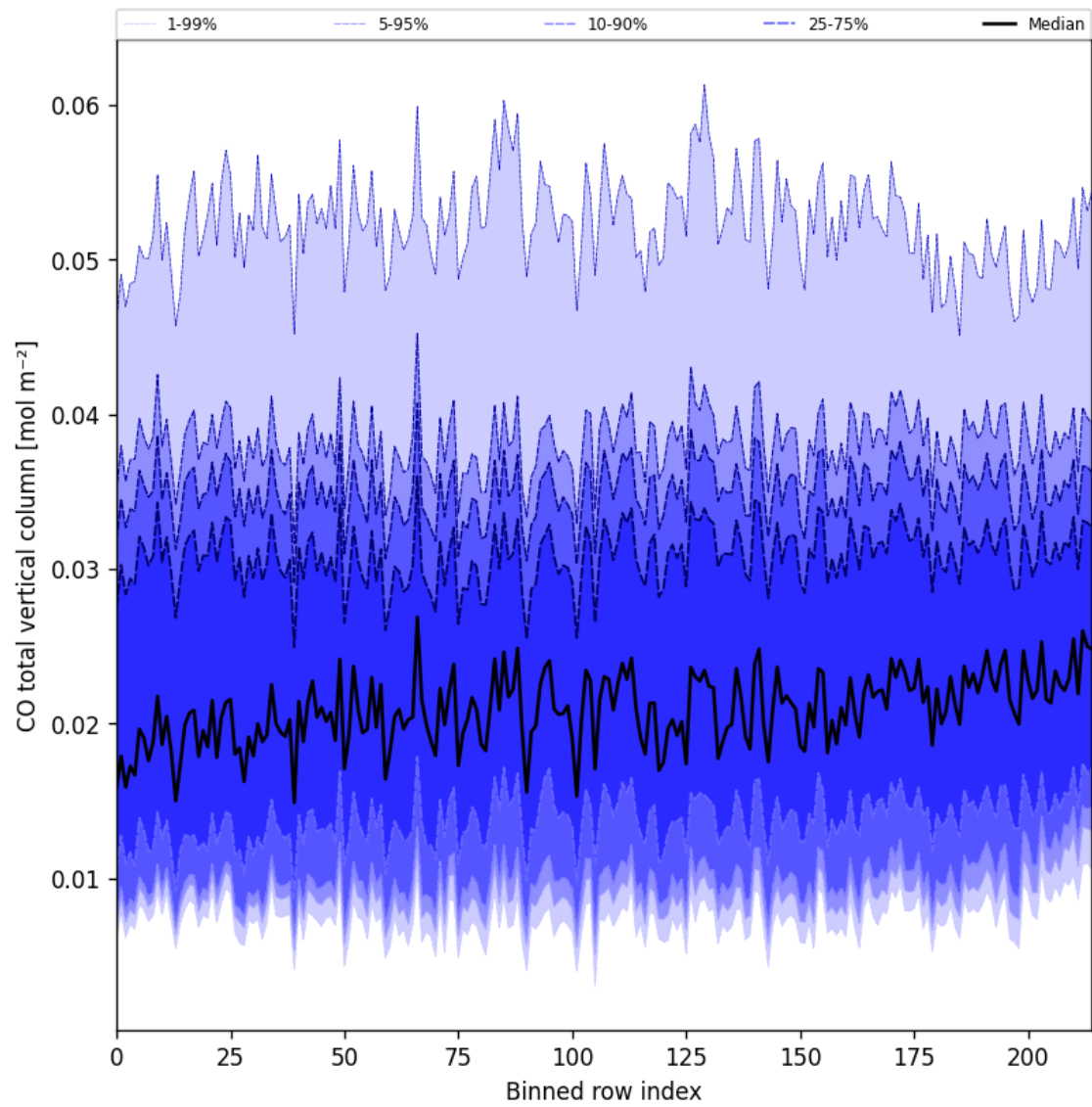
Figure 26: Along track statistics of “CO total vertical column” for 2025-01-13 to 2025-01-15
