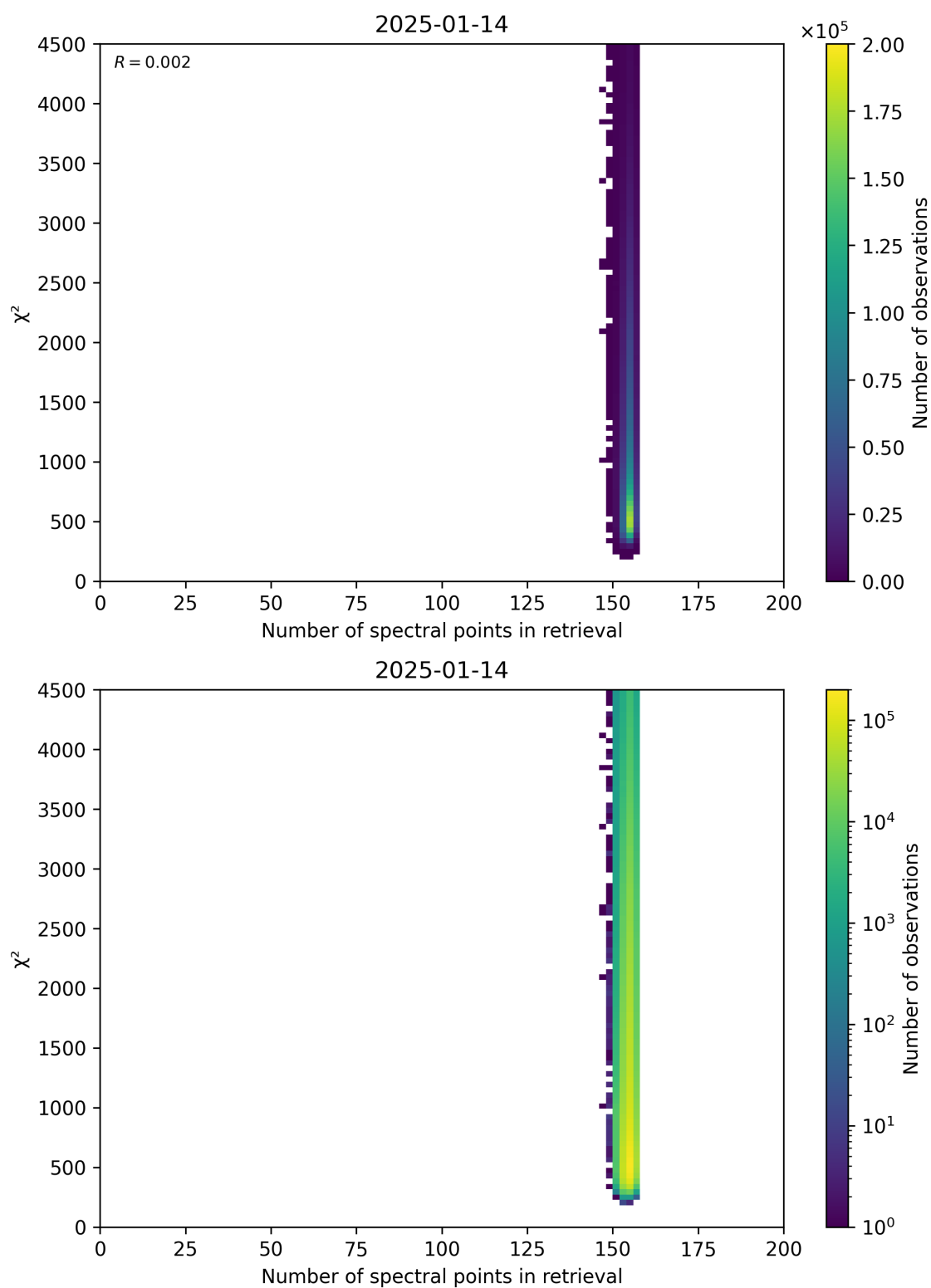
Figure 58: Scatter density plot of “Number of spectral points in retrieval” against “ \chi^2 ” for 2025-01-13 to 2025-01-15.
