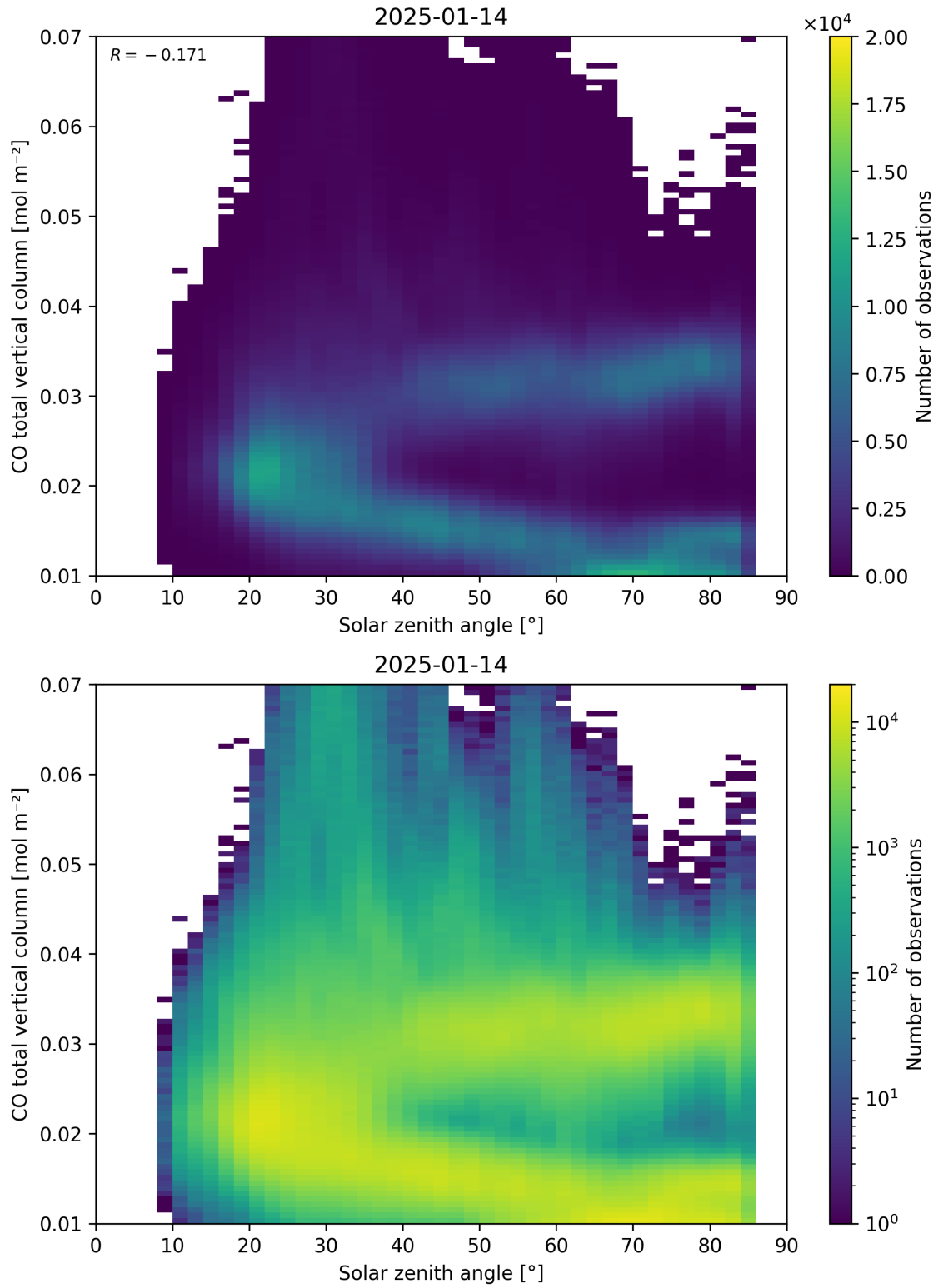
Figure 61: Scatter density plot of “Solar zenith angle” against “CO total vertical column” for 2025-01-13 to 2025-01-15.
