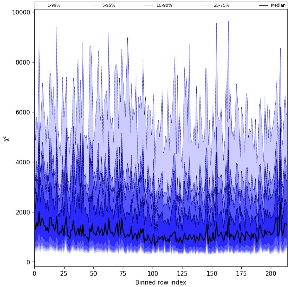
Figure 30: Along track statistics of “ \chi^2 ” for 2025-01-13 to 2025-01-15
