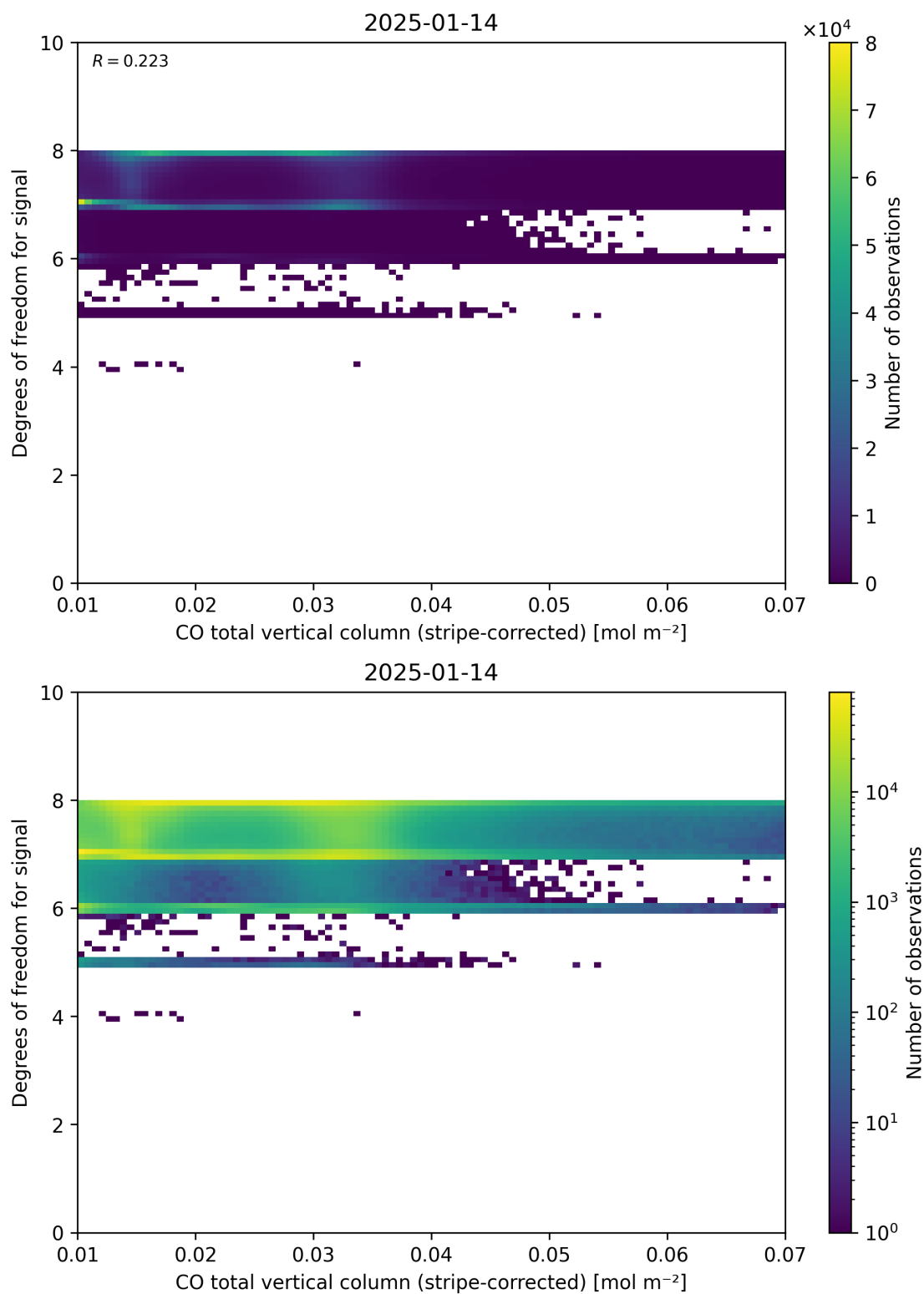
Figure 38: Scatter density plot of “CO total vertical column (stripe-corrected)” against “Degrees of freedom for signal” for 2025-01-13 to 2025-01-15.
