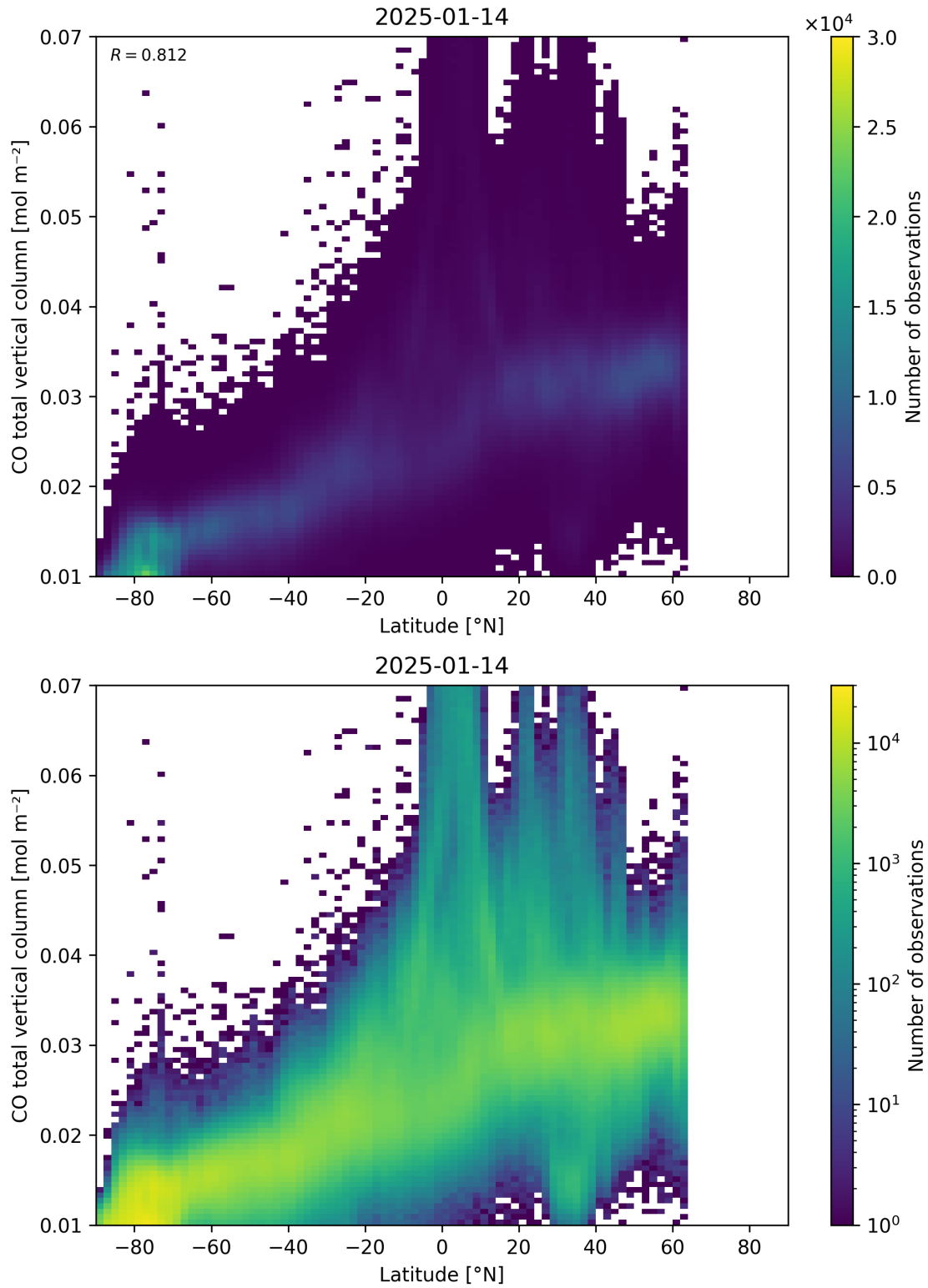
Figure 51: Scatter density plot of “Latitude” against “CO total vertical column” for 2025-01-13 to 2025-01-15.
