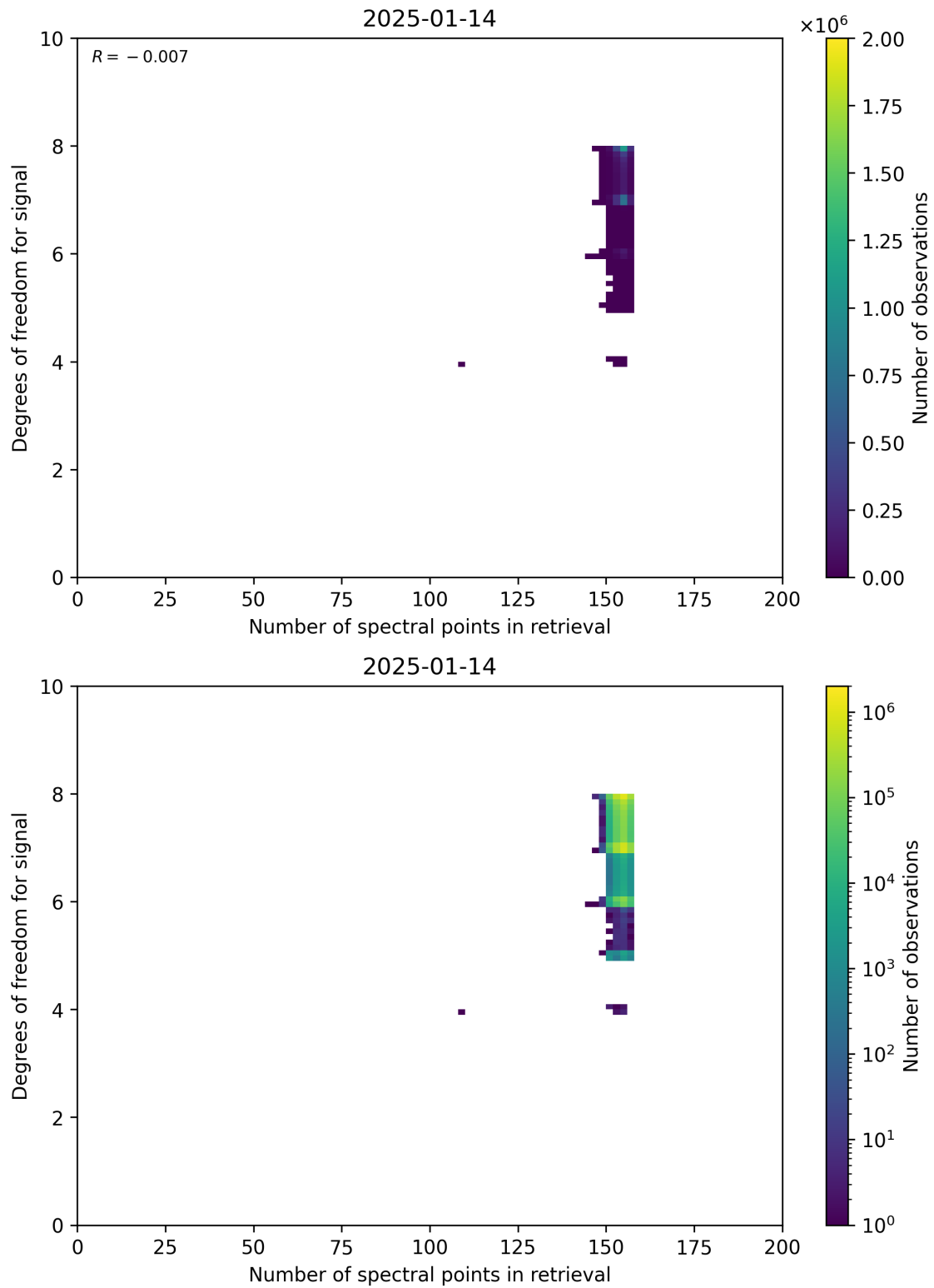
Figure 59: Scatter density plot of “Number of spectral points in retrieval” against “Degrees of freedom for signal” for 2025-01-13 to 2025-01-15.
