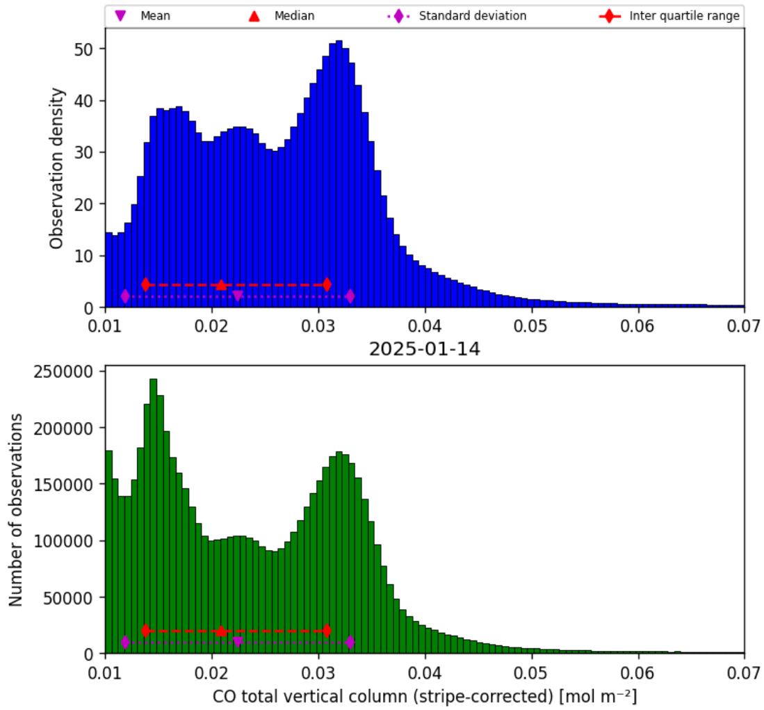
Figure 19: Histogram of “CO total vertical column (stripe-corrected)” for 2025-01-13 to 2025-01-15
