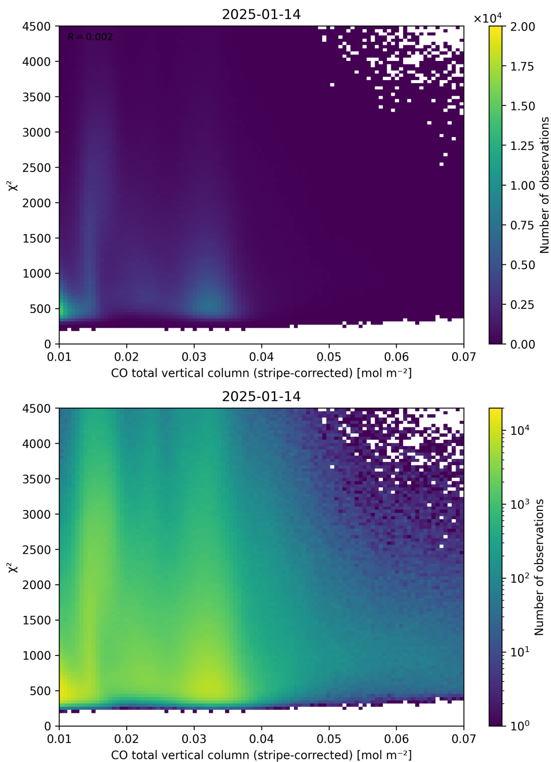
Figure 37: Scatter density plot of “CO total vertical column (stripe-corrected)” against “ \chi^2 ” for 2025-01-13 to 2025-01-15.
