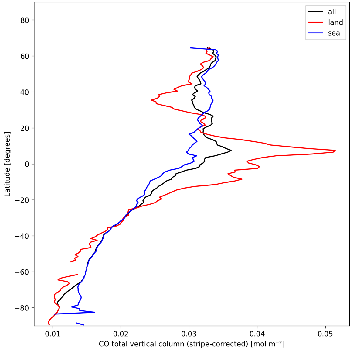
Figure 11: Zonal average of “CO total vertical column (stripe-corrected)” for 2025-01-14 to 2025-01-16.
