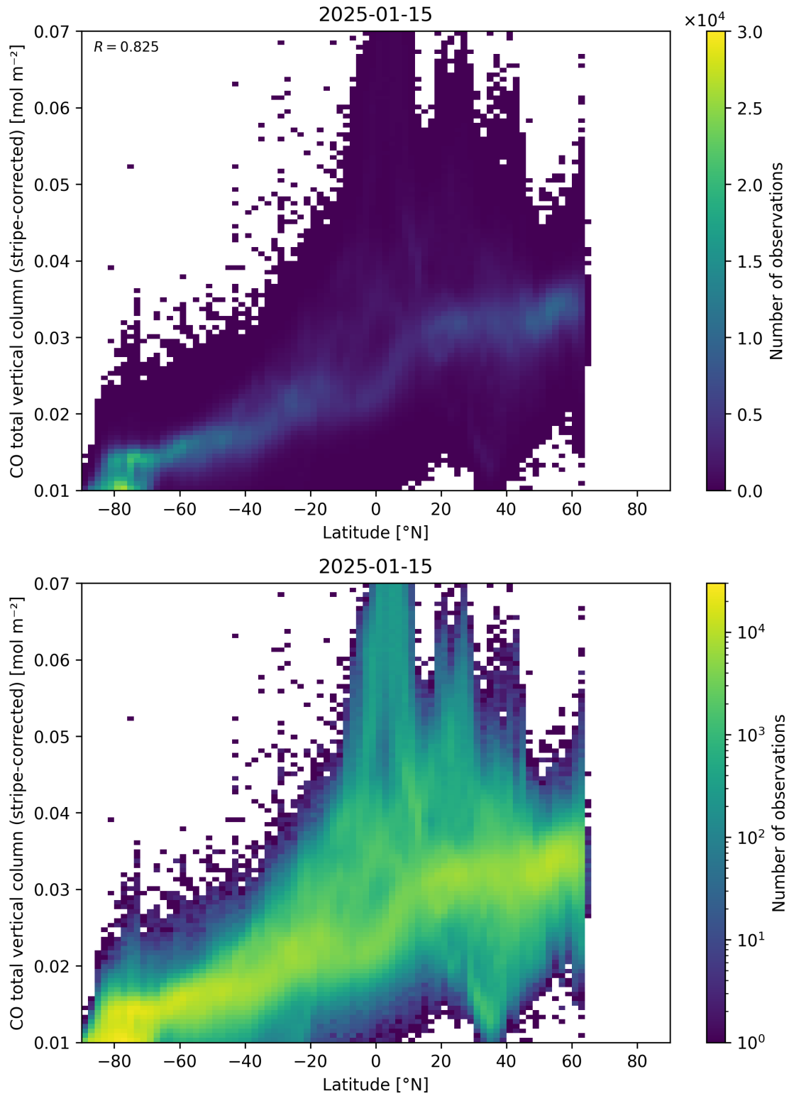
Figure 52: Scatter density plot of “Latitude” against “CO total vertical column (stripe-corrected)” for 2025-01-14 to 2025-01-16.
