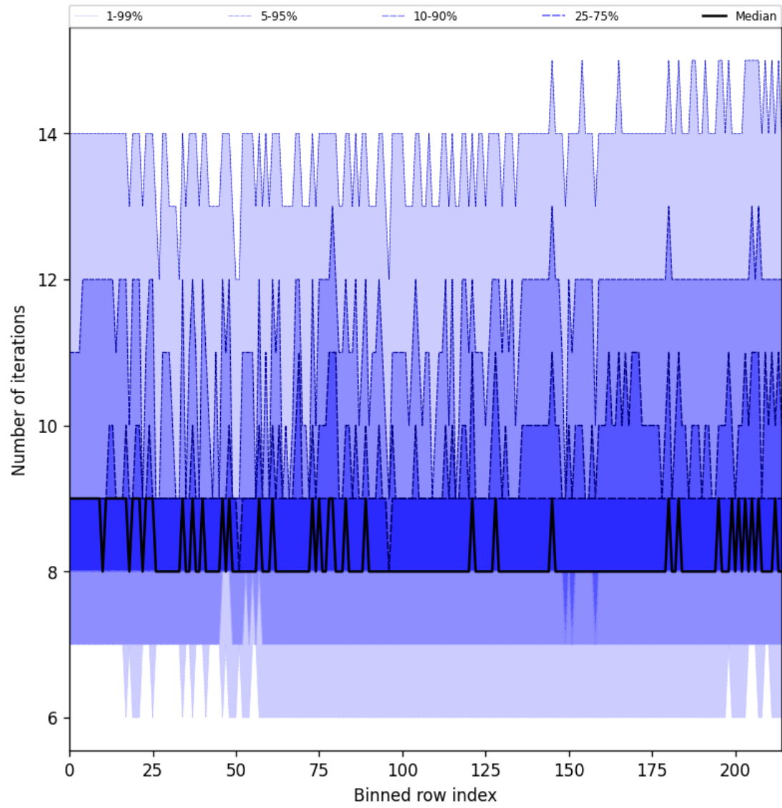
Figure 32: Along track statistics of “Number of iterations” for 2025-01-14 to 2025-01-16
