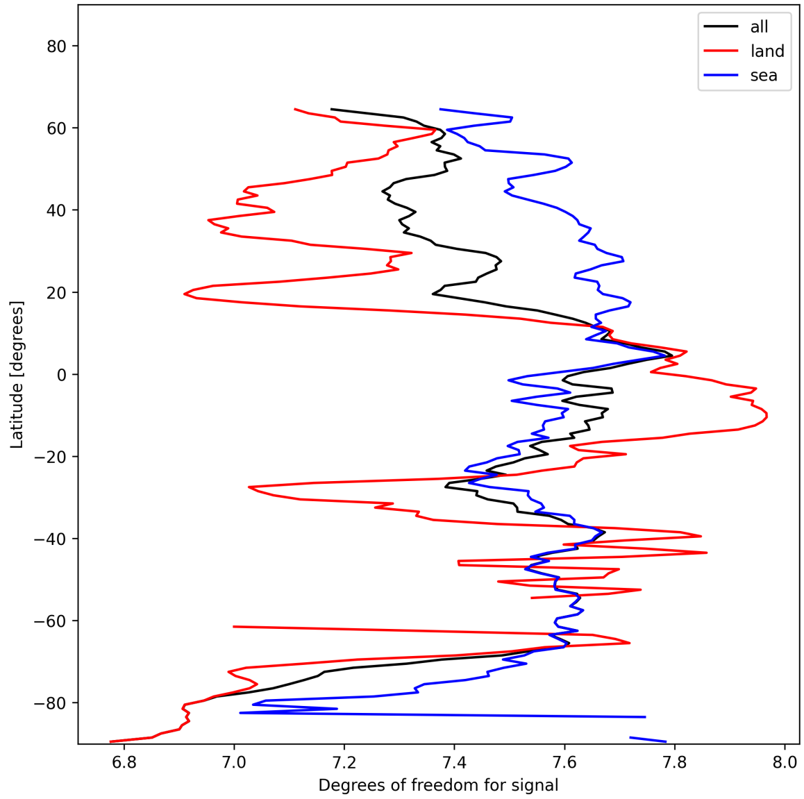
Figure 15: Zonal average of “Degrees of freedom for signal” for 2025-01-14 to 2025-01-16.
