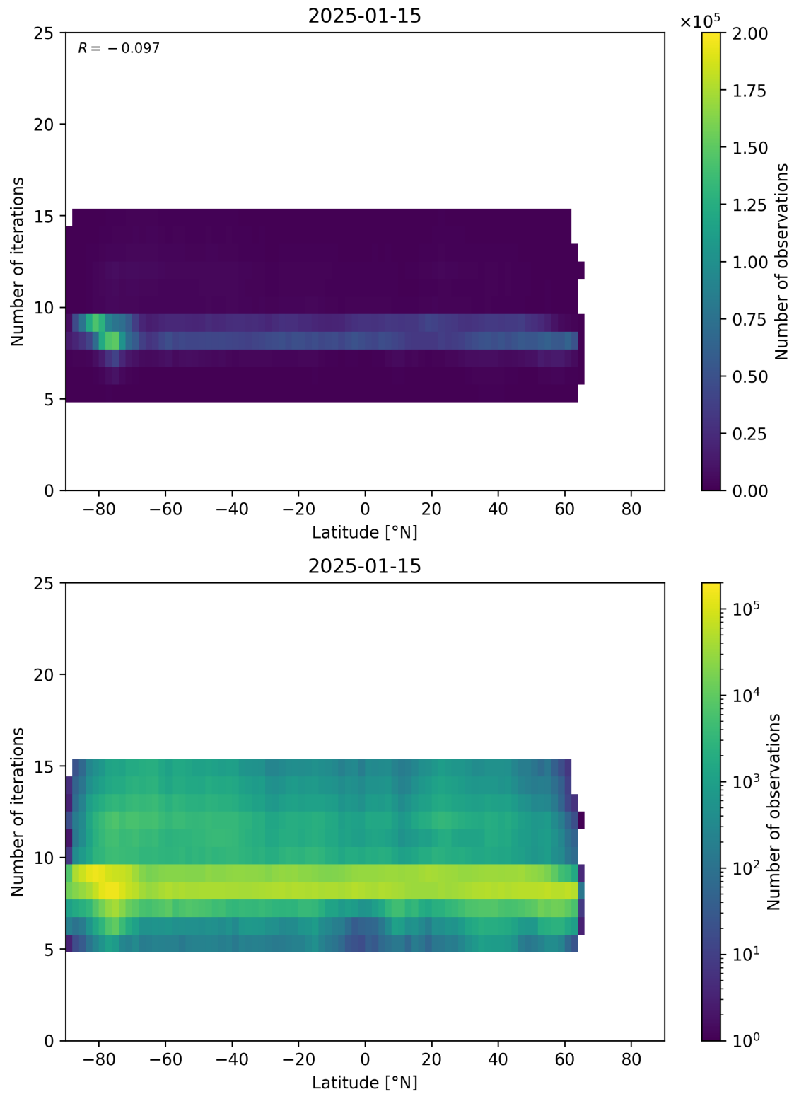
Figure 56: Scatter density plot of “Latitude” against “Number of iterations” for 2025-01-14 to 2025-01-16.
