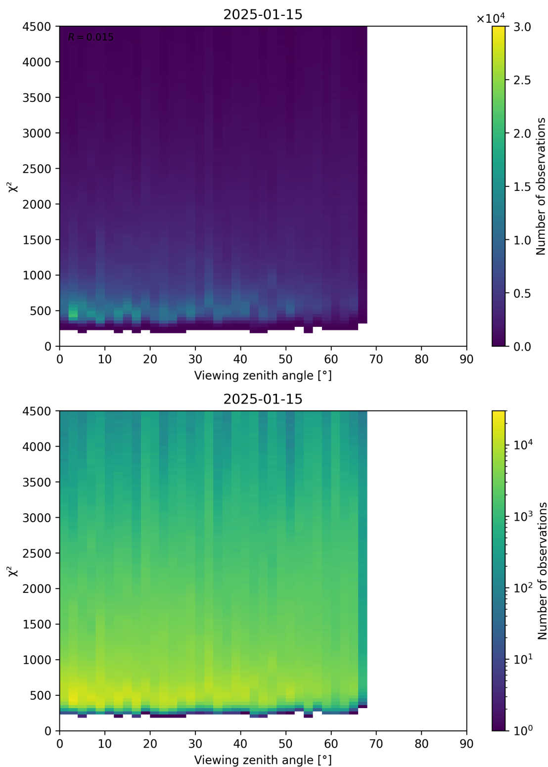
Figure 72: Scatter density plot of “Viewing zenith angle” against “ \chi^2 ” for 2025-01-14 to 2025-01-16.
