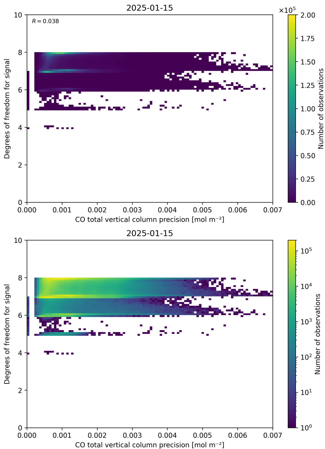
Figure 45: Scatter density plot of “CO total vertical column precision” against “Degrees of freedom for signal” for 2025-01-14 to 2025-01-16.
