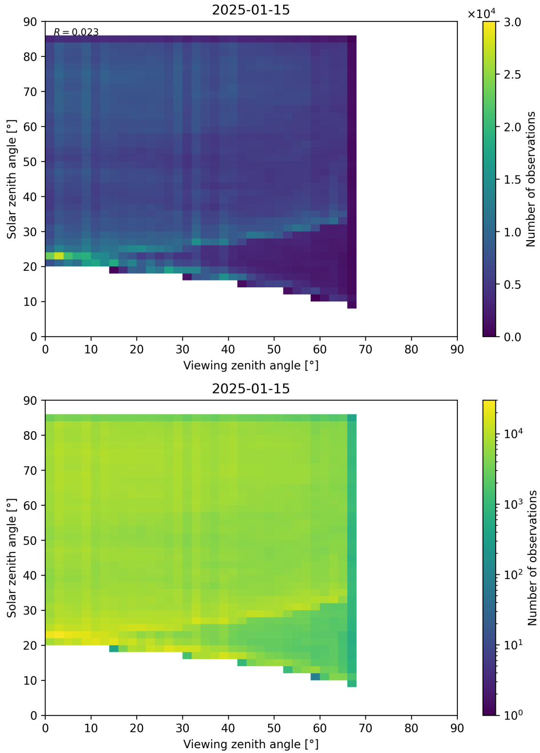
Figure 77: Scatter density plot of “Viewing zenith angle” against “Solar zenith angle” for 2025-01-14 to 2025-01-16.
