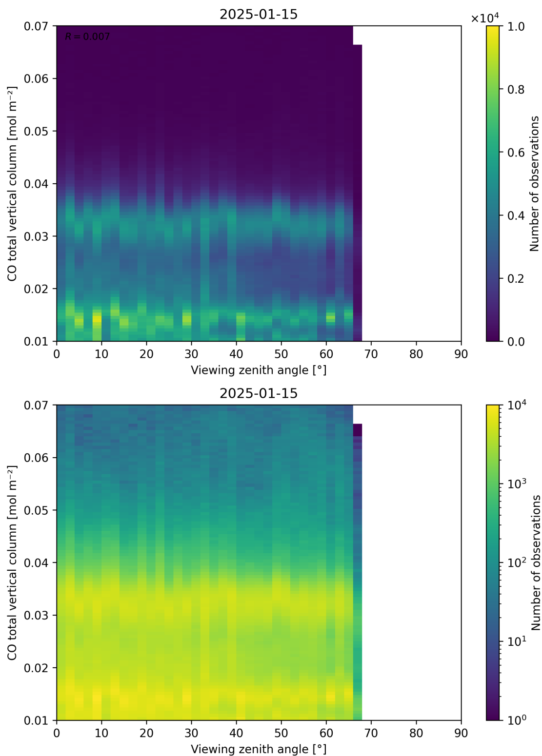
Figure 69: Scatter density plot of “Viewing zenith angle” against “CO total vertical column” for 2025-01-14 to 2025-01-16.
