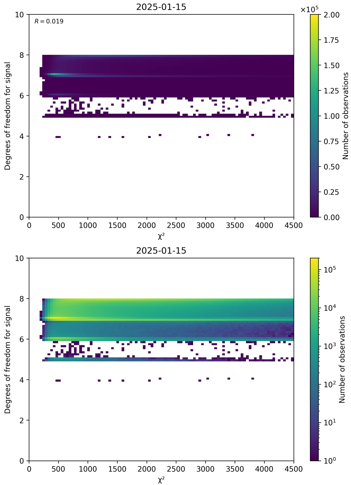
Figure 48: Scatter density plot of “ \chi^2 ” against “Degrees of freedom for signal” for 2025-01-14 to 2025-01-16.
