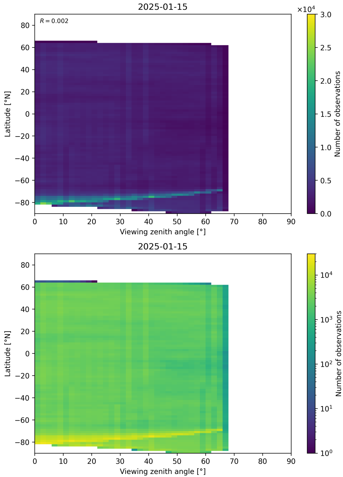
Figure 74: Scatter density plot of “Viewing zenith angle” against “Latitude” for 2025-01-14 to 2025-01-16.
