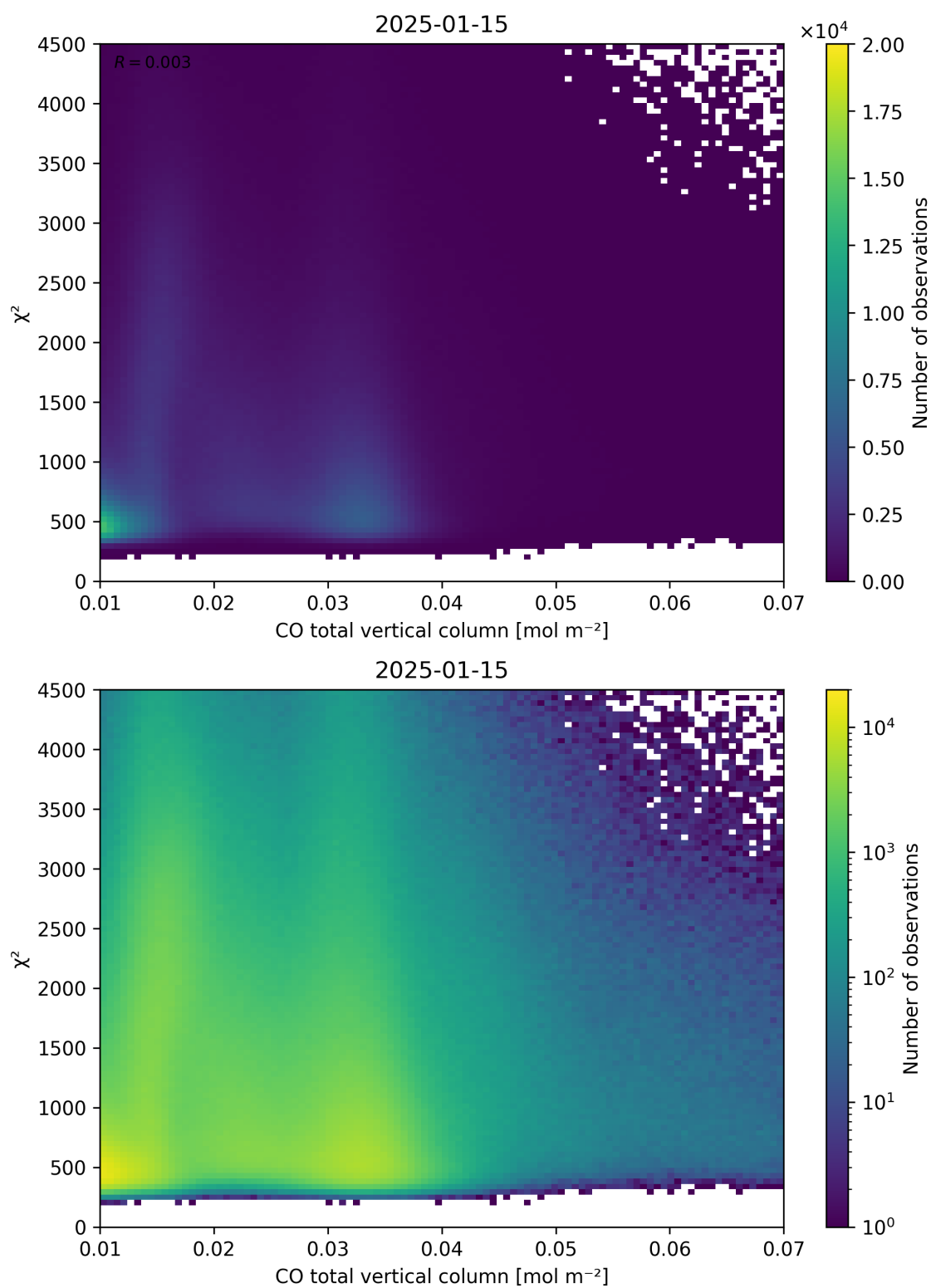
Figure 35: Scatter density plot of “CO total vertical column” against “ \chi^2 ” for 2025-01-14 to 2025-01-16.
