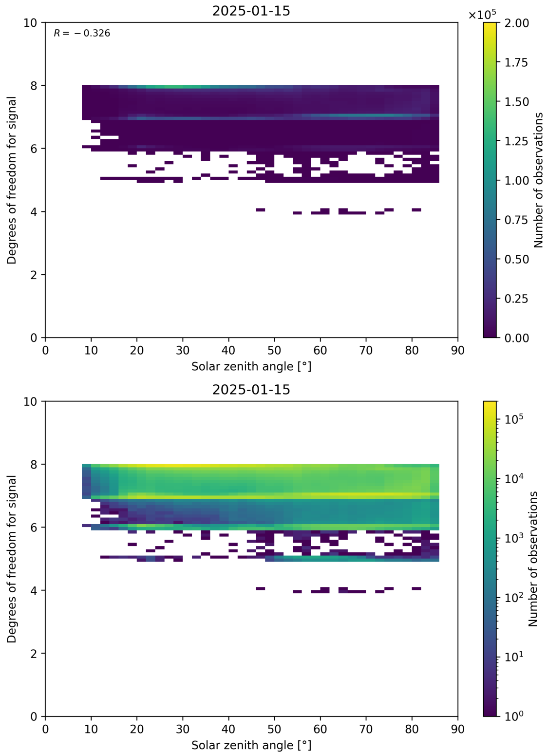
Figure 65: Scatter density plot of “Solar zenith angle” against “Degrees of freedom for signal” for 2025-01-14 to 2025-01-16.
