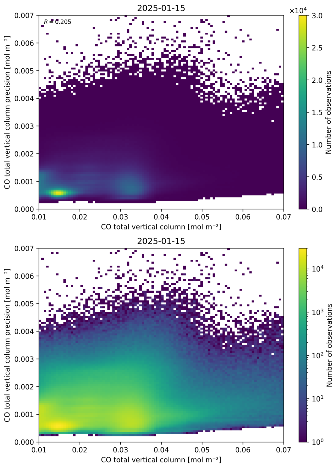
Figure 34: Scatter density plot of “CO total vertical column” against “CO total vertical column precision” for 2025-01-14 to 2025-01-16.
