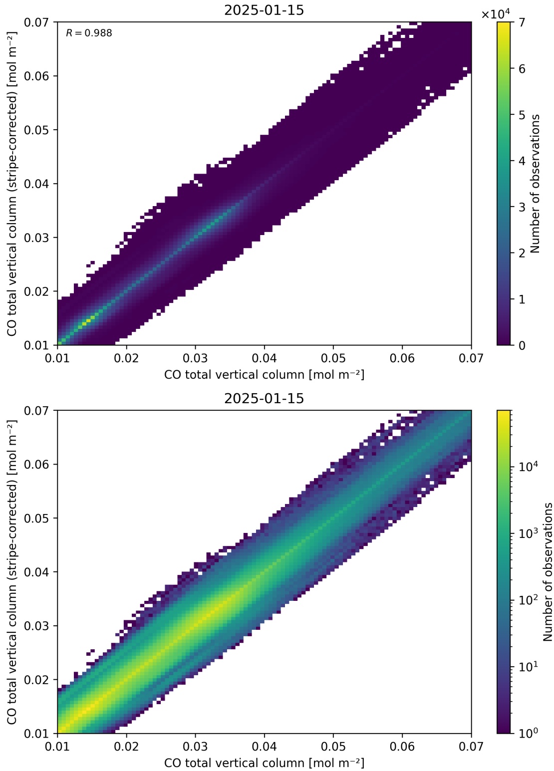
Figure 33: Scatter density plot of “CO total vertical column” against “CO total vertical column (stripe-corrected)” for 2025-01-14 to 2025-01-16.
