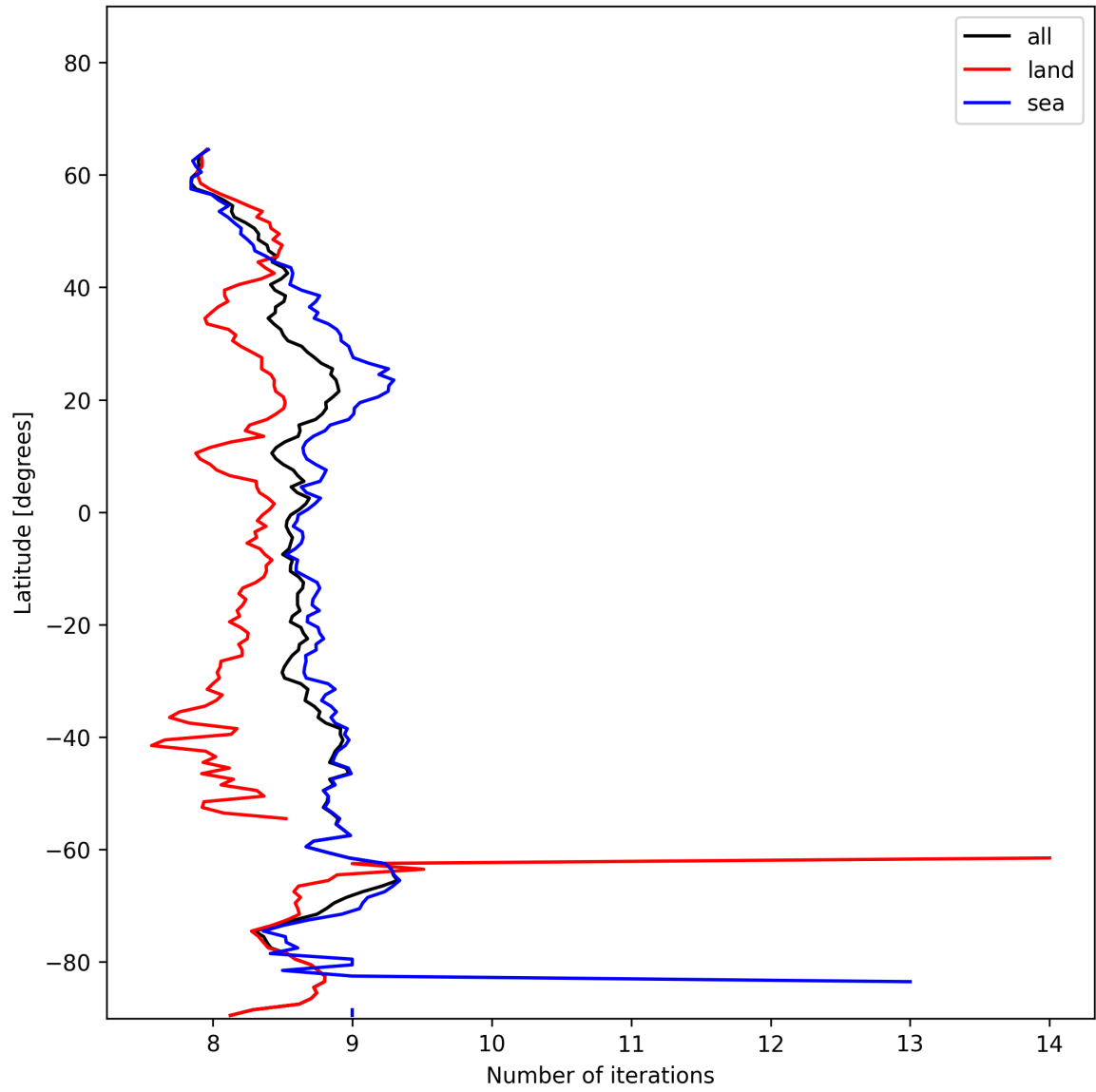
Figure 16: Zonal average of “Number of iterations” for 2025-01-14 to 2025-01-16.
