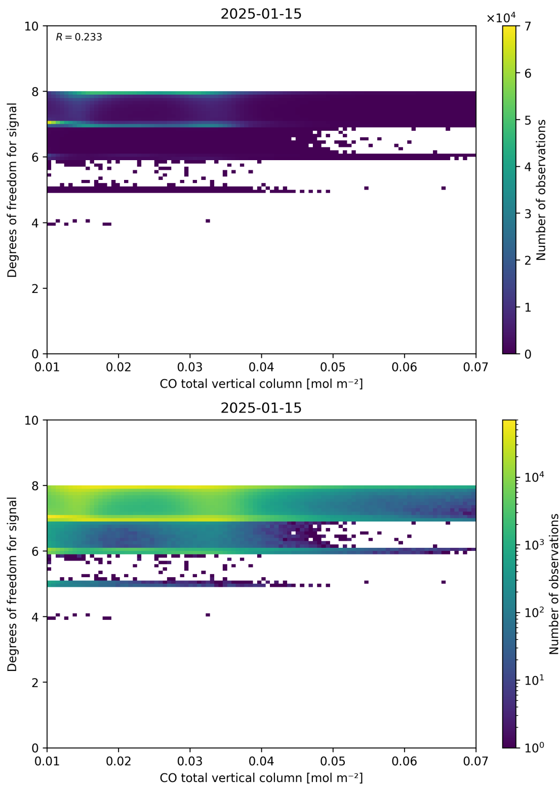
Figure 41: Scatter density plot of “CO total vertical column” against “Degrees of freedom for signal” for 2025-01-14 to 2025-01-16.
