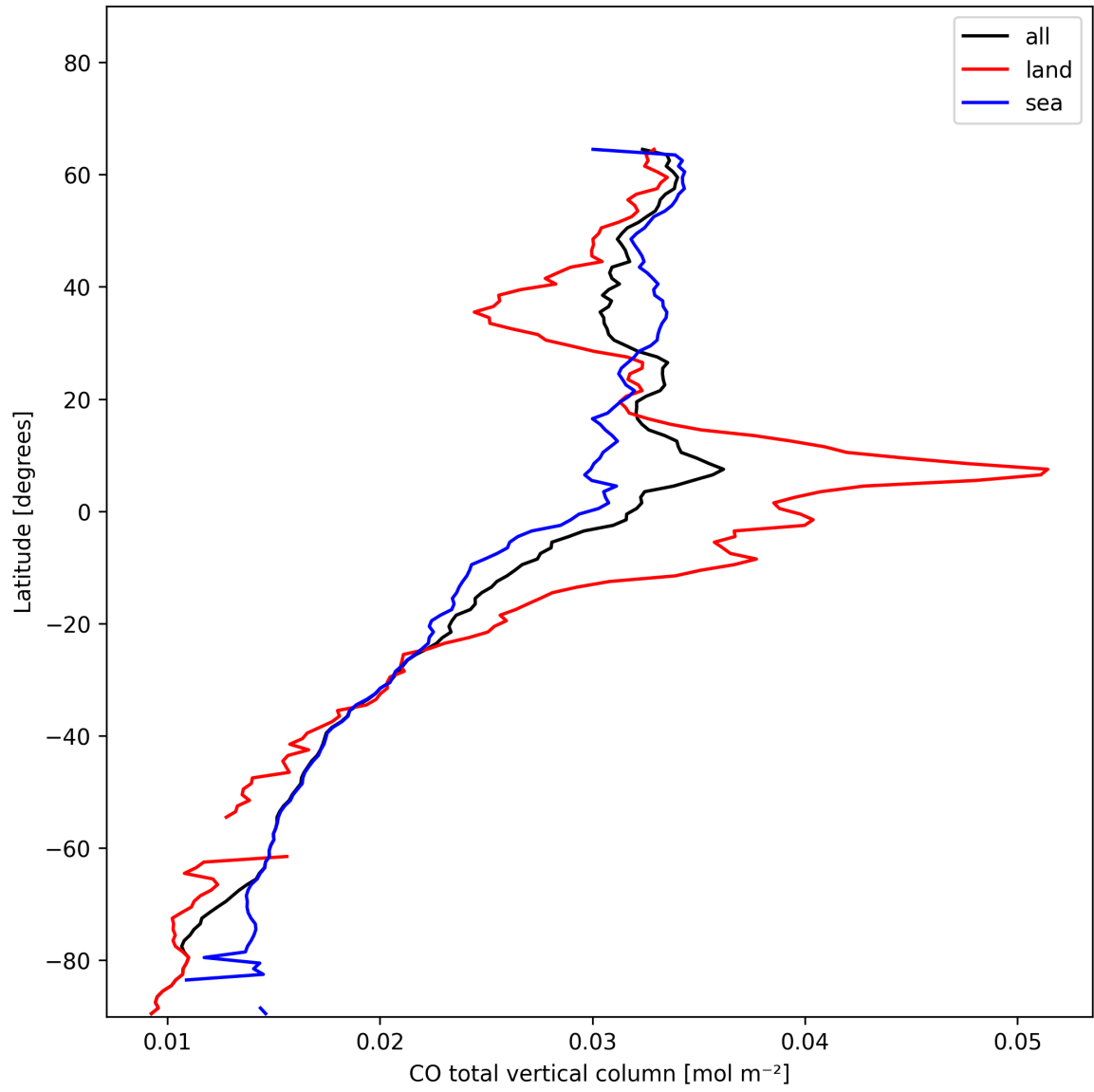
Figure 10: Zonal average of “CO total vertical column” for 2025-01-14 to 2025-01-16.
