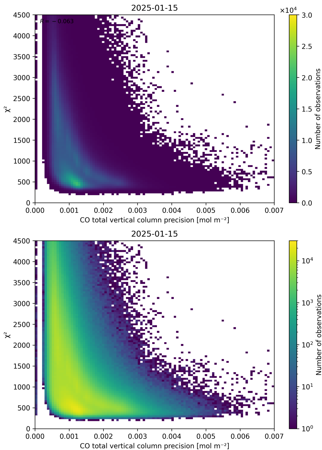
Figure 44: Scatter density plot of “CO total vertical column precision” against “ \chi^2 ” for 2025-01-14 to 2025-01-16.
