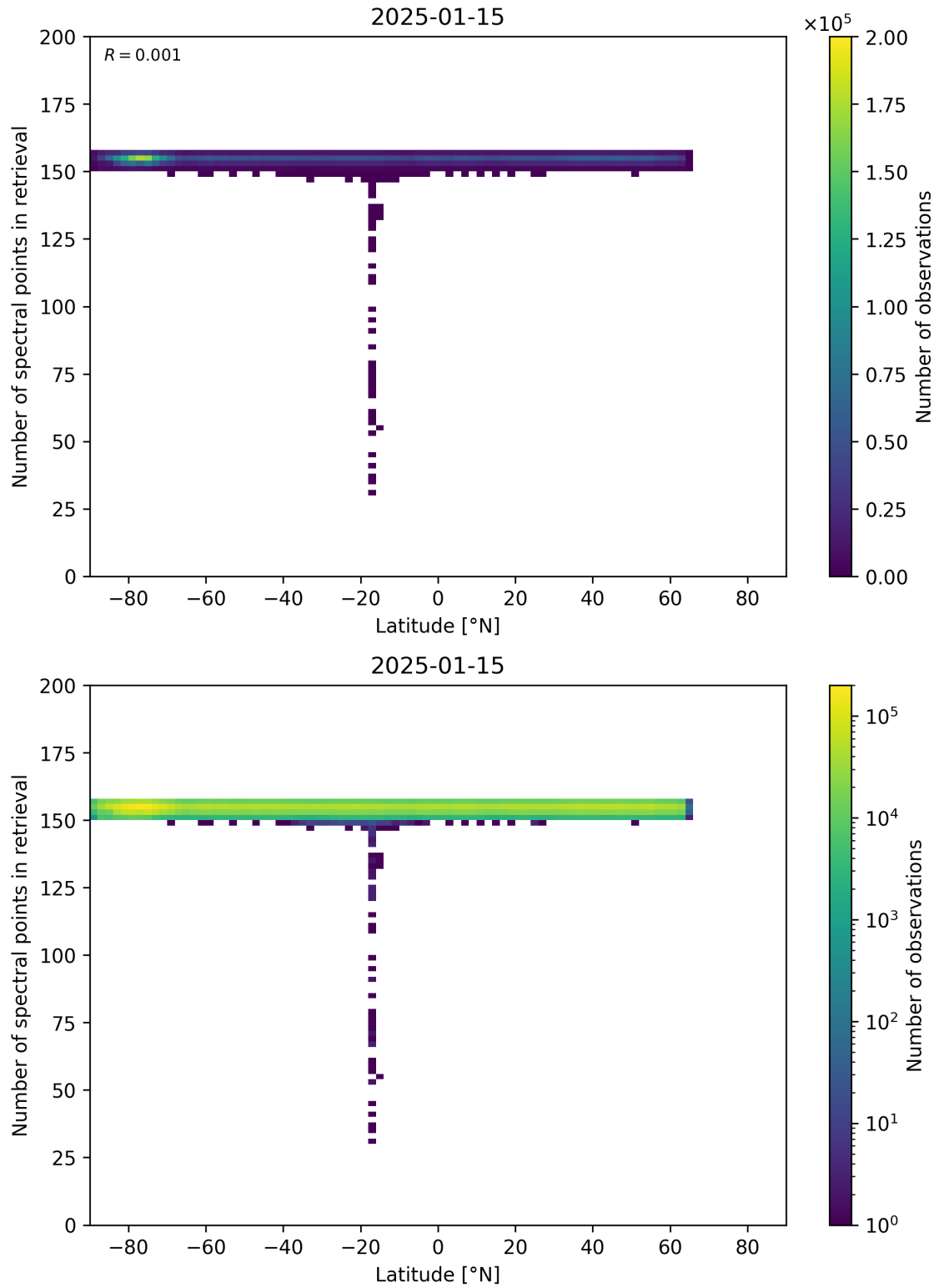
Figure 57: Scatter density plot of “Latitude” against “Number of spectral points in retrieval” for 2025-01-14 to 2025-01-16.
