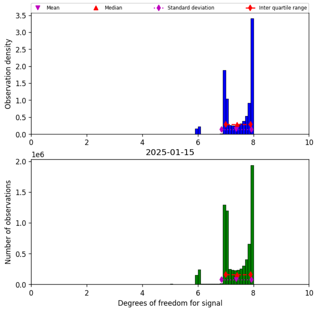
Figure 23: Histogram of “Degrees of freedom for signal” for 2025-01-14 to 2025-01-16
