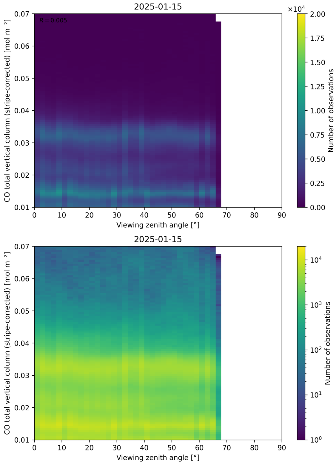
Figure 70: Scatter density plot of “Viewing zenith angle” against “CO total vertical column (stripe-corrected)” for 2025-01-14 to 2025-01-16.
