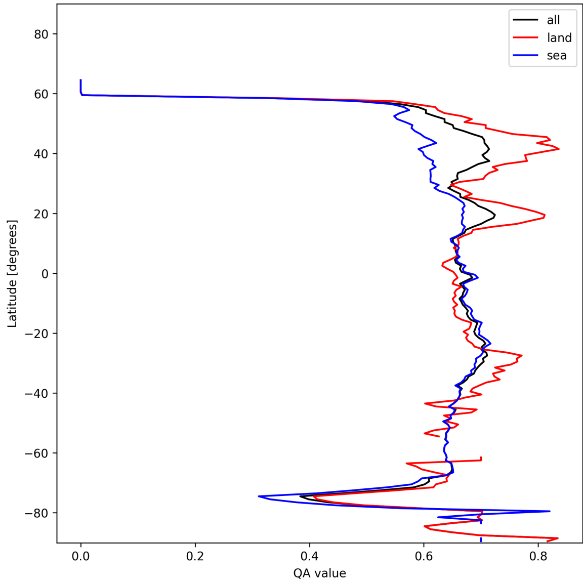
Figure 9: Zonal average of “QA value” for 2025-01-14 to 2025-01-16.
