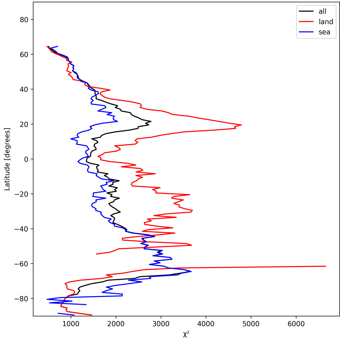
Figure 14: Zonal average of “ \chi^2 ” for 2025-01-14 to 2025-01-16.
