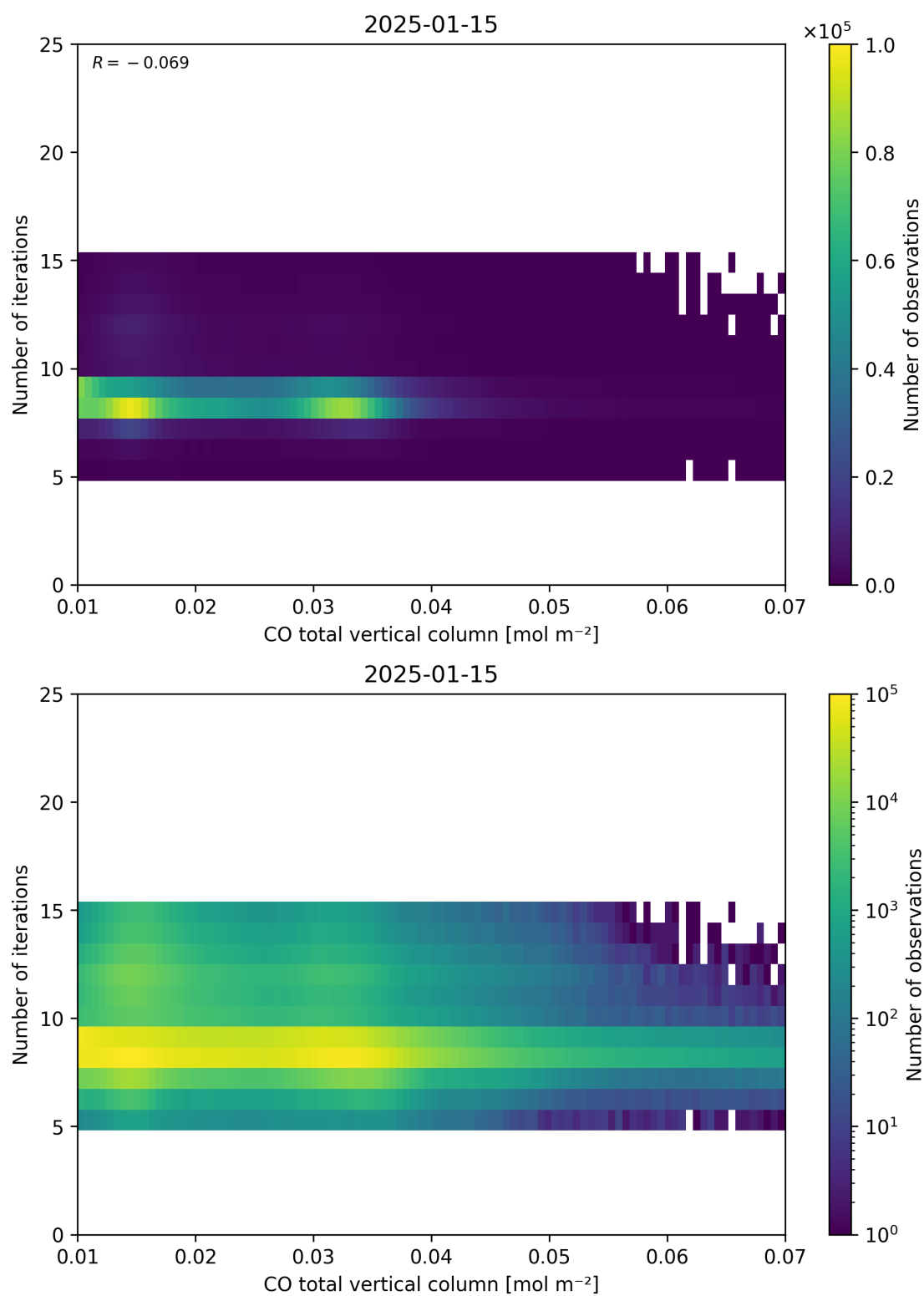
Figure 42: Scatter density plot of “CO total vertical column” against “Number of iterations” for 2025-01-14 to 2025-01-16.
