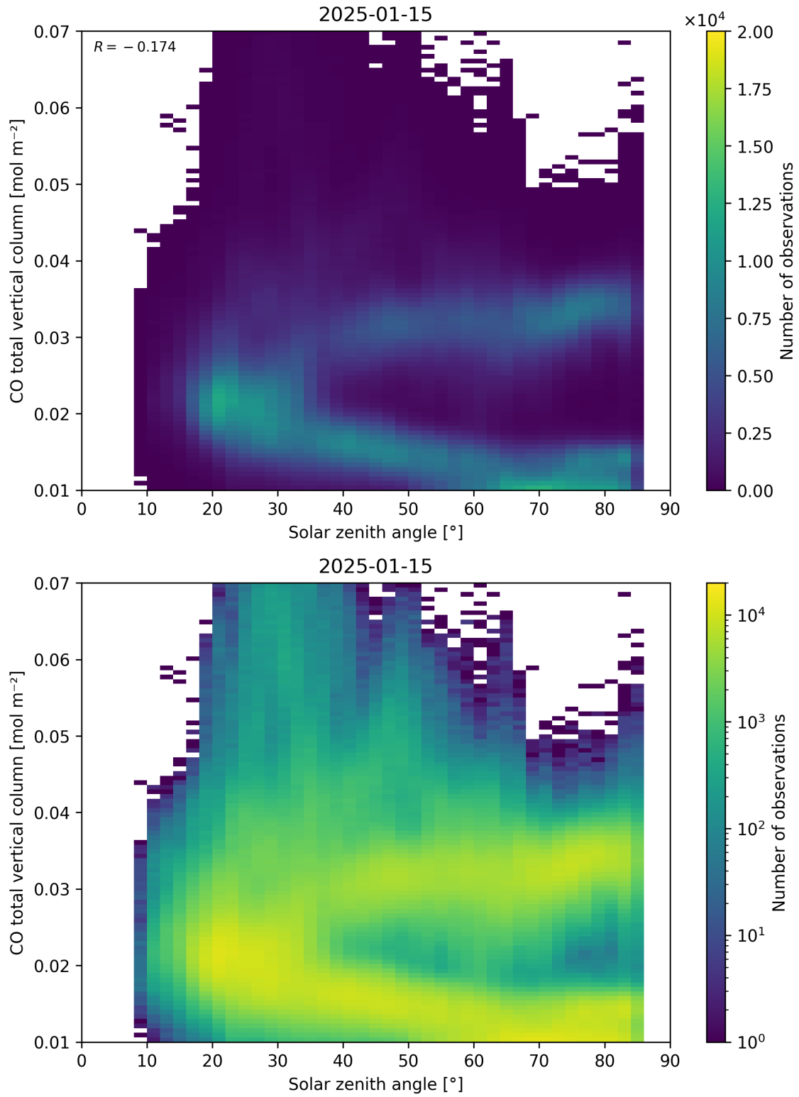
Figure 61: Scatter density plot of “Solar zenith angle” against “CO total vertical column” for 2025-01-14 to 2025-01-16.
