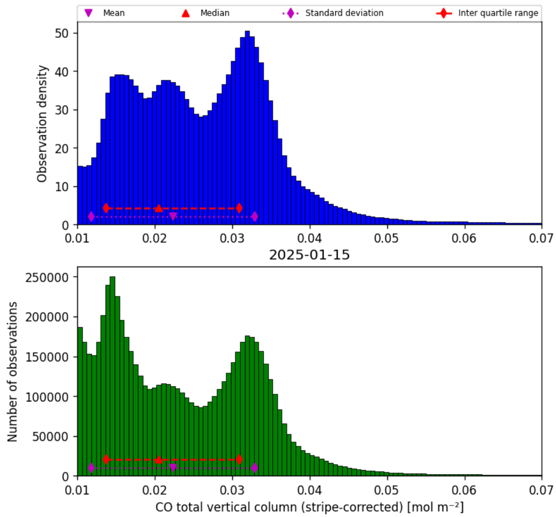
Figure 19: Histogram of “CO total vertical column (stripe-corrected)” for 2025-01-14 to 2025-01-16
