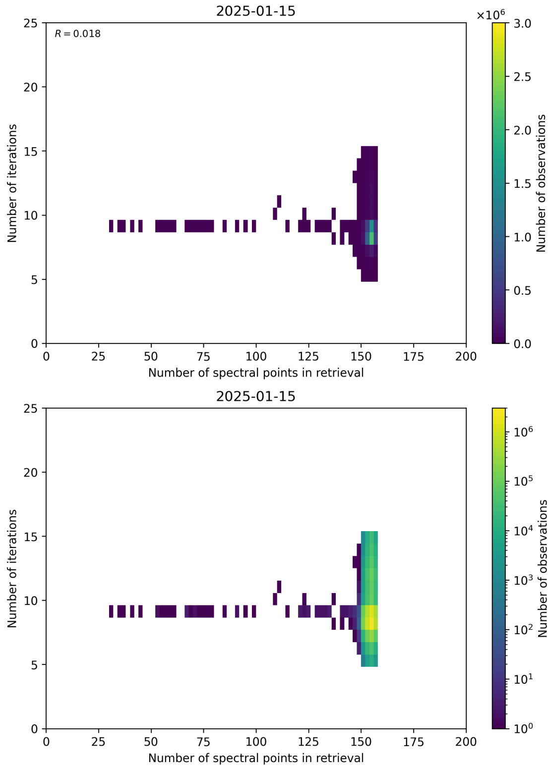
Figure 60: Scatter density plot of “Number of spectral points in retrieval” against “Number of iterations” for 2025-01-14 to 2025-01-16.
