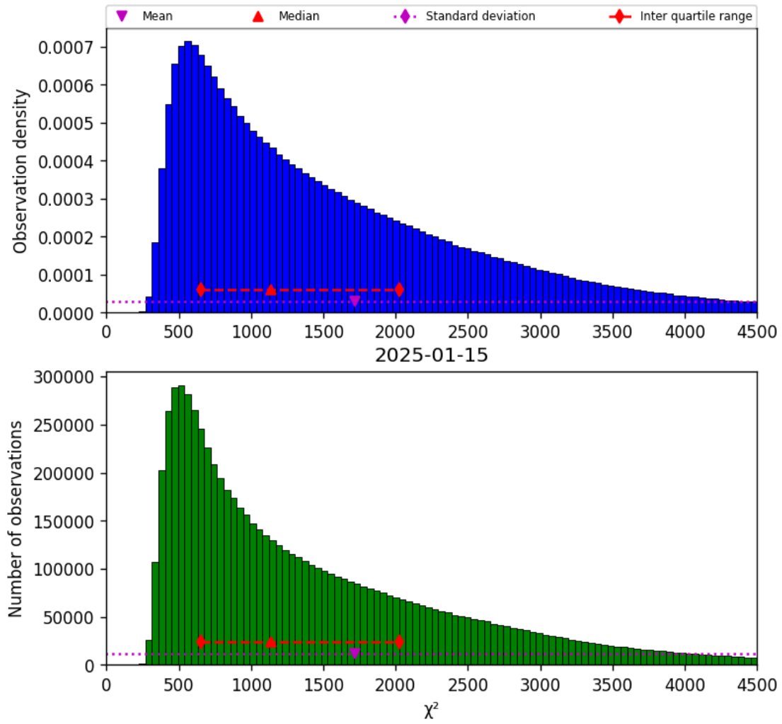
Figure 22: Histogram of “ \chi^2 ” for 2025-01-14 to 2025-01-16
