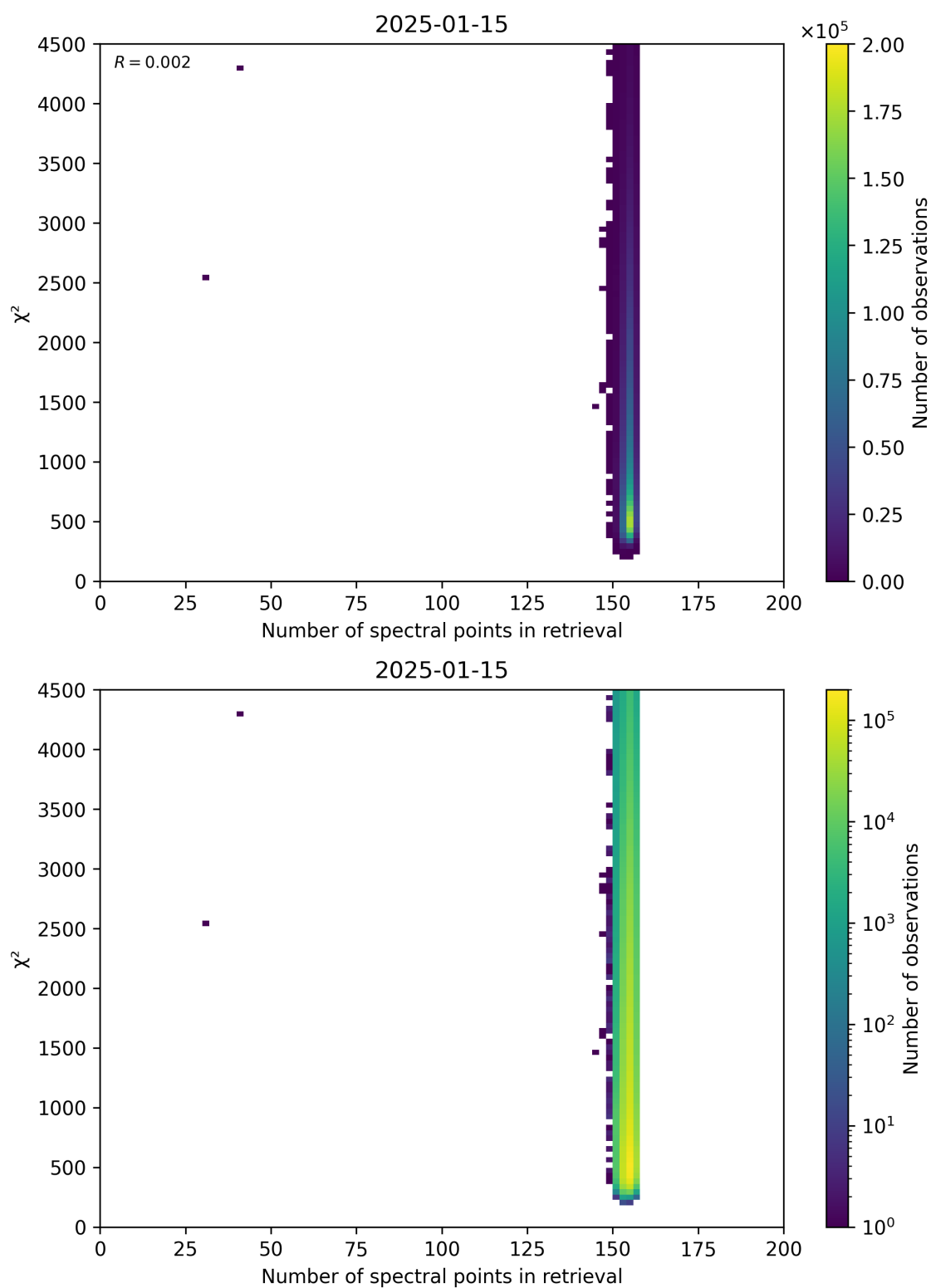
Figure 58: Scatter density plot of “Number of spectral points in retrieval” against “ \chi^2 ” for 2025-01-14 to 2025-01-16.
