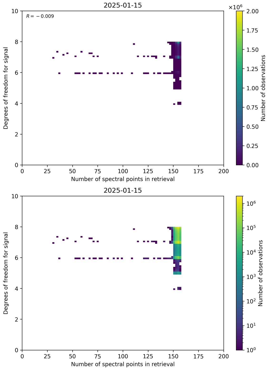
Figure 59: Scatter density plot of “Number of spectral points in retrieval” against “Degrees of freedom for signal” for 2025-01-14 to 2025-01-16.
