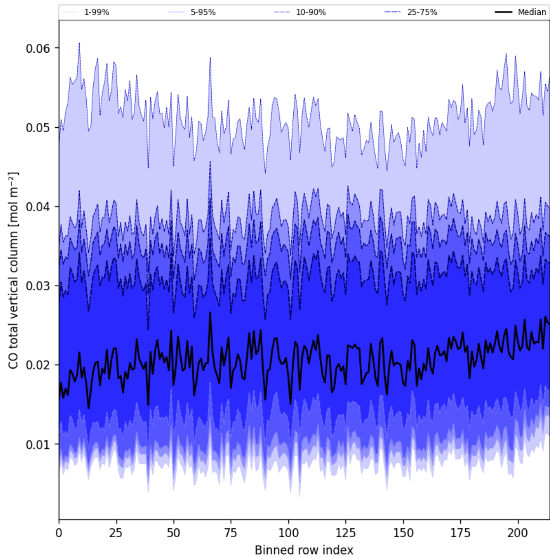
Figure 26: Along track statistics of “CO total vertical column” for 2025-01-14 to 2025-01-16
