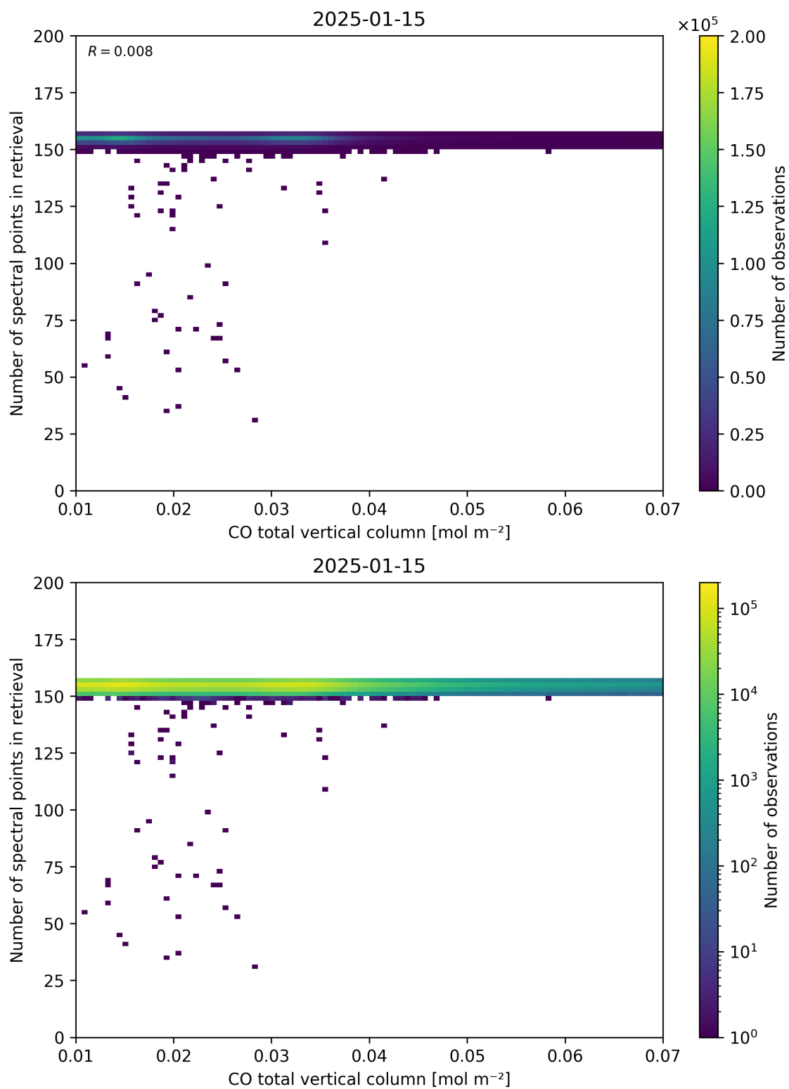
Figure 43: Scatter density plot of “CO total vertical column” against “Number of spectral points in retrieval” for 2025-01-14 to 2025-01-16.
