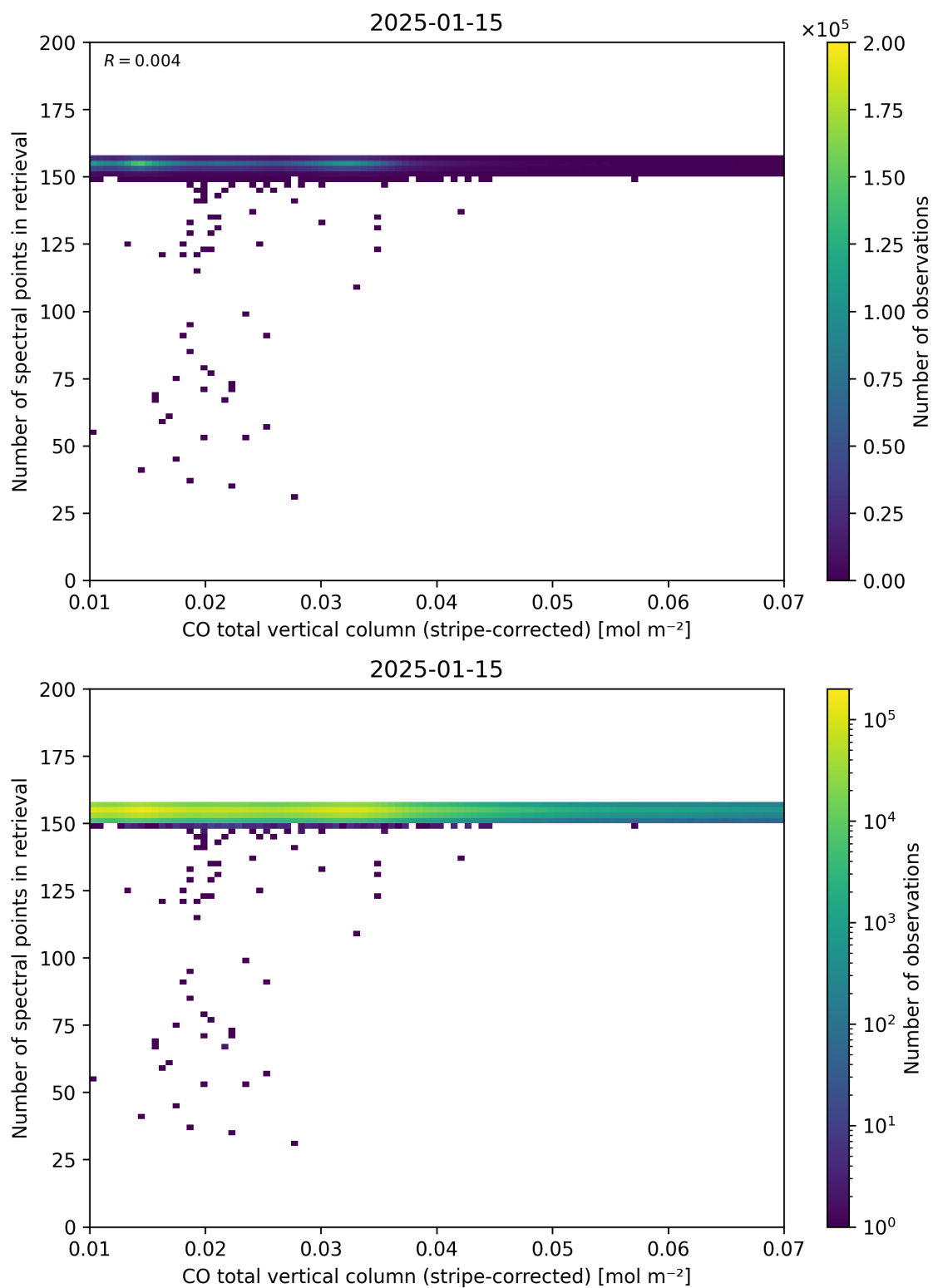
Figure 40: Scatter density plot of “CO total vertical column (stripe-corrected)” against “Number of spectral points in retrieval” for 2025-01-14 to 2025-01-16.
