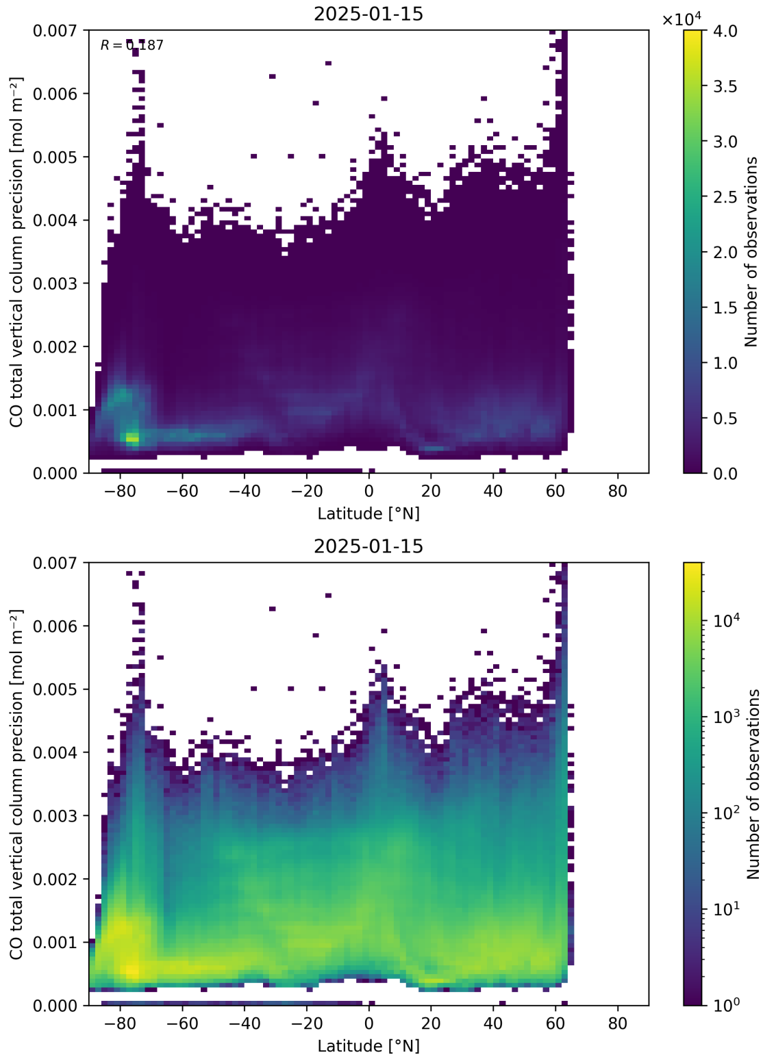
Figure 53: Scatter density plot of “Latitude” against “CO total vertical column precision” for 2025-01-14 to 2025-01-16.
