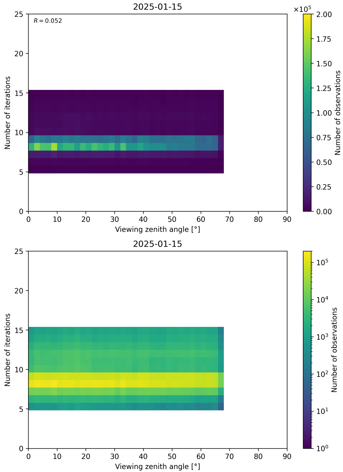
Figure 75: Scatter density plot of “Viewing zenith angle” against “Number of iterations” for 2025-01-14 to 2025-01-16.
