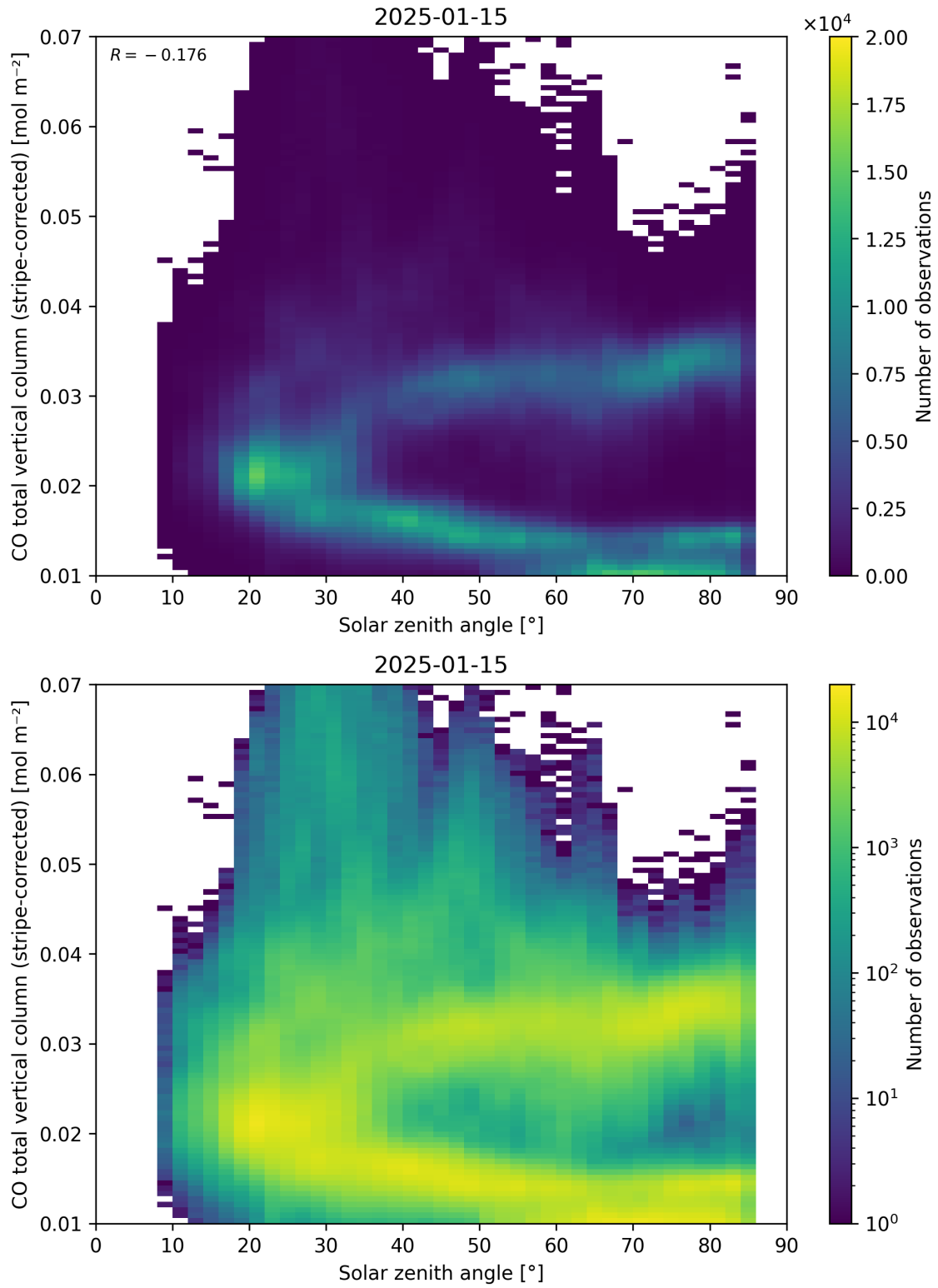
Figure 62: Scatter density plot of “Solar zenith angle” against “CO total vertical column (stripe-corrected)” for 2025-01-14 to 2025-01-16.
