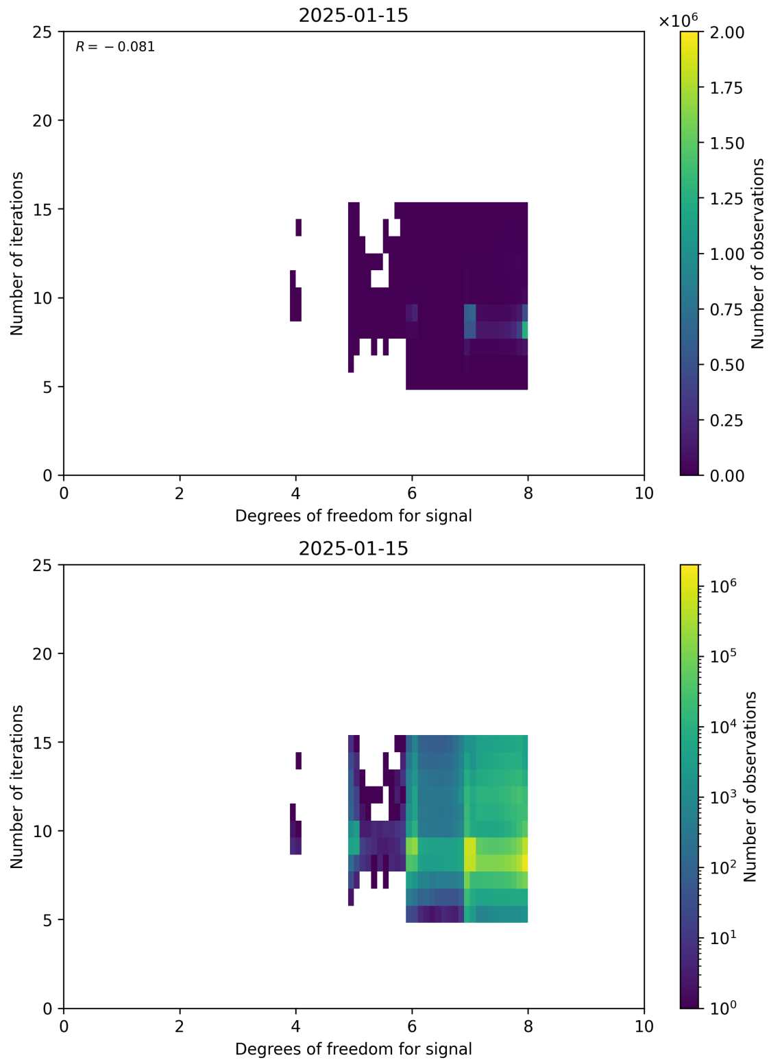
Figure 50: Scatter density plot of “Degrees of freedom for signal” against “Number of iterations” for 2025-01-14 to 2025-01-16.
