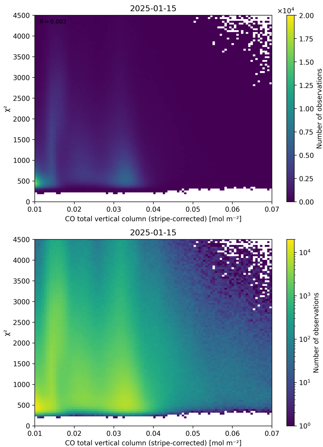
Figure 37: Scatter density plot of “CO total vertical column (stripe-corrected)” against “ \chi^2 ” for 2025-01-14 to 2025-01-16.
