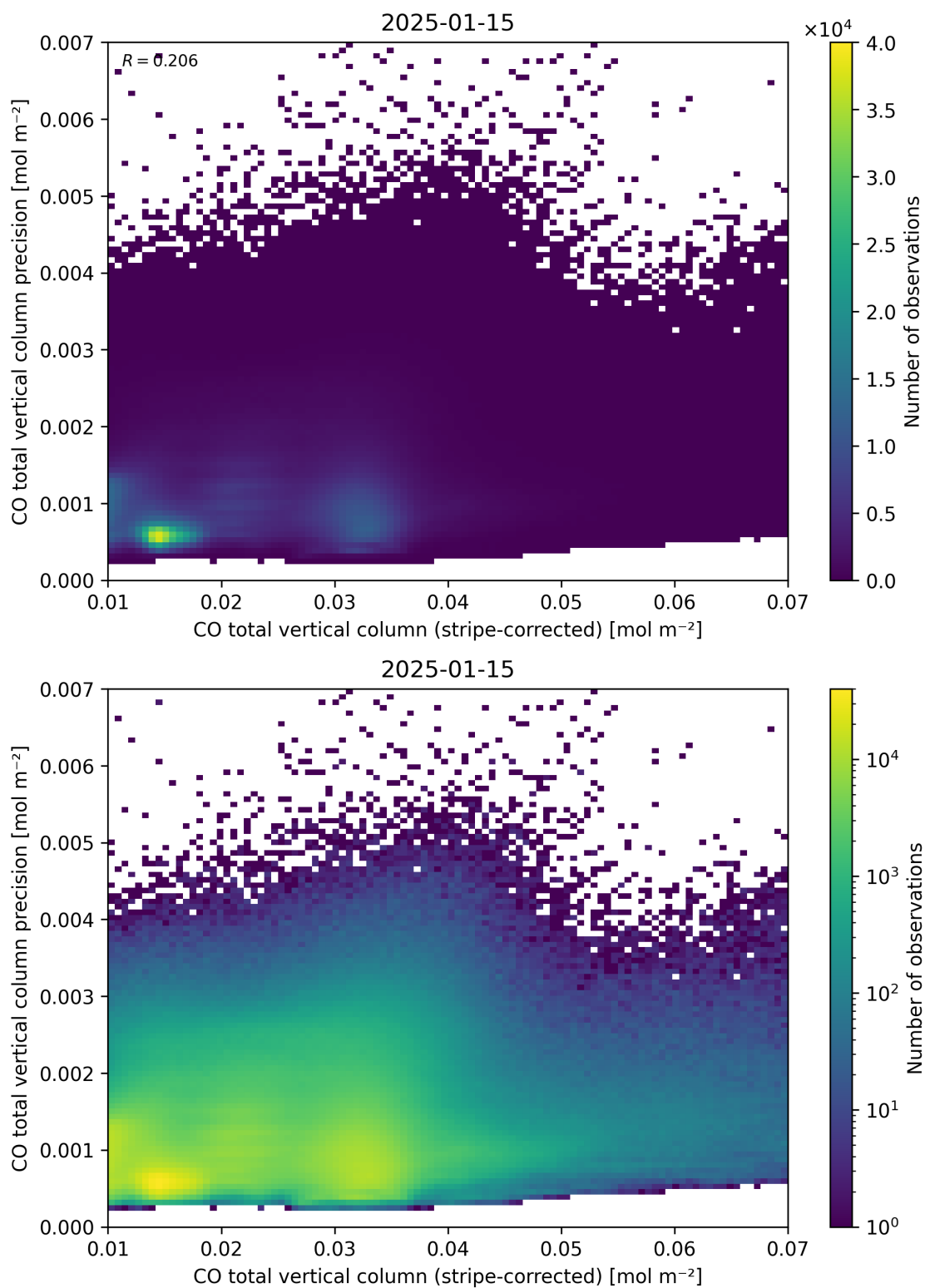
Figure 36: Scatter density plot of “CO total vertical column (stripe-corrected)” against “CO total vertical column precision” for 2025-01-14 to 2025-01-16.
