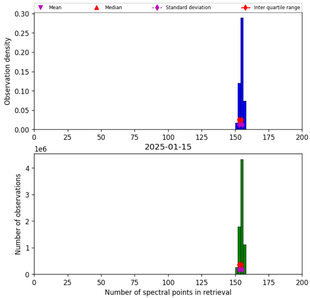
Figure 21: Histogram of “Number of spectral points in retrieval” for 2025-01-14 to 2025-01-16
