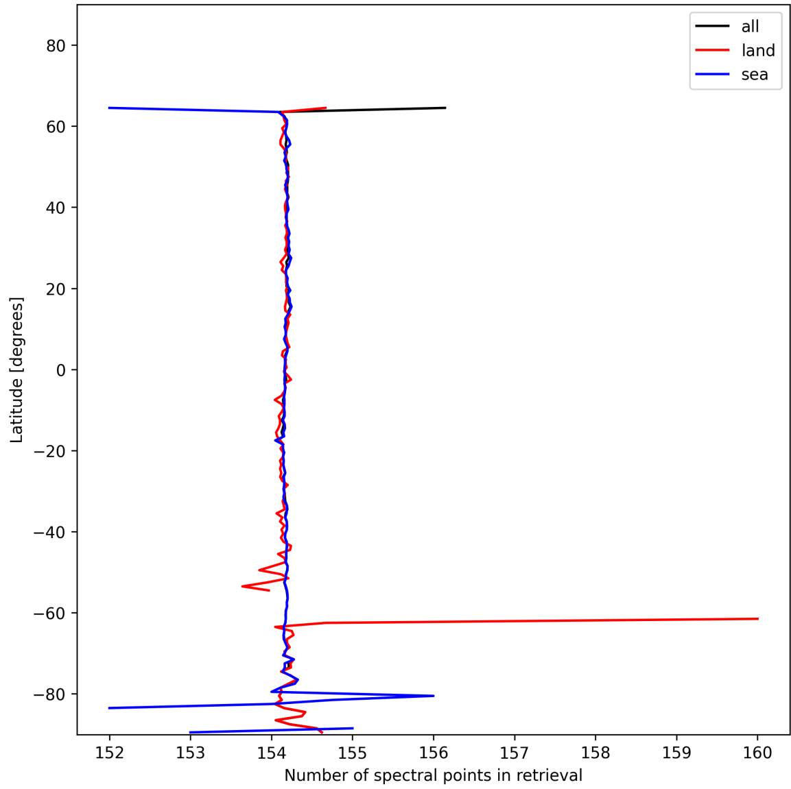
Figure 13: Zonal average of “Number of spectral points in retrieval” for 2025-01-14 to 2025-01-16.
