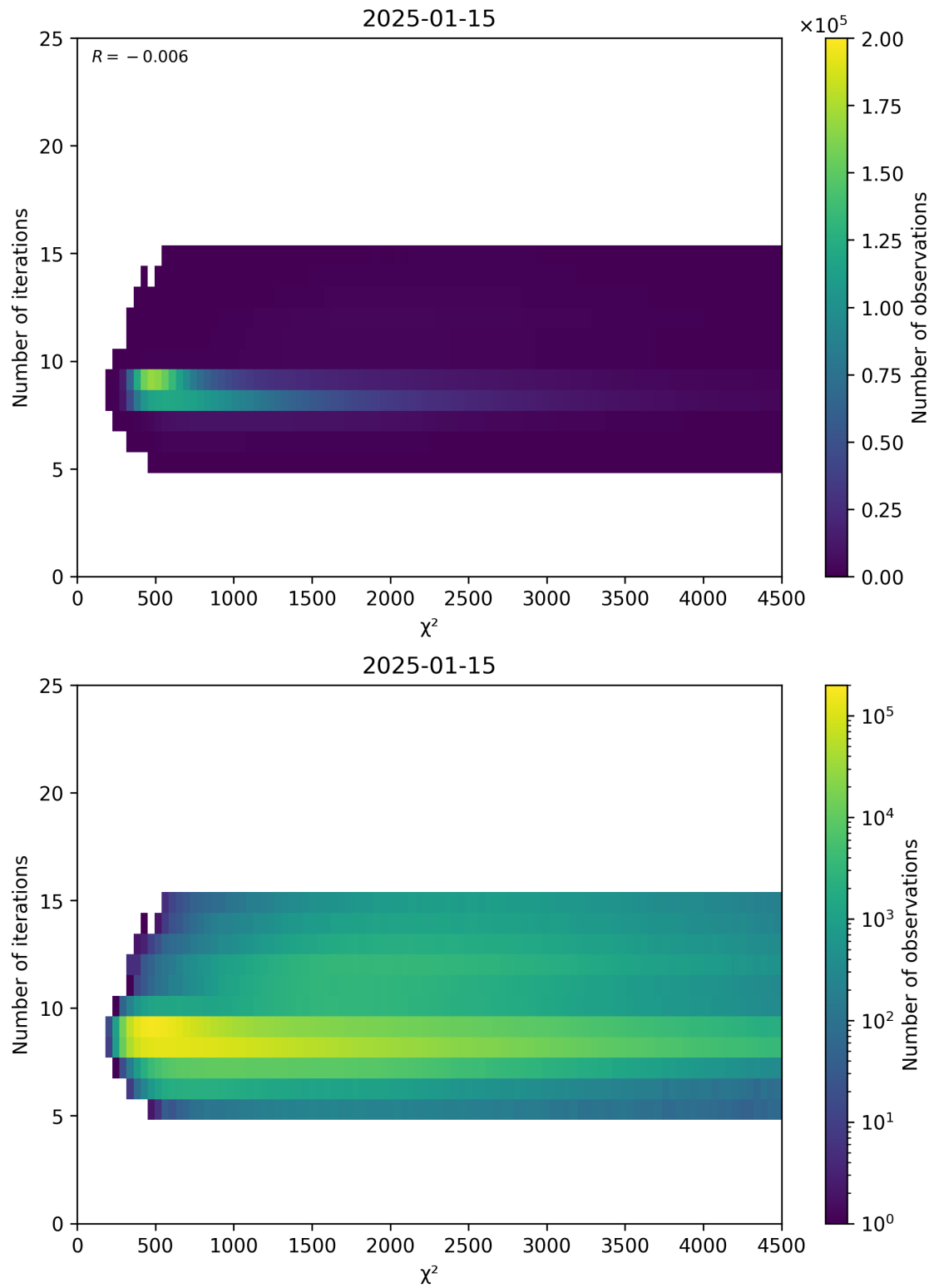
Figure 49: Scatter density plot of “ \chi^2 ” against “Number of iterations” for 2025-01-14 to 2025-01-16.
