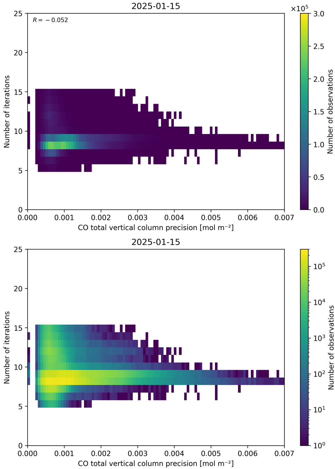
Figure 46: Scatter density plot of “CO total vertical column precision” against “Number of iterations” for 2025-01-14 to 2025-01-16.
