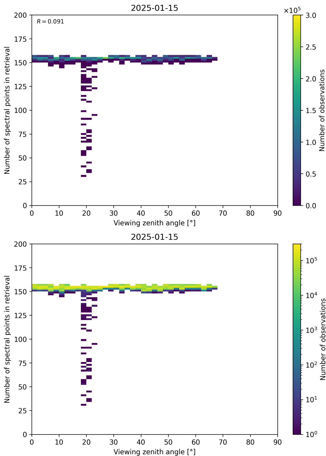
Figure 76: Scatter density plot of “Viewing zenith angle” against “Number of spectral points in retrieval” for 2025-01-14 to 2025-01-16.
