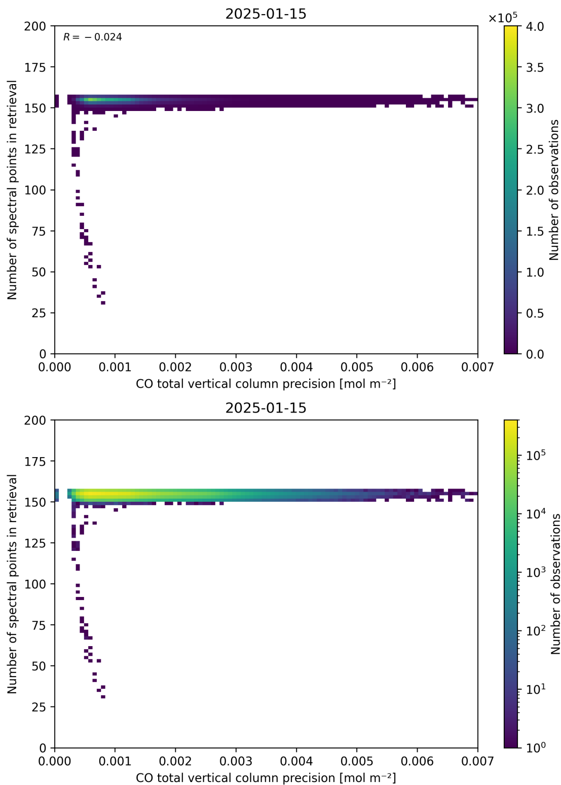
Figure 47: Scatter density plot of “CO total vertical column precision” against “Number of spectral points in retrieval” for 2025-01-14 to 2025-01-16.
