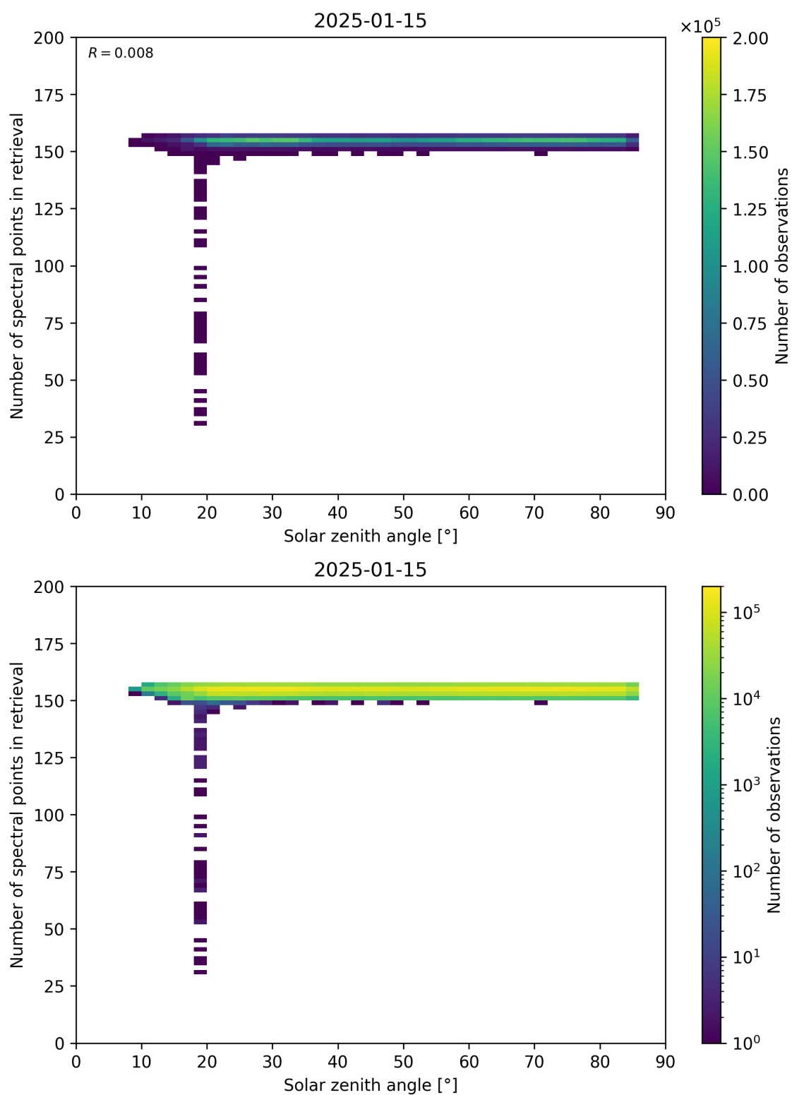
Figure 68: Scatter density plot of “Solar zenith angle” against “Number of spectral points in retrieval” for 2025-01-14 to 2025-01-16.
