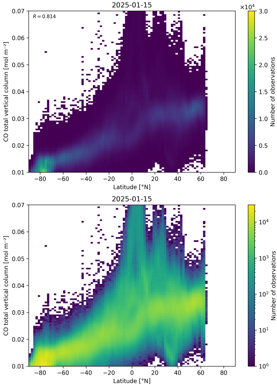
Figure 51: Scatter density plot of “Latitude” against “CO total vertical column” for 2025-01-14 to 2025-01-16.
