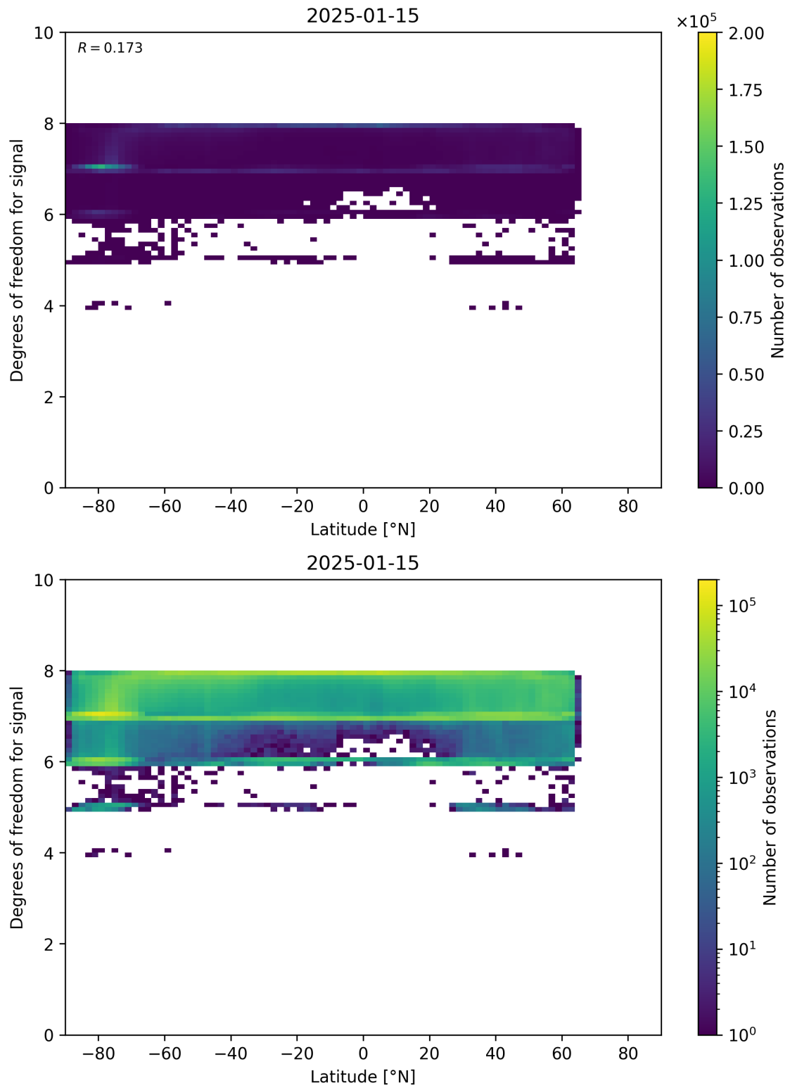
Figure 55: Scatter density plot of “Latitude” against “Degrees of freedom for signal” for 2025-01-14 to 2025-01-16.
