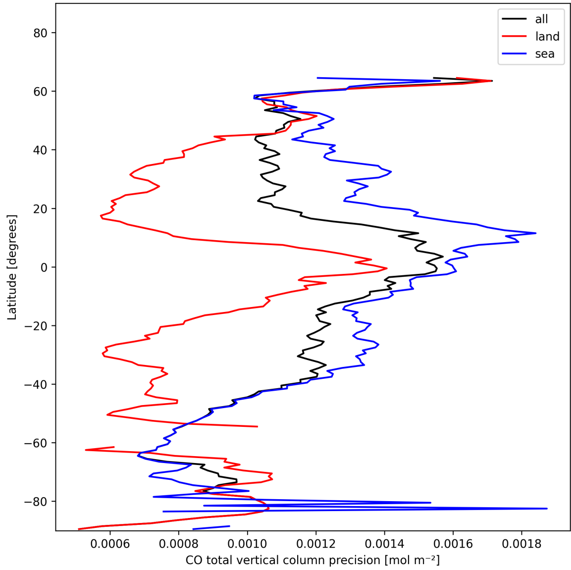
Figure 12: Zonal average of “CO total vertical column precision” for 2025-01-14 to 2025-01-16.
