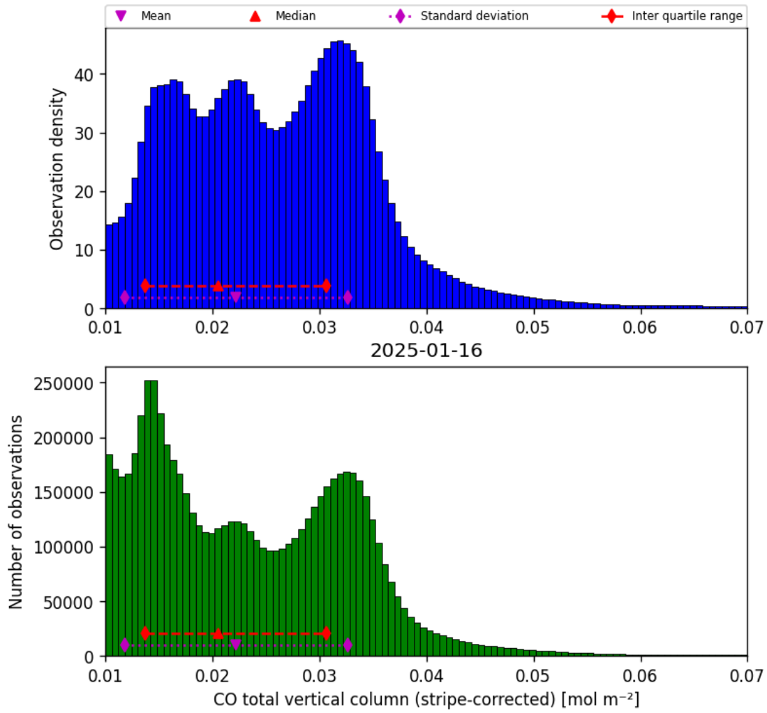
Figure 19: Histogram of “CO total vertical column (stripe-corrected)” for 2025-01-15 to 2025-01-17
