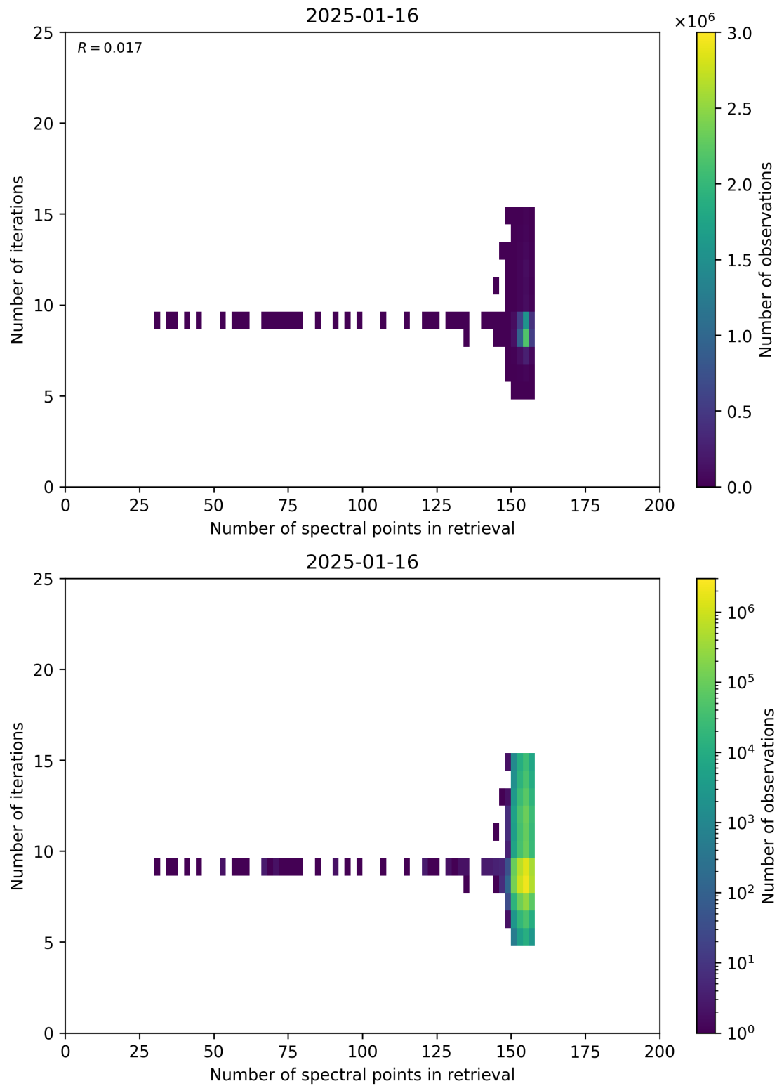
Figure 60: Scatter density plot of “Number of spectral points in retrieval” against “Number of iterations” for 2025-01-15 to 2025-01-17.
