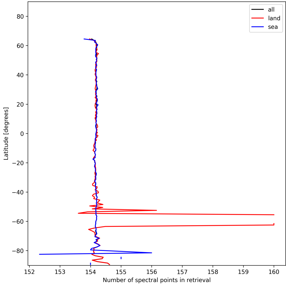
Figure 13: Zonal average of “Number of spectral points in retrieval” for 2025-01-15 to 2025-01-17.
