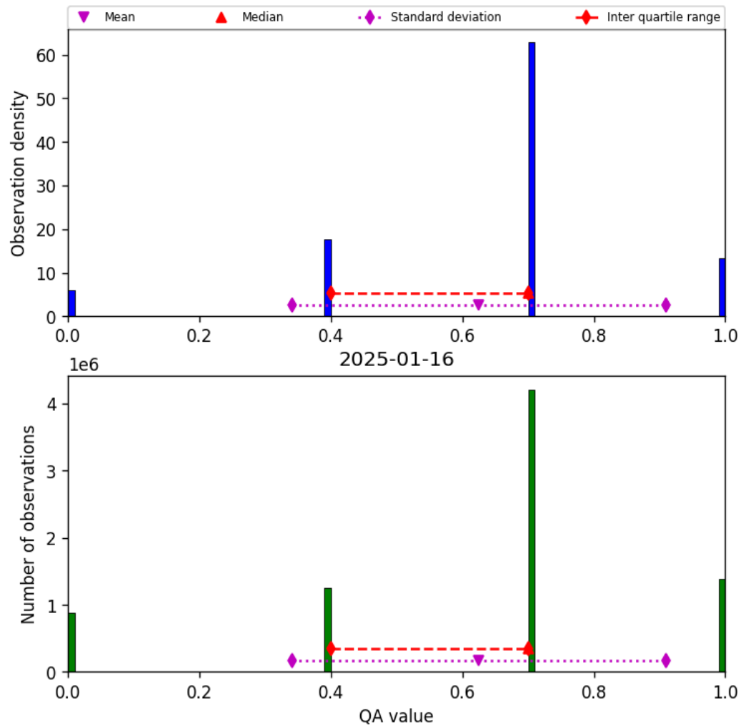
Figure 17: Histogram of “QA value” for 2025-01-15 to 2025-01-17
