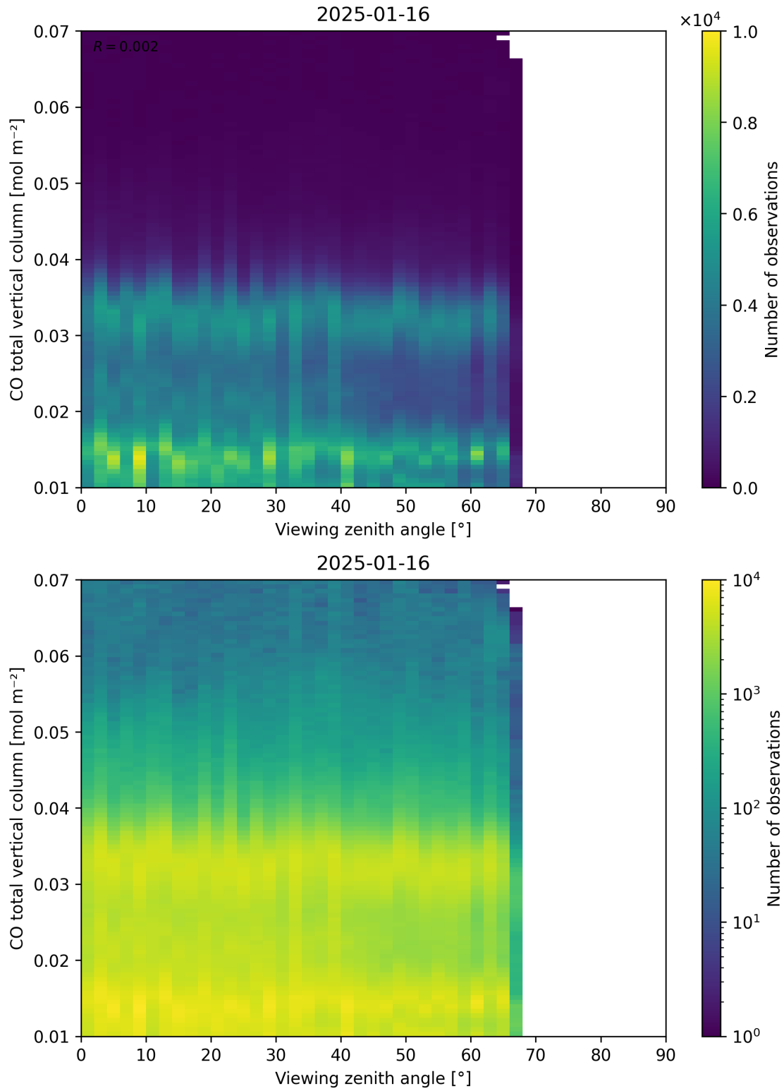
Figure 69: Scatter density plot of “Viewing zenith angle” against “CO total vertical column” for 2025-01-15 to 2025-01-17.
