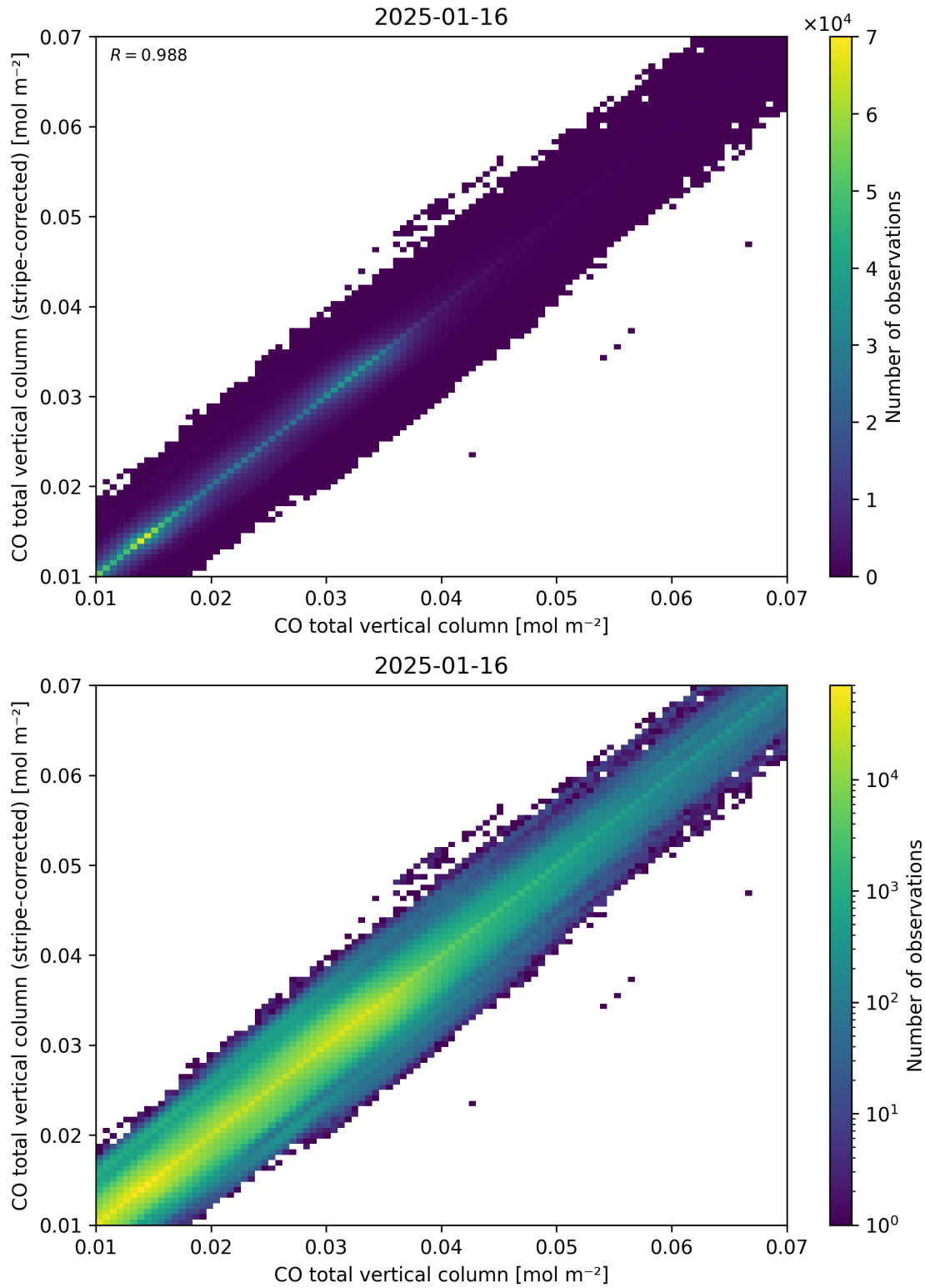
Figure 33: Scatter density plot of “CO total vertical column” against “CO total vertical column (stripe-corrected)” for 2025-01-15 to 2025-01-17.
