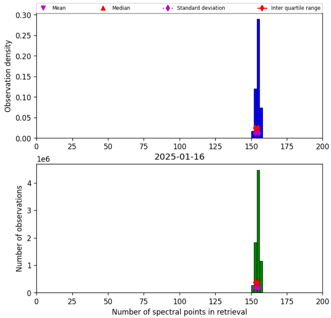
Figure 21: Histogram of “Number of spectral points in retrieval” for 2025-01-15 to 2025-01-17
