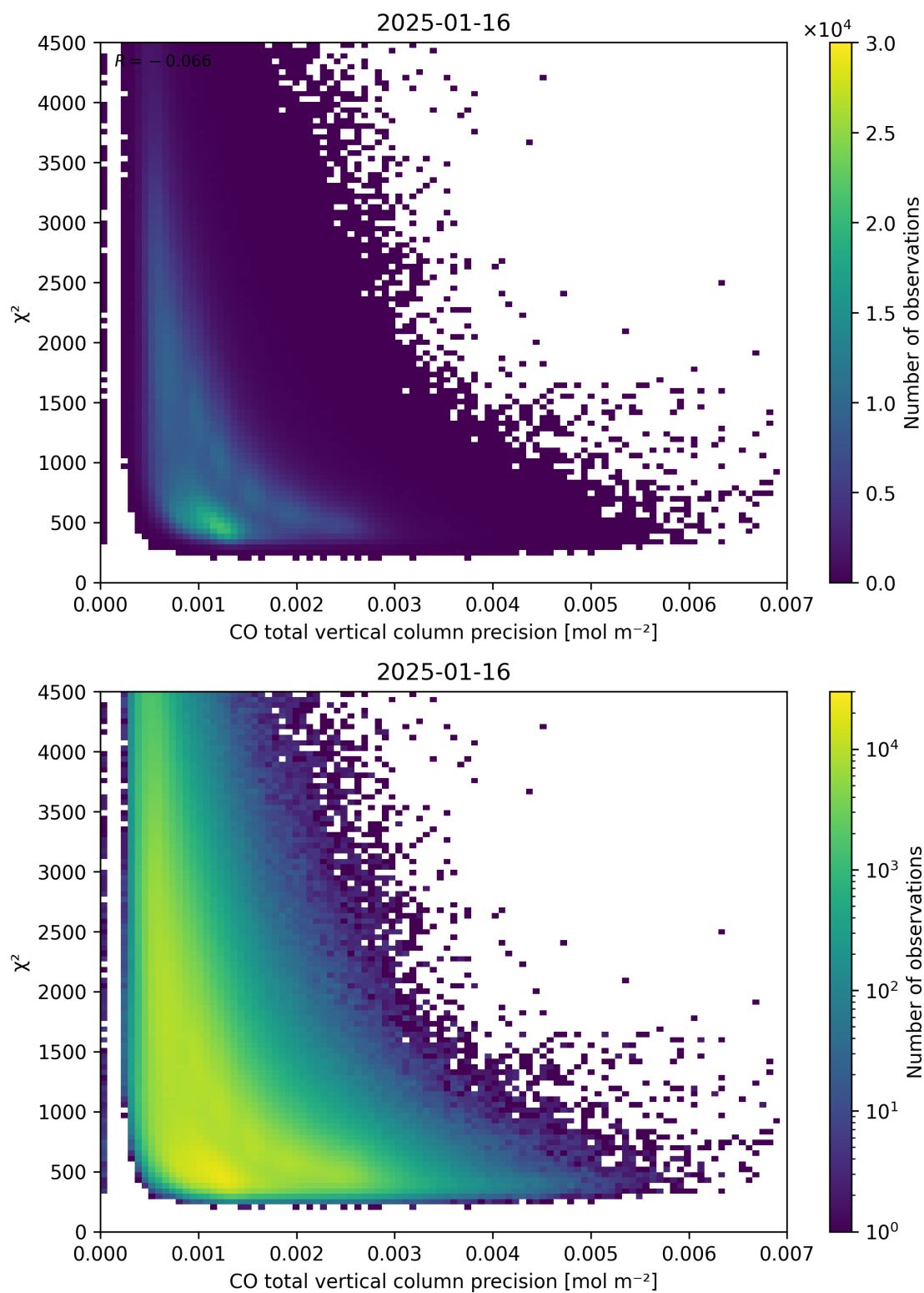
Figure 44: Scatter density plot of “CO total vertical column precision” against “ \chi^2 ” for 2025-01-15 to 2025-01-17.
