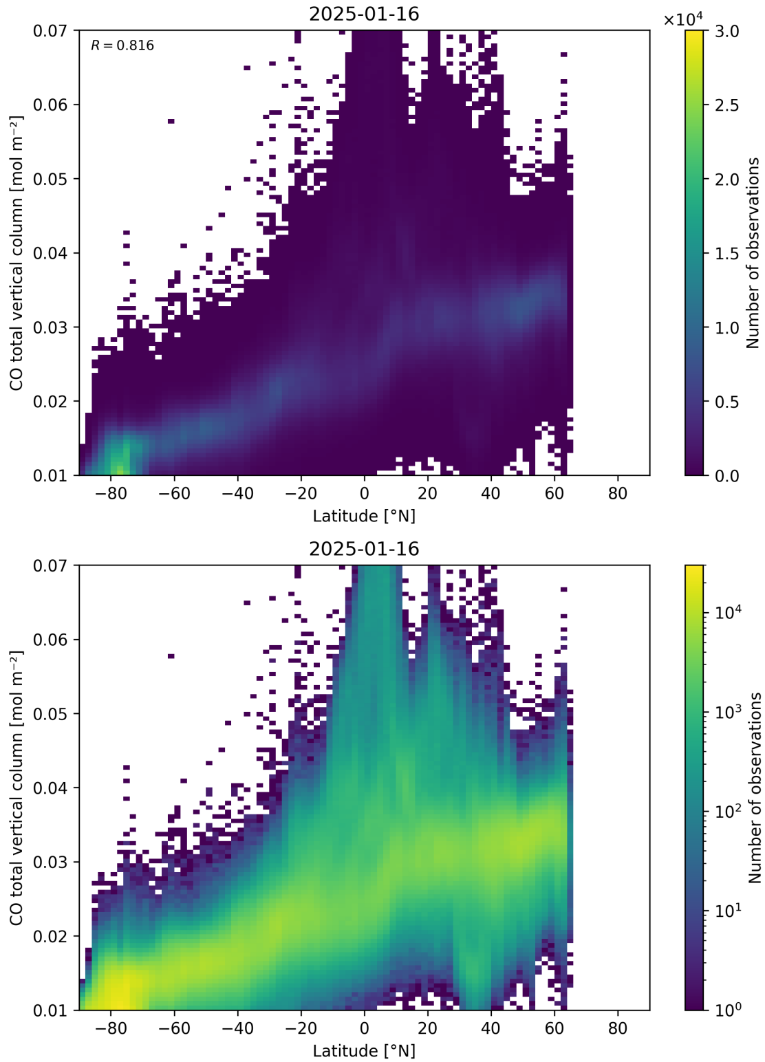
Figure 51: Scatter density plot of “Latitude” against “CO total vertical column” for 2025-01-15 to 2025-01-17.
