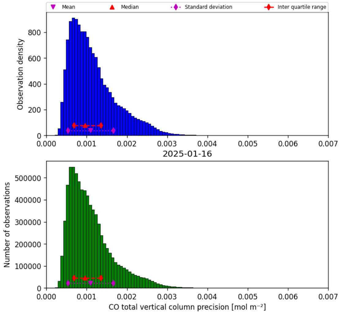
Figure 20: Histogram of “CO total vertical column precision” for 2025-01-15 to 2025-01-17
