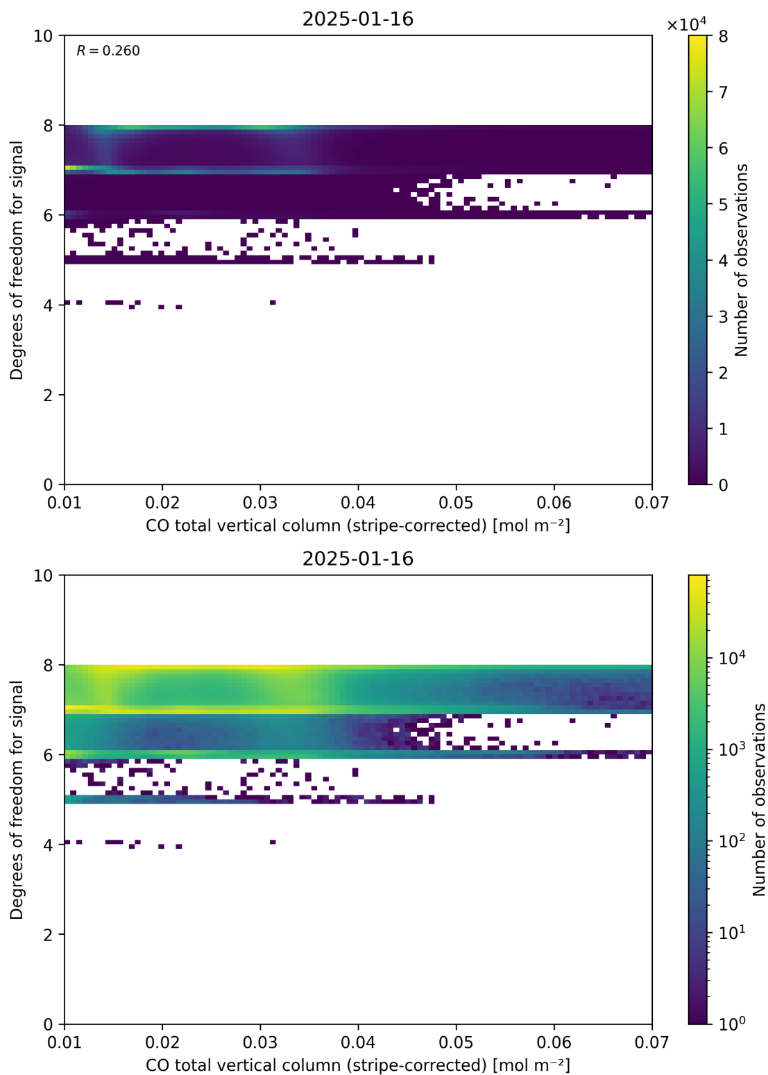
Figure 38: Scatter density plot of “CO total vertical column (stripe-corrected)” against “Degrees of freedom for signal” for 2025-01-15 to 2025-01-17.
