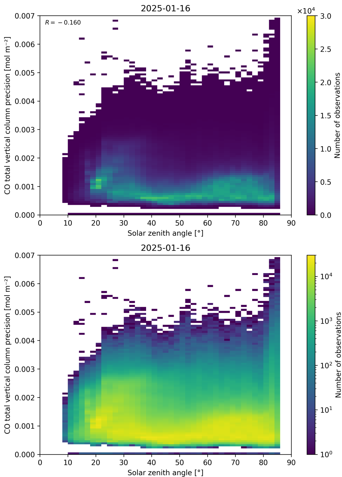
Figure 63: Scatter density plot of “Solar zenith angle” against “CO total vertical column precision” for 2025-01-15 to 2025-01-17.
