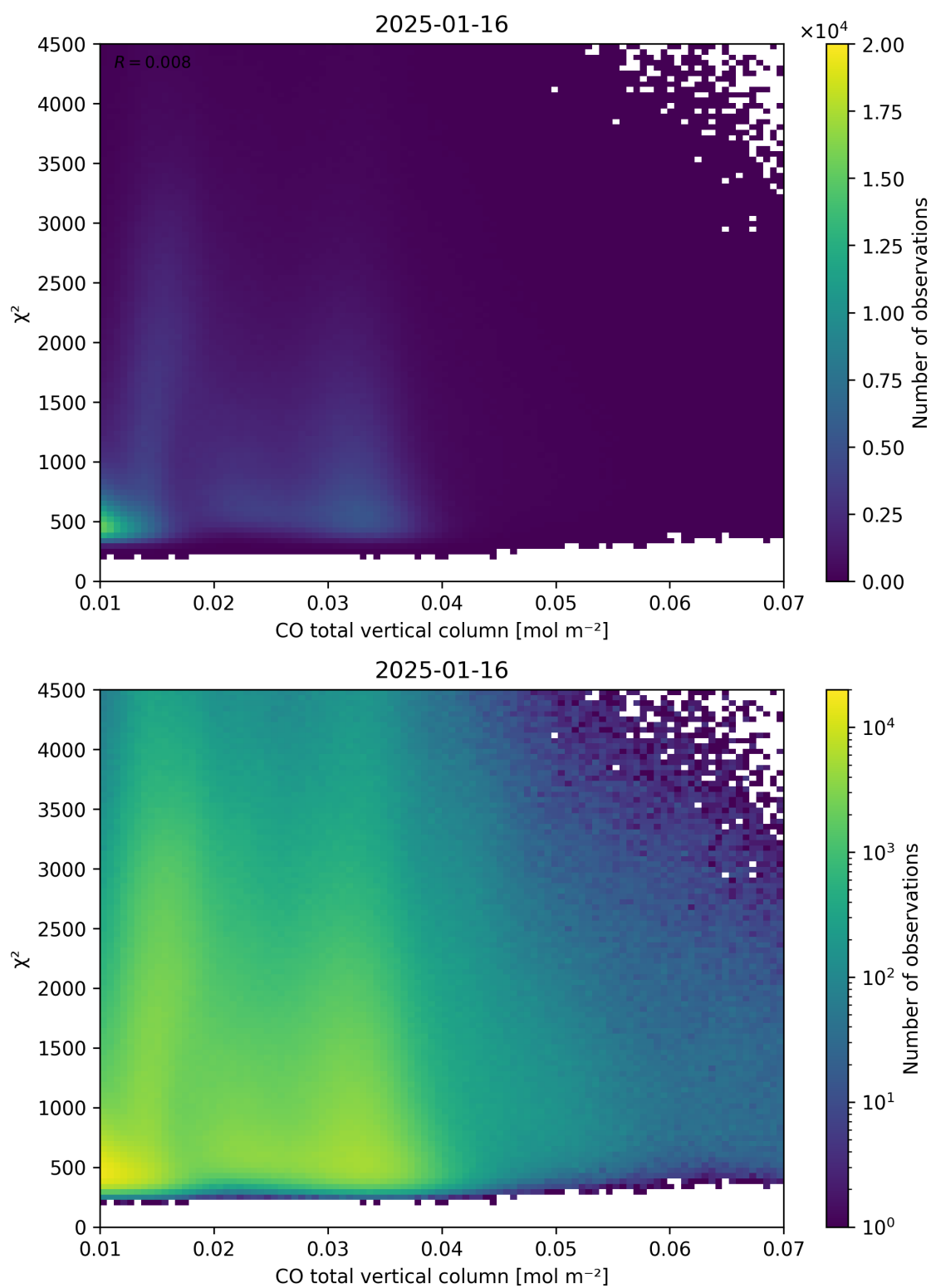
Figure 35: Scatter density plot of “CO total vertical column” against “ \chi^2 ” for 2025-01-15 to 2025-01-17.
