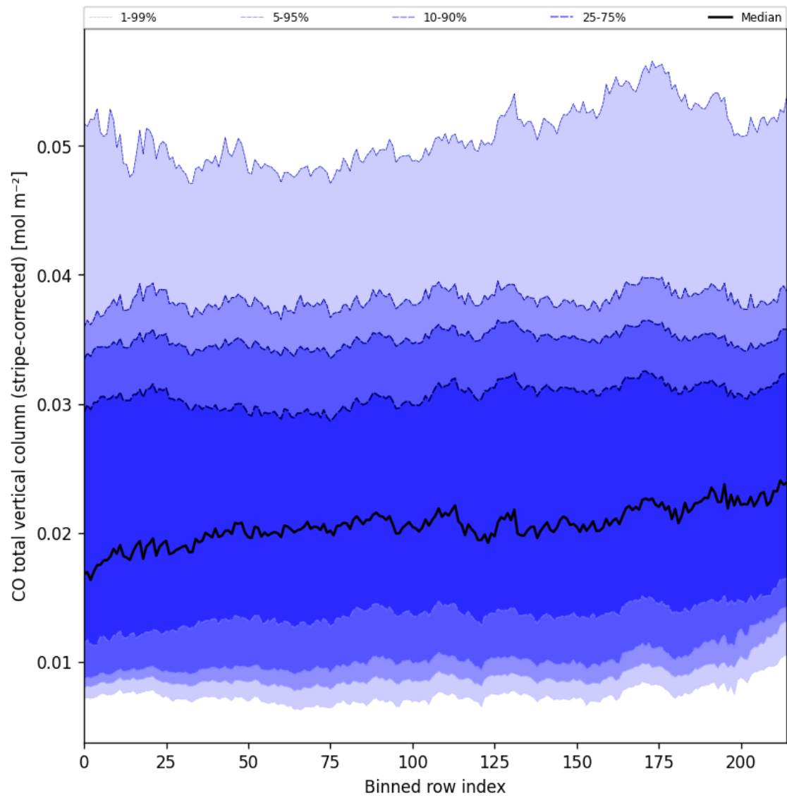
Figure 27: Along track statistics of “CO total vertical column (stripe-corrected)” for 2025-01-15 to 2025-01-17
