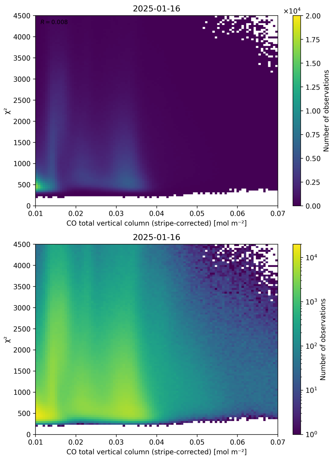
Figure 37: Scatter density plot of “CO total vertical column (stripe-corrected)” against “ \chi^2 ” for 2025-01-15 to 2025-01-17.
