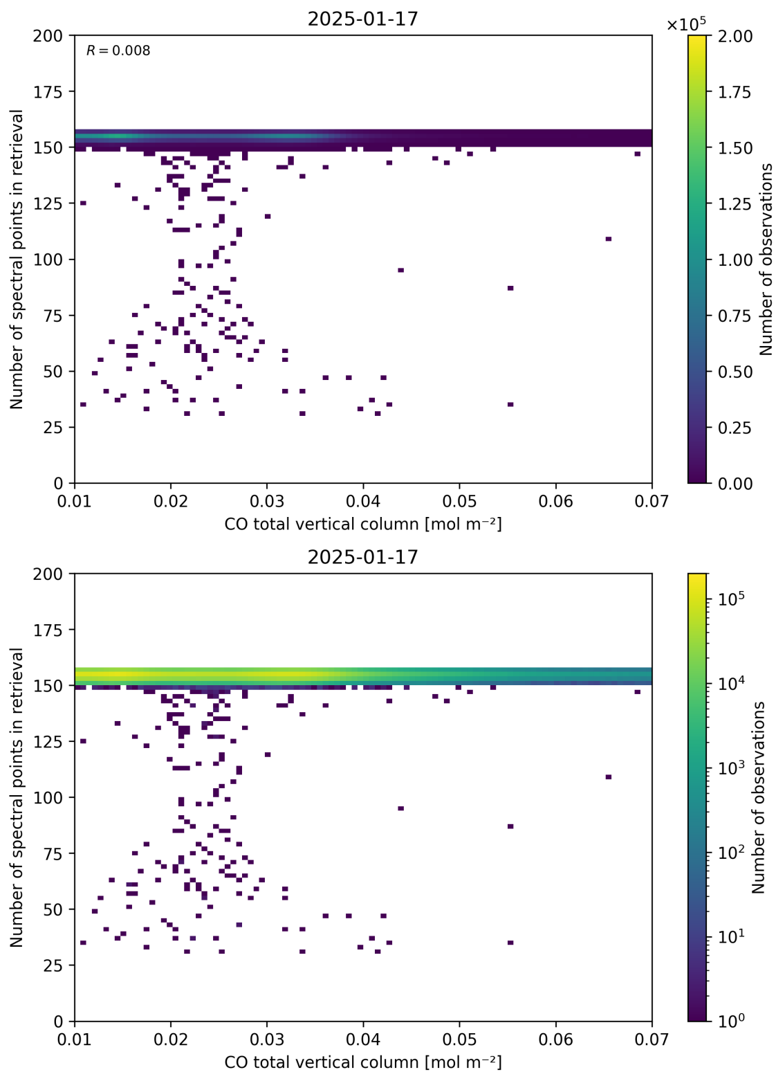
Figure 43: Scatter density plot of “CO total vertical column” against “Number of spectral points in retrieval” for 2025-01-17 to 2025-01-18.
