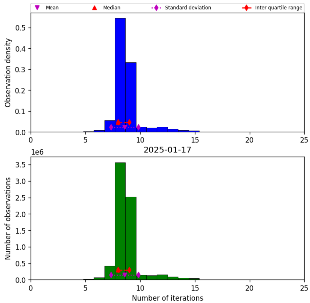
Figure 24: Histogram of “Number of iterations” for 2025-01-17 to 2025-01-18
