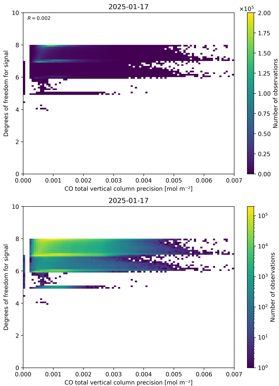
Figure 45: Scatter density plot of “CO total vertical column precision” against “Degrees of freedom for signal” for 2025-01-17 to 2025-01-18.
