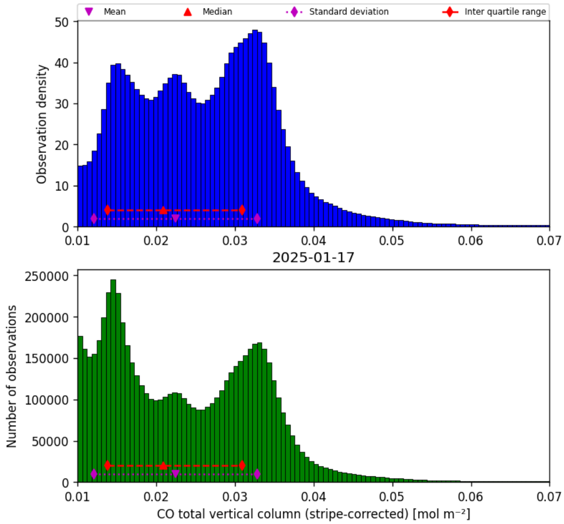
Figure 19: Histogram of “CO total vertical column (stripe-corrected)” for 2025-01-17 to 2025-01-18
