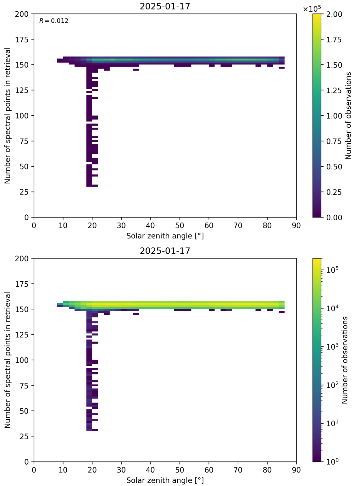
Figure 68: Scatter density plot of “Solar zenith angle” against “Number of spectral points in retrieval” for 2025-01-17 to 2025-01-18.
