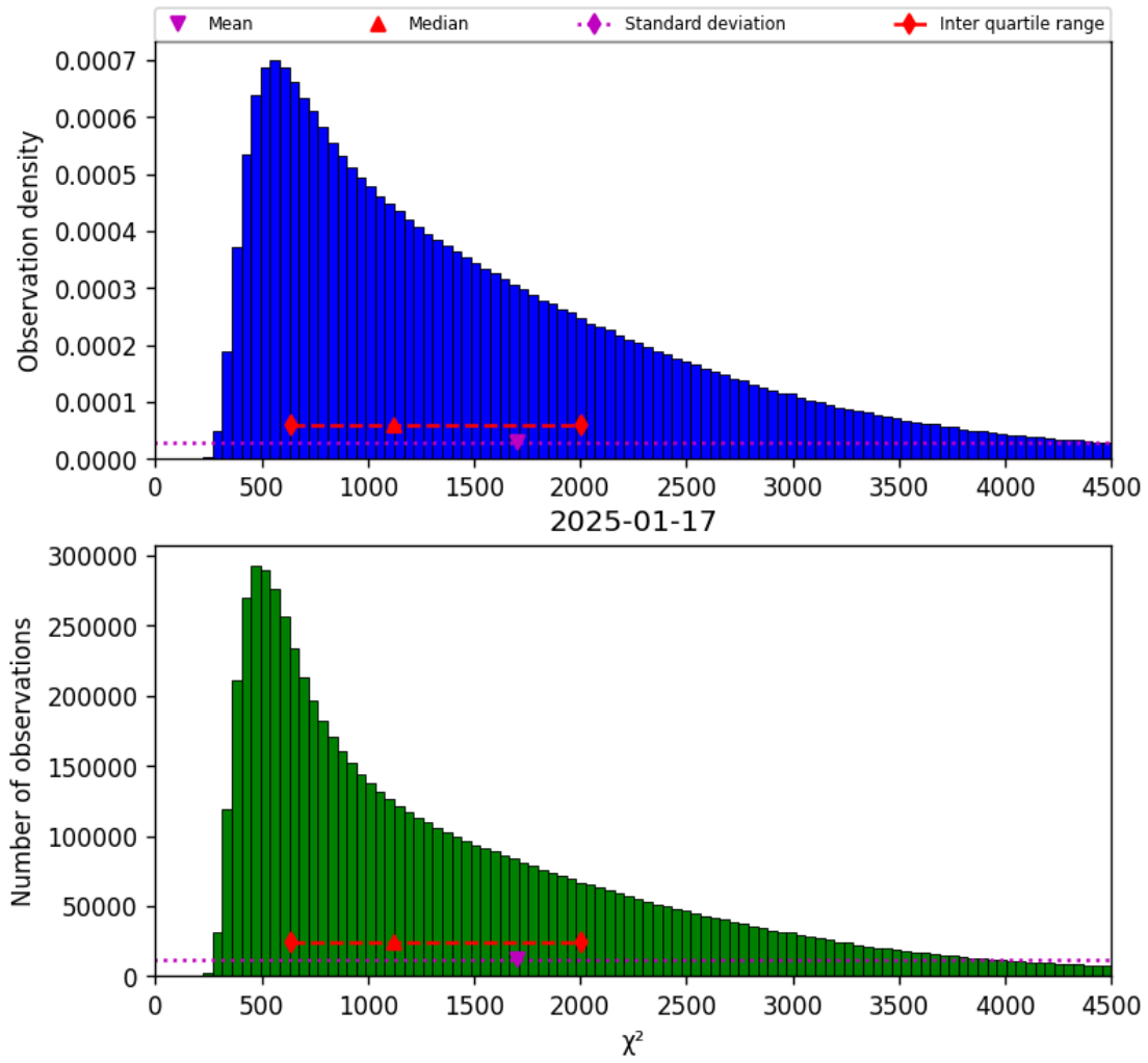
Figure 22: Histogram of “ \chi^2 ” for 2025-01-17 to 2025-01-18
