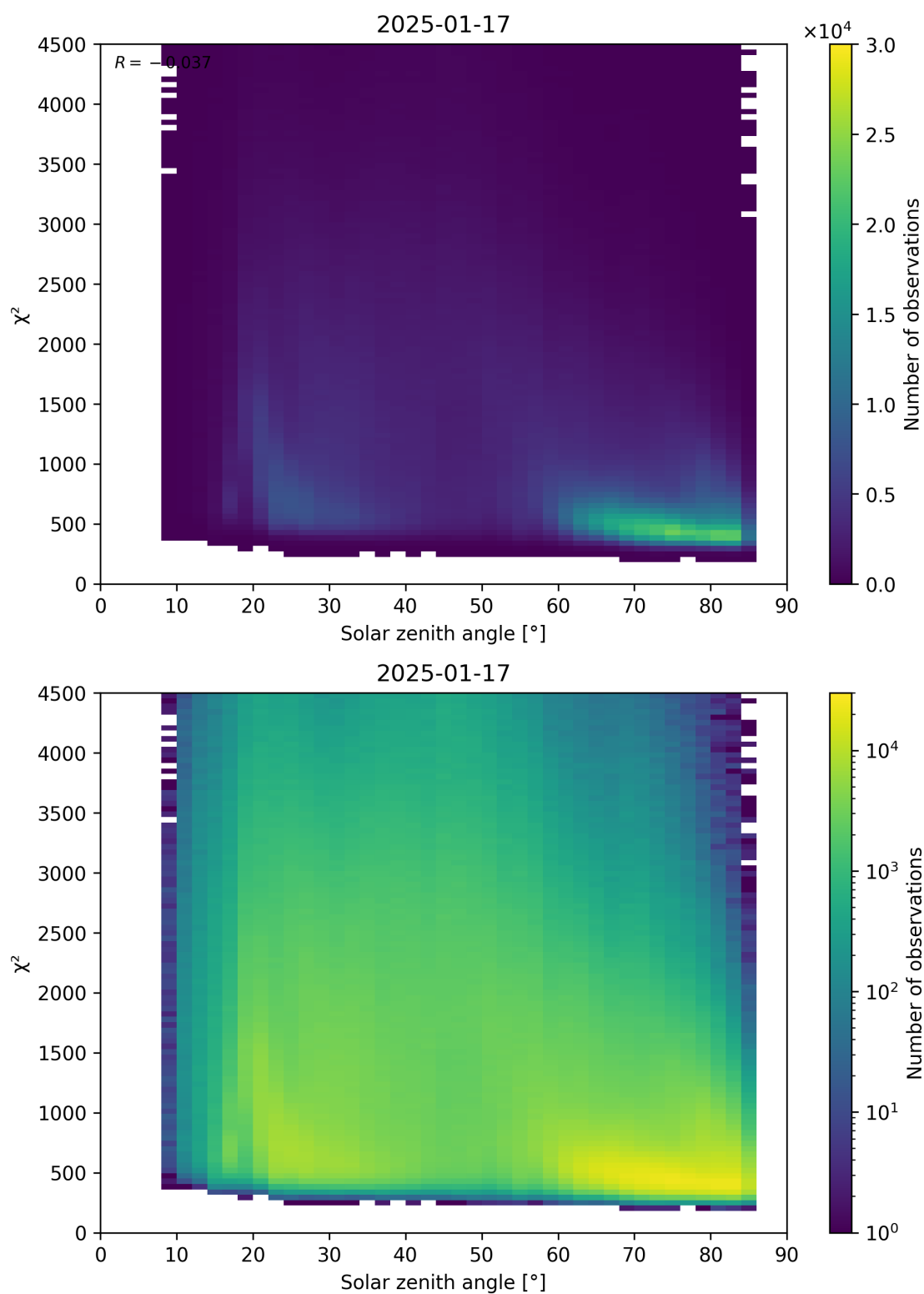
Figure 64: Scatter density plot of “Solar zenith angle” against “ \chi^2 ” for 2025-01-17 to 2025-01-18.
