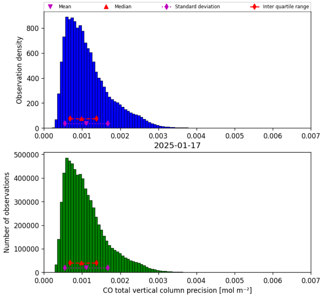
Figure 20: Histogram of “CO total vertical column precision” for 2025-01-17 to 2025-01-18
