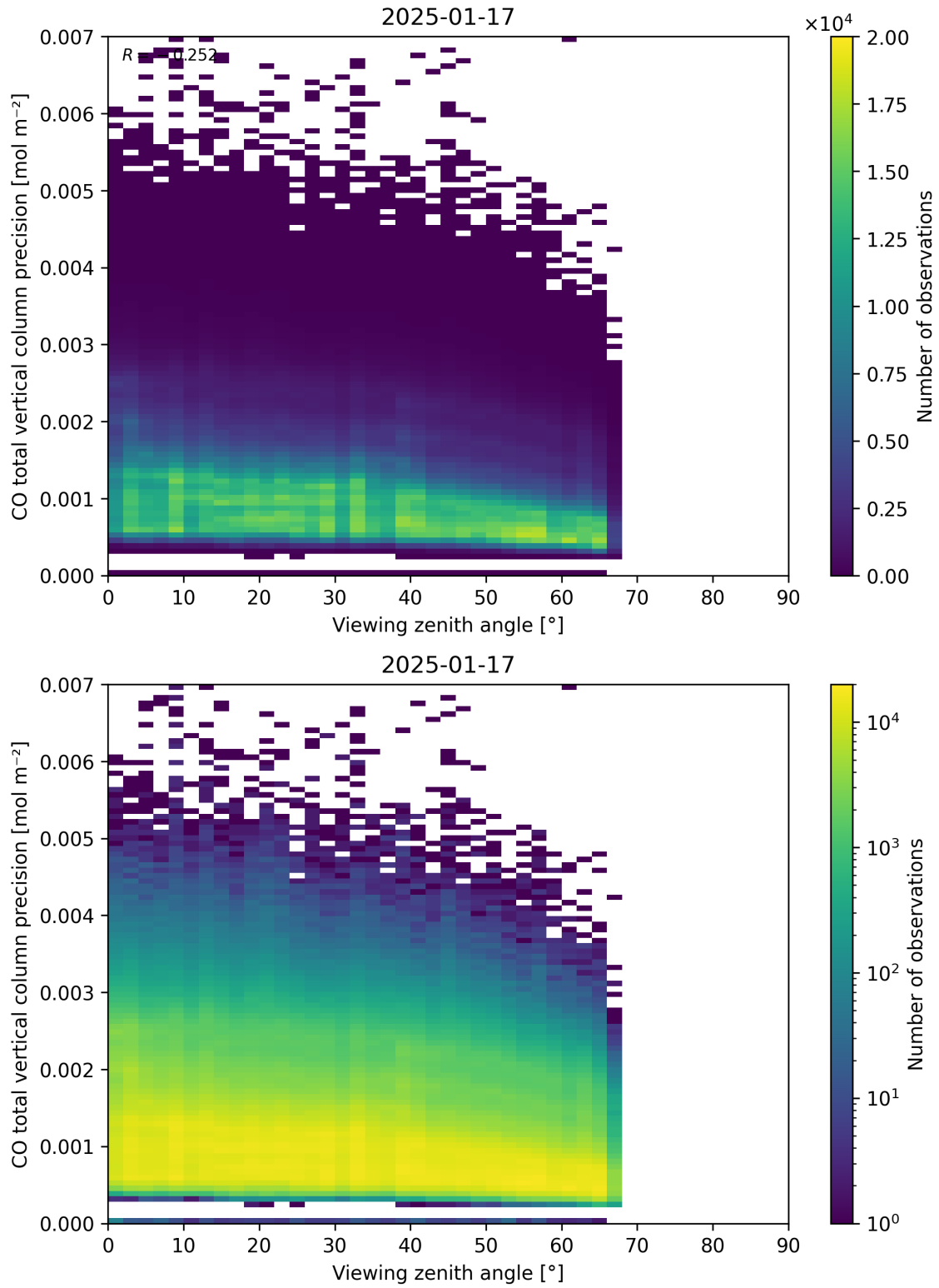
Figure 71: Scatter density plot of “Viewing zenith angle” against “CO total vertical column precision” for 2025-01-17 to 2025-01-18.
