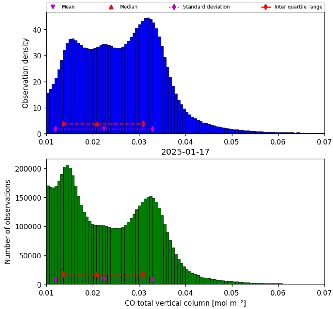
Figure 18: Histogram of “CO total vertical column” for 2025-01-17 to 2025-01-18
