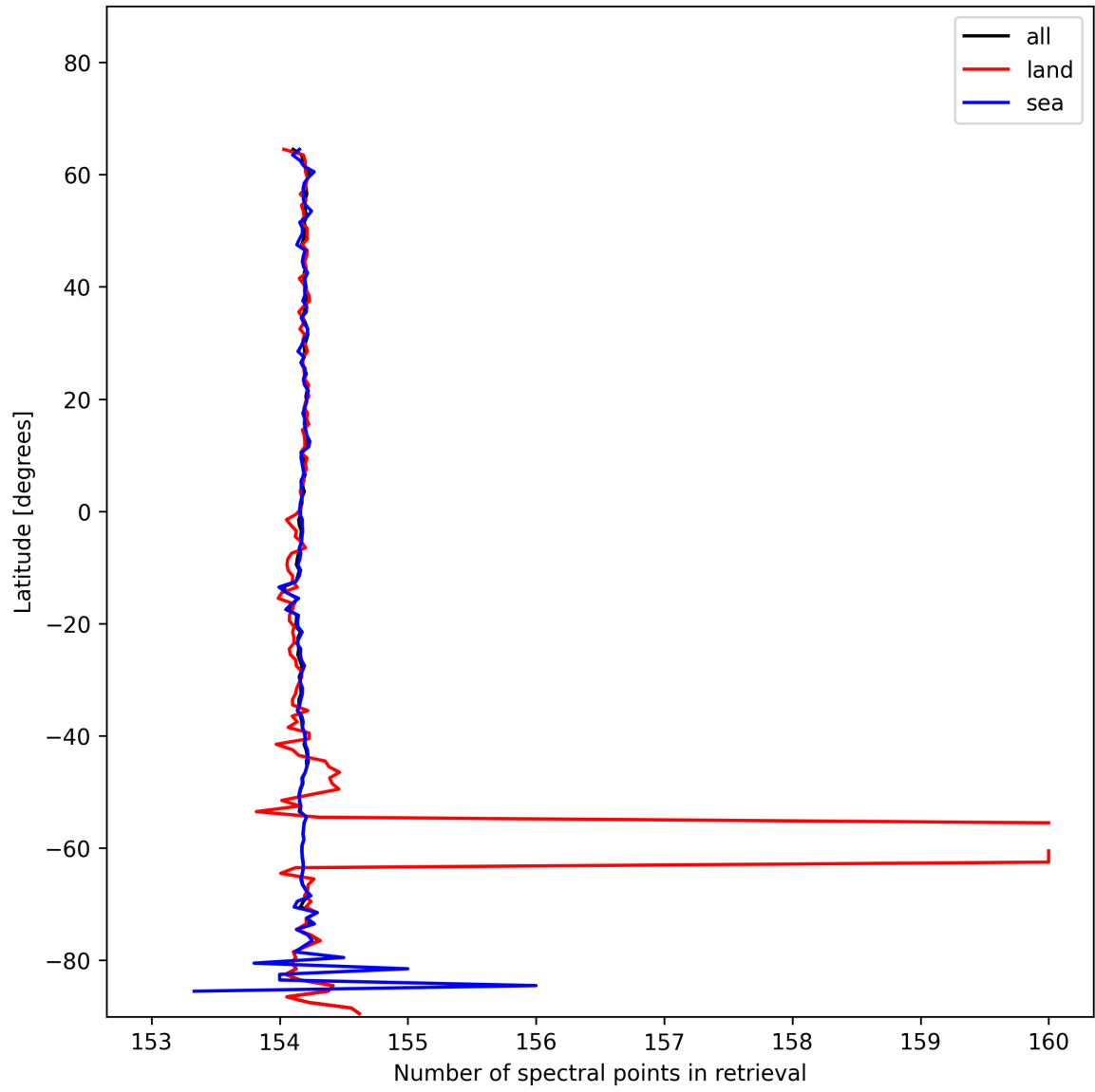
Figure 13: Zonal average of “Number of spectral points in retrieval” for 2025-01-17 to 2025-01-18.
