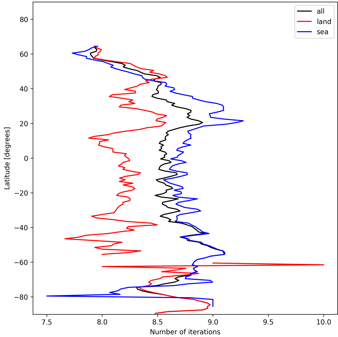
Figure 16: Zonal average of “Number of iterations” for 2025-01-17 to 2025-01-18.
