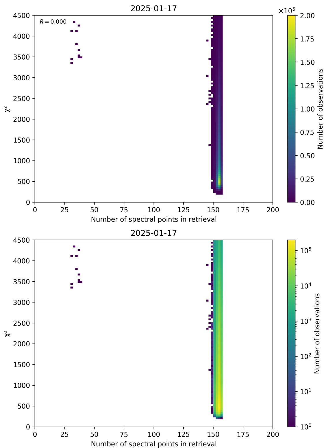
Figure 58: Scatter density plot of “Number of spectral points in retrieval” against “ \chi^2 ” for 2025-01-17 to 2025-01-18.
