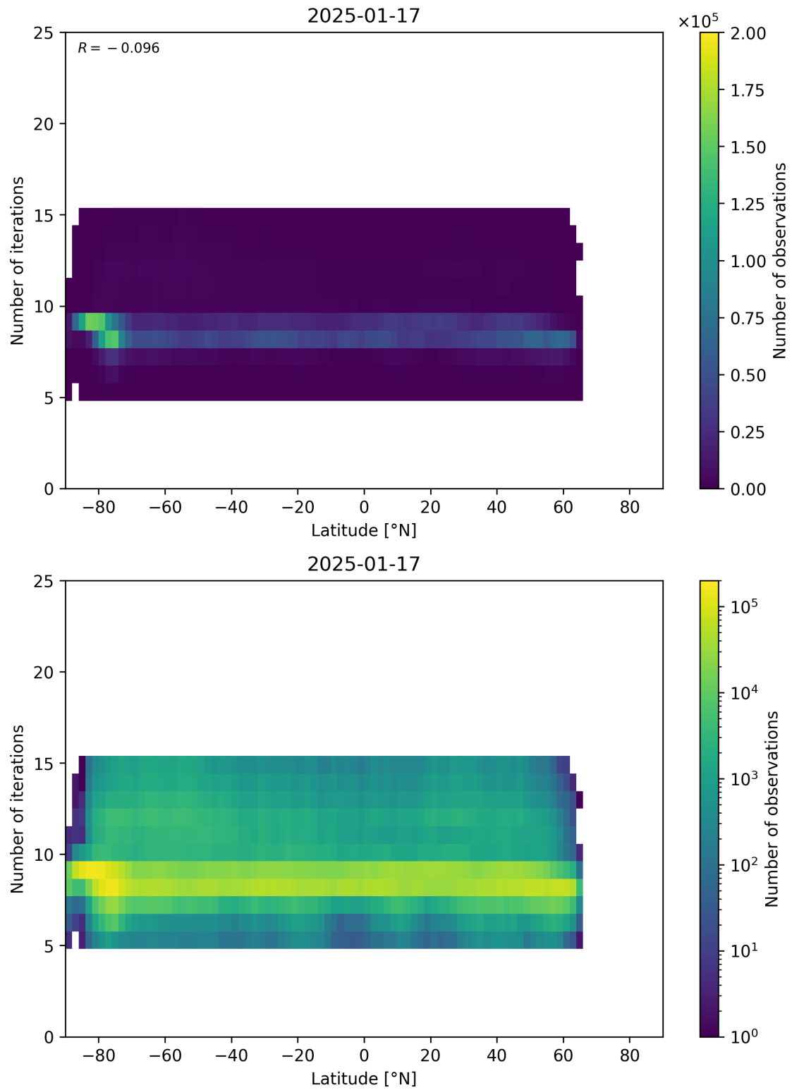
Figure 56: Scatter density plot of “Latitude” against “Number of iterations” for 2025-01-17 to 2025-01-18.
