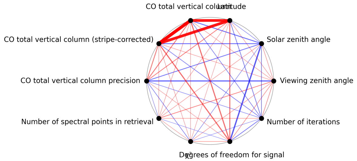
Figure 1: Map of correlation graph for 2025-01-17 to 2025-01-18.
