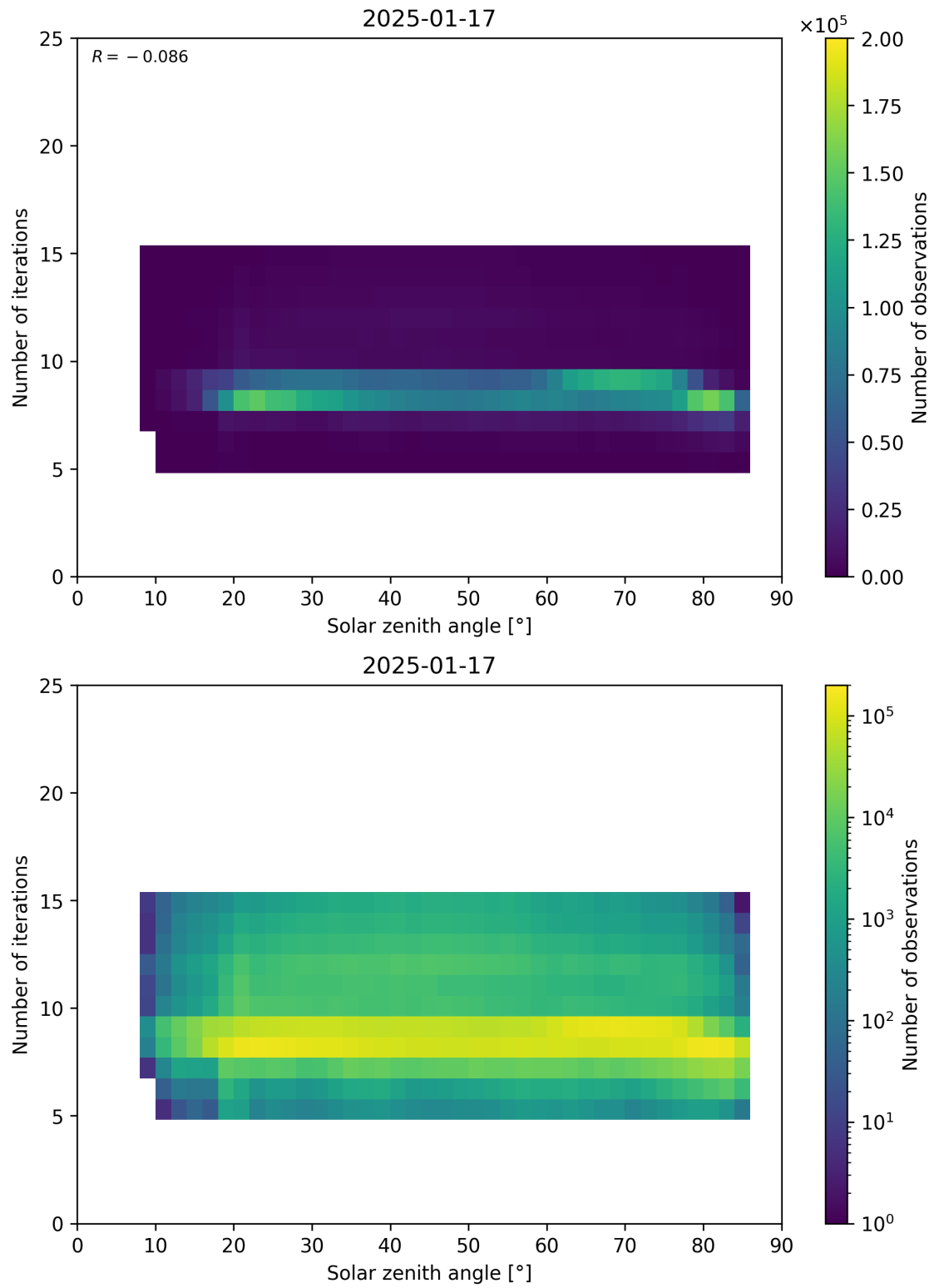
Figure 67: Scatter density plot of “Solar zenith angle” against “Number of iterations” for 2025-01-17 to 2025-01-18.
