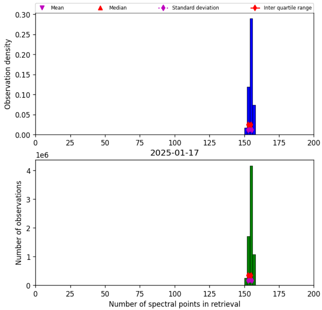
Figure 21: Histogram of “Number of spectral points in retrieval” for 2025-01-17 to 2025-01-18
