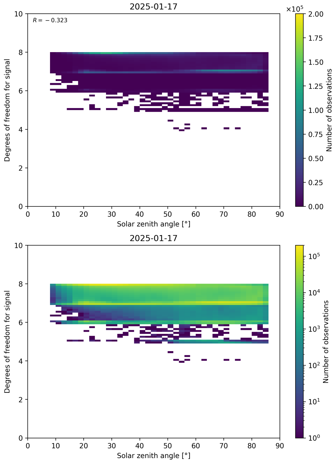
Figure 65: Scatter density plot of “Solar zenith angle” against “Degrees of freedom for signal” for 2025-01-17 to 2025-01-18.
