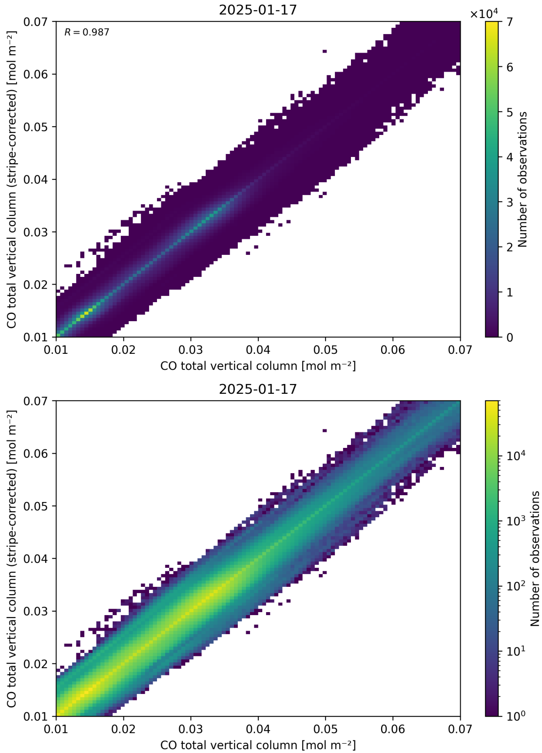
Figure 33: Scatter density plot of “CO total vertical column” against “CO total vertical column (stripe-corrected)” for 2025-01-17 to 2025-01-18.
