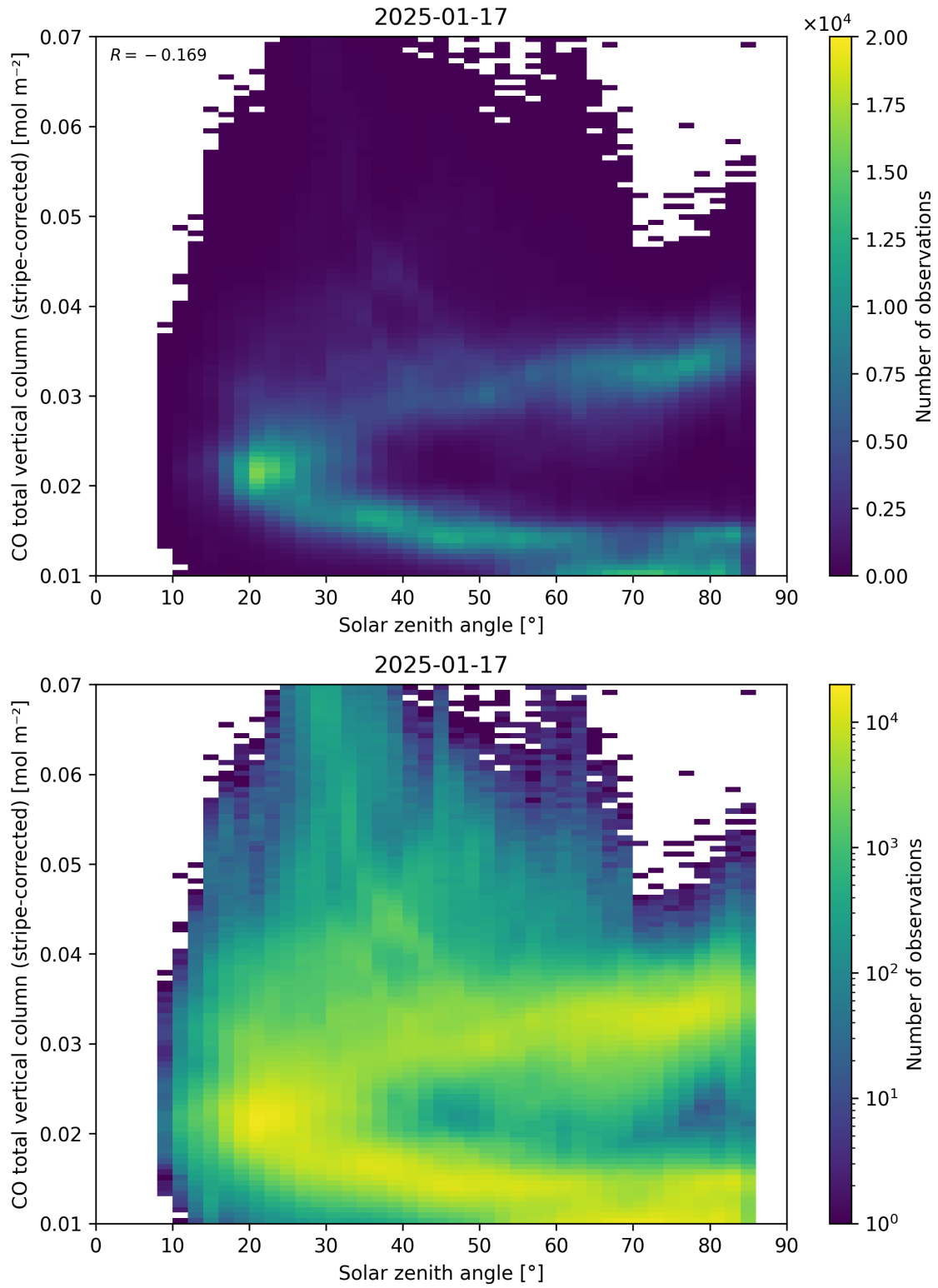
Figure 62: Scatter density plot of “Solar zenith angle” against “CO total vertical column (stripe-corrected)” for 2025-01-17 to 2025-01-18.
