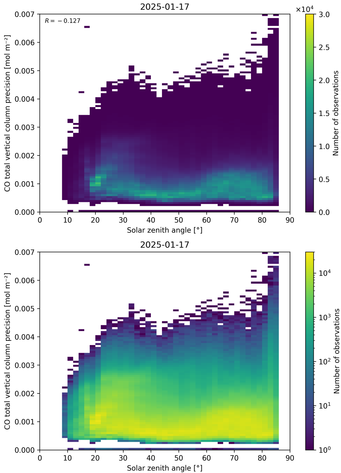
Figure 63: Scatter density plot of “Solar zenith angle” against “CO total vertical column precision” for 2025-01-17 to 2025-01-18.
