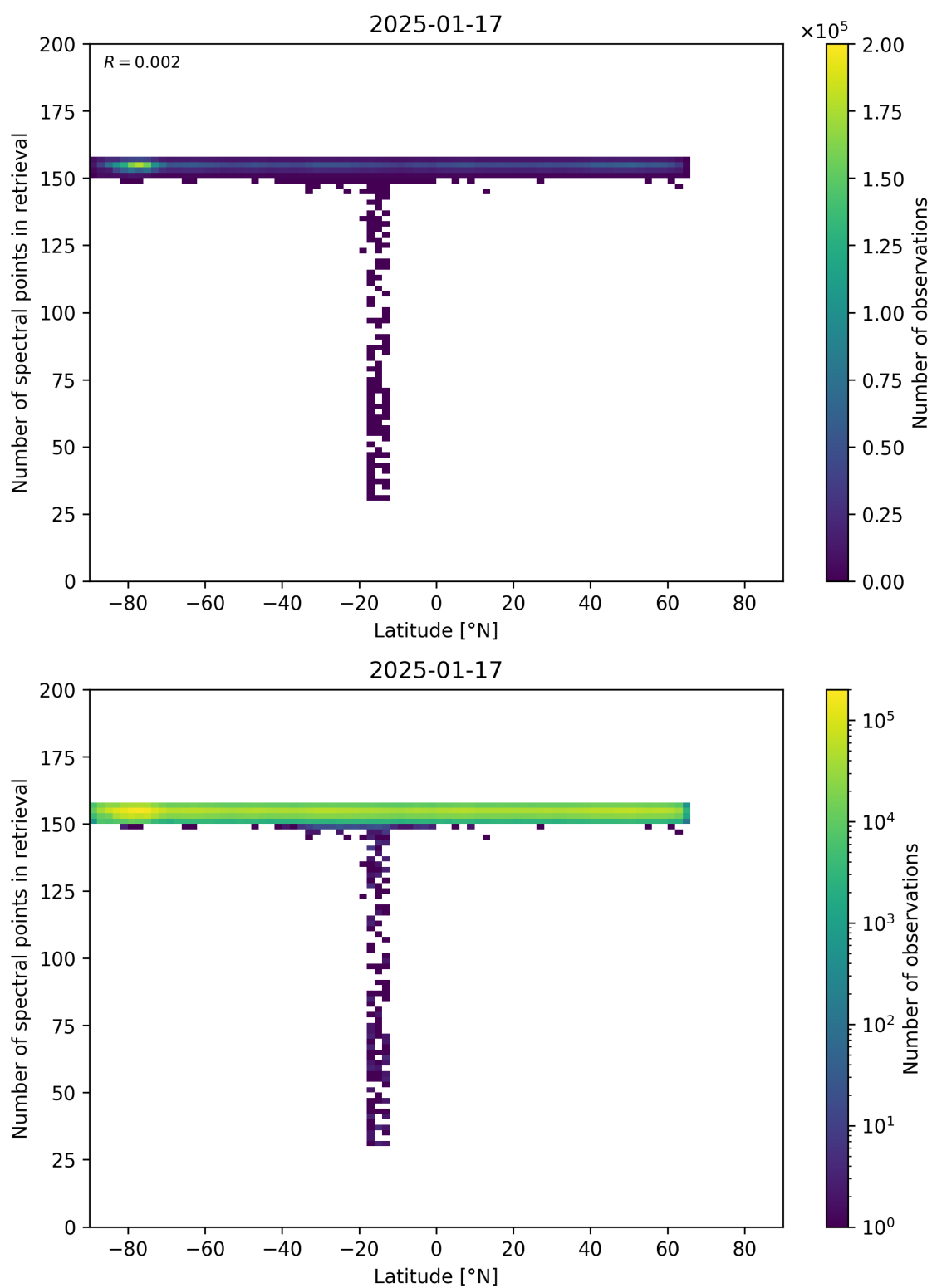
Figure 57: Scatter density plot of “Latitude” against “Number of spectral points in retrieval” for 2025-01-17 to 2025-01-18.
