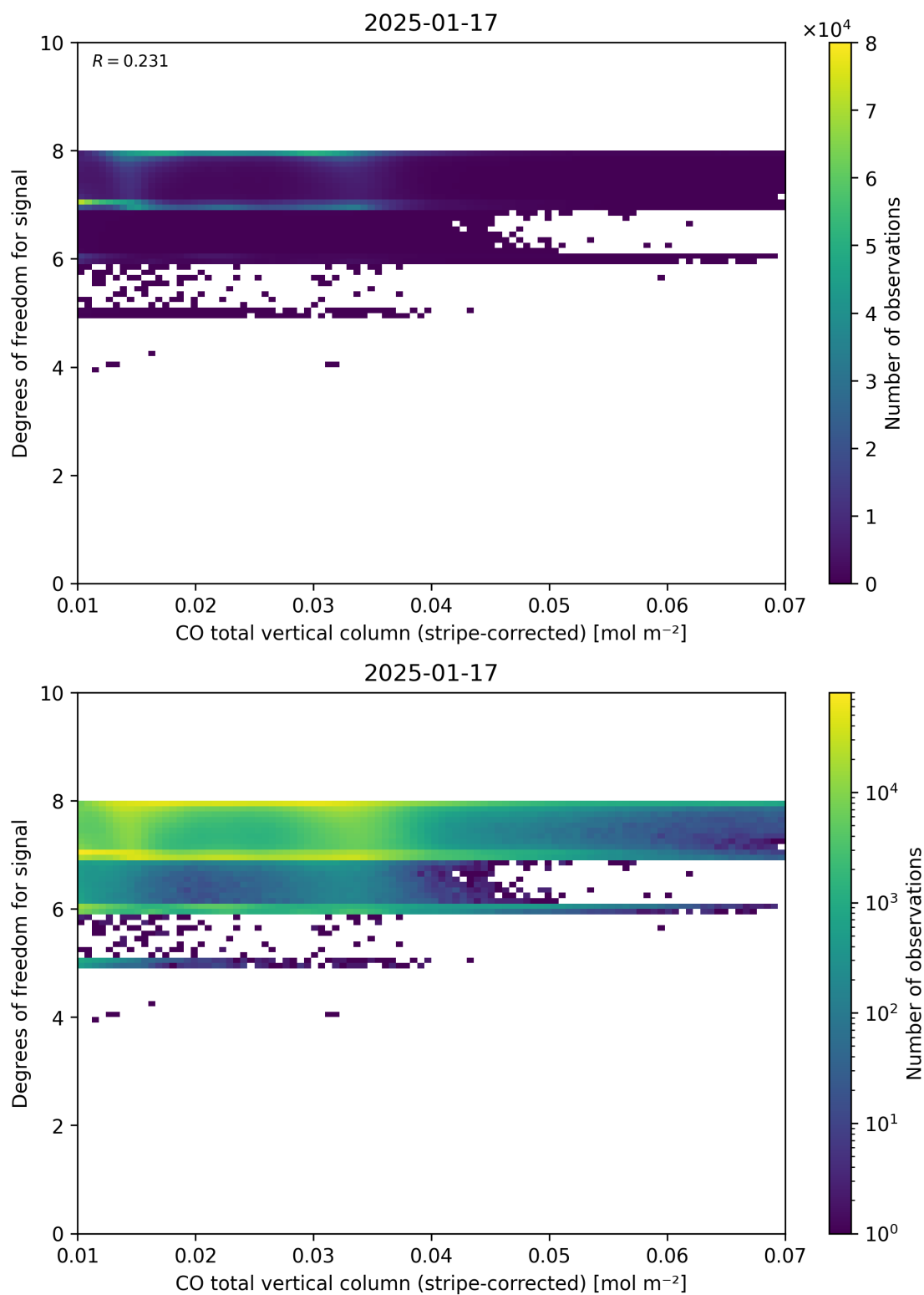
Figure 38: Scatter density plot of “CO total vertical column (stripe-corrected)” against “Degrees of freedom for signal” for 2025-01-17 to 2025-01-18.
