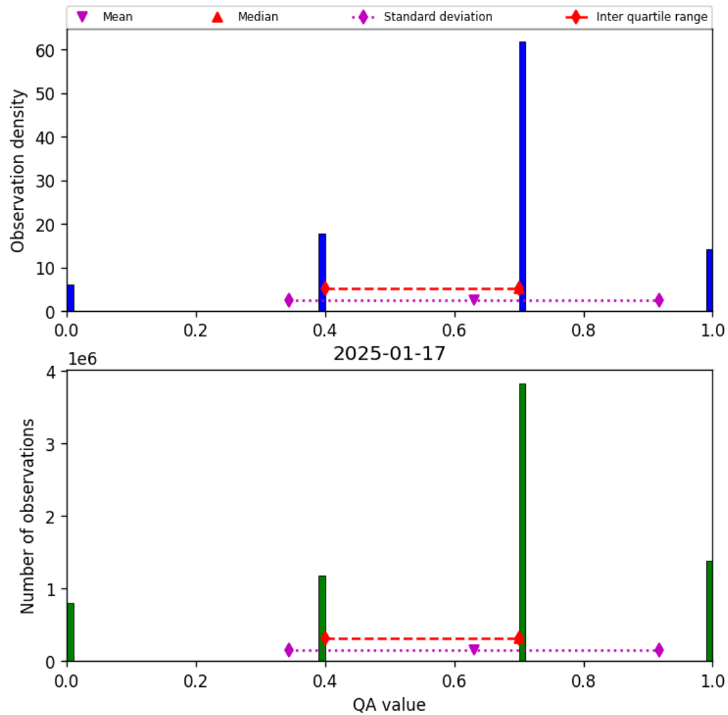
Figure 17: Histogram of “QA value” for 2025-01-17 to 2025-01-18
