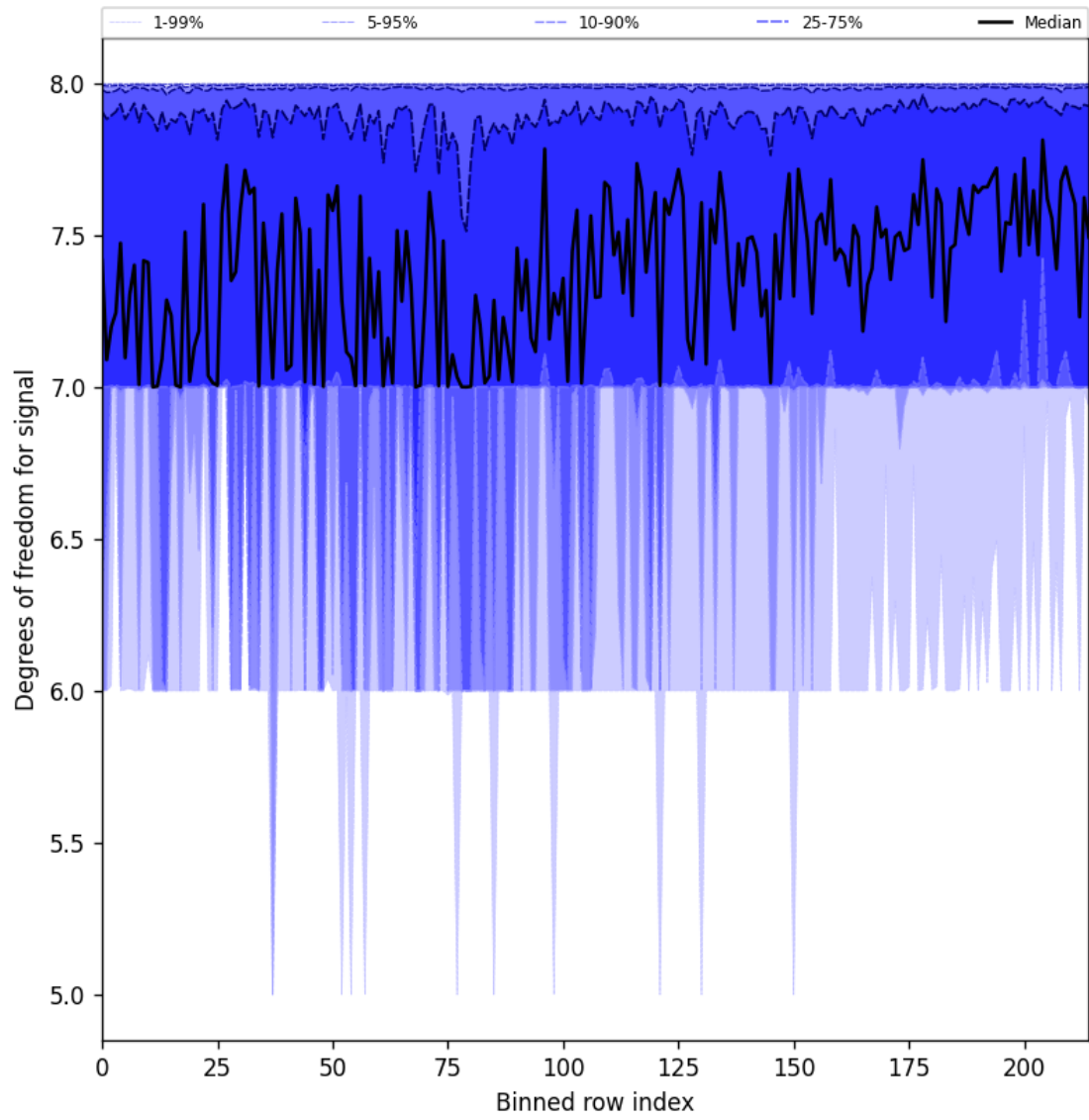
Figure 31: Along track statistics of “Degrees of freedom for signal” for 2025-01-17 to 2025-01-18
