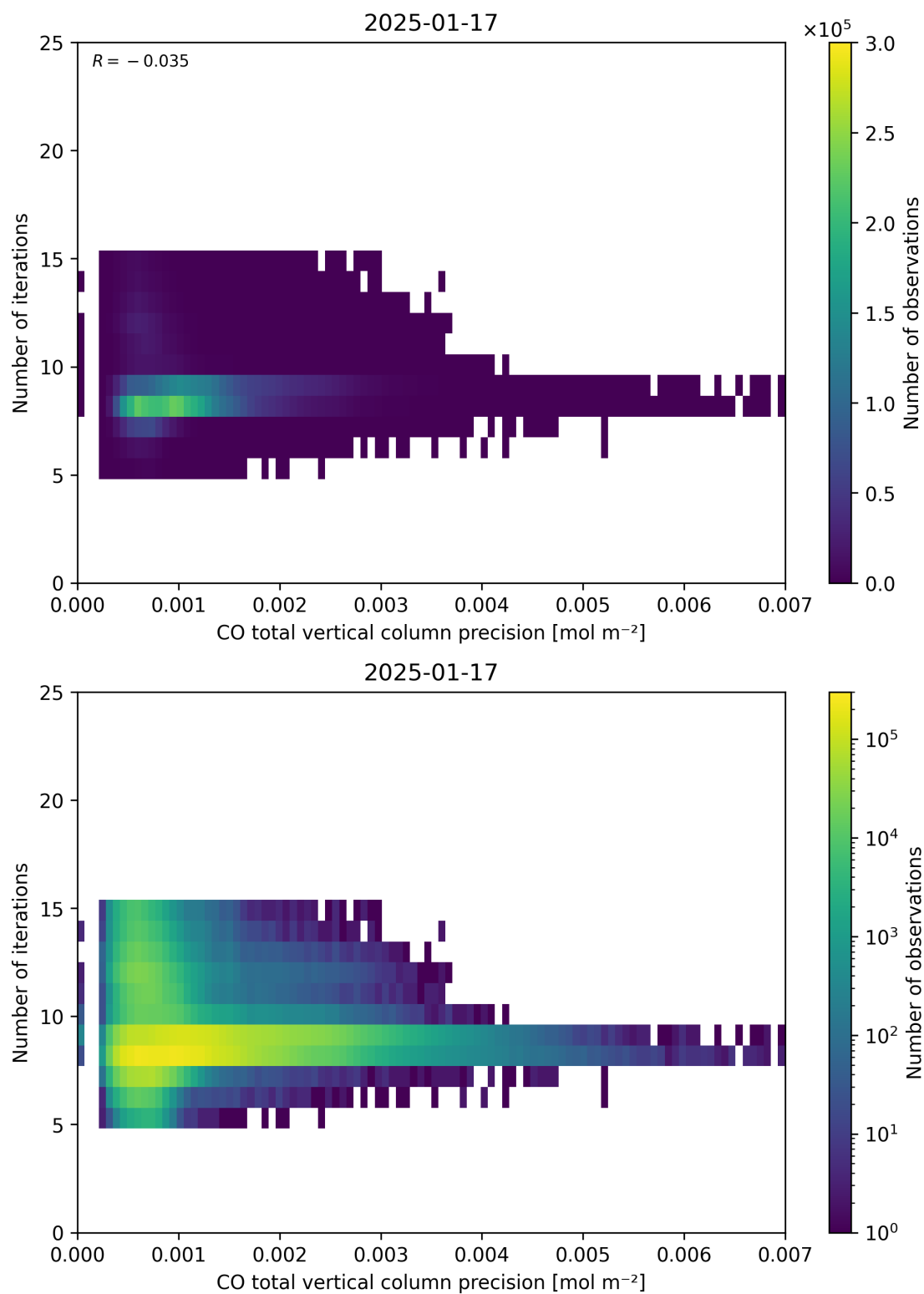
Figure 46: Scatter density plot of “CO total vertical column precision” against “Number of iterations” for 2025-01-17 to 2025-01-18.
