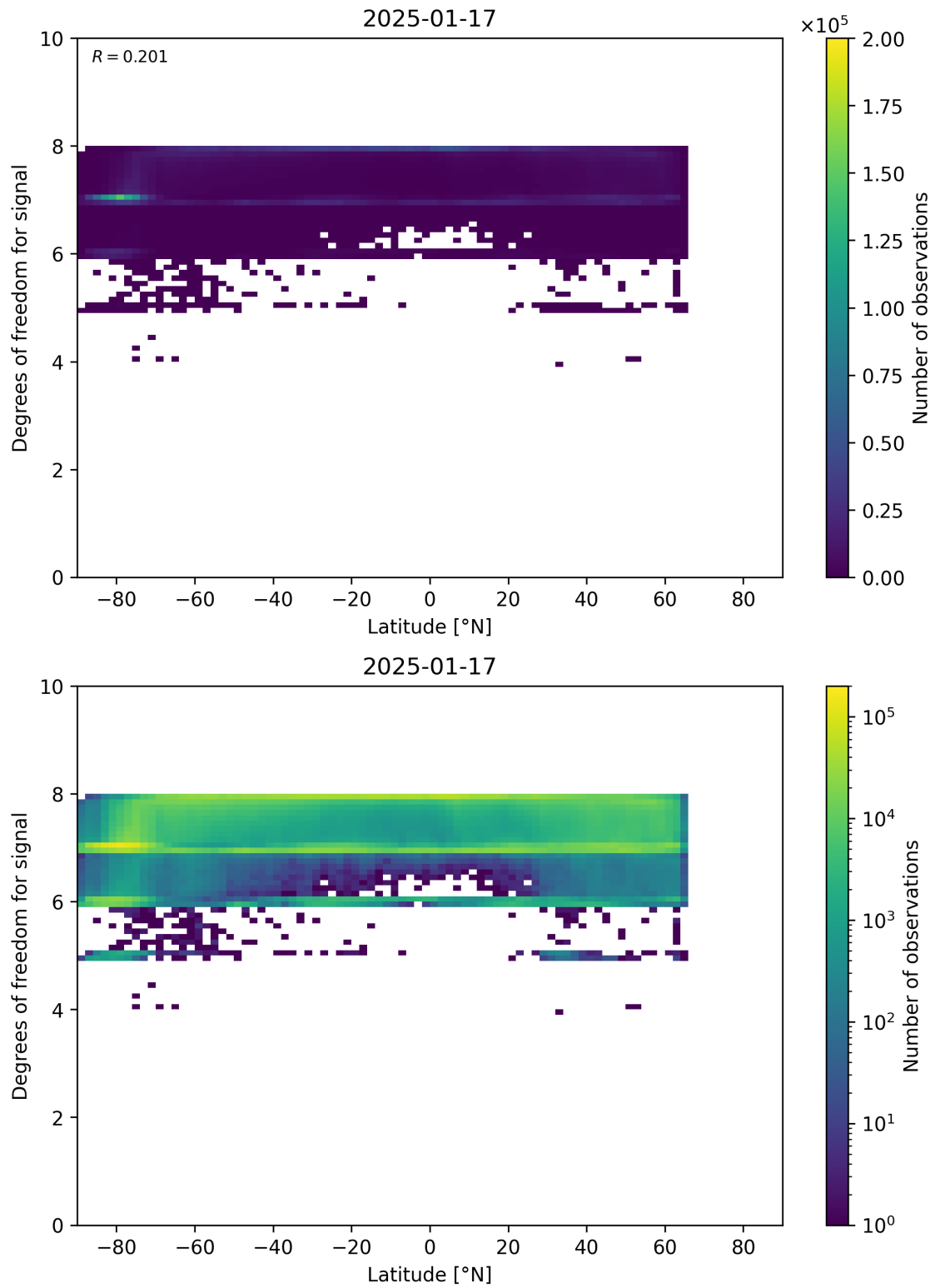
Figure 55: Scatter density plot of “Latitude” against “Degrees of freedom for signal” for 2025-01-17 to 2025-01-18.
