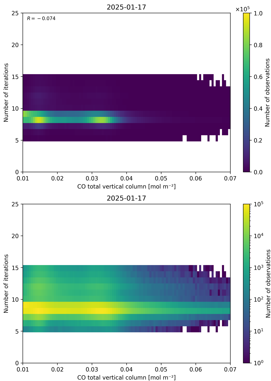
Figure 42: Scatter density plot of “CO total vertical column” against “Number of iterations” for 2025-01-17 to 2025-01-18.
