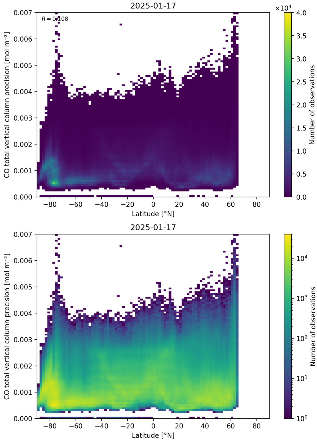
Figure 53: Scatter density plot of “Latitude” against “CO total vertical column precision” for 2025-01-17 to 2025-01-18.
