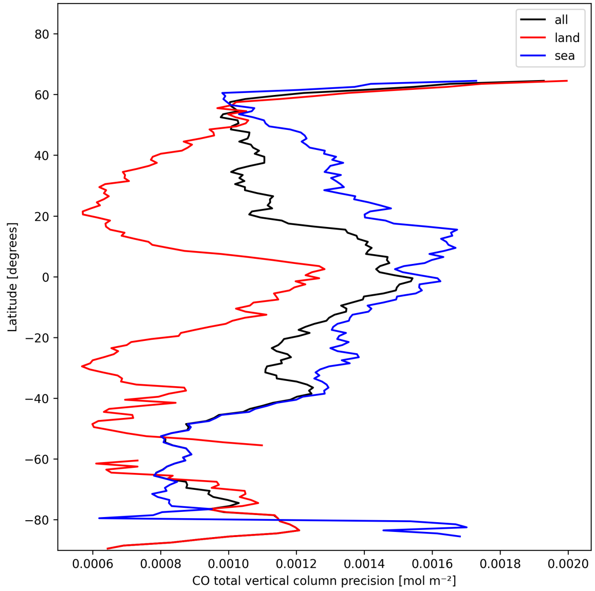
Figure 12: Zonal average of “CO total vertical column precision” for 2025-01-17 to 2025-01-18.
