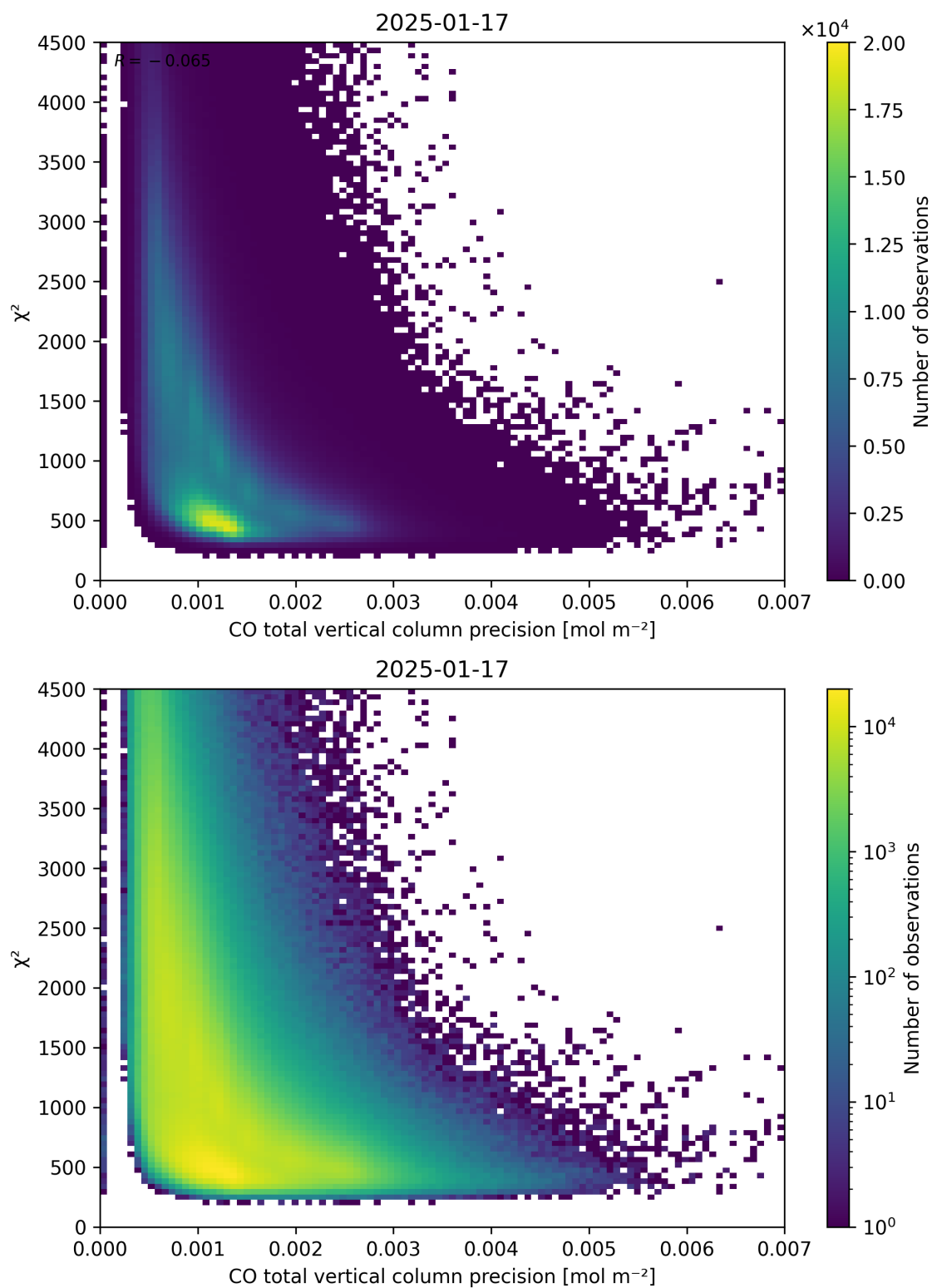
Figure 44: Scatter density plot of “CO total vertical column precision” against “ \chi^2 ” for 2025-01-17 to 2025-01-18.
