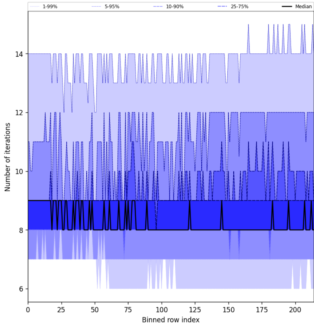
Figure 32: Along track statistics of “Number of iterations” for 2025-01-17 to 2025-01-18
