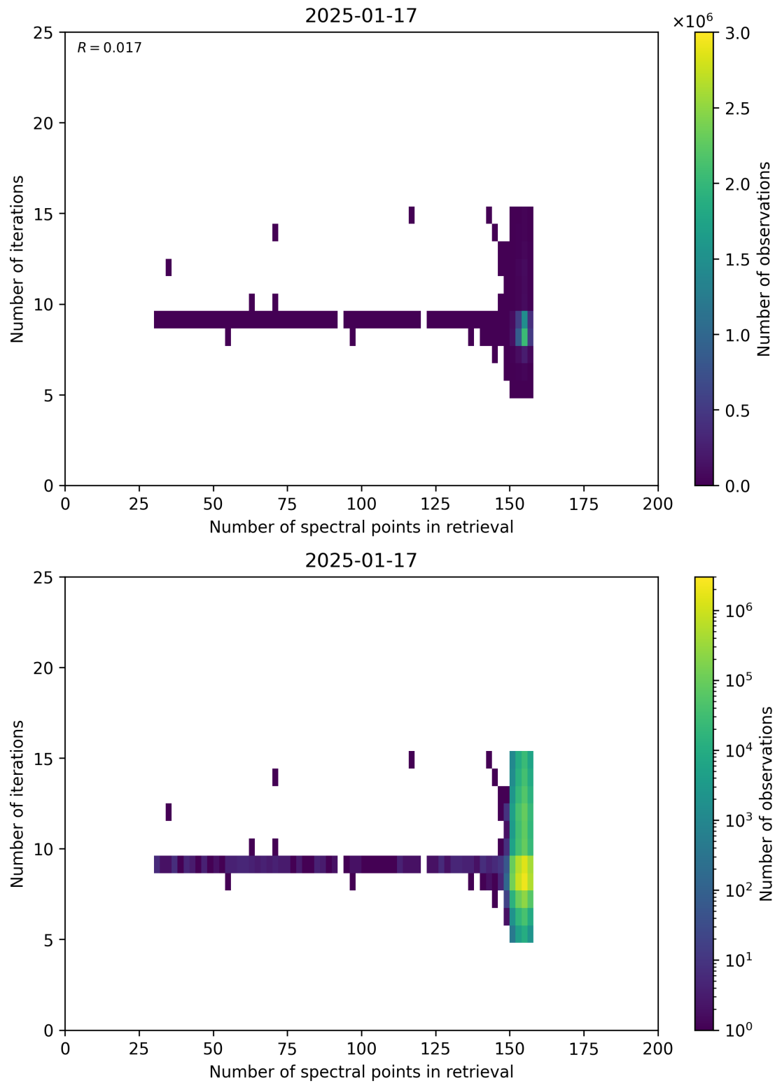
Figure 60: Scatter density plot of “Number of spectral points in retrieval” against “Number of iterations” for 2025-01-17 to 2025-01-18.
