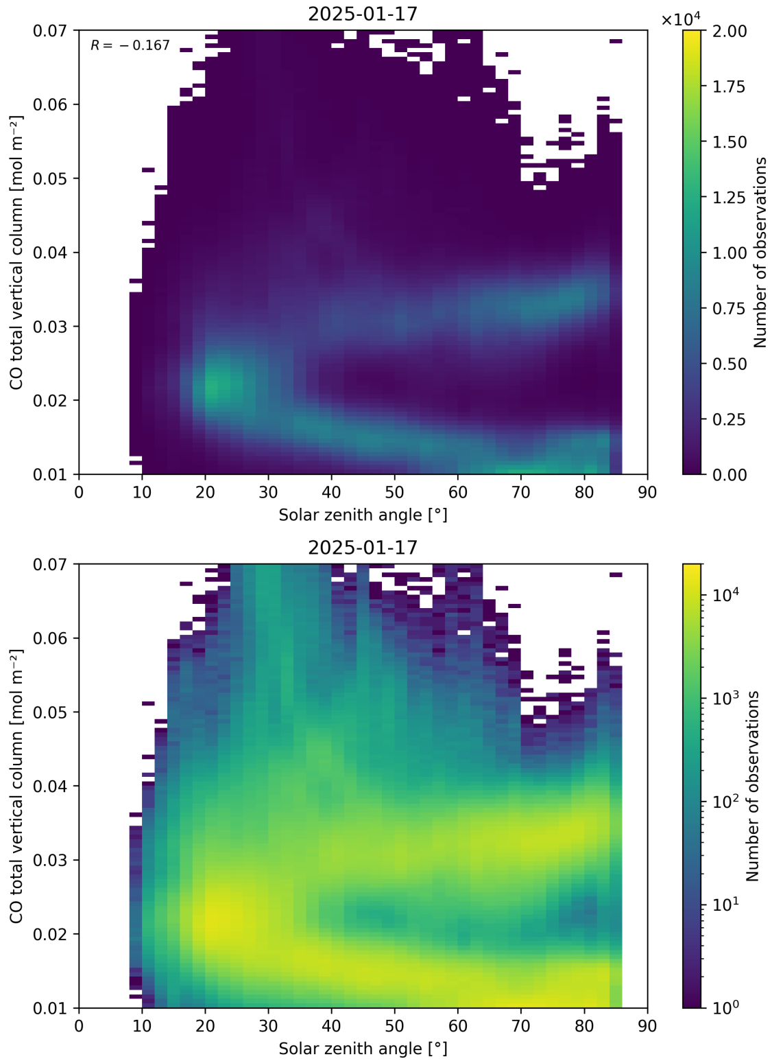
Figure 61: Scatter density plot of “Solar zenith angle” against “CO total vertical column” for 2025-01-17 to 2025-01-18.
