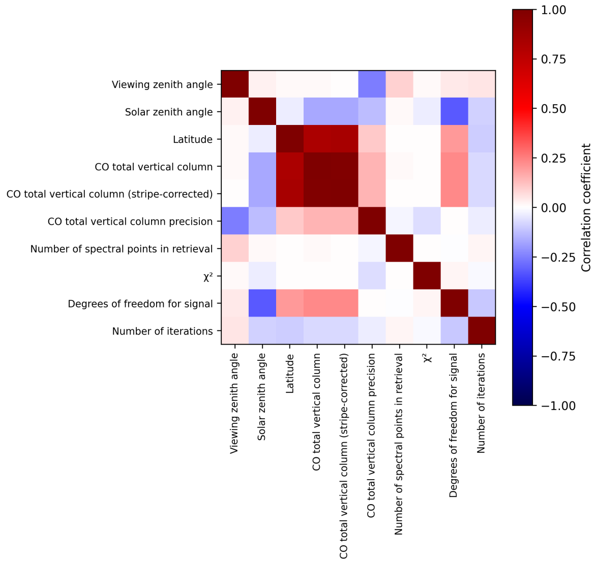
Figure 2: Map of correlation matrix for 2025-01-17 to 2025-01-18.
