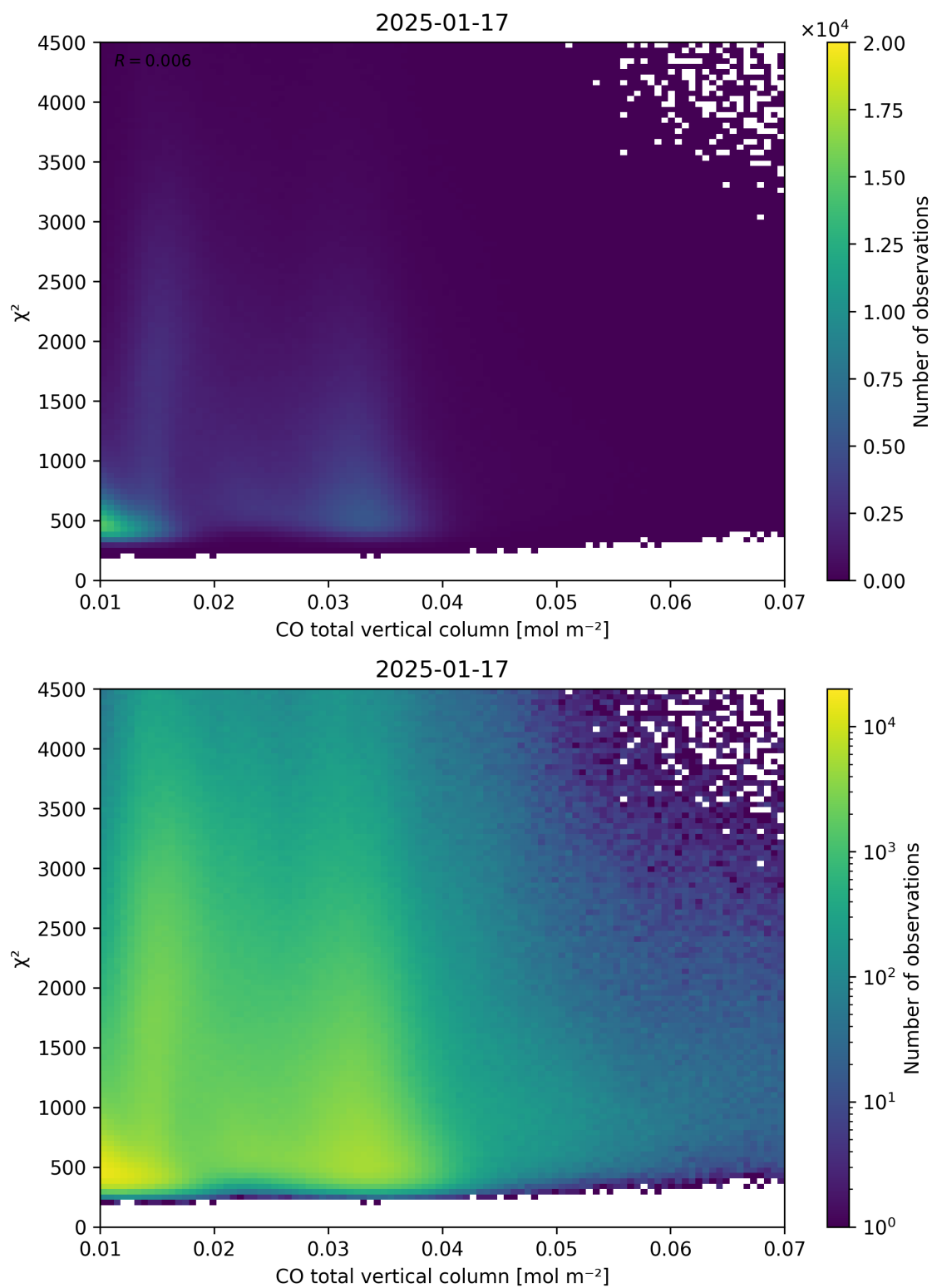
Figure 35: Scatter density plot of “CO total vertical column” against “ \chi^2 ” for 2025-01-17 to 2025-01-18.
