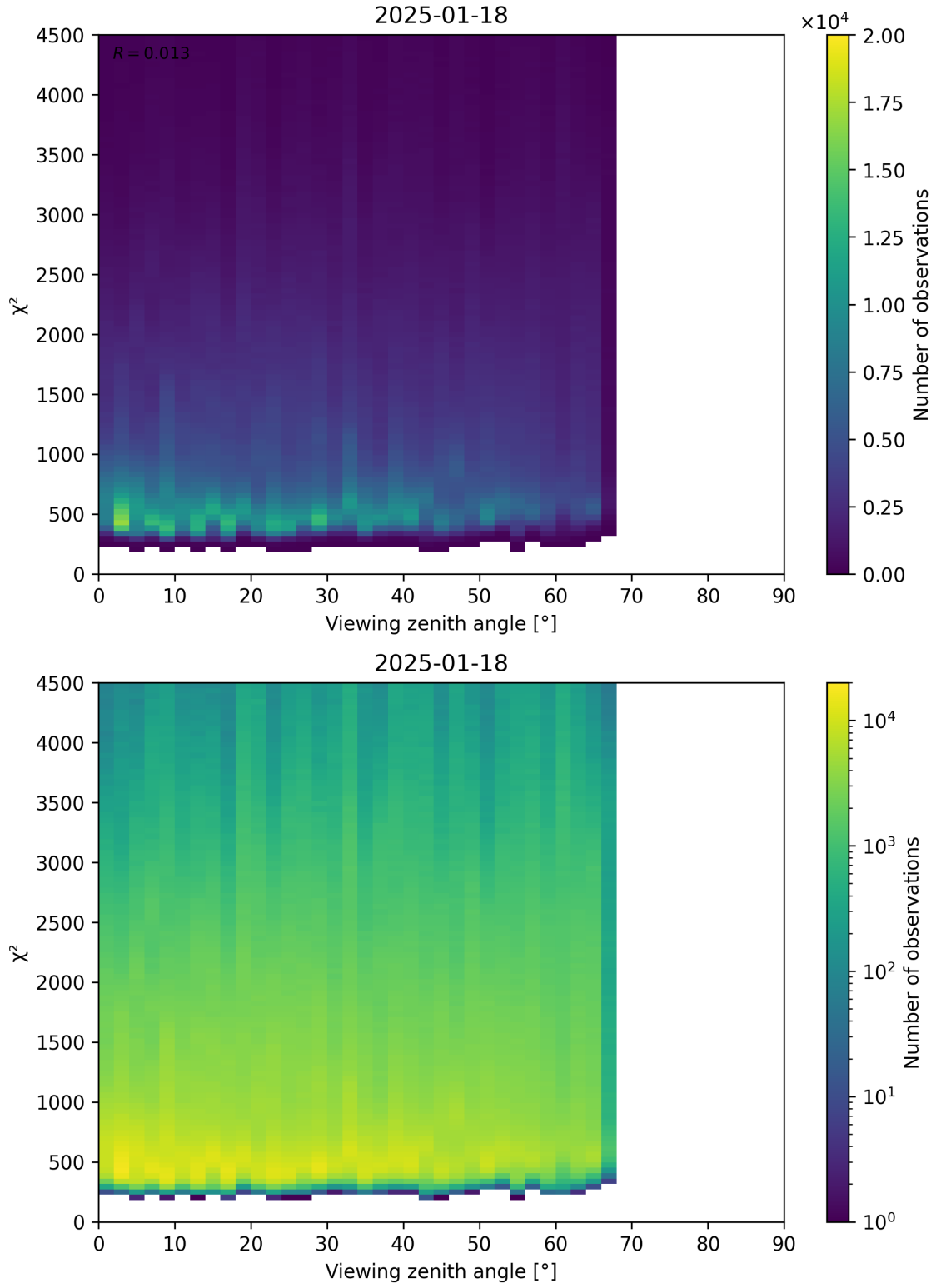
Figure 72: Scatter density plot of “Viewing zenith angle” against “ \chi^2 ” for 2025-01-17 to 2025-01-19.
