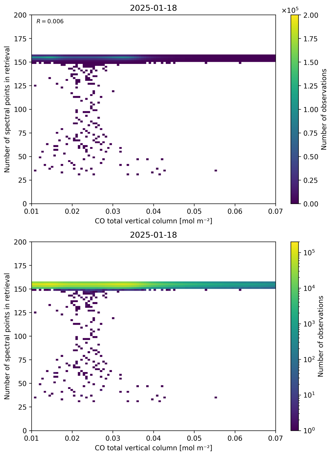
Figure 43: Scatter density plot of “CO total vertical column” against “Number of spectral points in retrieval” for 2025-01-17 to 2025-01-19.
