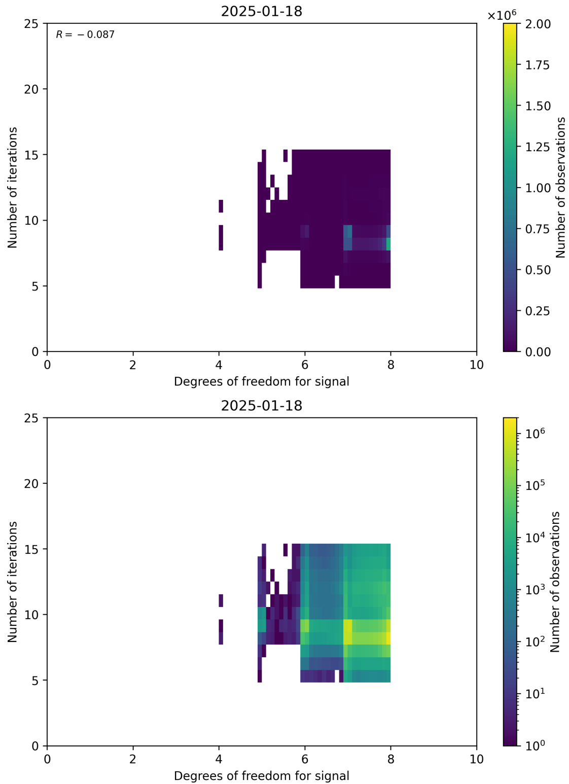
Figure 50: Scatter density plot of “Degrees of freedom for signal” against “Number of iterations” for 2025-01-17 to 2025-01-19.
