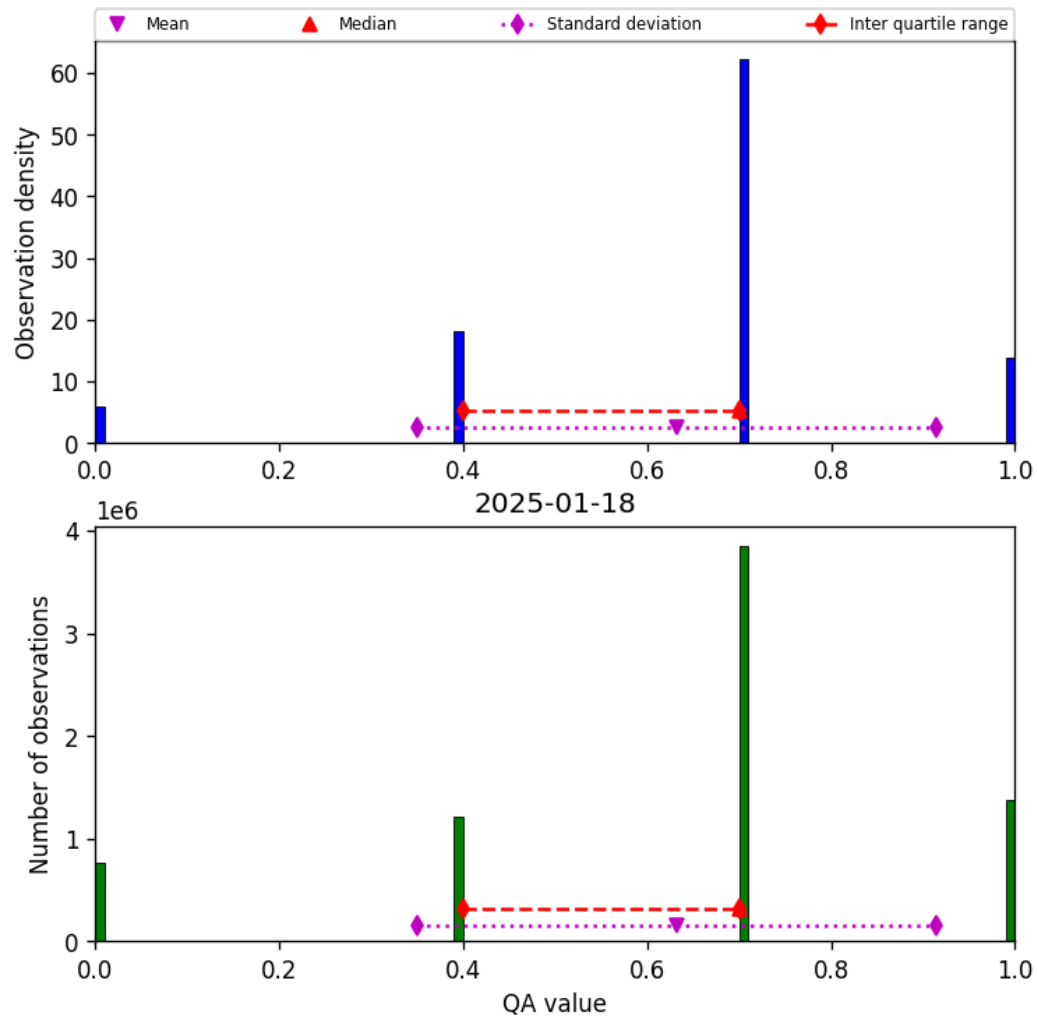
Figure 17: Histogram of “QA value” for 2025-01-17 to 2025-01-19
