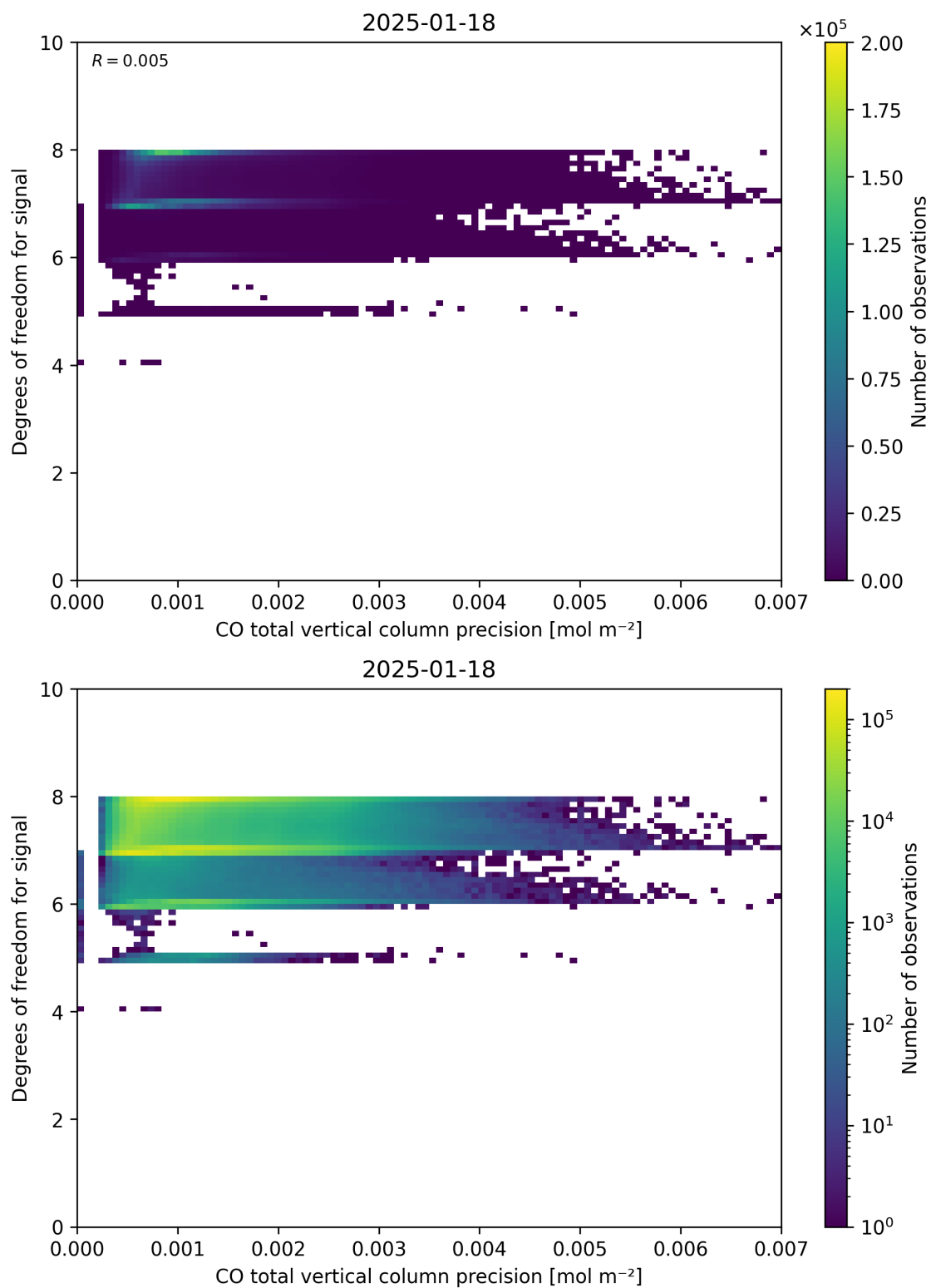
Figure 45: Scatter density plot of “CO total vertical column precision” against “Degrees of freedom for signal” for 2025-01-17 to 2025-01-19.
