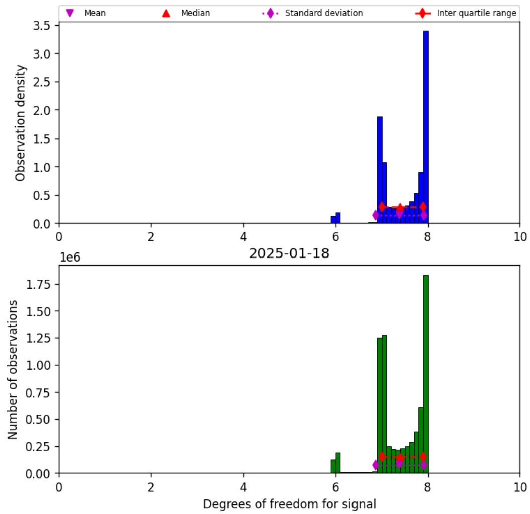
Figure 23: Histogram of “Degrees of freedom for signal” for 2025-01-17 to 2025-01-19
