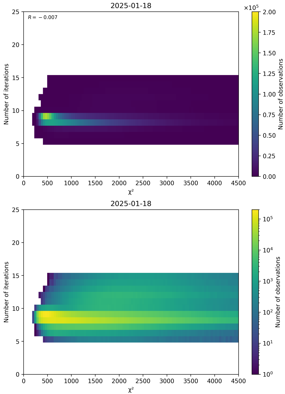
Figure 49: Scatter density plot of “ \chi^2 ” against “Number of iterations” for 2025-01-17 to 2025-01-19.
