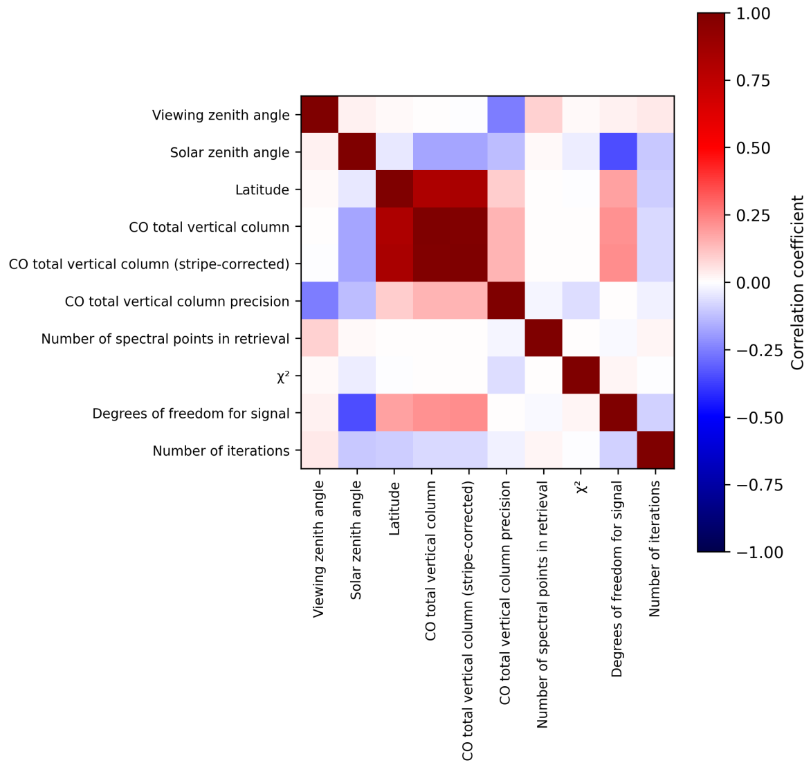
Figure 2: Map of correlation matrix for 2025-01-17 to 2025-01-19.
