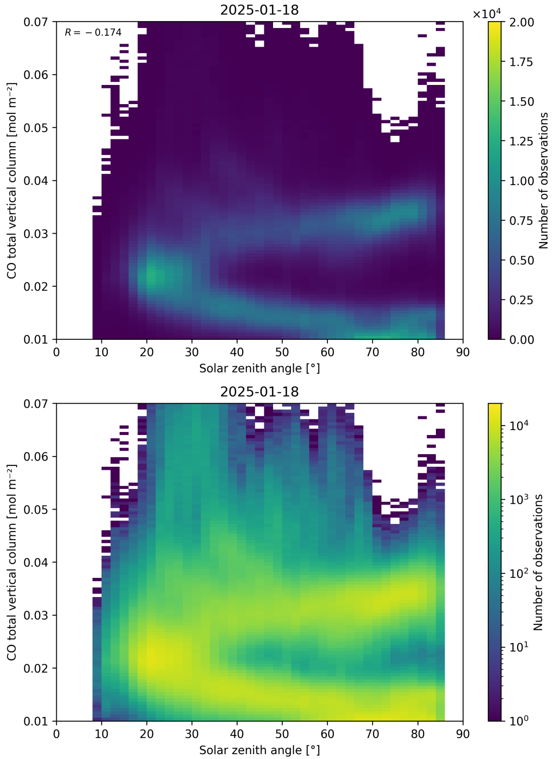
Figure 61: Scatter density plot of “Solar zenith angle” against “CO total vertical column” for 2025-01-17 to 2025-01-19.
