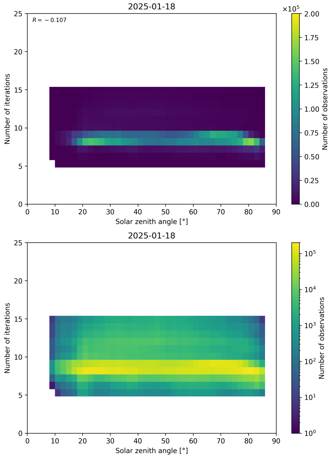
Figure 67: Scatter density plot of “Solar zenith angle” against “Number of iterations” for 2025-01-17 to 2025-01-19.
