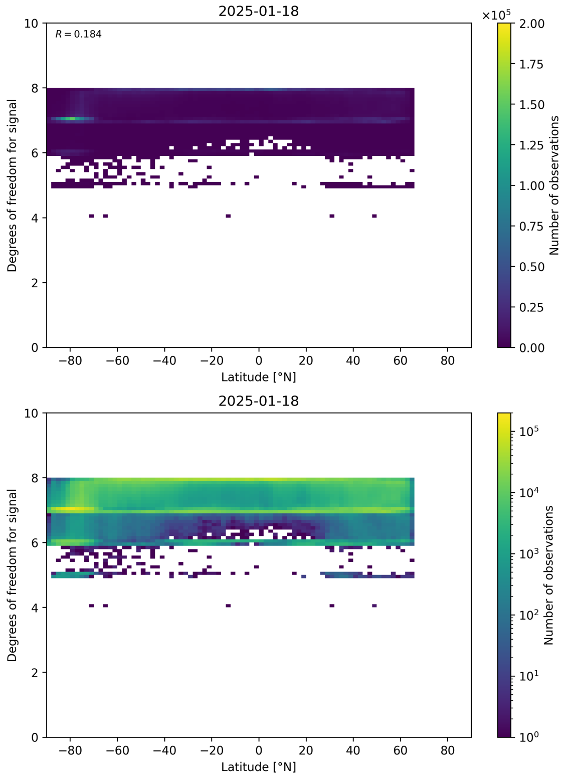
Figure 55: Scatter density plot of “Latitude” against “Degrees of freedom for signal” for 2025-01-17 to 2025-01-19.
