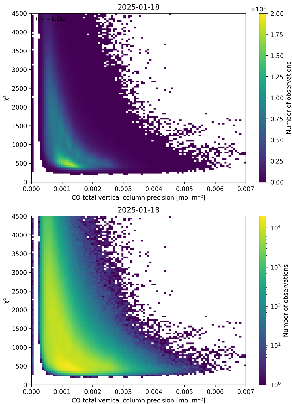
Figure 44: Scatter density plot of “CO total vertical column precision” against “ \chi^2 ” for 2025-01-17 to 2025-01-19.
