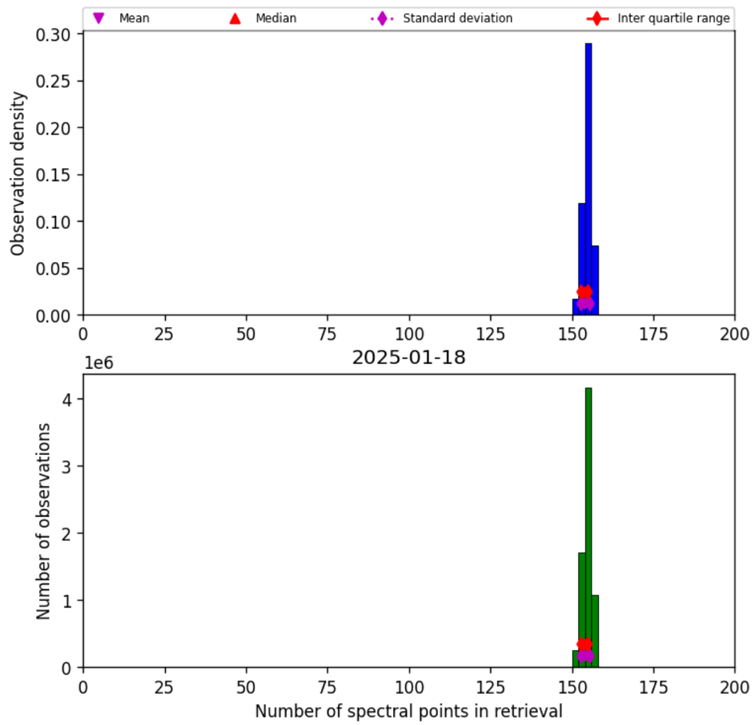
Figure 21: Histogram of “Number of spectral points in retrieval” for 2025-01-17 to 2025-01-19
