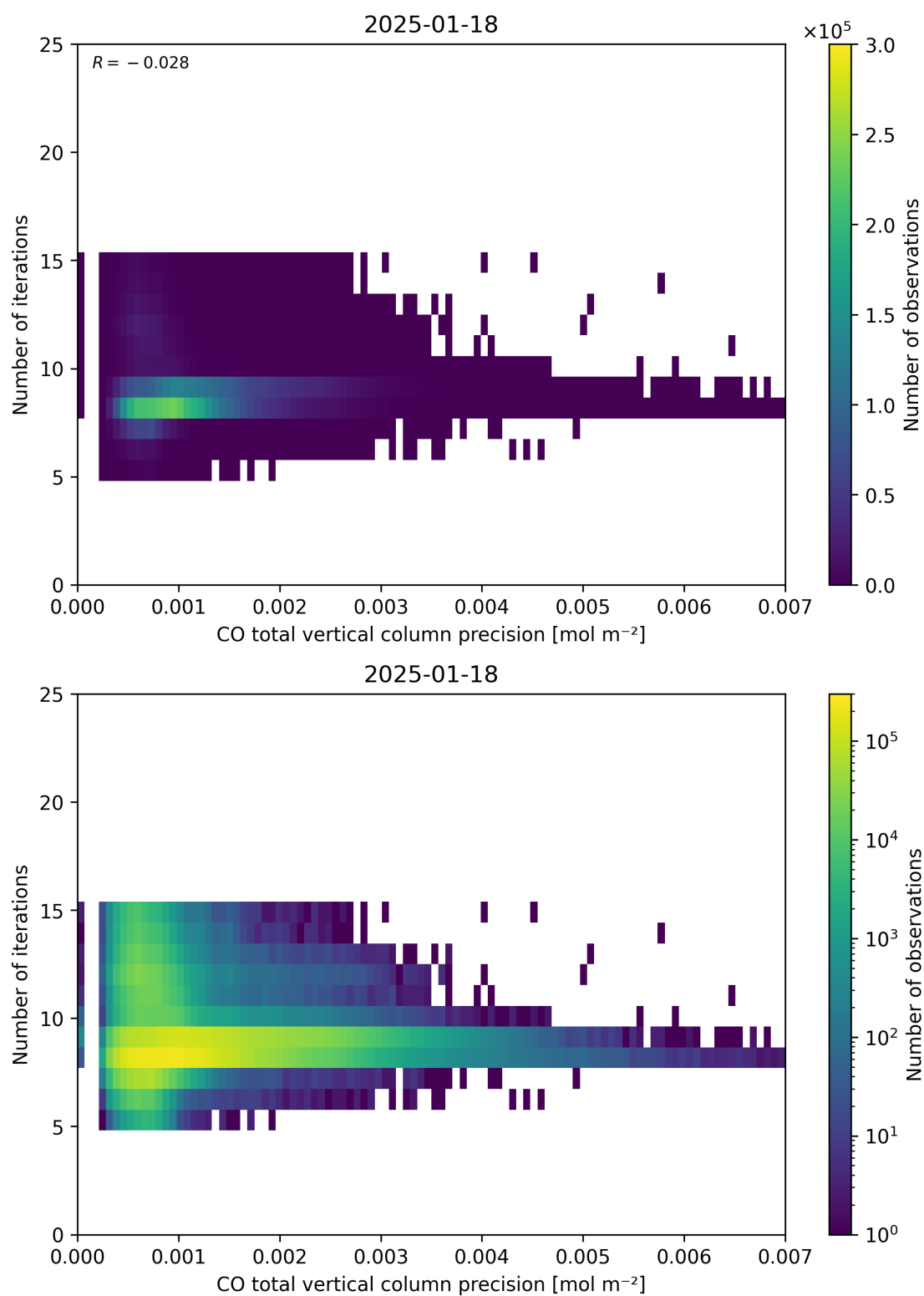
Figure 46: Scatter density plot of “CO total vertical column precision” against “Number of iterations” for 2025-01-17 to 2025-01-19.
