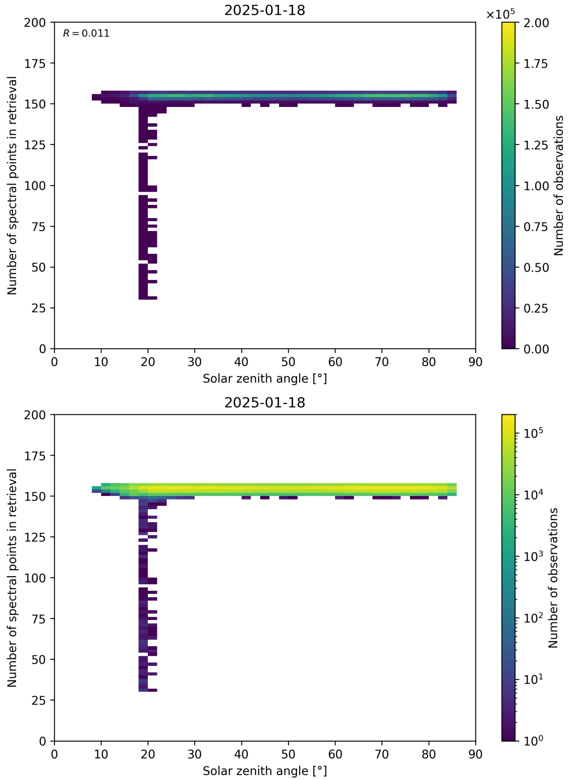
Figure 68: Scatter density plot of “Solar zenith angle” against “Number of spectral points in retrieval” for 2025-01-17 to 2025-01-19.
