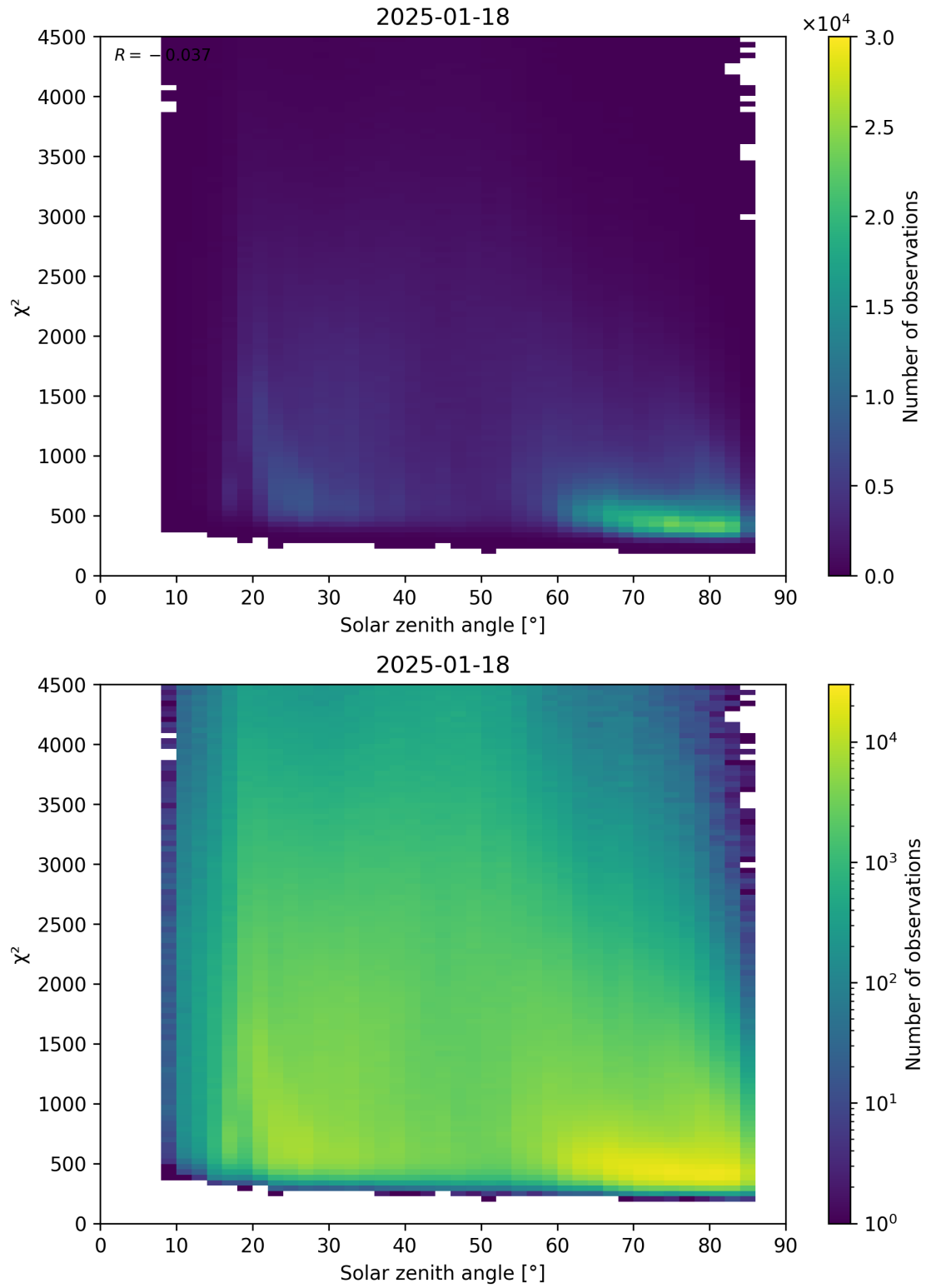
Figure 64: Scatter density plot of “Solar zenith angle” against “ \chi^2 ” for 2025-01-17 to 2025-01-19.
