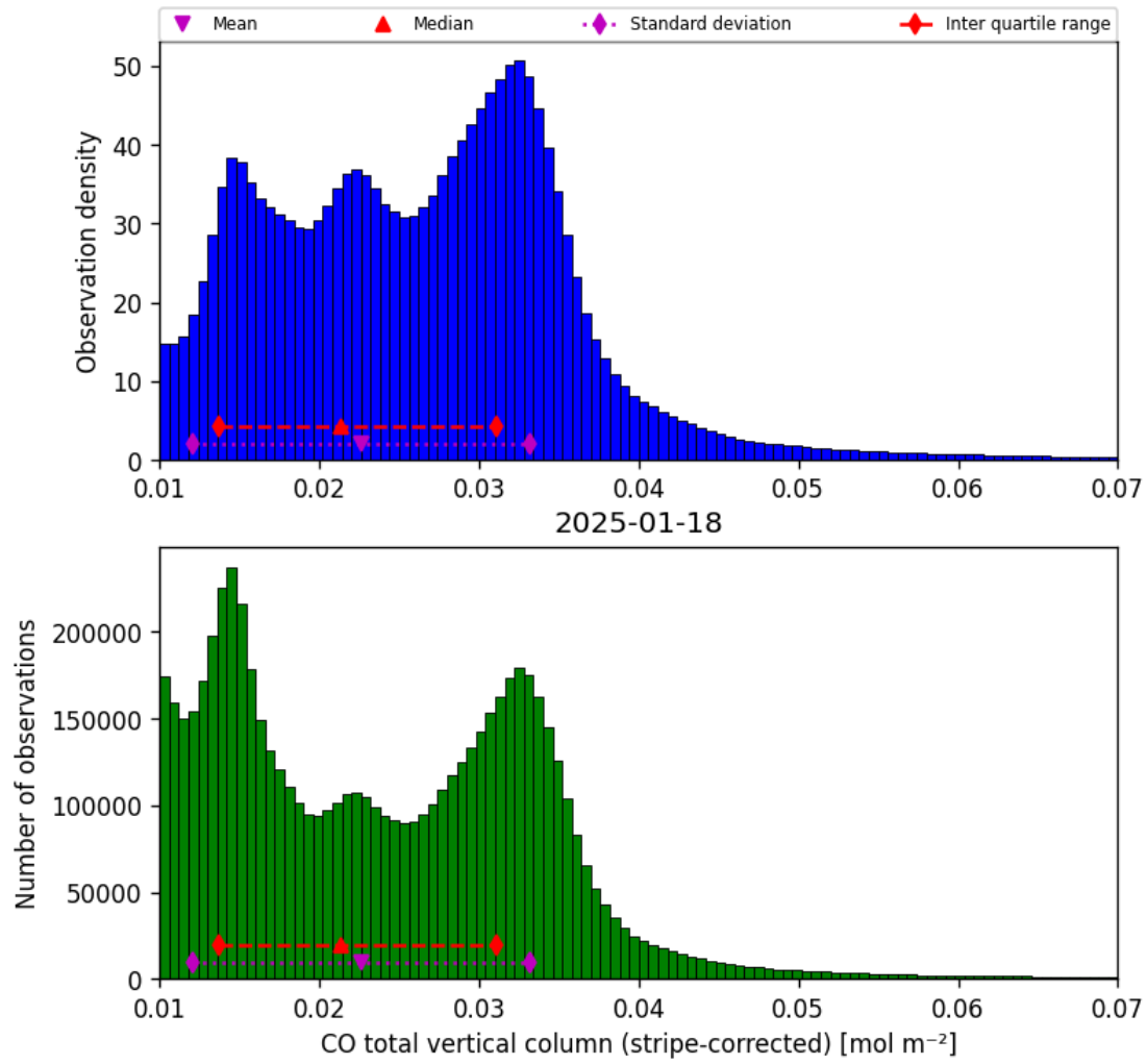
Figure 19: Histogram of “CO total vertical column (stripe-corrected)” for 2025-01-17 to 2025-01-19
