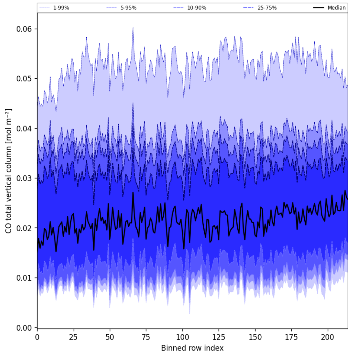
Figure 26: Along track statistics of “CO total vertical column” for 2025-01-17 to 2025-01-19
