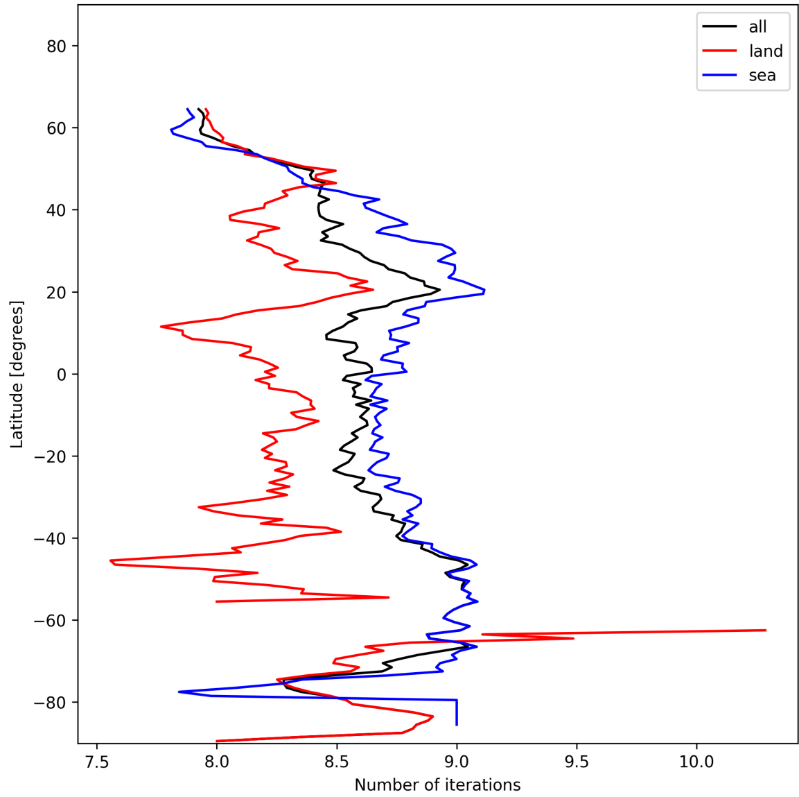
Figure 16: Zonal average of “Number of iterations” for 2025-01-17 to 2025-01-19.
