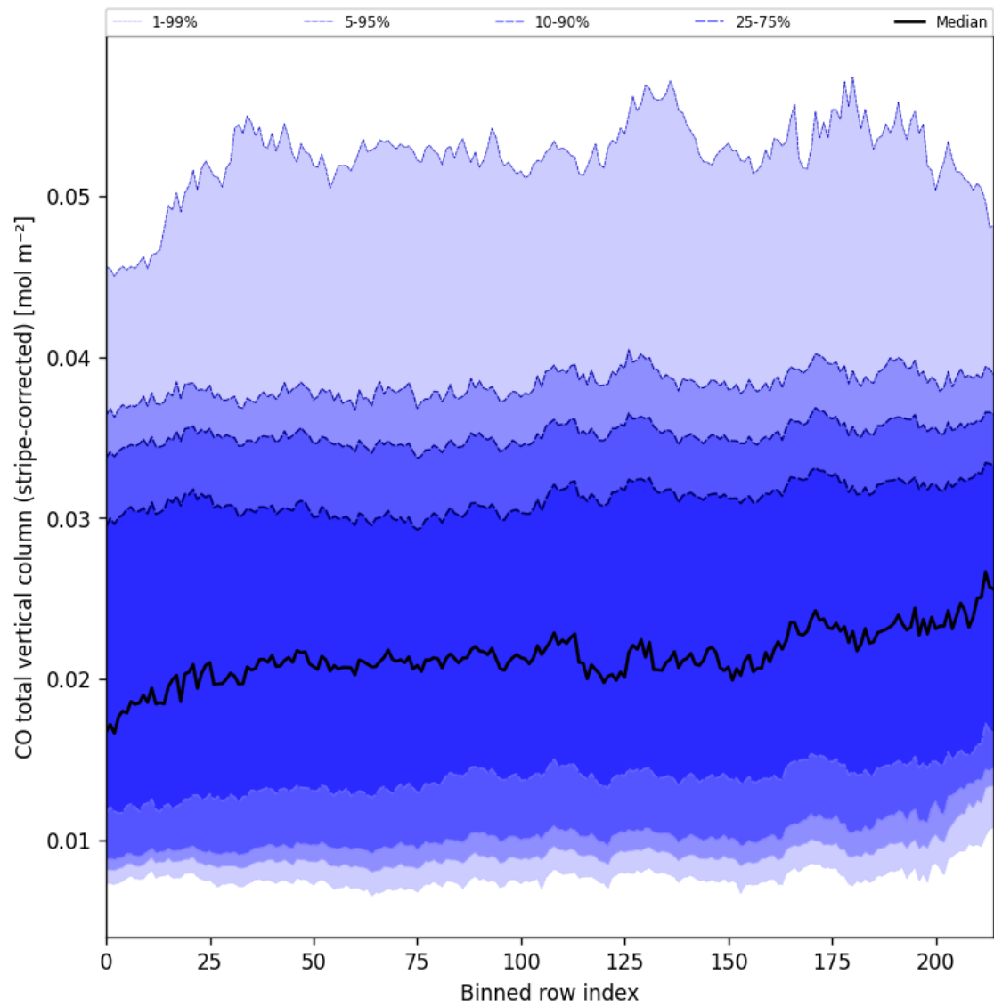
Figure 27: Along track statistics of “CO total vertical column (stripe-corrected)” for 2025-01-17 to 2025-01-19
