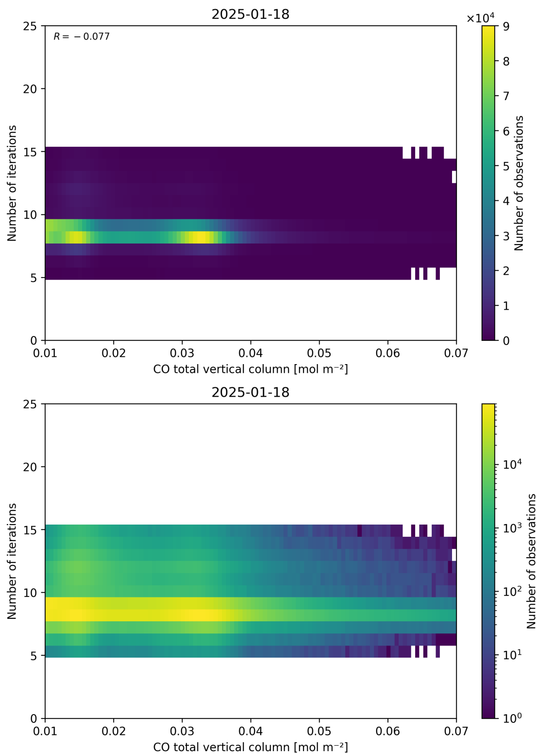
Figure 42: Scatter density plot of “CO total vertical column” against “Number of iterations” for 2025-01-17 to 2025-01-19.
