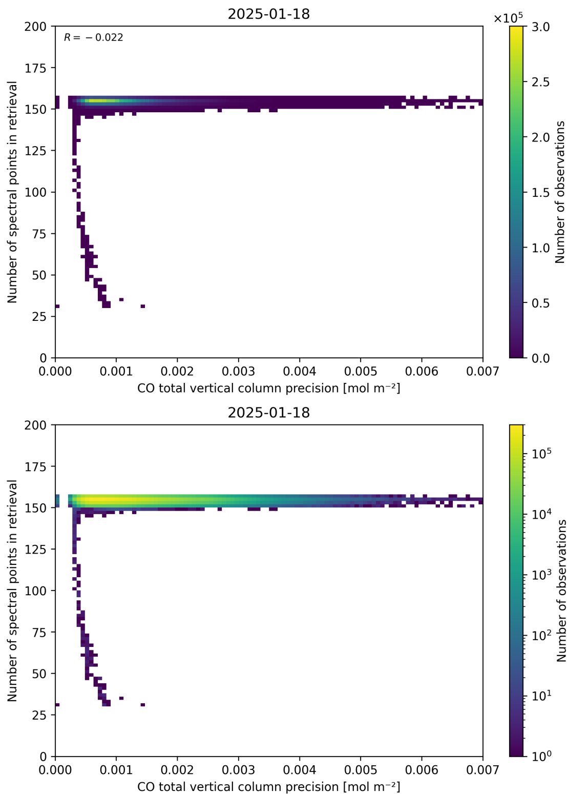
Figure 47: Scatter density plot of “CO total vertical column precision” against “Number of spectral points in retrieval” for 2025-01-17 to 2025-01-19.
