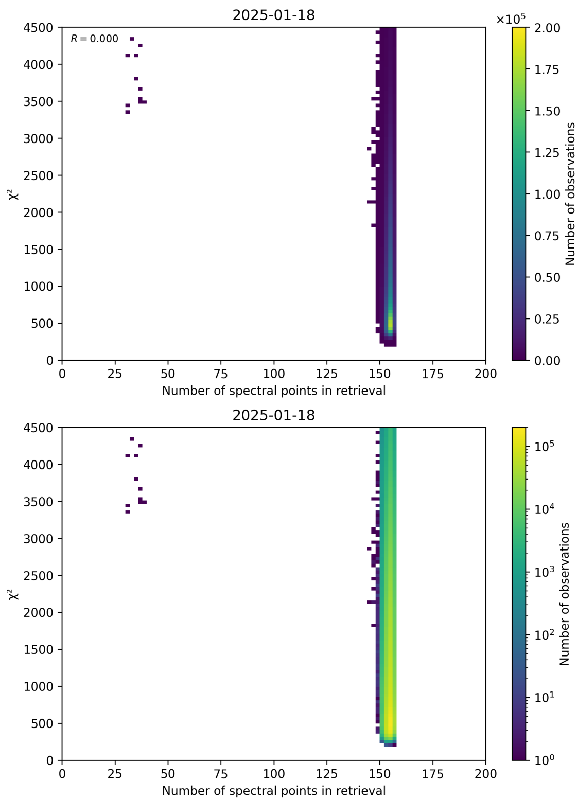
Figure 58: Scatter density plot of “Number of spectral points in retrieval” against “ \chi^2 ” for 2025-01-17 to 2025-01-19.
