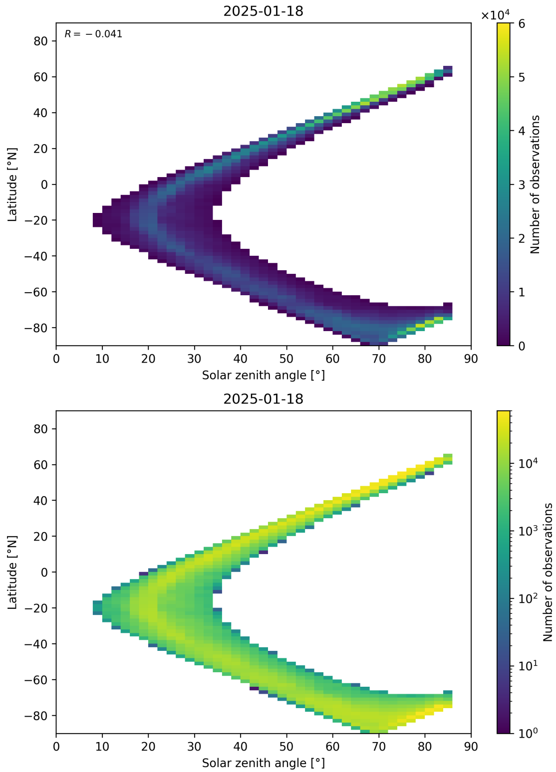
Figure 66: Scatter density plot of “Solar zenith angle” against “Latitude” for 2025-01-17 to 2025-01-19.
