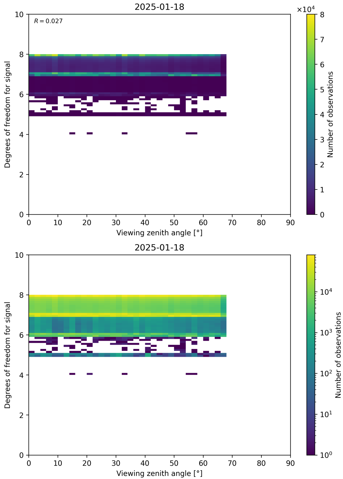
Figure 73: Scatter density plot of “Viewing zenith angle” against “Degrees of freedom for signal” for 2025-01-17 to 2025-01-19.
