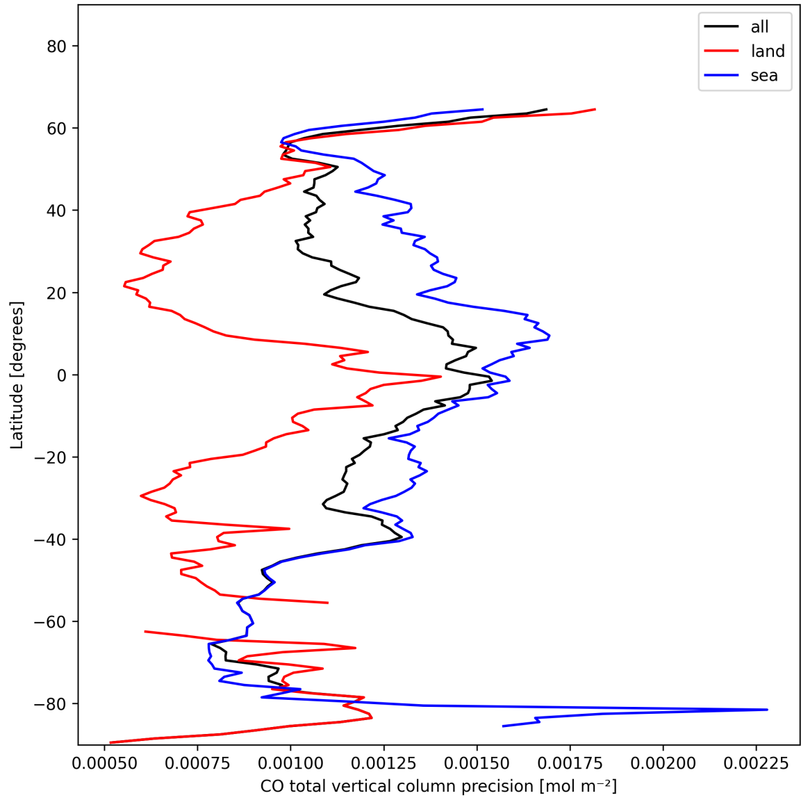
Figure 12: Zonal average of “CO total vertical column precision” for 2025-01-17 to 2025-01-19.
