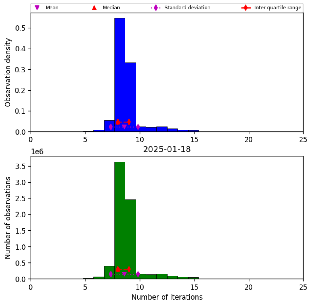
Figure 24: Histogram of “Number of iterations” for 2025-01-17 to 2025-01-19
