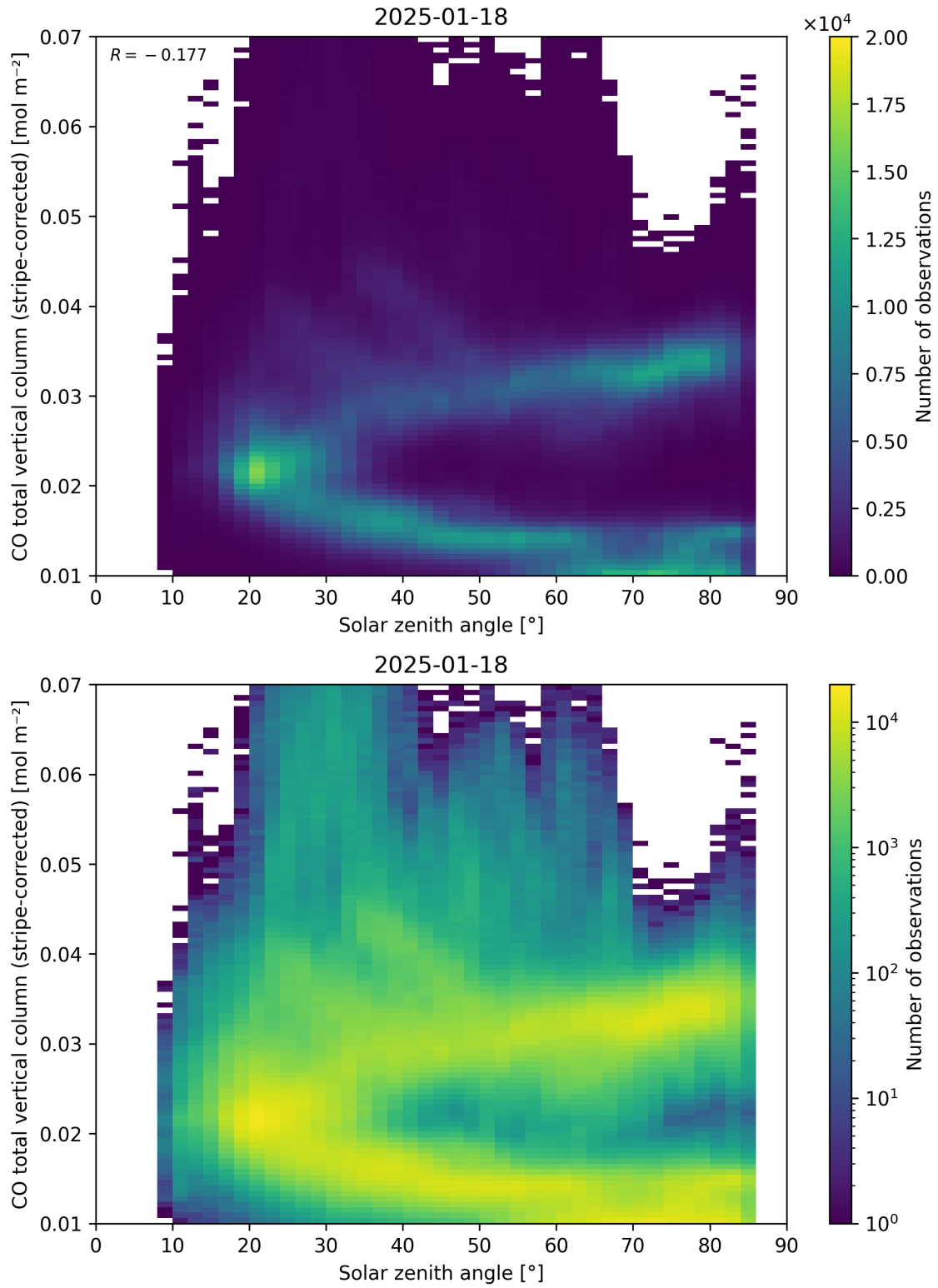
Figure 62: Scatter density plot of “Solar zenith angle” against “CO total vertical column (stripe-corrected)” for 2025-01-17 to 2025-01-19.
