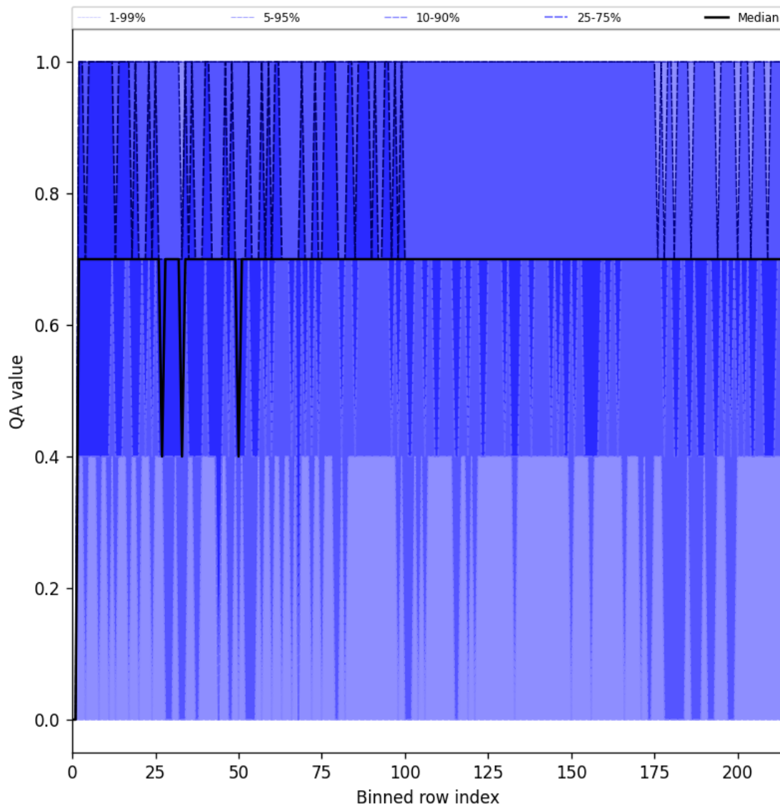
Figure 25: Along track statistics of “QA value” for 2025-01-17 to 2025-01-19
