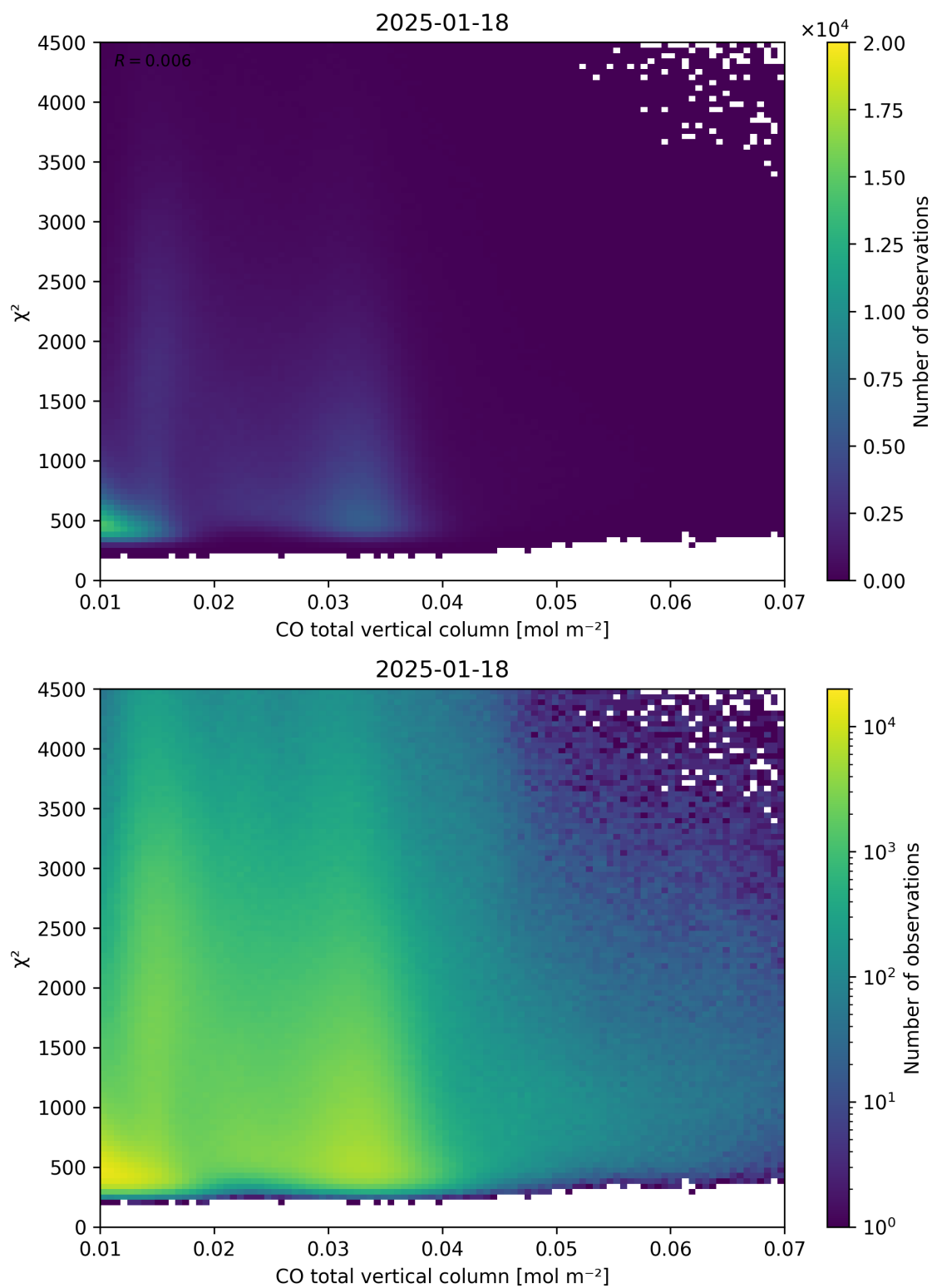
Figure 35: Scatter density plot of “CO total vertical column” against “ \chi^2 ” for 2025-01-17 to 2025-01-19.
