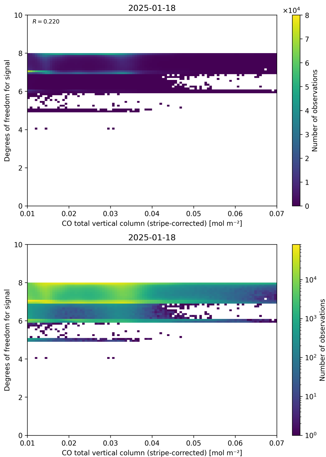
Figure 38: Scatter density plot of “CO total vertical column (stripe-corrected)” against “Degrees of freedom for signal” for 2025-01-17 to 2025-01-19.
