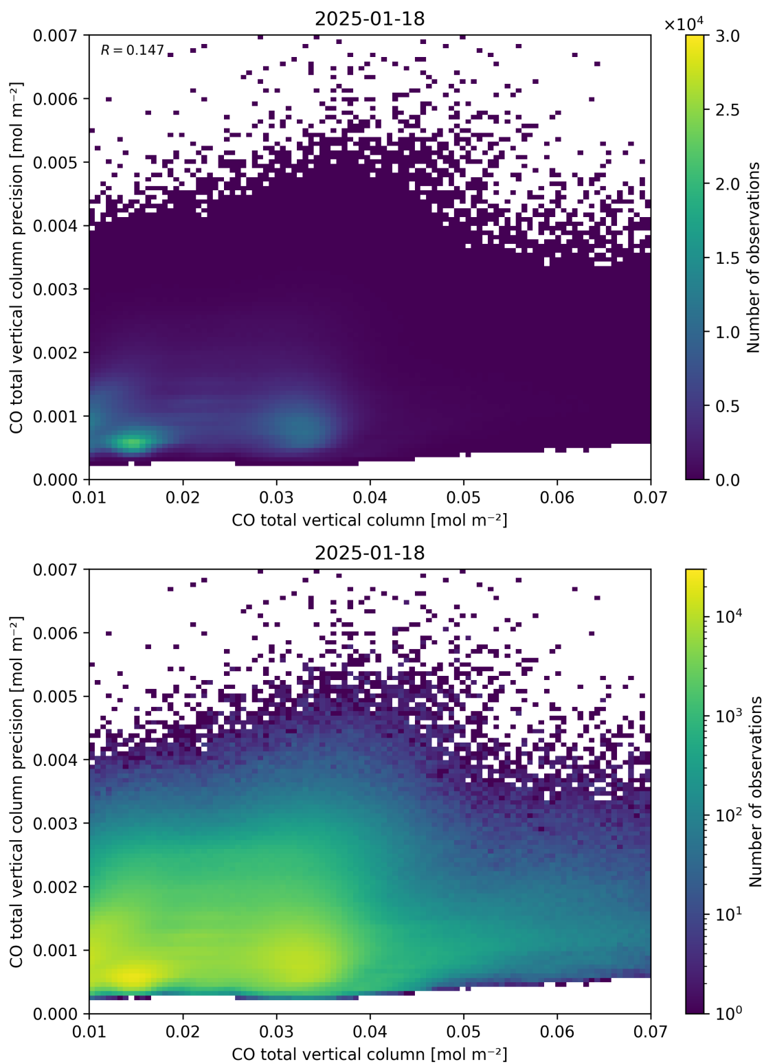
Figure 34: Scatter density plot of “CO total vertical column” against “CO total vertical column precision” for 2025-01-17 to 2025-01-19.
