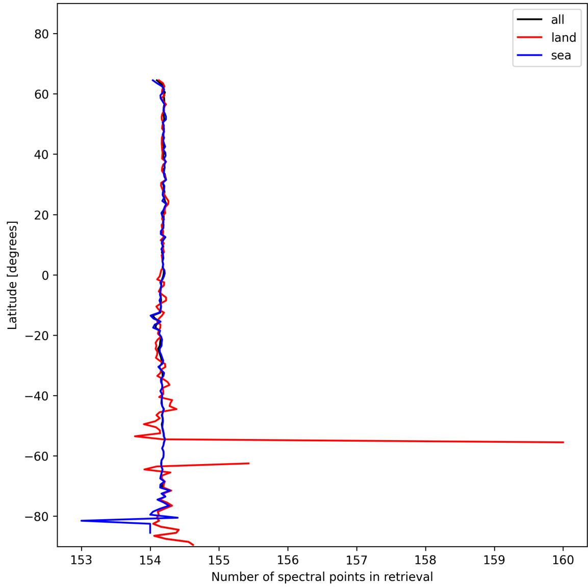
Figure 13: Zonal average of “Number of spectral points in retrieval” for 2025-01-17 to 2025-01-19.
