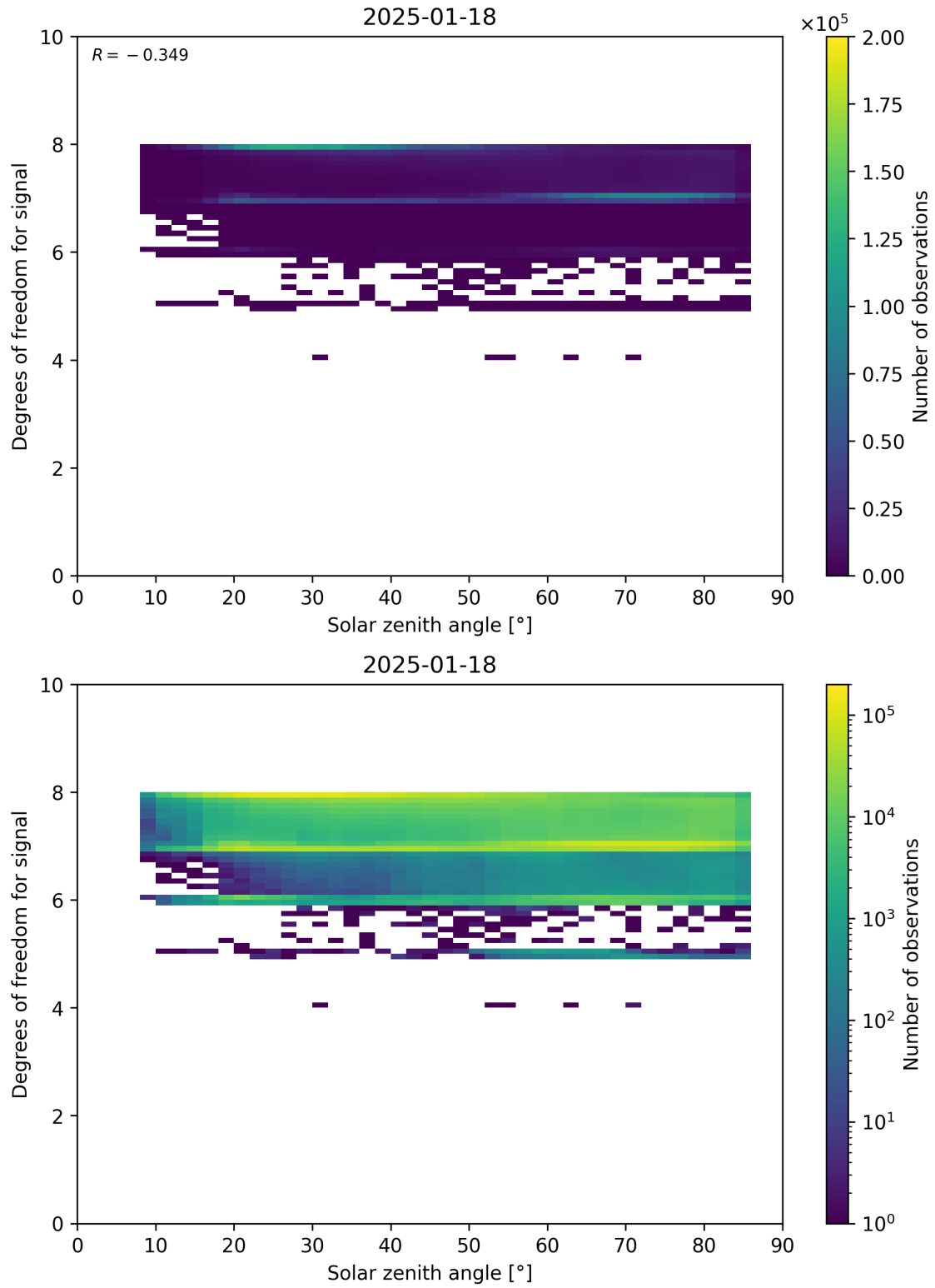
Figure 65: Scatter density plot of “Solar zenith angle” against “Degrees of freedom for signal” for 2025-01-17 to 2025-01-19.
