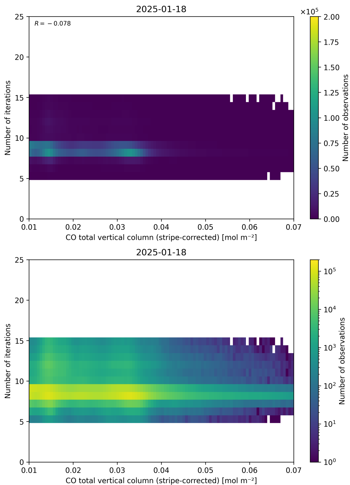
Figure 39: Scatter density plot of “CO total vertical column (stripe-corrected)” against “Number of iterations” for 2025-01-17 to 2025-01-19.
