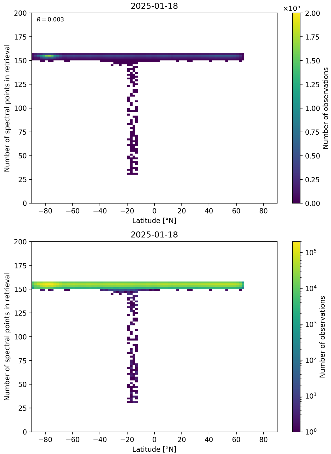
Figure 57: Scatter density plot of “Latitude” against “Number of spectral points in retrieval” for 2025-01-17 to 2025-01-19.
