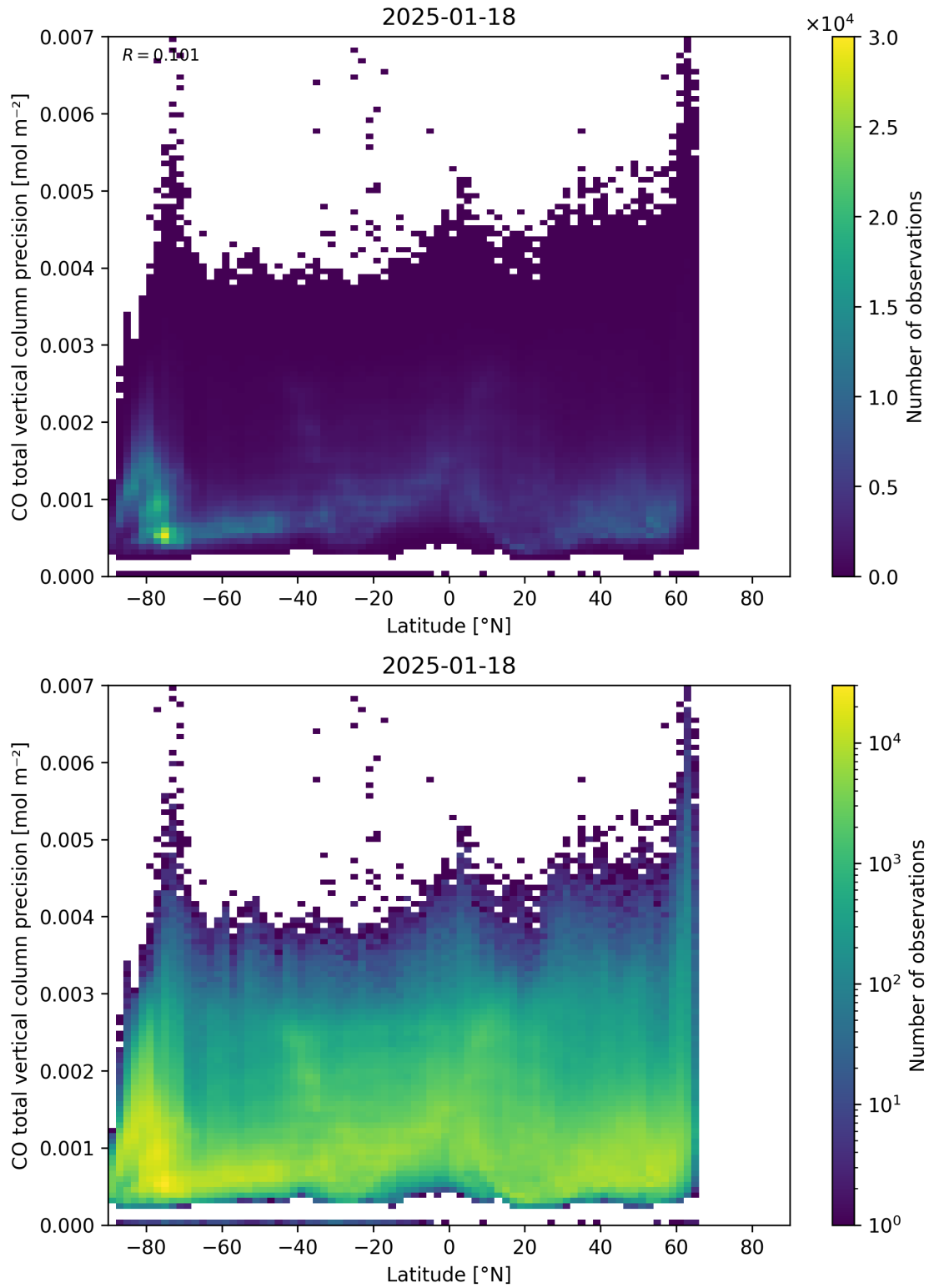
Figure 53: Scatter density plot of “Latitude” against “CO total vertical column precision” for 2025-01-17 to 2025-01-19.
