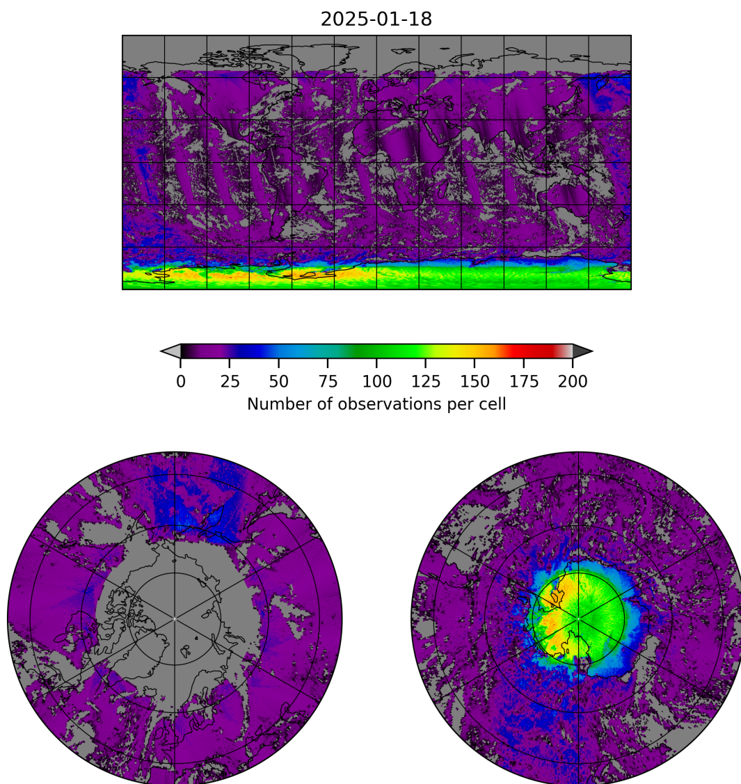
Figure 8: Map of the number of observations for 2025-01-17 to 2025-01-19
