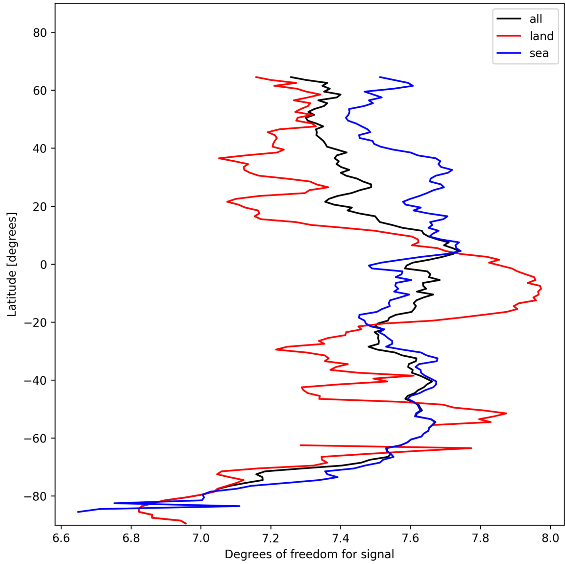
Figure 15: Zonal average of “Degrees of freedom for signal” for 2025-01-17 to 2025-01-19.
