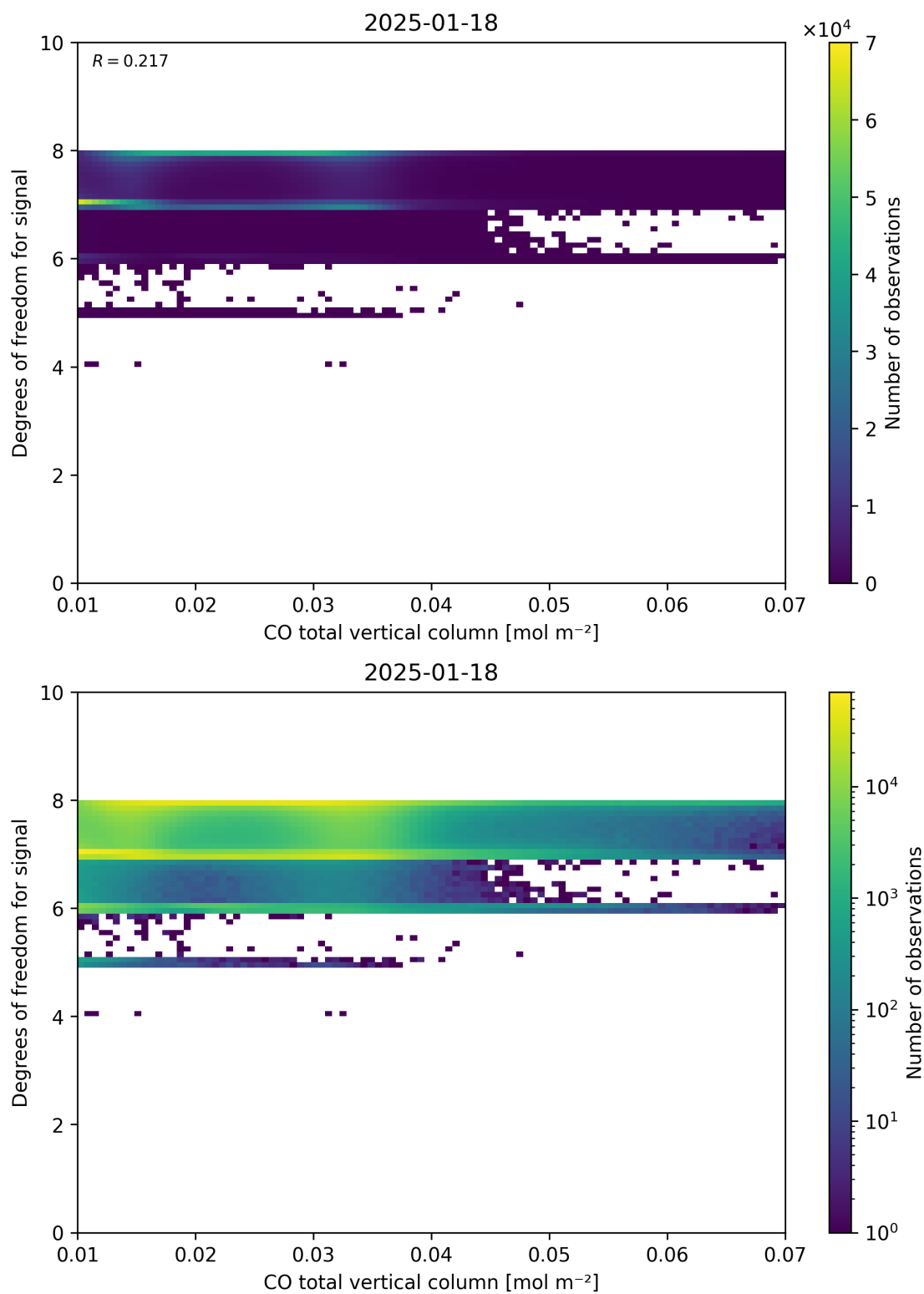
Figure 41: Scatter density plot of “CO total vertical column” against “Degrees of freedom for signal” for 2025-01-17 to 2025-01-19.
