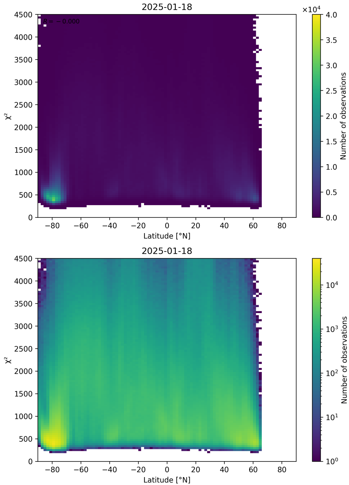
Figure 54: Scatter density plot of “Latitude” against “ \chi^2 ” for 2025-01-17 to 2025-01-19.
