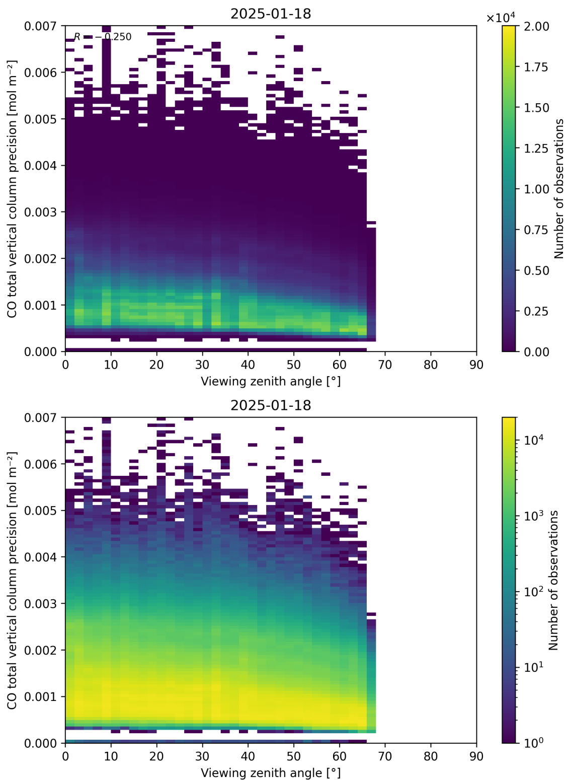
Figure 71: Scatter density plot of “Viewing zenith angle” against “CO total vertical column precision” for 2025-01-17 to 2025-01-19.
