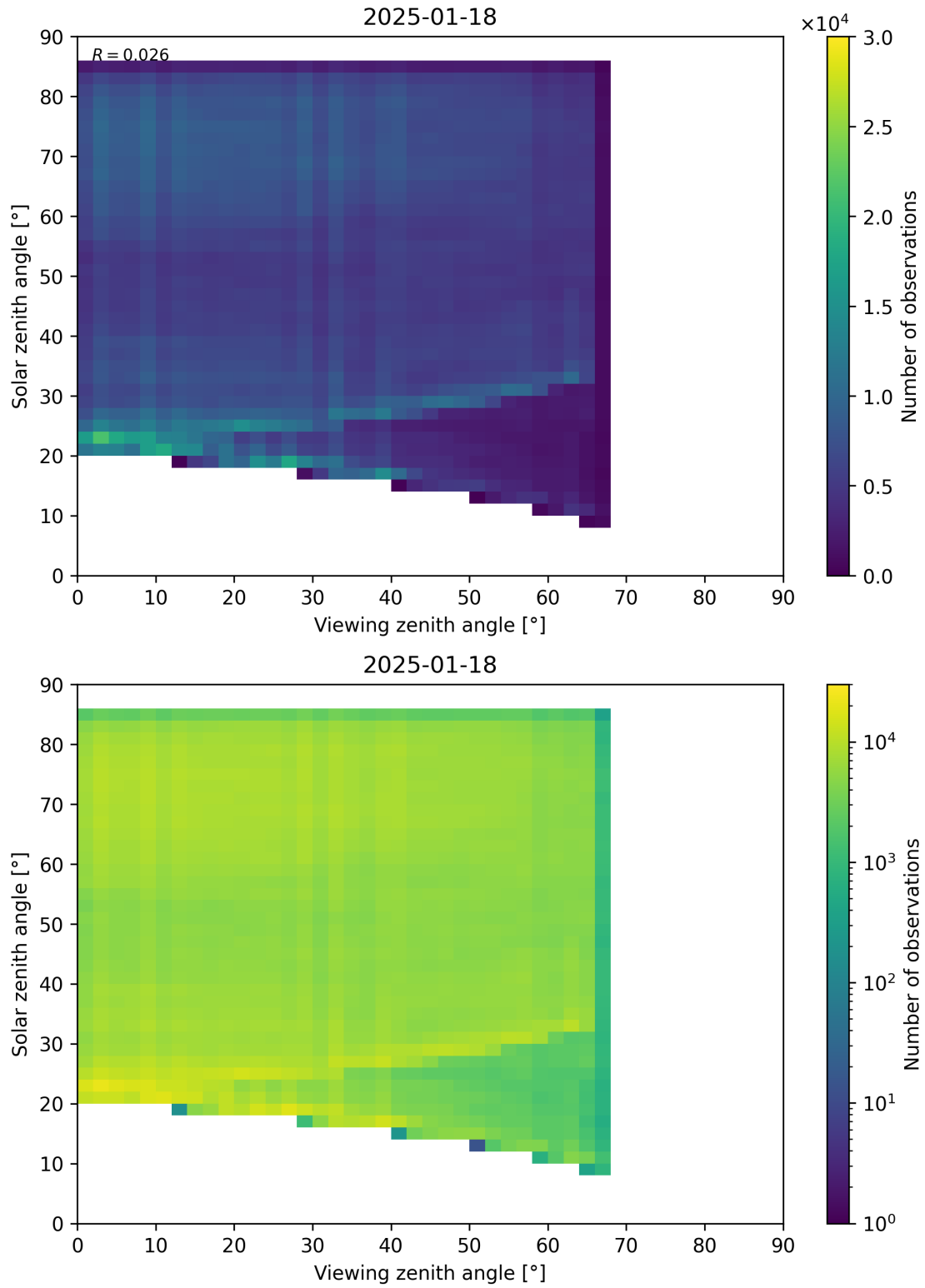
Figure 77: Scatter density plot of “Viewing zenith angle” against “Solar zenith angle” for 2025-01-17 to 2025-01-19.
