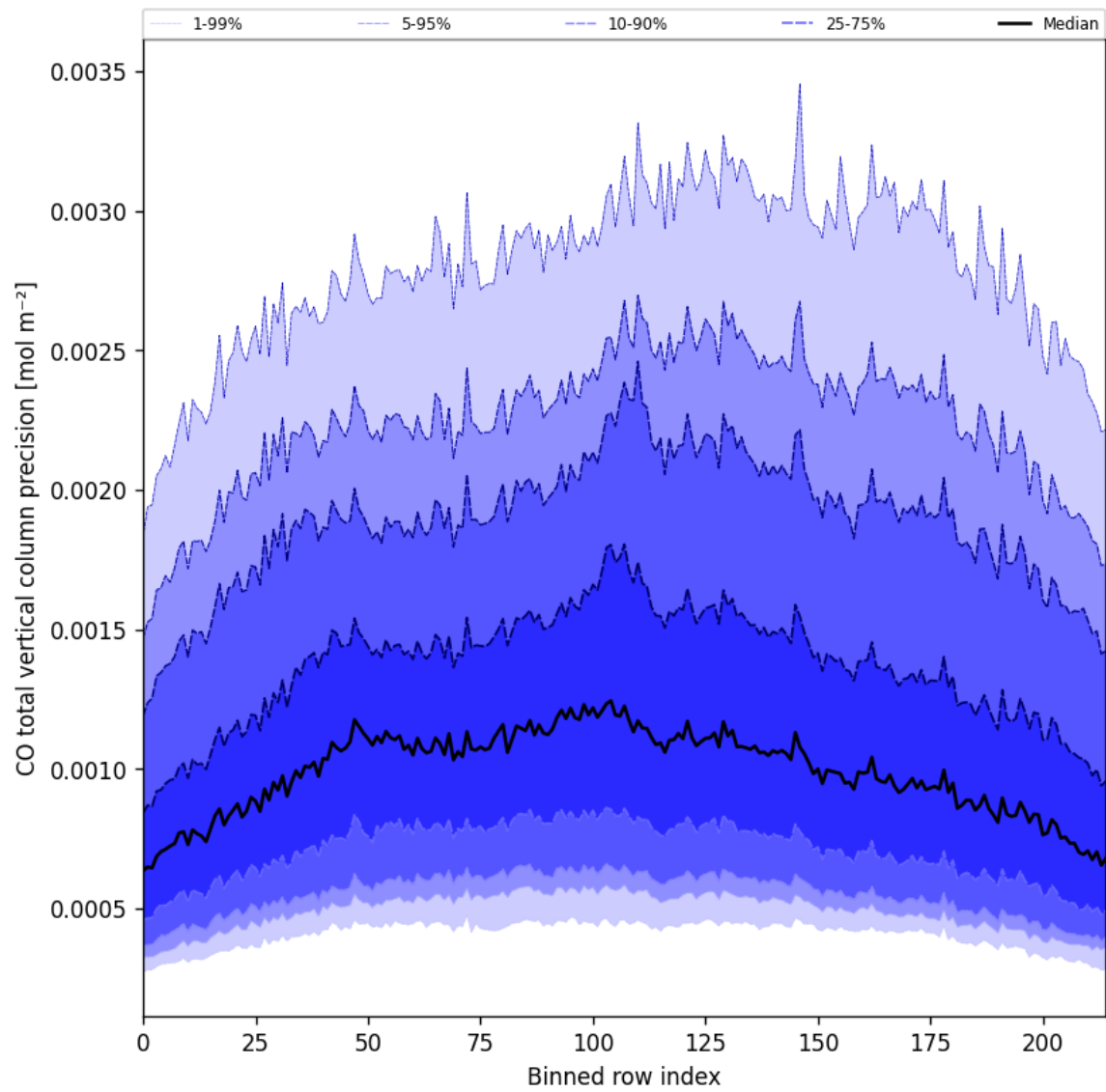
Figure 28: Along track statistics of “CO total vertical column precision” for 2025-01-17 to 2025-01-19
