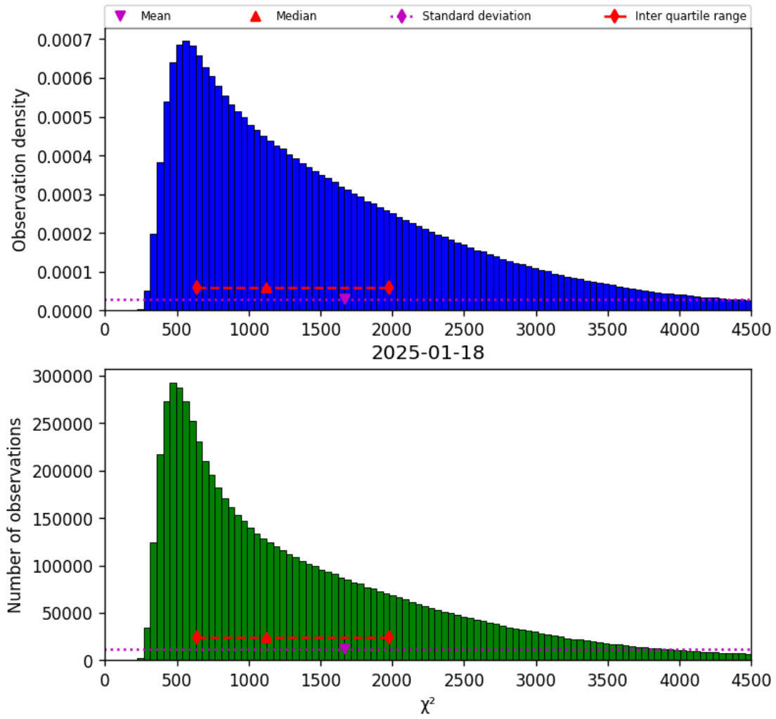
Figure 22: Histogram of “ \chi^2 ” for 2025-01-17 to 2025-01-19
