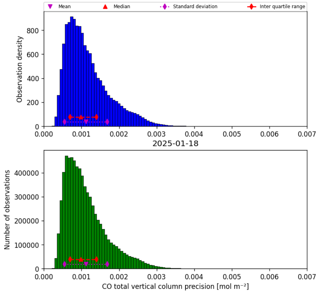
Figure 20: Histogram of “CO total vertical column precision” for 2025-01-17 to 2025-01-19
