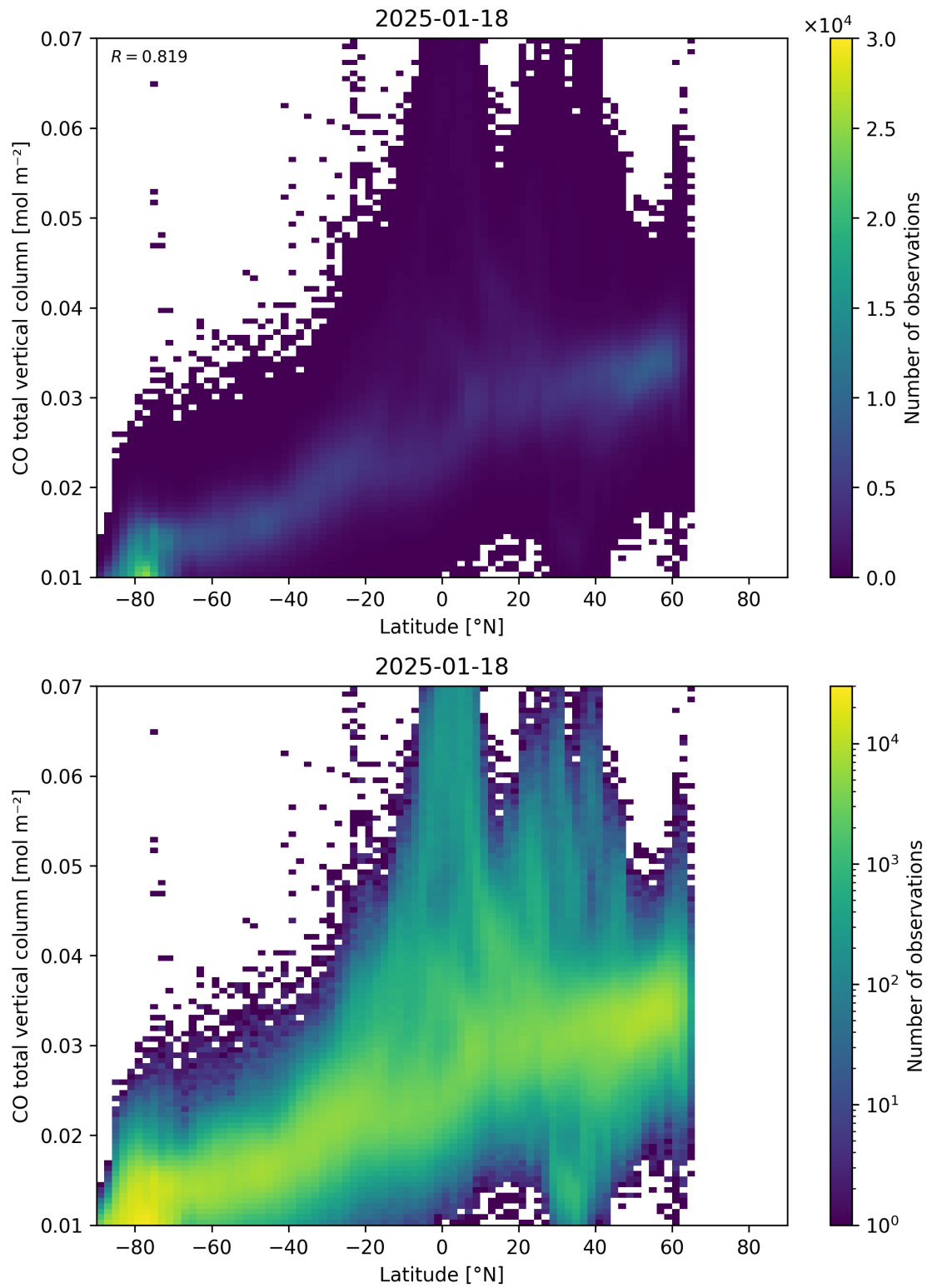
Figure 51: Scatter density plot of “Latitude” against “CO total vertical column” for 2025-01-17 to 2025-01-19.
