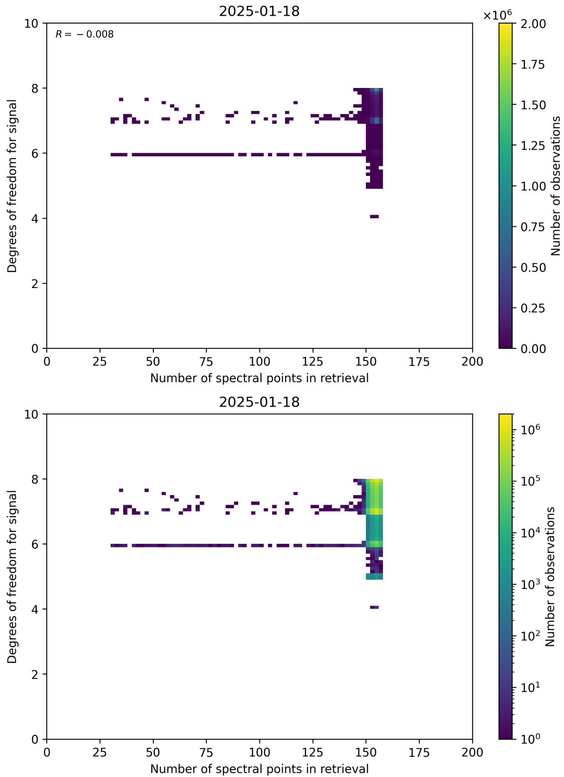
Figure 59: Scatter density plot of “Number of spectral points in retrieval” against “Degrees of freedom for signal” for 2025-01-17 to 2025-01-19.
