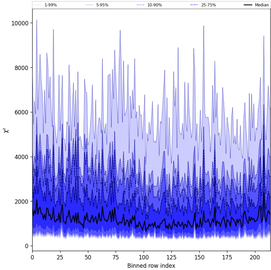
Figure 30: Along track statistics of “ \chi^2 ” for 2025-01-17 to 2025-01-19
