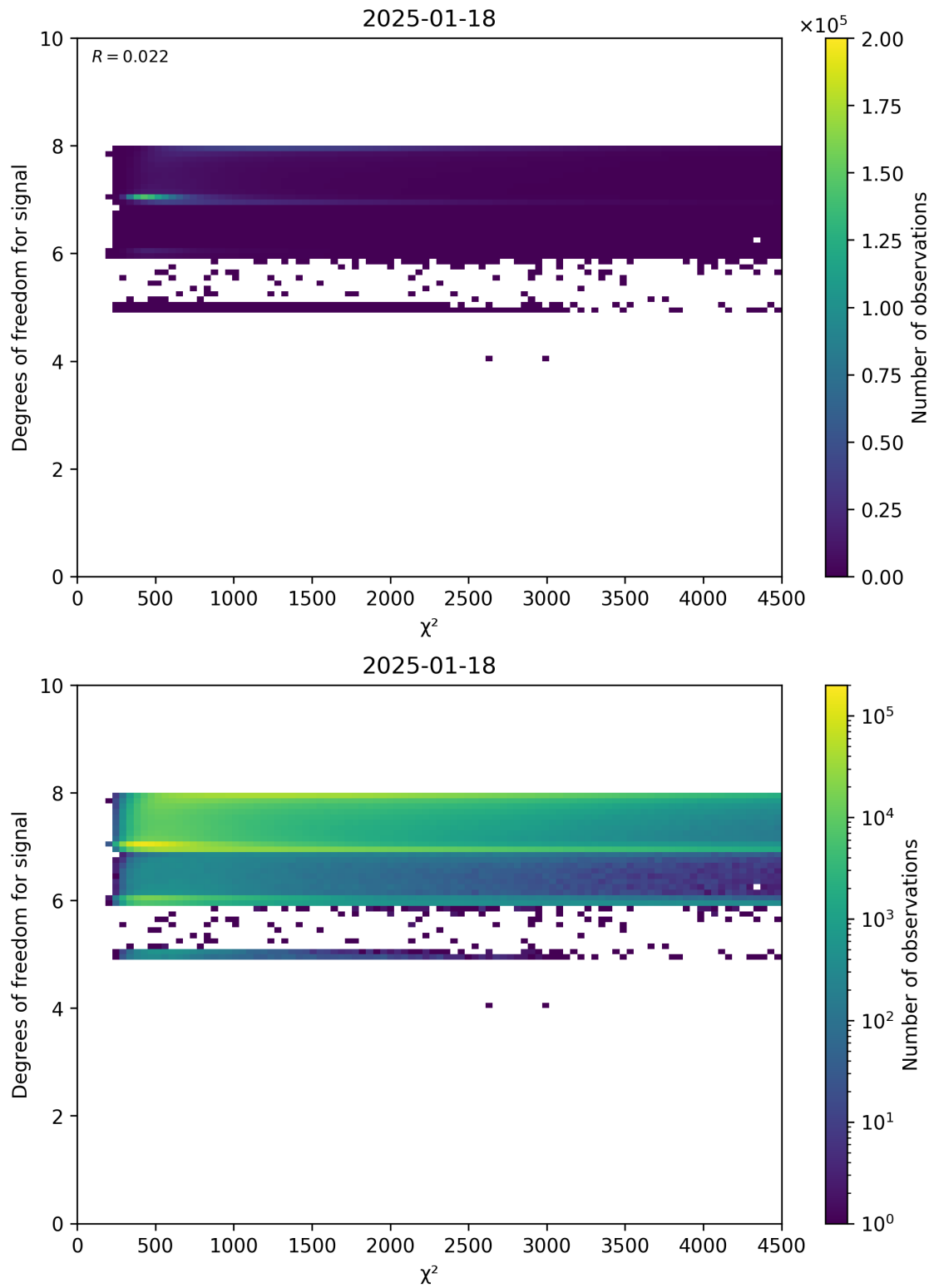
Figure 48: Scatter density plot of “ \chi^2 ” against “Degrees of freedom for signal” for 2025-01-17 to 2025-01-19.
