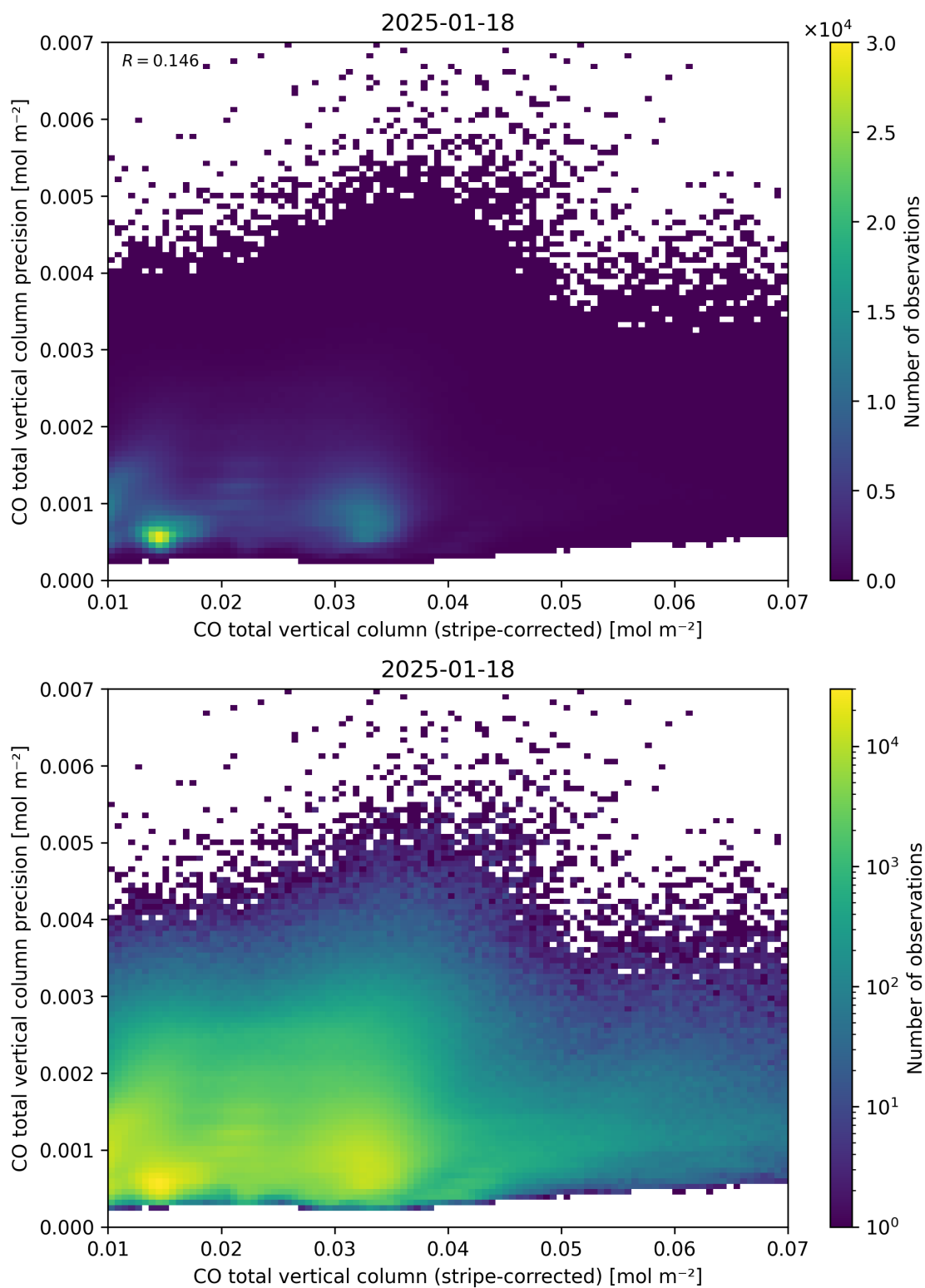
Figure 36: Scatter density plot of “CO total vertical column (stripe-corrected)” against “CO total vertical column precision” for 2025-01-17 to 2025-01-19.
