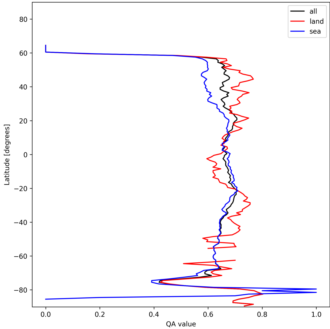
Figure 9: Zonal average of “QA value” for 2025-01-17 to 2025-01-19.
