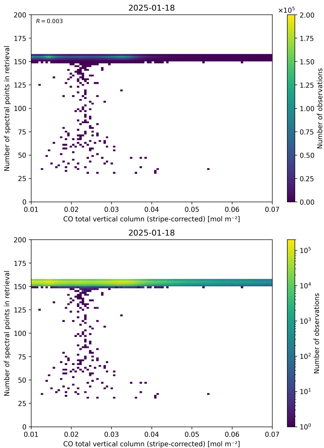
Figure 40: Scatter density plot of “CO total vertical column (stripe-corrected)” against “Number of spectral points in retrieval” for 2025-01-17 to 2025-01-19.
