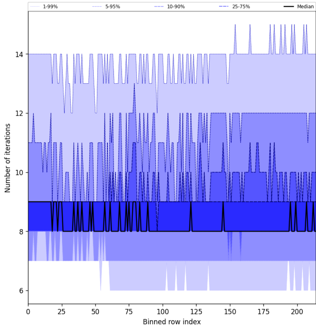
Figure 32: Along track statistics of “Number of iterations” for 2025-01-17 to 2025-01-19
