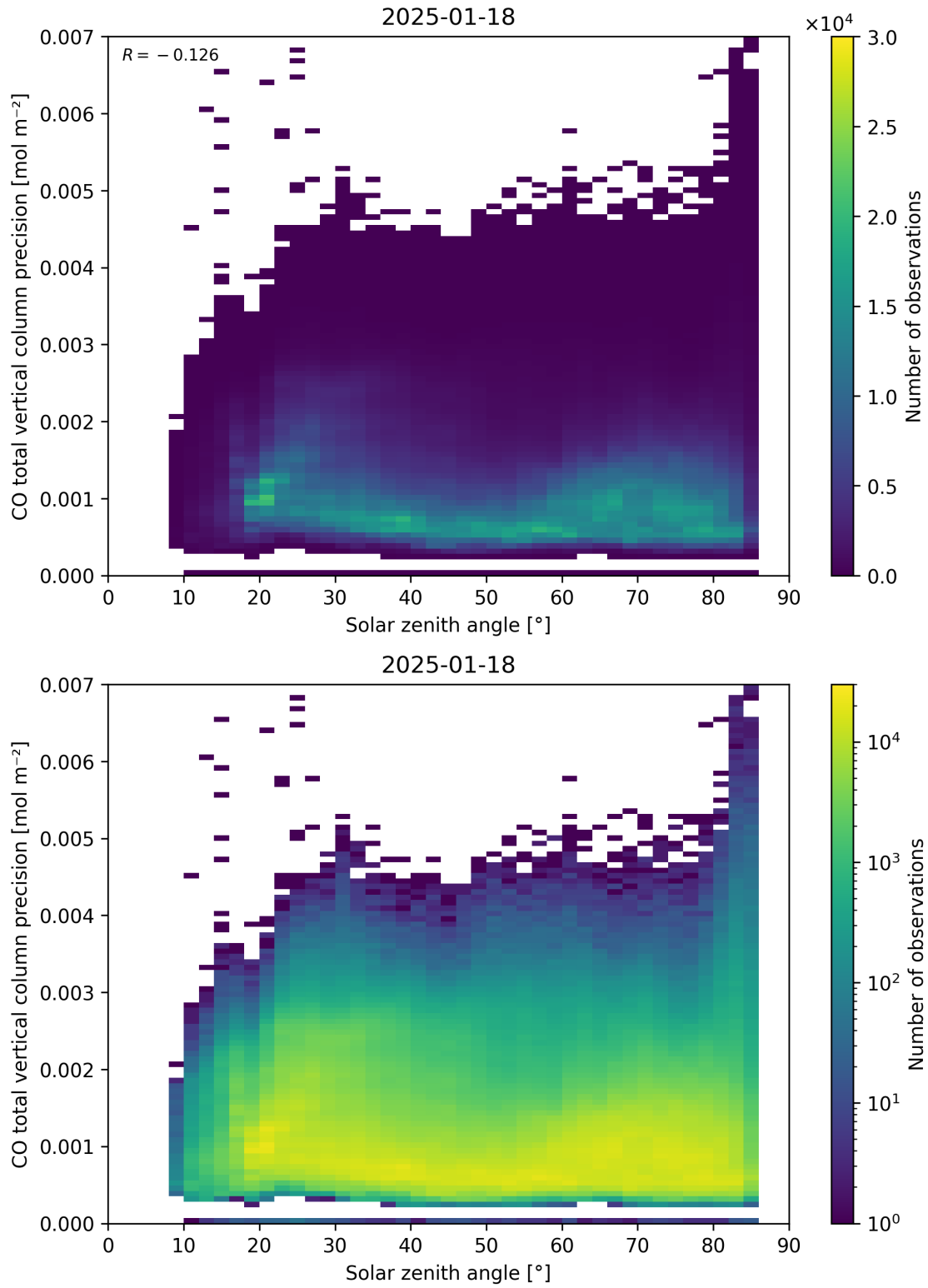
Figure 63: Scatter density plot of “Solar zenith angle” against “CO total vertical column precision” for 2025-01-17 to 2025-01-19.
