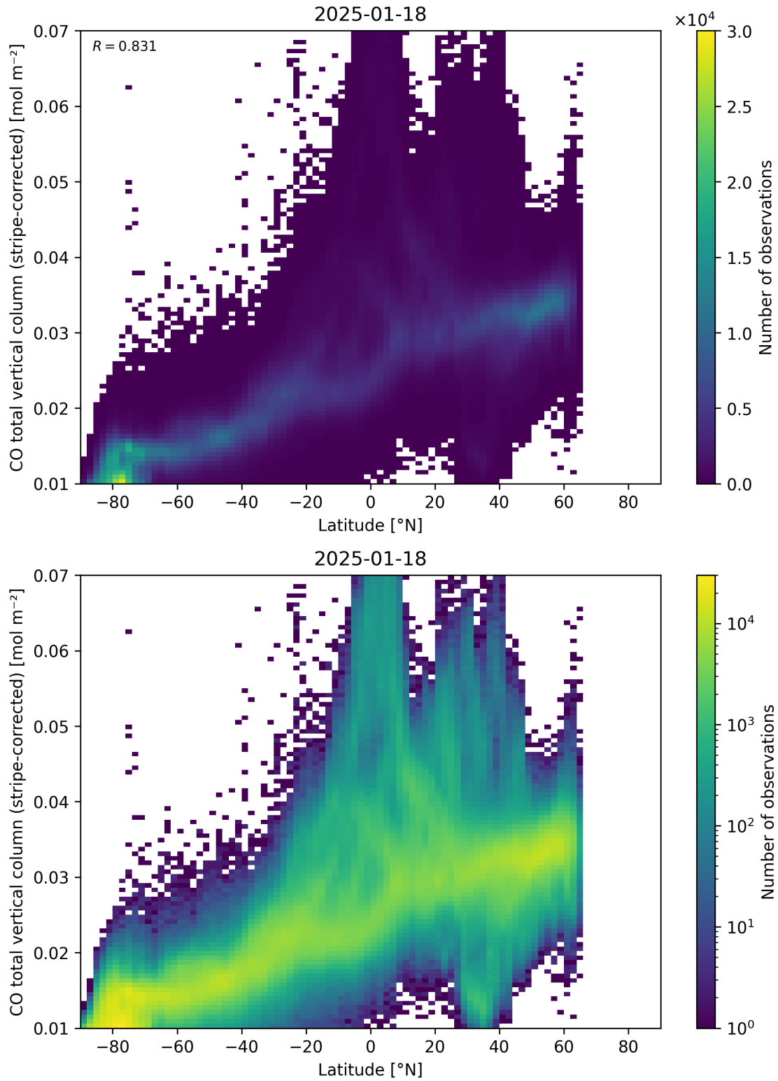
Figure 52: Scatter density plot of “Latitude” against “CO total vertical column (stripe-corrected)” for 2025-01-17 to 2025-01-19.
