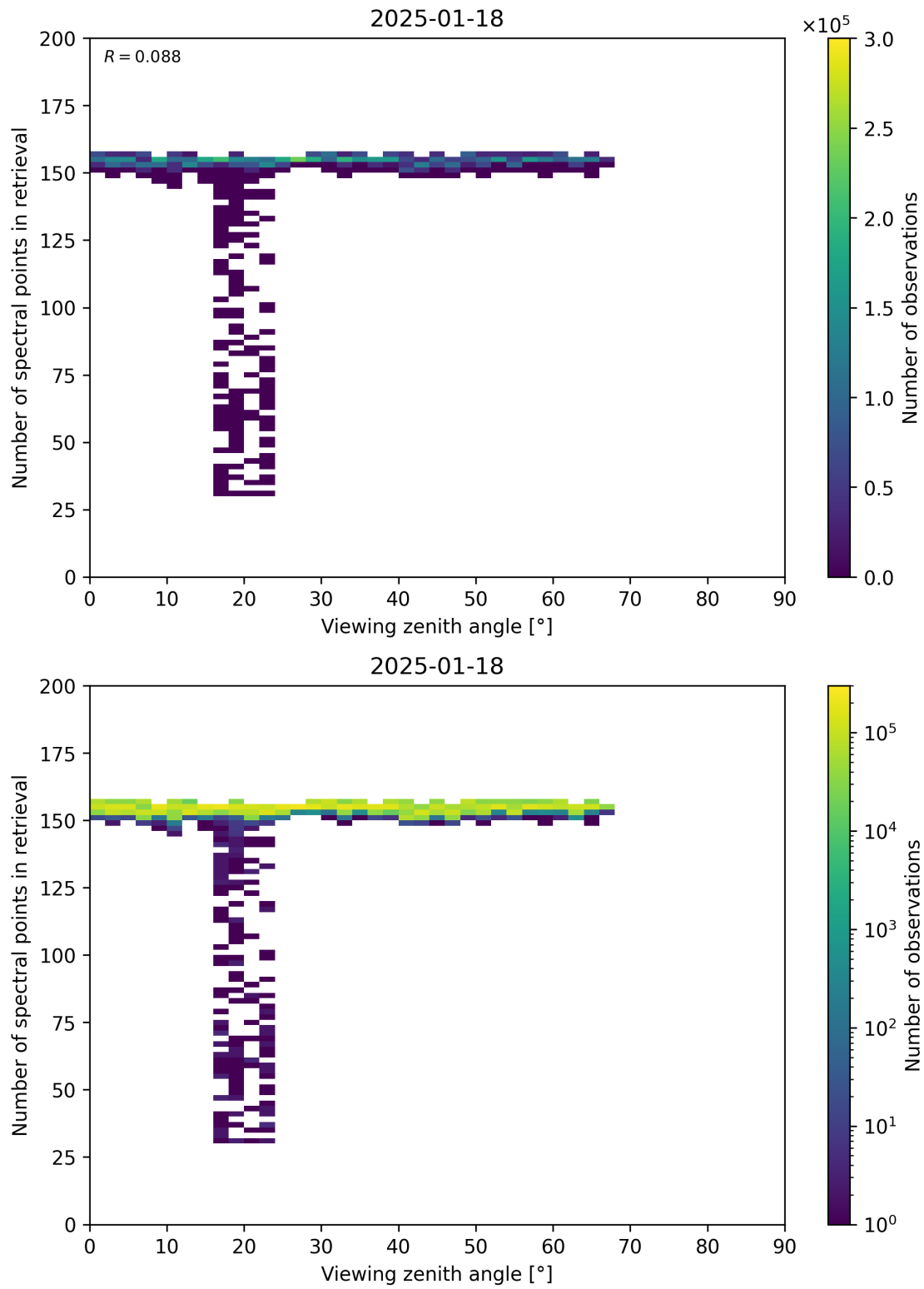
Figure 76: Scatter density plot of “Viewing zenith angle” against “Number of spectral points in retrieval” for 2025-01-17 to 2025-01-19.
