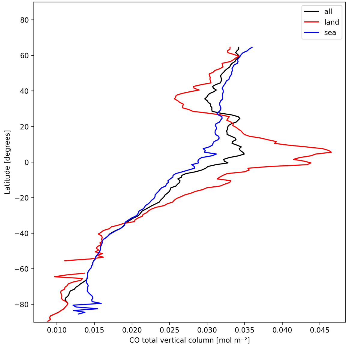
Figure 10: Zonal average of “CO total vertical column” for 2025-01-17 to 2025-01-19.
