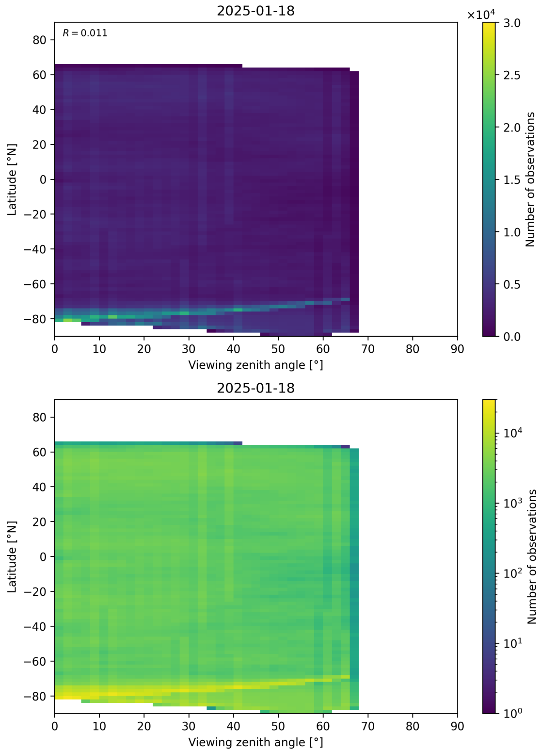
Figure 74: Scatter density plot of “Viewing zenith angle” against “Latitude” for 2025-01-17 to 2025-01-19.
