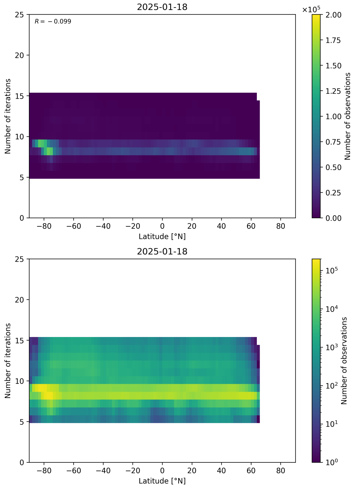
Figure 56: Scatter density plot of “Latitude” against “Number of iterations” for 2025-01-17 to 2025-01-19.
