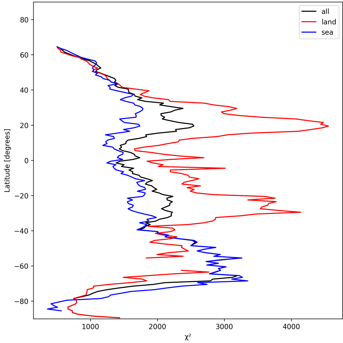
Figure 14: Zonal average of “ \chi^2 ” for 2025-01-17 to 2025-01-19.
