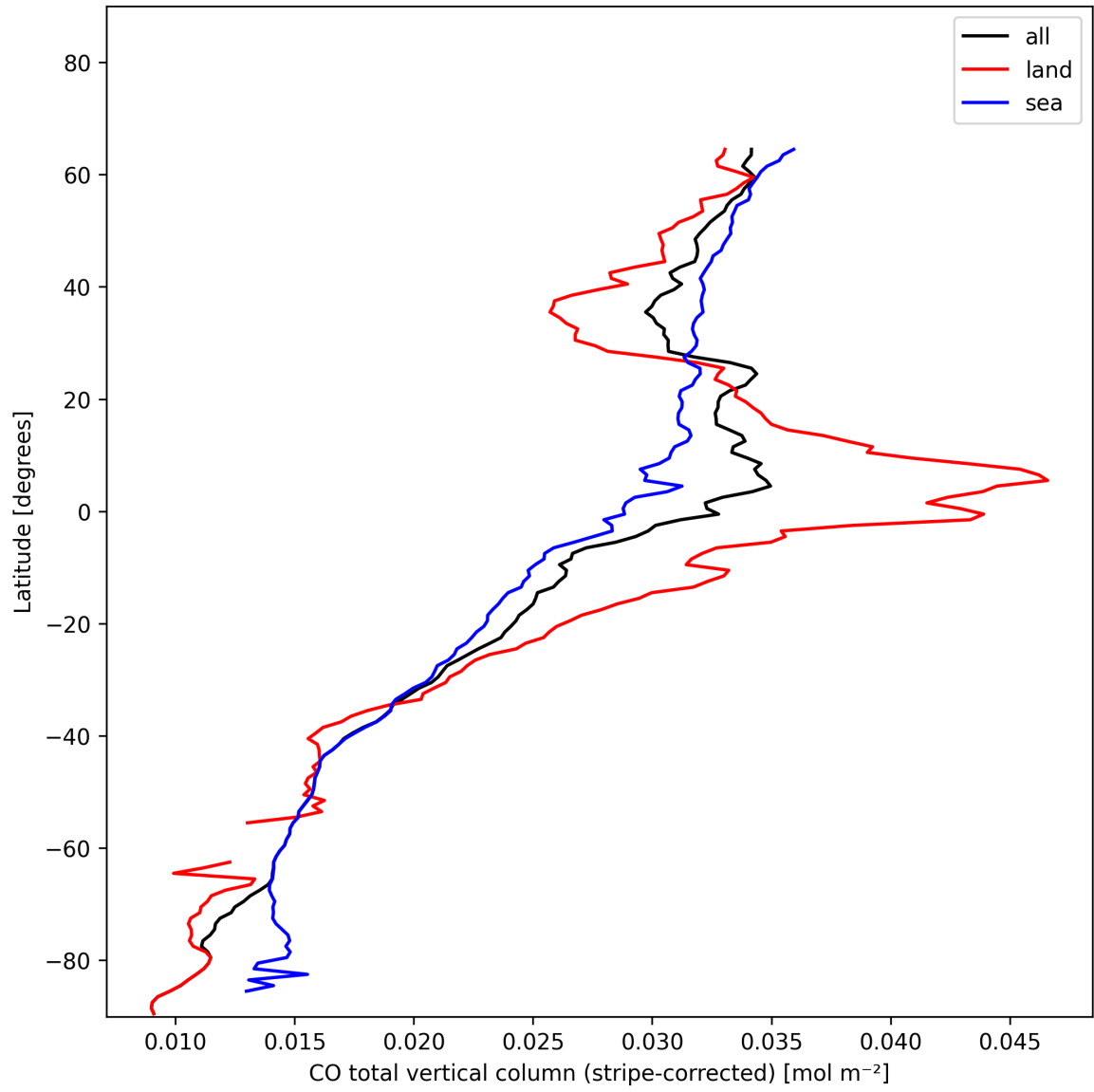
Figure 11: Zonal average of “CO total vertical column (stripe-corrected)” for 2025-01-17 to 2025-01-19.
