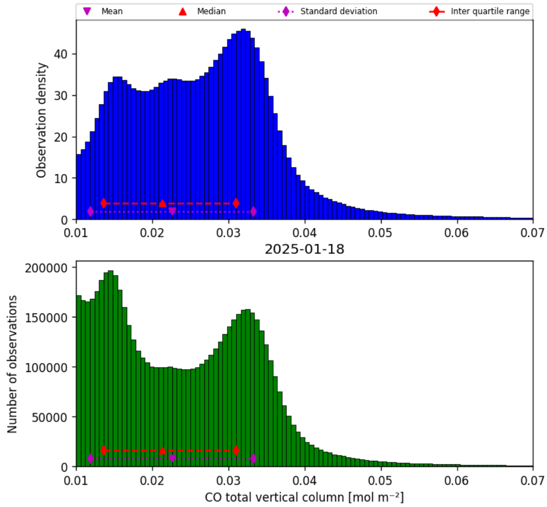
Figure 18: Histogram of “CO total vertical column” for 2025-01-17 to 2025-01-19
