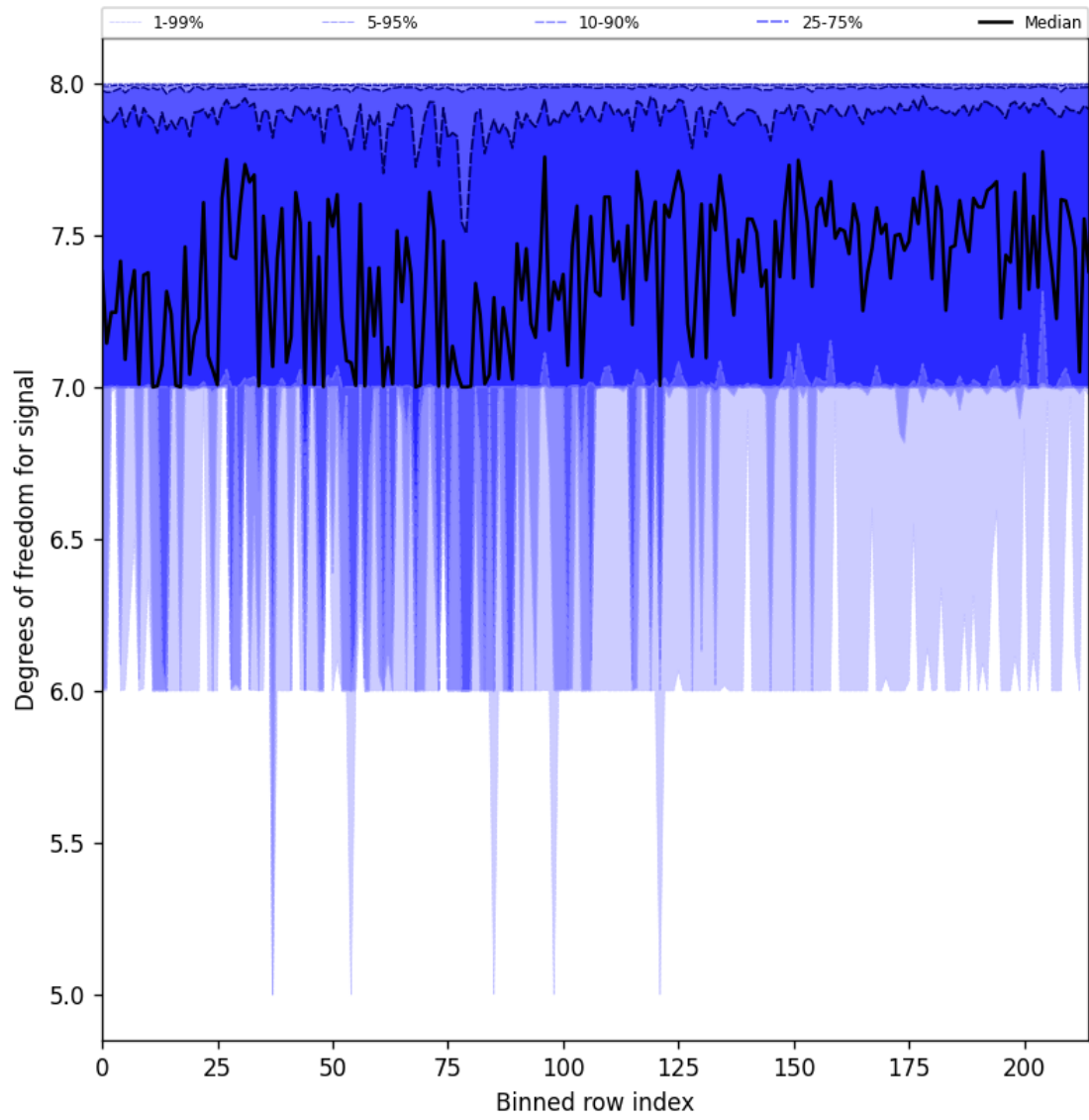
Figure 31: Along track statistics of “Degrees of freedom for signal” for 2025-01-17 to 2025-01-19
