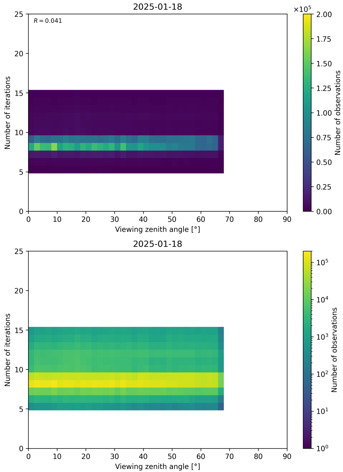
Figure 75: Scatter density plot of “Viewing zenith angle” against “Number of iterations” for 2025-01-17 to 2025-01-19.
