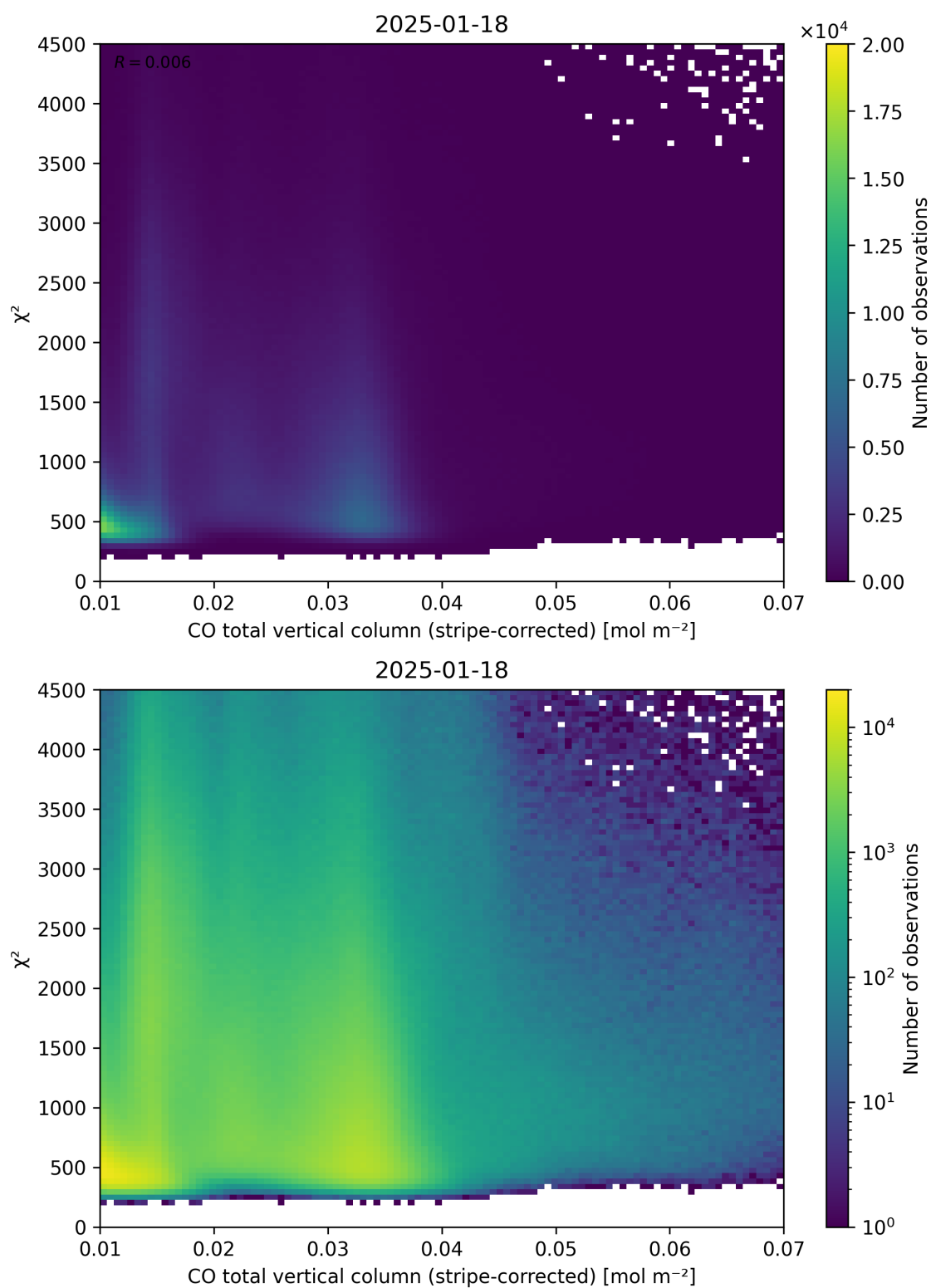
Figure 37: Scatter density plot of “CO total vertical column (stripe-corrected)” against “ \chi^2 ” for 2025-01-17 to 2025-01-19.
