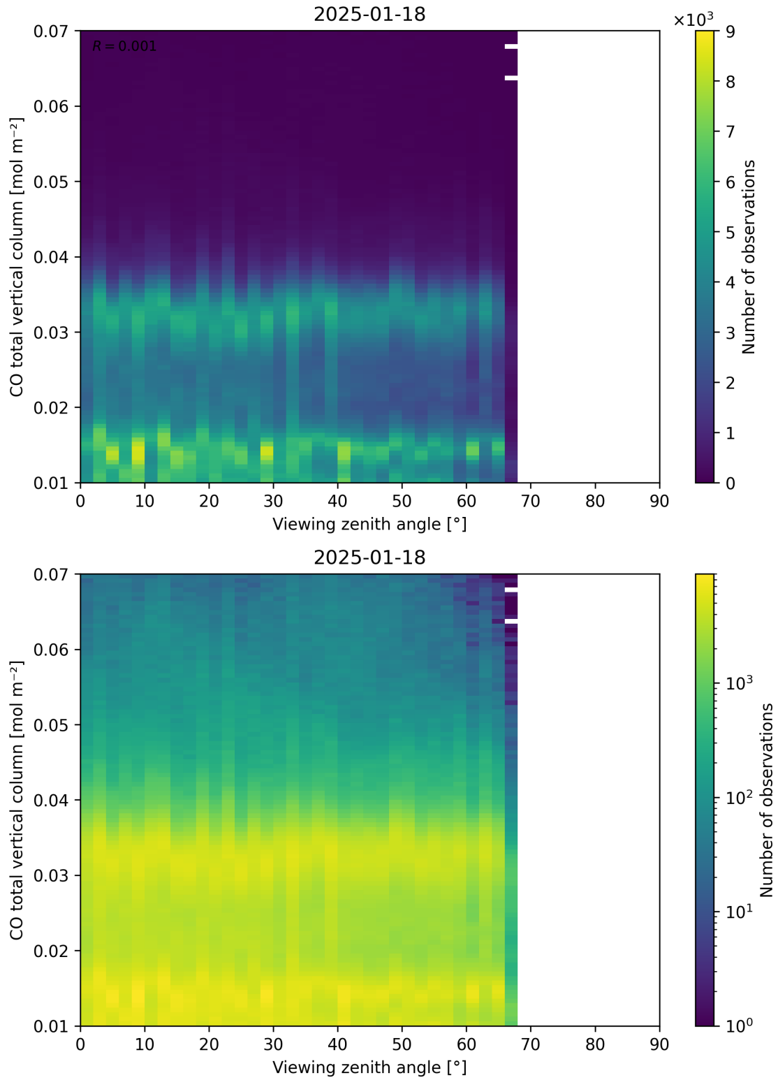
Figure 69: Scatter density plot of “Viewing zenith angle” against “CO total vertical column” for 2025-01-17 to 2025-01-19.
