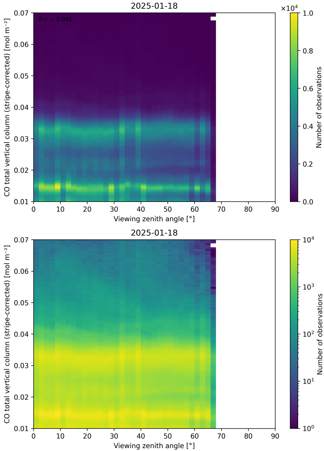
Figure 70: Scatter density plot of “Viewing zenith angle” against “CO total vertical column (stripe-corrected)” for 2025-01-17 to 2025-01-19.
