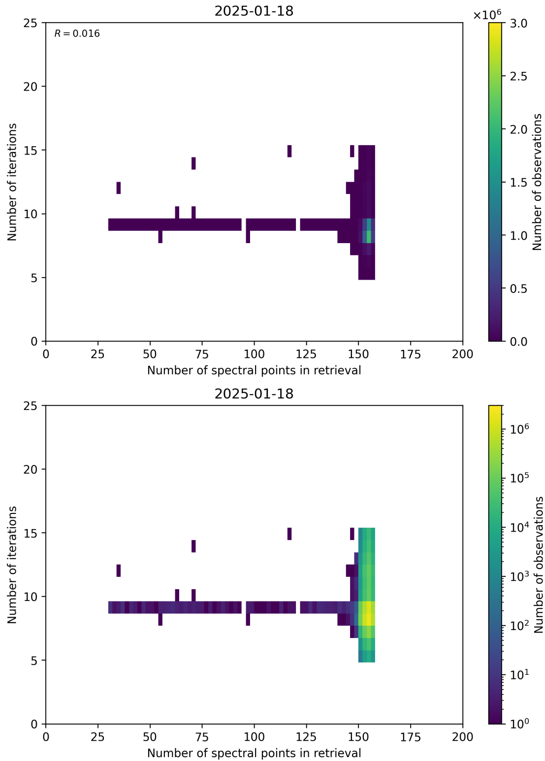
Figure 60: Scatter density plot of “Number of spectral points in retrieval” against “Number of iterations” for 2025-01-17 to 2025-01-19.
