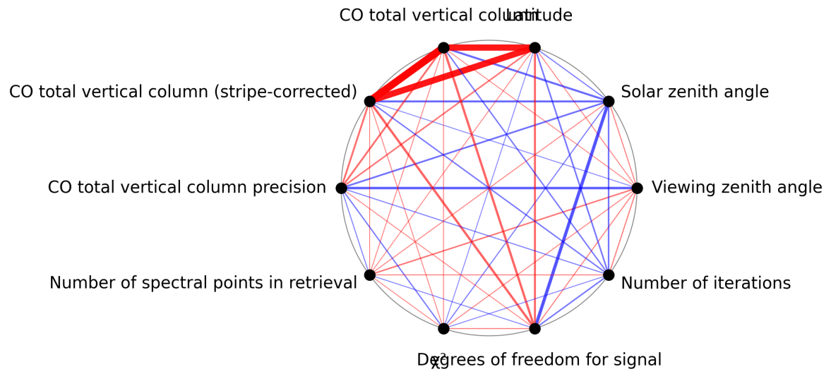
Figure 1: Map of correlation graph for 2025-01-17 to 2025-01-19.
