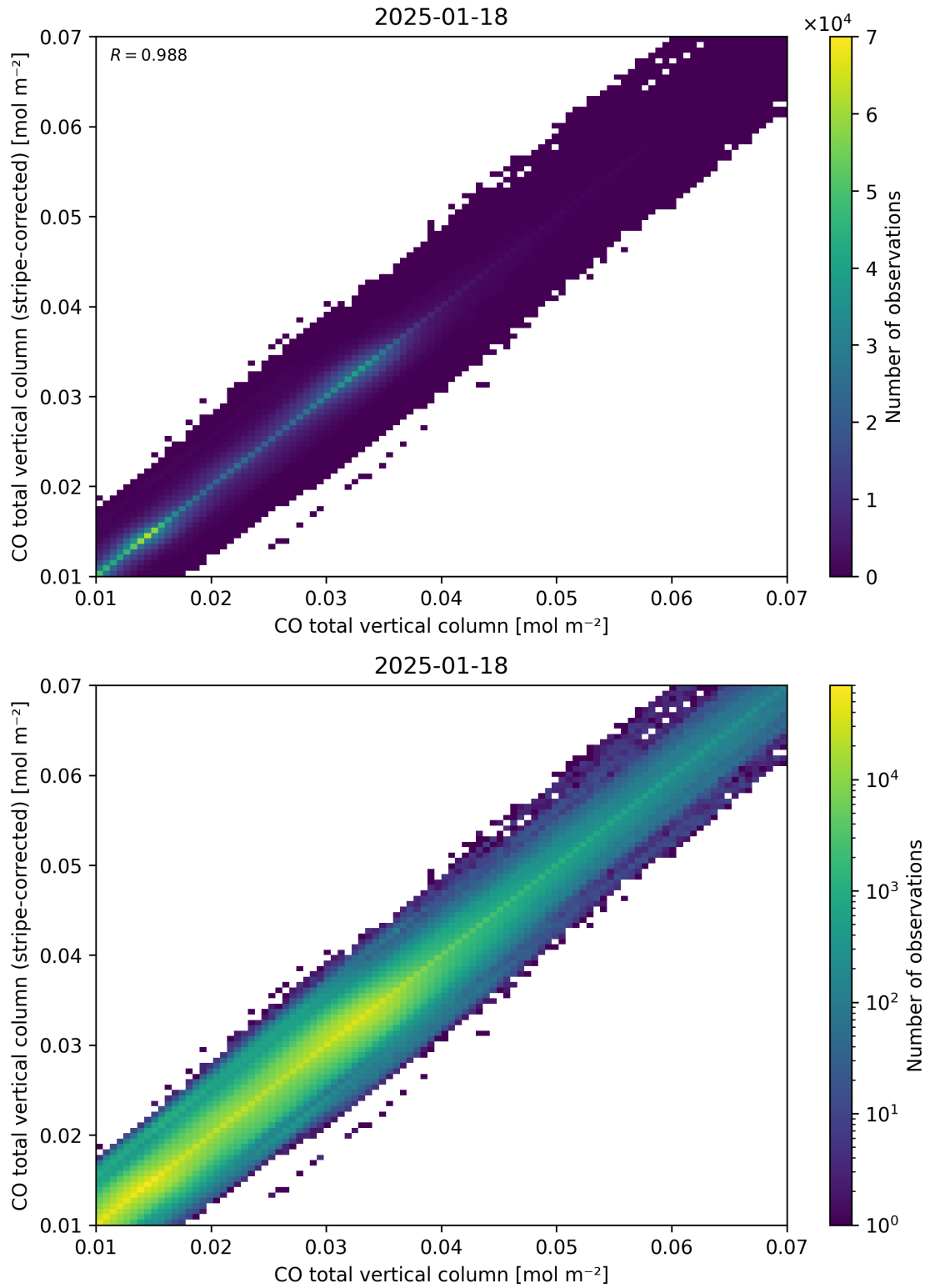
Figure 33: Scatter density plot of “CO total vertical column” against “CO total vertical column (stripe-corrected)” for 2025-01-17 to 2025-01-19.
