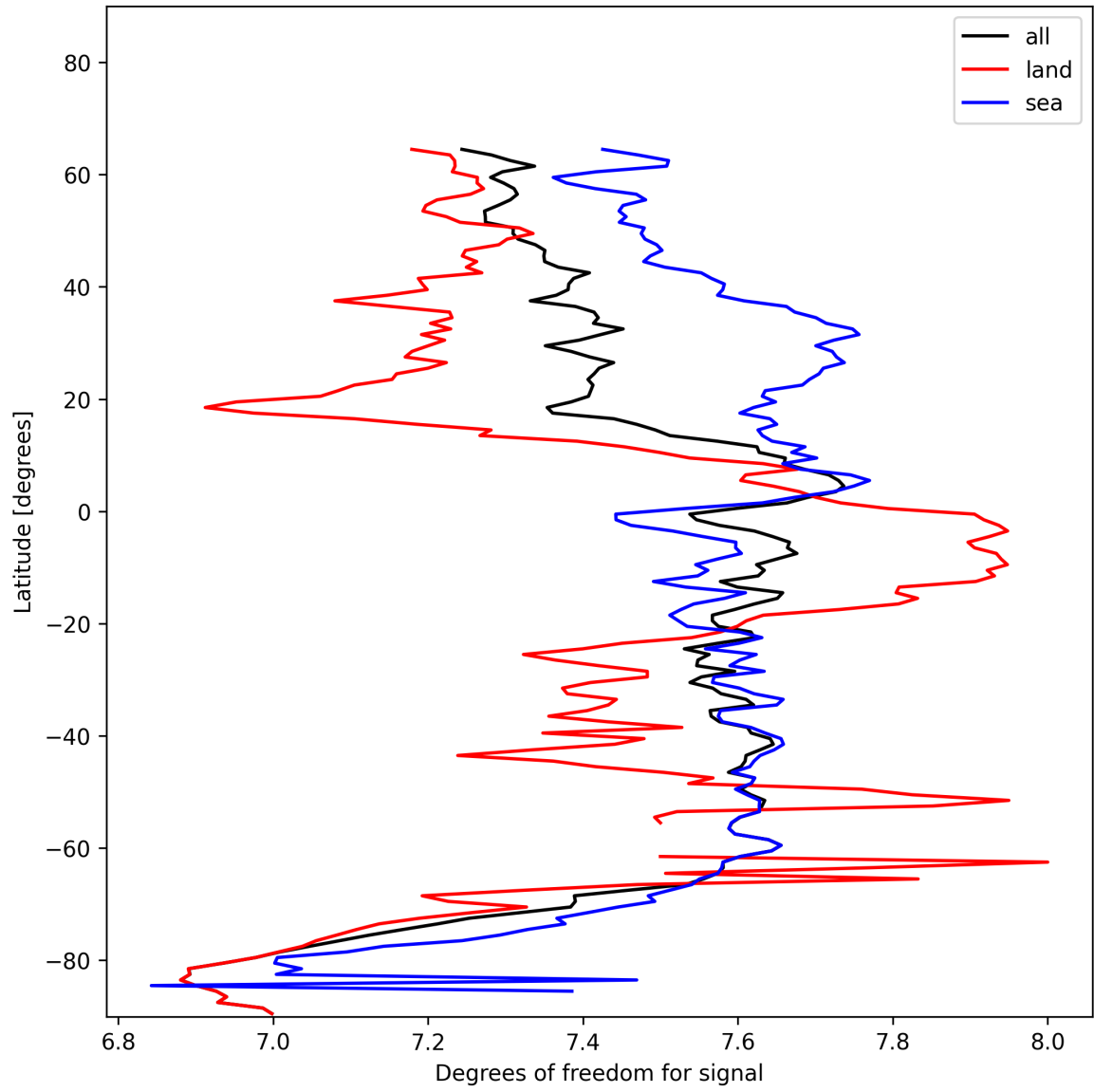
Figure 15: Zonal average of “Degrees of freedom for signal” for 2025-01-18 to 2025-01-20.
