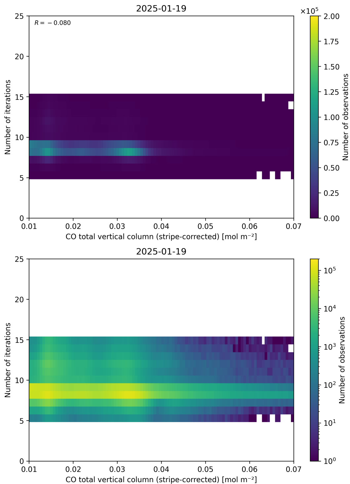
Figure 39: Scatter density plot of “CO total vertical column (stripe-corrected)” against “Number of iterations” for 2025-01-18 to 2025-01-20.
