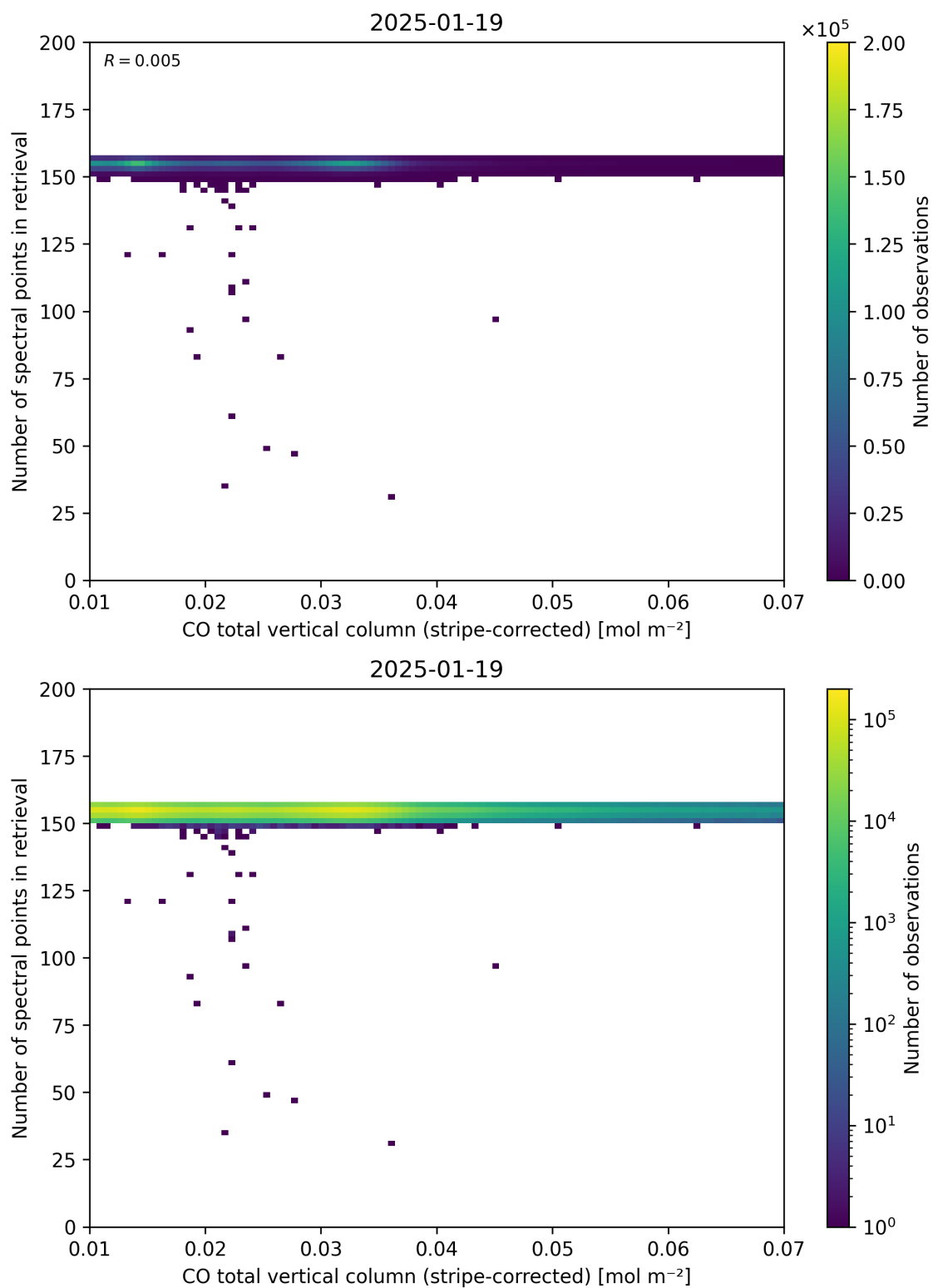
Figure 40: Scatter density plot of “CO total vertical column (stripe-corrected)” against “Number of spectral points in retrieval” for 2025-01-18 to 2025-01-20.
