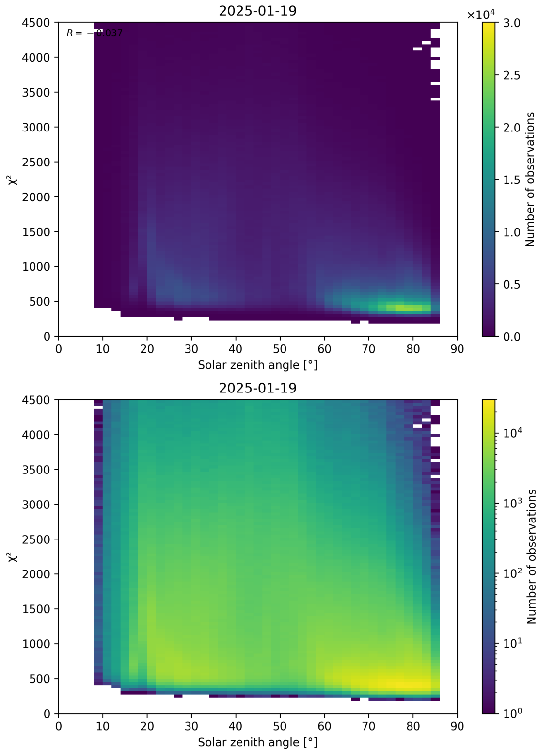
Figure 64: Scatter density plot of “Solar zenith angle” against “ \chi^2 ” for 2025-01-18 to 2025-01-20.
