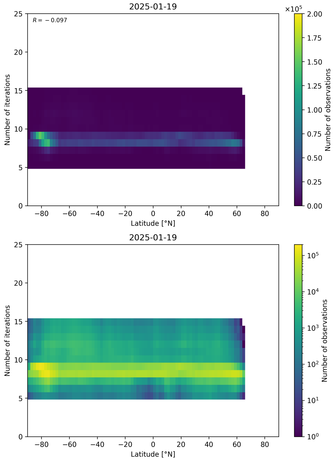
Figure 56: Scatter density plot of “Latitude” against “Number of iterations” for 2025-01-18 to 2025-01-20.
