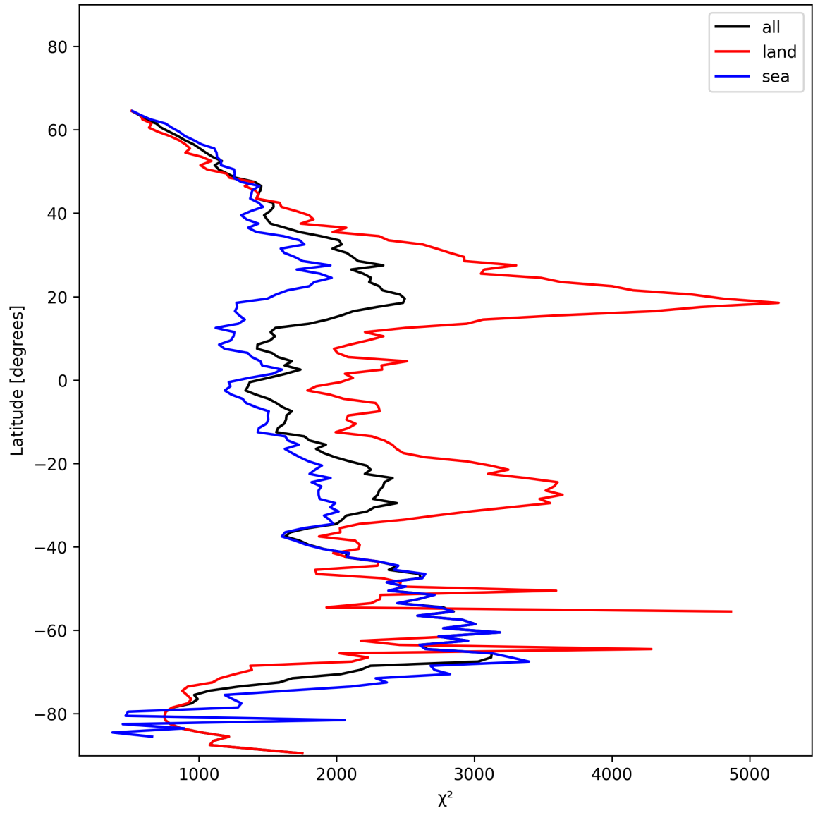
Figure 14: Zonal average of “ \chi^2 ” for 2025-01-18 to 2025-01-20.
