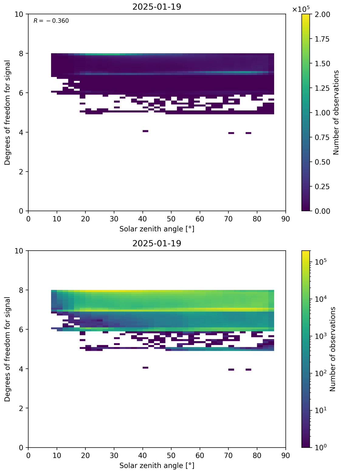
Figure 65: Scatter density plot of “Solar zenith angle” against “Degrees of freedom for signal” for 2025-01-18 to 2025-01-20.
