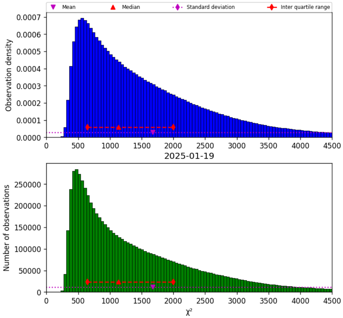
Figure 22: Histogram of “ \chi^2 ” for 2025-01-18 to 2025-01-20
