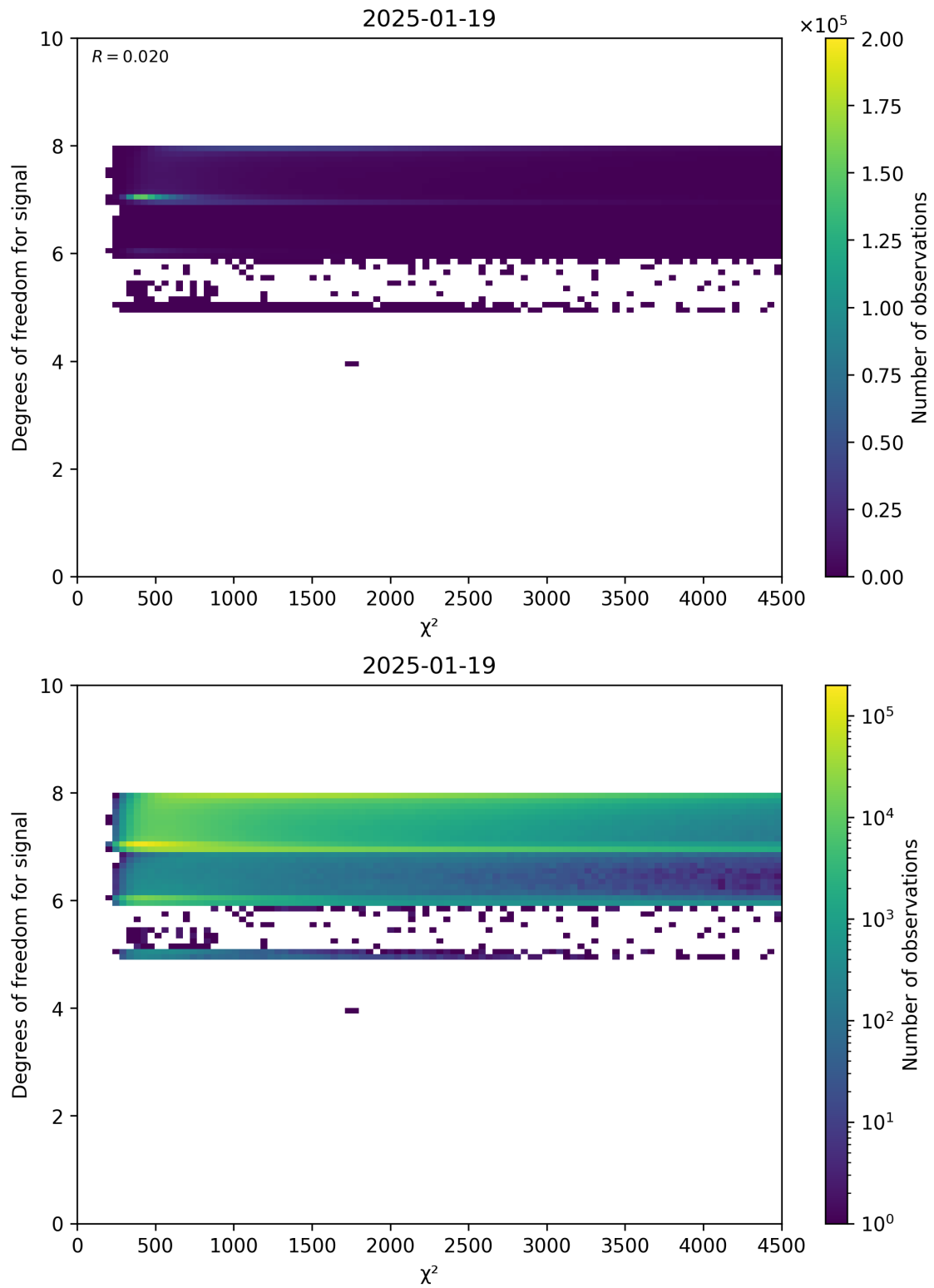
Figure 48: Scatter density plot of “ \chi^2 ” against “Degrees of freedom for signal” for 2025-01-18 to 2025-01-20.
