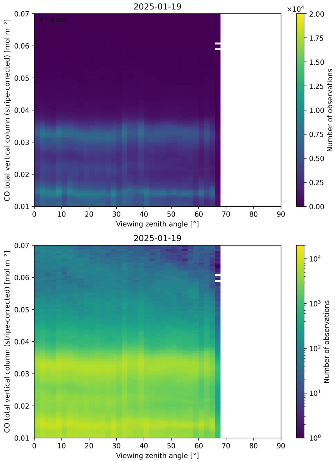
Figure 70: Scatter density plot of “Viewing zenith angle” against “CO total vertical column (stripe-corrected)” for 2025-01-18 to 2025-01-20.
