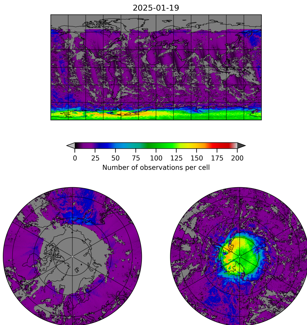
Figure 8: Map of the number of observations for 2025-01-18 to 2025-01-20
