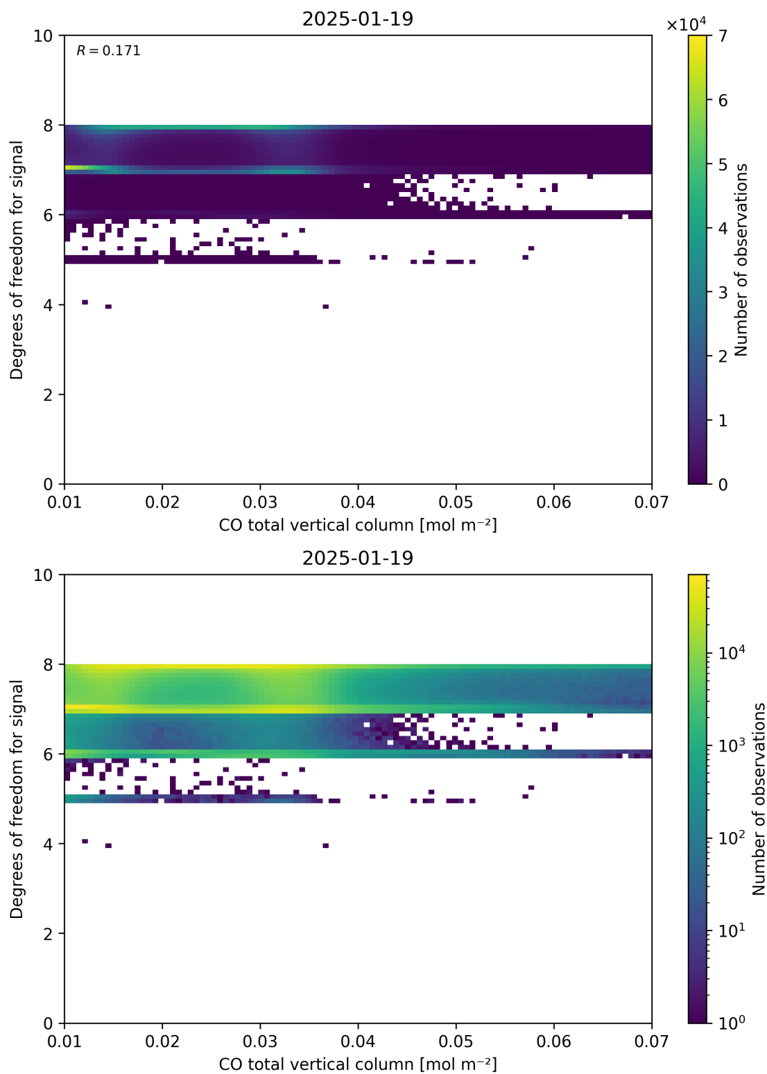
Figure 41: Scatter density plot of “CO total vertical column” against “Degrees of freedom for signal” for 2025-01-18 to 2025-01-20.
