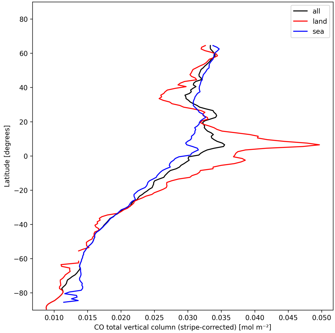
Figure 11: Zonal average of “CO total vertical column (stripe-corrected)” for 2025-01-18 to 2025-01-20.
