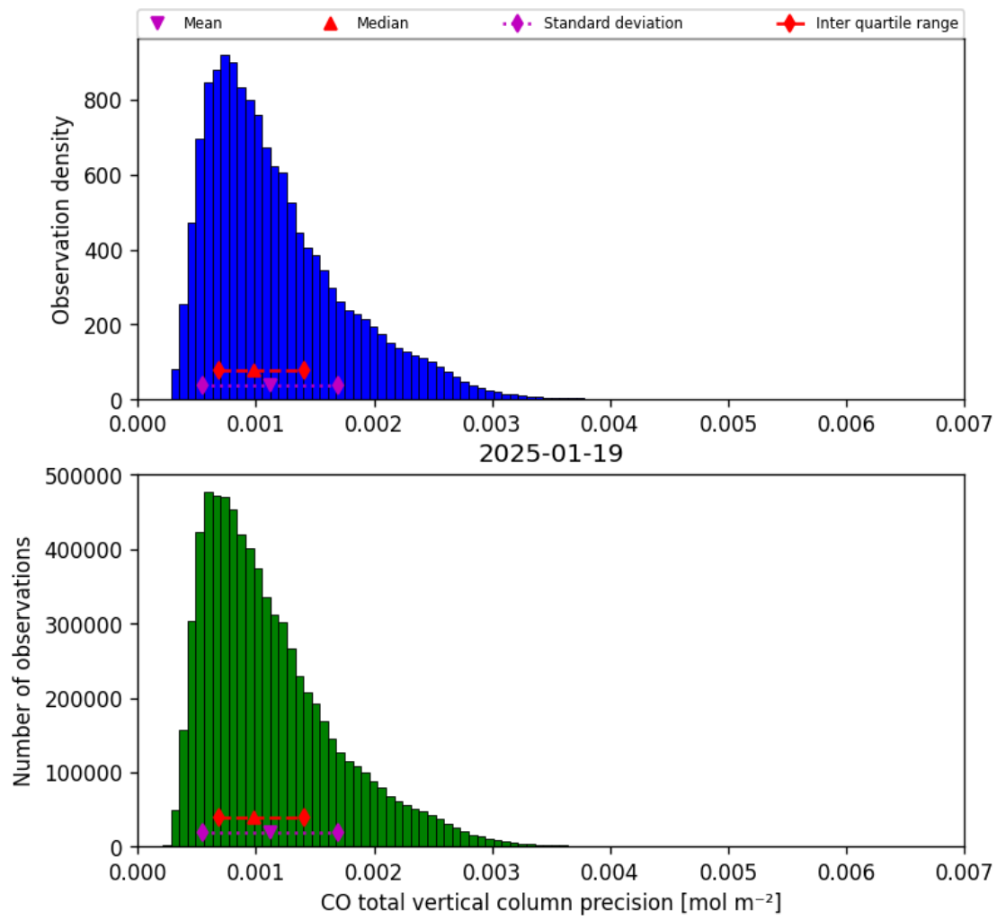
Figure 20: Histogram of “CO total vertical column precision” for 2025-01-18 to 2025-01-20
