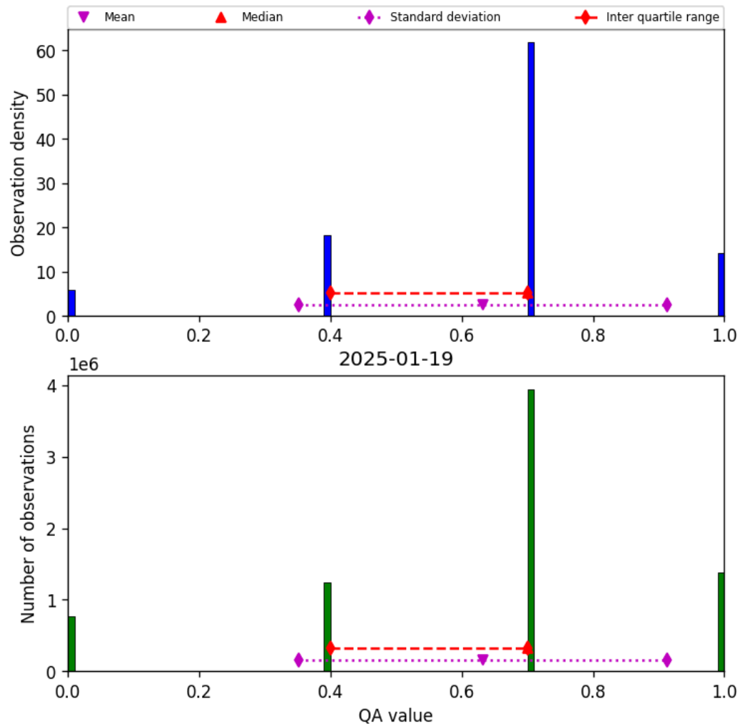
Figure 17: Histogram of “QA value” for 2025-01-18 to 2025-01-20
