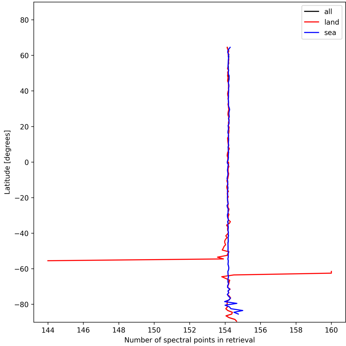
Figure 13: Zonal average of “Number of spectral points in retrieval” for 2025-01-18 to 2025-01-20.
