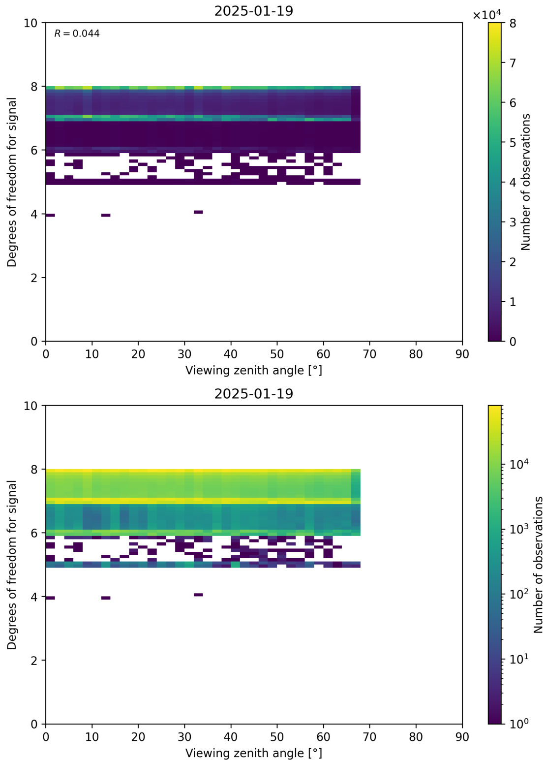
Figure 73: Scatter density plot of “Viewing zenith angle” against “Degrees of freedom for signal” for 2025-01-18 to 2025-01-20.
