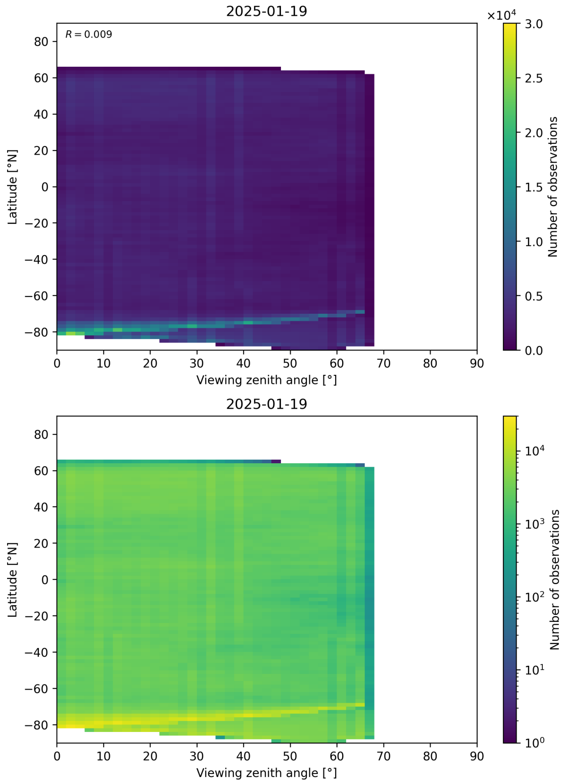
Figure 74: Scatter density plot of “Viewing zenith angle” against “Latitude” for 2025-01-18 to 2025-01-20.
