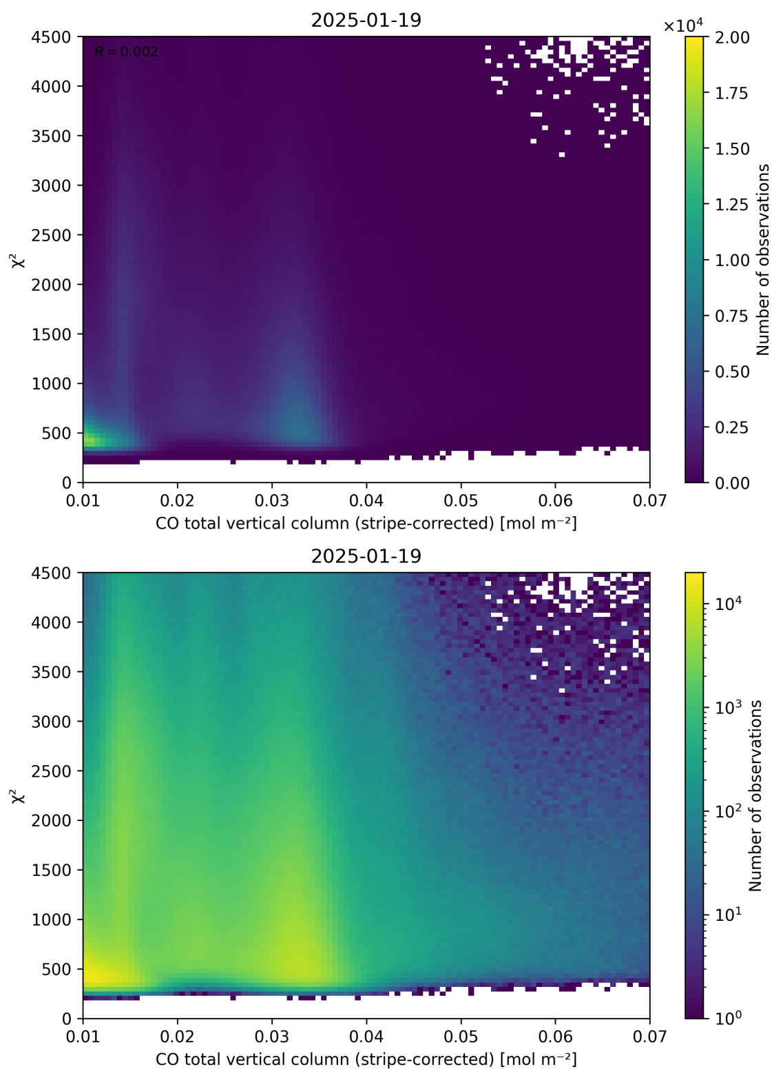
Figure 37: Scatter density plot of “CO total vertical column (stripe-corrected)” against “ \chi^2 ” for 2025-01-18 to 2025-01-20.
