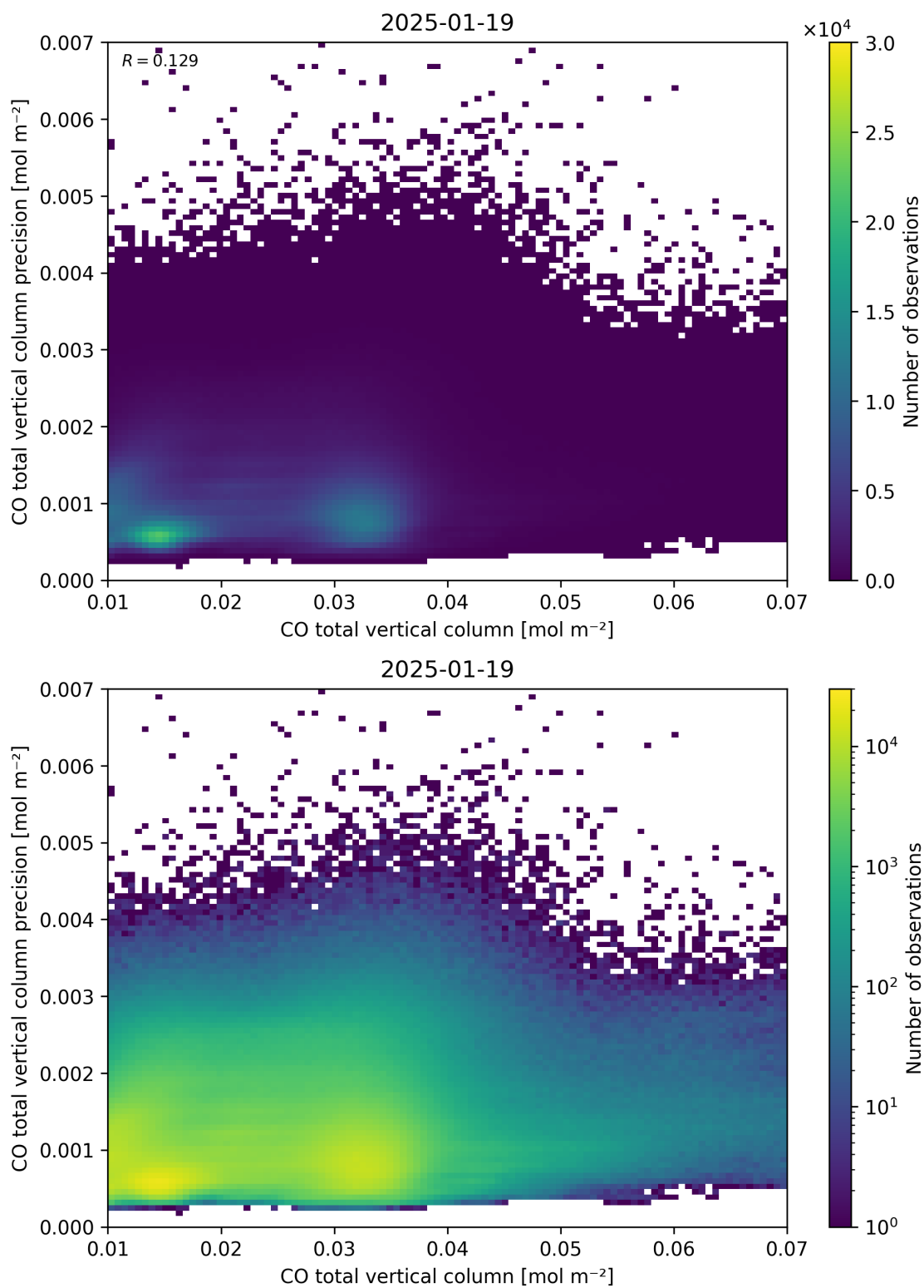
Figure 34: Scatter density plot of “CO total vertical column” against “CO total vertical column precision” for 2025-01-18 to 2025-01-20.
