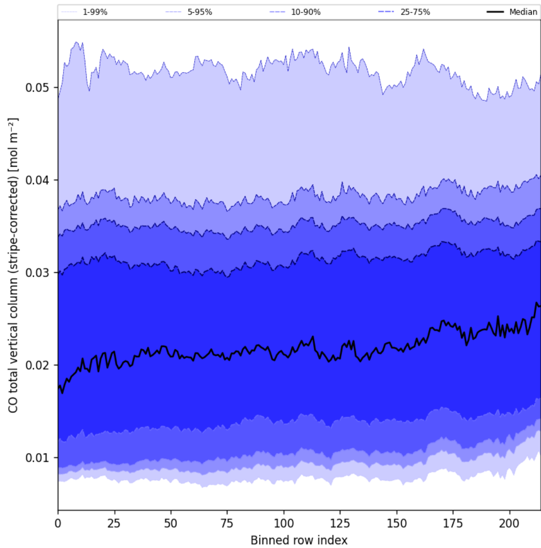
Figure 27: Along track statistics of “CO total vertical column (stripe-corrected)” for 2025-01-18 to 2025-01-20
