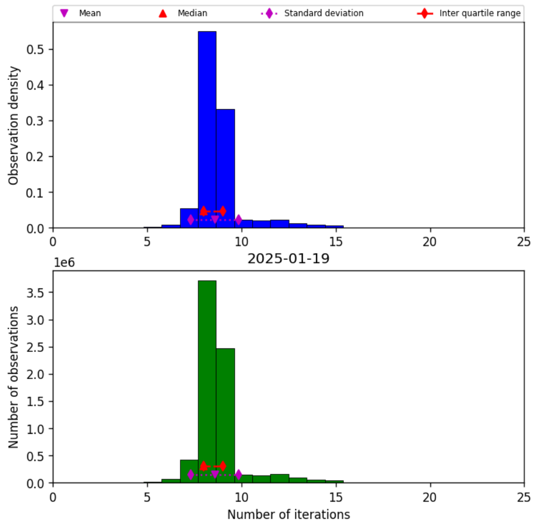
Figure 24: Histogram of “Number of iterations” for 2025-01-18 to 2025-01-20
