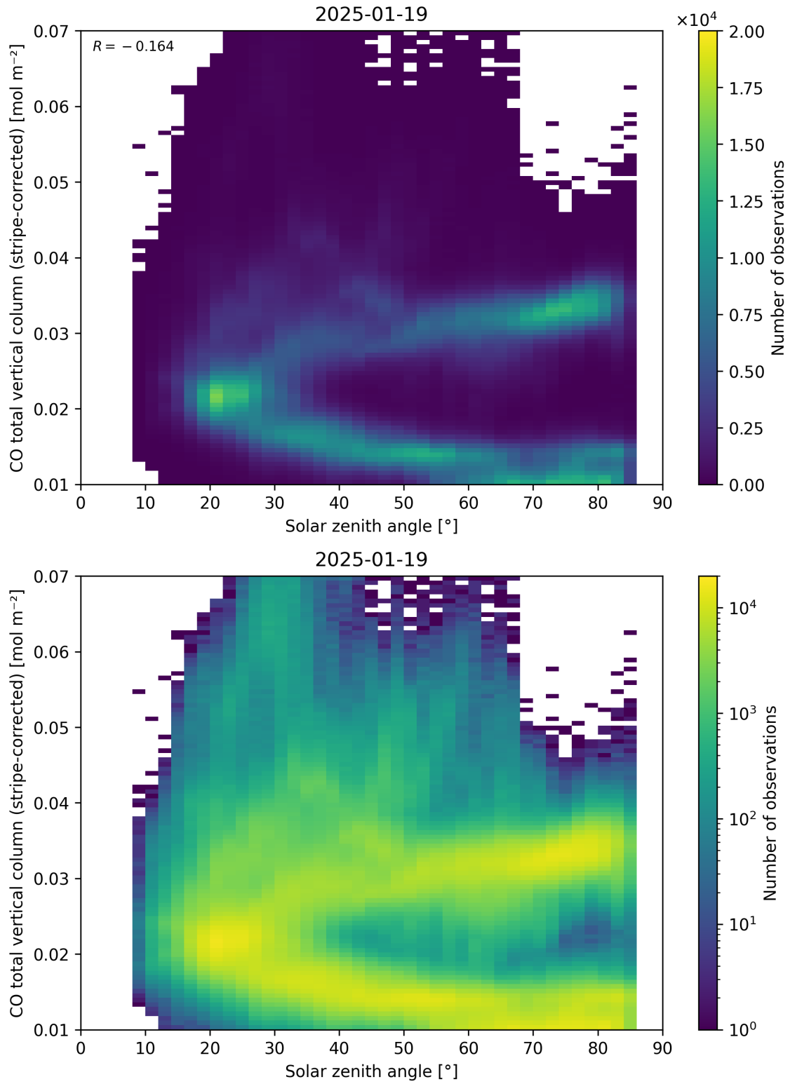
Figure 62: Scatter density plot of “Solar zenith angle” against “CO total vertical column (stripe-corrected)” for 2025-01-18 to 2025-01-20.
