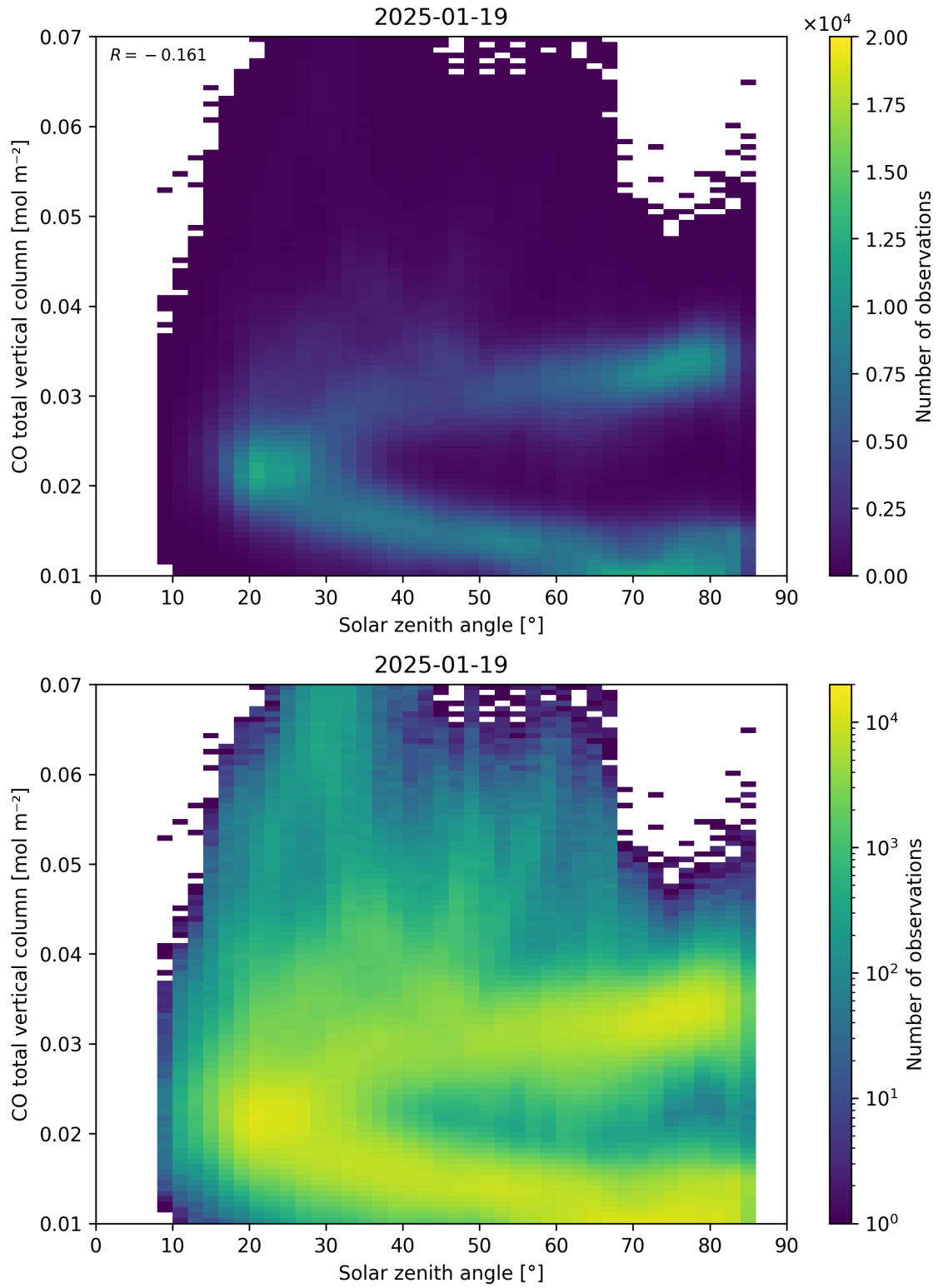
Figure 61: Scatter density plot of “Solar zenith angle” against “CO total vertical column” for 2025-01-18 to 2025-01-20.
