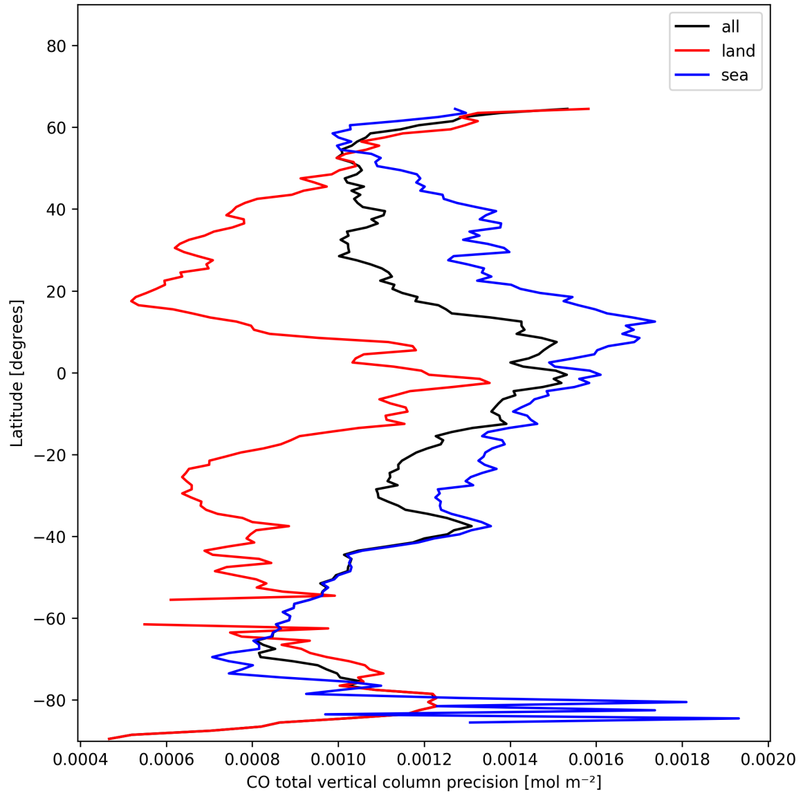
Figure 12: Zonal average of “CO total vertical column precision” for 2025-01-18 to 2025-01-20.
