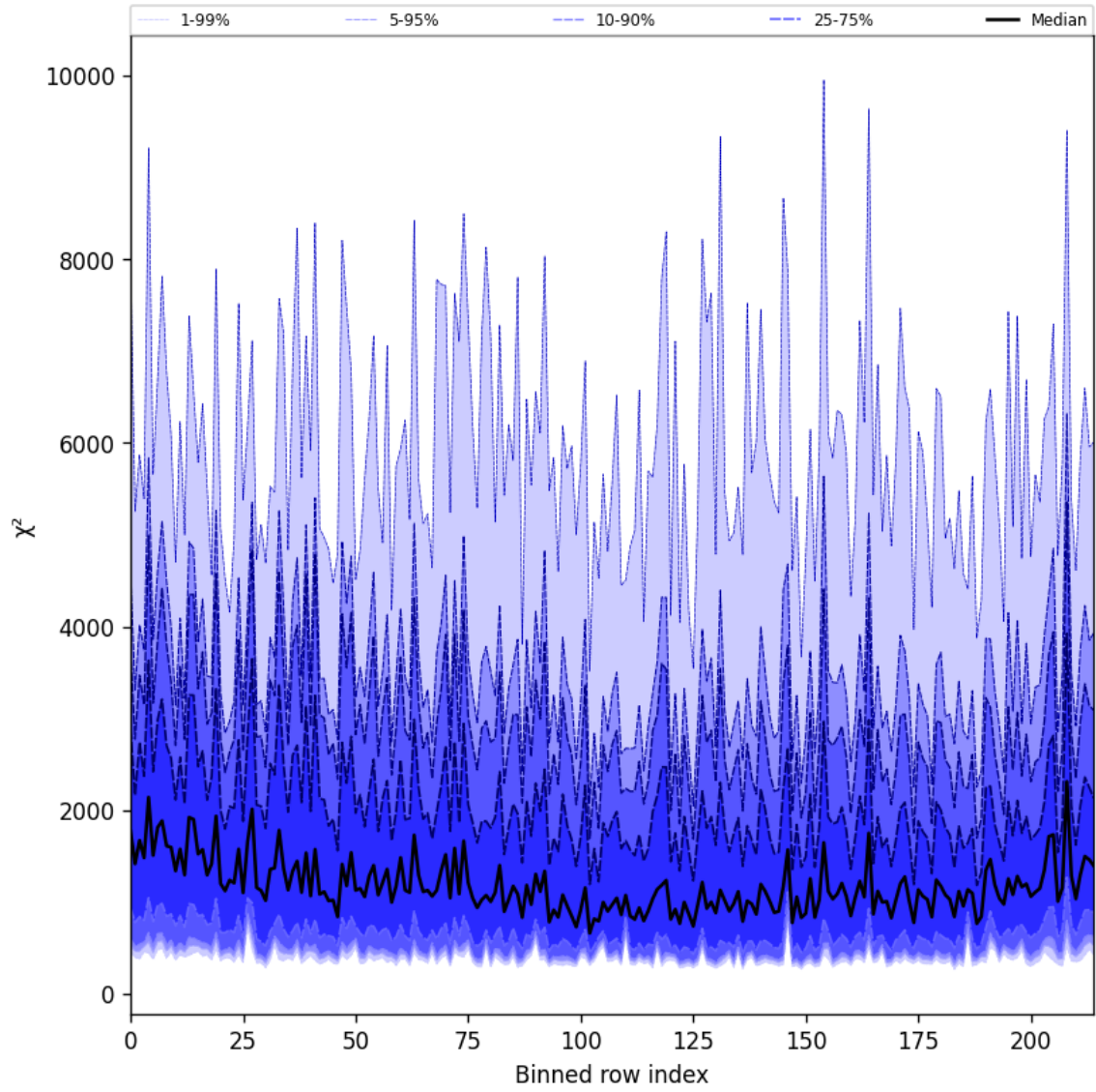
Figure 30: Along track statistics of “ \chi^2 ” for 2025-01-18 to 2025-01-20
