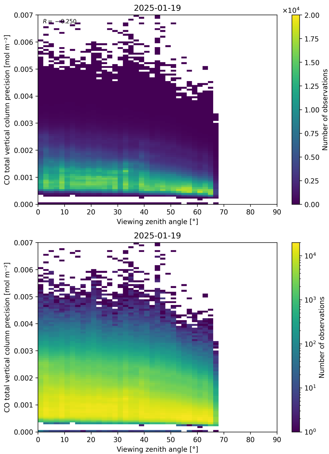
Figure 71: Scatter density plot of “Viewing zenith angle” against “CO total vertical column precision” for 2025-01-18 to 2025-01-20.
