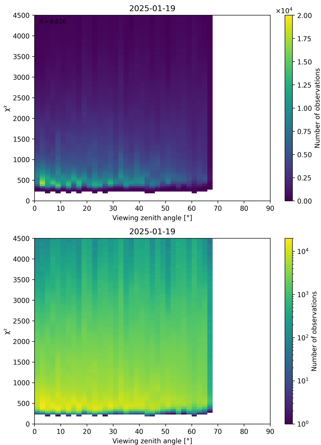
Figure 72: Scatter density plot of “Viewing zenith angle” against “ \chi^2 ” for 2025-01-18 to 2025-01-20.
