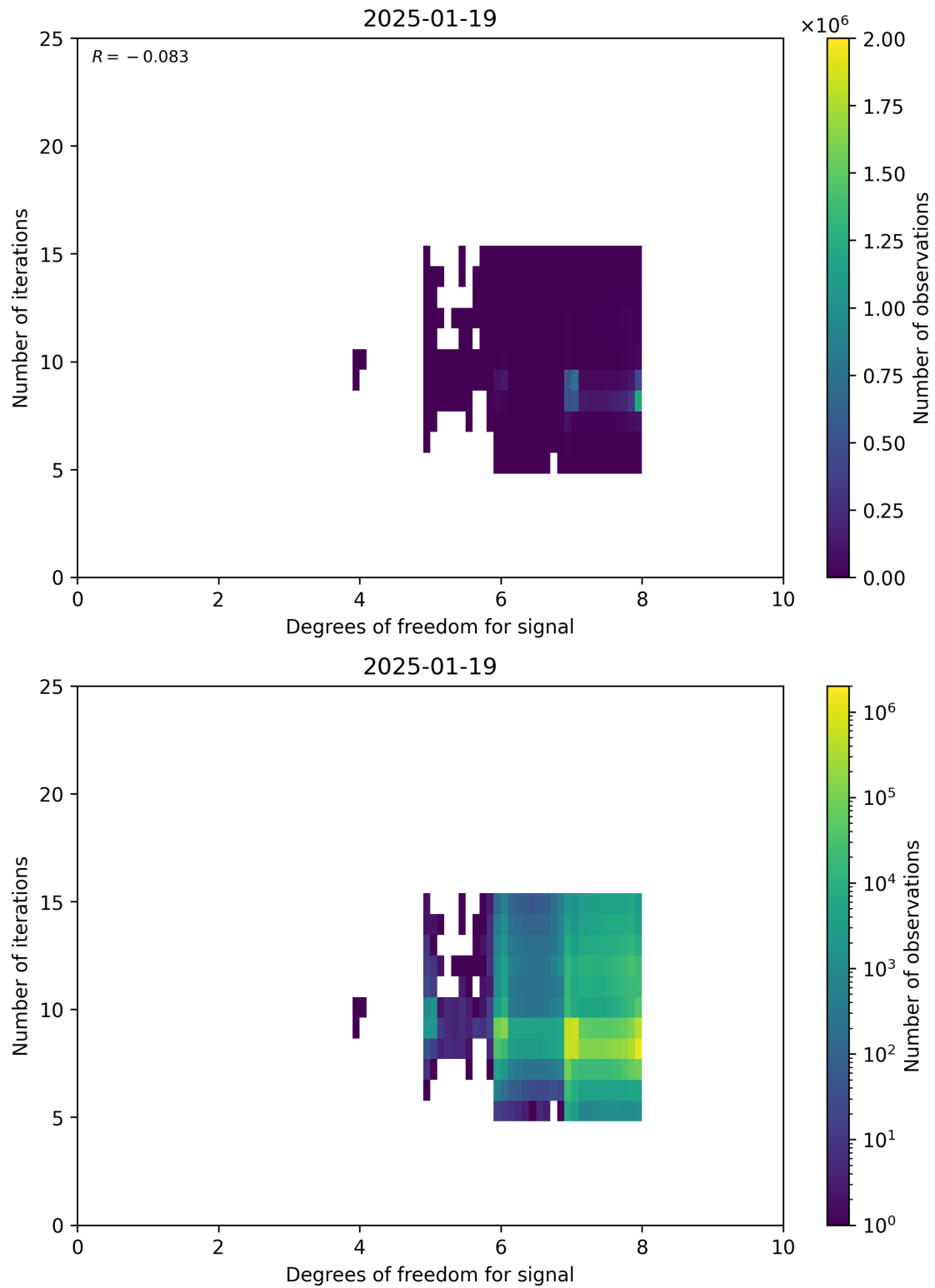
Figure 50: Scatter density plot of “Degrees of freedom for signal” against “Number of iterations” for 2025-01-18 to 2025-01-20.
