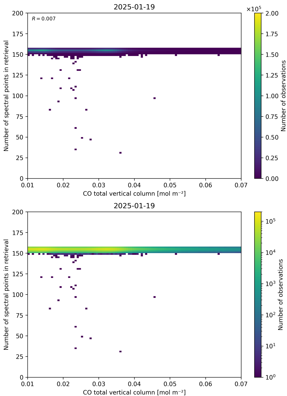
Figure 43: Scatter density plot of “CO total vertical column” against “Number of spectral points in retrieval” for 2025-01-18 to 2025-01-20.
