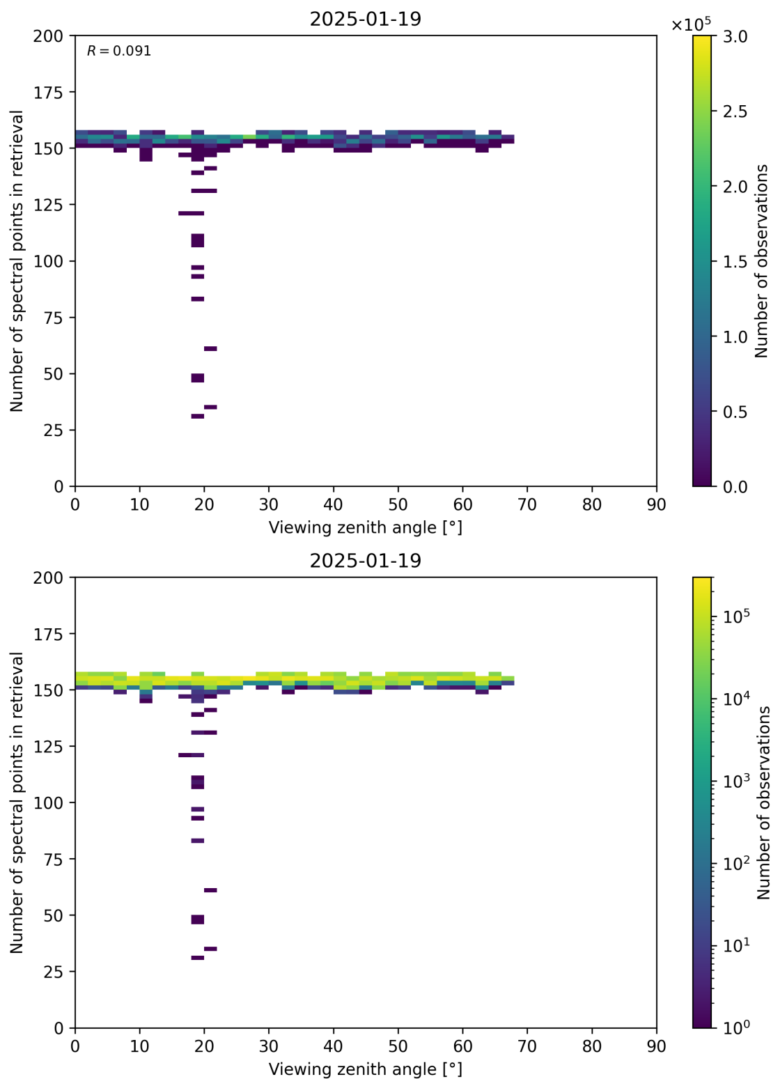
Figure 76: Scatter density plot of “Viewing zenith angle” against “Number of spectral points in retrieval” for 2025-01-18 to 2025-01-20.
