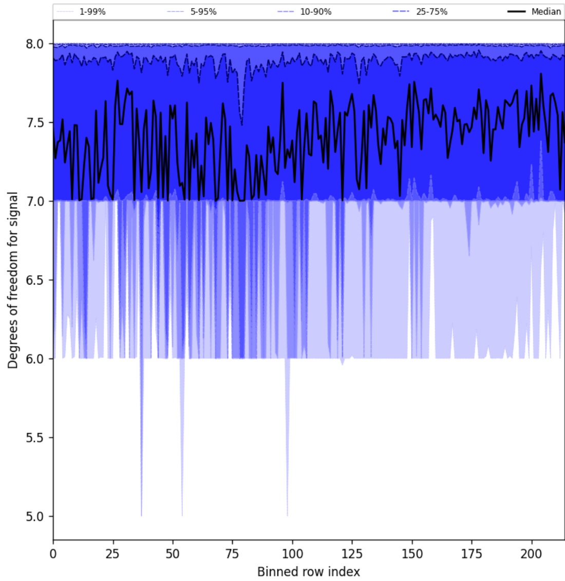
Figure 31: Along track statistics of “Degrees of freedom for signal” for 2025-01-18 to 2025-01-20
