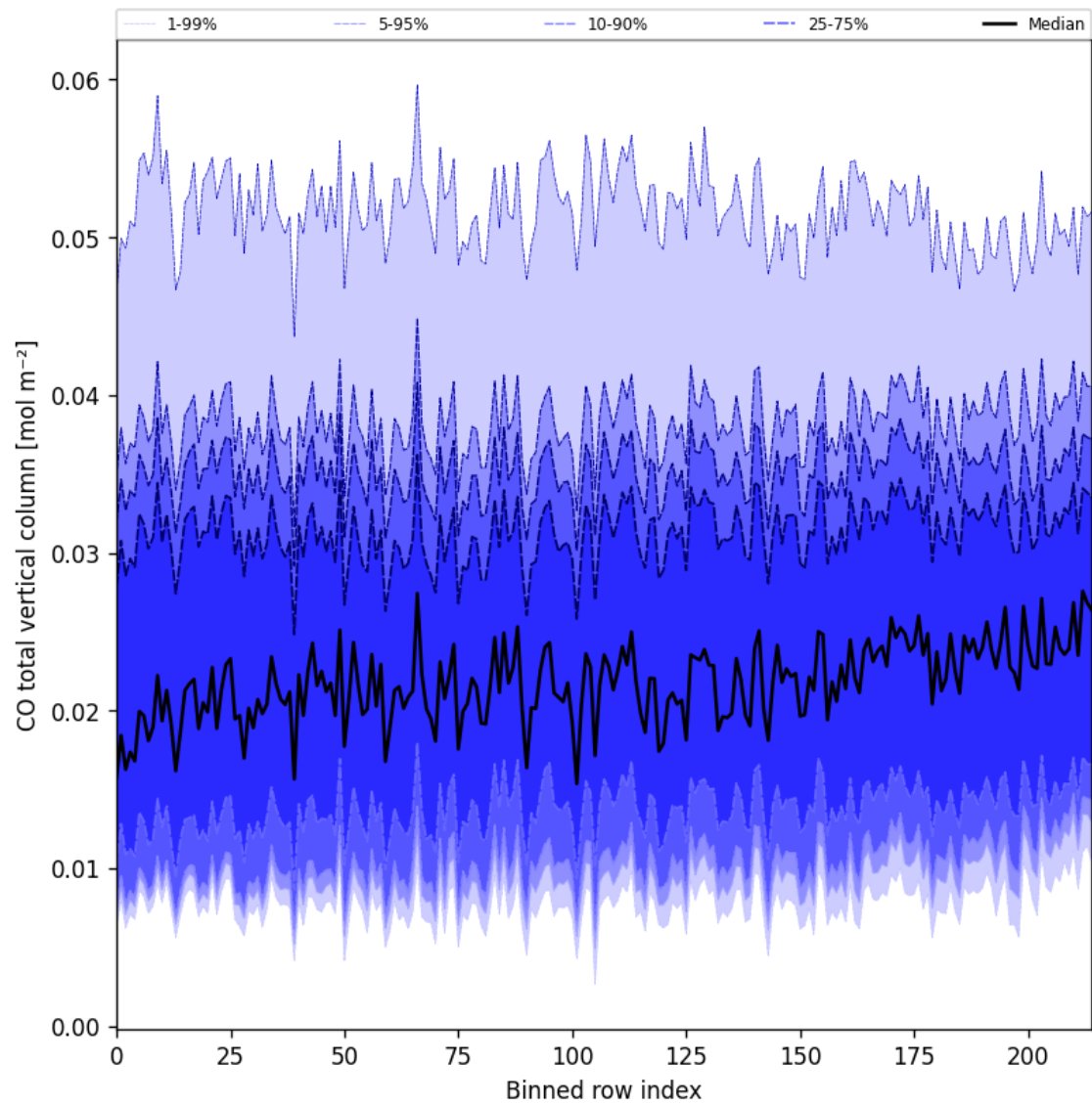
Figure 26: Along track statistics of “CO total vertical column” for 2025-01-18 to 2025-01-20
