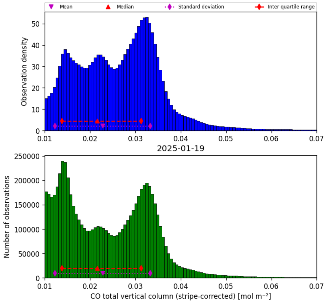
Figure 19: Histogram of “CO total vertical column (stripe-corrected)” for 2025-01-18 to 2025-01-20
