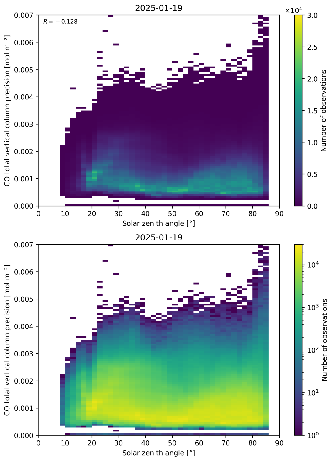
Figure 63: Scatter density plot of “Solar zenith angle” against “CO total vertical column precision” for 2025-01-18 to 2025-01-20.
