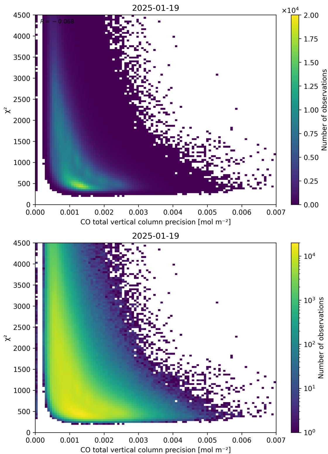
Figure 44: Scatter density plot of “CO total vertical column precision” against “ \chi^2 ” for 2025-01-18 to 2025-01-20.
