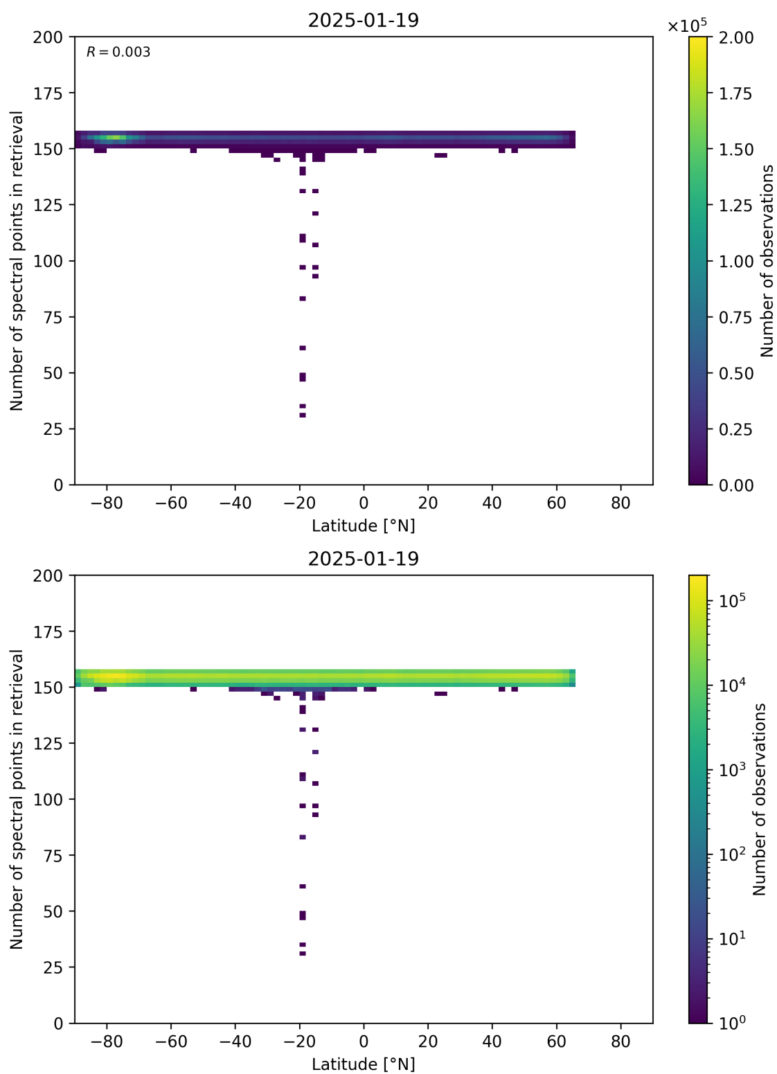
Figure 57: Scatter density plot of “Latitude” against “Number of spectral points in retrieval” for 2025-01-18 to 2025-01-20.
