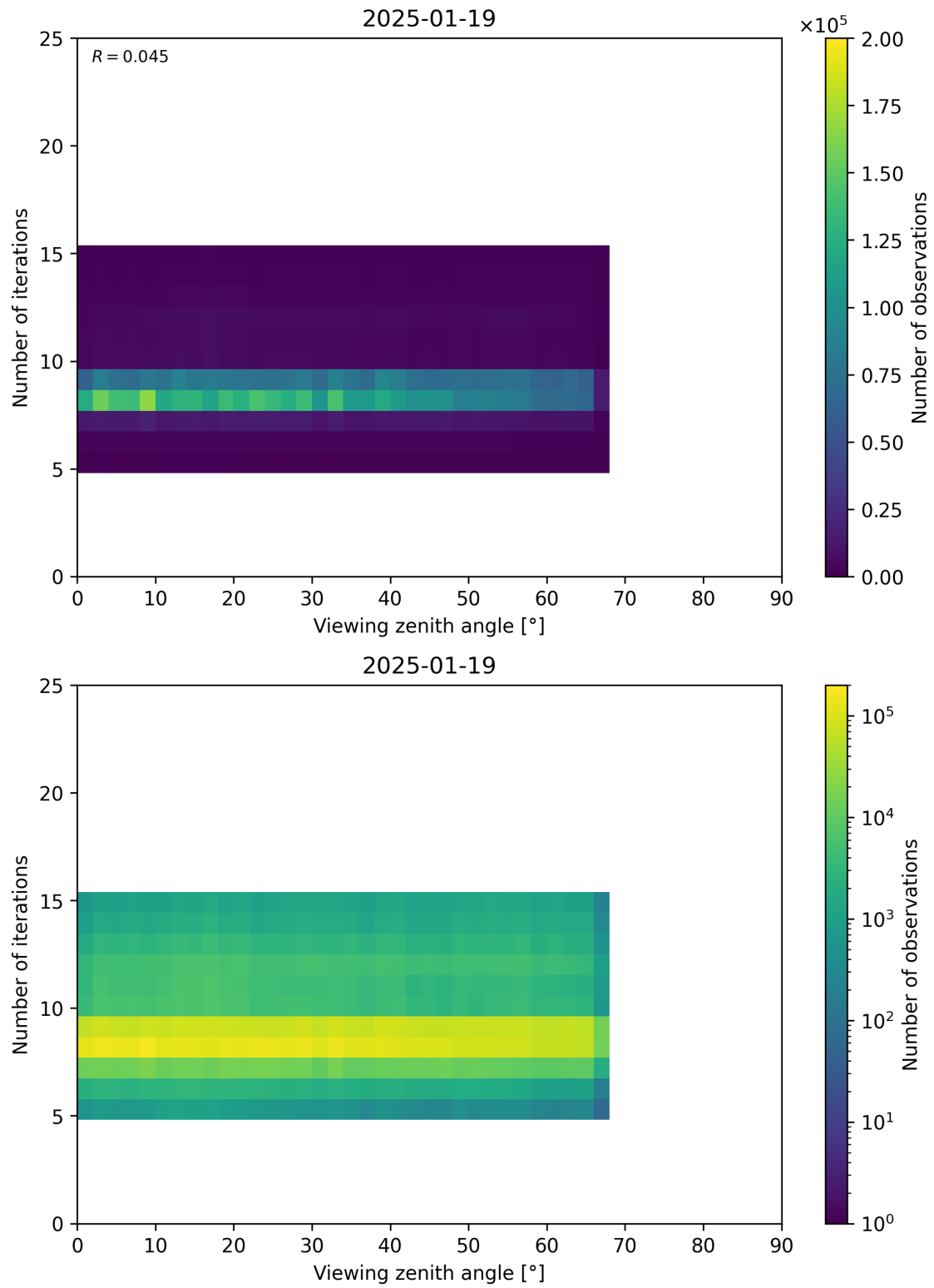
Figure 75: Scatter density plot of “Viewing zenith angle” against “Number of iterations” for 2025-01-18 to 2025-01-20.
