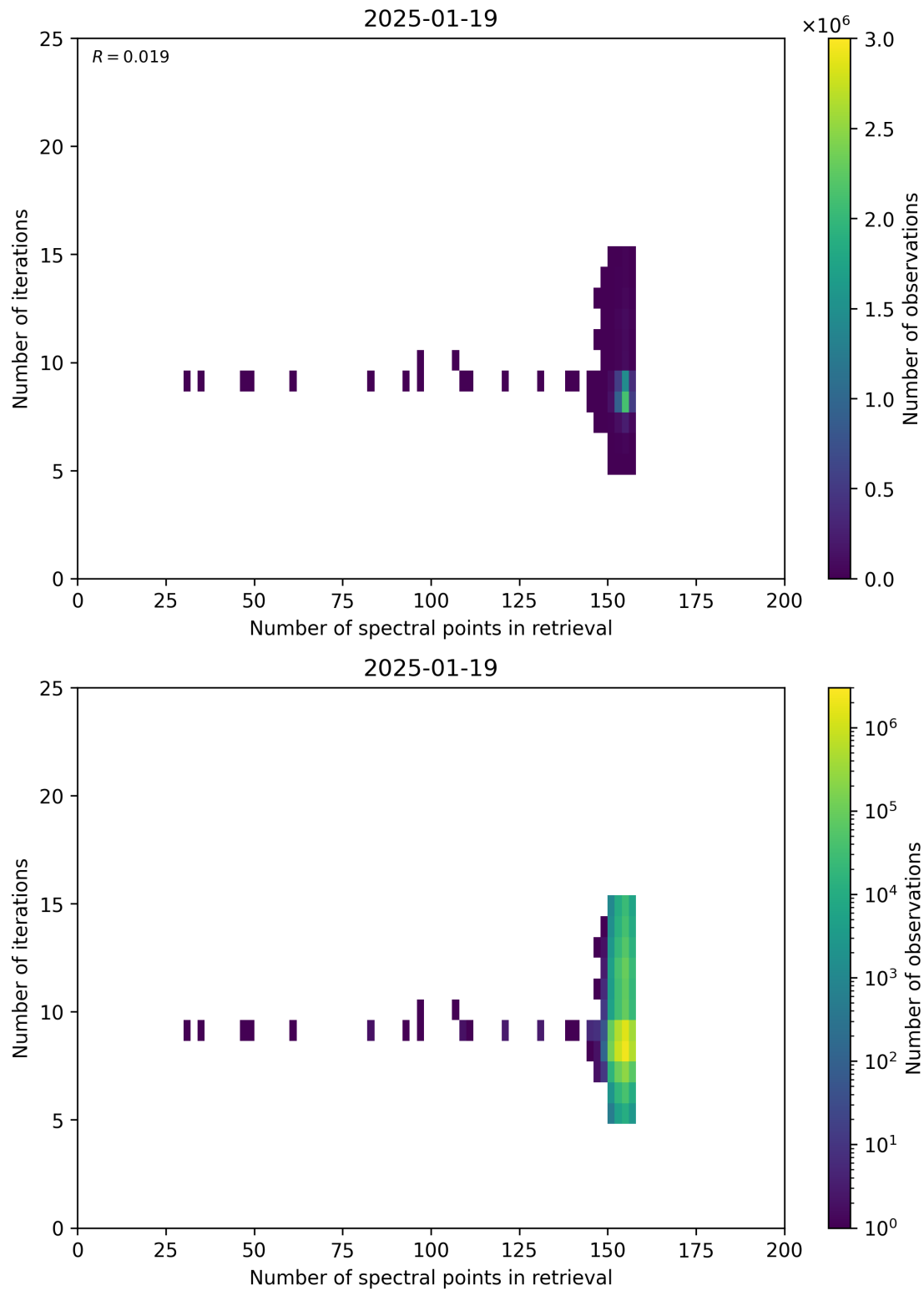
Figure 60: Scatter density plot of “Number of spectral points in retrieval” against “Number of iterations” for 2025-01-18 to 2025-01-20.
