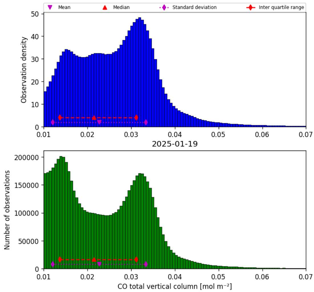
Figure 18: Histogram of “CO total vertical column” for 2025-01-18 to 2025-01-20
