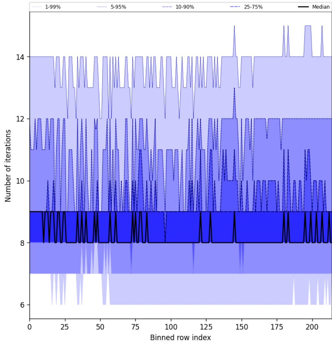
Figure 32: Along track statistics of “Number of iterations” for 2025-01-18 to 2025-01-20
