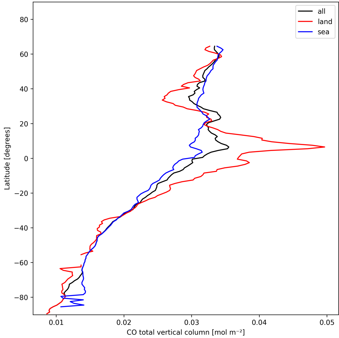
Figure 10: Zonal average of “CO total vertical column” for 2025-01-18 to 2025-01-20.
