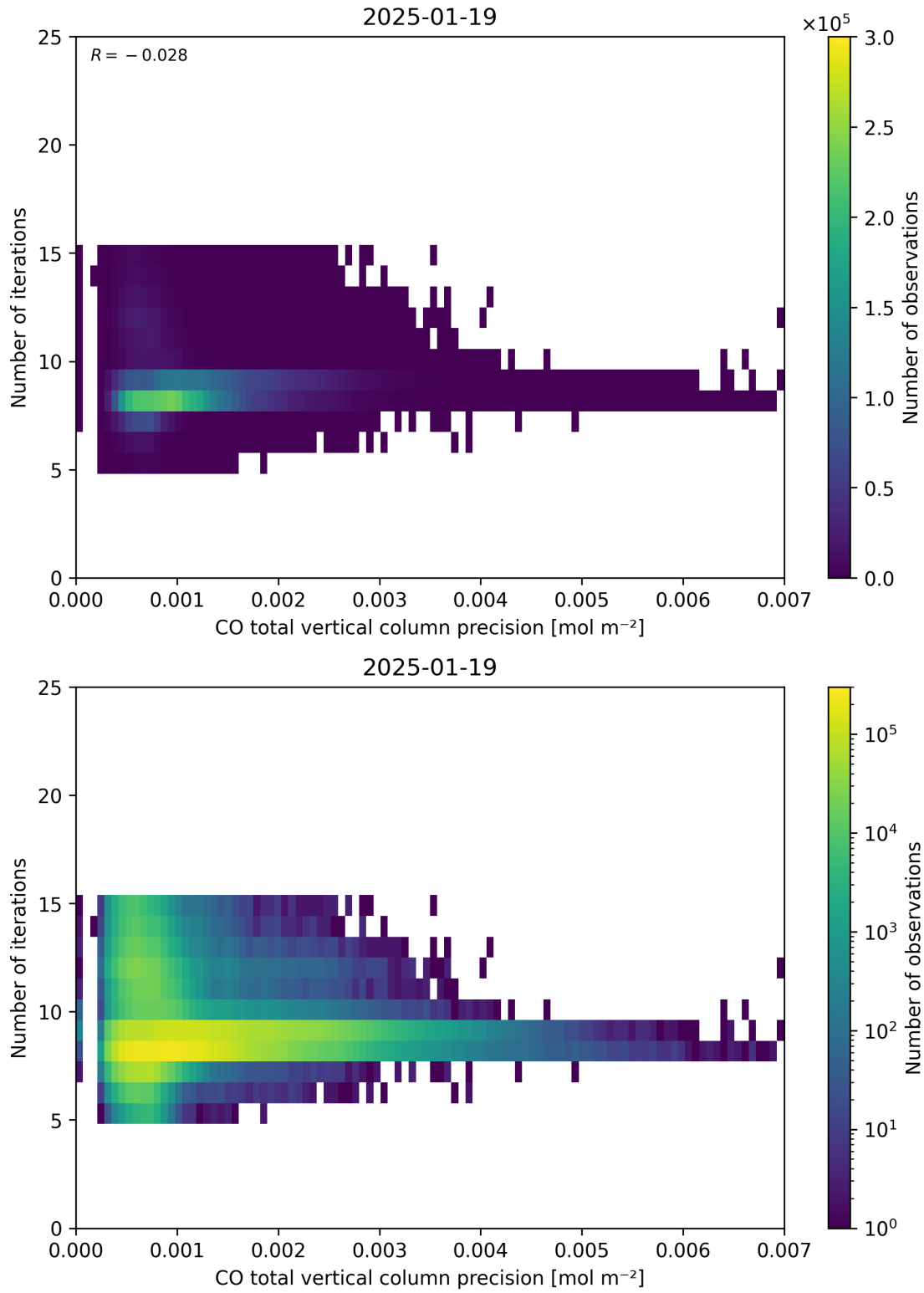
Figure 46: Scatter density plot of “CO total vertical column precision” against “Number of iterations” for 2025-01-18 to 2025-01-20.
