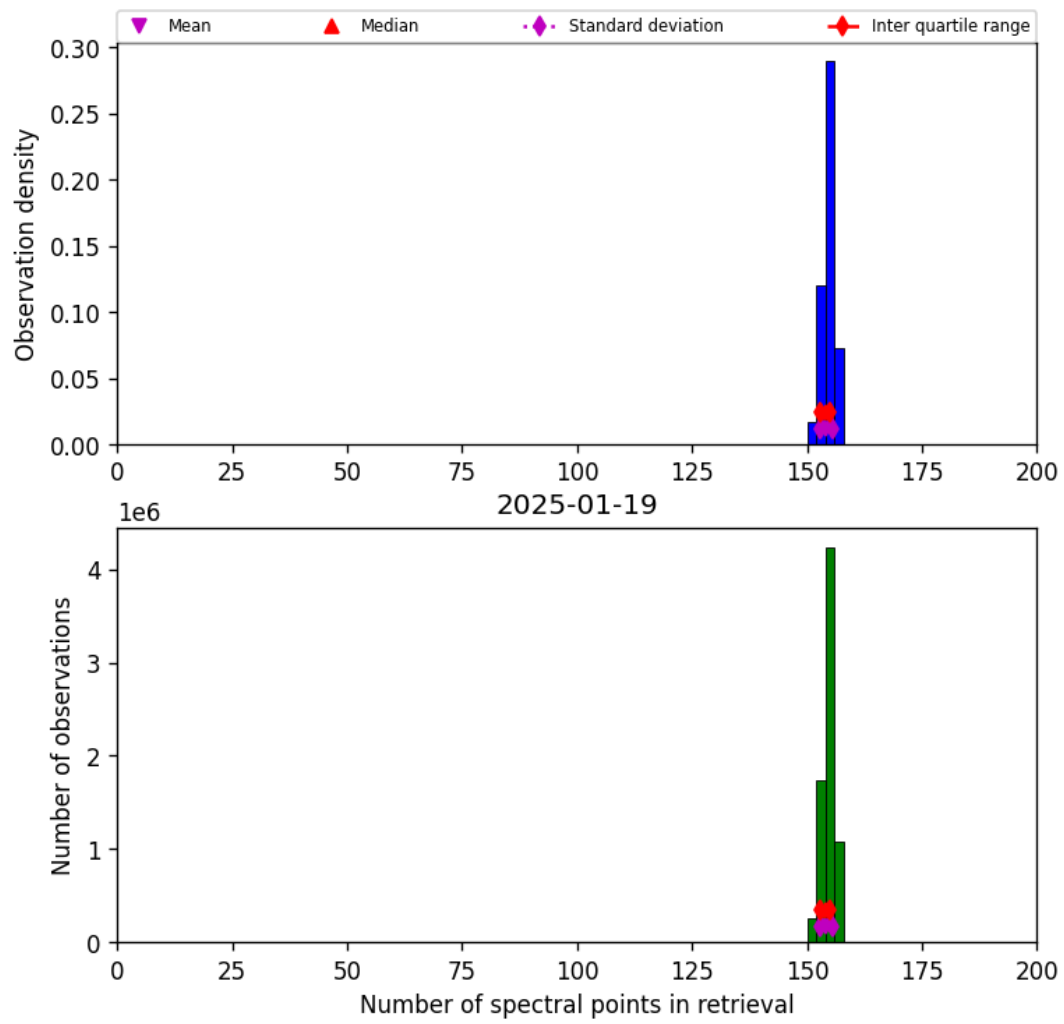
Figure 21: Histogram of “Number of spectral points in retrieval” for 2025-01-18 to 2025-01-20
