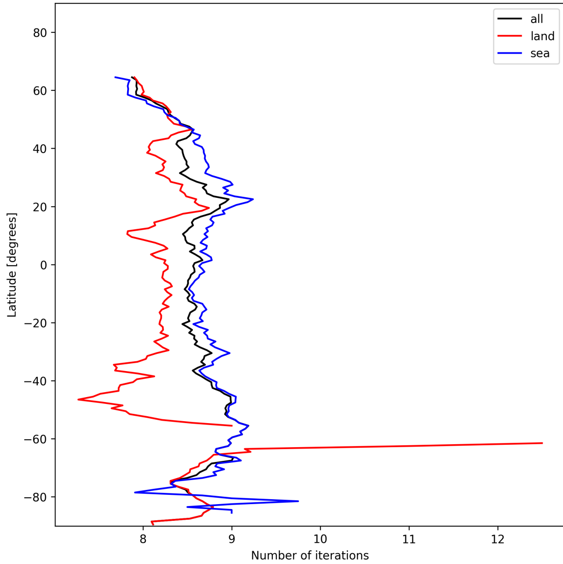
Figure 16: Zonal average of “Number of iterations” for 2025-01-18 to 2025-01-20.
