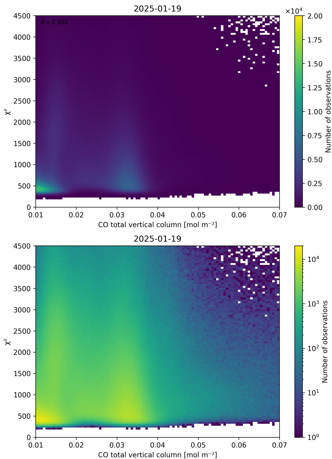
Figure 35: Scatter density plot of “CO total vertical column” against “ \chi^2 ” for 2025-01-18 to 2025-01-20.
