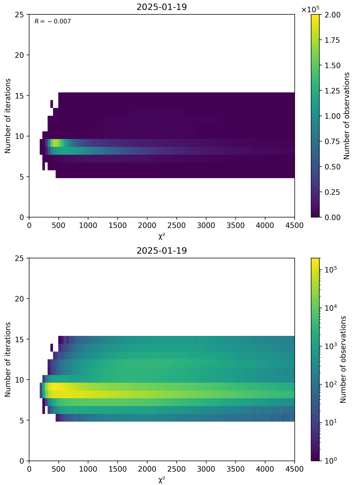
Figure 49: Scatter density plot of “ \chi^2 ” against “Number of iterations” for 2025-01-18 to 2025-01-20.
