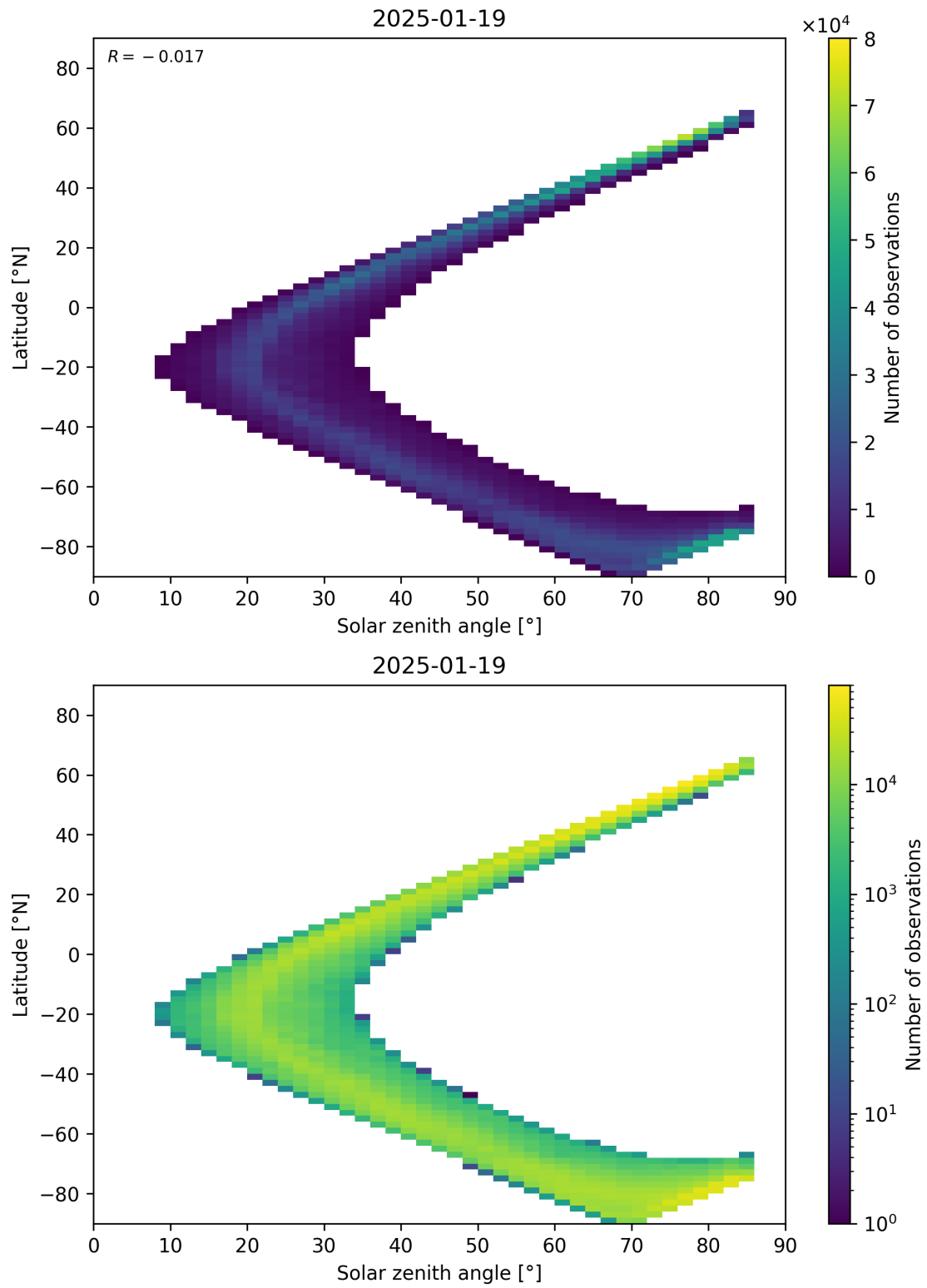
Figure 66: Scatter density plot of “Solar zenith angle” against “Latitude” for 2025-01-18 to 2025-01-20.
