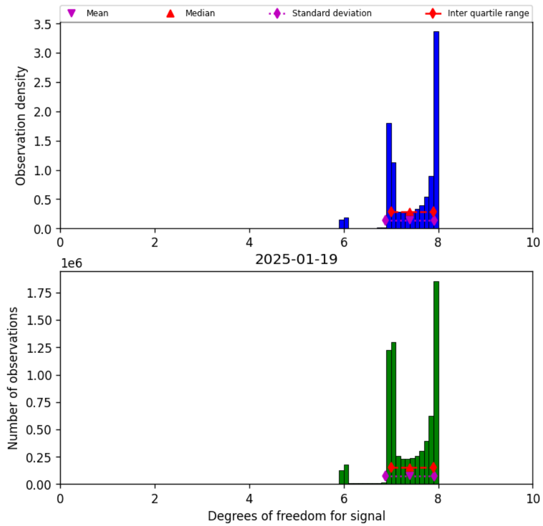
Figure 23: Histogram of “Degrees of freedom for signal” for 2025-01-18 to 2025-01-20
