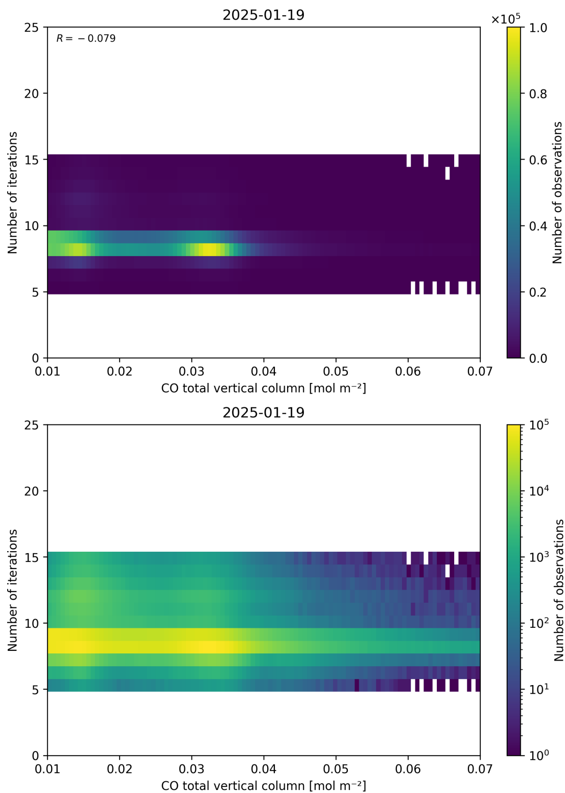
Figure 42: Scatter density plot of “CO total vertical column” against “Number of iterations” for 2025-01-18 to 2025-01-20.
