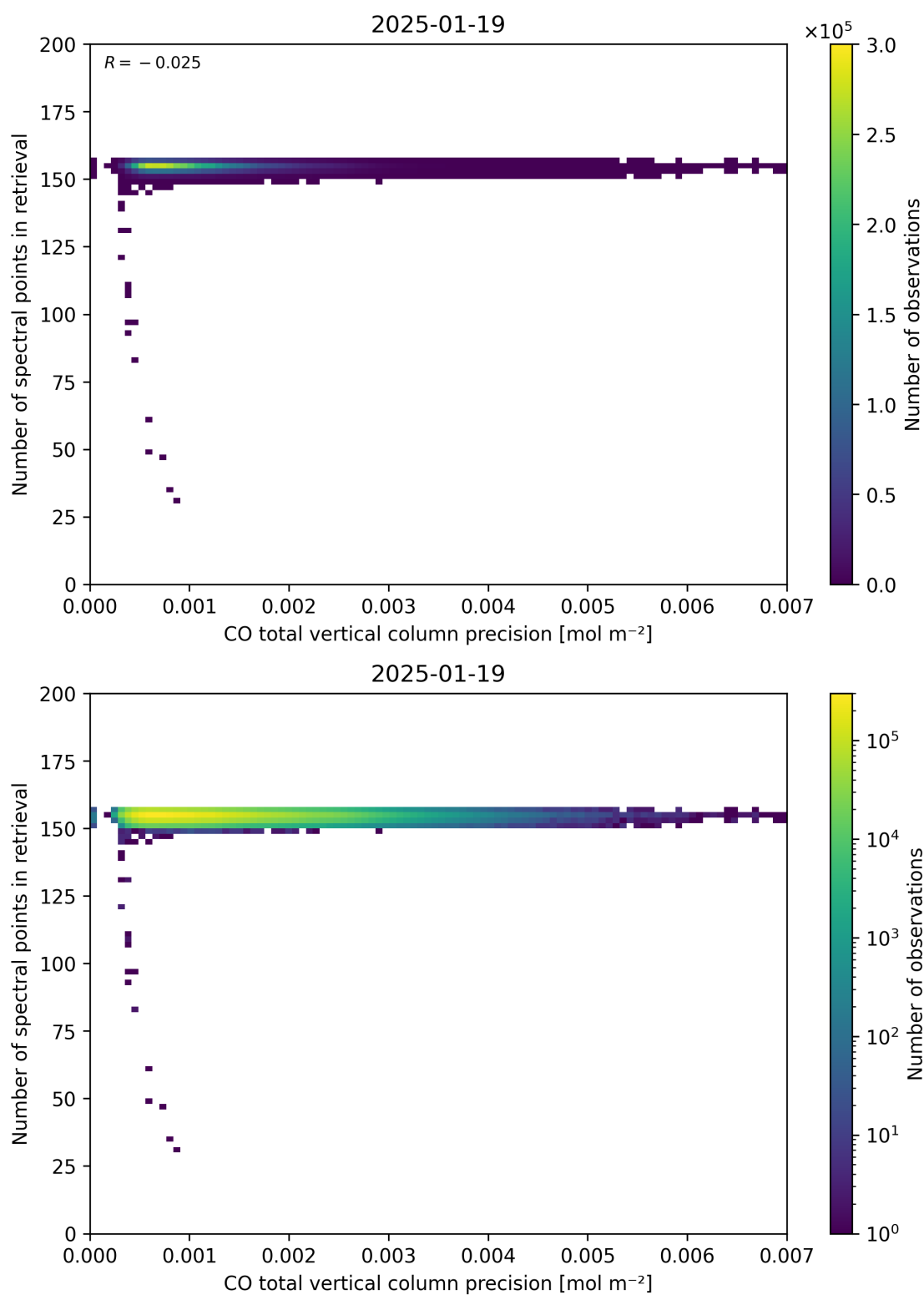
Figure 47: Scatter density plot of “CO total vertical column precision” against “Number of spectral points in retrieval” for 2025-01-18 to 2025-01-20.
