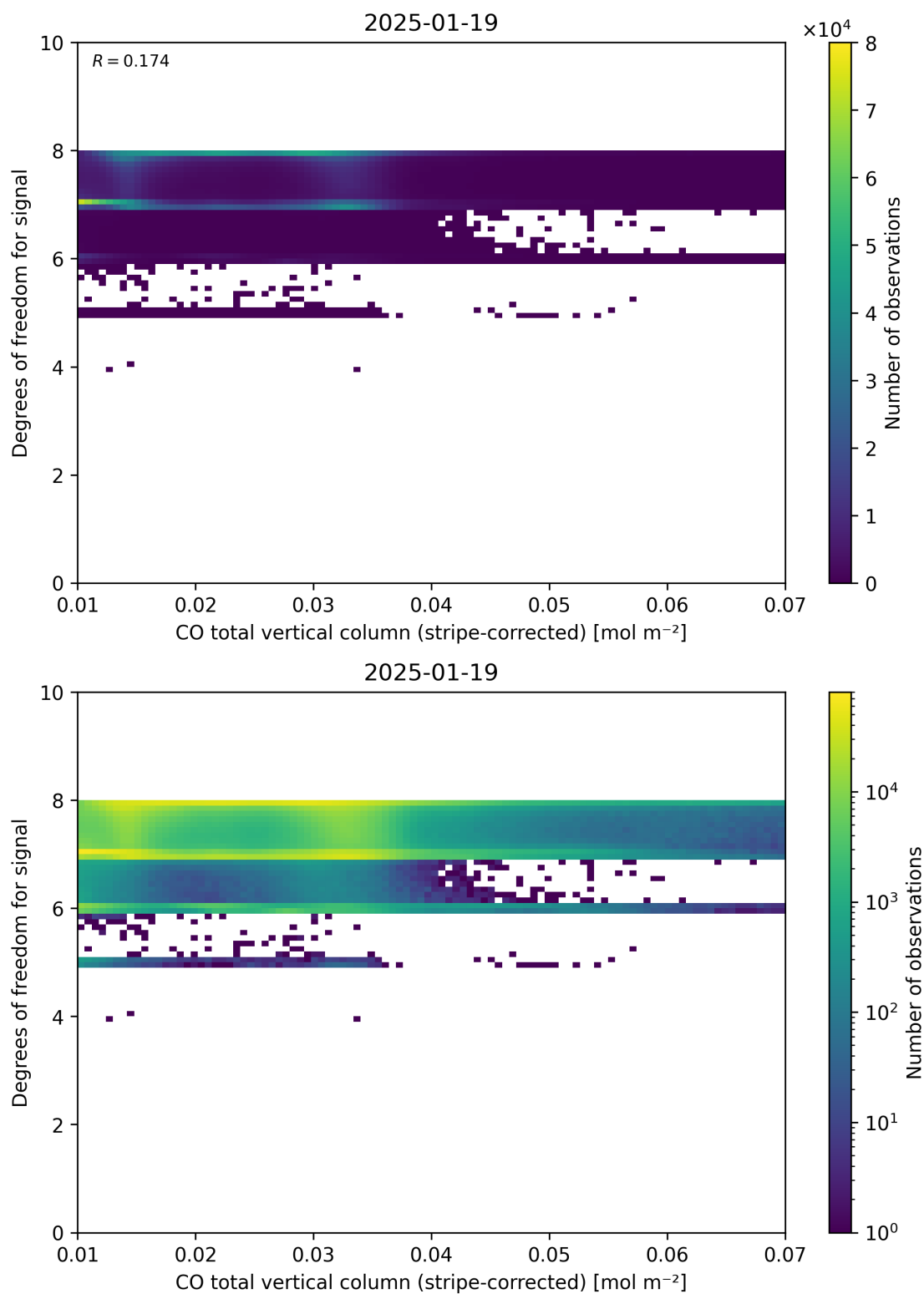
Figure 38: Scatter density plot of “CO total vertical column (stripe-corrected)” against “Degrees of freedom for signal” for 2025-01-18 to 2025-01-20.
