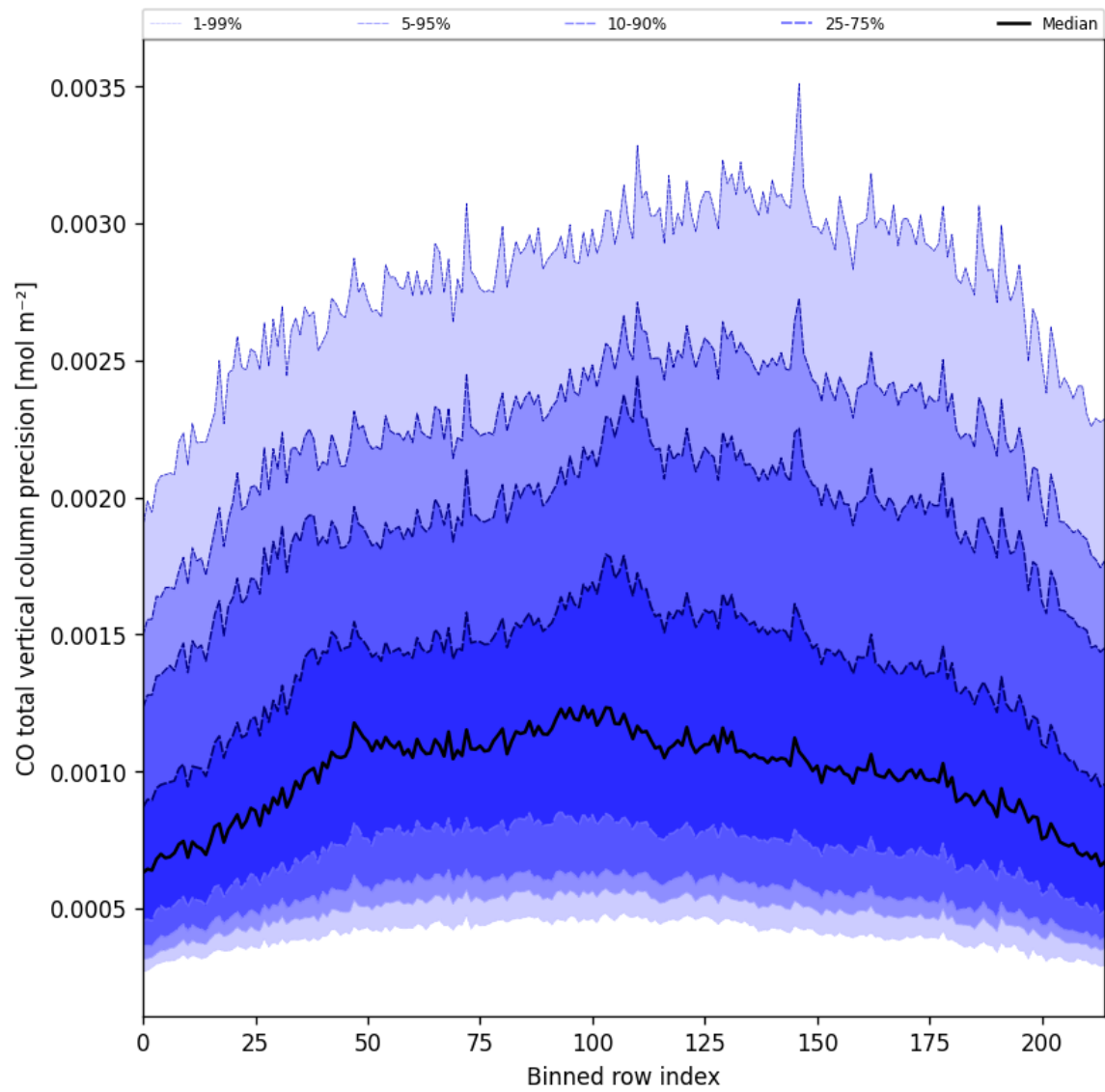
Figure 28: Along track statistics of “CO total vertical column precision” for 2025-01-18 to 2025-01-20
