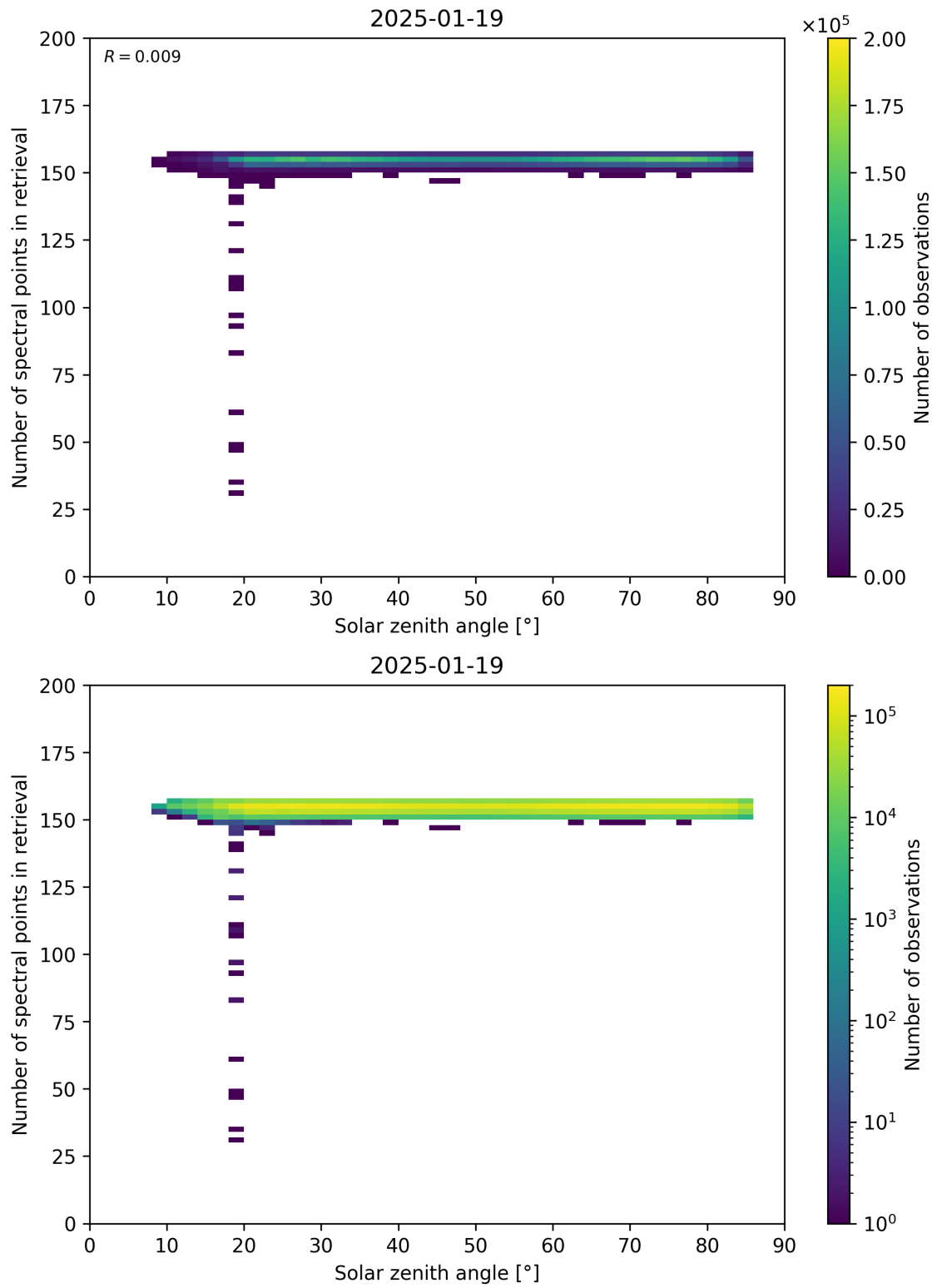
Figure 68: Scatter density plot of “Solar zenith angle” against “Number of spectral points in retrieval” for 2025-01-18 to 2025-01-20.
