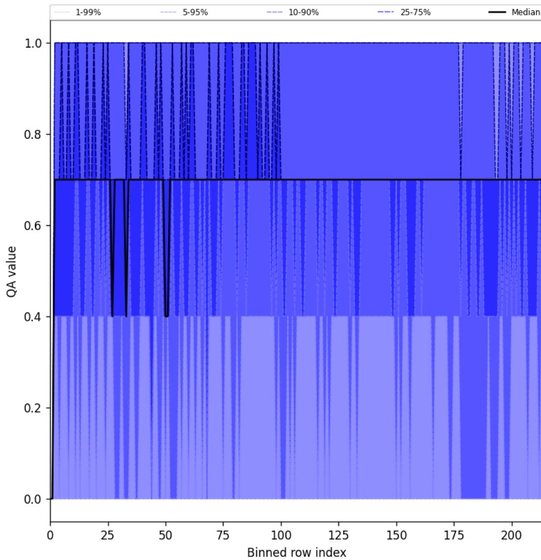
Figure 25: Along track statistics of “QA value” for 2025-01-18 to 2025-01-20
