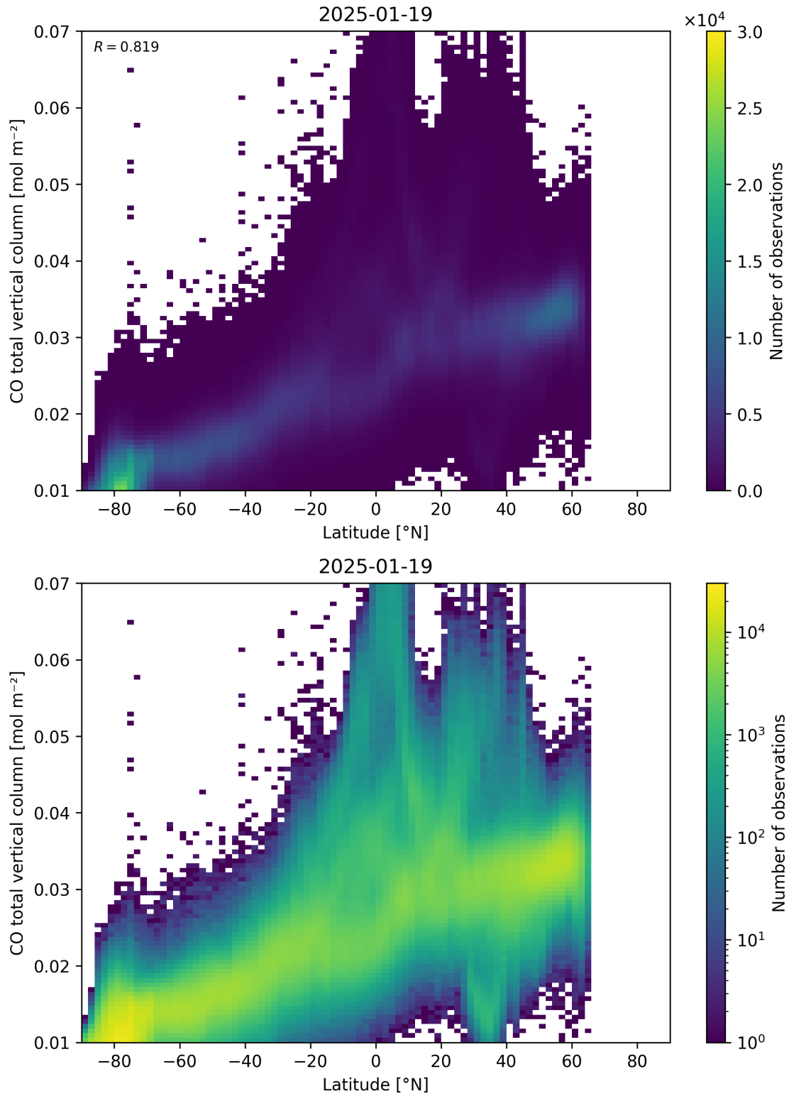
Figure 51: Scatter density plot of “Latitude” against “CO total vertical column” for 2025-01-18 to 2025-01-20.
