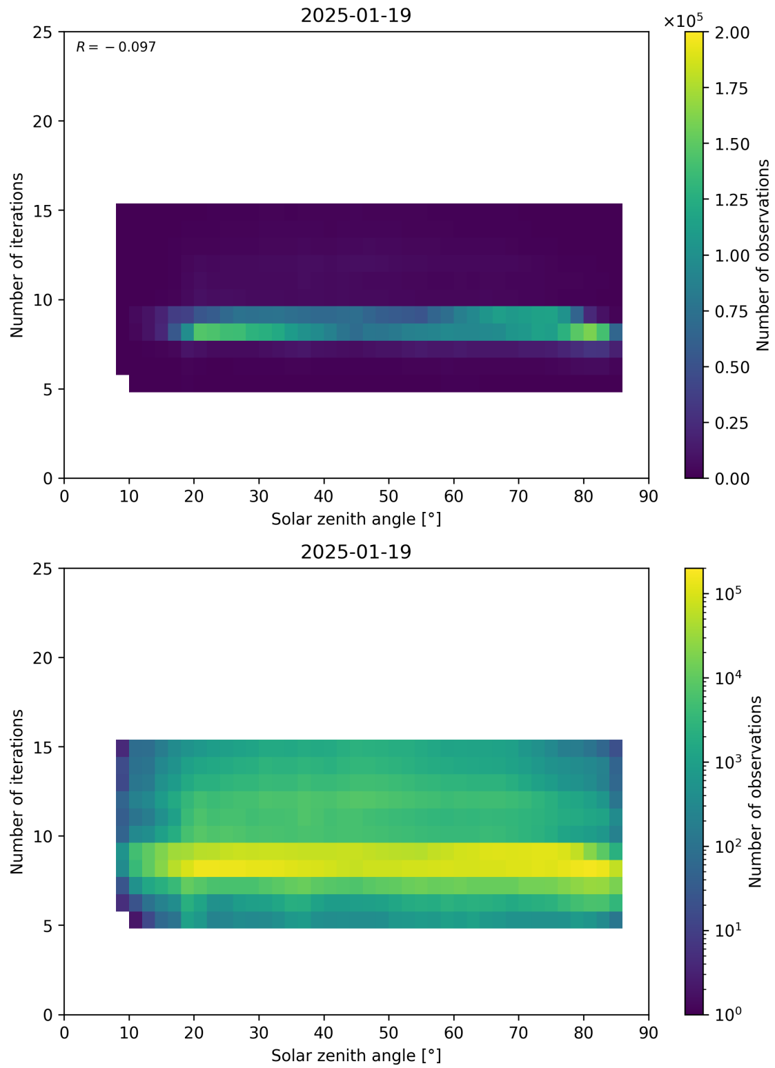
Figure 67: Scatter density plot of “Solar zenith angle” against “Number of iterations” for 2025-01-18 to 2025-01-20.
