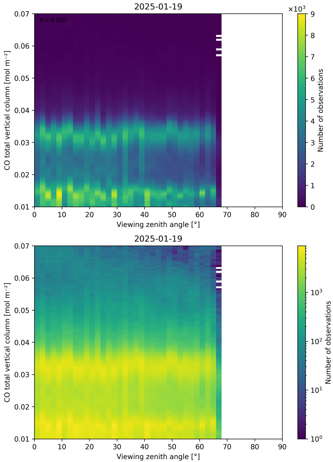
Figure 69: Scatter density plot of “Viewing zenith angle” against “CO total vertical column” for 2025-01-18 to 2025-01-20.
