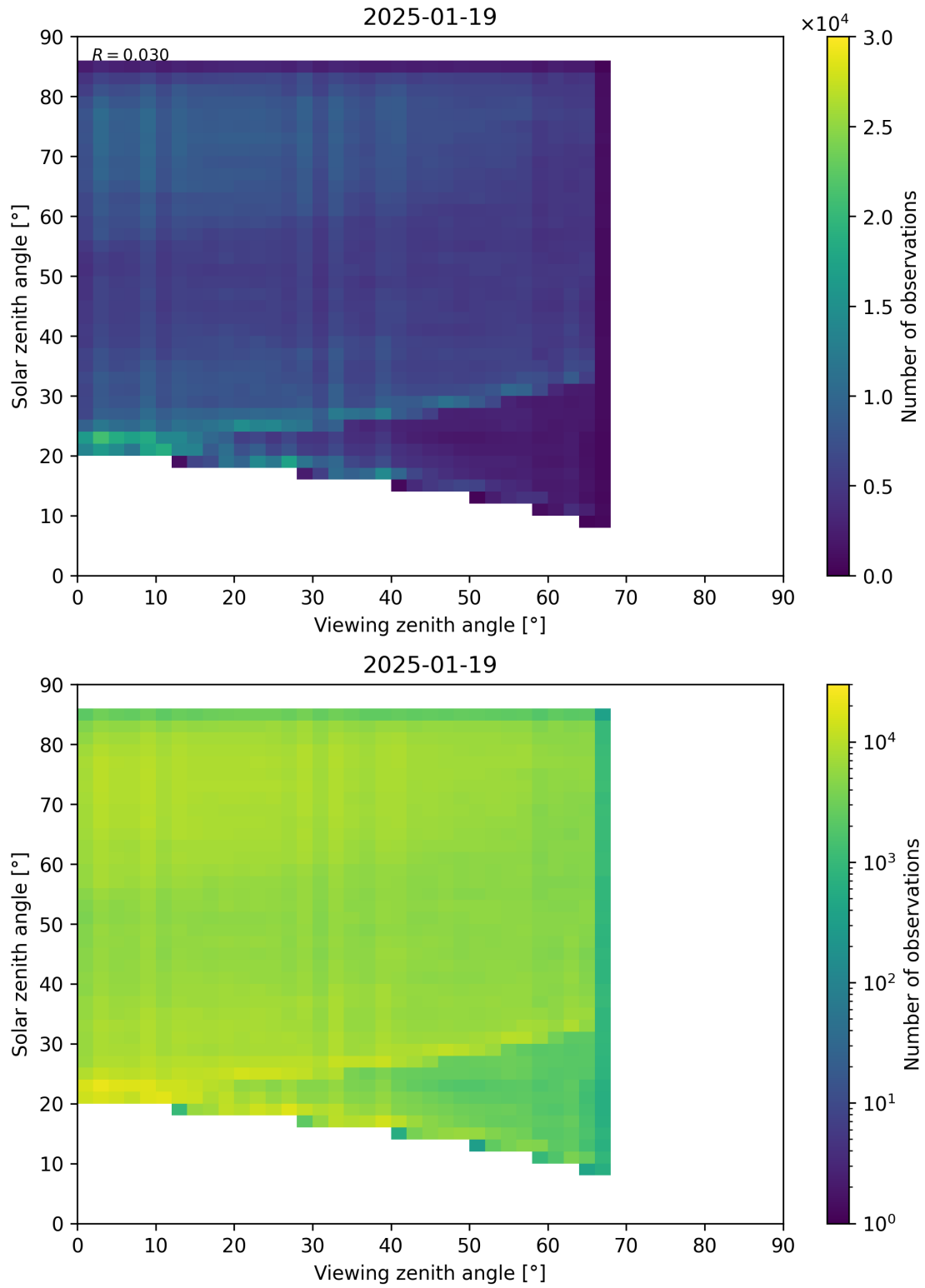
Figure 77: Scatter density plot of “Viewing zenith angle” against “Solar zenith angle” for 2025-01-18 to 2025-01-20.
