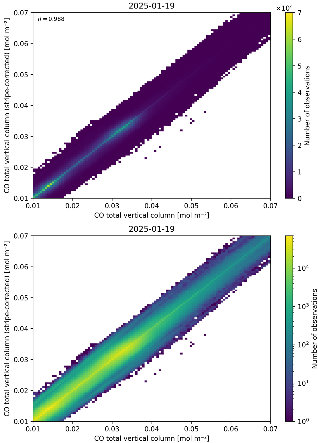
Figure 33: Scatter density plot of “CO total vertical column” against “CO total vertical column (stripe-corrected)” for 2025-01-18 to 2025-01-20.
