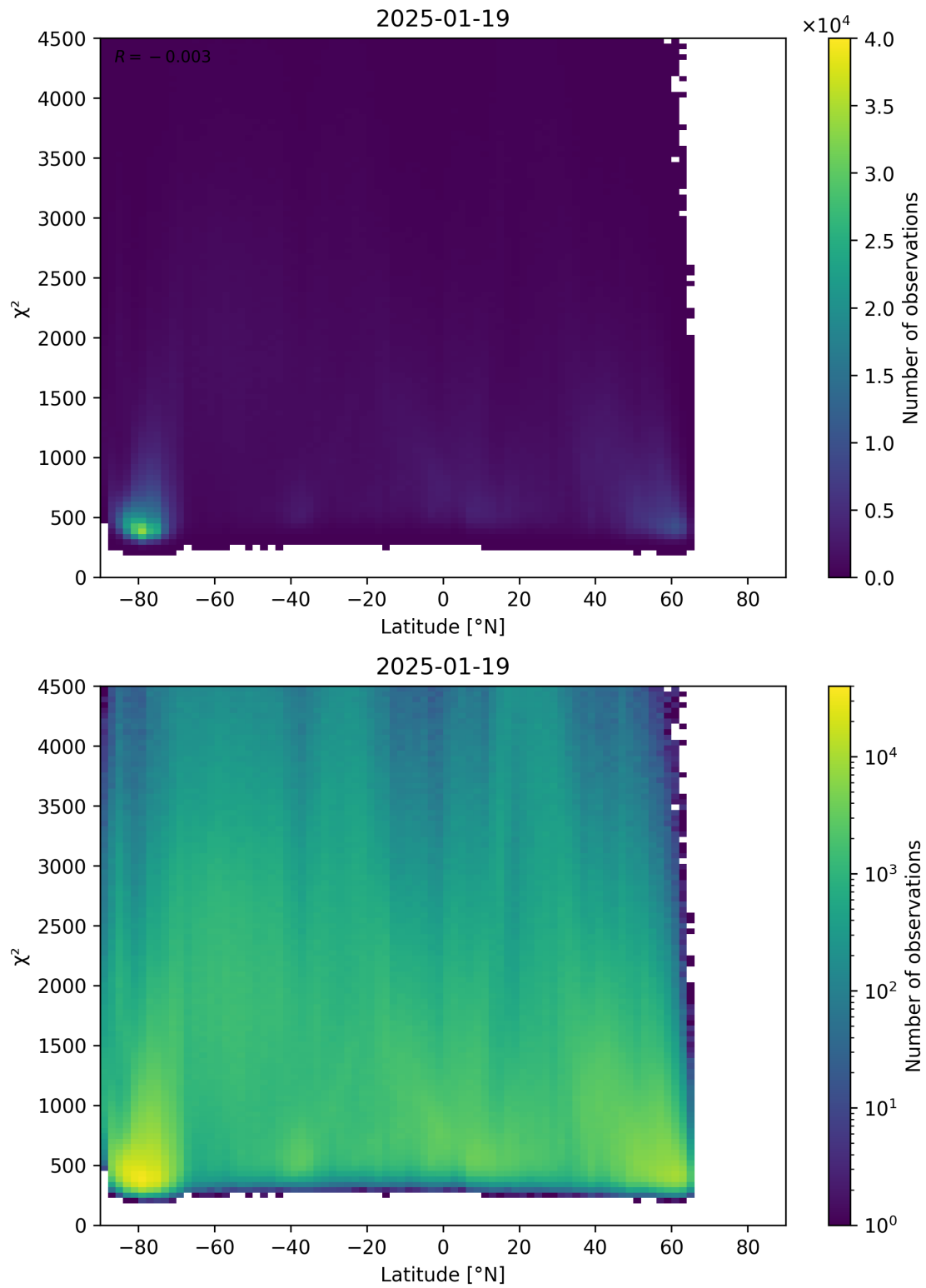
Figure 54: Scatter density plot of “Latitude” against “ \chi^2 ” for 2025-01-18 to 2025-01-20.
