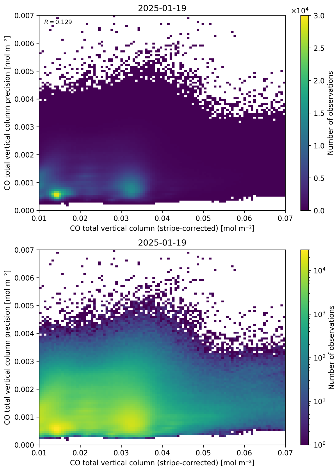
Figure 36: Scatter density plot of “CO total vertical column (stripe-corrected)” against “CO total vertical column precision” for 2025-01-18 to 2025-01-20.
