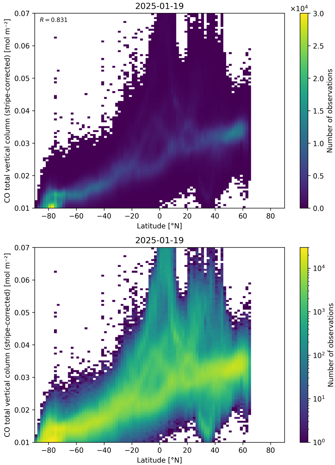
Figure 52: Scatter density plot of “Latitude” against “CO total vertical column (stripe-corrected)” for 2025-01-18 to 2025-01-20.
