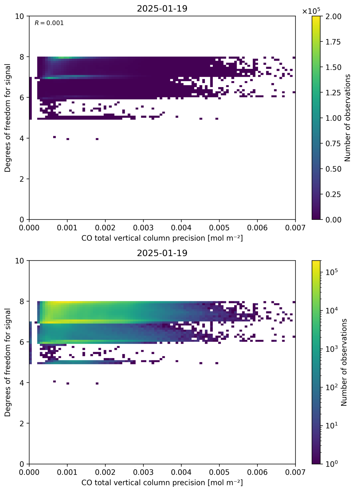
Figure 45: Scatter density plot of “CO total vertical column precision” against “Degrees of freedom for signal” for 2025-01-18 to 2025-01-20.
