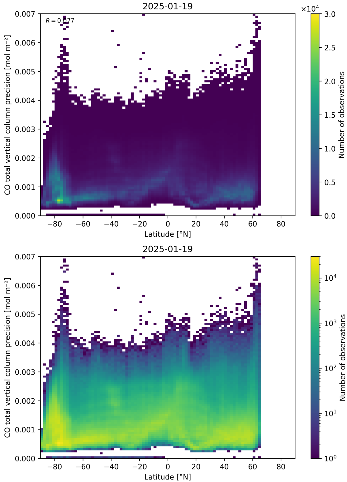
Figure 53: Scatter density plot of “Latitude” against “CO total vertical column precision” for 2025-01-18 to 2025-01-20.
