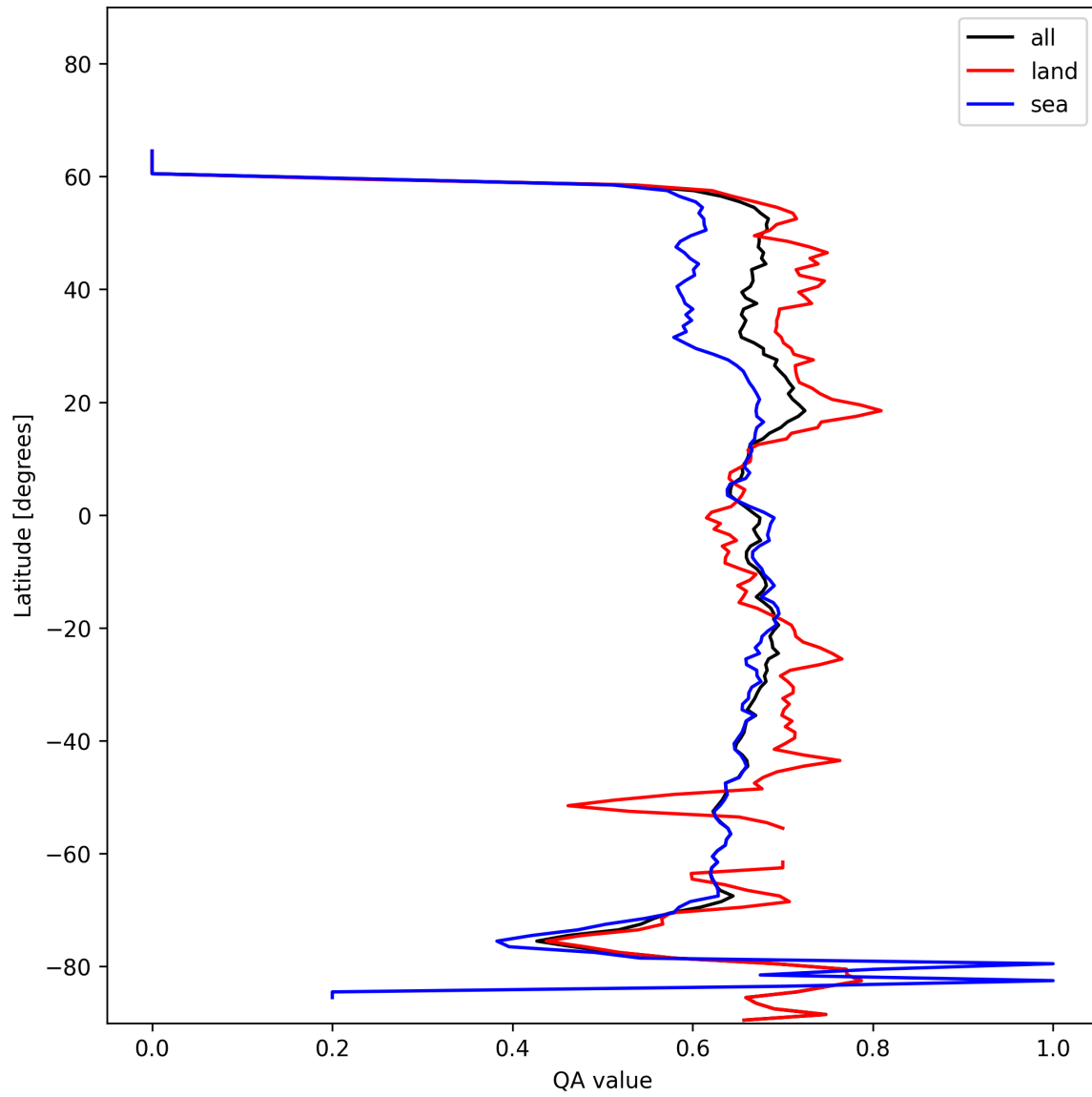
Figure 9: Zonal average of “QA value” for 2025-01-18 to 2025-01-20.
