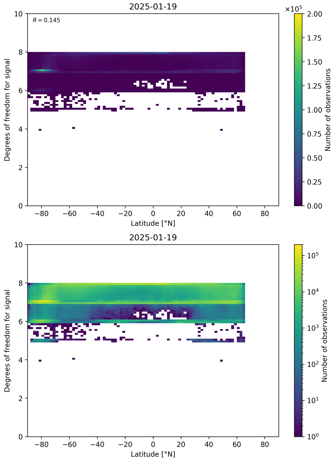
Figure 55: Scatter density plot of “Latitude” against “Degrees of freedom for signal” for 2025-01-18 to 2025-01-20.
