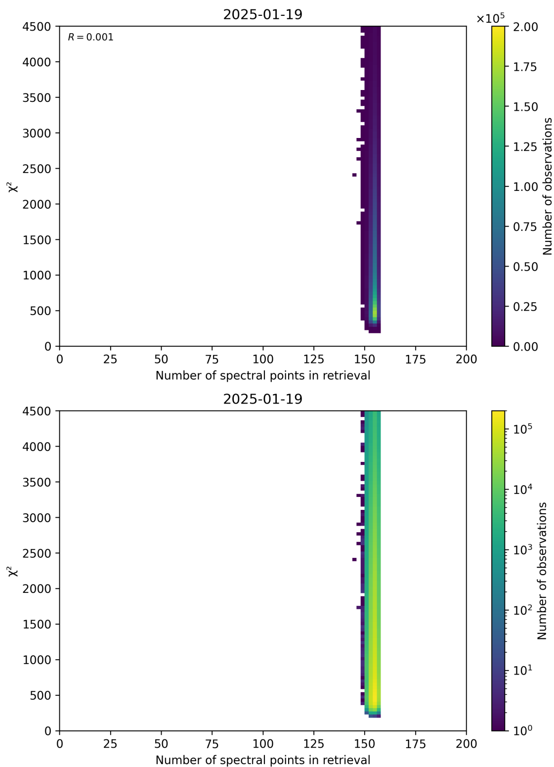
Figure 58: Scatter density plot of “Number of spectral points in retrieval” against “ \chi^2 ” for 2025-01-18 to 2025-01-20.
