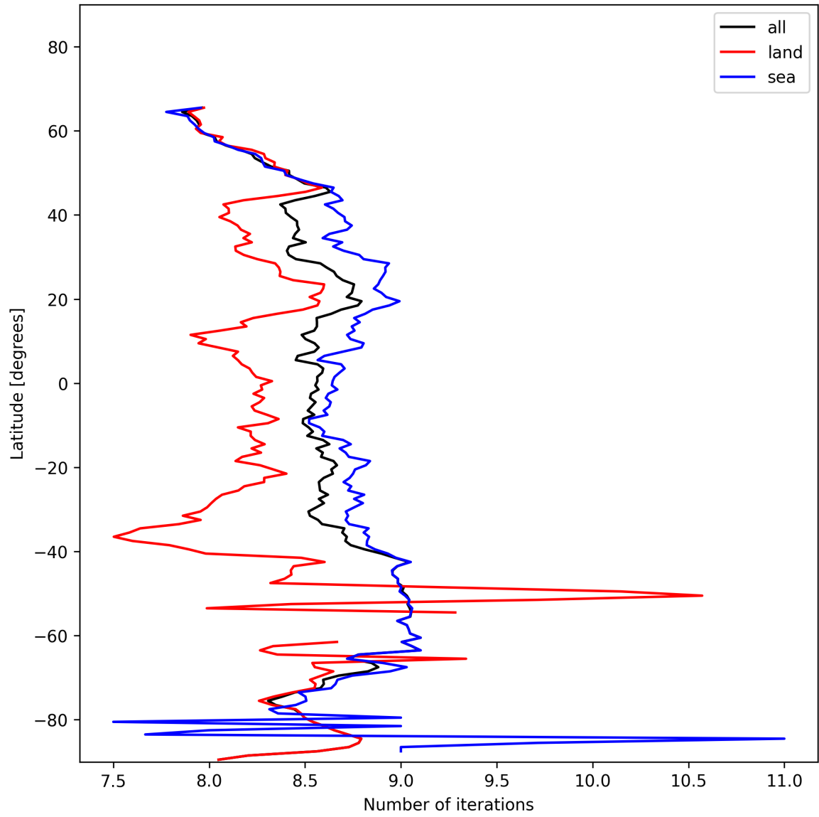
Figure 16: Zonal average of “Number of iterations” for 2025-01-19 to 2025-01-21.
