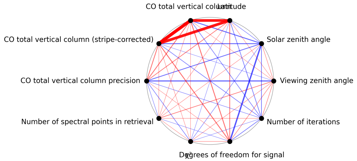
Figure 1: Map of correlation graph for 2025-01-19 to 2025-01-21.
