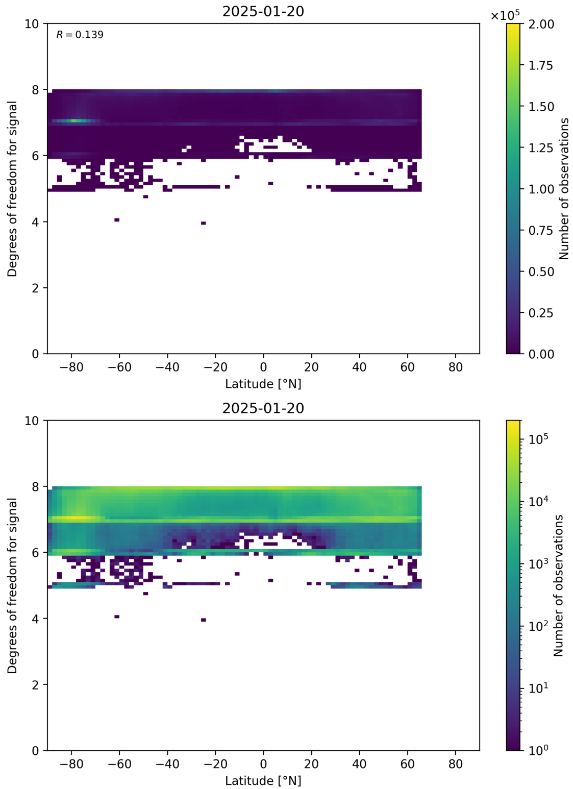
Figure 55: Scatter density plot of “Latitude” against “Degrees of freedom for signal” for 2025-01-19 to 2025-01-21.
