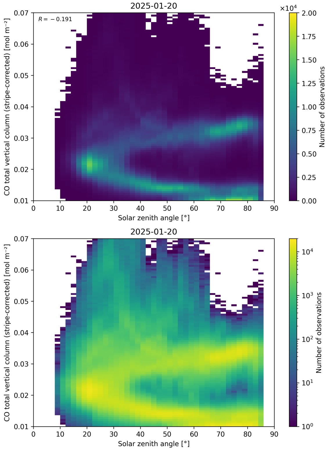
Figure 62: Scatter density plot of “Solar zenith angle” against “CO total vertical column (stripe-corrected)” for 2025-01-19 to 2025-01-21.
