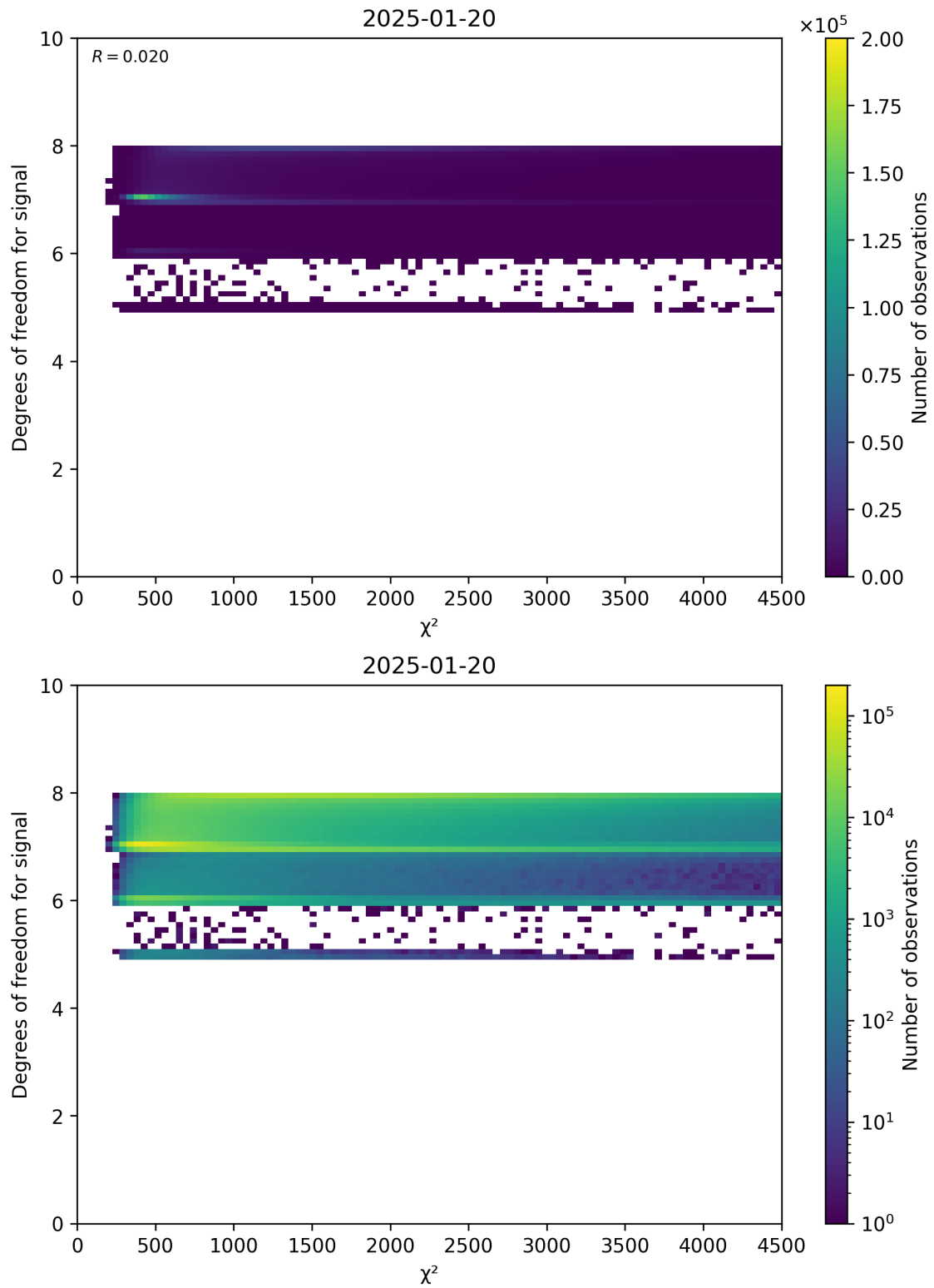
Figure 48: Scatter density plot of “ \chi^2 ” against “Degrees of freedom for signal” for 2025-01-19 to 2025-01-21.
