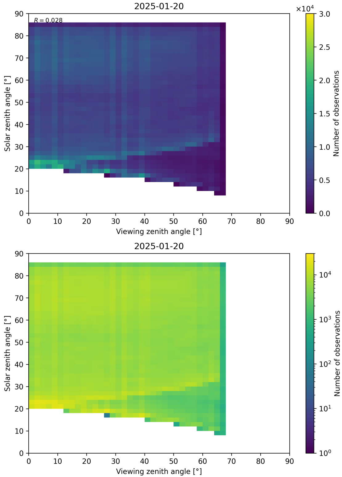
Figure 77: Scatter density plot of “Viewing zenith angle” against “Solar zenith angle” for 2025-01-19 to 2025-01-21.
