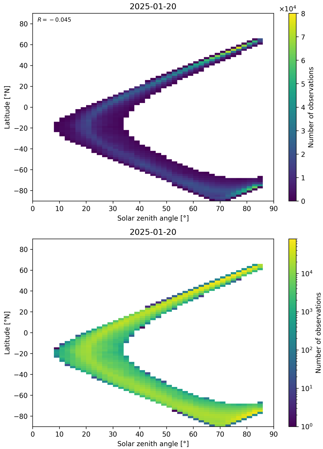
Figure 66: Scatter density plot of “Solar zenith angle” against “Latitude” for 2025-01-19 to 2025-01-21.
