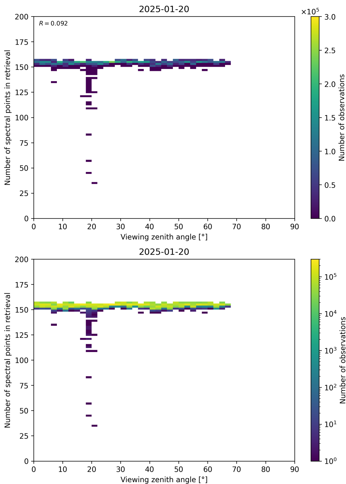
Figure 76: Scatter density plot of “Viewing zenith angle” against “Number of spectral points in retrieval” for 2025-01-19 to 2025-01-21.
