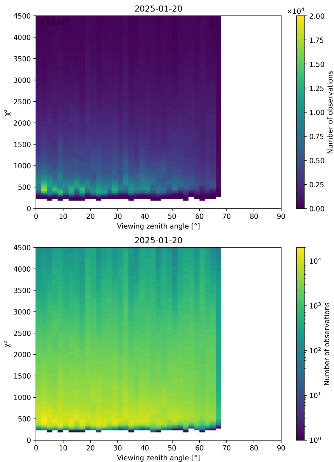
Figure 72: Scatter density plot of “Viewing zenith angle” against “ \chi^2 ” for 2025-01-19 to 2025-01-21.
