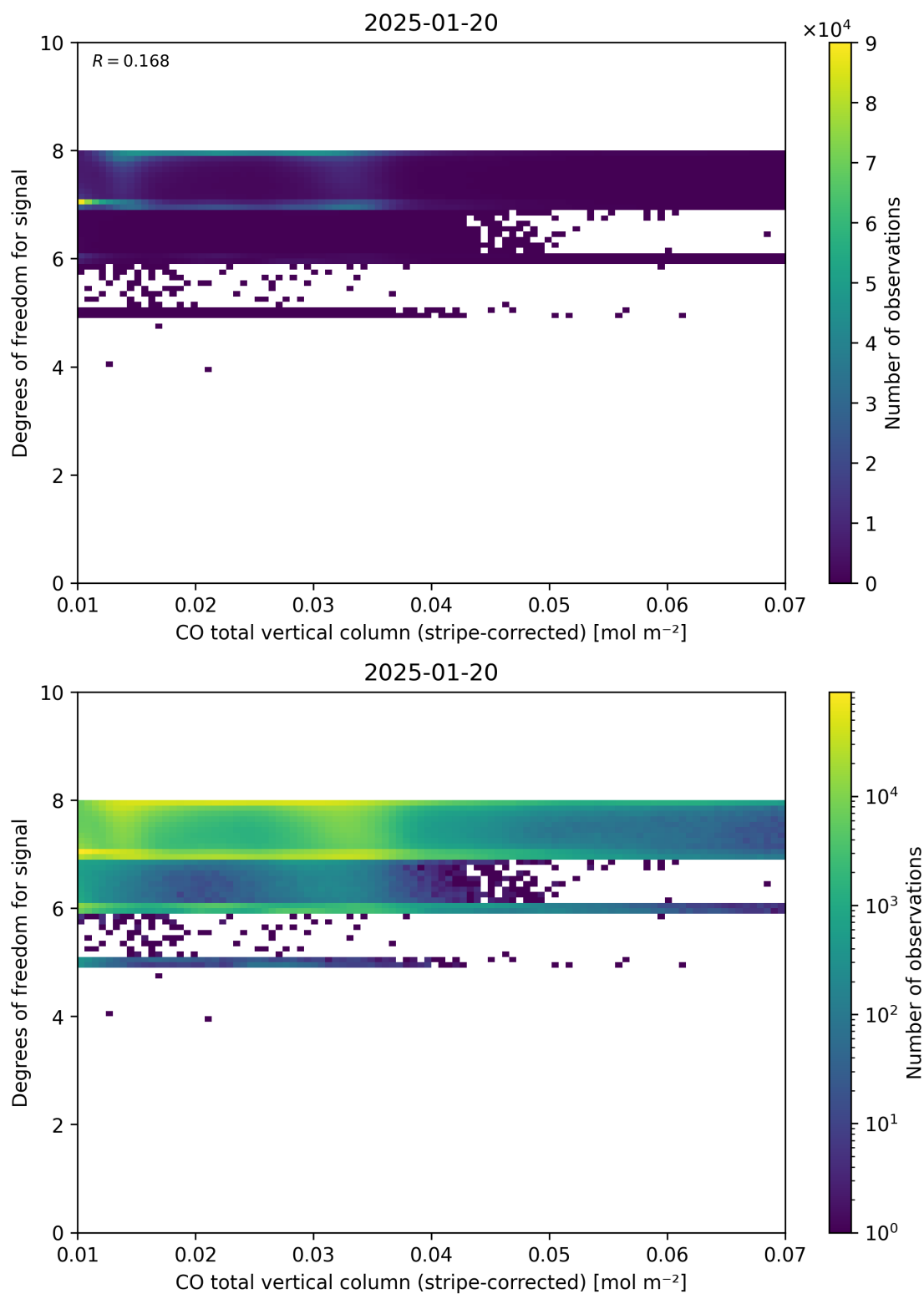
Figure 38: Scatter density plot of “CO total vertical column (stripe-corrected)” against “Degrees of freedom for signal” for 2025-01-19 to 2025-01-21.
