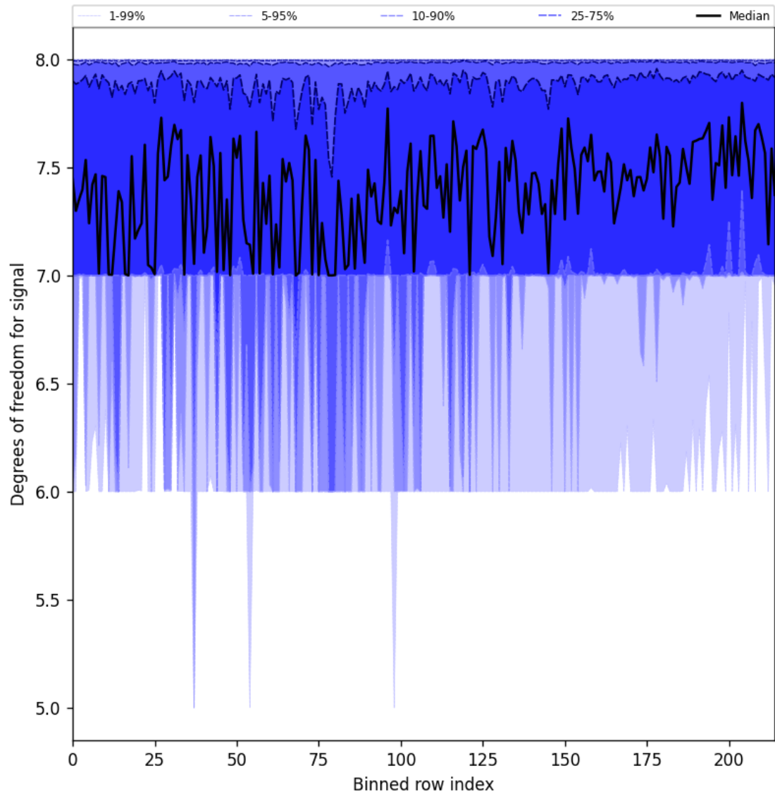
Figure 31: Along track statistics of “Degrees of freedom for signal” for 2025-01-19 to 2025-01-21
