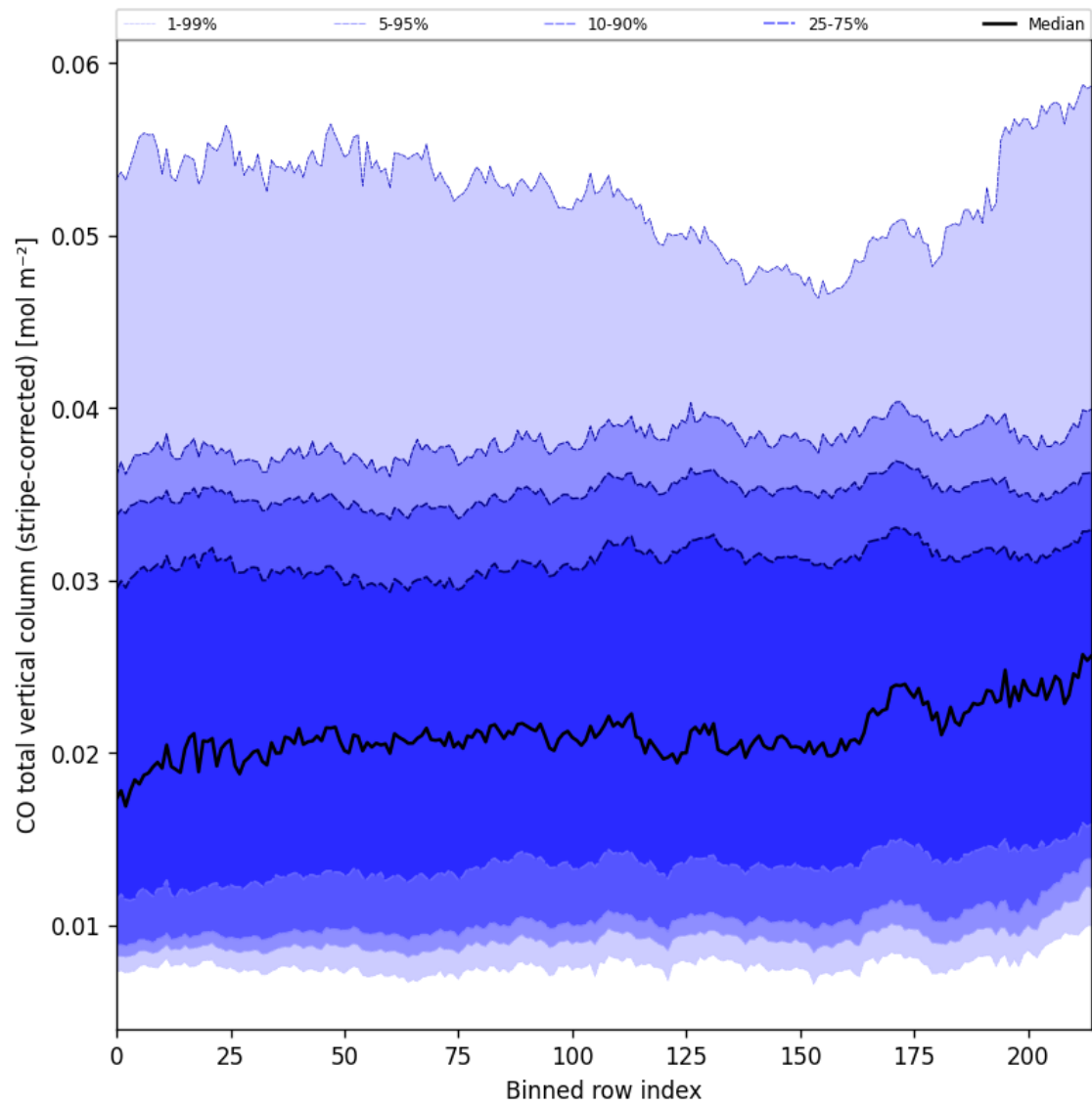
Figure 27: Along track statistics of “CO total vertical column (stripe-corrected)” for 2025-01-19 to 2025-01-21
