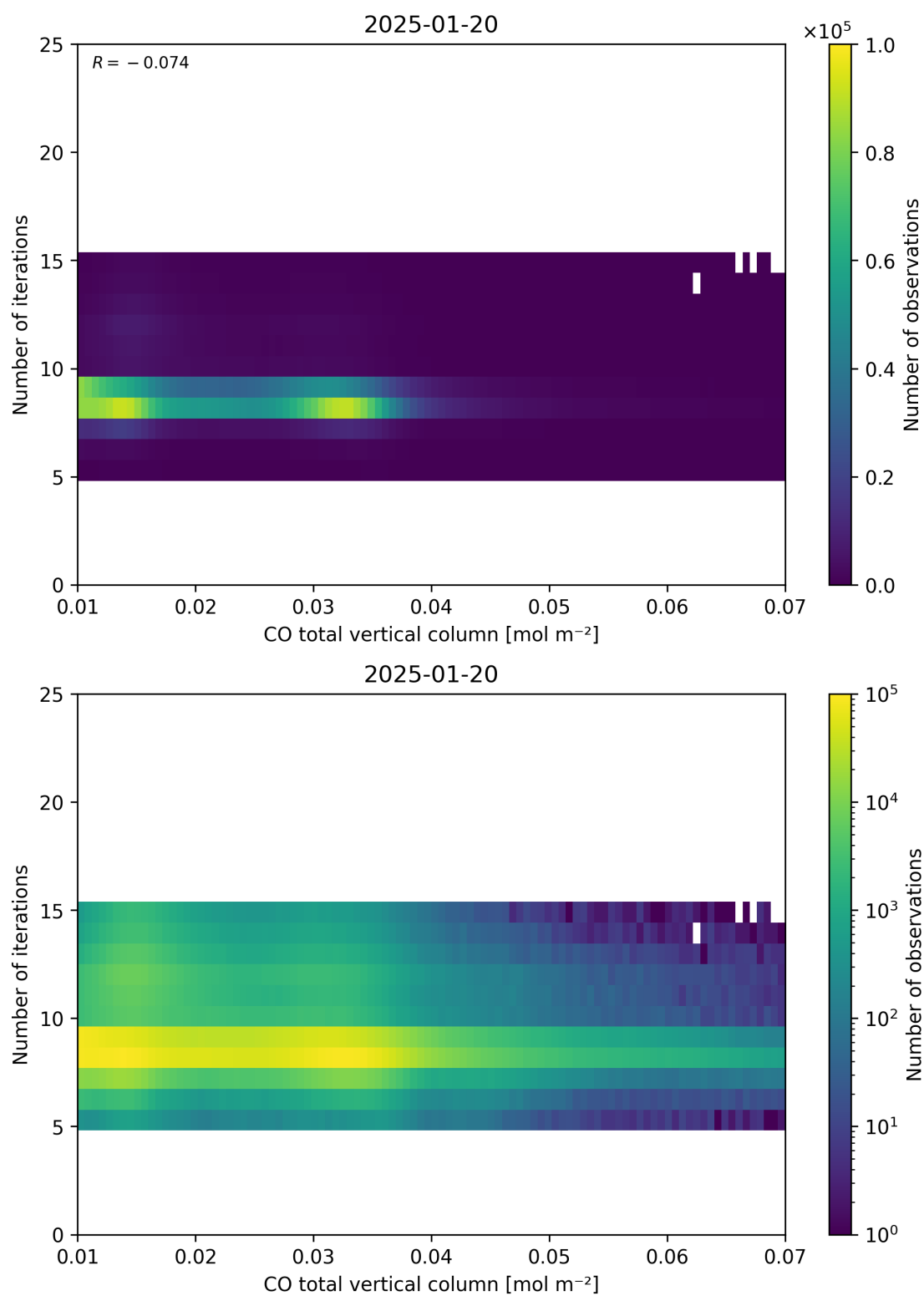
Figure 42: Scatter density plot of “CO total vertical column” against “Number of iterations” for 2025-01-19 to 2025-01-21.
