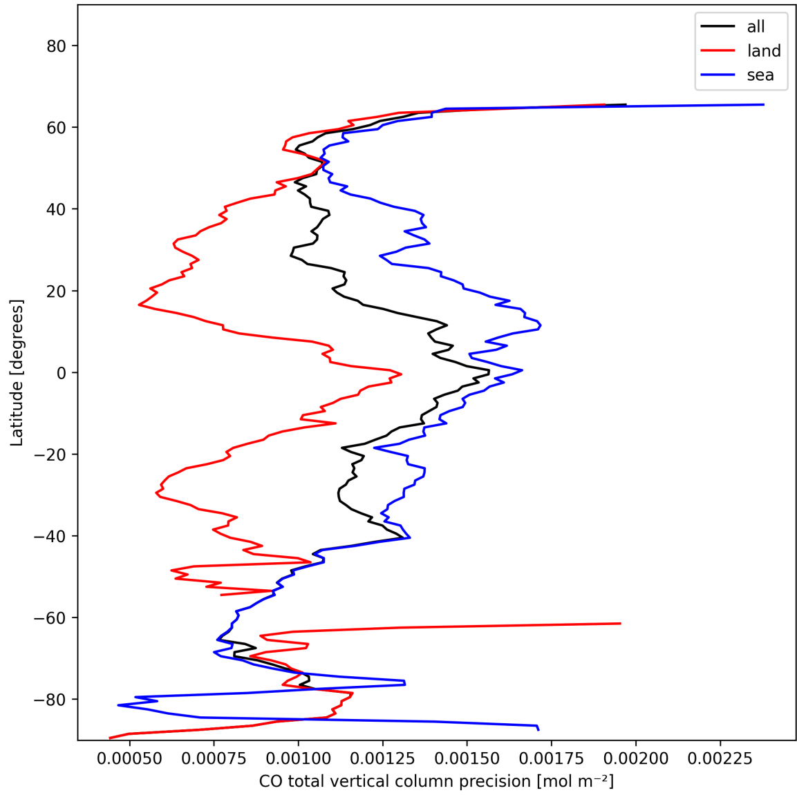
Figure 12: Zonal average of “CO total vertical column precision” for 2025-01-19 to 2025-01-21.
