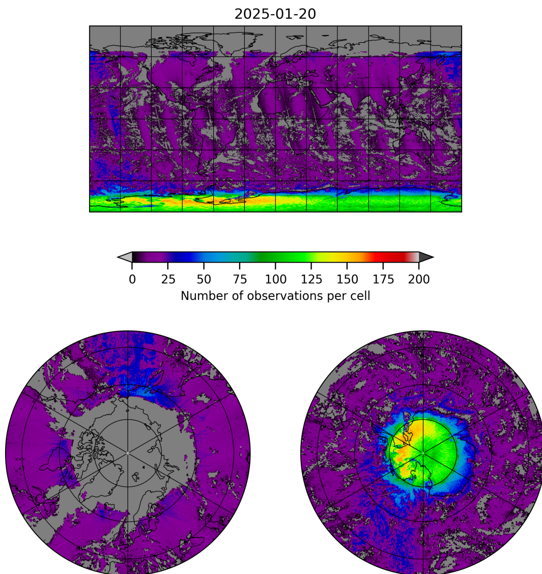
Figure 8: Map of the number of observations for 2025-01-19 to 2025-01-21
