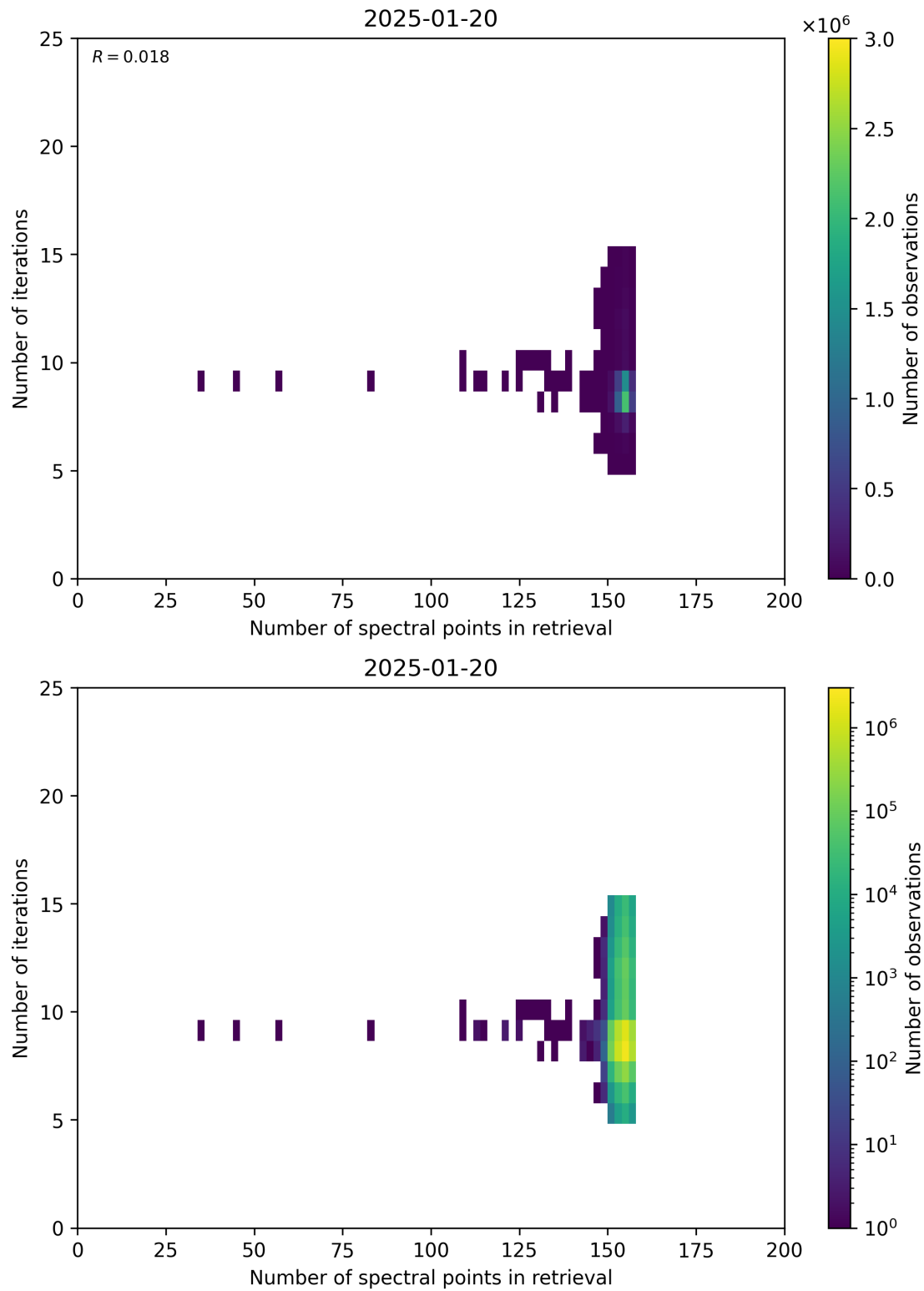
Figure 60: Scatter density plot of “Number of spectral points in retrieval” against “Number of iterations” for 2025-01-19 to 2025-01-21.
