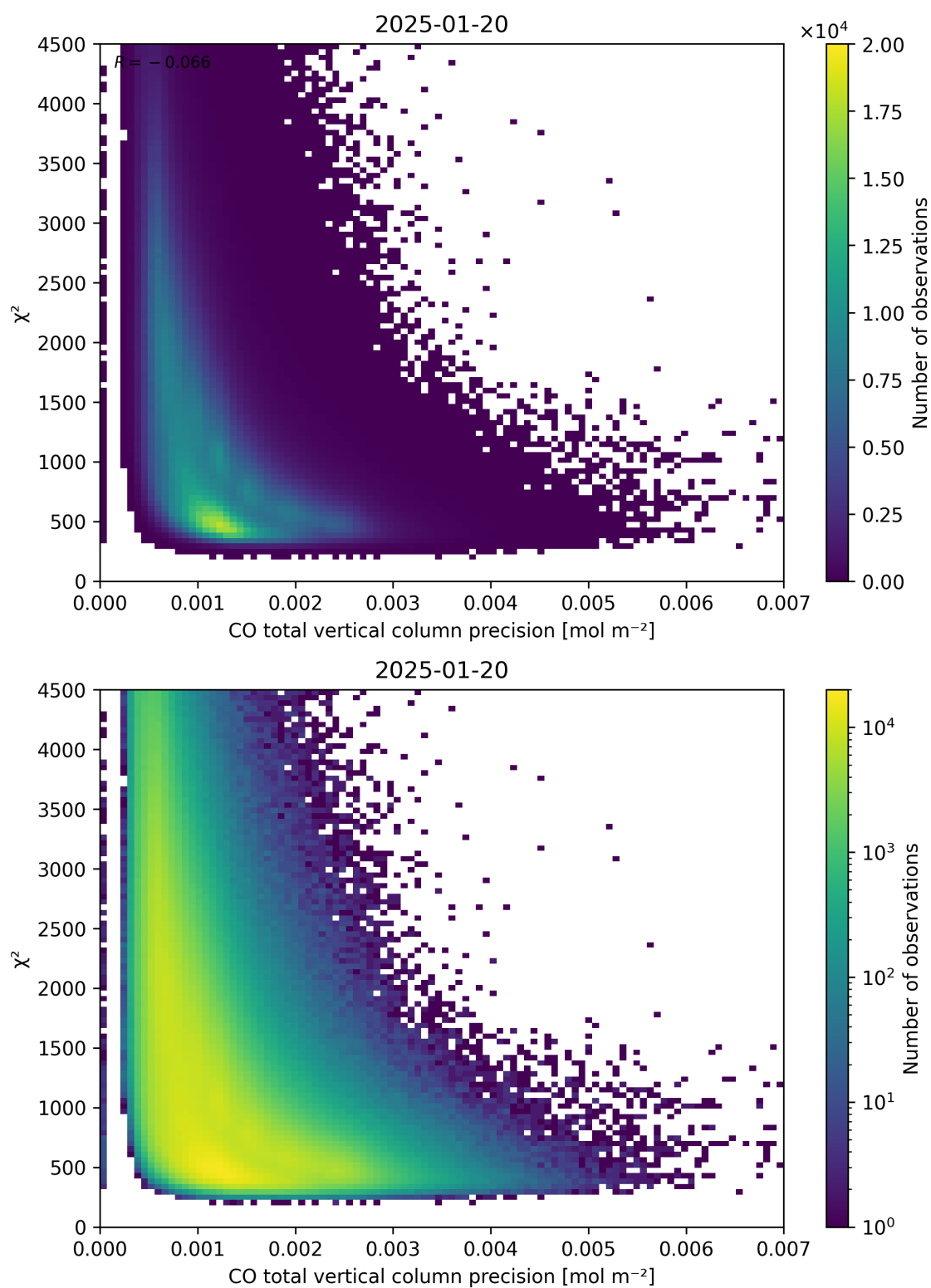
Figure 44: Scatter density plot of “CO total vertical column precision” against “ \chi^2 ” for 2025-01-19 to 2025-01-21.
