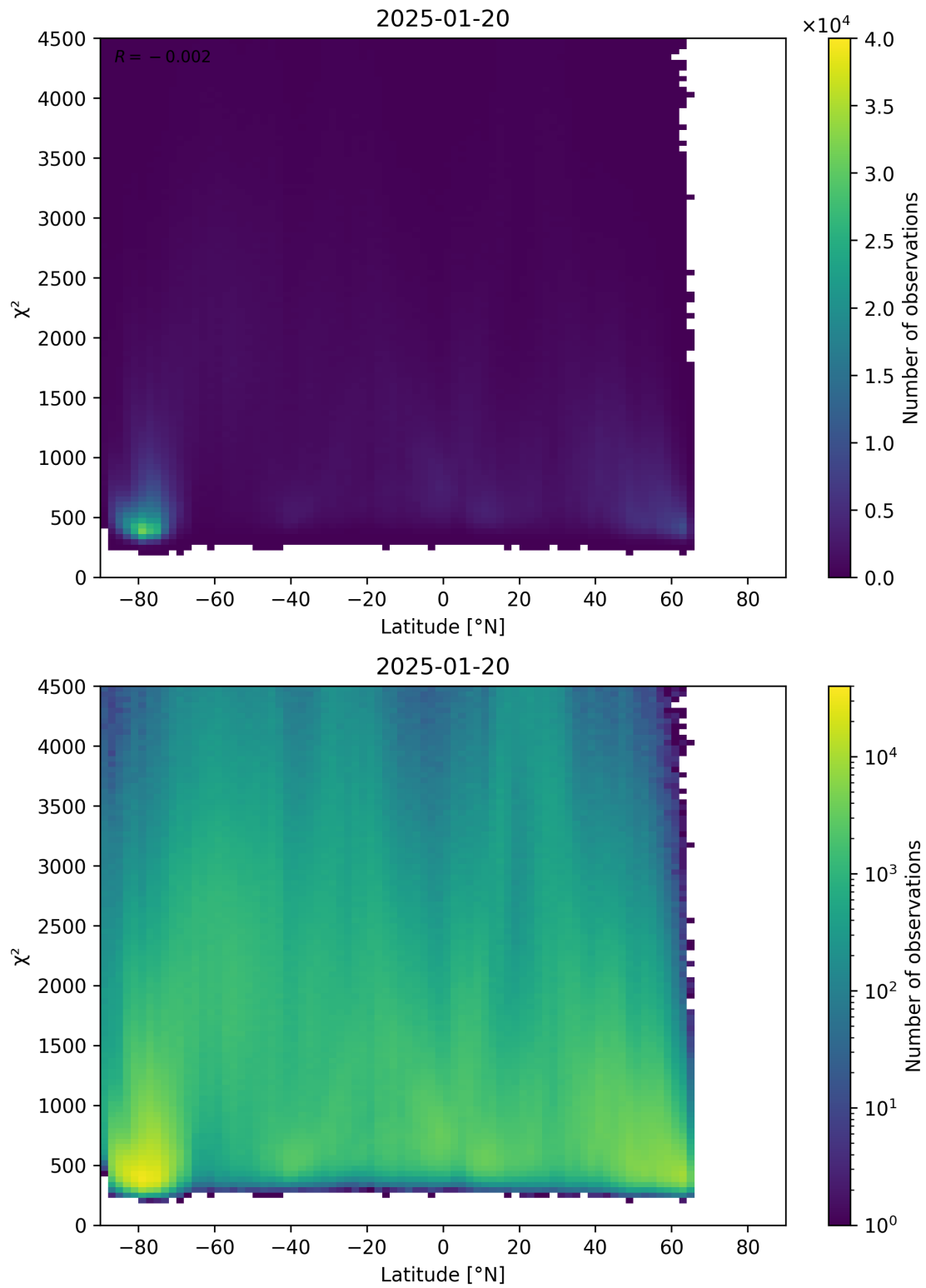
Figure 54: Scatter density plot of “Latitude” against “ \chi^2 ” for 2025-01-19 to 2025-01-21.
