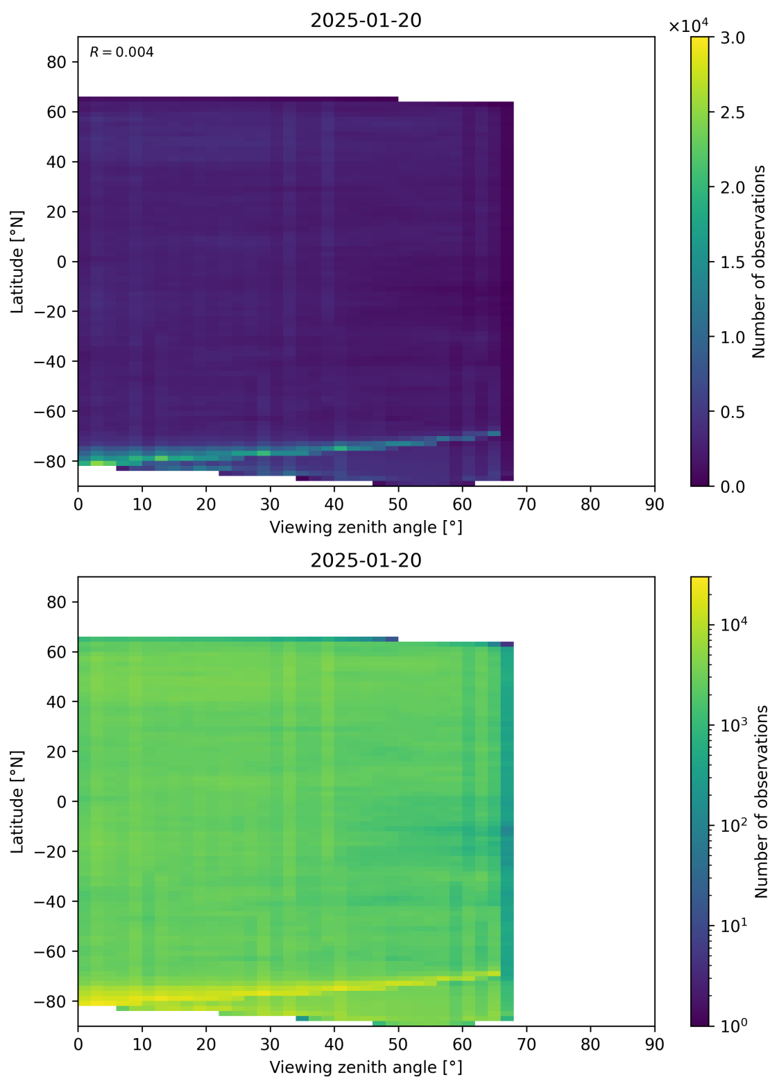
Figure 74: Scatter density plot of “Viewing zenith angle” against “Latitude” for 2025-01-19 to 2025-01-21.
