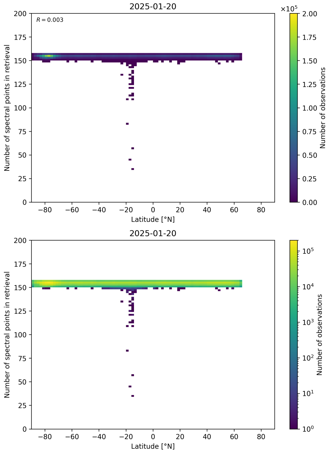
Figure 57: Scatter density plot of “Latitude” against “Number of spectral points in retrieval” for 2025-01-19 to 2025-01-21.
