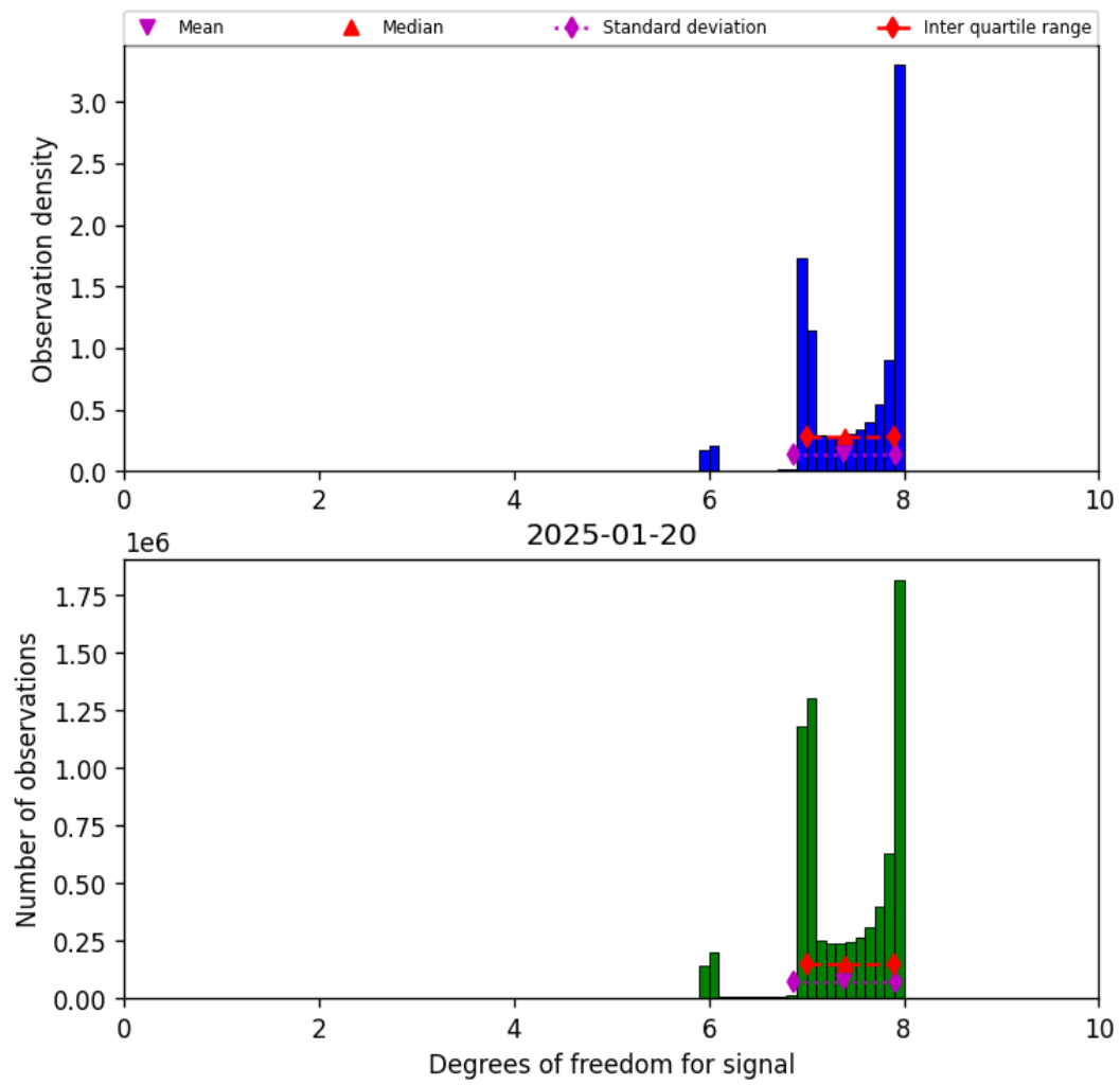
Figure 23: Histogram of “Degrees of freedom for signal” for 2025-01-19 to 2025-01-21
