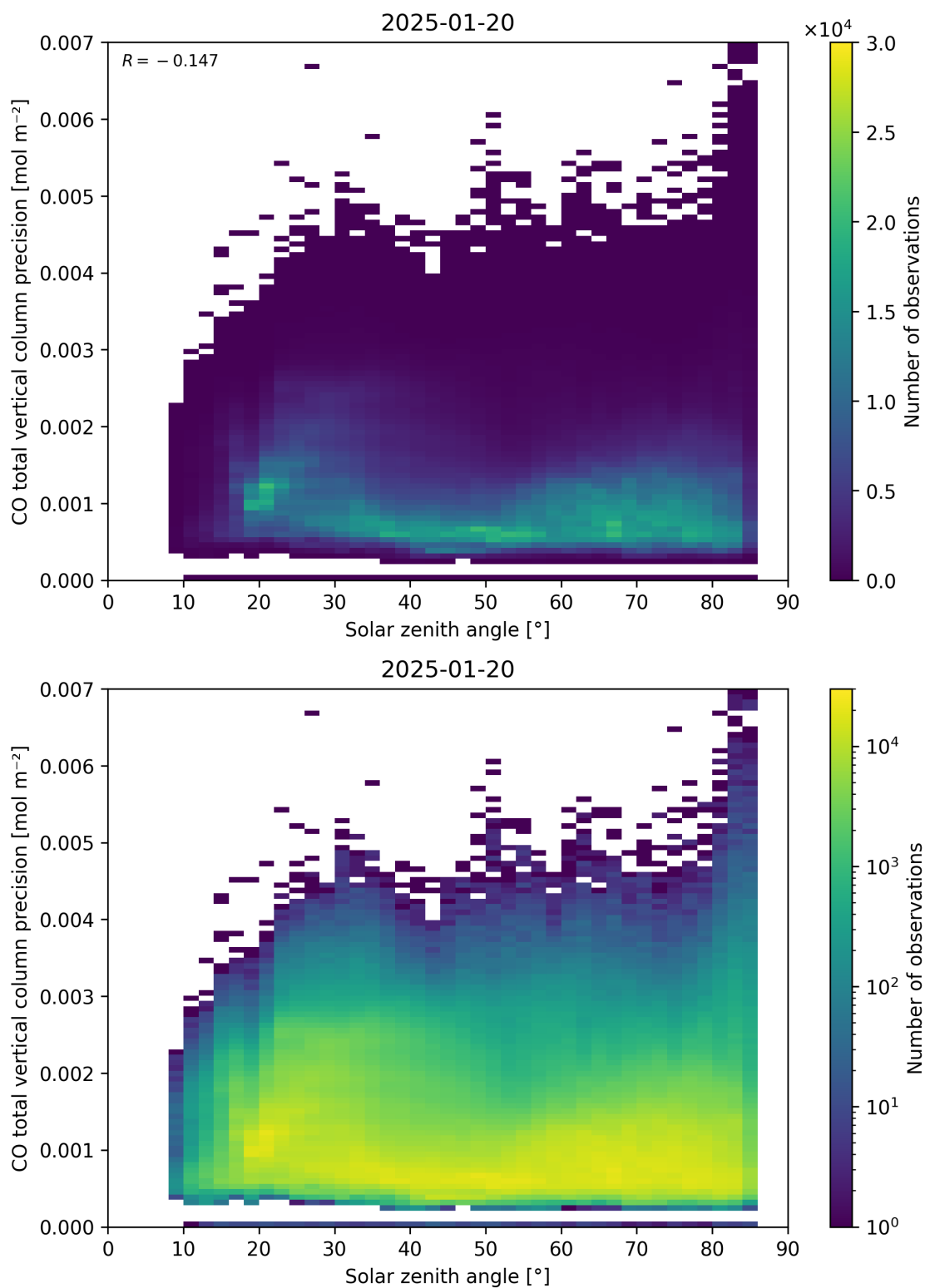
Figure 63: Scatter density plot of “Solar zenith angle” against “CO total vertical column precision” for 2025-01-19 to 2025-01-21.
