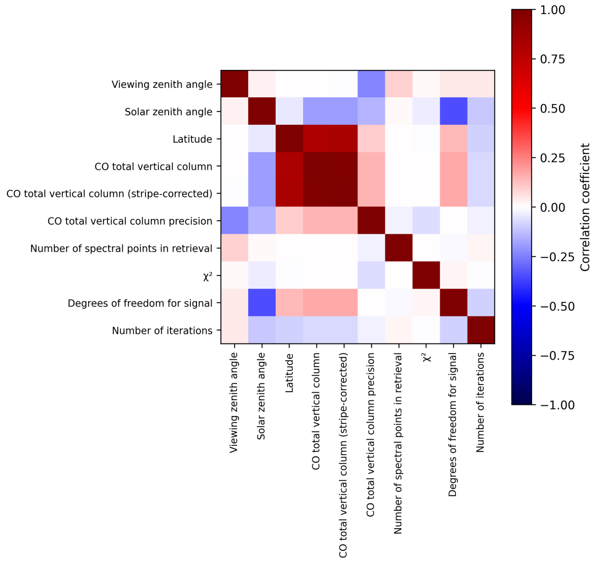
Figure 2: Map of correlation matrix for 2025-01-19 to 2025-01-21.
