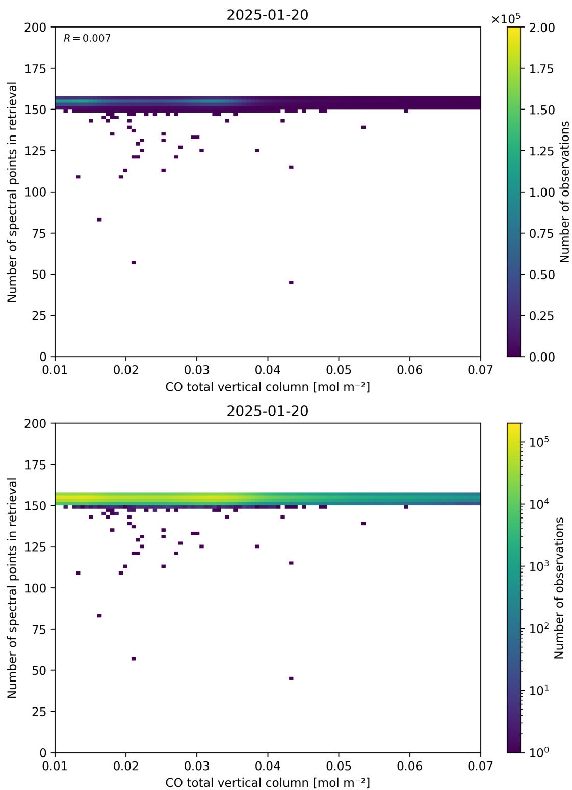
Figure 43: Scatter density plot of “CO total vertical column” against “Number of spectral points in retrieval” for 2025-01-19 to 2025-01-21.
