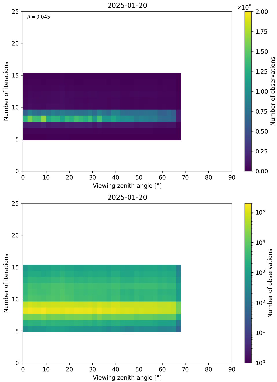
Figure 75: Scatter density plot of “Viewing zenith angle” against “Number of iterations” for 2025-01-19 to 2025-01-21.
