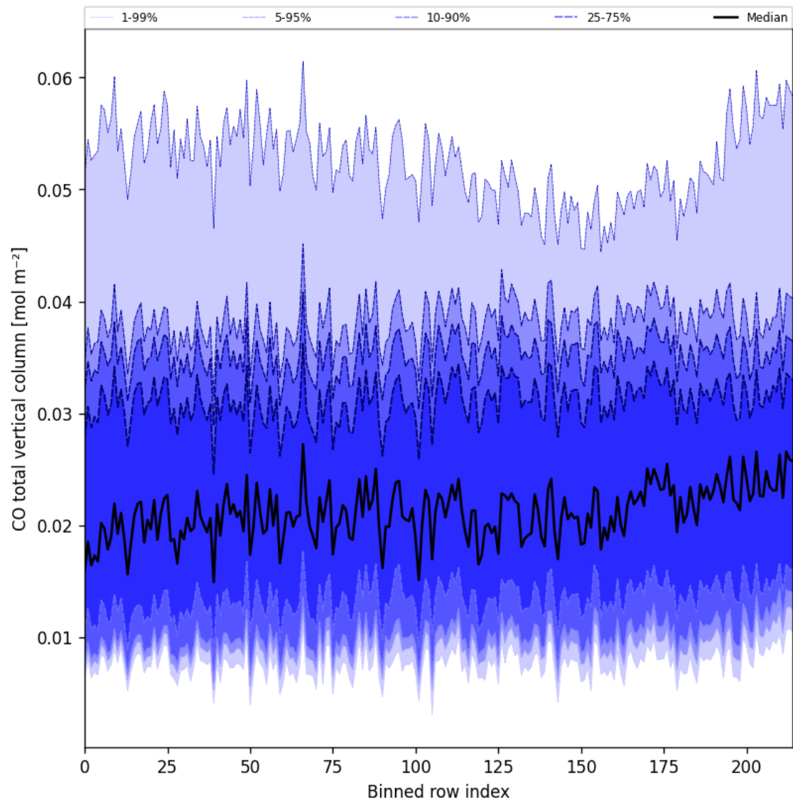
Figure 26: Along track statistics of “CO total vertical column” for 2025-01-19 to 2025-01-21
