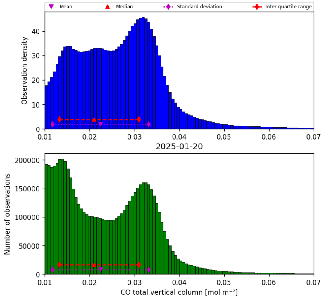
Figure 18: Histogram of “CO total vertical column” for 2025-01-19 to 2025-01-21
