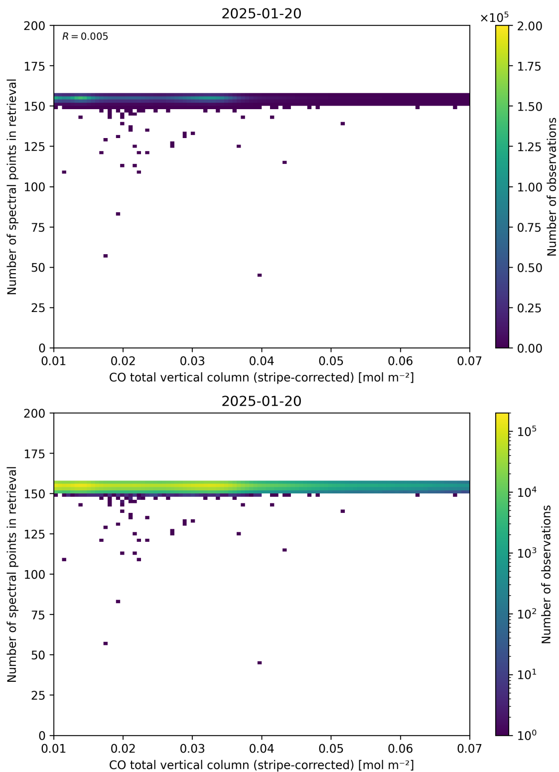
Figure 40: Scatter density plot of “CO total vertical column (stripe-corrected)” against “Number of spectral points in retrieval” for 2025-01-19 to 2025-01-21.
