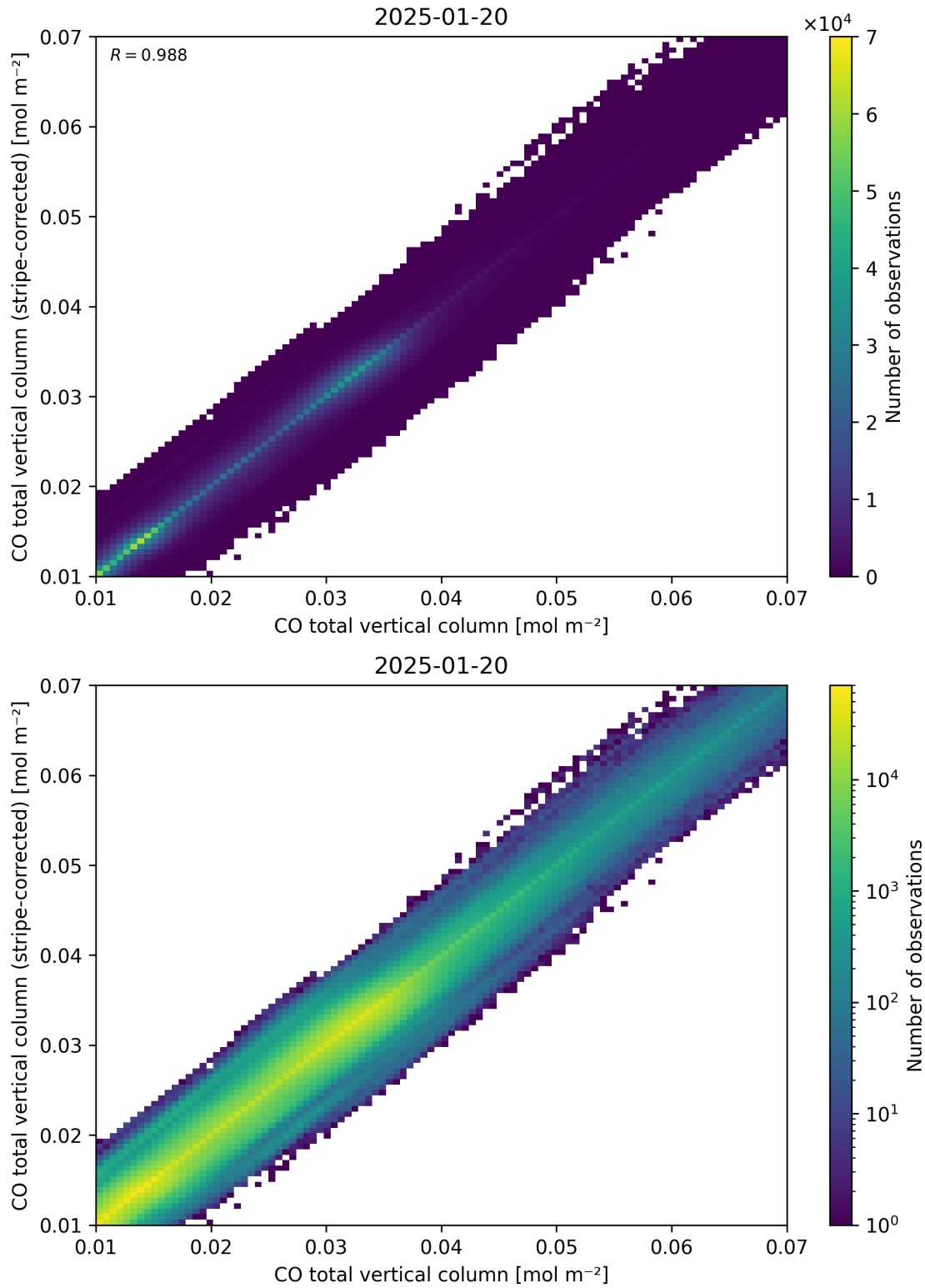
Figure 33: Scatter density plot of “CO total vertical column” against “CO total vertical column (stripe-corrected)” for 2025-01-19 to 2025-01-21.
