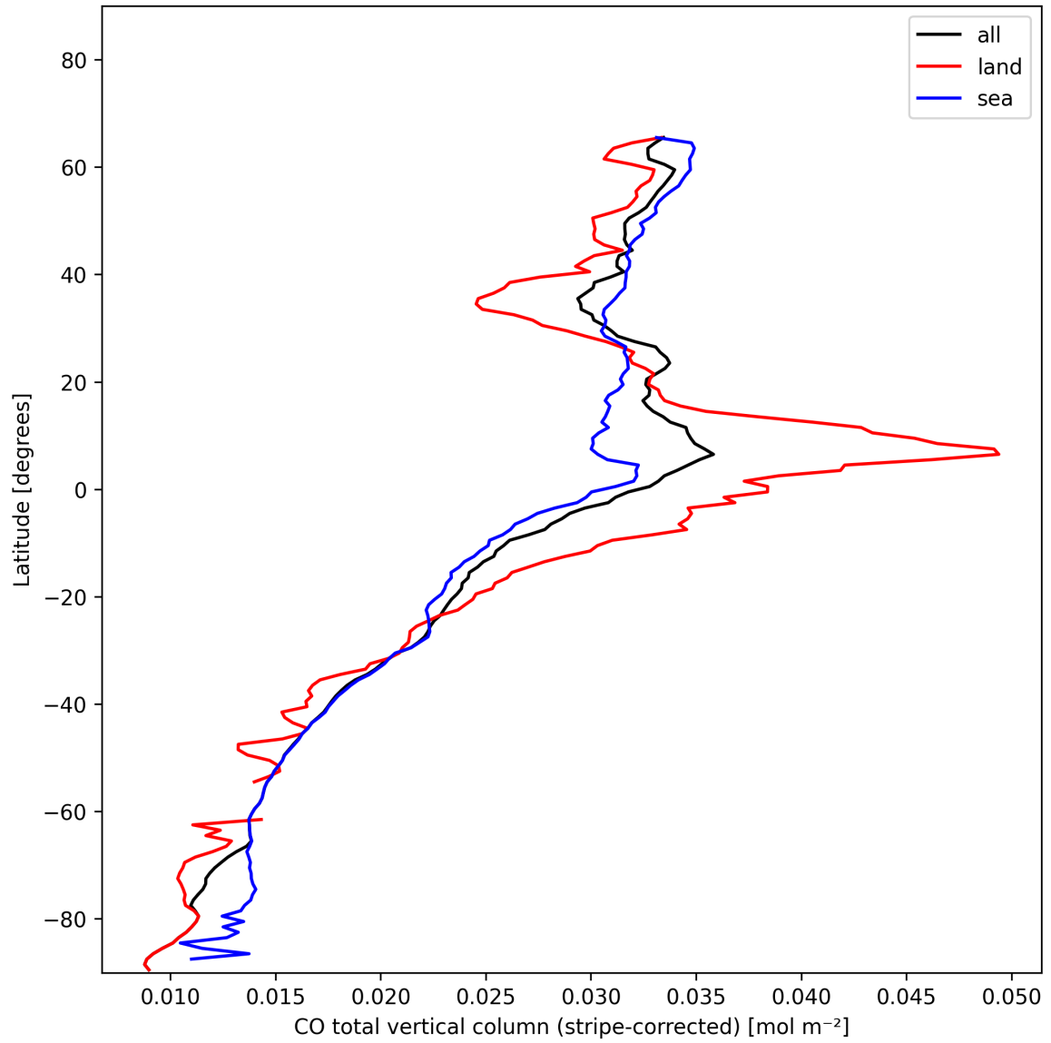
Figure 11: Zonal average of “CO total vertical column (stripe-corrected)” for 2025-01-19 to 2025-01-21.
