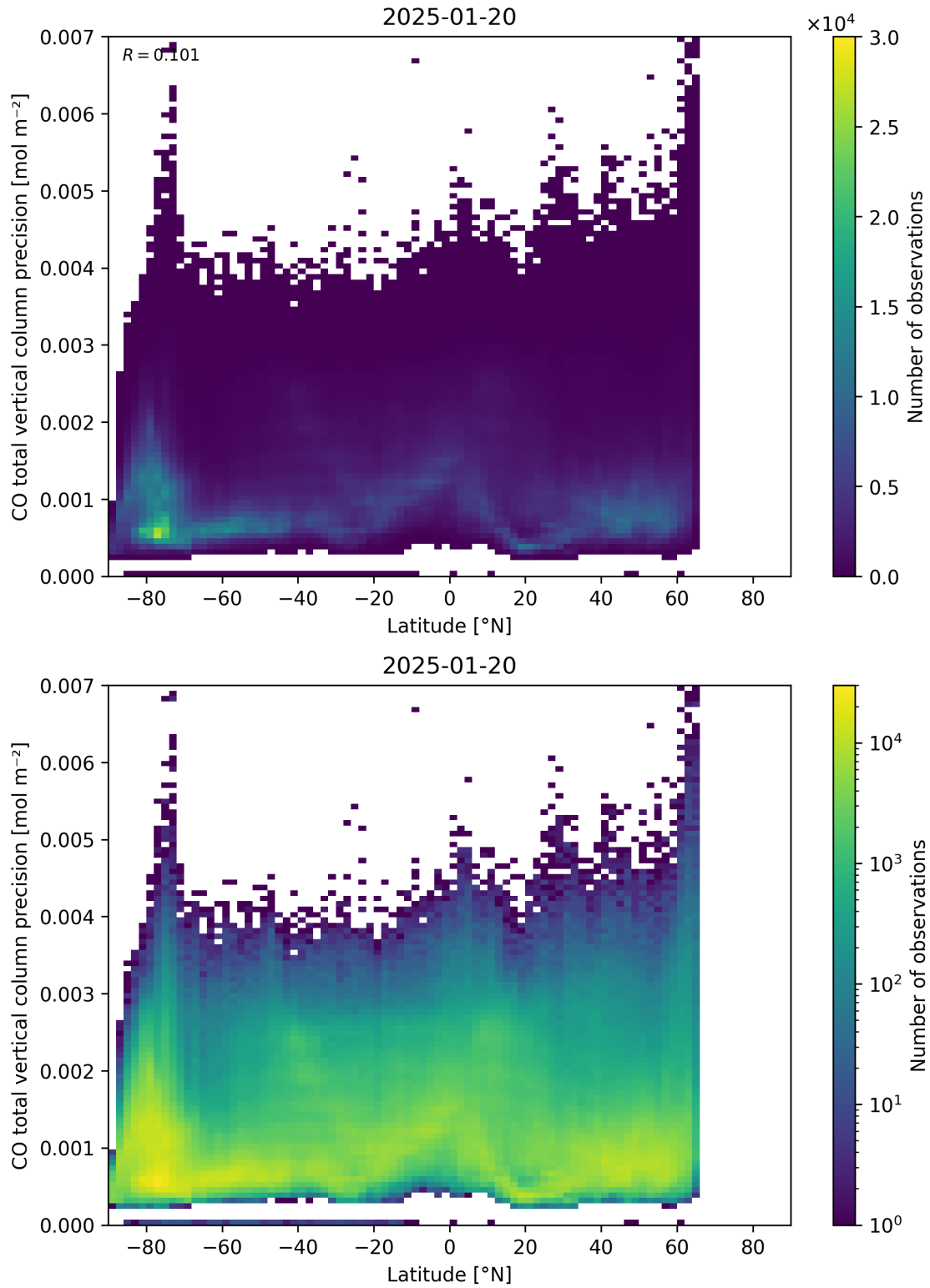
Figure 53: Scatter density plot of “Latitude” against “CO total vertical column precision” for 2025-01-19 to 2025-01-21.
