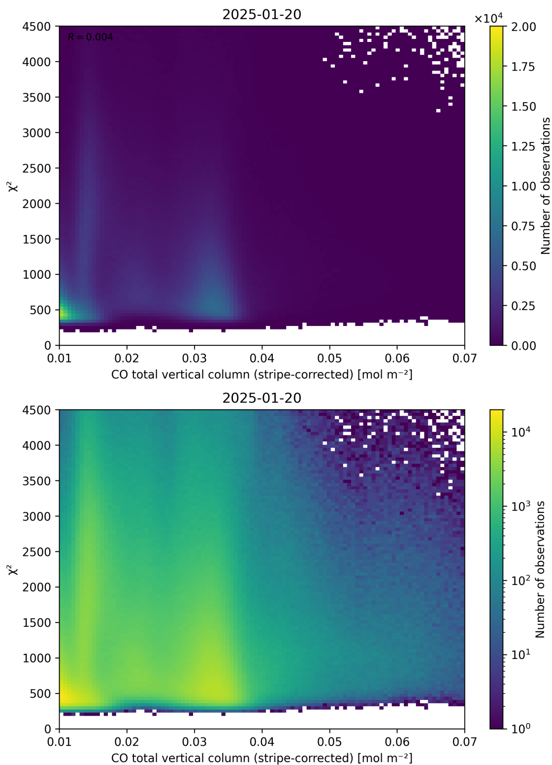
Figure 37: Scatter density plot of “CO total vertical column (stripe-corrected)” against “ \chi^2 ” for 2025-01-19 to 2025-01-21.
