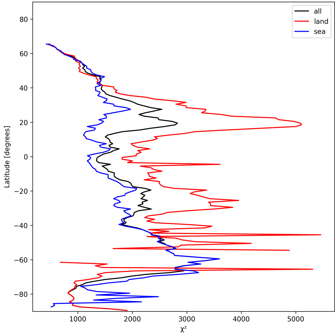
Figure 14: Zonal average of “ \chi^2 ” for 2025-01-19 to 2025-01-21.
