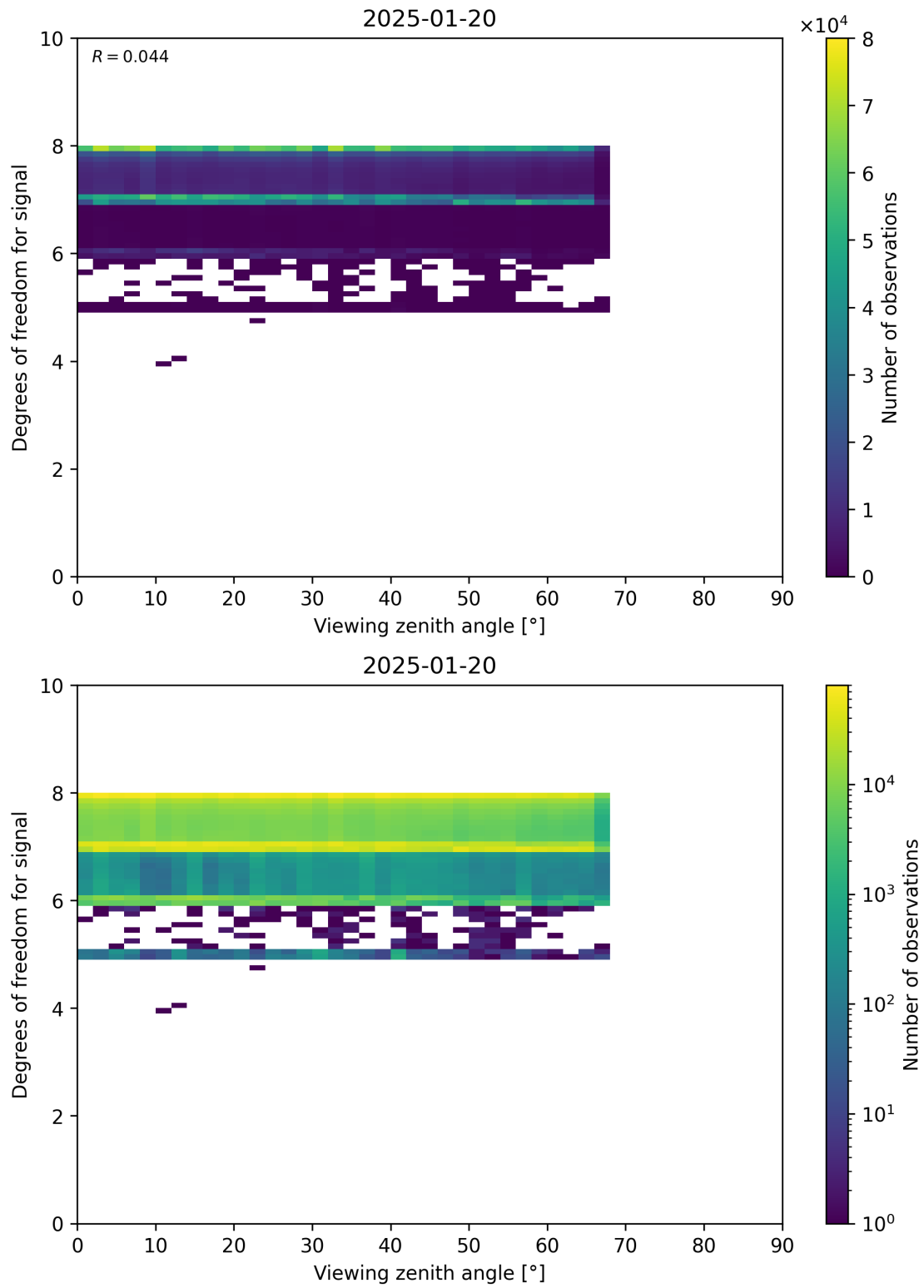
Figure 73: Scatter density plot of “Viewing zenith angle” against “Degrees of freedom for signal” for 2025-01-19 to 2025-01-21.
