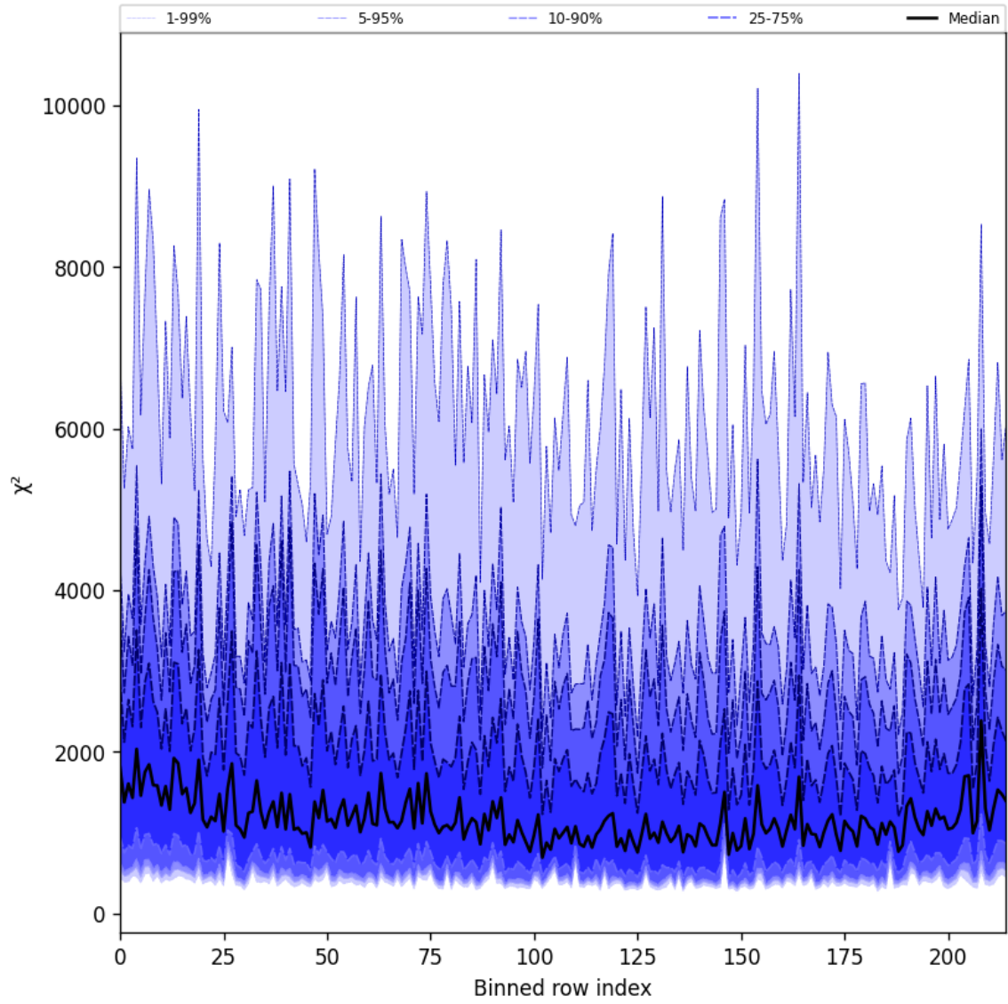
Figure 30: Along track statistics of “ \chi^2 ” for 2025-01-19 to 2025-01-21
