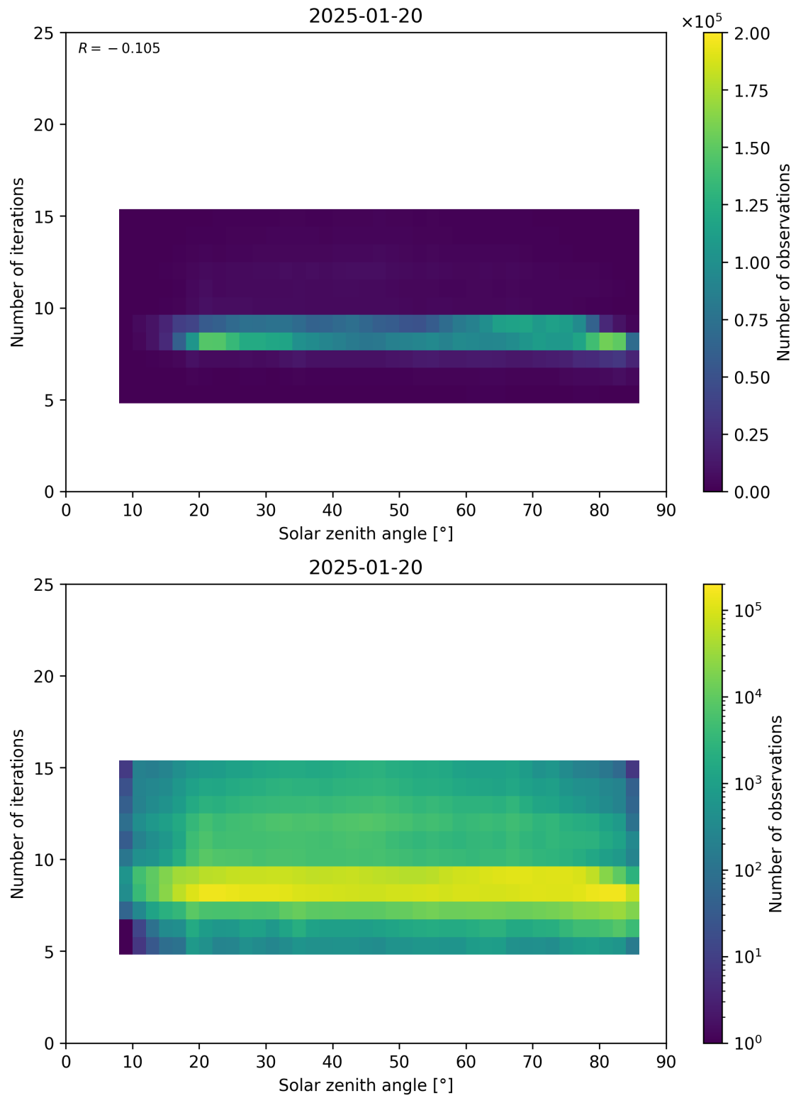
Figure 67: Scatter density plot of “Solar zenith angle” against “Number of iterations” for 2025-01-19 to 2025-01-21.
