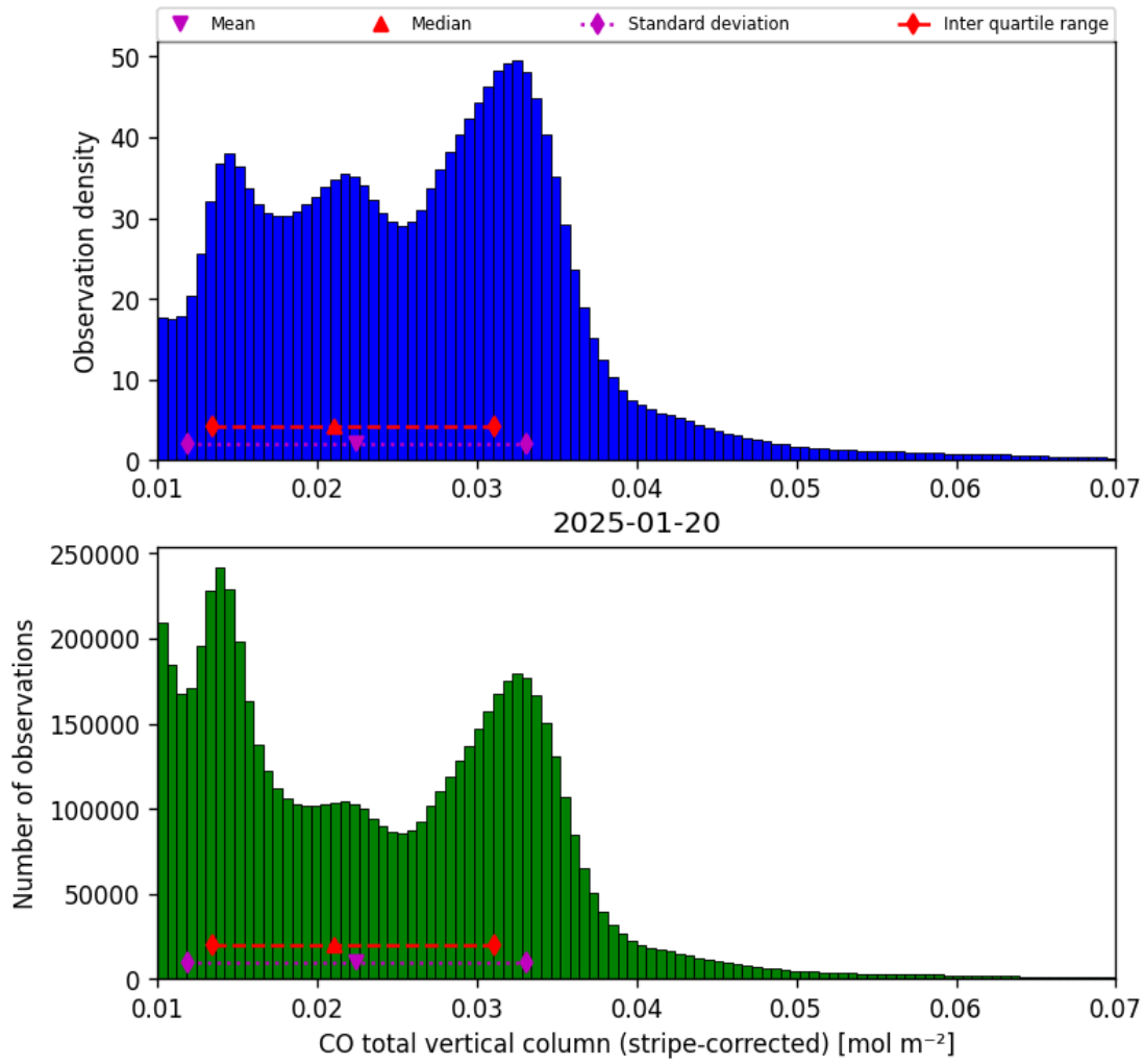
Figure 19: Histogram of “CO total vertical column (stripe-corrected)” for 2025-01-19 to 2025-01-21
