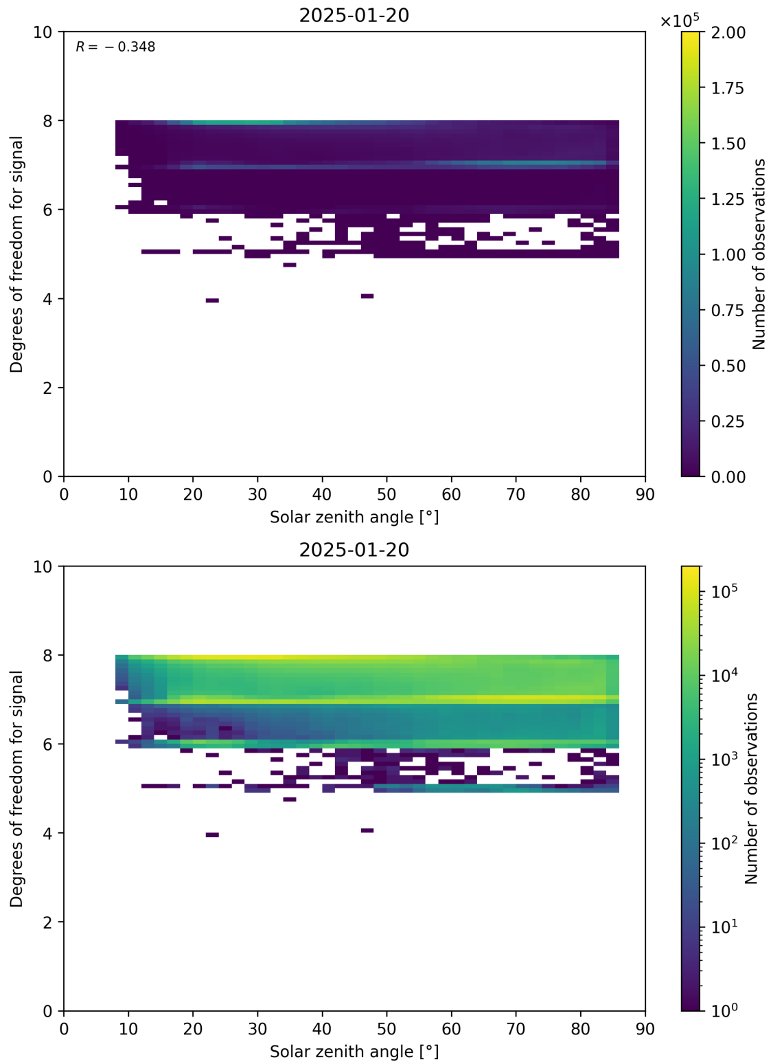
Figure 65: Scatter density plot of “Solar zenith angle” against “Degrees of freedom for signal” for 2025-01-19 to 2025-01-21.
