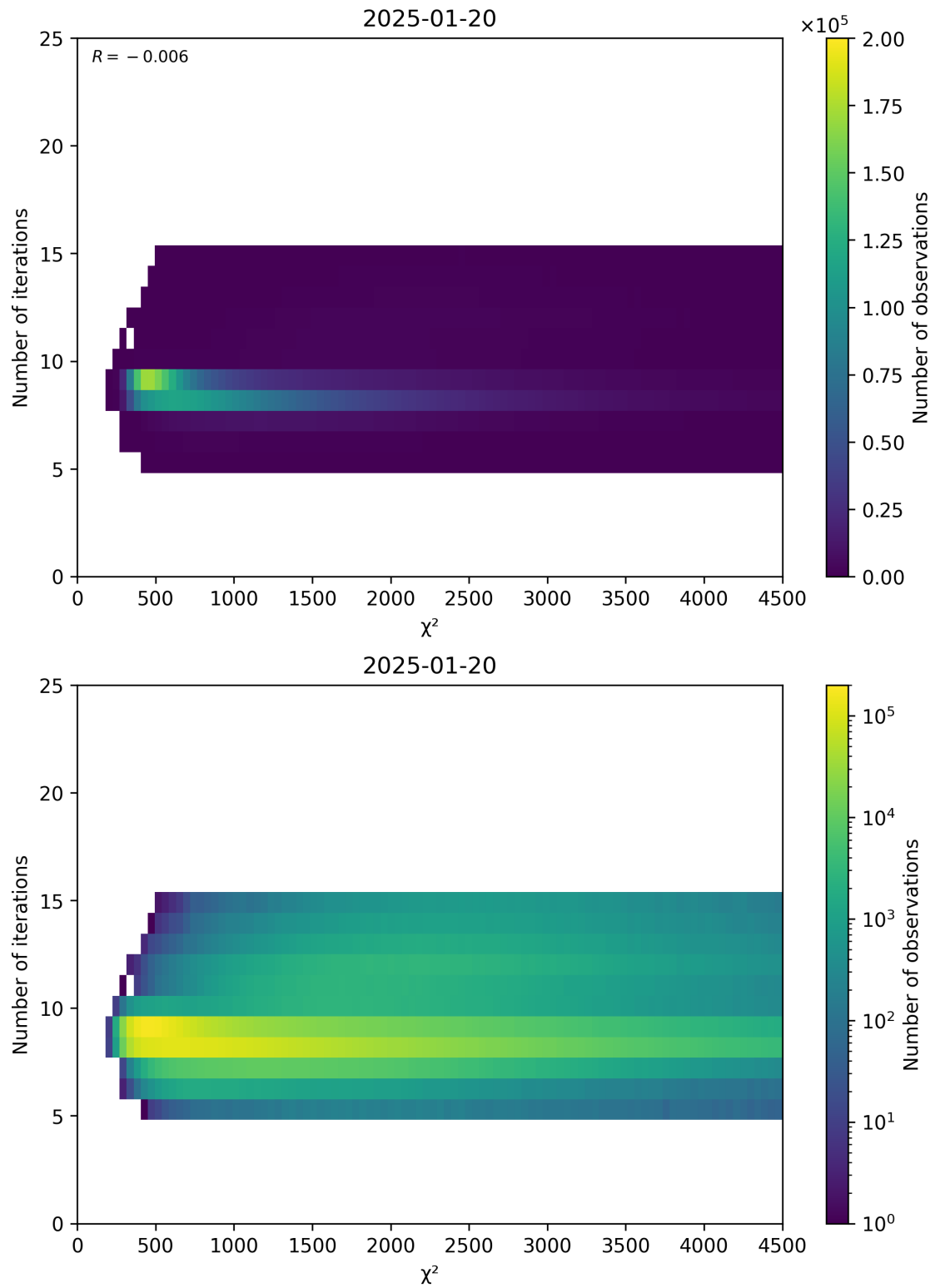
Figure 49: Scatter density plot of “ \chi^2 ” against “Number of iterations” for 2025-01-19 to 2025-01-21.
