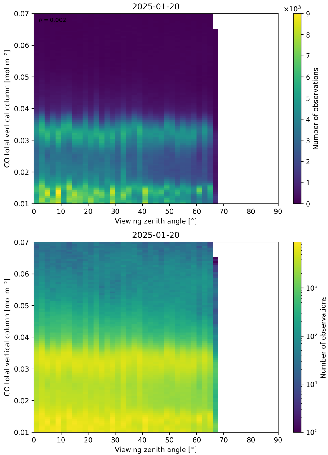
Figure 69: Scatter density plot of “Viewing zenith angle” against “CO total vertical column” for 2025-01-19 to 2025-01-21.
