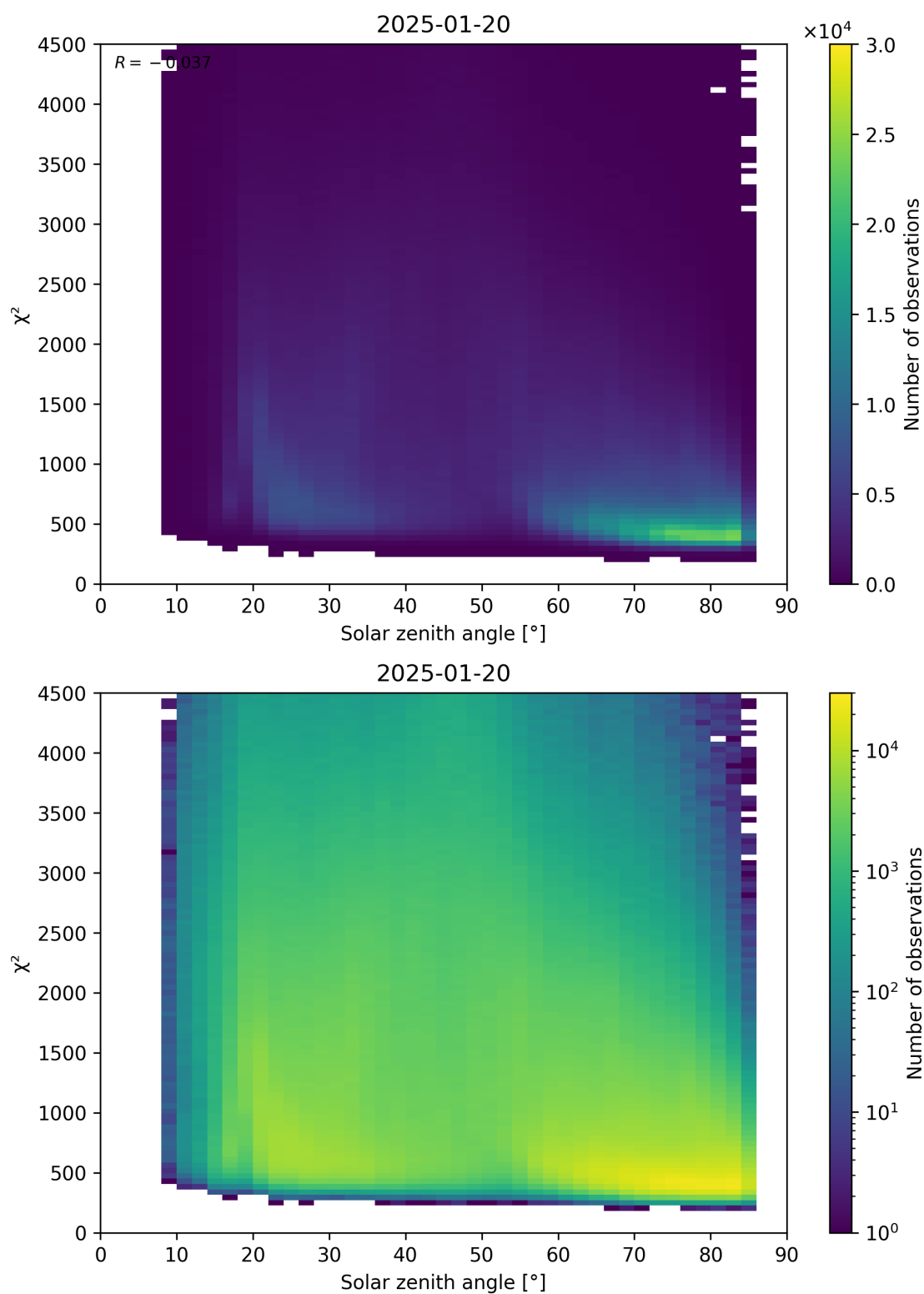
Figure 64: Scatter density plot of “Solar zenith angle” against “ \chi^2 ” for 2025-01-19 to 2025-01-21.
