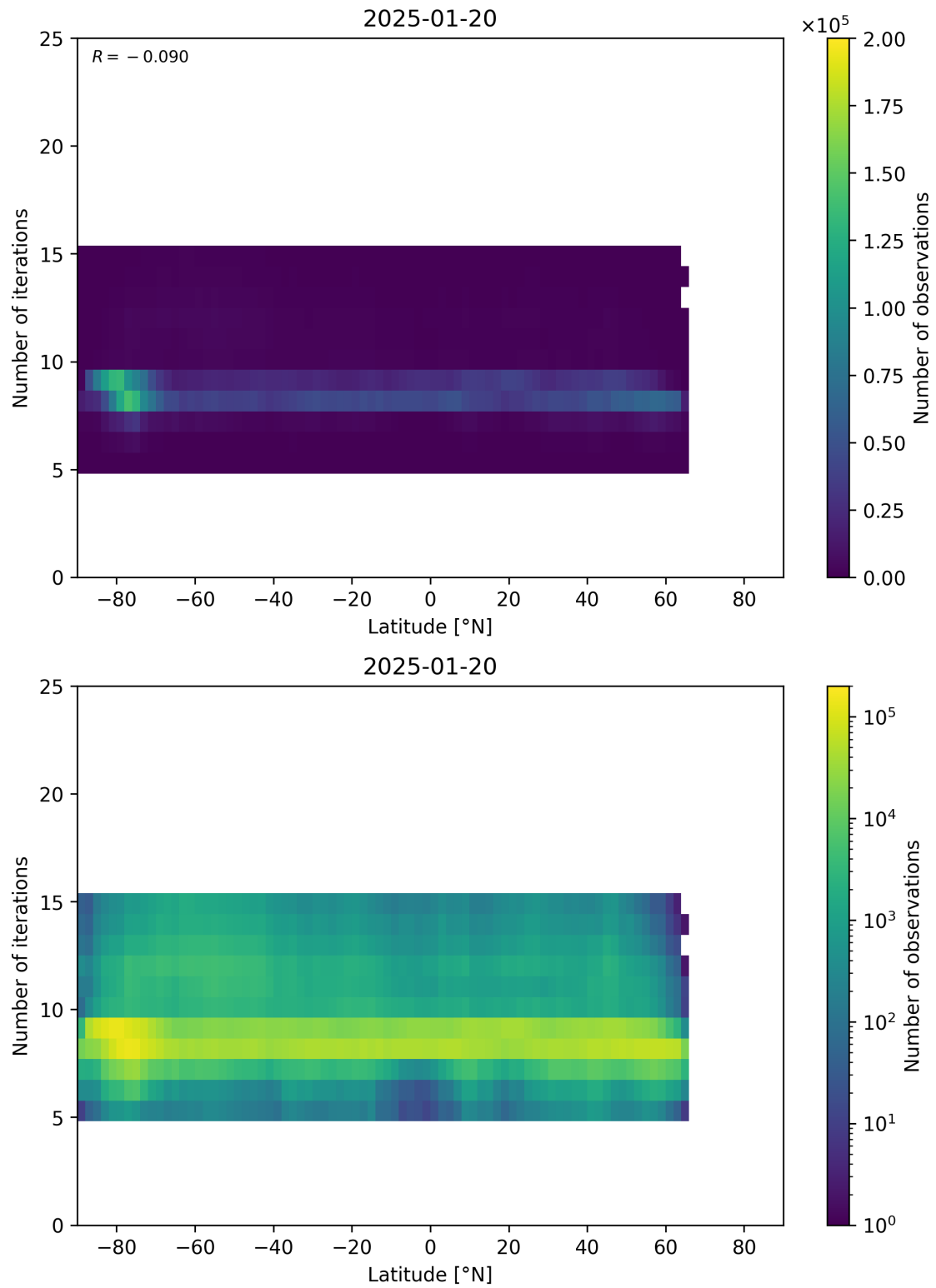
Figure 56: Scatter density plot of “Latitude” against “Number of iterations” for 2025-01-19 to 2025-01-21.
