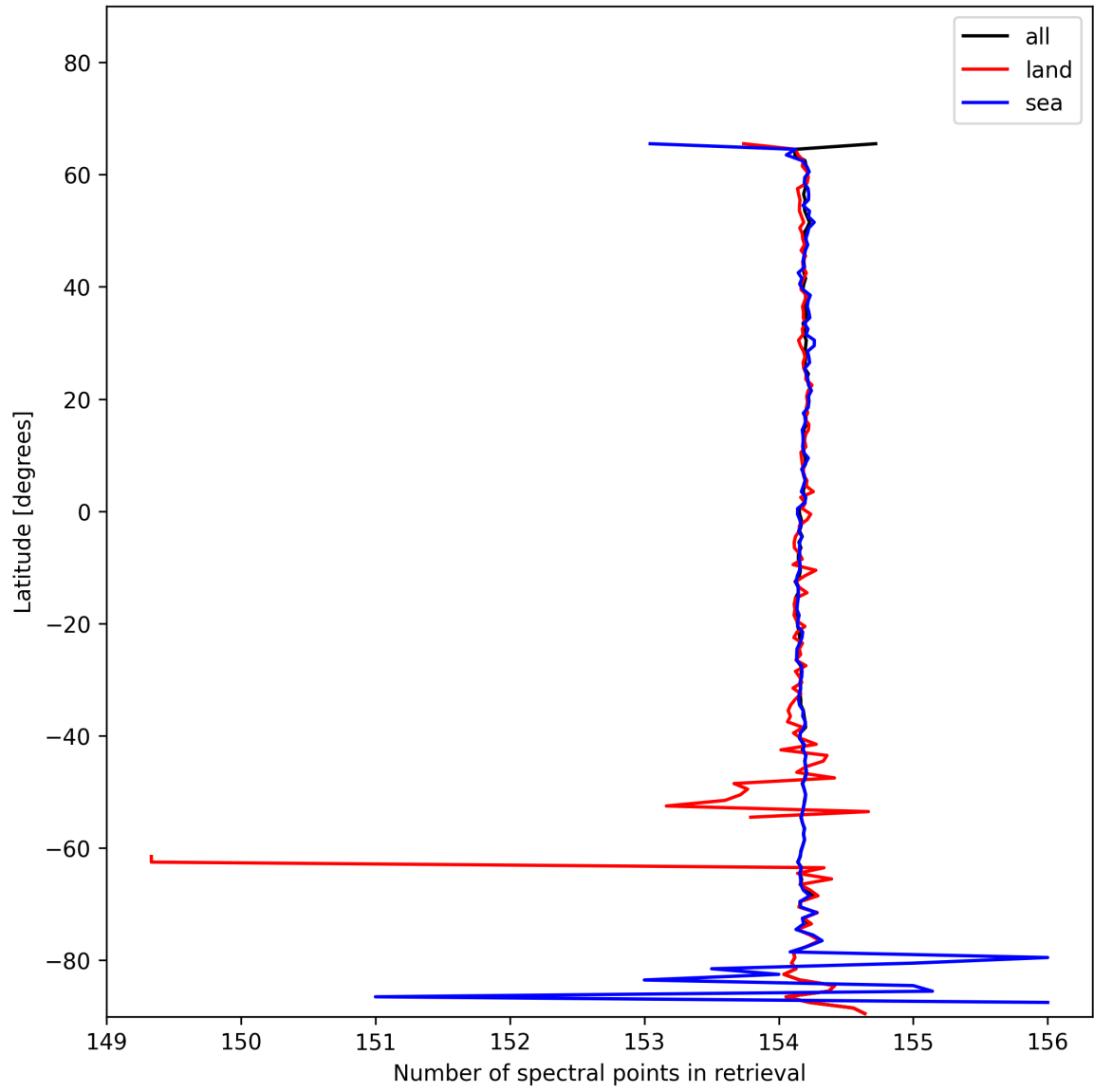
Figure 13: Zonal average of “Number of spectral points in retrieval” for 2025-01-19 to 2025-01-21.
