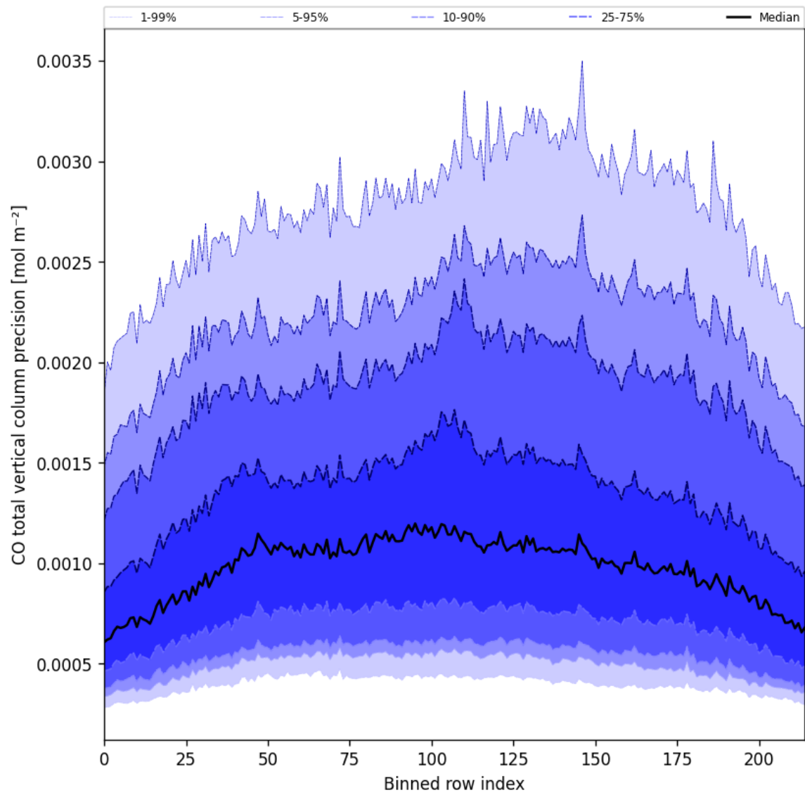
Figure 28: Along track statistics of “CO total vertical column precision” for 2025-01-19 to 2025-01-21
