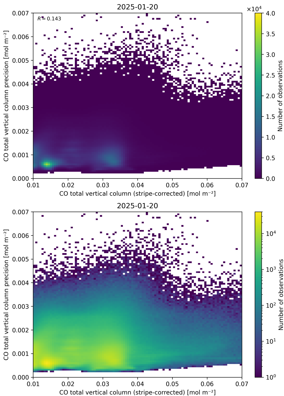
Figure 36: Scatter density plot of “CO total vertical column (stripe-corrected)” against “CO total vertical column precision” for 2025-01-19 to 2025-01-21.
