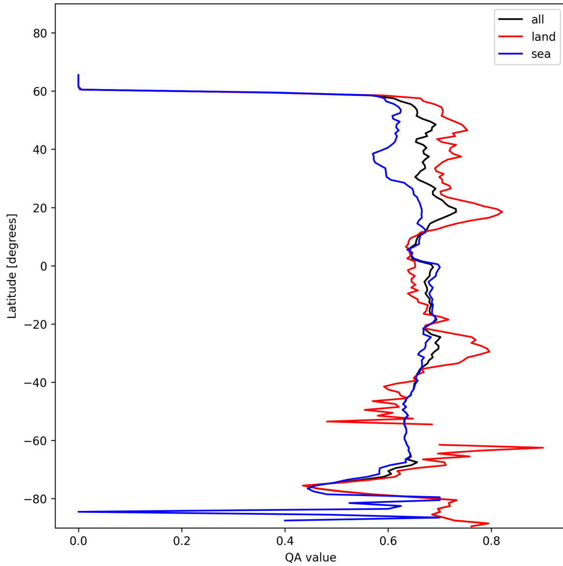
Figure 9: Zonal average of “QA value” for 2025-01-19 to 2025-01-21.
