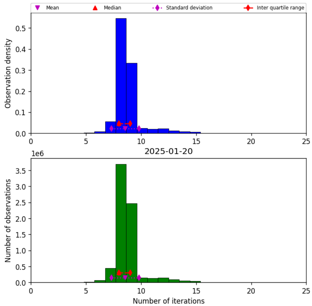
Figure 24: Histogram of “Number of iterations” for 2025-01-19 to 2025-01-21
