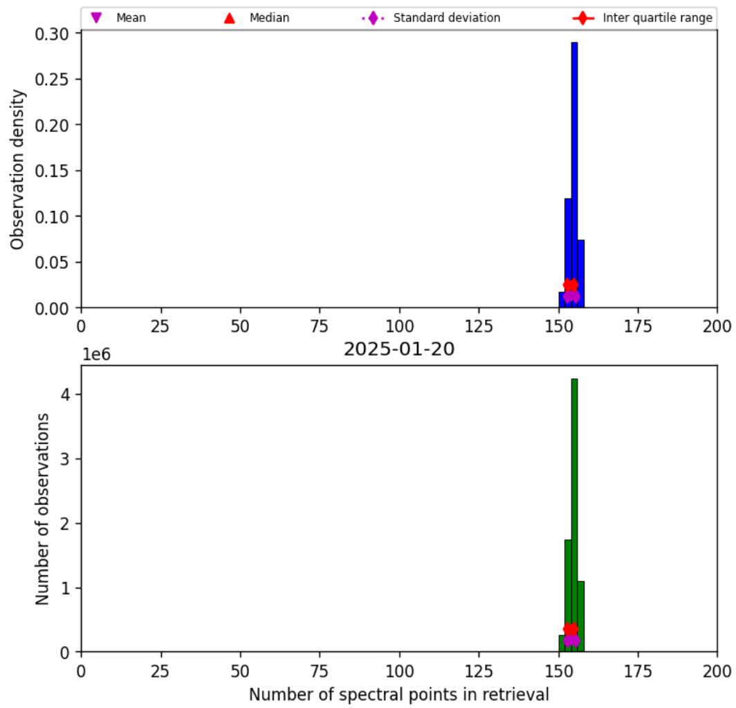
Figure 21: Histogram of “Number of spectral points in retrieval” for 2025-01-19 to 2025-01-21
