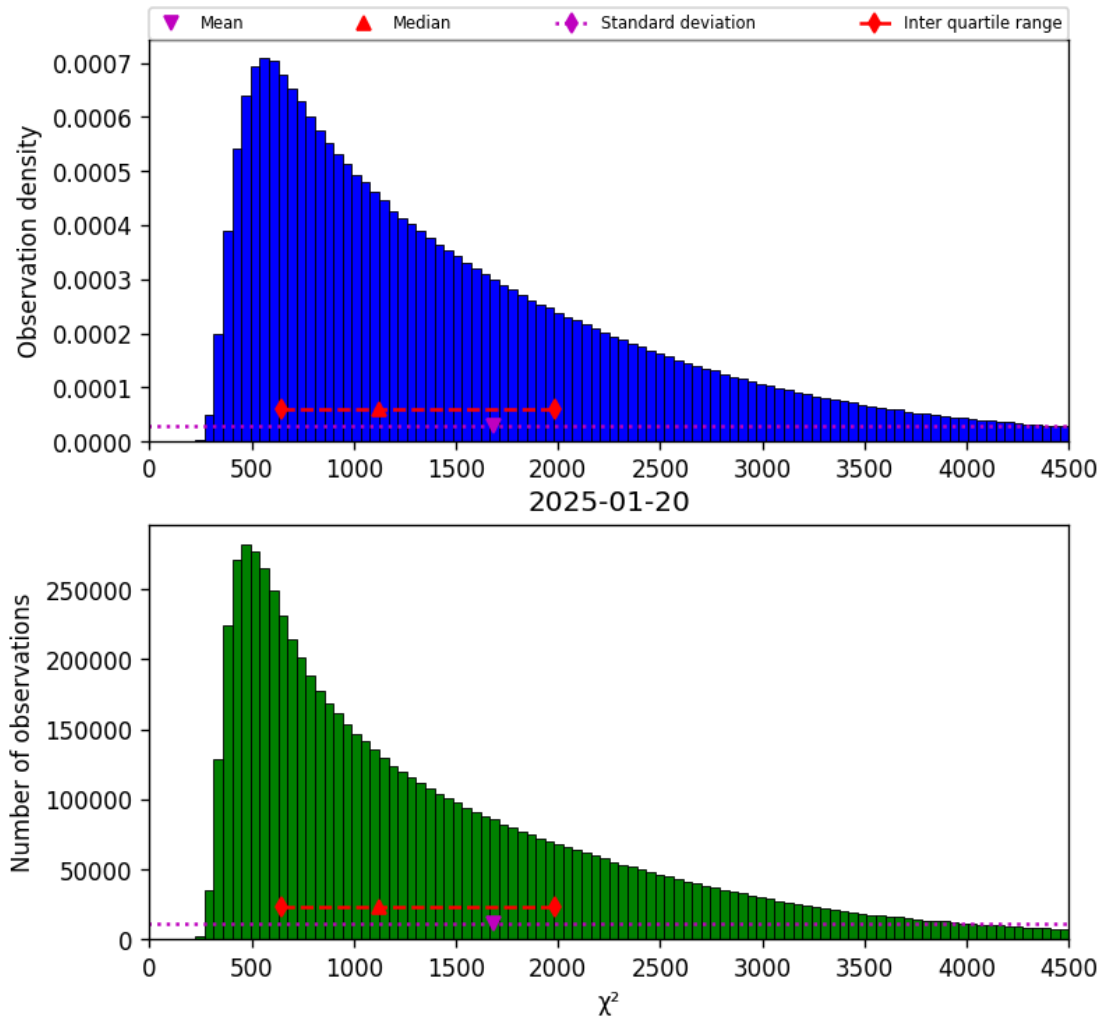
Figure 22: Histogram of “ \chi^2 ” for 2025-01-19 to 2025-01-21
