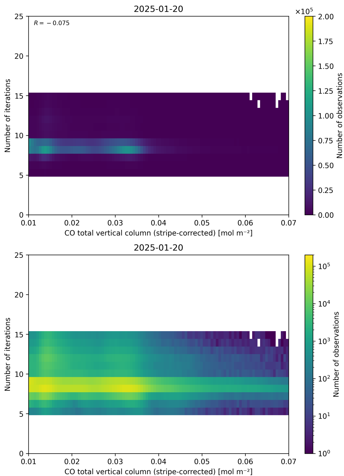
Figure 39: Scatter density plot of “CO total vertical column (stripe-corrected)” against “Number of iterations” for 2025-01-19 to 2025-01-21.
