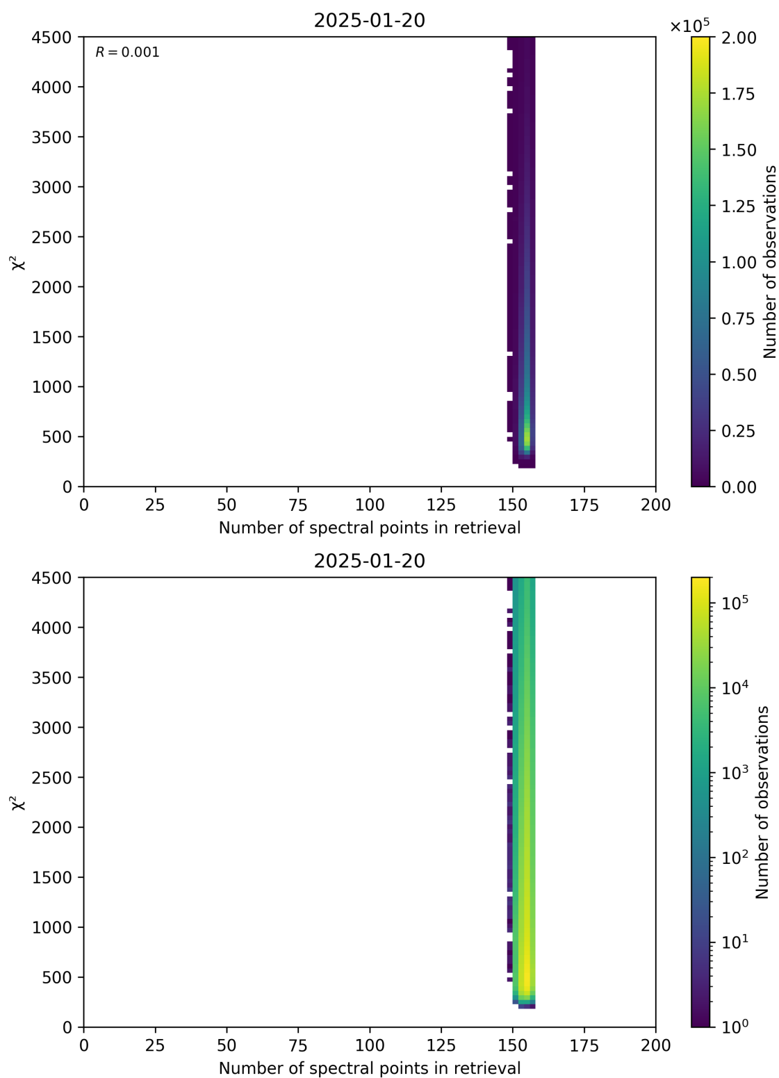
Figure 58: Scatter density plot of “Number of spectral points in retrieval” against “ \chi^2 ” for 2025-01-19 to 2025-01-21.
