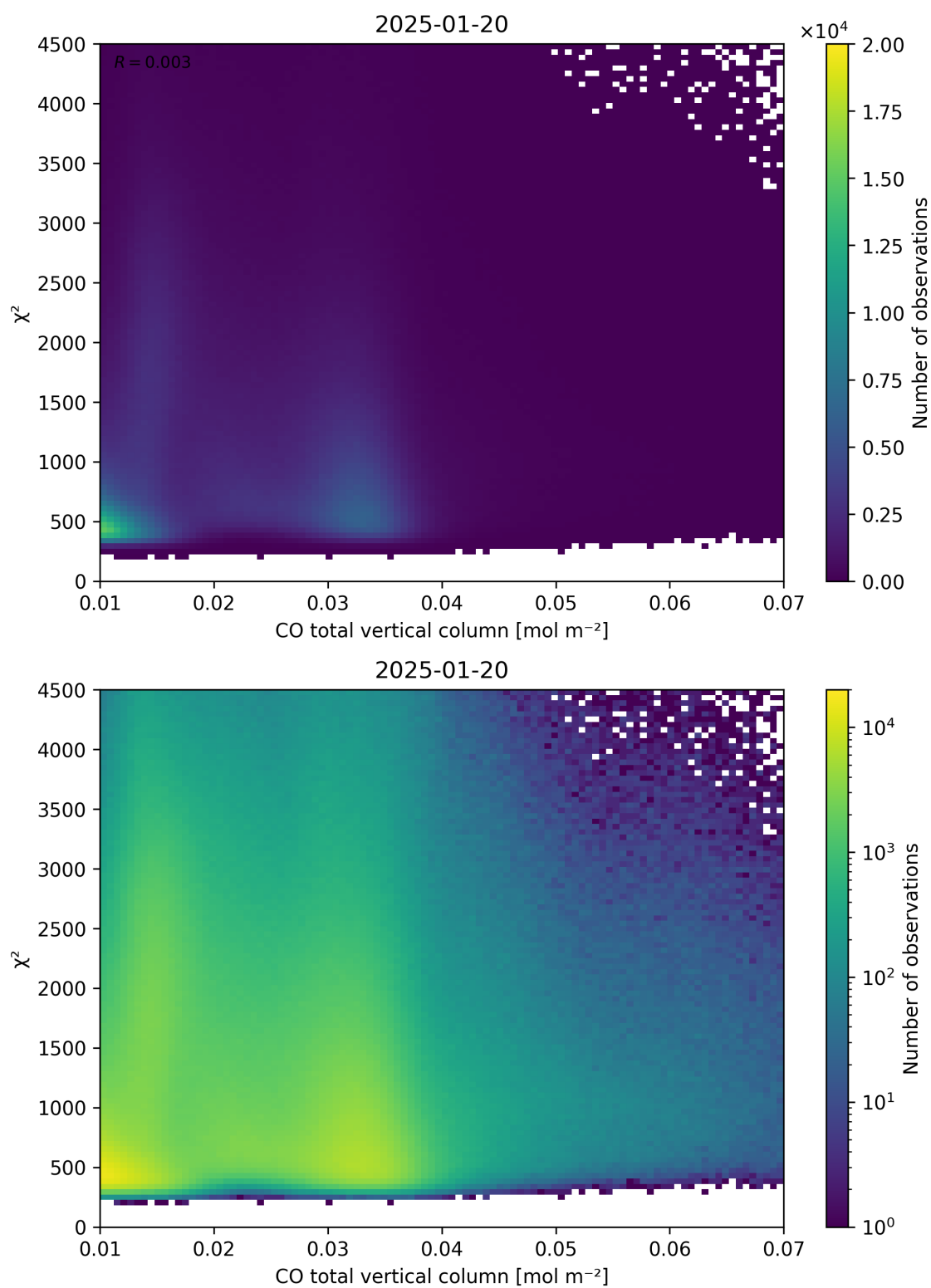
Figure 35: Scatter density plot of “CO total vertical column” against “ \chi^2 ” for 2025-01-19 to 2025-01-21.
