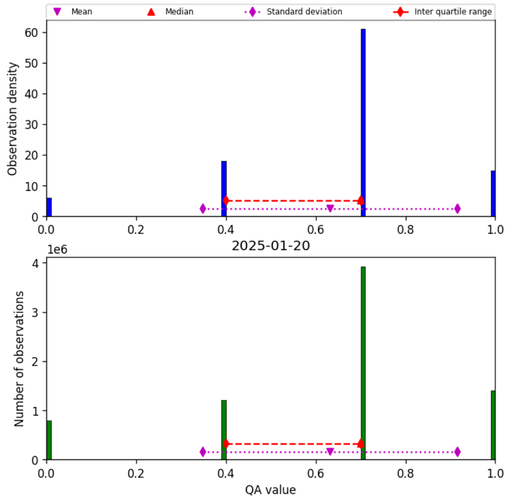
Figure 17: Histogram of “QA value” for 2025-01-19 to 2025-01-21
