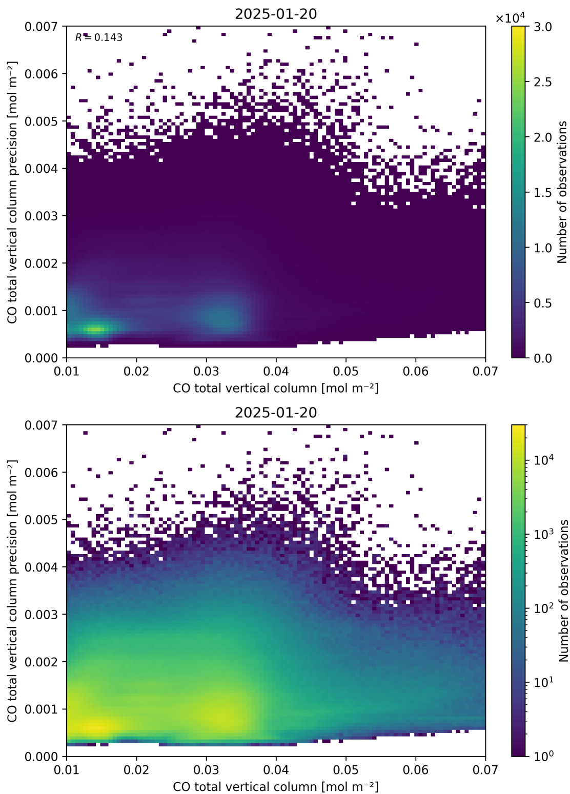
Figure 34: Scatter density plot of “CO total vertical column” against “CO total vertical column precision” for 2025-01-19 to 2025-01-21.
