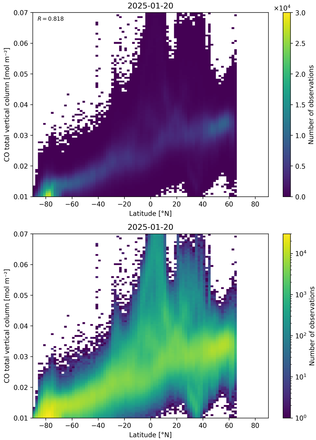
Figure 51: Scatter density plot of “Latitude” against “CO total vertical column” for 2025-01-19 to 2025-01-21.
