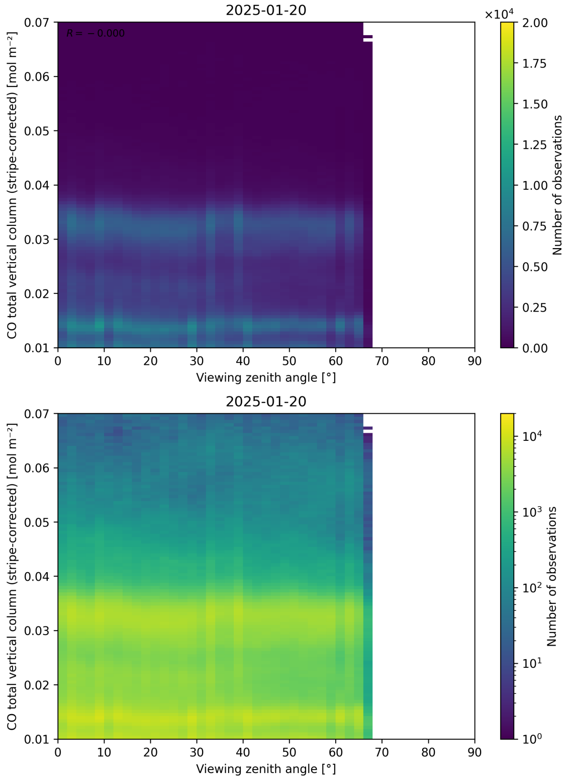
Figure 70: Scatter density plot of “Viewing zenith angle” against “CO total vertical column (stripe-corrected)” for 2025-01-19 to 2025-01-21.
