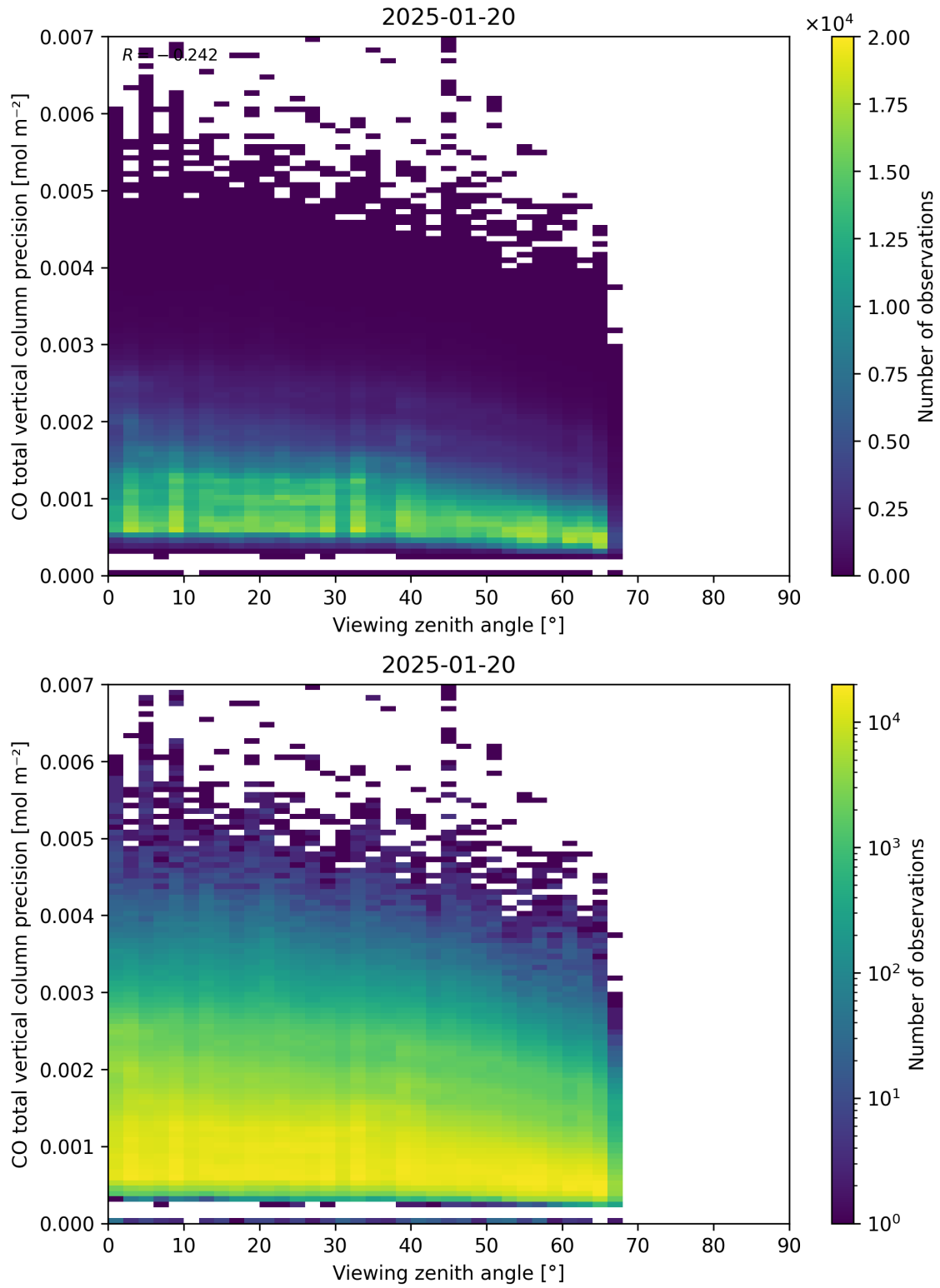
Figure 71: Scatter density plot of “Viewing zenith angle” against “CO total vertical column precision” for 2025-01-19 to 2025-01-21.
