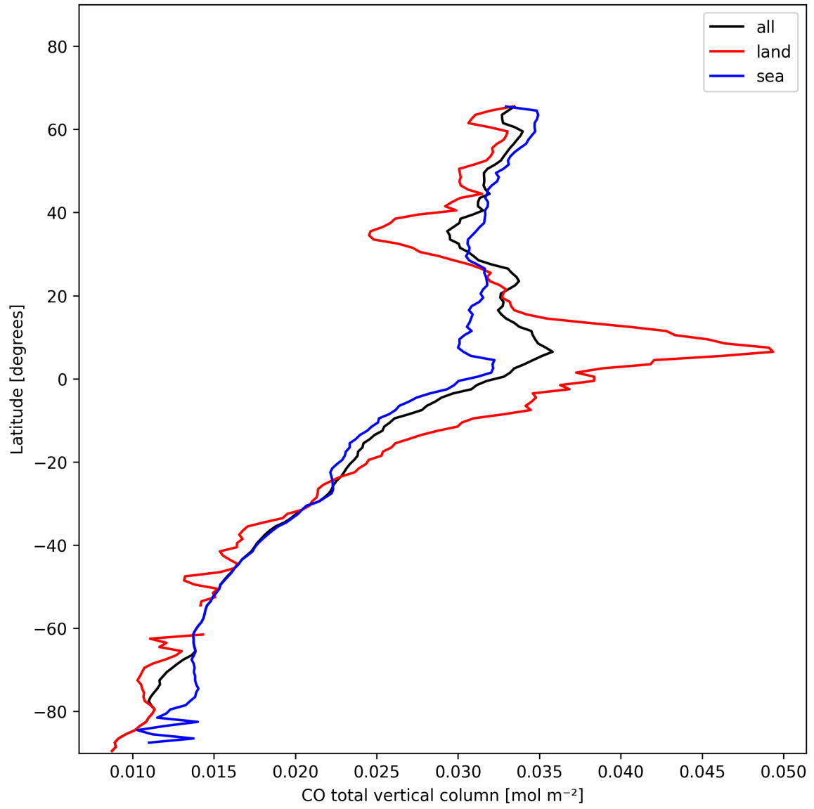
Figure 10: Zonal average of “CO total vertical column” for 2025-01-19 to 2025-01-21.
