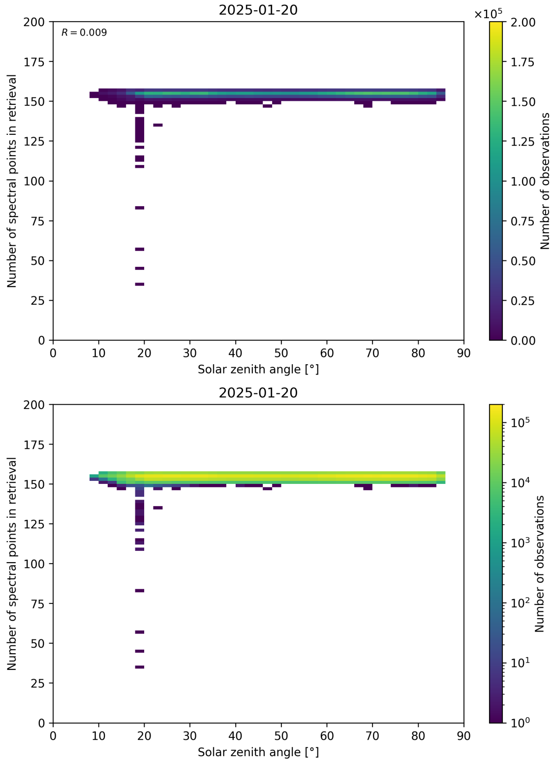
Figure 68: Scatter density plot of “Solar zenith angle” against “Number of spectral points in retrieval” for 2025-01-19 to 2025-01-21.
