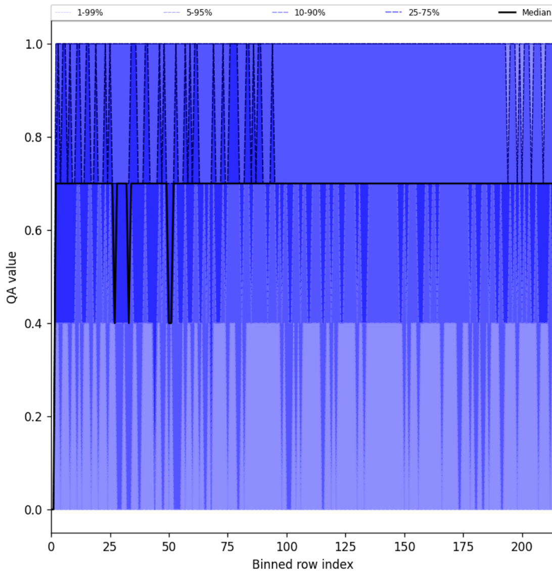
Figure 25: Along track statistics of “QA value” for 2025-01-19 to 2025-01-21
