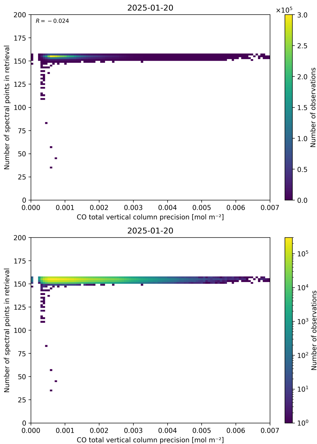
Figure 47: Scatter density plot of “CO total vertical column precision” against “Number of spectral points in retrieval” for 2025-01-19 to 2025-01-21.
