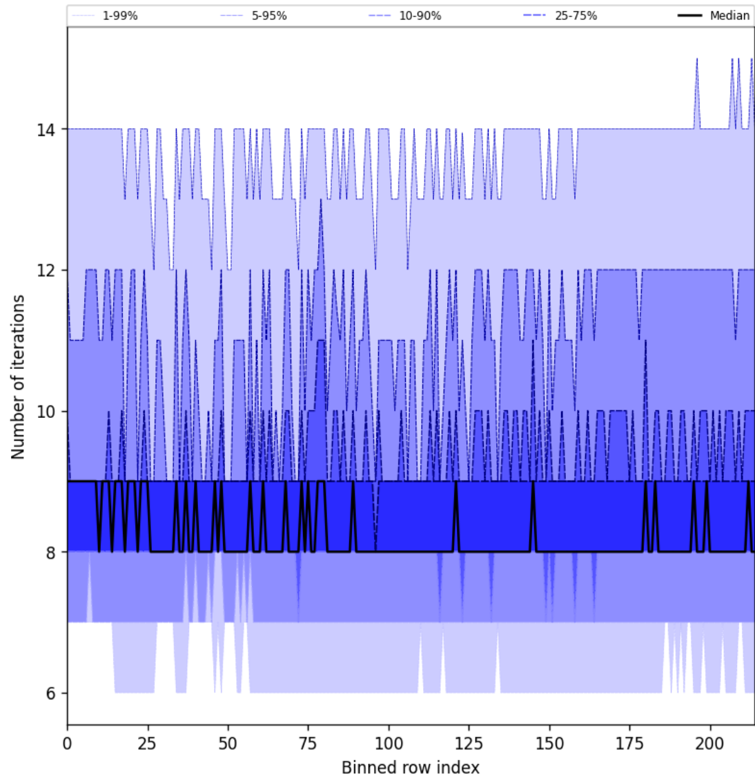
Figure 32: Along track statistics of “Number of iterations” for 2025-01-19 to 2025-01-21
