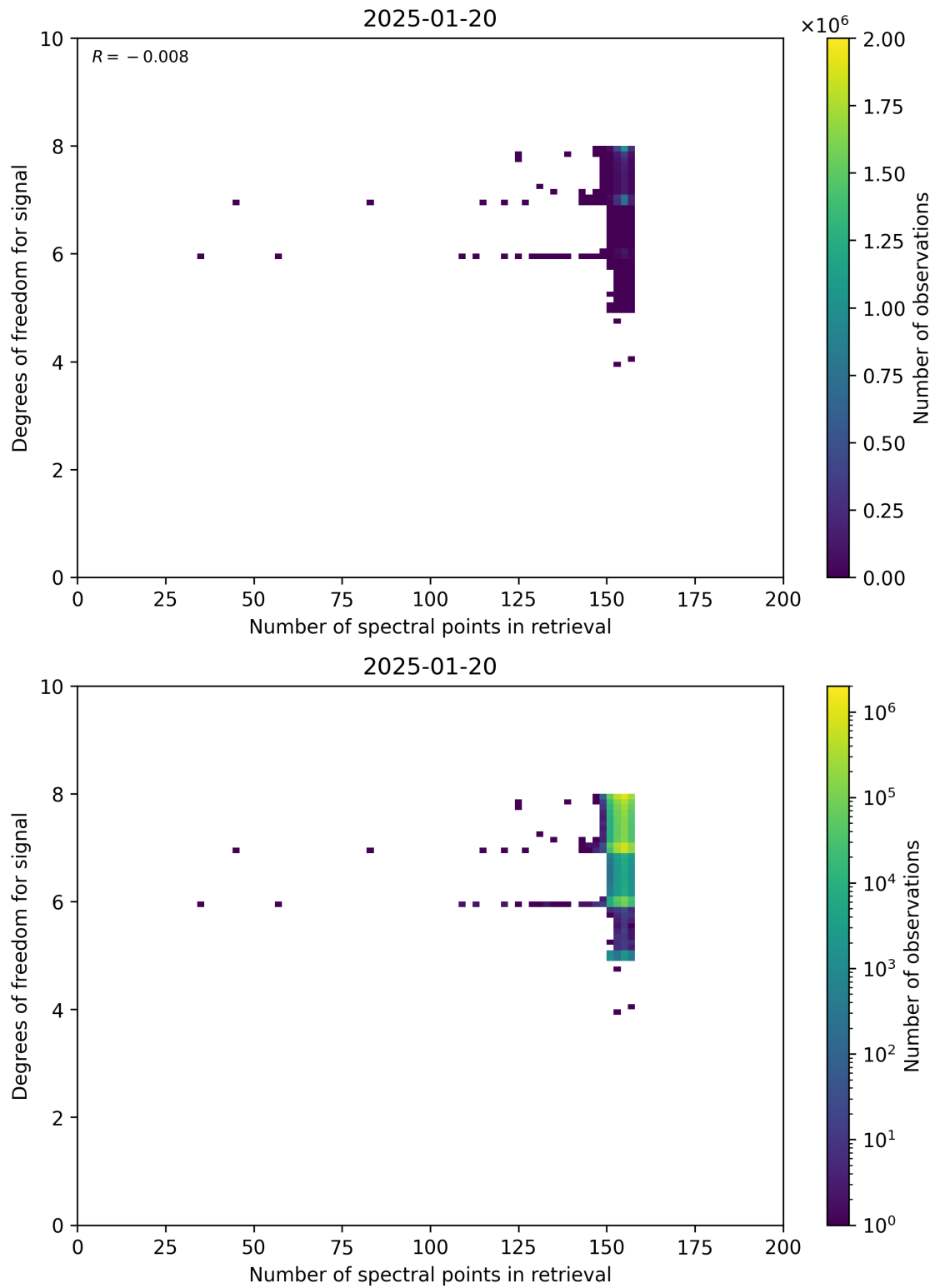
Figure 59: Scatter density plot of “Number of spectral points in retrieval” against “Degrees of freedom for signal” for 2025-01-19 to 2025-01-21.
