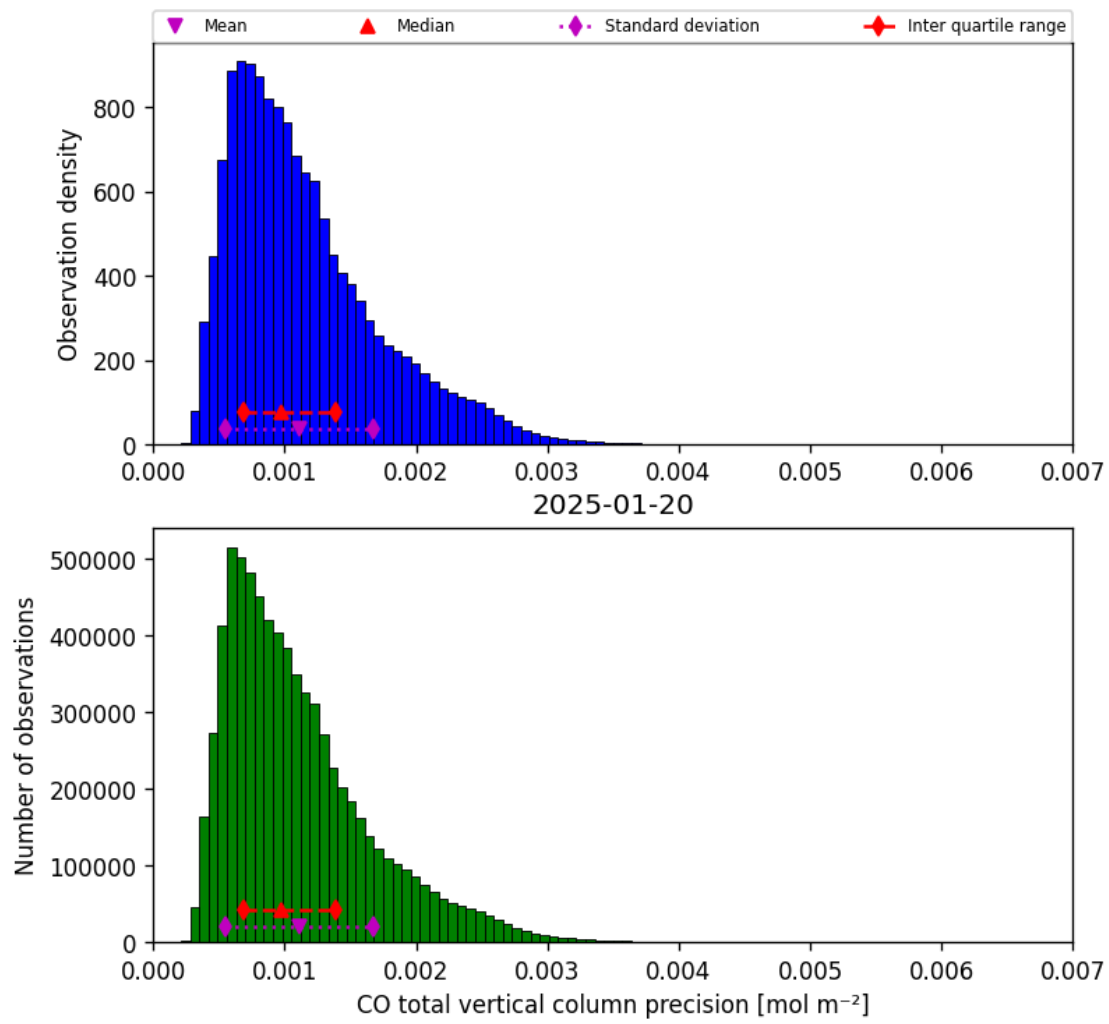
Figure 20: Histogram of “CO total vertical column precision” for 2025-01-19 to 2025-01-21
