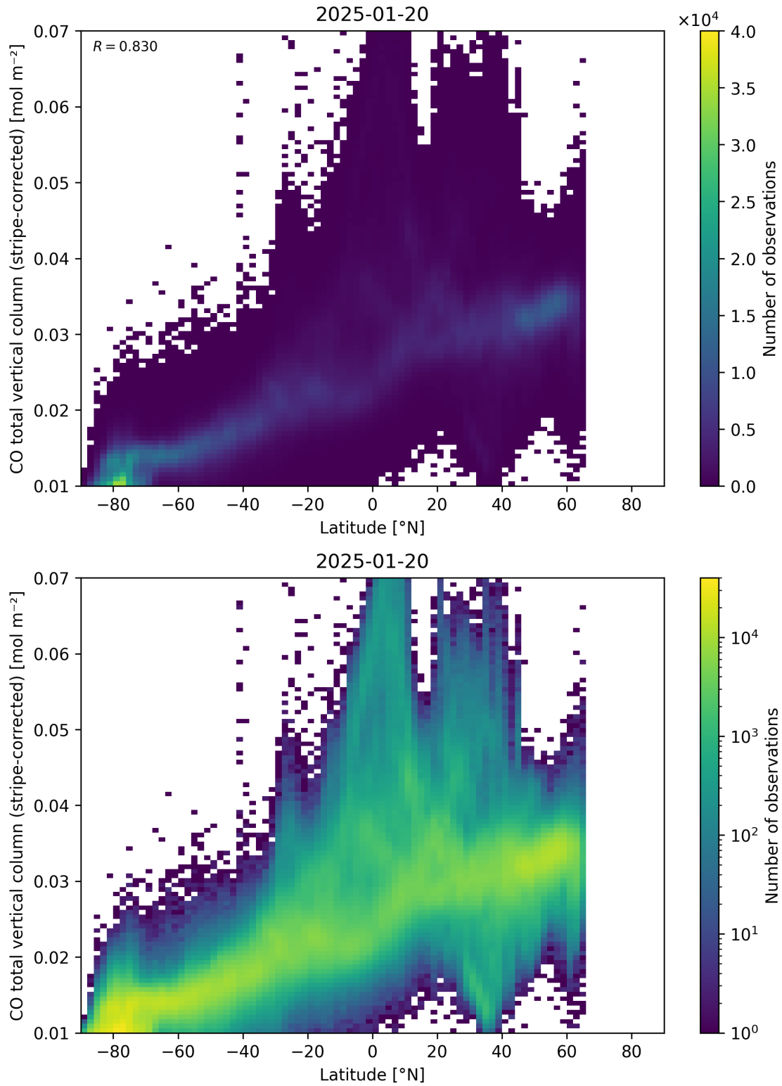
Figure 52: Scatter density plot of “Latitude” against “CO total vertical column (stripe-corrected)” for 2025-01-19 to 2025-01-21.
