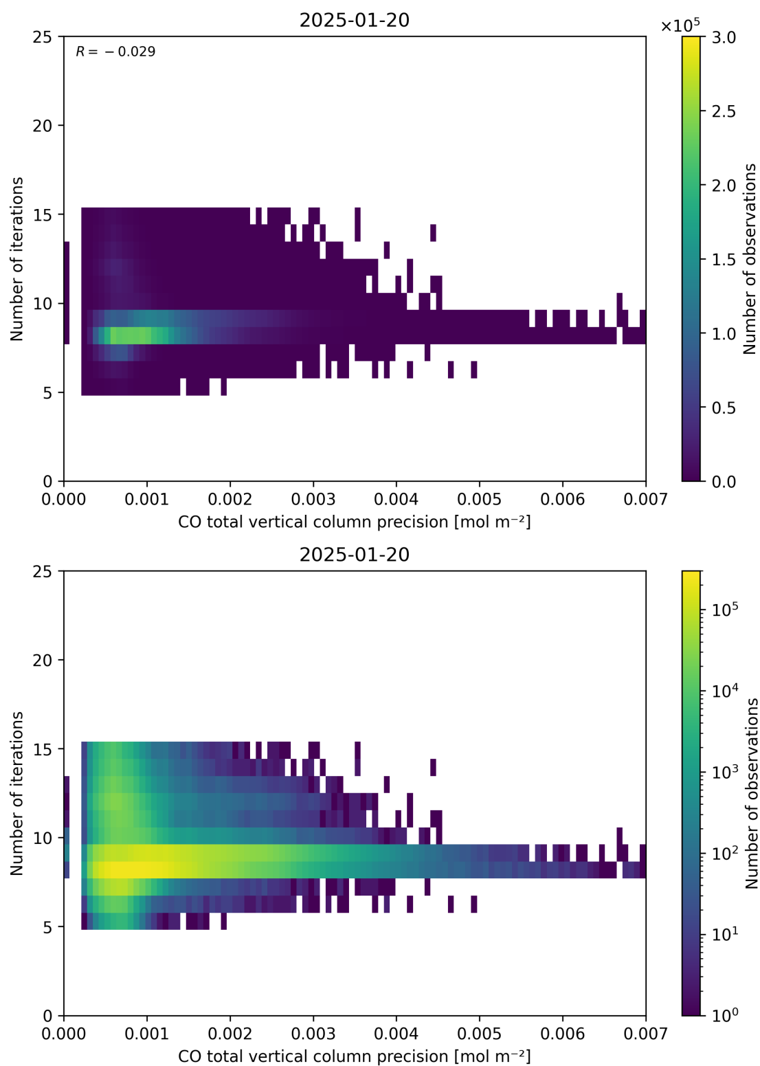
Figure 46: Scatter density plot of “CO total vertical column precision” against “Number of iterations” for 2025-01-19 to 2025-01-21.
