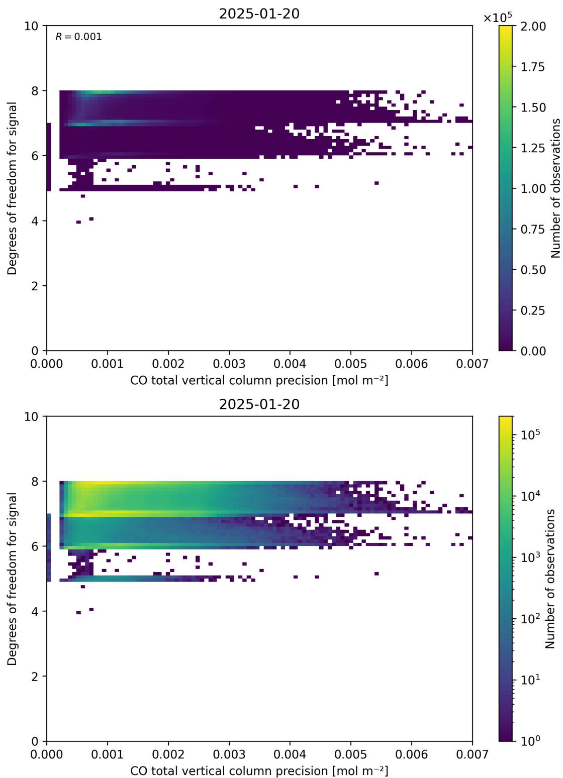
Figure 45: Scatter density plot of “CO total vertical column precision” against “Degrees of freedom for signal” for 2025-01-19 to 2025-01-21.
