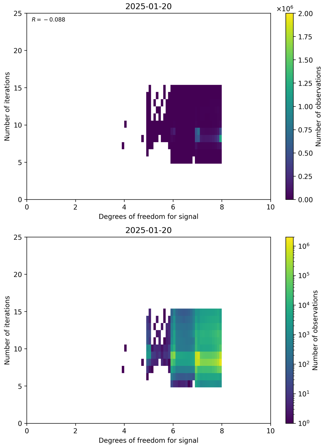
Figure 50: Scatter density plot of “Degrees of freedom for signal” against “Number of iterations” for 2025-01-19 to 2025-01-21.
