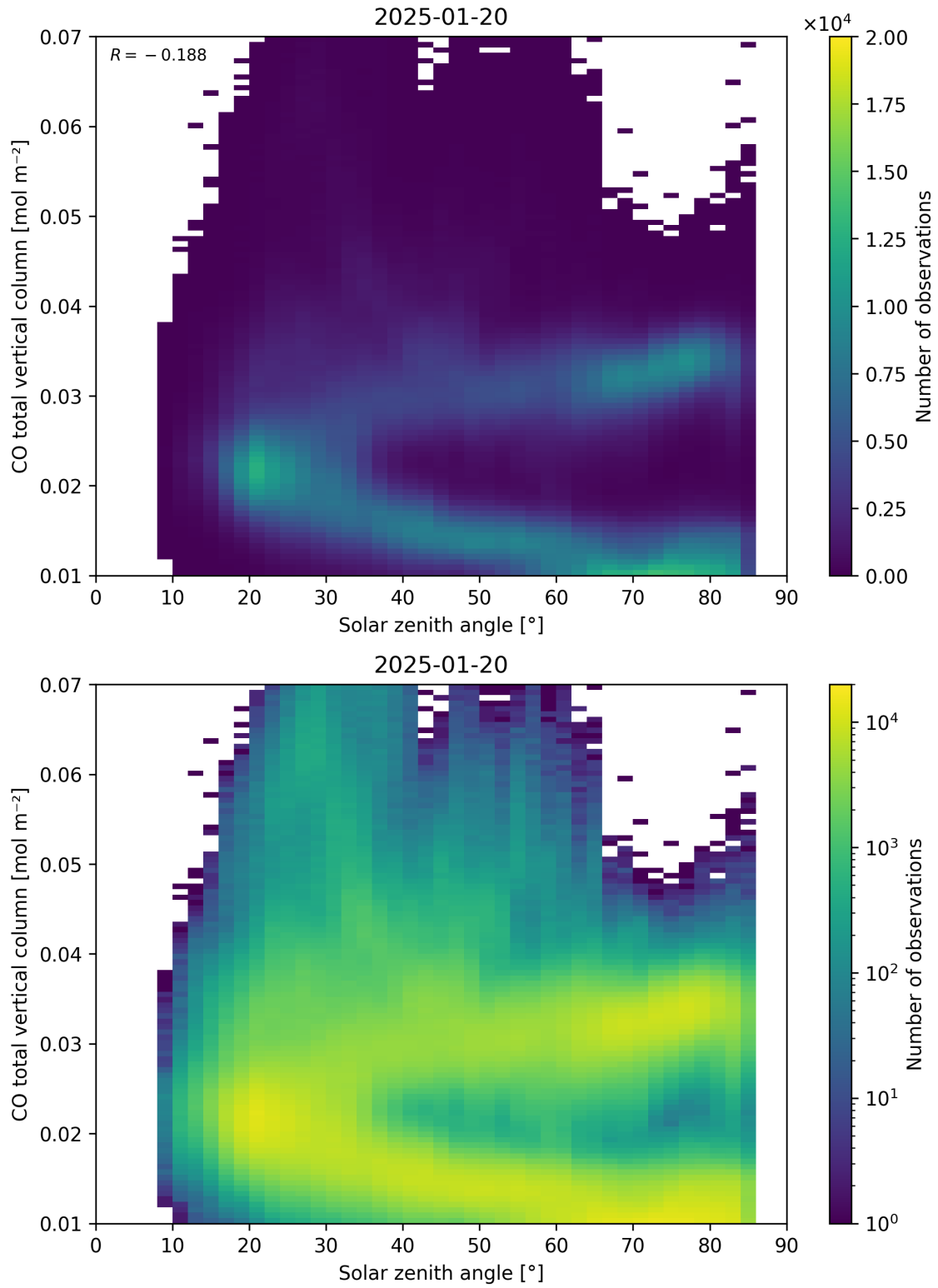
Figure 61: Scatter density plot of “Solar zenith angle” against “CO total vertical column” for 2025-01-19 to 2025-01-21.
