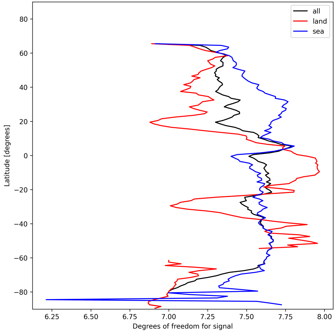
Figure 15: Zonal average of “Degrees of freedom for signal” for 2025-01-19 to 2025-01-21.
