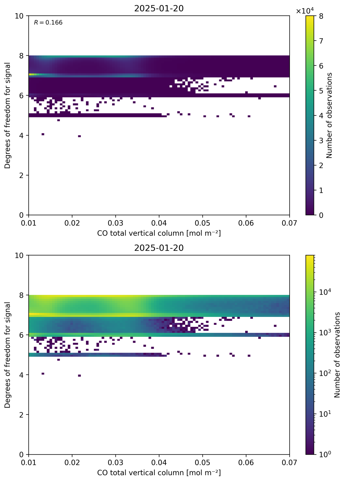
Figure 41: Scatter density plot of “CO total vertical column” against “Degrees of freedom for signal” for 2025-01-19 to 2025-01-21.
