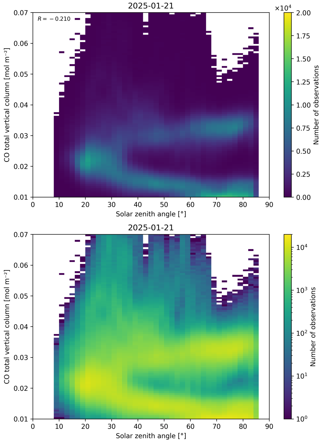
Figure 61: Scatter density plot of “Solar zenith angle” against “CO total vertical column” for 2025-01-20 to 2025-01-22.
