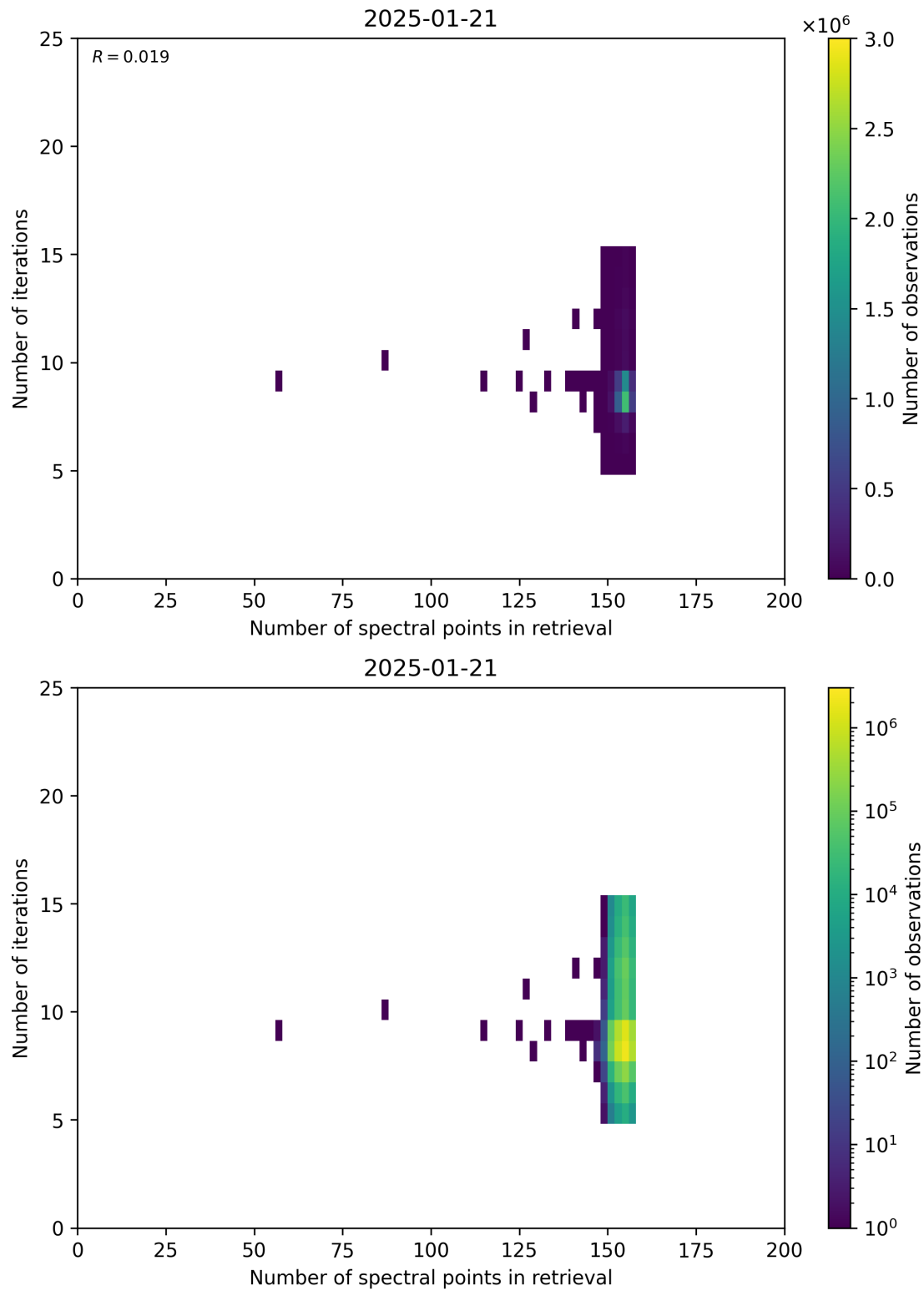
Figure 60: Scatter density plot of “Number of spectral points in retrieval” against “Number of iterations” for 2025-01-20 to 2025-01-22.
