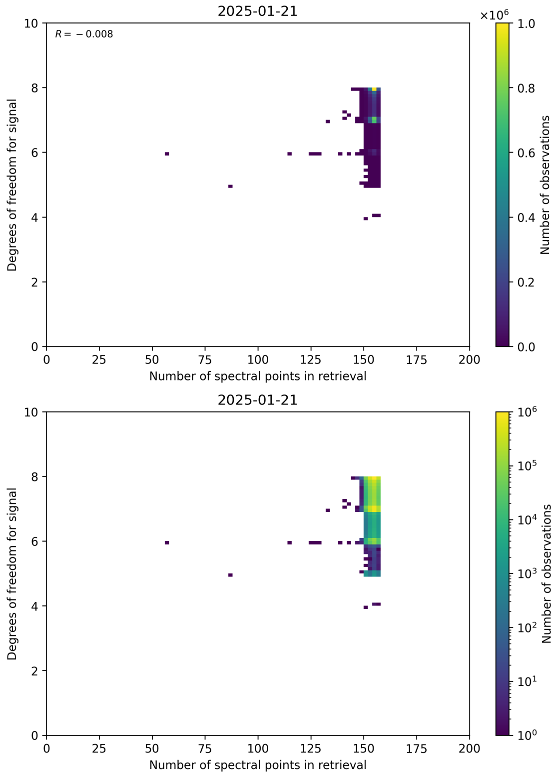
Figure 59: Scatter density plot of “Number of spectral points in retrieval” against “Degrees of freedom for signal” for 2025-01-20 to 2025-01-22.
