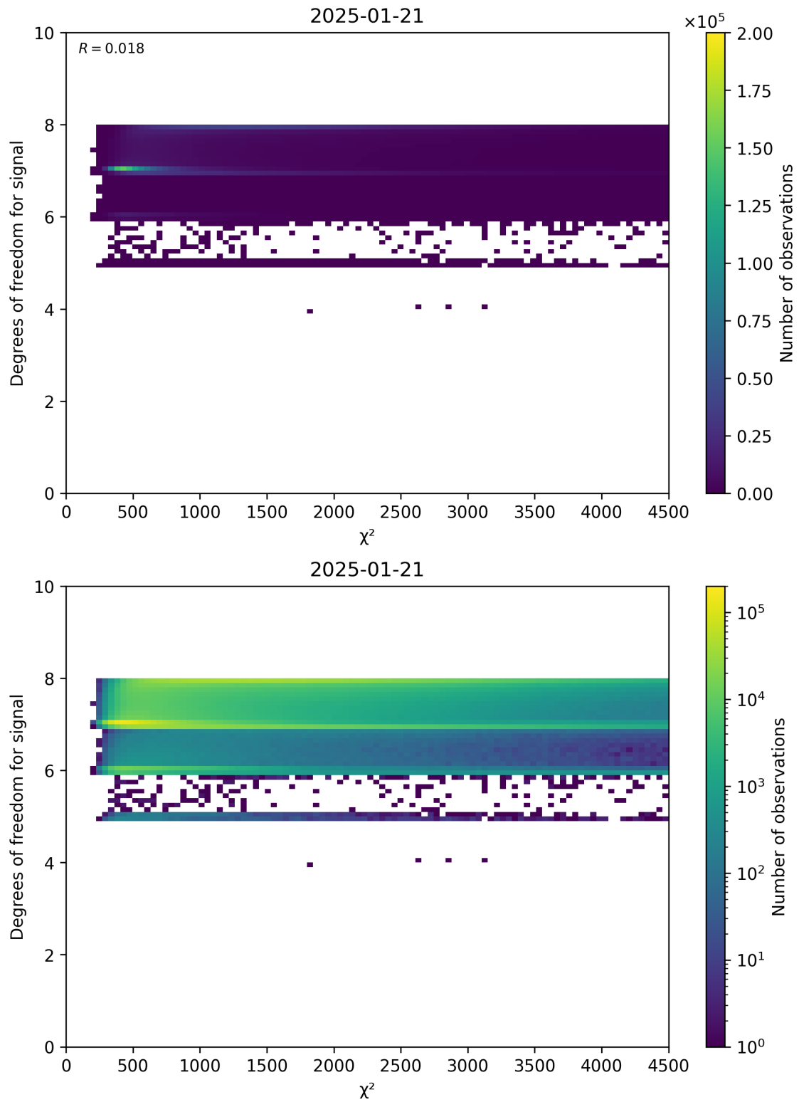
Figure 48: Scatter density plot of “ \chi^2 ” against “Degrees of freedom for signal” for 2025-01-20 to 2025-01-22.
