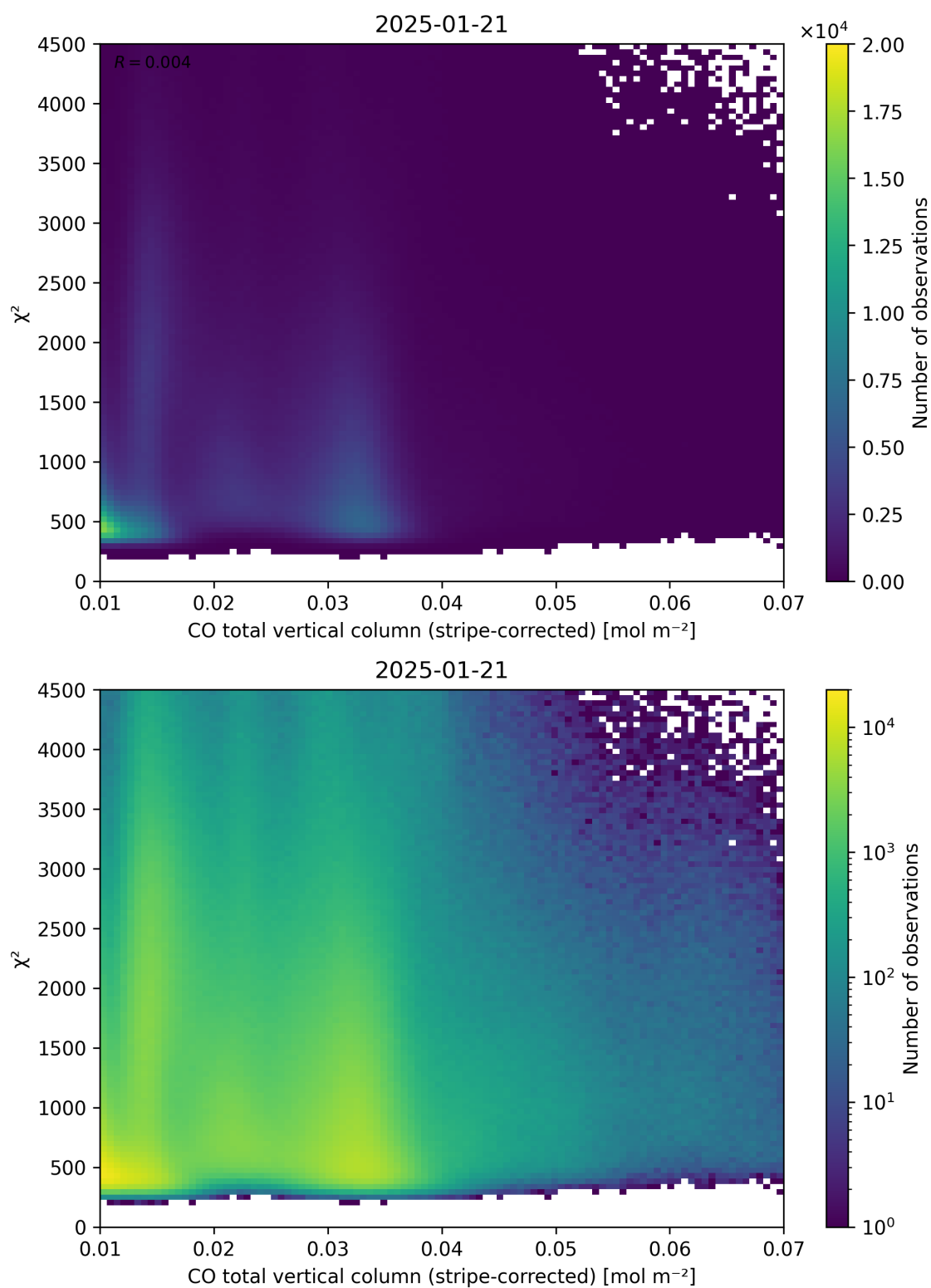
Figure 37: Scatter density plot of “CO total vertical column (stripe-corrected)” against “ \chi^2 ” for 2025-01-20 to 2025-01-22.
