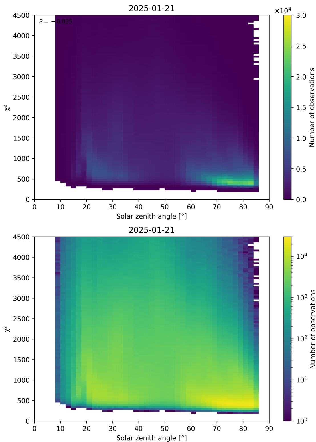
Figure 64: Scatter density plot of “Solar zenith angle” against “ \chi^2 ” for 2025-01-20 to 2025-01-22.
