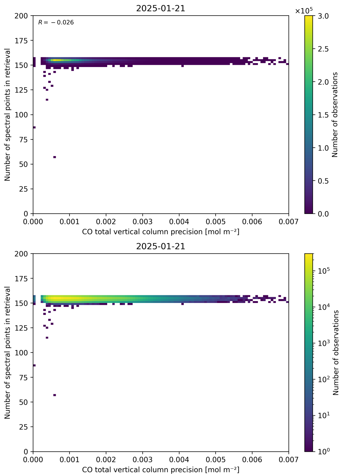
Figure 47: Scatter density plot of “CO total vertical column precision” against “Number of spectral points in retrieval” for 2025-01-20 to 2025-01-22.
