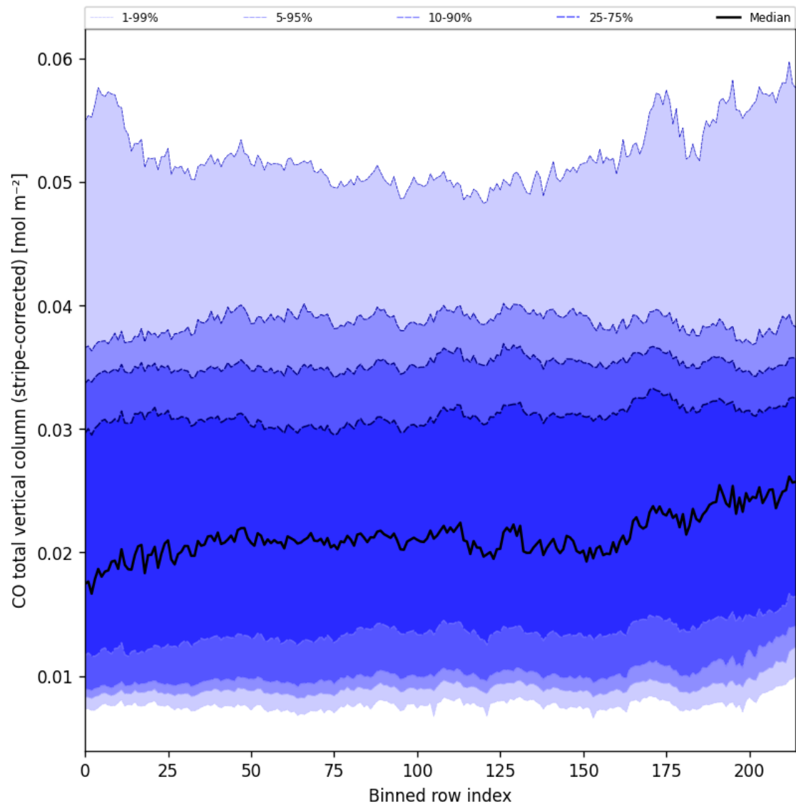
Figure 27: Along track statistics of “CO total vertical column (stripe-corrected)” for 2025-01-20 to 2025-01-22
