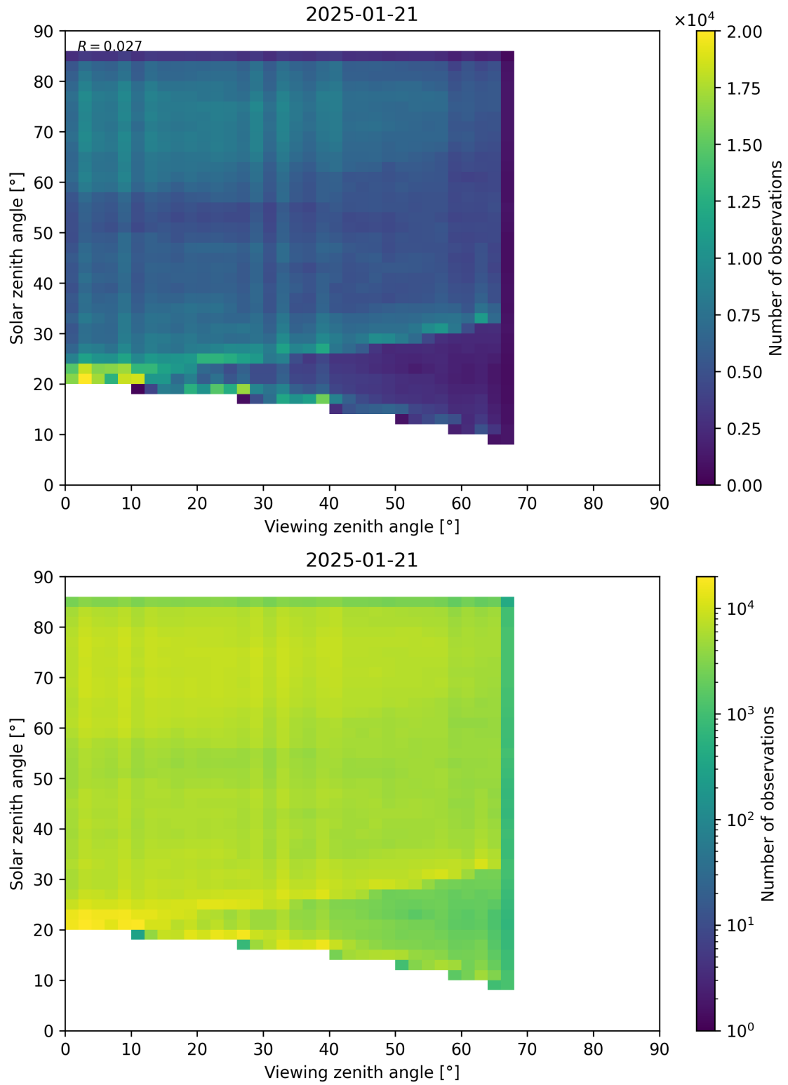
Figure 77: Scatter density plot of “Viewing zenith angle” against “Solar zenith angle” for 2025-01-20 to 2025-01-22.
