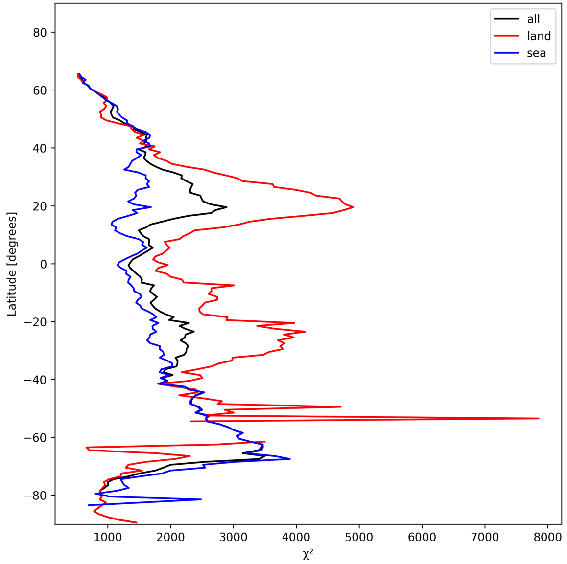
Figure 14: Zonal average of “ \chi^2 ” for 2025-01-20 to 2025-01-22.
