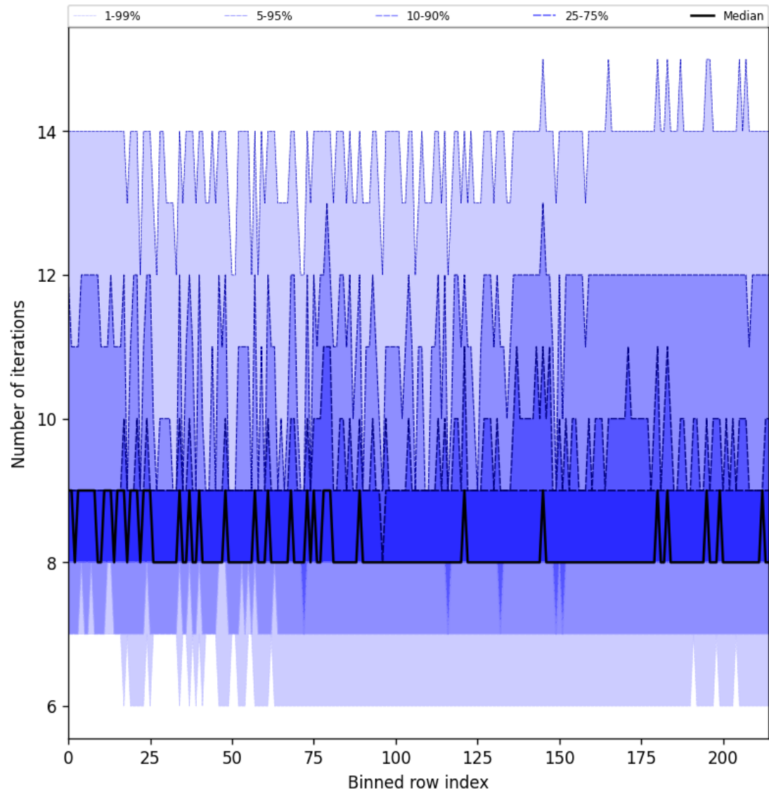
Figure 32: Along track statistics of “Number of iterations” for 2025-01-20 to 2025-01-22
