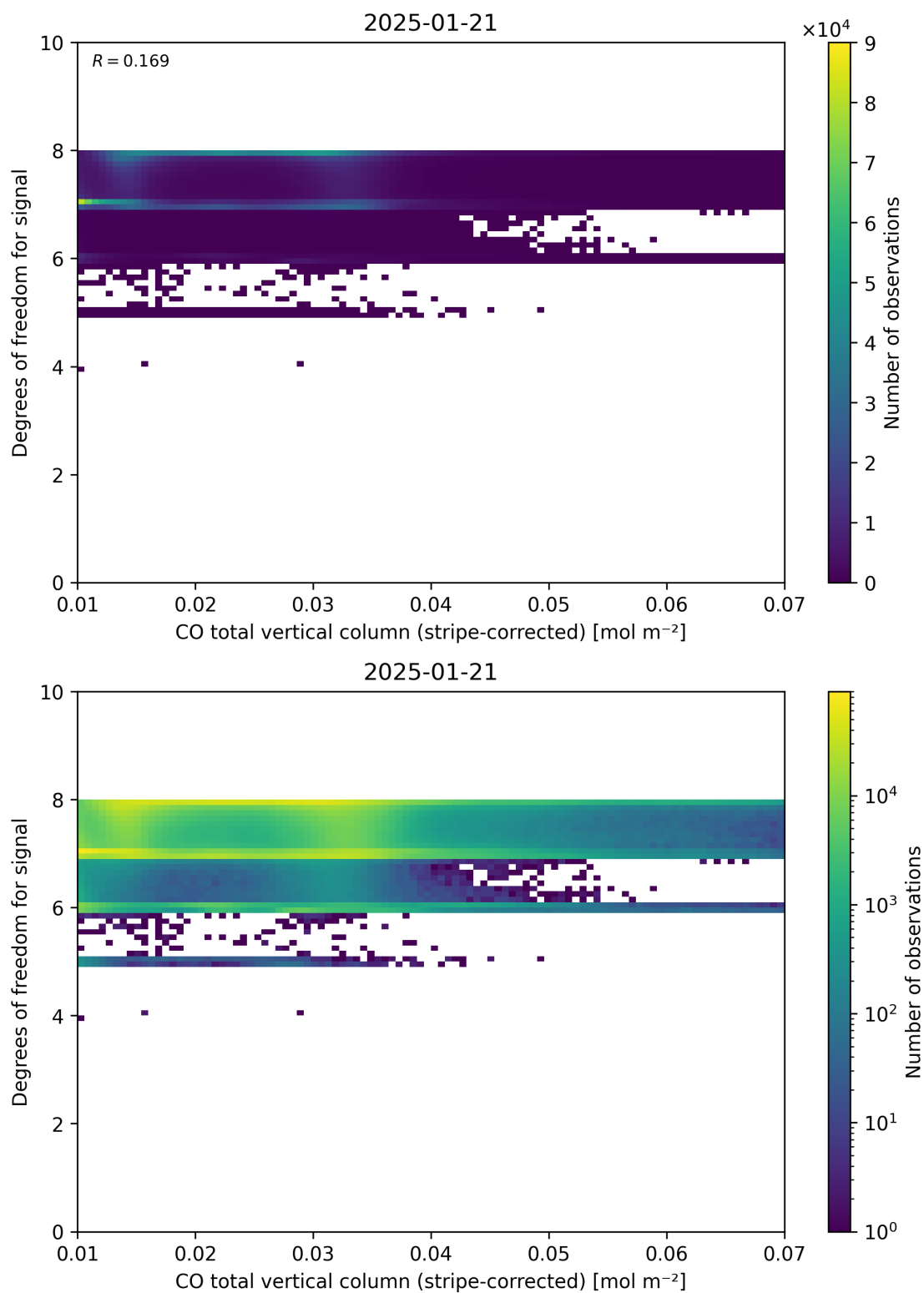
Figure 38: Scatter density plot of “CO total vertical column (stripe-corrected)” against “Degrees of freedom for signal” for 2025-01-20 to 2025-01-22.
