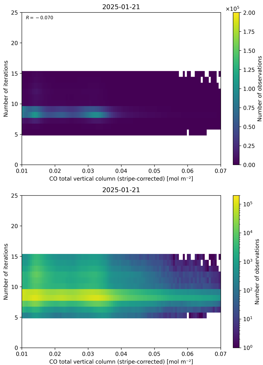
Figure 39: Scatter density plot of “CO total vertical column (stripe-corrected)” against “Number of iterations” for 2025-01-20 to 2025-01-22.
