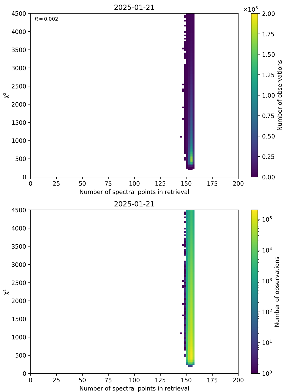
Figure 58: Scatter density plot of “Number of spectral points in retrieval” against “ \chi^2 ” for 2025-01-20 to 2025-01-22.
