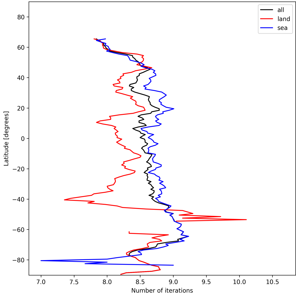
Figure 16: Zonal average of “Number of iterations” for 2025-01-20 to 2025-01-22.
