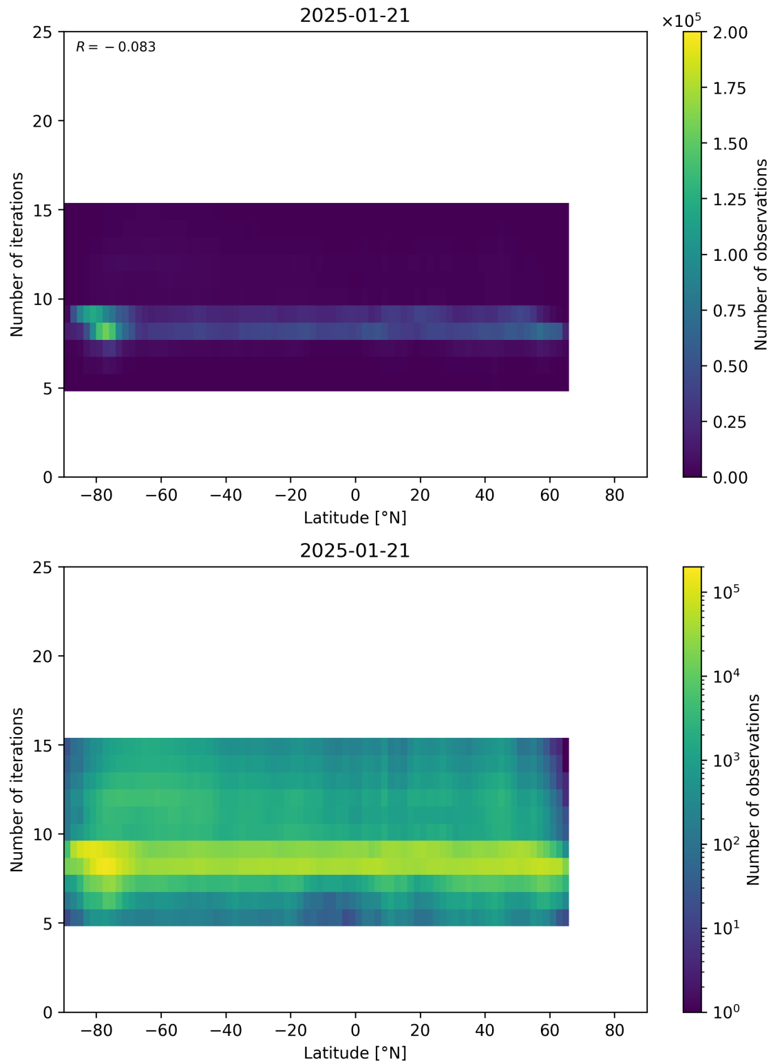
Figure 56: Scatter density plot of “Latitude” against “Number of iterations” for 2025-01-20 to 2025-01-22.
