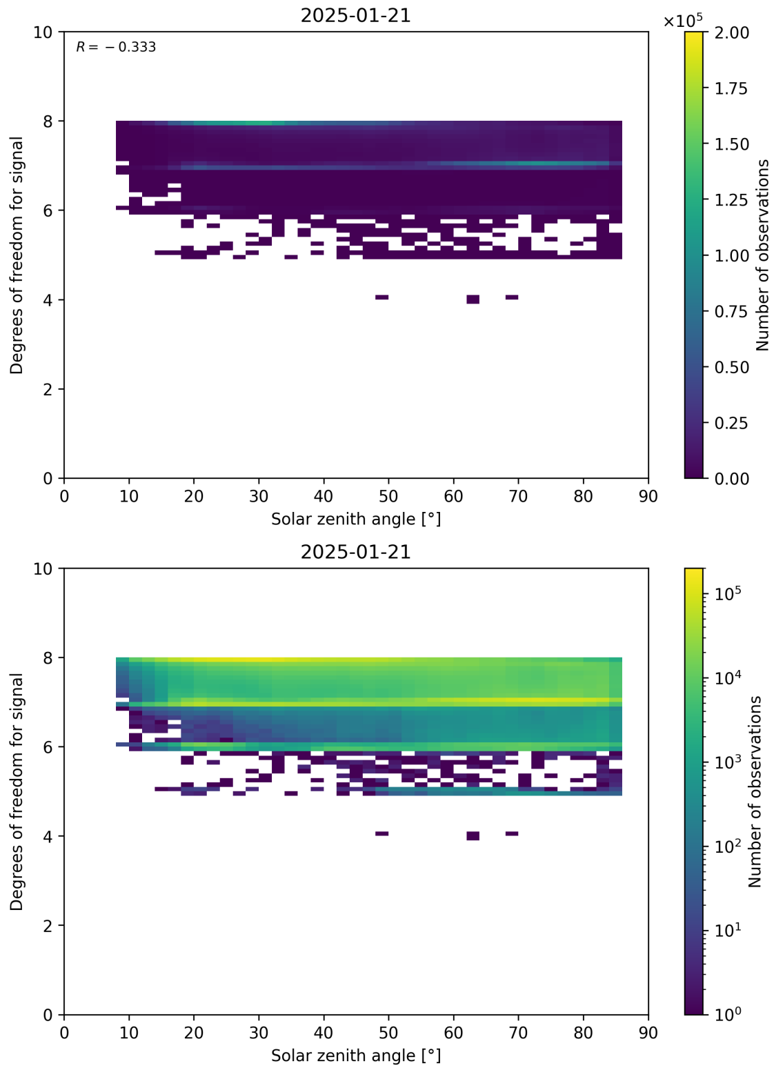
Figure 65: Scatter density plot of “Solar zenith angle” against “Degrees of freedom for signal” for 2025-01-20 to 2025-01-22.
