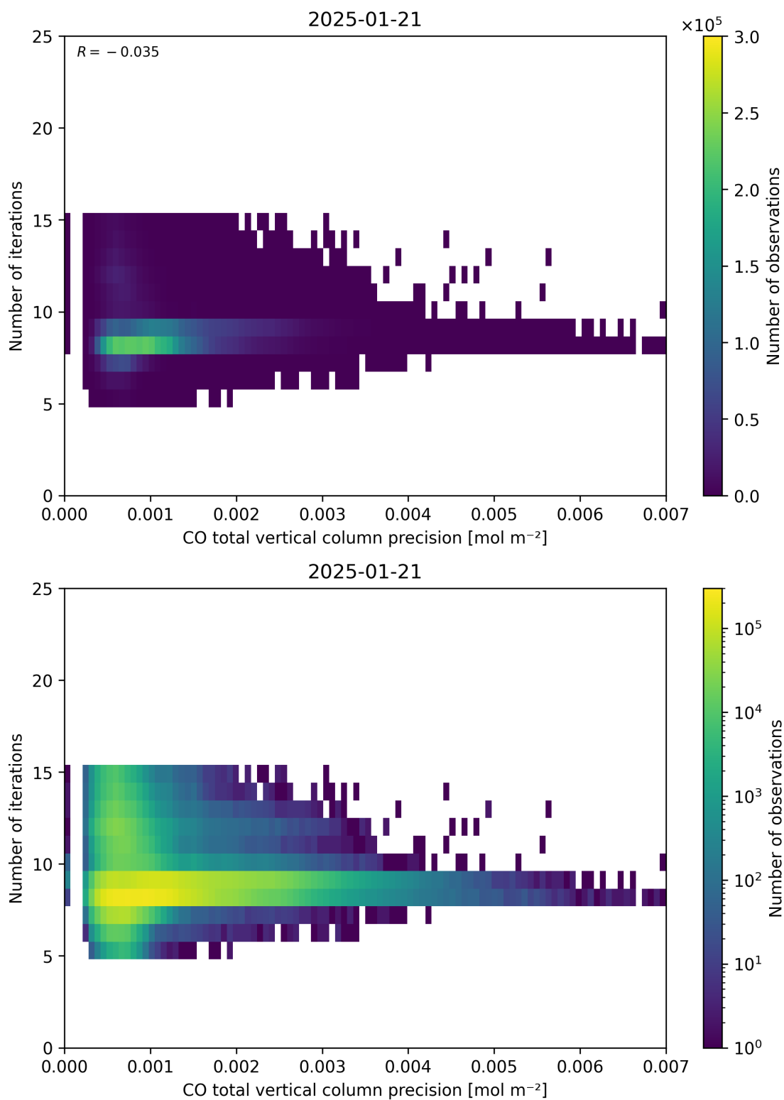
Figure 46: Scatter density plot of “CO total vertical column precision” against “Number of iterations” for 2025-01-20 to 2025-01-22.
