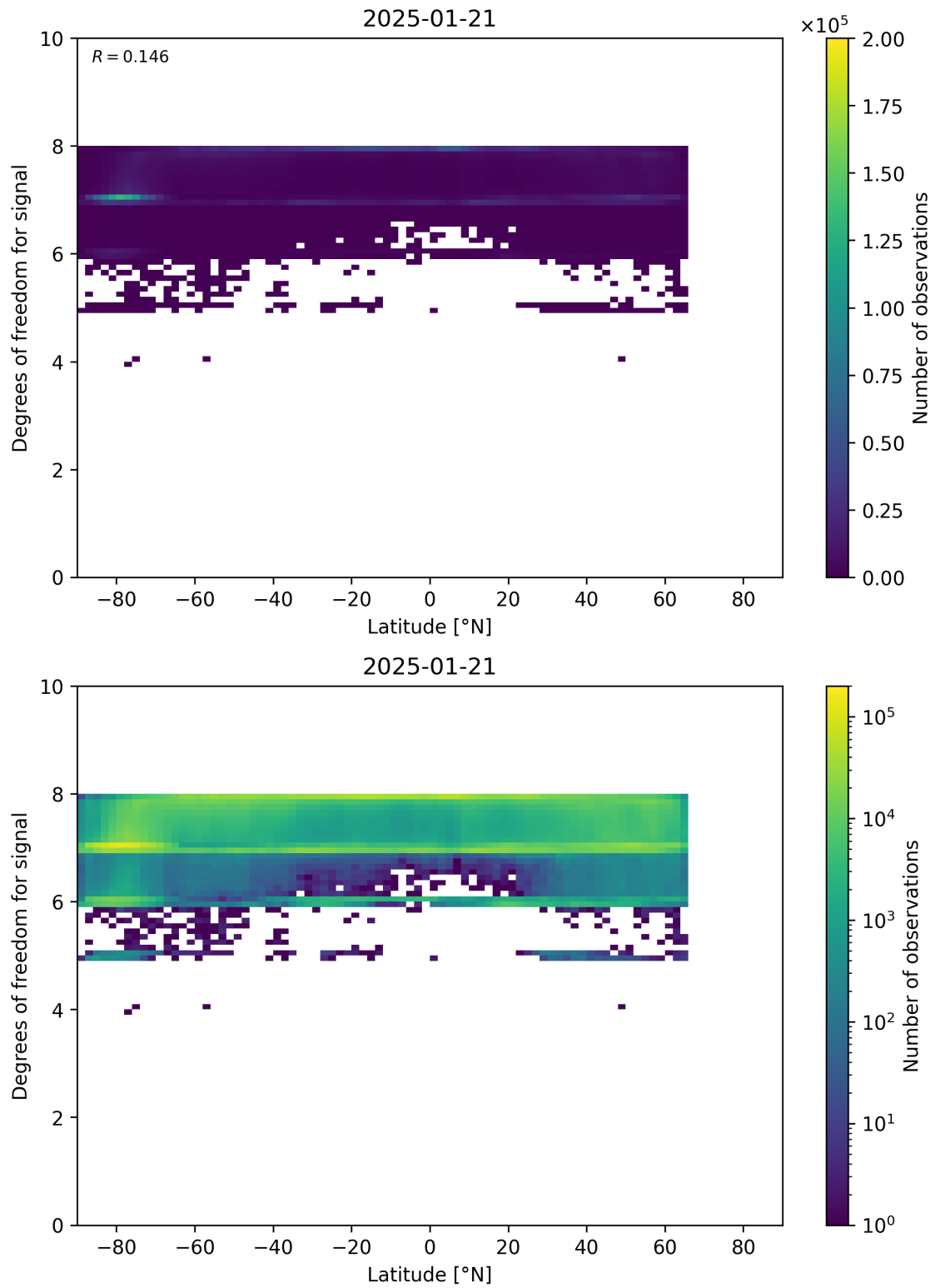
Figure 55: Scatter density plot of “Latitude” against “Degrees of freedom for signal” for 2025-01-20 to 2025-01-22.
