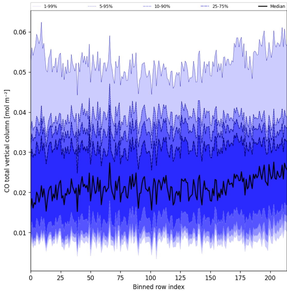
Figure 26: Along track statistics of “CO total vertical column” for 2025-01-20 to 2025-01-22
