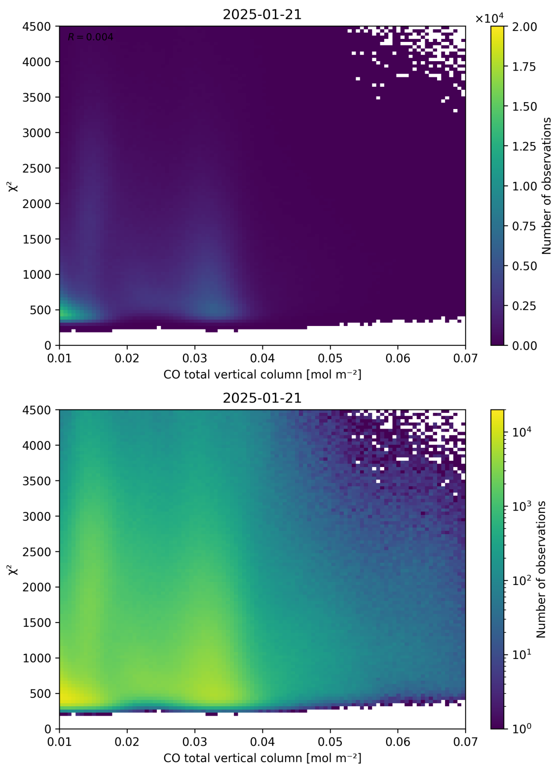
Figure 35: Scatter density plot of “CO total vertical column” against “ \chi^2 ” for 2025-01-20 to 2025-01-22.
