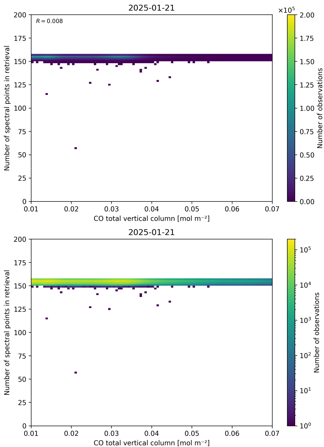
Figure 43: Scatter density plot of “CO total vertical column” against “Number of spectral points in retrieval” for 2025-01-20 to 2025-01-22.
