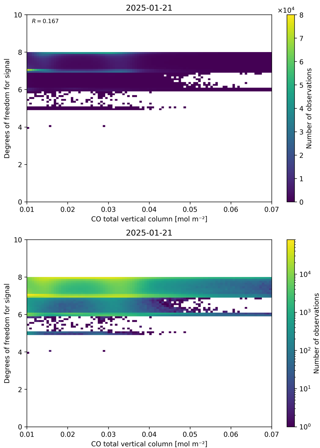
Figure 41: Scatter density plot of “CO total vertical column” against “Degrees of freedom for signal” for 2025-01-20 to 2025-01-22.
