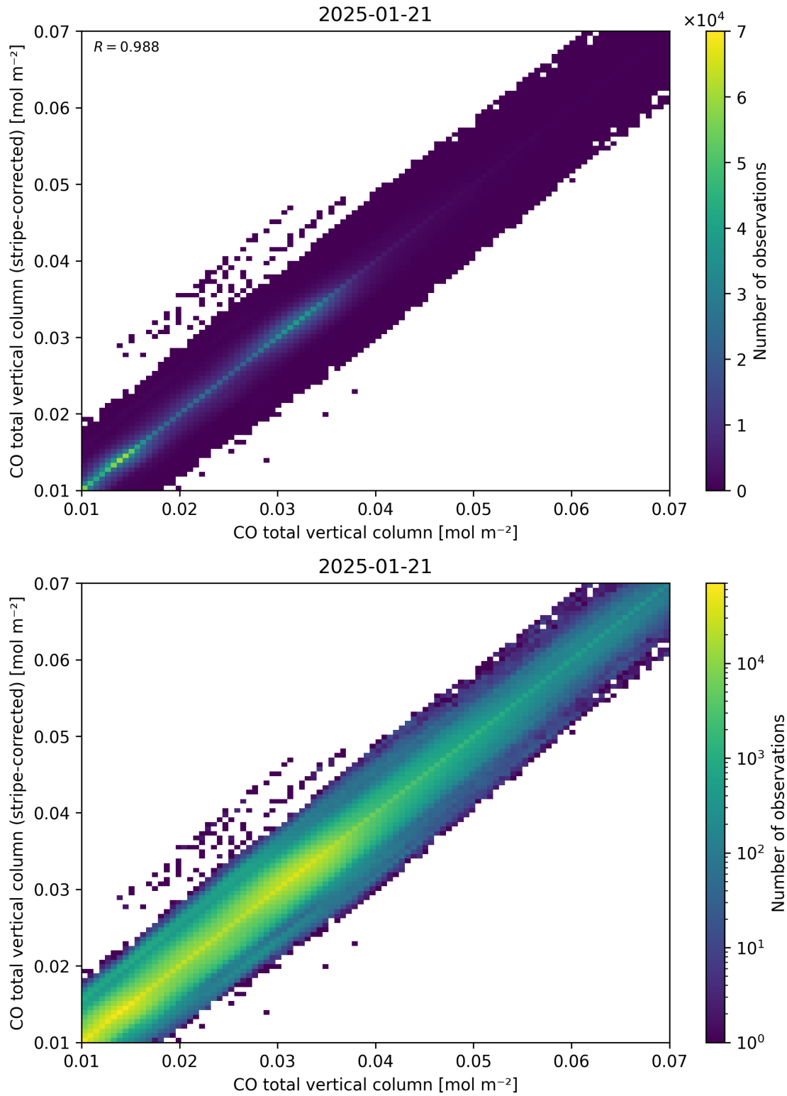
Figure 33: Scatter density plot of “CO total vertical column” against “CO total vertical column (stripe-corrected)” for 2025-01-20 to 2025-01-22.
