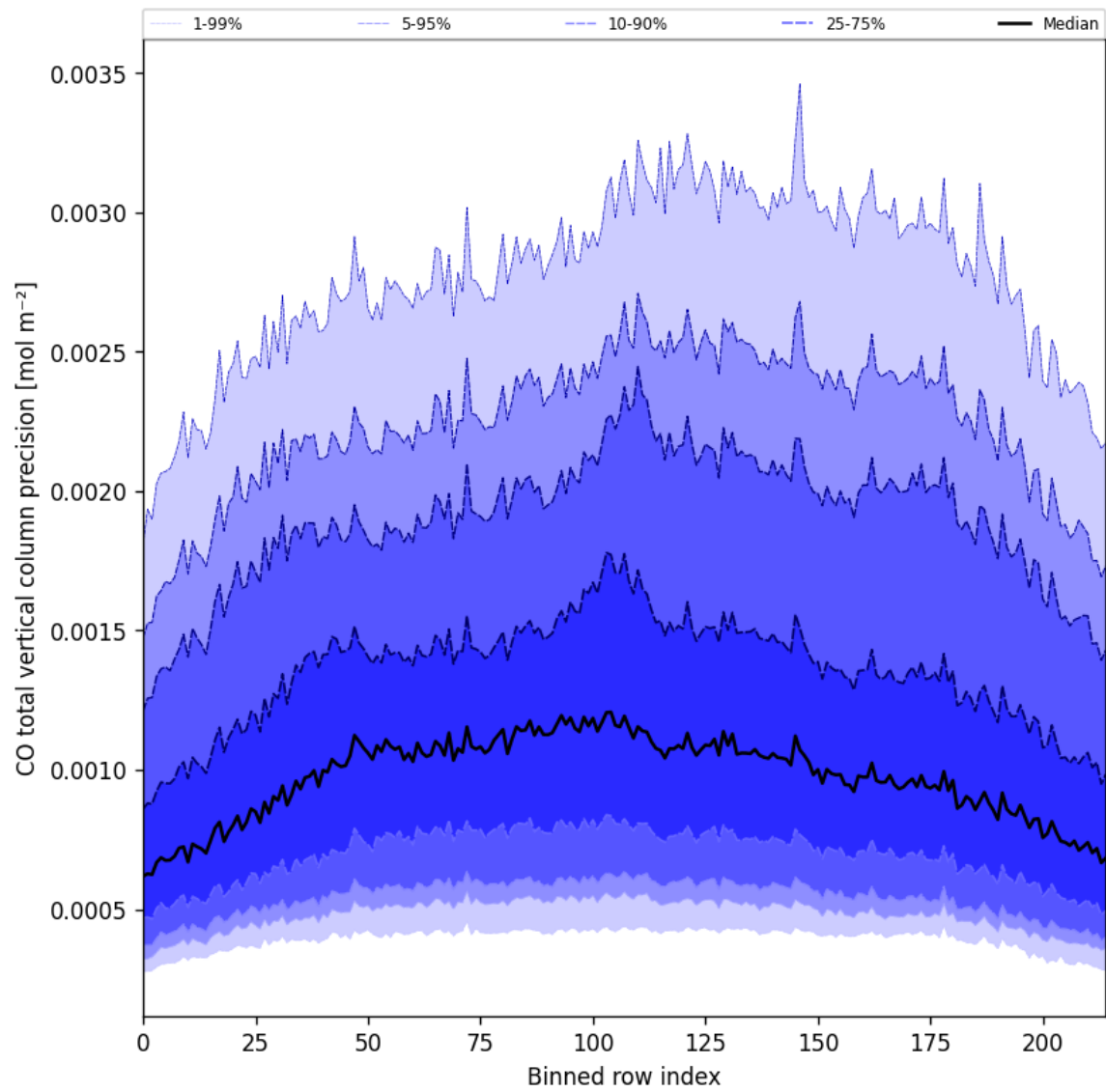
Figure 28: Along track statistics of “CO total vertical column precision” for 2025-01-20 to 2025-01-22
