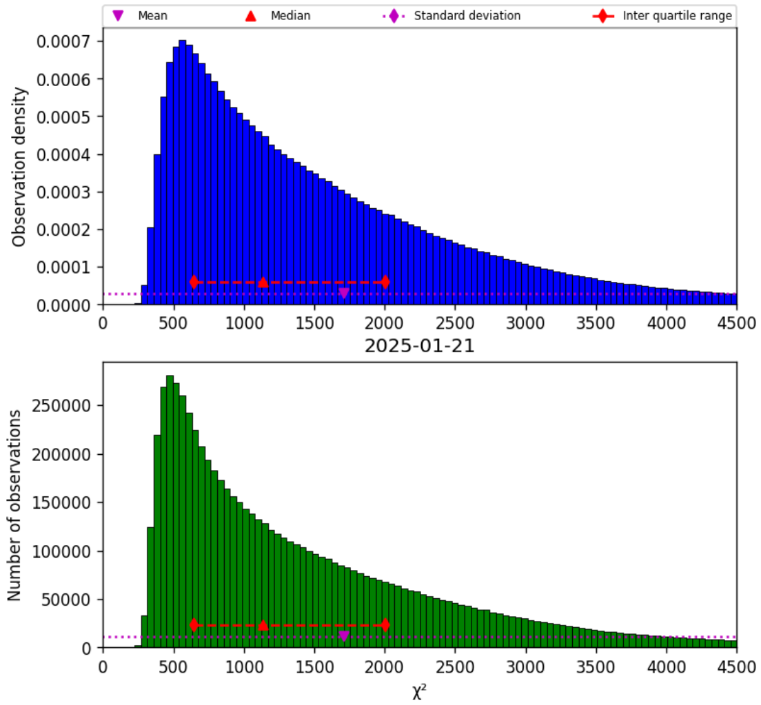
Figure 22: Histogram of “ \chi^2 ” for 2025-01-20 to 2025-01-22
