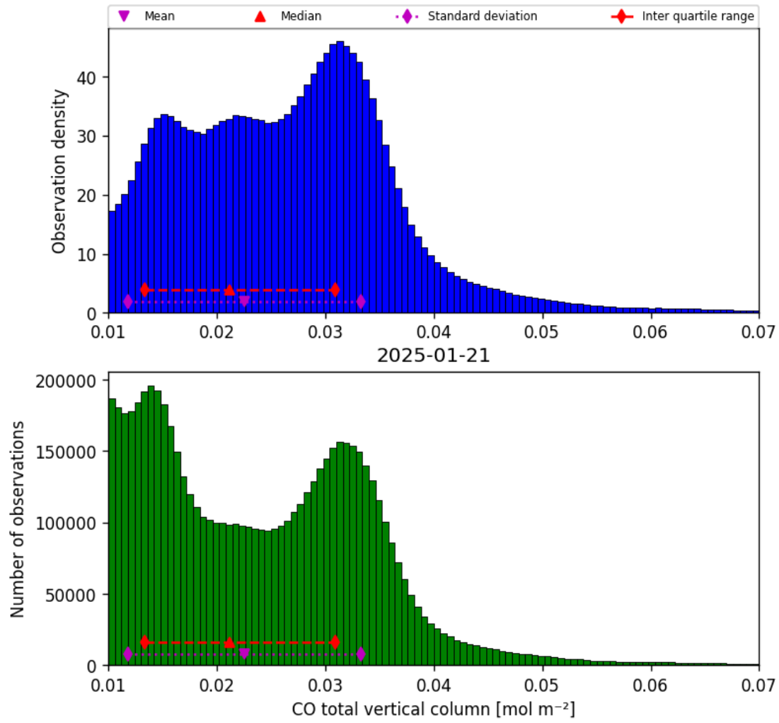
Figure 18: Histogram of “CO total vertical column” for 2025-01-20 to 2025-01-22
