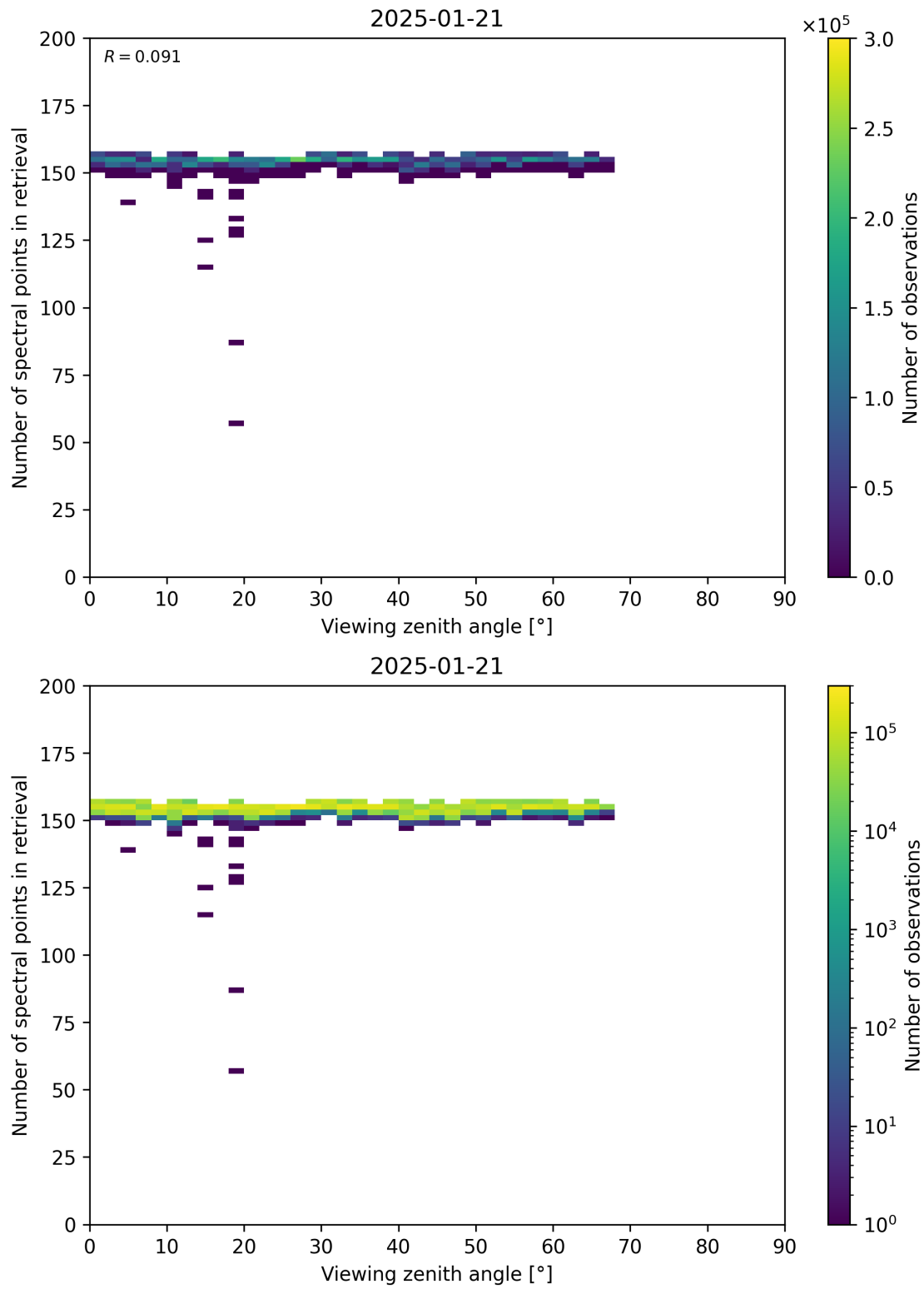
Figure 76: Scatter density plot of “Viewing zenith angle” against “Number of spectral points in retrieval” for 2025-01-20 to 2025-01-22.
