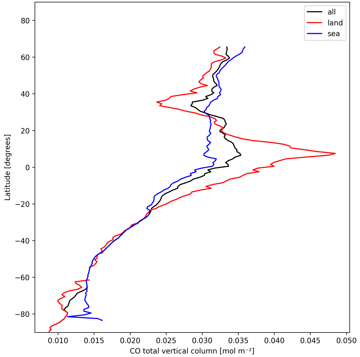
Figure 10: Zonal average of “CO total vertical column” for 2025-01-20 to 2025-01-22.
