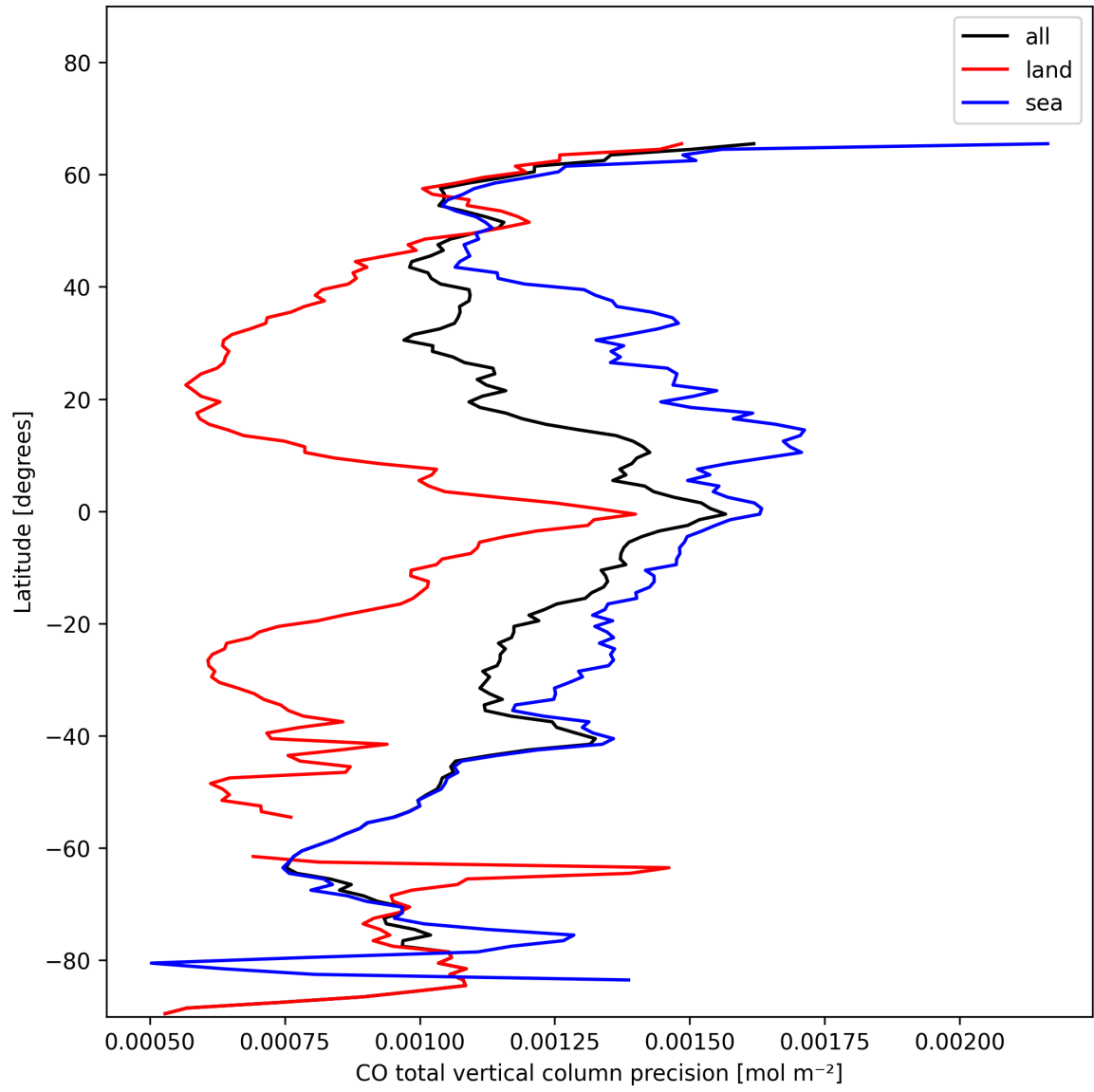
Figure 12: Zonal average of “CO total vertical column precision” for 2025-01-20 to 2025-01-22.
