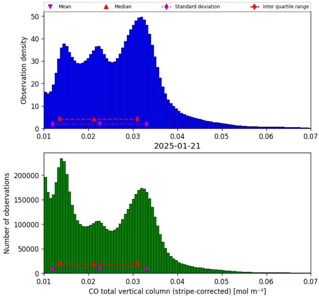
Figure 19: Histogram of “CO total vertical column (stripe-corrected)” for 2025-01-20 to 2025-01-22
