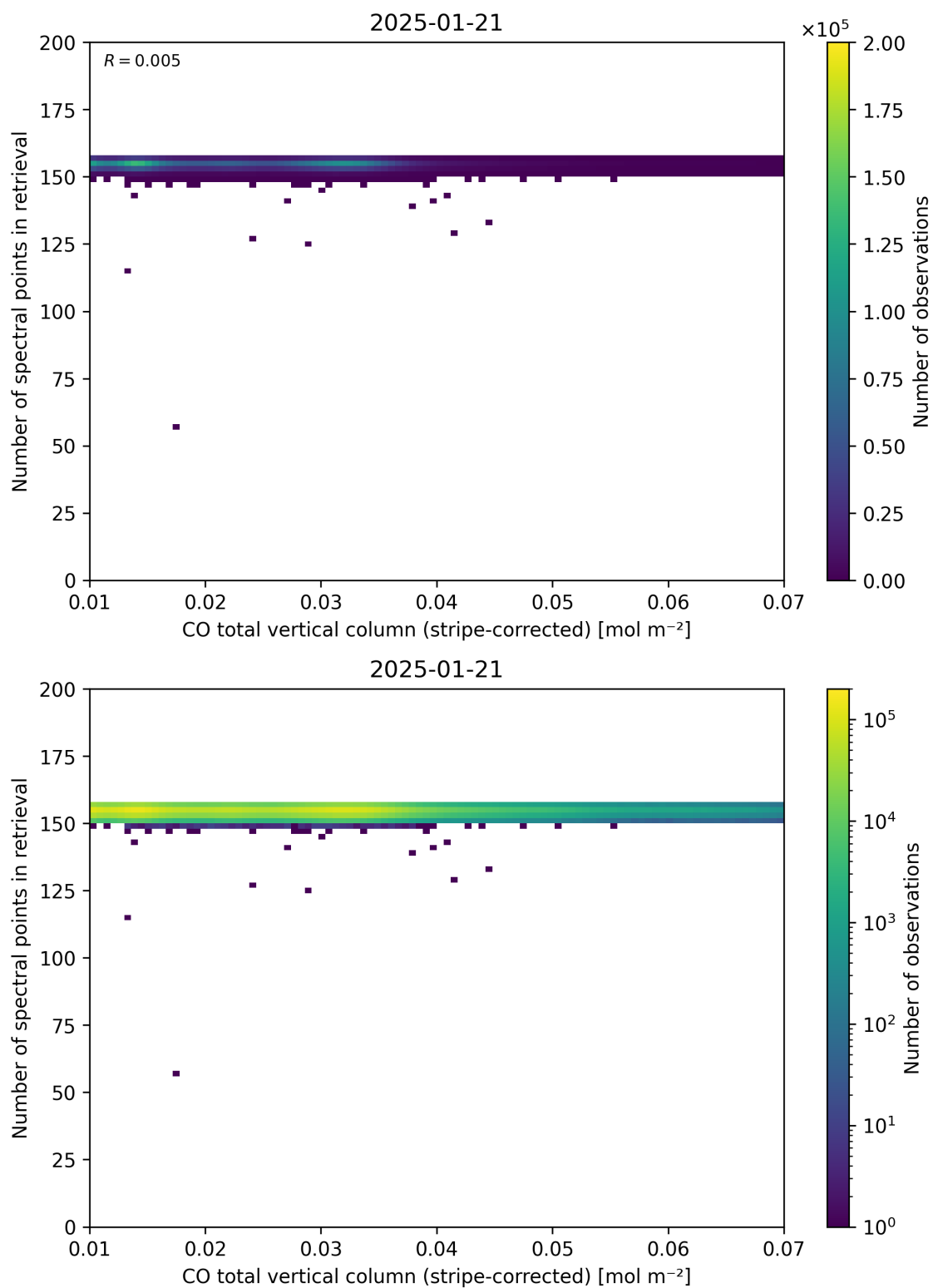
Figure 40: Scatter density plot of “CO total vertical column (stripe-corrected)” against “Number of spectral points in retrieval” for 2025-01-20 to 2025-01-22.
