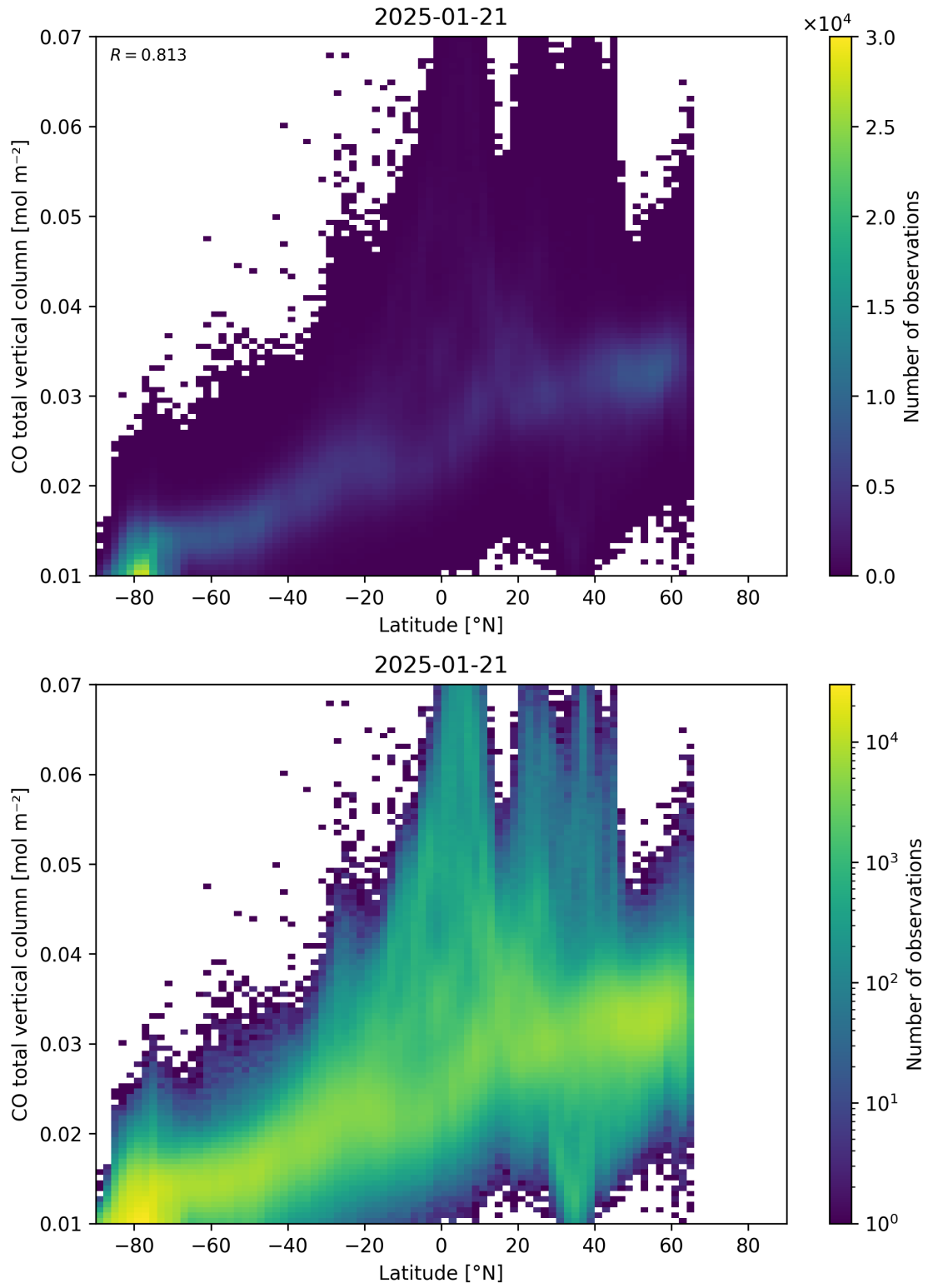
Figure 51: Scatter density plot of “Latitude” against “CO total vertical column” for 2025-01-20 to 2025-01-22.
